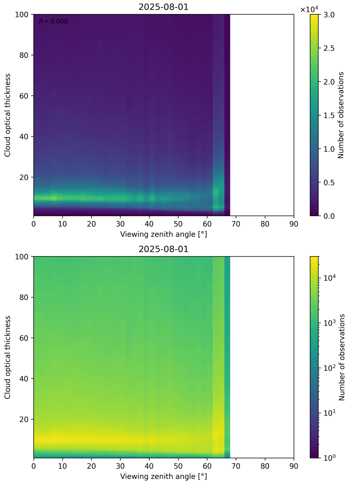
Figure 111: Scatter density plot of “Viewing zenith angle” against “Cloud optical thickness” for 2025-07-31 to 2025-08-02.
