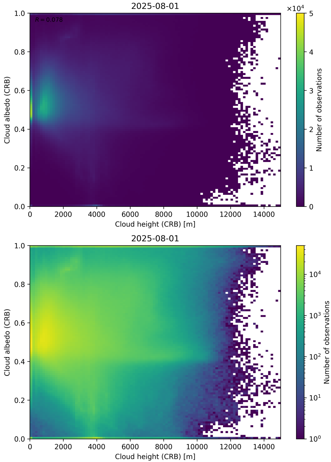
Figure 80: Scatter density plot of “Cloud height (CRB)” against “Cloud albedo (CRB)” for 2025-07-31 to 2025-08-02.
