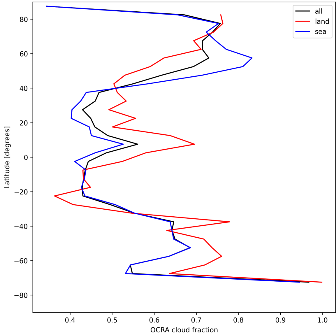
Figure 34: Zonal average of “OCRA cloud fraction” for 2025-07-31 to 2025-08-02.
