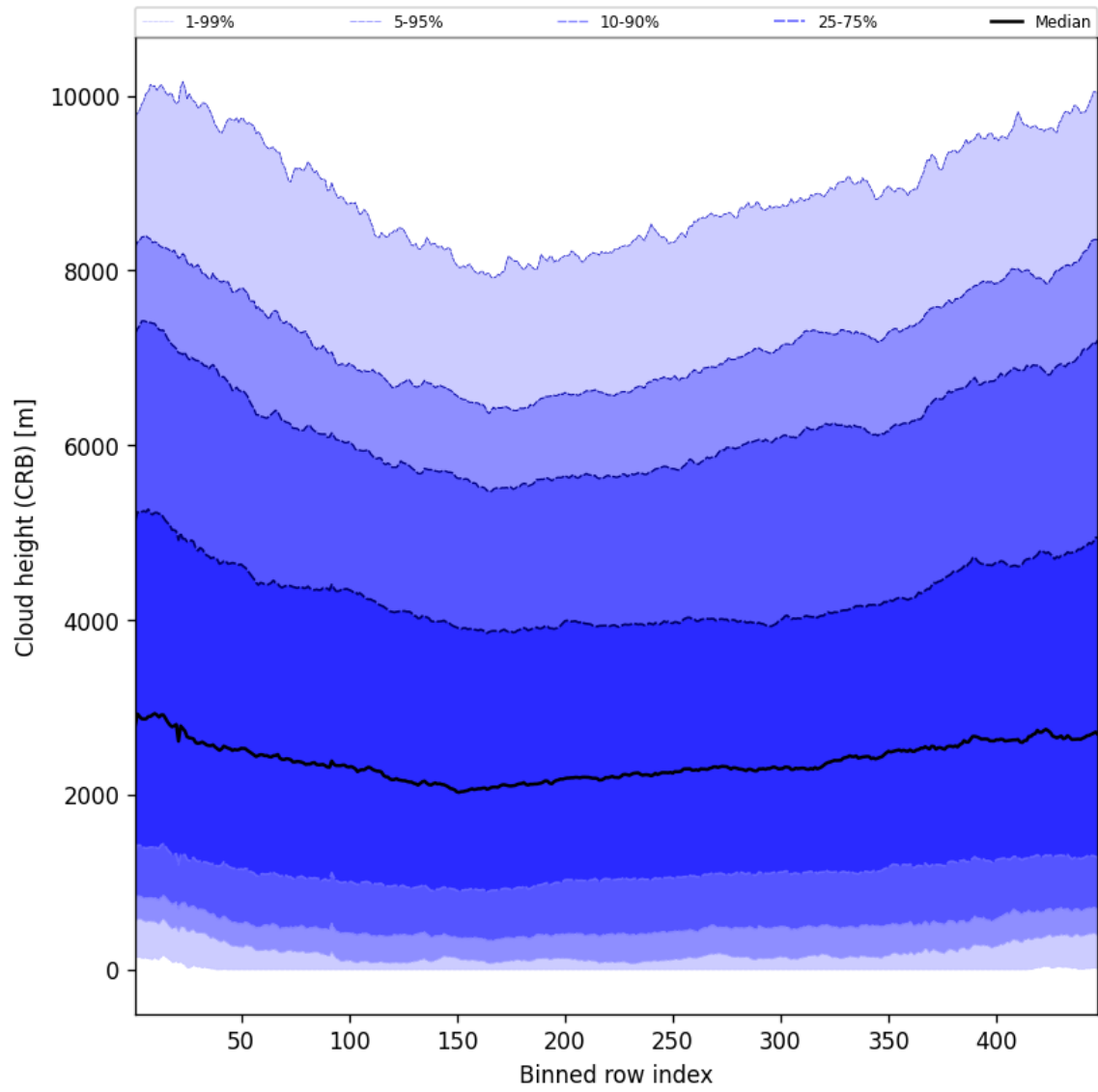
Figure 59: Along track statistics of “Cloud height (CRB)” for 2025-07-31 to 2025-08-02
