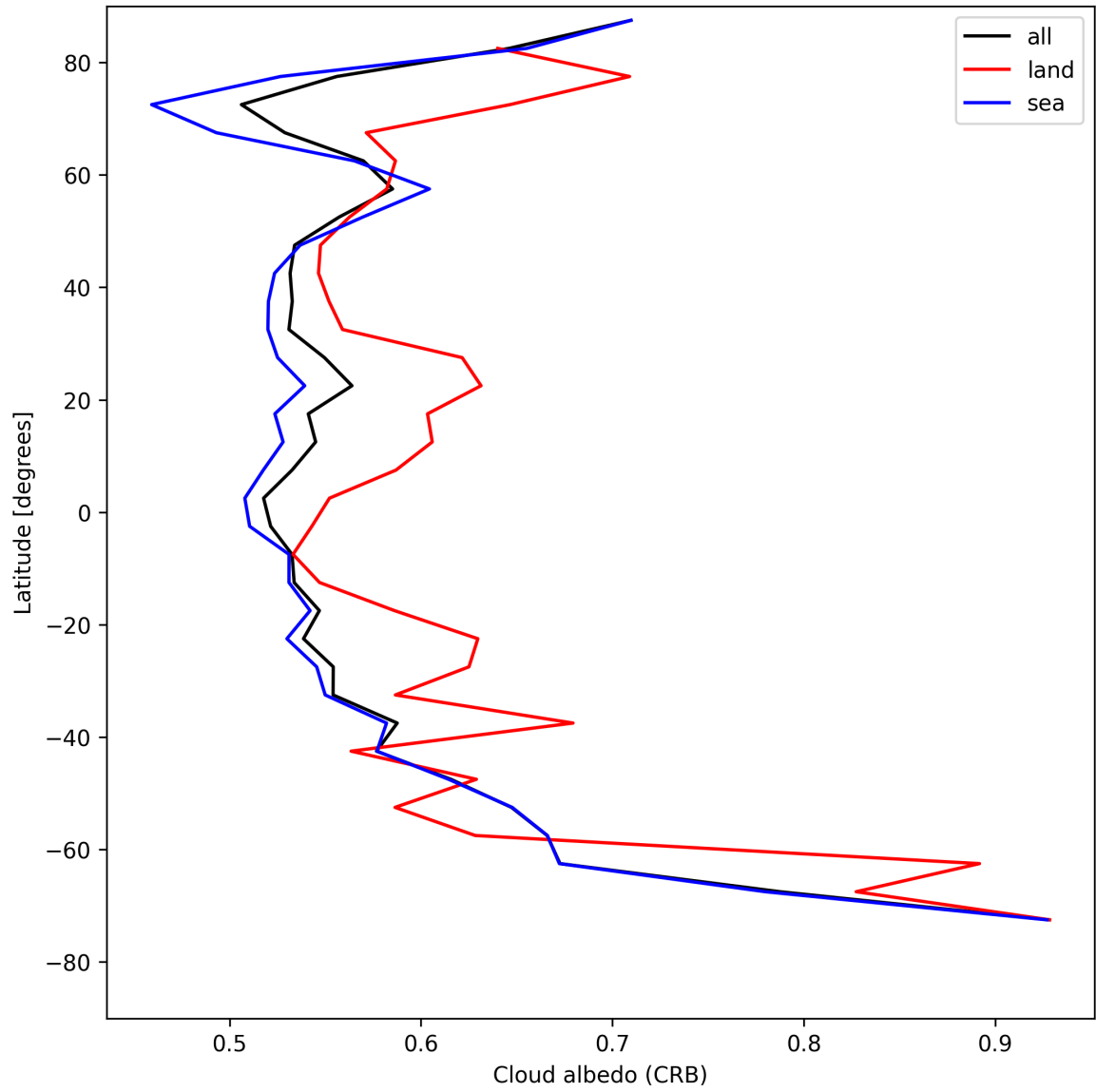
Figure 28: Zonal average of “Cloud albedo (CRB)” for 2025-07-31 to 2025-08-02.
