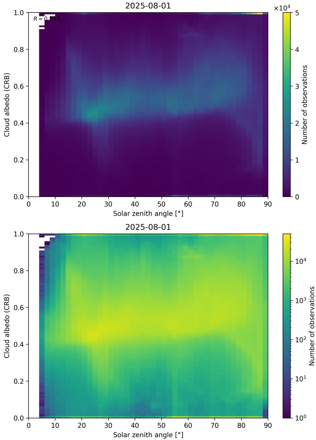
Figure 98: Scatter density plot of “Solar zenith angle” against “Cloud albedo (CRB)” for 2025-07-31 to 2025-08-02.
