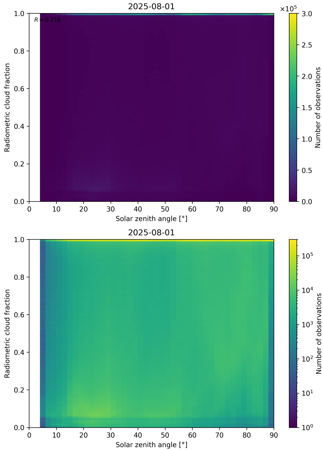
Figure 99: Scatter density plot of “Solar zenith angle” against “Radiometric cloud fraction” for 2025-07-31 to 2025-08-02.
