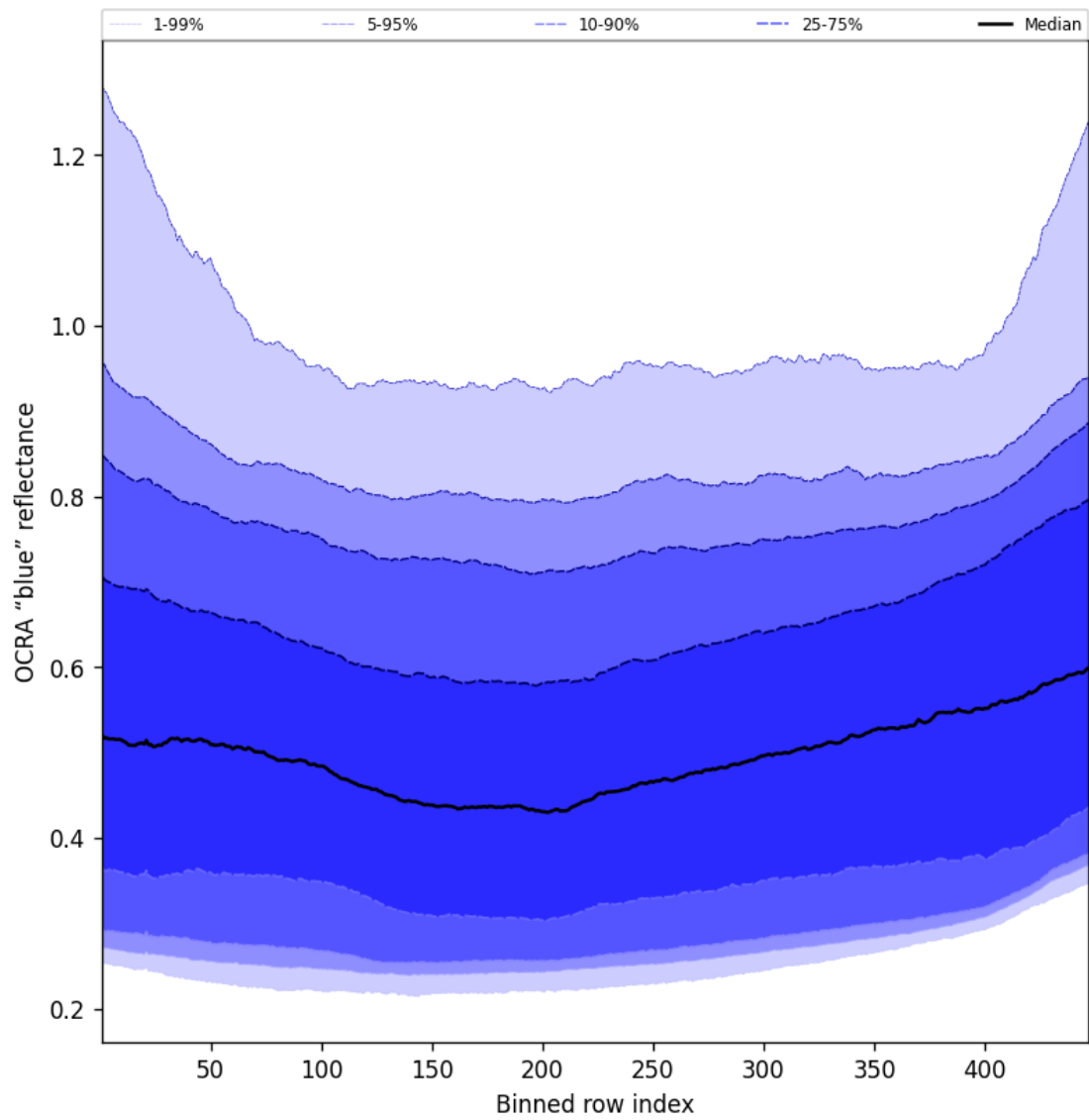
Figure 67: Along track statistics of “OCRA “blue” reflectance” for 2025-07-31 to 2025-08-02
