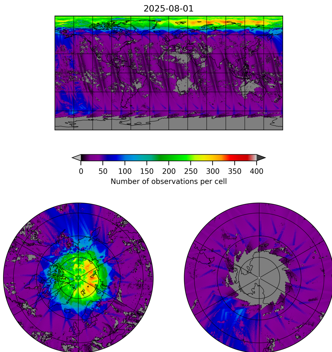
Figure 21: Map of the number of observations for 2025-07-31 to 2025-08-02
