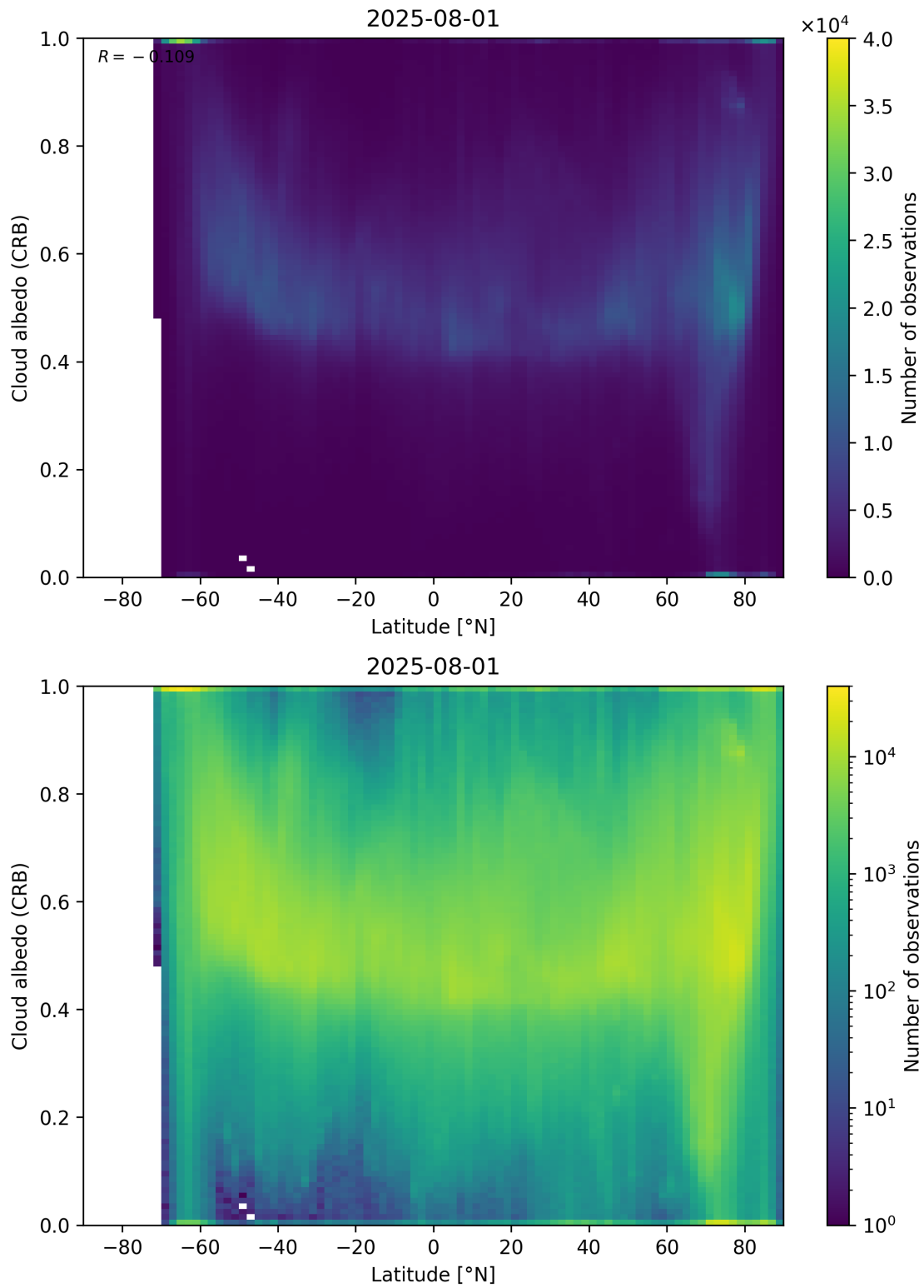
Figure 91: Scatter density plot of “Latitude” against “Cloud albedo (CRB)” for 2025-07-31 to 2025-08-02.
