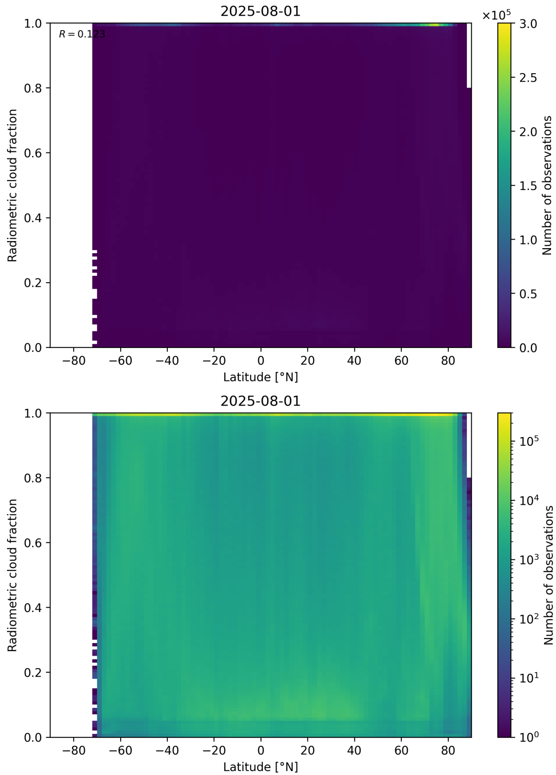
Figure 92: Scatter density plot of “Latitude” against “Radiometric cloud fraction” for 2025-07-31 to 2025-08-02.
