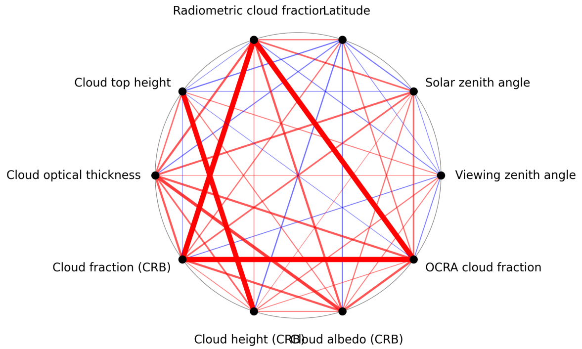
Figure 1: Map of correlation graph for 2025-07-31 to 2025-08-02.
