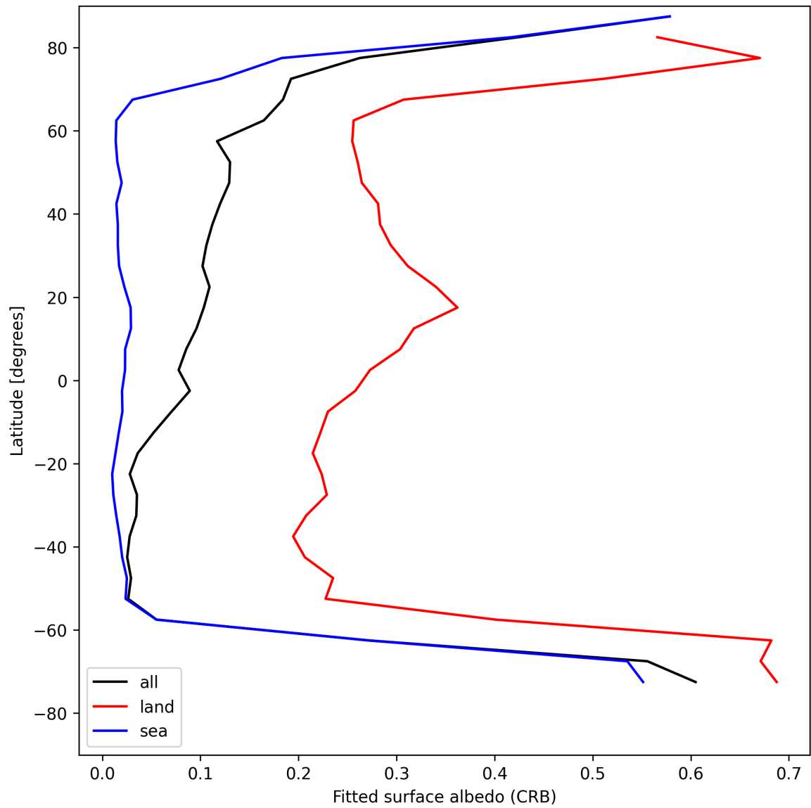
Figure 30: Zonal average of “Fitted surface albedo (CRB)” for 2025-07-31 to 2025-08-02.
