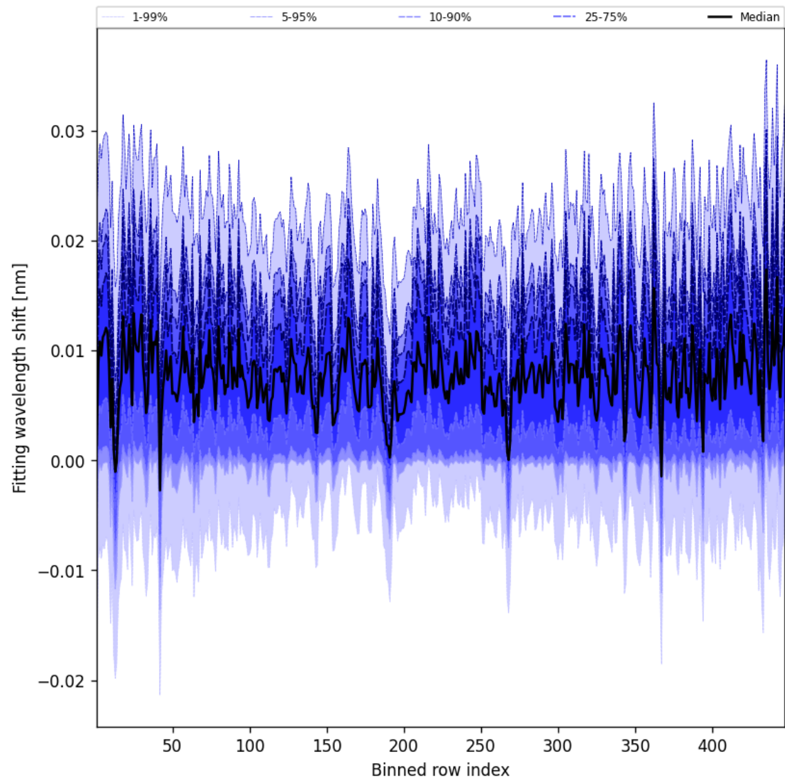
Figure 65: Along track statistics of “Fitting wavelength shift” for 2025-07-31 to 2025-08-02
