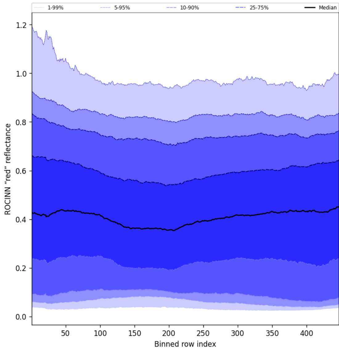
Figure 69: Along track statistics of "ROCINN "red" reflectance" for 2025-07-31 to 2025-08-02
