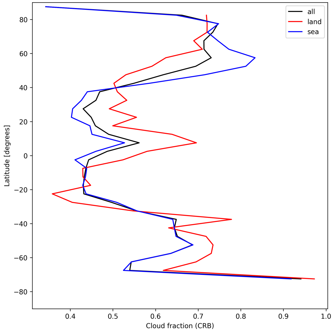
Figure 26: Zonal average of “Cloud fraction (CRB)” for 2025-07-31 to 2025-08-02.
