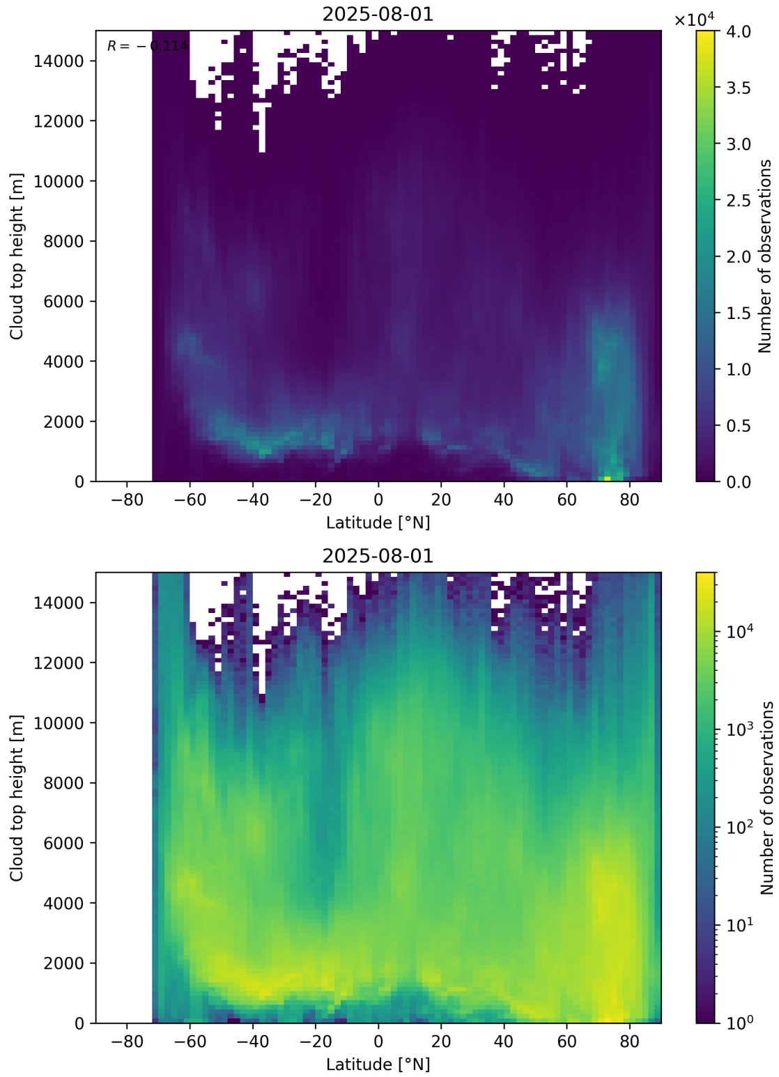
Figure 97: Scatter density plot of “Latitude” against “Cloud top height” for 2025-07-31 to 2025-08-02.
