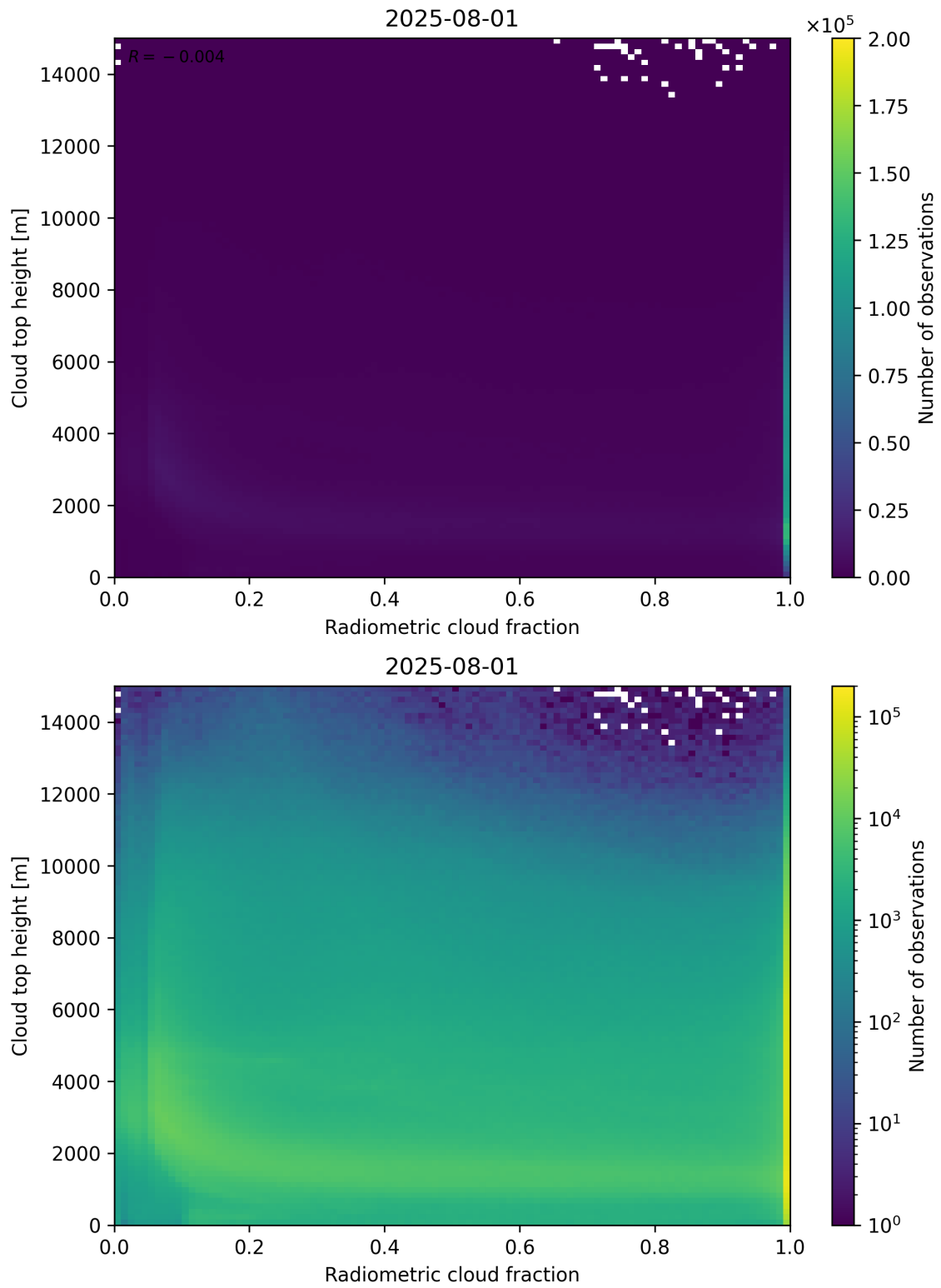
Figure 76: Scatter density plot of “Radiometric cloud fraction” against “Cloud top height” for 2025-07-31 to 2025-08-02.
