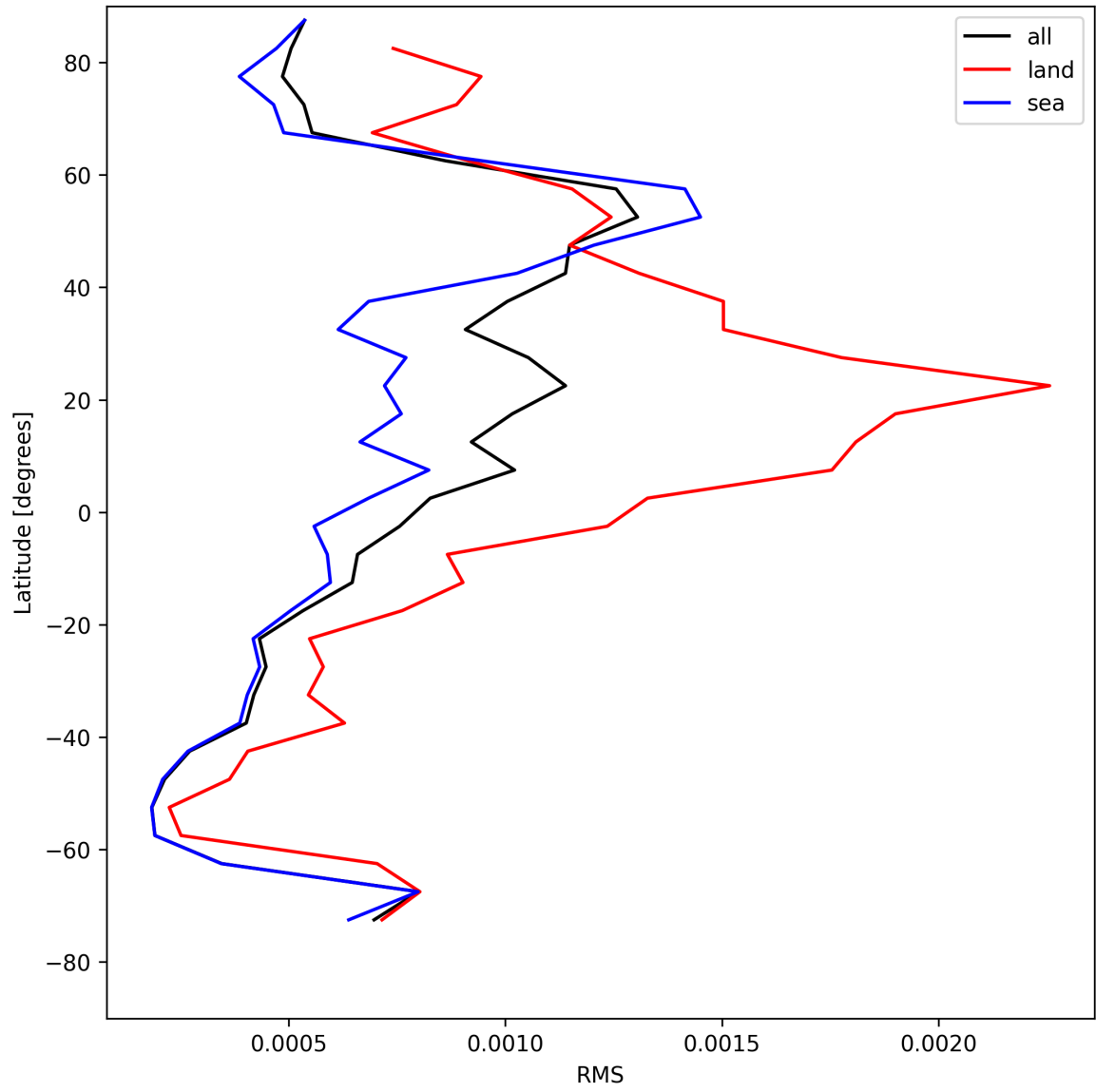
Figure 31: Zonal average of “RMS” for 2025-07-31 to 2025-08-02.
