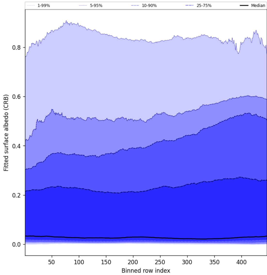
Figure 62: Along track statistics of “Fitted surface albedo (CRB)” for 2025-07-31 to 2025-08-02
