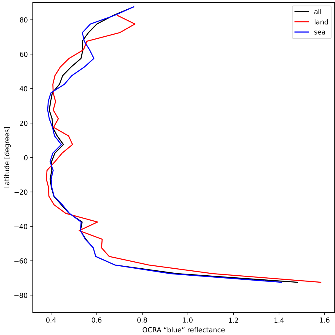
Figure 35: Zonal average of “OCRA “blue” reflectance” for 2025-07-31 to 2025-08-02.
