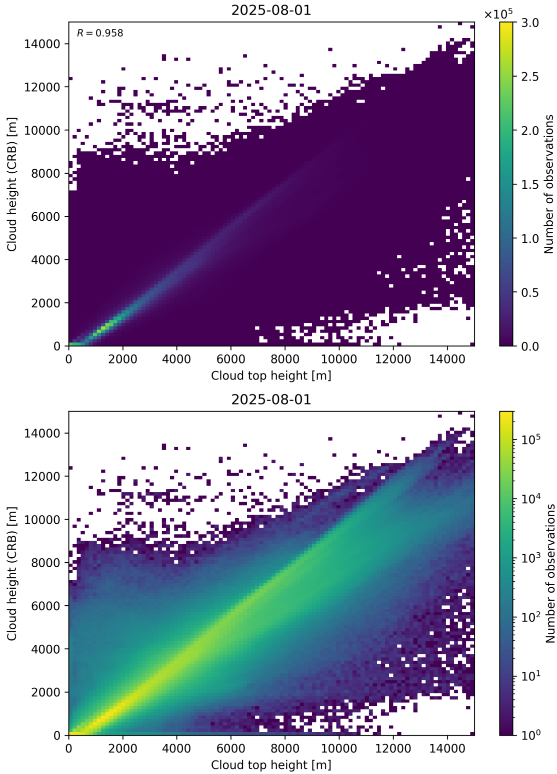
Figure 89: Scatter density plot of “Cloud top height” against “Cloud height (CRB)” for 2025-07-31 to 2025-08-02.
