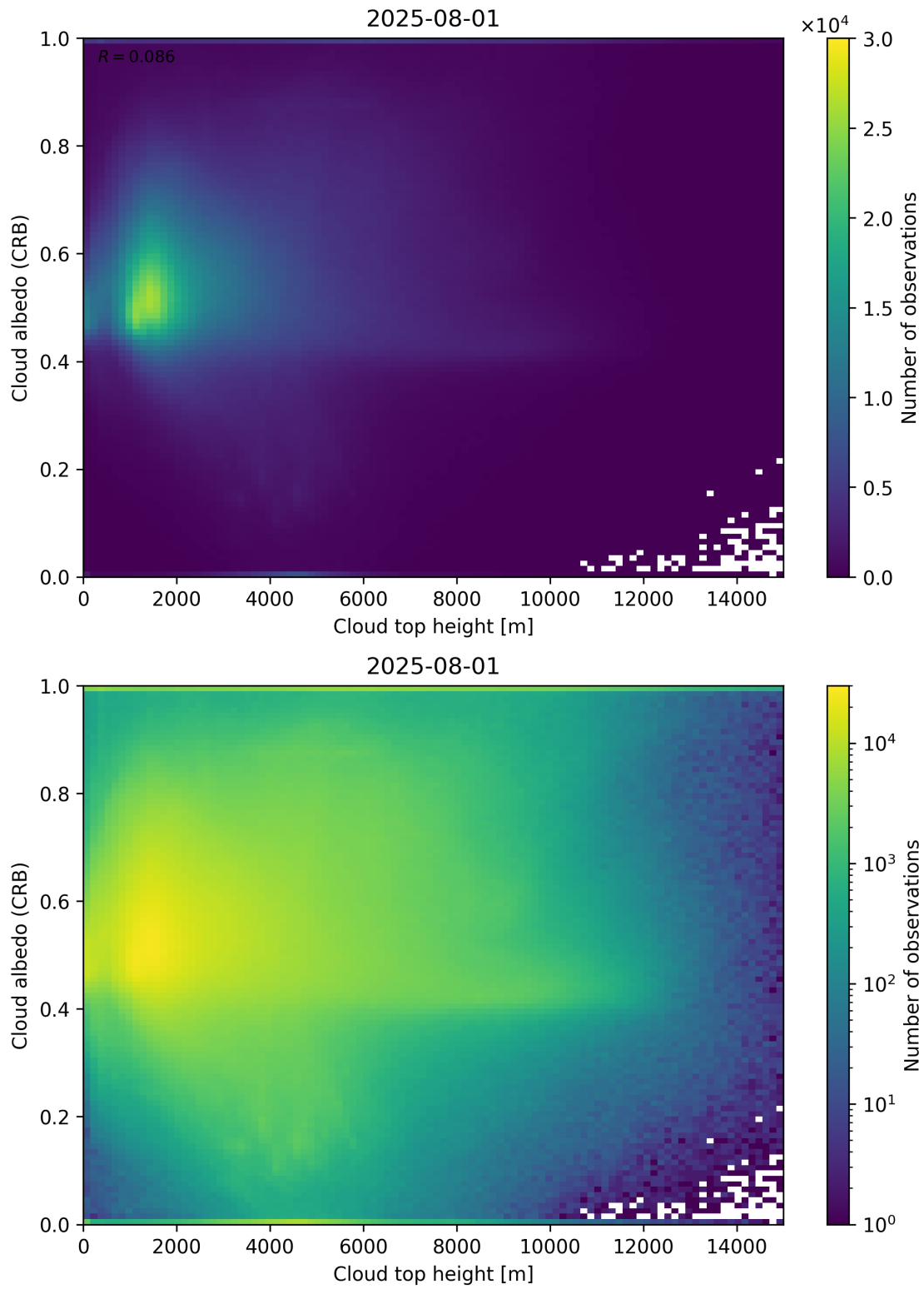
Figure 86: Scatter density plot of “Cloud top height” against “Cloud albedo (CRB)” for 2025-07-31 to 2025-08-02.
