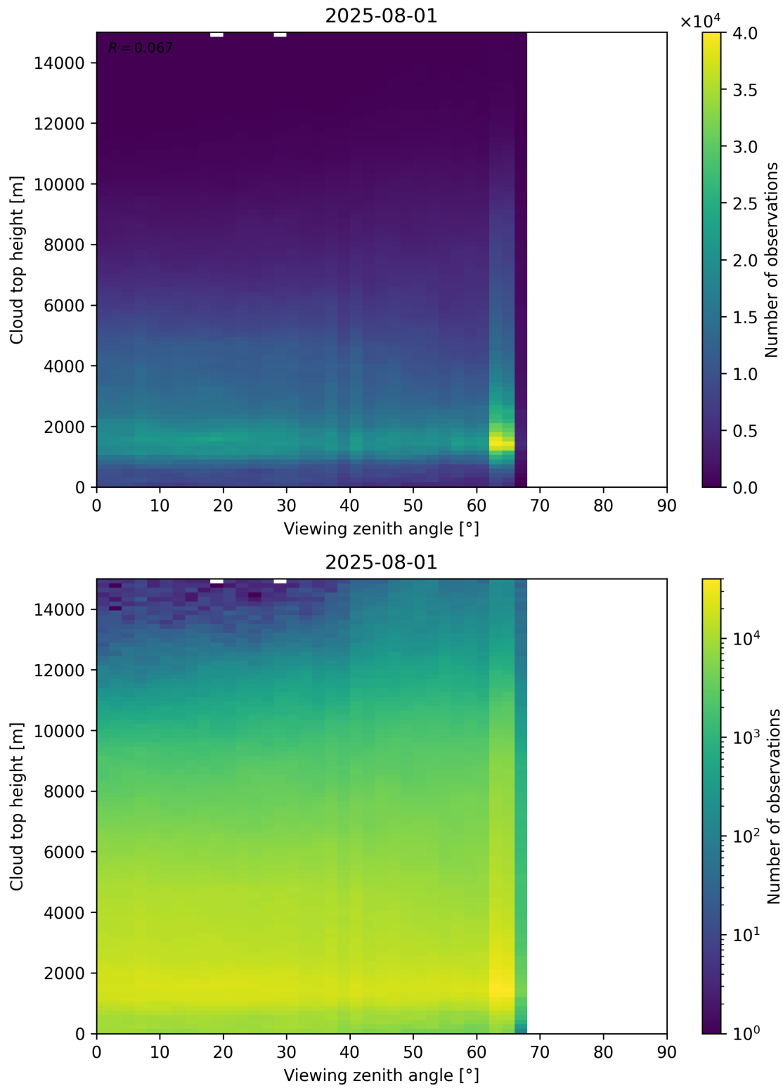
Figure 112: Scatter density plot of “Viewing zenith angle” against “Cloud top height” for 2025-07-31 to 2025-08-02.
