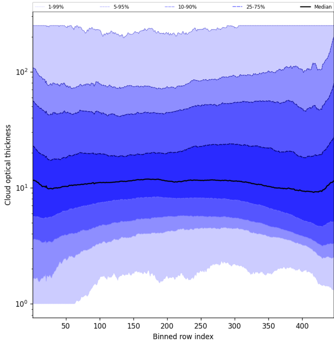
Figure 57: Along track statistics of “Cloud optical thickness” for 2025-07-31 to 2025-08-02
