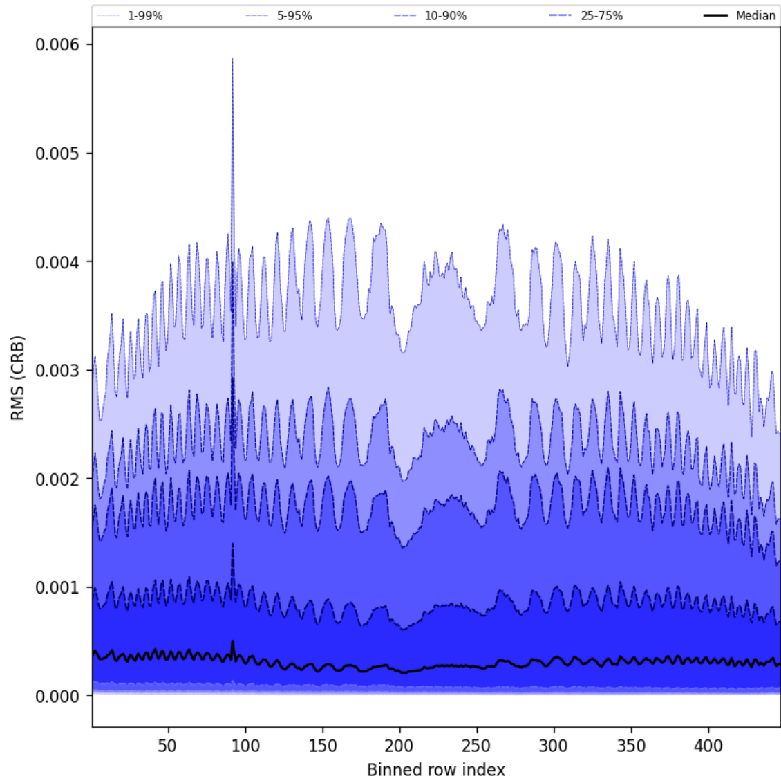
Figure 64: Along track statistics of “RMS (CRB)” for 2025-07-31 to 2025-08-02
