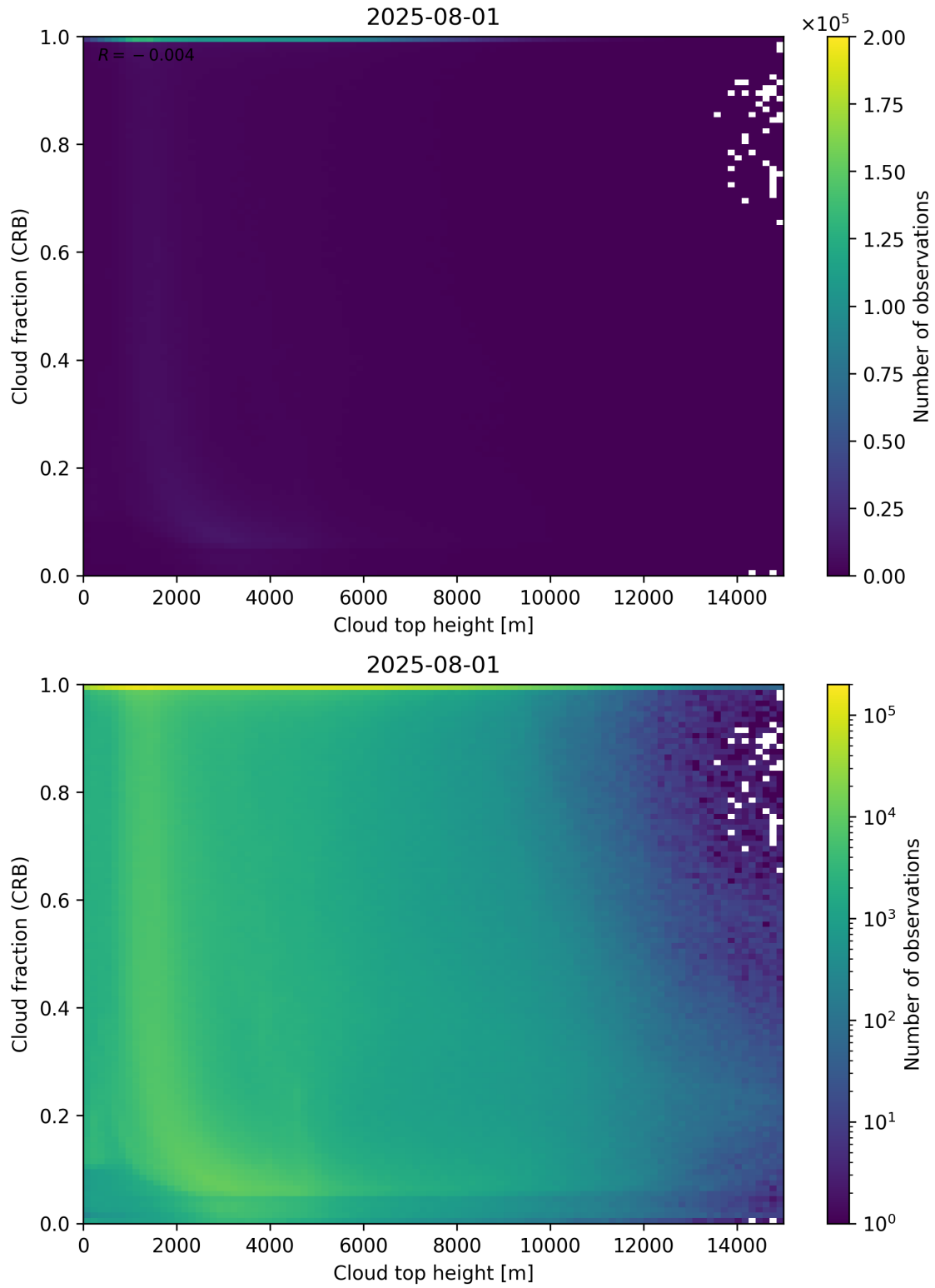
Figure 88: Scatter density plot of “Cloud top height” against “Cloud fraction (CRB)” for 2025-07-31 to 2025-08-02.
