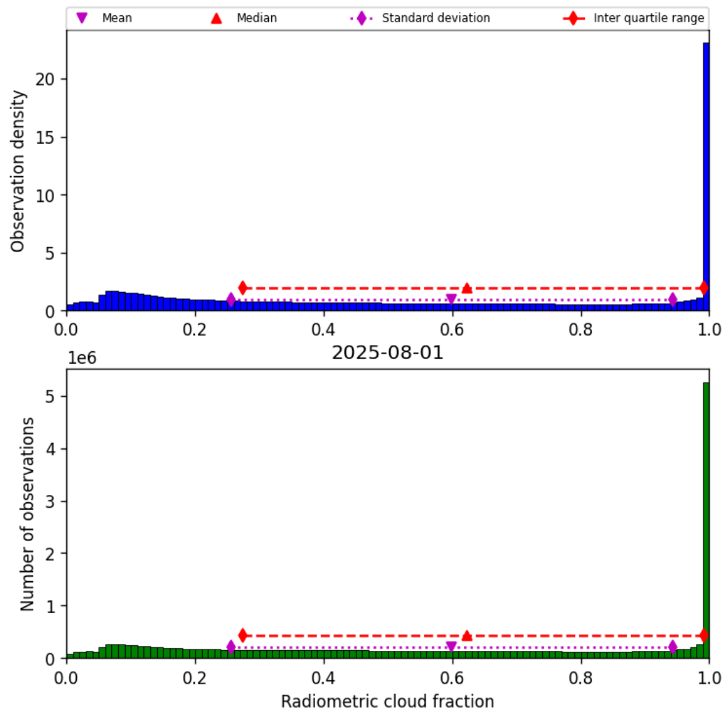
Figure 39: Histogram of “Radiometric cloud fraction” for 2025-07-31 to 2025-08-02
