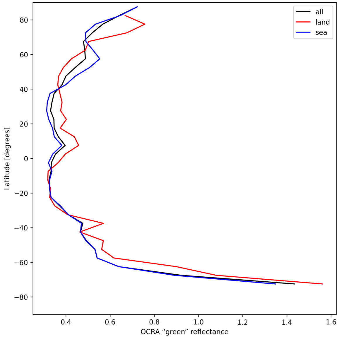
Figure 36: Zonal average of “OCRA “green” reflectance” for 2025-07-31 to 2025-08-02.
