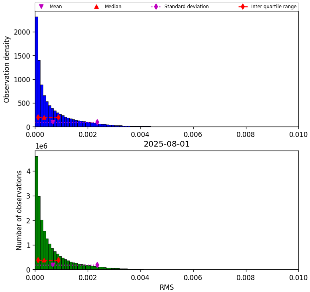
Figure 47: Histogram of “RMS” for 2025-07-31 to 2025-08-02
