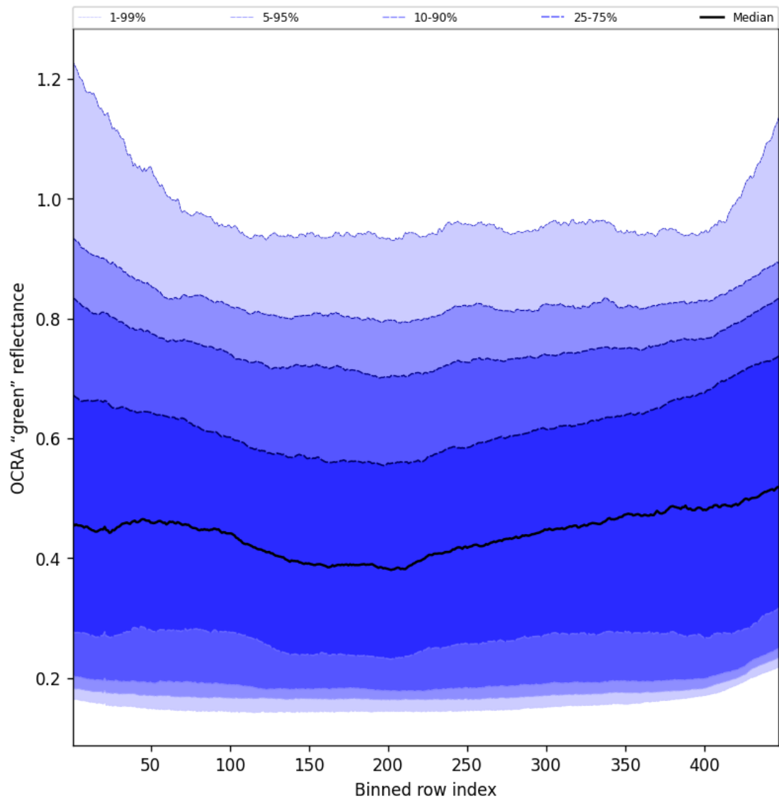
Figure 68: Along track statistics of “OCRA “green” reflectance” for 2025-07-31 to 2025-08-02
