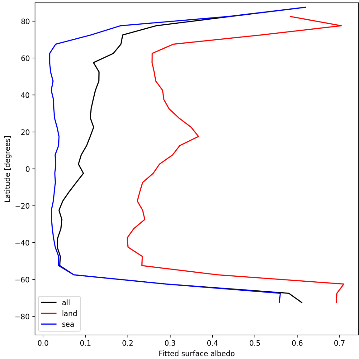
Figure 29: Zonal average of “Fitted surface albedo” for 2025-07-31 to 2025-08-02.
