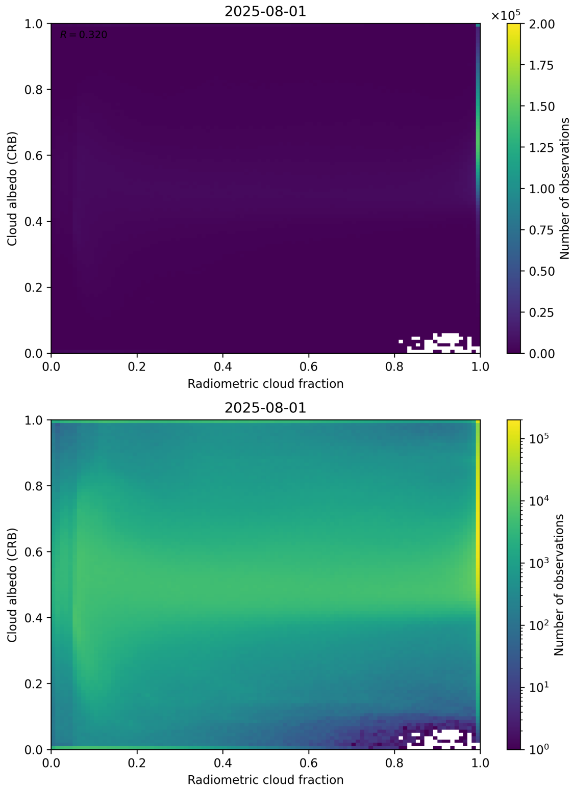
Figure 71: Scatter density plot of “Radiometric cloud fraction” against “Cloud albedo (CRB)” for 2025-07-31 to 2025-08-02.
