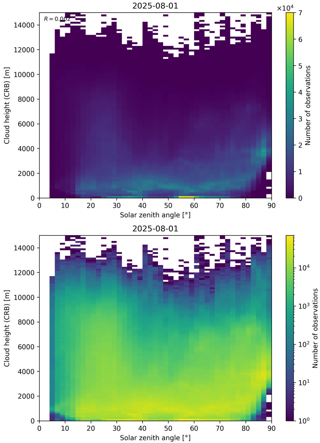
Figure 102: Scatter density plot of “Solar zenith angle” against “Cloud height (CRB)” for 2025-07-31 to 2025-08-02.
