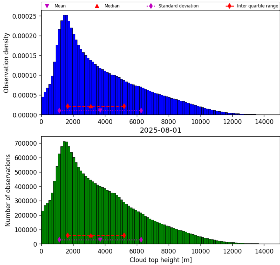
Figure 40: Histogram of “Cloud top height” for 2025-07-31 to 2025-08-02
