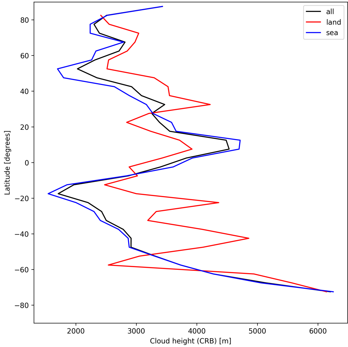
Figure 27: Zonal average of “Cloud height (CRB)” for 2025-07-31 to 2025-08-02.
