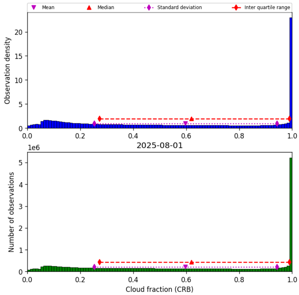
Figure 42: Histogram of “Cloud fraction (CRB)” for 2025-07-31 to 2025-08-02
