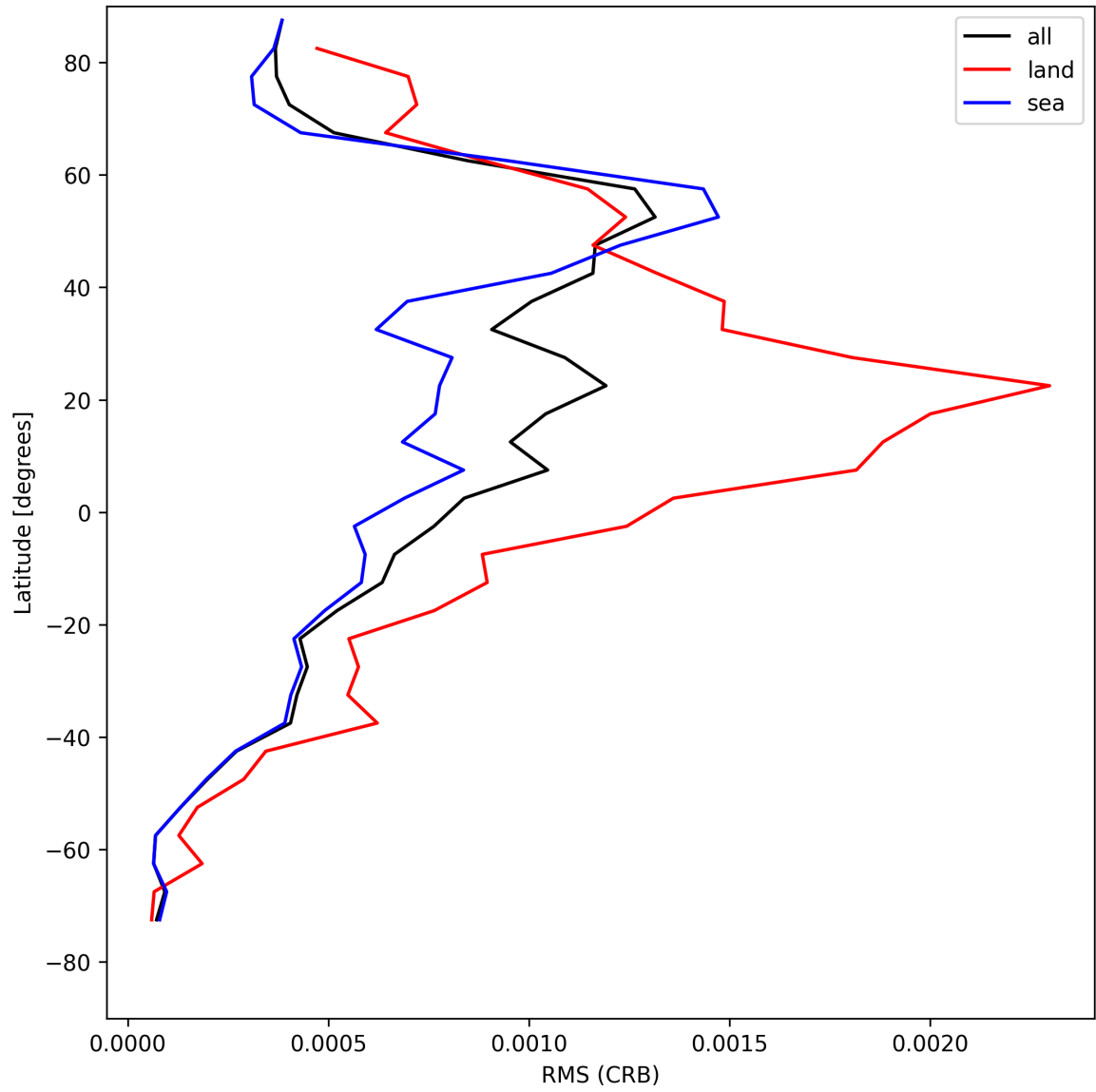
Figure 32: Zonal average of “RMS (CRB)” for 2025-07-31 to 2025-08-02.
