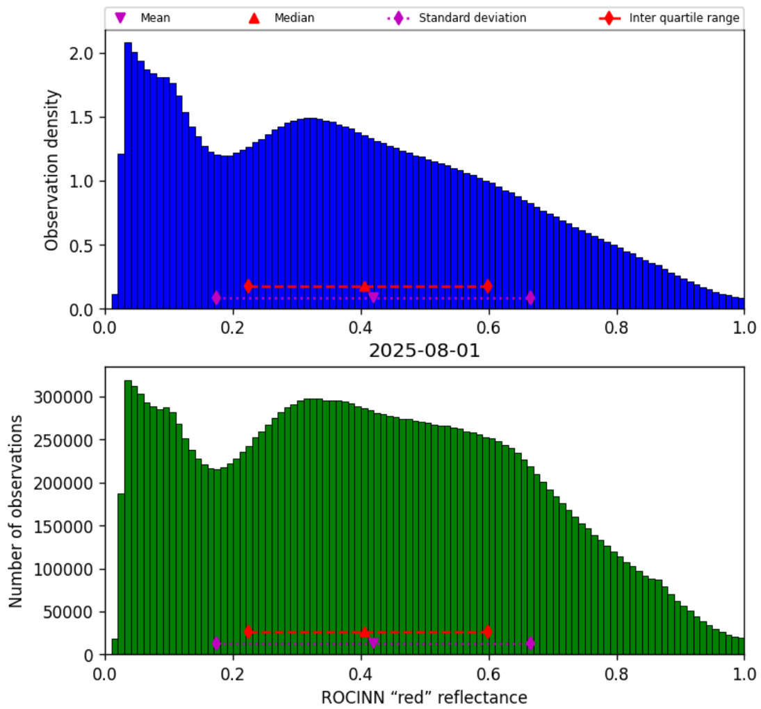
Figure 53: Histogram of “ROCINN “red” reflectance” for 2025-07-31 to 2025-08-02
