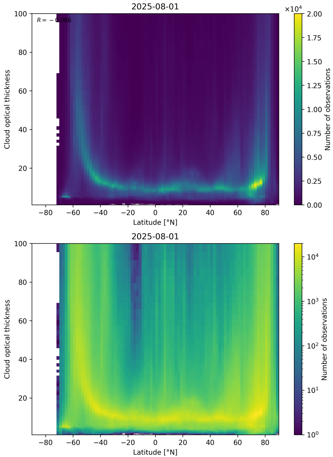
Figure 96: Scatter density plot of “Latitude” against “Cloud optical thickness” for 2025-07-31 to 2025-08-02.
