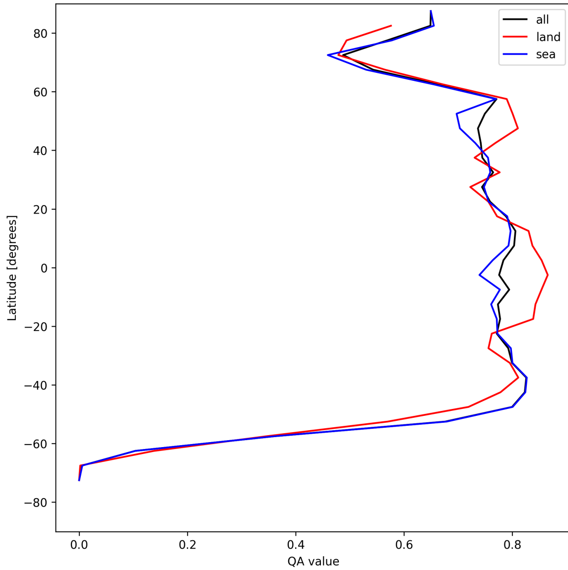
Figure 22: Zonal average of “QA value” for 2025-07-31 to 2025-08-02.
