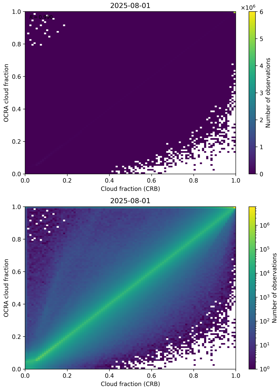
Figure 78: Scatter density plot of “Cloud fraction (CRB)” against “OCRA cloud fraction” for 2025-07-31 to 2025-08-02.
