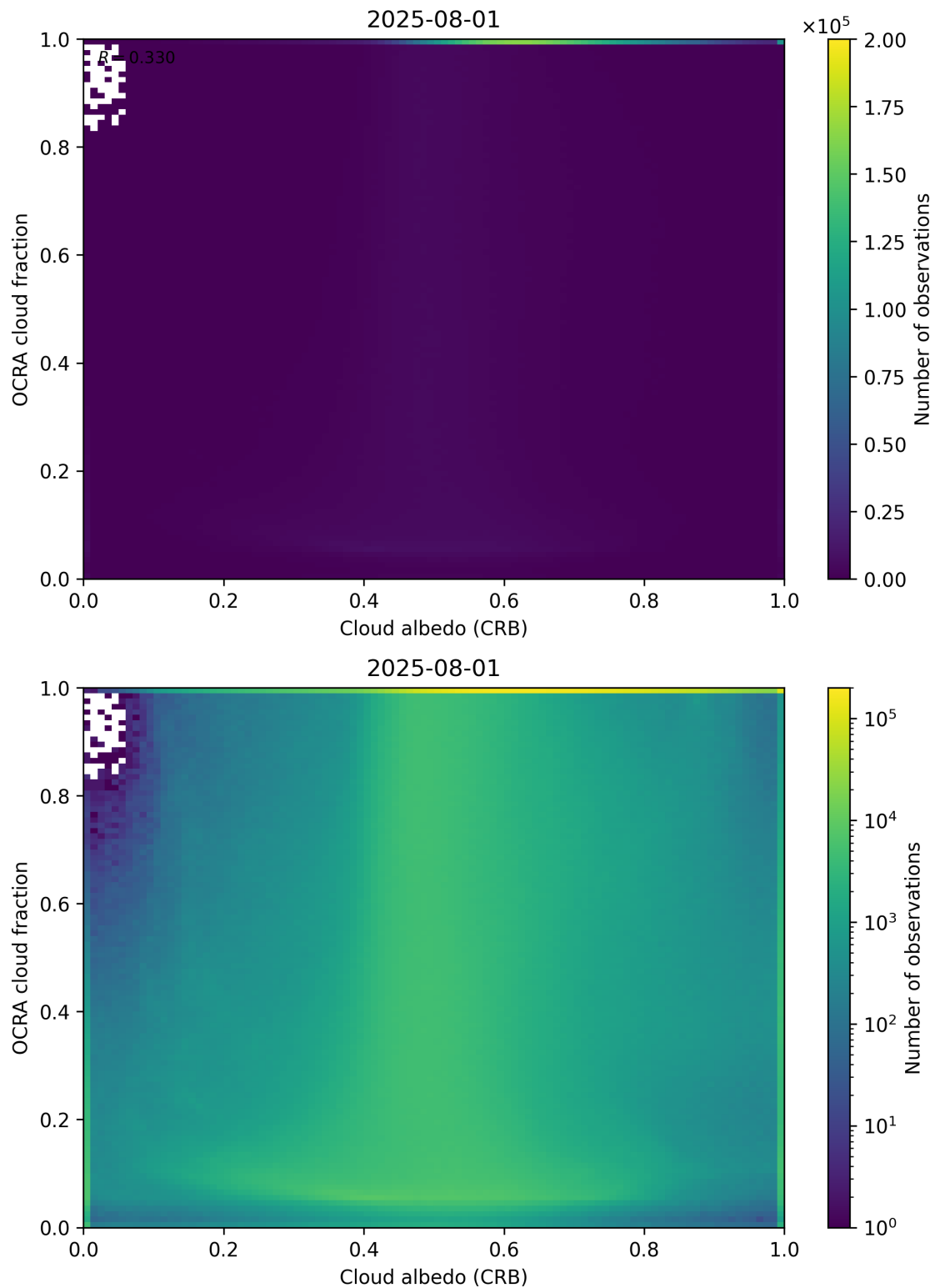
Figure 70: Scatter density plot of “Cloud albedo (CRB)” against “OCRA cloud fraction” for 2025-07-31 to 2025-08-02.
