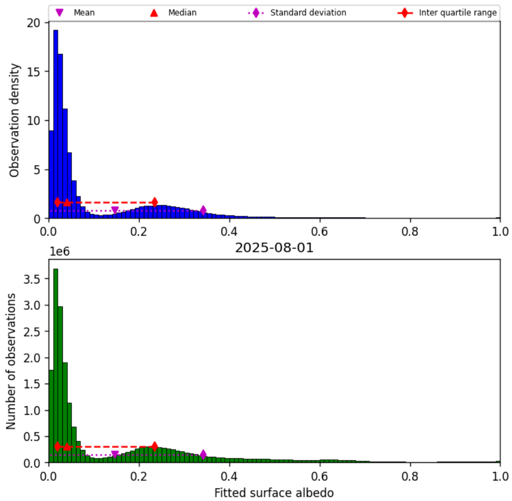
Figure 45: Histogram of “Fitted surface albedo” for 2025-07-31 to 2025-08-02
