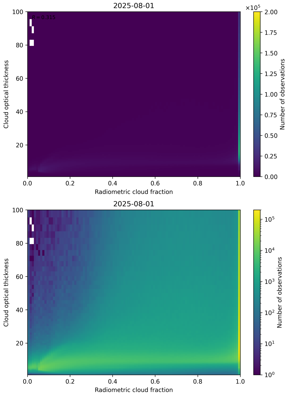
Figure 75: Scatter density plot of “Radiometric cloud fraction” against “Cloud optical thickness” for 2025-07-31 to 2025-08-02.
