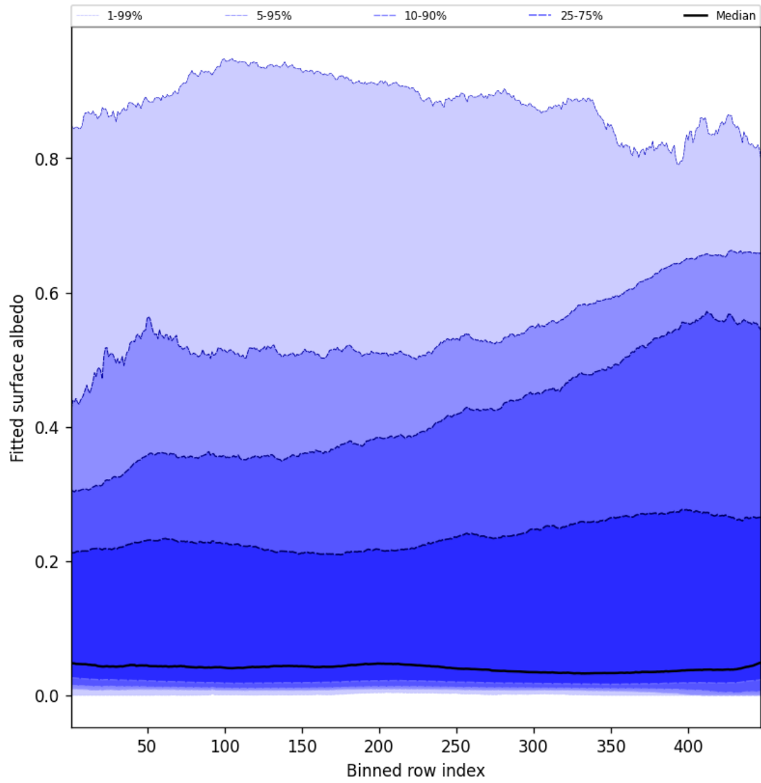
Figure 61: Along track statistics of “Fitted surface albedo” for 2025-07-31 to 2025-08-02
