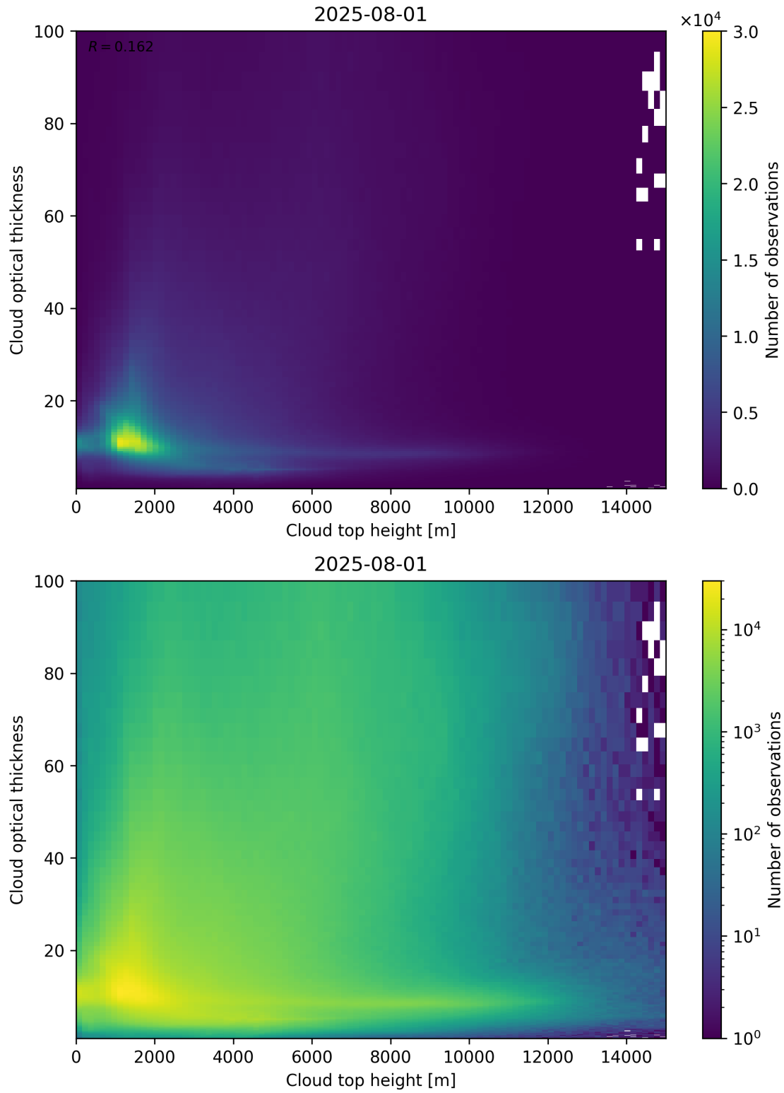
Figure 90: Scatter density plot of “Cloud top height” against “Cloud optical thickness” for 2025-07-31 to 2025-08-02.
