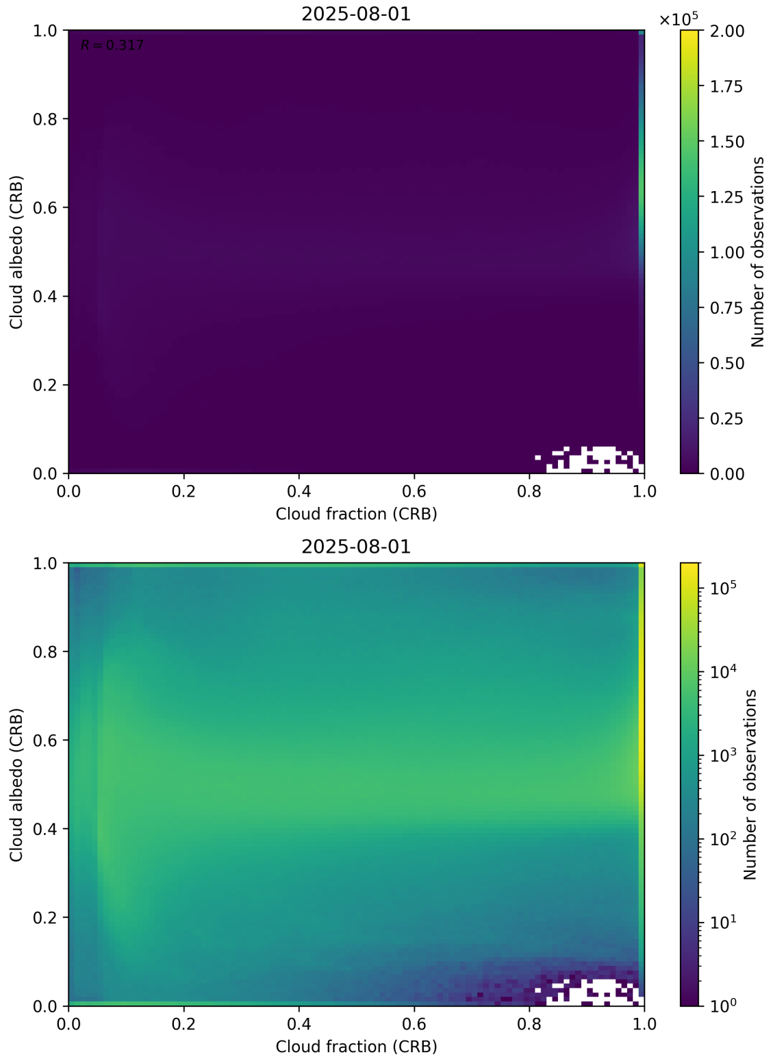
Figure 77: Scatter density plot of “Cloud fraction (CRB)” against “Cloud albedo (CRB)” for 2025-07-31 to 2025-08-02.
