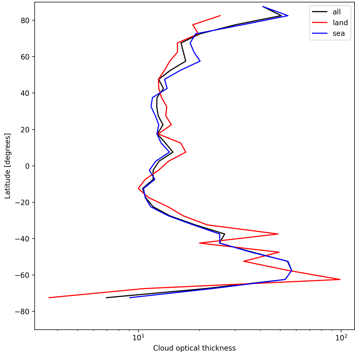
Figure 25: Zonal average of “Cloud optical thickness” for 2025-07-31 to 2025-08-02.
