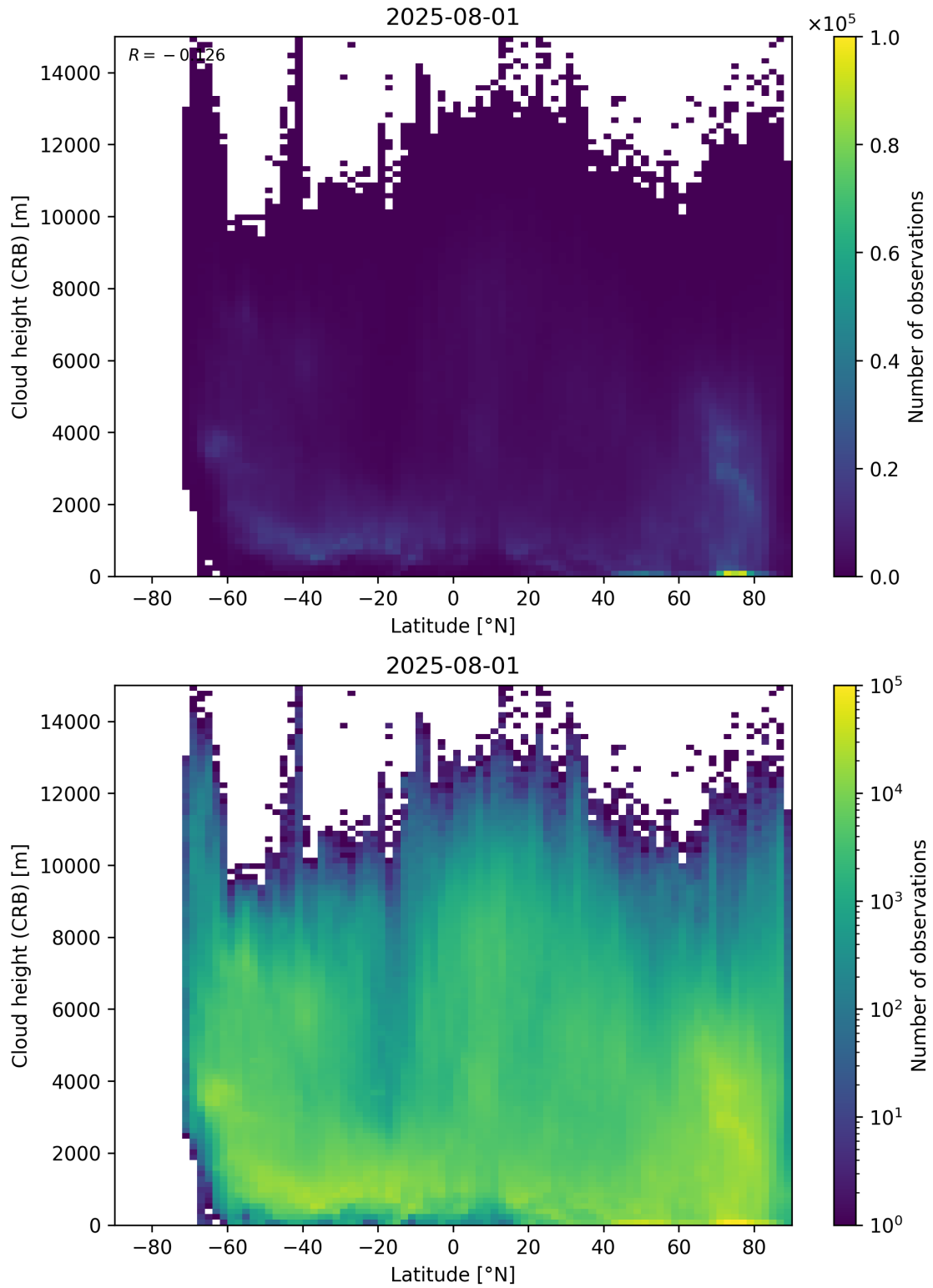
Figure 95: Scatter density plot of “Latitude” against “Cloud height (CRB)” for 2025-07-31 to 2025-08-02.
