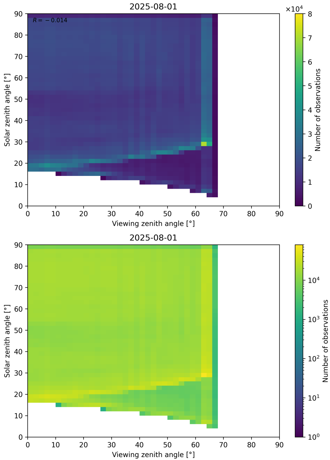
Figure 114: Scatter density plot of “Viewing zenith angle” against “Solar zenith angle” for 2025-07-31 to 2025-08-02.
