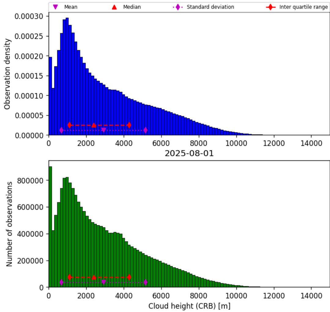
Figure 43: Histogram of “Cloud height (CRB)” for 2025-07-31 to 2025-08-02
