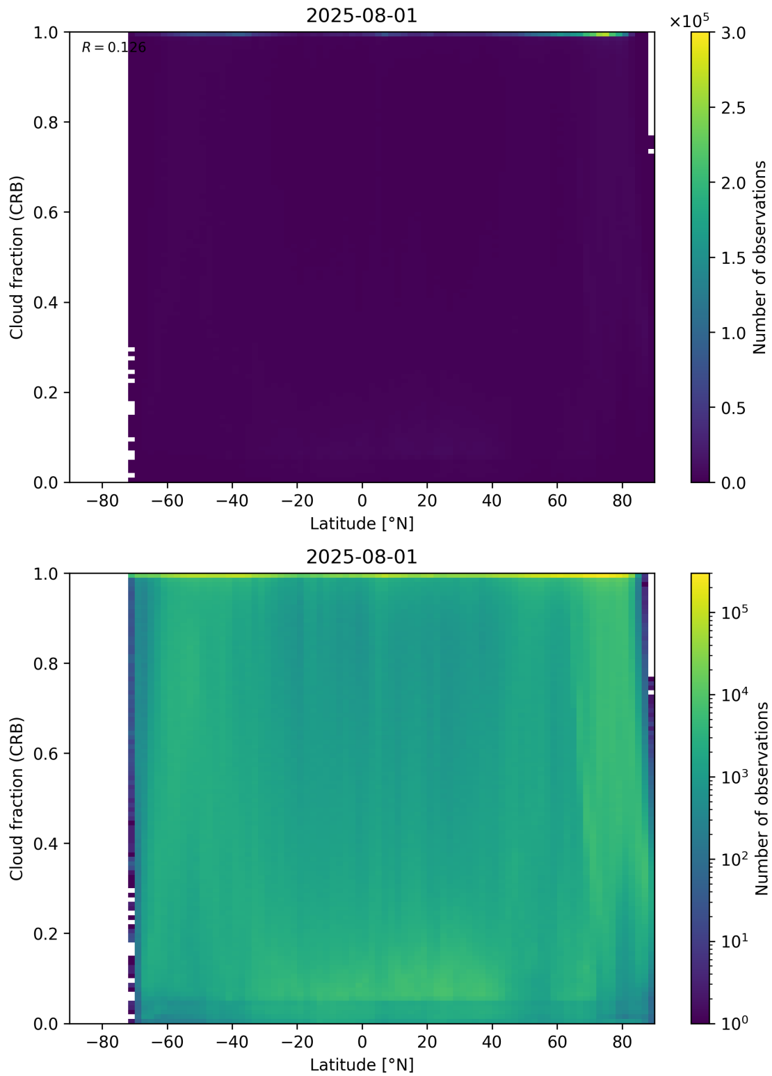
Figure 94: Scatter density plot of “Latitude” against “Cloud fraction (CRB)” for 2025-07-31 to 2025-08-02.
