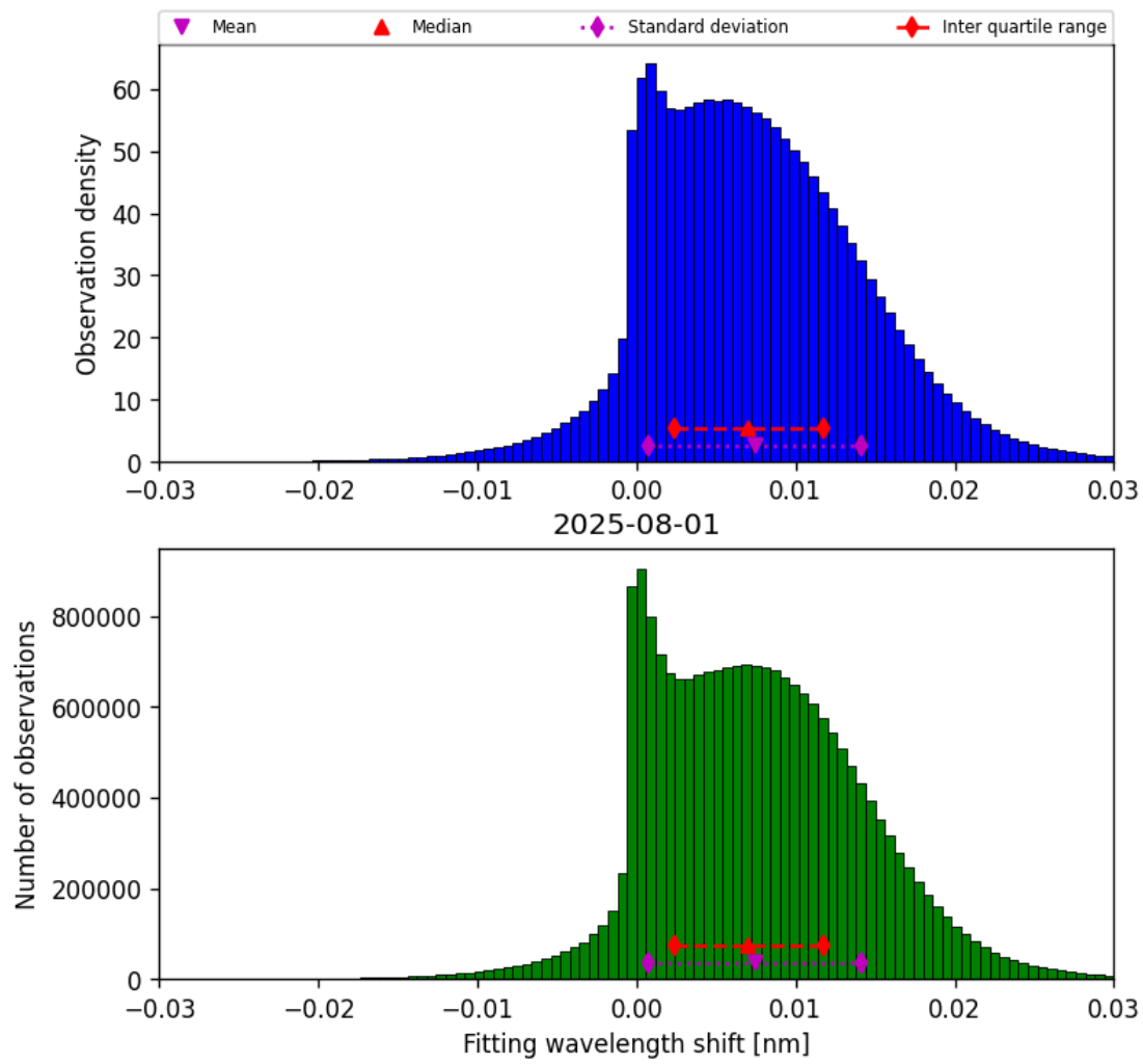
Figure 49: Histogram of “Fitting wavelength shift” for 2025-07-31 to 2025-08-02
