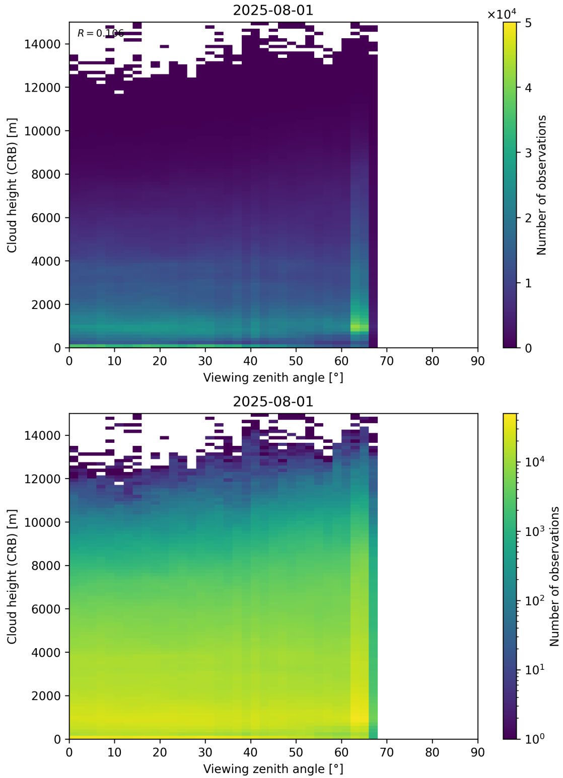
Figure 110: Scatter density plot of “Viewing zenith angle” against “Cloud height (CRB)” for 2025-07-31 to 2025-08-02.
