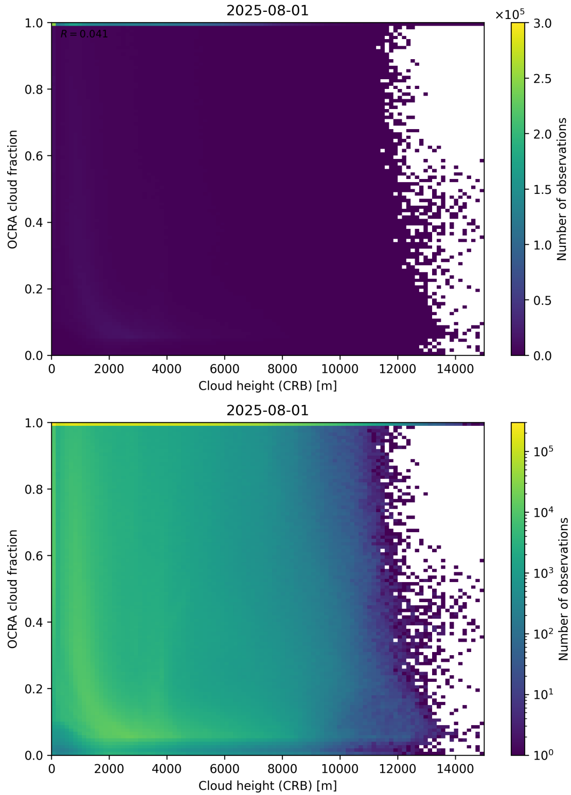
Figure 81: Scatter density plot of “Cloud height (CRB)” against “OCRA cloud fraction” for 2025-07-31 to 2025-08-02.
