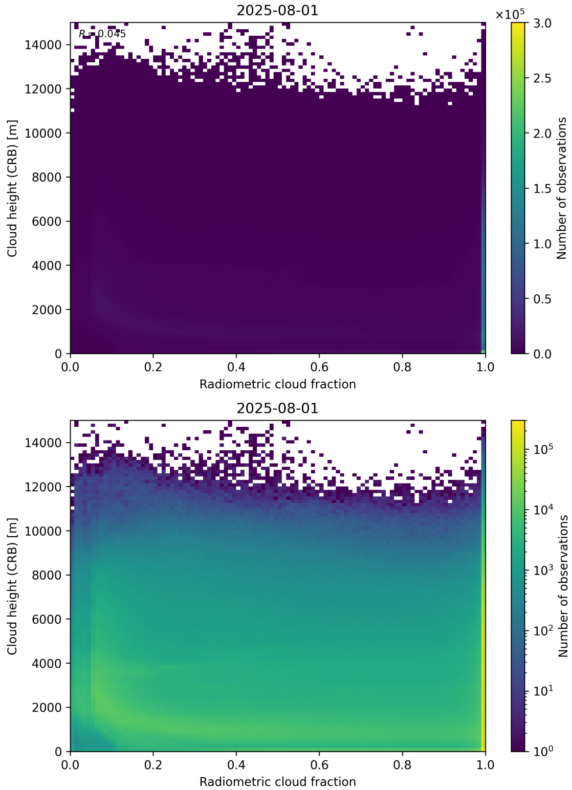
Figure 74: Scatter density plot of “Radiometric cloud fraction” against “Cloud height (CRB)” for 2025-07-31 to 2025-08-02.
