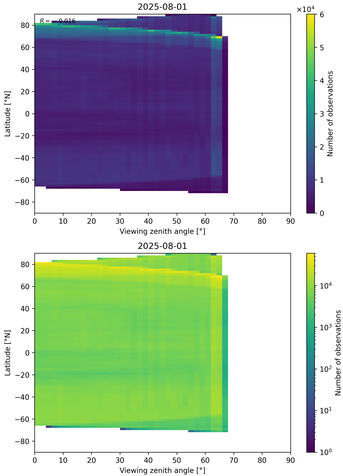
Figure 113: Scatter density plot of “Viewing zenith angle” against “Latitude” for 2025-07-31 to 2025-08-02.
