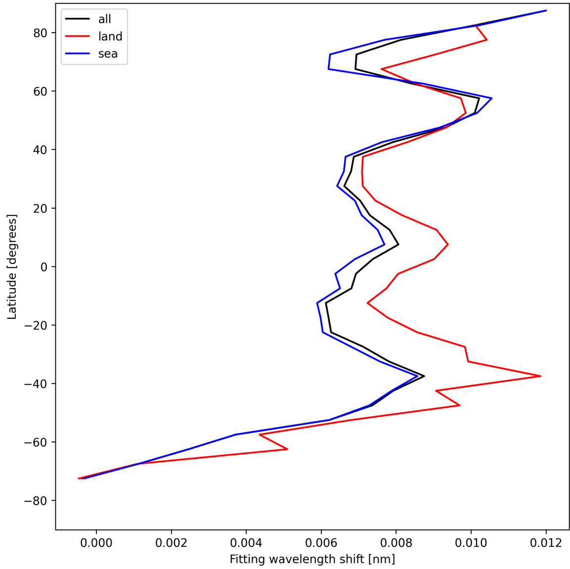
Figure 33: Zonal average of “Fitting wavelength shift” for 2025-07-31 to 2025-08-02.
