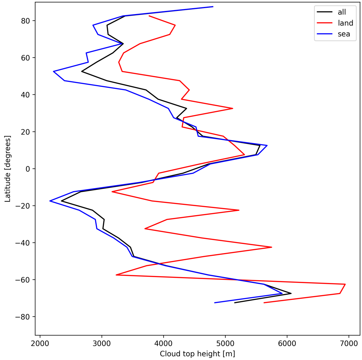
Figure 24: Zonal average of “Cloud top height” for 2025-07-31 to 2025-08-02.
