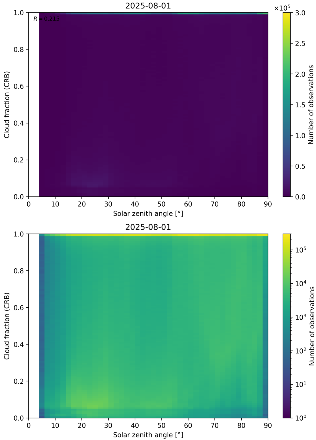
Figure 101: Scatter density plot of “Solar zenith angle” against “Cloud fraction (CRB)” for 2025-07-31 to 2025-08-02.
