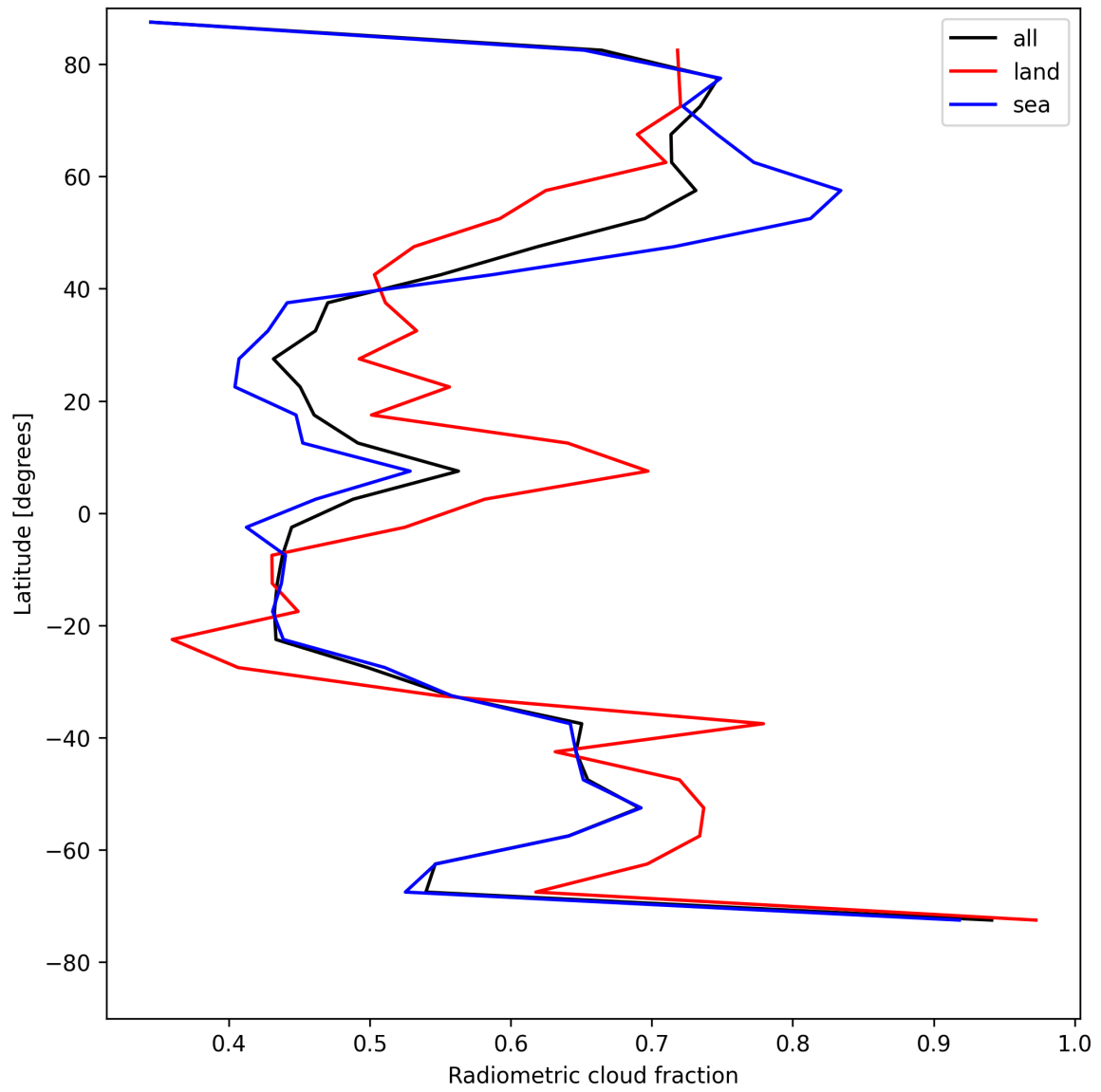
Figure 23: Zonal average of “Radiometric cloud fraction” for 2025-07-31 to 2025-08-02.
