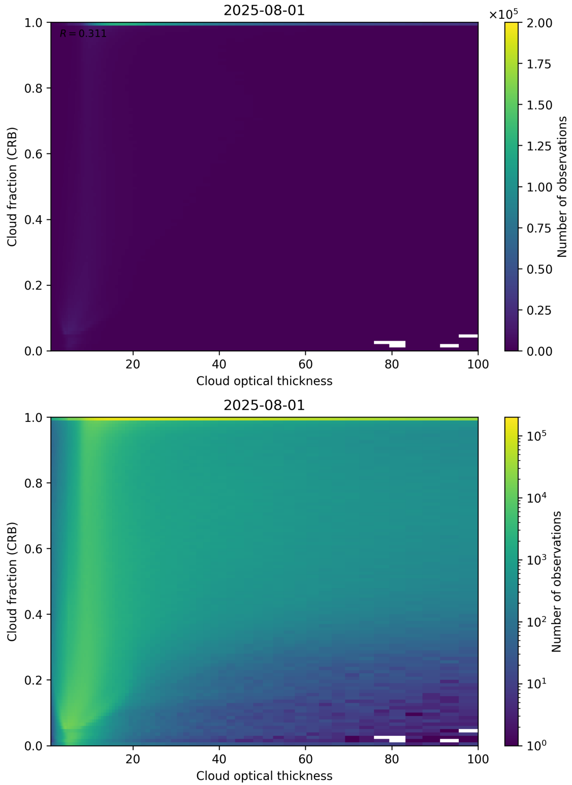
Figure 84: Scatter density plot of “Cloud optical thickness” against “Cloud fraction (CRB)” for 2025-07-31 to 2025-08-02.
