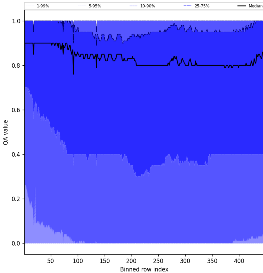
Figure 54: Along track statistics of “QA value” for 2025-07-31 to 2025-08-02
