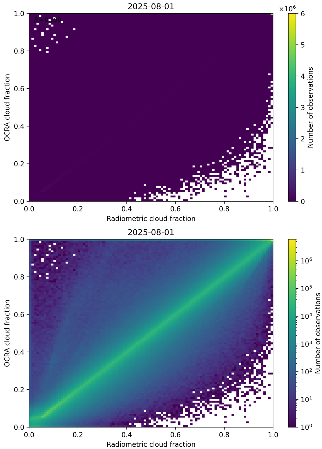
Figure 72: Scatter density plot of “Radiometric cloud fraction” against “OCRA cloud fraction” for 2025-07-31 to 2025-08-02.
