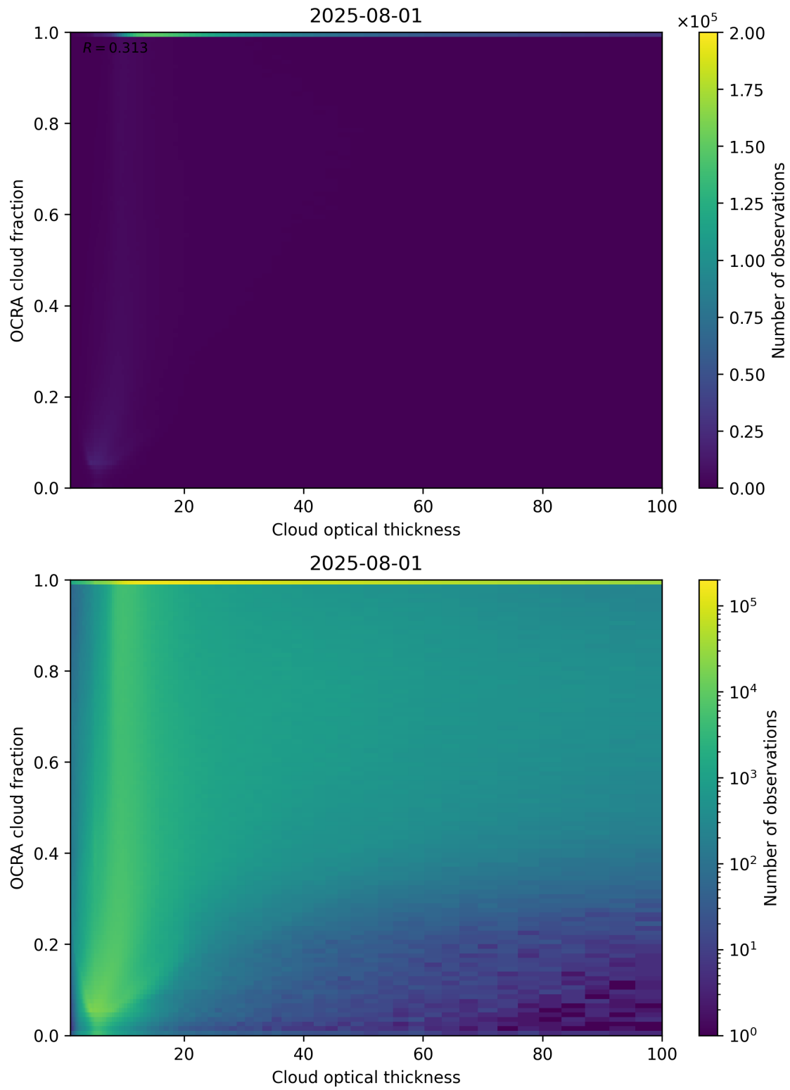
Figure 83: Scatter density plot of “Cloud optical thickness” against “OCRA cloud fraction” for 2025-07-31 to 2025-08-02.
