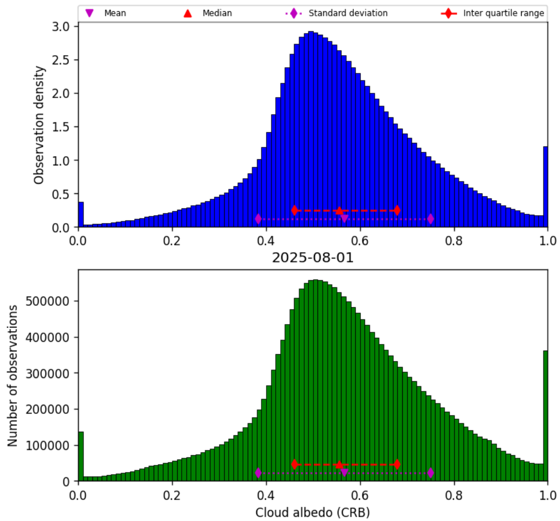
Figure 44: Histogram of “Cloud albedo (CRB)” for 2025-07-31 to 2025-08-02
