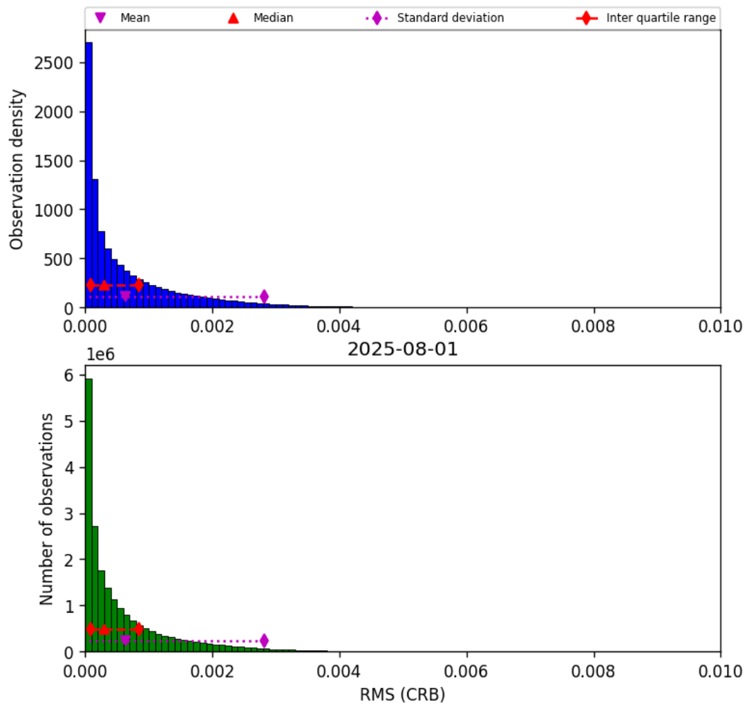
Figure 48: Histogram of “RMS (CRB)” for 2025-07-31 to 2025-08-02
