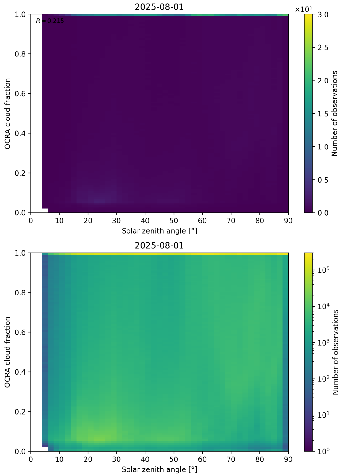
Figure 100: Scatter density plot of “Solar zenith angle” against “OCRA cloud fraction” for 2025-07-31 to 2025-08-02.
