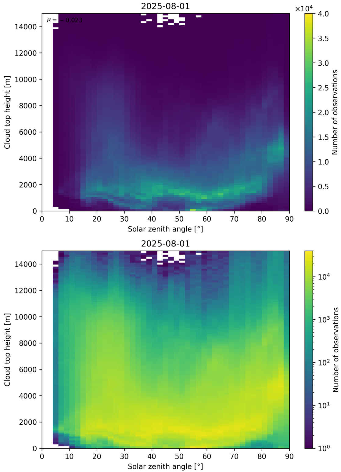
Figure 104: Scatter density plot of “Solar zenith angle” against “Cloud top height” for 2025-07-31 to 2025-08-02.
