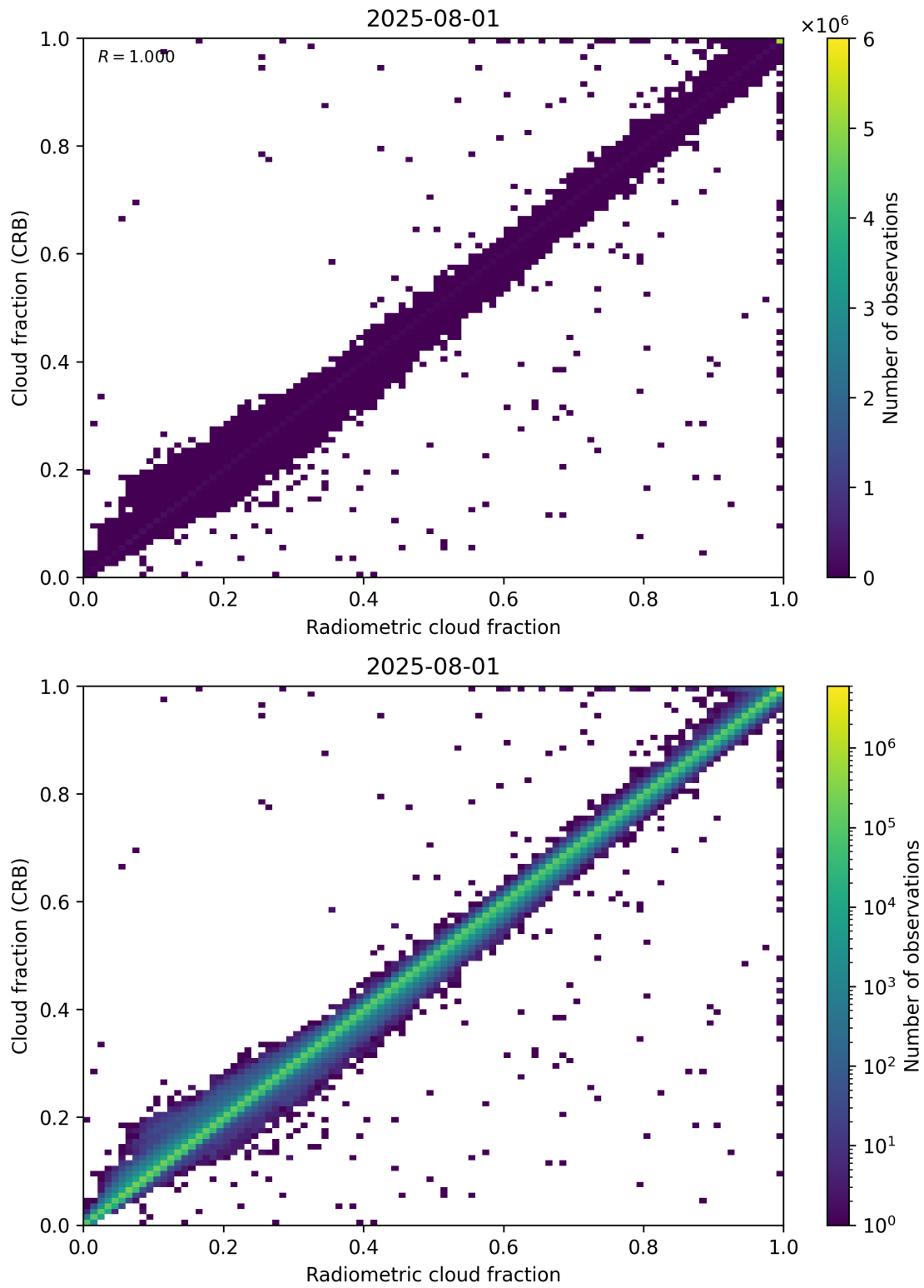
Figure 73: Scatter density plot of “Radiometric cloud fraction” against “Cloud fraction (CRB)” for 2025-07-31 to 2025-08-02.
