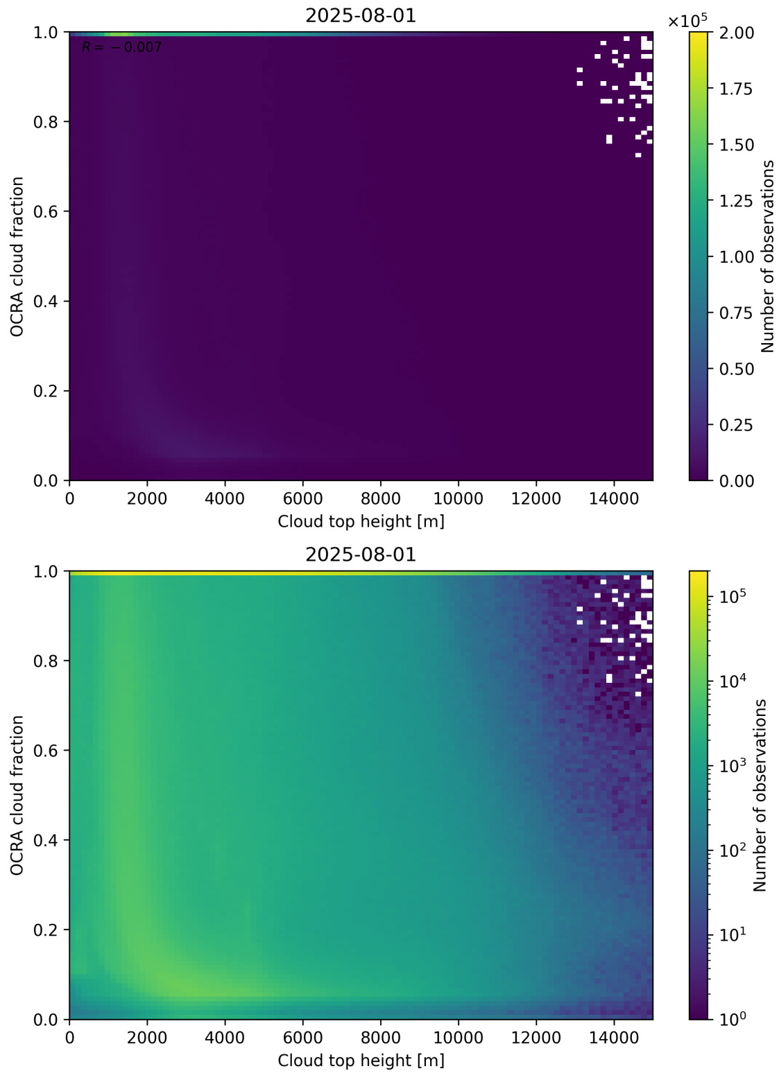
Figure 87: Scatter density plot of “Cloud top height” against “OCRA cloud fraction” for 2025-07-31 to 2025-08-02.
