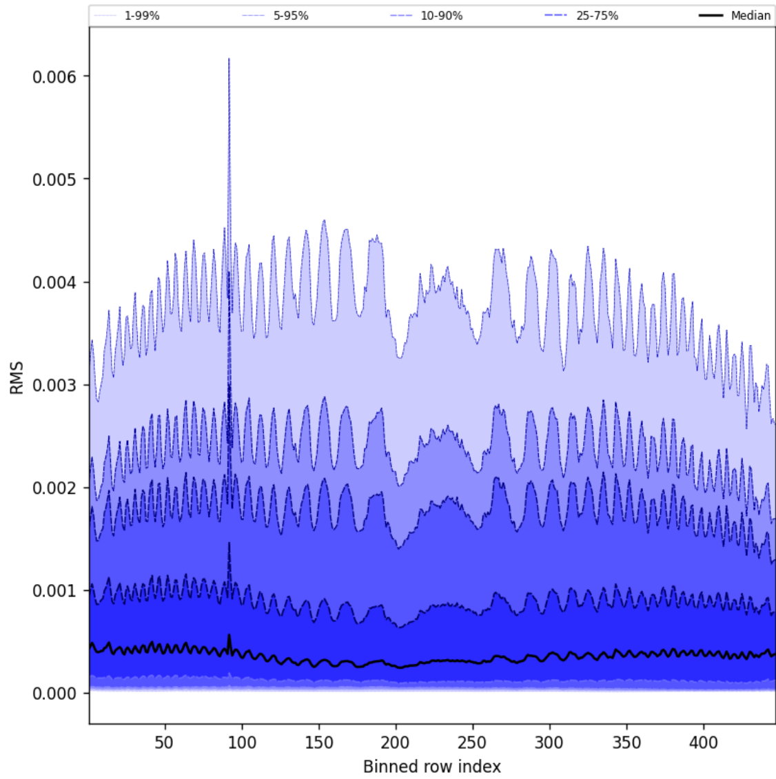
Figure 63: Along track statistics of “RMS” for 2025-07-31 to 2025-08-02
