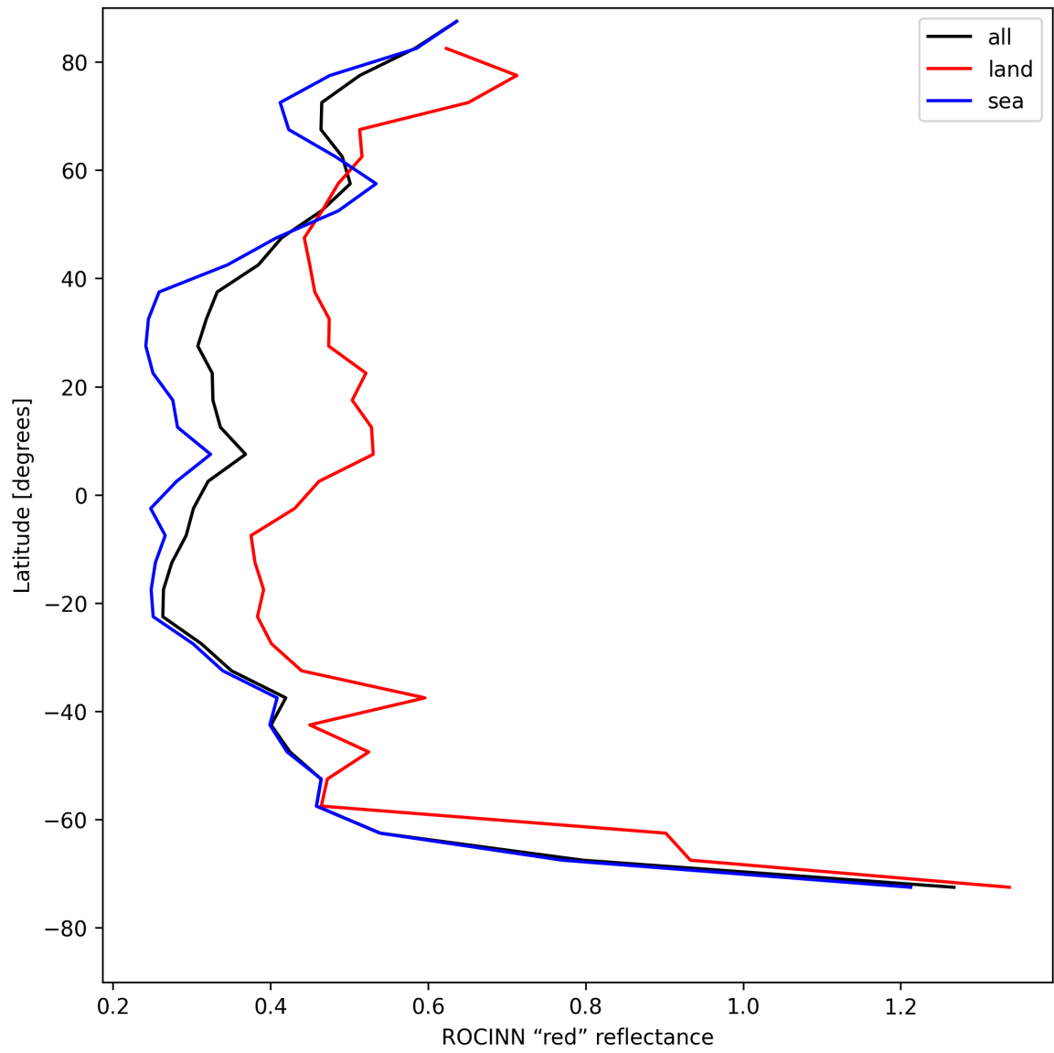
Figure 37: Zonal average of “ROCINN “red” reflectance” for 2025-07-31 to 2025-08-02.
