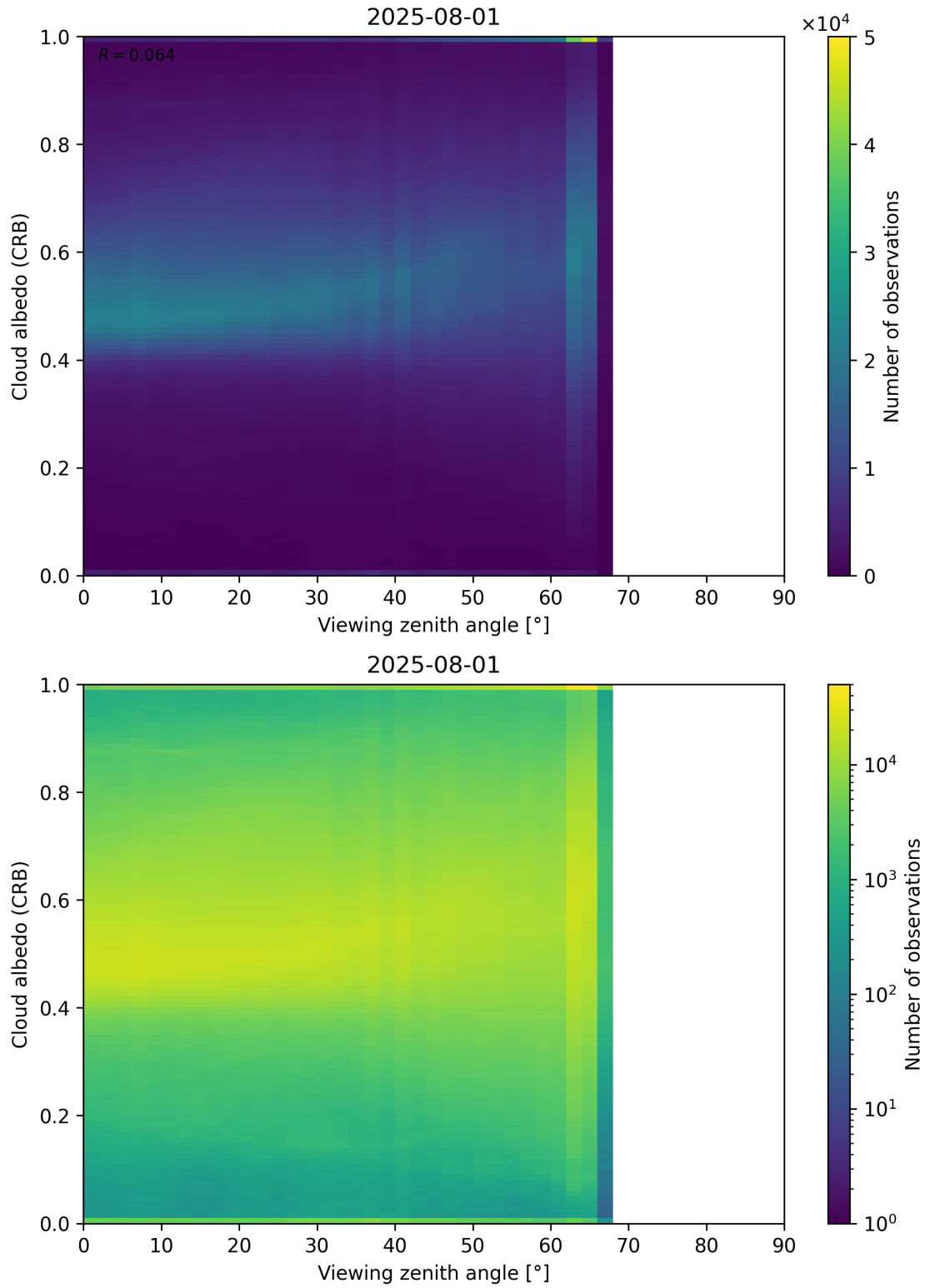
Figure 106: Scatter density plot of “Viewing zenith angle” against “Cloud albedo (CRB)” for 2025-07-31 to 2025-08-02.
