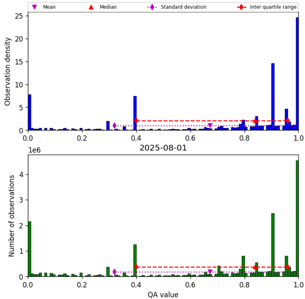
Figure 38: Histogram of “QA value” for 2025-07-31 to 2025-08-02
