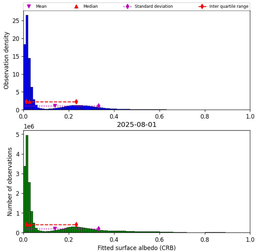
Figure 46: Histogram of “Fitted surface albedo (CRB)” for 2025-07-31 to 2025-08-02
