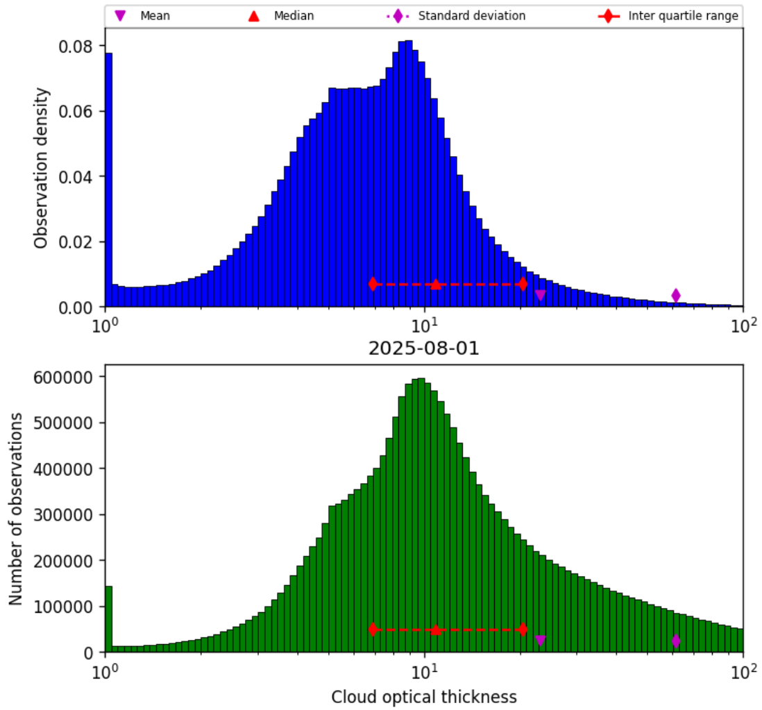
Figure 41: Histogram of “Cloud optical thickness” for 2025-07-31 to 2025-08-02
