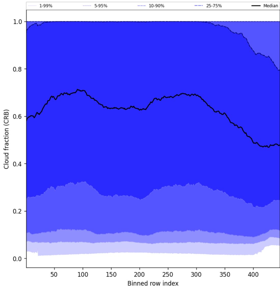
Figure 58: Along track statistics of “Cloud fraction (CRB)” for 2025-07-31 to 2025-08-02
