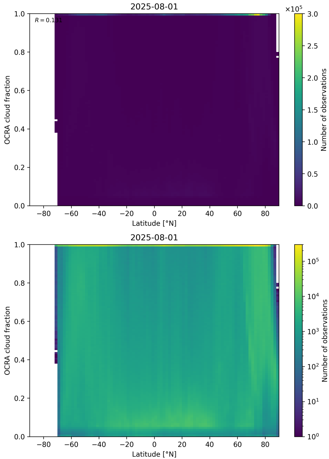
Figure 93: Scatter density plot of “Latitude” against “OCRA cloud fraction” for 2025-07-31 to 2025-08-02.
