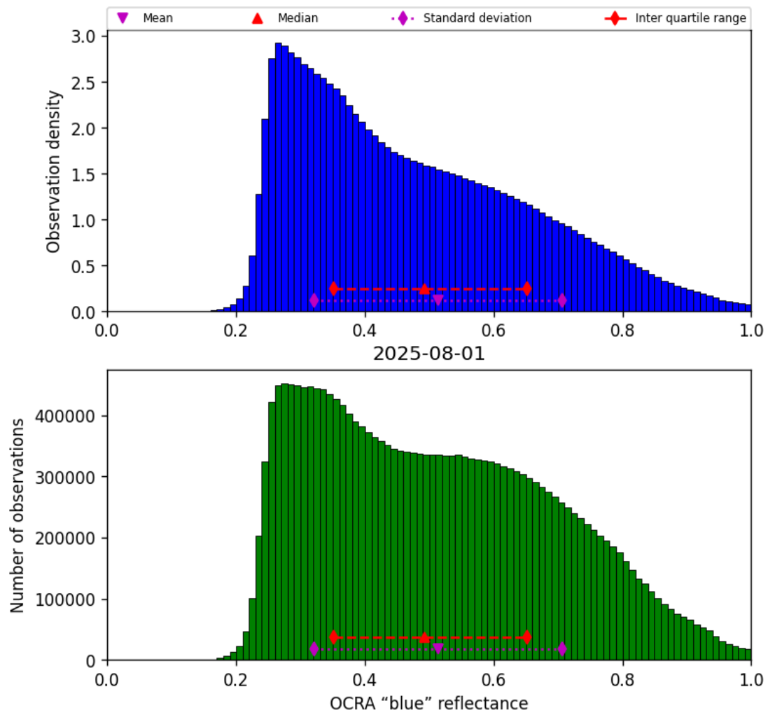
Figure 51: Histogram of “OCRA “blue” reflectance” for 2025-07-31 to 2025-08-02
