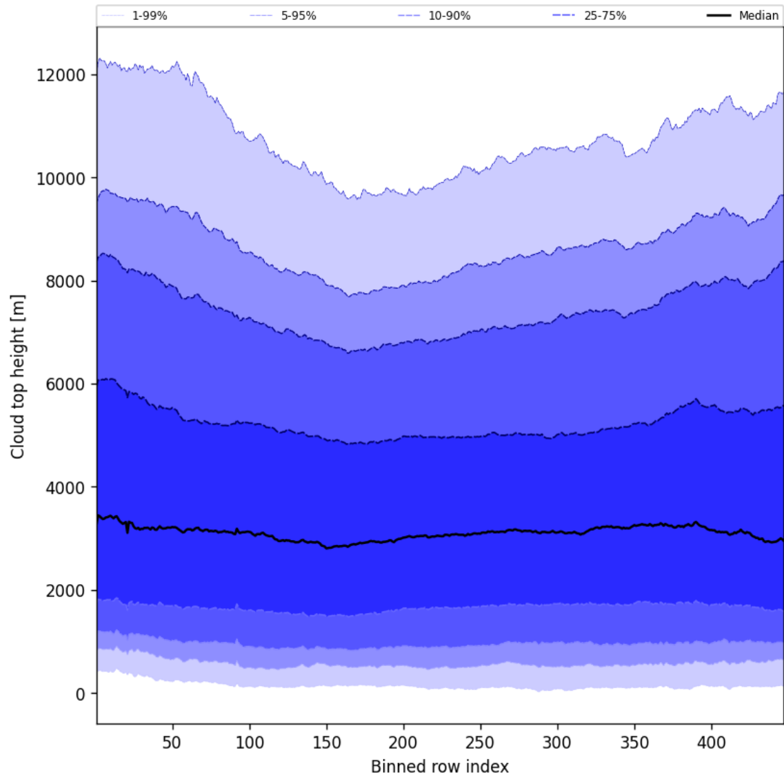
Figure 56: Along track statistics of “Cloud top height” for 2025-07-31 to 2025-08-02
