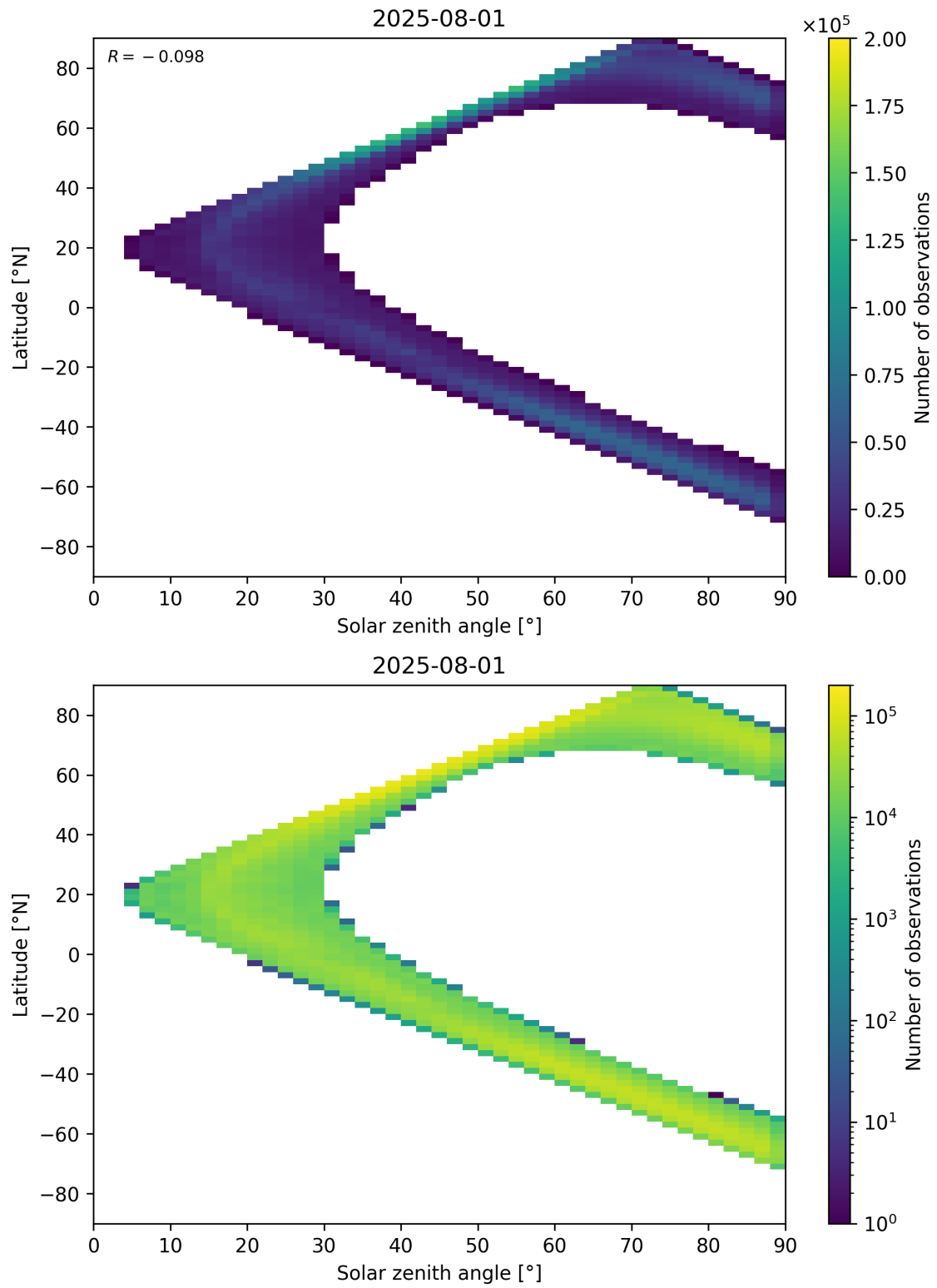
Figure 105: Scatter density plot of “Solar zenith angle” against “Latitude” for 2025-07-31 to 2025-08-02.
