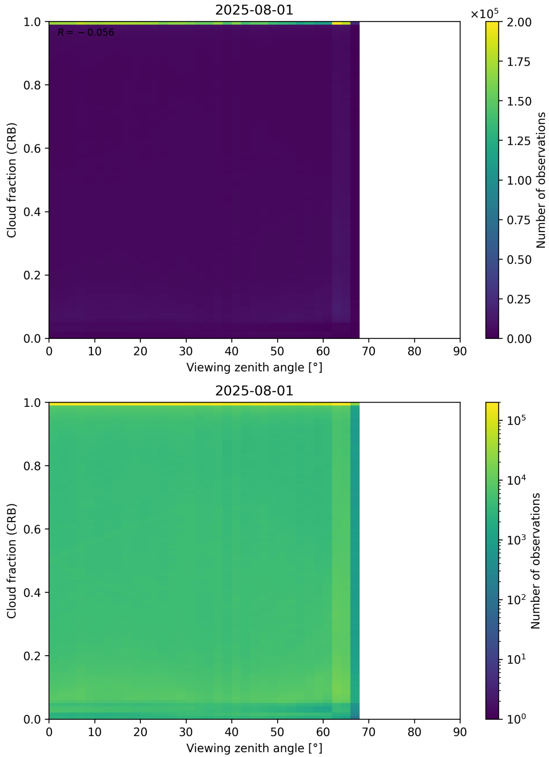
Figure 109: Scatter density plot of “Viewing zenith angle” against “Cloud fraction (CRB)” for 2025-07-31 to 2025-08-02.
