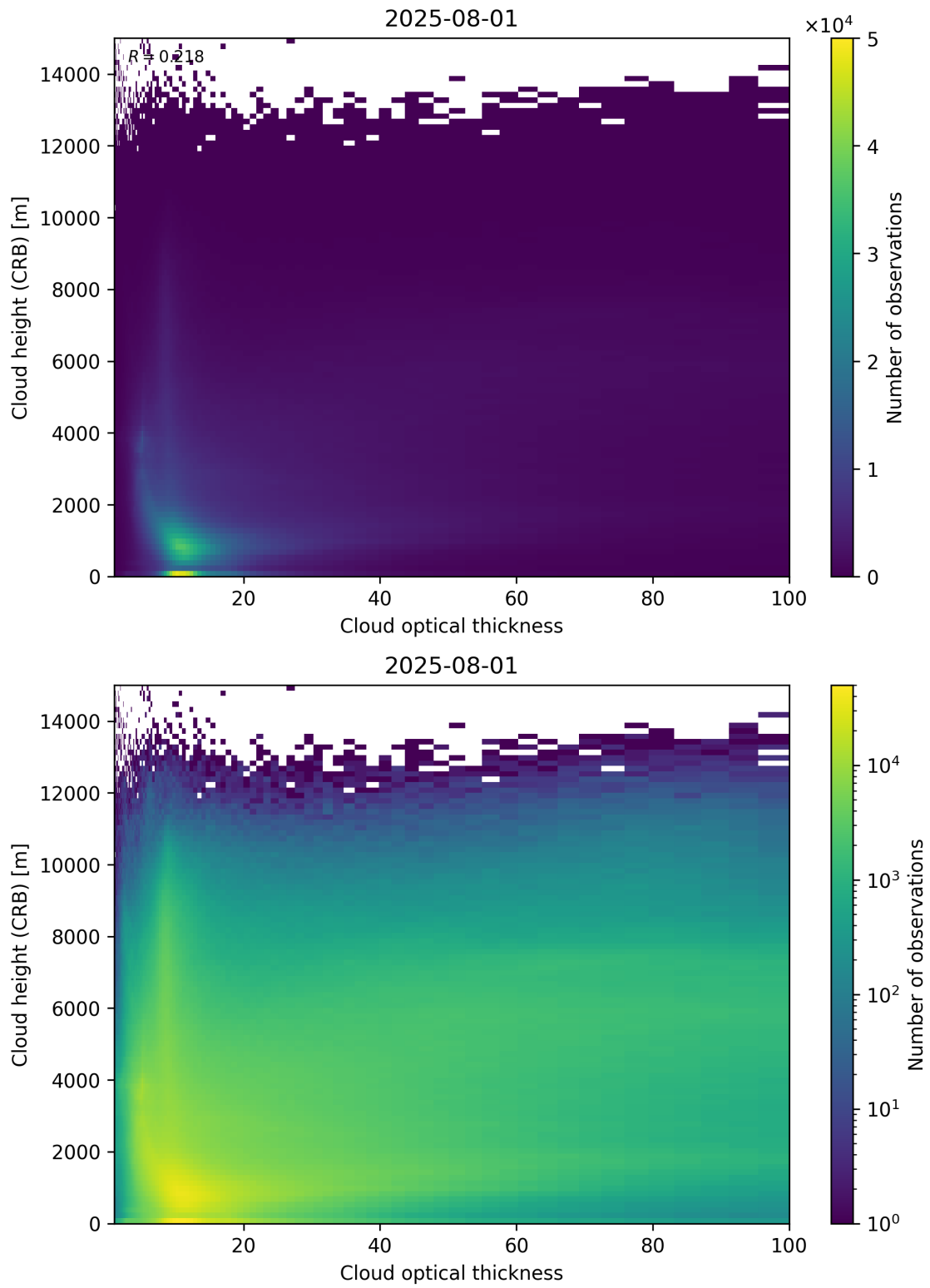
Figure 85: Scatter density plot of “Cloud optical thickness” against “Cloud height (CRB)” for 2025-07-31 to 2025-08-02.
