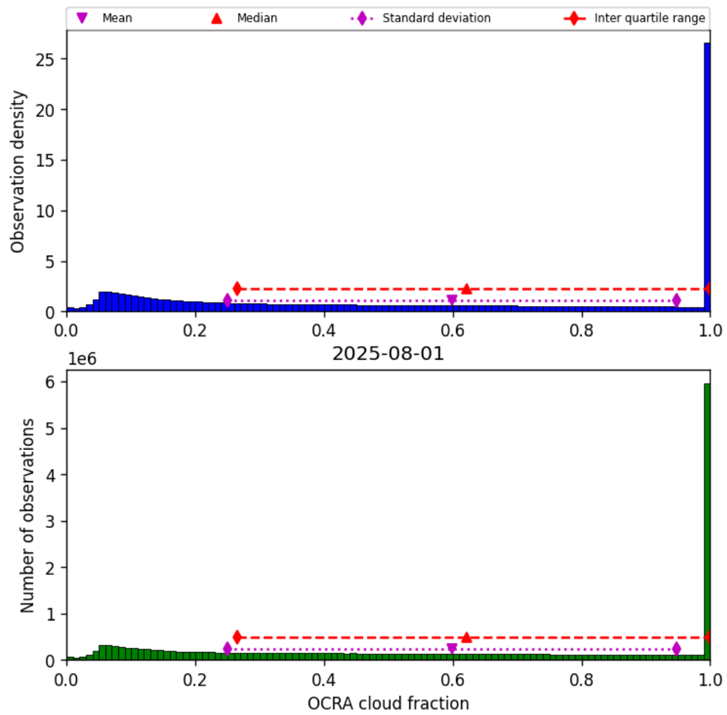
Figure 50: Histogram of “OCRA cloud fraction” for 2025-07-31 to 2025-08-02
