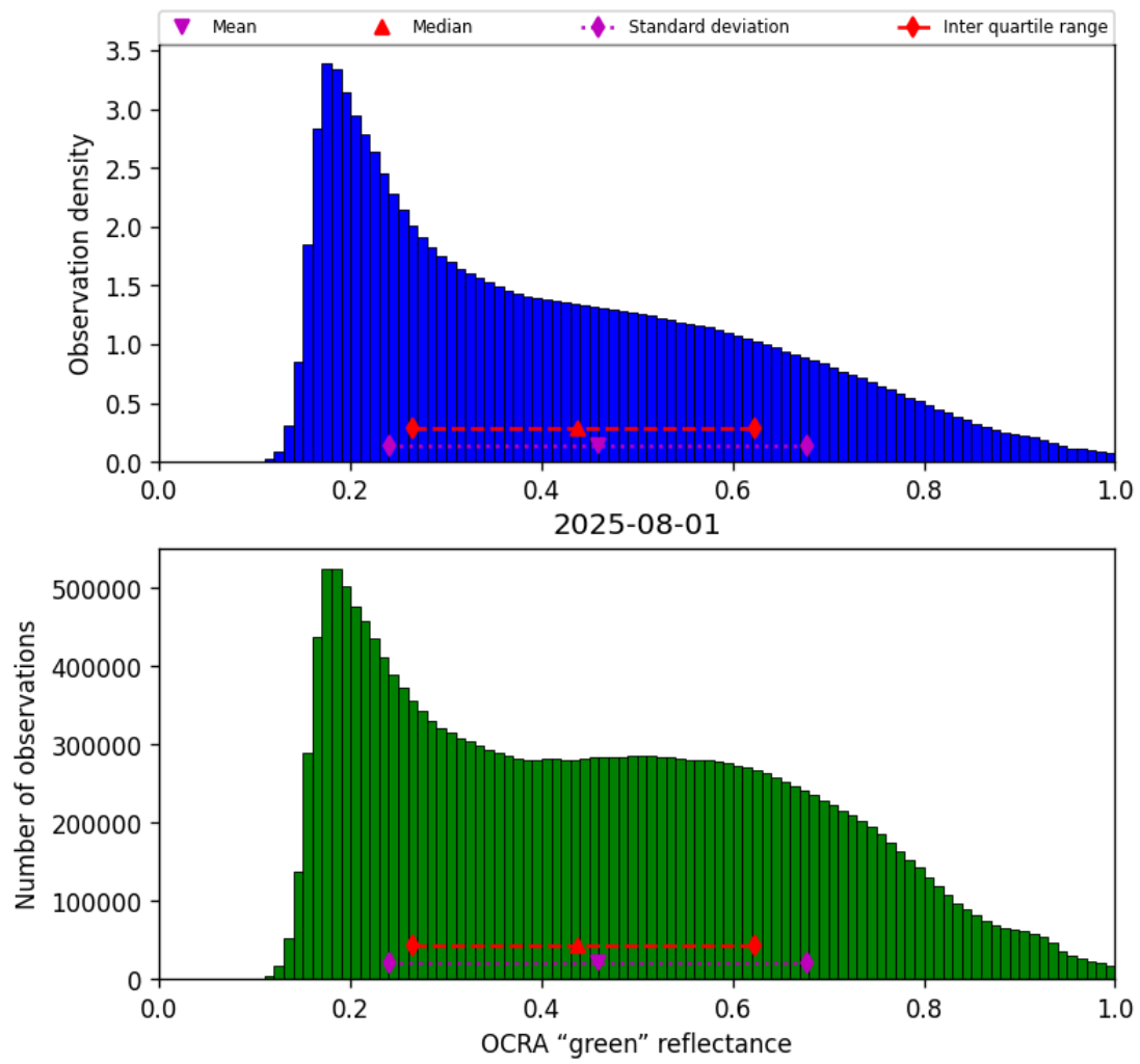
Figure 52: Histogram of “OCRA “green” reflectance” for 2025-07-31 to 2025-08-02
