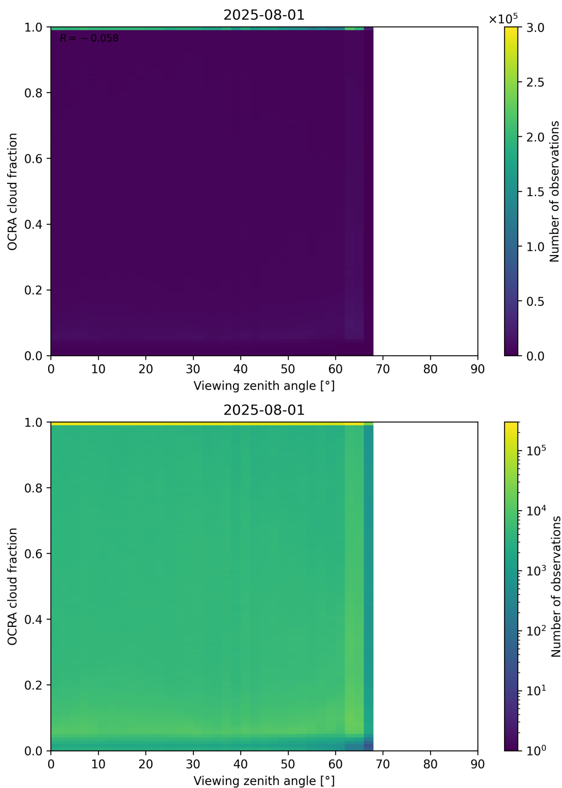
Figure 108: Scatter density plot of “Viewing zenith angle” against “OCRA cloud fraction” for 2025-07-31 to 2025-08-02.
