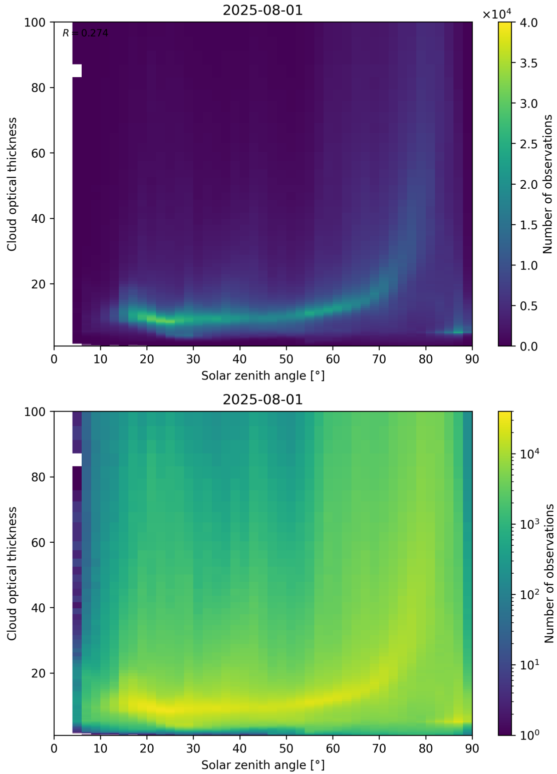
Figure 103: Scatter density plot of “Solar zenith angle” against “Cloud optical thickness” for 2025-07-31 to 2025-08-02.
