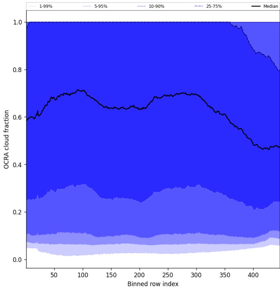
Figure 66: Along track statistics of “OCRA cloud fraction” for 2025-07-31 to 2025-08-02
