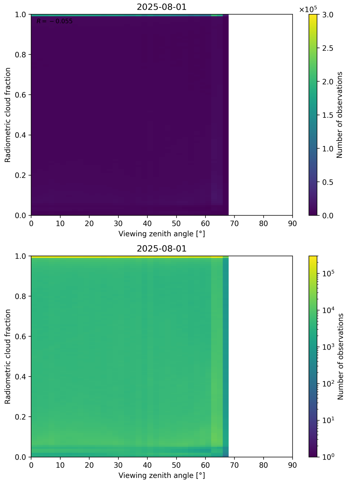
Figure 107: Scatter density plot of “Viewing zenith angle” against “Radiometric cloud fraction” for 2025-07-31 to 2025-08-02.
