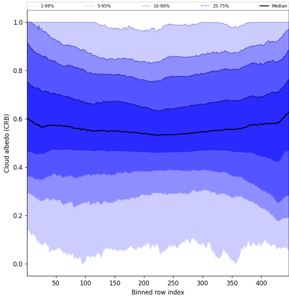
Figure 60: Along track statistics of “Cloud albedo (CRB)” for 2025-07-31 to 2025-08-02
