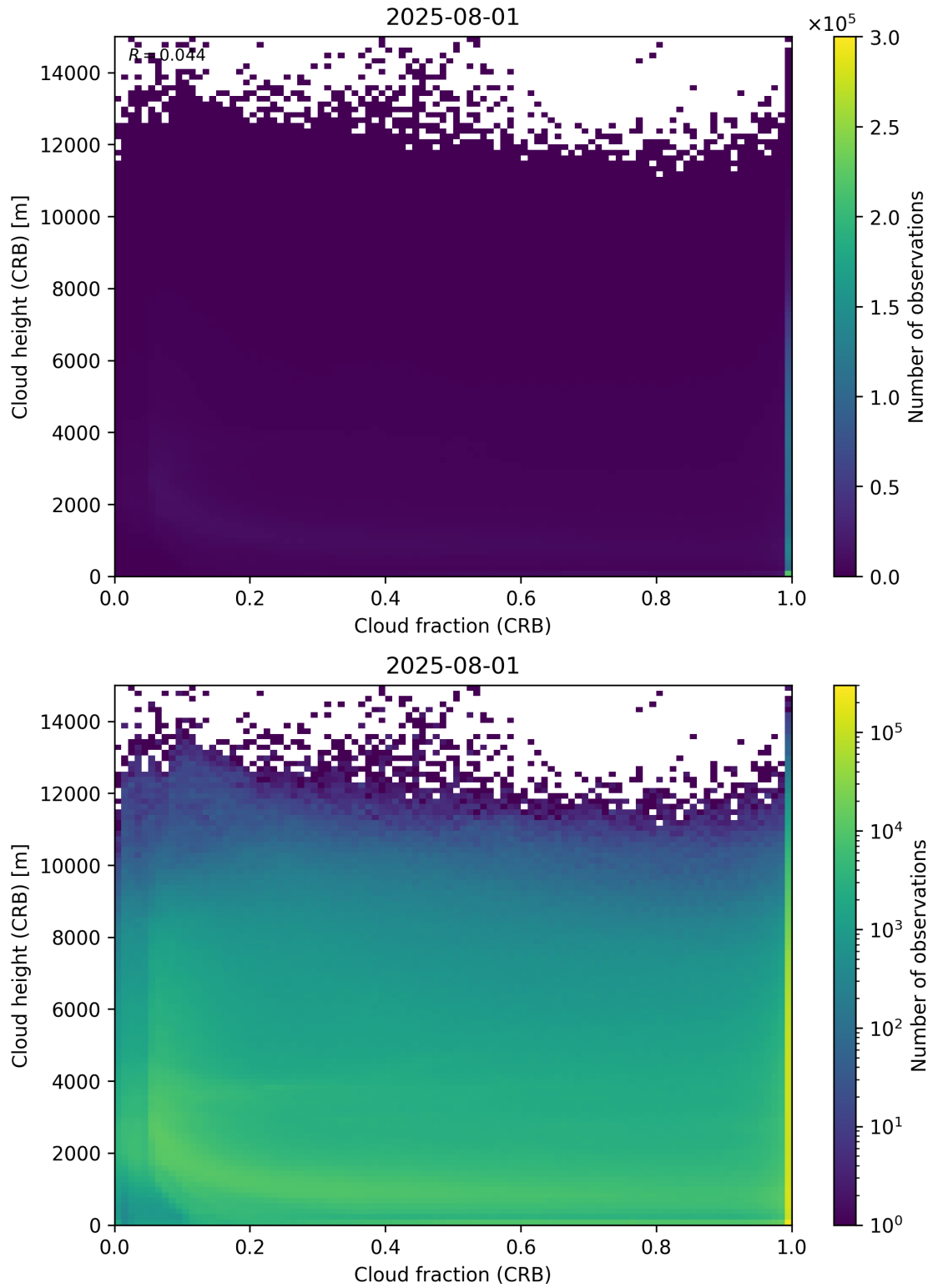
Figure 79: Scatter density plot of “Cloud fraction (CRB)” against “Cloud height (CRB)” for 2025-07-31 to 2025-08-02.
