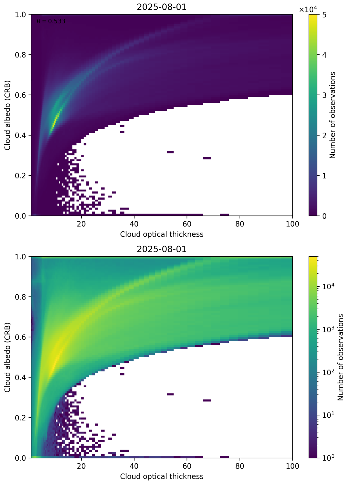
Figure 82: Scatter density plot of “Cloud optical thickness” against “Cloud albedo (CRB)” for 2025-07-31 to 2025-08-02.
