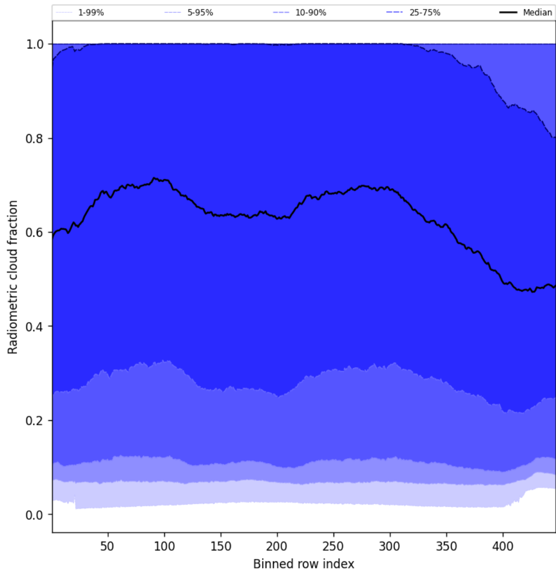
Figure 55: Along track statistics of “Radiometric cloud fraction” for 2025-07-31 to 2025-08-02
