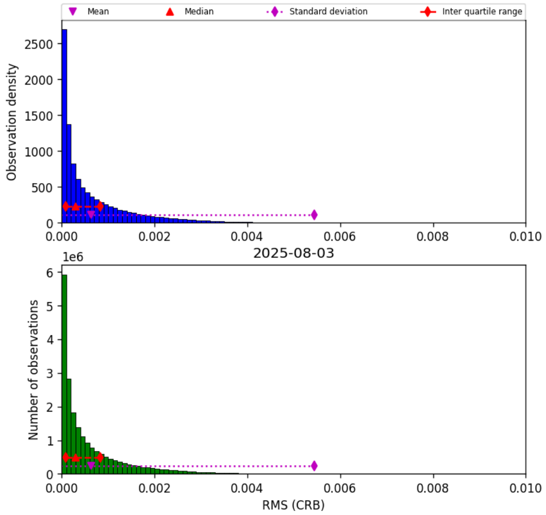
Figure 48: Histogram of “RMS (CRB)” for 2025-08-03 to 2025-08-04
