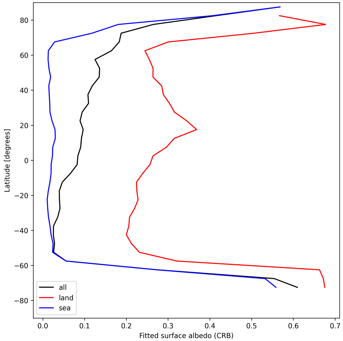
Figure 30: Zonal average of “Fitted surface albedo (CRB)” for 2025-08-03 to 2025-08-04.
