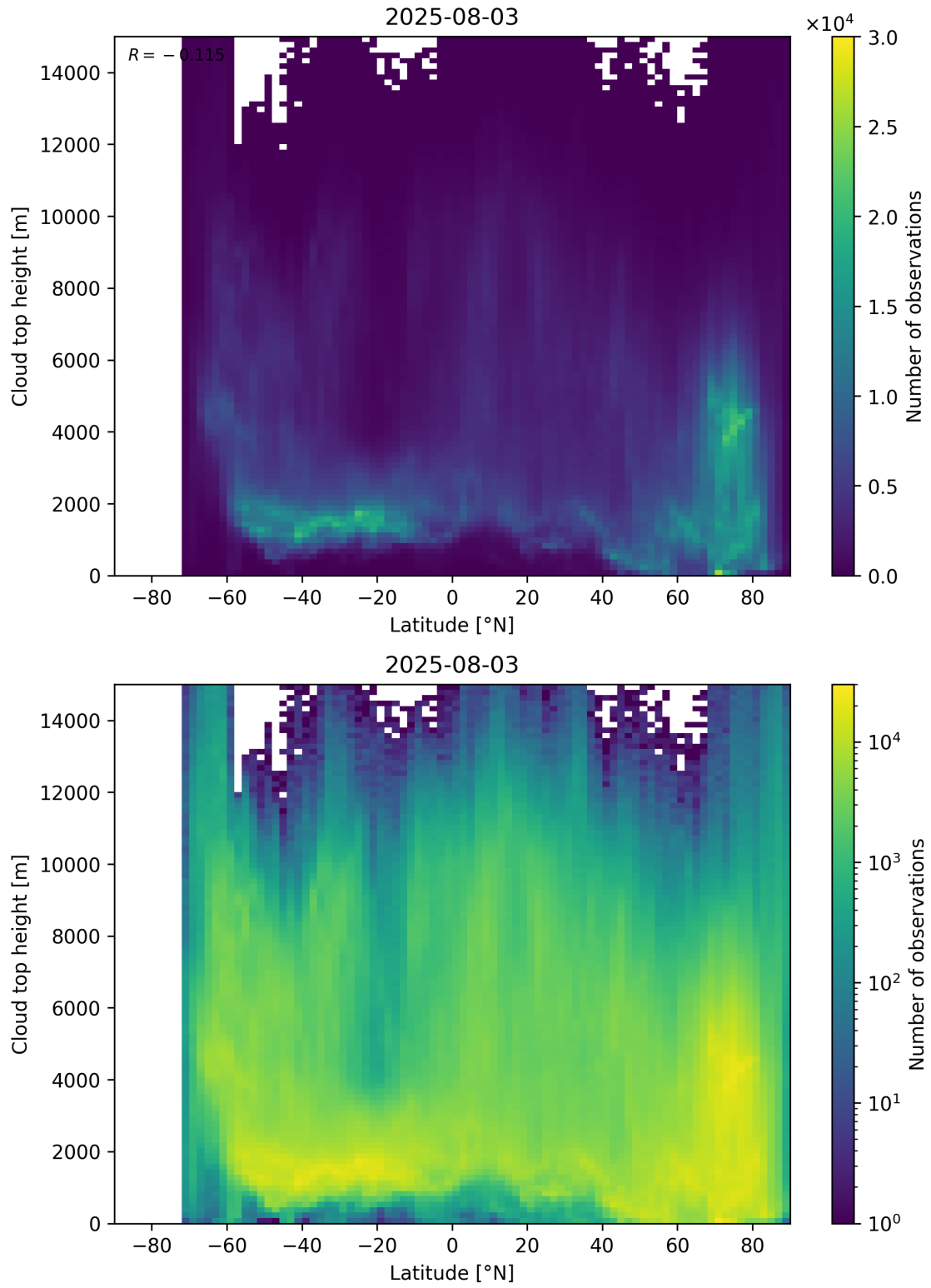
Figure 97: Scatter density plot of “Latitude” against “Cloud top height” for 2025-08-03 to 2025-08-04.
