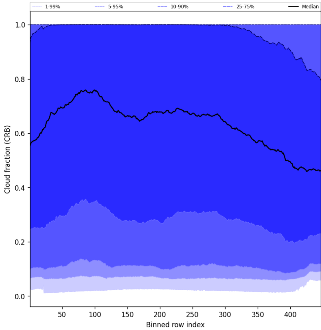
Figure 58: Along track statistics of “Cloud fraction (CRB)” for 2025-08-03 to 2025-08-04
