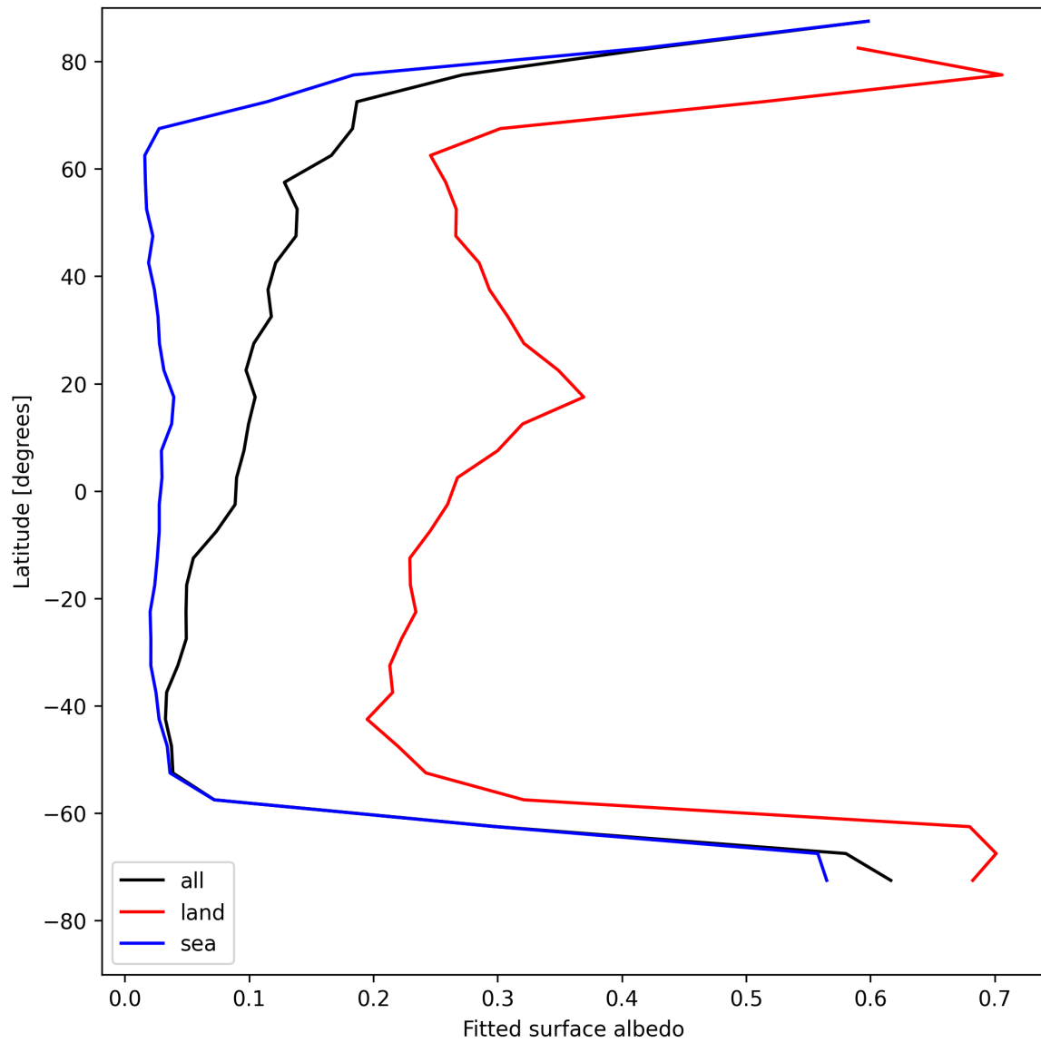
Figure 29: Zonal average of “Fitted surface albedo” for 2025-08-03 to 2025-08-04.
