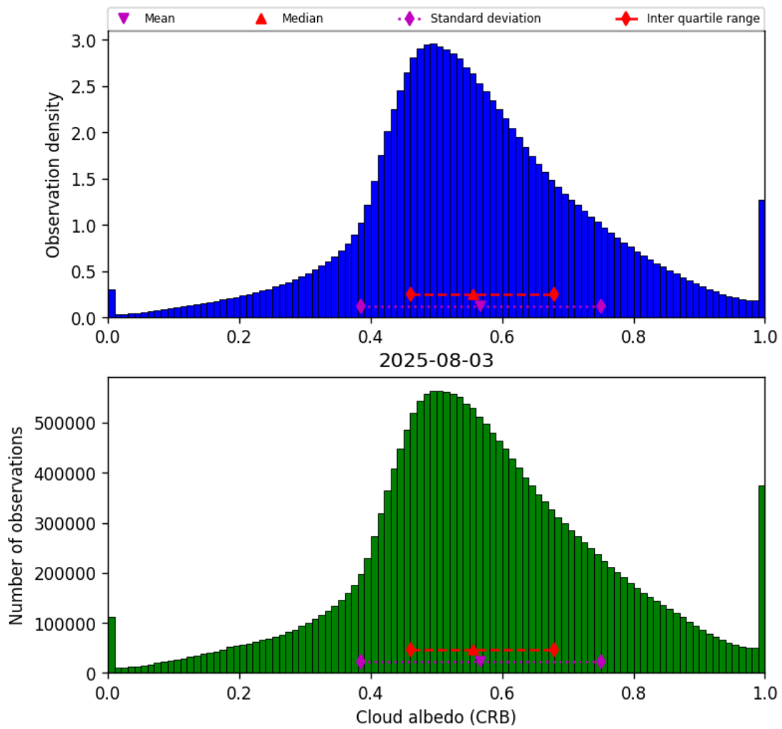
Figure 44: Histogram of “Cloud albedo (CRB)” for 2025-08-03 to 2025-08-04
