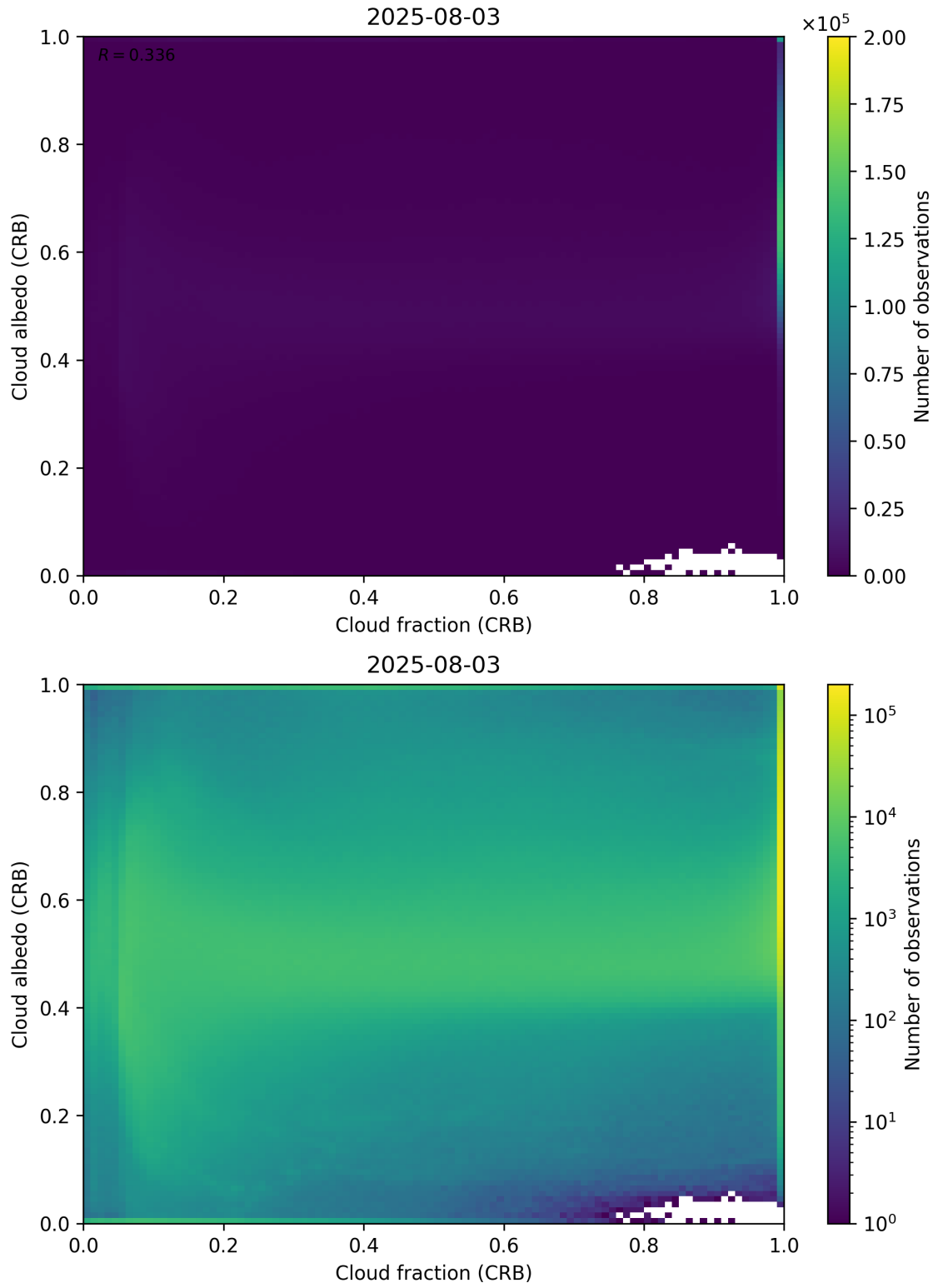
Figure 77: Scatter density plot of “Cloud fraction (CRB)” against “Cloud albedo (CRB)” for 2025-08-03 to 2025-08-04.
