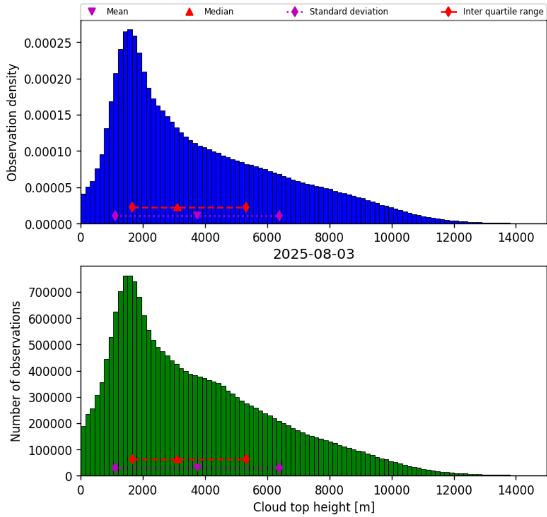
Figure 40: Histogram of “Cloud top height” for 2025-08-03 to 2025-08-04
