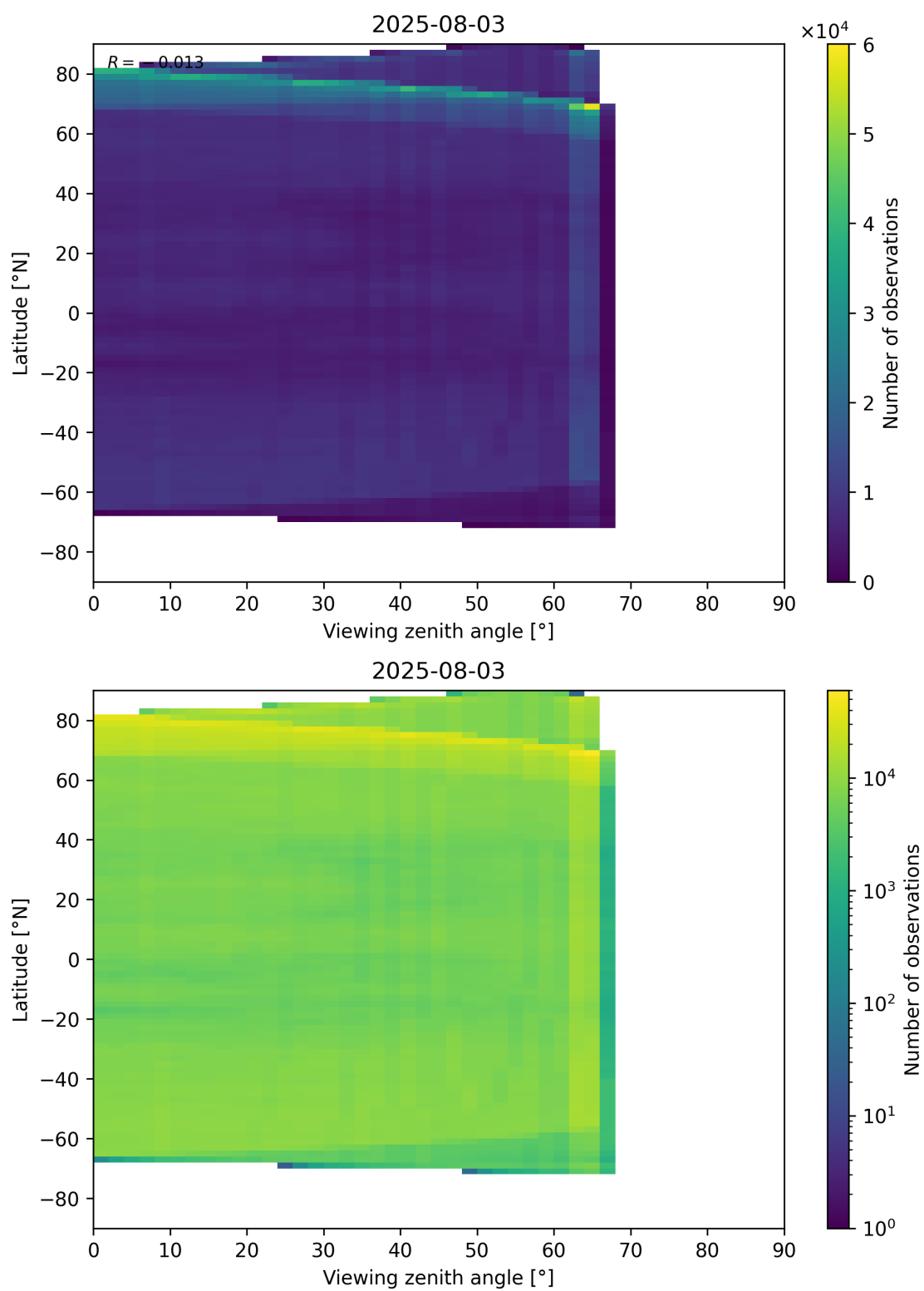
Figure 113: Scatter density plot of “Viewing zenith angle” against “Latitude” for 2025-08-03 to 2025-08-04.
