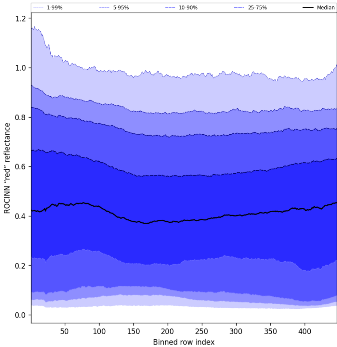
Figure 69: Along track statistics of “ROCINN “red” reflectance” for 2025-08-03 to 2025-08-04
