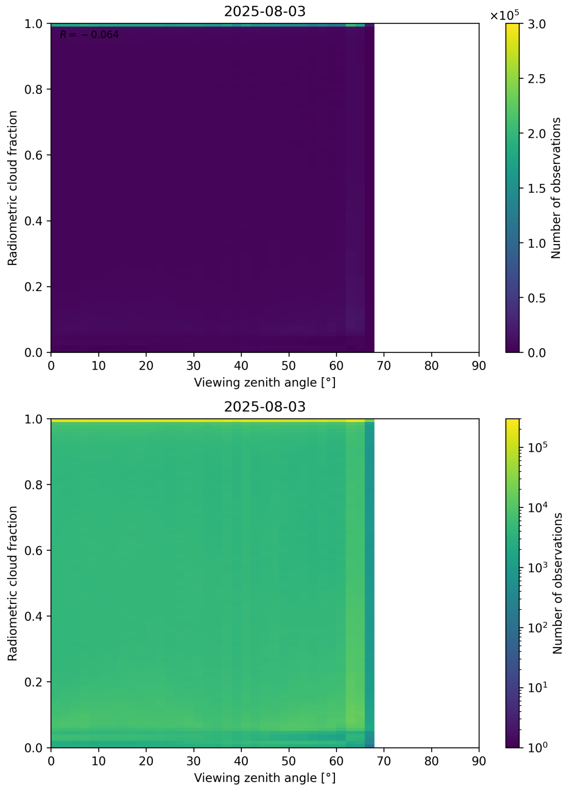
Figure 107: Scatter density plot of “Viewing zenith angle” against “Radiometric cloud fraction” for 2025-08-03 to 2025-08-04.
