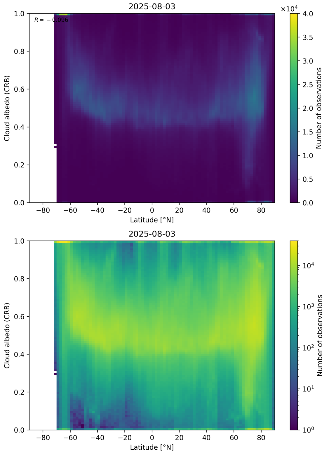
Figure 91: Scatter density plot of “Latitude” against “Cloud albedo (CRB)” for 2025-08-03 to 2025-08-04.
