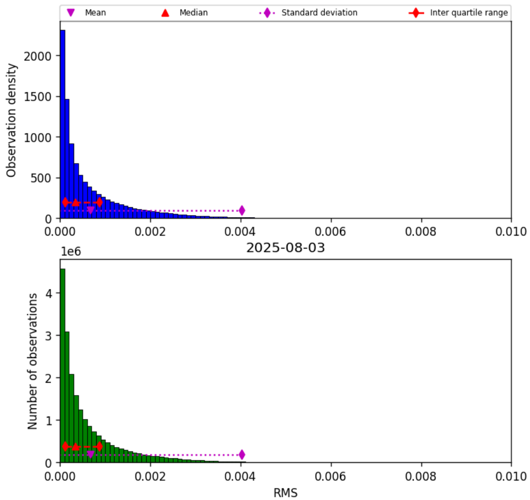
Figure 47: Histogram of “RMS” for 2025-08-03 to 2025-08-04
