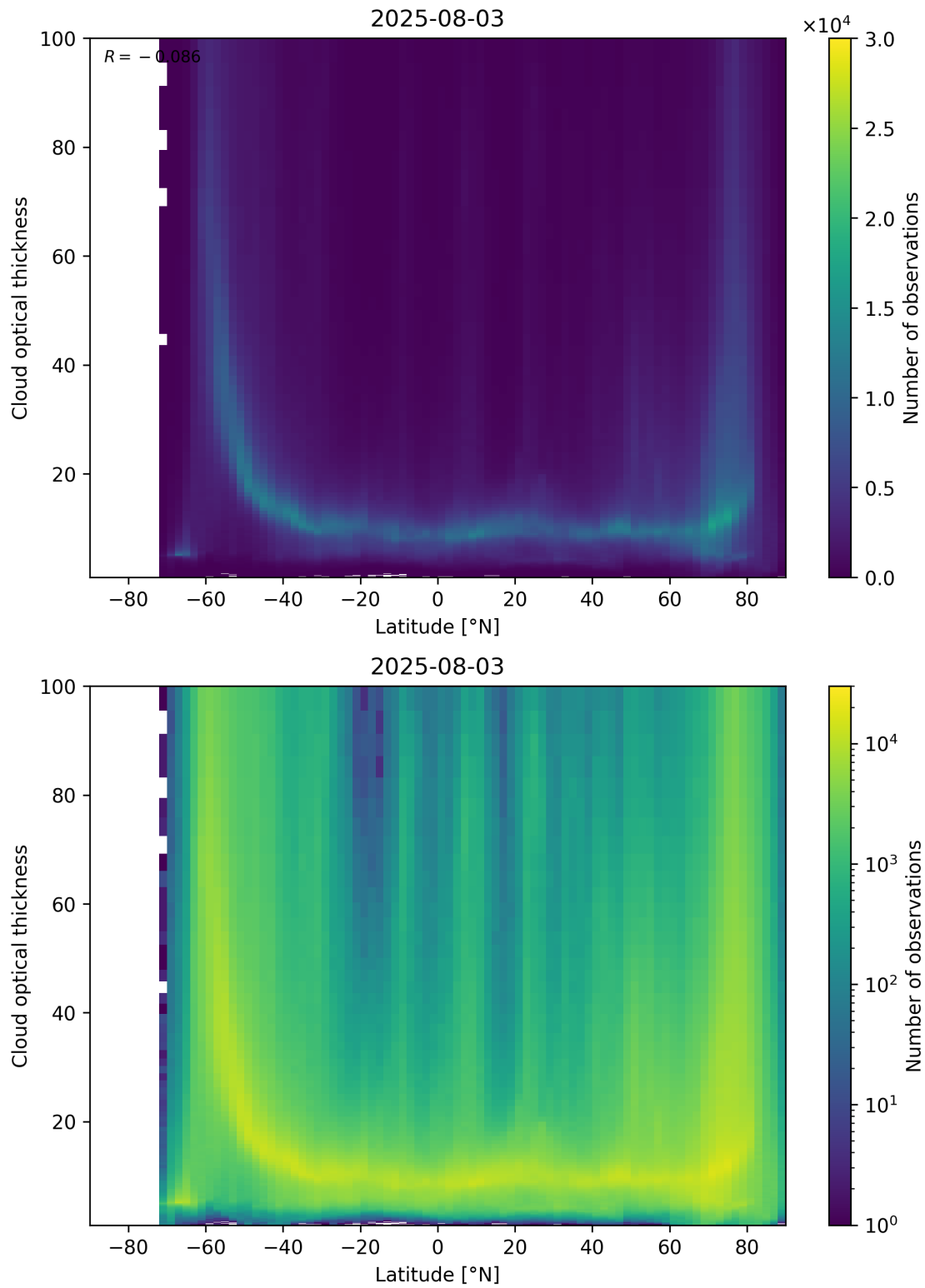
Figure 96: Scatter density plot of “Latitude” against “Cloud optical thickness” for 2025-08-03 to 2025-08-04.
