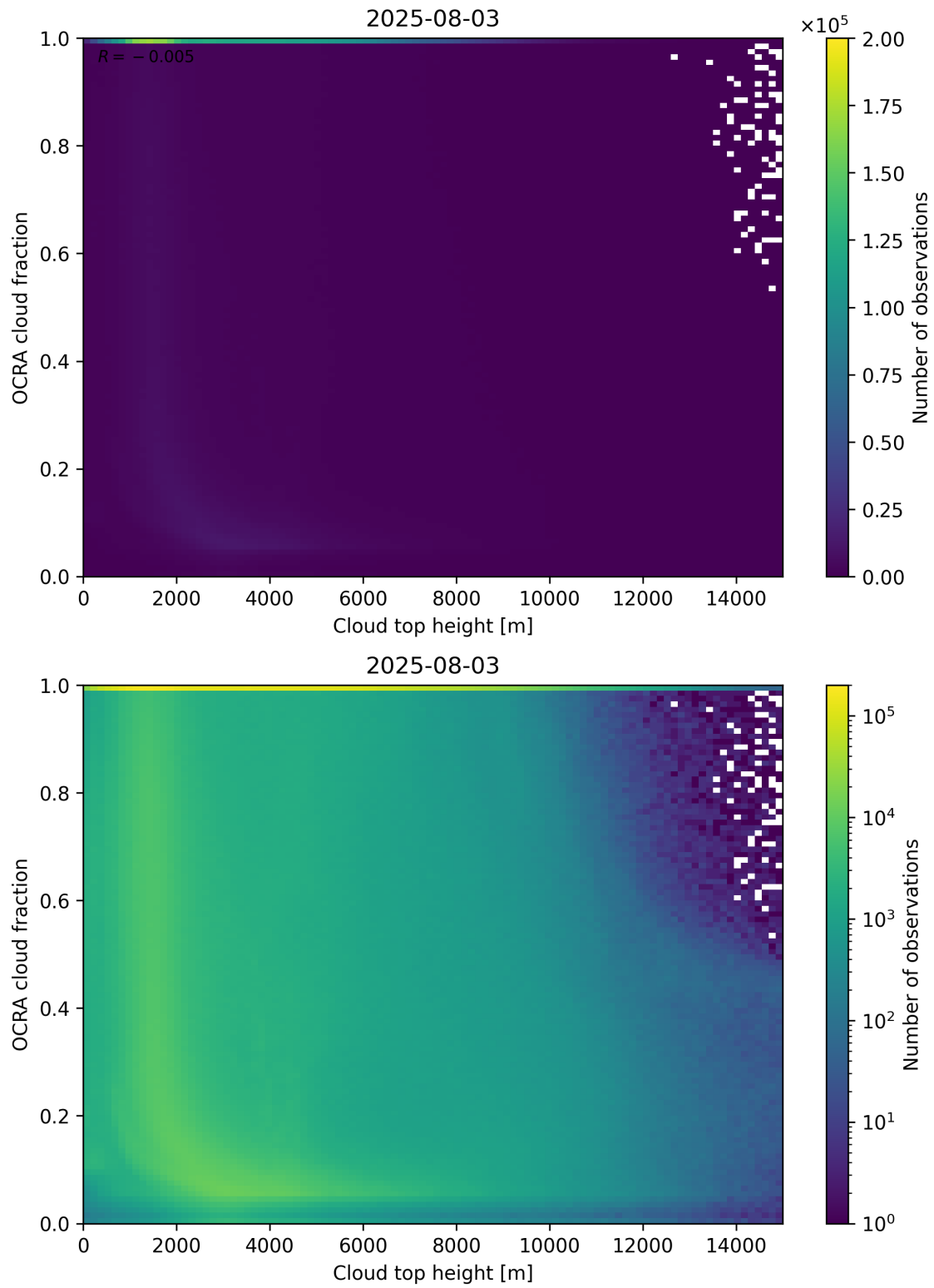
Figure 87: Scatter density plot of “Cloud top height” against “OCRA cloud fraction” for 2025-08-03 to 2025-08-04.
