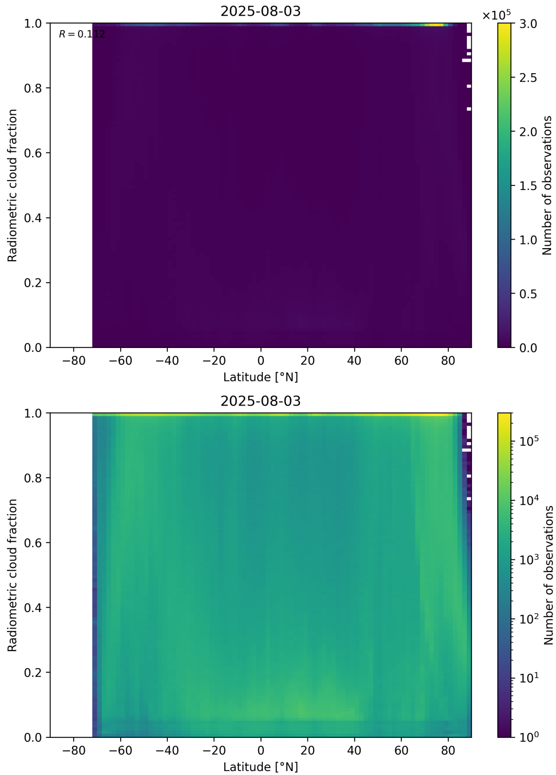
Figure 92: Scatter density plot of “Latitude” against “Radiometric cloud fraction” for 2025-08-03 to 2025-08-04.
