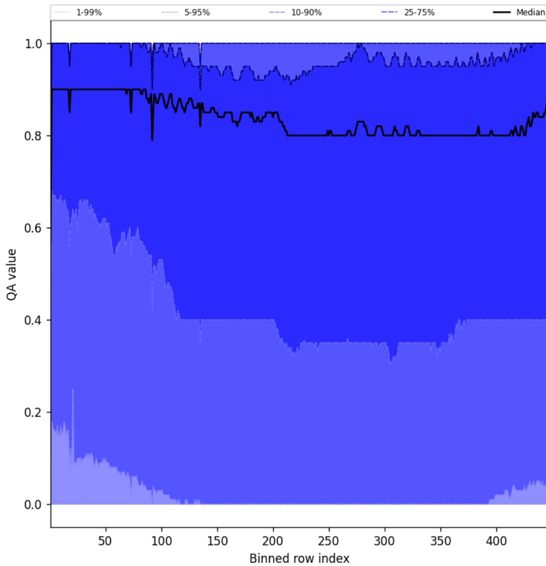
Figure 54: Along track statistics of “QA value” for 2025-08-03 to 2025-08-04
