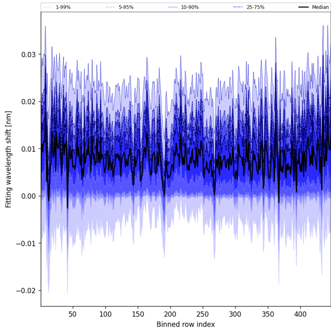
Figure 65: Along track statistics of “Fitting wavelength shift” for 2025-08-03 to 2025-08-04
