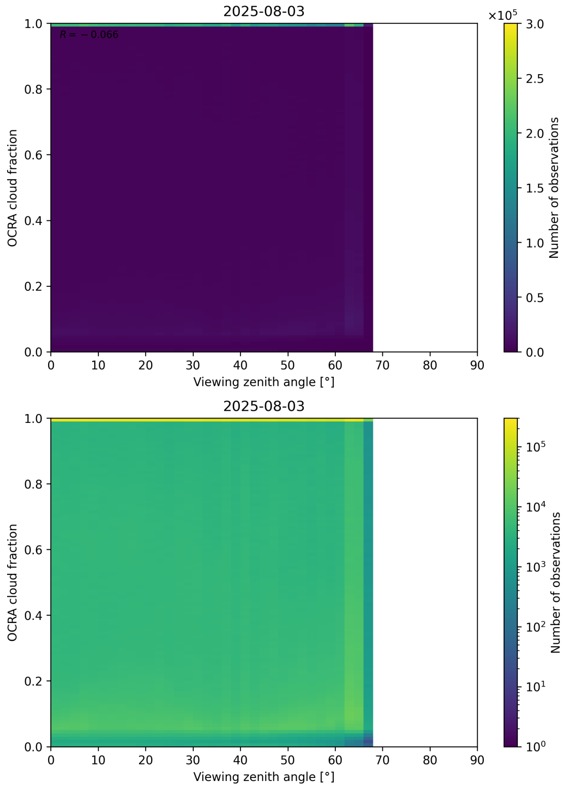
Figure 108: Scatter density plot of “Viewing zenith angle” against “OCRA cloud fraction” for 2025-08-03 to 2025-08-04.
