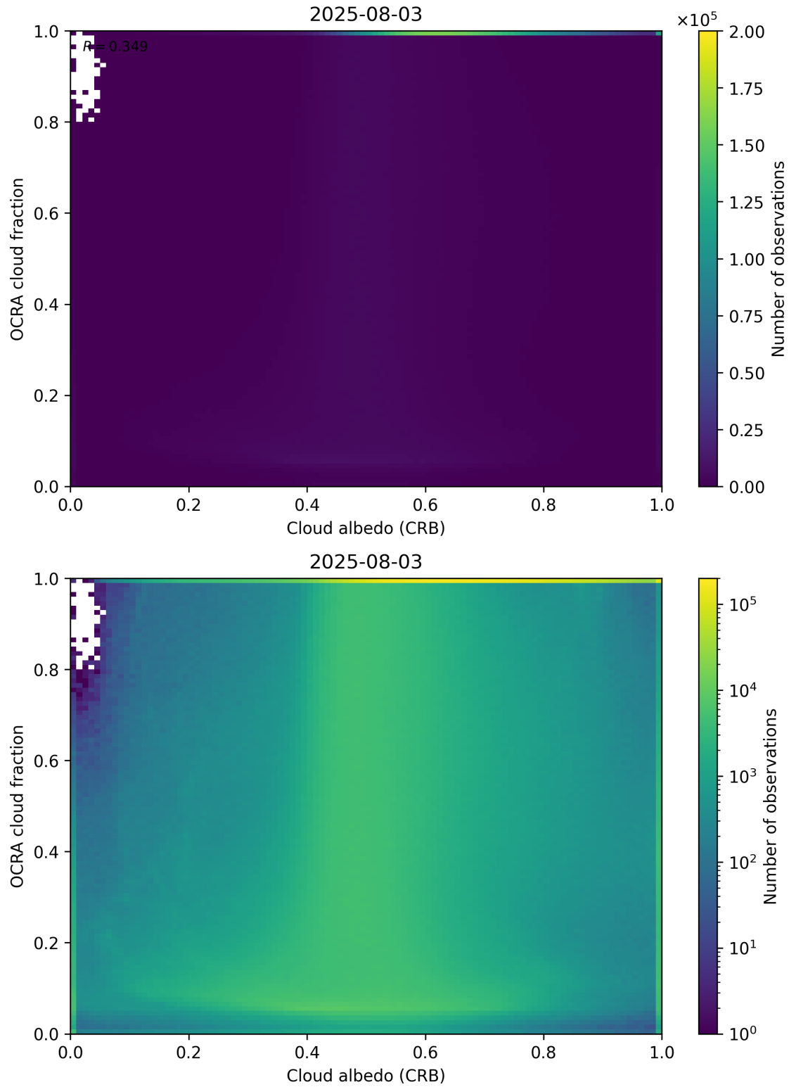
Figure 70: Scatter density plot of “Cloud albedo (CRB)” against “OCRA cloud fraction” for 2025-08-03 to 2025-08-04.
