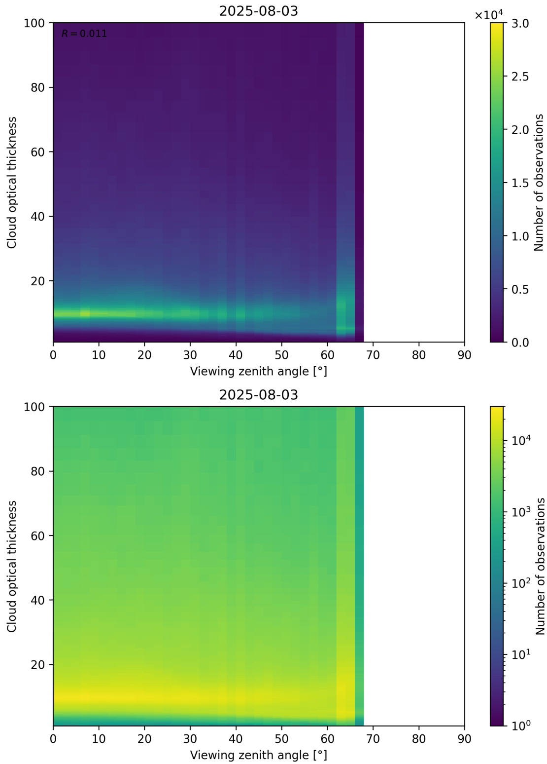
Figure 111: Scatter density plot of “Viewing zenith angle” against “Cloud optical thickness” for 2025-08-03 to 2025-08-04.
