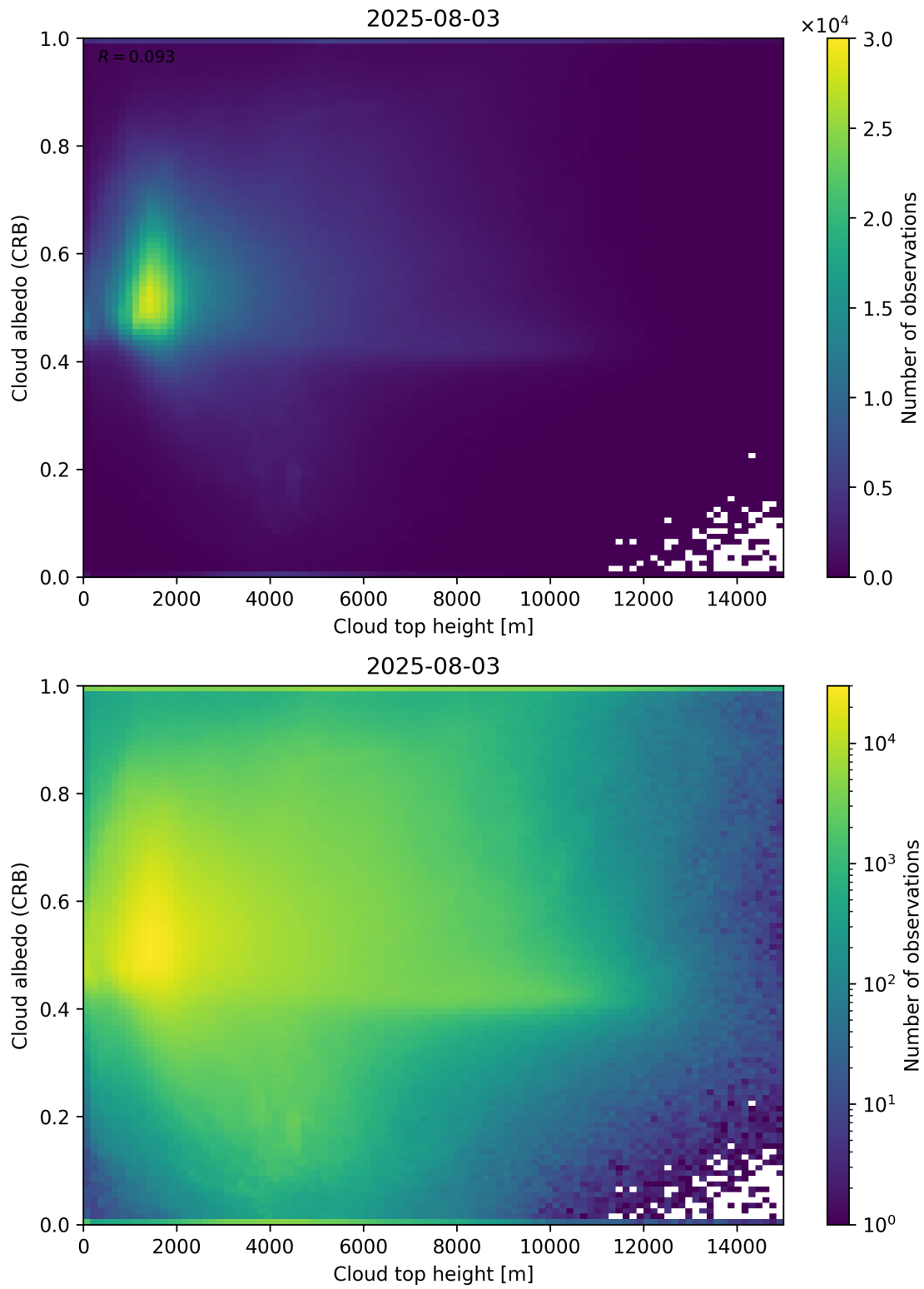
Figure 86: Scatter density plot of “Cloud top height” against “Cloud albedo (CRB)” for 2025-08-03 to 2025-08-04.
