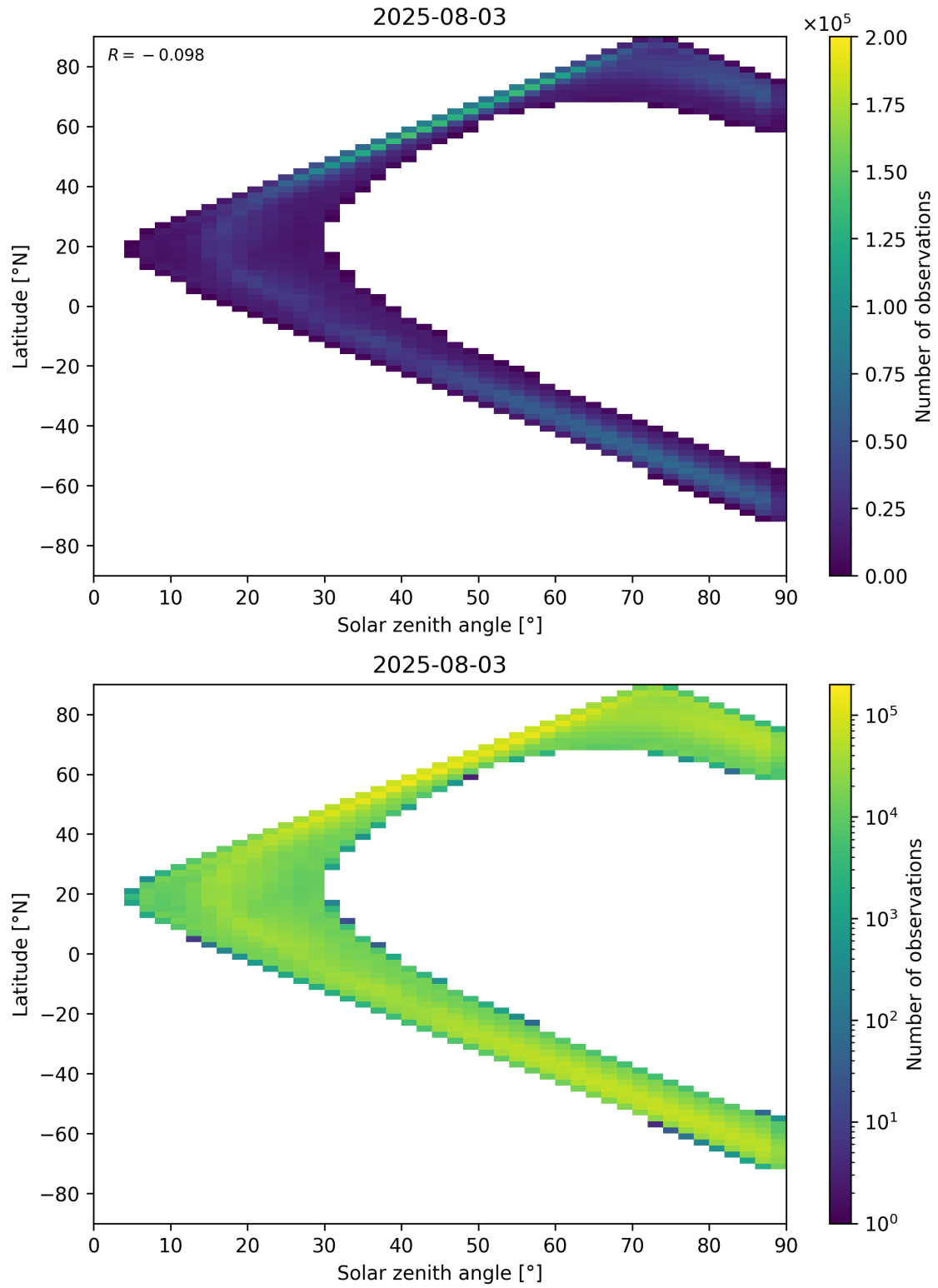
Figure 105: Scatter density plot of “Solar zenith angle” against “Latitude” for 2025-08-03 to 2025-08-04.
