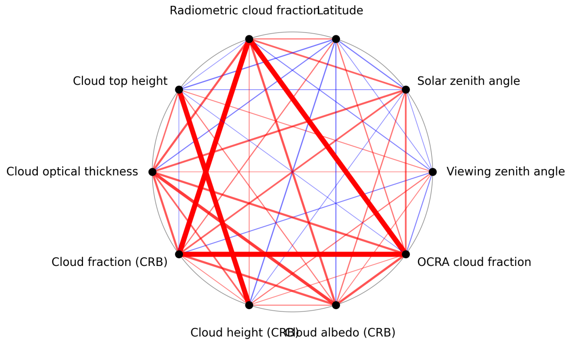
Figure 1: Map of correlation graph for 2025-08-03 to 2025-08-04.
