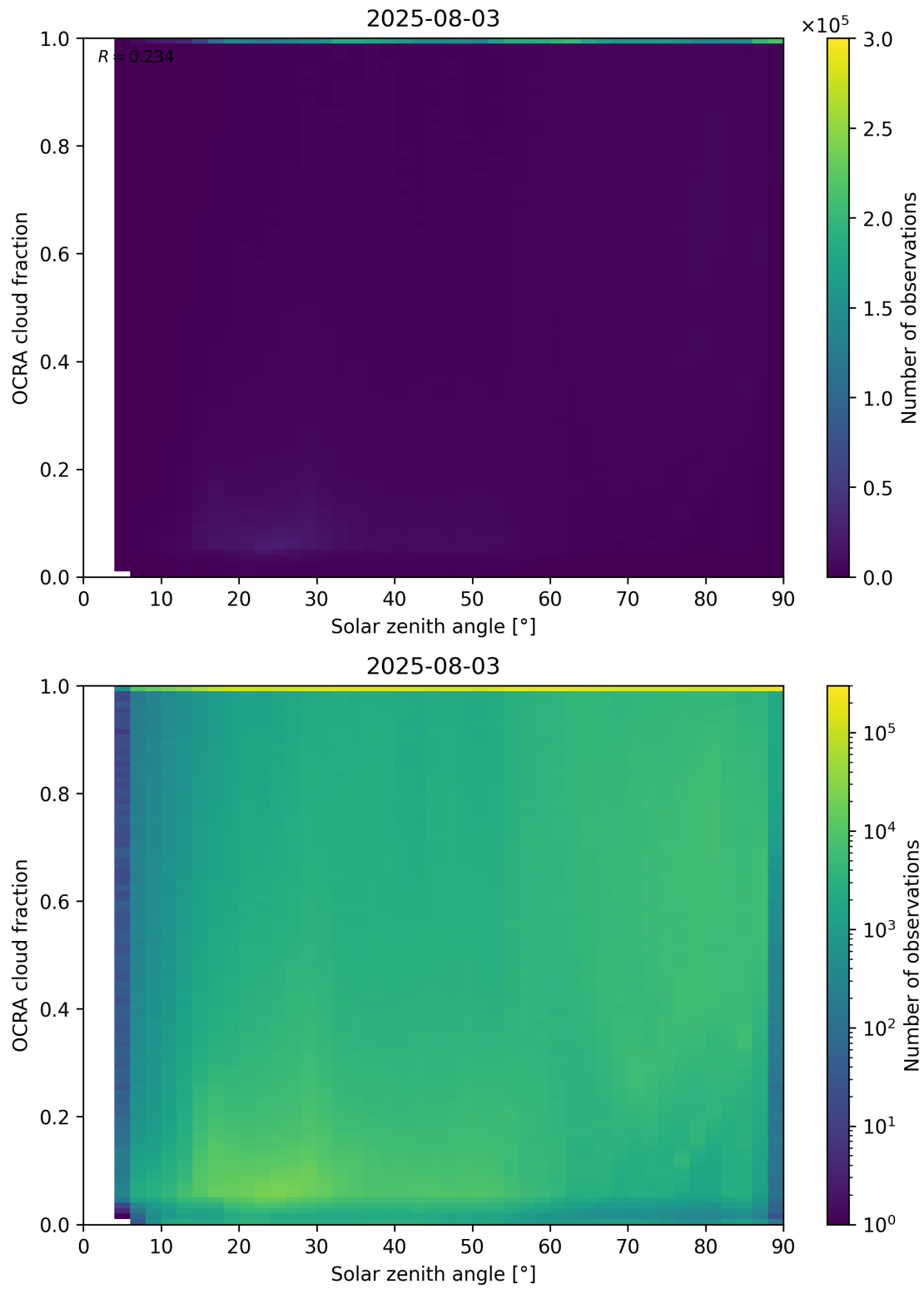
Figure 100: Scatter density plot of “Solar zenith angle” against “OCRA cloud fraction” for 2025-08-03 to 2025-08-04.
