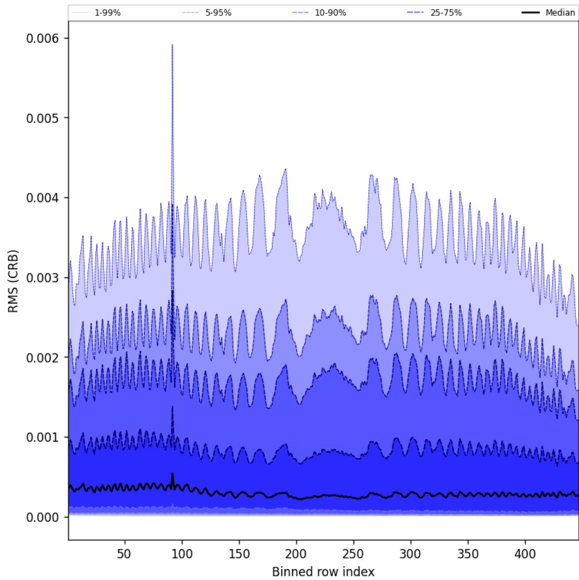
Figure 64: Along track statistics of “RMS (CRB)” for 2025-08-03 to 2025-08-04
