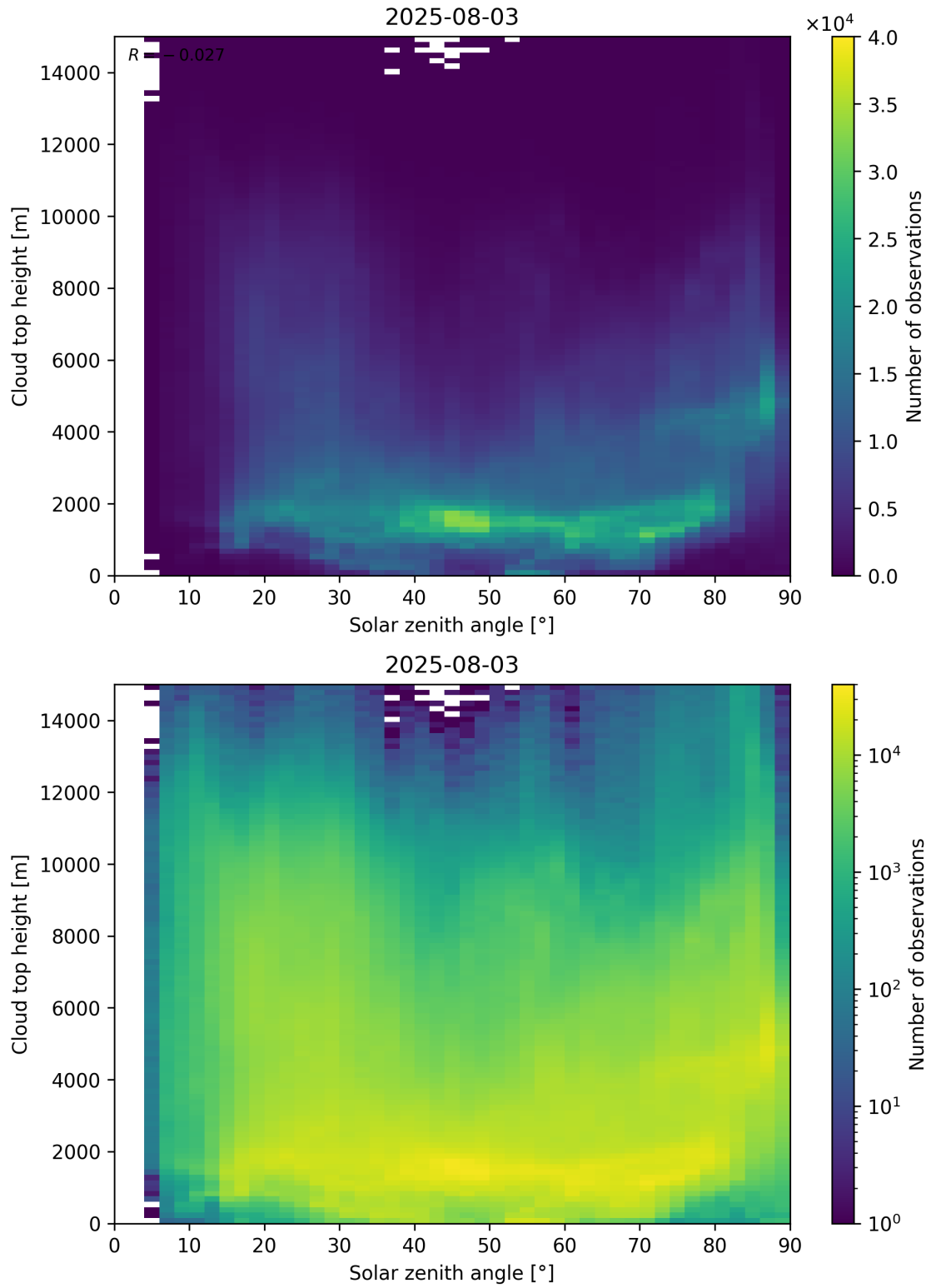
Figure 104: Scatter density plot of “Solar zenith angle” against “Cloud top height” for 2025-08-03 to 2025-08-04.
