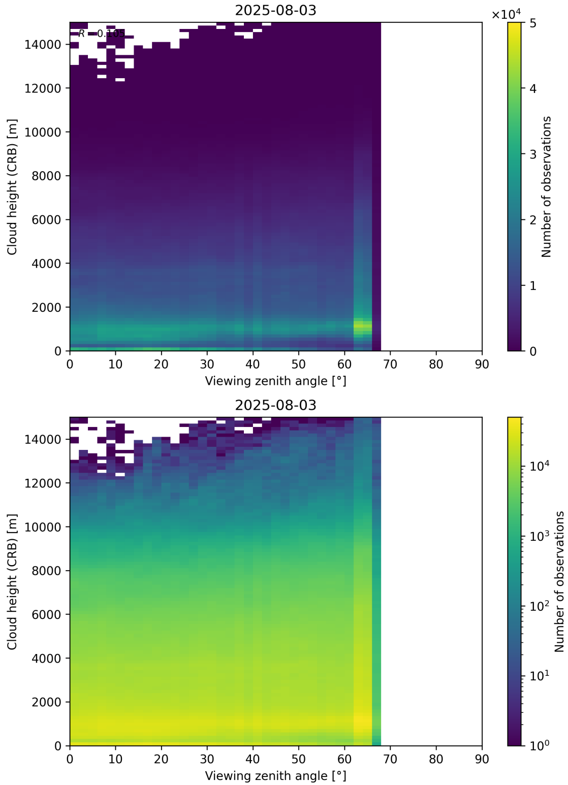
Figure 110: Scatter density plot of “Viewing zenith angle” against “Cloud height (CRB)” for 2025-08-03 to 2025-08-04.
