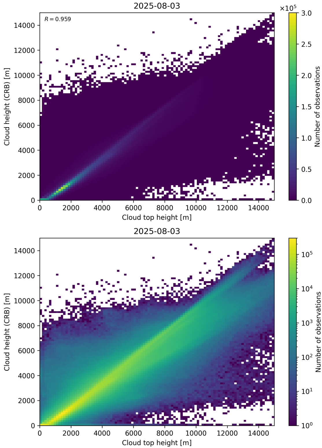
Figure 89: Scatter density plot of “Cloud top height” against “Cloud height (CRB)” for 2025-08-03 to 2025-08-04.
