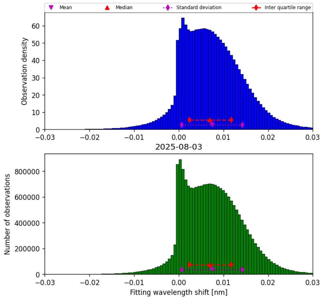
Figure 49: Histogram of “Fitting wavelength shift” for 2025-08-03 to 2025-08-04
