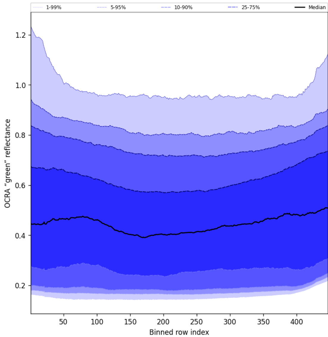
Figure 68: Along track statistics of "OCRA "green" reflectance" for 2025-08-03 to 2025-08-04
