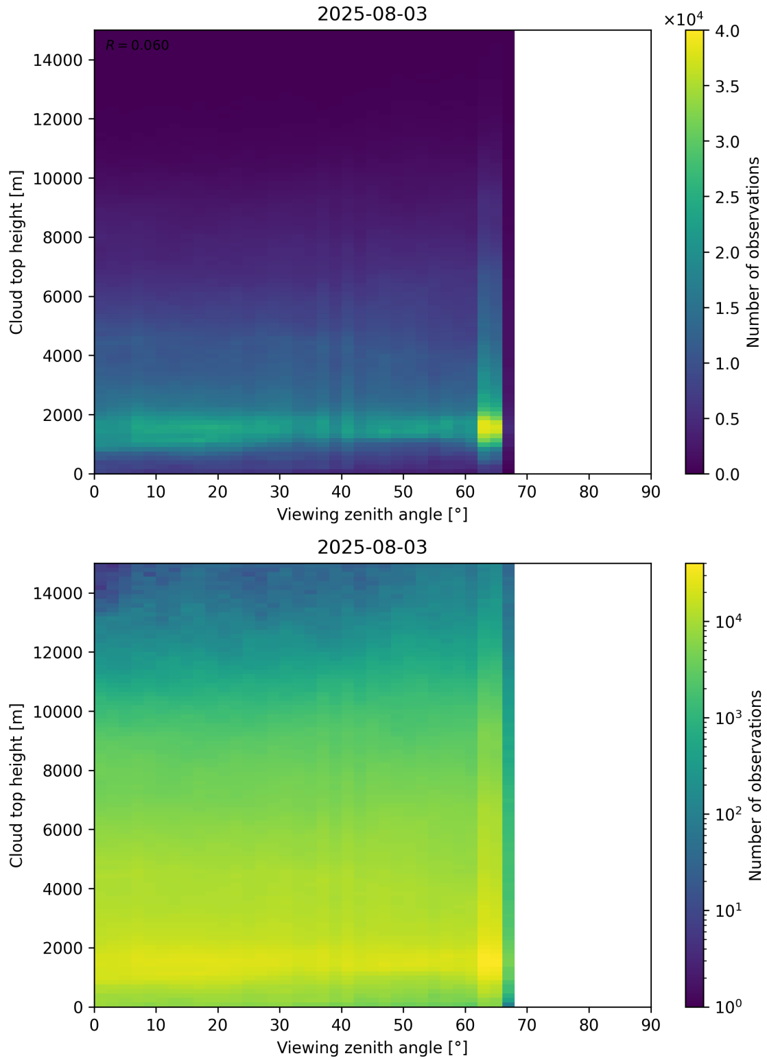
Figure 112: Scatter density plot of “Viewing zenith angle” against “Cloud top height” for 2025-08-03 to 2025-08-04.
