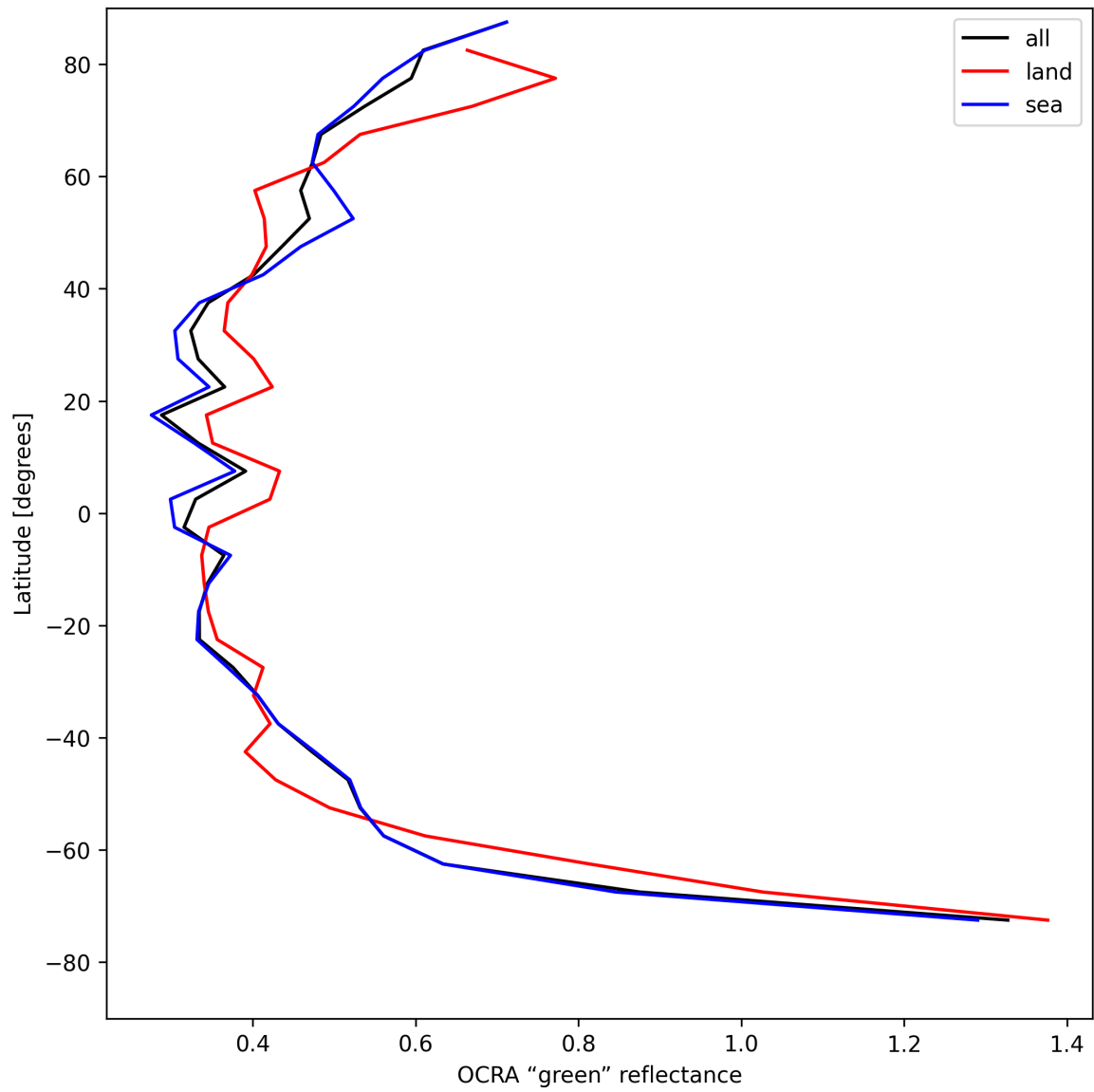
Figure 36: Zonal average of “OCRA “green” reflectance” for 2025-08-03 to 2025-08-04.
