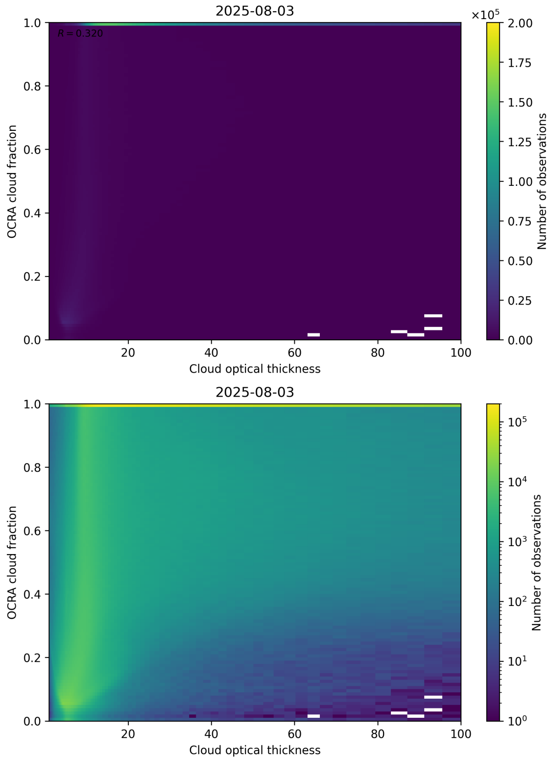
Figure 83: Scatter density plot of “Cloud optical thickness” against “OCRA cloud fraction” for 2025-08-03 to 2025-08-04.
