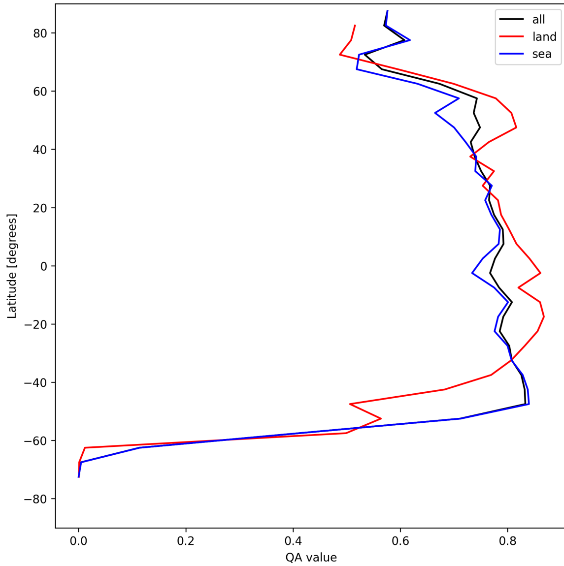
Figure 22: Zonal average of “QA value” for 2025-08-03 to 2025-08-04.
