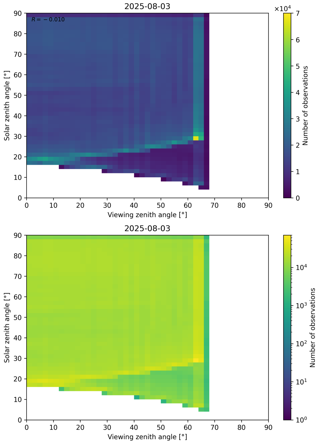
Figure 114: Scatter density plot of “Viewing zenith angle” against “Solar zenith angle” for 2025-08-03 to 2025-08-04.
