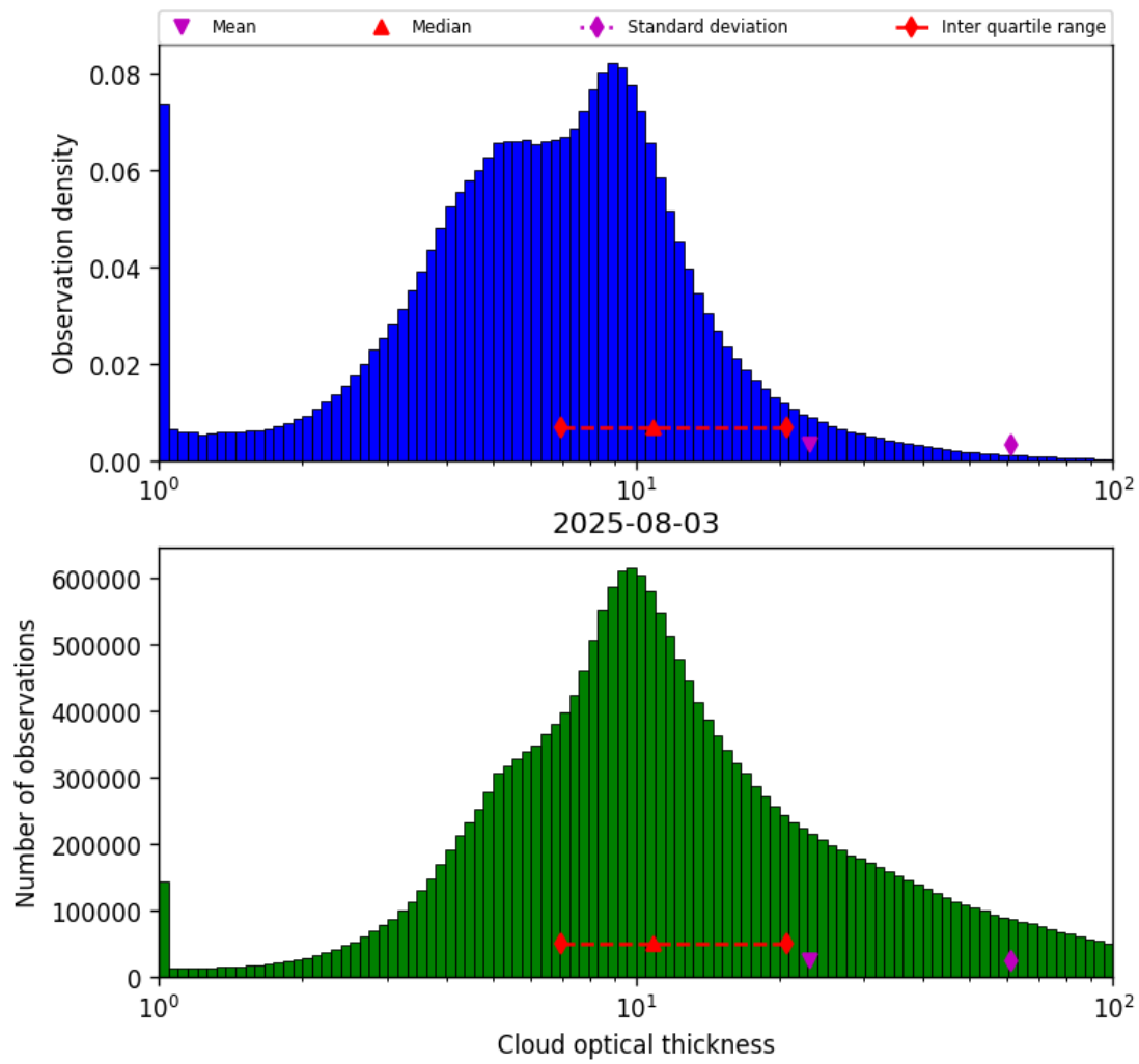
Figure 41: Histogram of “Cloud optical thickness” for 2025-08-03 to 2025-08-04
