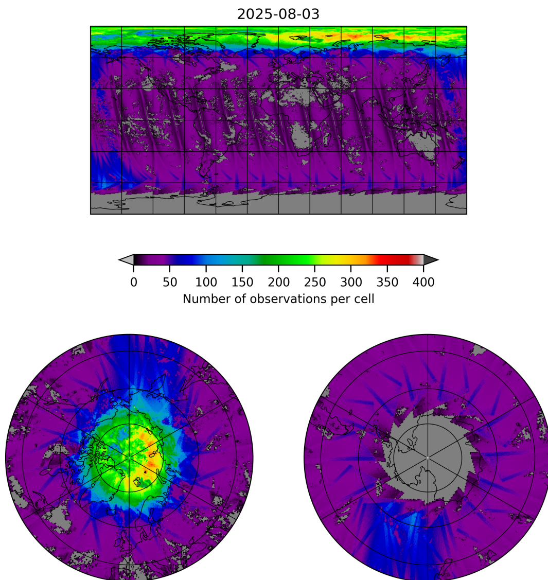
Figure 21: Map of the number of observations for 2025-08-03 to 2025-08-04
