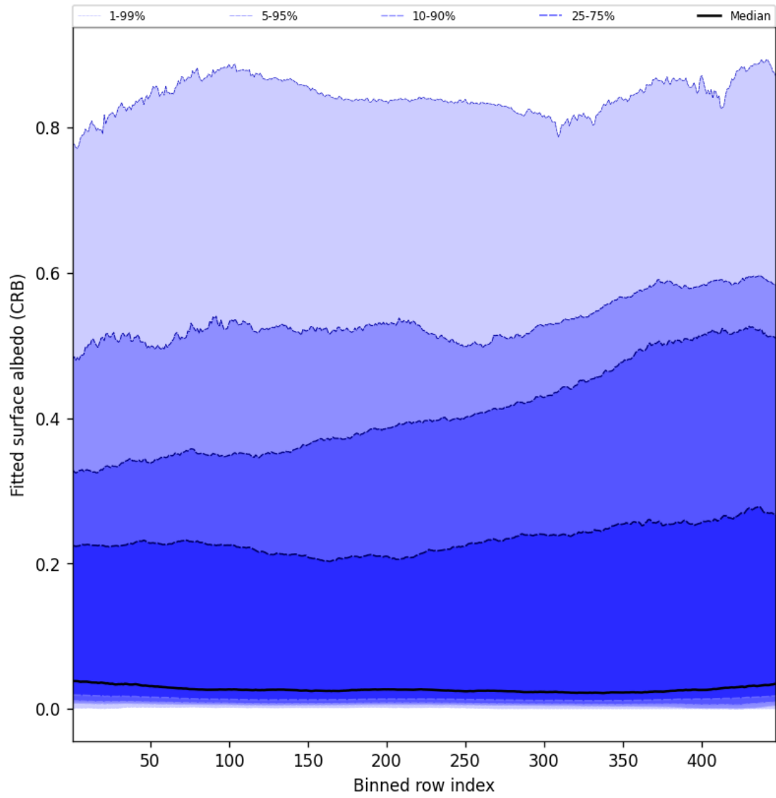
Figure 62: Along track statistics of “Fitted surface albedo (CRB)” for 2025-08-03 to 2025-08-04
