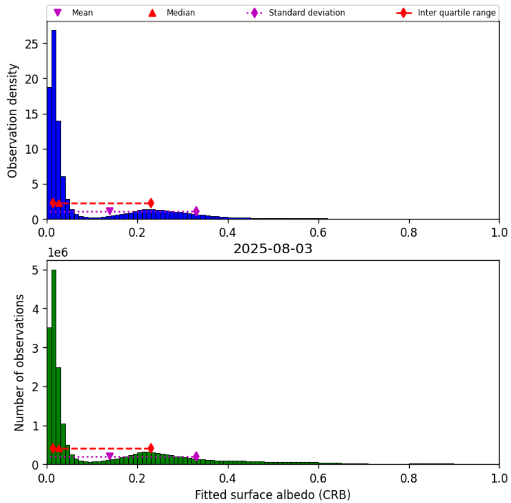
Figure 46: Histogram of “Fitted surface albedo (CRB)” for 2025-08-03 to 2025-08-04
