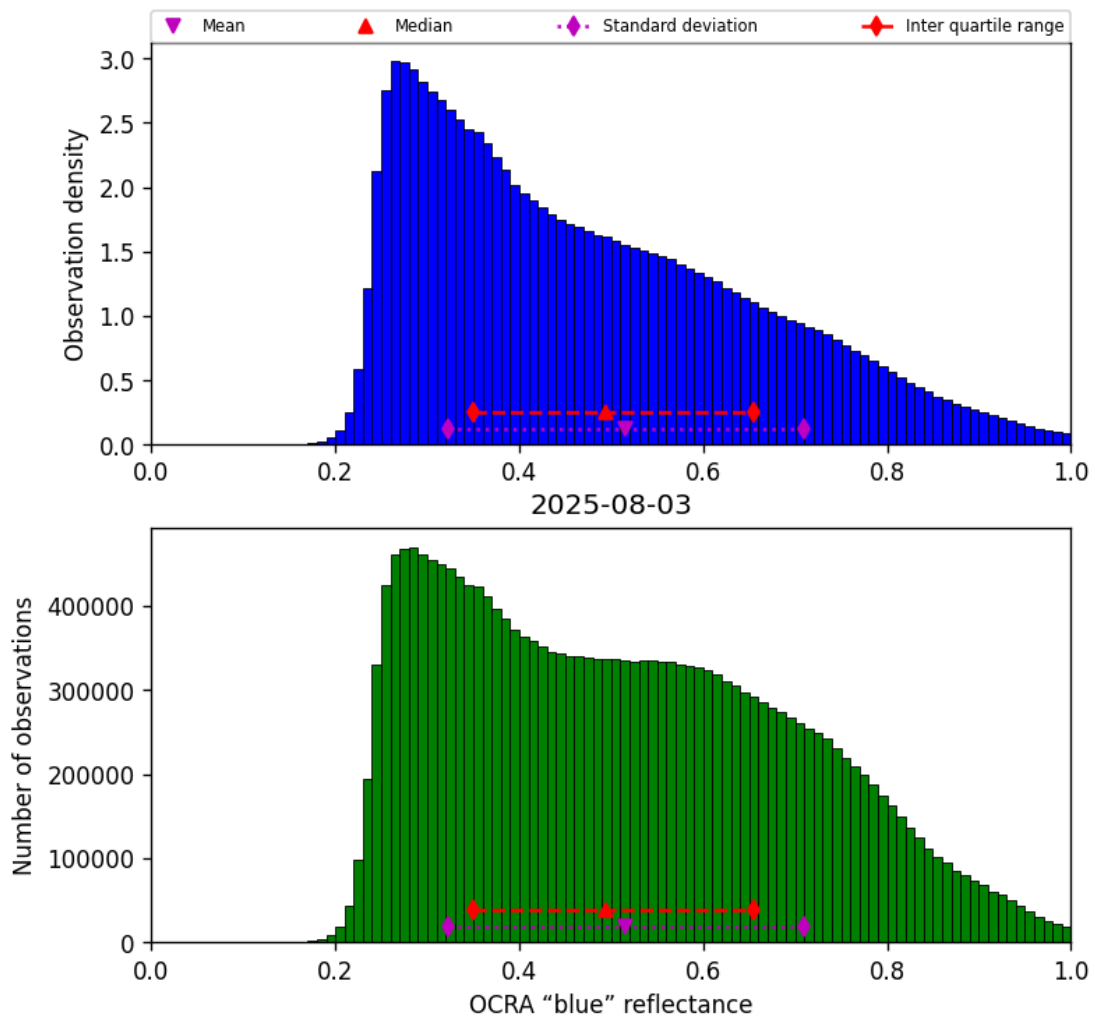
Figure 51: Histogram of “OCRA “blue” reflectance” for 2025-08-03 to 2025-08-04
