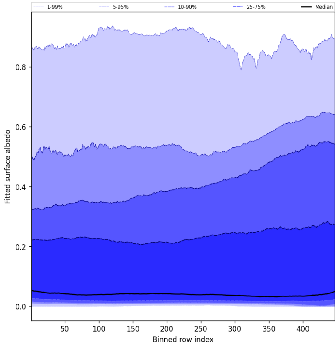
Figure 61: Along track statistics of “Fitted surface albedo” for 2025-08-03 to 2025-08-04
