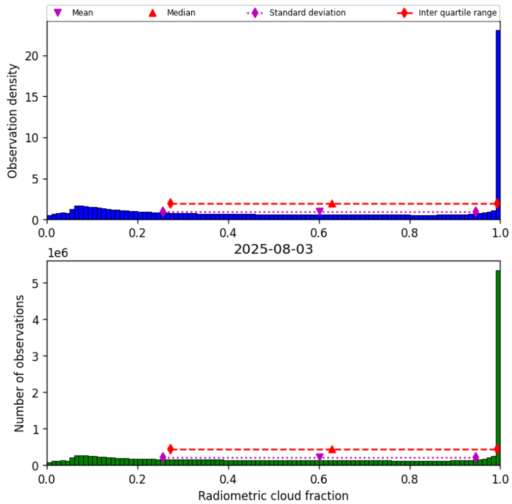
Figure 39: Histogram of “Radiometric cloud fraction” for 2025-08-03 to 2025-08-04
