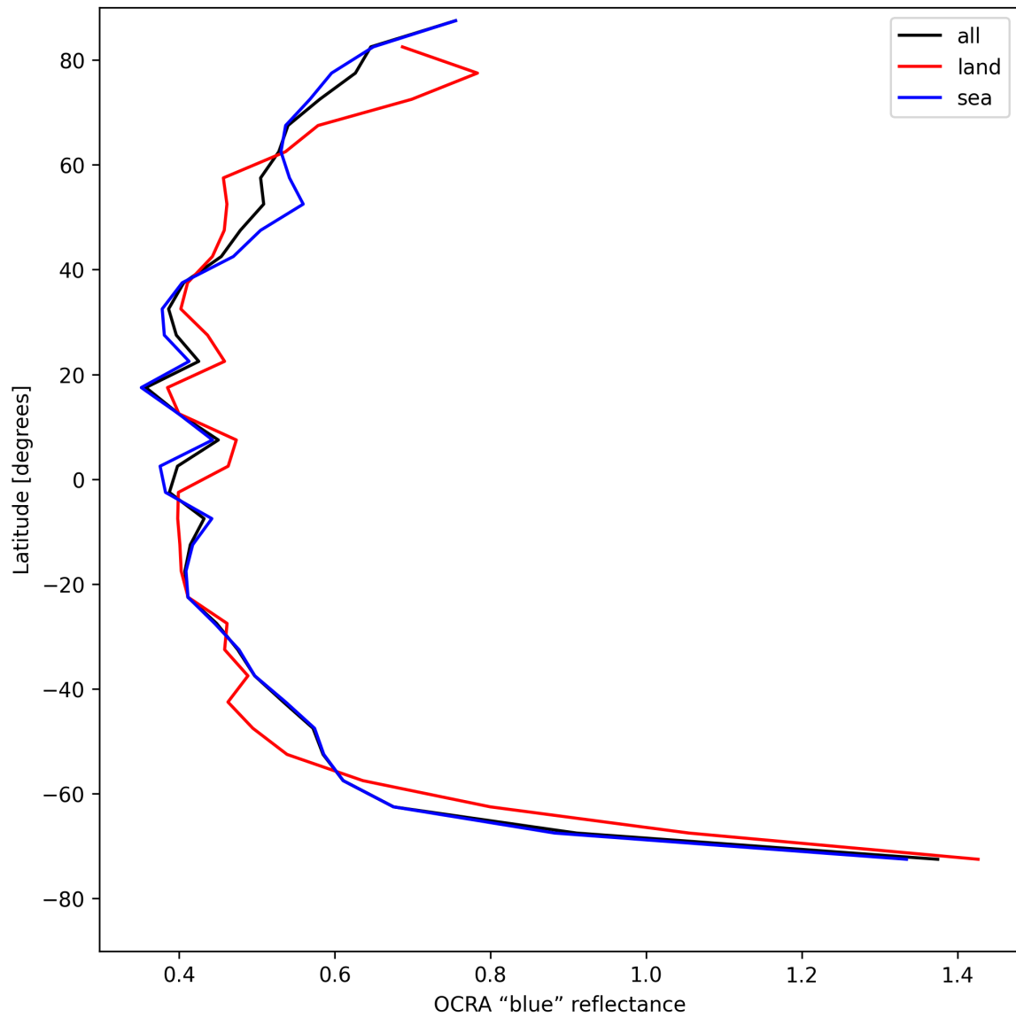
Figure 35: Zonal average of “OCRA “blue” reflectance” for 2025-08-03 to 2025-08-04.
