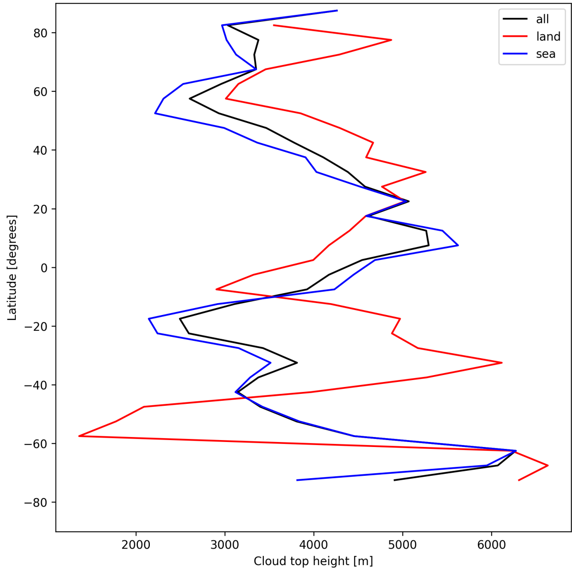
Figure 24: Zonal average of “Cloud top height” for 2025-08-03 to 2025-08-04.
