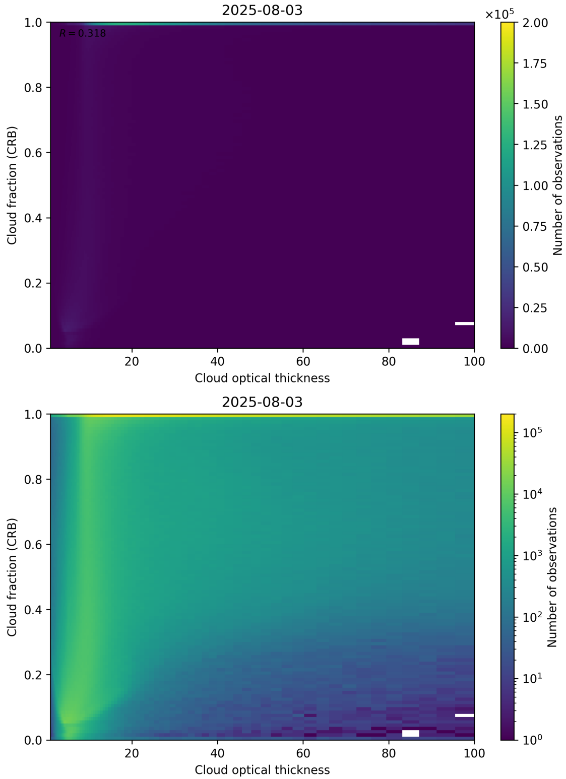
Figure 84: Scatter density plot of “Cloud optical thickness” against “Cloud fraction (CRB)” for 2025-08-03 to 2025-08-04.
