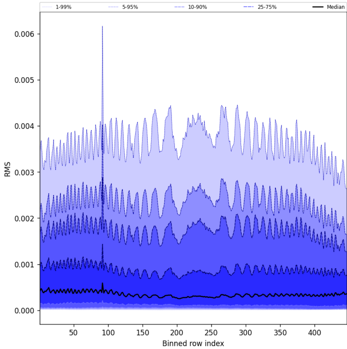
Figure 63: Along track statistics of “RMS” for 2025-08-03 to 2025-08-04
