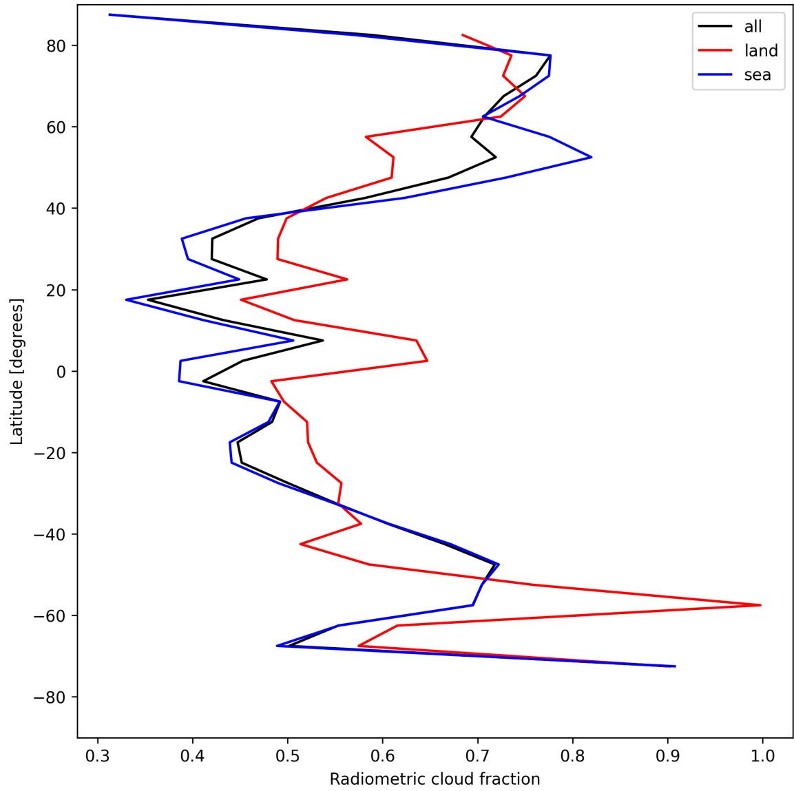
Figure 23: Zonal average of “Radiometric cloud fraction” for 2025-08-03 to 2025-08-04.
