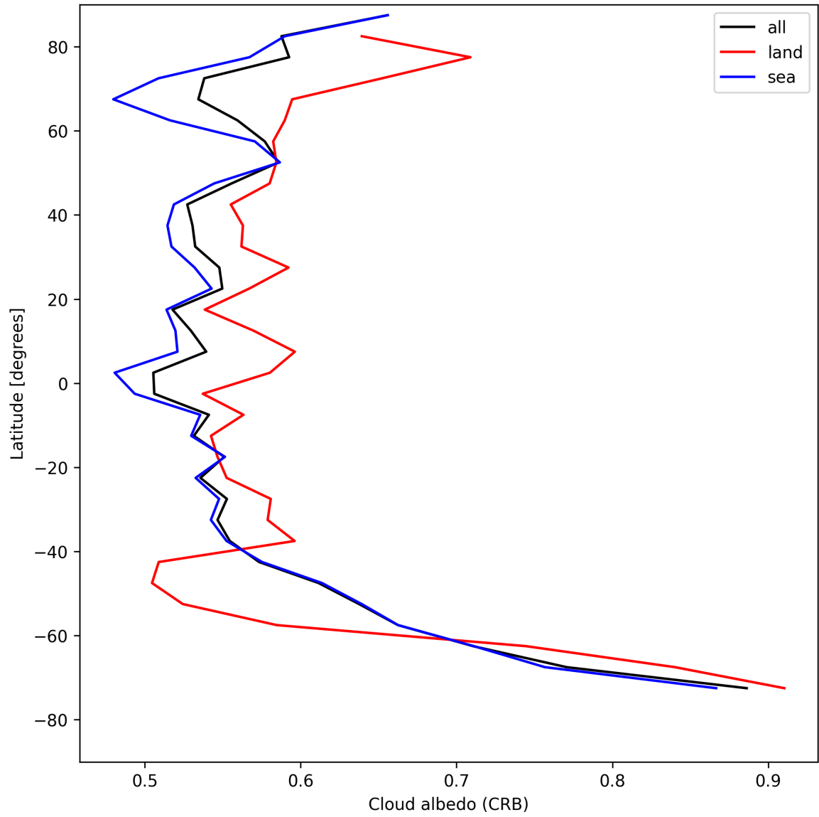
Figure 28: Zonal average of “Cloud albedo (CRB)” for 2025-08-03 to 2025-08-04.
