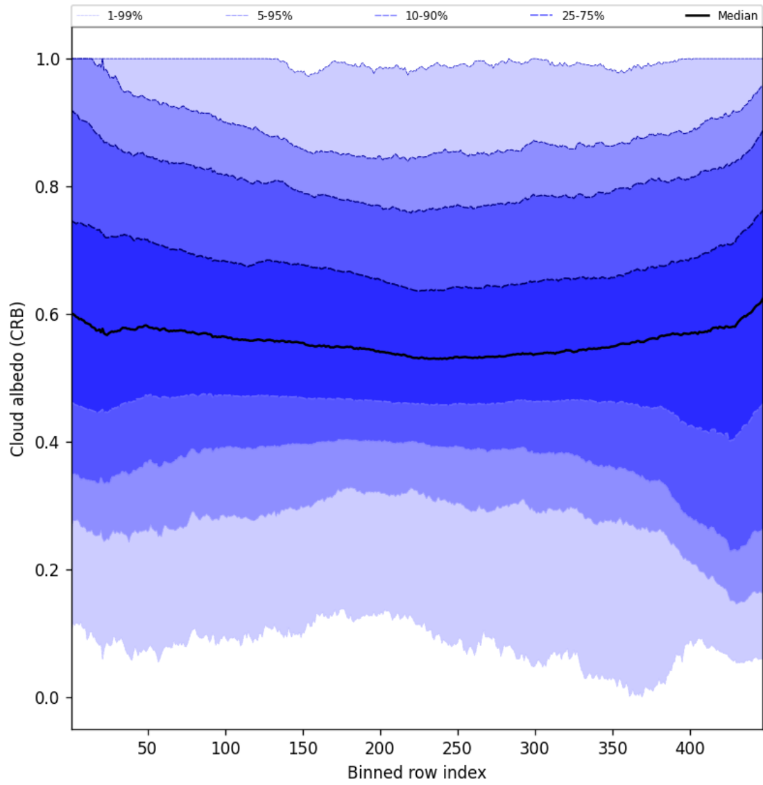
Figure 60: Along track statistics of “Cloud albedo (CRB)” for 2025-08-03 to 2025-08-04
