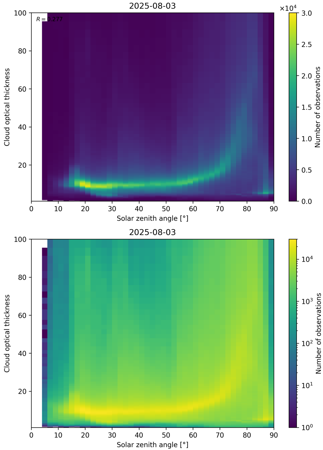
Figure 103: Scatter density plot of “Solar zenith angle” against “Cloud optical thickness” for 2025-08-03 to 2025-08-04.
