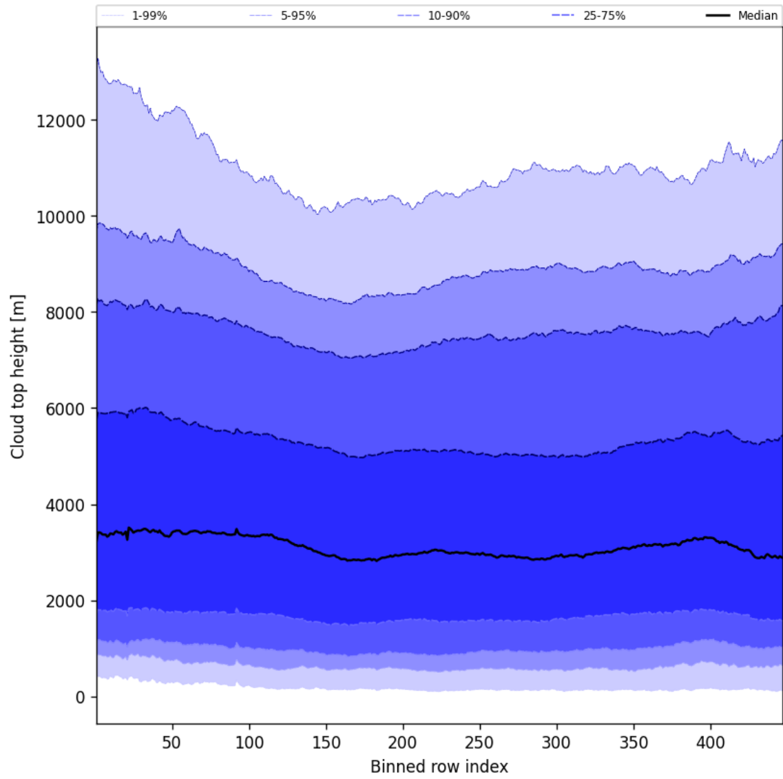
Figure 56: Along track statistics of “Cloud top height” for 2025-08-03 to 2025-08-04
