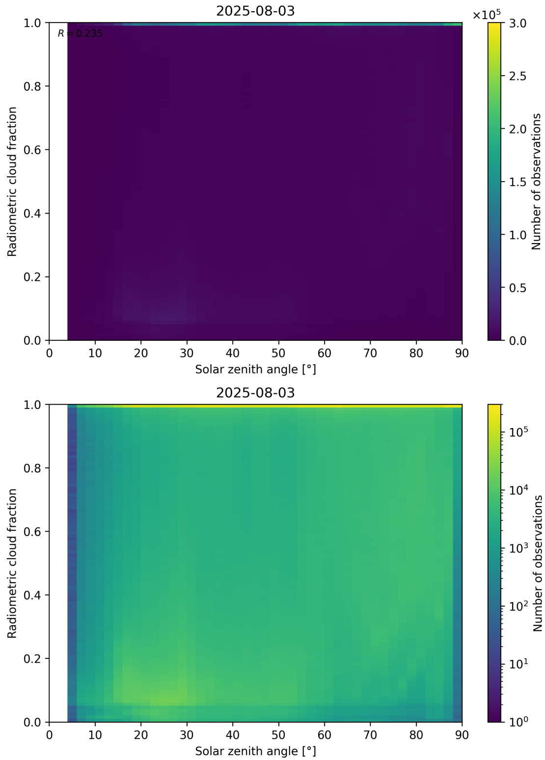
Figure 99: Scatter density plot of “Solar zenith angle” against “Radiometric cloud fraction” for 2025-08-03 to 2025-08-04.
