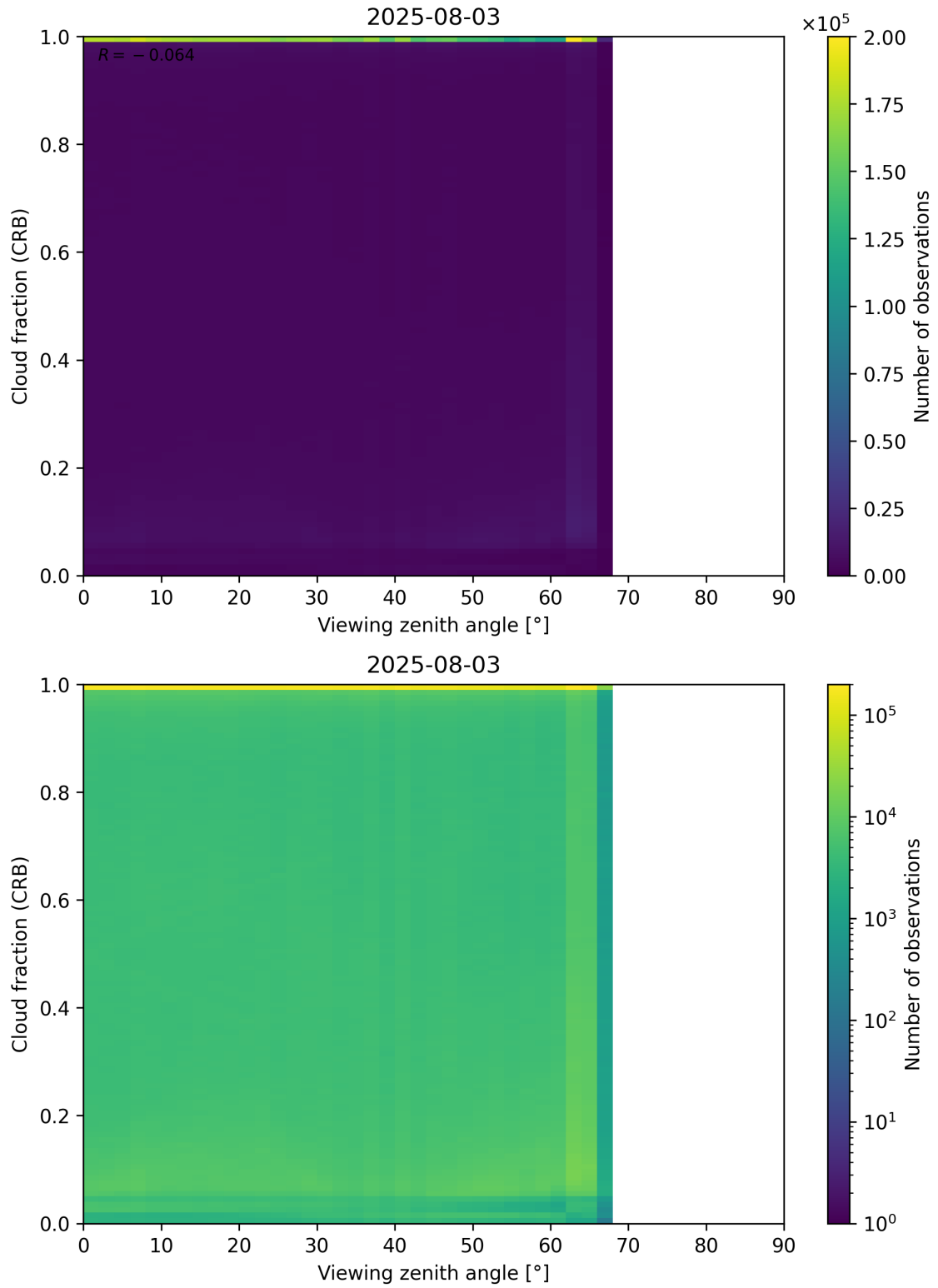
Figure 109: Scatter density plot of “Viewing zenith angle” against “Cloud fraction (CRB)” for 2025-08-03 to 2025-08-04.
