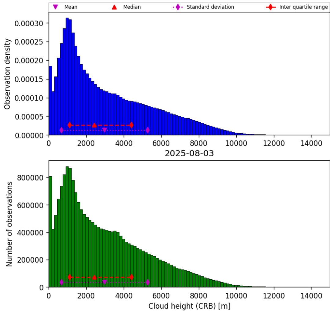
Figure 43: Histogram of “Cloud height (CRB)” for 2025-08-03 to 2025-08-04
