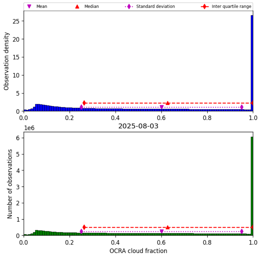
Figure 50: Histogram of “OCRA cloud fraction” for 2025-08-03 to 2025-08-04
