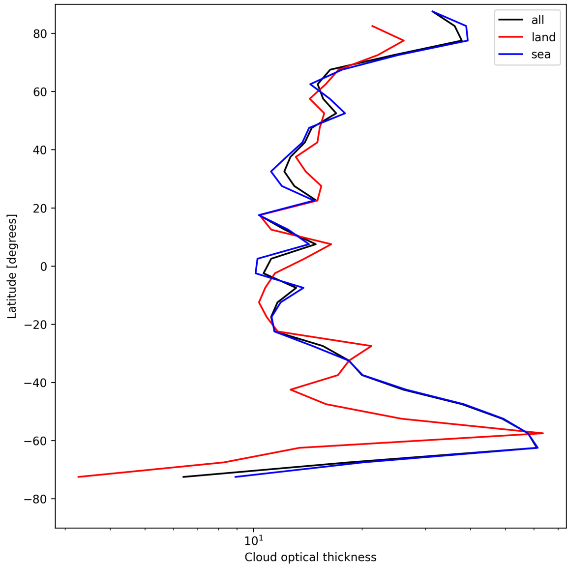
Figure 25: Zonal average of “Cloud optical thickness” for 2025-08-03 to 2025-08-04.
