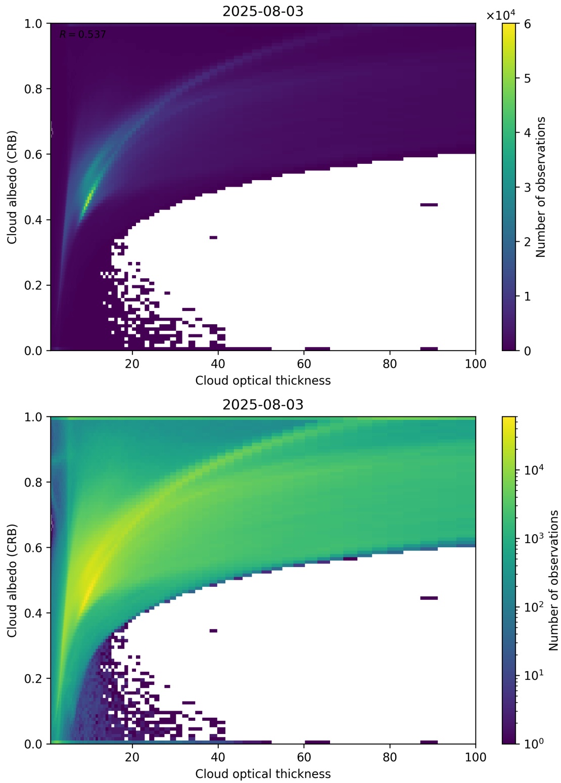
Figure 82: Scatter density plot of “Cloud optical thickness” against “Cloud albedo (CRB)” for 2025-08-03 to 2025-08-04.
