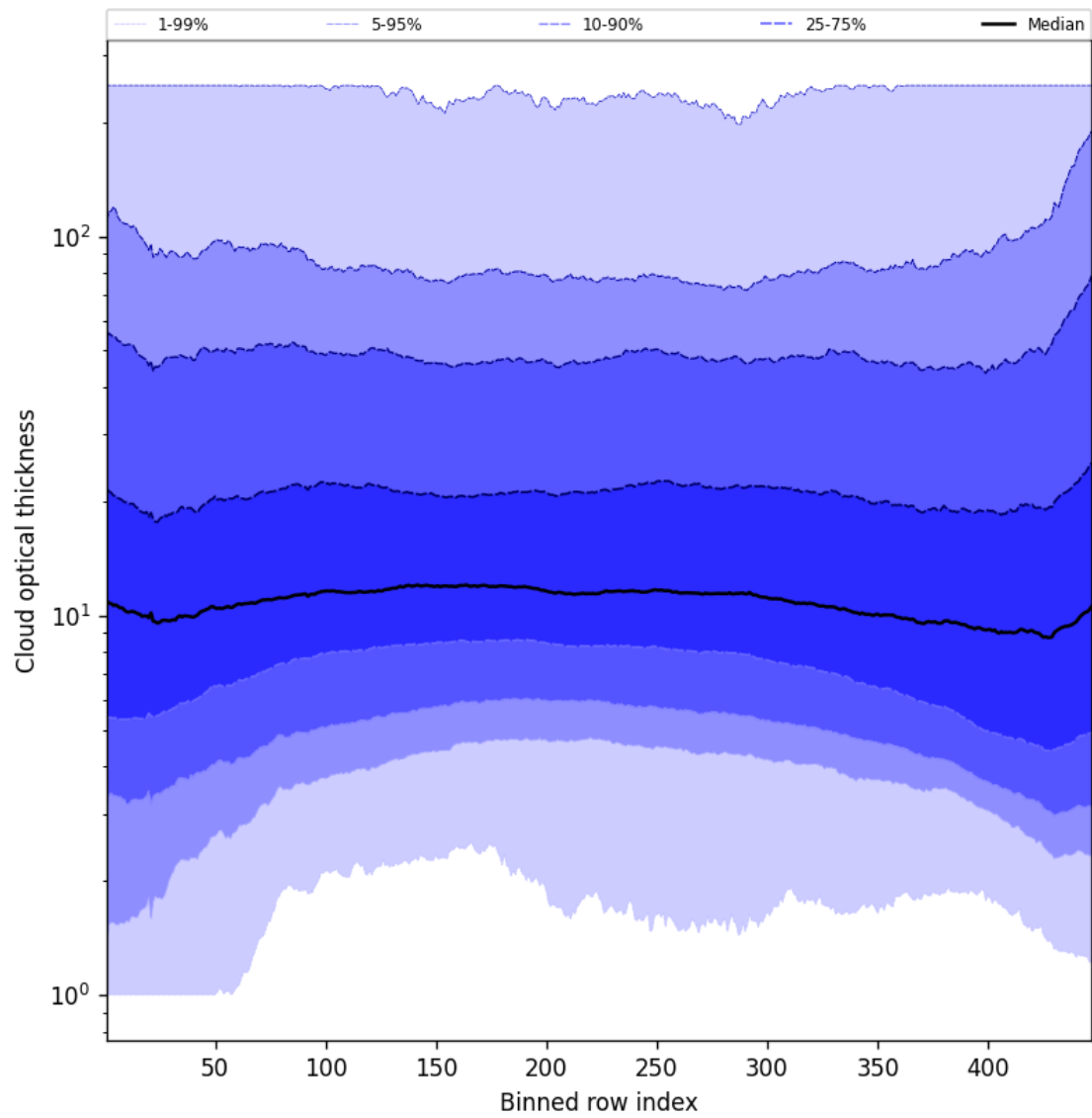
Figure 57: Along track statistics of “Cloud optical thickness” for 2025-08-03 to 2025-08-04
