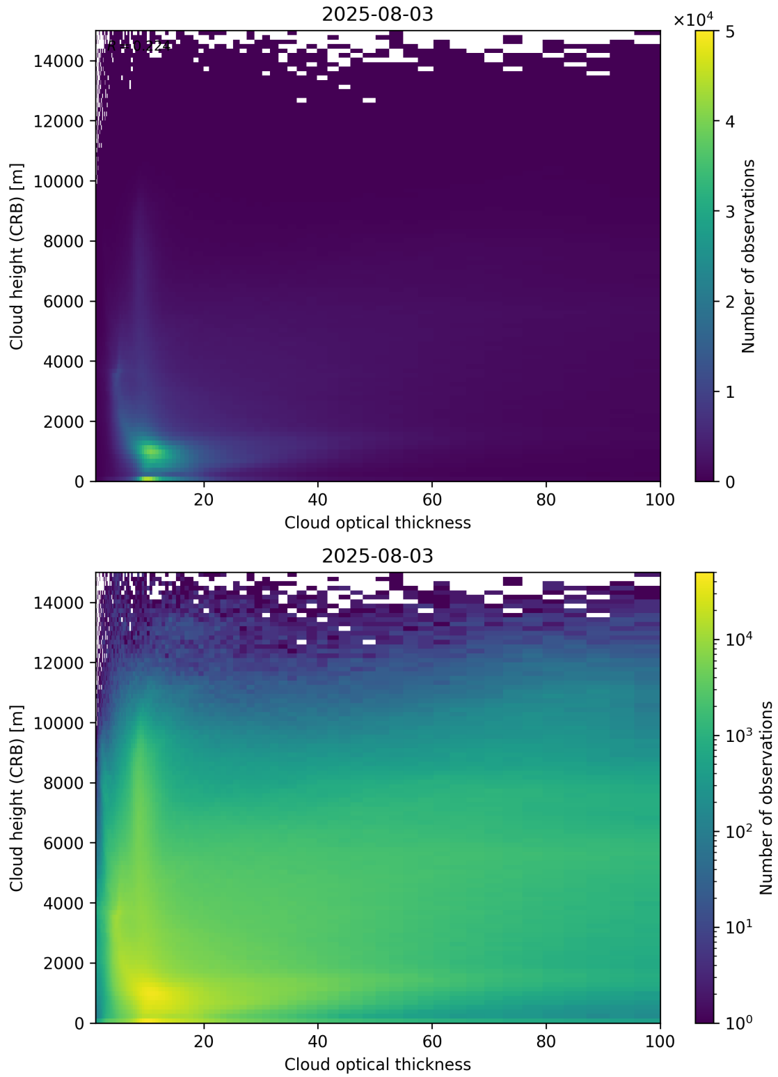
Figure 85: Scatter density plot of “Cloud optical thickness” against “Cloud height (CRB)” for 2025-08-03 to 2025-08-04.
