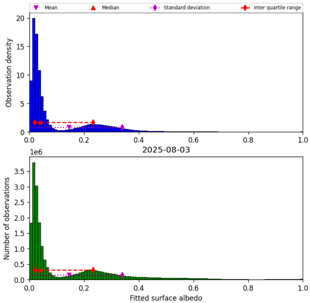
Figure 45: Histogram of “Fitted surface albedo” for 2025-08-03 to 2025-08-04
