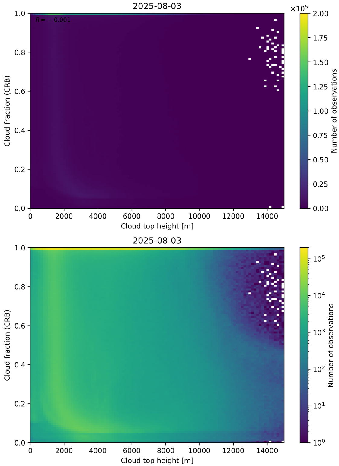
Figure 88: Scatter density plot of “Cloud top height” against “Cloud fraction (CRB)” for 2025-08-03 to 2025-08-04.
