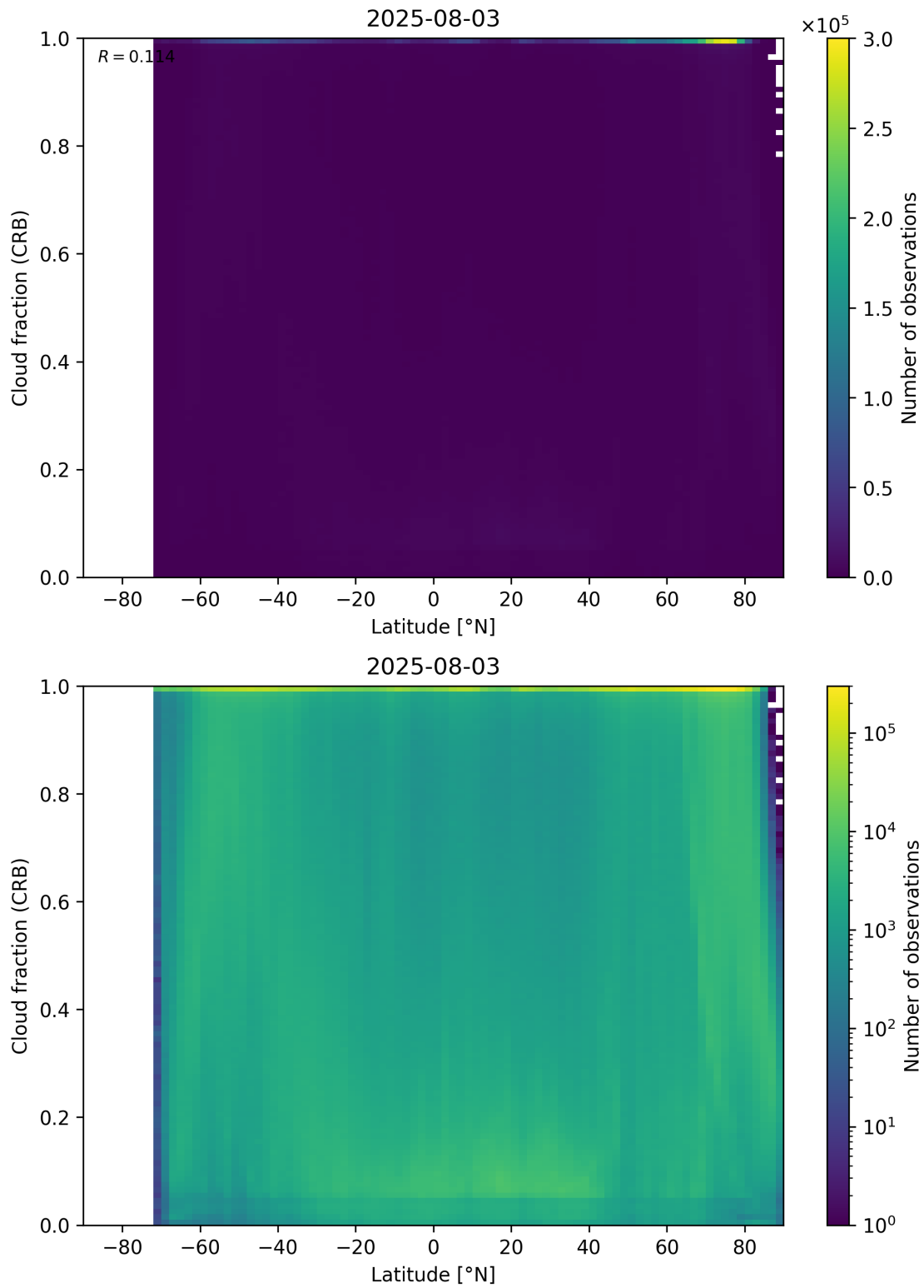
Figure 94: Scatter density plot of “Latitude” against “Cloud fraction (CRB)” for 2025-08-03 to 2025-08-04.
