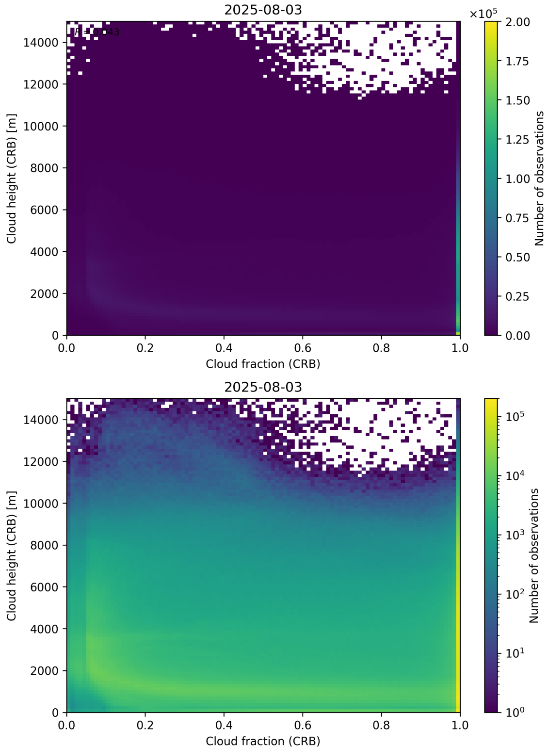
Figure 79: Scatter density plot of “Cloud fraction (CRB)” against “Cloud height (CRB)” for 2025-08-03 to 2025-08-04.
