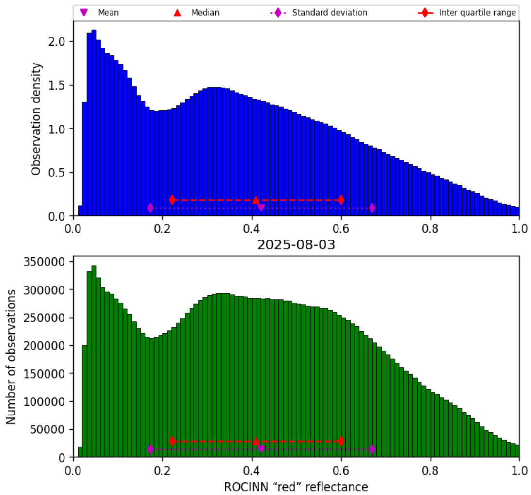
Figure 53: Histogram of “ROCINN “red” reflectance” for 2025-08-03 to 2025-08-04
