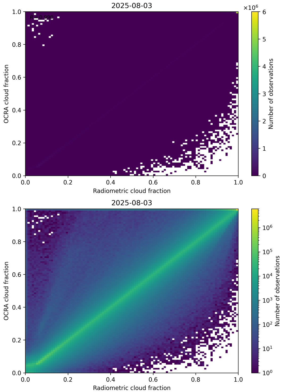
Figure 72: Scatter density plot of “Radiometric cloud fraction” against “OCRA cloud fraction” for 2025-08-03 to 2025-08-04.
