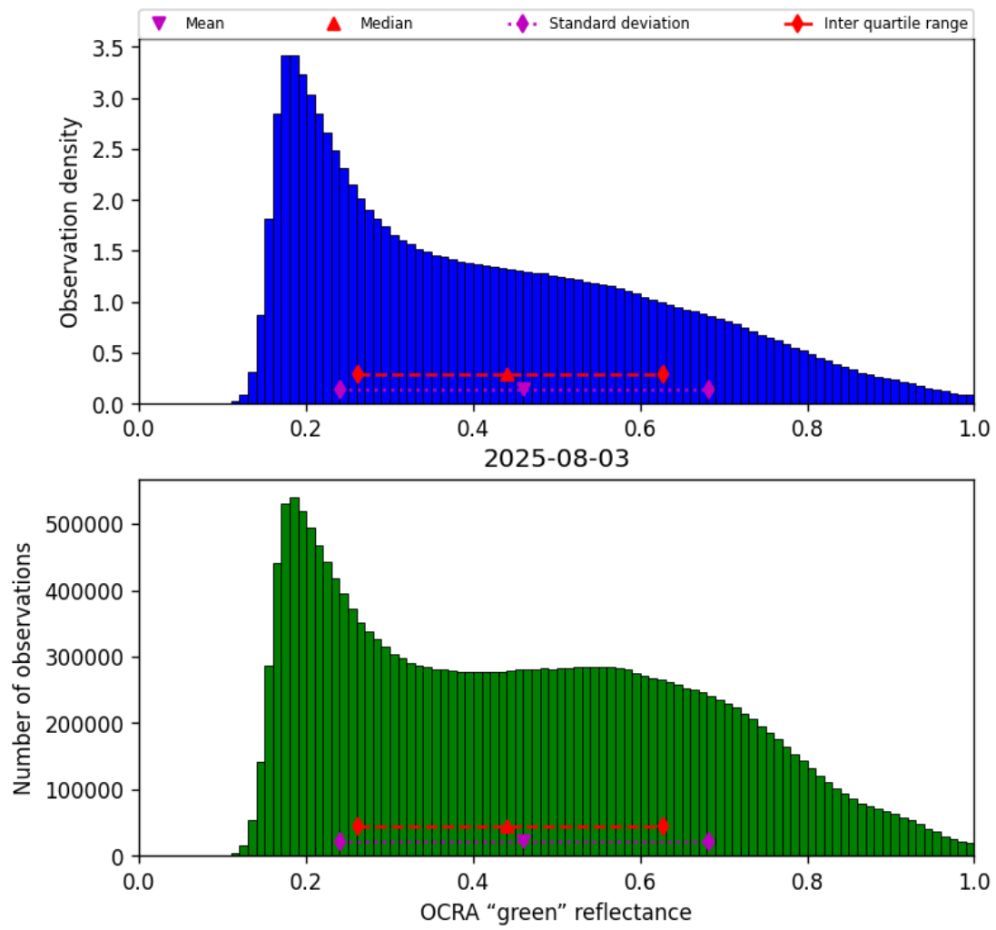
Figure 52: Histogram of “OCRA “green” reflectance” for 2025-08-03 to 2025-08-04
