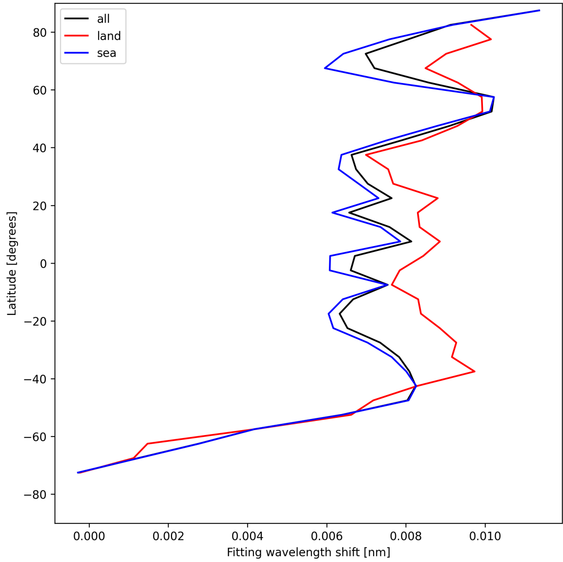
Figure 33: Zonal average of “Fitting wavelength shift” for 2025-08-03 to 2025-08-04.
