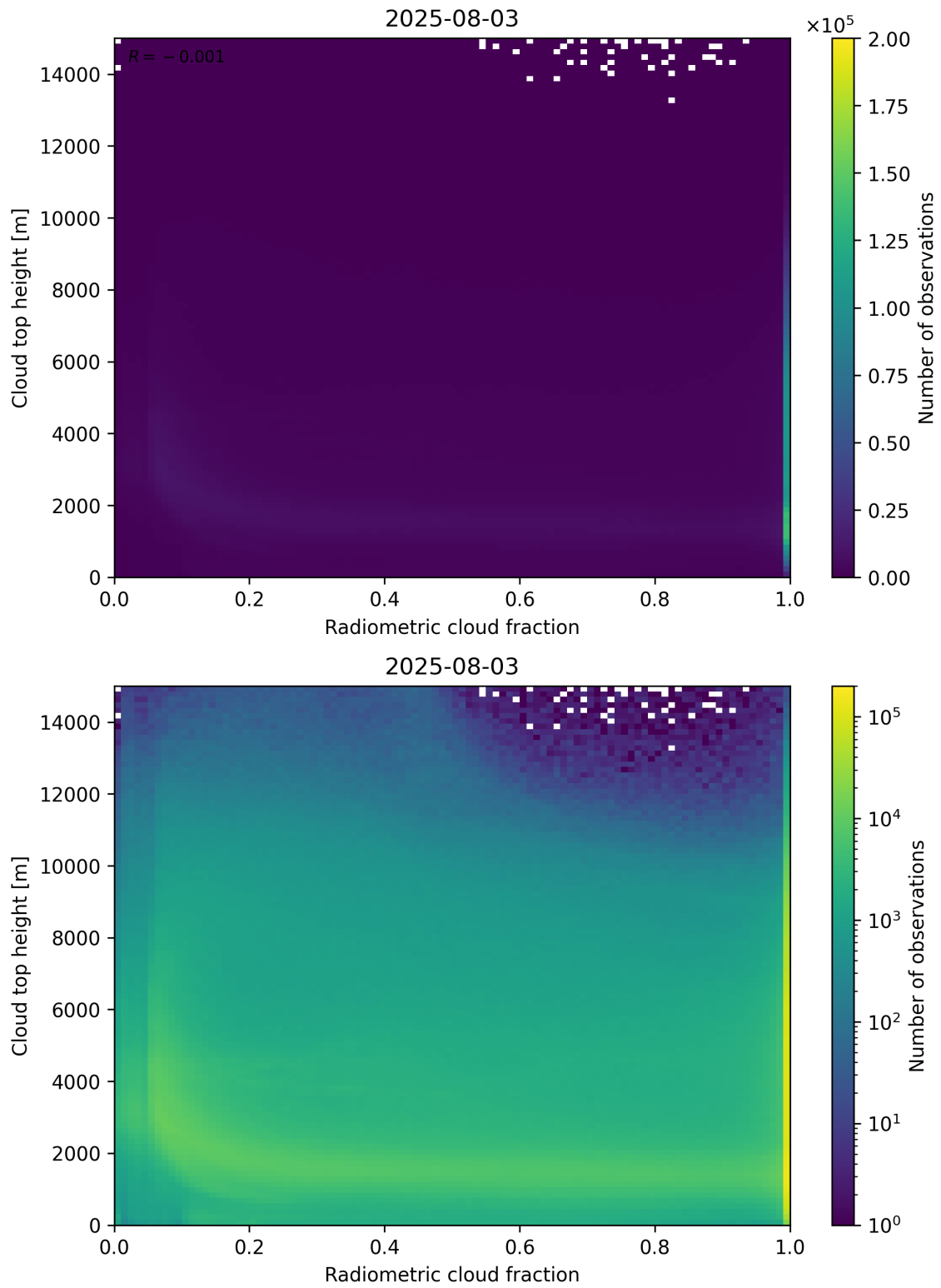
Figure 76: Scatter density plot of “Radiometric cloud fraction” against “Cloud top height” for 2025-08-03 to 2025-08-04.
