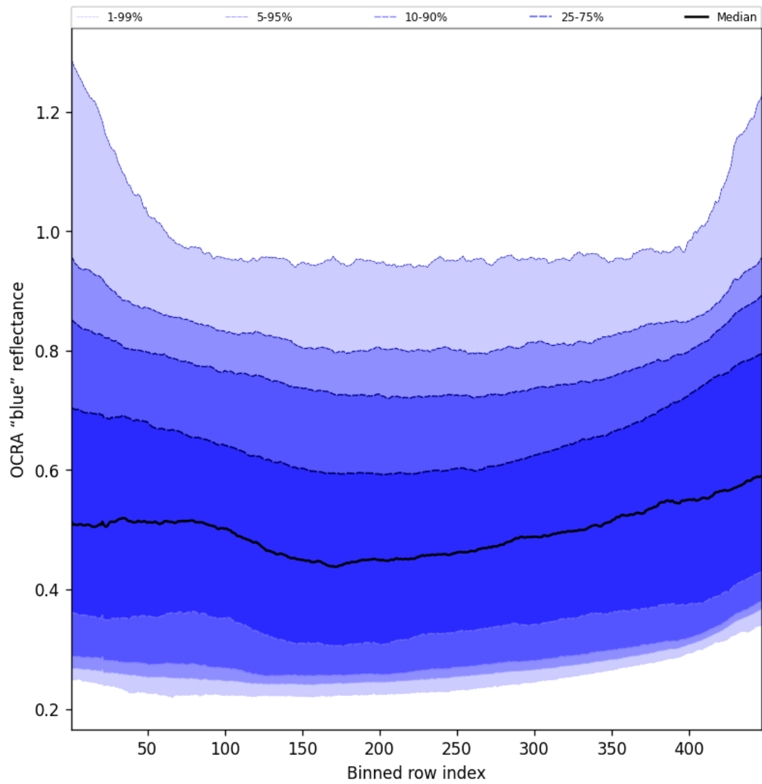
Figure 67: Along track statistics of "OCRA "blue" reflectance" for 2025-08-03 to 2025-08-04
