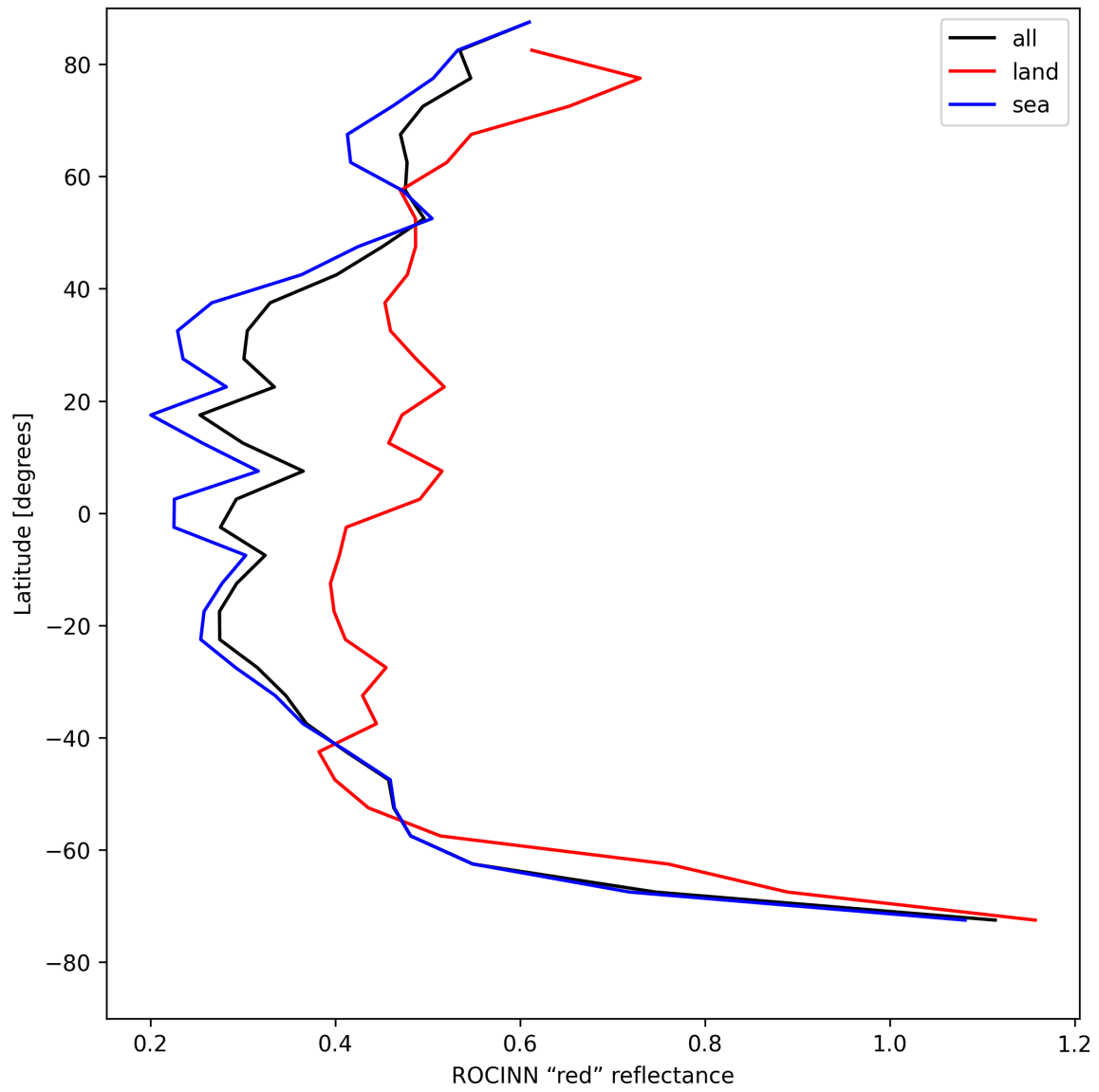
Figure 37: Zonal average of “ROCINN “red” reflectance” for 2025-08-03 to 2025-08-04.
