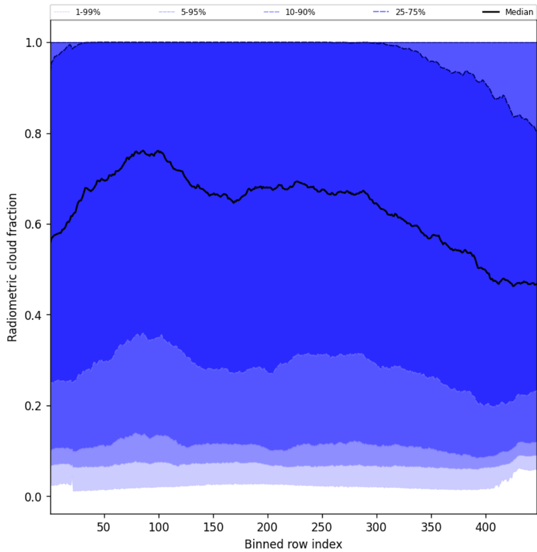
Figure 55: Along track statistics of “Radiometric cloud fraction” for 2025-08-03 to 2025-08-04
