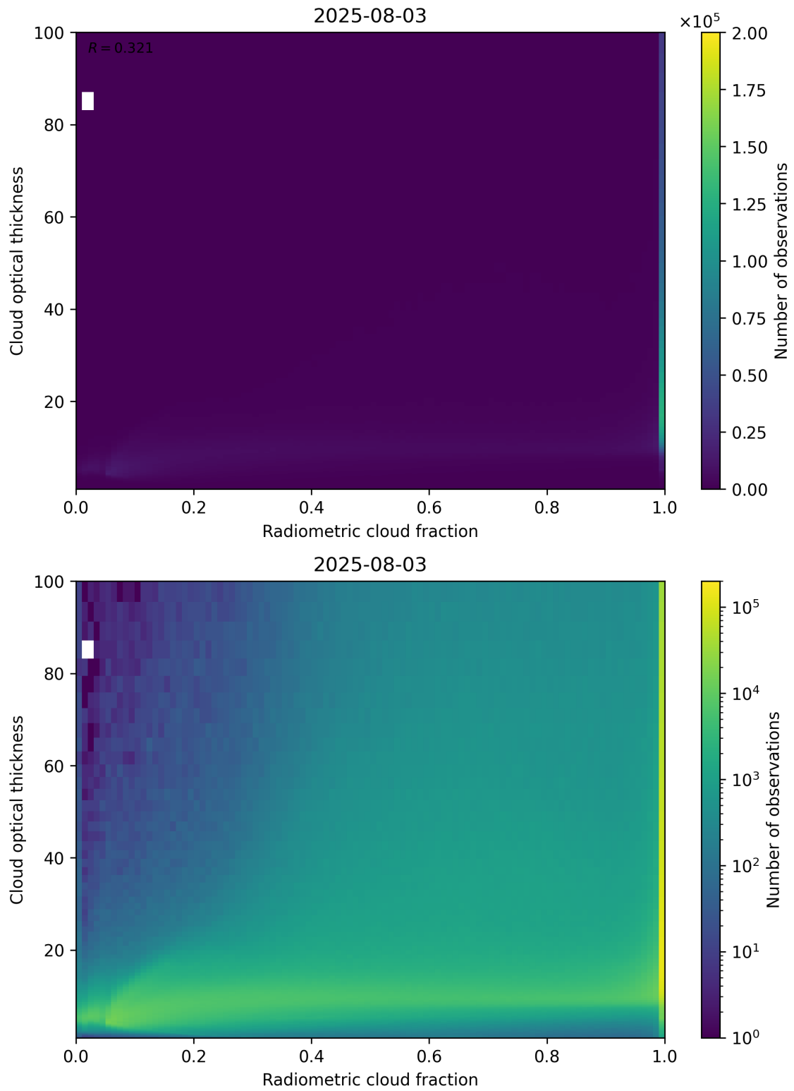
Figure 75: Scatter density plot of “Radiometric cloud fraction” against “Cloud optical thickness” for 2025-08-03 to 2025-08-04.
