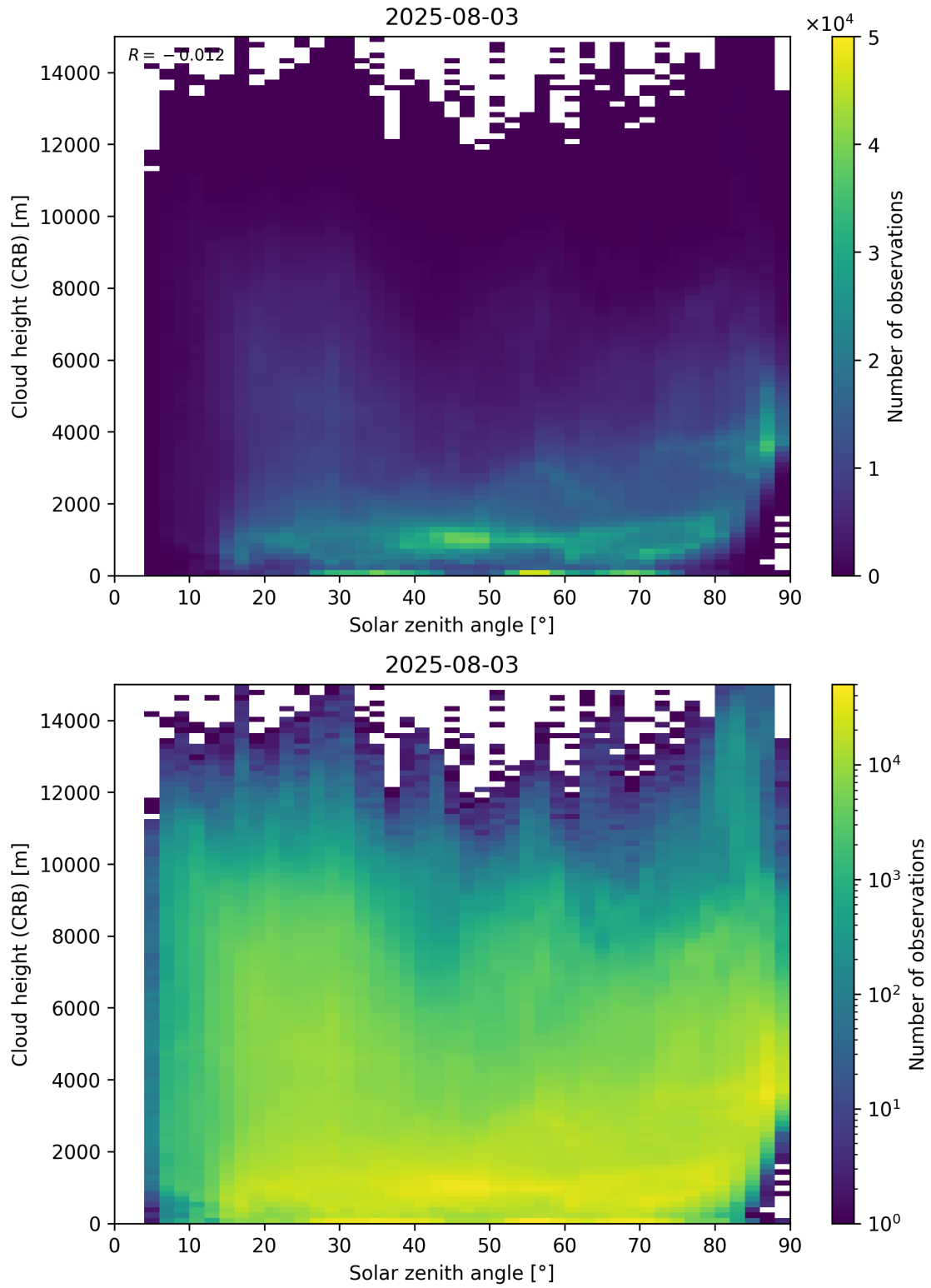
Figure 102: Scatter density plot of “Solar zenith angle” against “Cloud height (CRB)” for 2025-08-03 to 2025-08-04.
