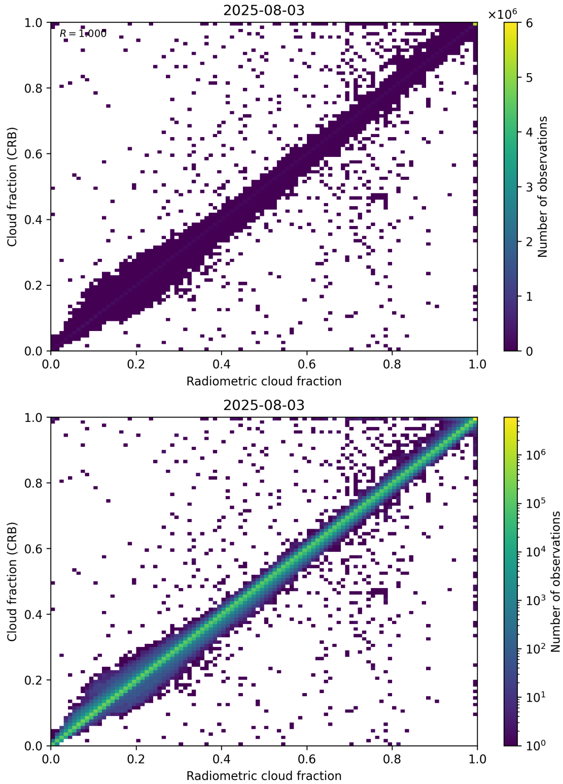
Figure 73: Scatter density plot of “Radiometric cloud fraction” against “Cloud fraction (CRB)” for 2025-08-03 to 2025-08-04.
