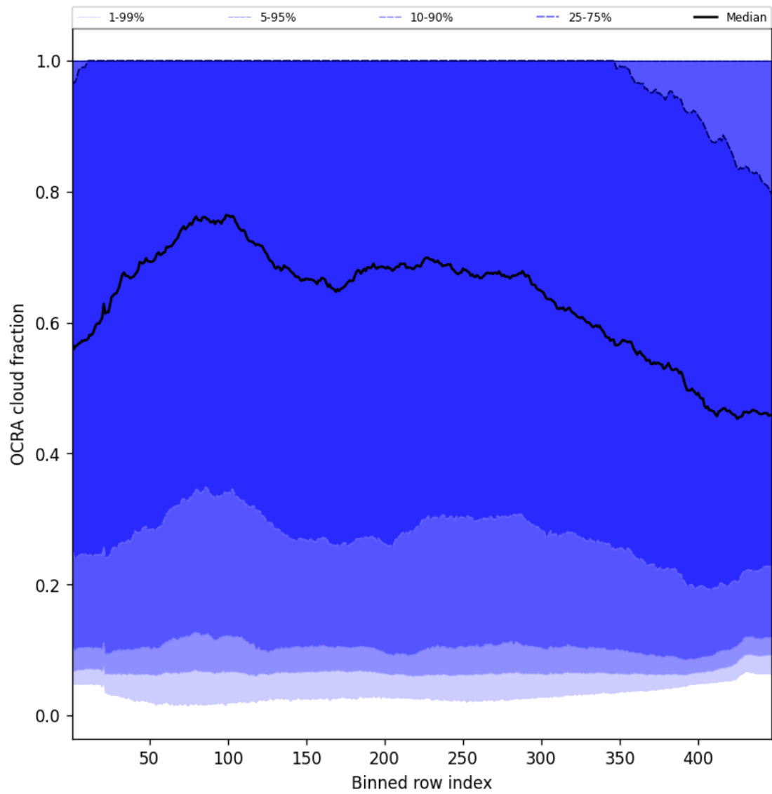
Figure 66: Along track statistics of “OCRA cloud fraction” for 2025-08-03 to 2025-08-04
