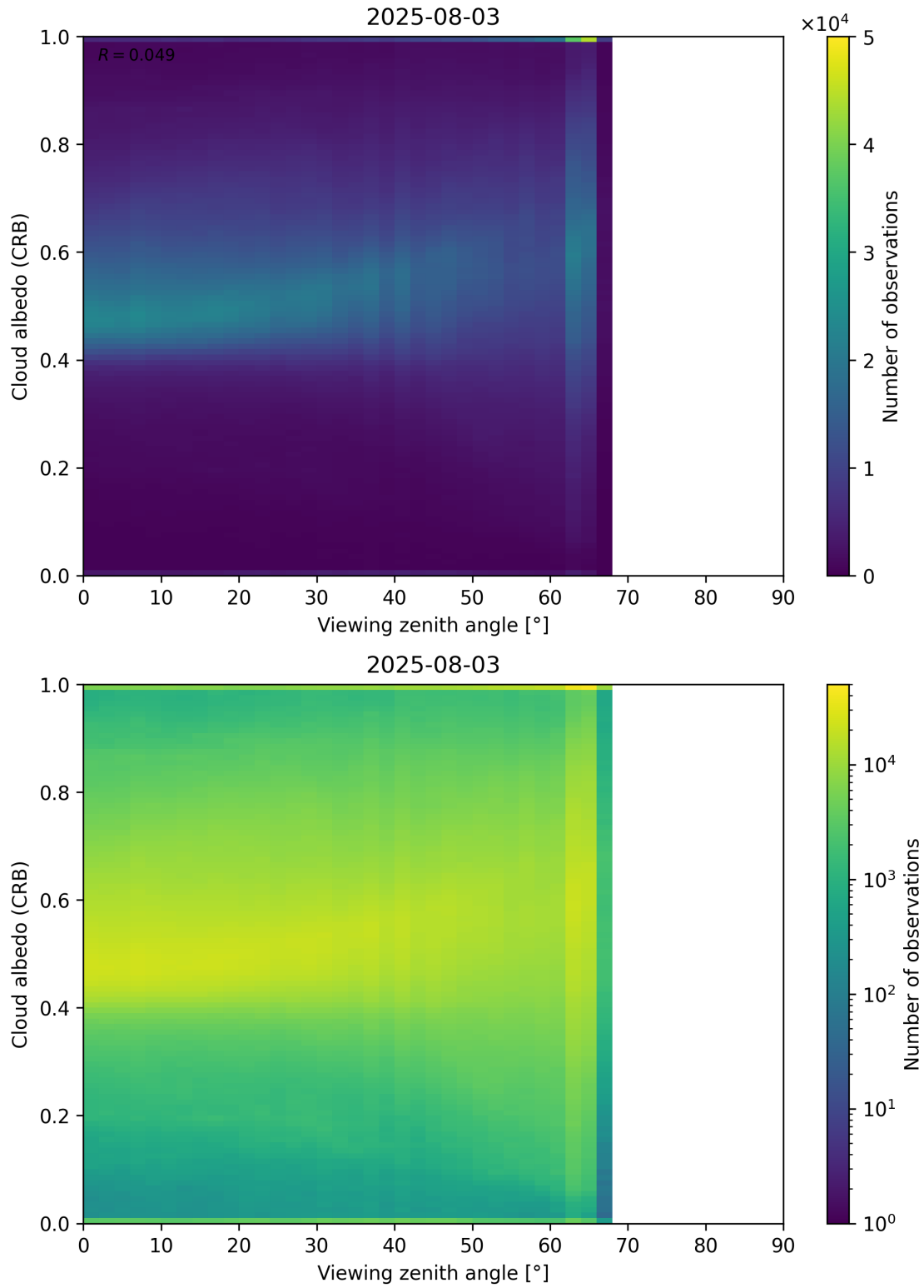
Figure 106: Scatter density plot of “Viewing zenith angle” against “Cloud albedo (CRB)” for 2025-08-03 to 2025-08-04.
