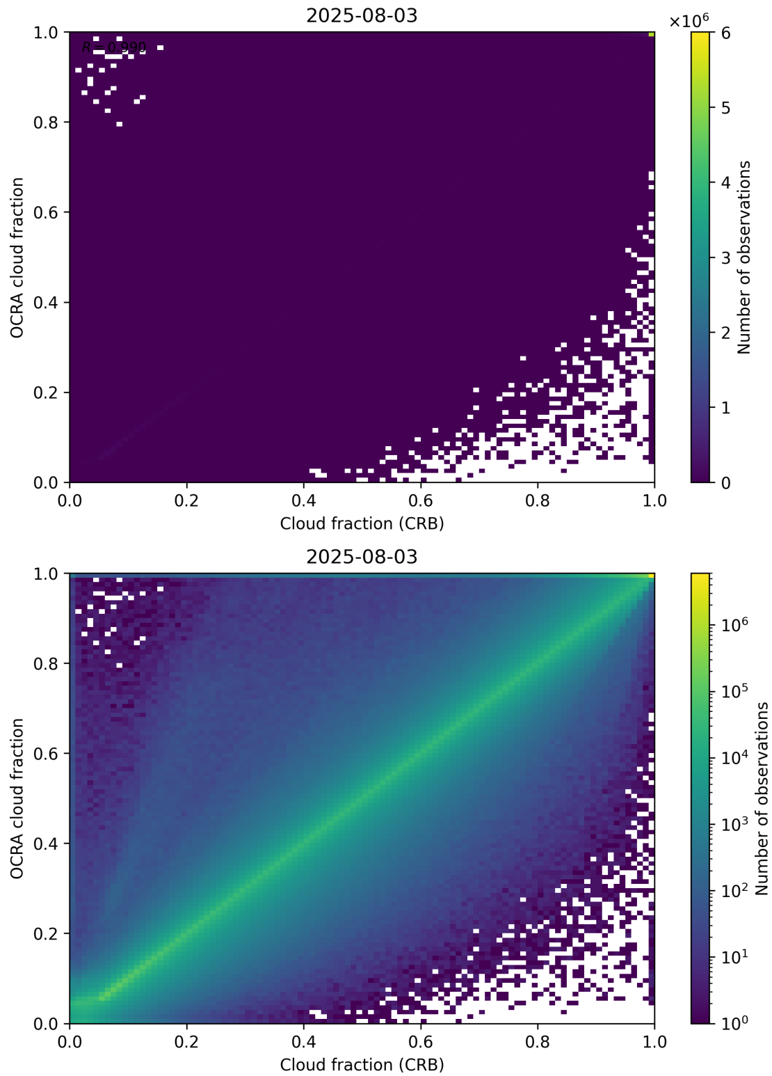
Figure 78: Scatter density plot of “Cloud fraction (CRB)” against “OCRA cloud fraction” for 2025-08-03 to 2025-08-04.
