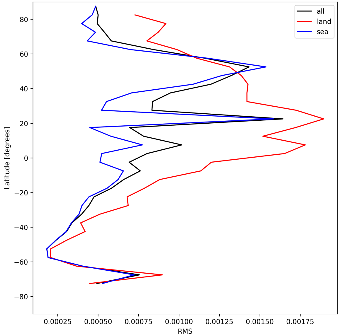
Figure 31: Zonal average of “RMS” for 2025-08-03 to 2025-08-04.
