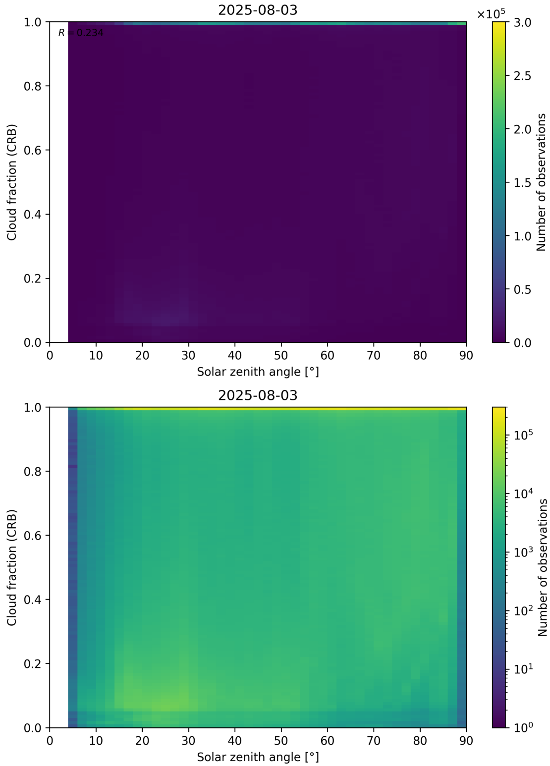
Figure 101: Scatter density plot of “Solar zenith angle” against “Cloud fraction (CRB)” for 2025-08-03 to 2025-08-04.
