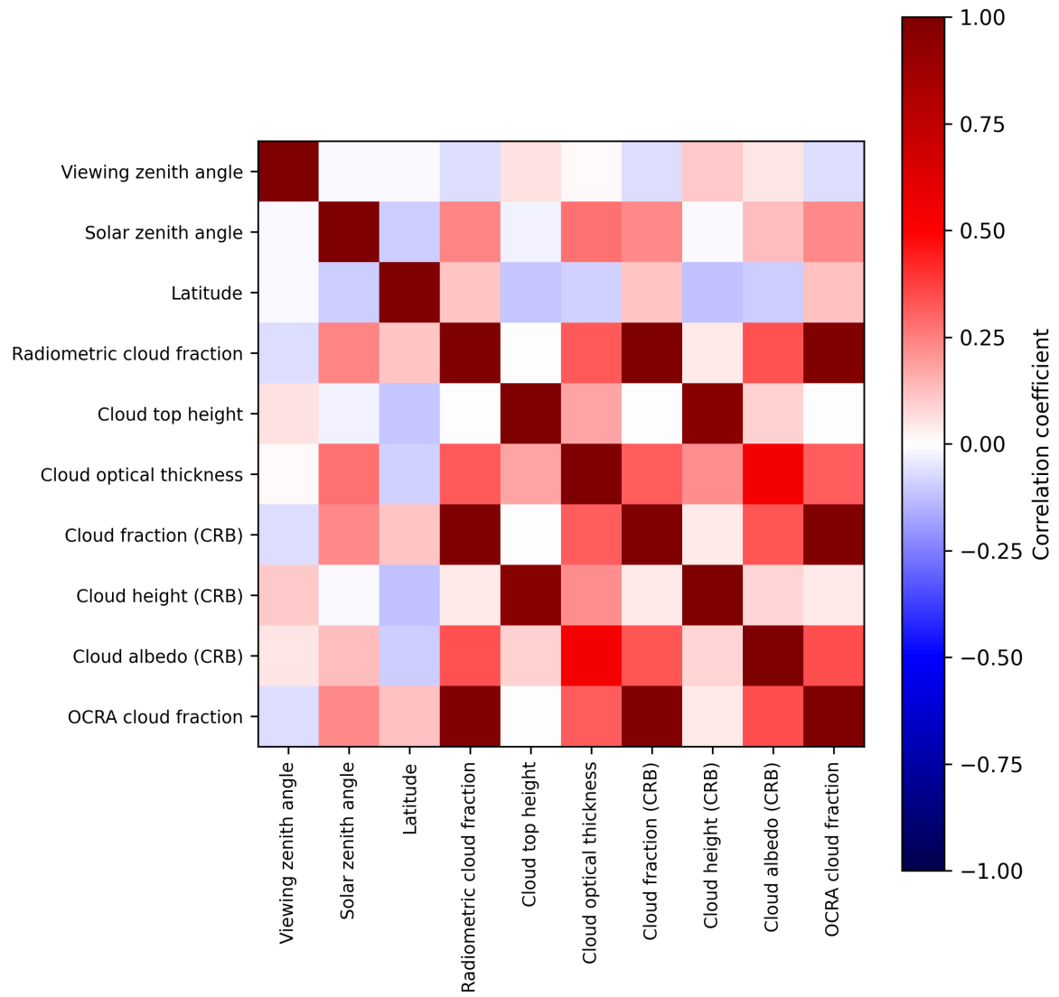
Figure 2: Map of correlation matrix for 2025-08-03 to 2025-08-04.
