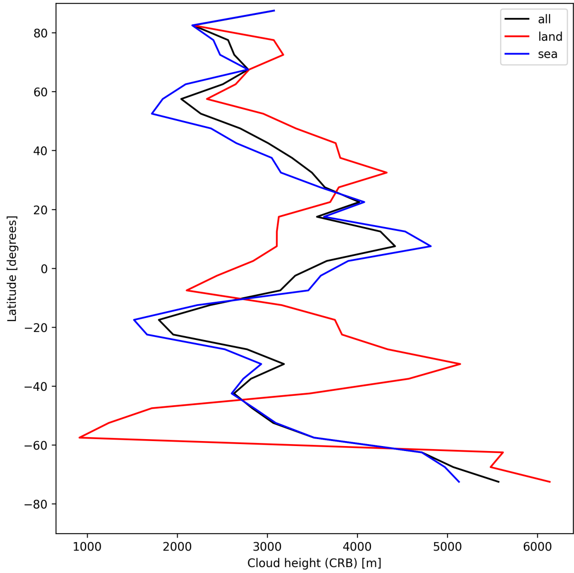
Figure 27: Zonal average of “Cloud height (CRB)” for 2025-08-03 to 2025-08-04.
