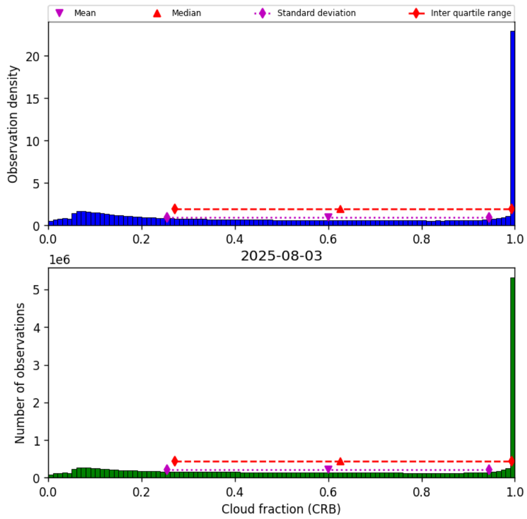
Figure 42: Histogram of “Cloud fraction (CRB)” for 2025-08-03 to 2025-08-04
