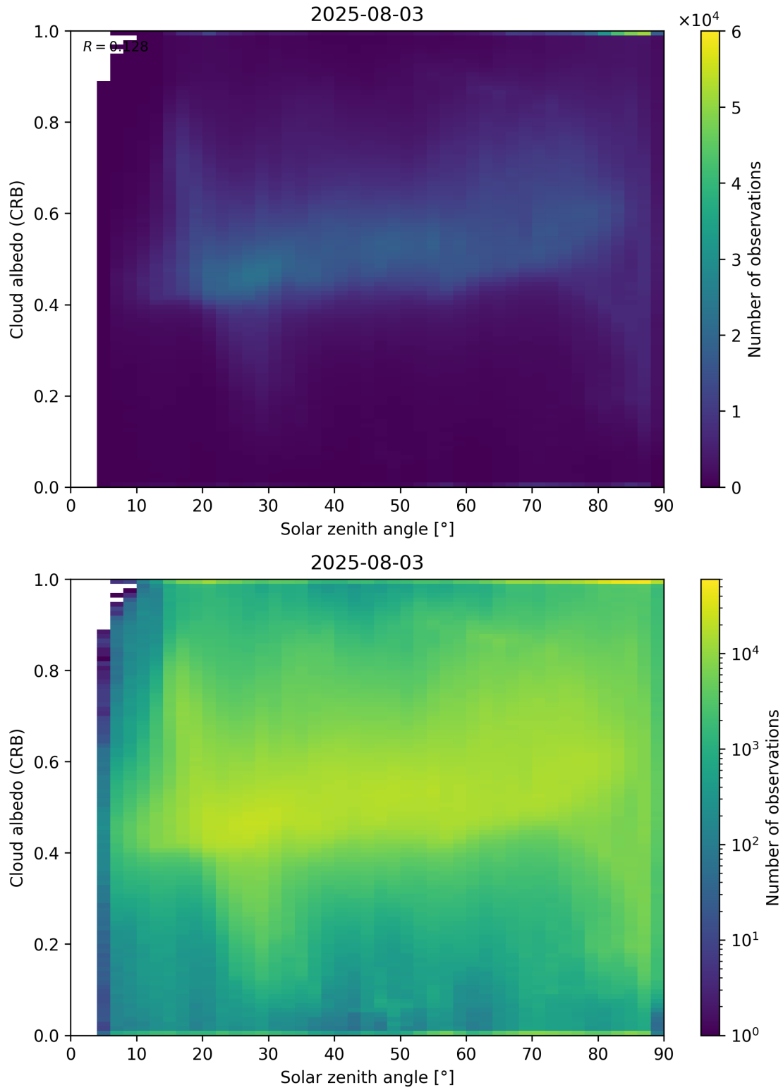
Figure 98: Scatter density plot of “Solar zenith angle” against “Cloud albedo (CRB)” for 2025-08-03 to 2025-08-04.
