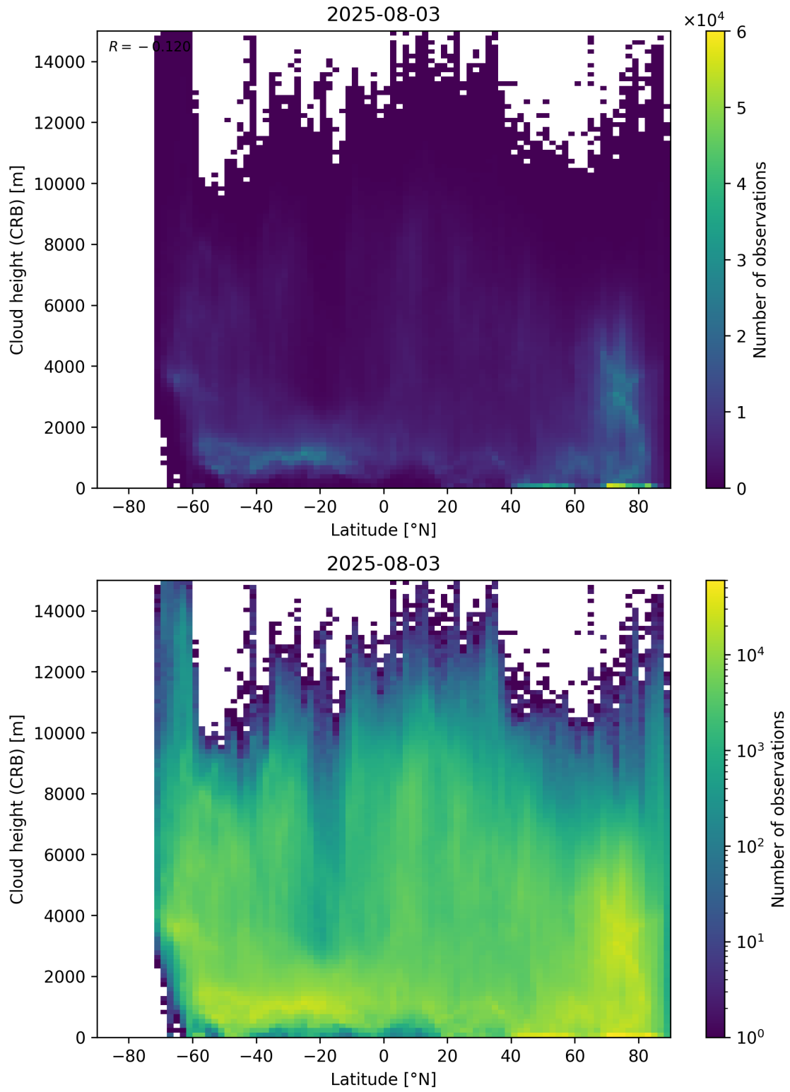
Figure 95: Scatter density plot of “Latitude” against “Cloud height (CRB)” for 2025-08-03 to 2025-08-04.
