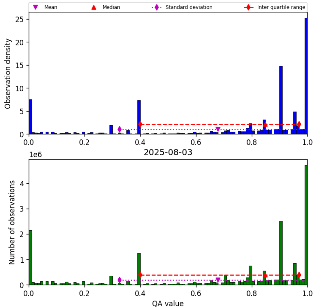
Figure 38: Histogram of “QA value” for 2025-08-03 to 2025-08-04
