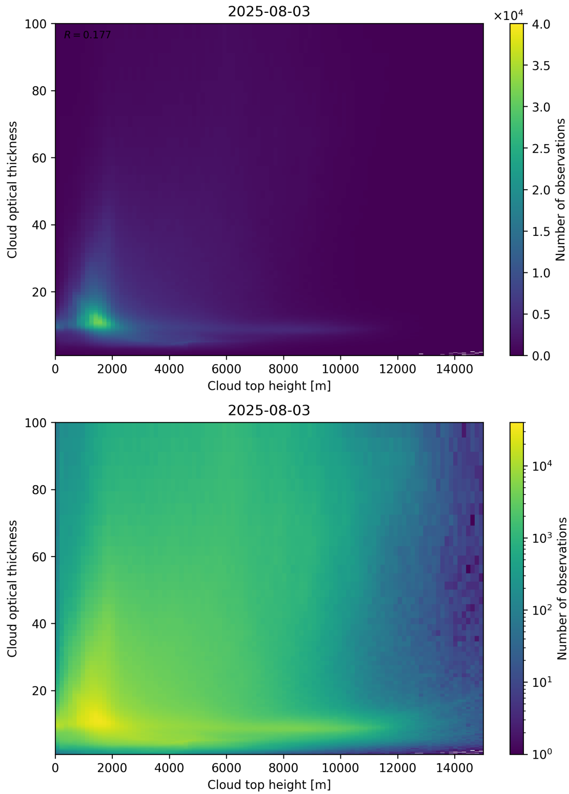
Figure 90: Scatter density plot of “Cloud top height” against “Cloud optical thickness” for 2025-08-03 to 2025-08-04.
