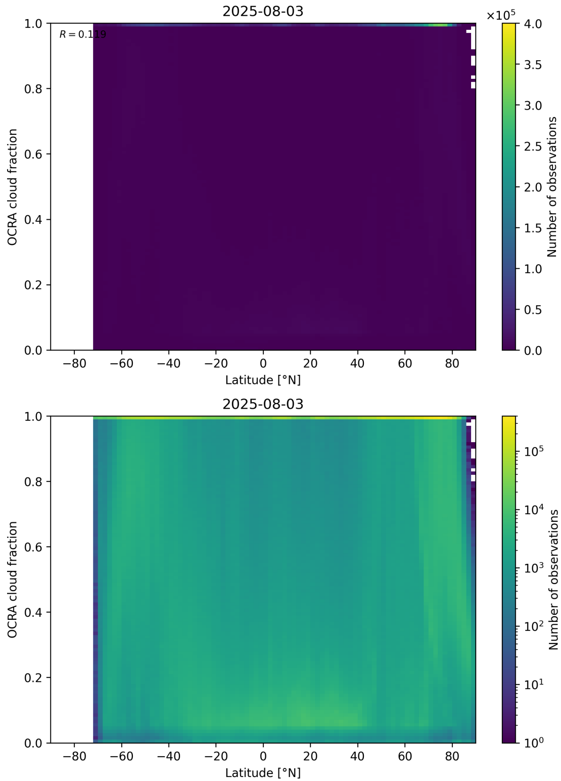
Figure 93: Scatter density plot of “Latitude” against “OCRA cloud fraction” for 2025-08-03 to 2025-08-04.
