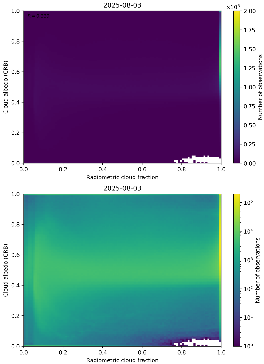
Figure 71: Scatter density plot of “Radiometric cloud fraction” against “Cloud albedo (CRB)” for 2025-08-03 to 2025-08-04.
