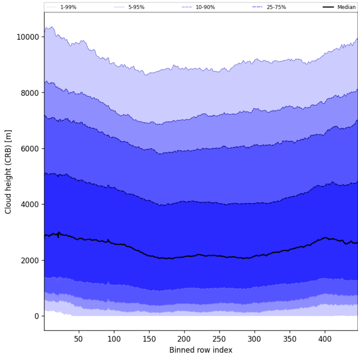
Figure 59: Along track statistics of “Cloud height (CRB)” for 2025-08-03 to 2025-08-04
