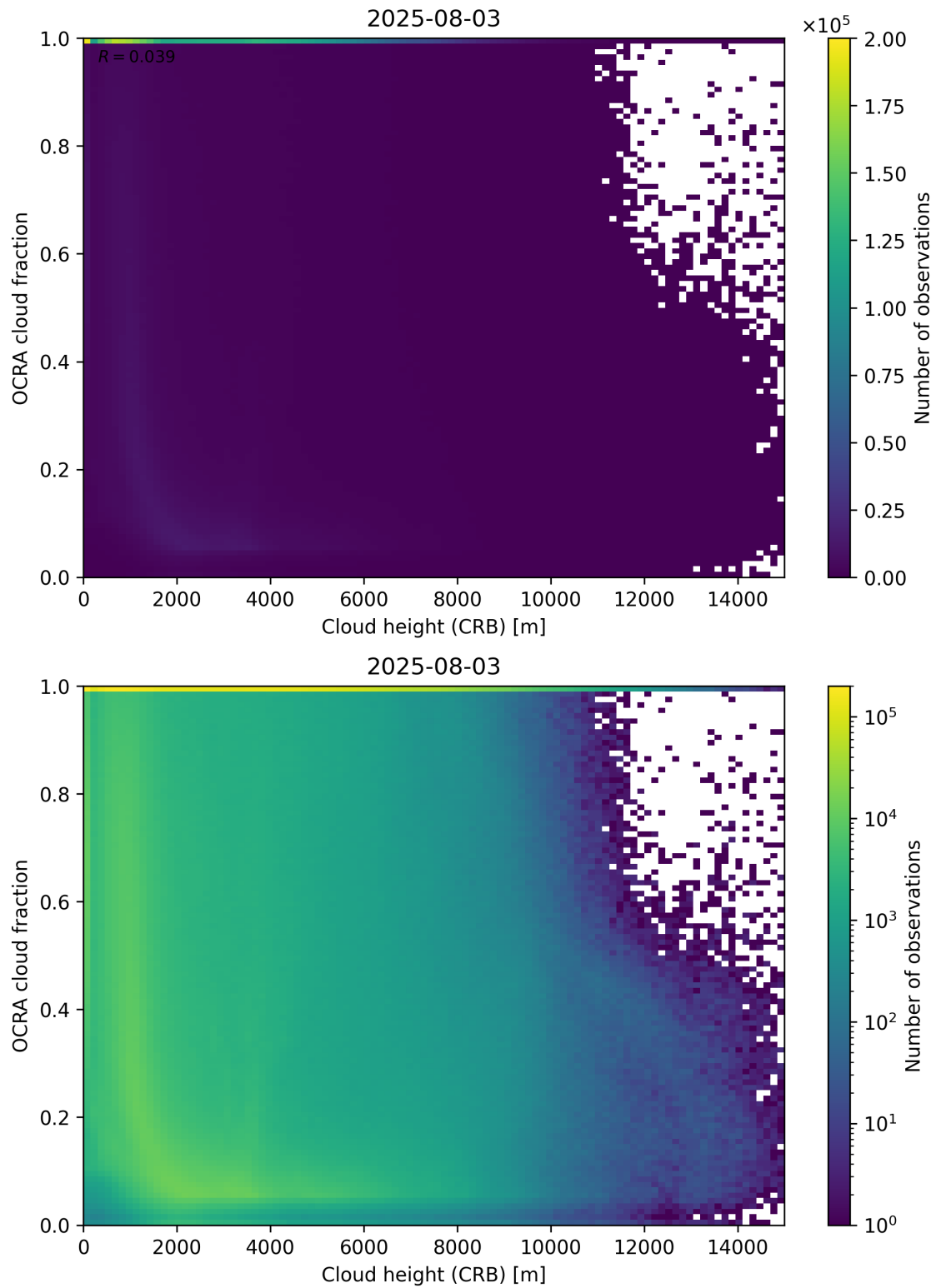
Figure 81: Scatter density plot of “Cloud height (CRB)” against “OCRA cloud fraction” for 2025-08-03 to 2025-08-04.
