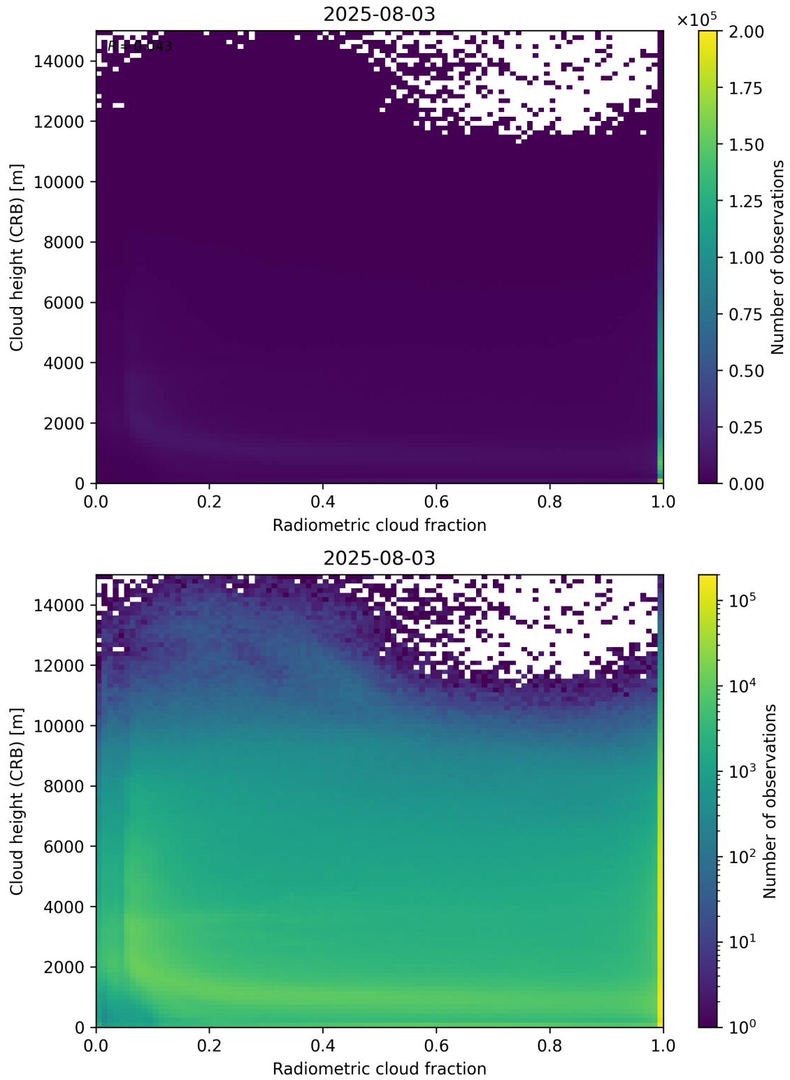
Figure 74: Scatter density plot of “Radiometric cloud fraction” against “Cloud height (CRB)” for 2025-08-03 to 2025-08-04.
