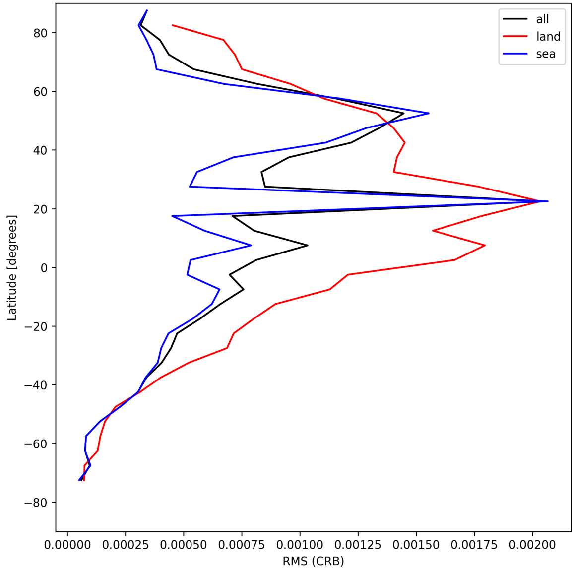
Figure 32: Zonal average of “RMS (CRB)” for 2025-08-03 to 2025-08-04.
