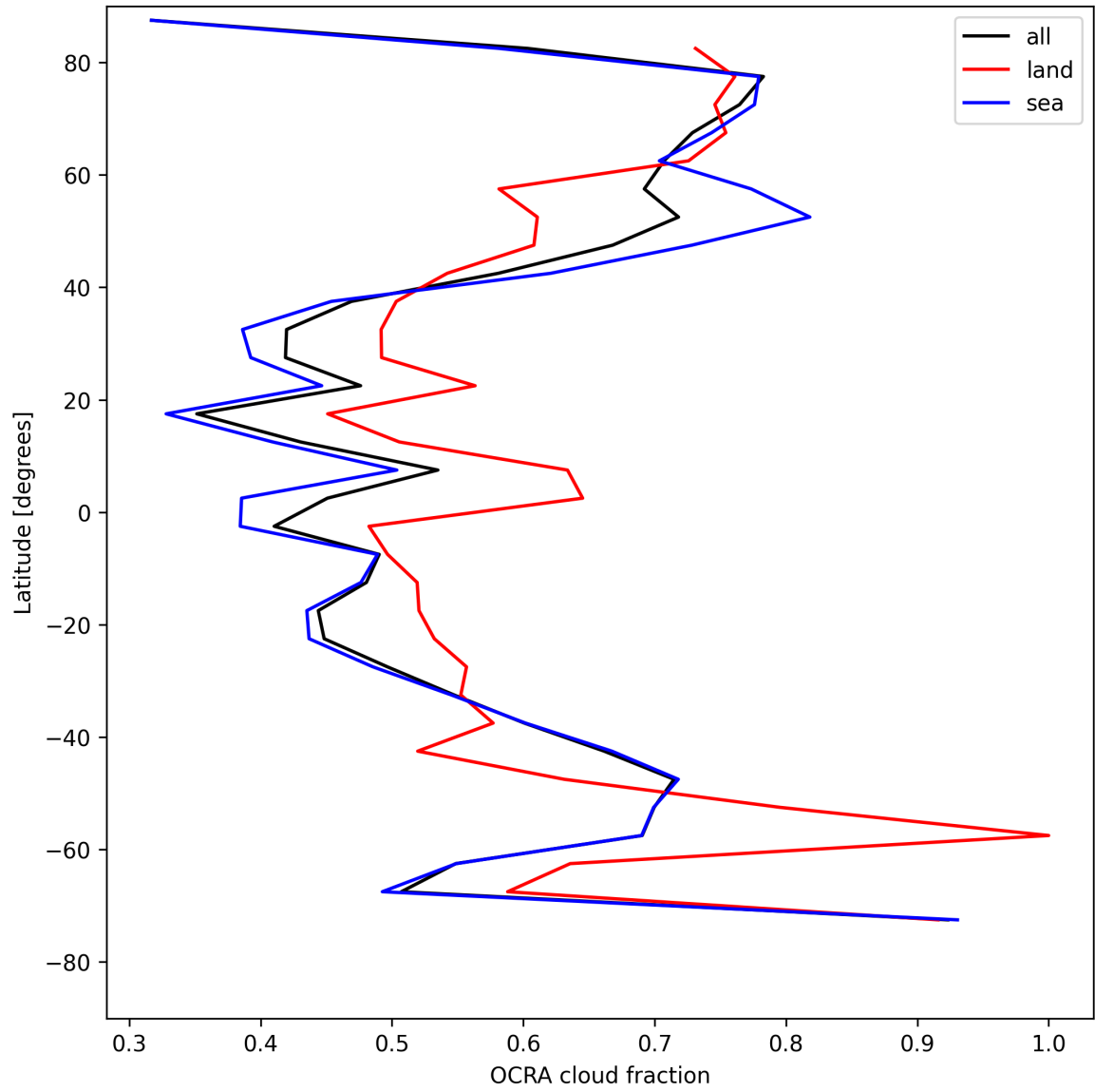
Figure 34: Zonal average of “OCRA cloud fraction” for 2025-08-03 to 2025-08-04.
