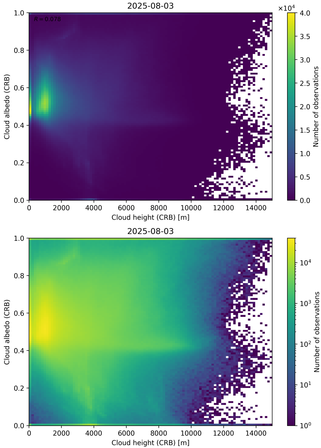
Figure 80: Scatter density plot of “Cloud height (CRB)” against “Cloud albedo (CRB)” for 2025-08-03 to 2025-08-04.
