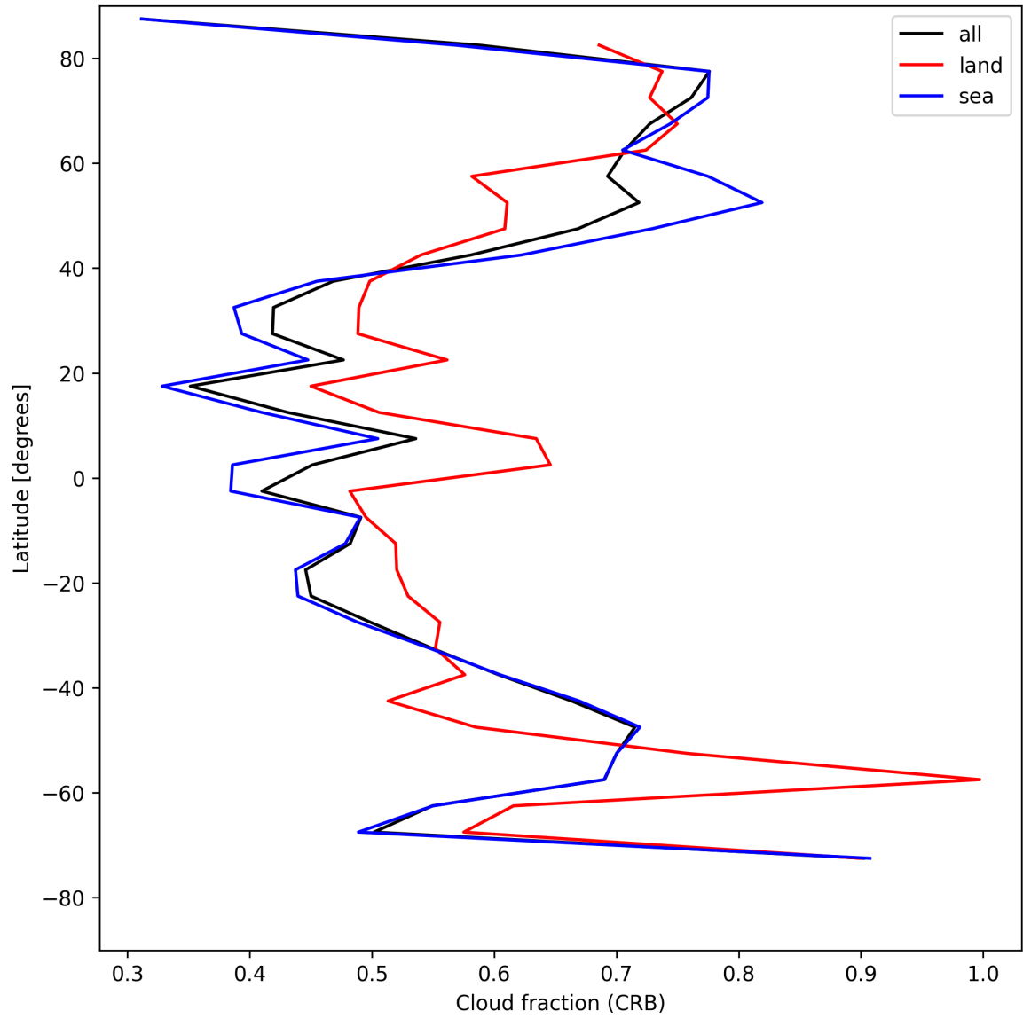
Figure 26: Zonal average of “Cloud fraction (CRB)” for 2025-08-03 to 2025-08-04.
