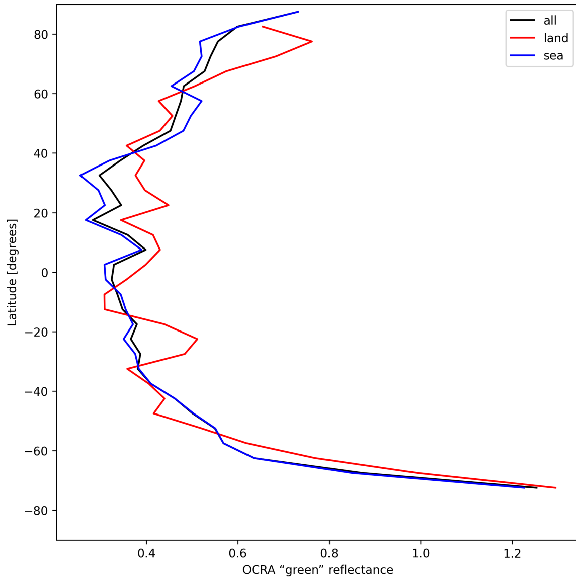
Figure 36: Zonal average of “OCRA “green” reflectance” for 2025-08-04 to 2025-08-05.
