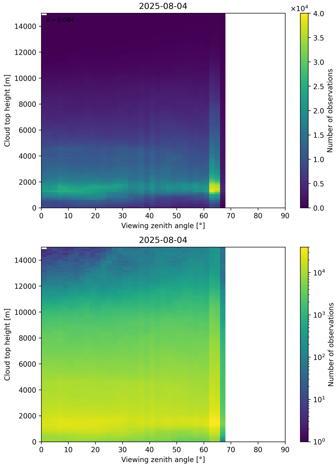
Figure 112: Scatter density plot of “Viewing zenith angle” against “Cloud top height” for 2025-08-04 to 2025-08-05.
