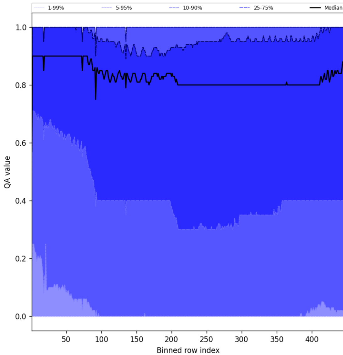
Figure 54: Along track statistics of “QA value” for 2025-08-04 to 2025-08-05
