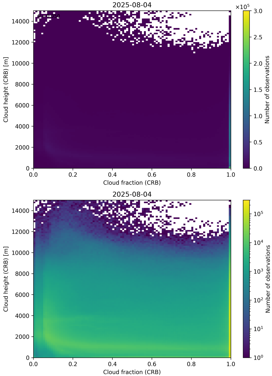
Figure 79: Scatter density plot of “Cloud fraction (CRB)” against “Cloud height (CRB)” for 2025-08-04 to 2025-08-05.
