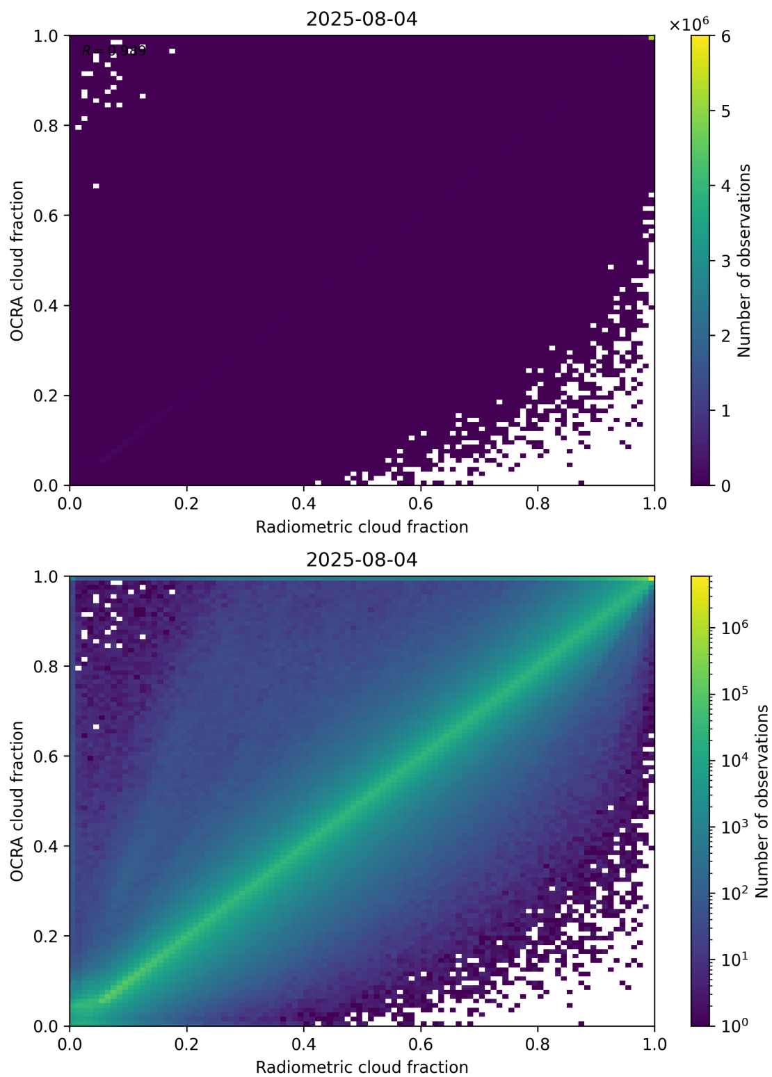
Figure 72: Scatter density plot of “Radiometric cloud fraction” against “OCRA cloud fraction” for 2025-08-04 to 2025-08-05.
