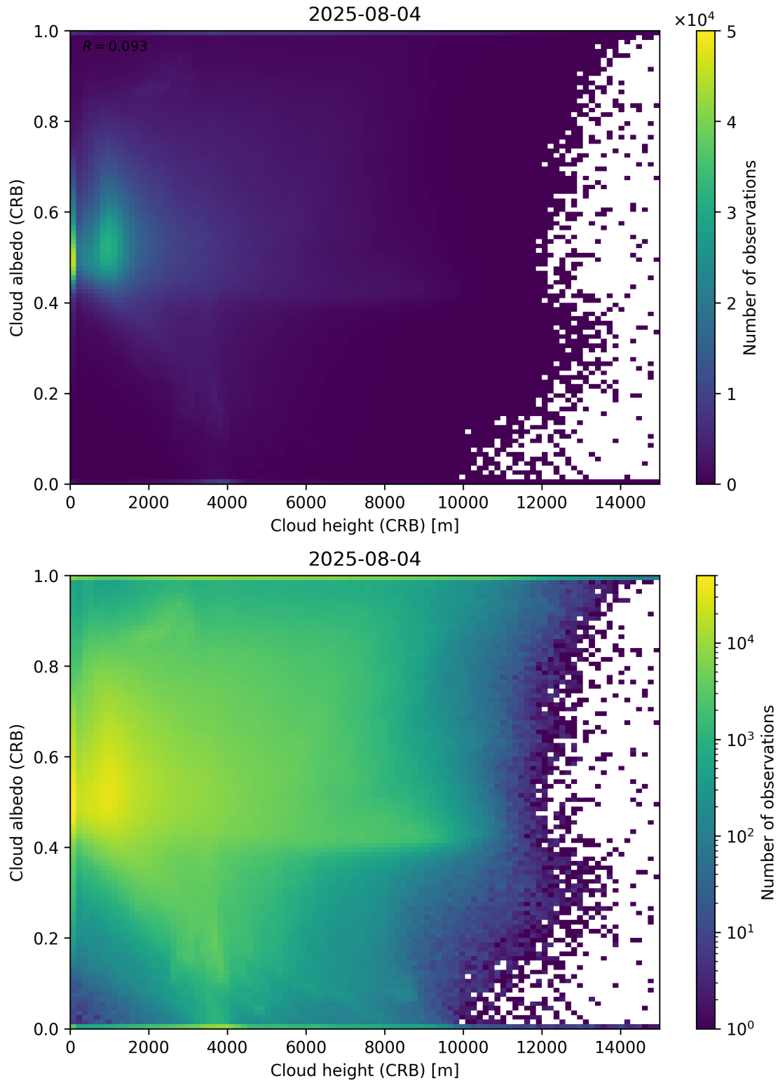
Figure 80: Scatter density plot of “Cloud height (CRB)” against “Cloud albedo (CRB)” for 2025-08-04 to 2025-08-05.
