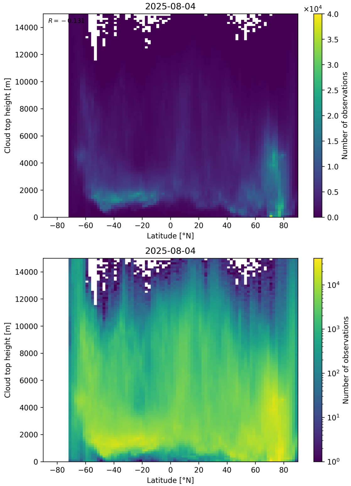
Figure 97: Scatter density plot of “Latitude” against “Cloud top height” for 2025-08-04 to 2025-08-05.
