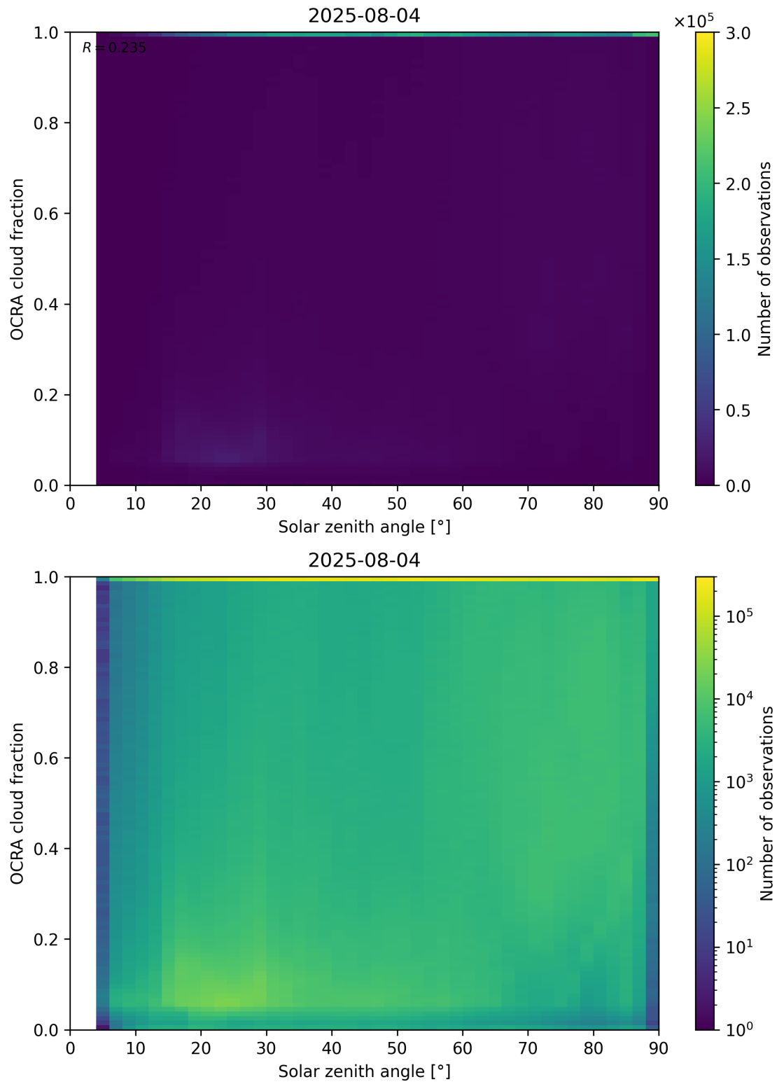
Figure 100: Scatter density plot of “Solar zenith angle” against “OCRA cloud fraction” for 2025-08-04 to 2025-08-05.
