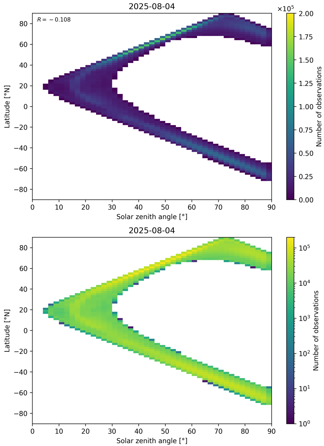
Figure 105: Scatter density plot of “Solar zenith angle” against “Latitude” for 2025-08-04 to 2025-08-05.
