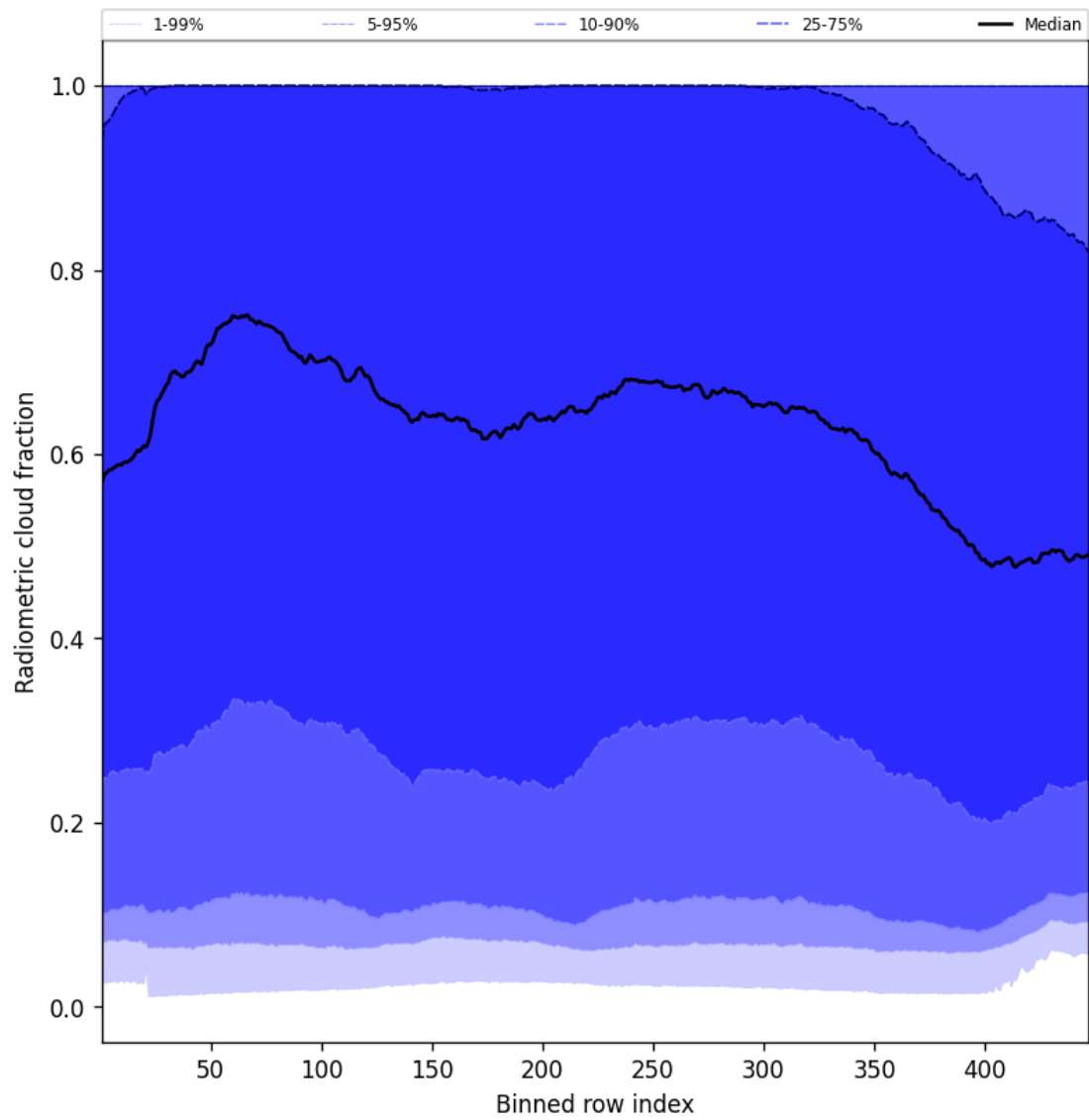
Figure 55: Along track statistics of “Radiometric cloud fraction” for 2025-08-04 to 2025-08-05
