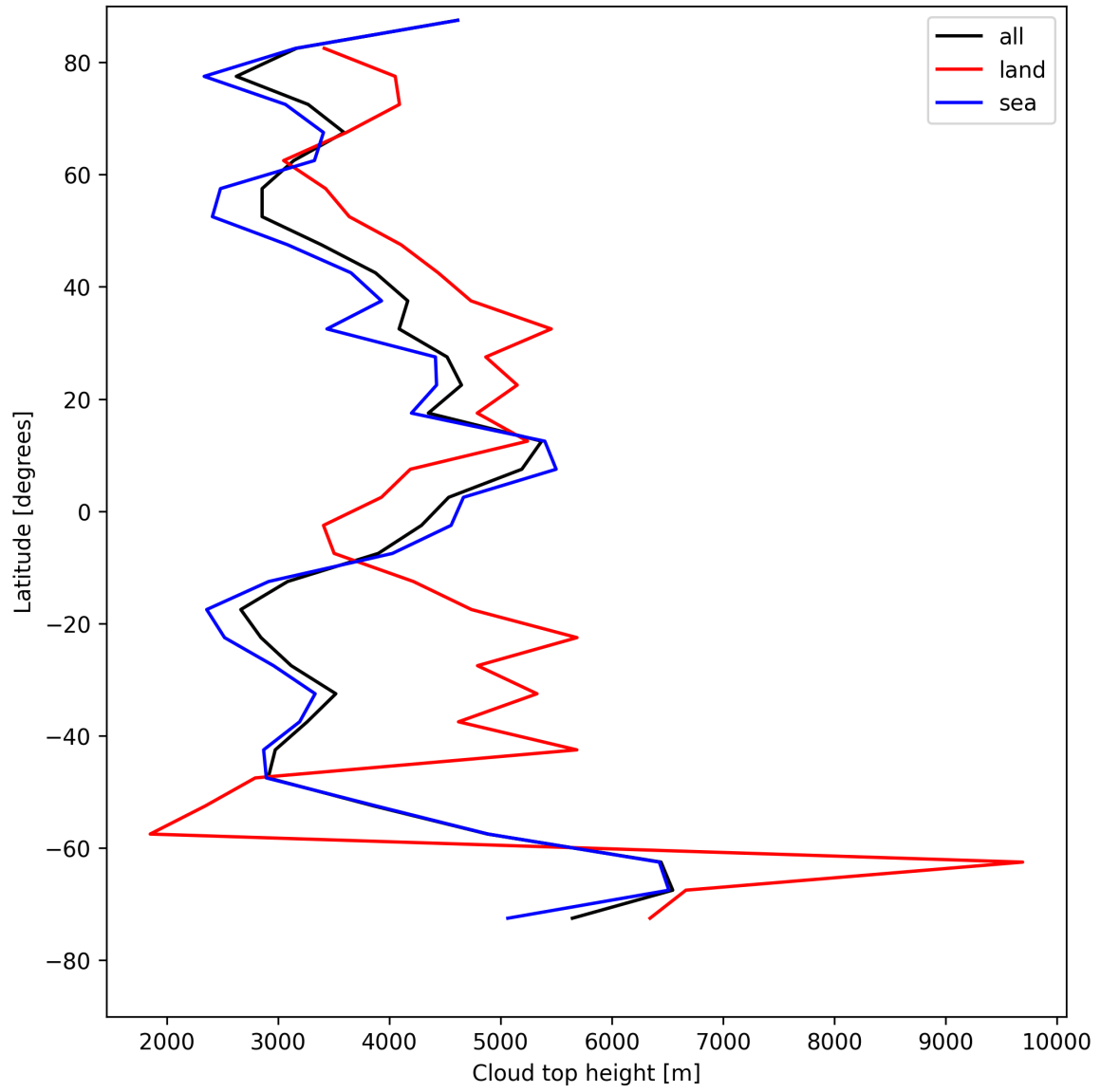
Figure 24: Zonal average of “Cloud top height” for 2025-08-04 to 2025-08-05.
