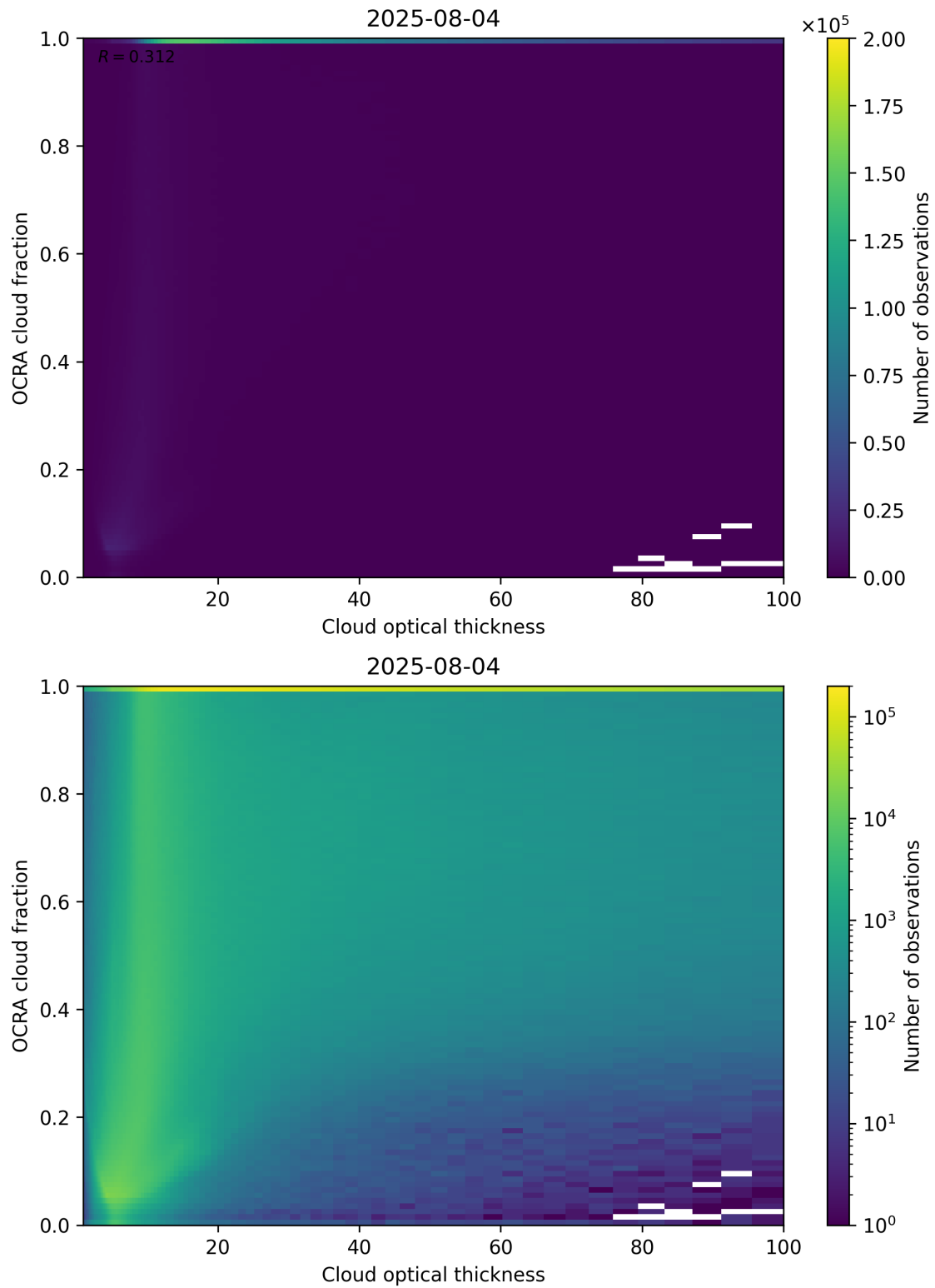
Figure 83: Scatter density plot of “Cloud optical thickness” against “OCRA cloud fraction” for 2025-08-04 to 2025-08-05.
