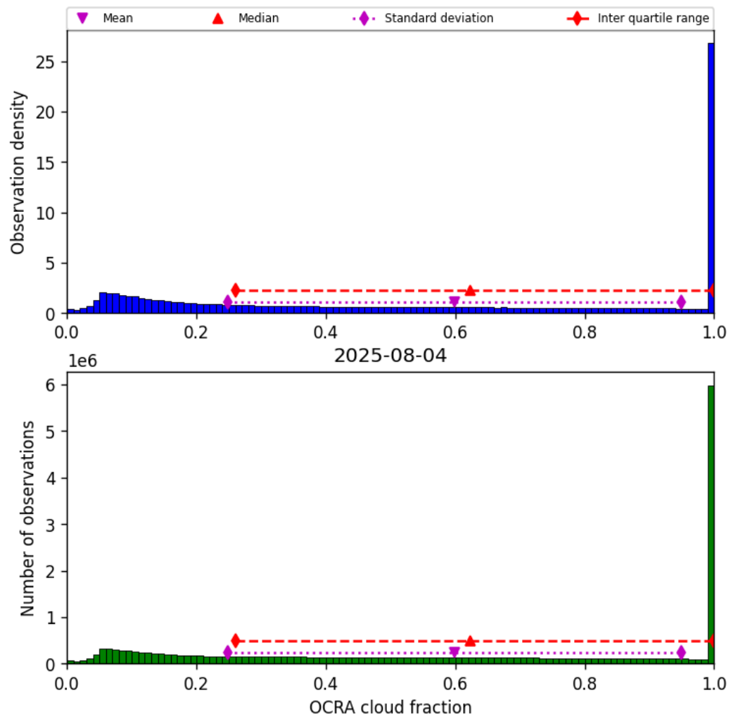
Figure 50: Histogram of “OCRA cloud fraction” for 2025-08-04 to 2025-08-05
