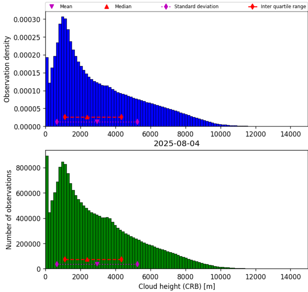
Figure 43: Histogram of “Cloud height (CRB)” for 2025-08-04 to 2025-08-05
