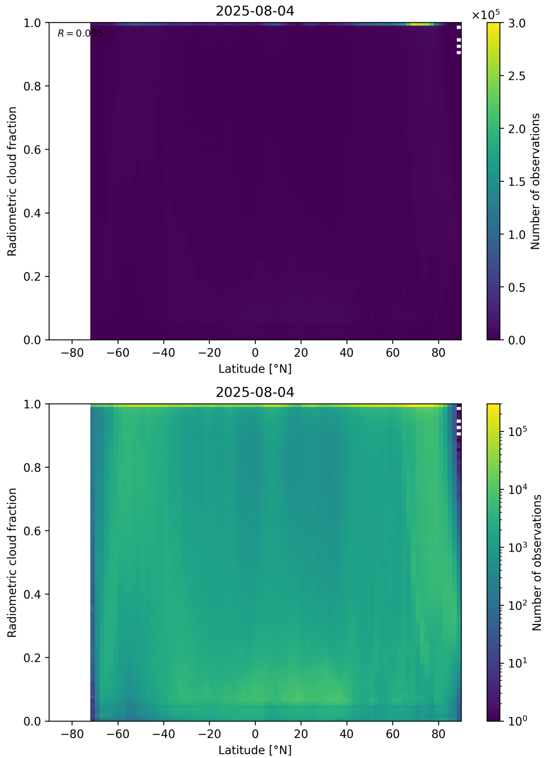
Figure 92: Scatter density plot of “Latitude” against “Radiometric cloud fraction” for 2025-08-04 to 2025-08-05.
