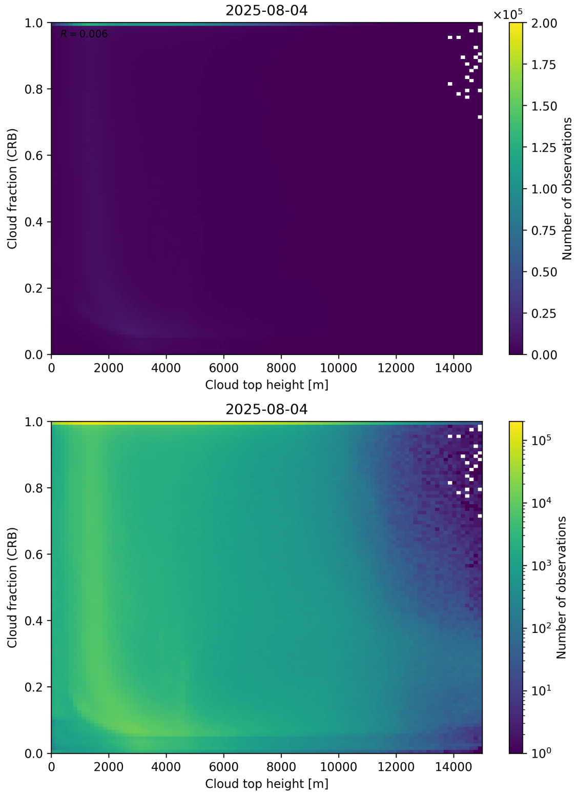
Figure 88: Scatter density plot of “Cloud top height” against “Cloud fraction (CRB)” for 2025-08-04 to 2025-08-05.
