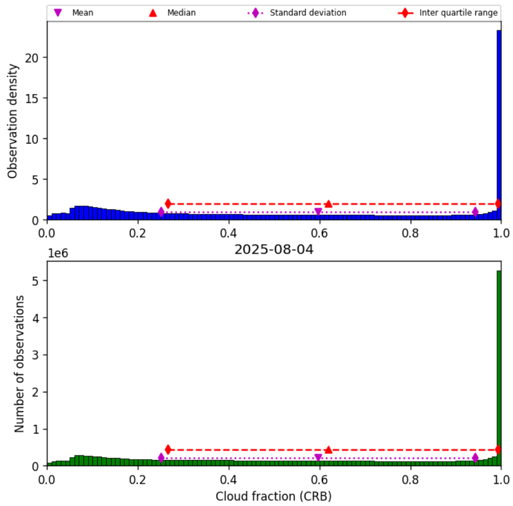
Figure 42: Histogram of “Cloud fraction (CRB)” for 2025-08-04 to 2025-08-05
