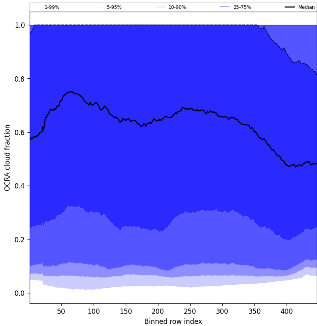
Figure 66: Along track statistics of “OCRA cloud fraction” for 2025-08-04 to 2025-08-05
