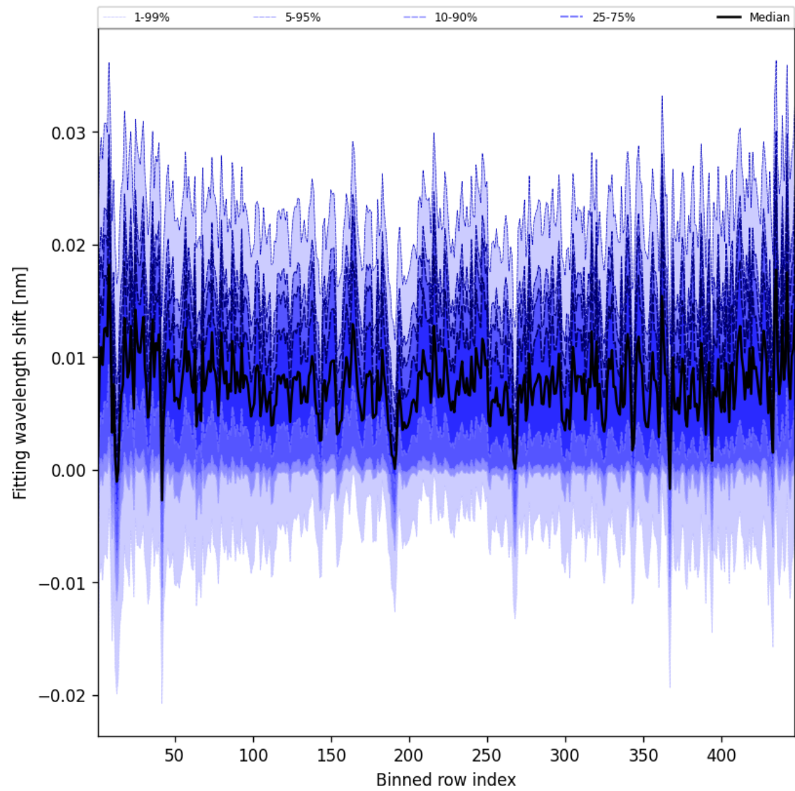
Figure 65: Along track statistics of “Fitting wavelength shift” for 2025-08-04 to 2025-08-05
