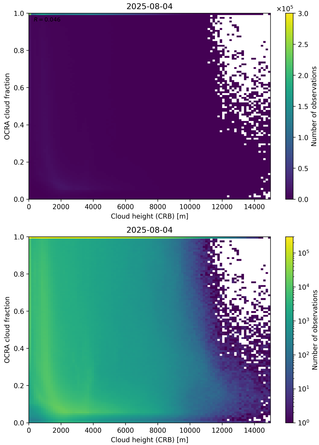
Figure 81: Scatter density plot of “Cloud height (CRB)” against “OCRA cloud fraction” for 2025-08-04 to 2025-08-05.
