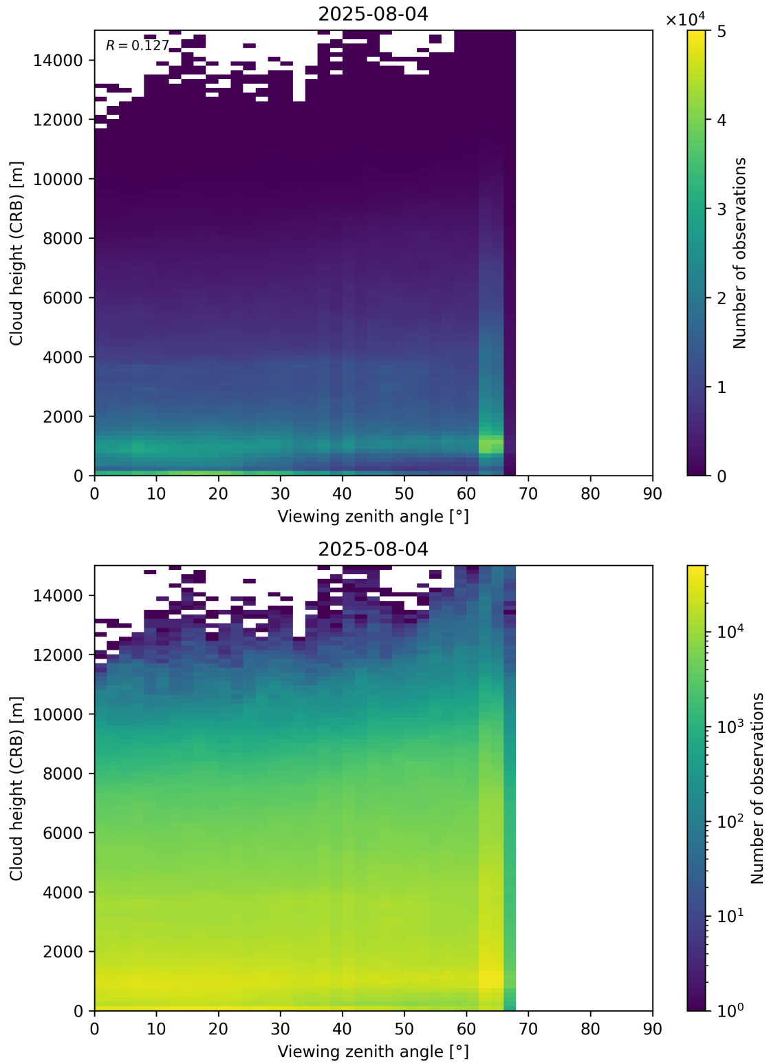
Figure 110: Scatter density plot of “Viewing zenith angle” against “Cloud height (CRB)” for 2025-08-04 to 2025-08-05.
