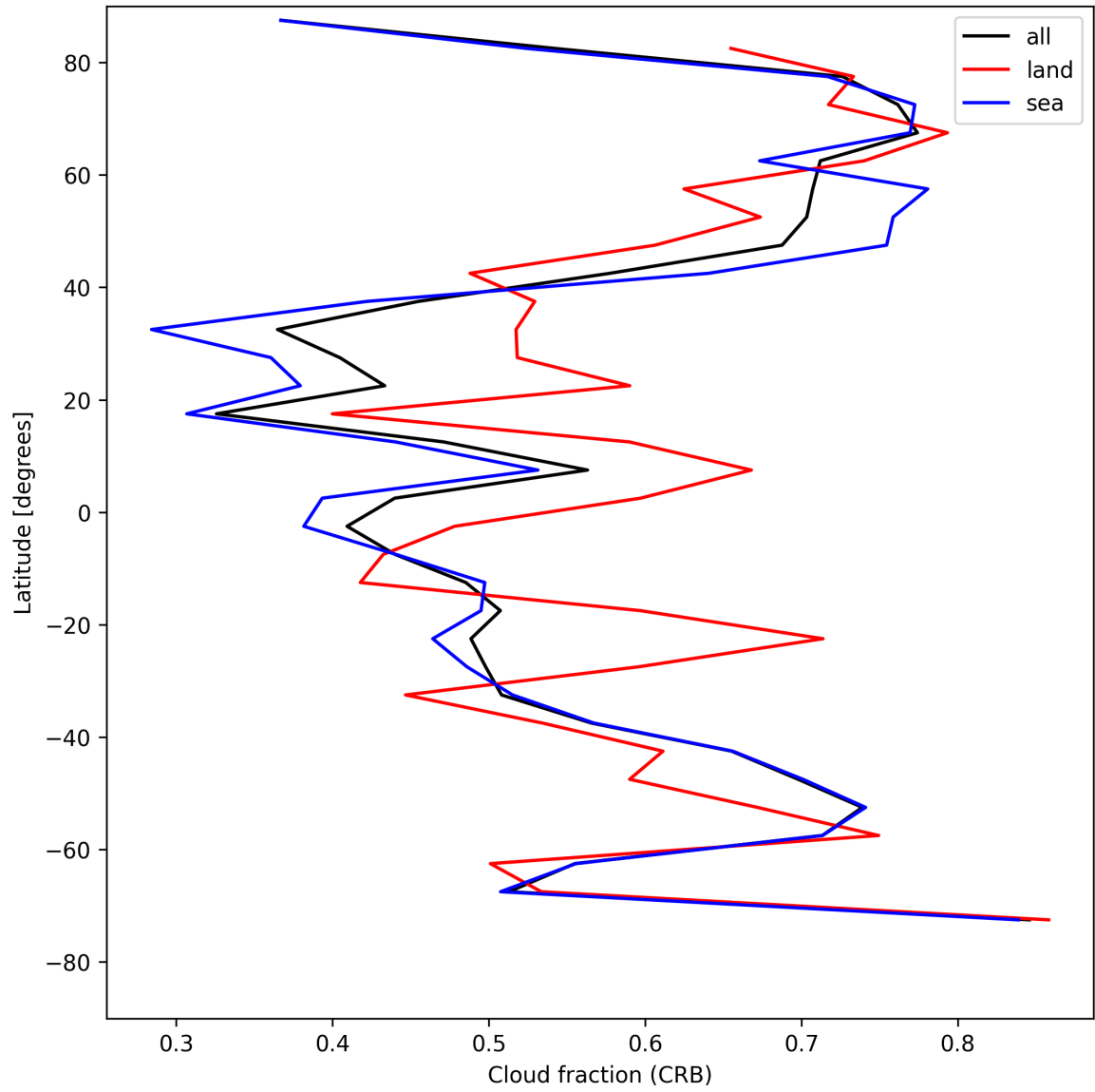
Figure 26: Zonal average of “Cloud fraction (CRB)” for 2025-08-04 to 2025-08-05.
