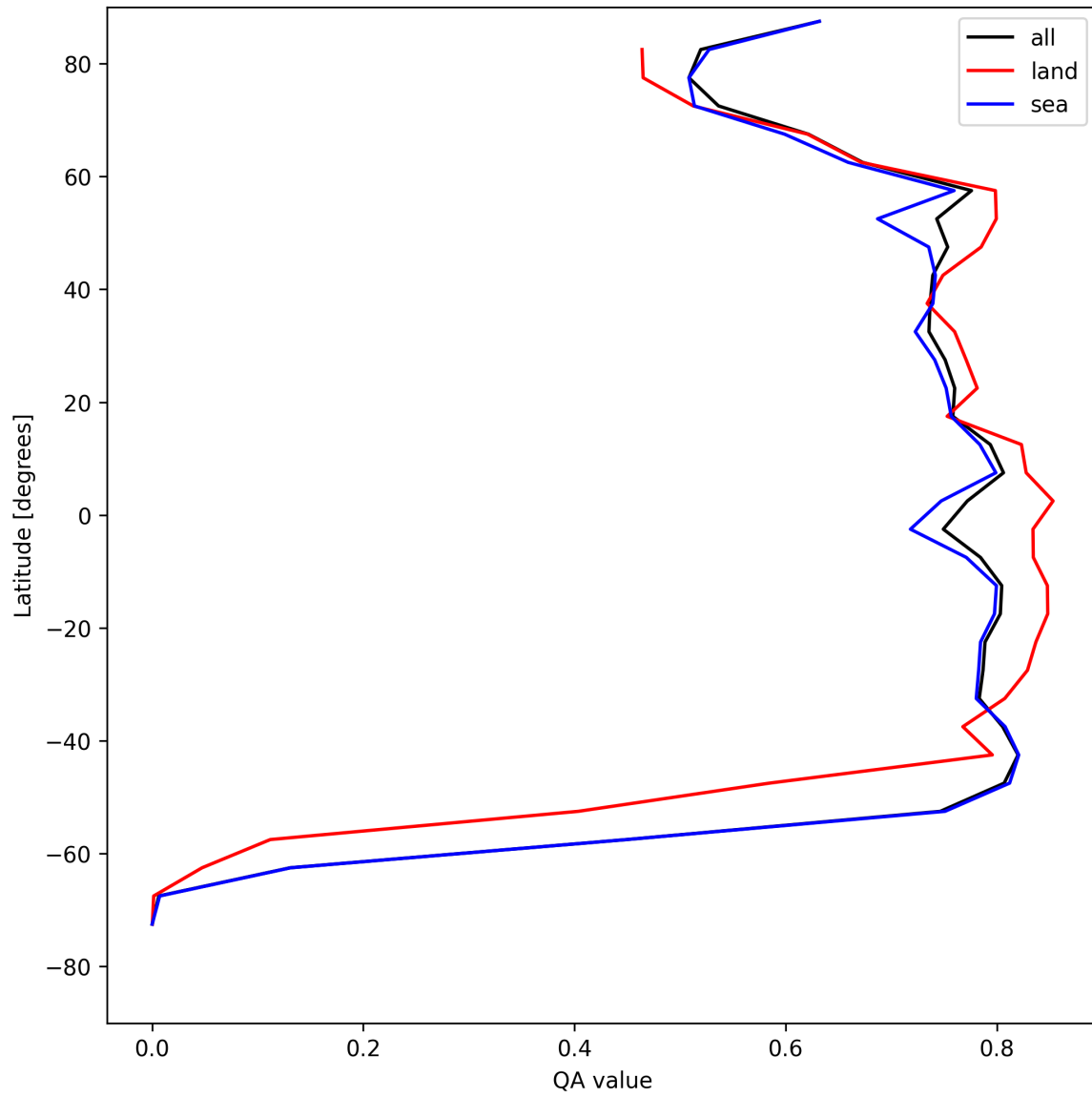
Figure 22: Zonal average of “QA value” for 2025-08-04 to 2025-08-05.
