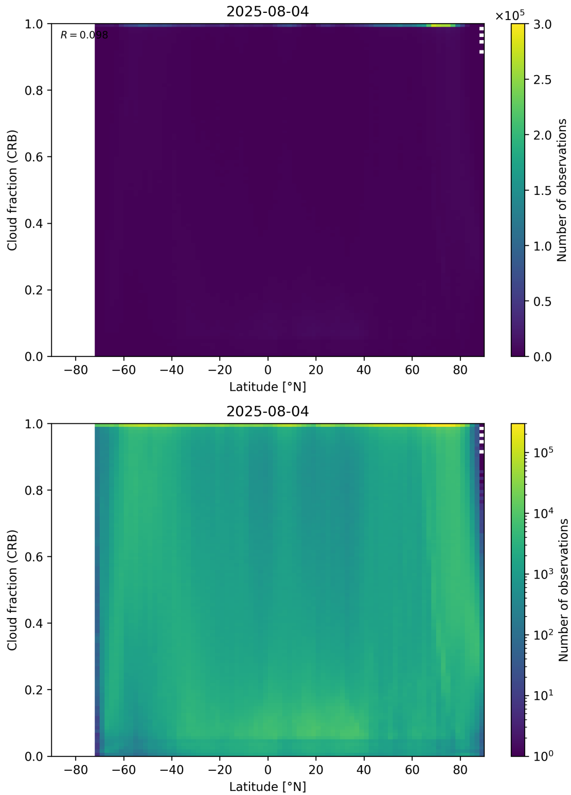
Figure 94: Scatter density plot of “Latitude” against “Cloud fraction (CRB)” for 2025-08-04 to 2025-08-05.
