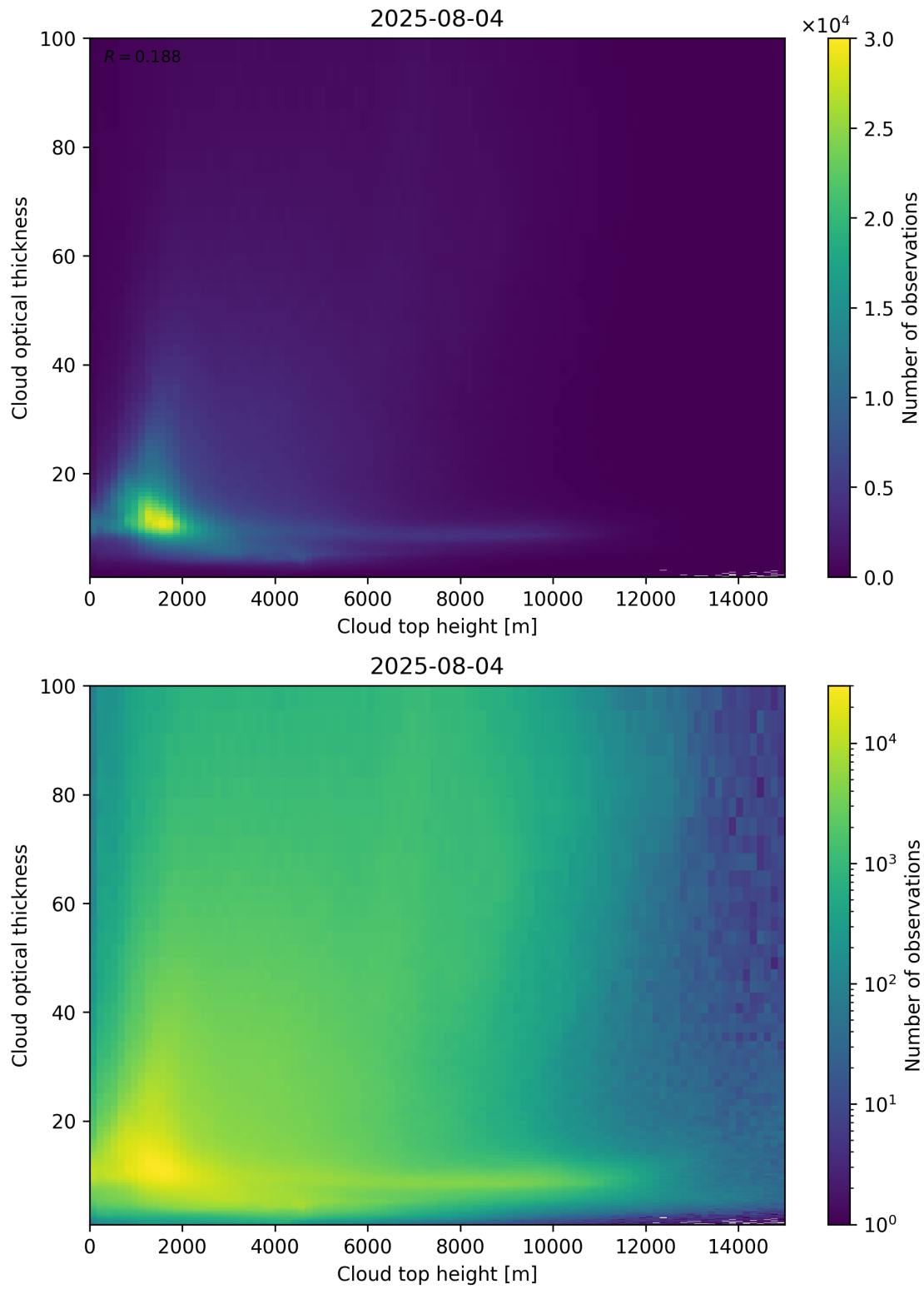
Figure 90: Scatter density plot of “Cloud top height” against “Cloud optical thickness” for 2025-08-04 to 2025-08-05.
