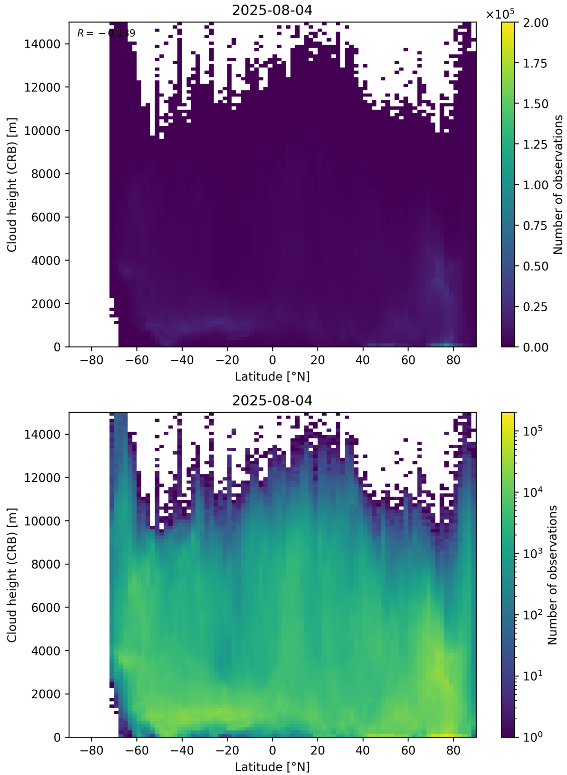
Figure 95: Scatter density plot of “Latitude” against “Cloud height (CRB)” for 2025-08-04 to 2025-08-05.
