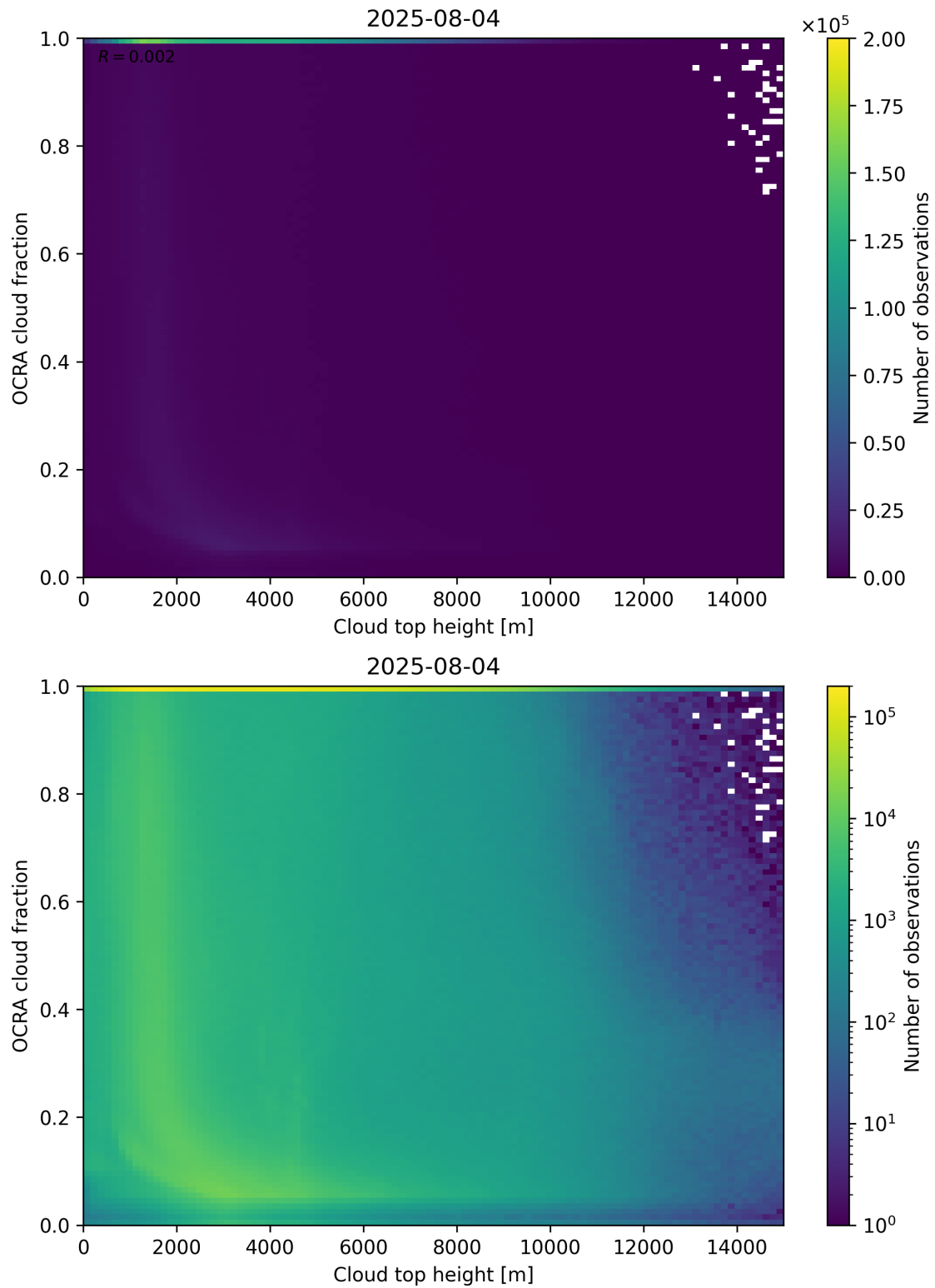
Figure 87: Scatter density plot of “Cloud top height” against “OCRA cloud fraction” for 2025-08-04 to 2025-08-05.
