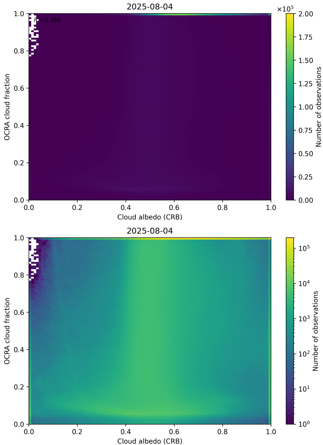
Figure 70: Scatter density plot of “Cloud albedo (CRB)” against “OCRA cloud fraction” for 2025-08-04 to 2025-08-05.
