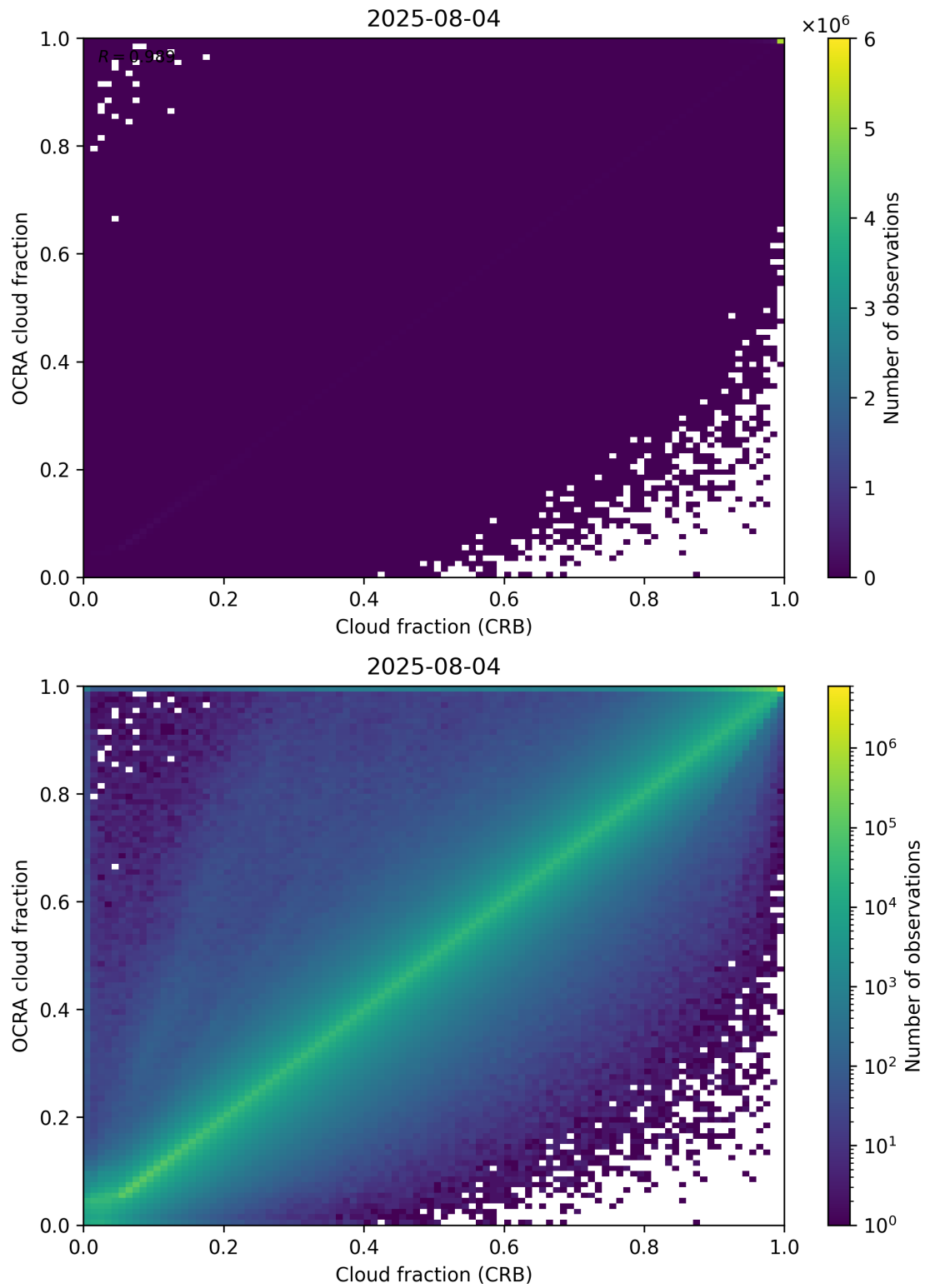
Figure 78: Scatter density plot of “Cloud fraction (CRB)” against “OCRA cloud fraction” for 2025-08-04 to 2025-08-05.
