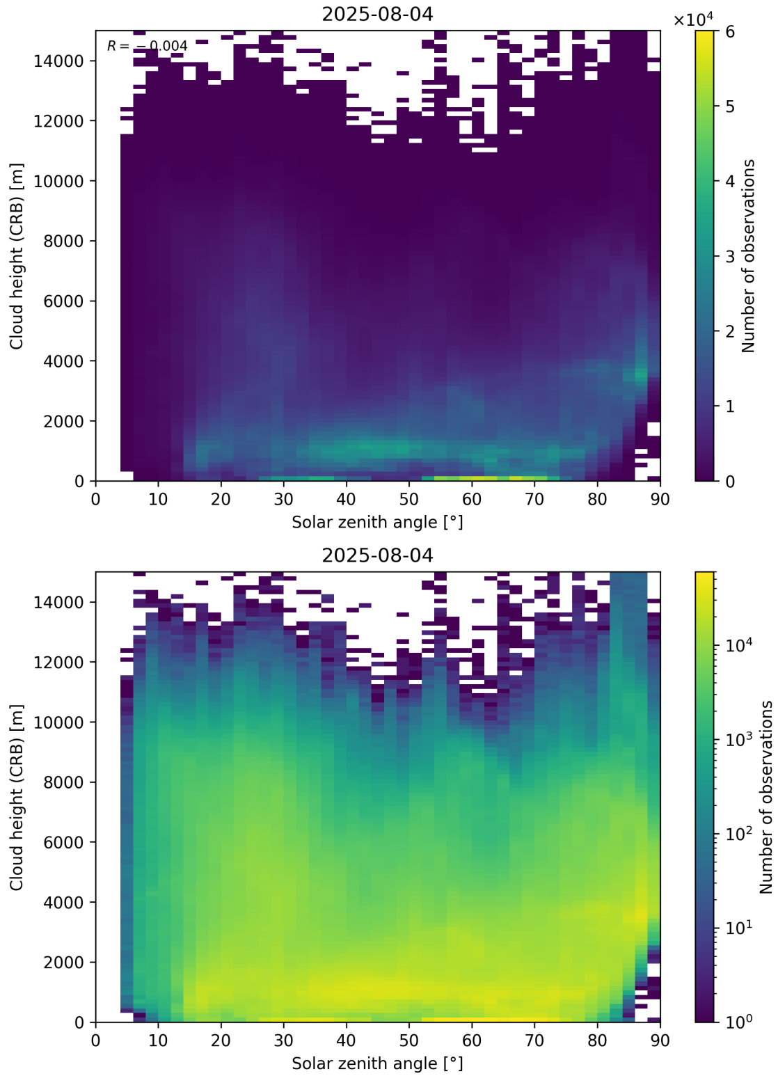
Figure 102: Scatter density plot of “Solar zenith angle” against “Cloud height (CRB)” for 2025-08-04 to 2025-08-05.
