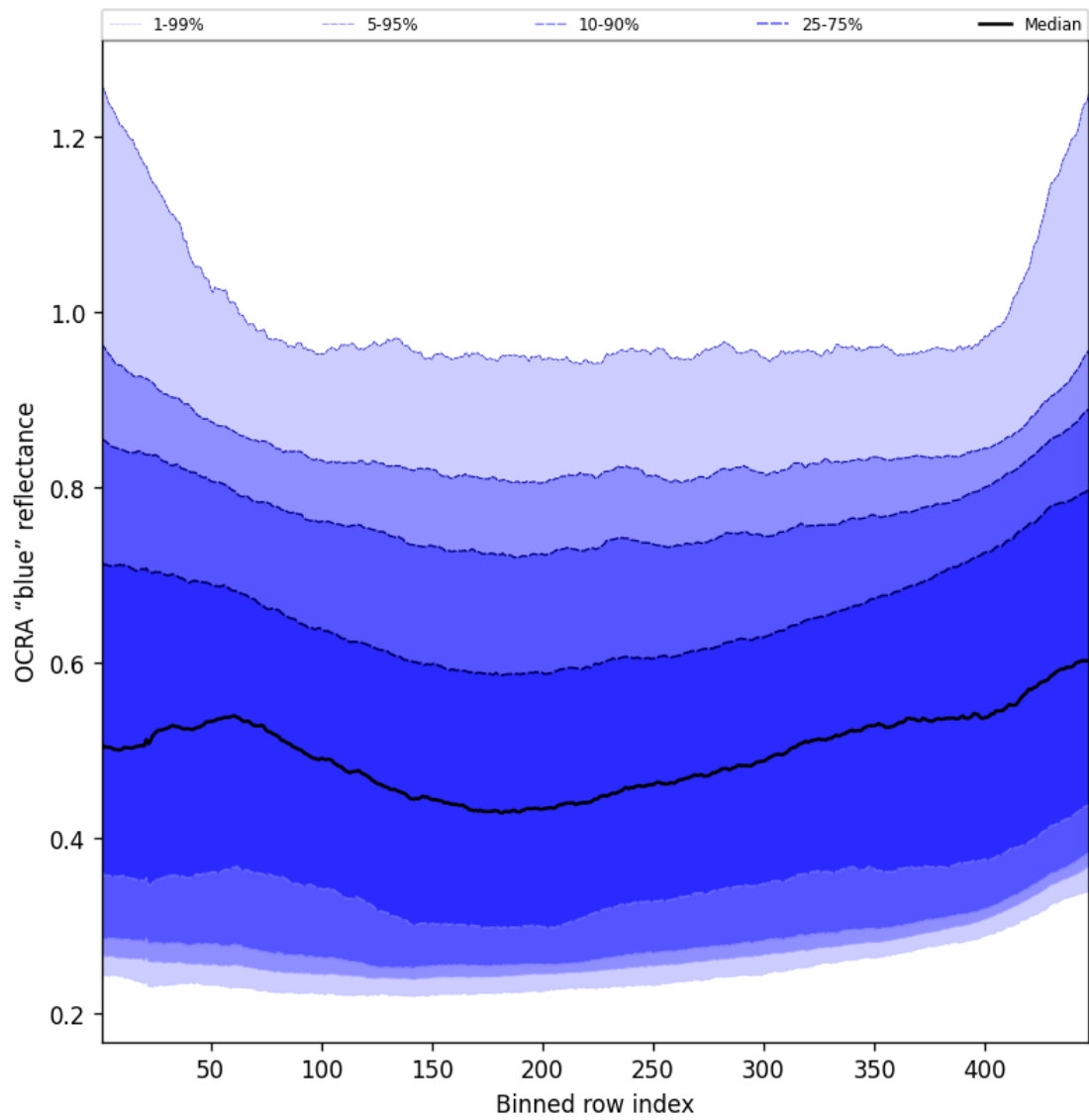
Figure 67: Along track statistics of “OCRA “blue” reflectance” for 2025-08-04 to 2025-08-05
