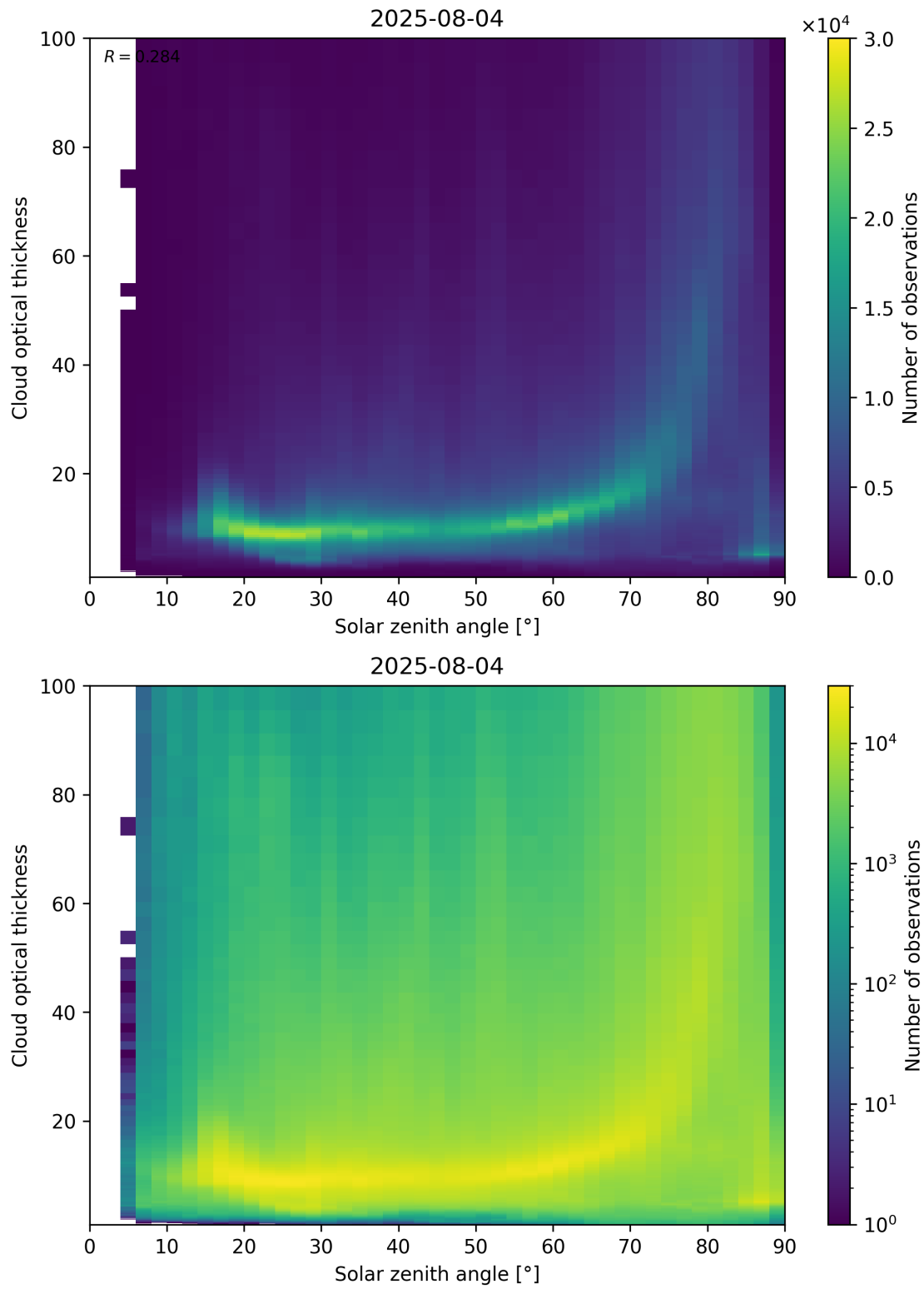
Figure 103: Scatter density plot of “Solar zenith angle” against “Cloud optical thickness” for 2025-08-04 to 2025-08-05.
