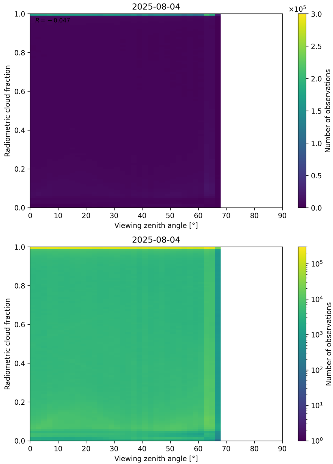
Figure 107: Scatter density plot of “Viewing zenith angle” against “Radiometric cloud fraction” for 2025-08-04 to 2025-08-05.
