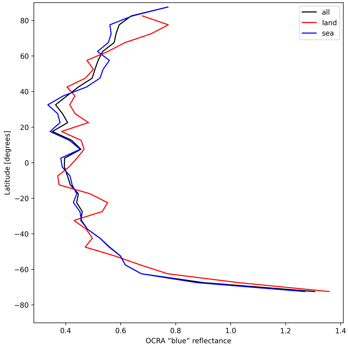
Figure 35: Zonal average of “OCRA “blue” reflectance” for 2025-08-04 to 2025-08-05.
