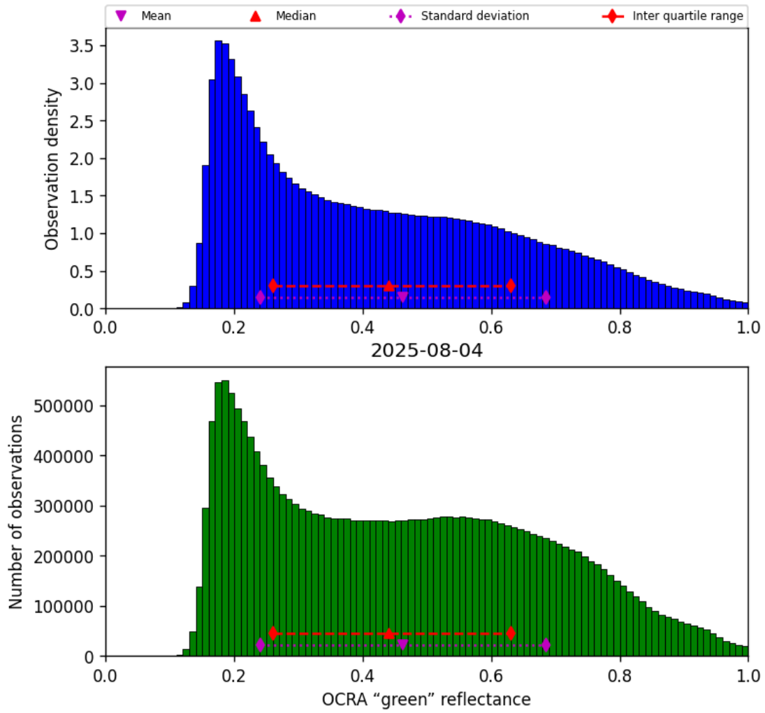
Figure 52: Histogram of “OCRA “green” reflectance” for 2025-08-04 to 2025-08-05
