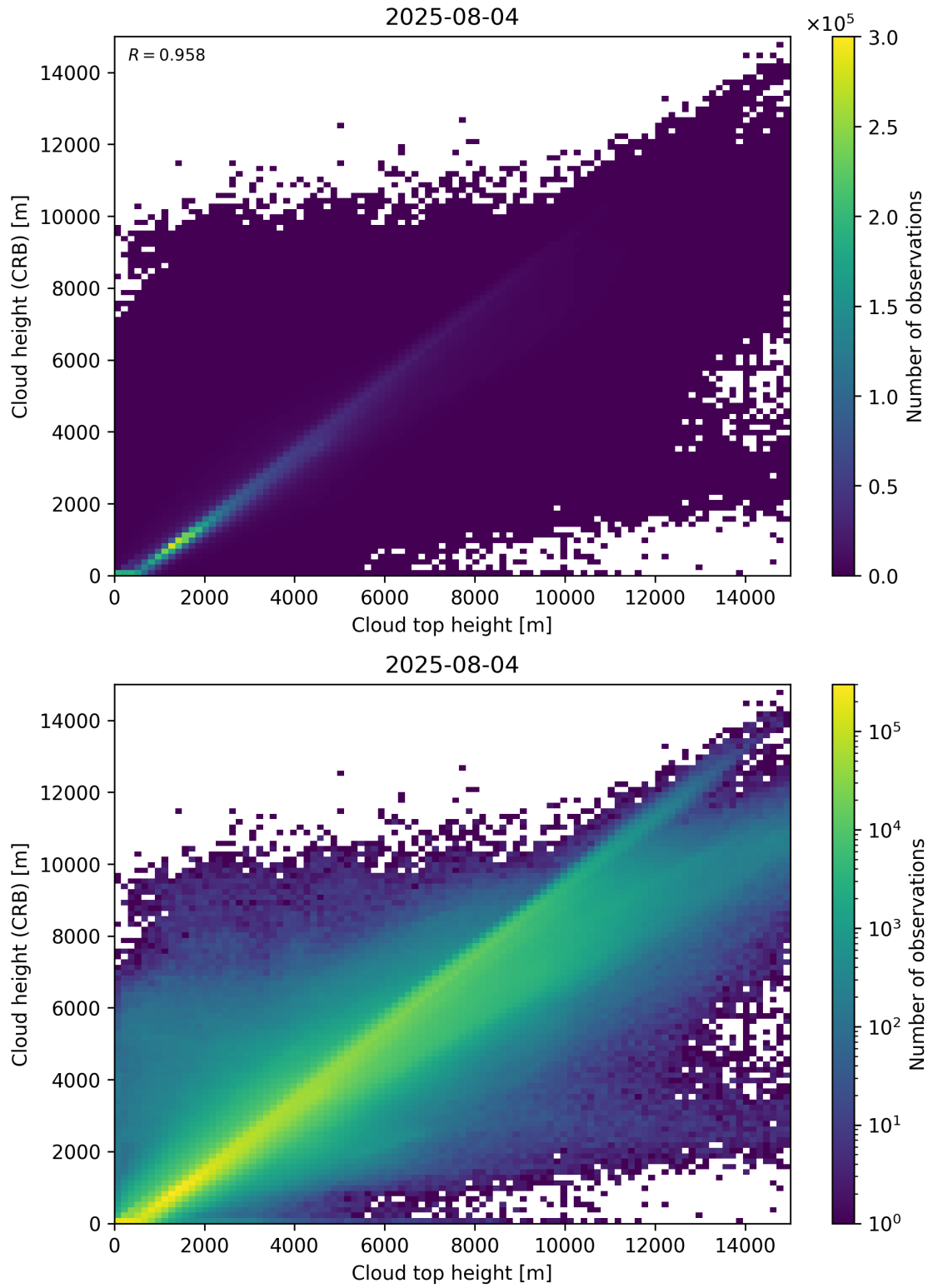
Figure 89: Scatter density plot of “Cloud top height” against “Cloud height (CRB)” for 2025-08-04 to 2025-08-05.
