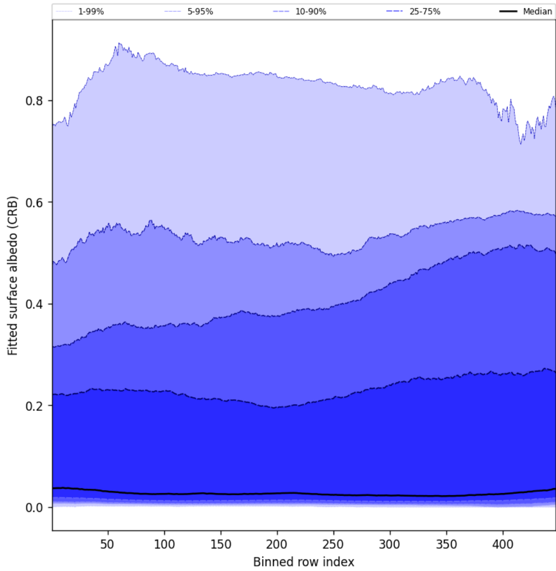
Figure 62: Along track statistics of “Fitted surface albedo (CRB)” for 2025-08-04 to 2025-08-05
