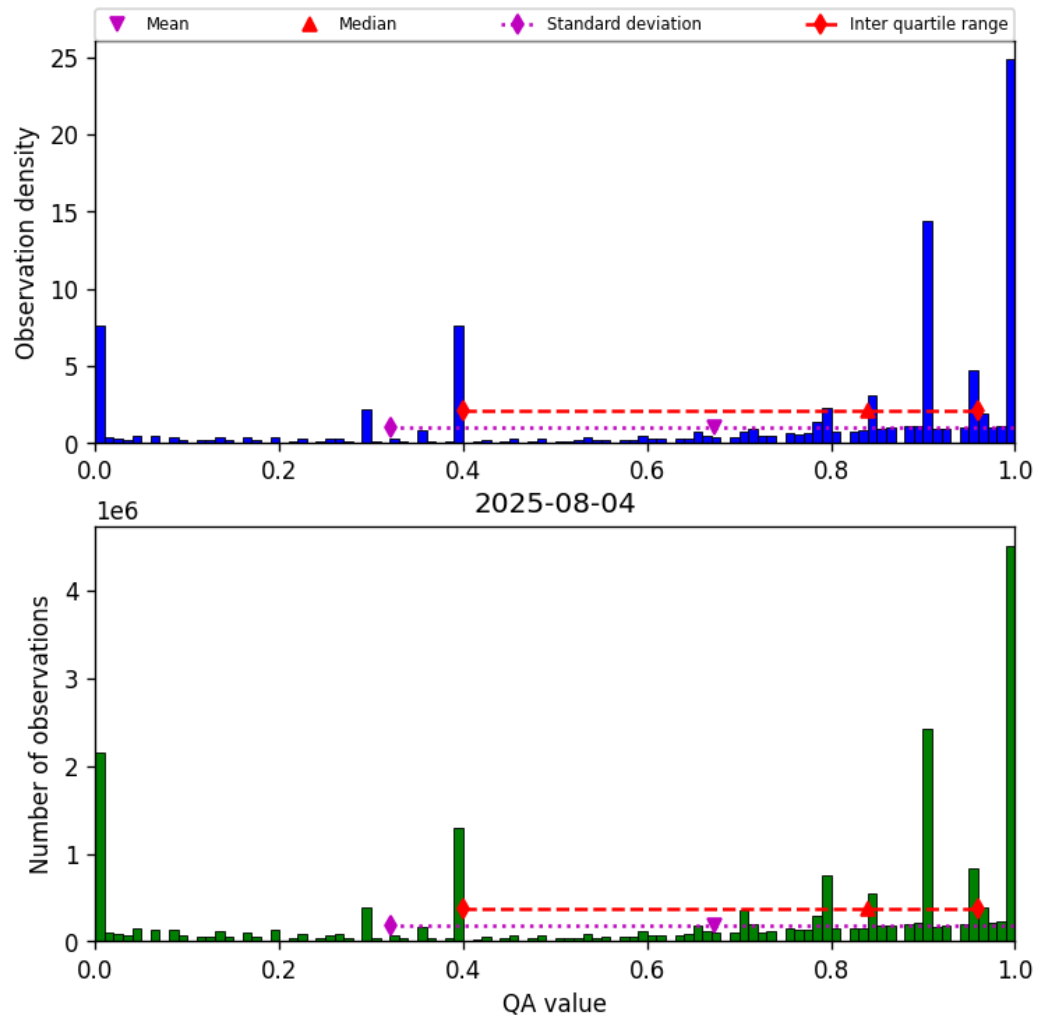
Figure 38: Histogram of “QA value” for 2025-08-04 to 2025-08-05
