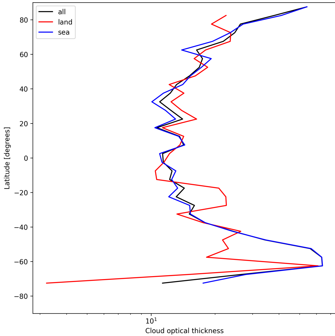
Figure 25: Zonal average of “Cloud optical thickness” for 2025-08-04 to 2025-08-05.
