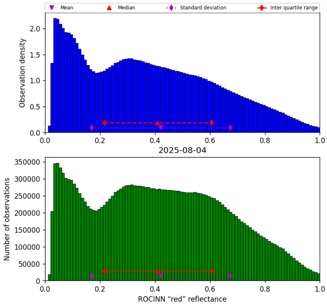
Figure 53: Histogram of “ROCINN “red” reflectance” for 2025-08-04 to 2025-08-05
