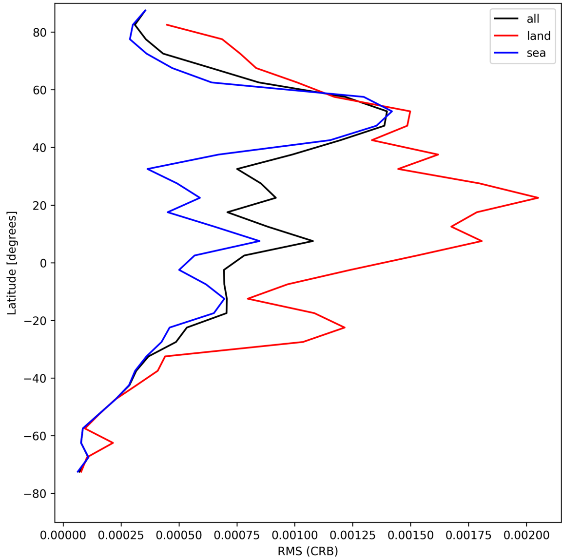
Figure 32: Zonal average of “RMS (CRB)” for 2025-08-04 to 2025-08-05.
