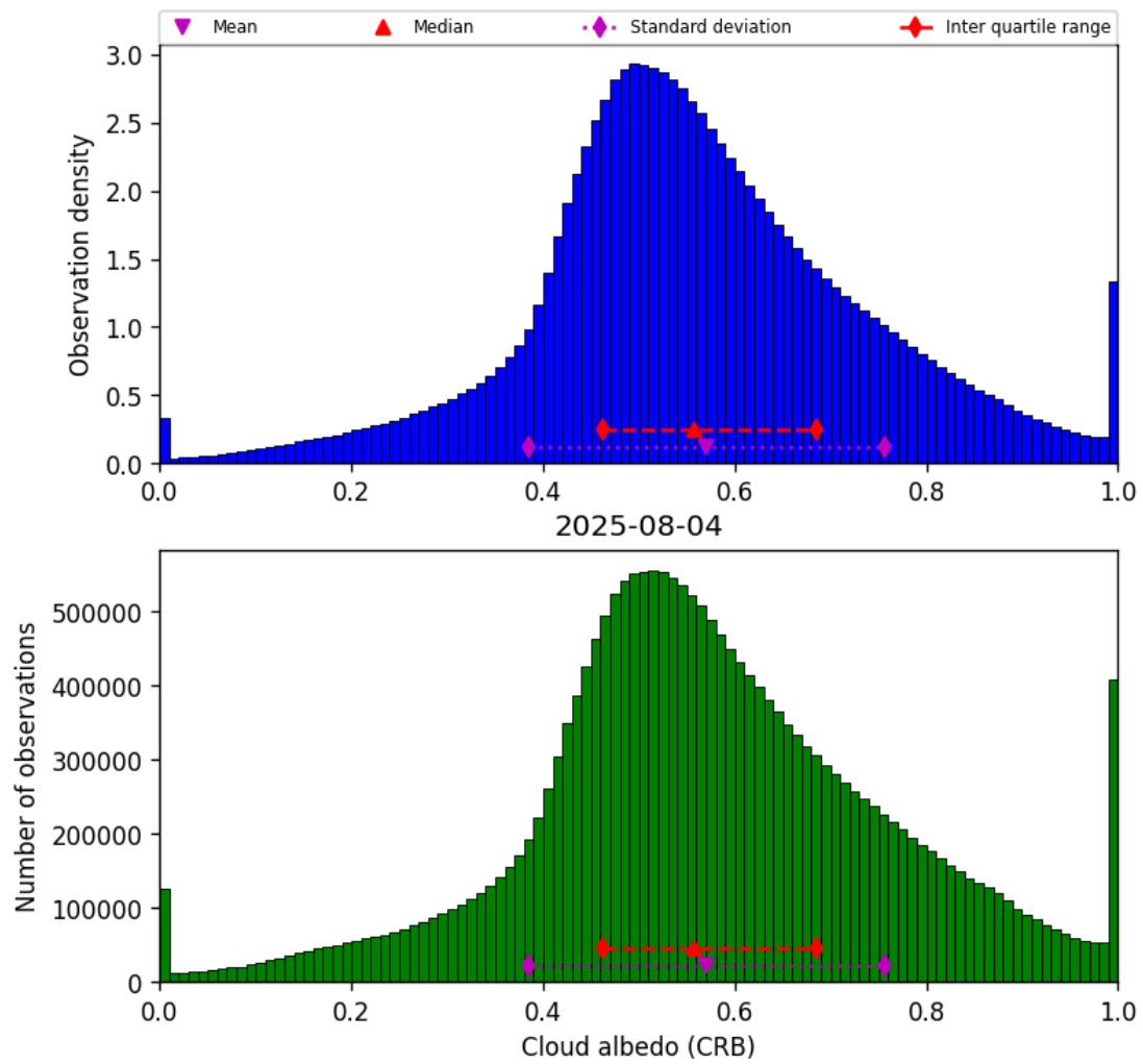
Figure 44: Histogram of “Cloud albedo (CRB)” for 2025-08-04 to 2025-08-05
