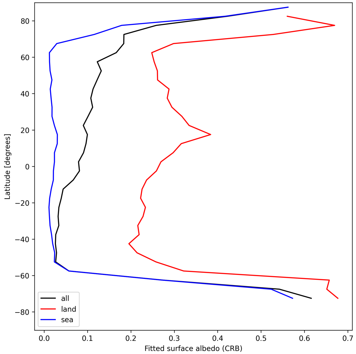
Figure 30: Zonal average of “Fitted surface albedo (CRB)” for 2025-08-04 to 2025-08-05.
