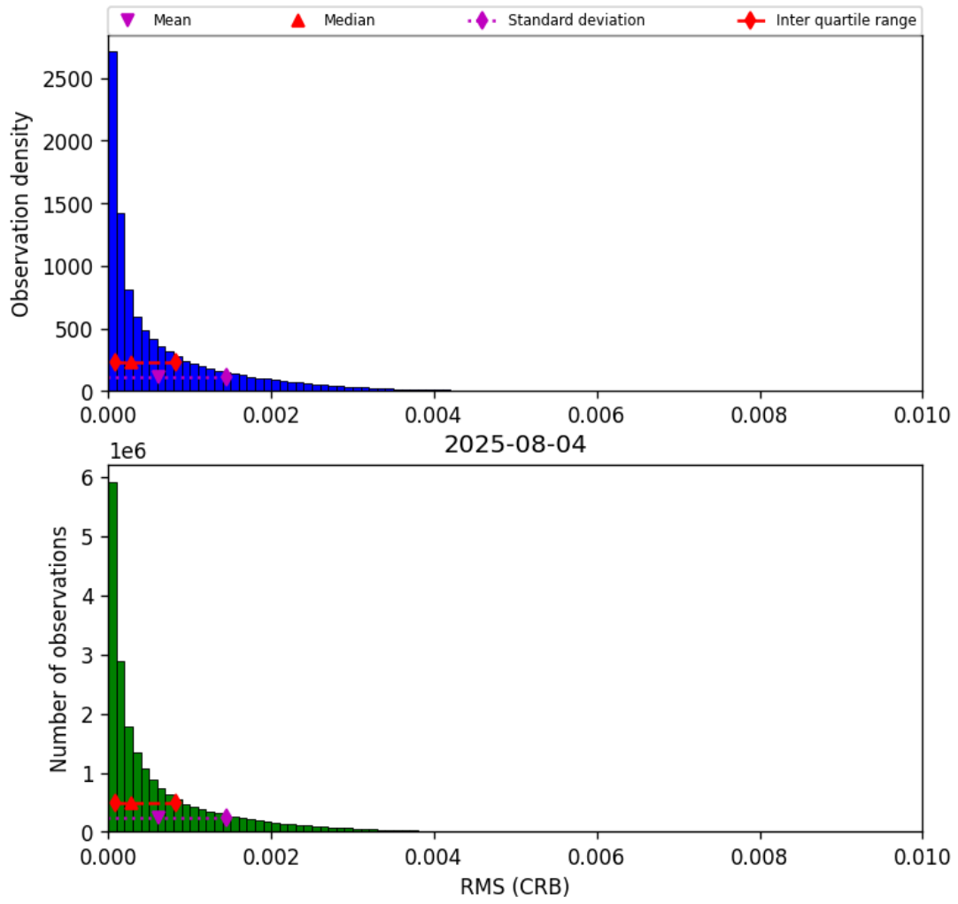
Figure 48: Histogram of “RMS (CRB)” for 2025-08-04 to 2025-08-05
