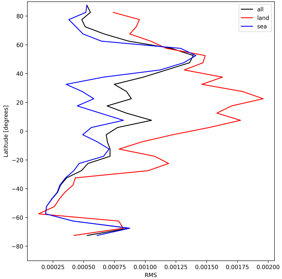
Figure 31: Zonal average of “RMS” for 2025-08-04 to 2025-08-05.
