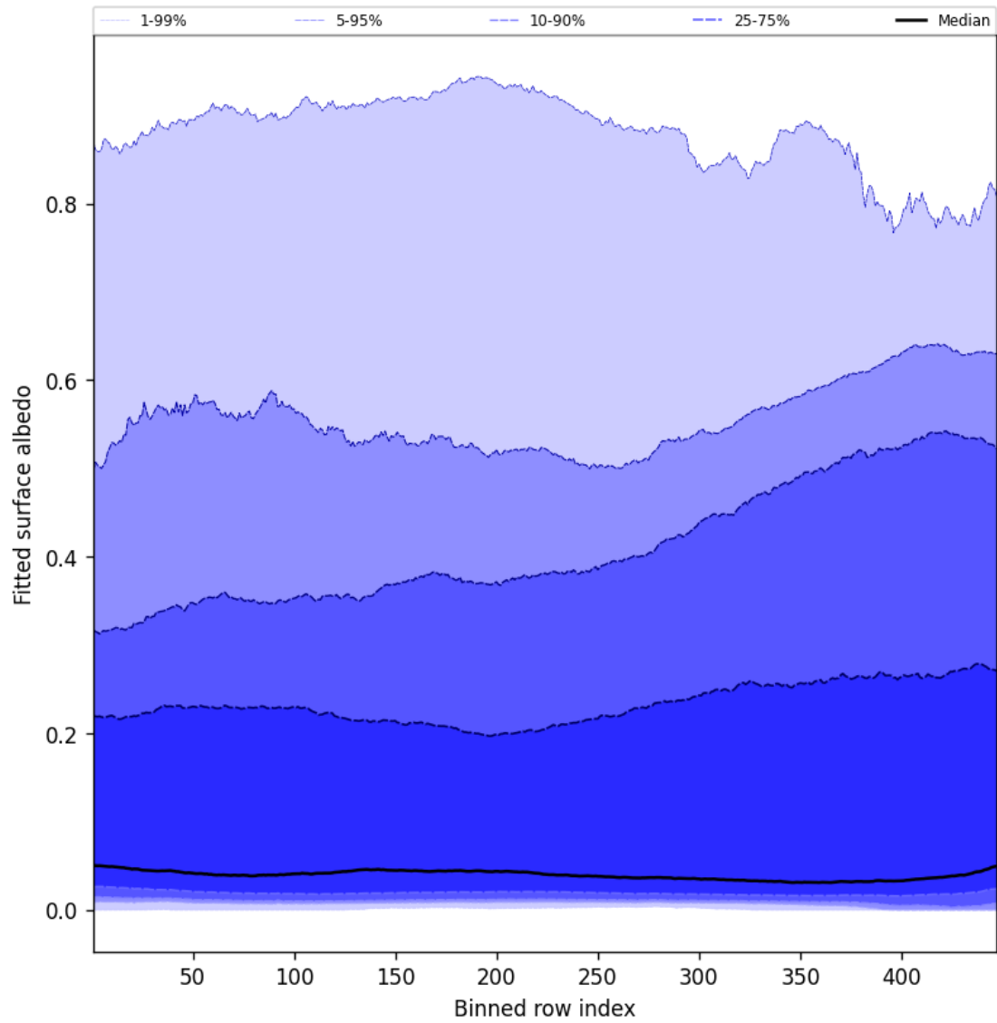
Figure 61: Along track statistics of “Fitted surface albedo” for 2025-08-04 to 2025-08-05
