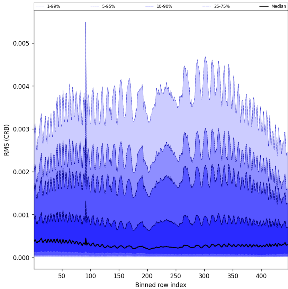
Figure 64: Along track statistics of “RMS (CRB)” for 2025-08-04 to 2025-08-05
