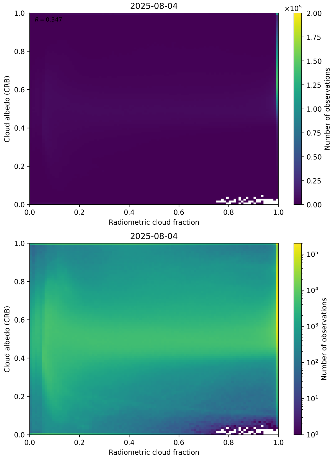
Figure 71: Scatter density plot of “Radiometric cloud fraction” against “Cloud albedo (CRB)” for 2025-08-04 to 2025-08-05.
