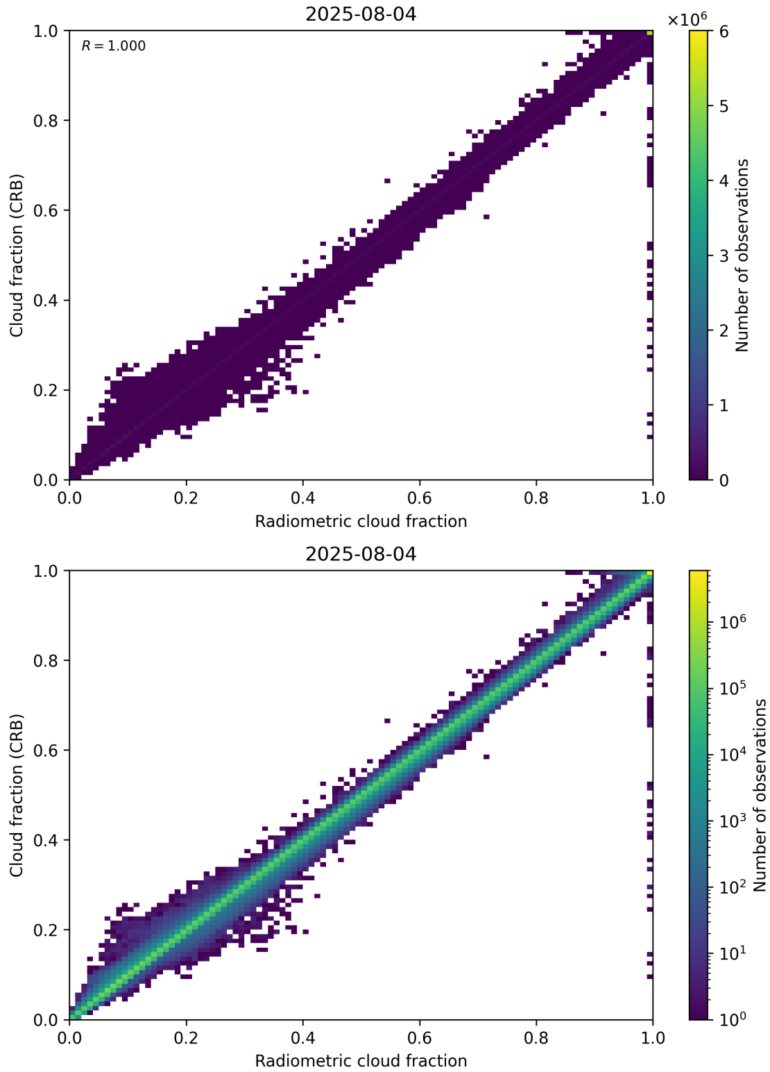
Figure 73: Scatter density plot of “Radiometric cloud fraction” against “Cloud fraction (CRB)” for 2025-08-04 to 2025-08-05.
