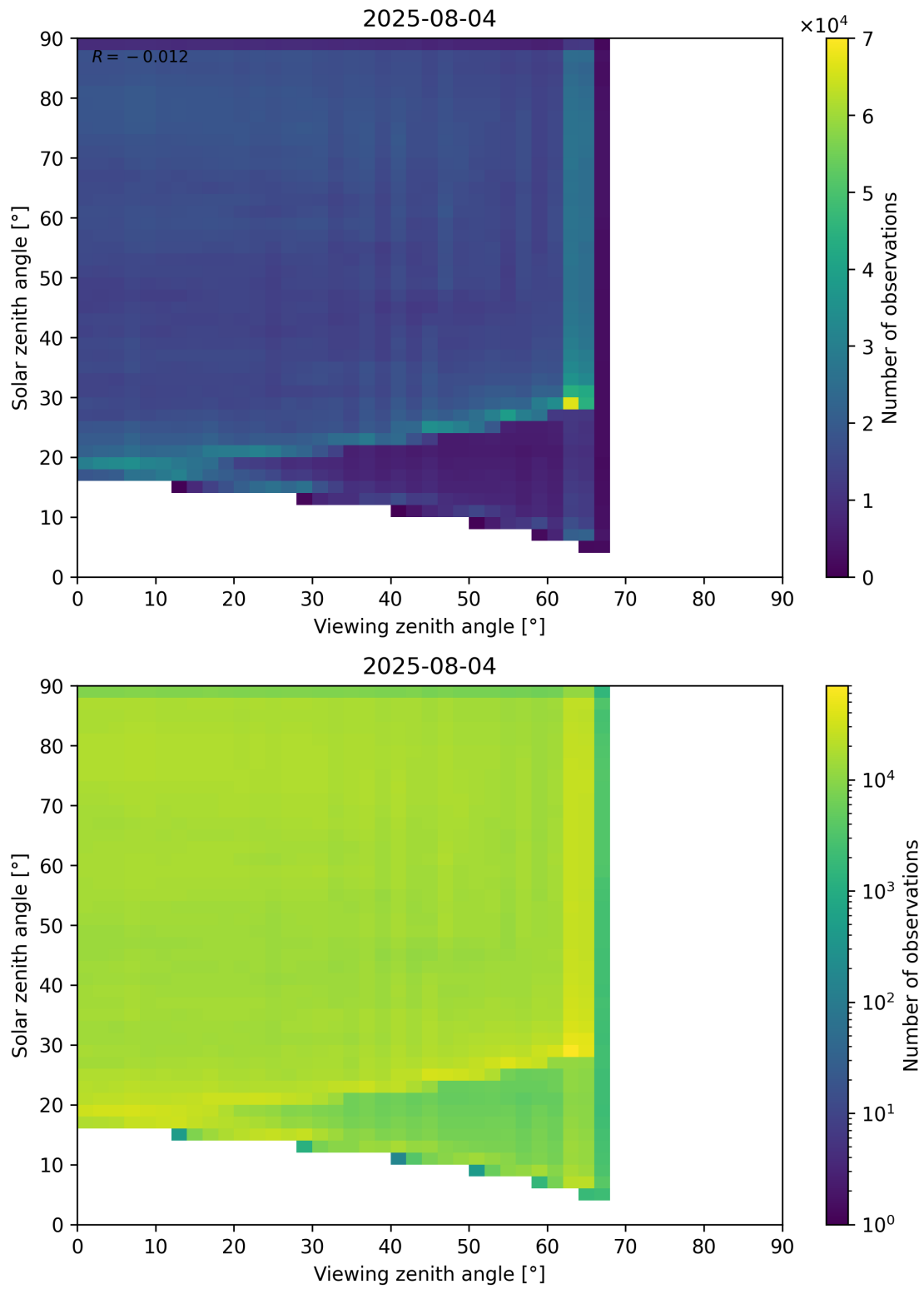
Figure 114: Scatter density plot of “Viewing zenith angle” against “Solar zenith angle” for 2025-08-04 to 2025-08-05.
