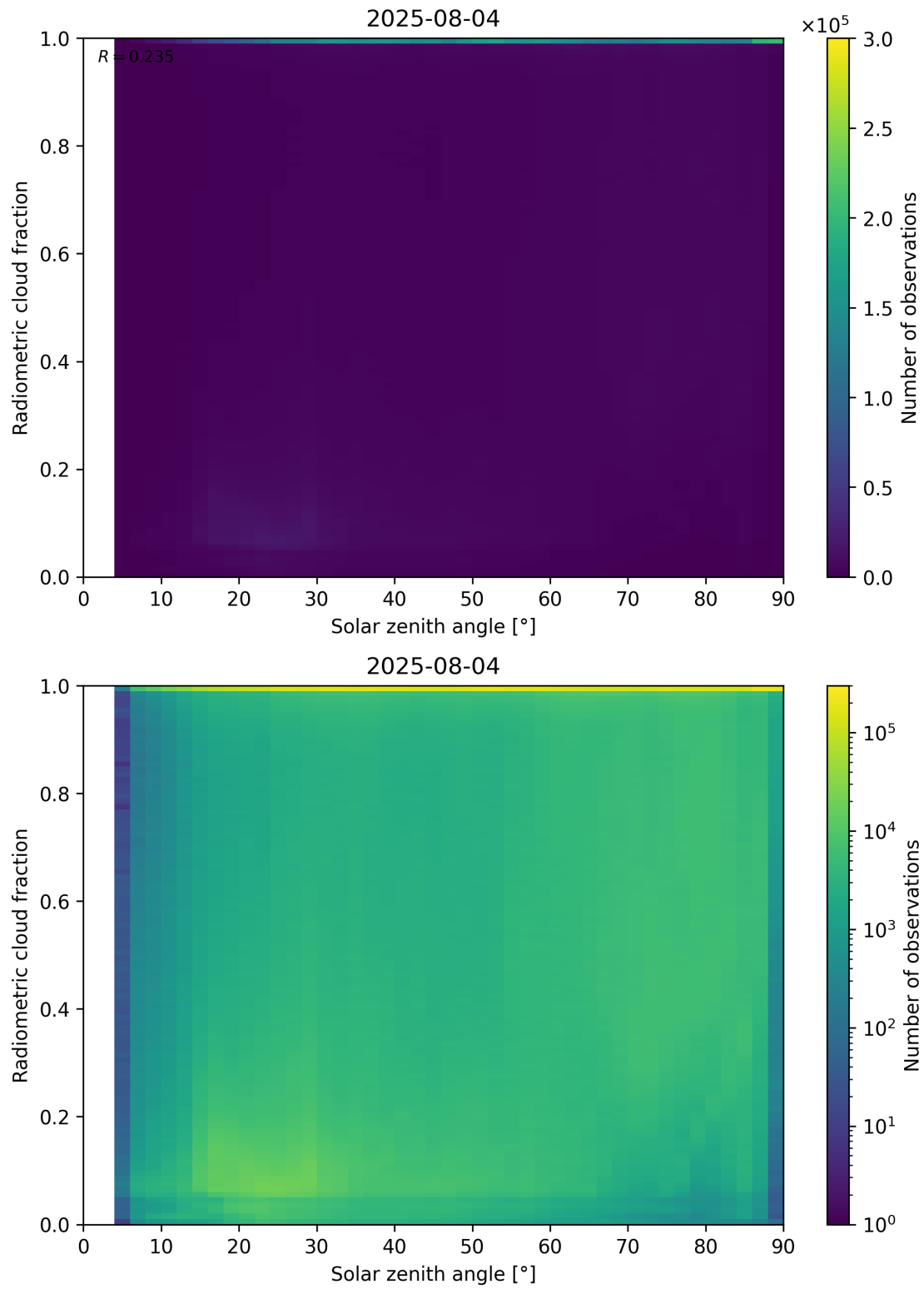
Figure 99: Scatter density plot of “Solar zenith angle” against “Radiometric cloud fraction” for 2025-08-04 to 2025-08-05.
