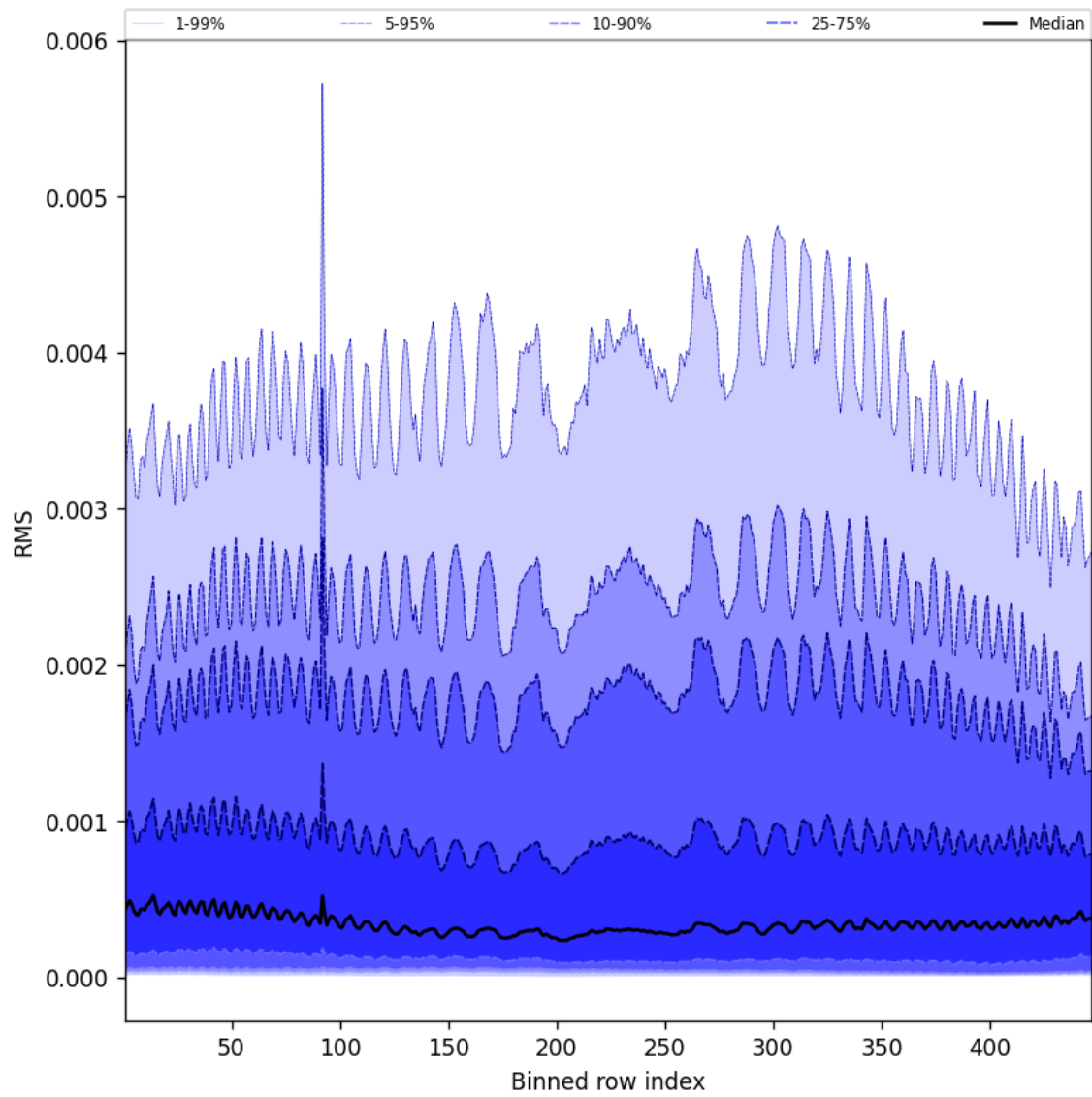
Figure 63: Along track statistics of “RMS” for 2025-08-04 to 2025-08-05
