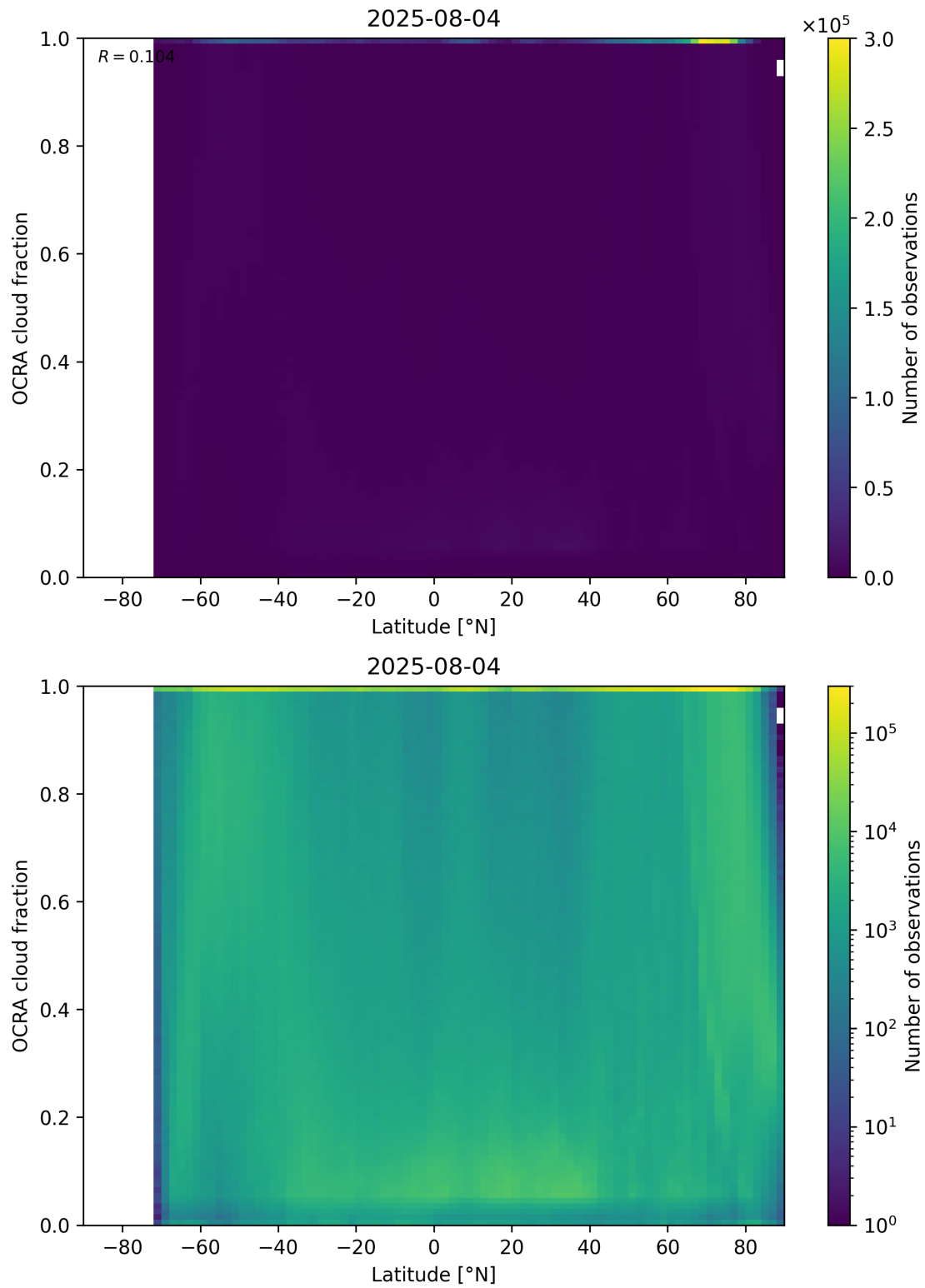
Figure 93: Scatter density plot of “Latitude” against “OCRA cloud fraction” for 2025-08-04 to 2025-08-05.
