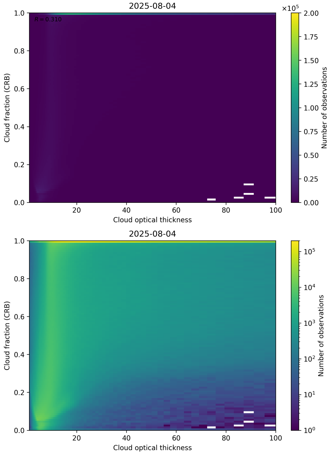
Figure 84: Scatter density plot of “Cloud optical thickness” against “Cloud fraction (CRB)” for 2025-08-04 to 2025-08-05.
