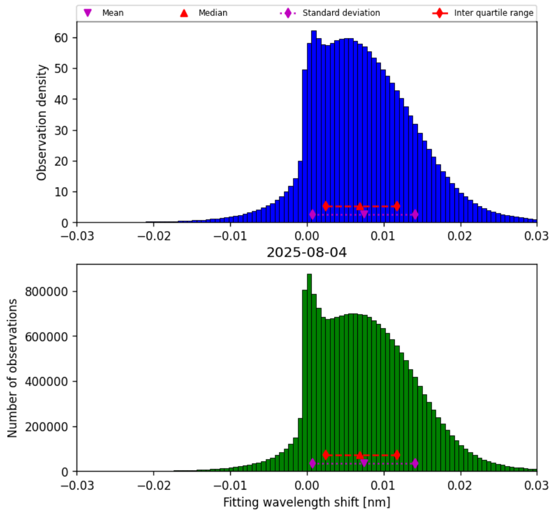
Figure 49: Histogram of “Fitting wavelength shift” for 2025-08-04 to 2025-08-05
