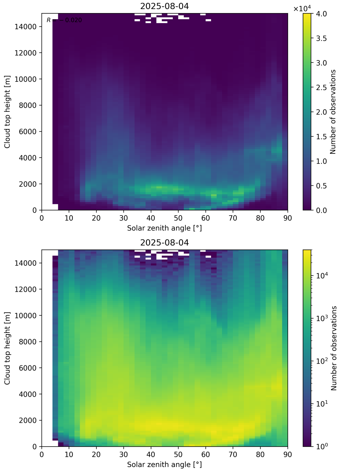
Figure 104: Scatter density plot of “Solar zenith angle” against “Cloud top height” for 2025-08-04 to 2025-08-05.
