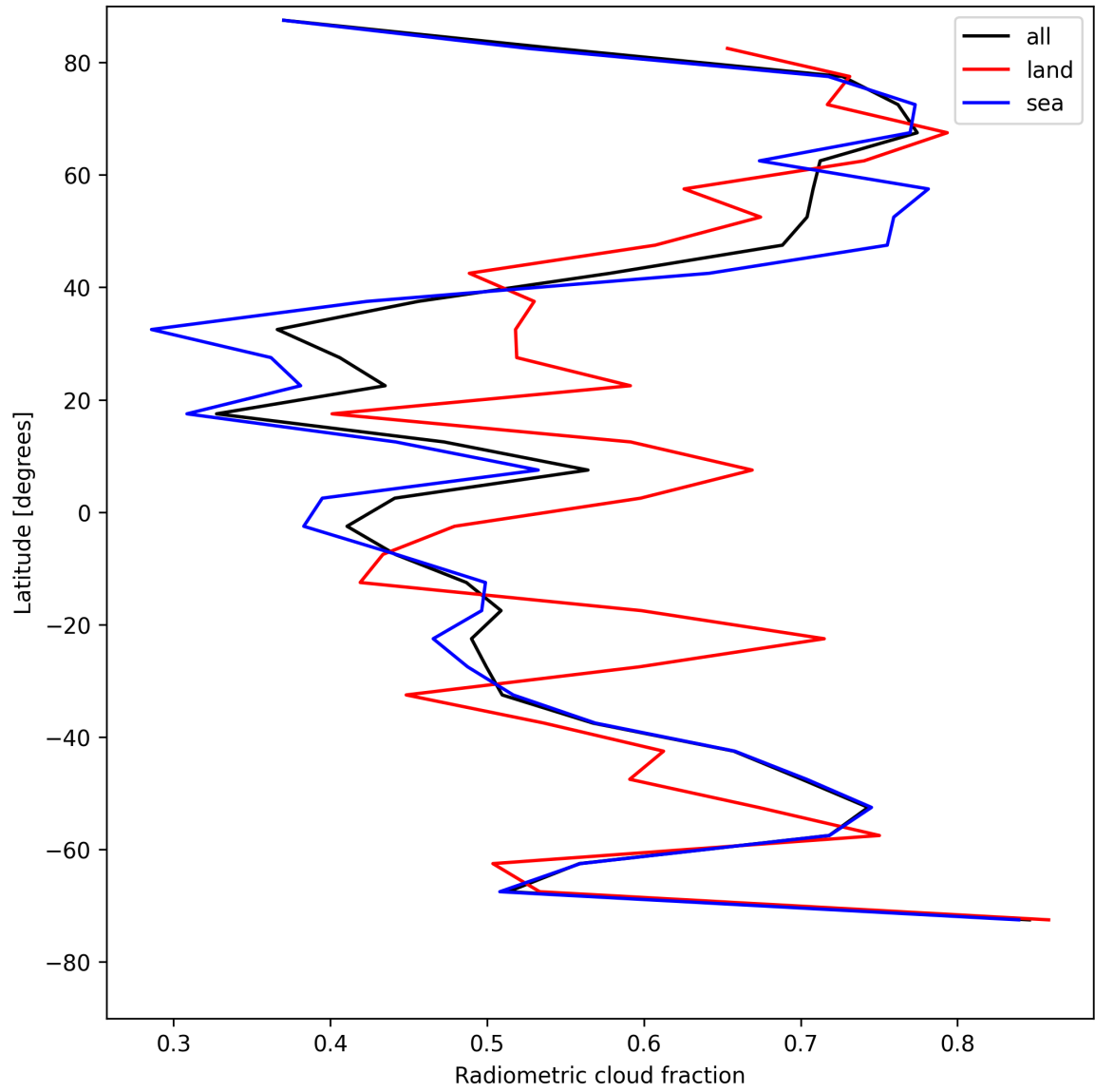
Figure 23: Zonal average of “Radiometric cloud fraction” for 2025-08-04 to 2025-08-05.
