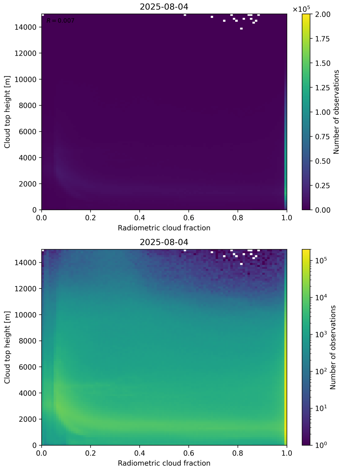
Figure 76: Scatter density plot of “Radiometric cloud fraction” against “Cloud top height” for 2025-08-04 to 2025-08-05.
