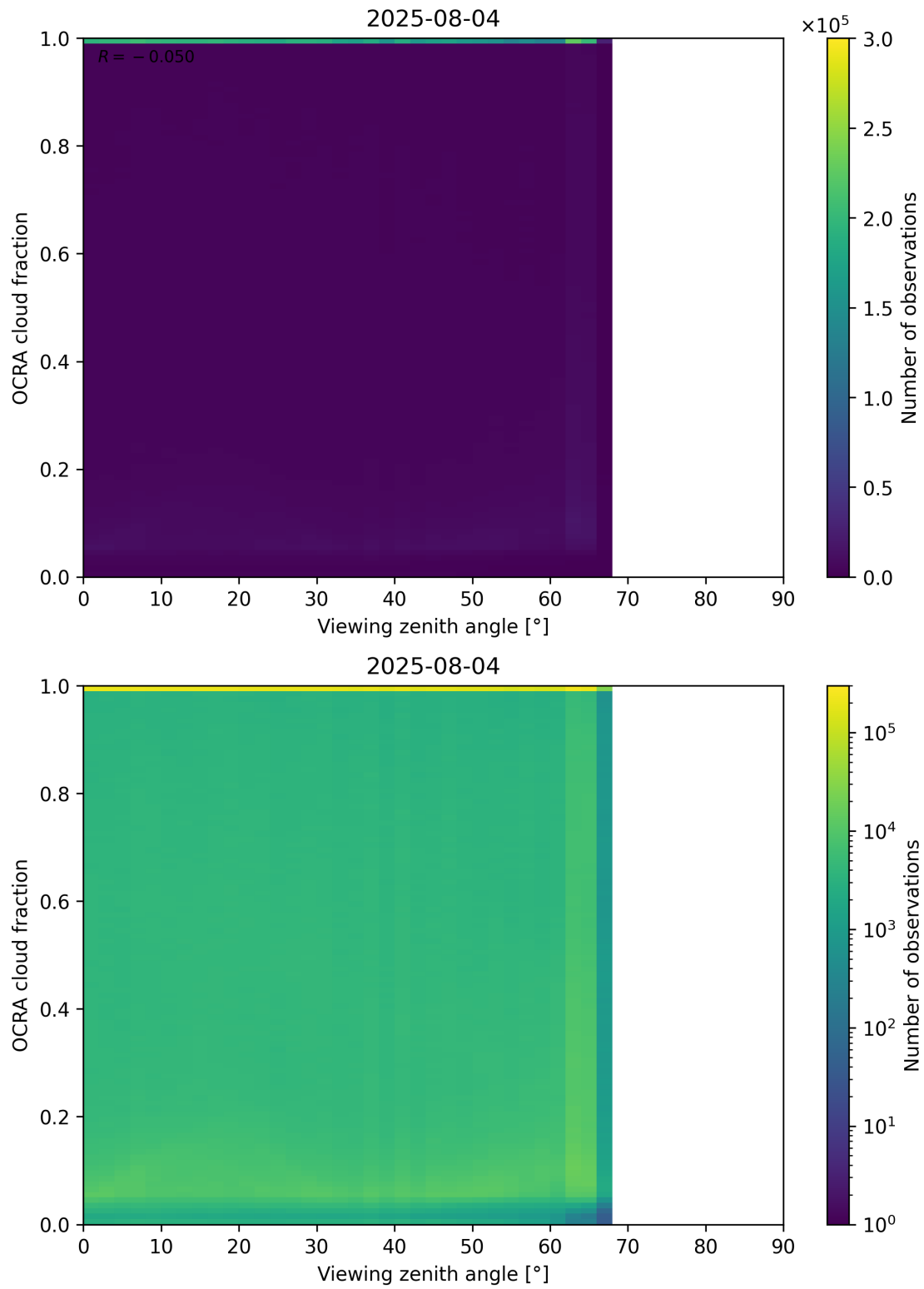
Figure 108: Scatter density plot of “Viewing zenith angle” against “OCRA cloud fraction” for 2025-08-04 to 2025-08-05.
