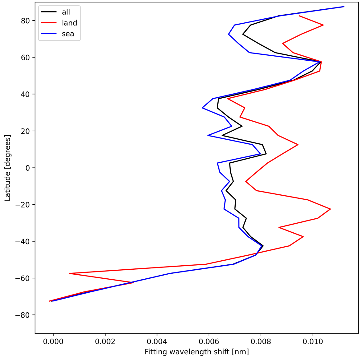
Figure 33: Zonal average of “Fitting wavelength shift” for 2025-08-04 to 2025-08-05.
