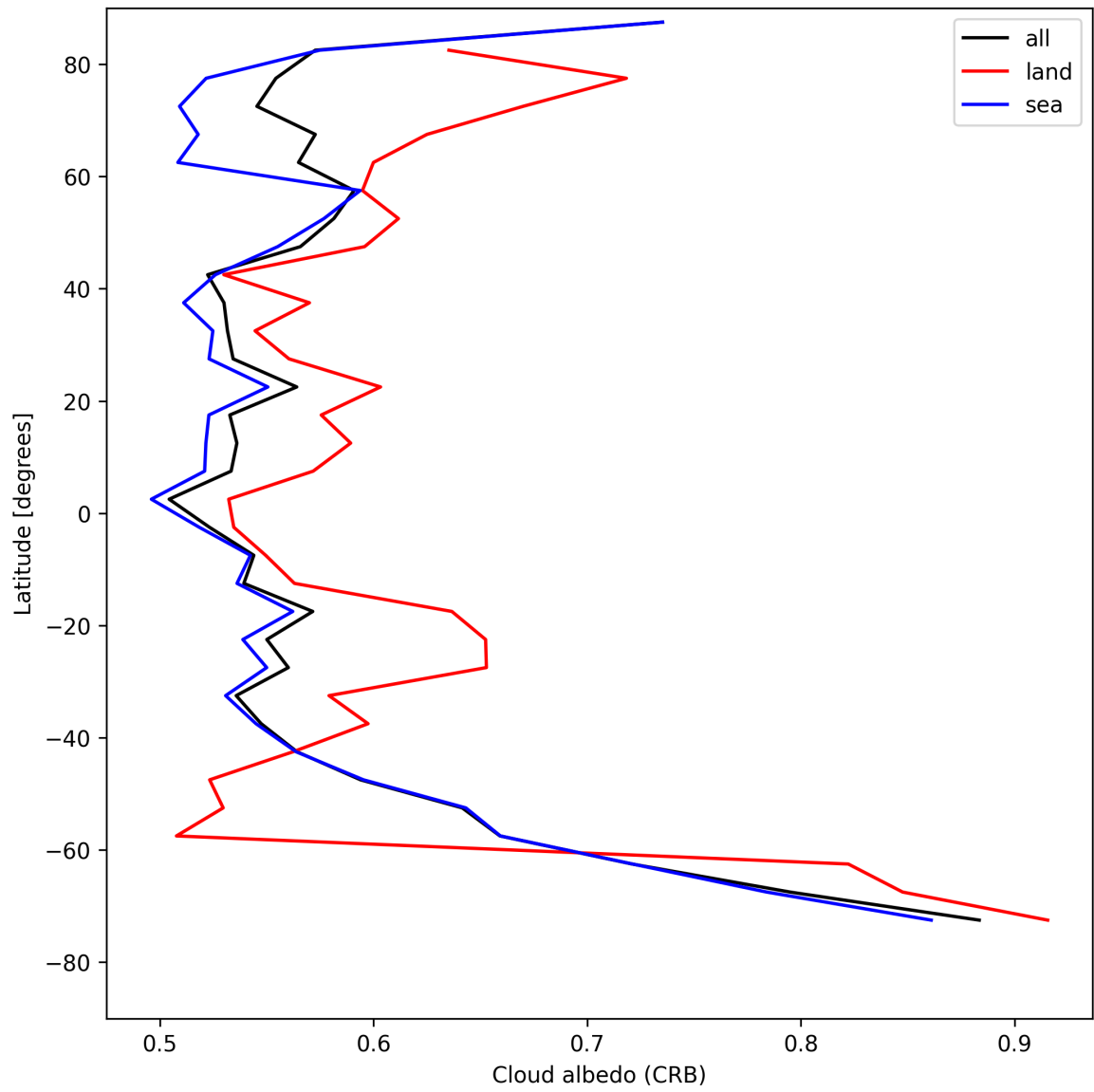
Figure 28: Zonal average of “Cloud albedo (CRB)” for 2025-08-04 to 2025-08-05.
