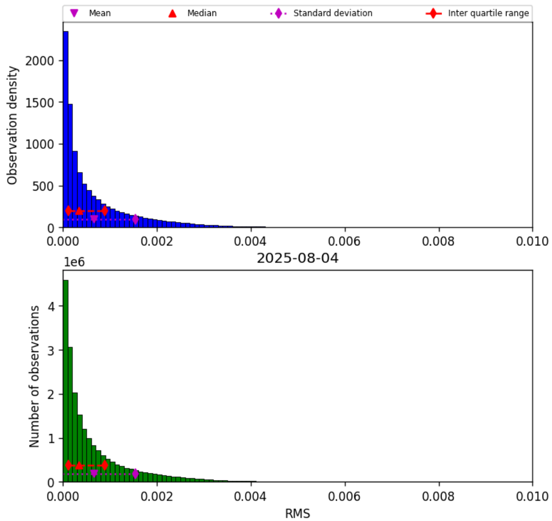
Figure 47: Histogram of “RMS” for 2025-08-04 to 2025-08-05
