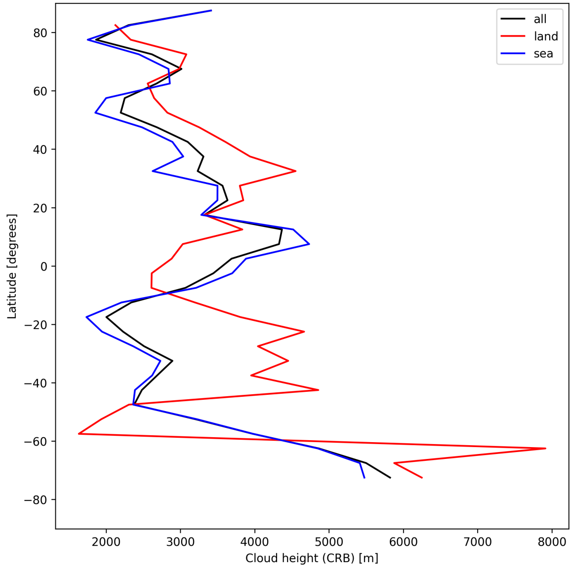
Figure 27: Zonal average of “Cloud height (CRB)” for 2025-08-04 to 2025-08-05.
