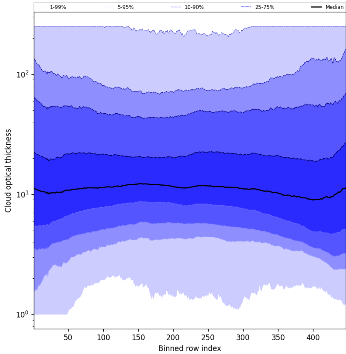
Figure 57: Along track statistics of “Cloud optical thickness” for 2025-08-04 to 2025-08-05
