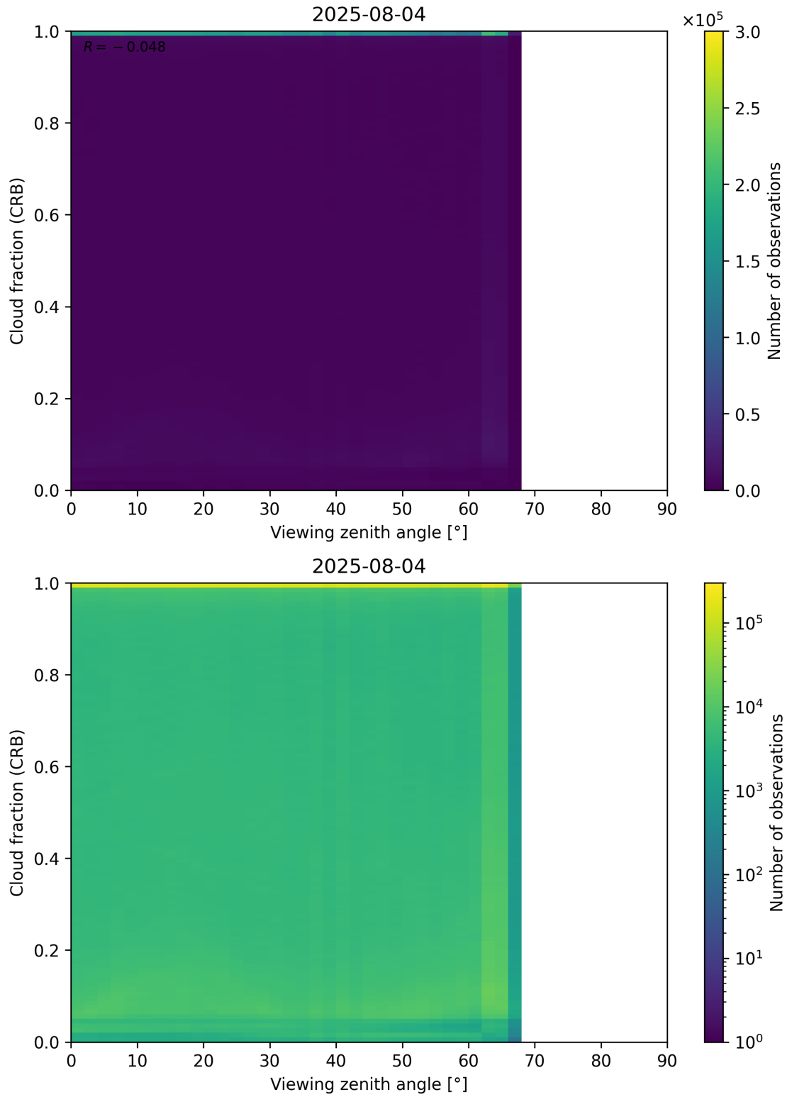
Figure 109: Scatter density plot of “Viewing zenith angle” against “Cloud fraction (CRB)” for 2025-08-04 to 2025-08-05.
