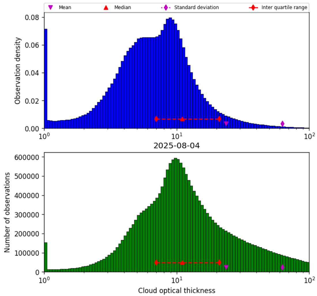
Figure 41: Histogram of “Cloud optical thickness” for 2025-08-04 to 2025-08-05
