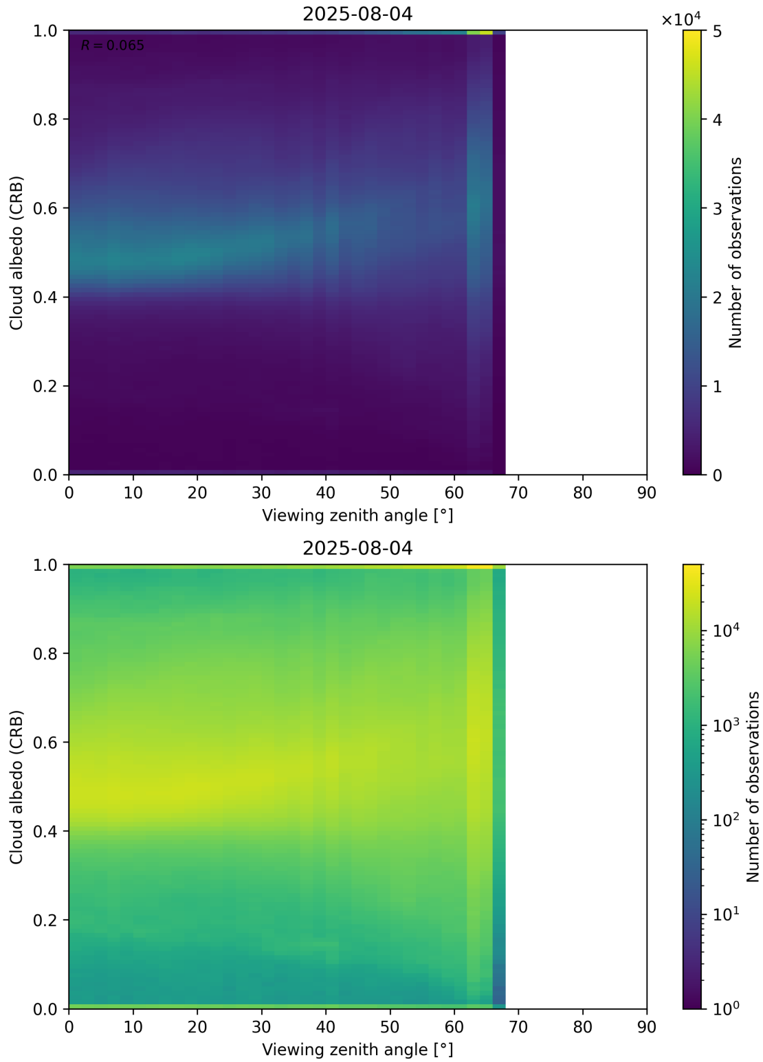
Figure 106: Scatter density plot of “Viewing zenith angle” against “Cloud albedo (CRB)” for 2025-08-04 to 2025-08-05.
