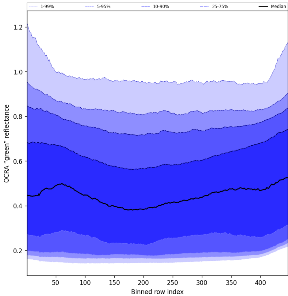
Figure 68: Along track statistics of “OCRA “green” reflectance” for 2025-08-04 to 2025-08-05
