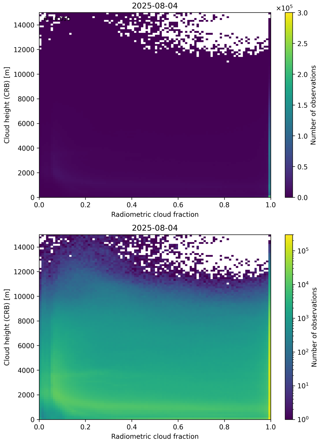
Figure 74: Scatter density plot of “Radiometric cloud fraction” against “Cloud height (CRB)” for 2025-08-04 to 2025-08-05.
