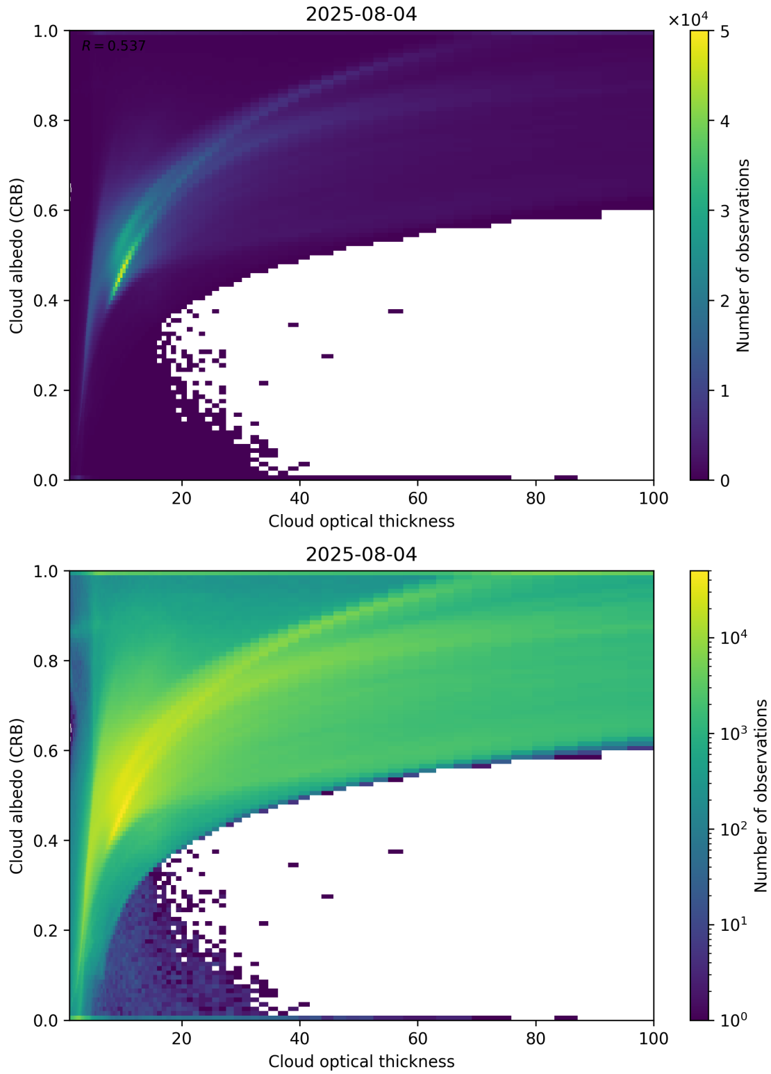
Figure 82: Scatter density plot of “Cloud optical thickness” against “Cloud albedo (CRB)” for 2025-08-04 to 2025-08-05.
