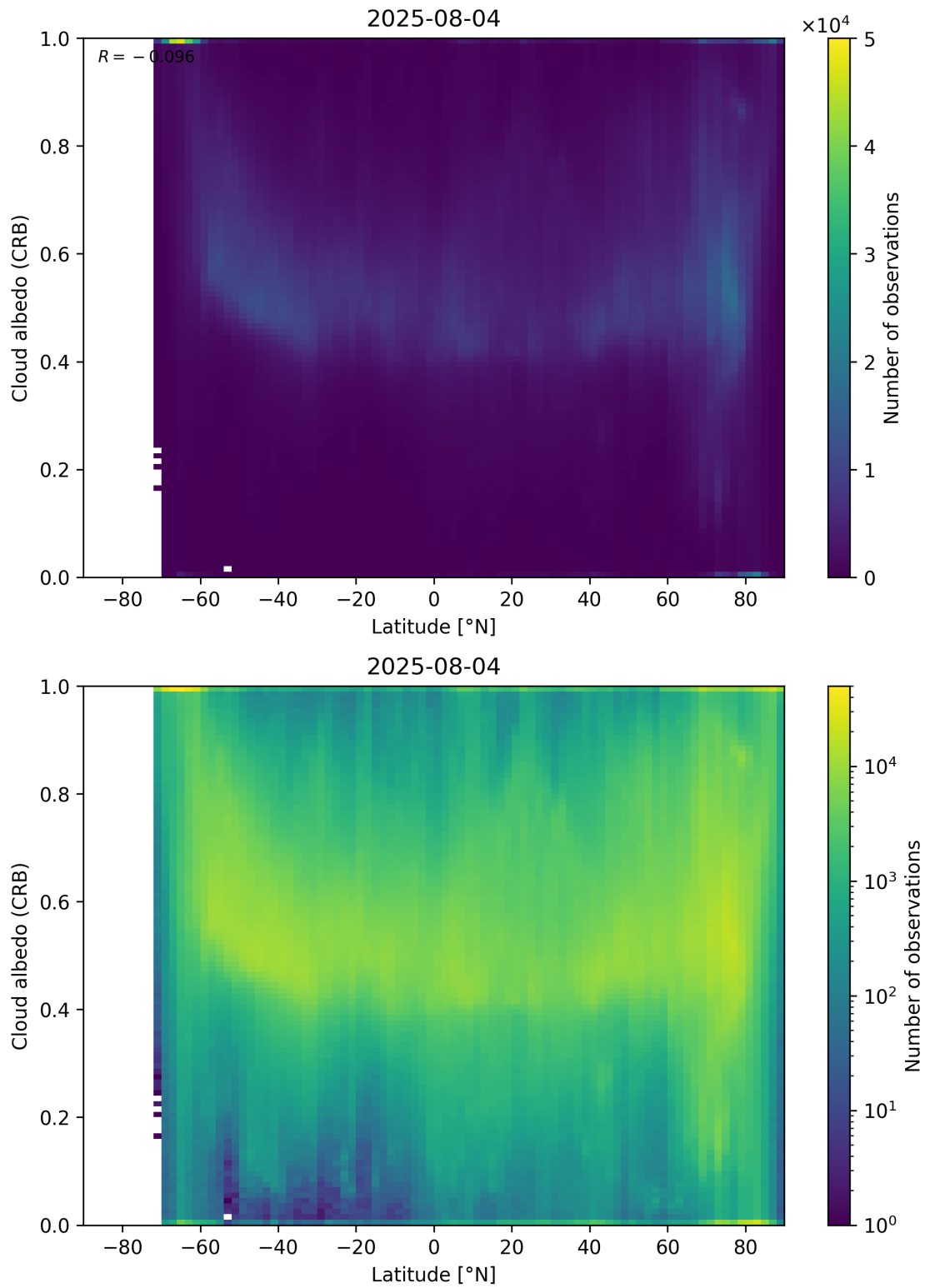
Figure 91: Scatter density plot of “Latitude” against “Cloud albedo (CRB)” for 2025-08-04 to 2025-08-05.
