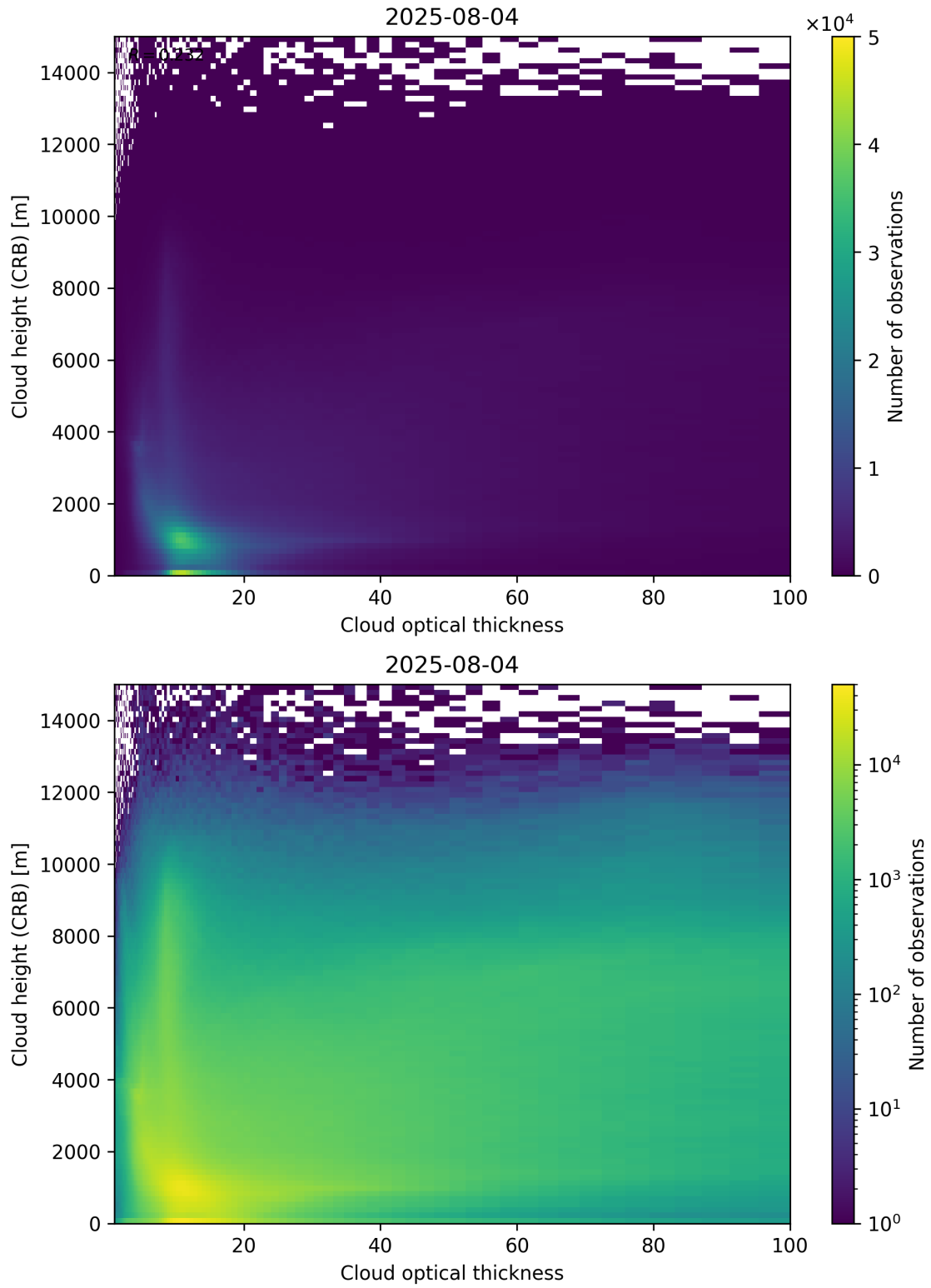
Figure 85: Scatter density plot of “Cloud optical thickness” against “Cloud height (CRB)” for 2025-08-04 to 2025-08-05.
