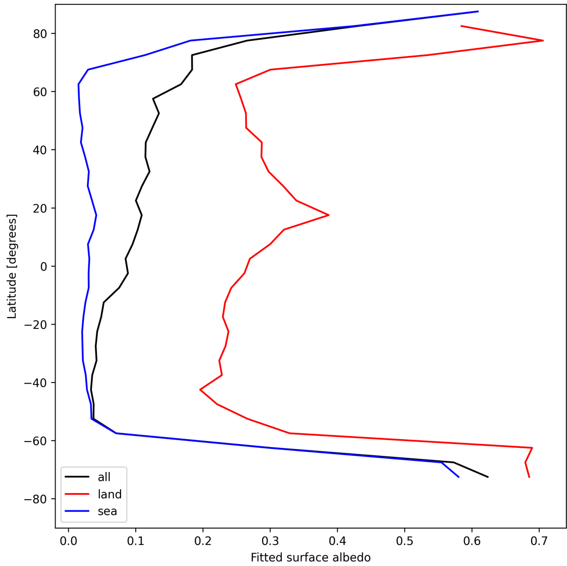
Figure 29: Zonal average of “Fitted surface albedo” for 2025-08-04 to 2025-08-05.
