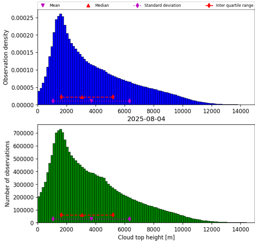
Figure 40: Histogram of “Cloud top height” for 2025-08-04 to 2025-08-05
