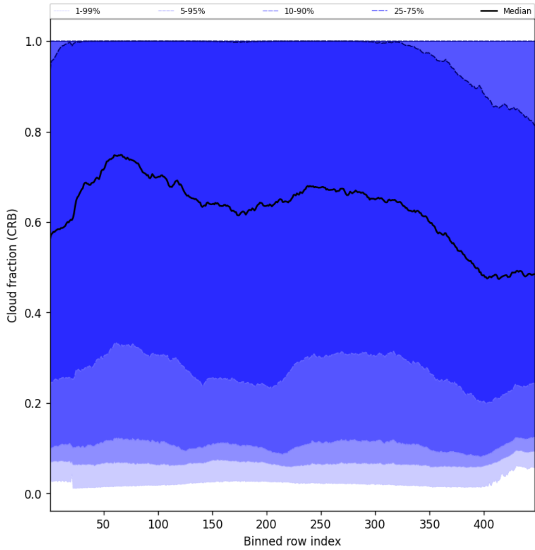
Figure 58: Along track statistics of “Cloud fraction (CRB)” for 2025-08-04 to 2025-08-05
