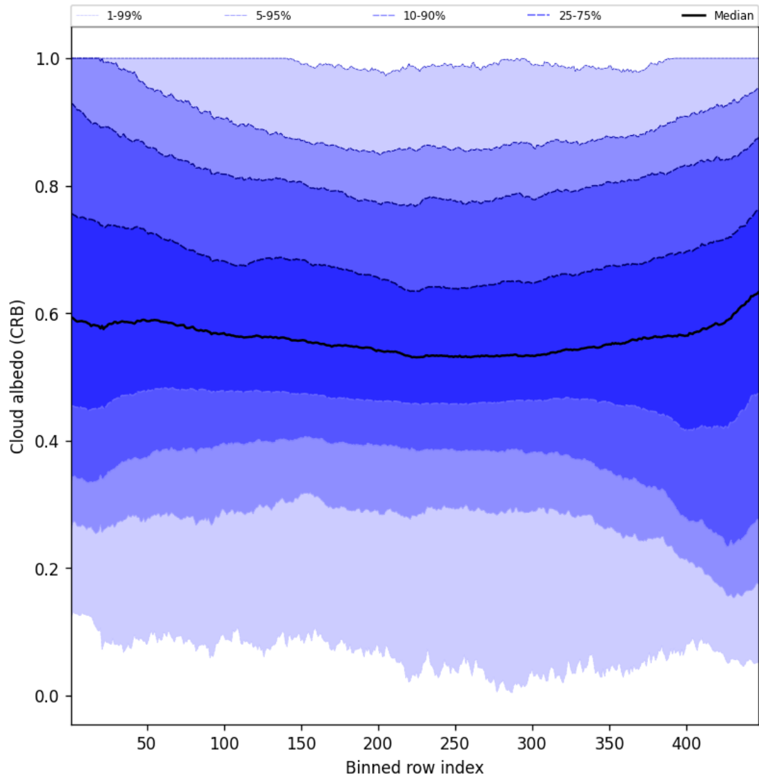
Figure 60: Along track statistics of “Cloud albedo (CRB)” for 2025-08-04 to 2025-08-05
