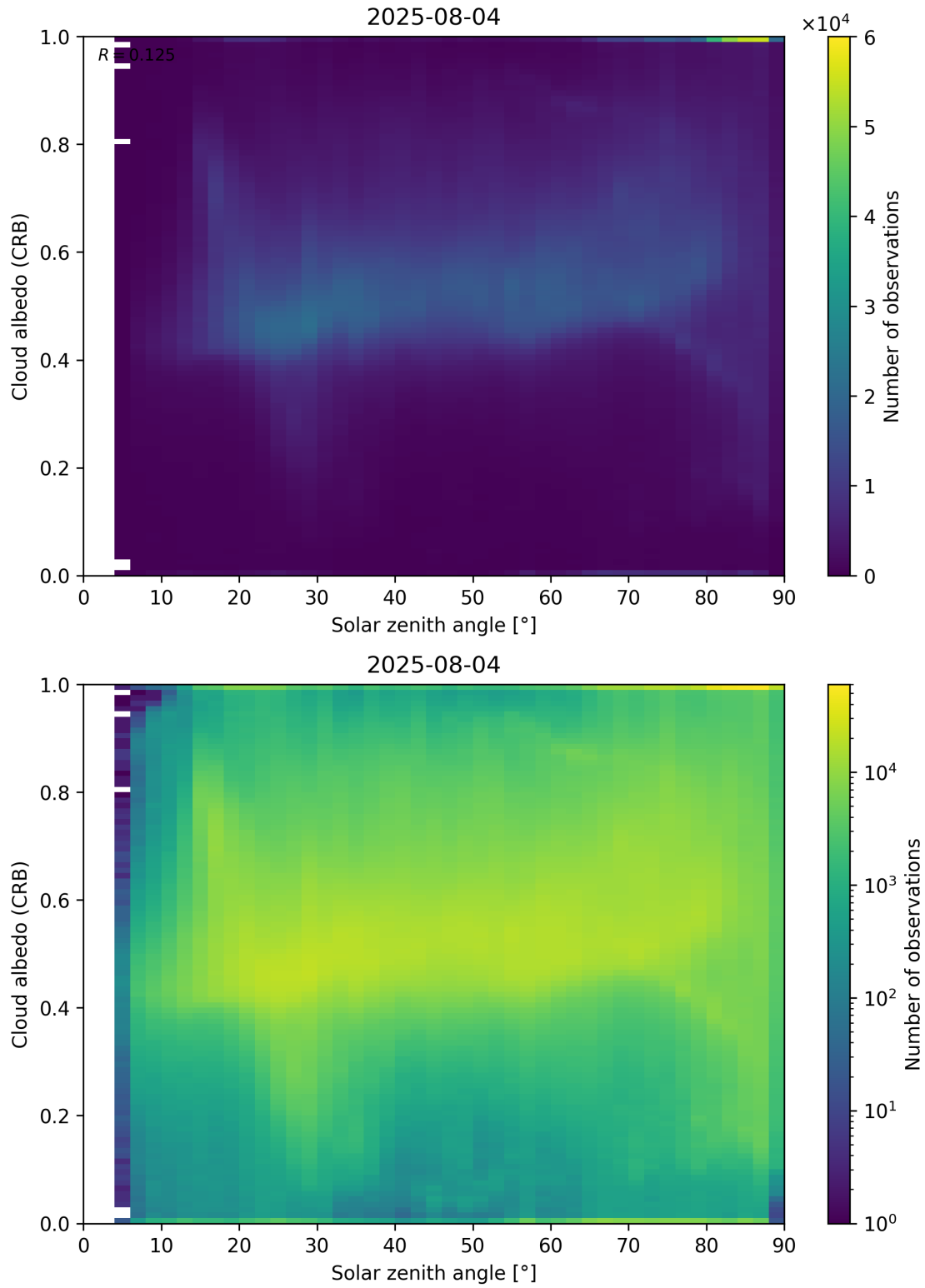
Figure 98: Scatter density plot of “Solar zenith angle” against “Cloud albedo (CRB)” for 2025-08-04 to 2025-08-05.
