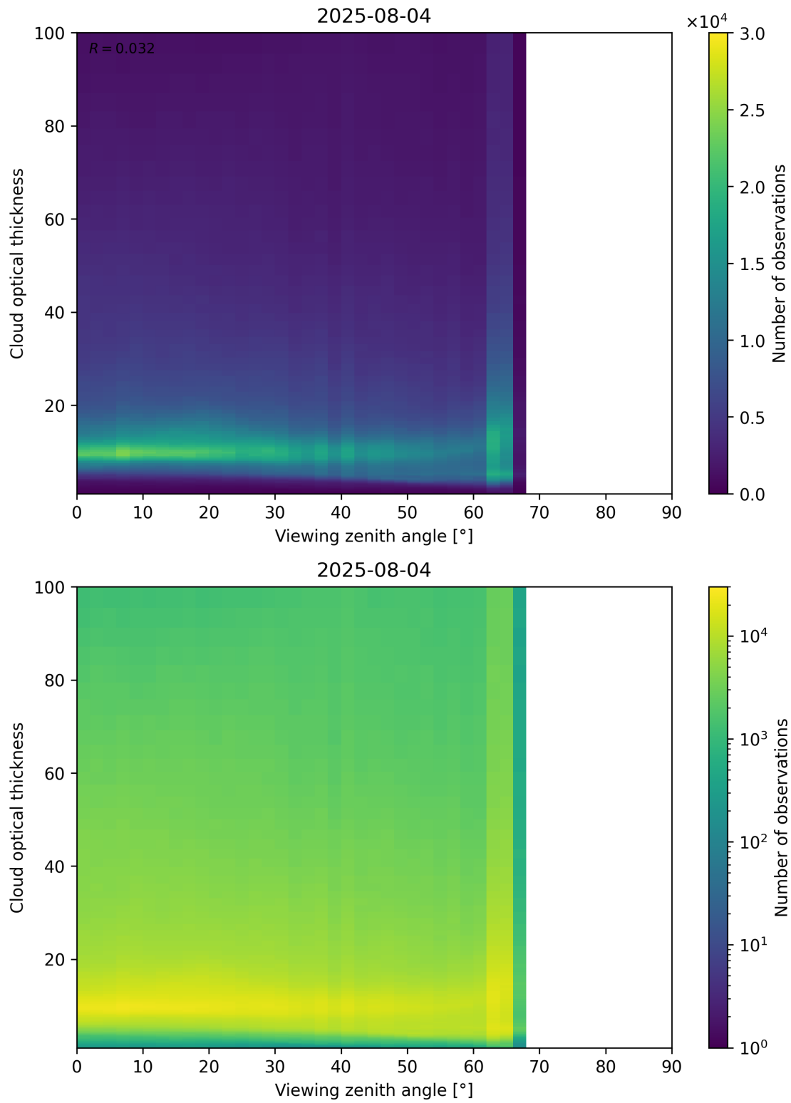
Figure 111: Scatter density plot of “Viewing zenith angle” against “Cloud optical thickness” for 2025-08-04 to 2025-08-05.
