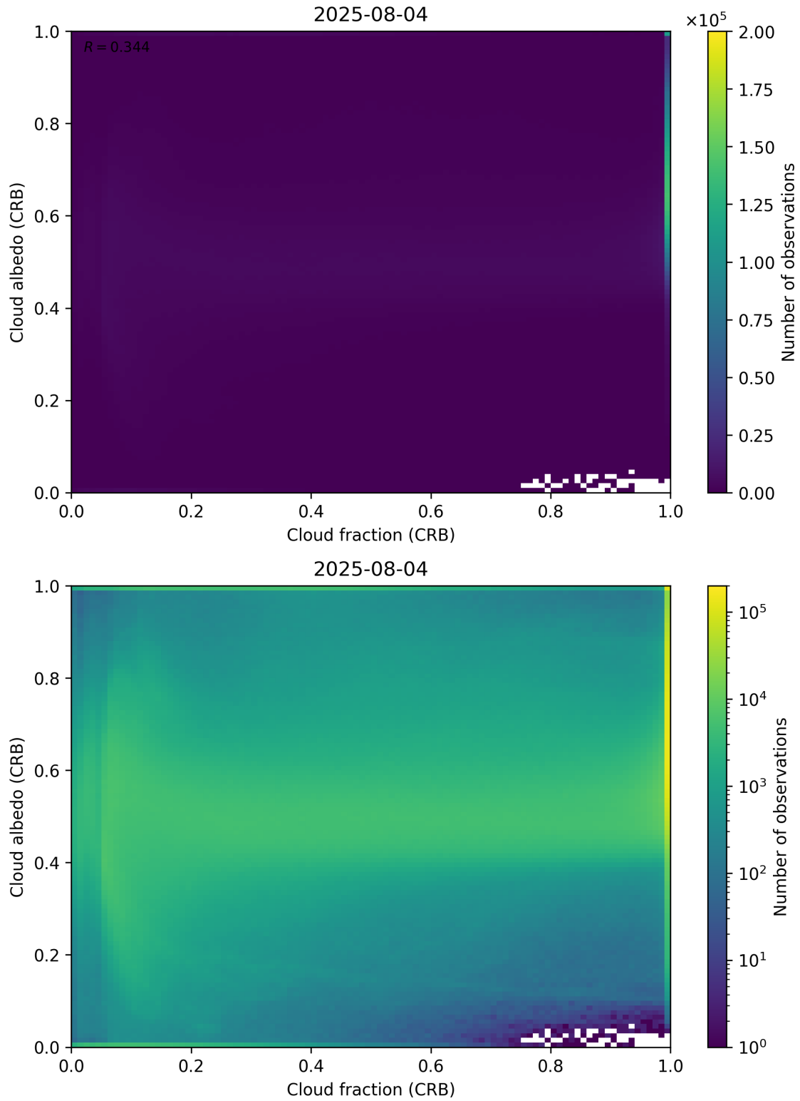
Figure 77: Scatter density plot of “Cloud fraction (CRB)” against “Cloud albedo (CRB)” for 2025-08-04 to 2025-08-05.
