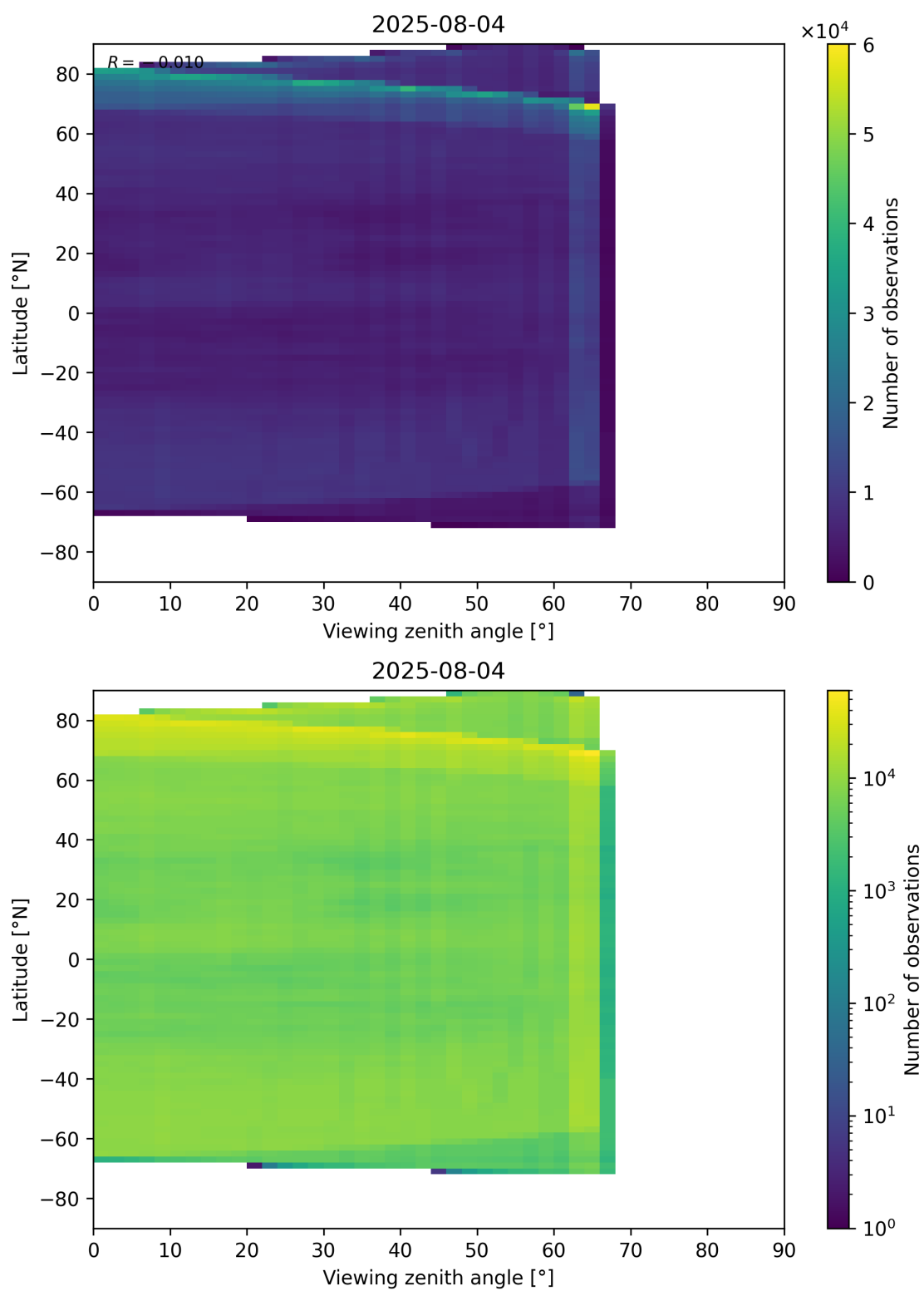
Figure 113: Scatter density plot of “Viewing zenith angle” against “Latitude” for 2025-08-04 to 2025-08-05.
