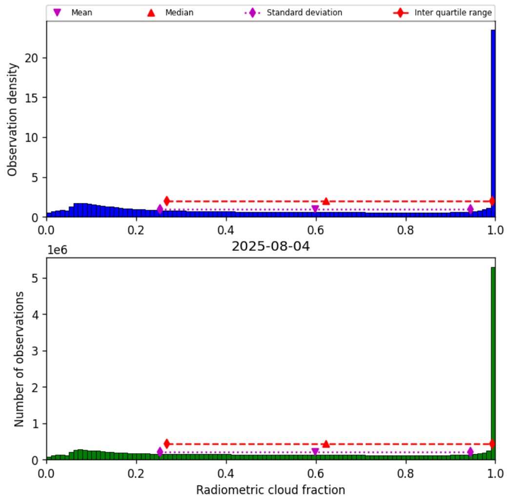
Figure 39: Histogram of “Radiometric cloud fraction” for 2025-08-04 to 2025-08-05
