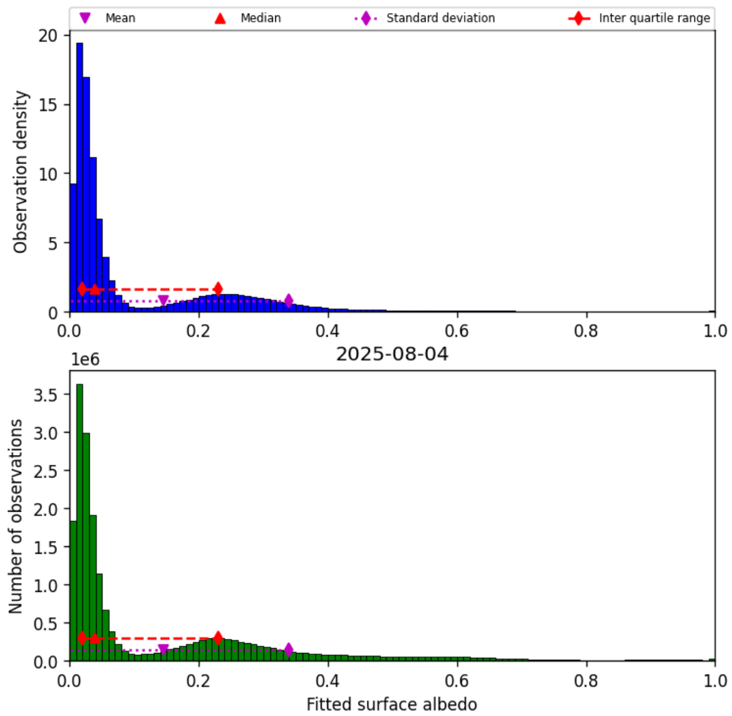
Figure 45: Histogram of “Fitted surface albedo” for 2025-08-04 to 2025-08-05
