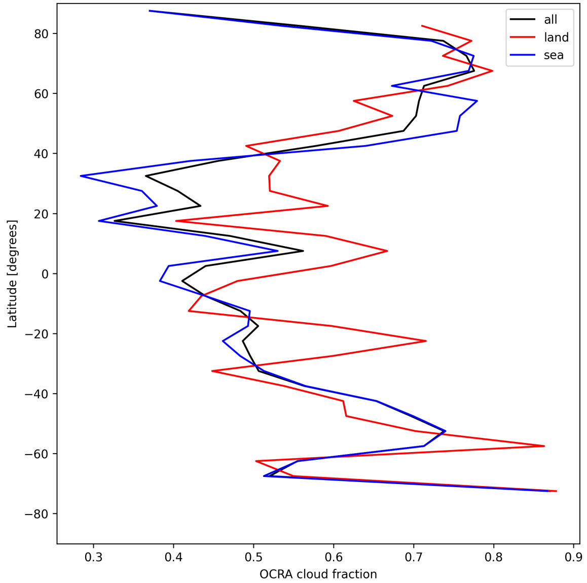
Figure 34: Zonal average of “OCRA cloud fraction” for 2025-08-04 to 2025-08-05.
