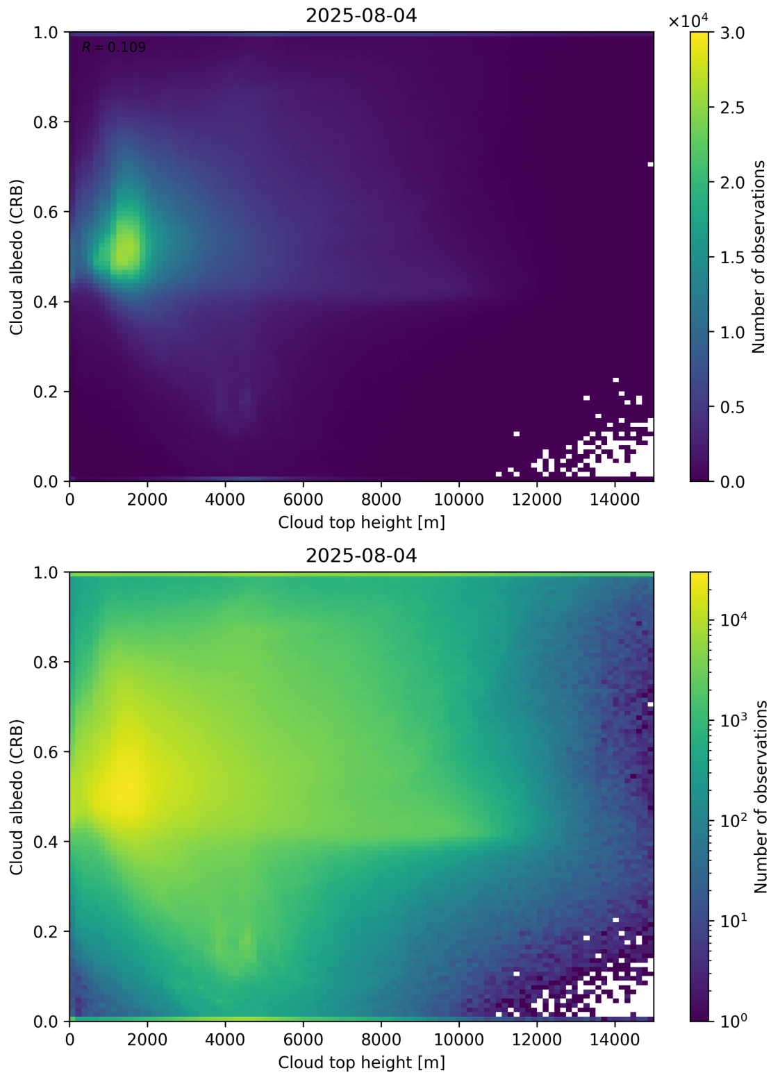
Figure 86: Scatter density plot of “Cloud top height” against “Cloud albedo (CRB)” for 2025-08-04 to 2025-08-05.
