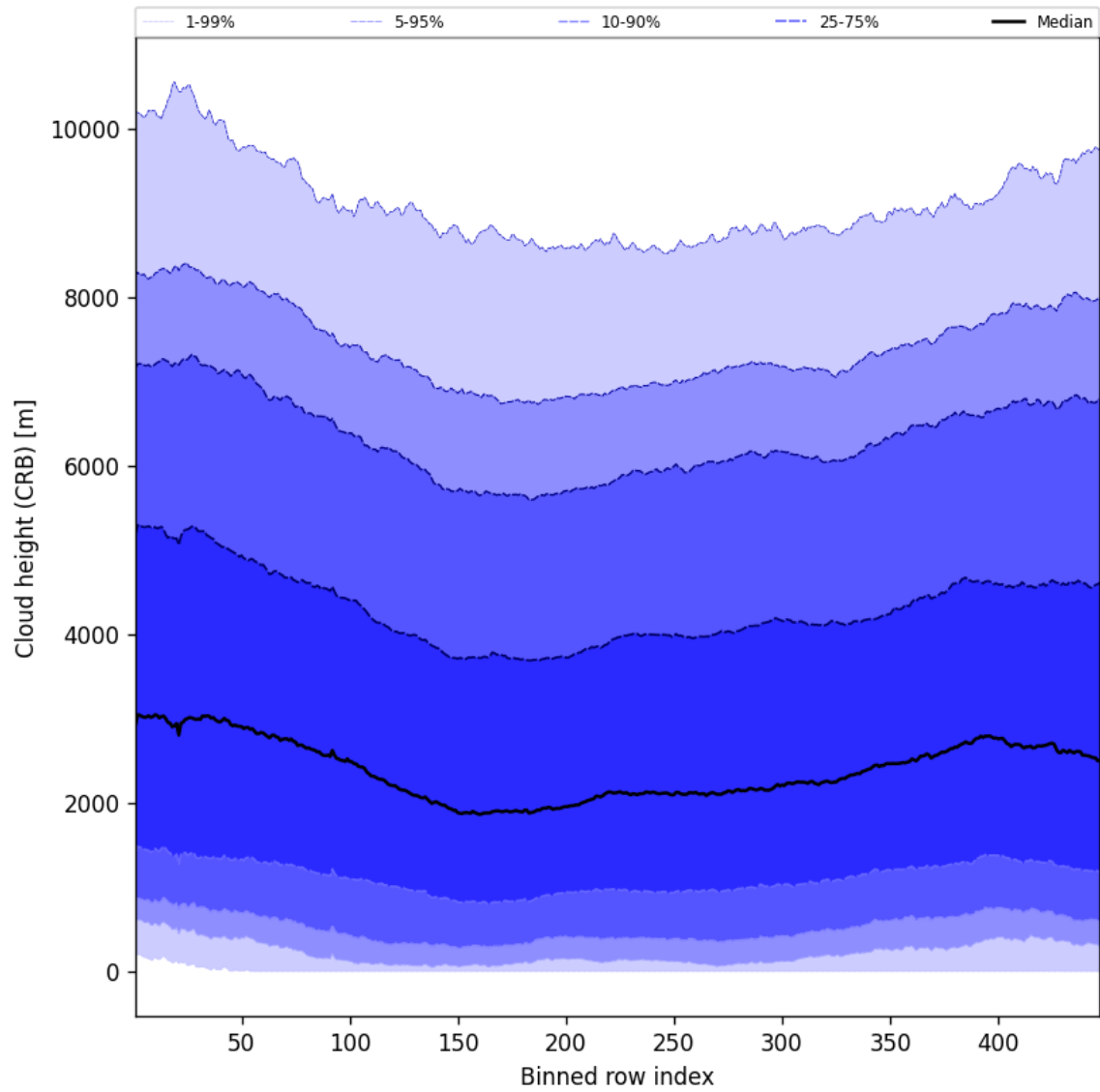
Figure 59: Along track statistics of “Cloud height (CRB)” for 2025-08-04 to 2025-08-05
