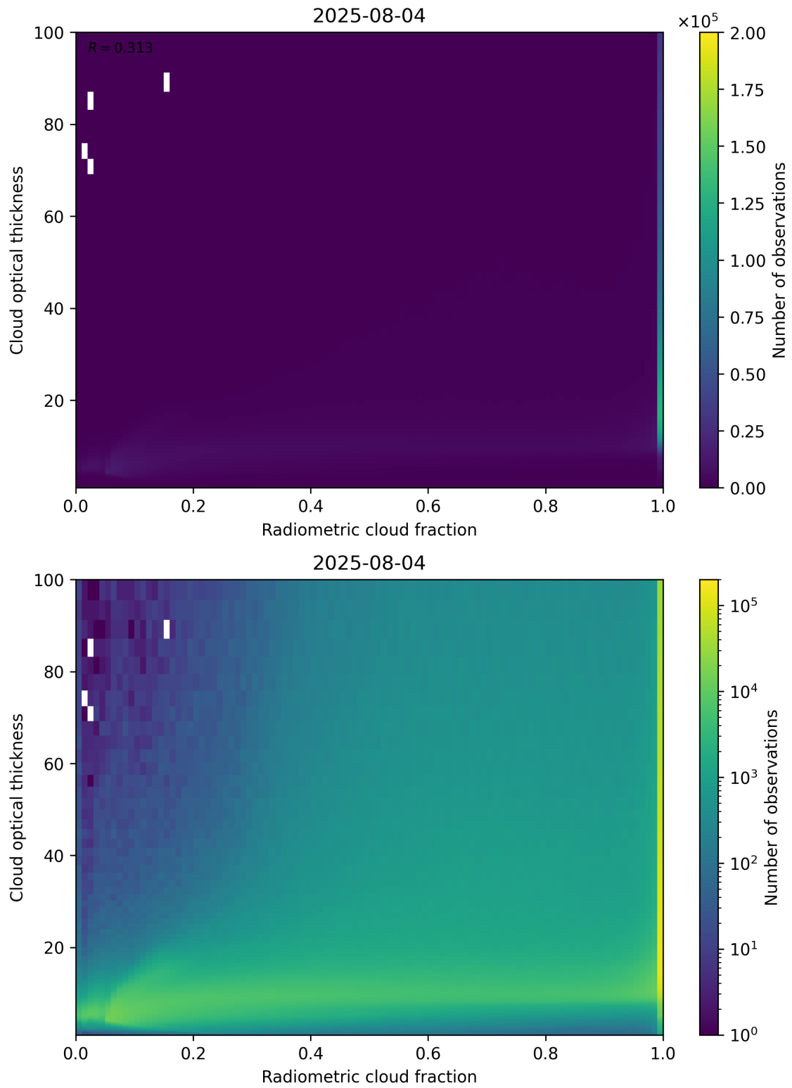
Figure 75: Scatter density plot of “Radiometric cloud fraction” against “Cloud optical thickness” for 2025-08-04 to 2025-08-05.
