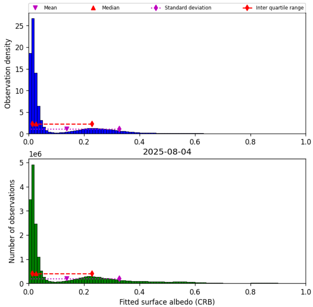
Figure 46: Histogram of “Fitted surface albedo (CRB)” for 2025-08-04 to 2025-08-05
