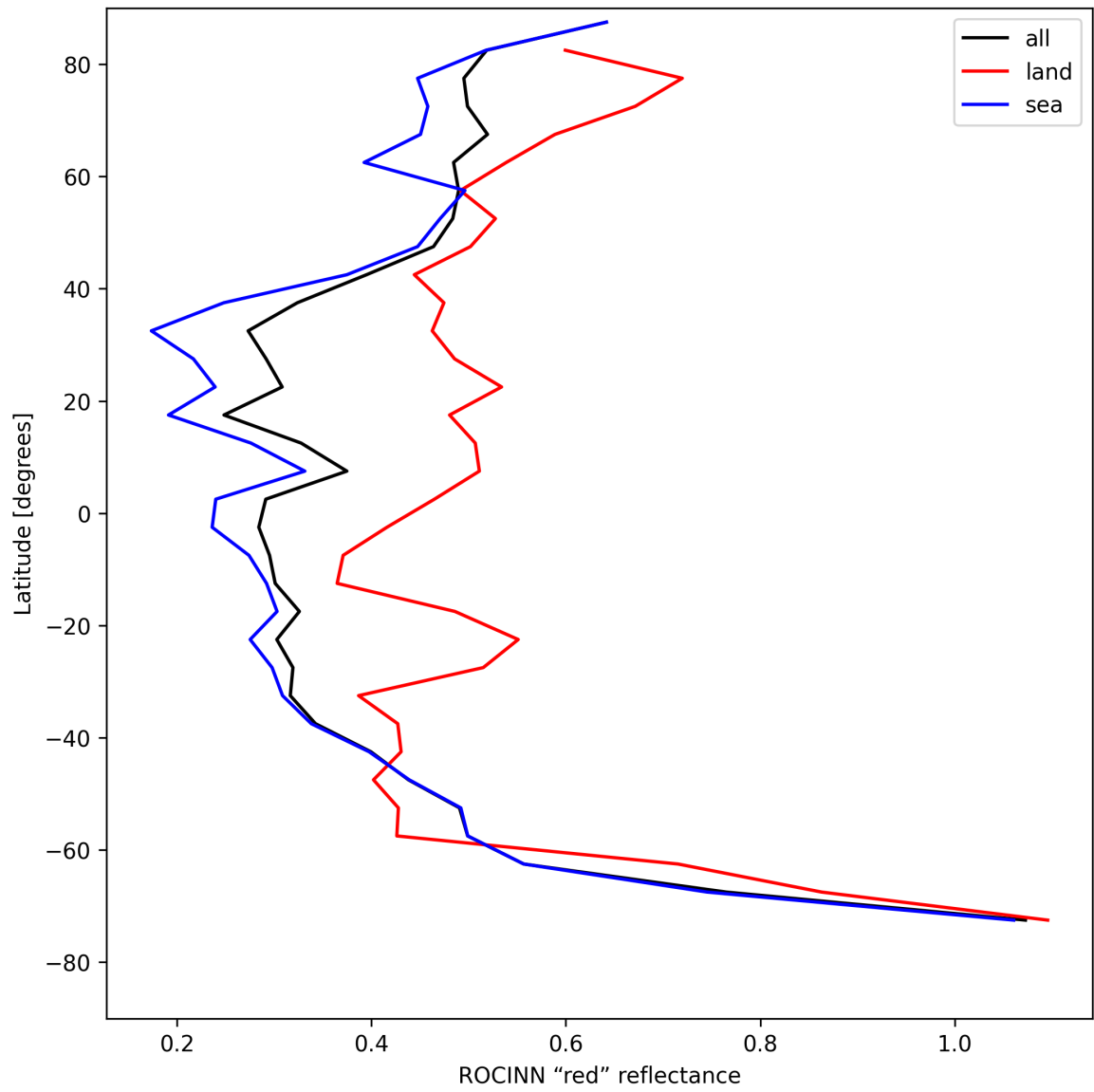
Figure 37: Zonal average of “ROCINN “red” reflectance” for 2025-08-04 to 2025-08-05.
