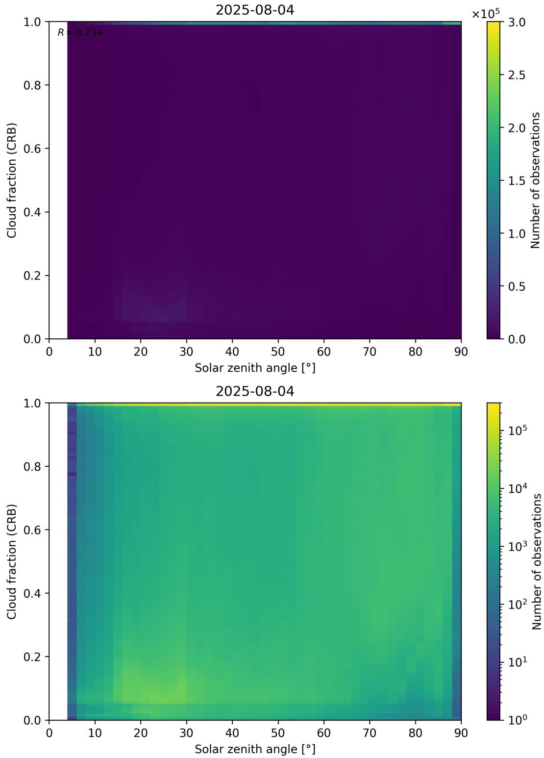
Figure 101: Scatter density plot of “Solar zenith angle” against “Cloud fraction (CRB)” for 2025-08-04 to 2025-08-05.
