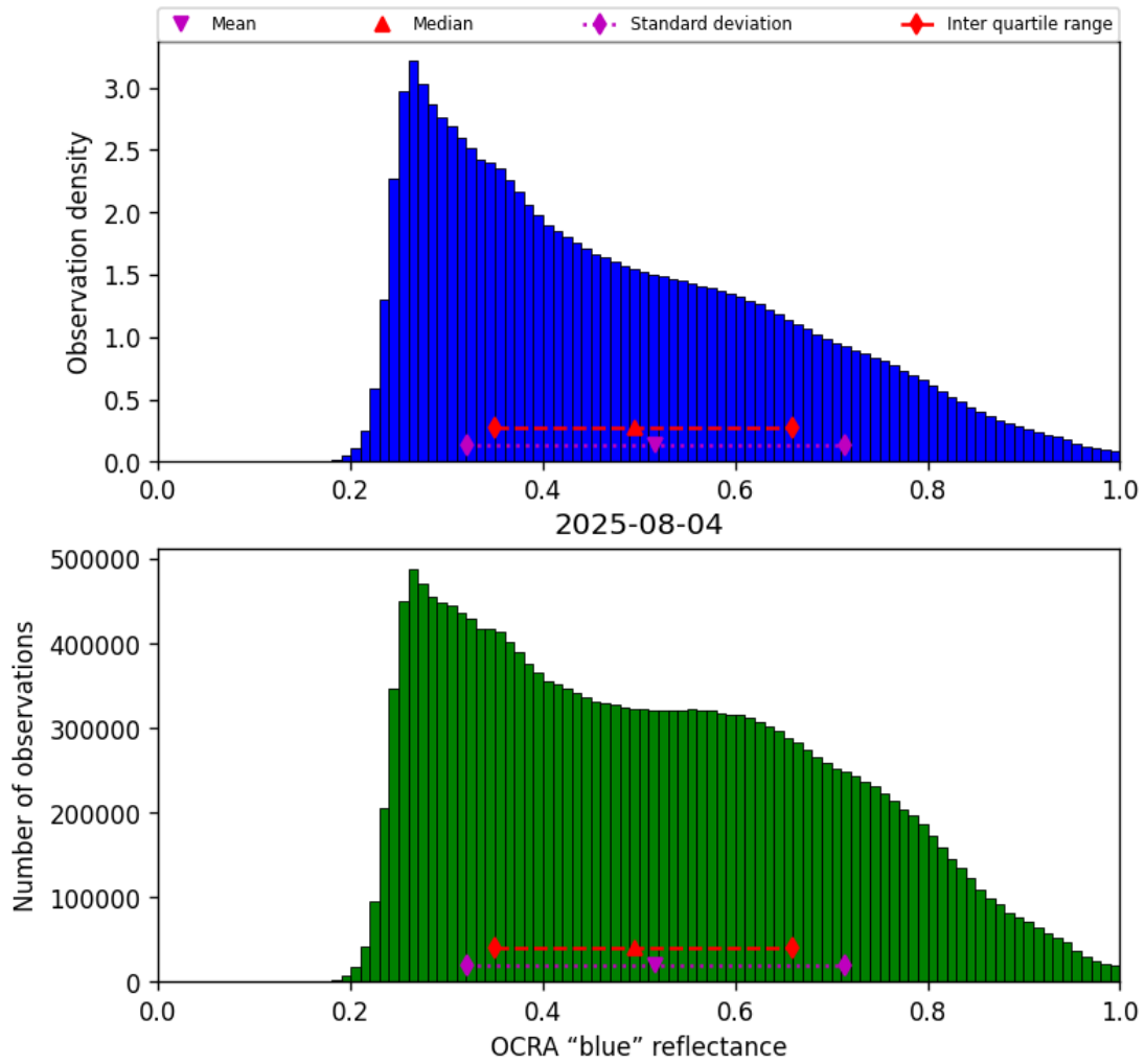
Figure 51: Histogram of “OCRA “blue” reflectance” for 2025-08-04 to 2025-08-05
