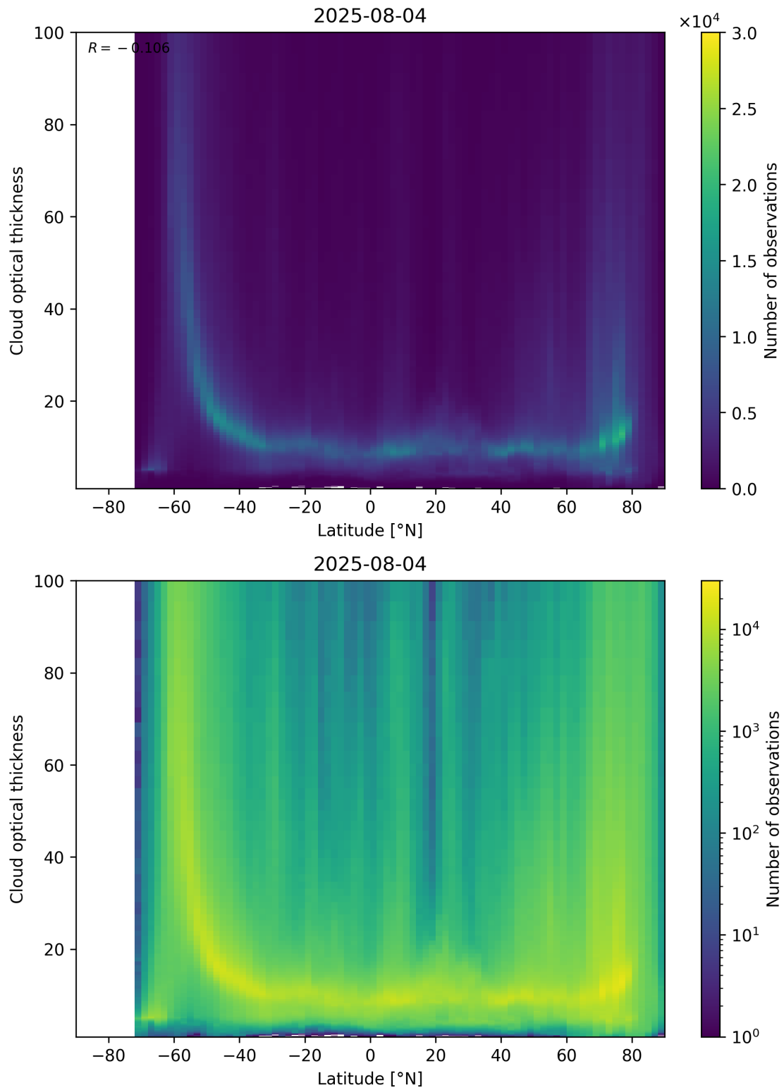
Figure 96: Scatter density plot of “Latitude” against “Cloud optical thickness” for 2025-08-04 to 2025-08-05.
