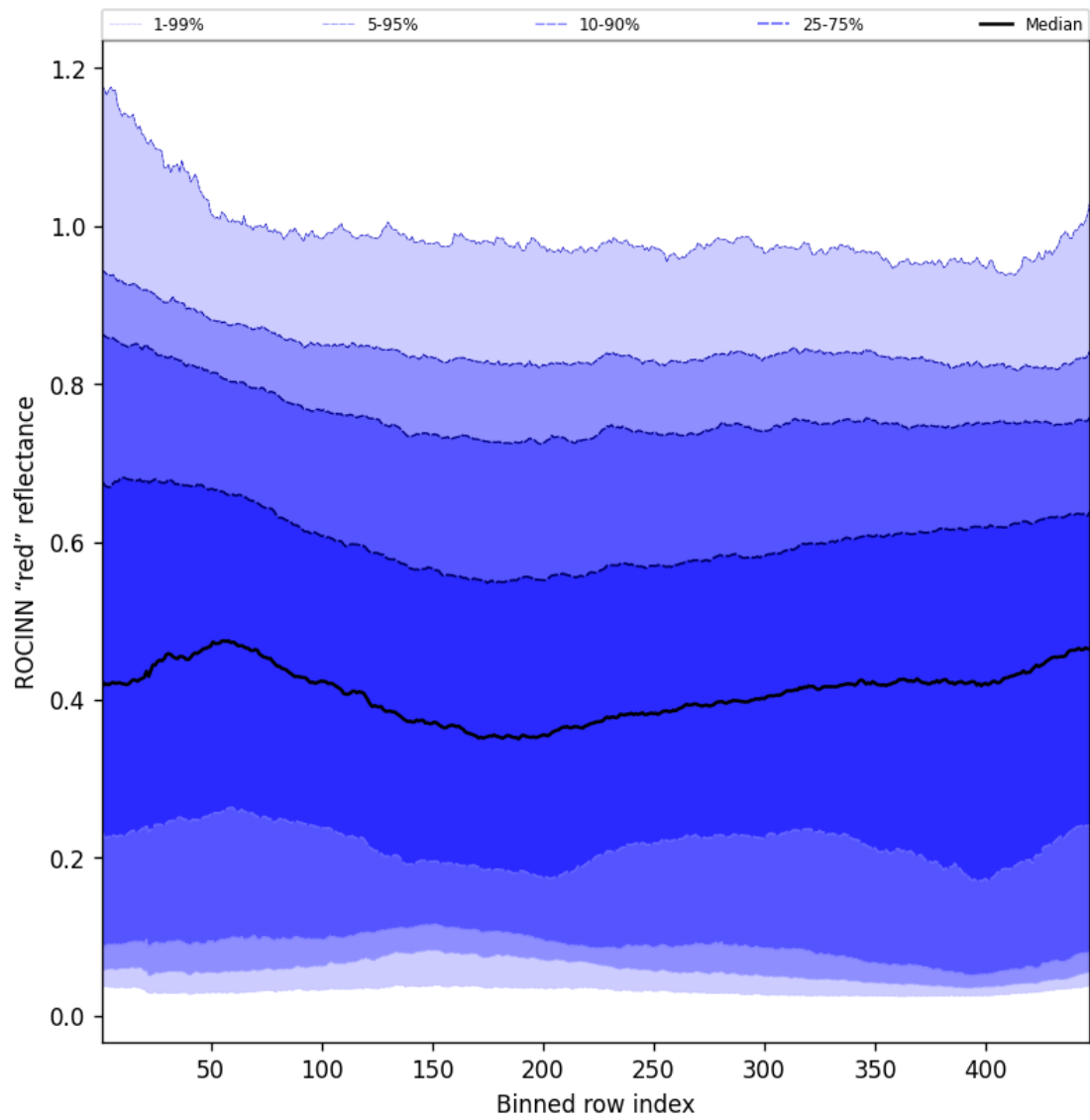
Figure 69: Along track statistics of "ROCINN "red" reflectance" for 2025-08-04 to 2025-08-05
