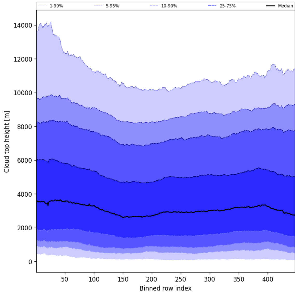
Figure 56: Along track statistics of “Cloud top height” for 2025-08-04 to 2025-08-05
