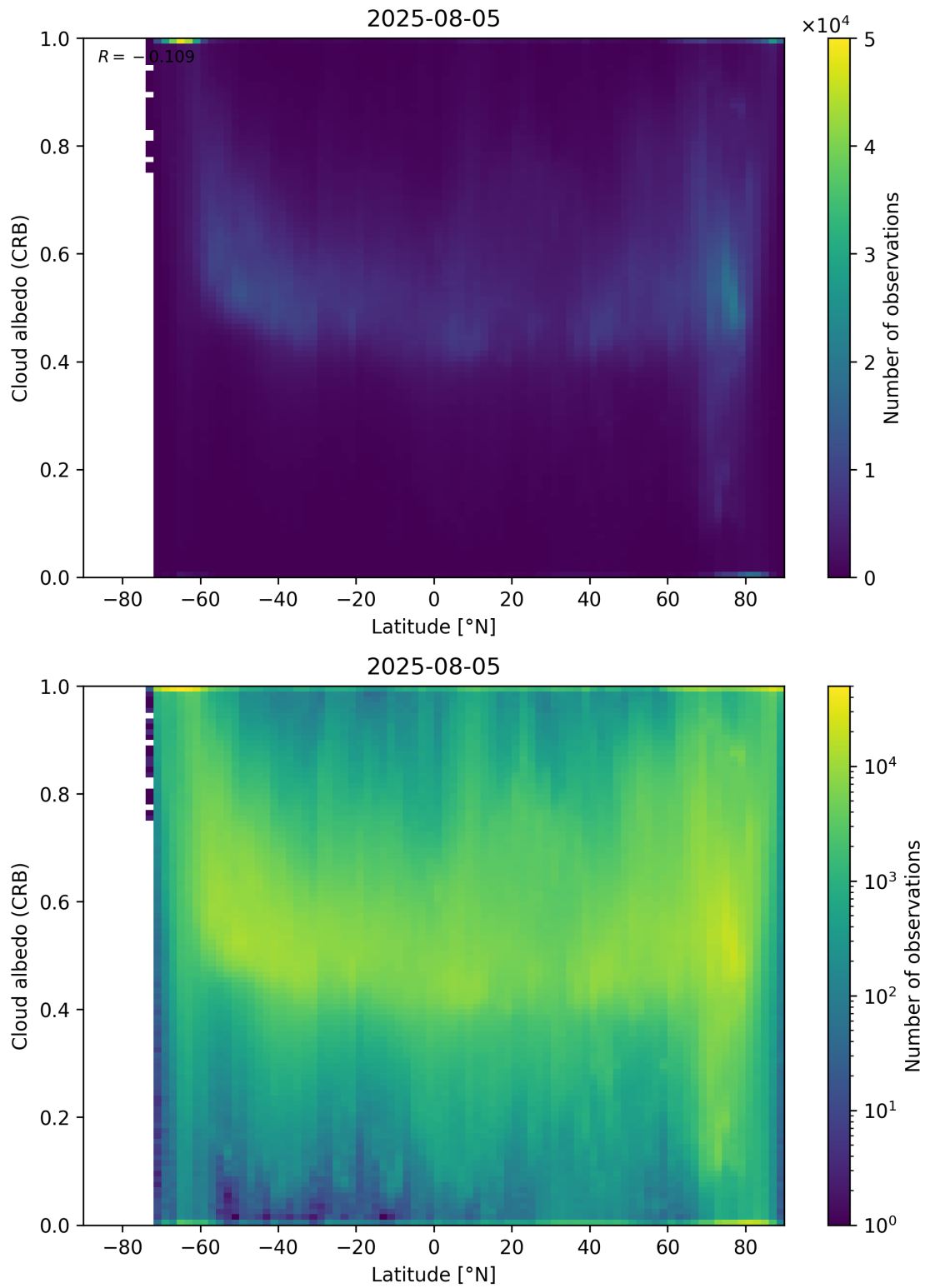
Figure 91: Scatter density plot of “Latitude” against “Cloud albedo (CRB)” for 2025-08-04 to 2025-08-06.
