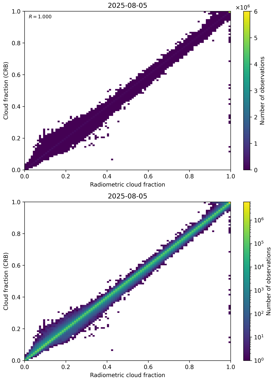
Figure 73: Scatter density plot of “Radiometric cloud fraction” against “Cloud fraction (CRB)” for 2025-08-04 to 2025-08-06.
