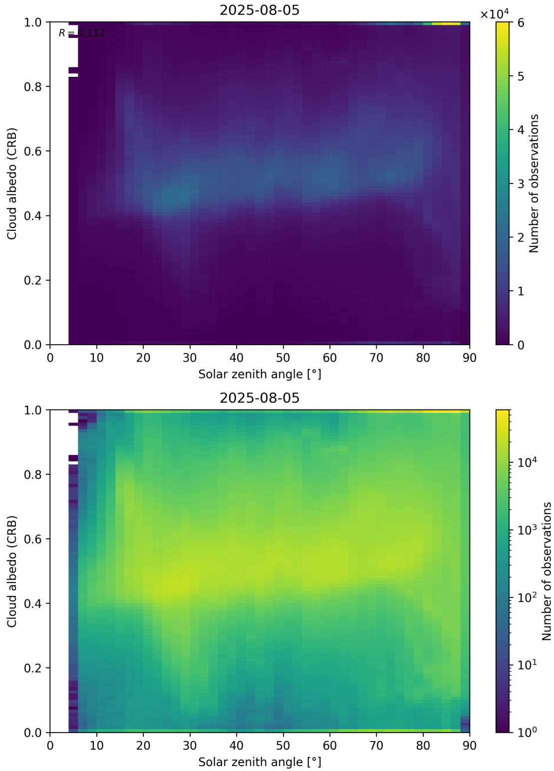
Figure 98: Scatter density plot of “Solar zenith angle” against “Cloud albedo (CRB)” for 2025-08-04 to 2025-08-06.
