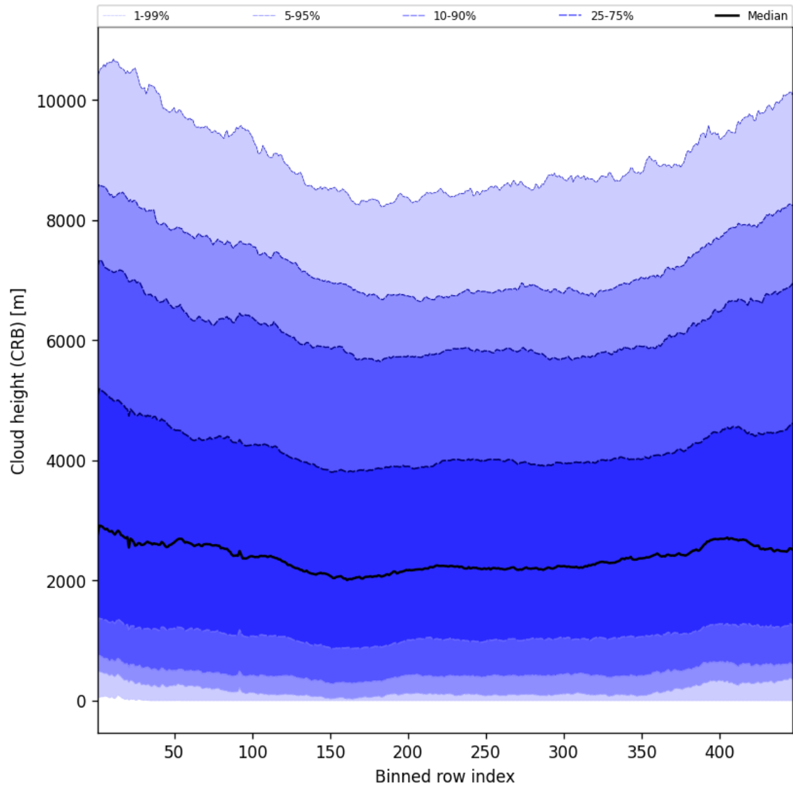
Figure 59: Along track statistics of “Cloud height (CRB)” for 2025-08-04 to 2025-08-06
