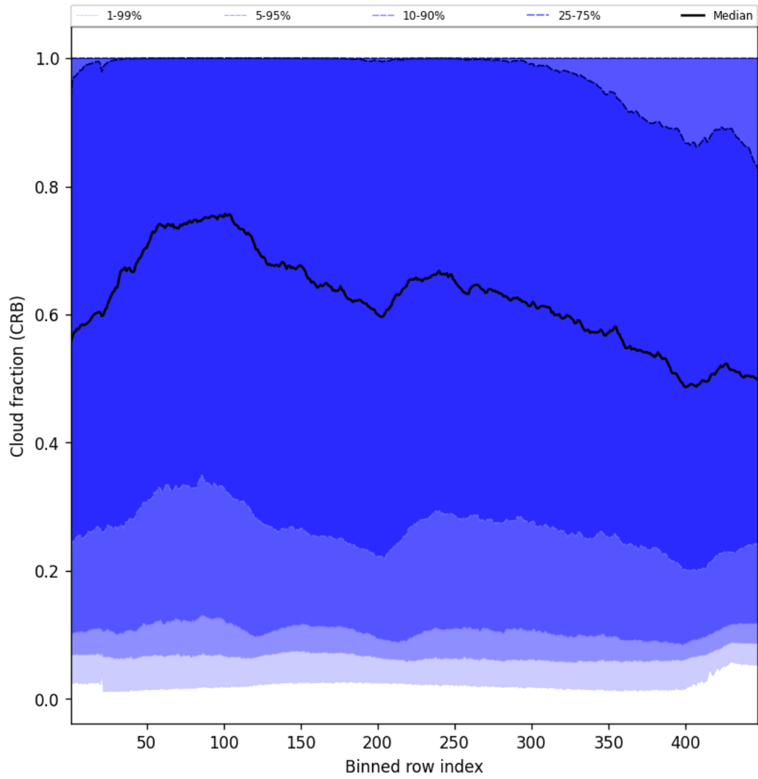
Figure 58: Along track statistics of “Cloud fraction (CRB)” for 2025-08-04 to 2025-08-06
