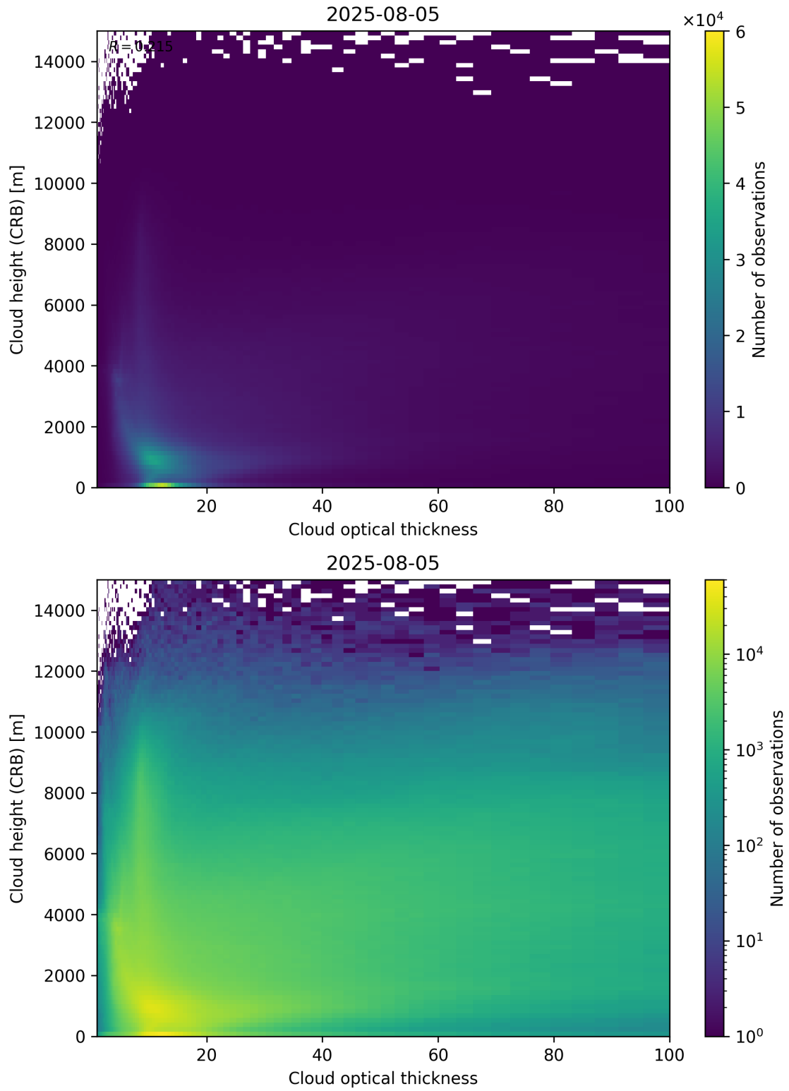
Figure 85: Scatter density plot of “Cloud optical thickness” against “Cloud height (CRB)” for 2025-08-04 to 2025-08-06.
