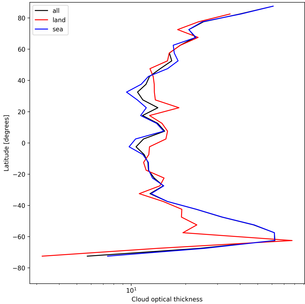
Figure 25: Zonal average of “Cloud optical thickness” for 2025-08-04 to 2025-08-06.
