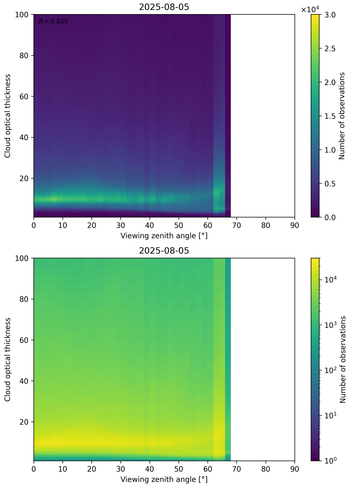
Figure 111: Scatter density plot of “Viewing zenith angle” against “Cloud optical thickness” for 2025-08-04 to 2025-08-06.
