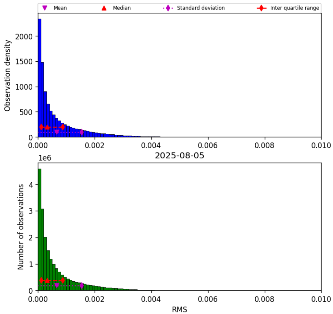
Figure 47: Histogram of “RMS” for 2025-08-04 to 2025-08-06
