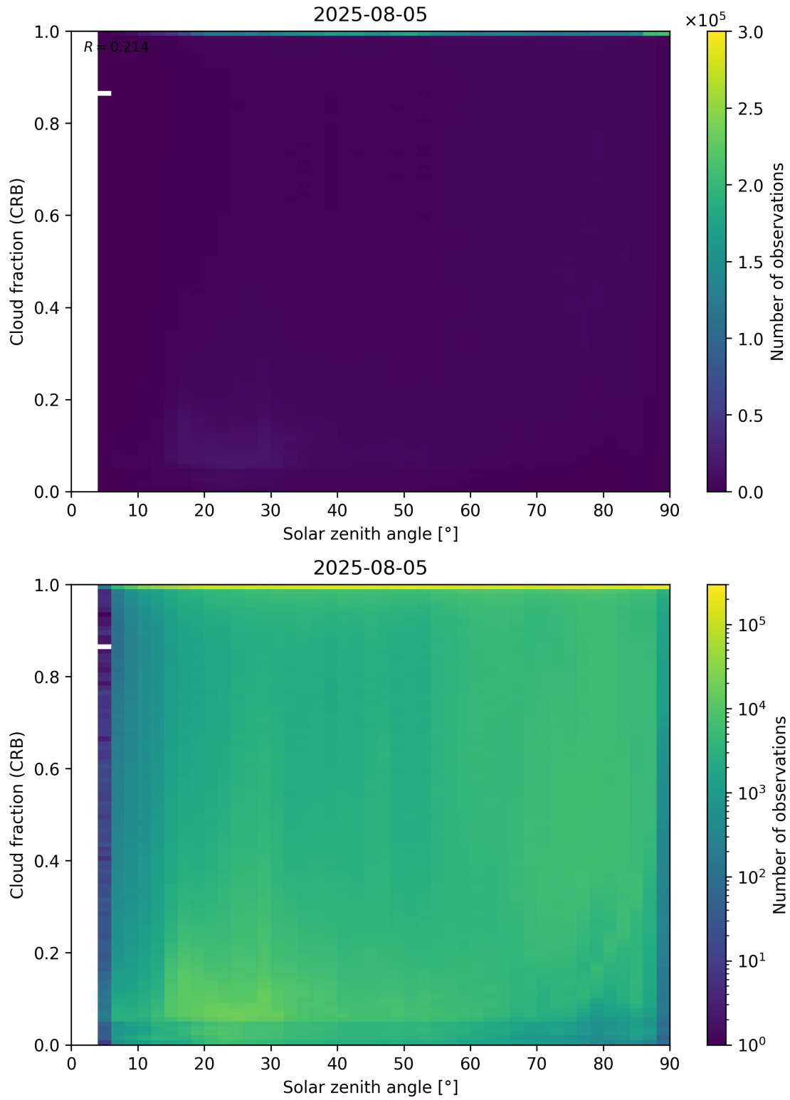
Figure 101: Scatter density plot of “Solar zenith angle” against “Cloud fraction (CRB)” for 2025-08-04 to 2025-08-06.
