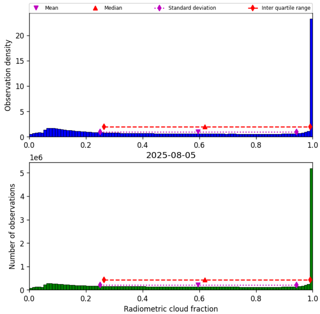
Figure 39: Histogram of “Radiometric cloud fraction” for 2025-08-04 to 2025-08-06
