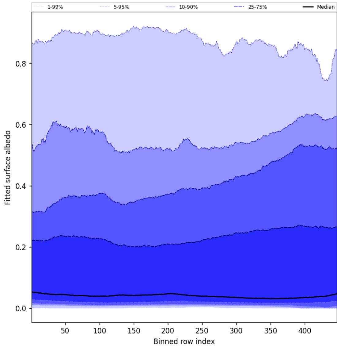
Figure 61: Along track statistics of “Fitted surface albedo” for 2025-08-04 to 2025-08-06
