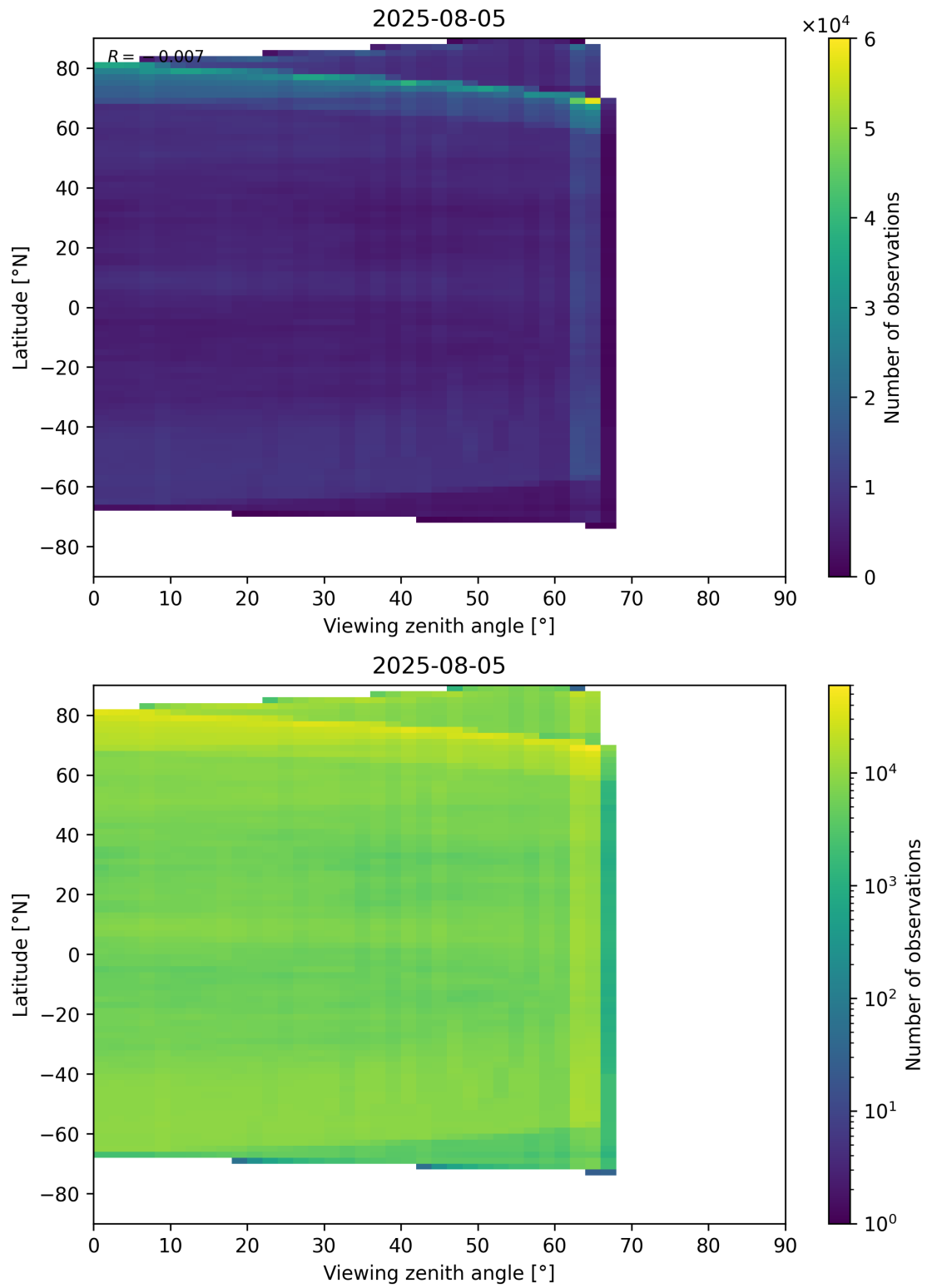
Figure 113: Scatter density plot of “Viewing zenith angle” against “Latitude” for 2025-08-04 to 2025-08-06.
