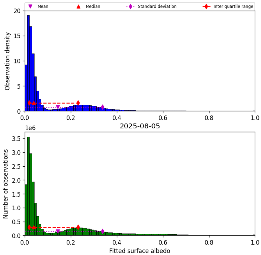
Figure 45: Histogram of “Fitted surface albedo” for 2025-08-04 to 2025-08-06
