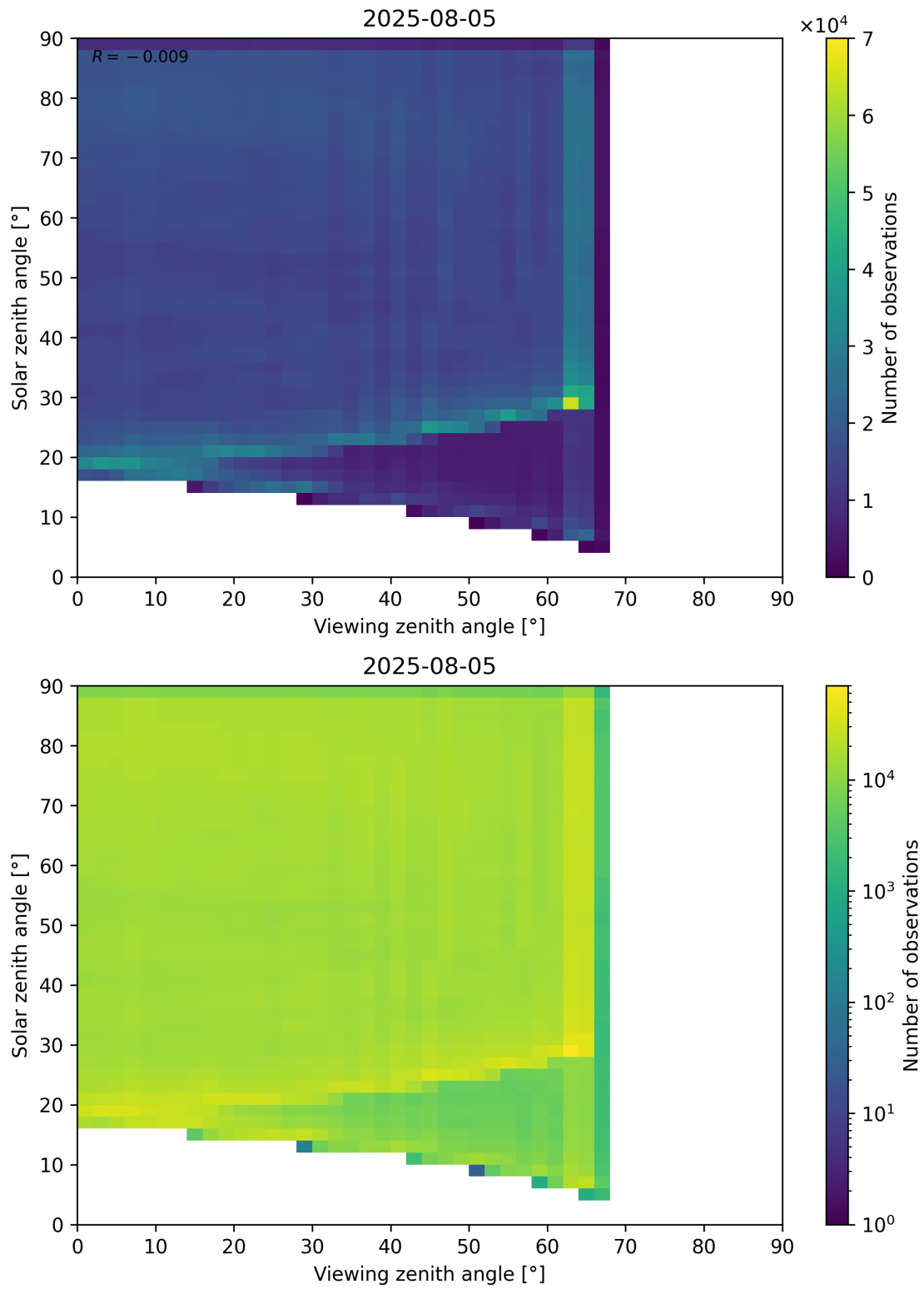
Figure 114: Scatter density plot of “Viewing zenith angle” against “Solar zenith angle” for 2025-08-04 to 2025-08-06.
