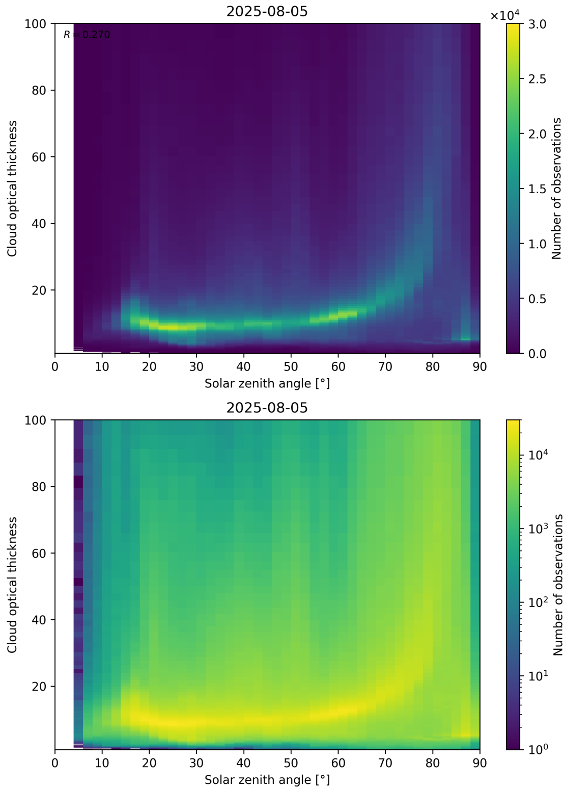
Figure 103: Scatter density plot of “Solar zenith angle” against “Cloud optical thickness” for 2025-08-04 to 2025-08-06.
