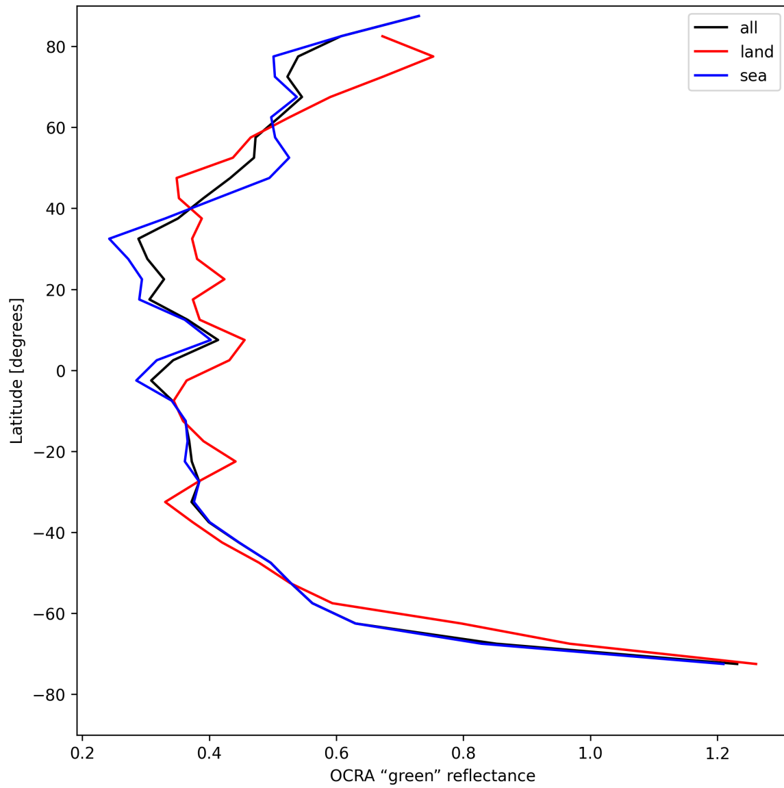
Figure 36: Zonal average of “OCRA “green” reflectance” for 2025-08-04 to 2025-08-06.
