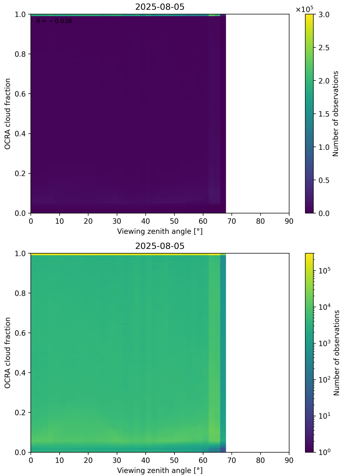
Figure 108: Scatter density plot of “Viewing zenith angle” against “OCRA cloud fraction” for 2025-08-04 to 2025-08-06.
