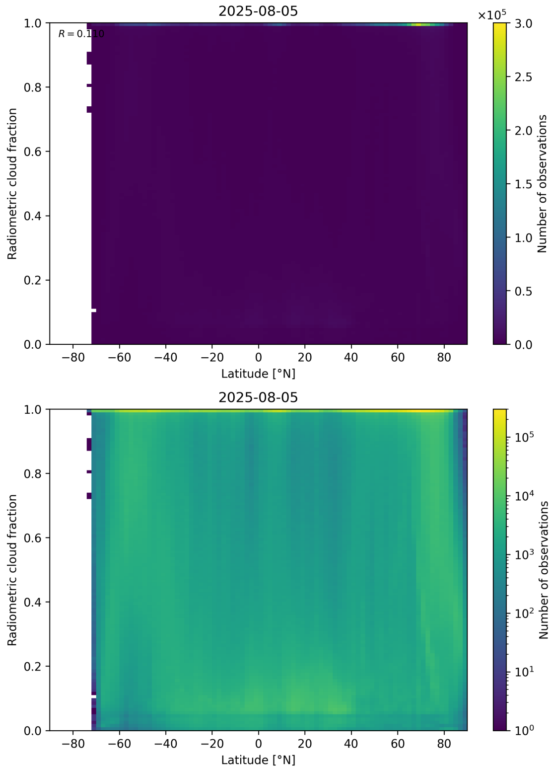
Figure 92: Scatter density plot of “Latitude” against “Radiometric cloud fraction” for 2025-08-04 to 2025-08-06.
