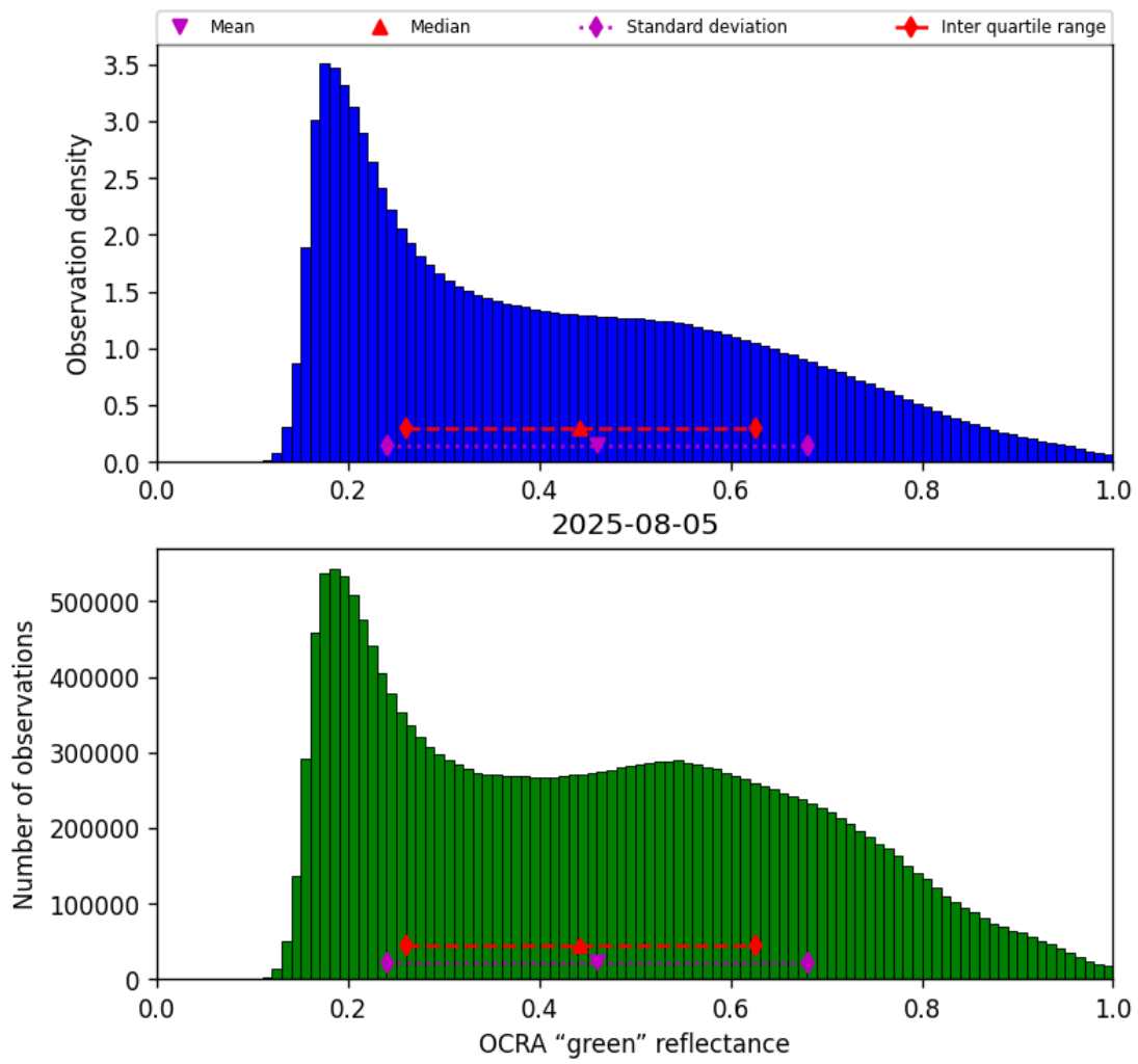
Figure 52: Histogram of “OCRA “green” reflectance” for 2025-08-04 to 2025-08-06
