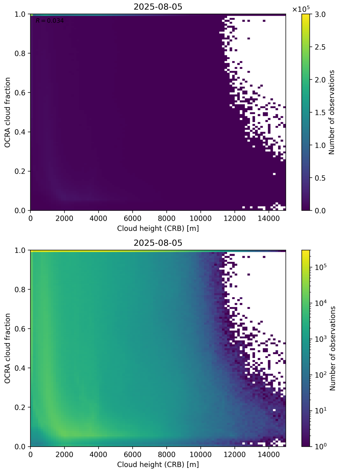
Figure 81: Scatter density plot of “Cloud height (CRB)” against “OCRA cloud fraction” for 2025-08-04 to 2025-08-06.
