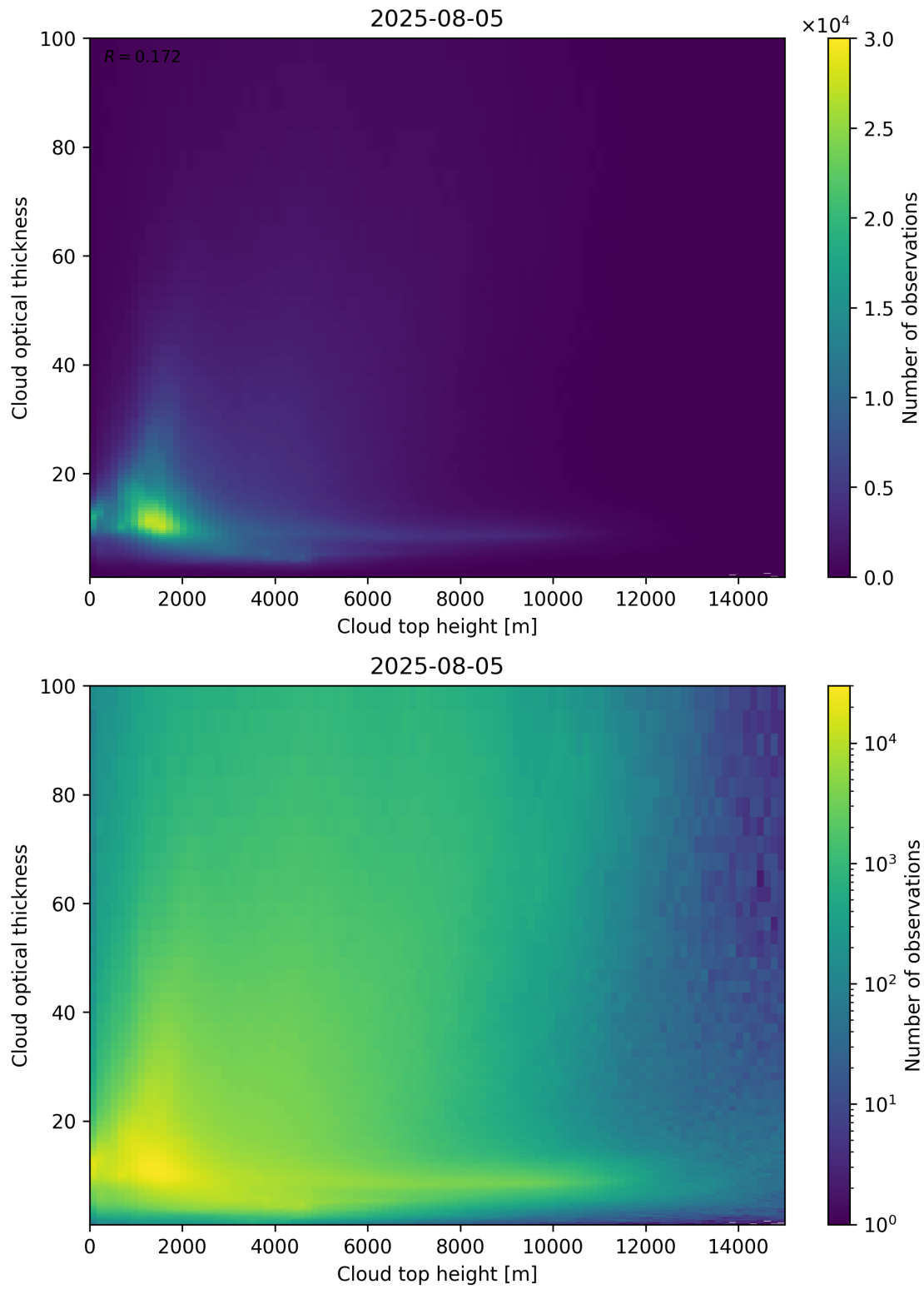
Figure 90: Scatter density plot of “Cloud top height” against “Cloud optical thickness” for 2025-08-04 to 2025-08-06.
