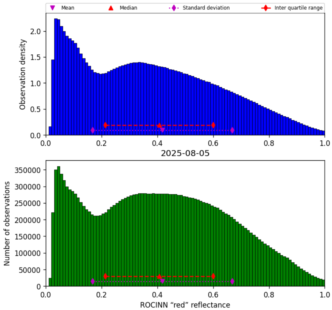
Figure 53: Histogram of “ROCINN “red” reflectance” for 2025-08-04 to 2025-08-06
