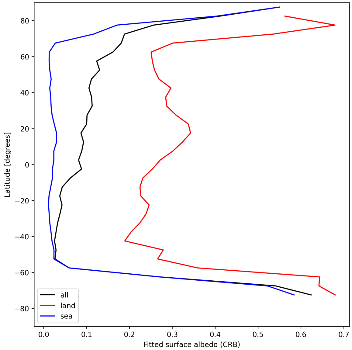
Figure 30: Zonal average of “Fitted surface albedo (CRB)” for 2025-08-04 to 2025-08-06.
