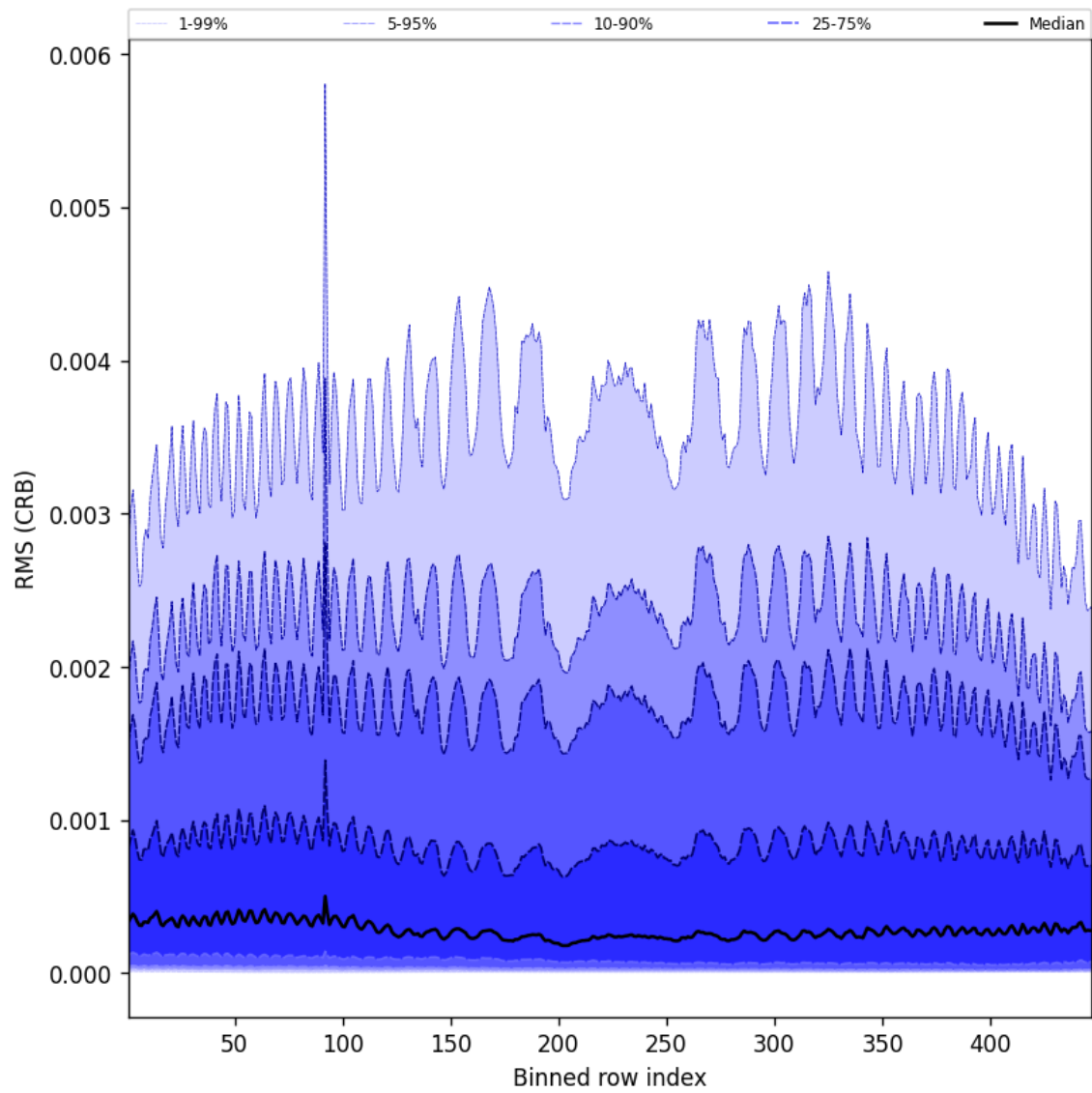
Figure 64: Along track statistics of “RMS (CRB)” for 2025-08-04 to 2025-08-06
