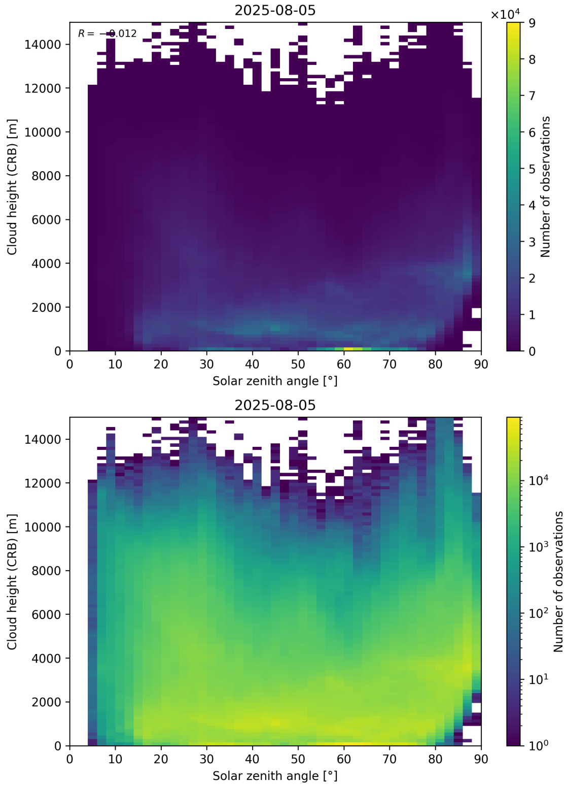
Figure 102: Scatter density plot of “Solar zenith angle” against “Cloud height (CRB)” for 2025-08-04 to 2025-08-06.
