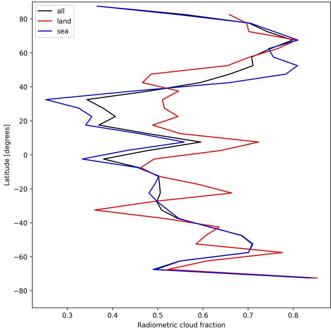
Figure 23: Zonal average of “Radiometric cloud fraction” for 2025-08-04 to 2025-08-06.
