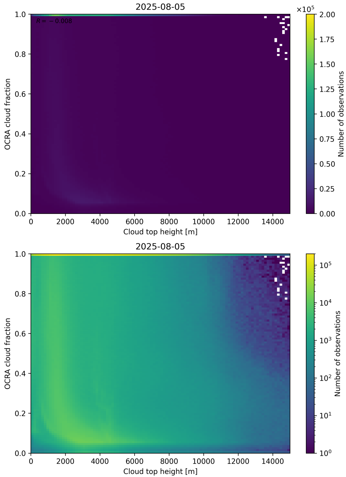
Figure 87: Scatter density plot of “Cloud top height” against “OCRA cloud fraction” for 2025-08-04 to 2025-08-06.
