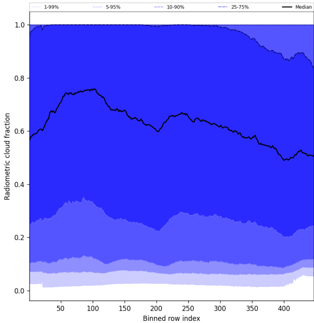
Figure 55: Along track statistics of “Radiometric cloud fraction” for 2025-08-04 to 2025-08-06
