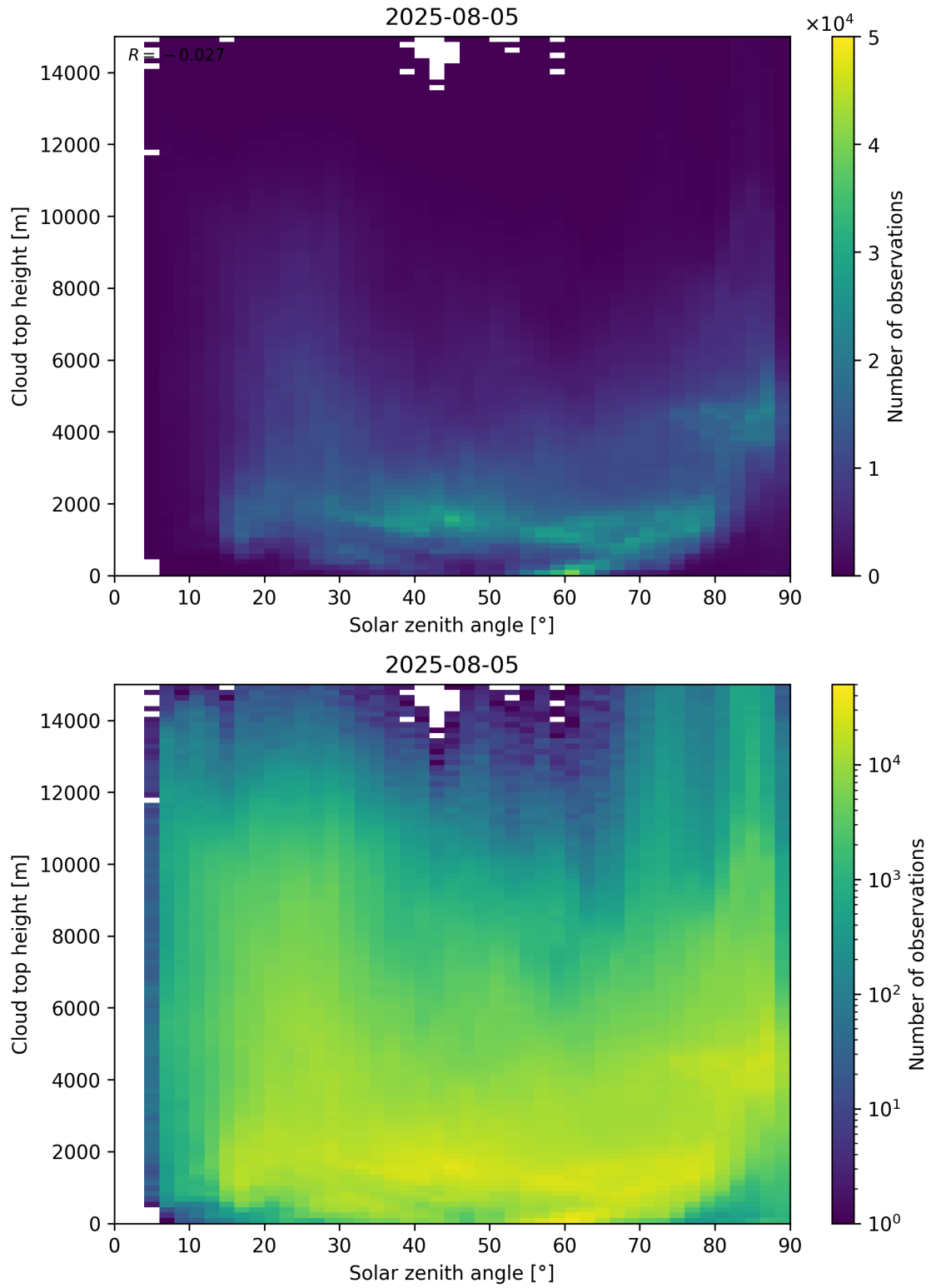
Figure 104: Scatter density plot of “Solar zenith angle” against “Cloud top height” for 2025-08-04 to 2025-08-06.
