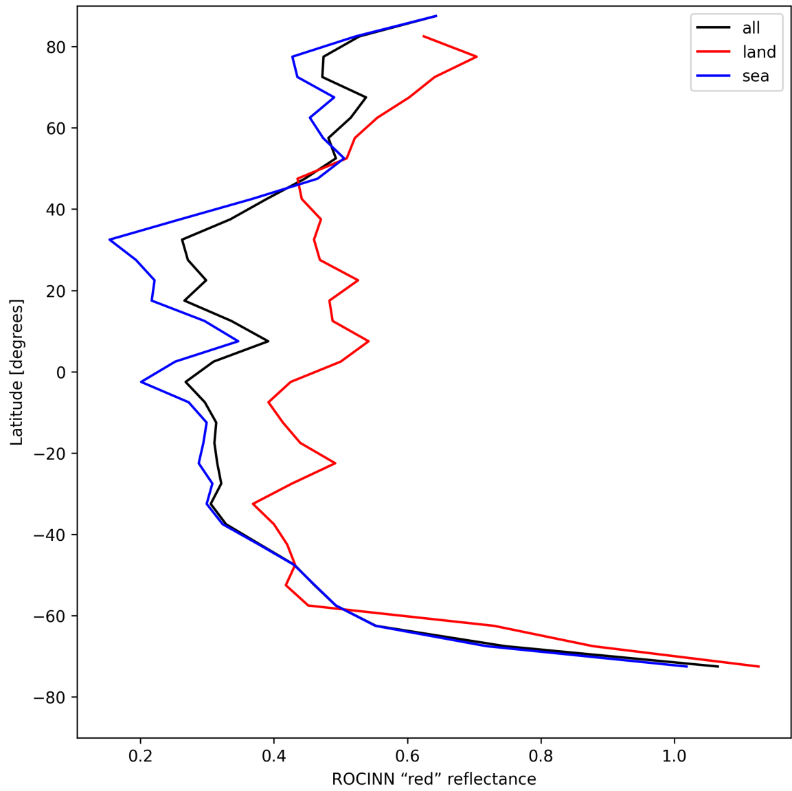
Figure 37: Zonal average of “ROCINN “red” reflectance” for 2025-08-04 to 2025-08-06.
