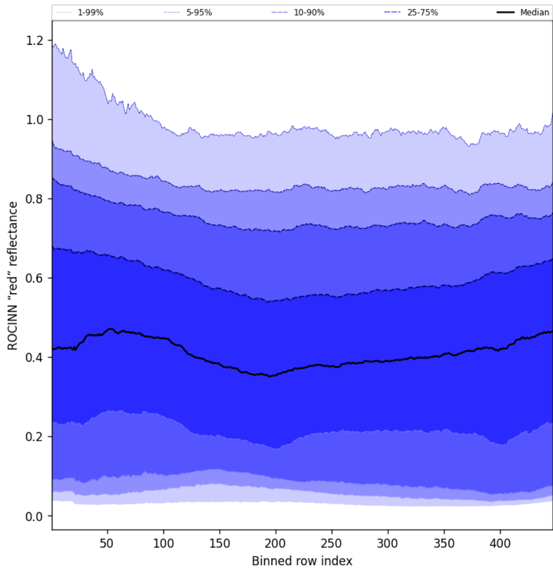
Figure 69: Along track statistics of “ROCINN “red” reflectance” for 2025-08-04 to 2025-08-06
