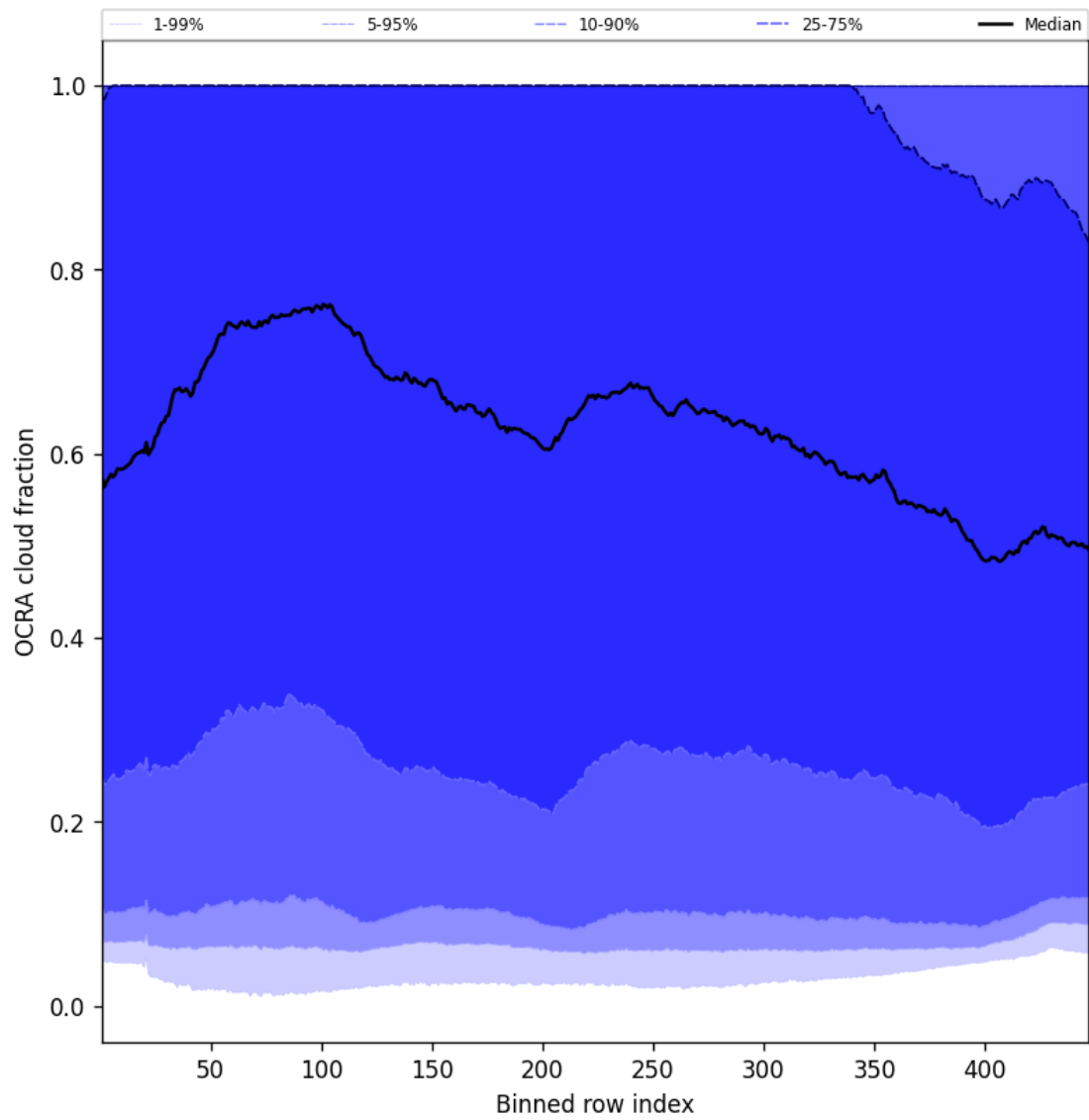
Figure 66: Along track statistics of “OCRA cloud fraction” for 2025-08-04 to 2025-08-06
