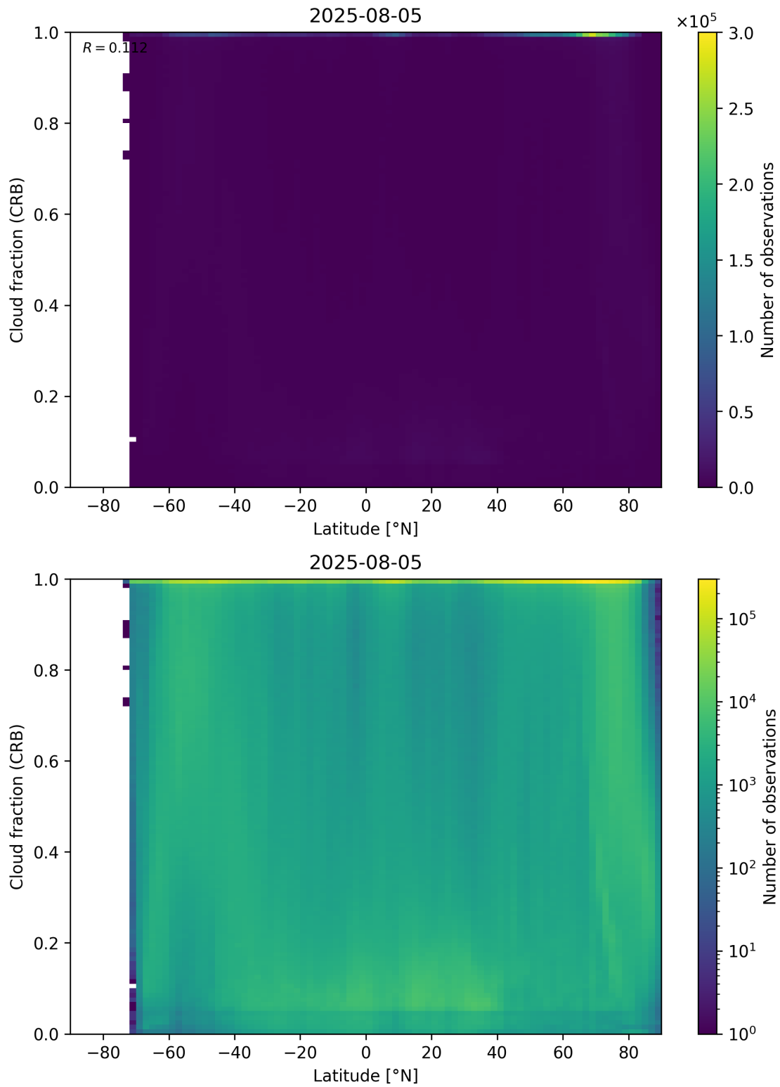
Figure 94: Scatter density plot of “Latitude” against “Cloud fraction (CRB)” for 2025-08-04 to 2025-08-06.
