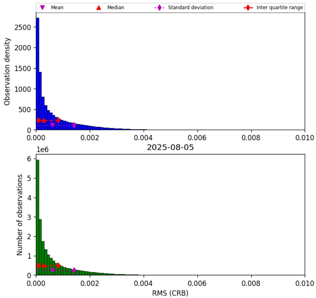
Figure 48: Histogram of “RMS (CRB)” for 2025-08-04 to 2025-08-06
