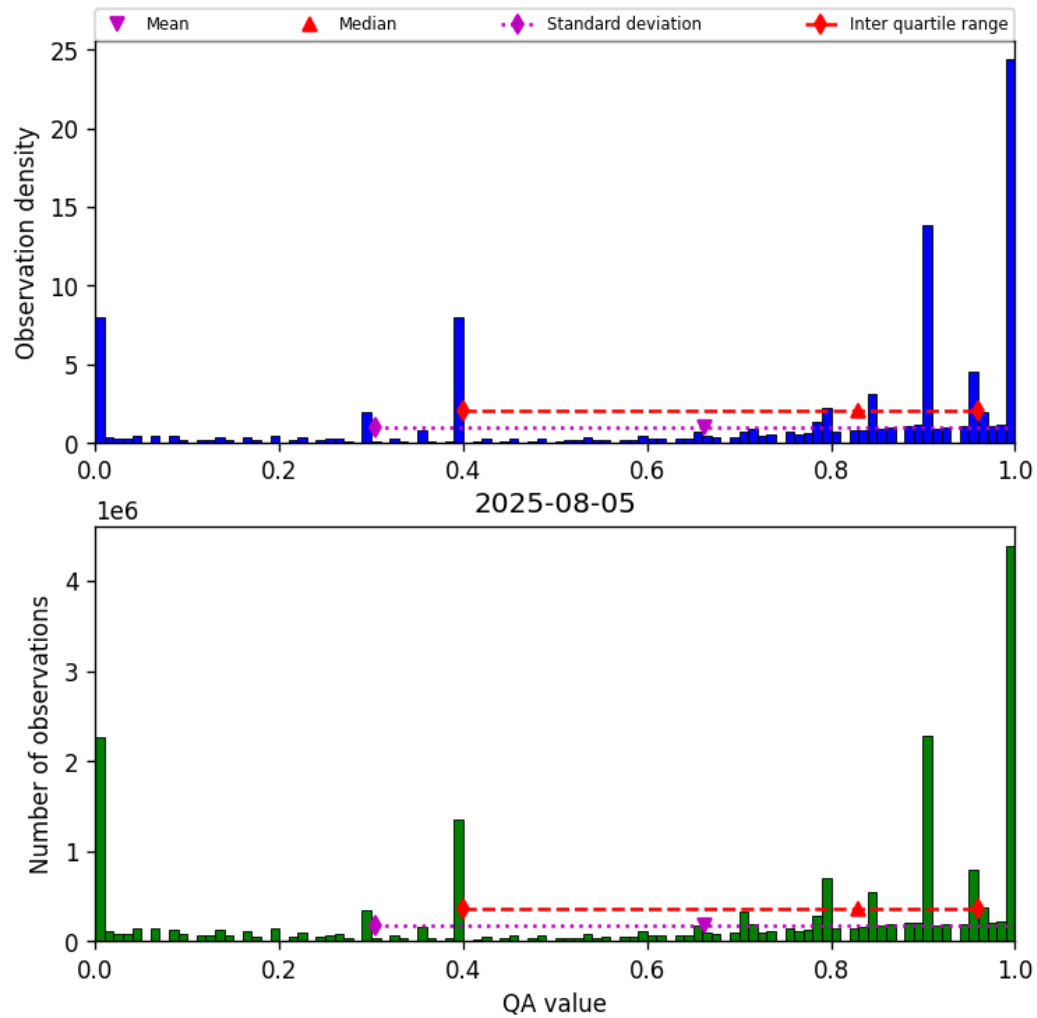
Figure 38: Histogram of “QA value” for 2025-08-04 to 2025-08-06
