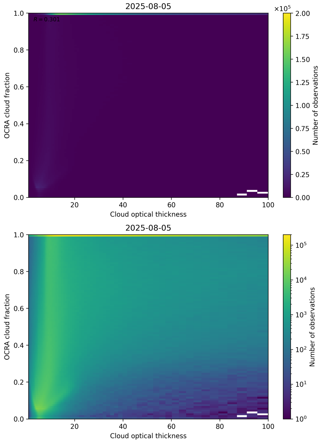
Figure 83: Scatter density plot of “Cloud optical thickness” against “OCRA cloud fraction” for 2025-08-04 to 2025-08-06.
