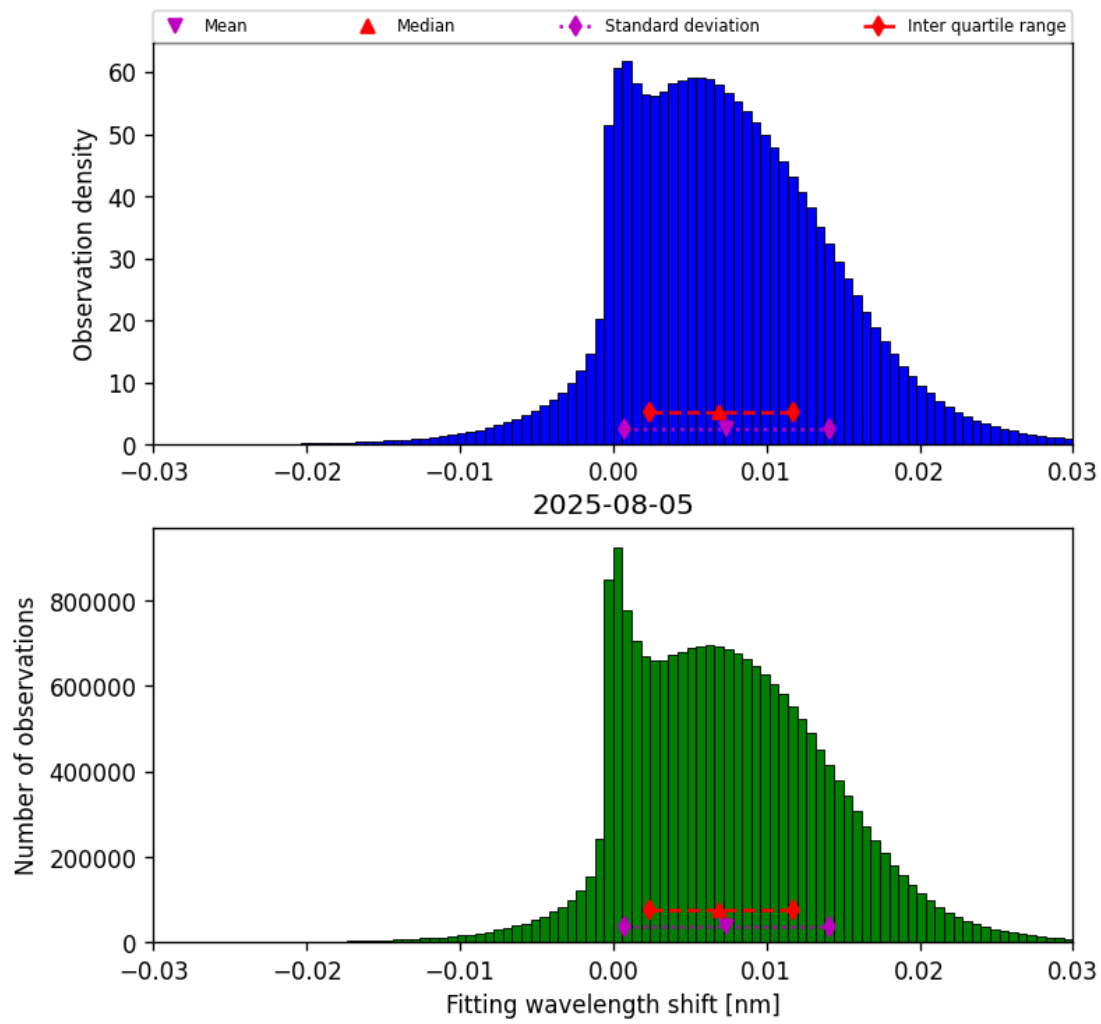
Figure 49: Histogram of “Fitting wavelength shift” for 2025-08-04 to 2025-08-06
