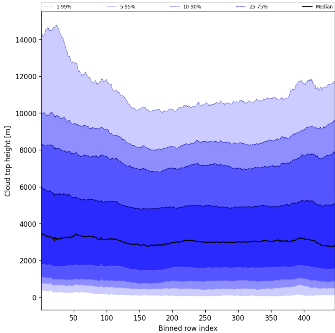
Figure 56: Along track statistics of “Cloud top height” for 2025-08-04 to 2025-08-06
