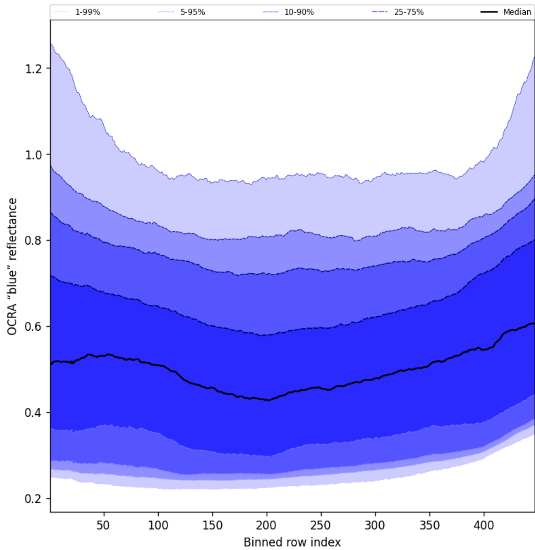
Figure 67: Along track statistics of "OCRA "blue" reflectance" for 2025-08-04 to 2025-08-06
