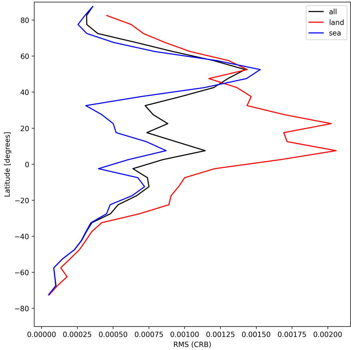
Figure 32: Zonal average of “RMS (CRB)” for 2025-08-04 to 2025-08-06.
