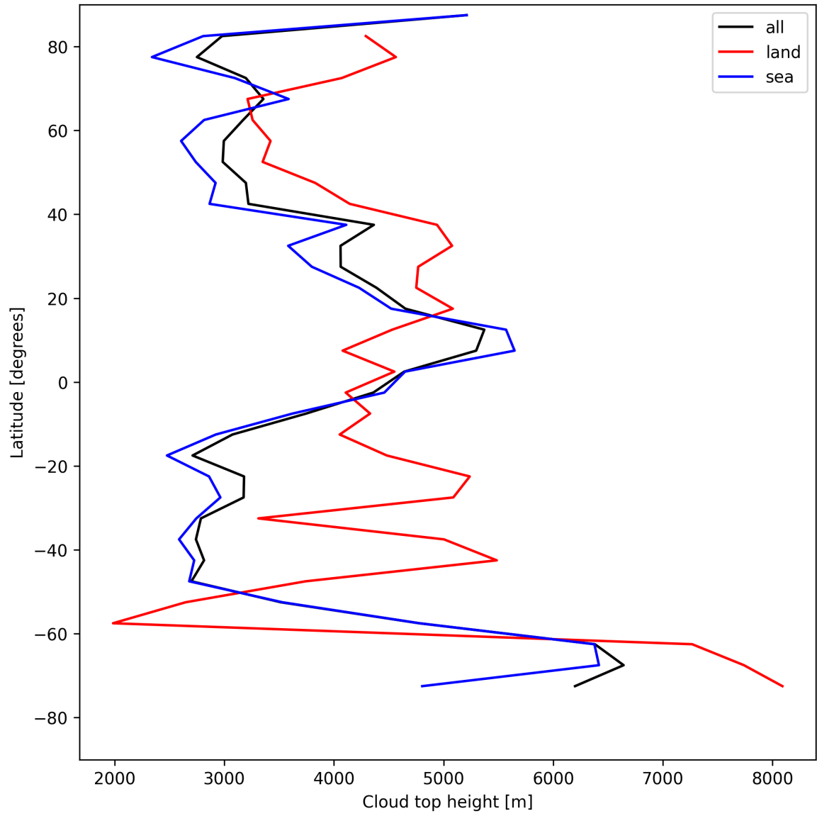
Figure 24: Zonal average of “Cloud top height” for 2025-08-04 to 2025-08-06.
