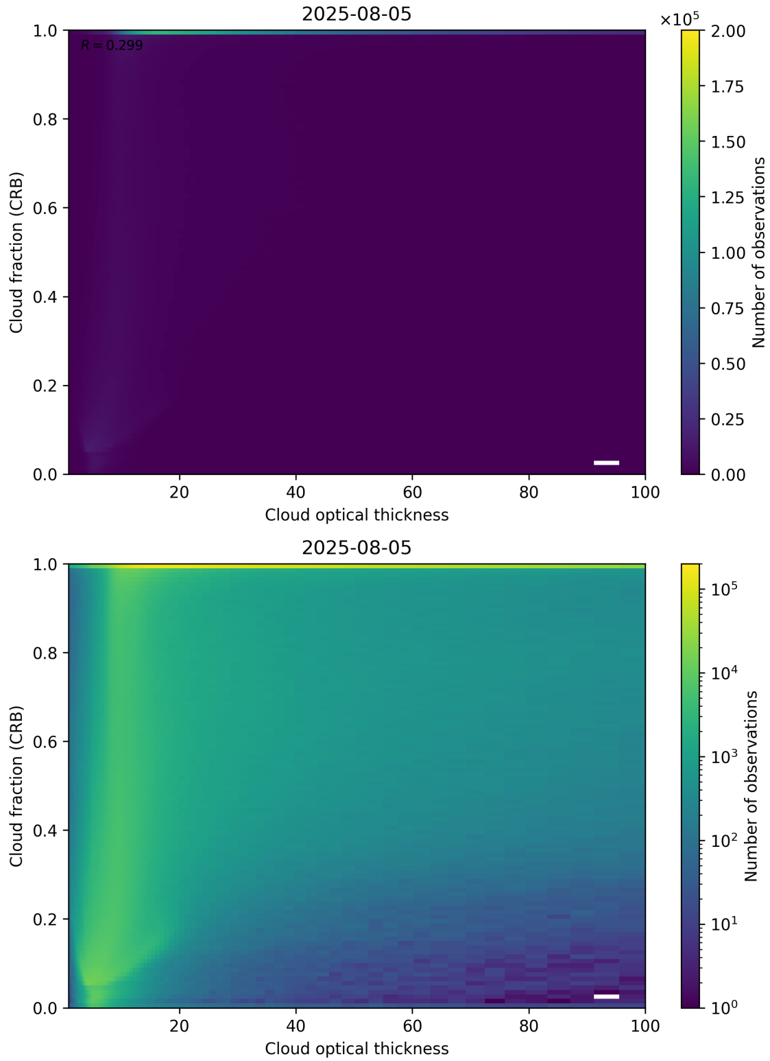
Figure 84: Scatter density plot of “Cloud optical thickness” against “Cloud fraction (CRB)” for 2025-08-04 to 2025-08-06.
