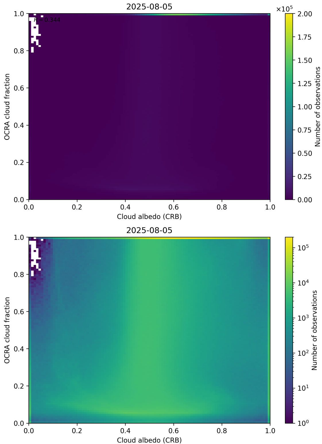
Figure 70: Scatter density plot of “Cloud albedo (CRB)” against “OCRA cloud fraction” for 2025-08-04 to 2025-08-06.
