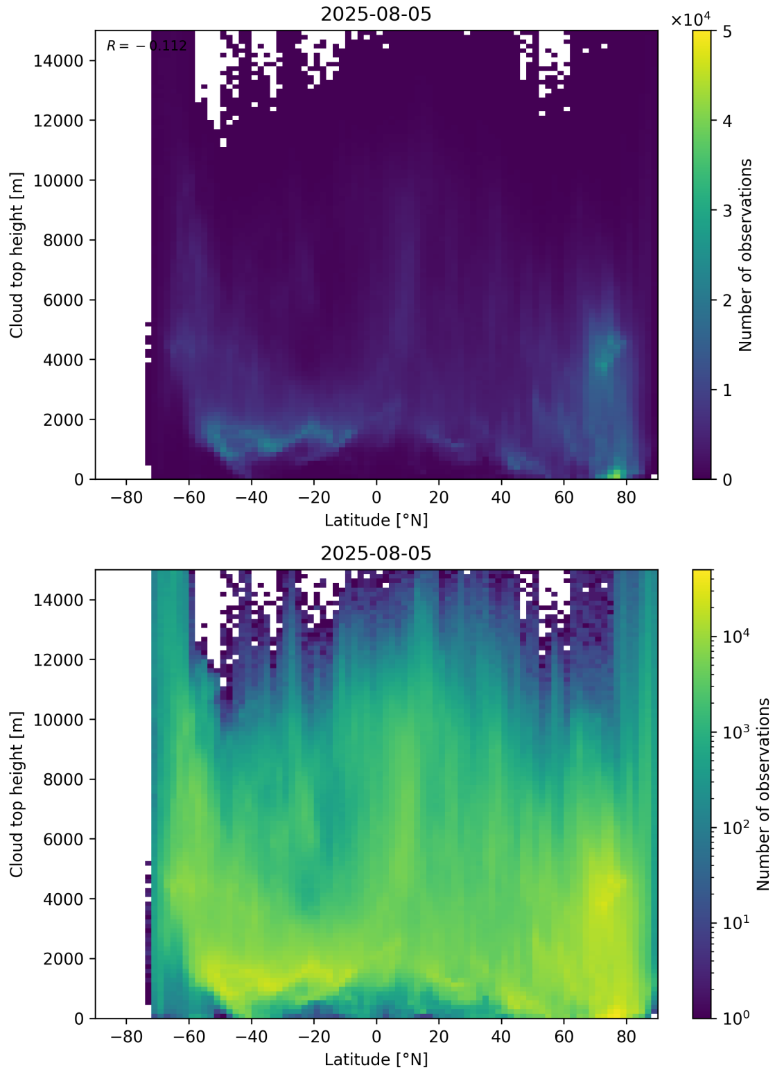
Figure 97: Scatter density plot of “Latitude” against “Cloud top height” for 2025-08-04 to 2025-08-06.
