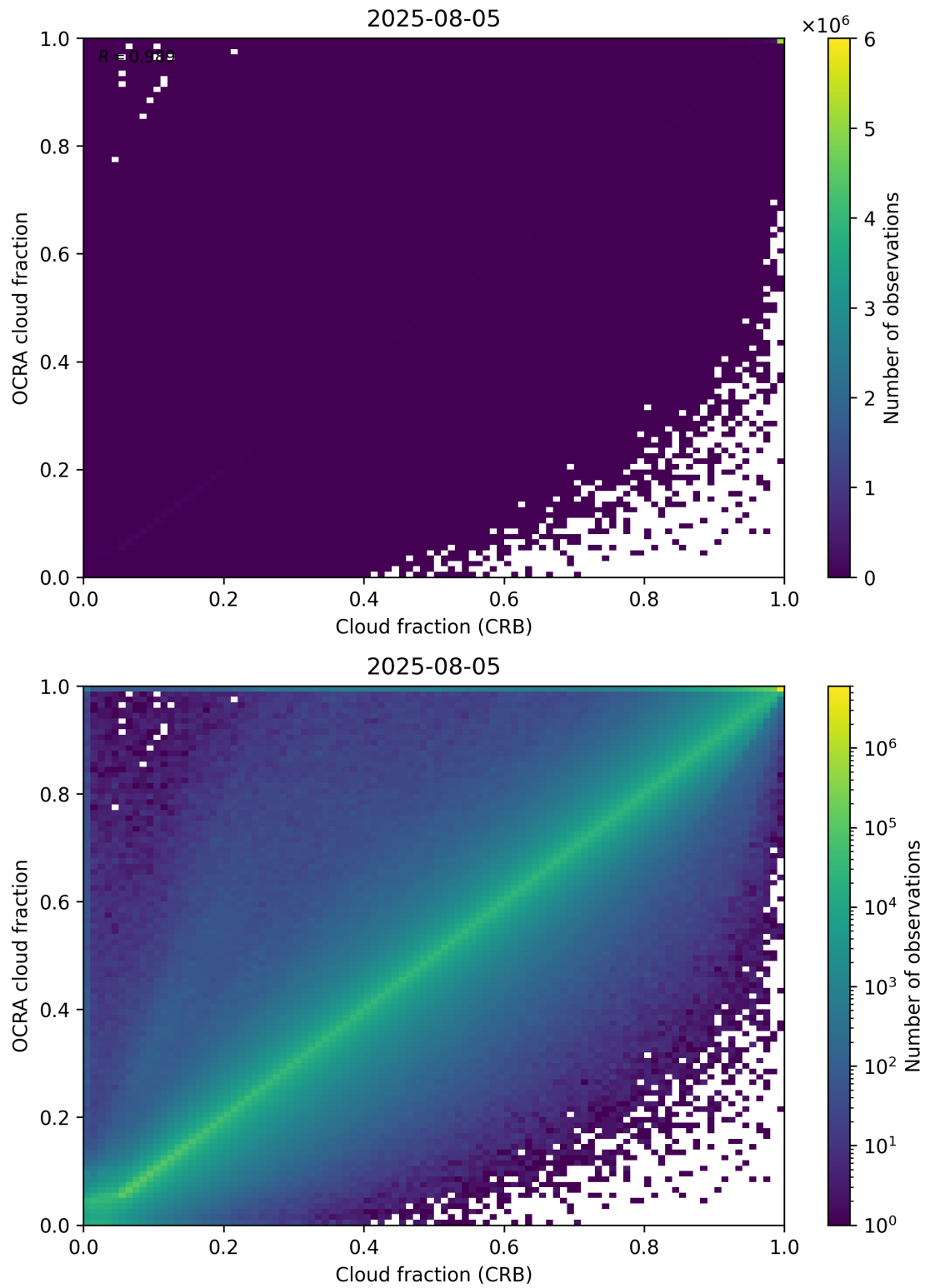
Figure 78: Scatter density plot of “Cloud fraction (CRB)” against “OCRA cloud fraction” for 2025-08-04 to 2025-08-06.
