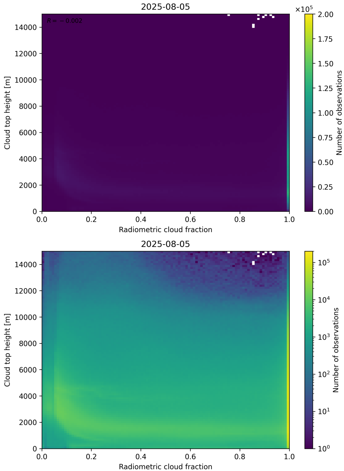
Figure 76: Scatter density plot of “Radiometric cloud fraction” against “Cloud top height” for 2025-08-04 to 2025-08-06.
