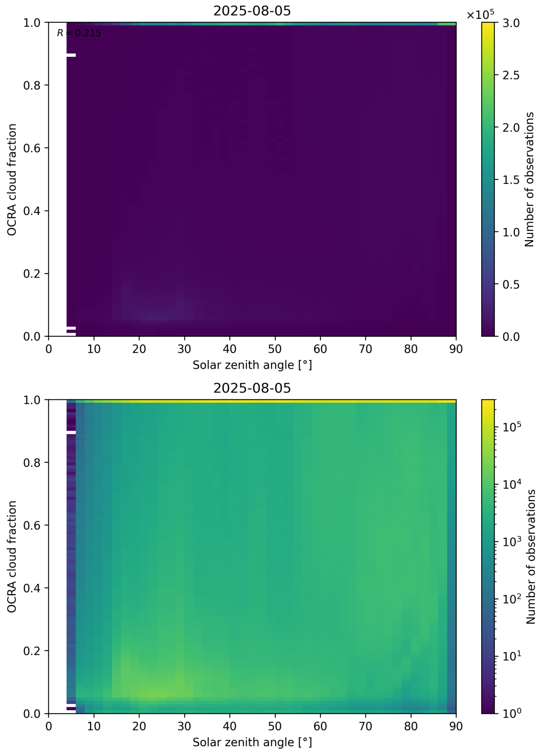
Figure 100: Scatter density plot of “Solar zenith angle” against “OCRA cloud fraction” for 2025-08-04 to 2025-08-06.
