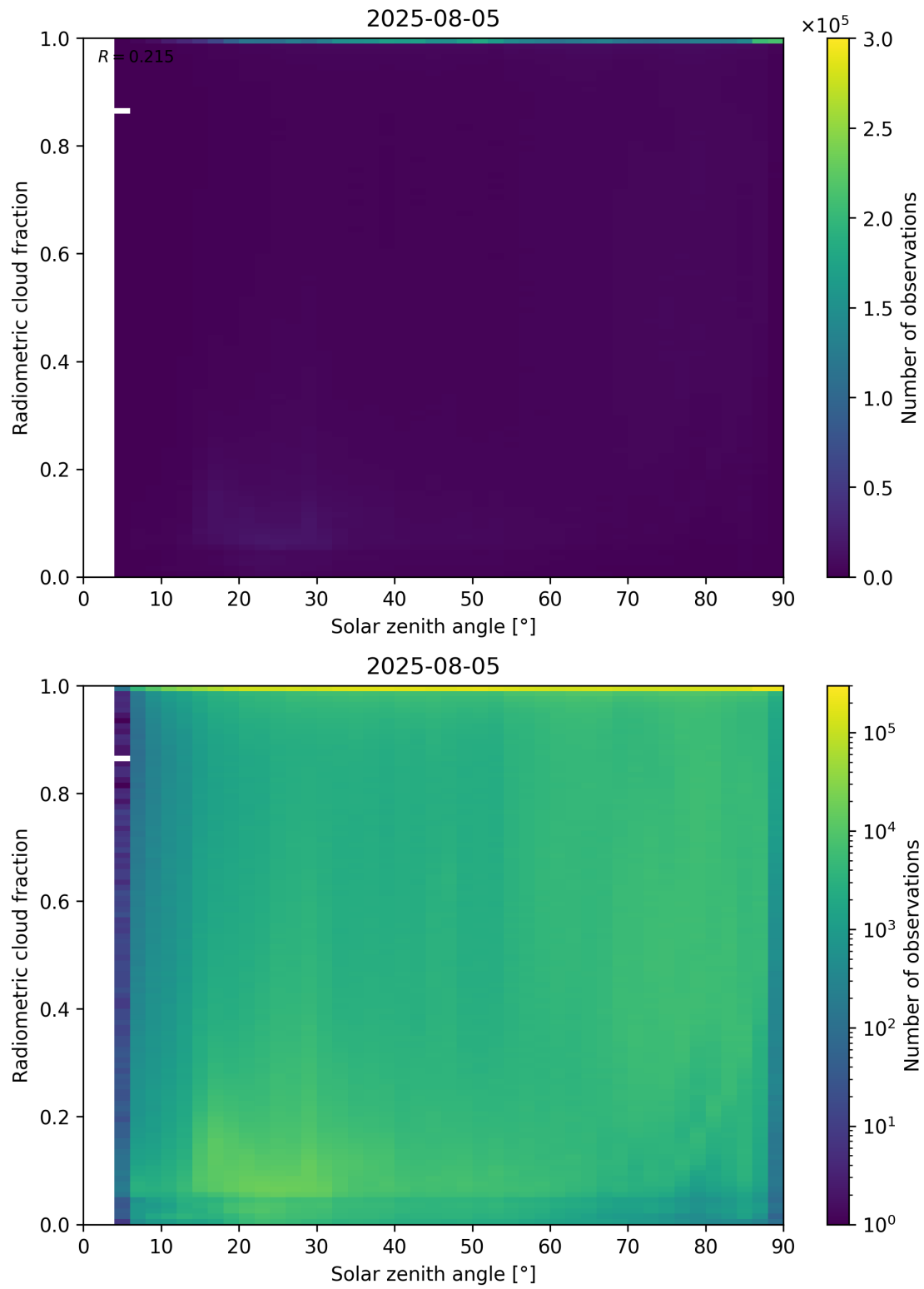
Figure 99: Scatter density plot of “Solar zenith angle” against “Radiometric cloud fraction” for 2025-08-04 to 2025-08-06.
