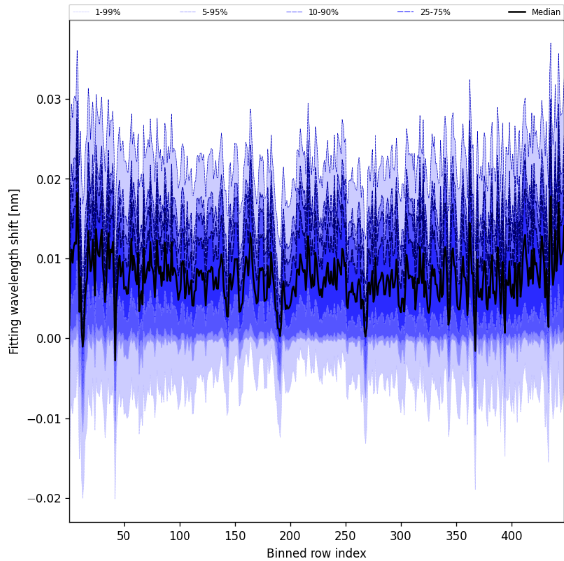
Figure 65: Along track statistics of “Fitting wavelength shift” for 2025-08-04 to 2025-08-06
