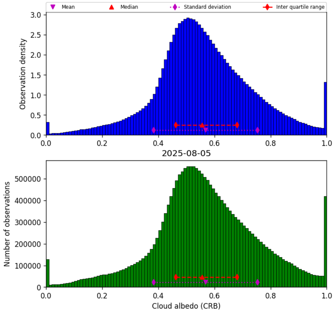
Figure 44: Histogram of “Cloud albedo (CRB)” for 2025-08-04 to 2025-08-06
