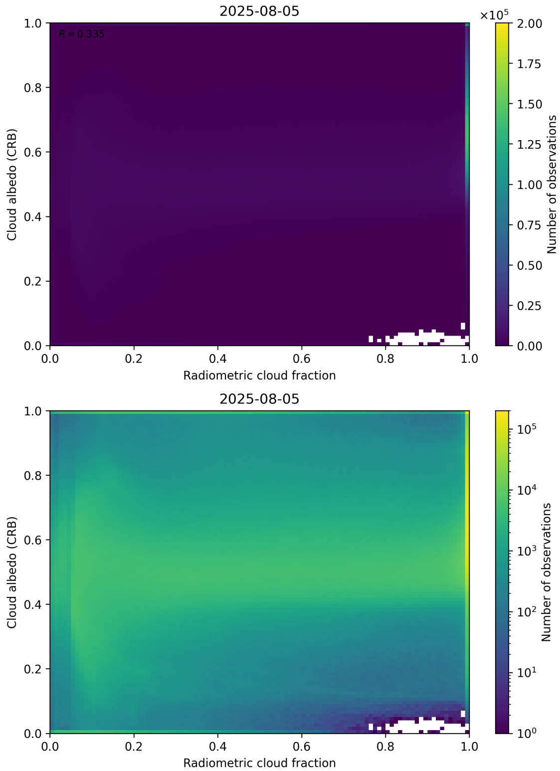
Figure 71: Scatter density plot of “Radiometric cloud fraction” against “Cloud albedo (CRB)” for 2025-08-04 to 2025-08-06.
