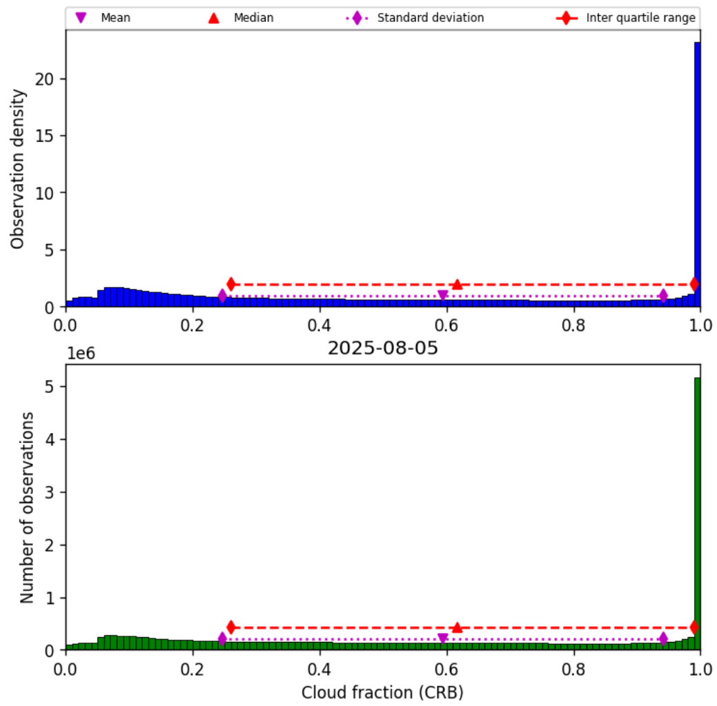
Figure 42: Histogram of “Cloud fraction (CRB)” for 2025-08-04 to 2025-08-06
