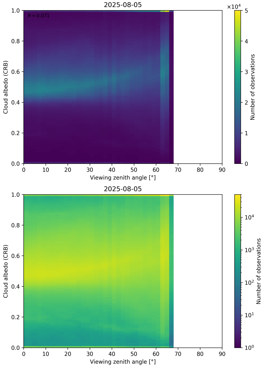
Figure 106: Scatter density plot of “Viewing zenith angle” against “Cloud albedo (CRB)” for 2025-08-04 to 2025-08-06.
