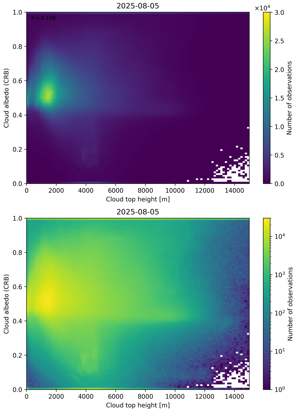
Figure 86: Scatter density plot of “Cloud top height” against “Cloud albedo (CRB)” for 2025-08-04 to 2025-08-06.
