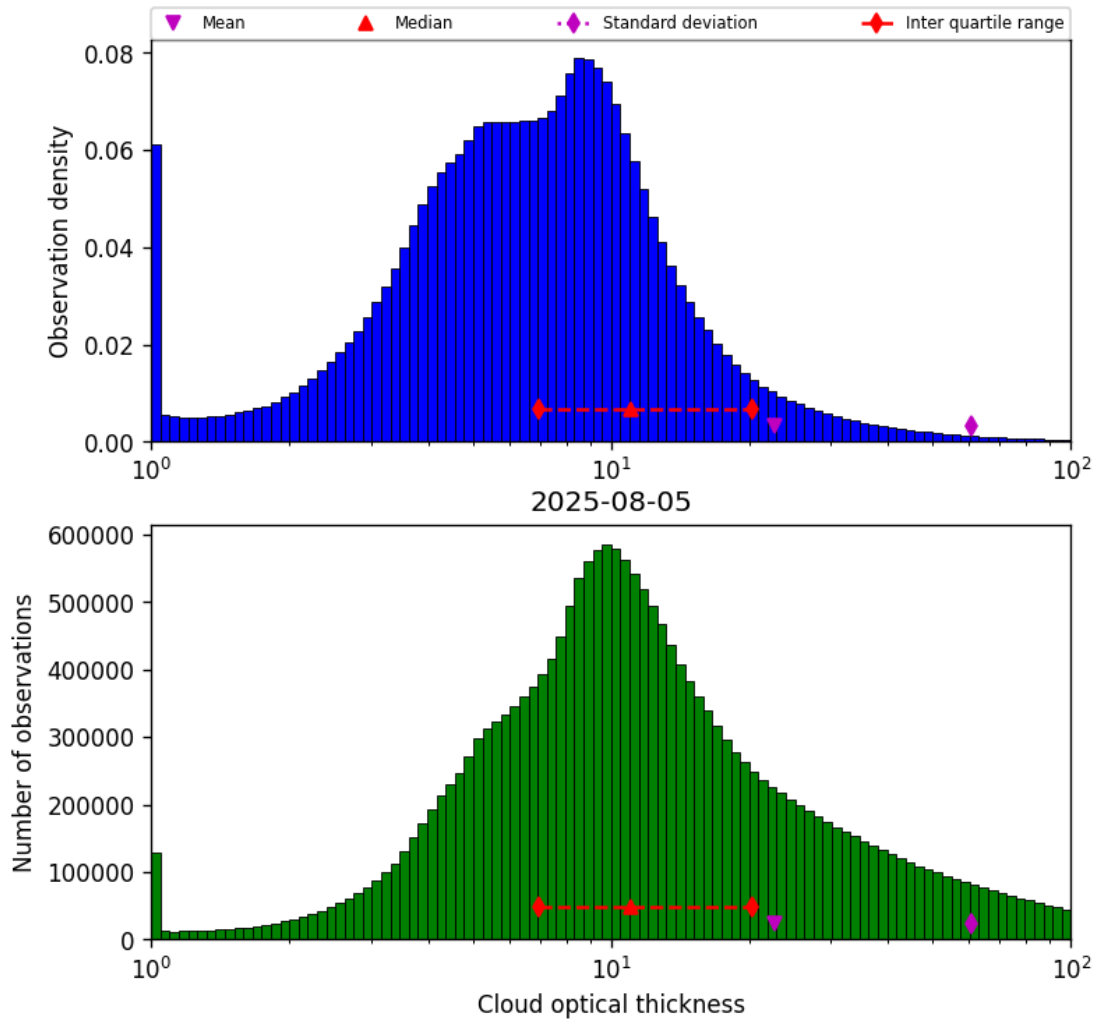
Figure 41: Histogram of “Cloud optical thickness” for 2025-08-04 to 2025-08-06
