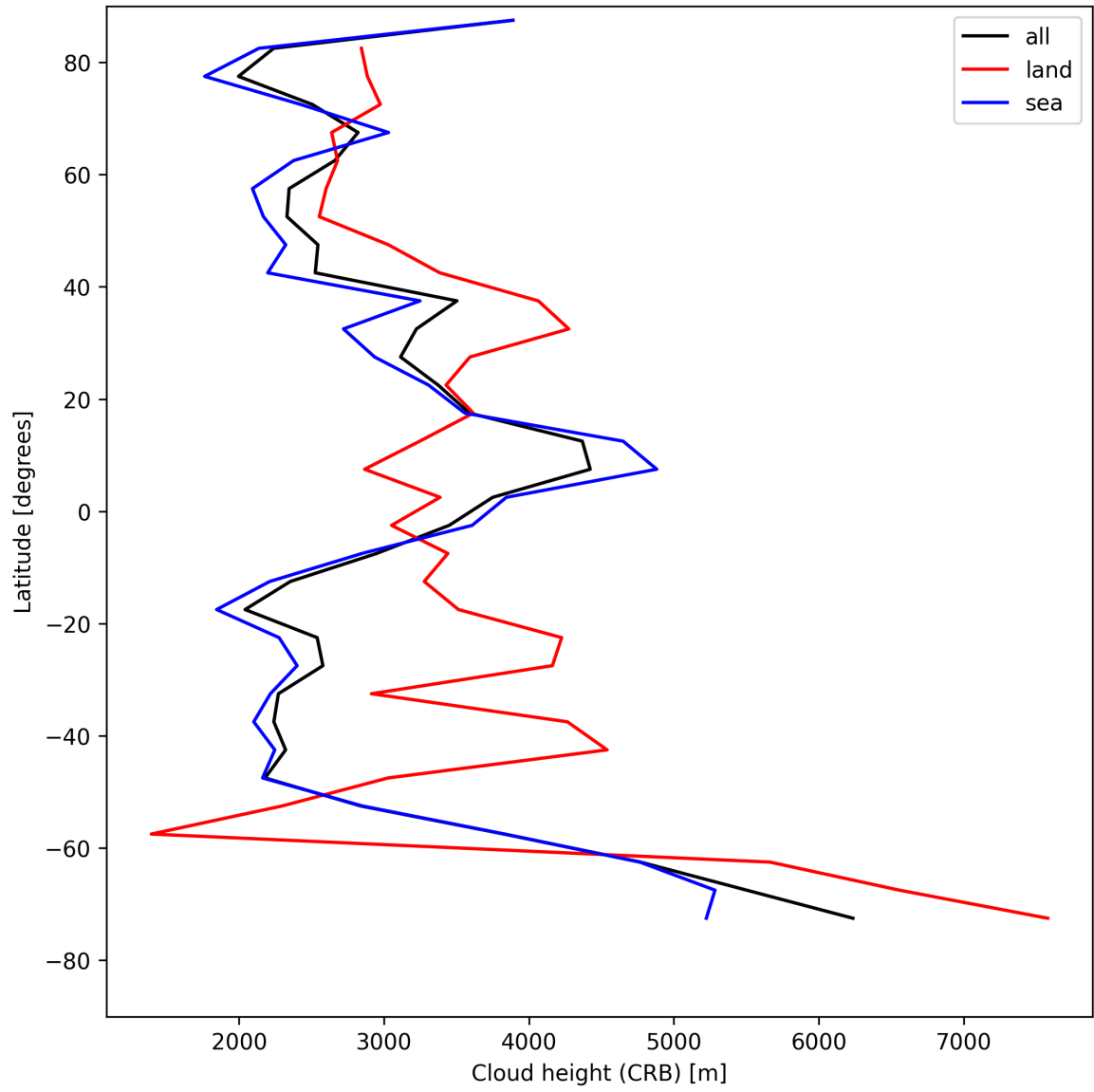
Figure 27: Zonal average of “Cloud height (CRB)” for 2025-08-04 to 2025-08-06.
