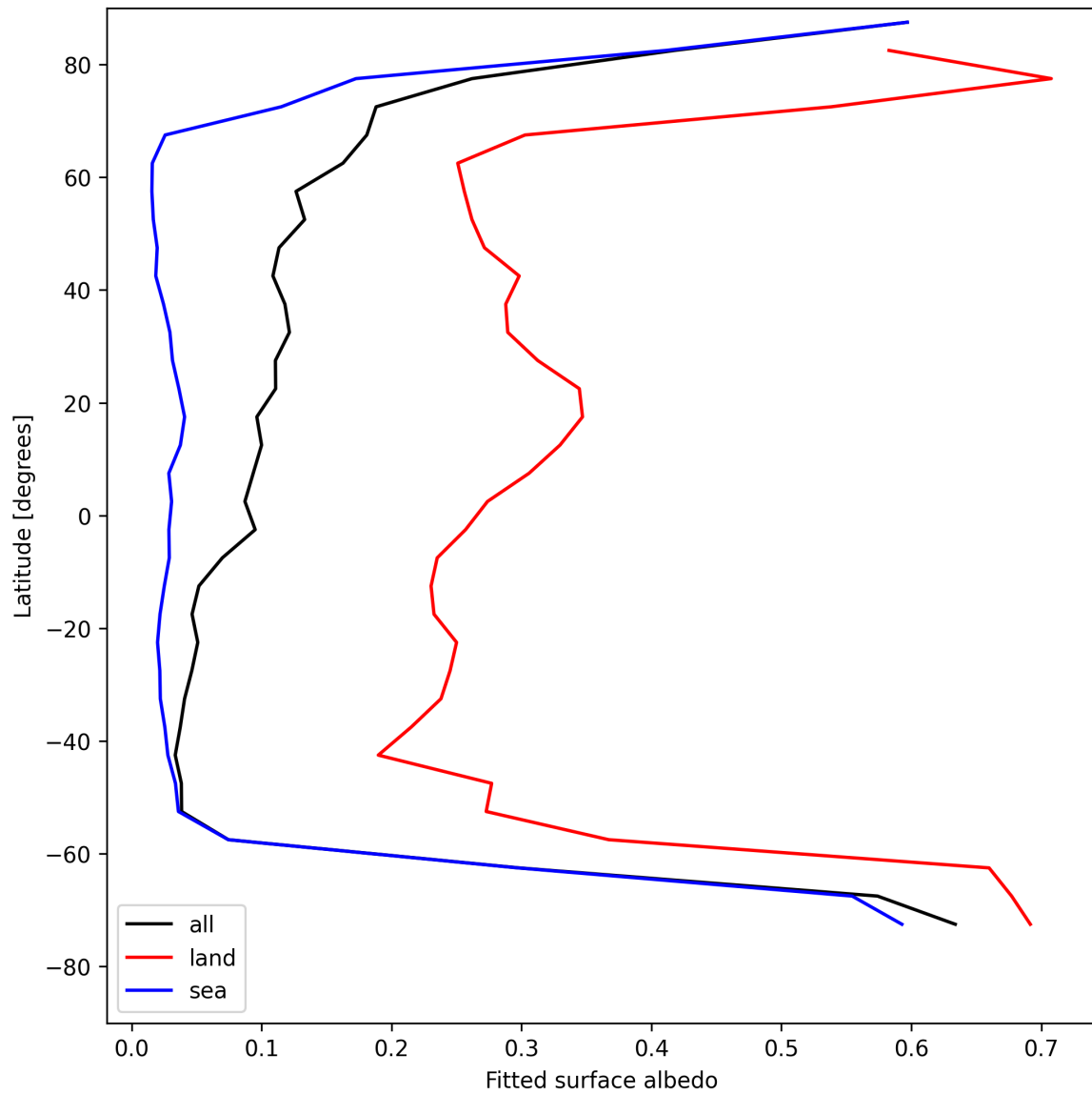
Figure 29: Zonal average of “Fitted surface albedo” for 2025-08-04 to 2025-08-06.
