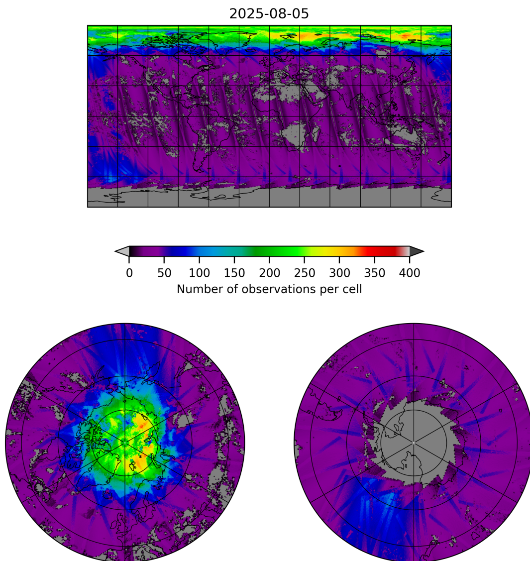
Figure 21: Map of the number of observations for 2025-08-04 to 2025-08-06
