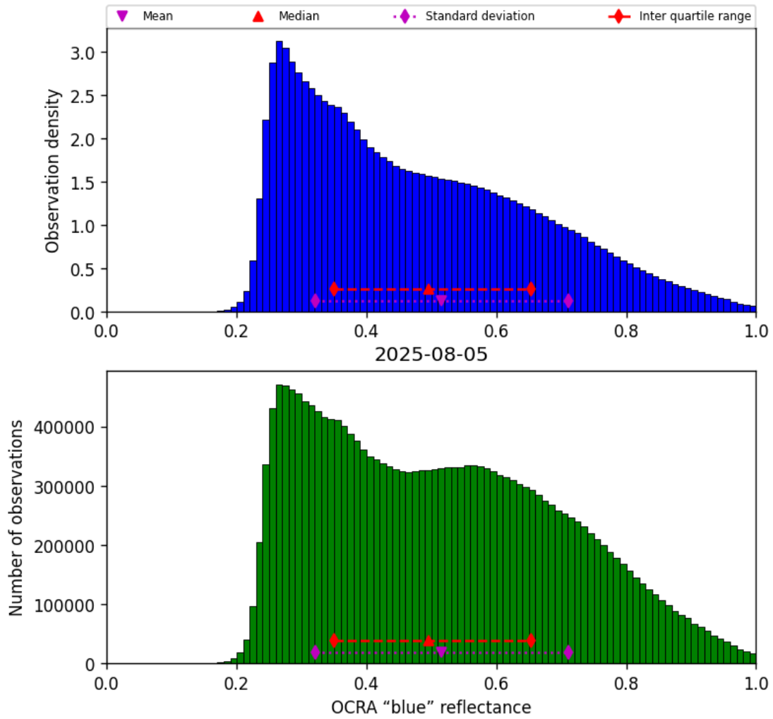
Figure 51: Histogram of “OCRA “blue” reflectance” for 2025-08-04 to 2025-08-06
