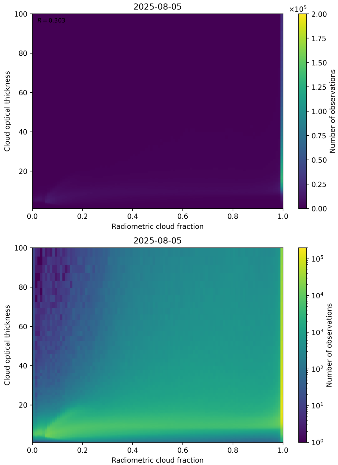
Figure 75: Scatter density plot of “Radiometric cloud fraction” against “Cloud optical thickness” for 2025-08-04 to 2025-08-06.
