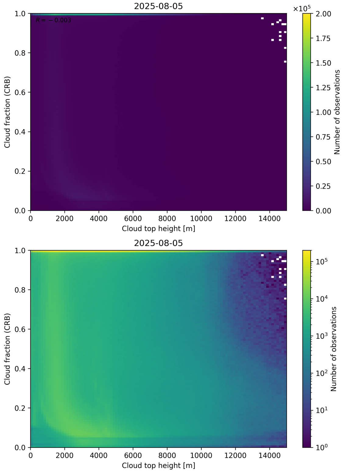
Figure 88: Scatter density plot of “Cloud top height” against “Cloud fraction (CRB)” for 2025-08-04 to 2025-08-06.
