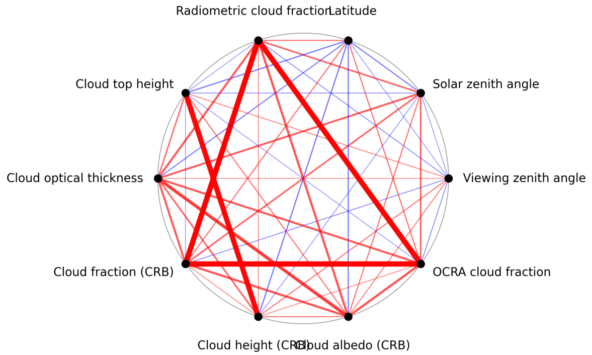
Figure 1: Map of correlation graph for 2025-08-04 to 2025-08-06.
