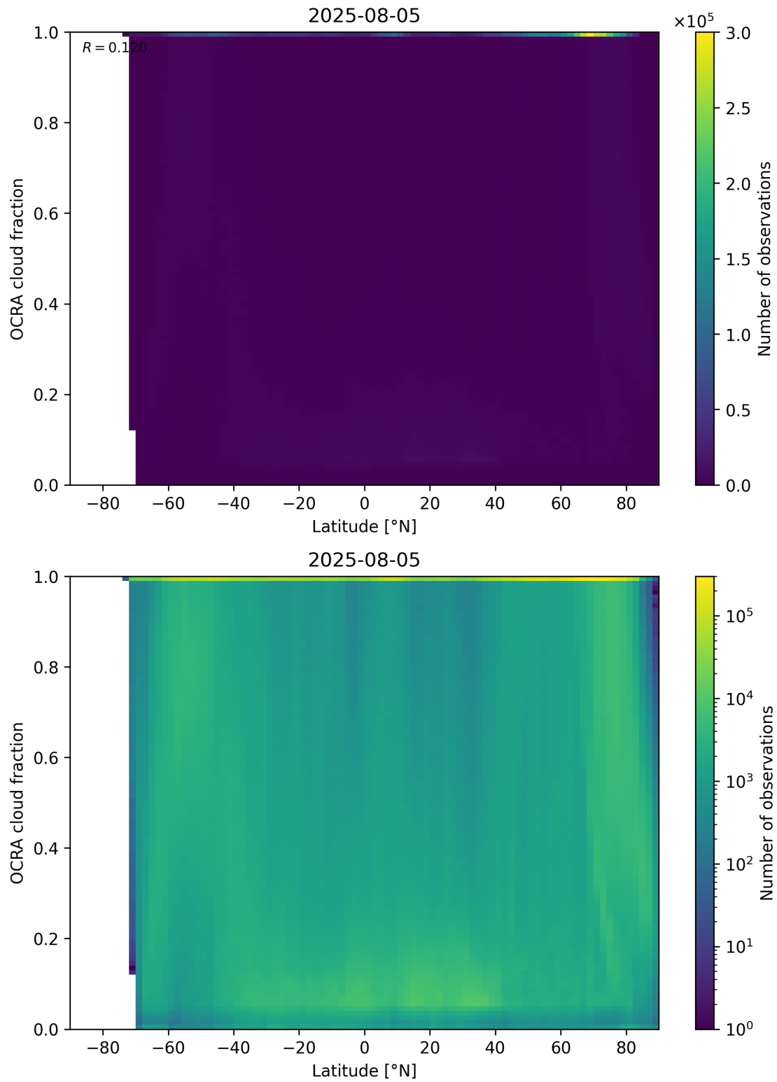
Figure 93: Scatter density plot of “Latitude” against “OCRA cloud fraction” for 2025-08-04 to 2025-08-06.
