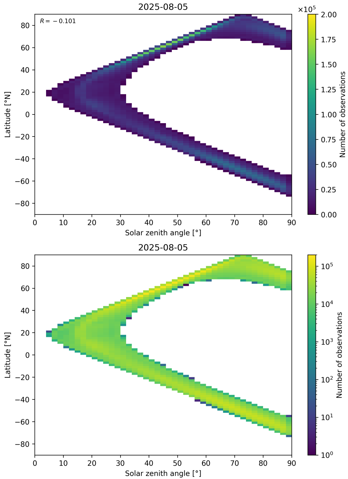
Figure 105: Scatter density plot of “Solar zenith angle” against “Latitude” for 2025-08-04 to 2025-08-06.
