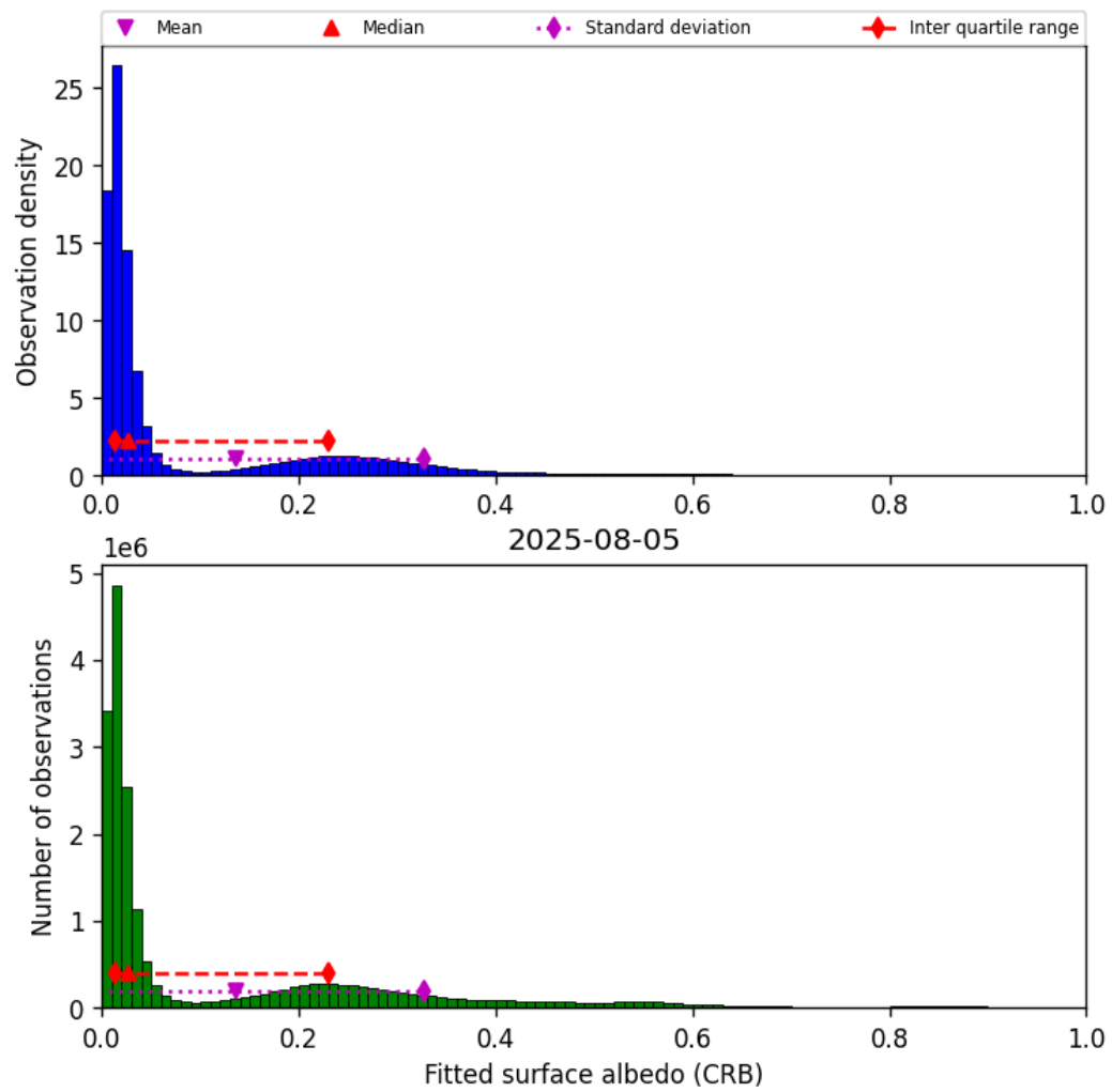
Figure 46: Histogram of “Fitted surface albedo (CRB)” for 2025-08-04 to 2025-08-06
