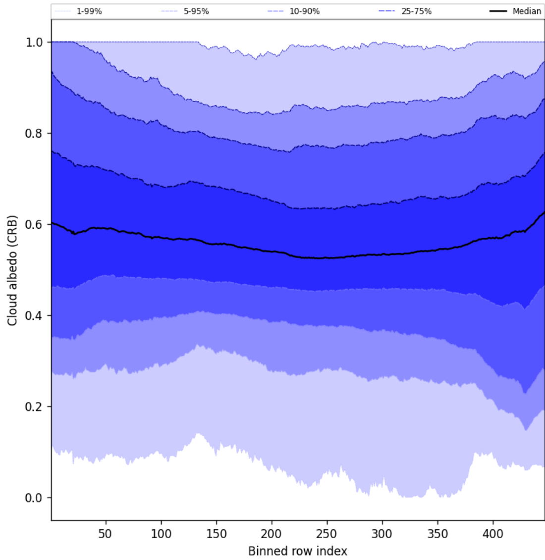
Figure 60: Along track statistics of “Cloud albedo (CRB)” for 2025-08-04 to 2025-08-06
