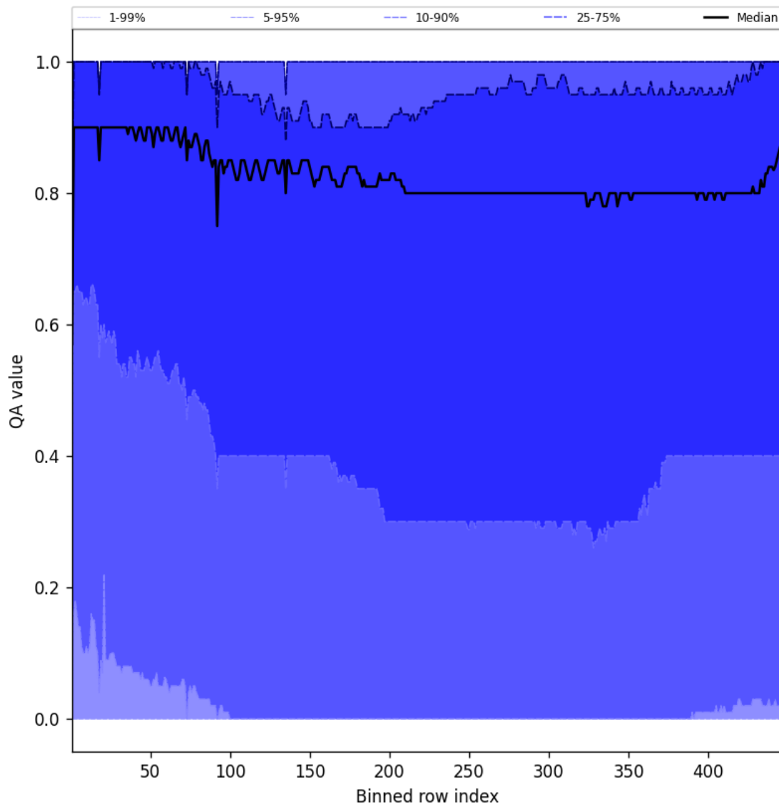
Figure 54: Along track statistics of “QA value” for 2025-08-04 to 2025-08-06
