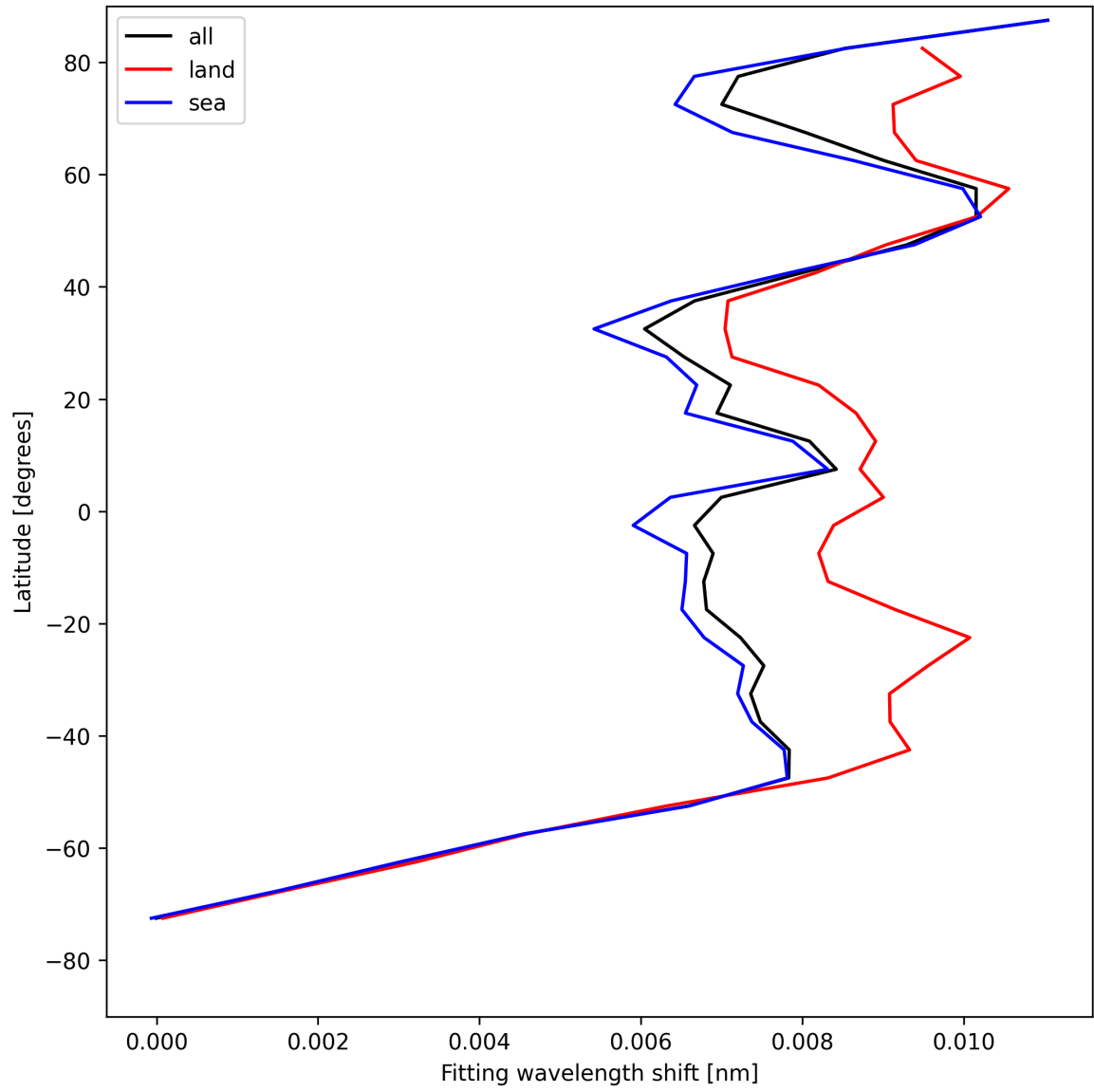
Figure 33: Zonal average of “Fitting wavelength shift” for 2025-08-04 to 2025-08-06.
