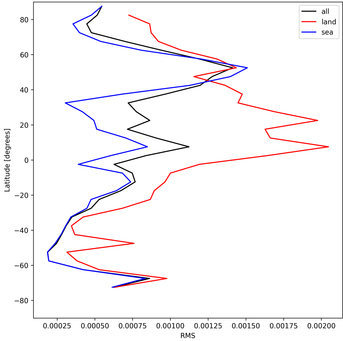
Figure 31: Zonal average of “RMS” for 2025-08-04 to 2025-08-06.
