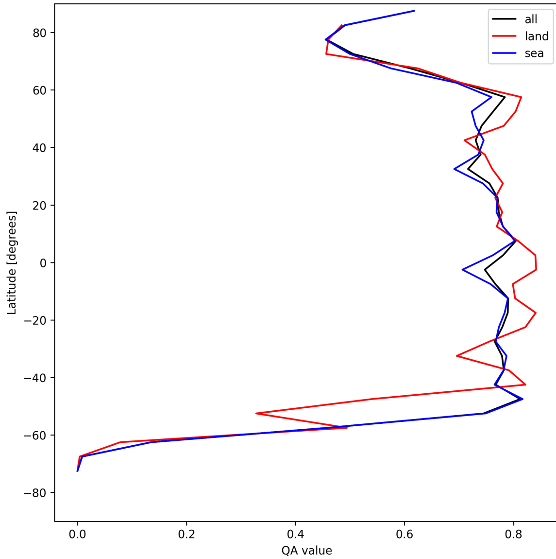
Figure 22: Zonal average of “QA value” for 2025-08-04 to 2025-08-06.
