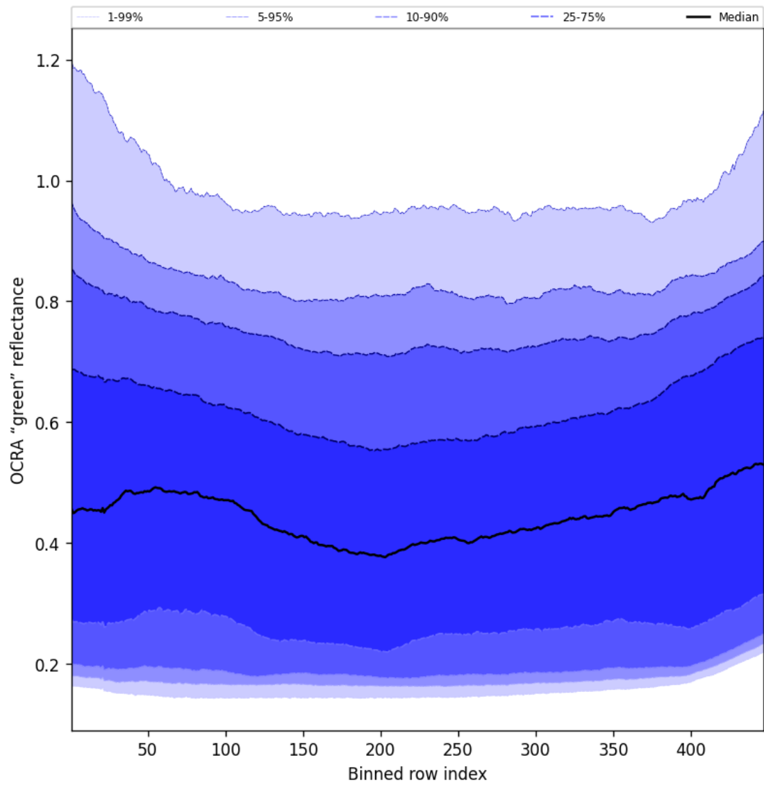
Figure 68: Along track statistics of “OCRA “green” reflectance” for 2025-08-04 to 2025-08-06
