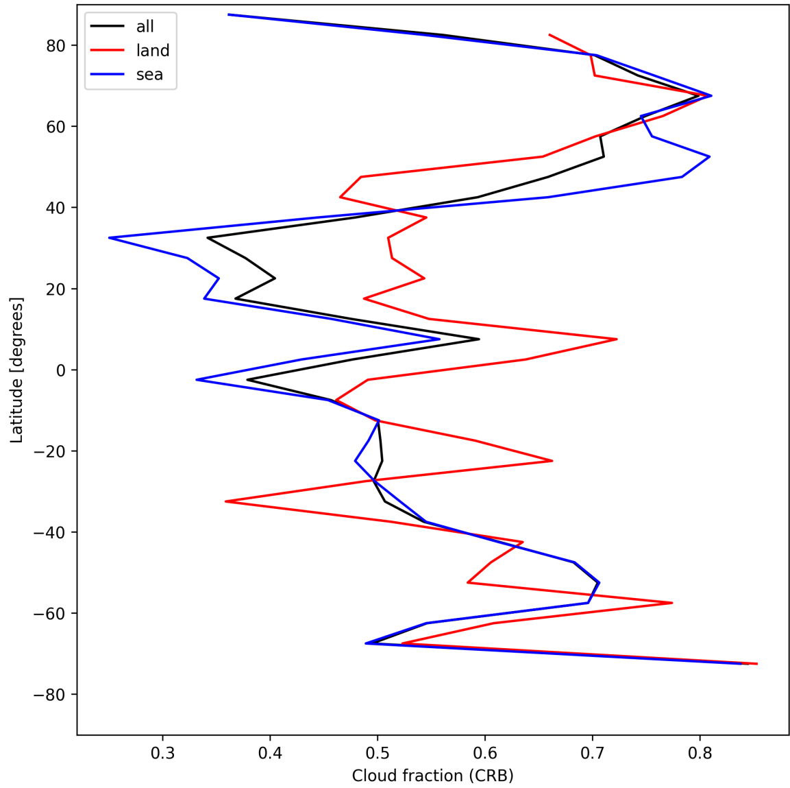
Figure 26: Zonal average of “Cloud fraction (CRB)” for 2025-08-04 to 2025-08-06.
