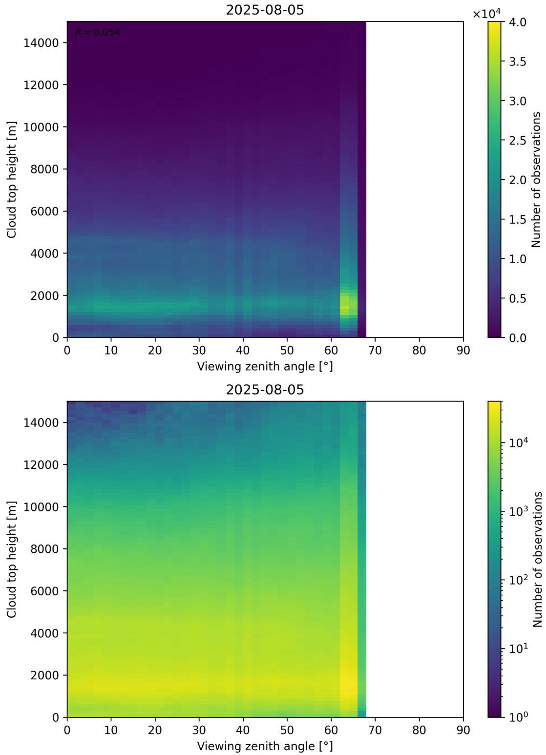
Figure 112: Scatter density plot of “Viewing zenith angle” against “Cloud top height” for 2025-08-04 to 2025-08-06.
