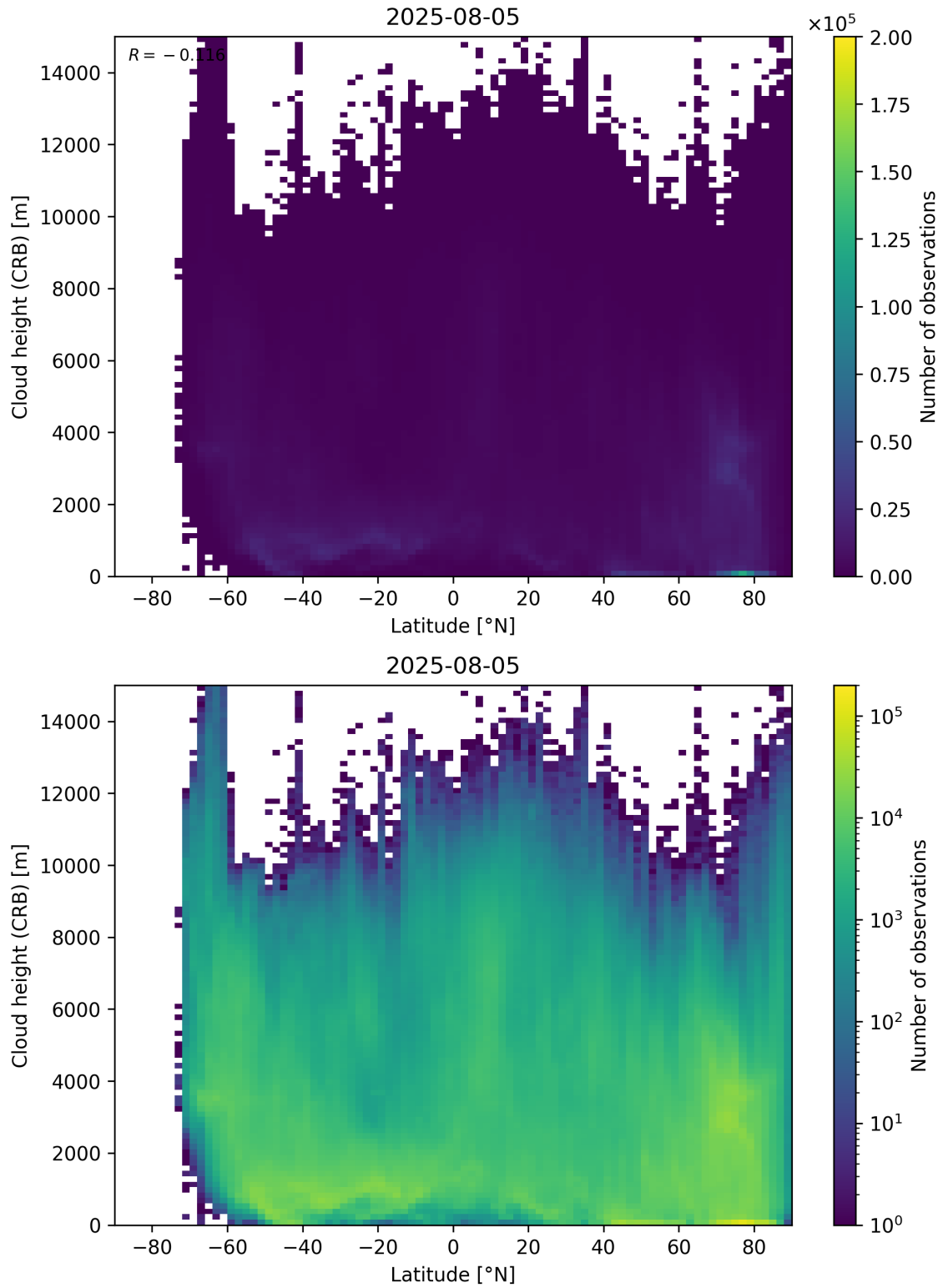
Figure 95: Scatter density plot of “Latitude” against “Cloud height (CRB)” for 2025-08-04 to 2025-08-06.
