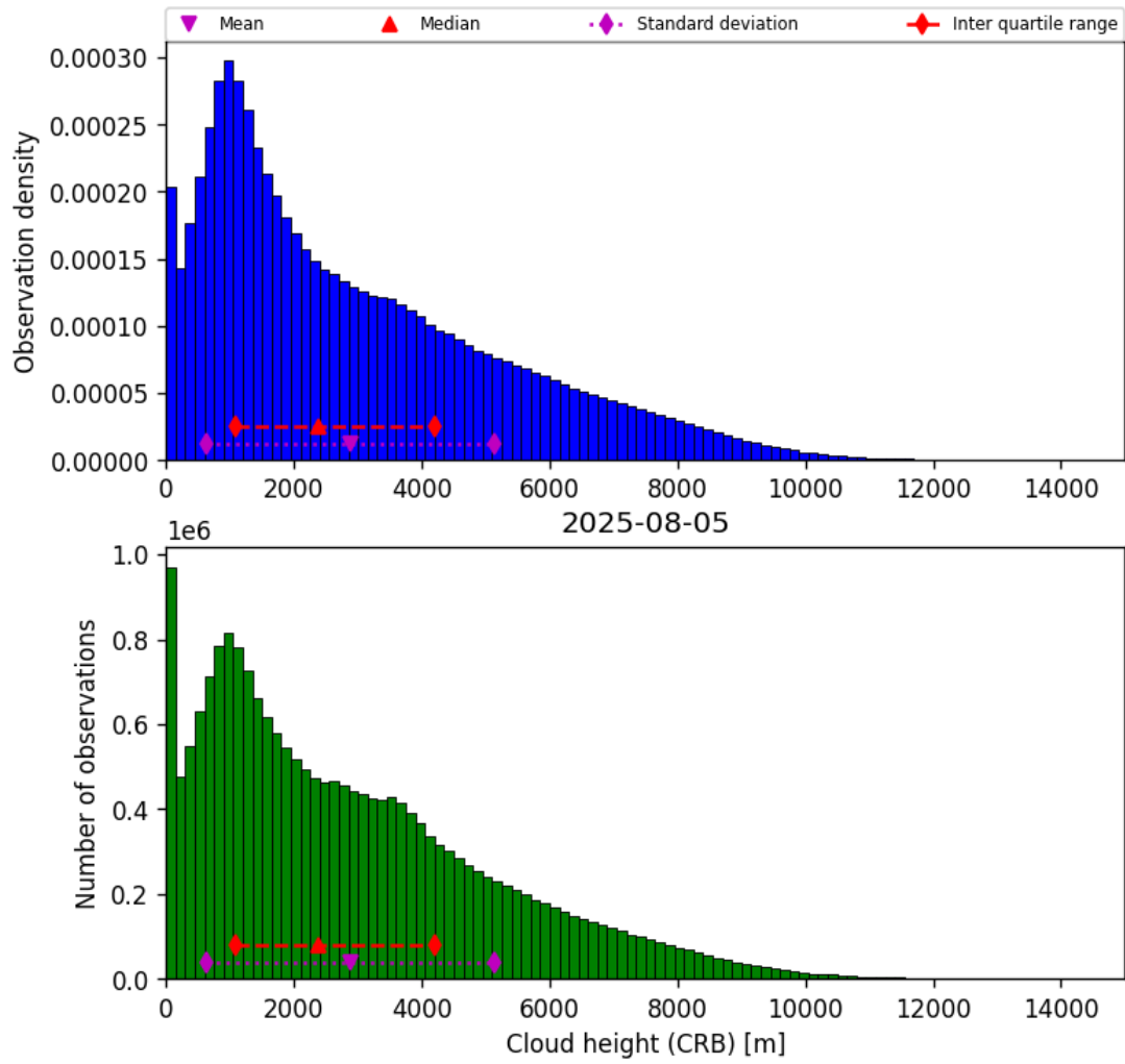
Figure 43: Histogram of “Cloud height (CRB)” for 2025-08-04 to 2025-08-06
