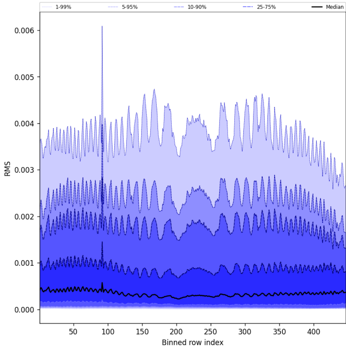
Figure 63: Along track statistics of “RMS” for 2025-08-04 to 2025-08-06
