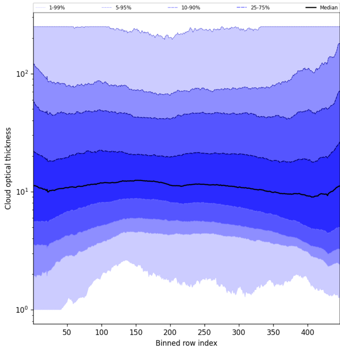
Figure 57: Along track statistics of “Cloud optical thickness” for 2025-08-04 to 2025-08-06
