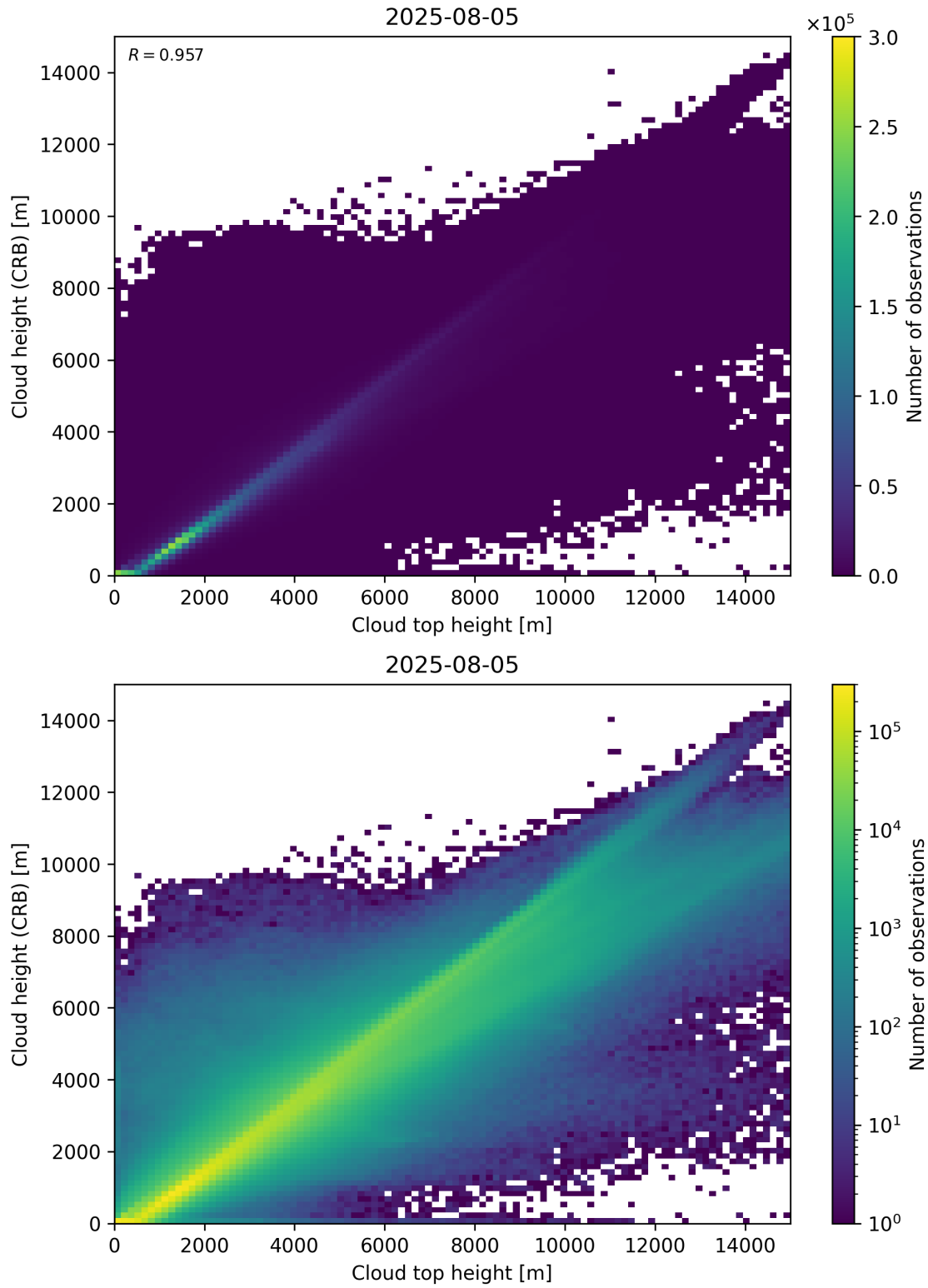
Figure 89: Scatter density plot of “Cloud top height” against “Cloud height (CRB)” for 2025-08-04 to 2025-08-06.
