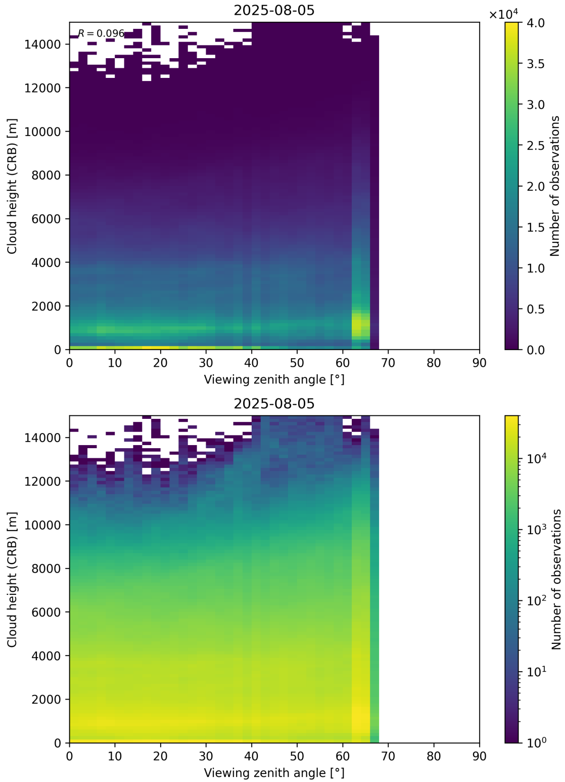
Figure 110: Scatter density plot of “Viewing zenith angle” against “Cloud height (CRB)” for 2025-08-04 to 2025-08-06.
