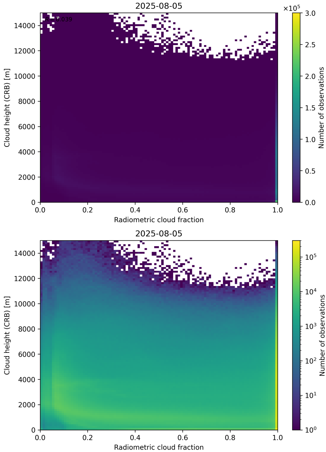
Figure 74: Scatter density plot of “Radiometric cloud fraction” against “Cloud height (CRB)” for 2025-08-04 to 2025-08-06.
