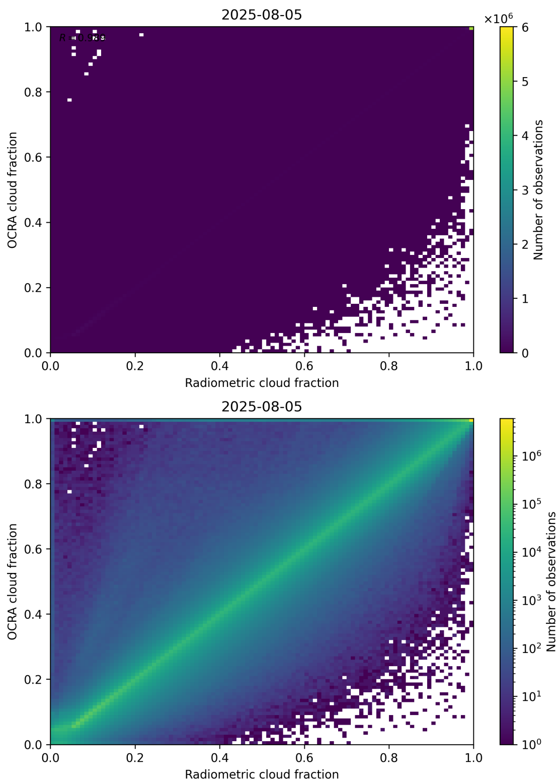
Figure 72: Scatter density plot of “Radiometric cloud fraction” against “OCRA cloud fraction” for 2025-08-04 to 2025-08-06.
