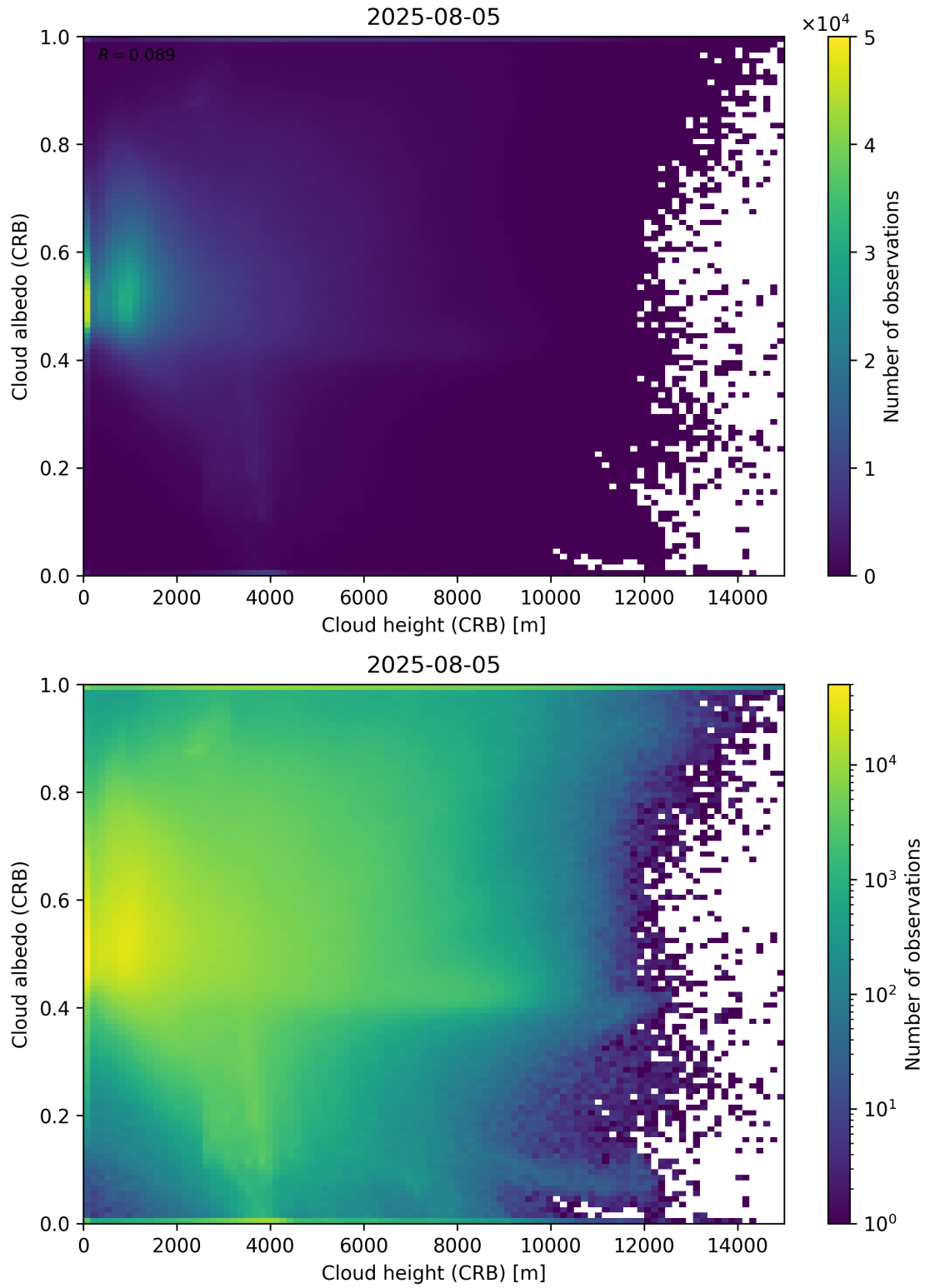
Figure 80: Scatter density plot of “Cloud height (CRB)” against “Cloud albedo (CRB)” for 2025-08-04 to 2025-08-06.
