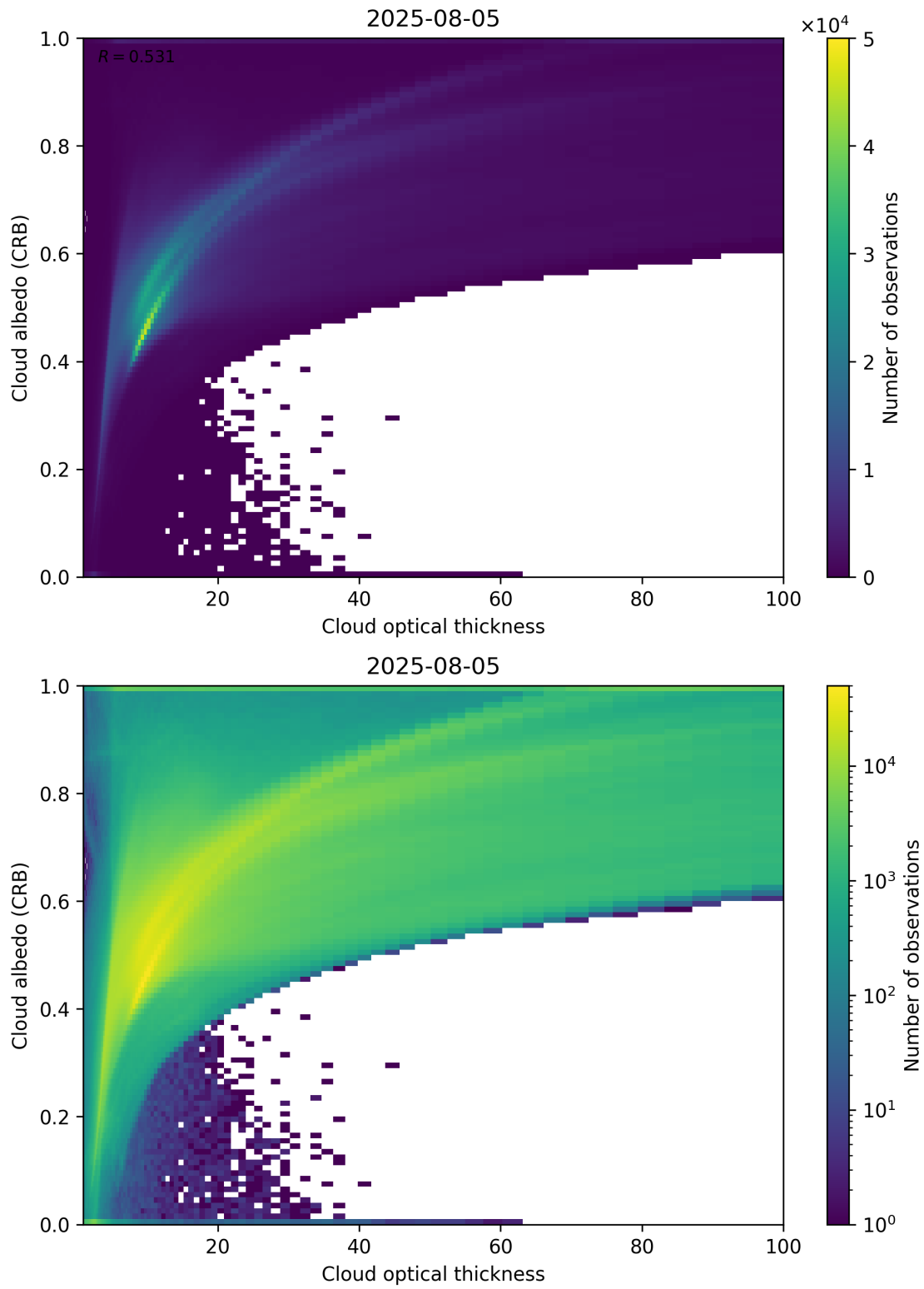
Figure 82: Scatter density plot of “Cloud optical thickness” against “Cloud albedo (CRB)” for 2025-08-04 to 2025-08-06.
