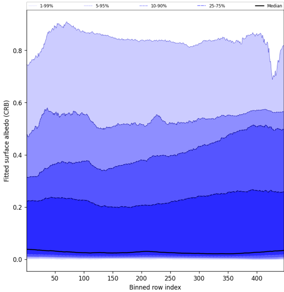
Figure 62: Along track statistics of “Fitted surface albedo (CRB)” for 2025-08-04 to 2025-08-06
