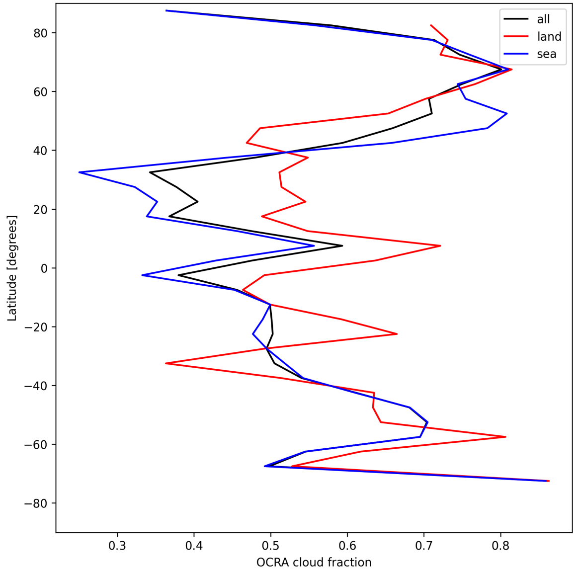
Figure 34: Zonal average of “OCRA cloud fraction” for 2025-08-04 to 2025-08-06.
