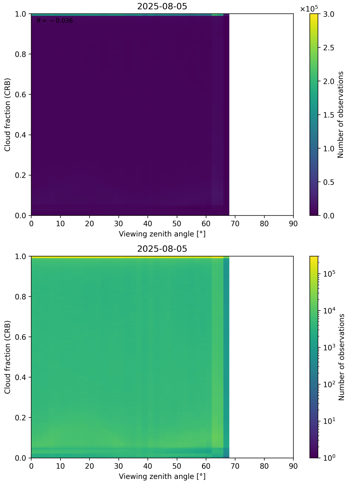
Figure 109: Scatter density plot of “Viewing zenith angle” against “Cloud fraction (CRB)” for 2025-08-04 to 2025-08-06.
