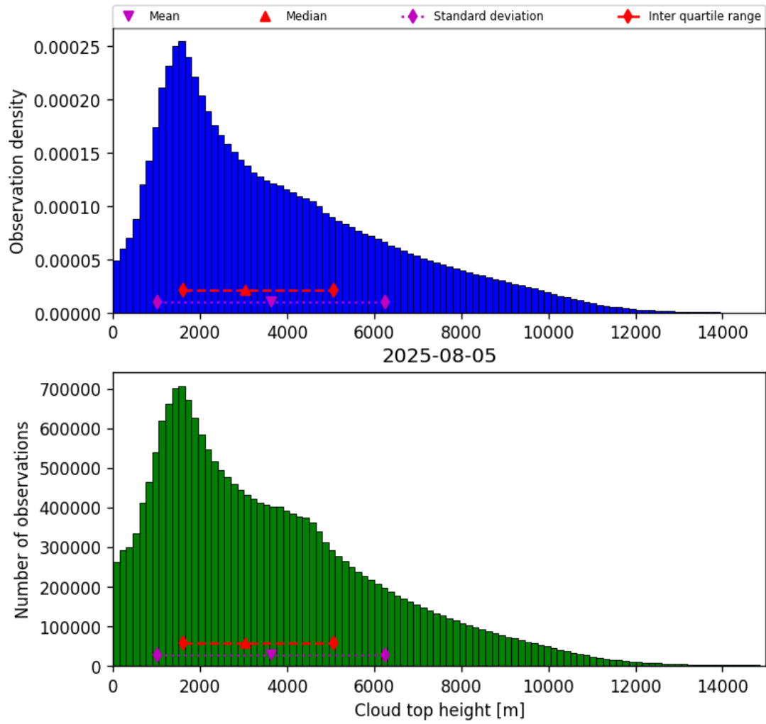
Figure 40: Histogram of “Cloud top height” for 2025-08-04 to 2025-08-06
