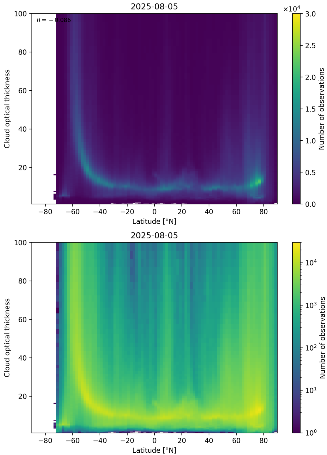
Figure 96: Scatter density plot of “Latitude” against “Cloud optical thickness” for 2025-08-04 to 2025-08-06.
