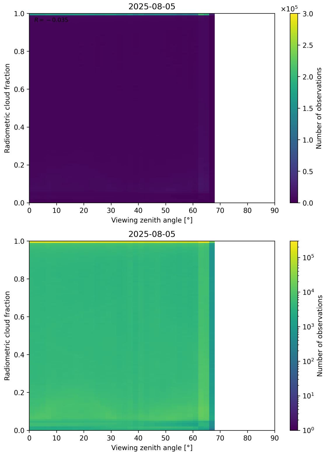
Figure 107: Scatter density plot of “Viewing zenith angle” against “Radiometric cloud fraction” for 2025-08-04 to 2025-08-06.
