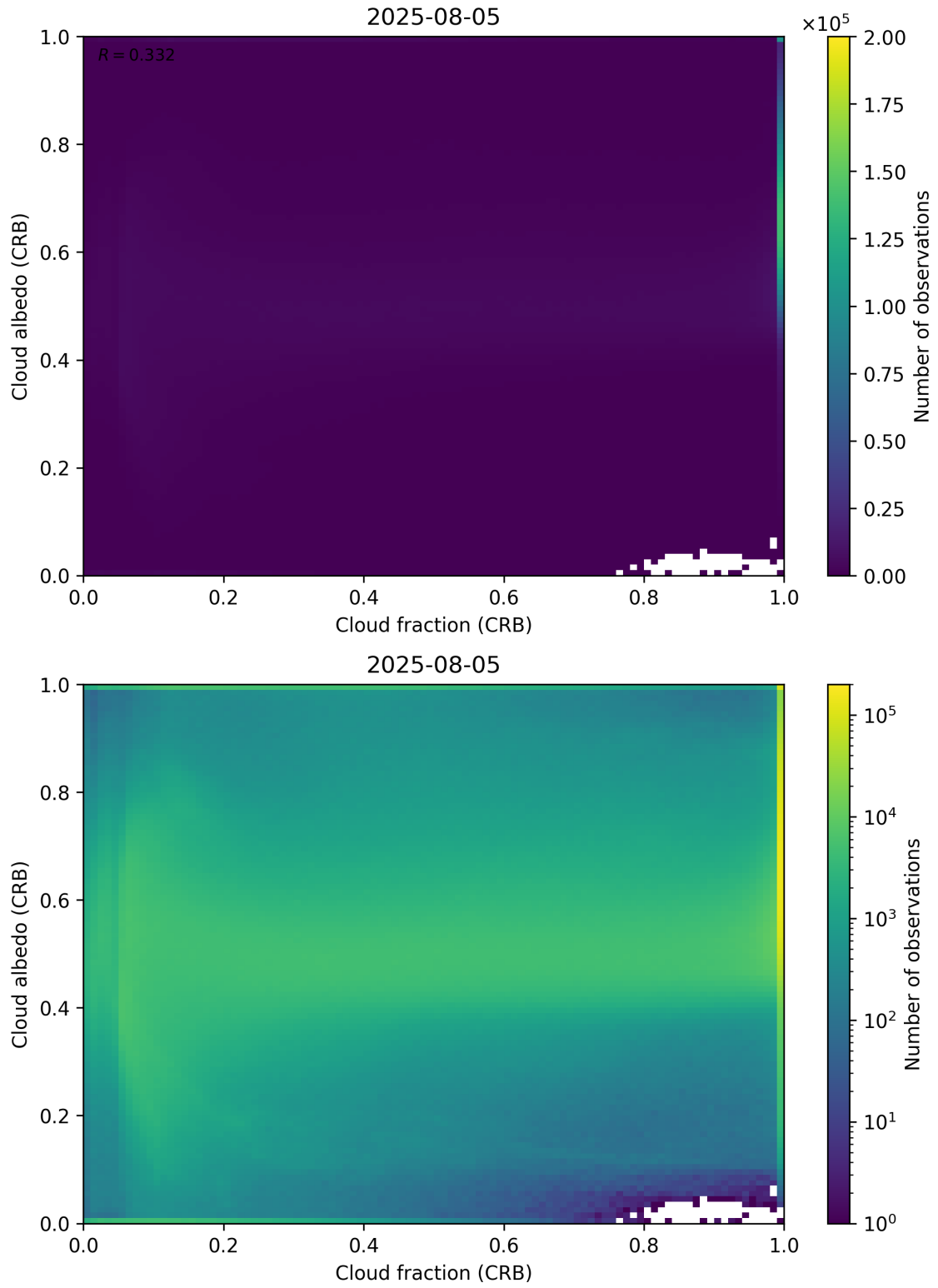
Figure 77: Scatter density plot of “Cloud fraction (CRB)” against “Cloud albedo (CRB)” for 2025-08-04 to 2025-08-06.
