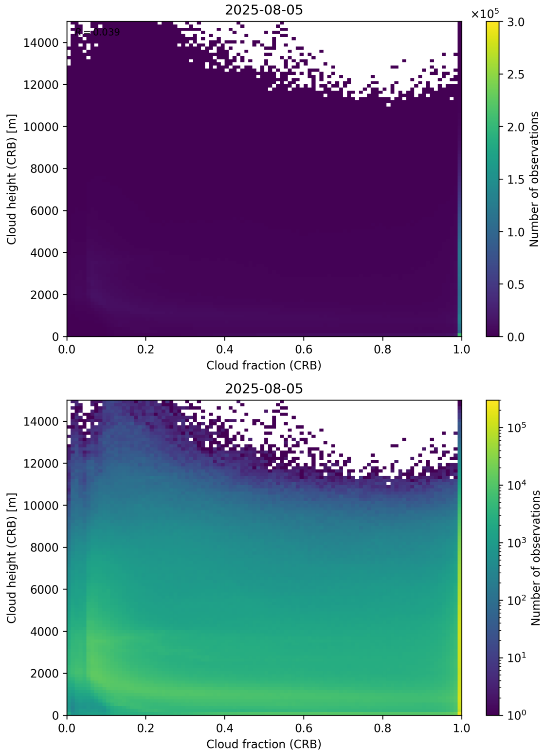
Figure 79: Scatter density plot of “Cloud fraction (CRB)” against “Cloud height (CRB)” for 2025-08-04 to 2025-08-06.
