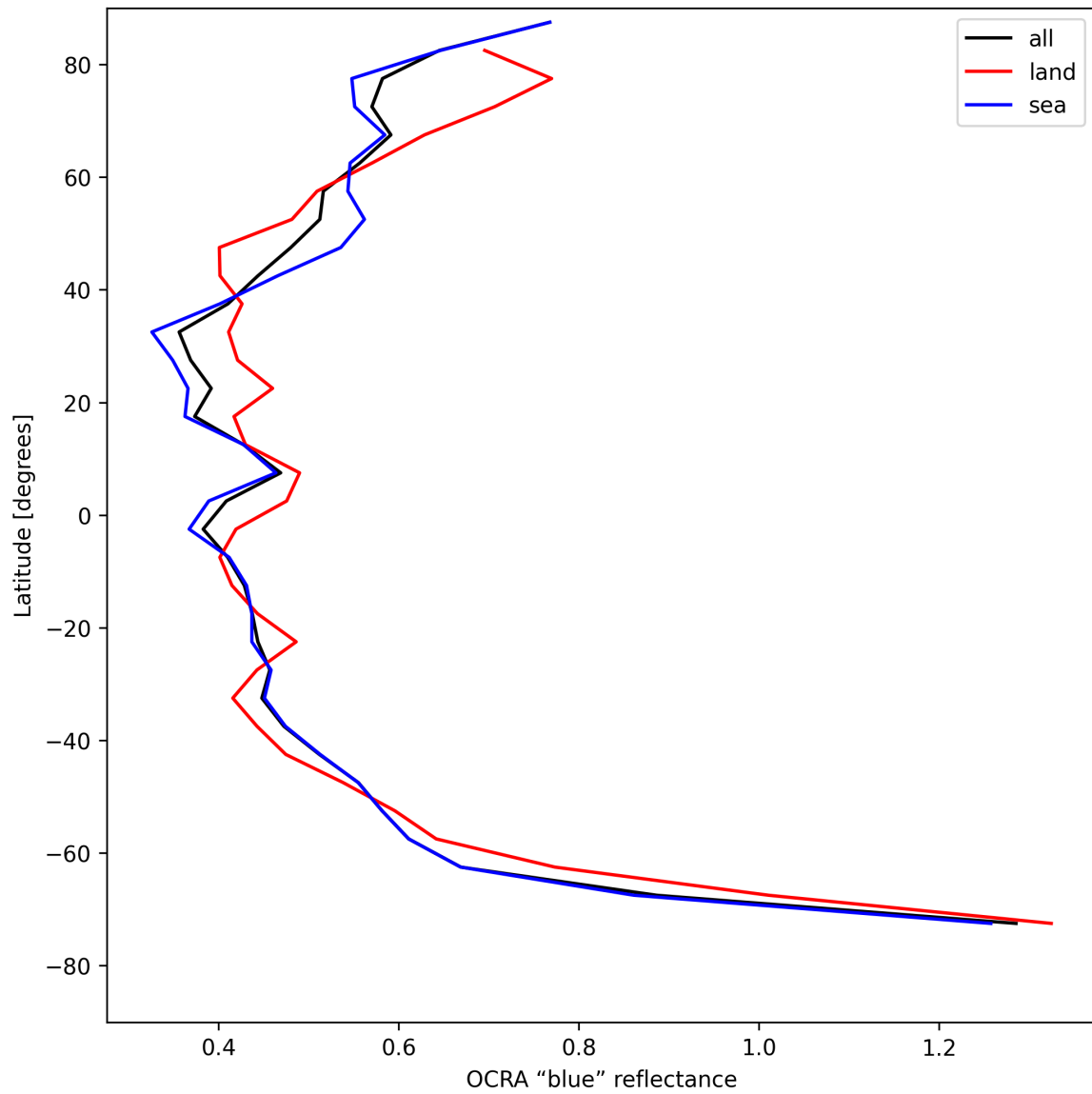
Figure 35: Zonal average of "OCRA "blue" reflectance" for 2025-08-04 to 2025-08-06.
