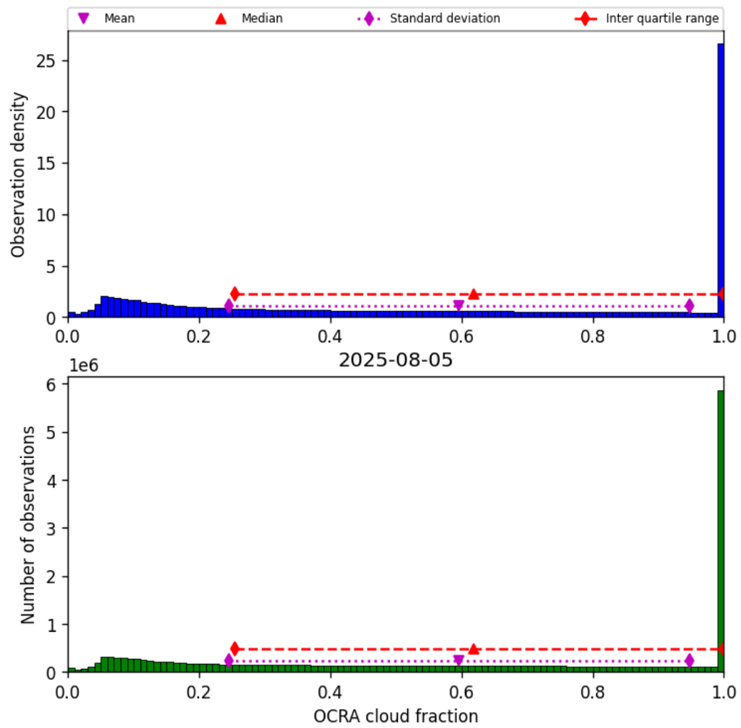
Figure 50: Histogram of “OCRA cloud fraction” for 2025-08-04 to 2025-08-06
