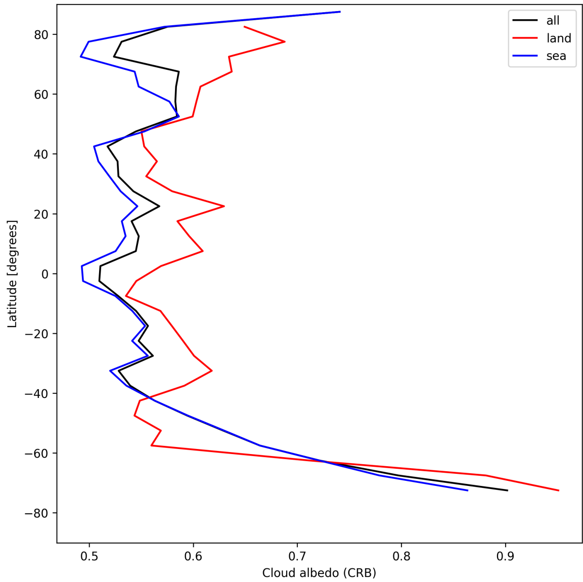
Figure 28: Zonal average of “Cloud albedo (CRB)” for 2025-08-04 to 2025-08-06.
