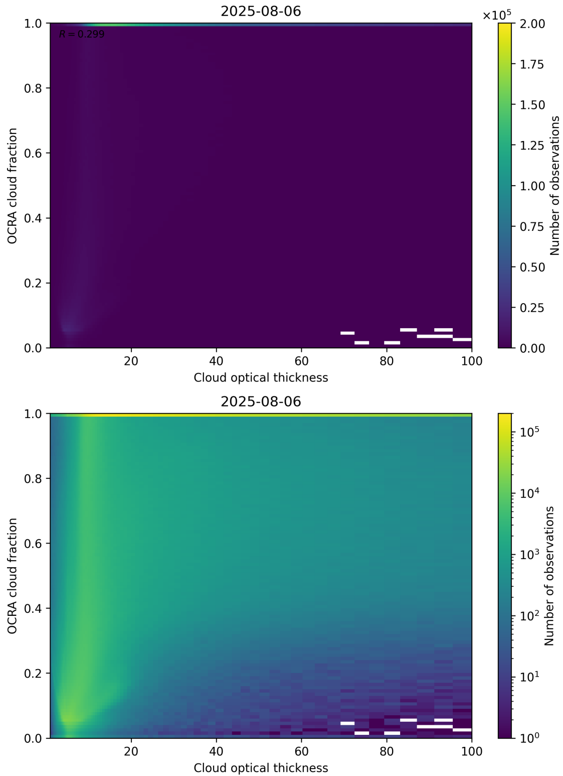
Figure 83: Scatter density plot of “Cloud optical thickness” against “OCRA cloud fraction” for 2025-08-05 to 2025-08-07.
