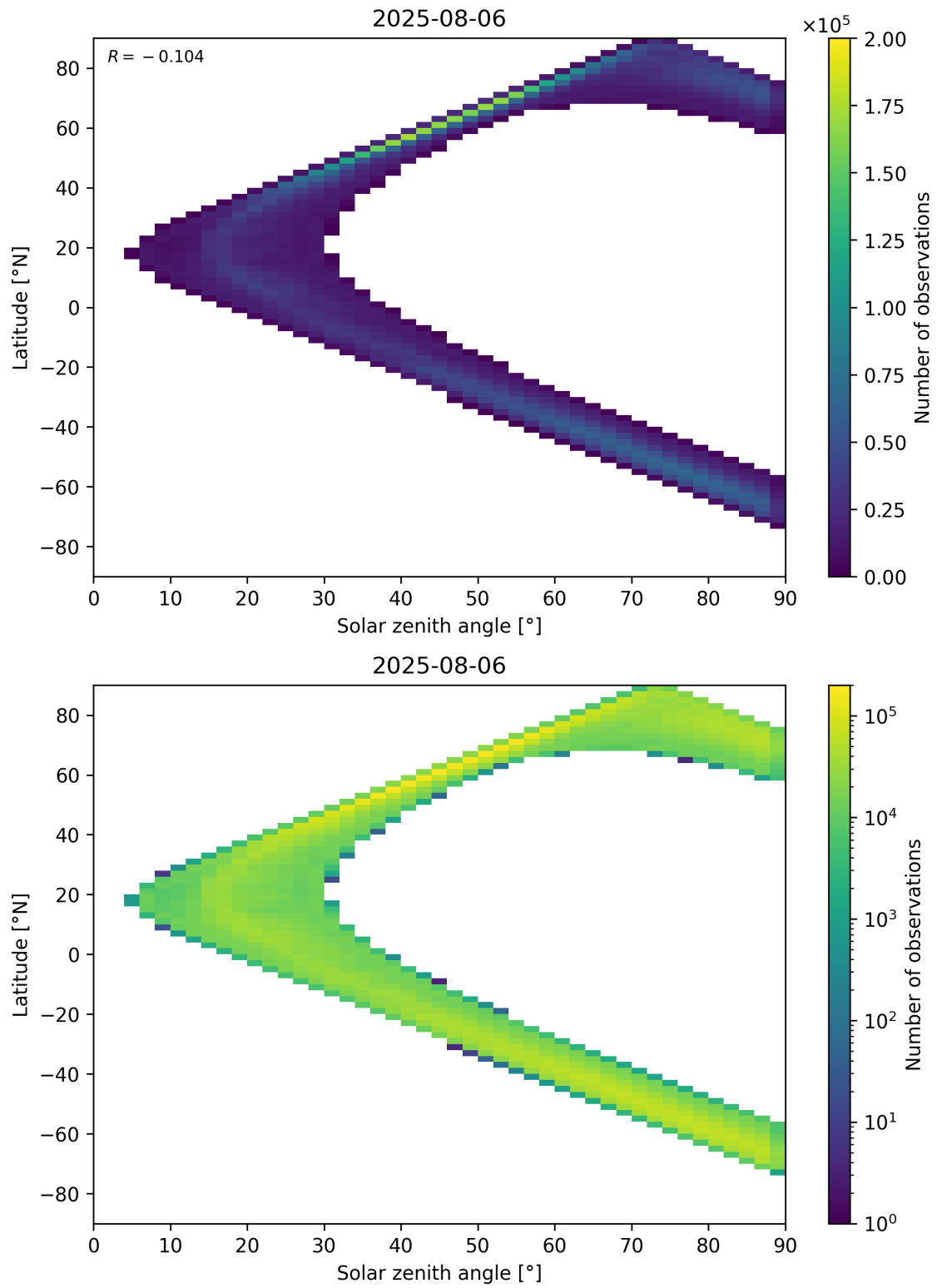
Figure 105: Scatter density plot of “Solar zenith angle” against “Latitude” for 2025-08-05 to 2025-08-07.
