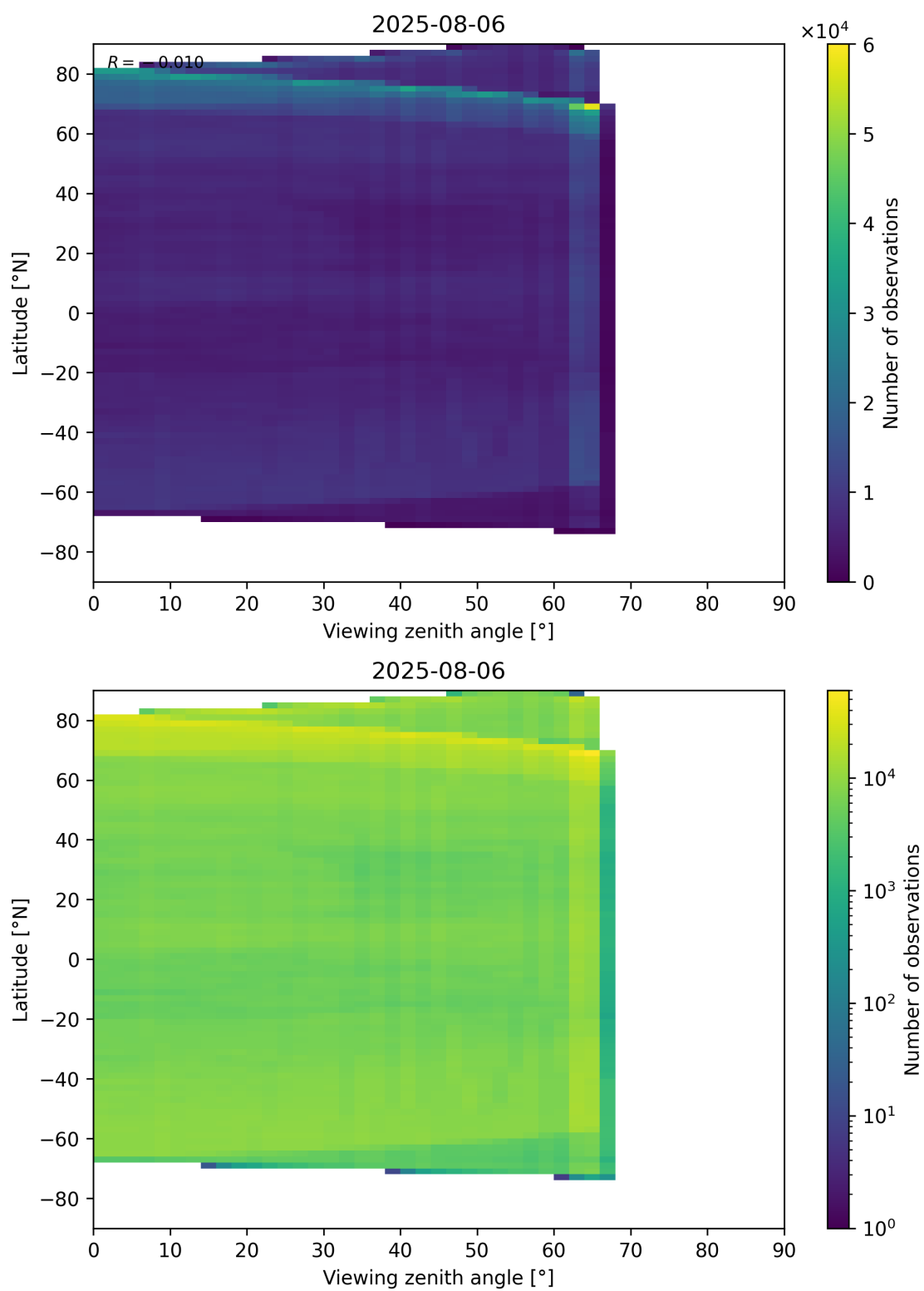
Figure 113: Scatter density plot of “Viewing zenith angle” against “Latitude” for 2025-08-05 to 2025-08-07.
