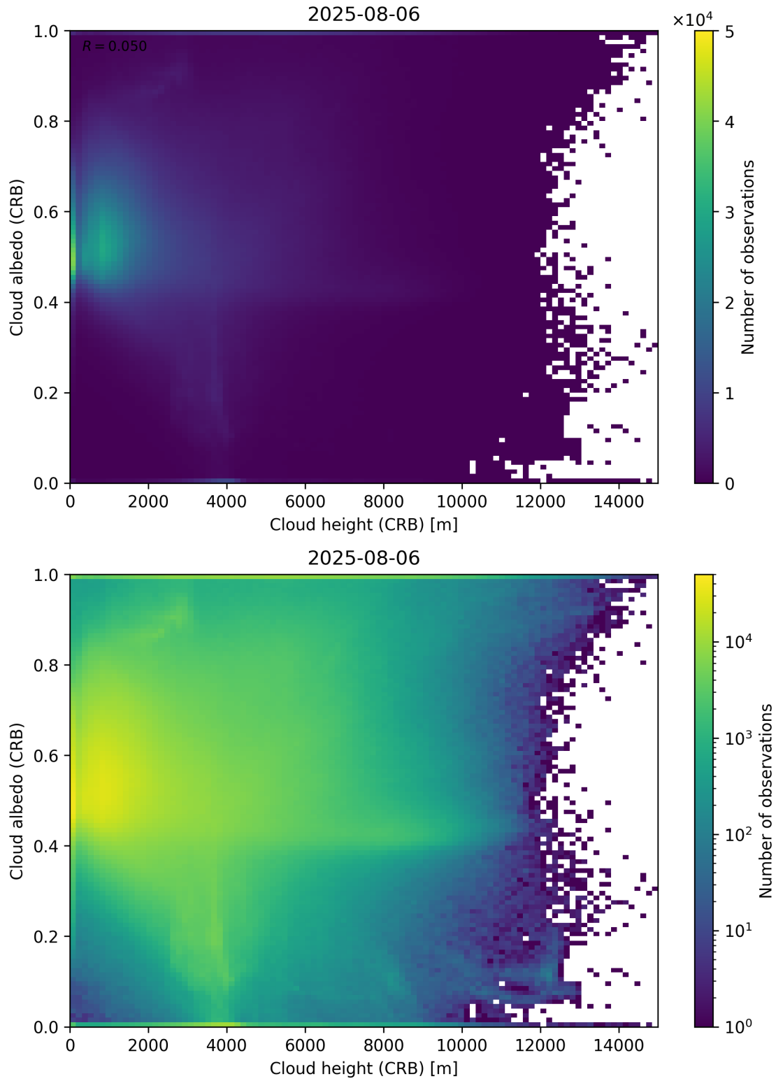
Figure 80: Scatter density plot of “Cloud height (CRB)” against “Cloud albedo (CRB)” for 2025-08-05 to 2025-08-07.
