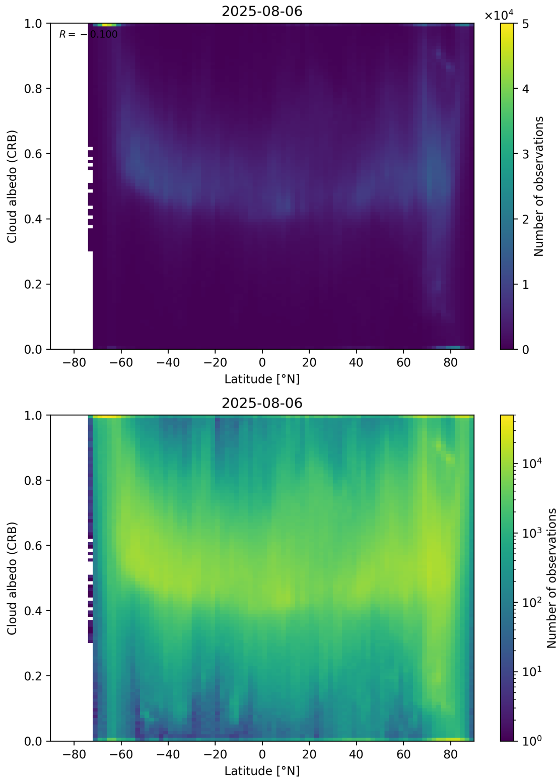
Figure 91: Scatter density plot of “Latitude” against “Cloud albedo (CRB)” for 2025-08-05 to 2025-08-07.
