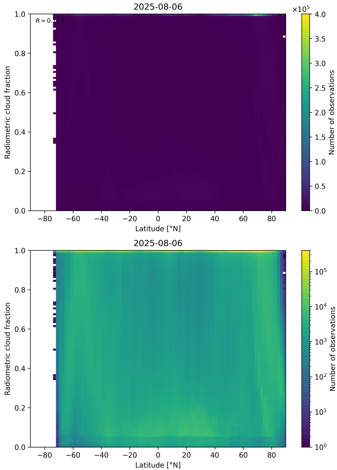
Figure 92: Scatter density plot of “Latitude” against “Radiometric cloud fraction” for 2025-08-05 to 2025-08-07.
