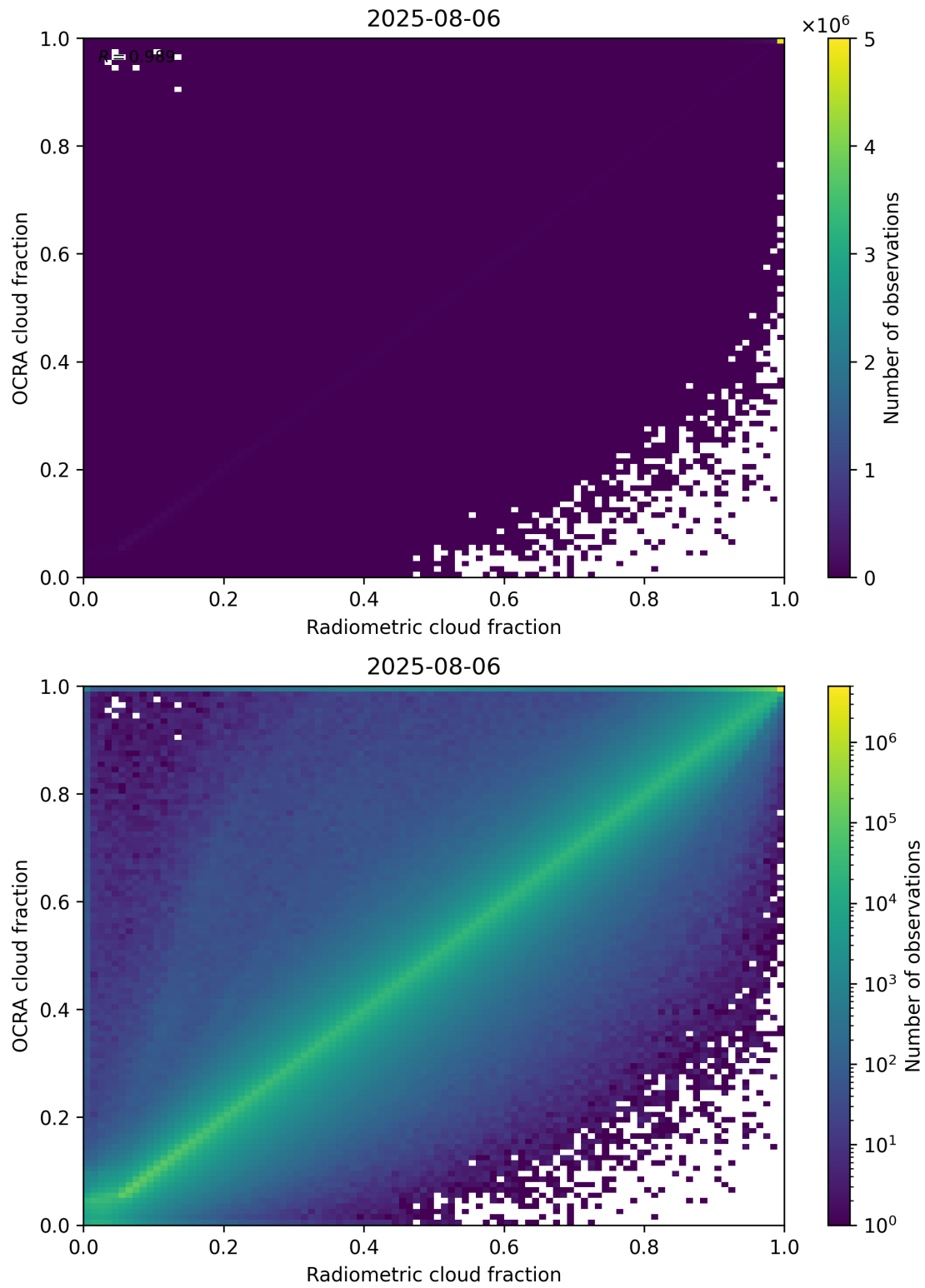
Figure 72: Scatter density plot of “Radiometric cloud fraction” against “OCRA cloud fraction” for 2025-08-05 to 2025-08-07.
