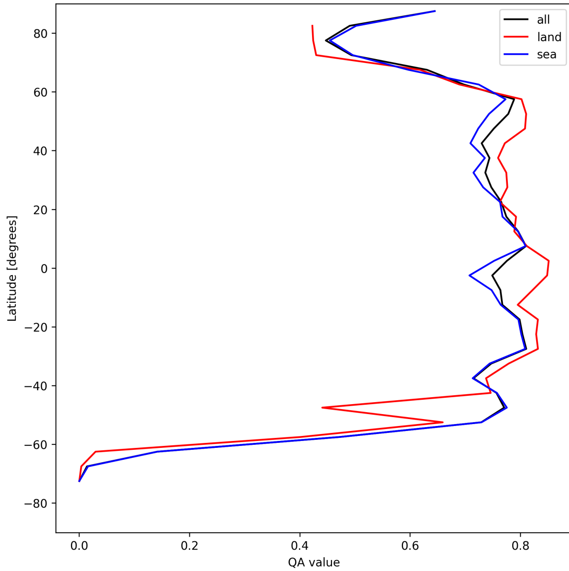
Figure 22: Zonal average of “QA value” for 2025-08-05 to 2025-08-07.
