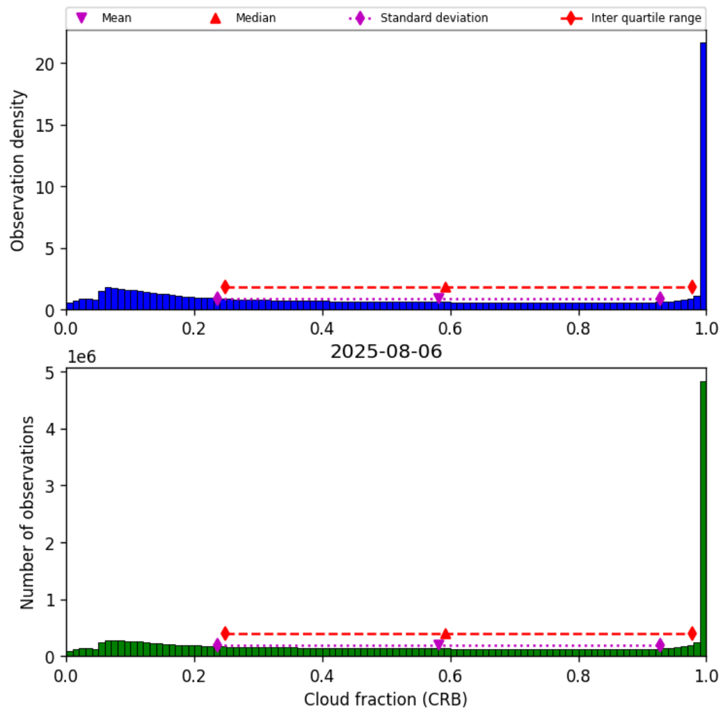
Figure 42: Histogram of “Cloud fraction (CRB)” for 2025-08-05 to 2025-08-07
