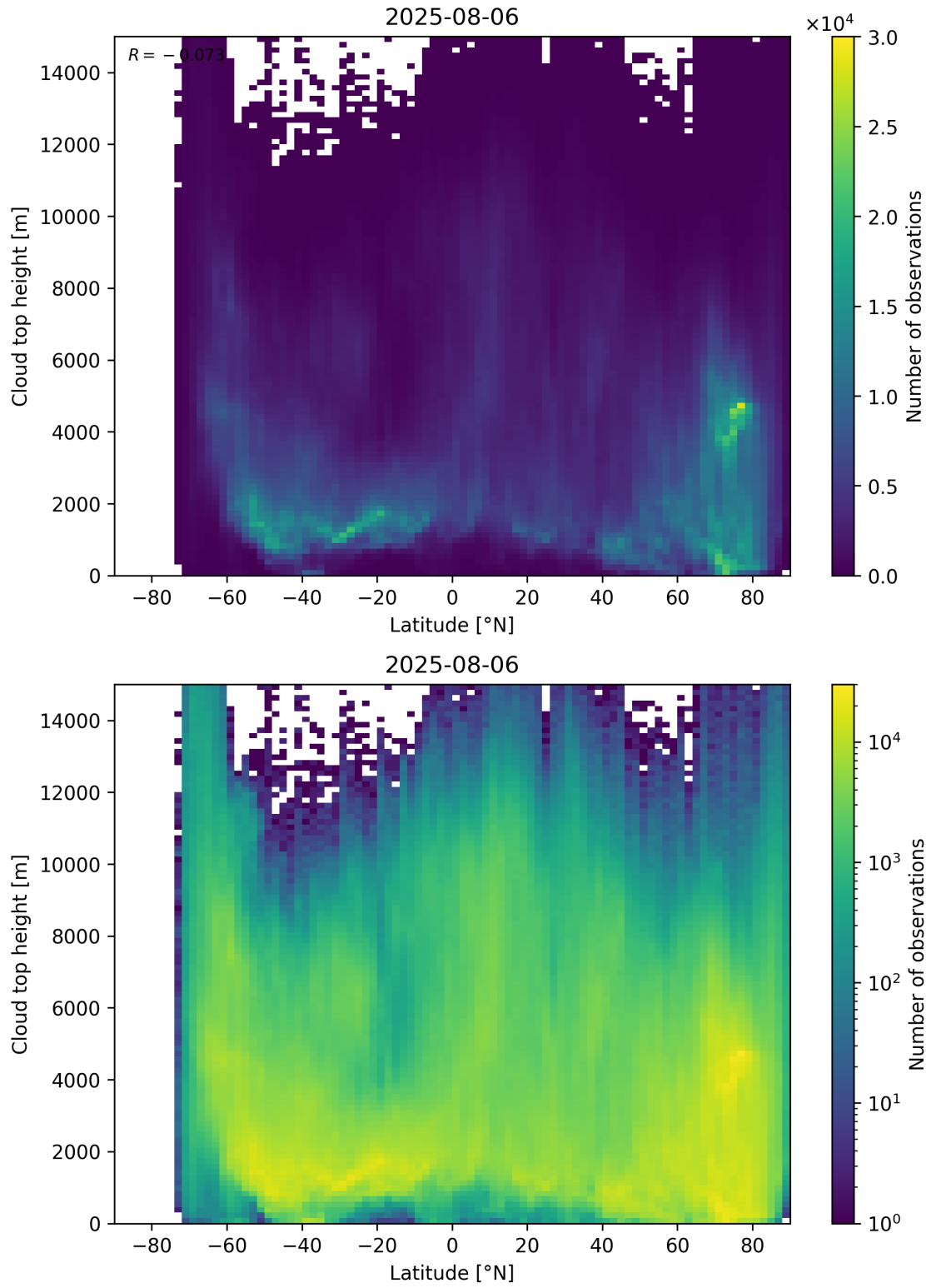
Figure 97: Scatter density plot of “Latitude” against “Cloud top height” for 2025-08-05 to 2025-08-07.
