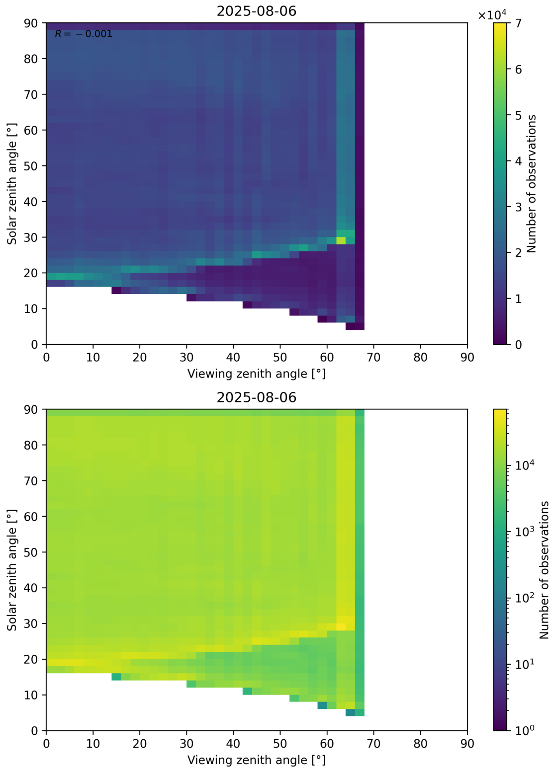
Figure 114: Scatter density plot of “Viewing zenith angle” against “Solar zenith angle” for 2025-08-05 to 2025-08-07.
