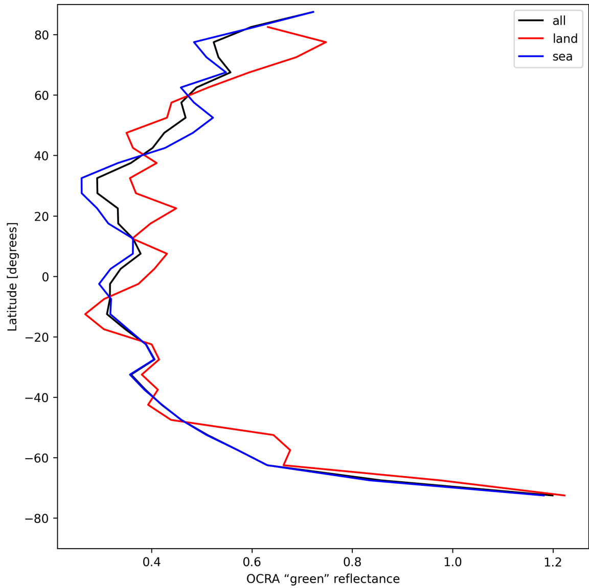
Figure 36: Zonal average of “OCRA “green” reflectance” for 2025-08-05 to 2025-08-07.
