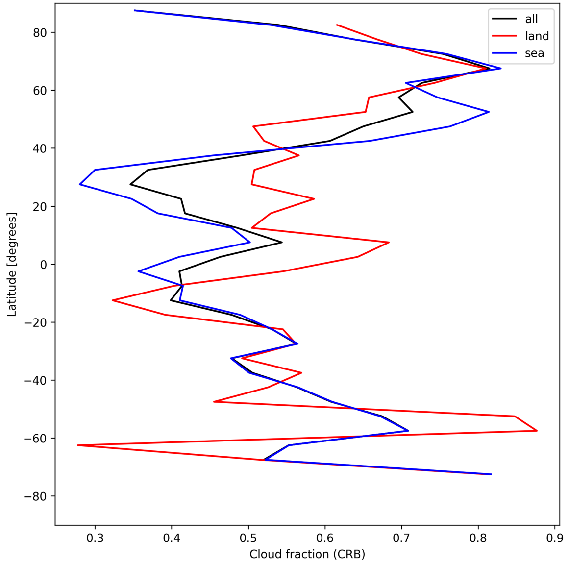
Figure 26: Zonal average of “Cloud fraction (CRB)” for 2025-08-05 to 2025-08-07.
