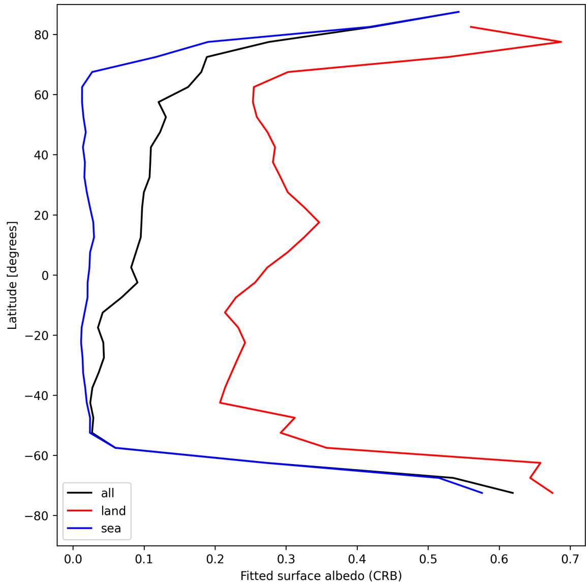
Figure 30: Zonal average of “Fitted surface albedo (CRB)” for 2025-08-05 to 2025-08-07.
