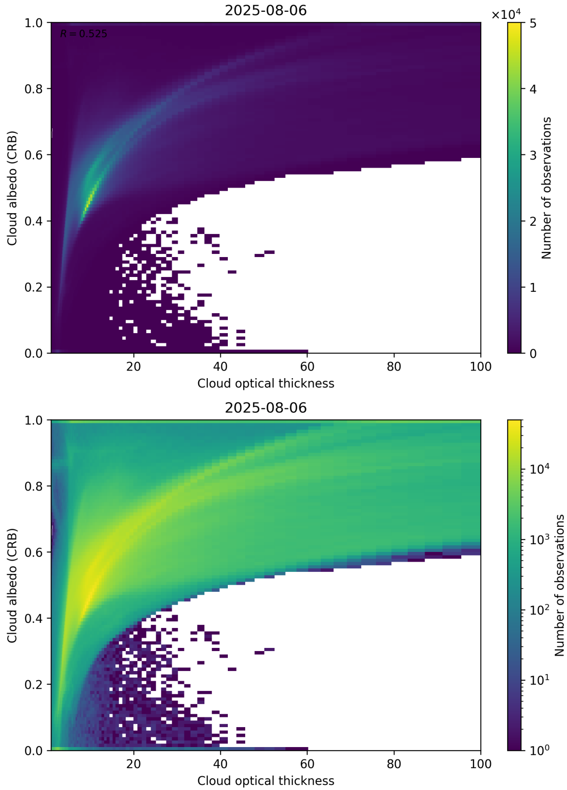
Figure 82: Scatter density plot of “Cloud optical thickness” against “Cloud albedo (CRB)” for 2025-08-05 to 2025-08-07.
