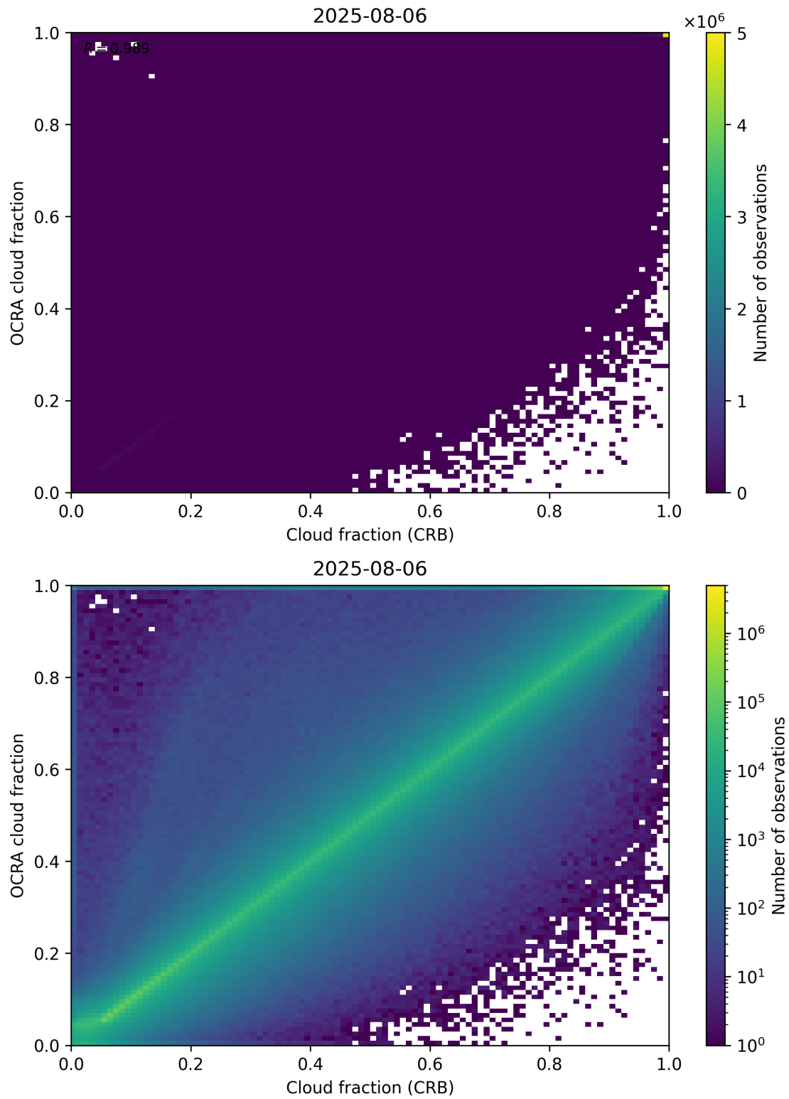
Figure 78: Scatter density plot of “Cloud fraction (CRB)” against “OCRA cloud fraction” for 2025-08-05 to 2025-08-07.
