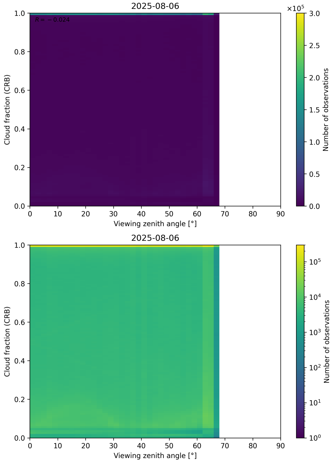
Figure 109: Scatter density plot of “Viewing zenith angle” against “Cloud fraction (CRB)” for 2025-08-05 to 2025-08-07.
