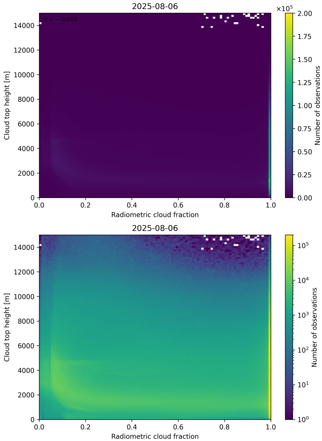
Figure 76: Scatter density plot of “Radiometric cloud fraction” against “Cloud top height” for 2025-08-05 to 2025-08-07.
