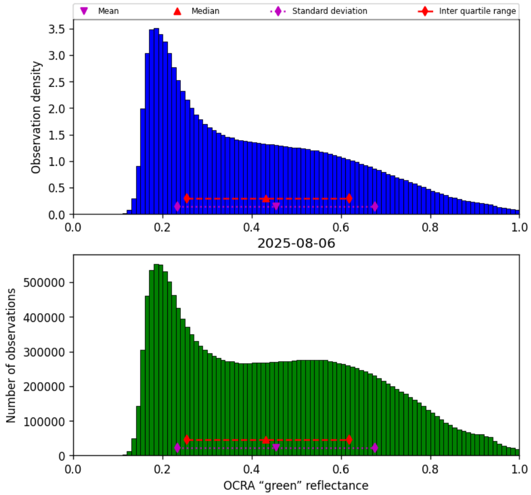
Figure 52: Histogram of “OCRA “green” reflectance” for 2025-08-05 to 2025-08-07
