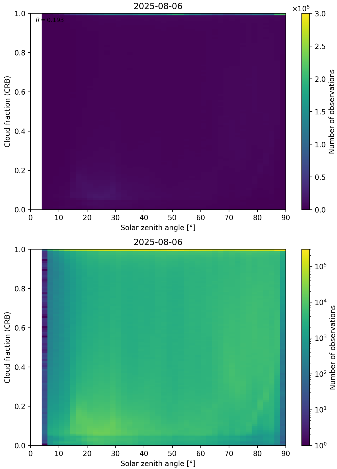
Figure 101: Scatter density plot of “Solar zenith angle” against “Cloud fraction (CRB)” for 2025-08-05 to 2025-08-07.
