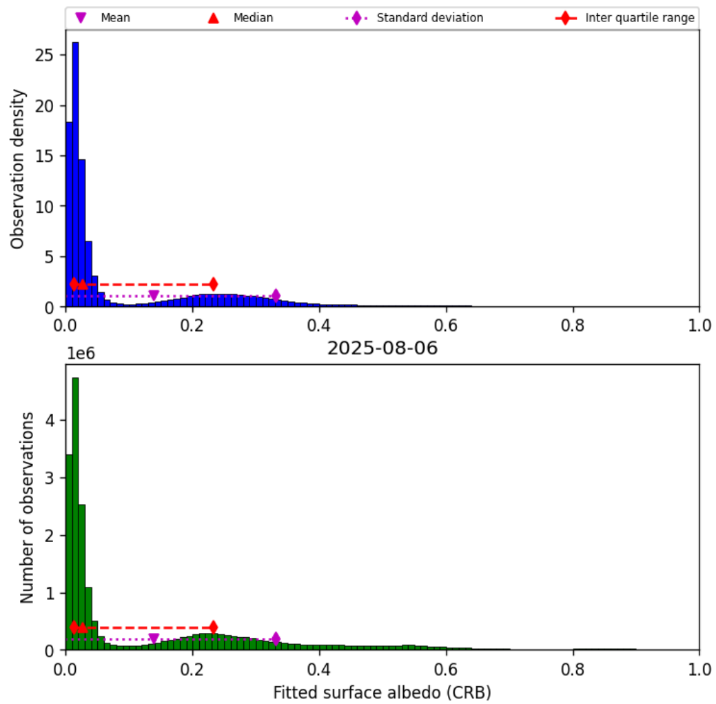
Figure 46: Histogram of “Fitted surface albedo (CRB)” for 2025-08-05 to 2025-08-07
