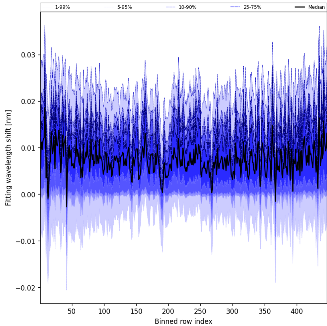
Figure 65: Along track statistics of “Fitting wavelength shift” for 2025-08-05 to 2025-08-07
