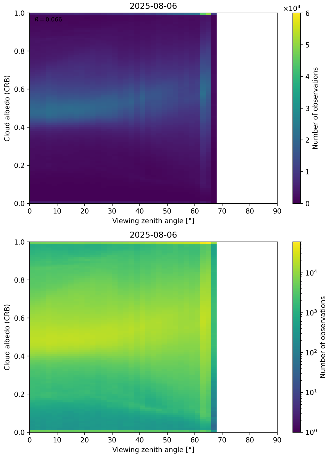
Figure 106: Scatter density plot of “Viewing zenith angle” against “Cloud albedo (CRB)” for 2025-08-05 to 2025-08-07.
