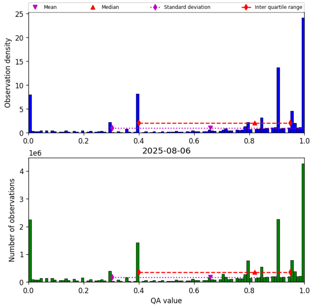
Figure 38: Histogram of “QA value” for 2025-08-05 to 2025-08-07
