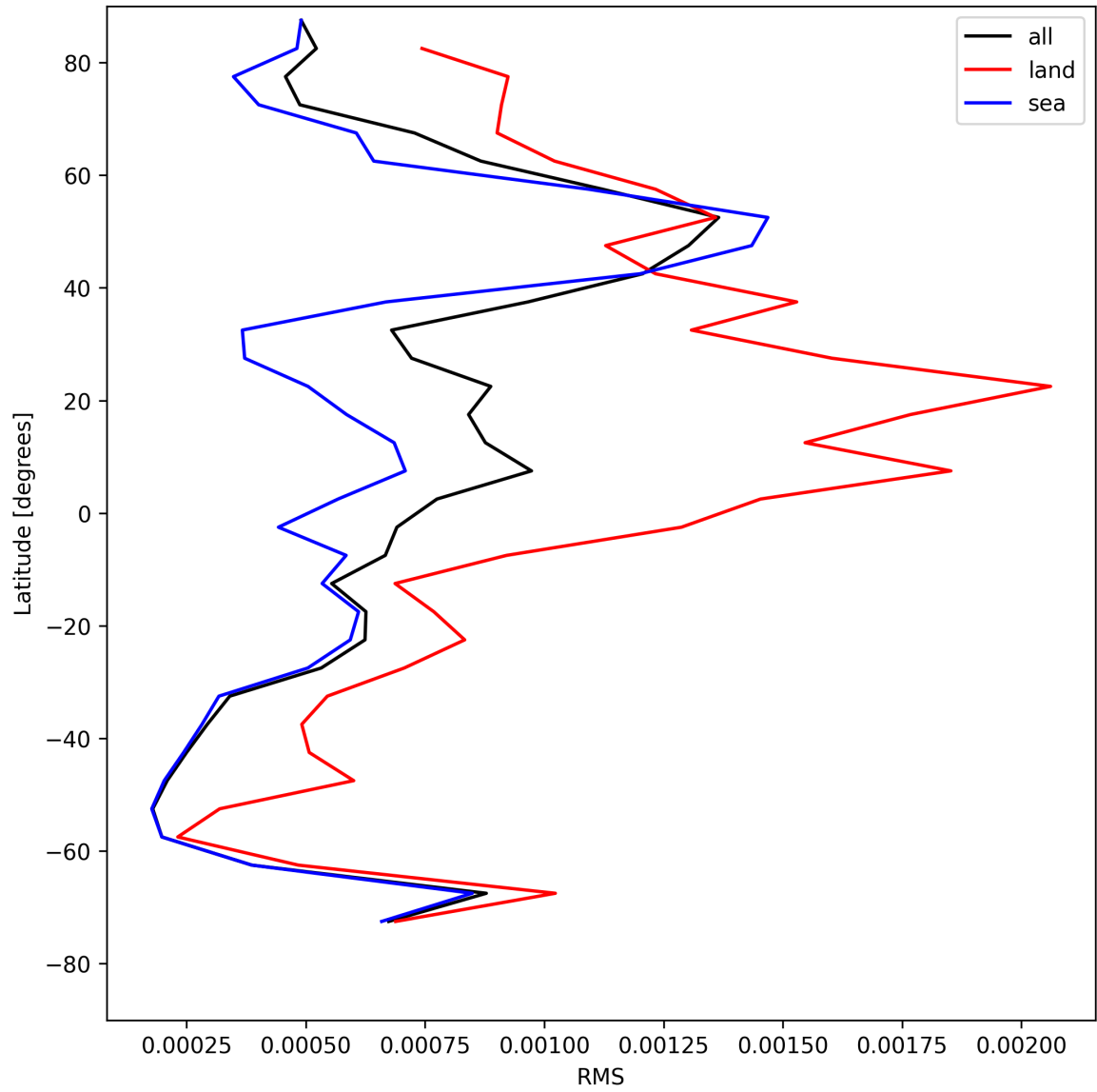
Figure 31: Zonal average of “RMS” for 2025-08-05 to 2025-08-07.
