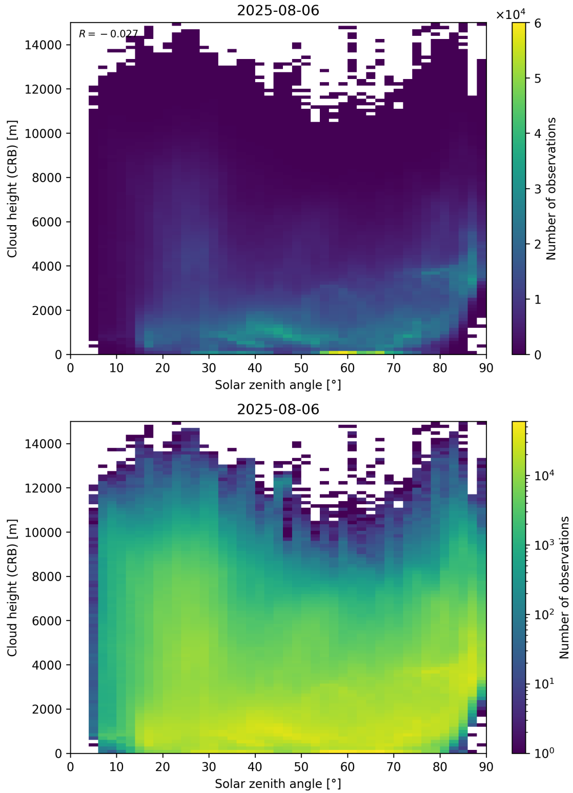
Figure 102: Scatter density plot of “Solar zenith angle” against “Cloud height (CRB)” for 2025-08-05 to 2025-08-07.
