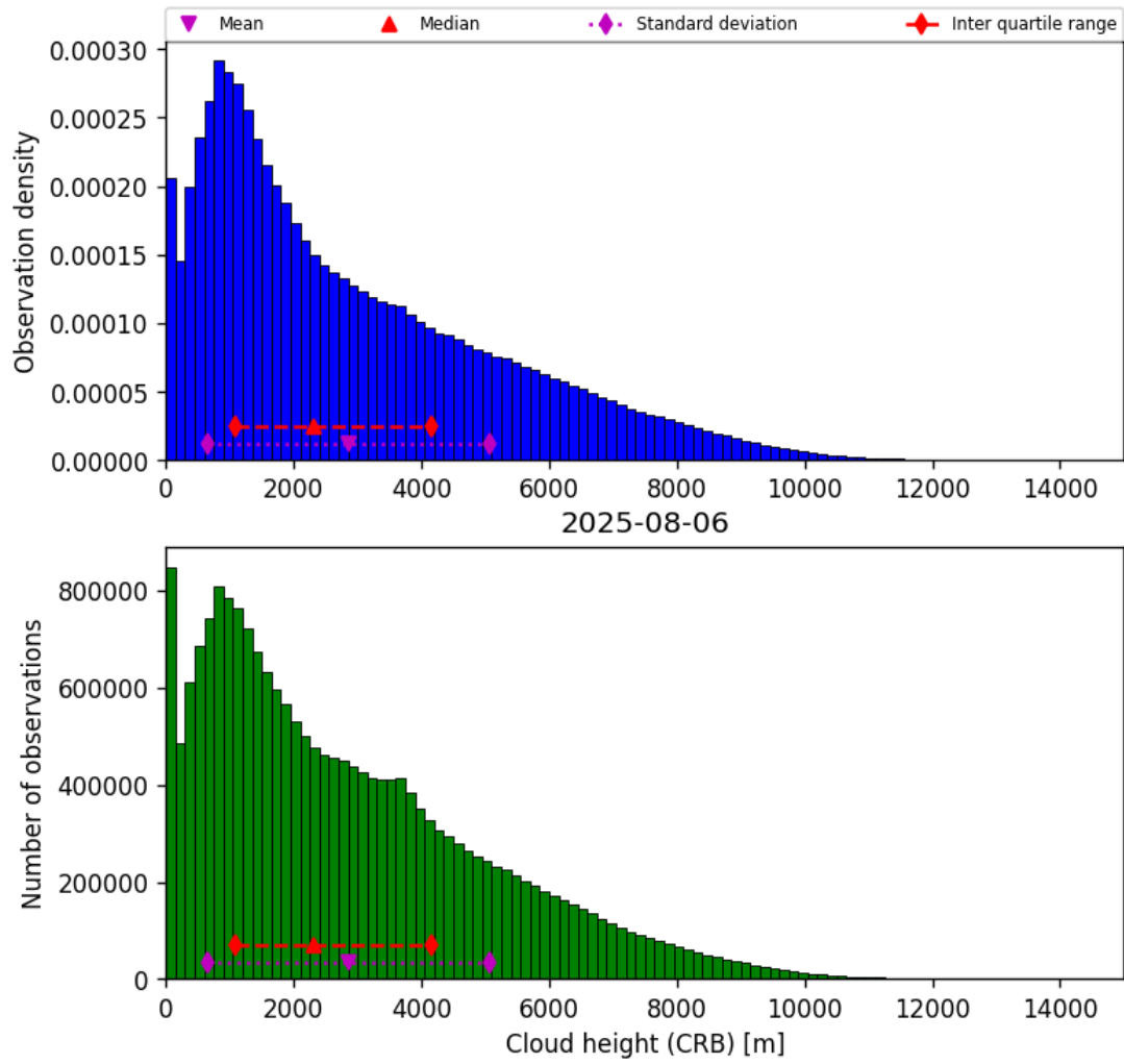
Figure 43: Histogram of “Cloud height (CRB)” for 2025-08-05 to 2025-08-07
