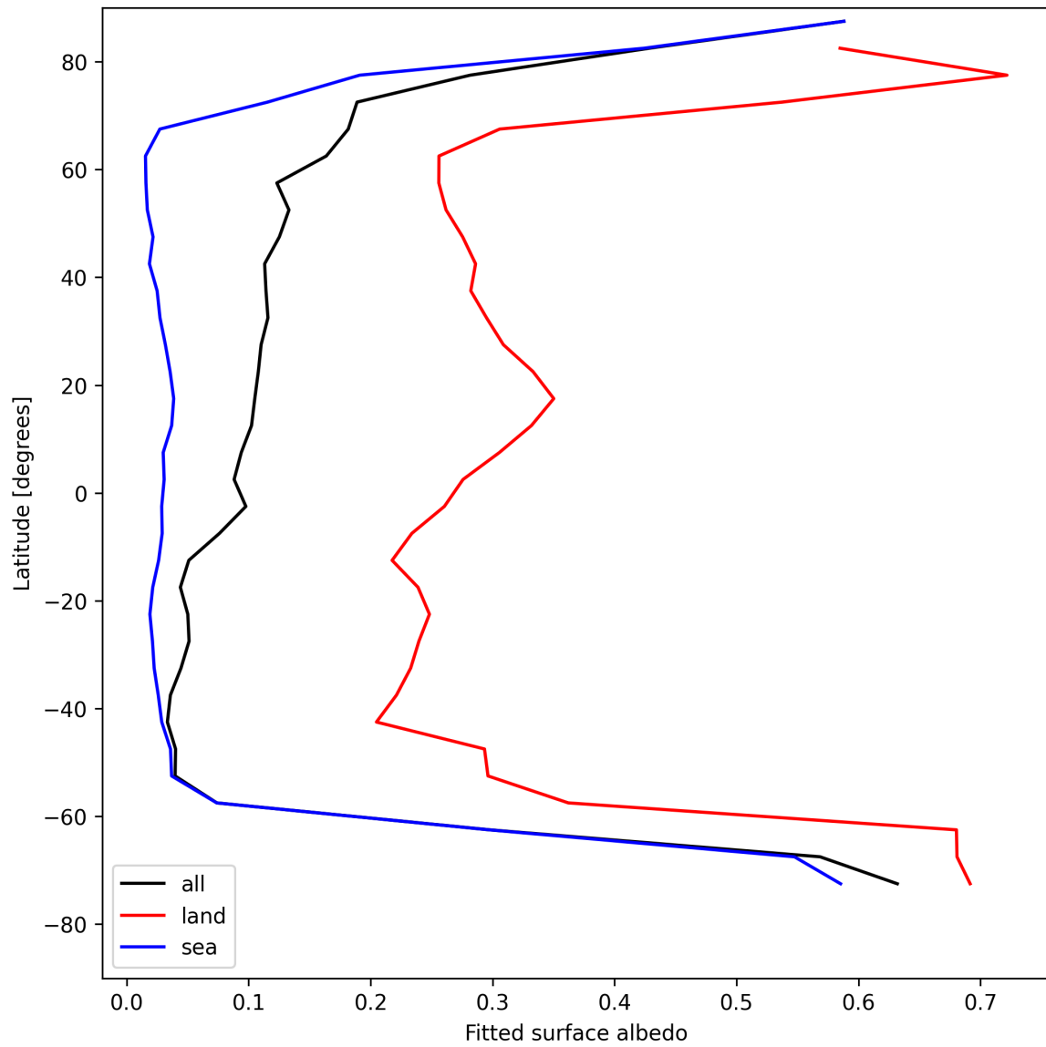
Figure 29: Zonal average of “Fitted surface albedo” for 2025-08-05 to 2025-08-07.
