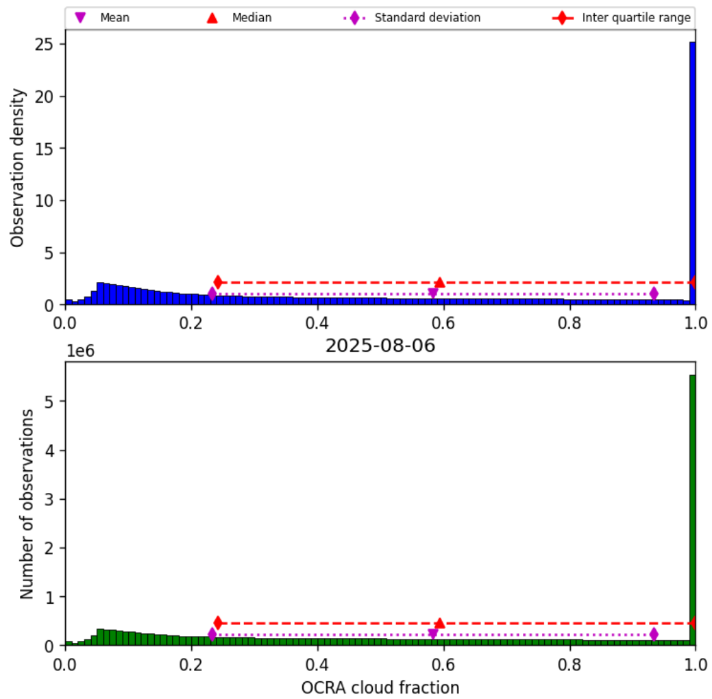
Figure 50: Histogram of “OCRA cloud fraction” for 2025-08-05 to 2025-08-07
