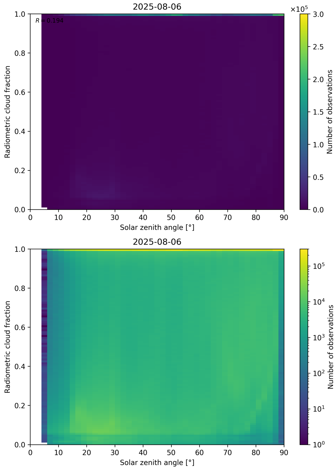
Figure 99: Scatter density plot of “Solar zenith angle” against “Radiometric cloud fraction” for 2025-08-05 to 2025-08-07.
