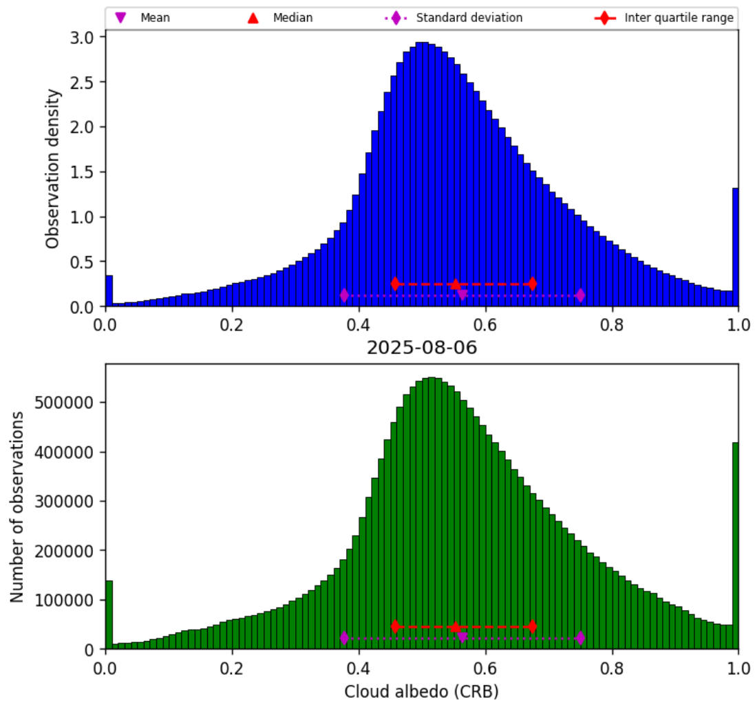
Figure 44: Histogram of “Cloud albedo (CRB)” for 2025-08-05 to 2025-08-07
