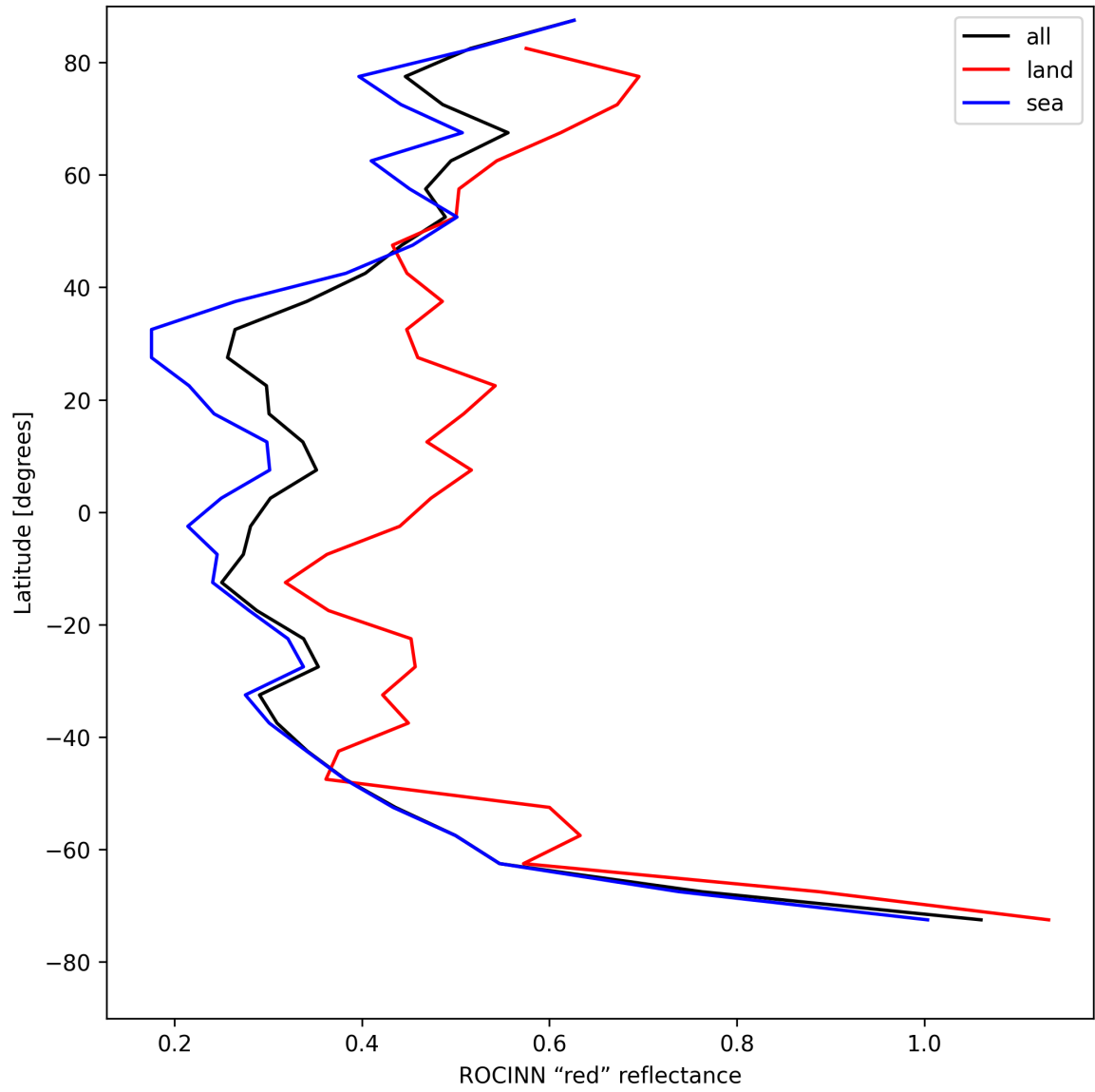
Figure 37: Zonal average of “ROCINN “red” reflectance” for 2025-08-05 to 2025-08-07.
