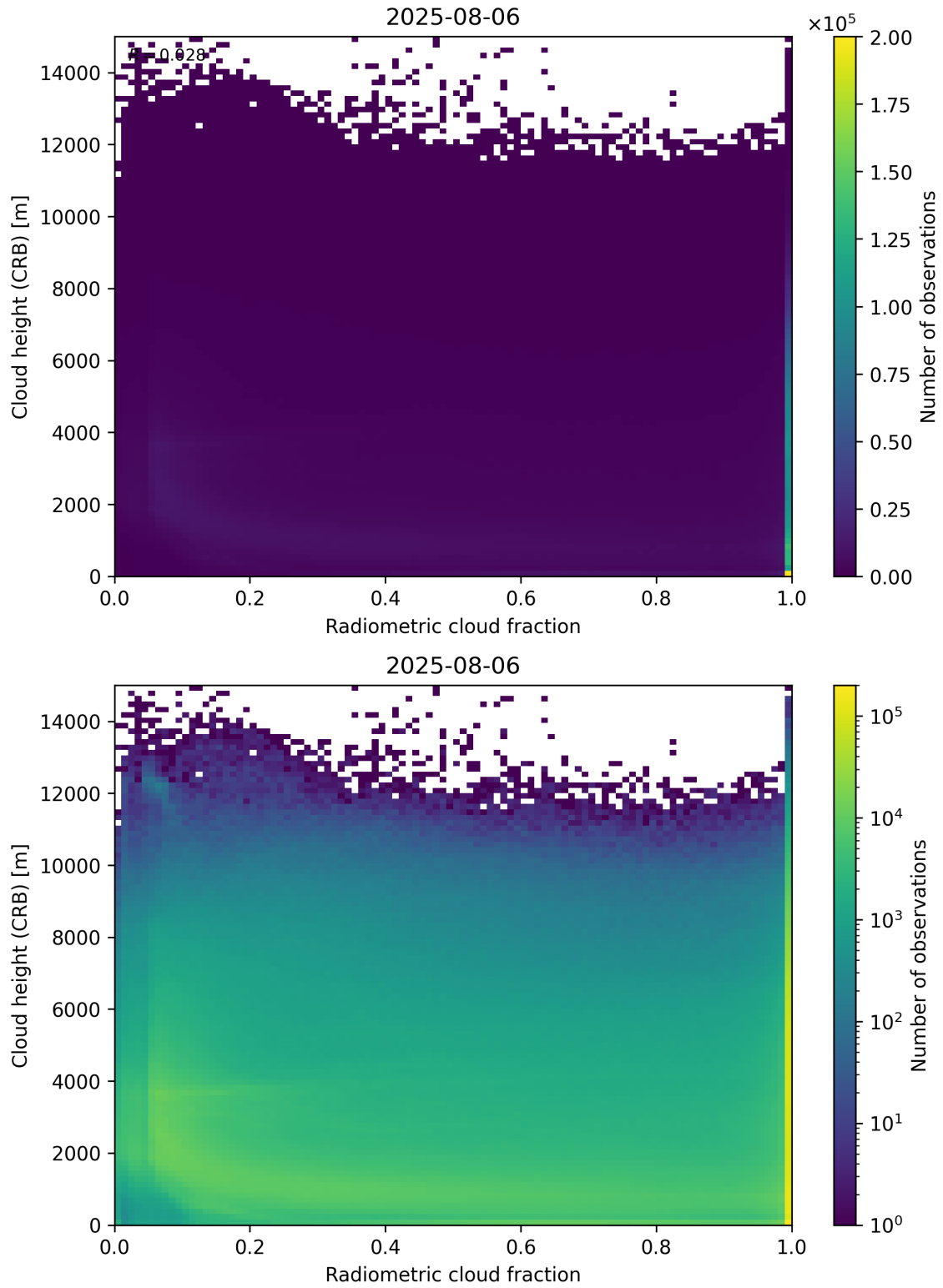
Figure 74: Scatter density plot of “Radiometric cloud fraction” against “Cloud height (CRB)” for 2025-08-05 to 2025-08-07.
