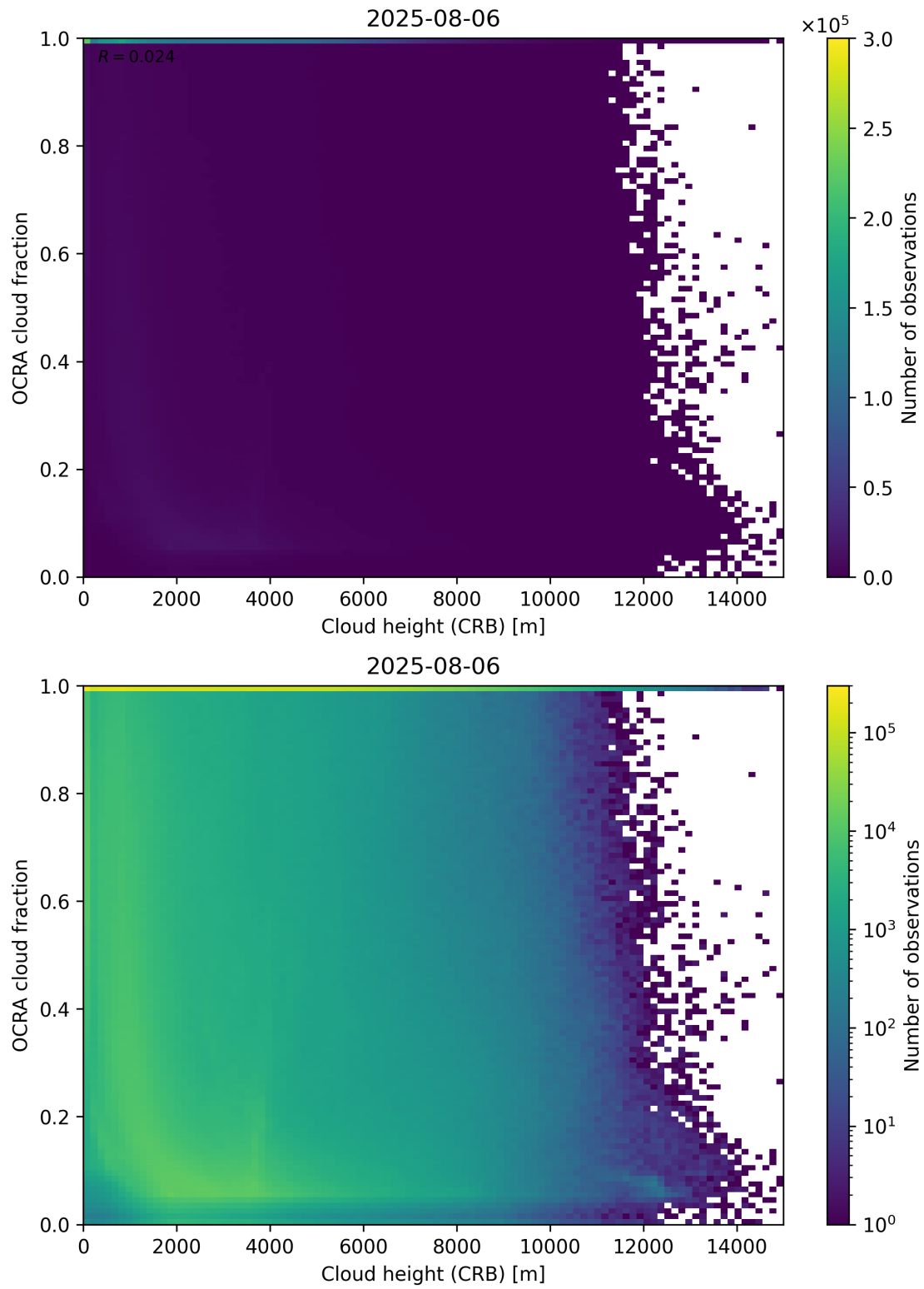
Figure 81: Scatter density plot of “Cloud height (CRB)” against “OCRA cloud fraction” for 2025-08-05 to 2025-08-07.
