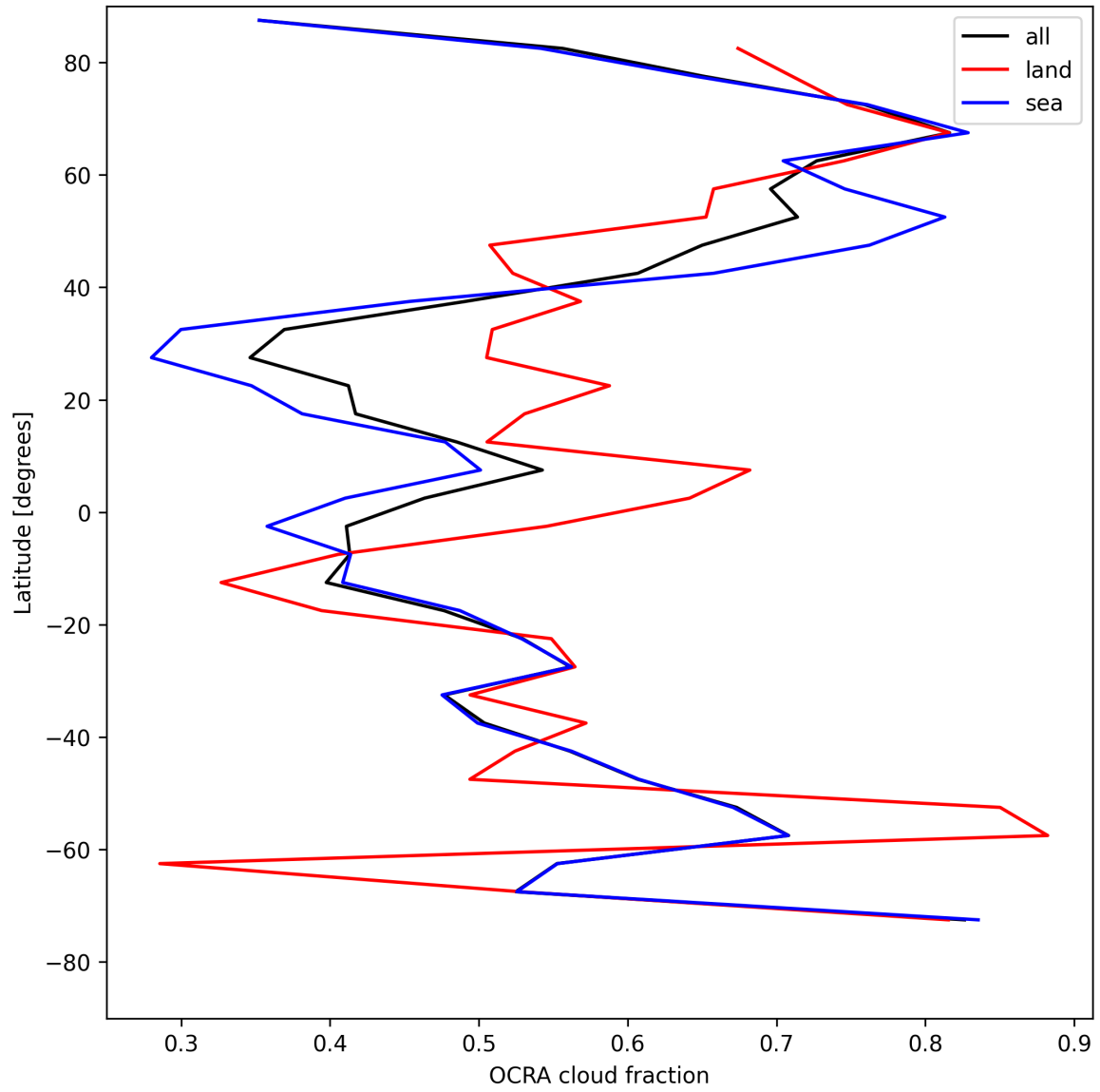
Figure 34: Zonal average of “OCRA cloud fraction” for 2025-08-05 to 2025-08-07.
