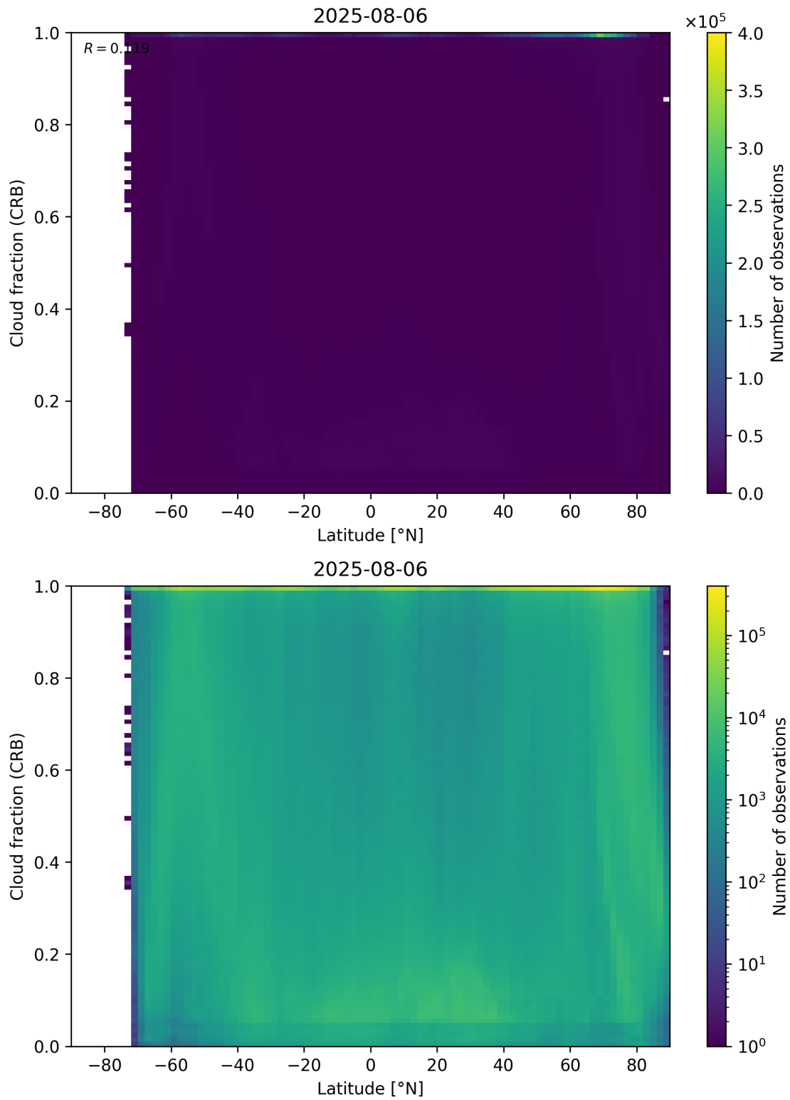
Figure 94: Scatter density plot of “Latitude” against “Cloud fraction (CRB)” for 2025-08-05 to 2025-08-07.
