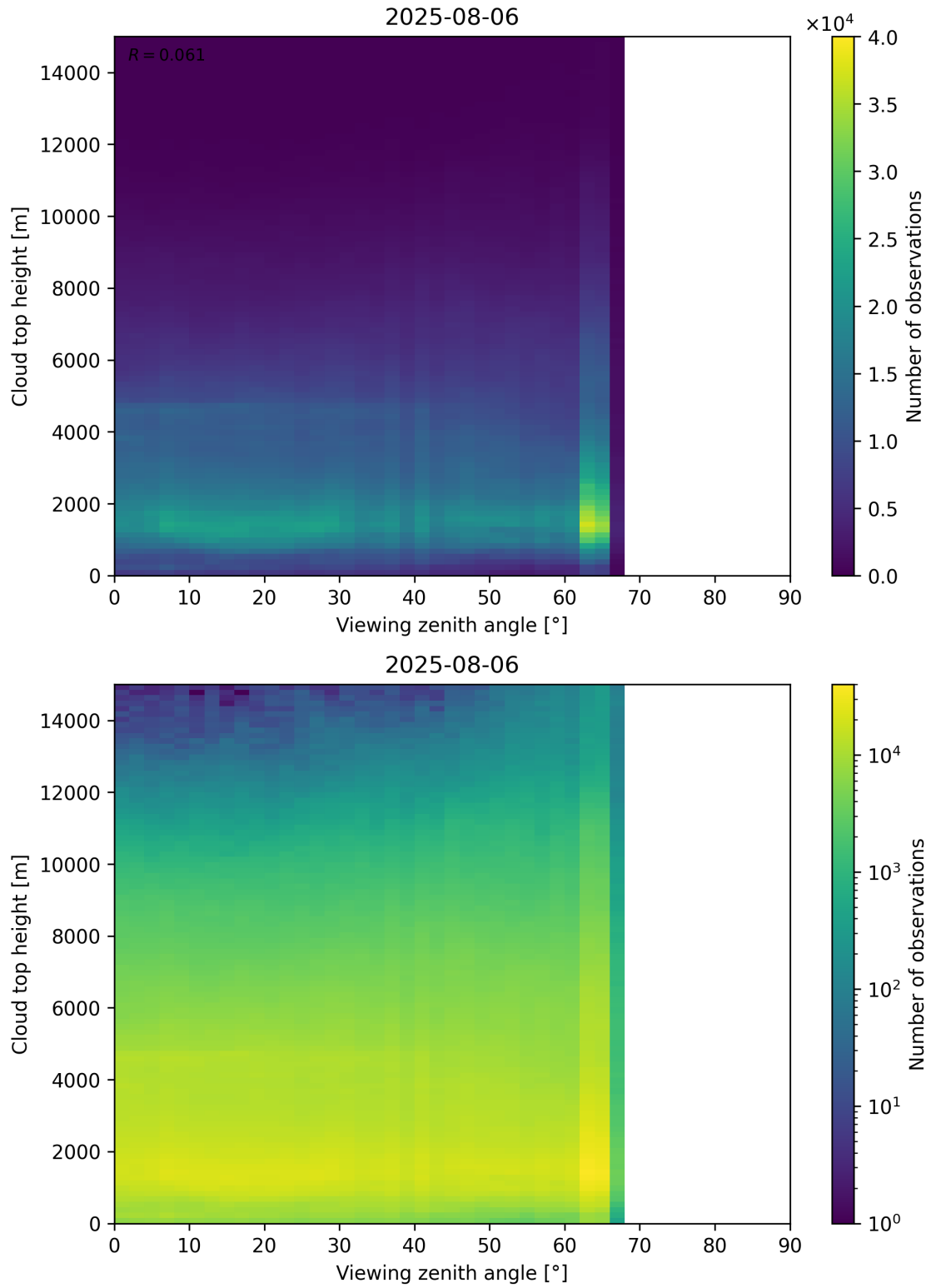
Figure 112: Scatter density plot of “Viewing zenith angle” against “Cloud top height” for 2025-08-05 to 2025-08-07.
