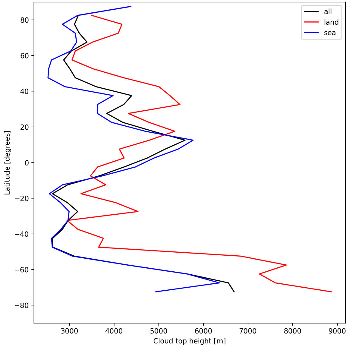
Figure 24: Zonal average of “Cloud top height” for 2025-08-05 to 2025-08-07.
