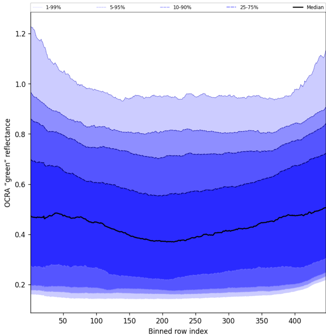
Figure 68: Along track statistics of "OCRA "green" reflectance" for 2025-08-05 to 2025-08-07
