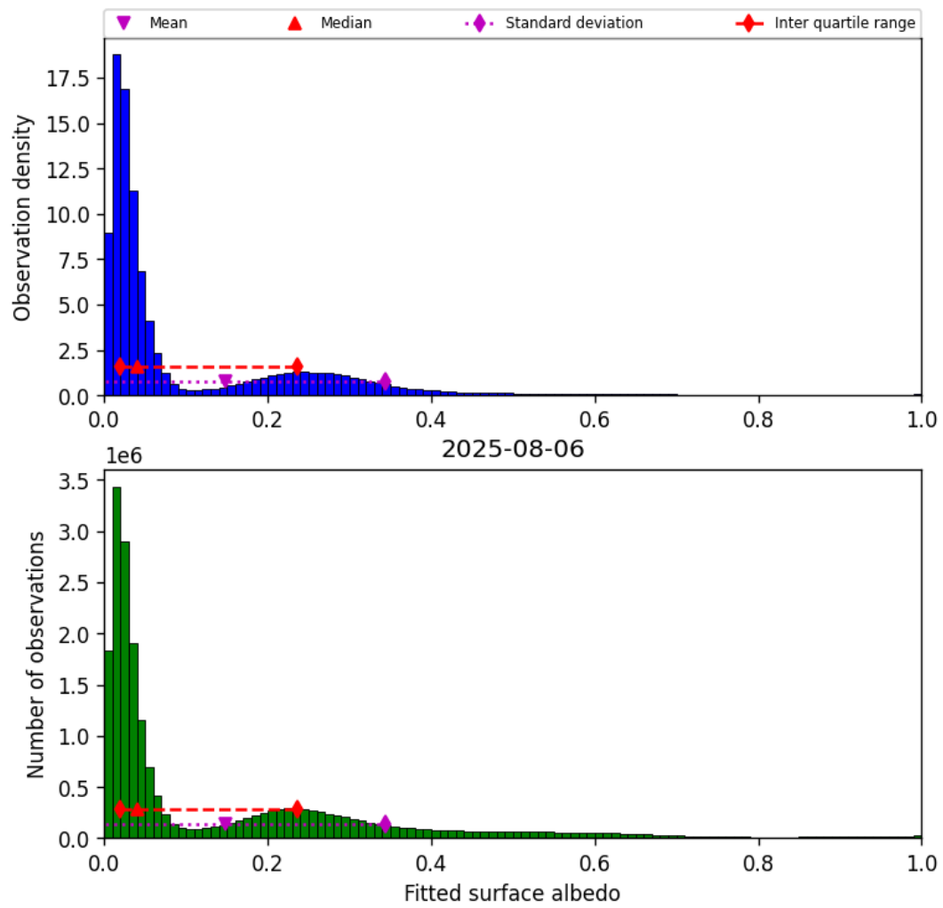
Figure 45: Histogram of “Fitted surface albedo” for 2025-08-05 to 2025-08-07
