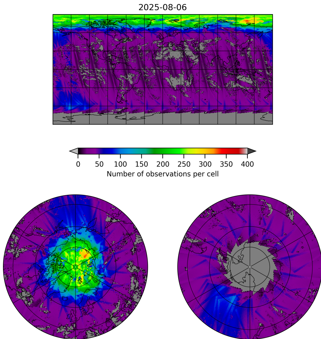
Figure 21: Map of the number of observations for 2025-08-05 to 2025-08-07
