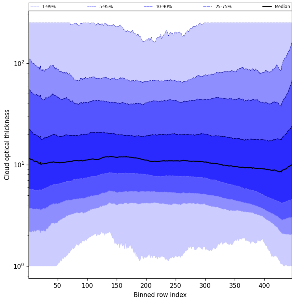
Figure 57: Along track statistics of “Cloud optical thickness” for 2025-08-05 to 2025-08-07
