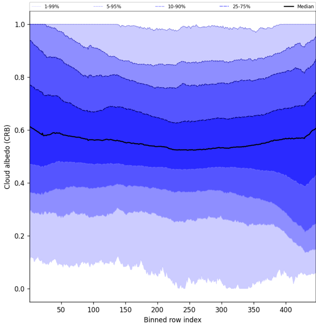
Figure 60: Along track statistics of “Cloud albedo (CRB)” for 2025-08-05 to 2025-08-07
