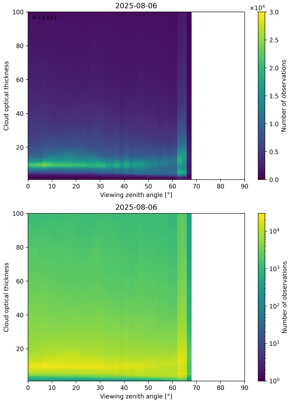
Figure 111: Scatter density plot of “Viewing zenith angle” against “Cloud optical thickness” for 2025-08-05 to 2025-08-07.
