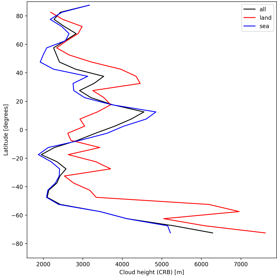
Figure 27: Zonal average of “Cloud height (CRB)” for 2025-08-05 to 2025-08-07.
