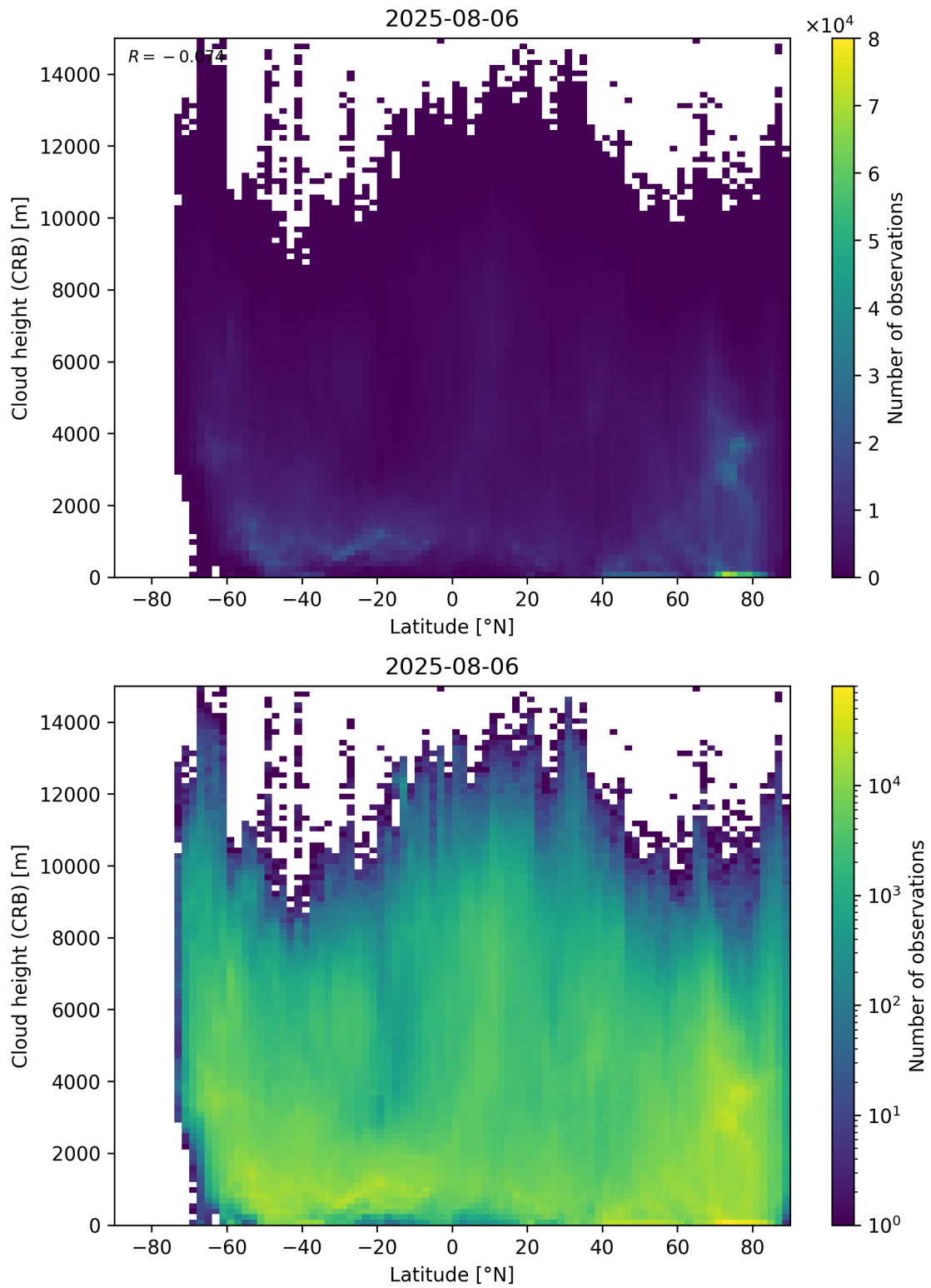
Figure 95: Scatter density plot of “Latitude” against “Cloud height (CRB)” for 2025-08-05 to 2025-08-07.
