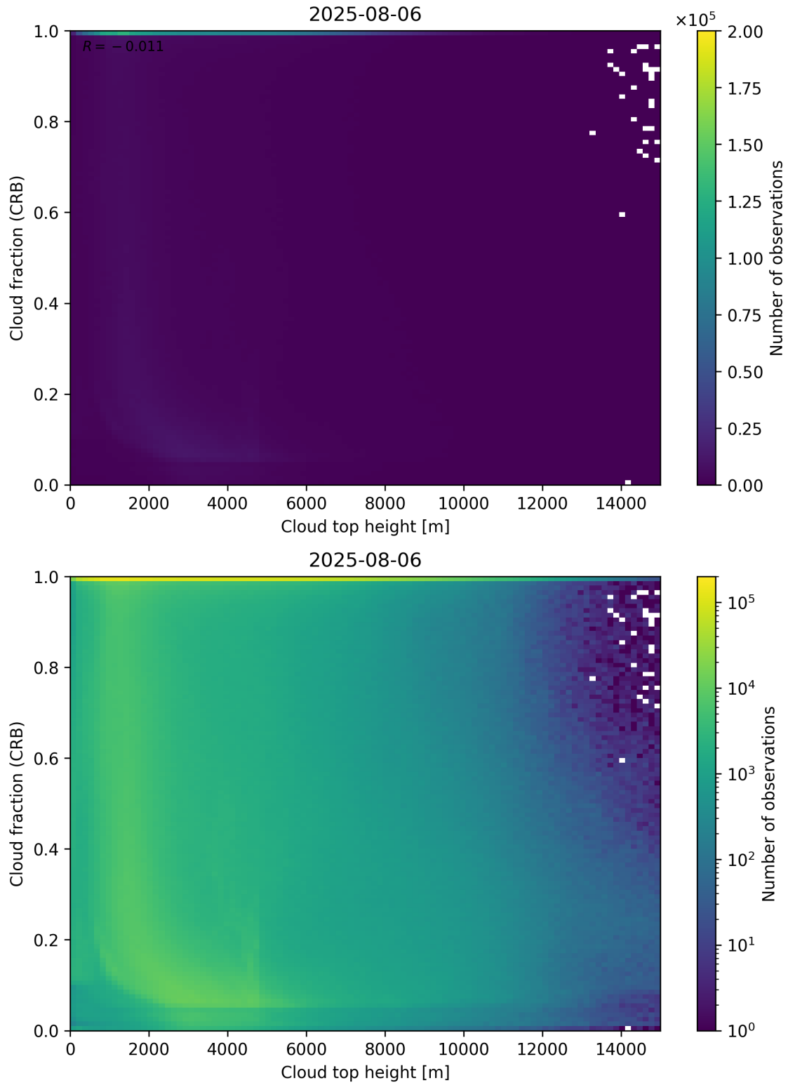
Figure 88: Scatter density plot of “Cloud top height” against “Cloud fraction (CRB)” for 2025-08-05 to 2025-08-07.
