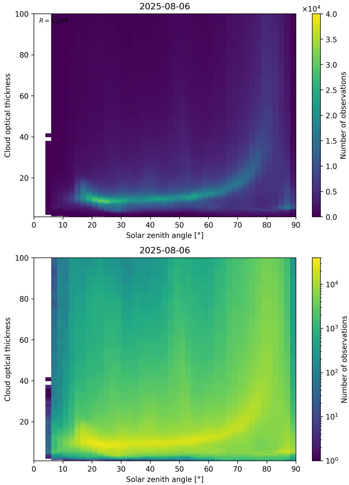
Figure 103: Scatter density plot of “Solar zenith angle” against “Cloud optical thickness” for 2025-08-05 to 2025-08-07.
