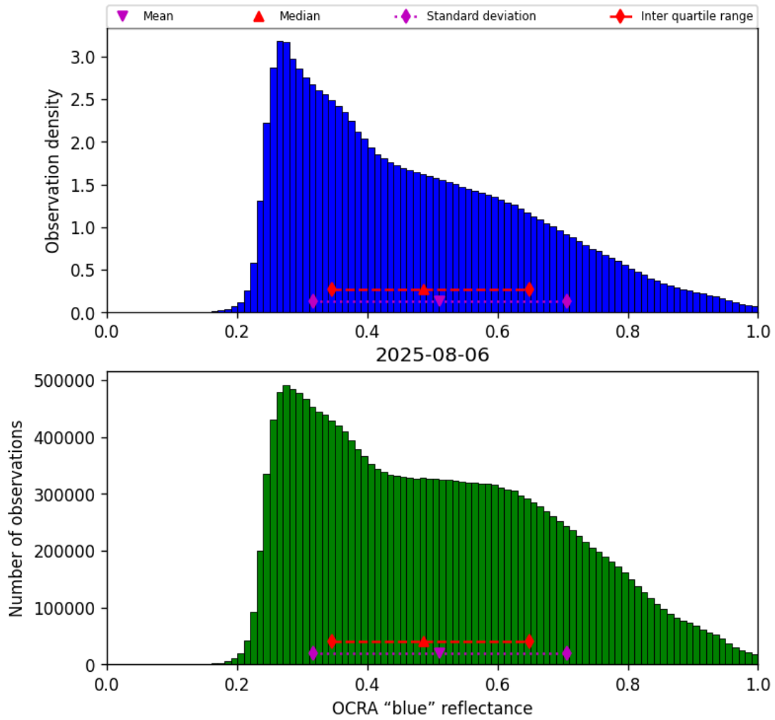
Figure 51: Histogram of “OCRA “blue” reflectance” for 2025-08-05 to 2025-08-07
