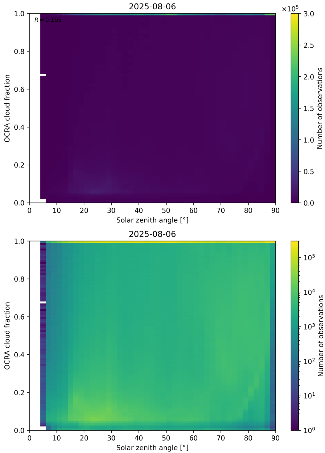
Figure 100: Scatter density plot of “Solar zenith angle” against “OCRA cloud fraction” for 2025-08-05 to 2025-08-07.
