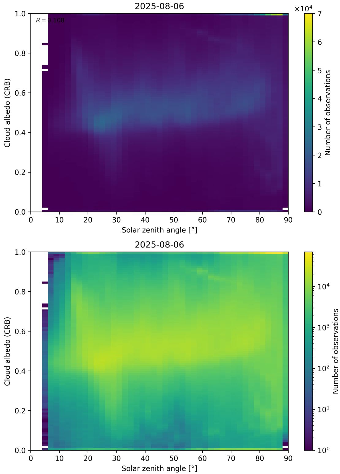
Figure 98: Scatter density plot of “Solar zenith angle” against “Cloud albedo (CRB)” for 2025-08-05 to 2025-08-07.
