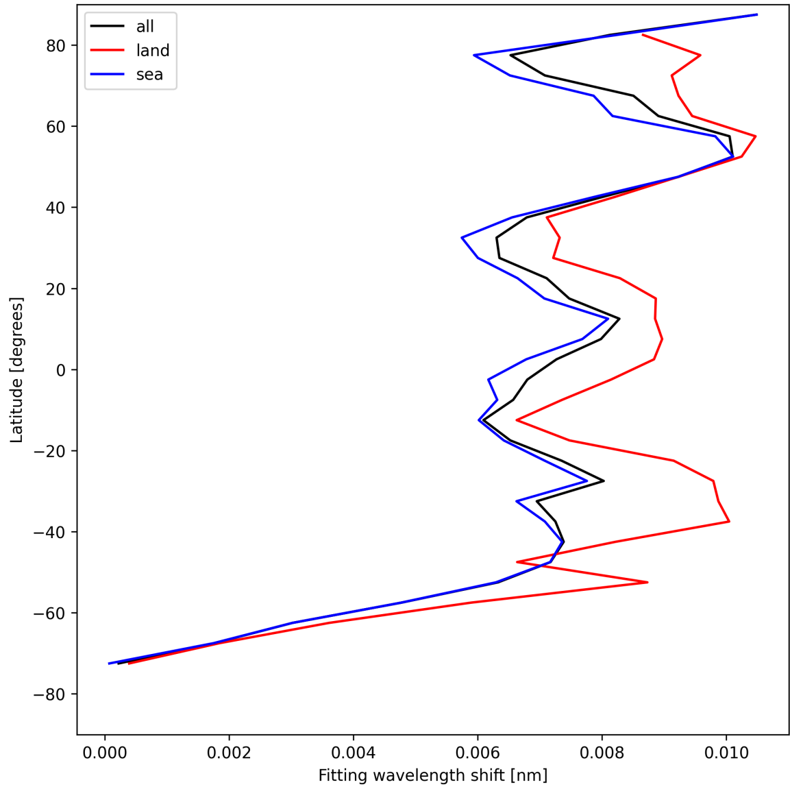
Figure 33: Zonal average of “Fitting wavelength shift” for 2025-08-05 to 2025-08-07.
