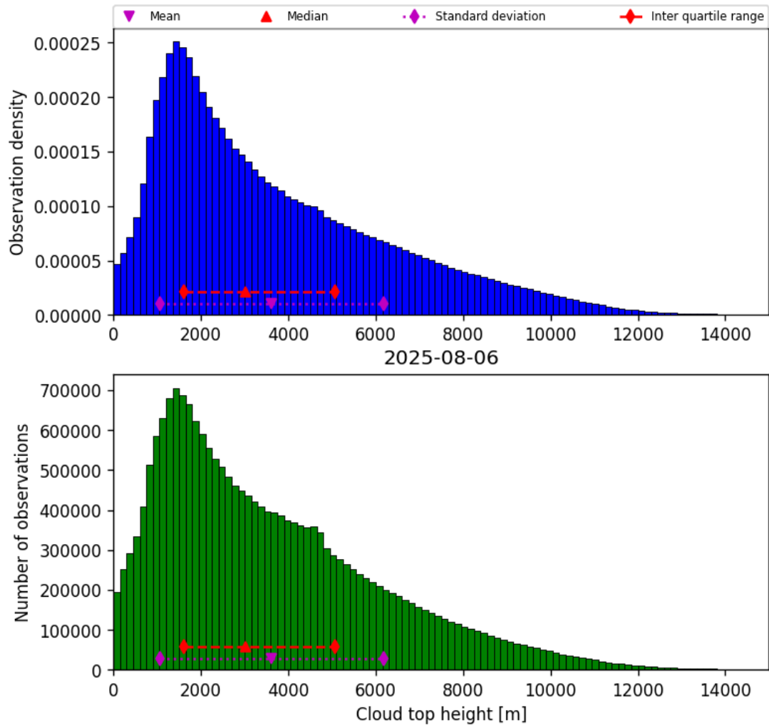
Figure 40: Histogram of “Cloud top height” for 2025-08-05 to 2025-08-07
