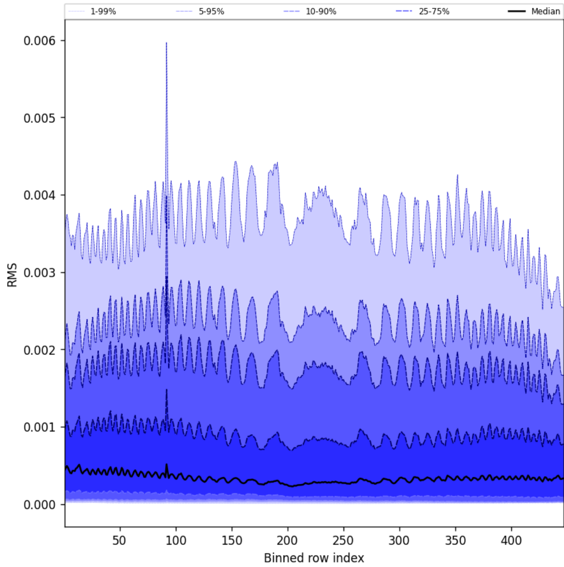
Figure 63: Along track statistics of “RMS” for 2025-08-05 to 2025-08-07
