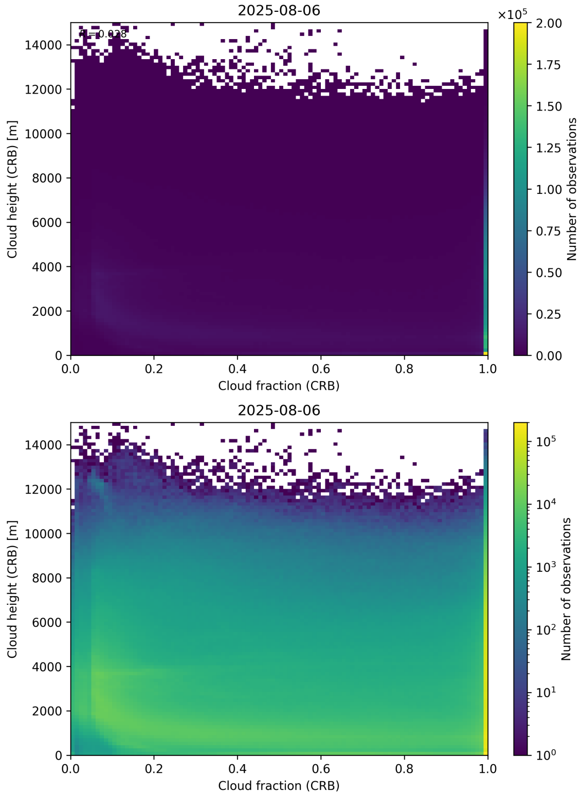
Figure 79: Scatter density plot of “Cloud fraction (CRB)” against “Cloud height (CRB)” for 2025-08-05 to 2025-08-07.
