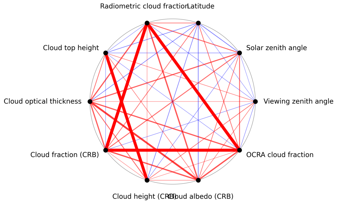
Figure 1: Map of correlation graph for 2025-08-05 to 2025-08-07.
