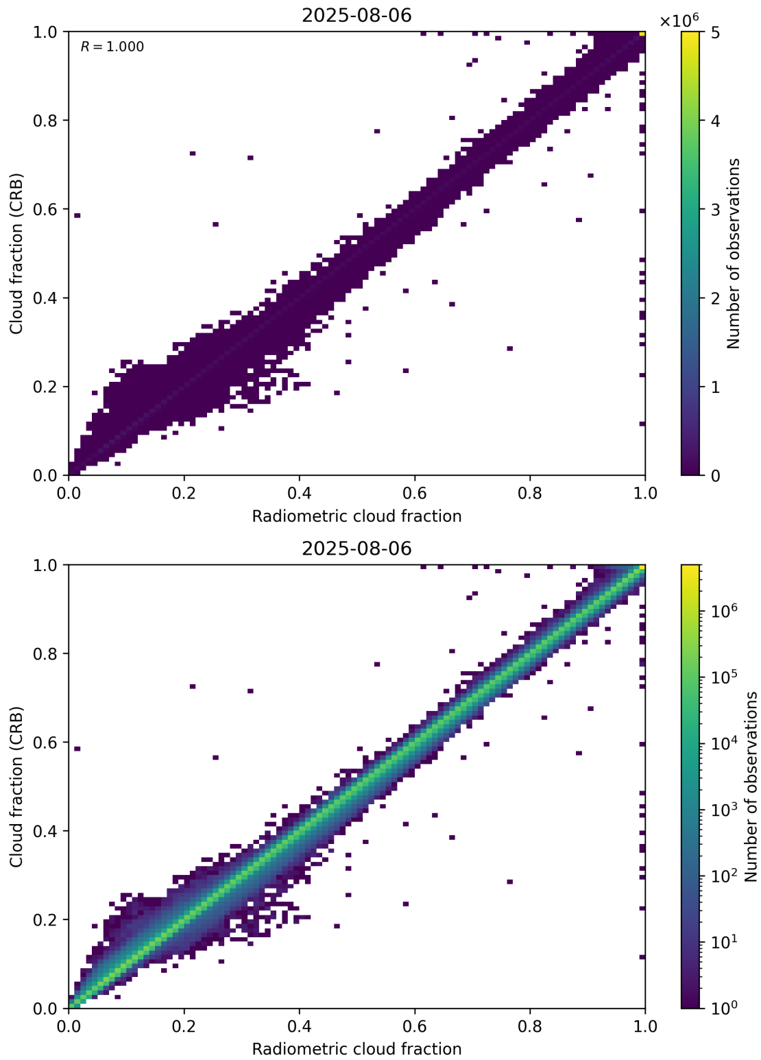
Figure 73: Scatter density plot of “Radiometric cloud fraction” against “Cloud fraction (CRB)” for 2025-08-05 to 2025-08-07.
