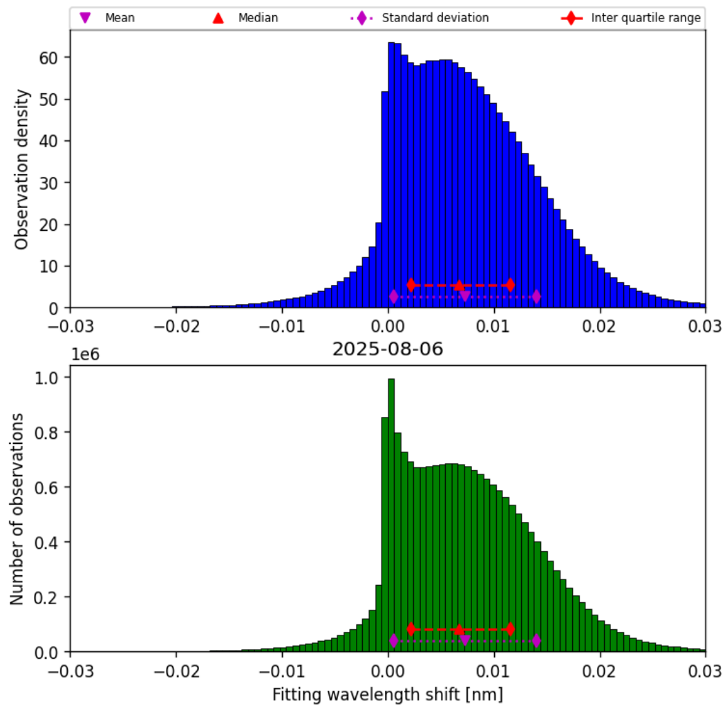
Figure 49: Histogram of “Fitting wavelength shift” for 2025-08-05 to 2025-08-07
