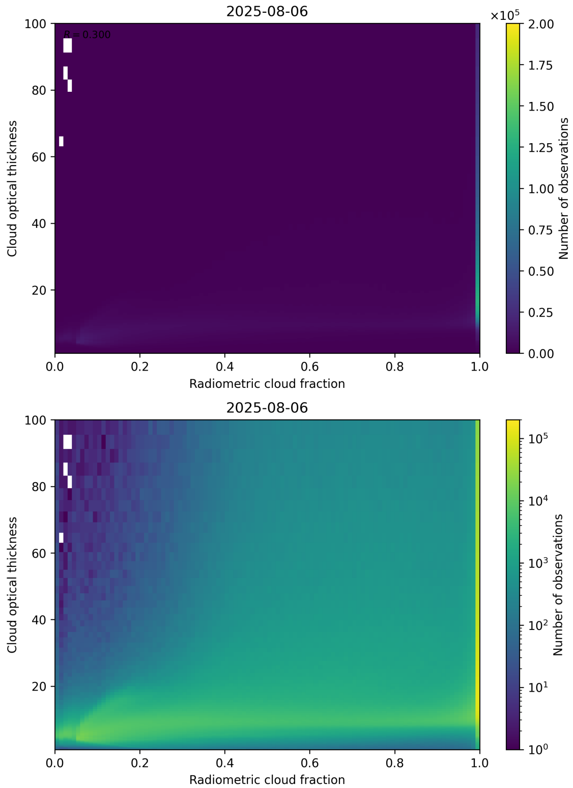
Figure 75: Scatter density plot of “Radiometric cloud fraction” against “Cloud optical thickness” for 2025-08-05 to 2025-08-07.
