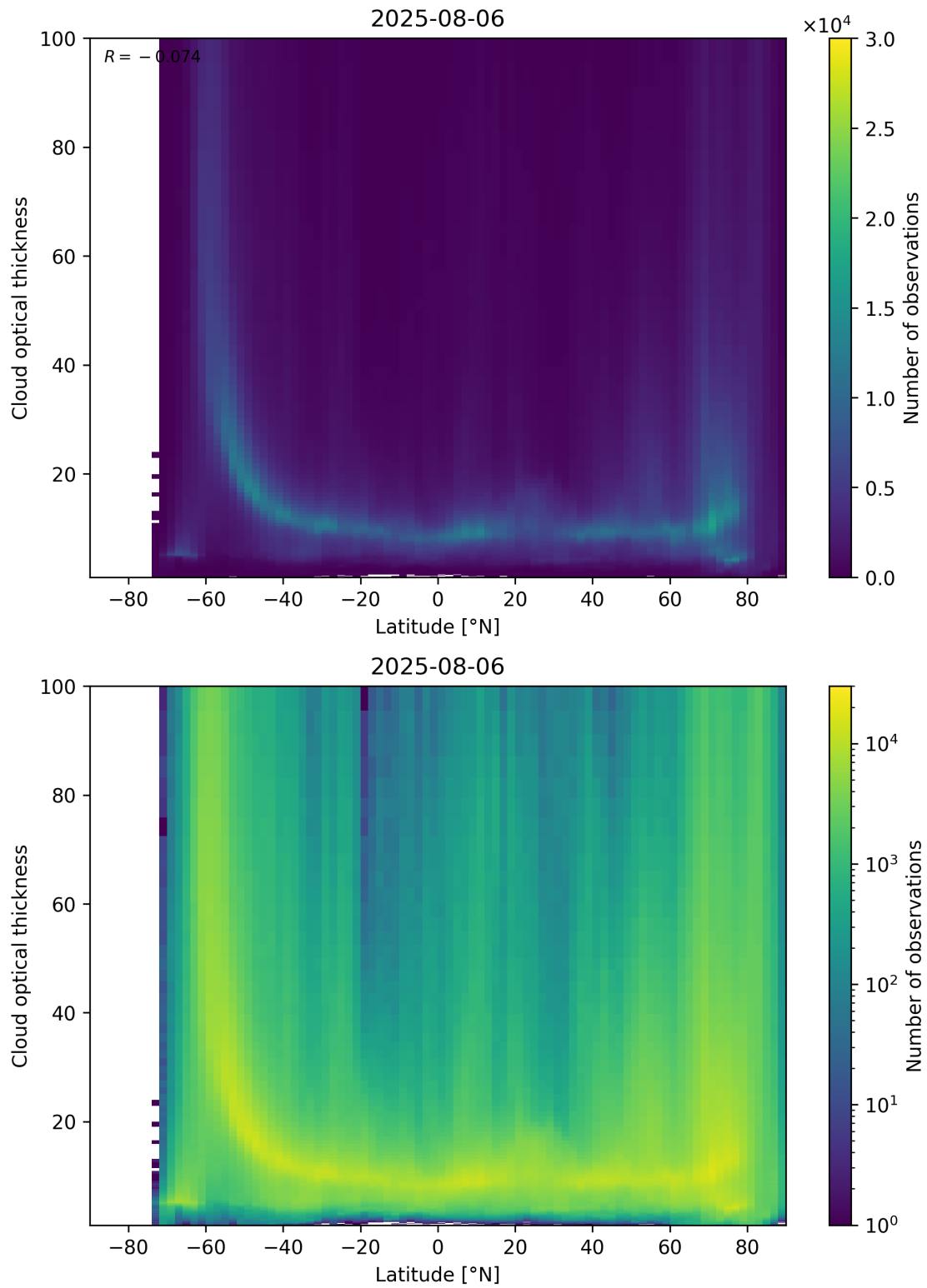
Figure 96: Scatter density plot of “Latitude” against “Cloud optical thickness” for 2025-08-05 to 2025-08-07.
