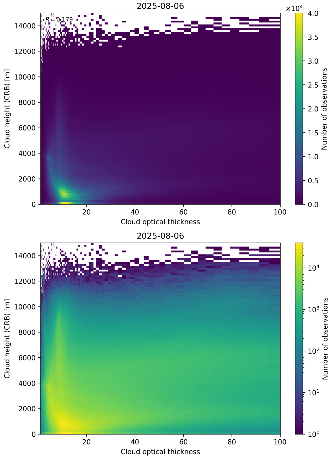
Figure 85: Scatter density plot of “Cloud optical thickness” against “Cloud height (CRB)” for 2025-08-05 to 2025-08-07.
