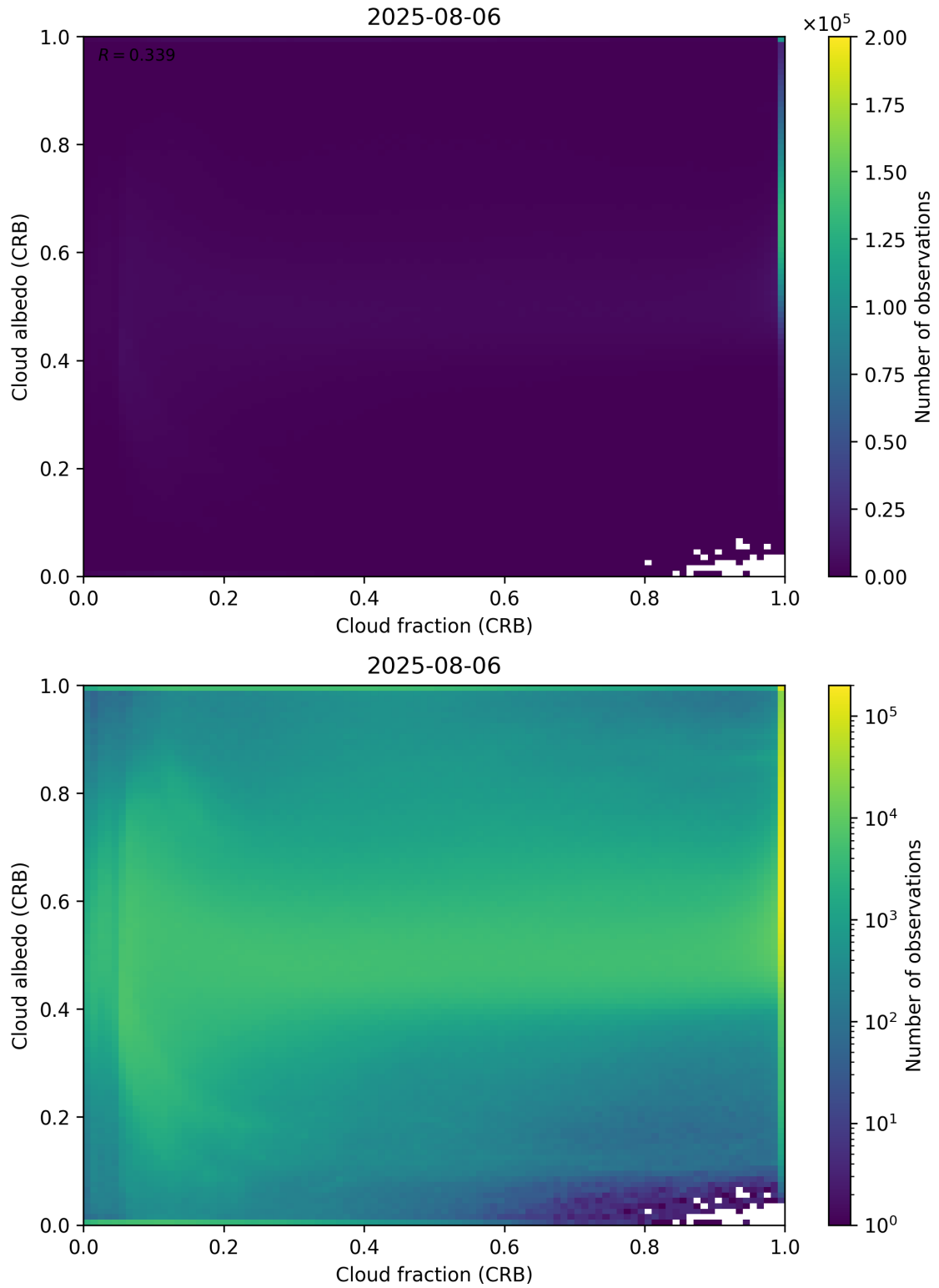
Figure 77: Scatter density plot of “Cloud fraction (CRB)” against “Cloud albedo (CRB)” for 2025-08-05 to 2025-08-07.
