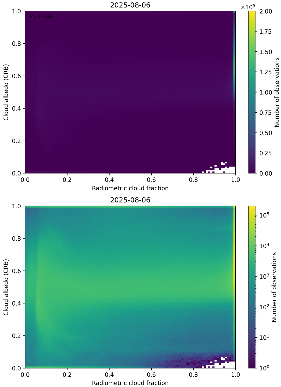
Figure 71: Scatter density plot of “Radiometric cloud fraction” against “Cloud albedo (CRB)” for 2025-08-05 to 2025-08-07.
