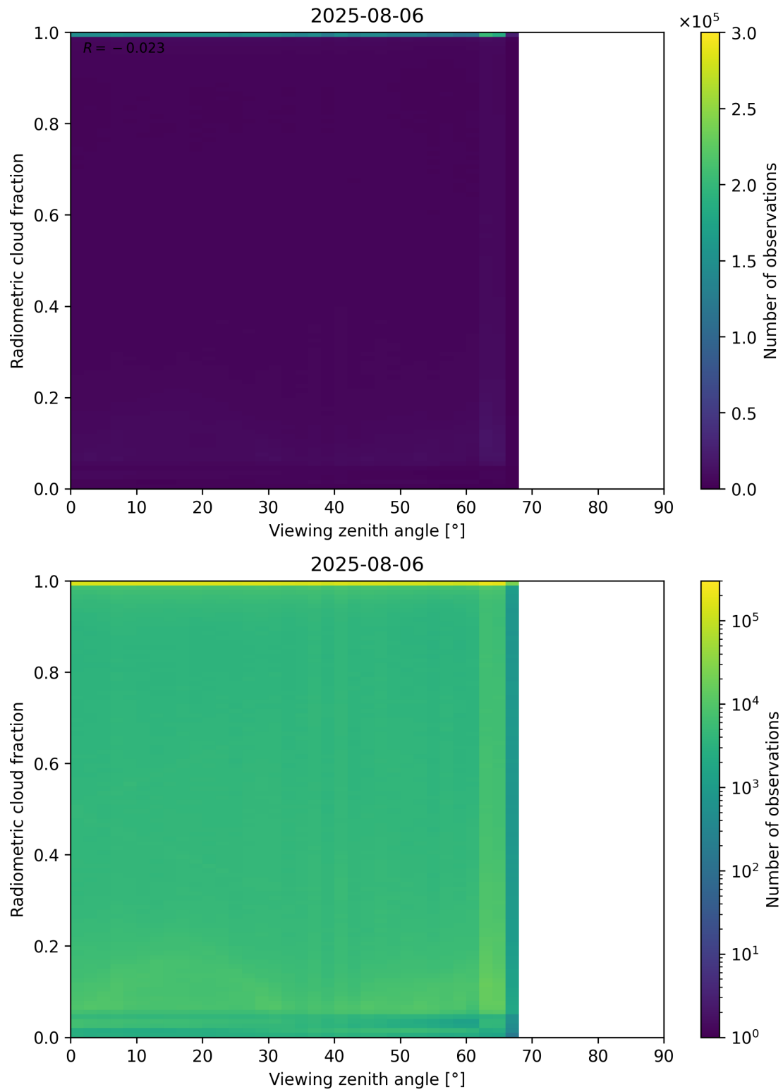
Figure 107: Scatter density plot of “Viewing zenith angle” against “Radiometric cloud fraction” for 2025-08-05 to 2025-08-07.
