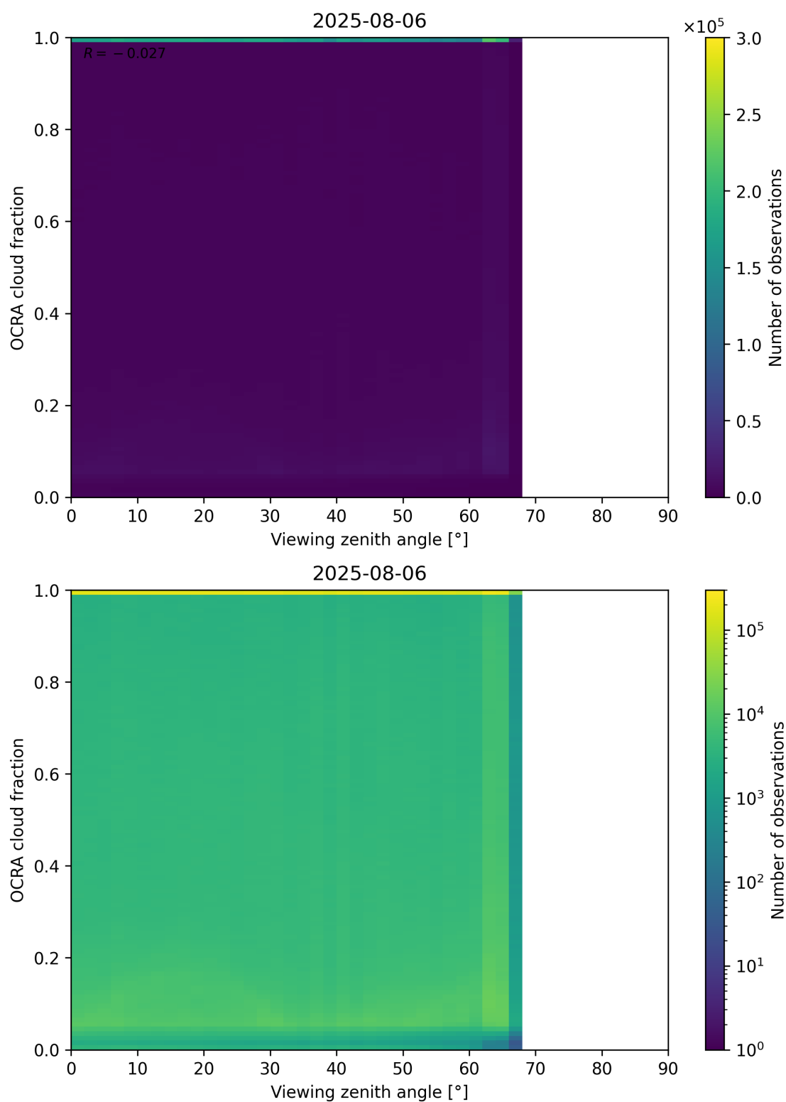
Figure 108: Scatter density plot of “Viewing zenith angle” against “OCRA cloud fraction” for 2025-08-05 to 2025-08-07.
