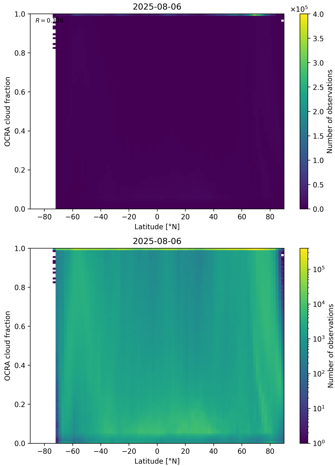
Figure 93: Scatter density plot of “Latitude” against “OCRA cloud fraction” for 2025-08-05 to 2025-08-07.
