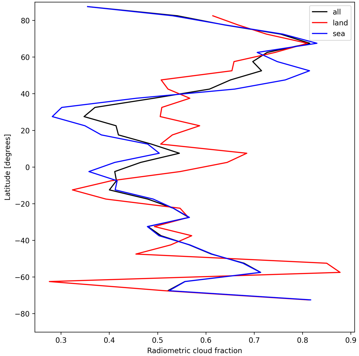
Figure 23: Zonal average of “Radiometric cloud fraction” for 2025-08-05 to 2025-08-07.
