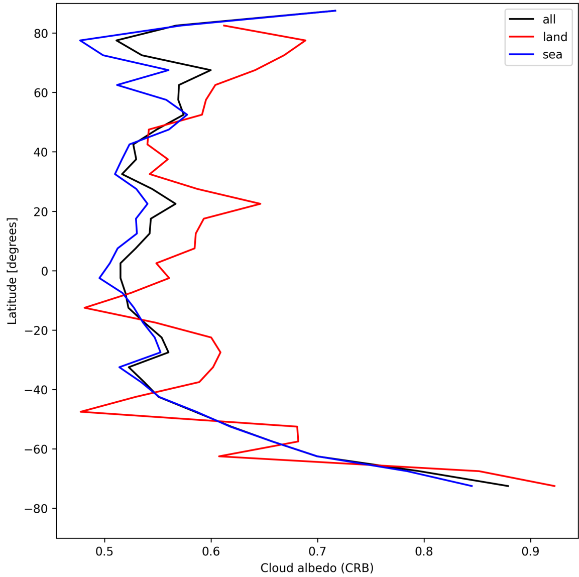
Figure 28: Zonal average of “Cloud albedo (CRB)” for 2025-08-05 to 2025-08-07.
