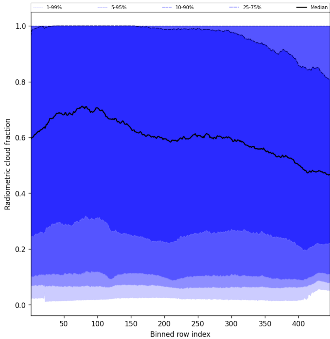
Figure 55: Along track statistics of “Radiometric cloud fraction” for 2025-08-05 to 2025-08-07
