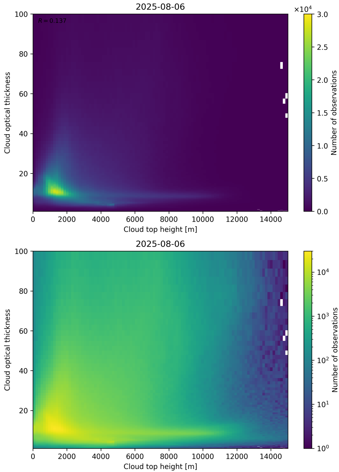
Figure 90: Scatter density plot of “Cloud top height” against “Cloud optical thickness” for 2025-08-05 to 2025-08-07.
