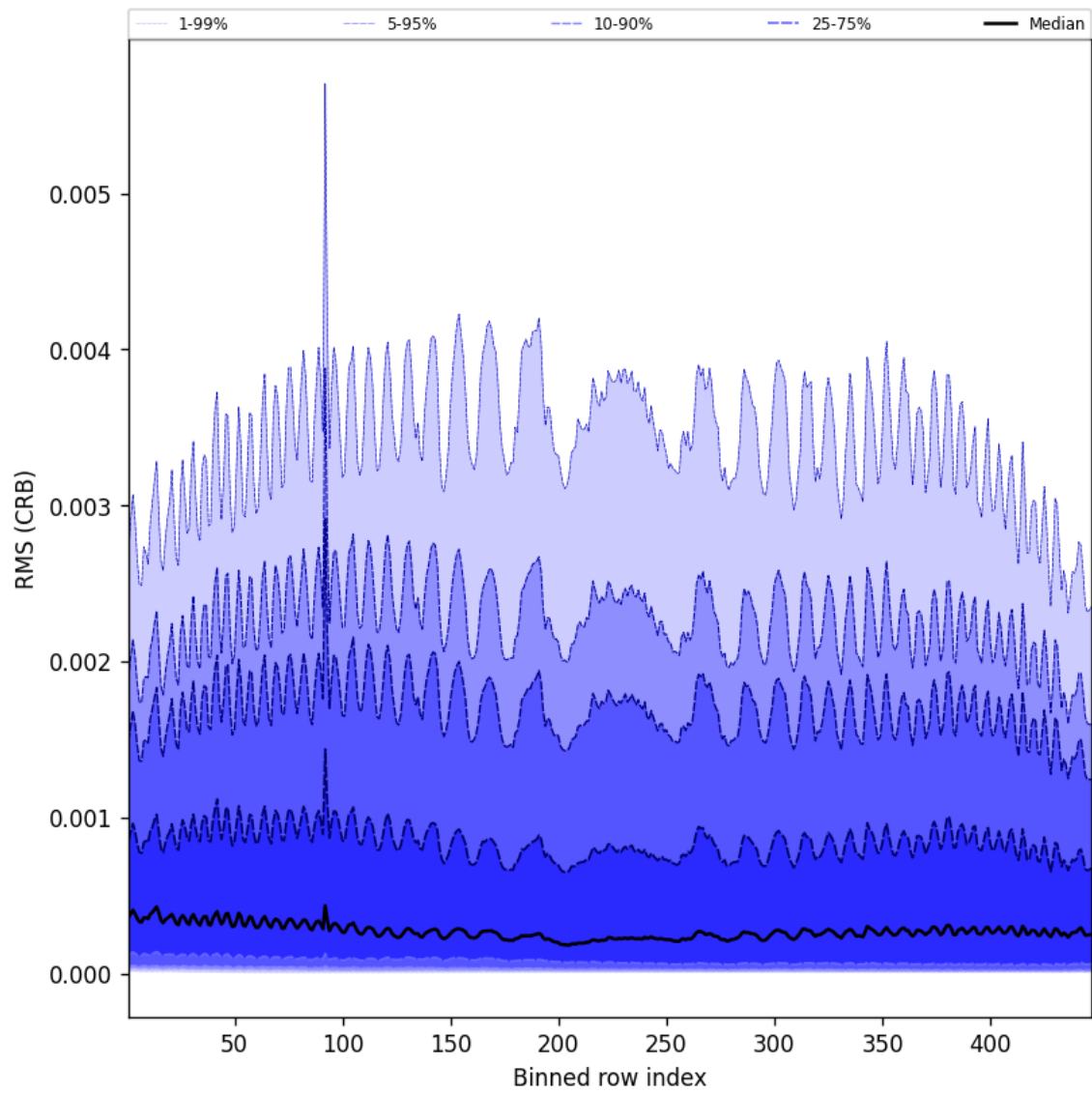
Figure 64: Along track statistics of “RMS (CRB)” for 2025-08-05 to 2025-08-07
