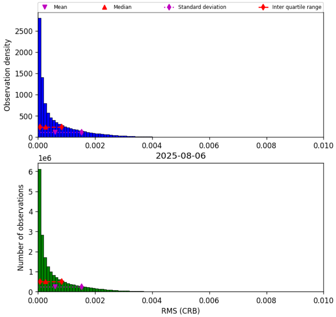
Figure 48: Histogram of “RMS (CRB)” for 2025-08-05 to 2025-08-07
