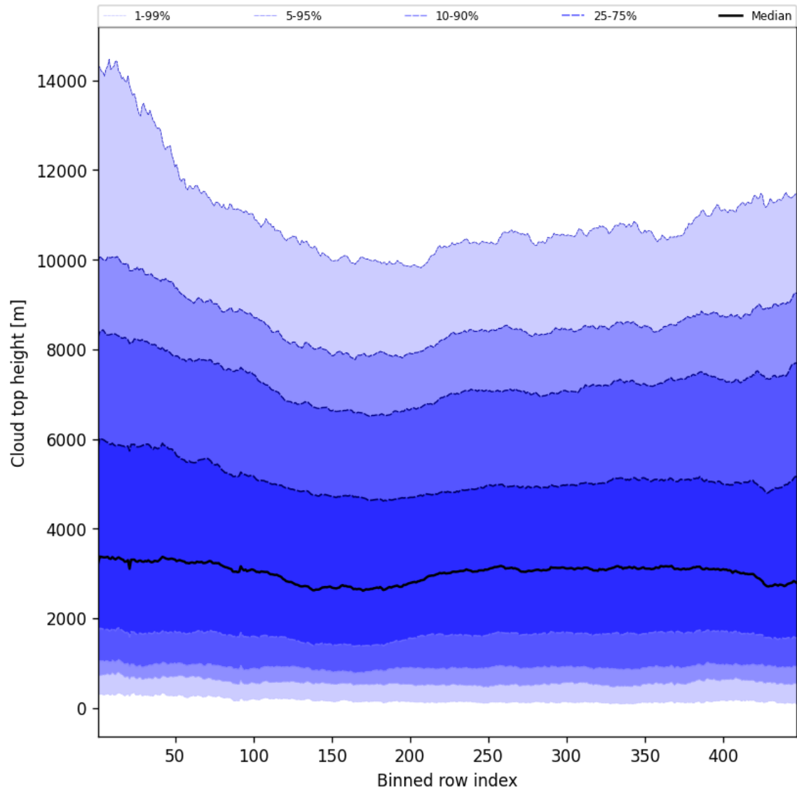
Figure 56: Along track statistics of “Cloud top height” for 2025-08-05 to 2025-08-07
