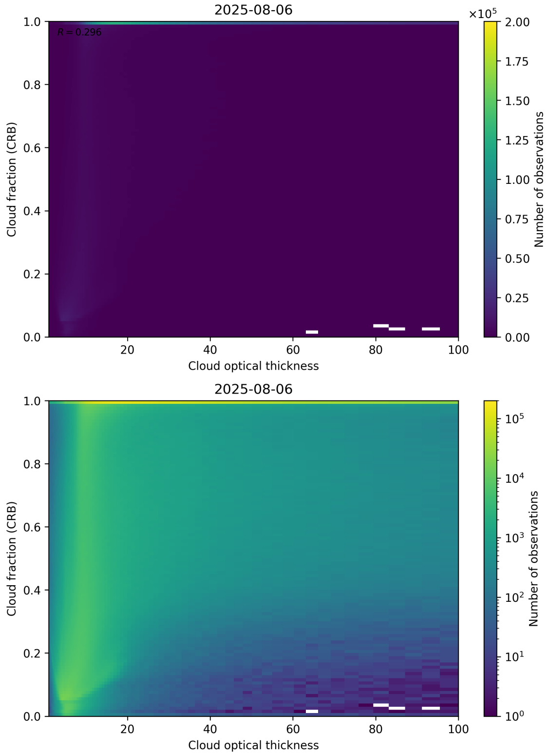
Figure 84: Scatter density plot of “Cloud optical thickness” against “Cloud fraction (CRB)” for 2025-08-05 to 2025-08-07.
