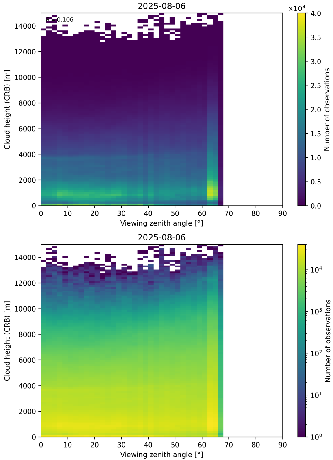
Figure 110: Scatter density plot of “Viewing zenith angle” against “Cloud height (CRB)” for 2025-08-05 to 2025-08-07.
