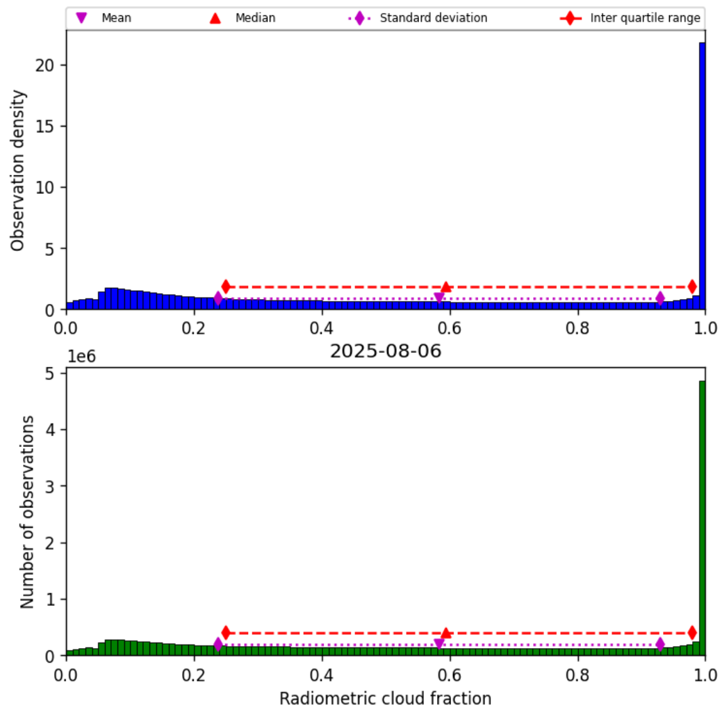
Figure 39: Histogram of “Radiometric cloud fraction” for 2025-08-05 to 2025-08-07
