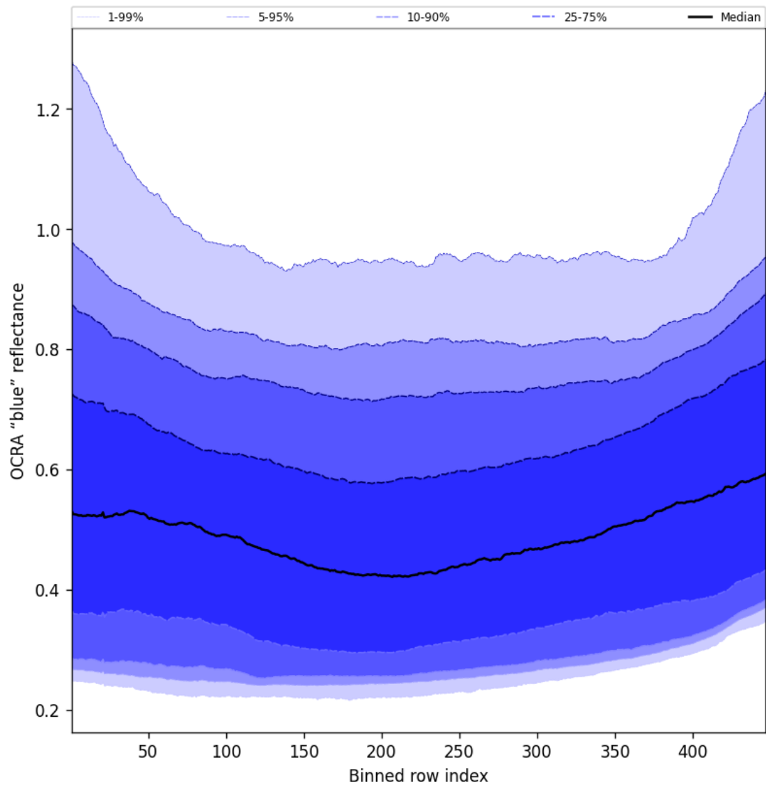
Figure 67: Along track statistics of “OCRA “blue” reflectance” for 2025-08-05 to 2025-08-07
