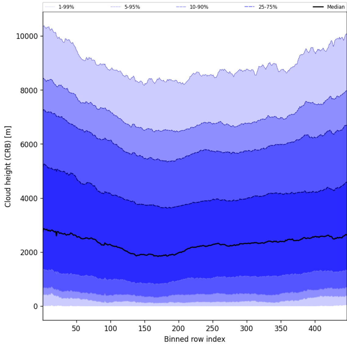
Figure 59: Along track statistics of “Cloud height (CRB)” for 2025-08-05 to 2025-08-07
