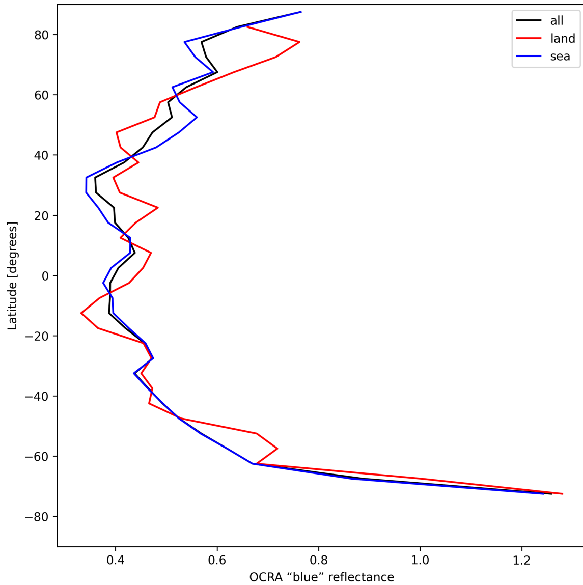
Figure 35: Zonal average of “OCRA “blue” reflectance” for 2025-08-05 to 2025-08-07.
