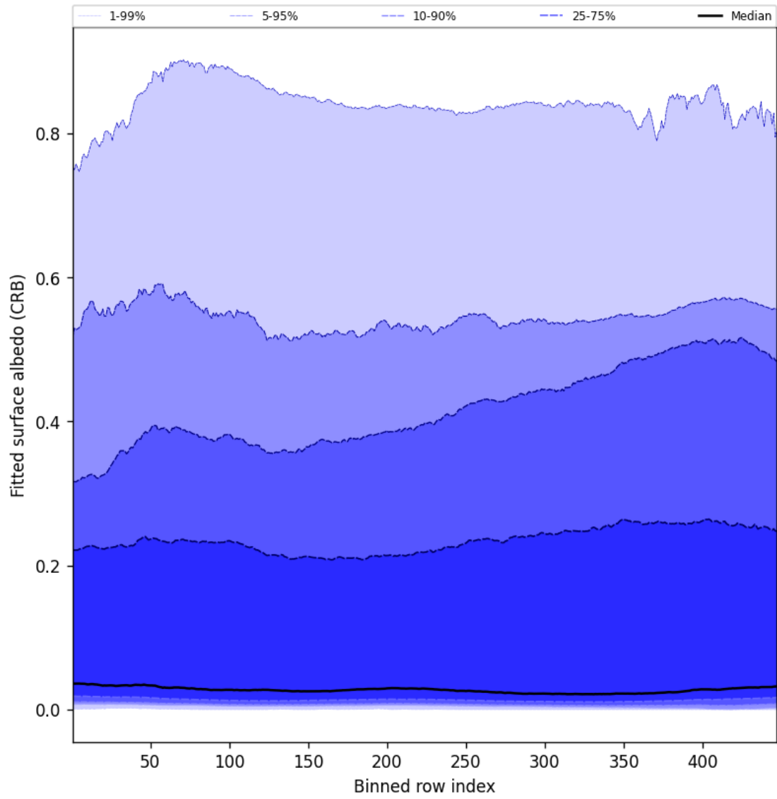
Figure 62: Along track statistics of “Fitted surface albedo (CRB)” for 2025-08-05 to 2025-08-07
