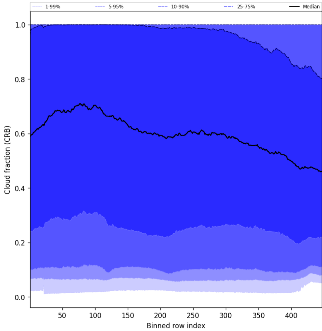
Figure 58: Along track statistics of “Cloud fraction (CRB)” for 2025-08-05 to 2025-08-07
