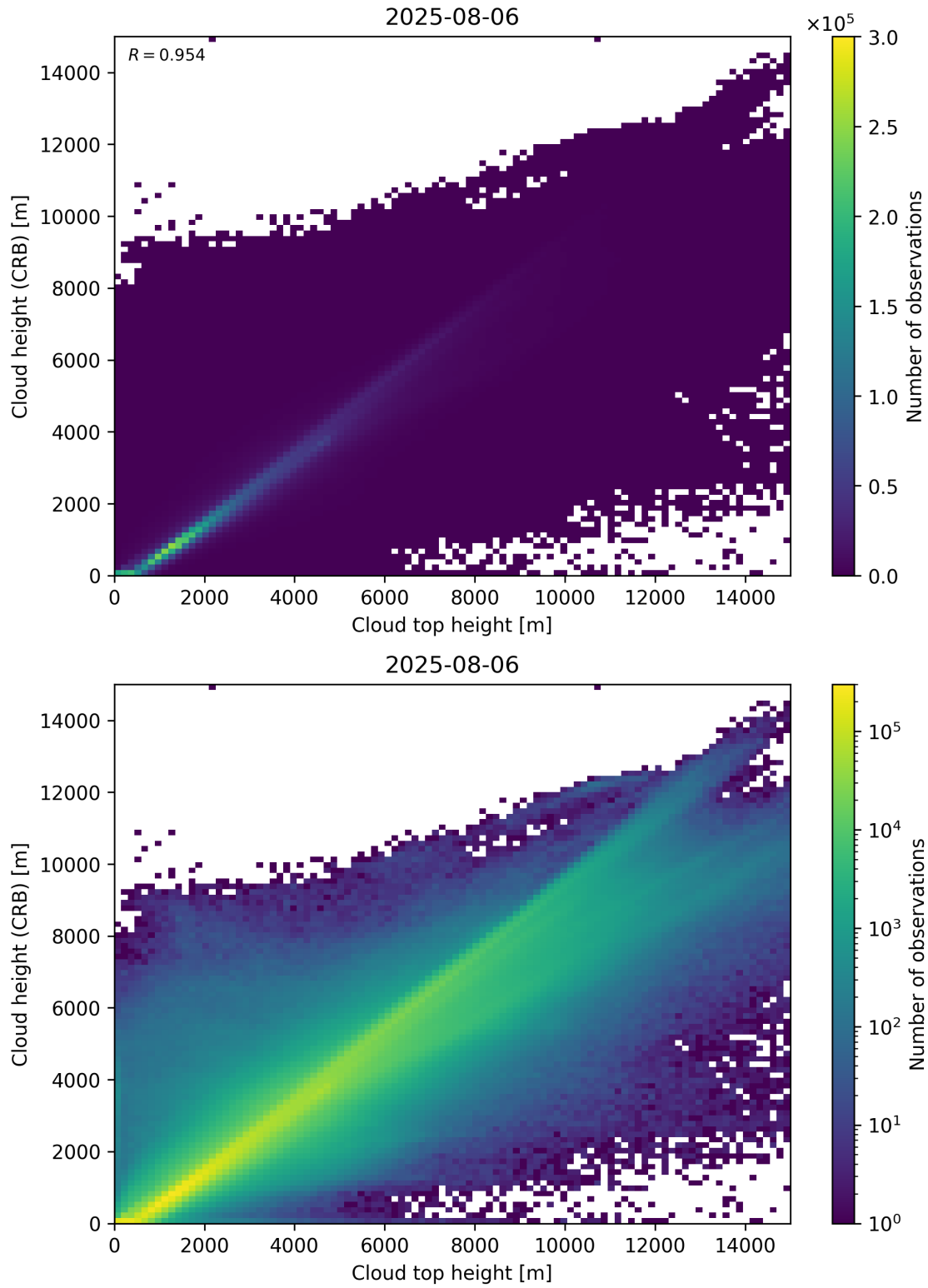
Figure 89: Scatter density plot of “Cloud top height” against “Cloud height (CRB)” for 2025-08-05 to 2025-08-07.
