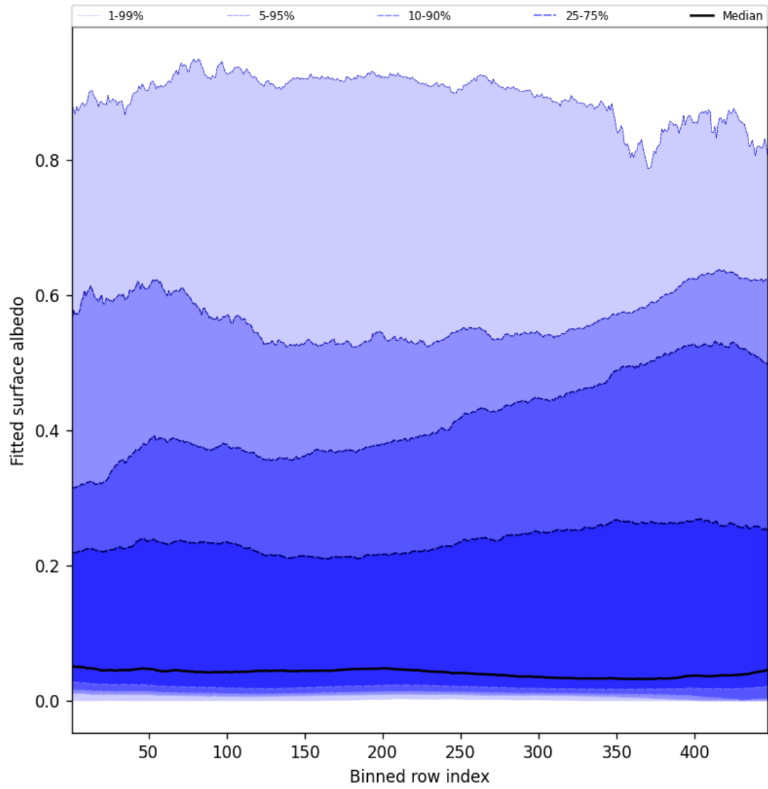
Figure 61: Along track statistics of “Fitted surface albedo” for 2025-08-05 to 2025-08-07
