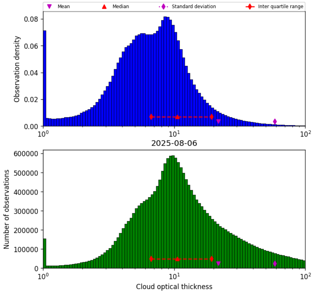
Figure 41: Histogram of “Cloud optical thickness” for 2025-08-05 to 2025-08-07
