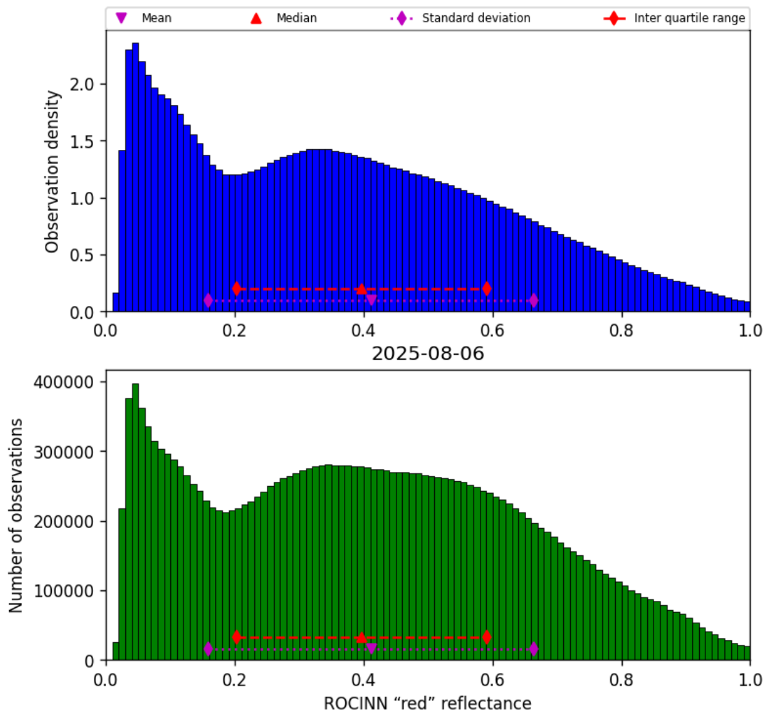
Figure 53: Histogram of “ROCINN “red” reflectance” for 2025-08-05 to 2025-08-07
