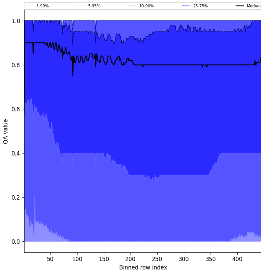
Figure 54: Along track statistics of “QA value” for 2025-08-05 to 2025-08-07
