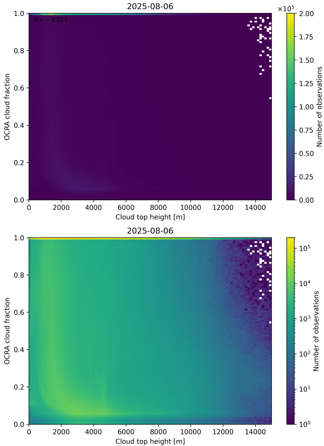
Figure 87: Scatter density plot of “Cloud top height” against “OCRA cloud fraction” for 2025-08-05 to 2025-08-07.
