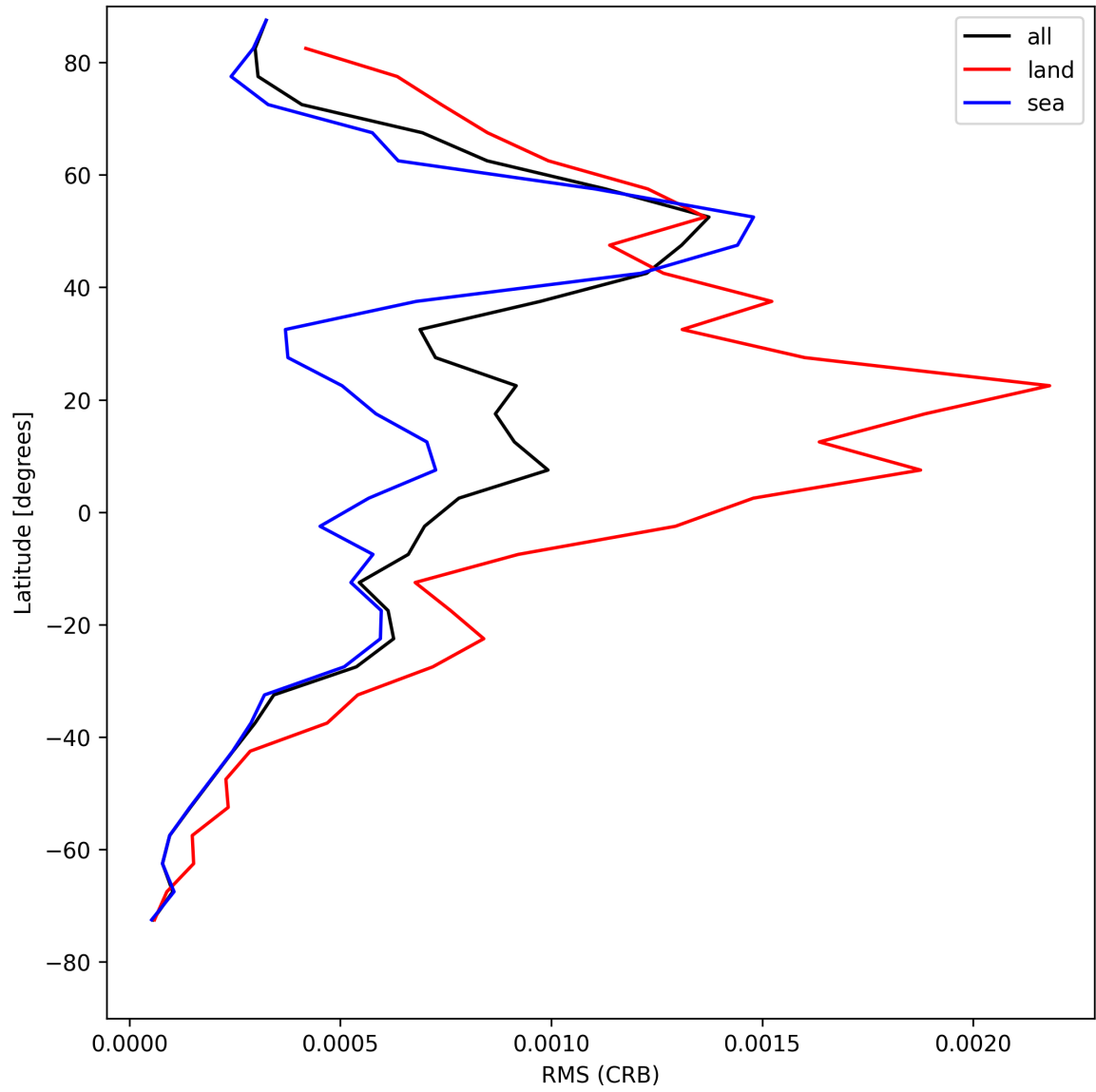
Figure 32: Zonal average of “RMS (CRB)” for 2025-08-05 to 2025-08-07.
