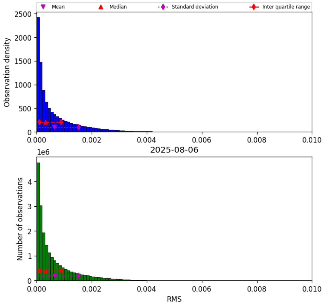
Figure 47: Histogram of “RMS” for 2025-08-05 to 2025-08-07
