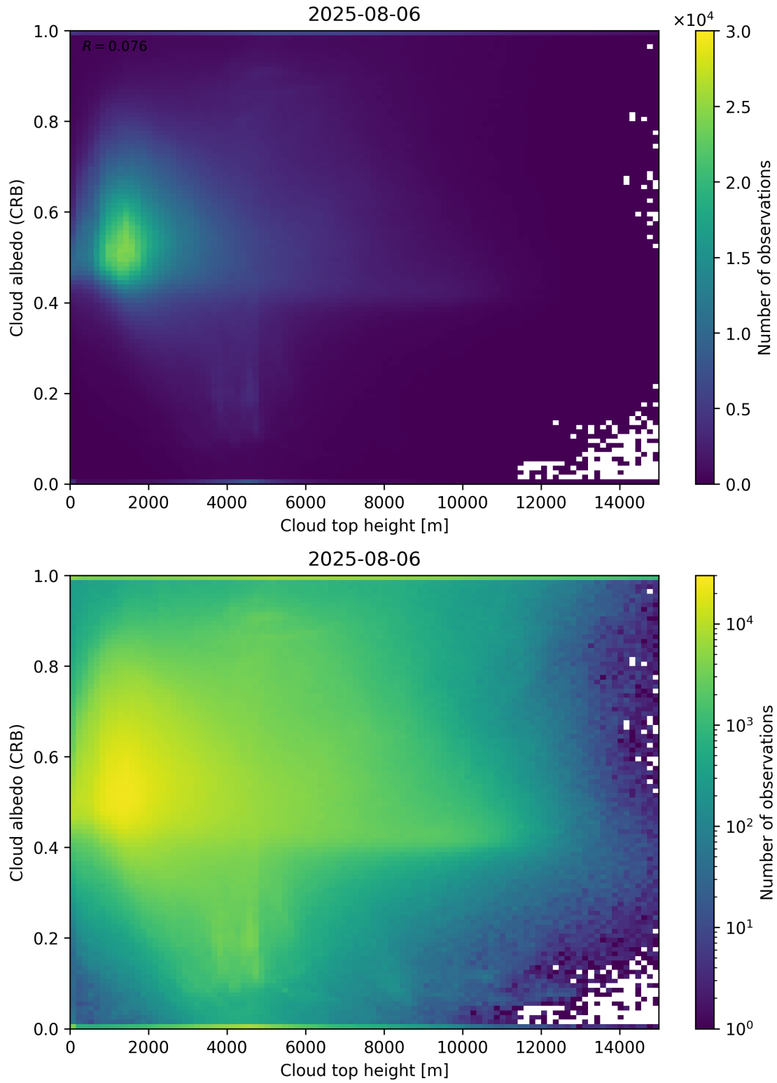
Figure 86: Scatter density plot of “Cloud top height” against “Cloud albedo (CRB)” for 2025-08-05 to 2025-08-07.
