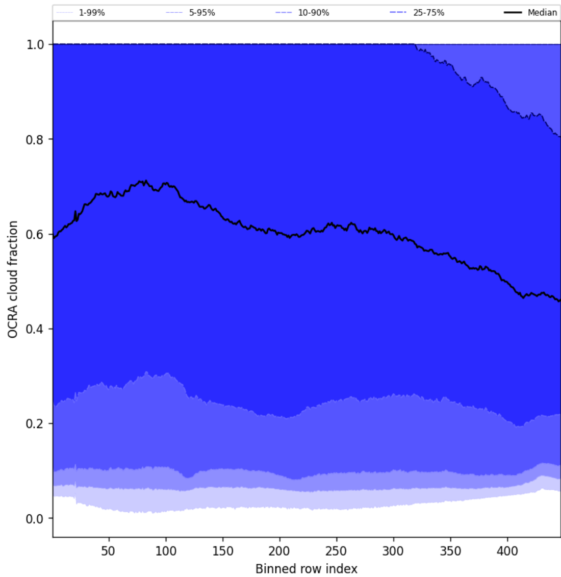
Figure 66: Along track statistics of “OCRA cloud fraction” for 2025-08-05 to 2025-08-07
