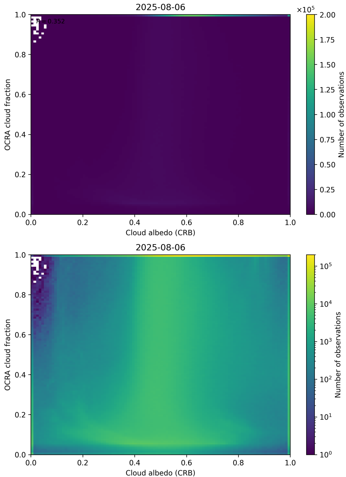
Figure 70: Scatter density plot of “Cloud albedo (CRB)” against “OCRA cloud fraction” for 2025-08-05 to 2025-08-07.
