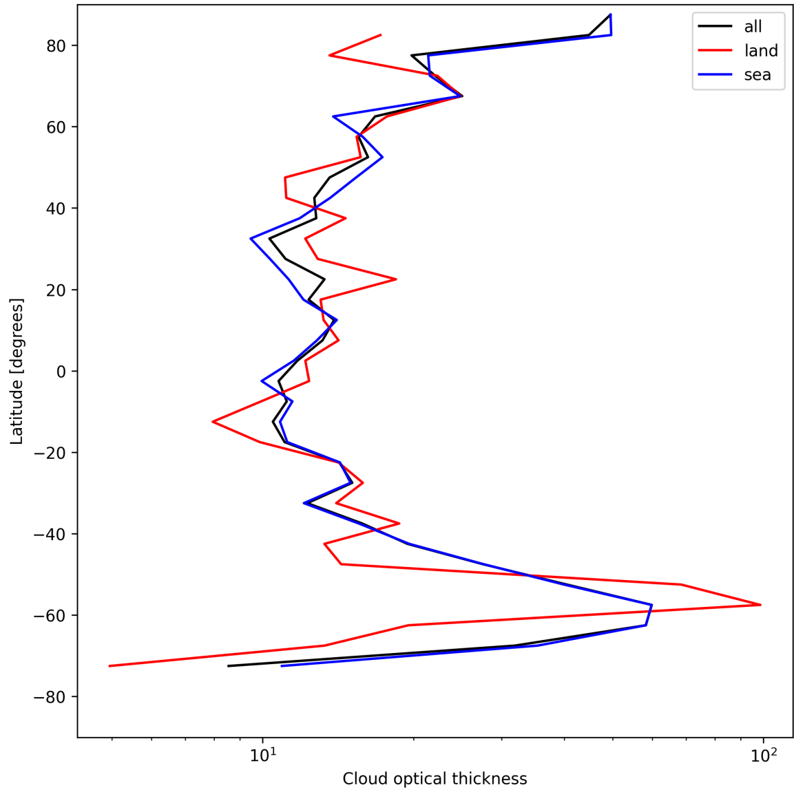
Figure 25: Zonal average of “Cloud optical thickness” for 2025-08-05 to 2025-08-07.
