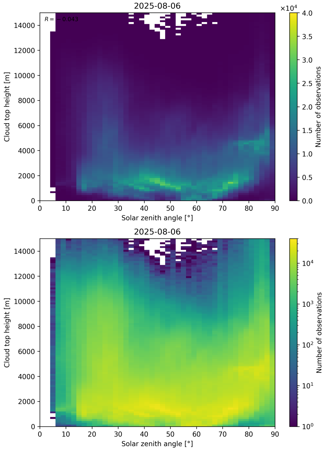
Figure 104: Scatter density plot of “Solar zenith angle” against “Cloud top height” for 2025-08-05 to 2025-08-07.
