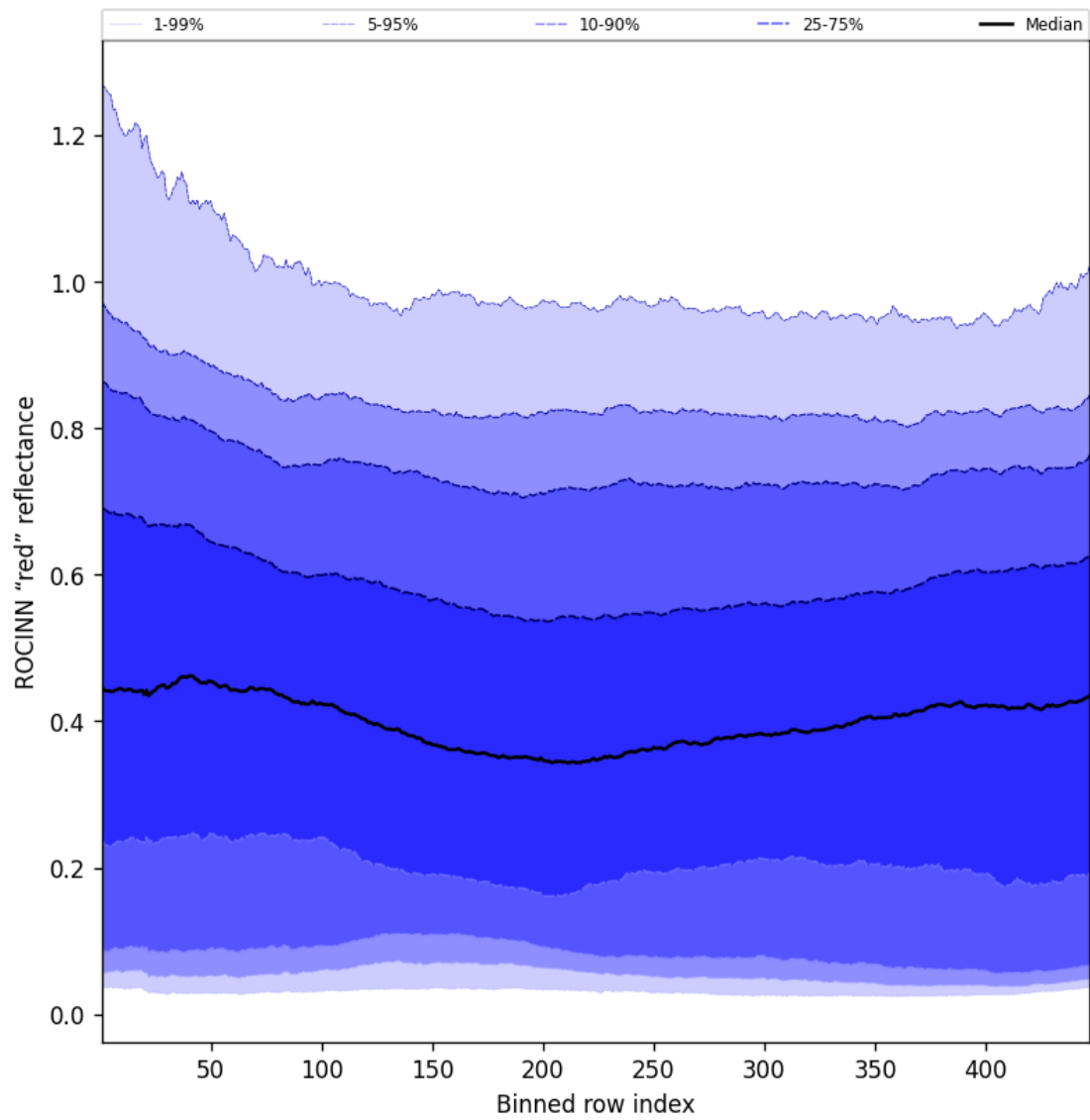
Figure 69: Along track statistics of “ROCINN “red” reflectance” for 2025-08-05 to 2025-08-07
