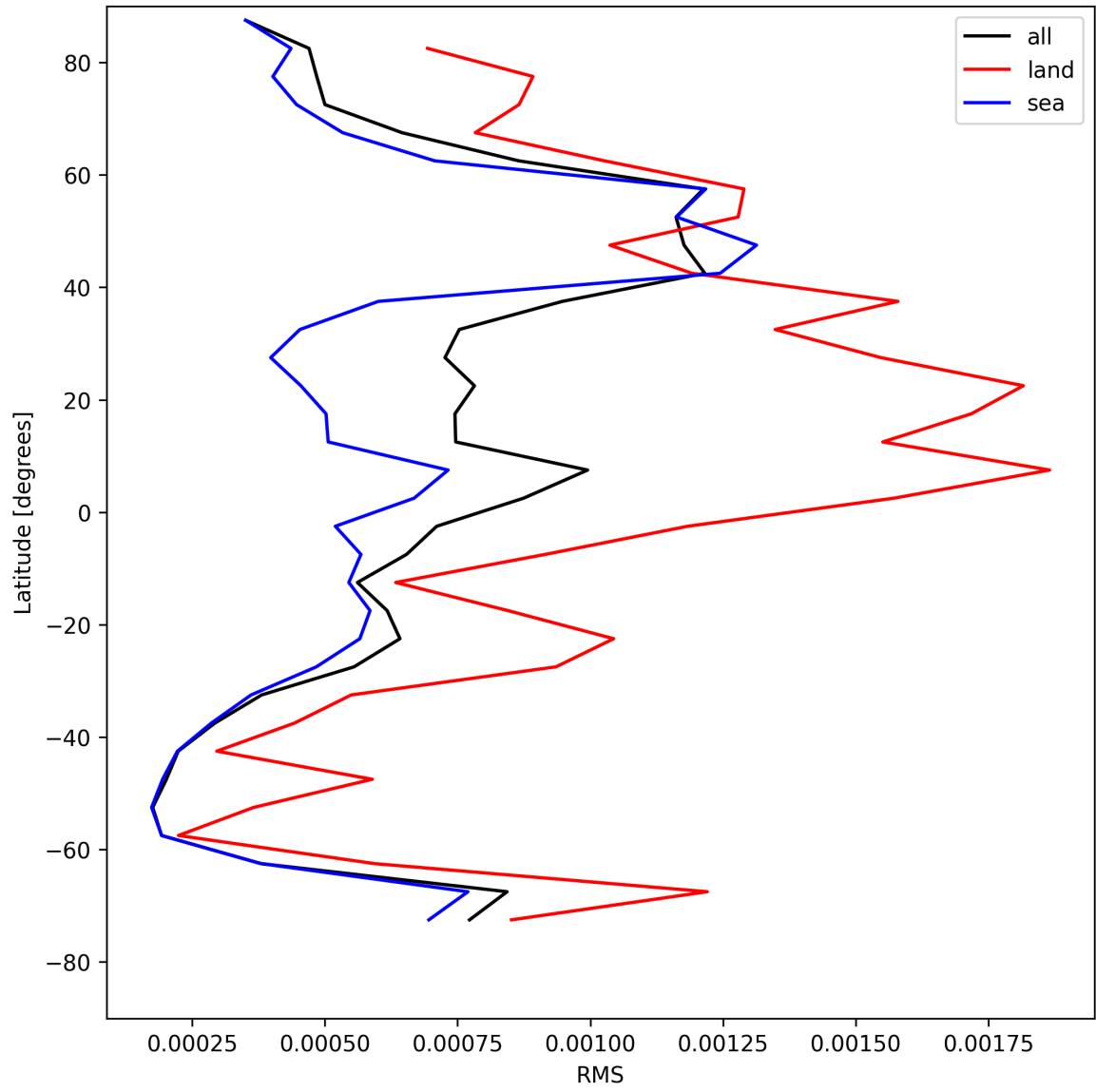
Figure 31: Zonal average of “RMS” for 2025-08-06 to 2025-08-08.
