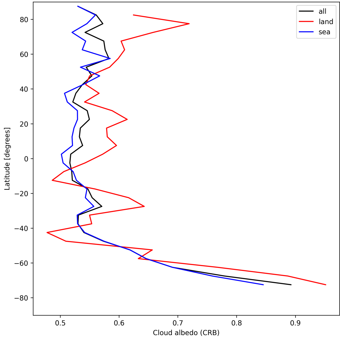
Figure 28: Zonal average of “Cloud albedo (CRB)” for 2025-08-06 to 2025-08-08.
