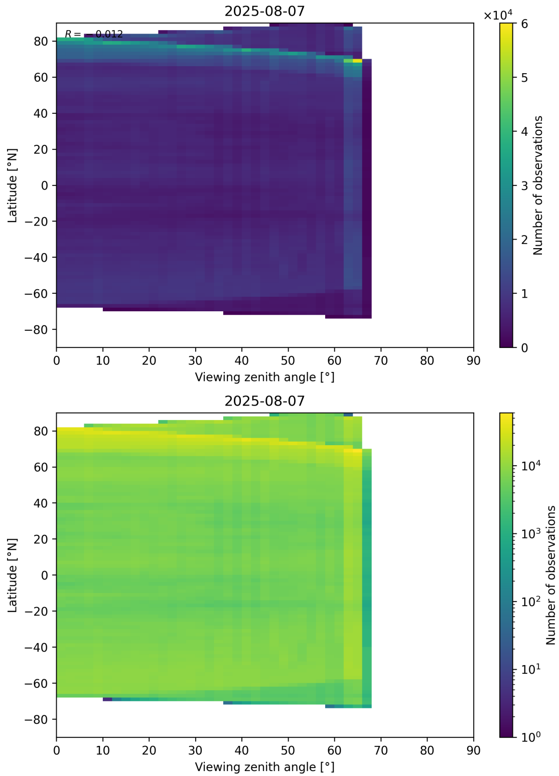
Figure 113: Scatter density plot of “Viewing zenith angle” against “Latitude” for 2025-08-06 to 2025-08-08.
