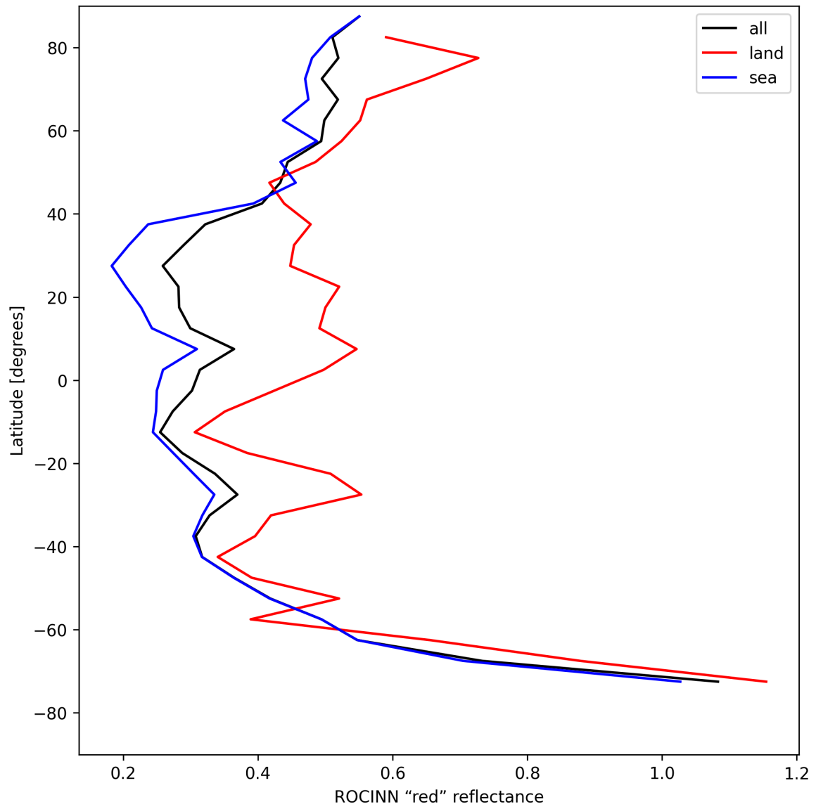
Figure 37: Zonal average of “ROCINN “red” reflectance” for 2025-08-06 to 2025-08-08.
