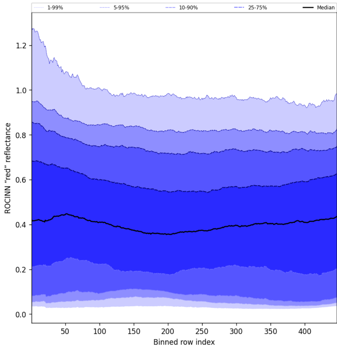
Figure 69: Along track statistics of “ROCINN “red” reflectance” for 2025-08-06 to 2025-08-08
