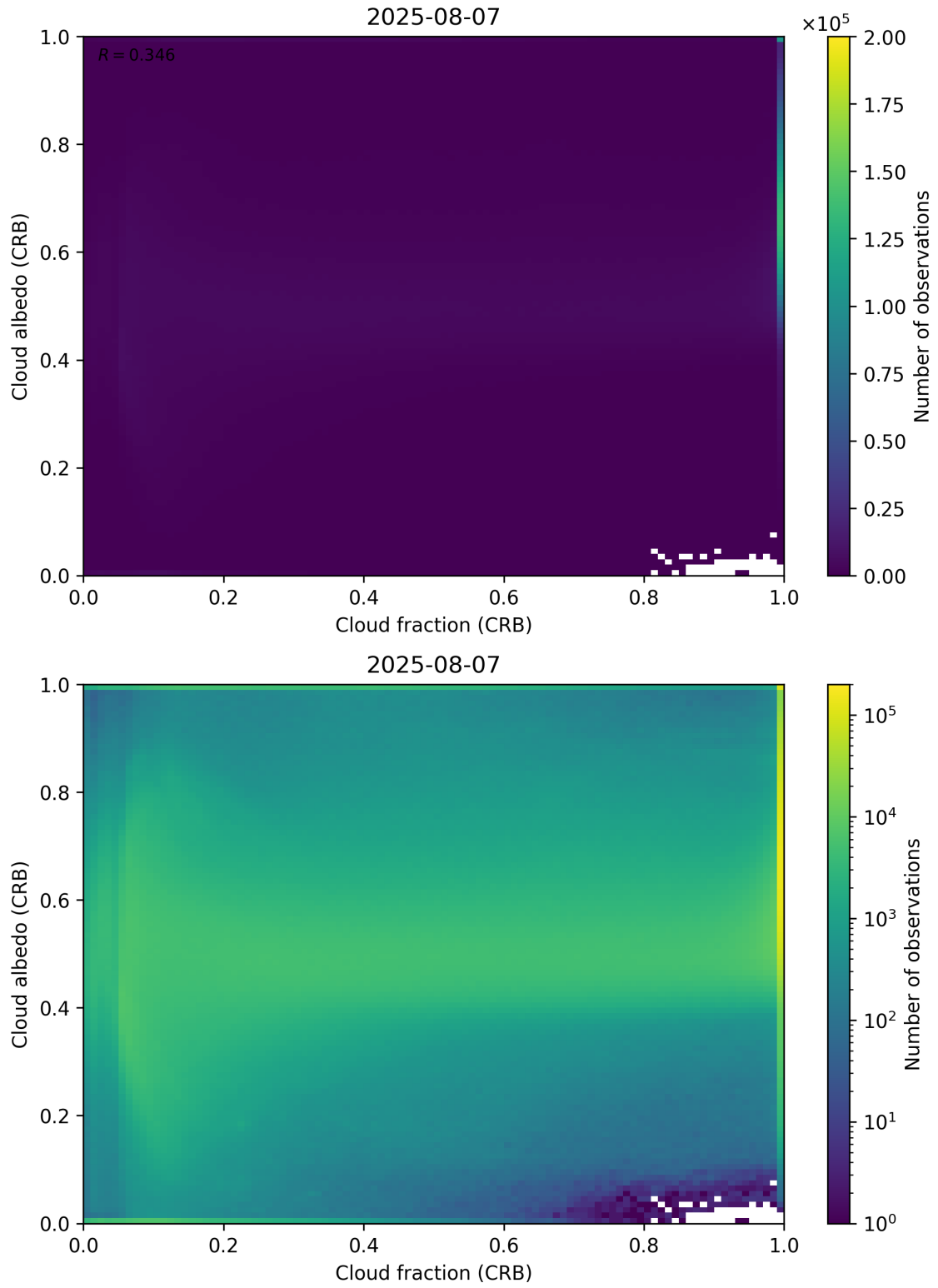
Figure 77: Scatter density plot of “Cloud fraction (CRB)” against “Cloud albedo (CRB)” for 2025-08-06 to 2025-08-08.
