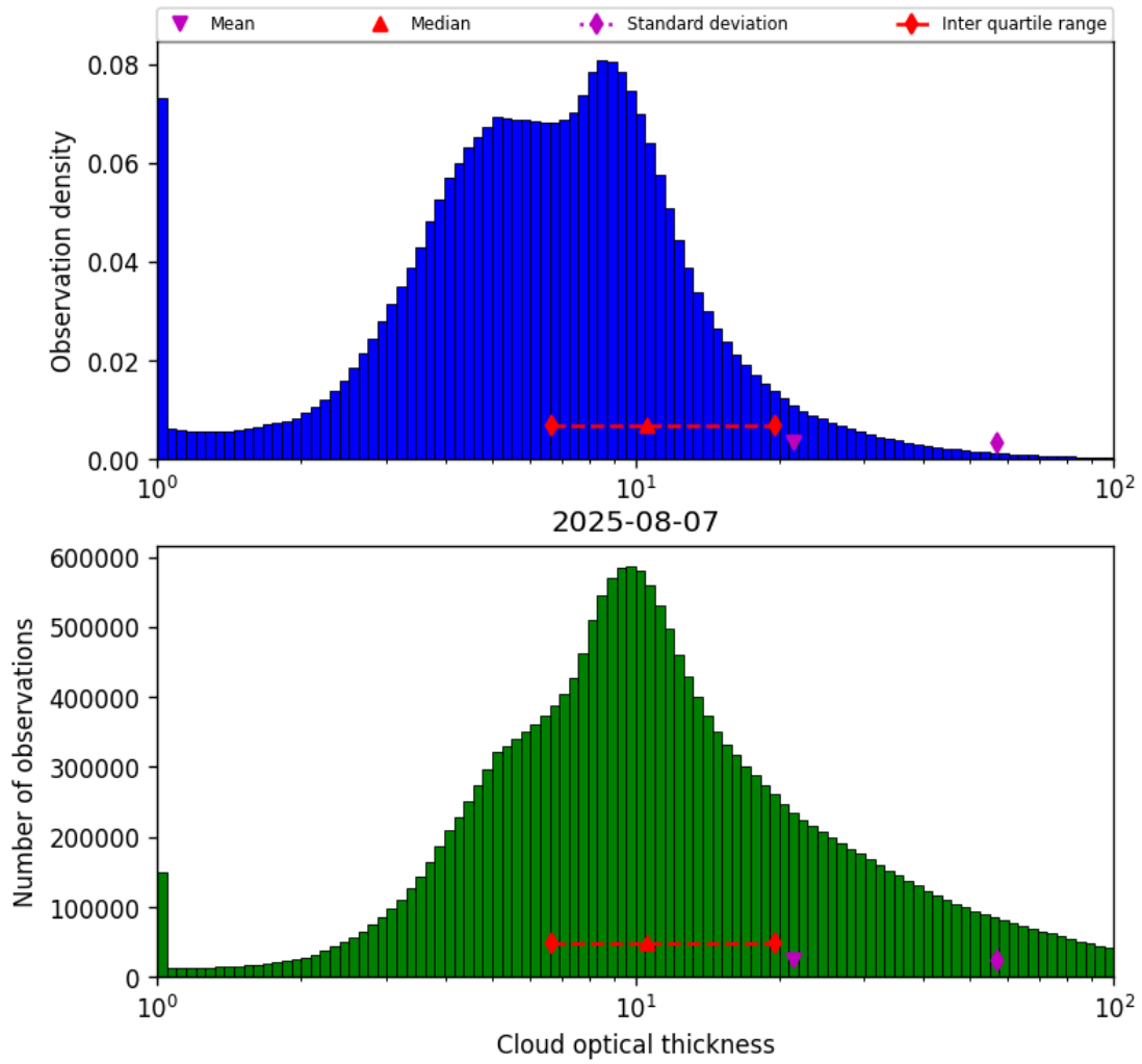
Figure 41: Histogram of “Cloud optical thickness” for 2025-08-06 to 2025-08-08
