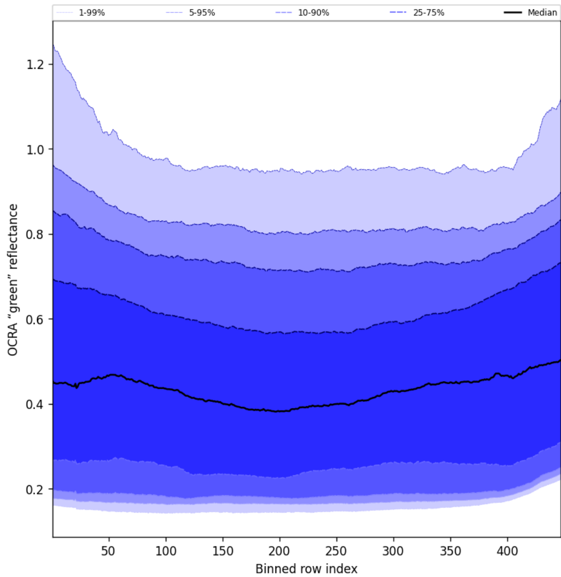
Figure 68: Along track statistics of “OCRA “green” reflectance” for 2025-08-06 to 2025-08-08
