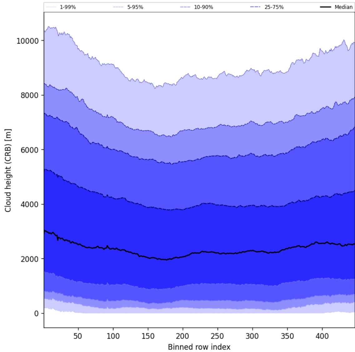
Figure 59: Along track statistics of “Cloud height (CRB)” for 2025-08-06 to 2025-08-08
