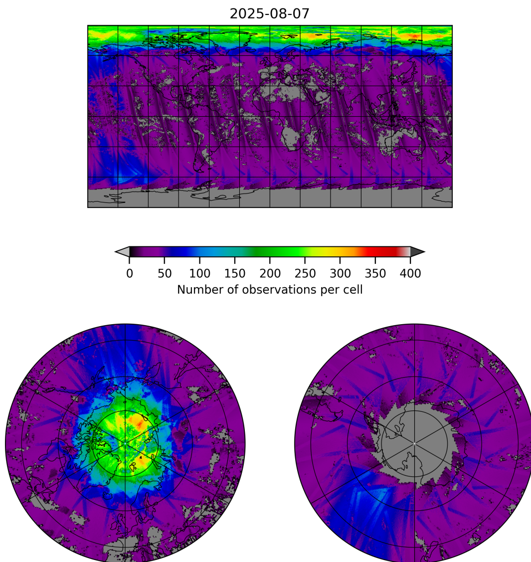
Figure 21: Map of the number of observations for 2025-08-06 to 2025-08-08
