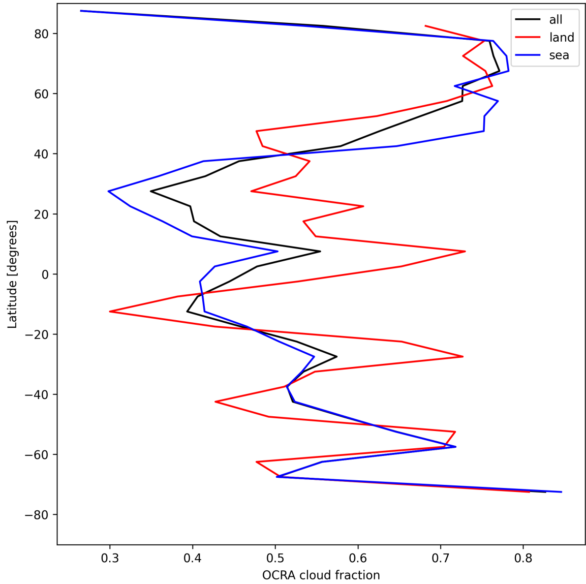
Figure 34: Zonal average of “OCRA cloud fraction” for 2025-08-06 to 2025-08-08.
