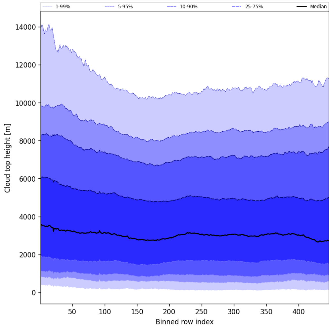
Figure 56: Along track statistics of “Cloud top height” for 2025-08-06 to 2025-08-08
