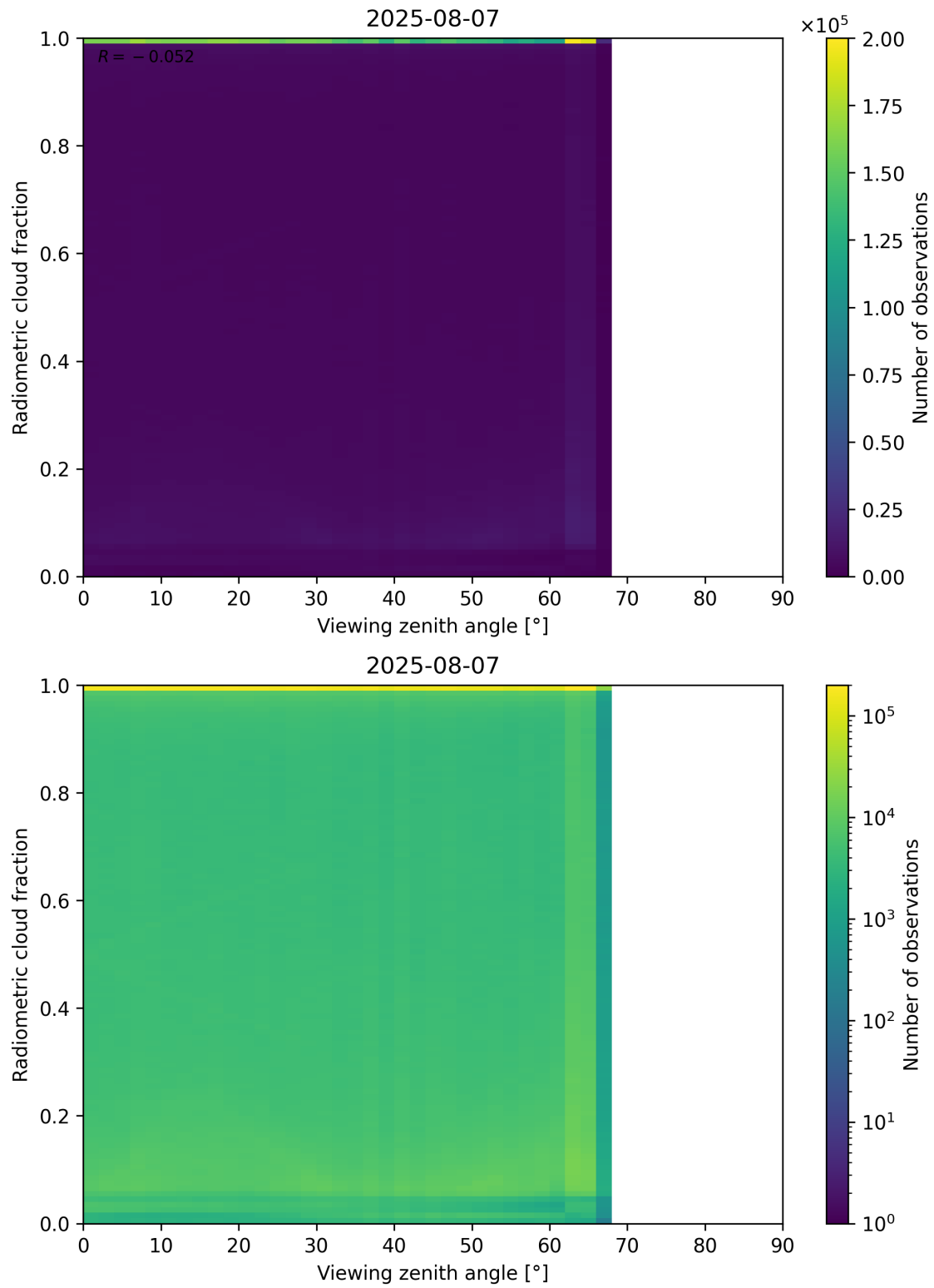
Figure 107: Scatter density plot of “Viewing zenith angle” against “Radiometric cloud fraction” for 2025-08-06 to 2025-08-08.
