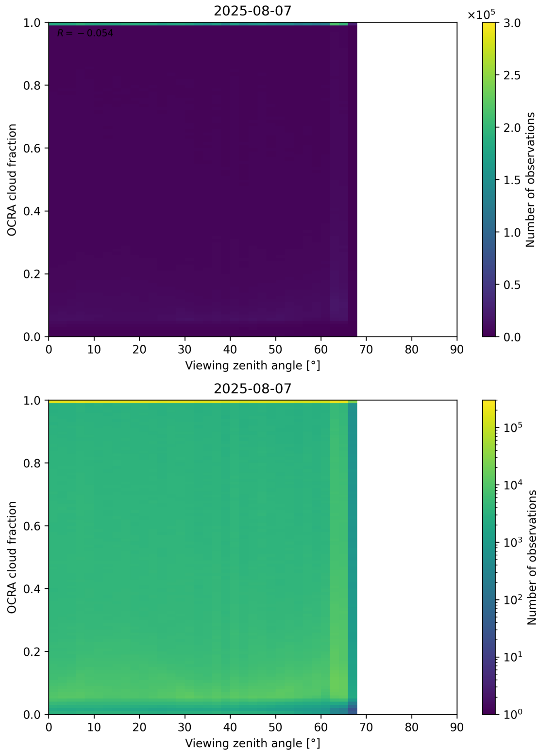
Figure 108: Scatter density plot of “Viewing zenith angle” against “OCRA cloud fraction” for 2025-08-06 to 2025-08-08.
