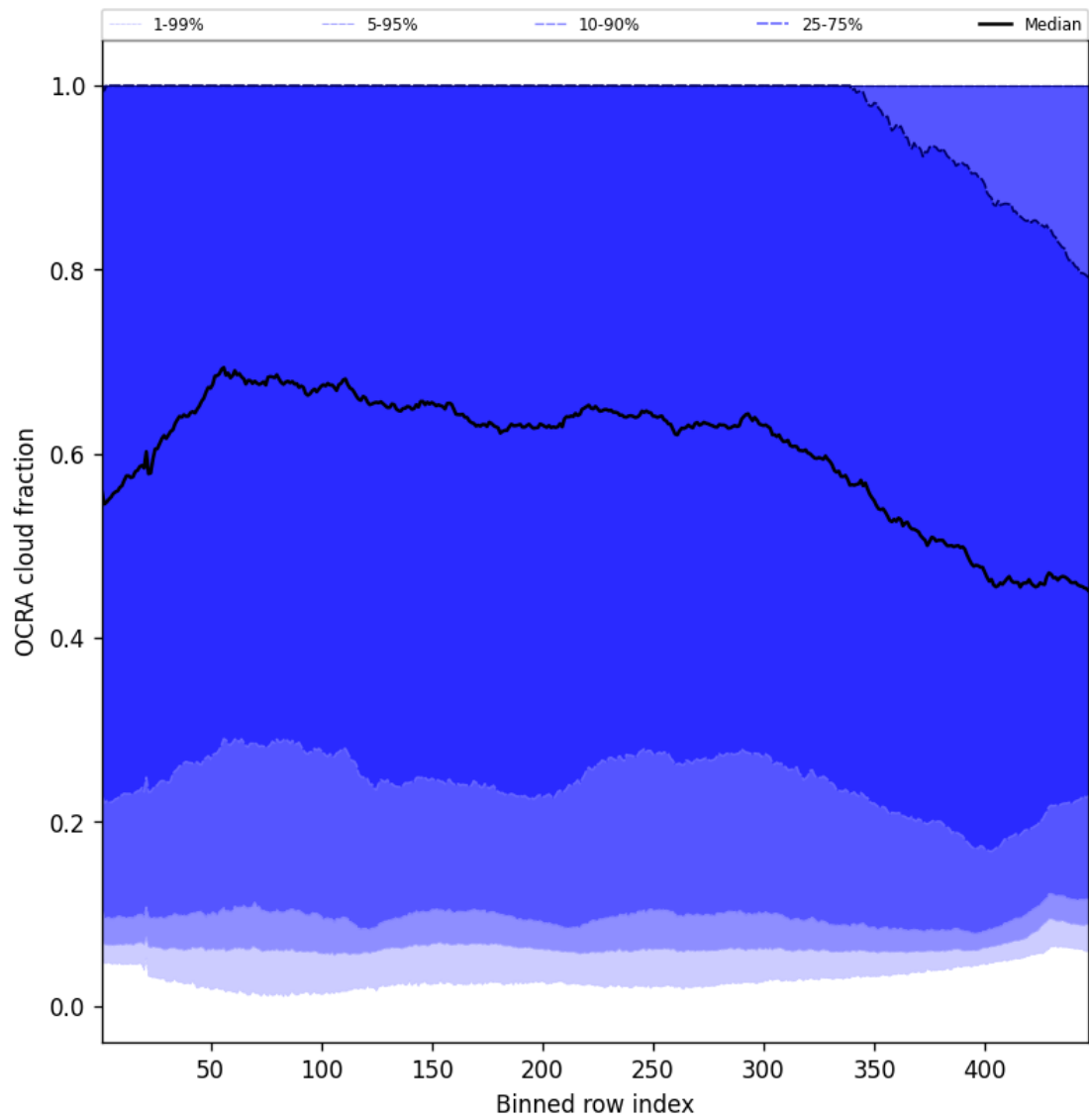
Figure 66: Along track statistics of “OCRA cloud fraction” for 2025-08-06 to 2025-08-08
