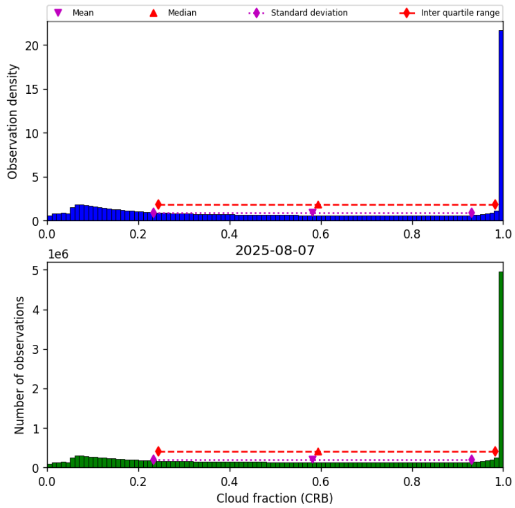
Figure 42: Histogram of “Cloud fraction (CRB)” for 2025-08-06 to 2025-08-08
