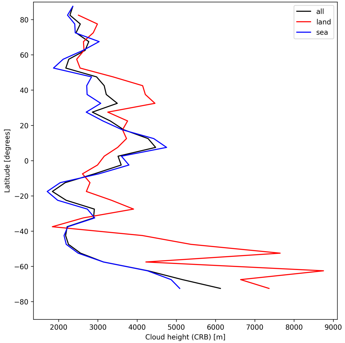
Figure 27: Zonal average of “Cloud height (CRB)” for 2025-08-06 to 2025-08-08.
