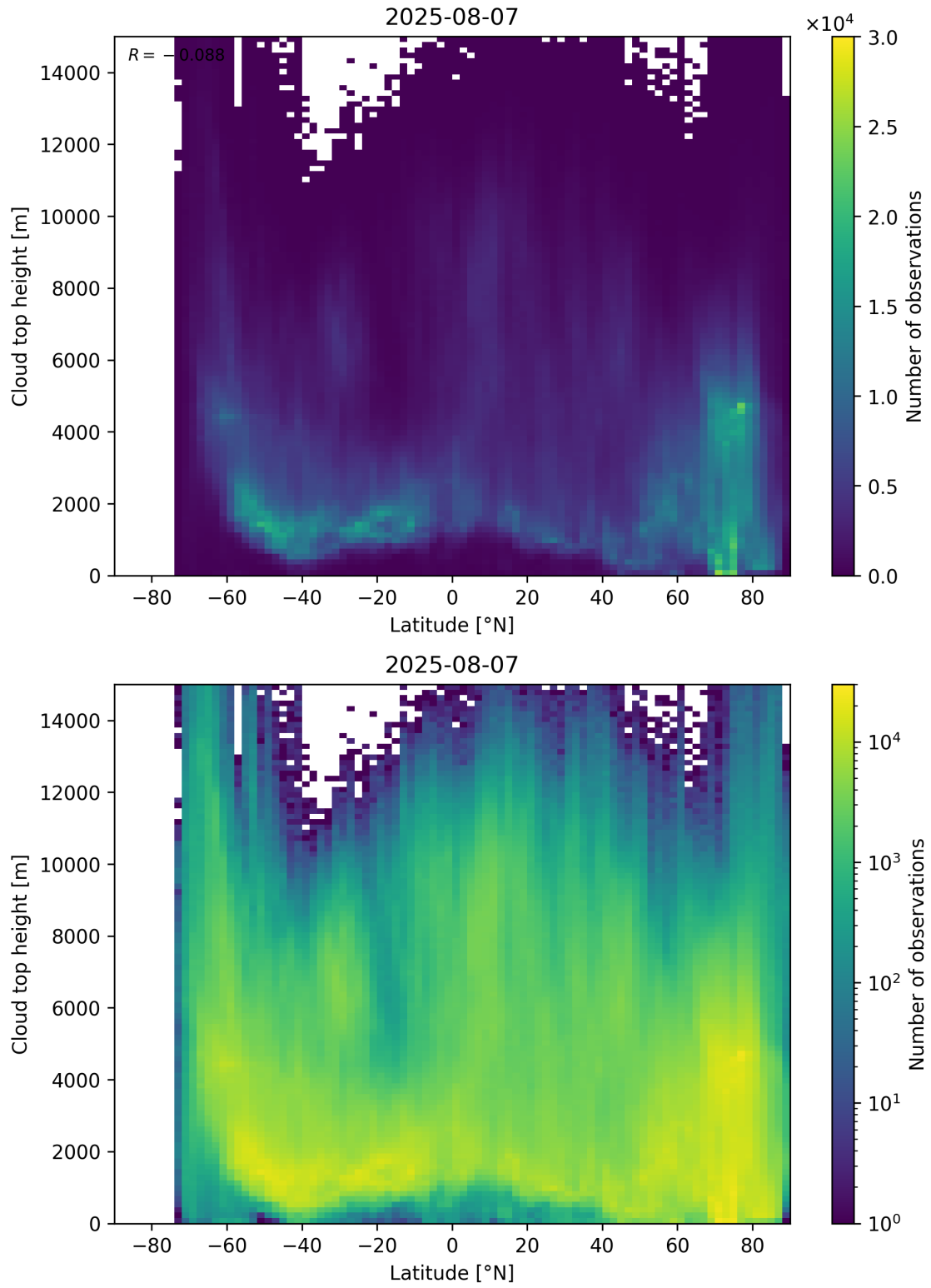
Figure 97: Scatter density plot of “Latitude” against “Cloud top height” for 2025-08-06 to 2025-08-08.
