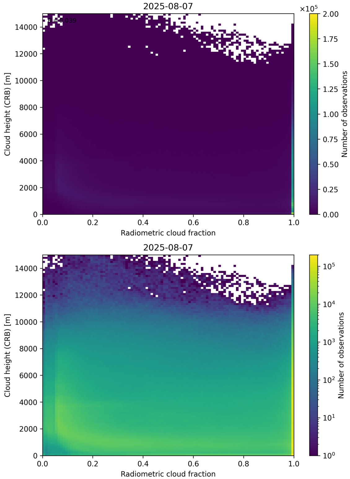
Figure 74: Scatter density plot of “Radiometric cloud fraction” against “Cloud height (CRB)” for 2025-08-06 to 2025-08-08.
