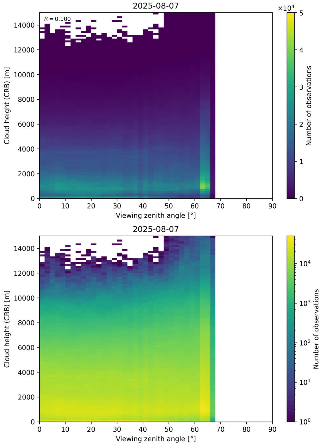
Figure 110: Scatter density plot of “Viewing zenith angle” against “Cloud height (CRB)” for 2025-08-06 to 2025-08-08.
