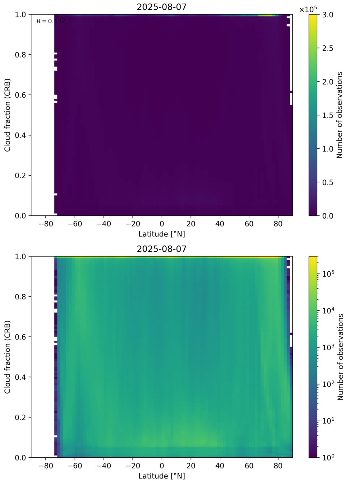
Figure 94: Scatter density plot of “Latitude” against “Cloud fraction (CRB)” for 2025-08-06 to 2025-08-08.
