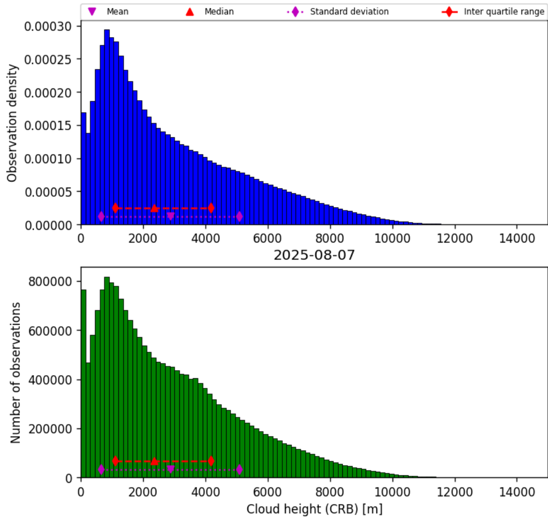
Figure 43: Histogram of “Cloud height (CRB)” for 2025-08-06 to 2025-08-08
