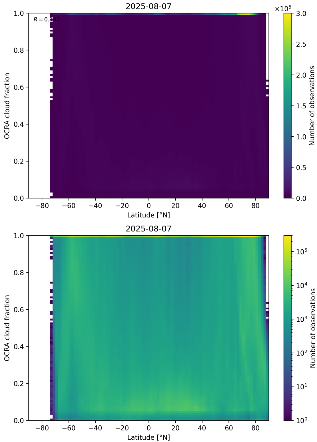
Figure 93: Scatter density plot of “Latitude” against “OCRA cloud fraction” for 2025-08-06 to 2025-08-08.
