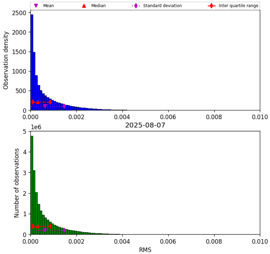
Figure 47: Histogram of “RMS” for 2025-08-06 to 2025-08-08
