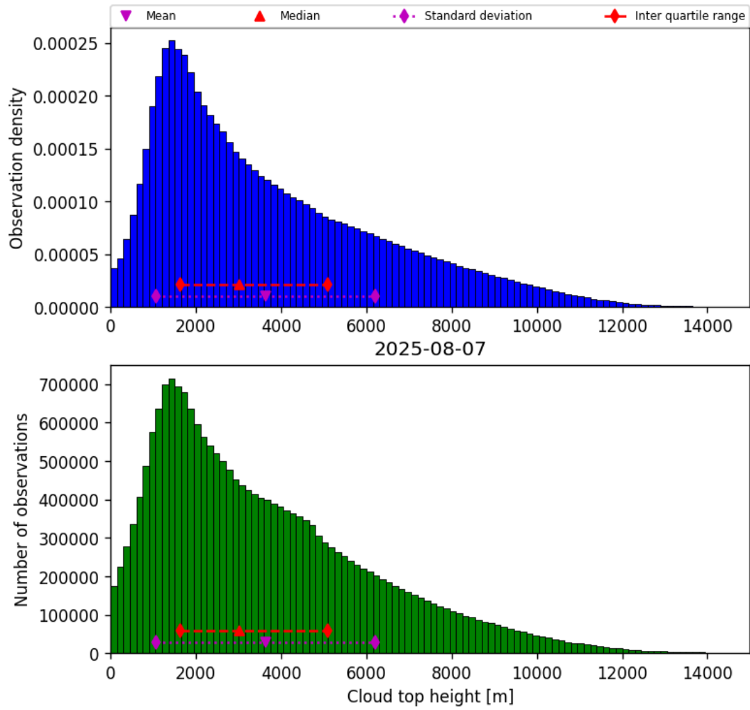
Figure 40: Histogram of “Cloud top height” for 2025-08-06 to 2025-08-08
