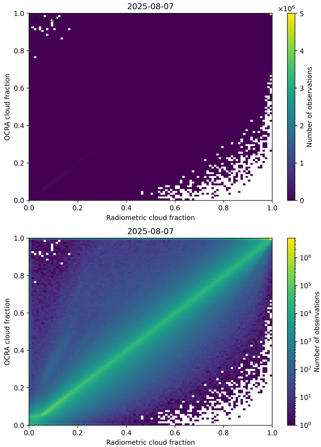
Figure 72: Scatter density plot of “Radiometric cloud fraction” against “OCRA cloud fraction” for 2025-08-06 to 2025-08-08.
