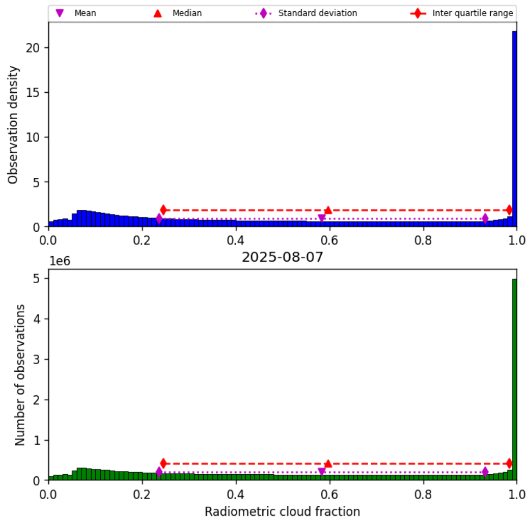
Figure 39: Histogram of “Radiometric cloud fraction” for 2025-08-06 to 2025-08-08
