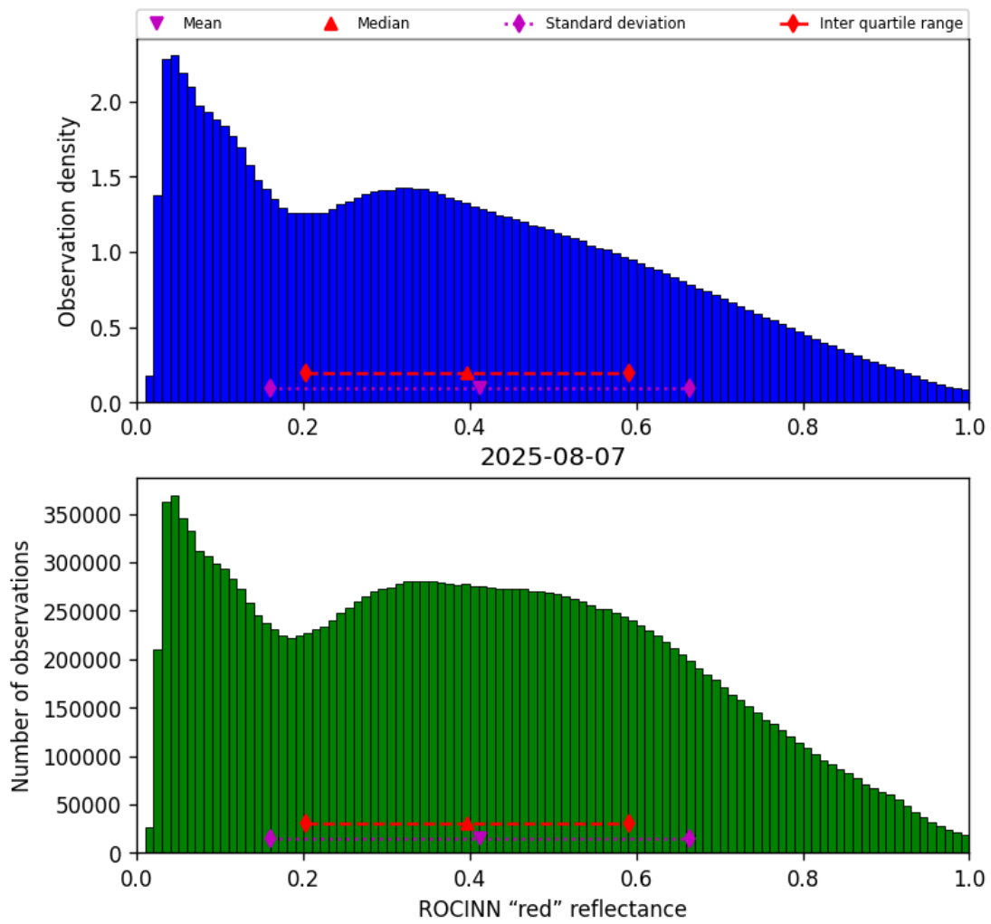
Figure 53: Histogram of “ROCINN “red” reflectance” for 2025-08-06 to 2025-08-08
