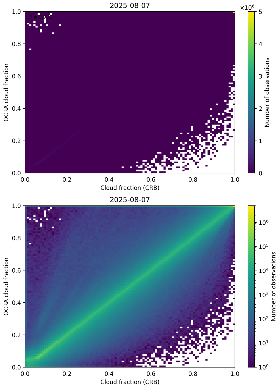
Figure 78: Scatter density plot of “Cloud fraction (CRB)” against “OCRA cloud fraction” for 2025-08-06 to 2025-08-08.
