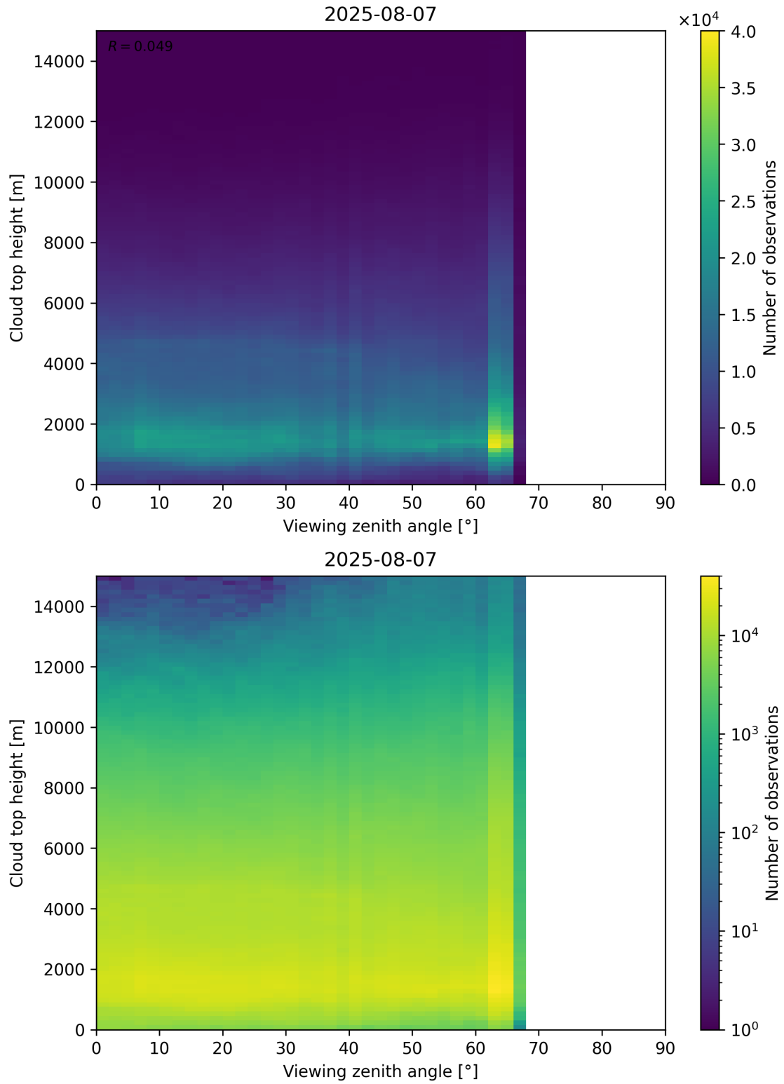
Figure 112: Scatter density plot of “Viewing zenith angle” against “Cloud top height” for 2025-08-06 to 2025-08-08.
