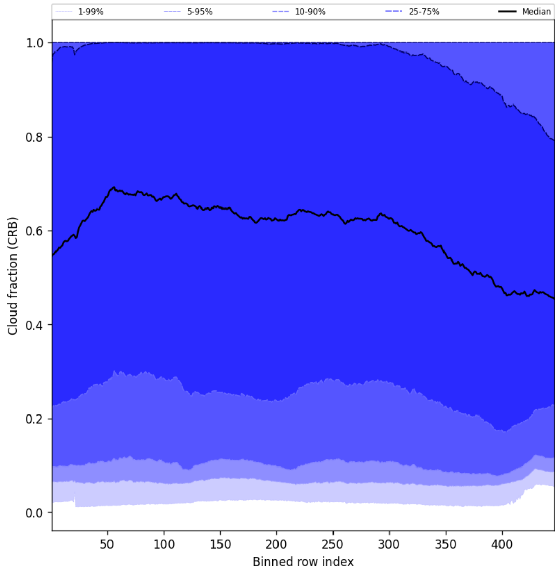
Figure 58: Along track statistics of “Cloud fraction (CRB)” for 2025-08-06 to 2025-08-08
