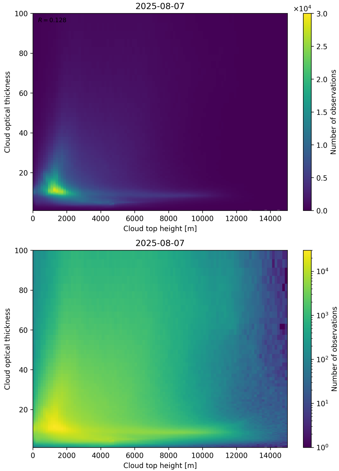
Figure 90: Scatter density plot of “Cloud top height” against “Cloud optical thickness” for 2025-08-06 to 2025-08-08.
