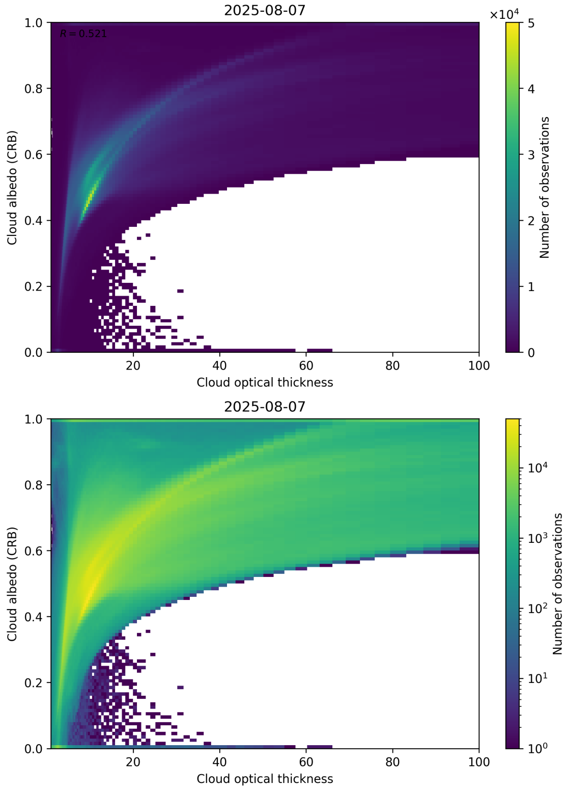
Figure 82: Scatter density plot of “Cloud optical thickness” against “Cloud albedo (CRB)” for 2025-08-06 to 2025-08-08.
