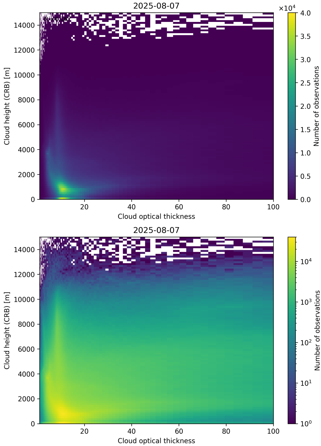
Figure 85: Scatter density plot of “Cloud optical thickness” against “Cloud height (CRB)” for 2025-08-06 to 2025-08-08.
