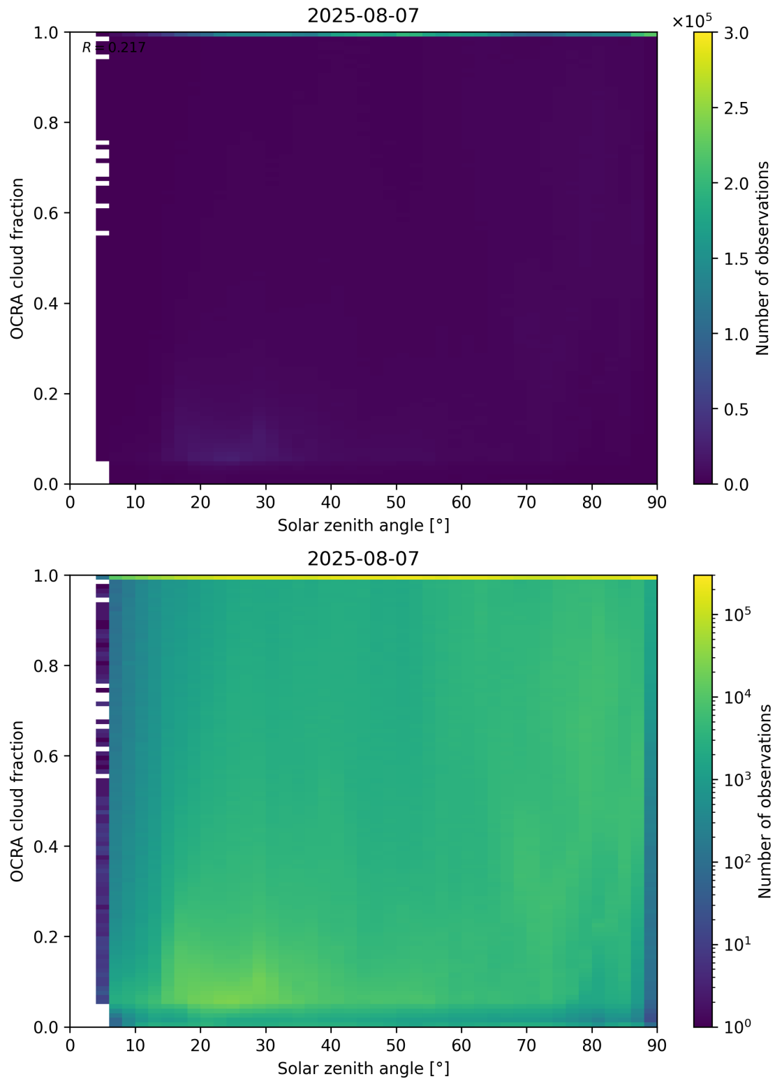
Figure 100: Scatter density plot of “Solar zenith angle” against “OCRA cloud fraction” for 2025-08-06 to 2025-08-08.
