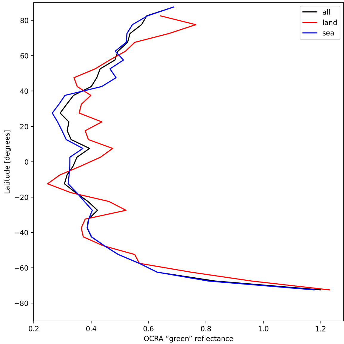
Figure 36: Zonal average of “OCRA “green” reflectance” for 2025-08-06 to 2025-08-08.
