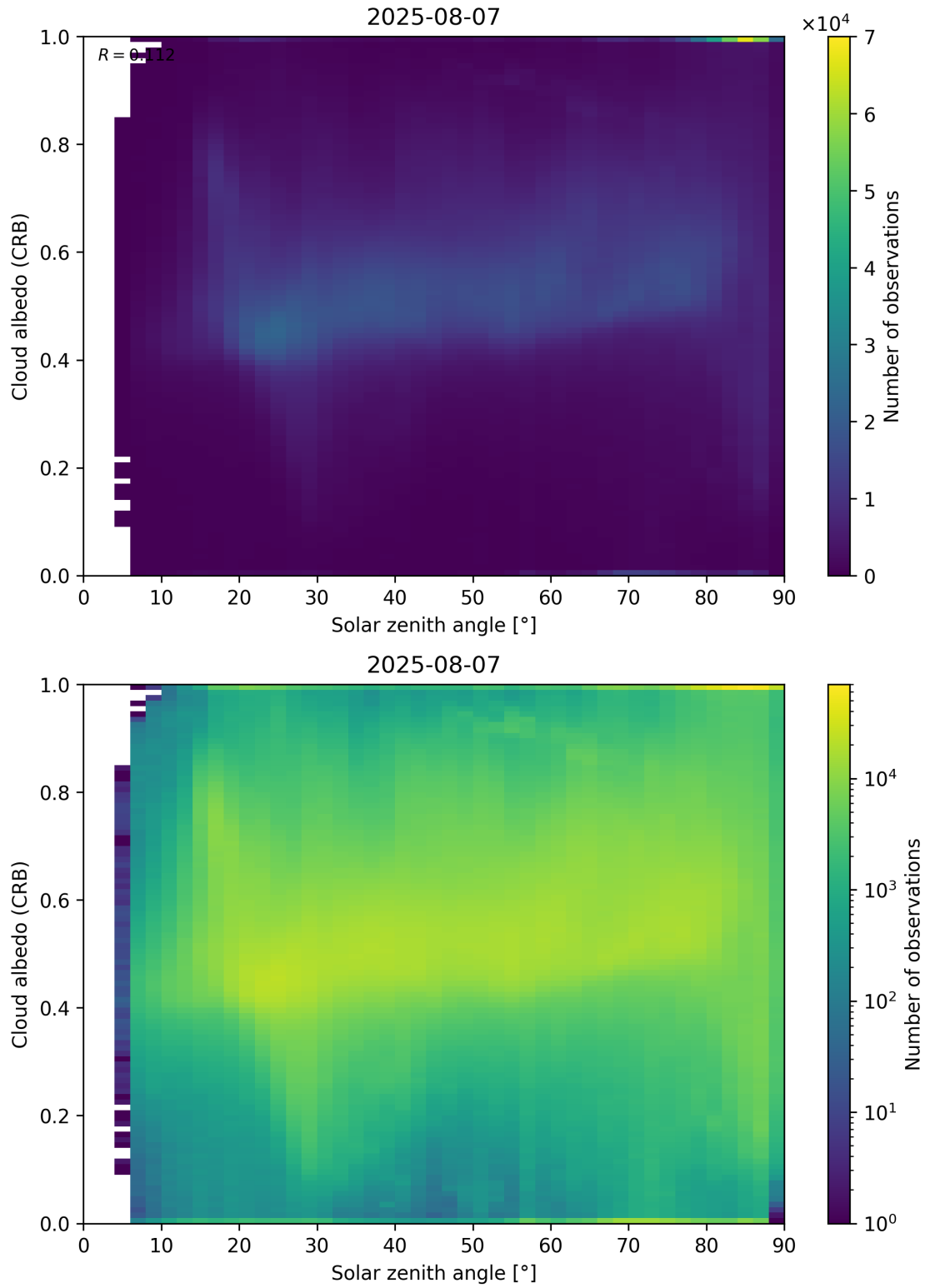
Figure 98: Scatter density plot of “Solar zenith angle” against “Cloud albedo (CRB)” for 2025-08-06 to 2025-08-08.
