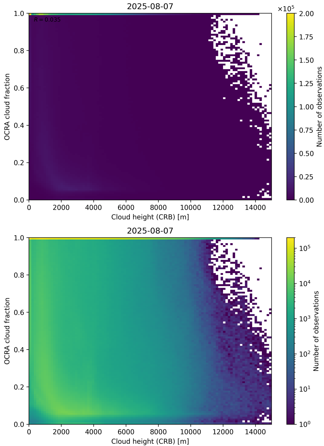
Figure 81: Scatter density plot of “Cloud height (CRB)” against “OCRA cloud fraction” for 2025-08-06 to 2025-08-08.
