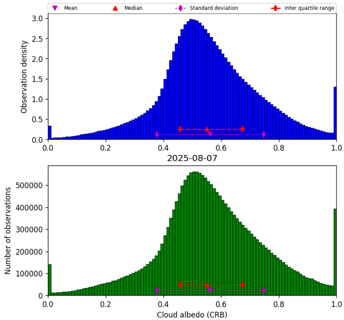
Figure 44: Histogram of “Cloud albedo (CRB)” for 2025-08-06 to 2025-08-08
