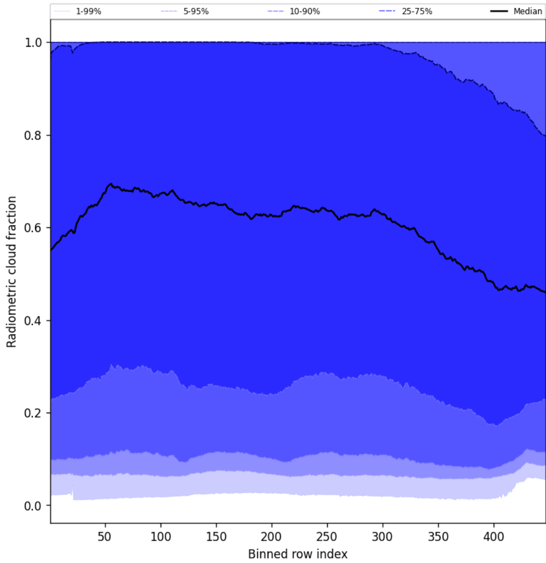
Figure 55: Along track statistics of “Radiometric cloud fraction” for 2025-08-06 to 2025-08-08
