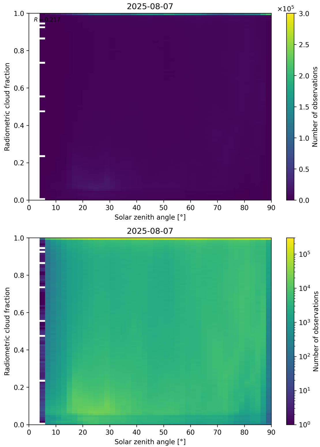
Figure 99: Scatter density plot of “Solar zenith angle” against “Radiometric cloud fraction” for 2025-08-06 to 2025-08-08.
