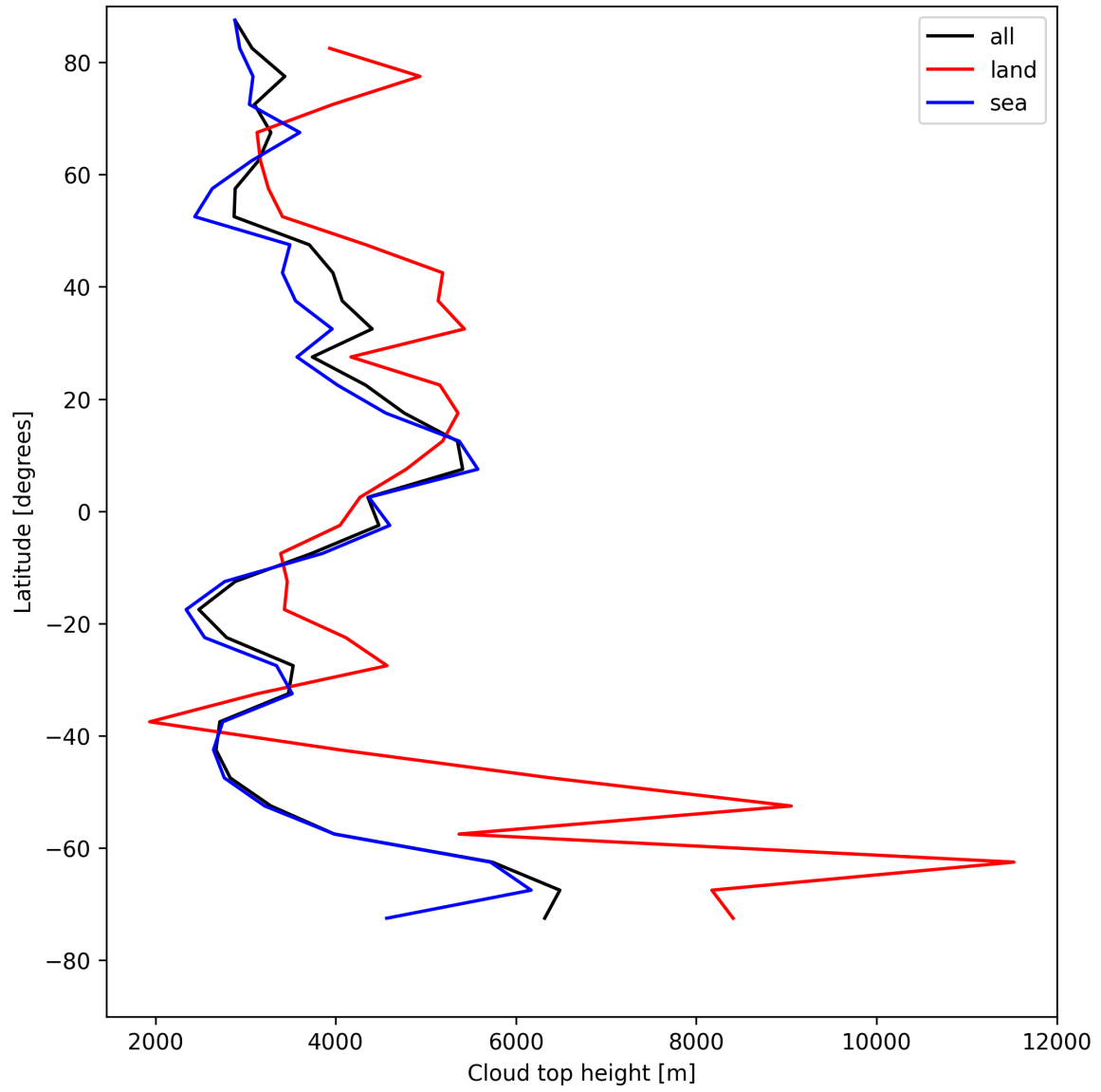
Figure 24: Zonal average of “Cloud top height” for 2025-08-06 to 2025-08-08.
