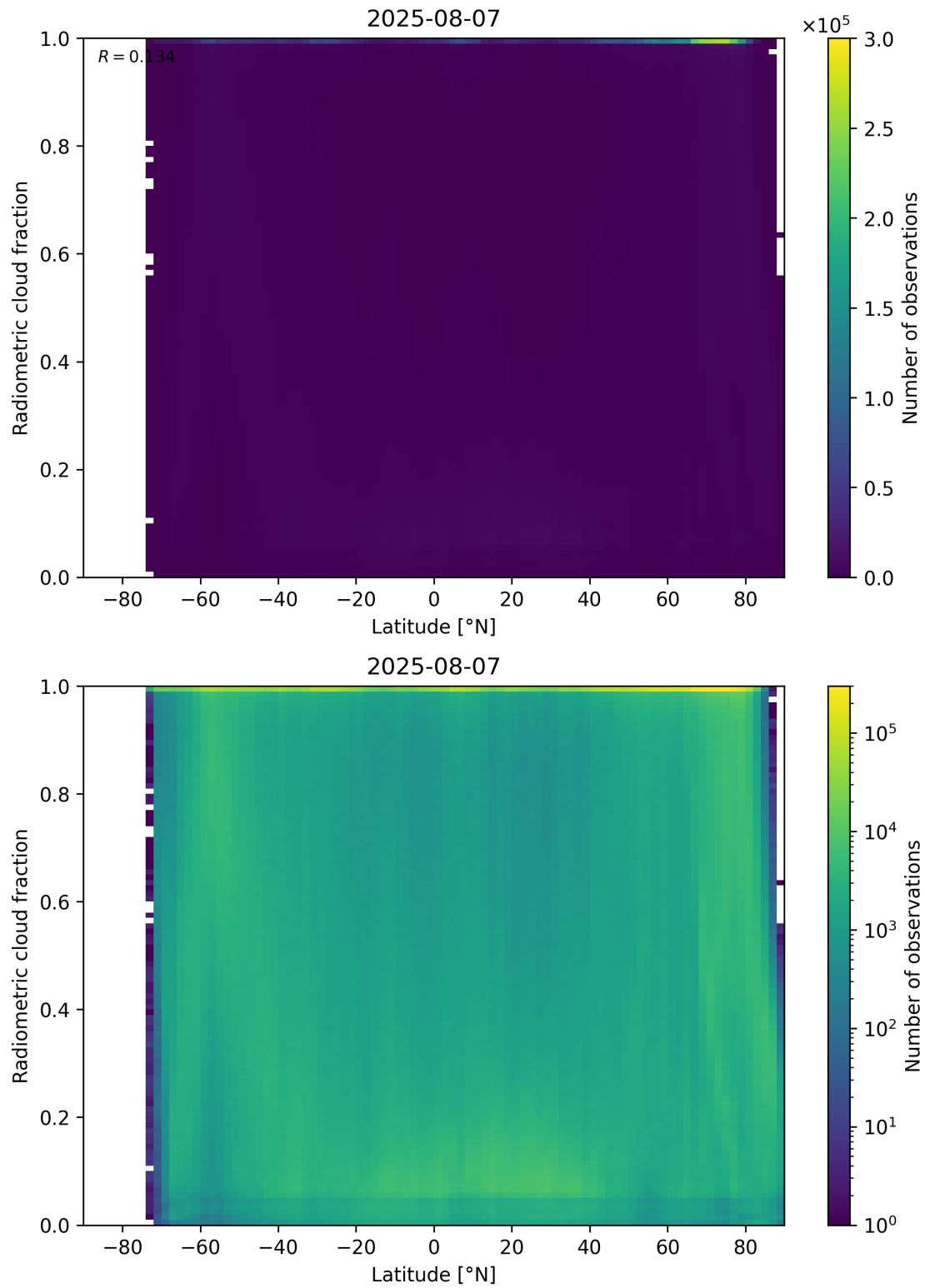
Figure 92: Scatter density plot of “Latitude” against “Radiometric cloud fraction” for 2025-08-06 to 2025-08-08.
