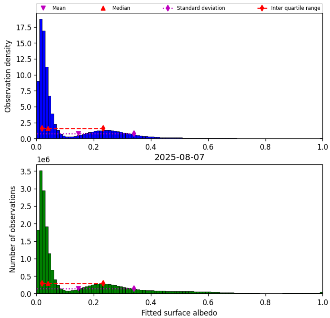
Figure 45: Histogram of “Fitted surface albedo” for 2025-08-06 to 2025-08-08
