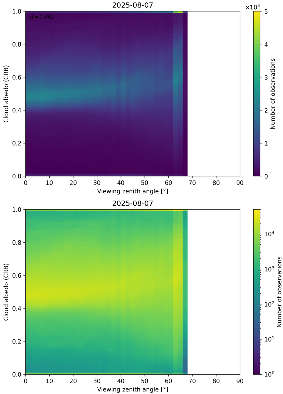
Figure 106: Scatter density plot of “Viewing zenith angle” against “Cloud albedo (CRB)” for 2025-08-06 to 2025-08-08.
