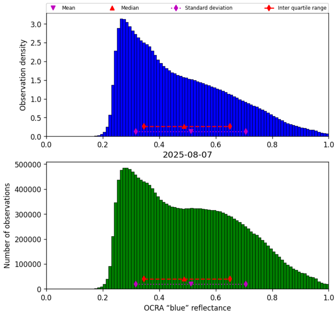
Figure 51: Histogram of “OCRA “blue” reflectance” for 2025-08-06 to 2025-08-08
