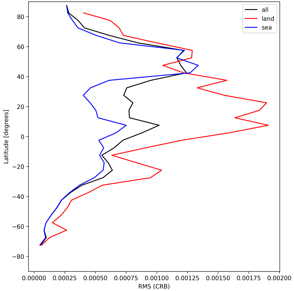
Figure 32: Zonal average of “RMS (CRB)” for 2025-08-06 to 2025-08-08.
