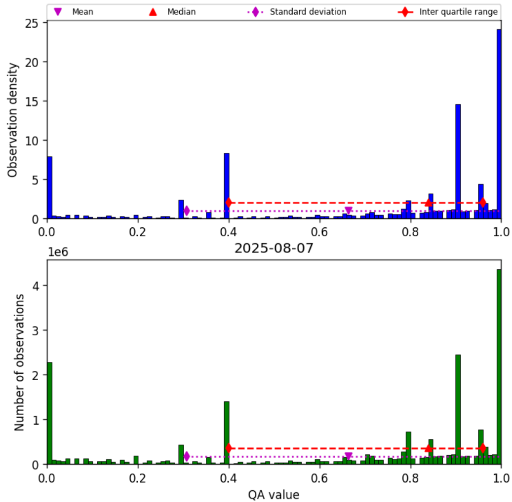
Figure 38: Histogram of “QA value” for 2025-08-06 to 2025-08-08
