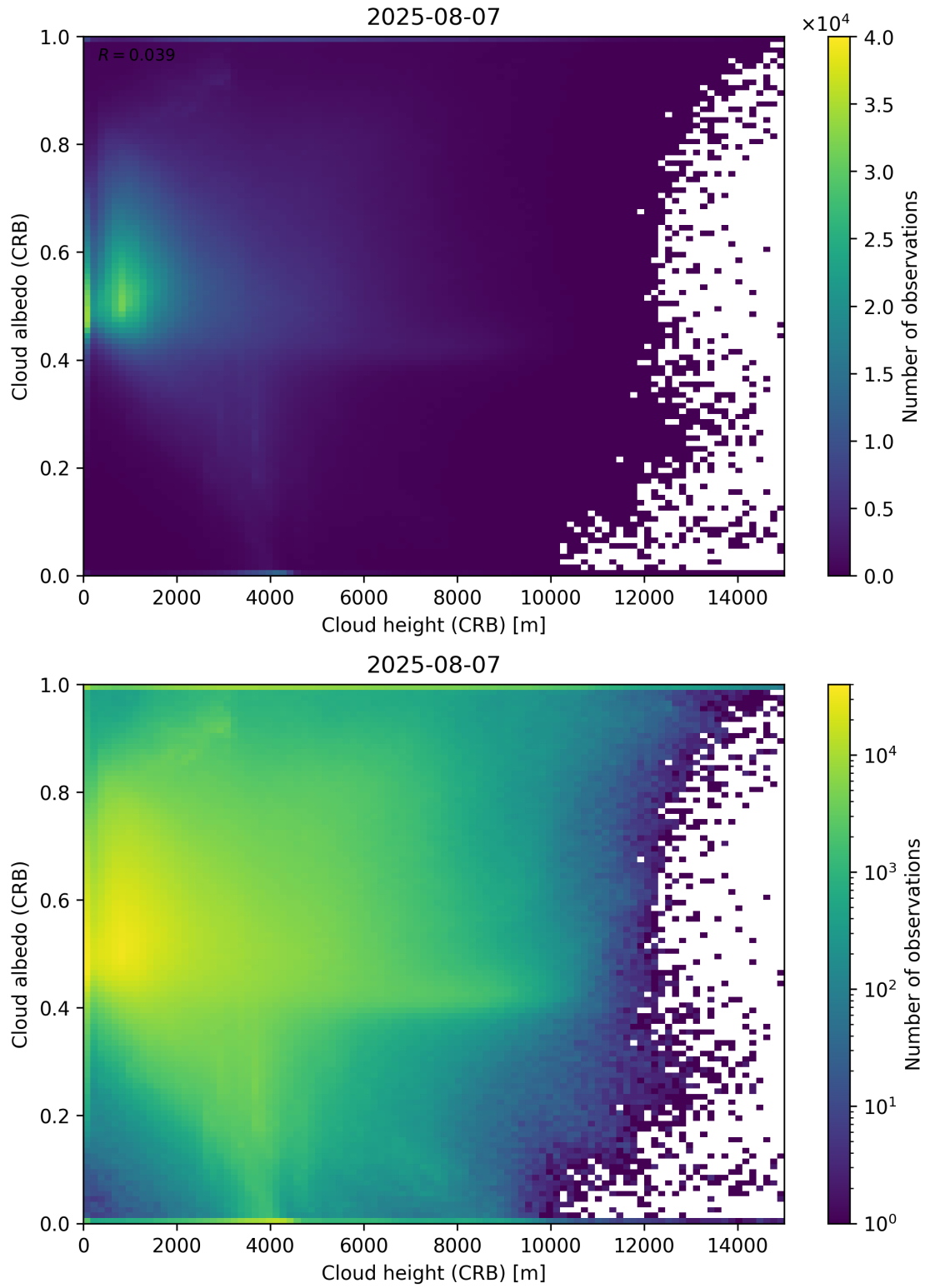
Figure 80: Scatter density plot of “Cloud height (CRB)” against “Cloud albedo (CRB)” for 2025-08-06 to 2025-08-08.
