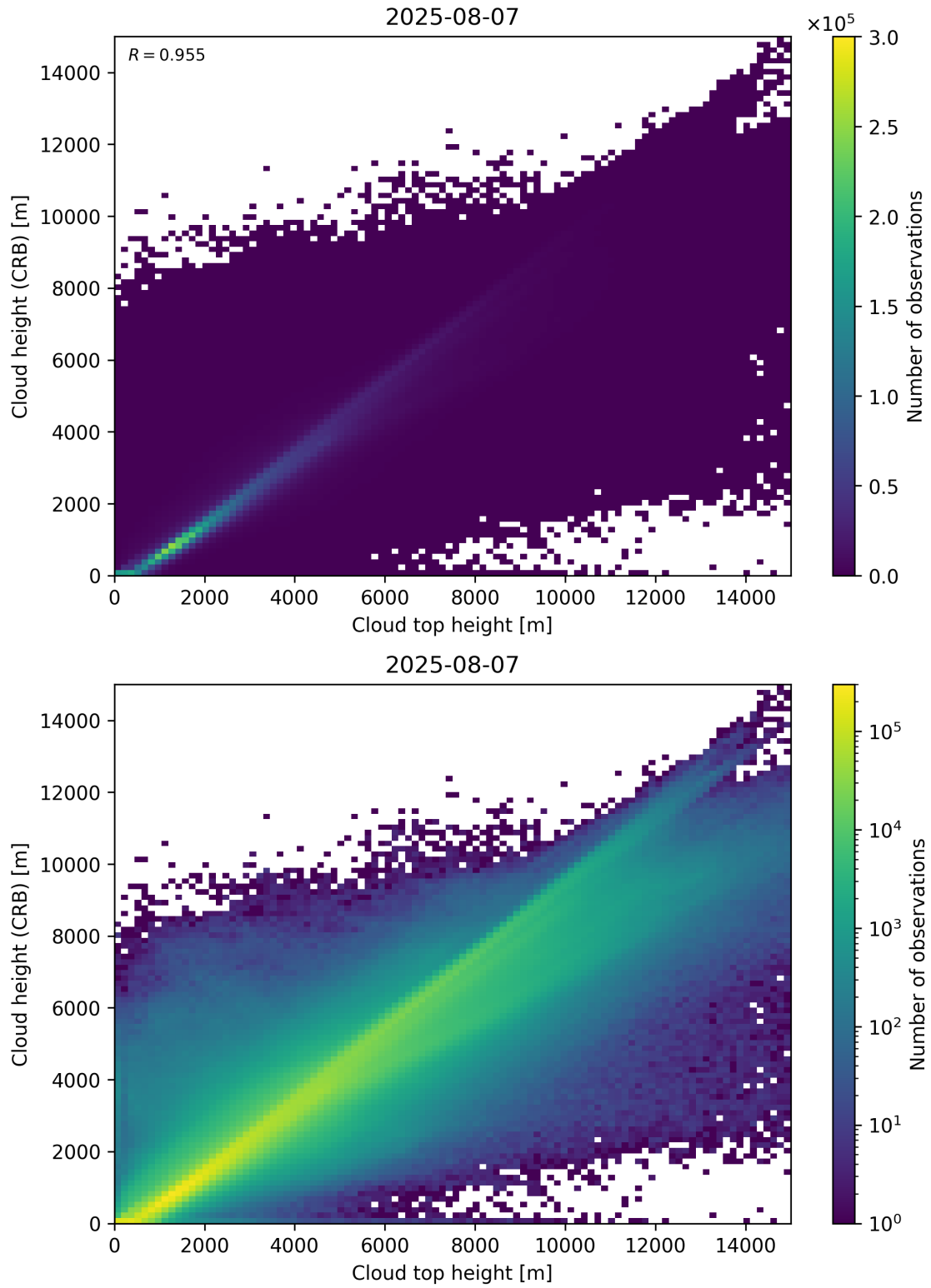
Figure 89: Scatter density plot of “Cloud top height” against “Cloud height (CRB)” for 2025-08-06 to 2025-08-08.
