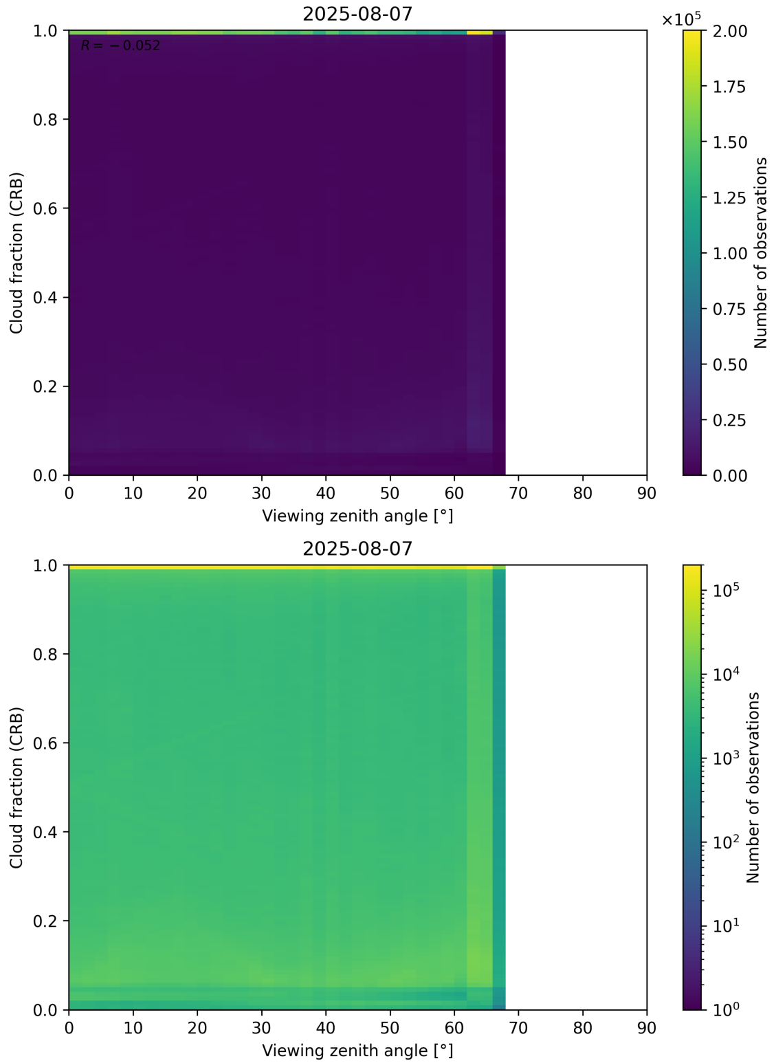
Figure 109: Scatter density plot of “Viewing zenith angle” against “Cloud fraction (CRB)” for 2025-08-06 to 2025-08-08.
