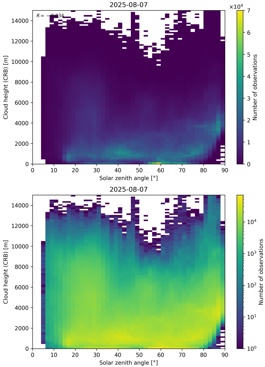
Figure 102: Scatter density plot of “Solar zenith angle” against “Cloud height (CRB)” for 2025-08-06 to 2025-08-08.
