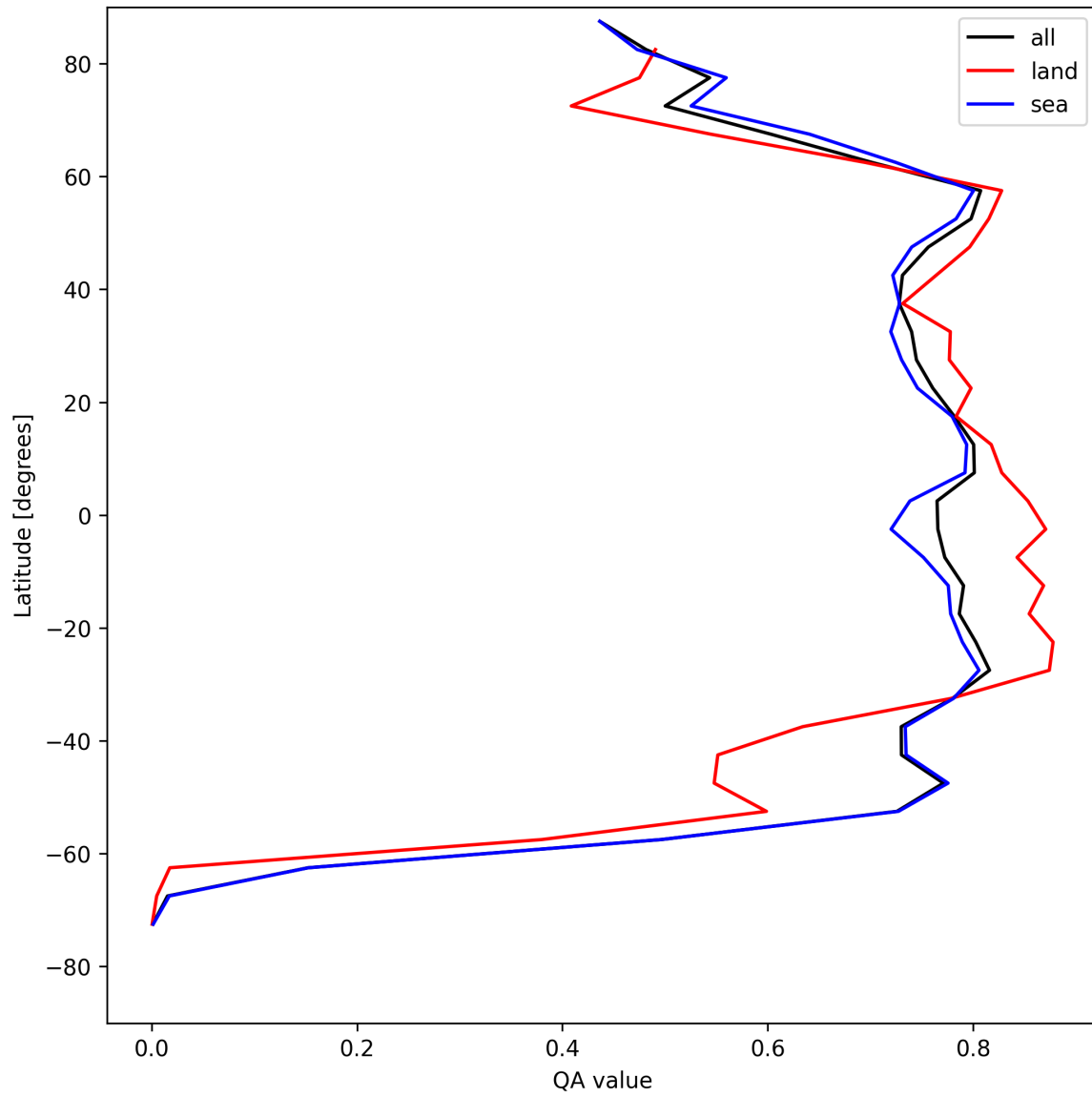
Figure 22: Zonal average of “QA value” for 2025-08-06 to 2025-08-08.
