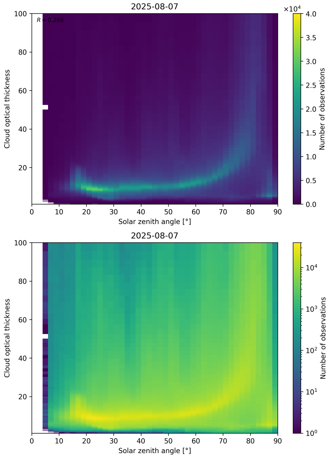
Figure 103: Scatter density plot of “Solar zenith angle” against “Cloud optical thickness” for 2025-08-06 to 2025-08-08.
