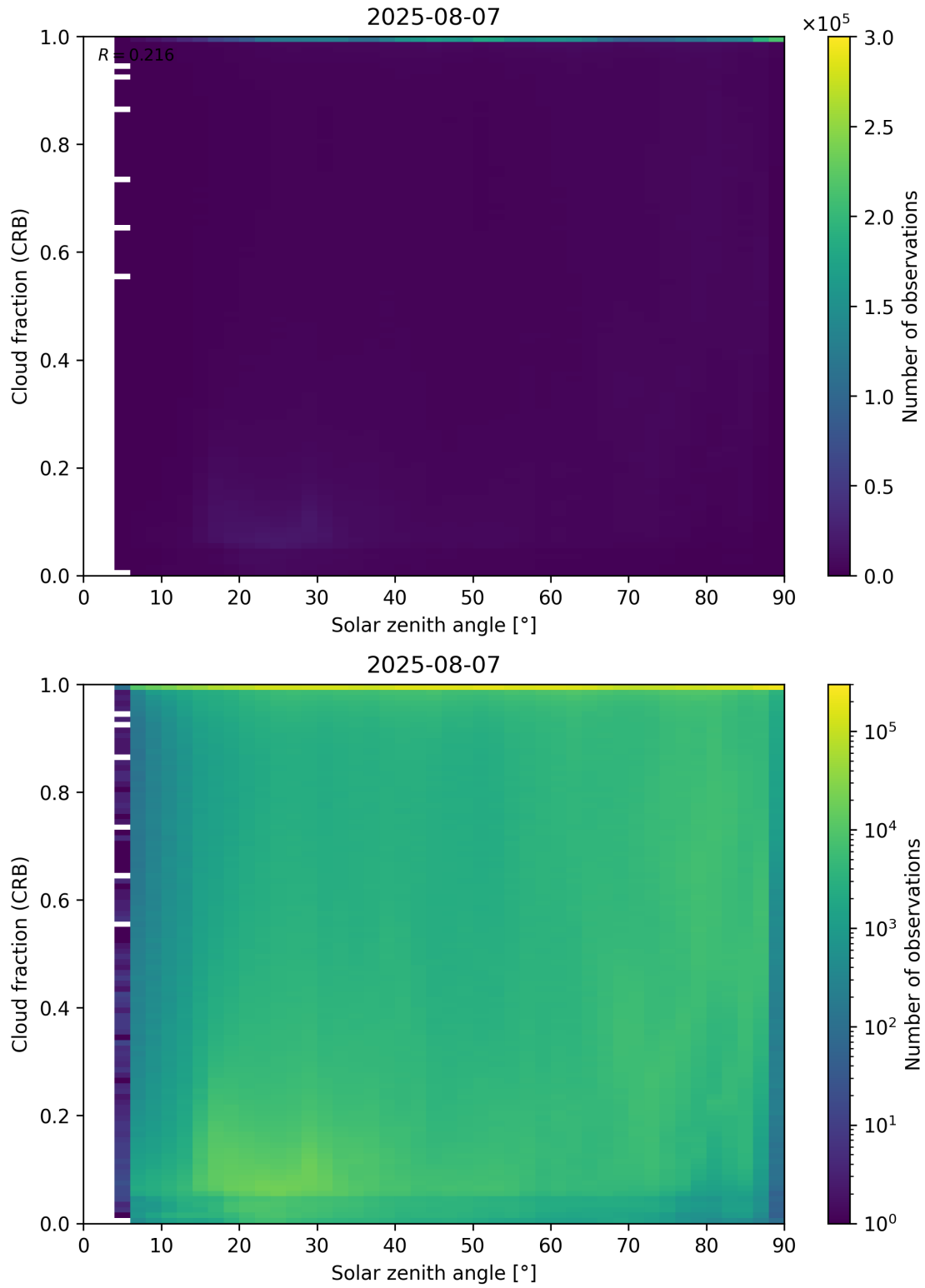
Figure 101: Scatter density plot of “Solar zenith angle” against “Cloud fraction (CRB)” for 2025-08-06 to 2025-08-08.
