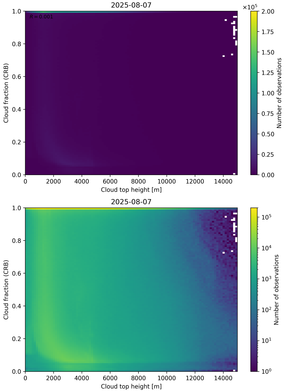
Figure 88: Scatter density plot of “Cloud top height” against “Cloud fraction (CRB)” for 2025-08-06 to 2025-08-08.
