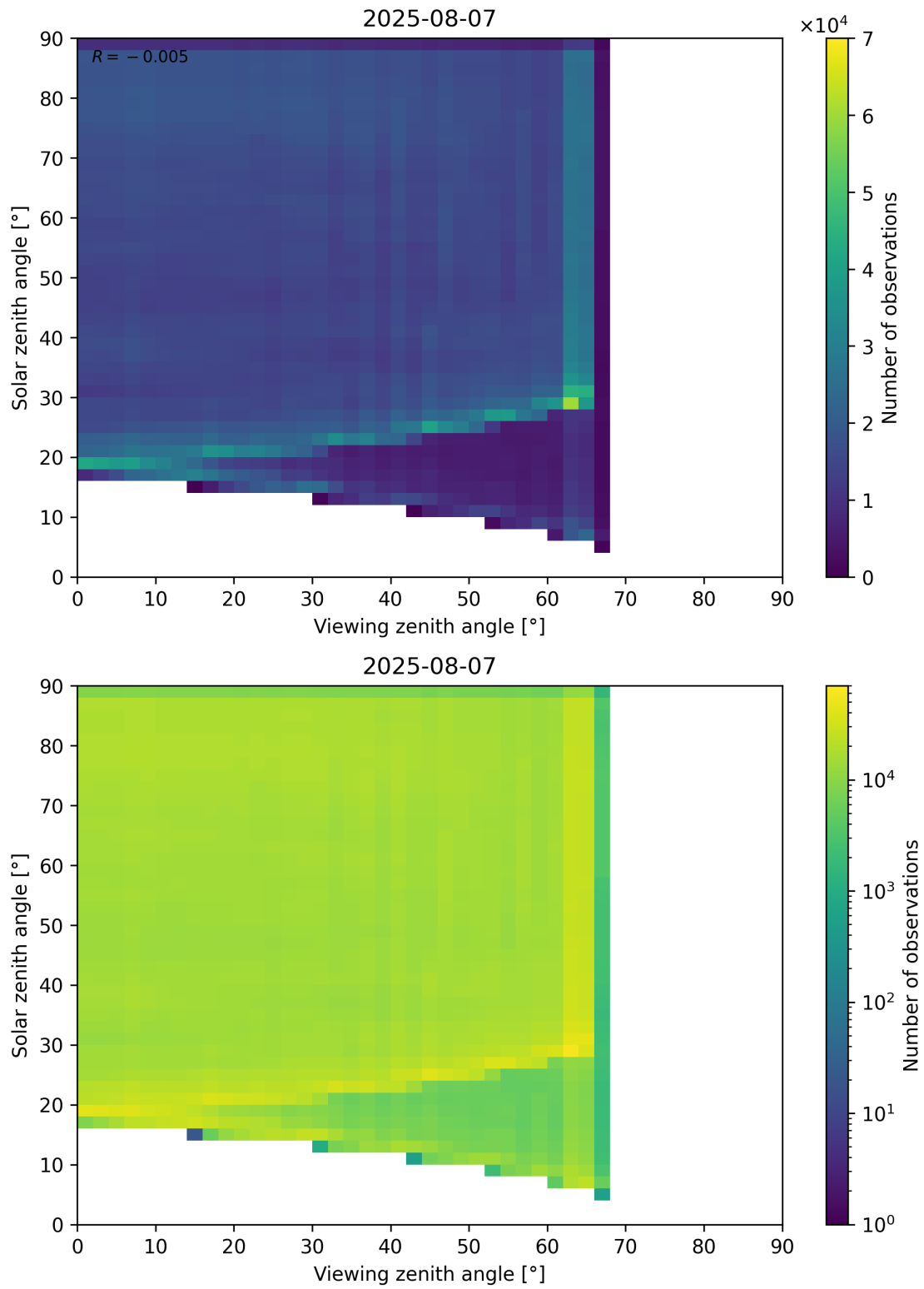
Figure 114: Scatter density plot of “Viewing zenith angle” against “Solar zenith angle” for 2025-08-06 to 2025-08-08.
