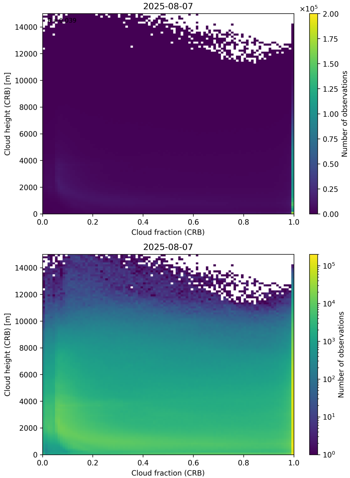
Figure 79: Scatter density plot of “Cloud fraction (CRB)” against “Cloud height (CRB)” for 2025-08-06 to 2025-08-08.
