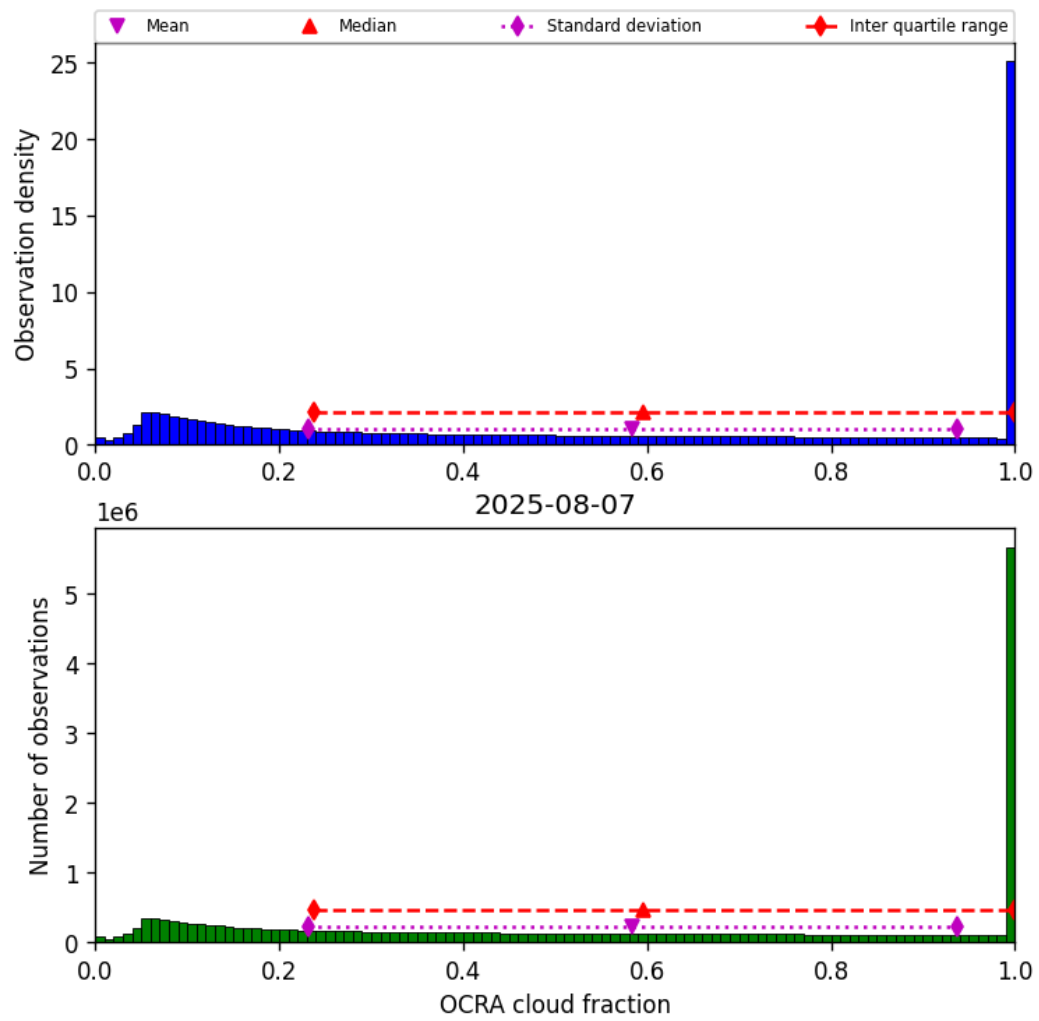
Figure 50: Histogram of “OCRA cloud fraction” for 2025-08-06 to 2025-08-08
