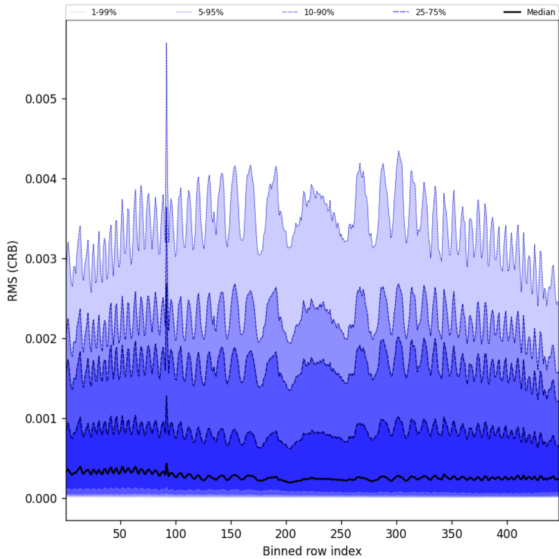
Figure 64: Along track statistics of “RMS (CRB)” for 2025-08-06 to 2025-08-08
