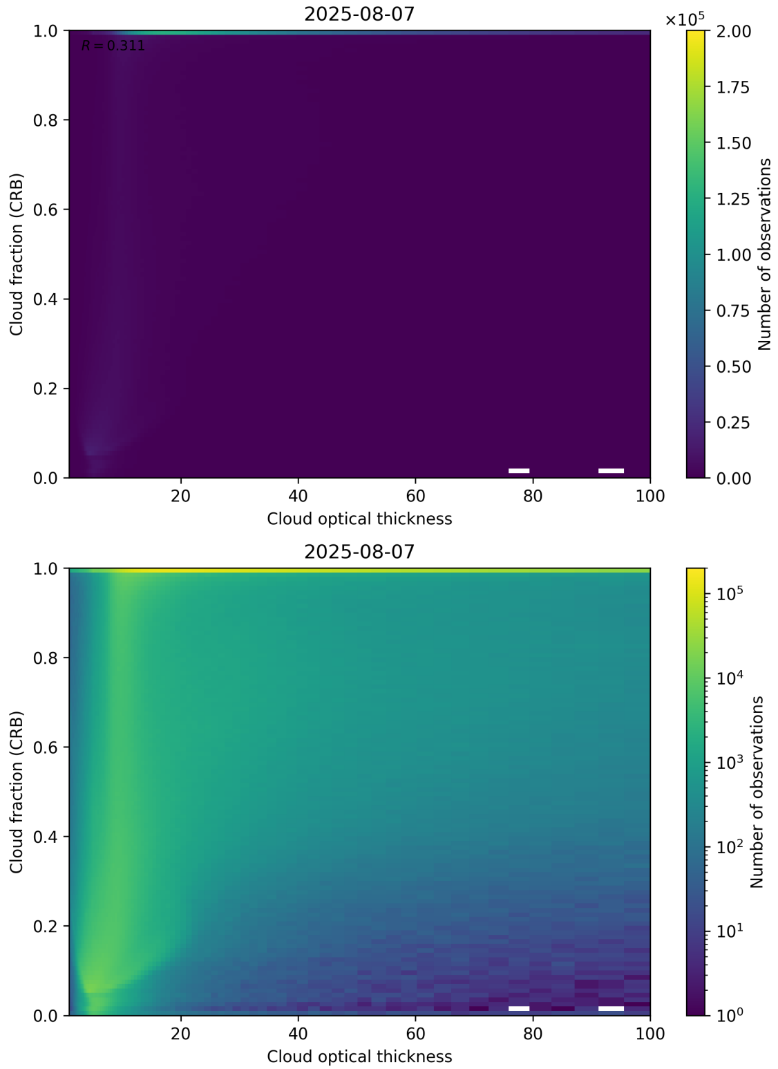
Figure 84: Scatter density plot of “Cloud optical thickness” against “Cloud fraction (CRB)” for 2025-08-06 to 2025-08-08.
