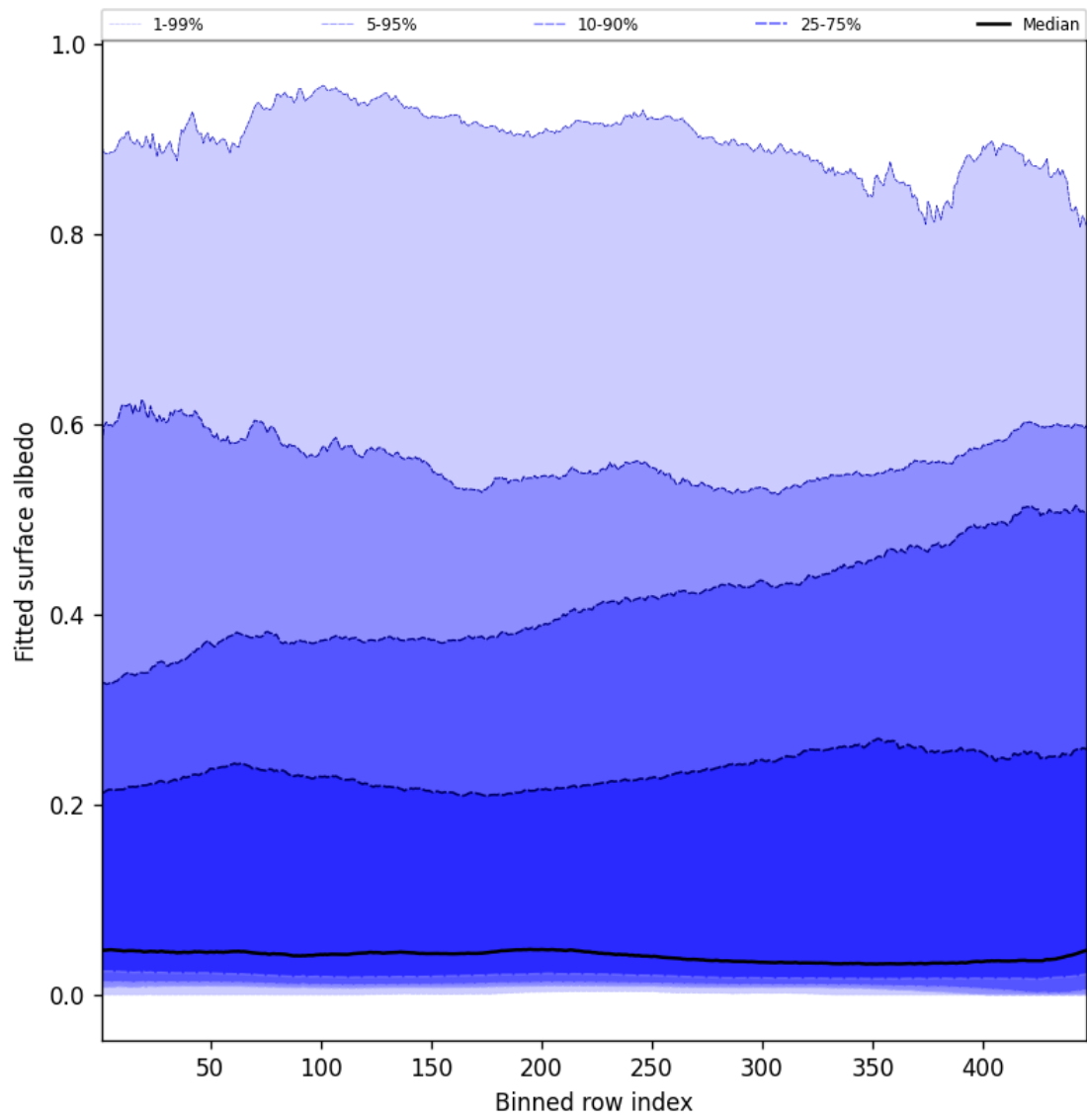
Figure 61: Along track statistics of “Fitted surface albedo” for 2025-08-06 to 2025-08-08
