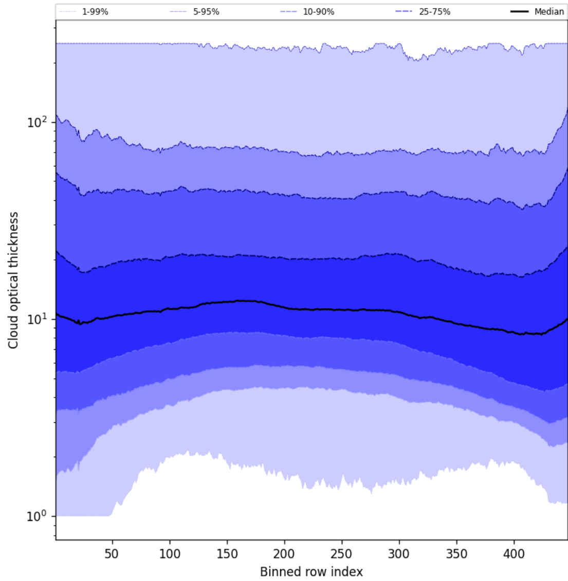
Figure 57: Along track statistics of “Cloud optical thickness” for 2025-08-06 to 2025-08-08
