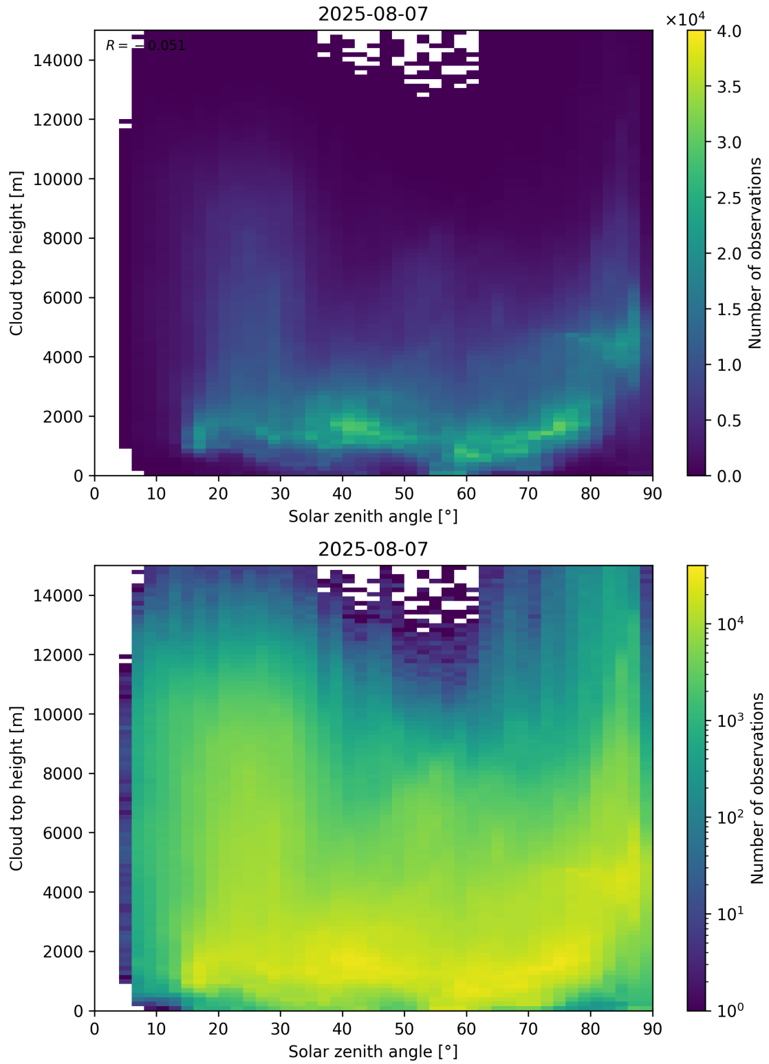
Figure 104: Scatter density plot of “Solar zenith angle” against “Cloud top height” for 2025-08-06 to 2025-08-08.
