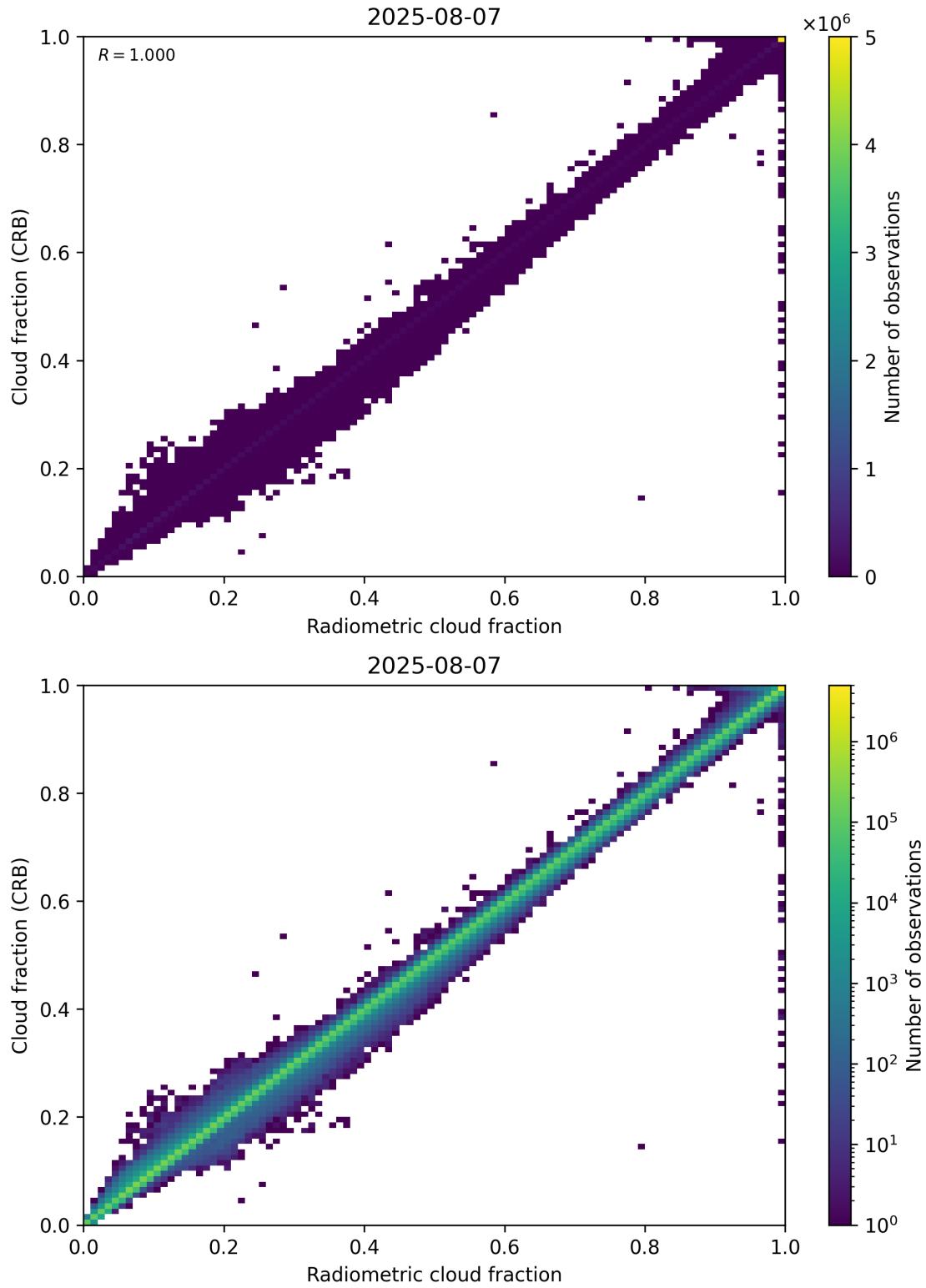
Figure 73: Scatter density plot of “Radiometric cloud fraction” against “Cloud fraction (CRB)” for 2025-08-06 to 2025-08-08.
