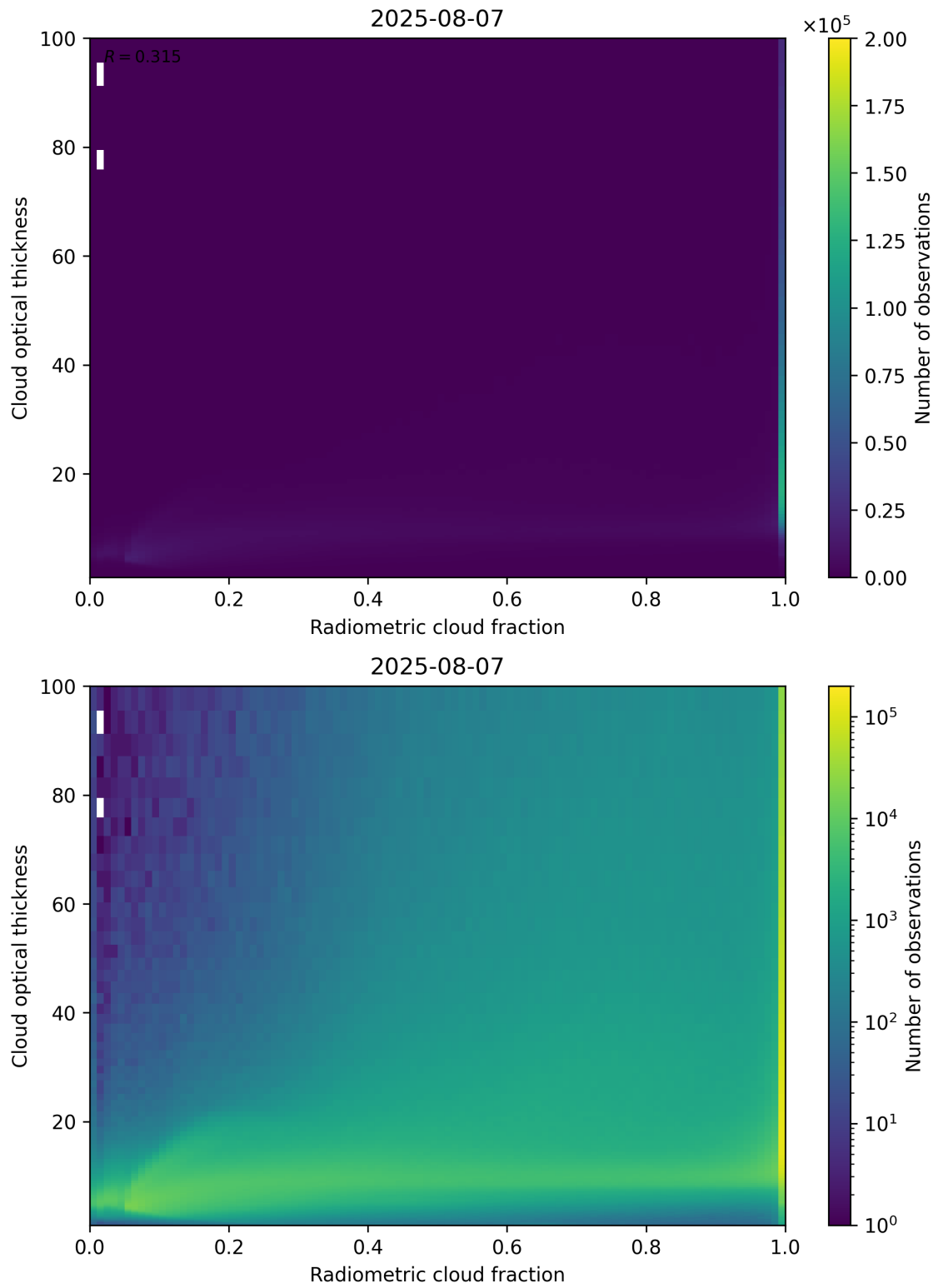
Figure 75: Scatter density plot of “Radiometric cloud fraction” against “Cloud optical thickness” for 2025-08-06 to 2025-08-08.
