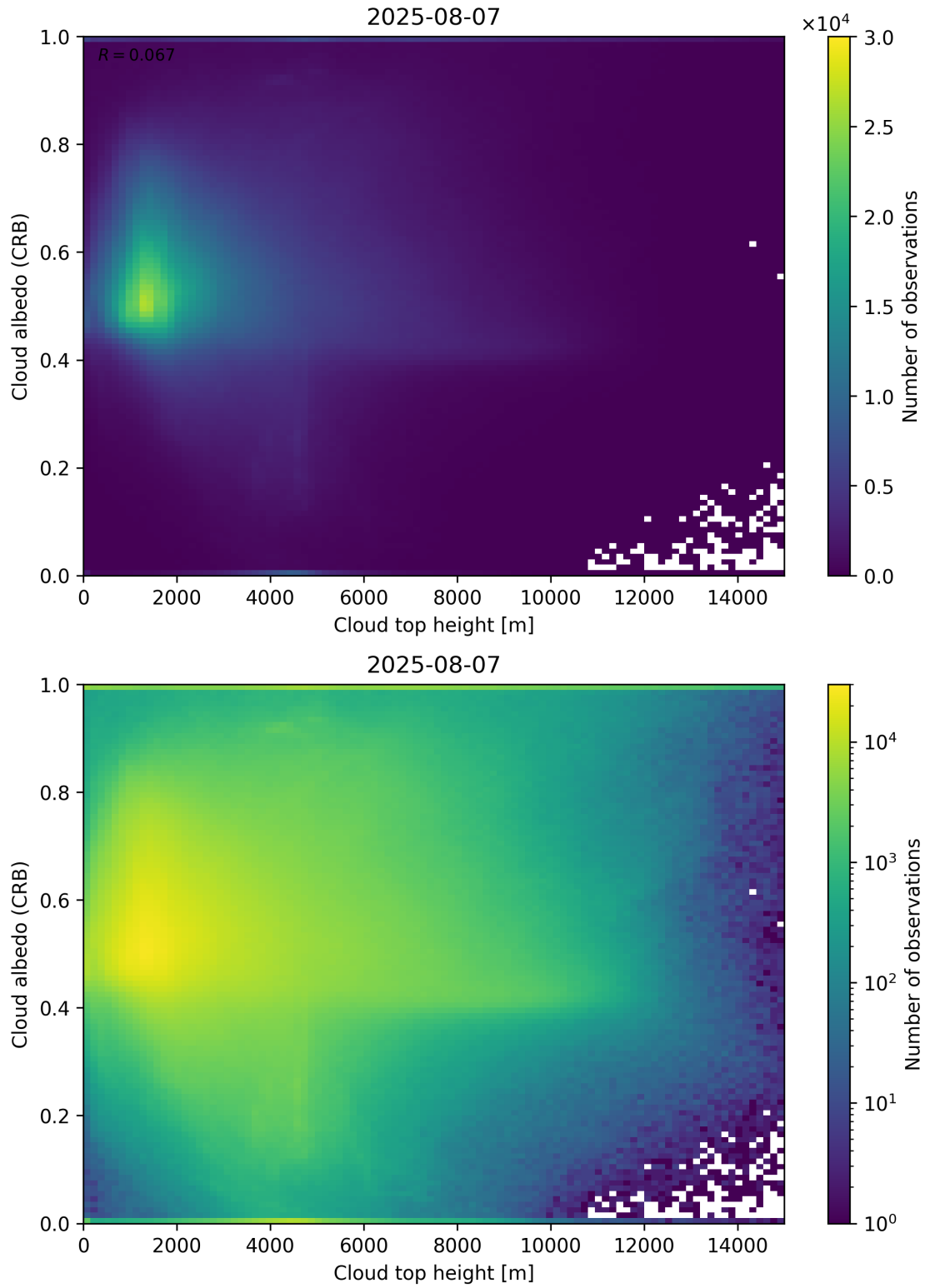
Figure 86: Scatter density plot of “Cloud top height” against “Cloud albedo (CRB)” for 2025-08-06 to 2025-08-08.
