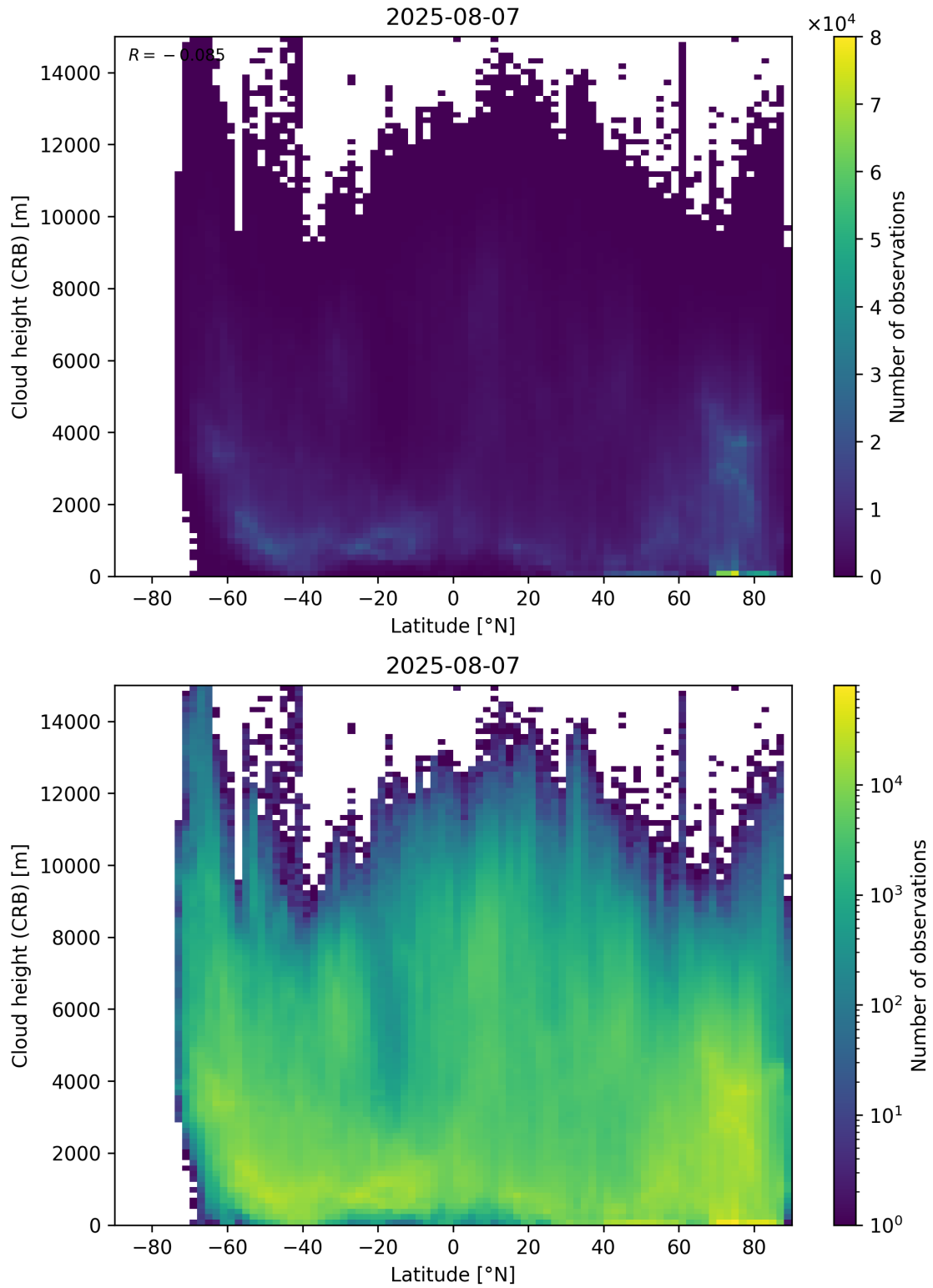
Figure 95: Scatter density plot of “Latitude” against “Cloud height (CRB)” for 2025-08-06 to 2025-08-08.
