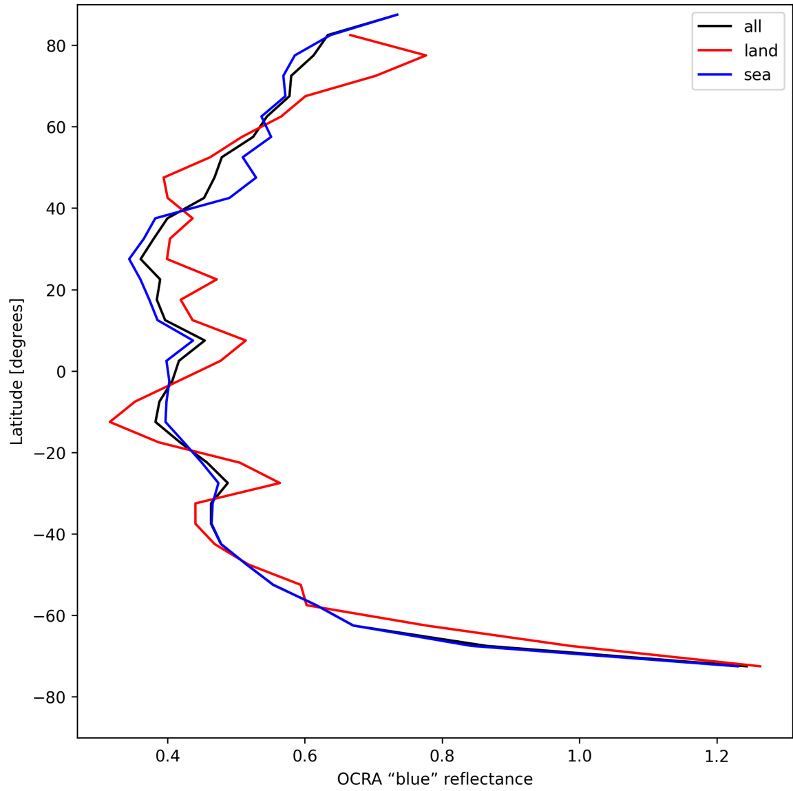
Figure 35: Zonal average of "OCRA "blue" reflectance" for 2025-08-06 to 2025-08-08.
