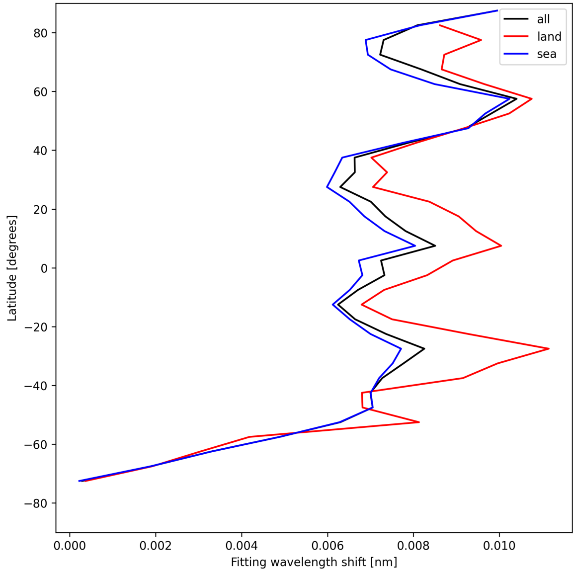
Figure 33: Zonal average of “Fitting wavelength shift” for 2025-08-06 to 2025-08-08.
