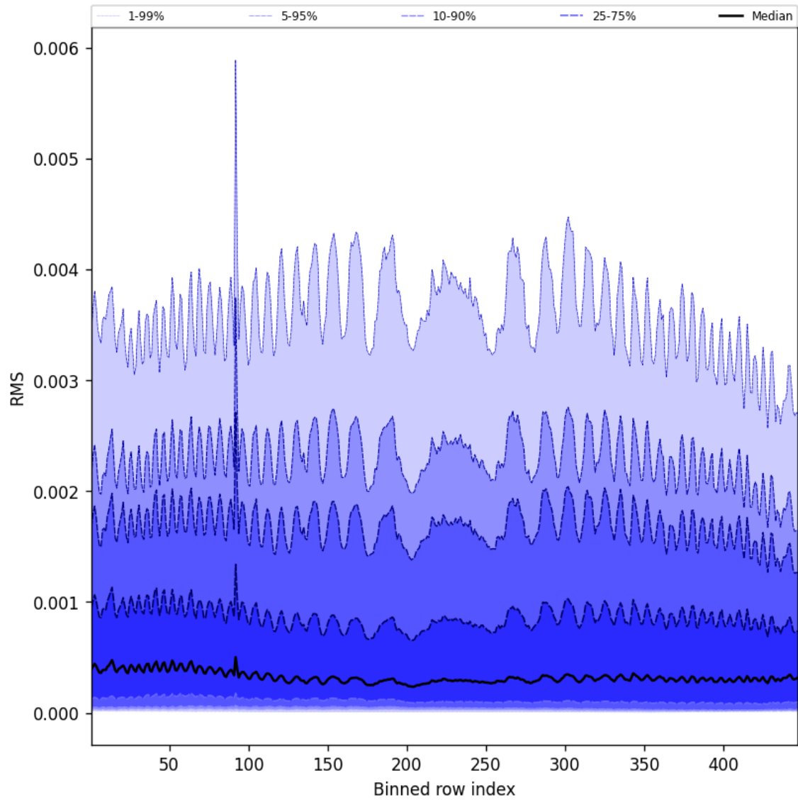
Figure 63: Along track statistics of “RMS” for 2025-08-06 to 2025-08-08
