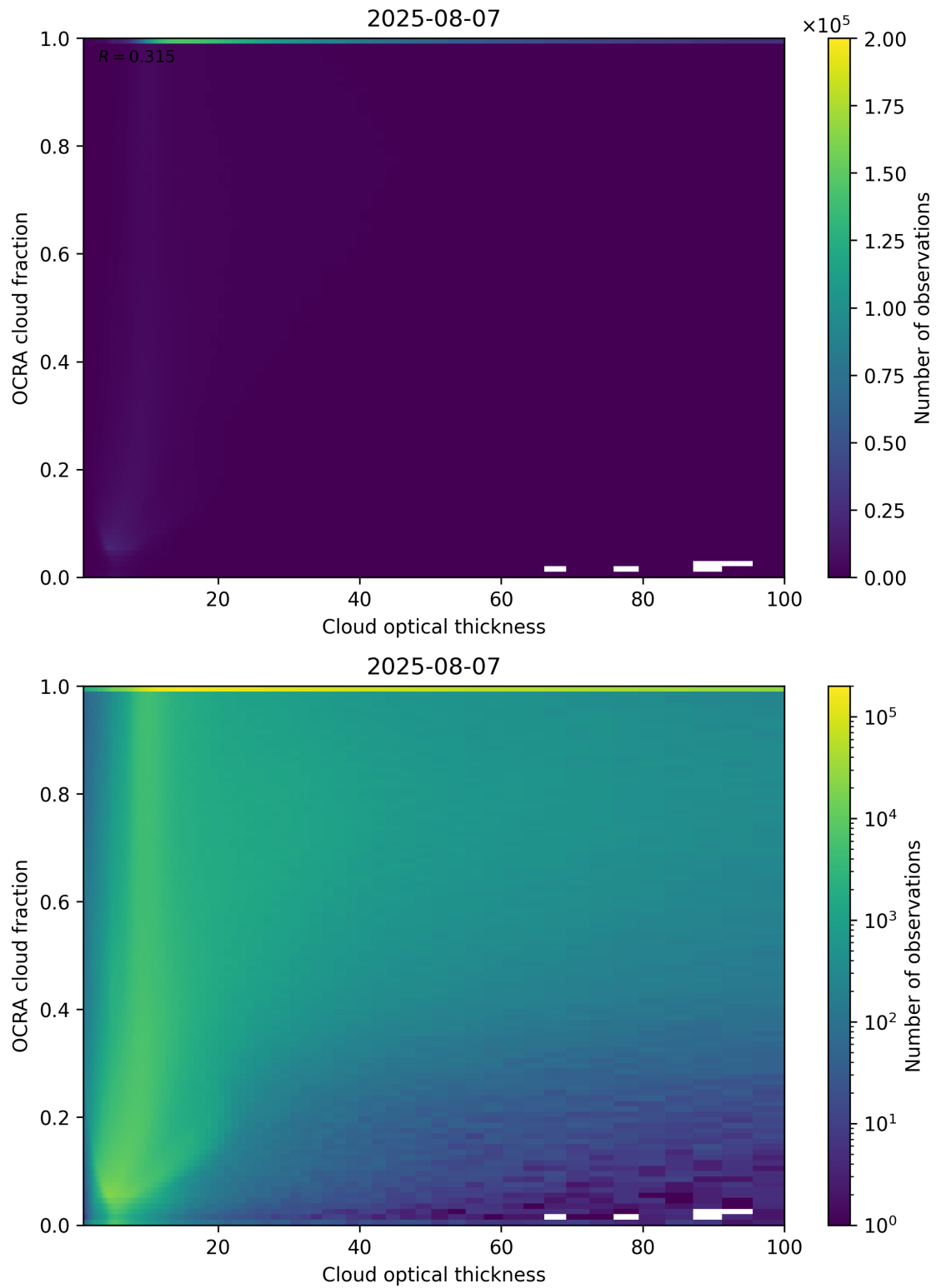
Figure 83: Scatter density plot of “Cloud optical thickness” against “OCRA cloud fraction” for 2025-08-06 to 2025-08-08.
