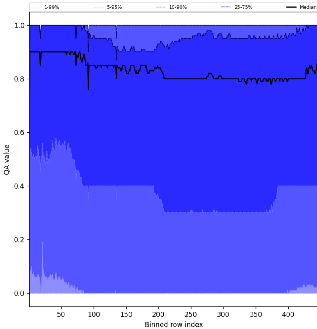
Figure 54: Along track statistics of “QA value” for 2025-08-06 to 2025-08-08
