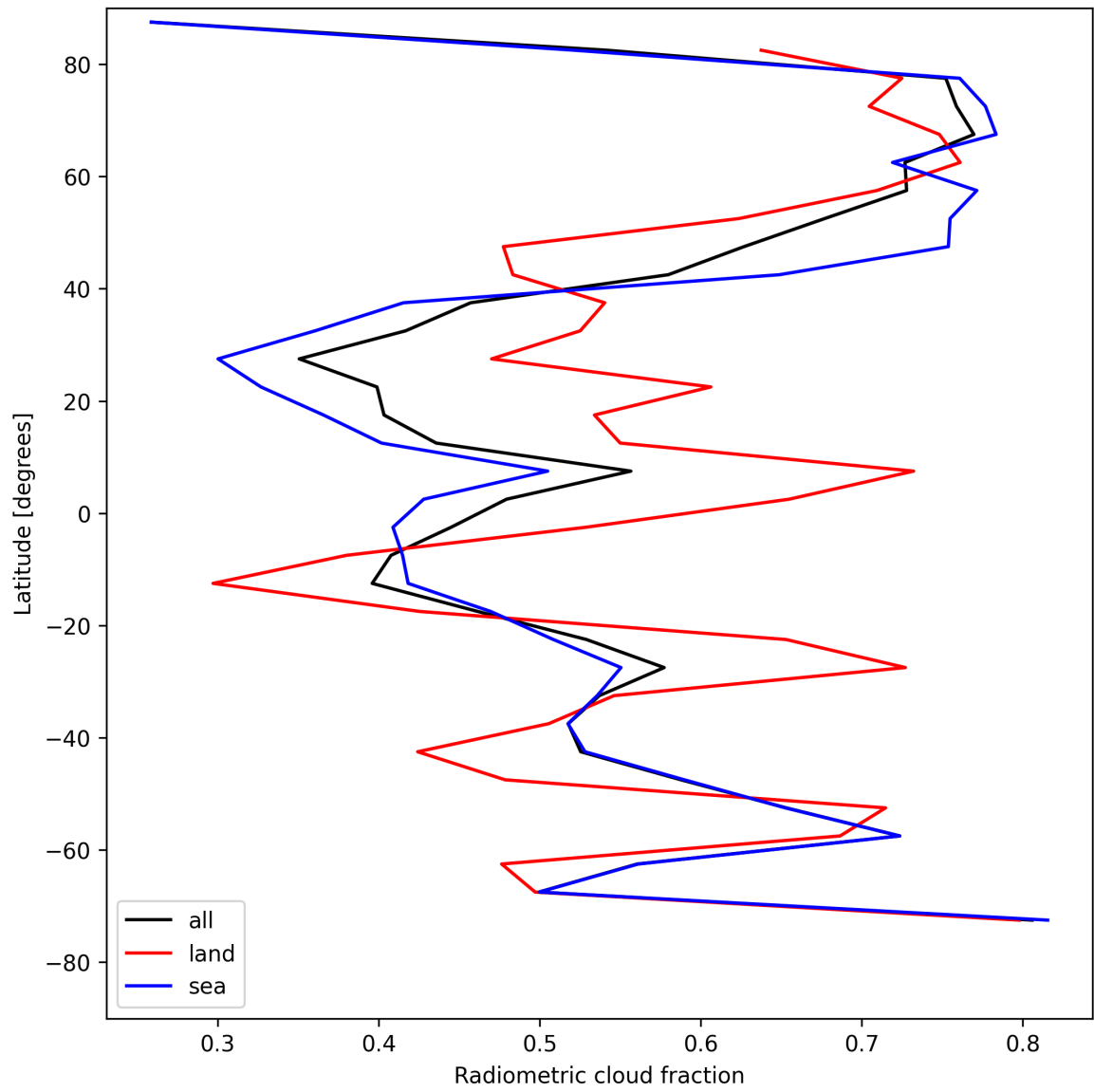
Figure 23: Zonal average of “Radiometric cloud fraction” for 2025-08-06 to 2025-08-08.
