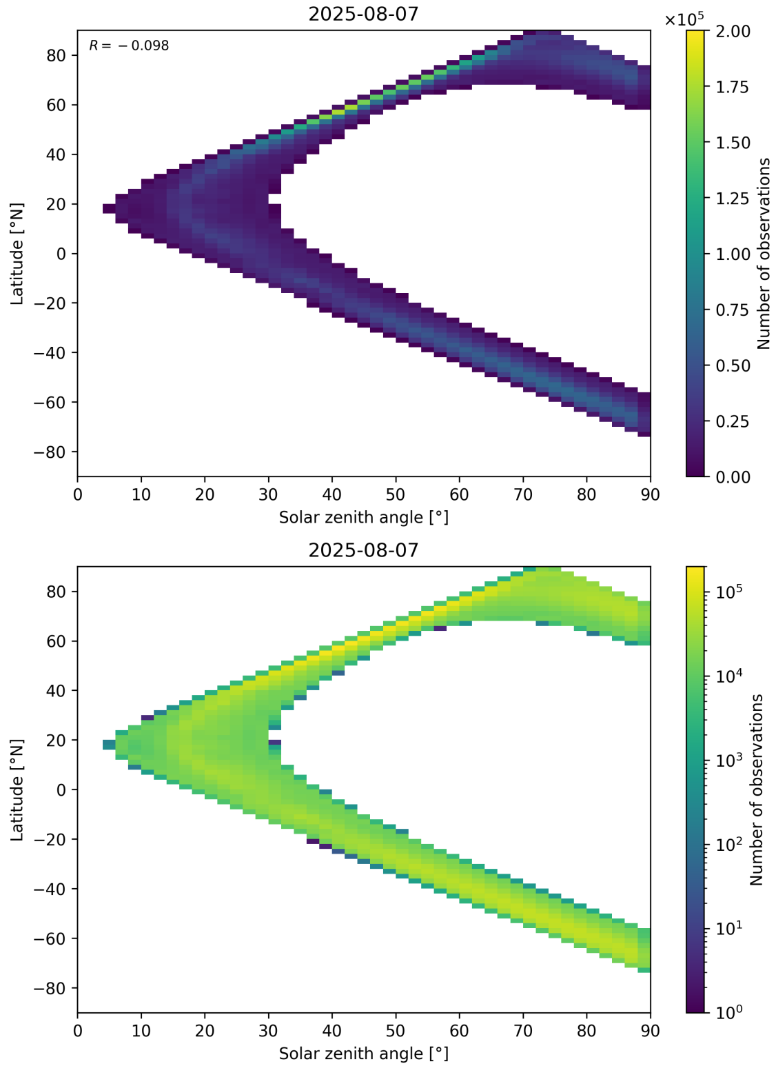
Figure 105: Scatter density plot of “Solar zenith angle” against “Latitude” for 2025-08-06 to 2025-08-08.
