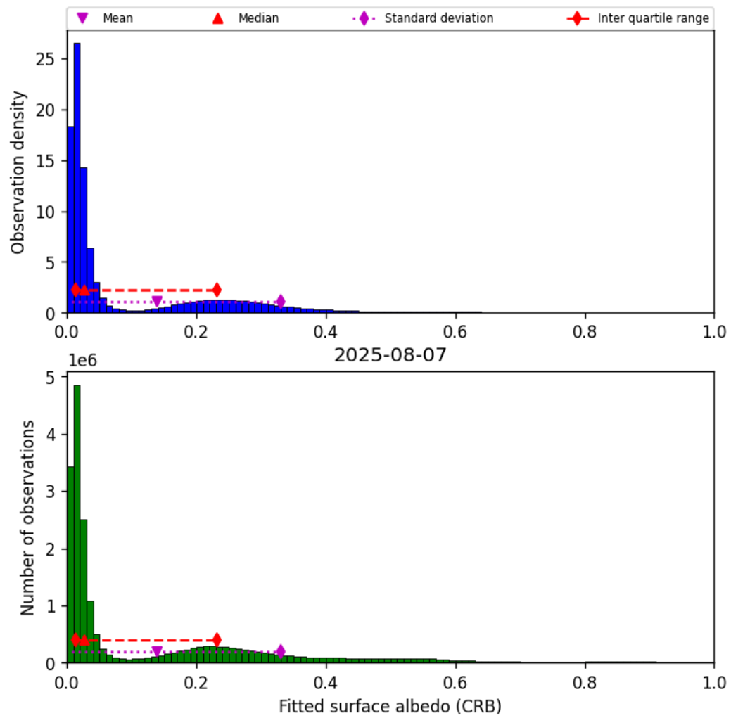
Figure 46: Histogram of “Fitted surface albedo (CRB)” for 2025-08-06 to 2025-08-08
