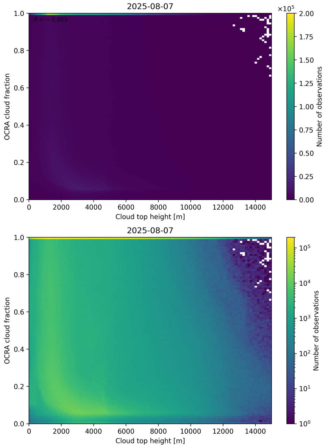
Figure 87: Scatter density plot of “Cloud top height” against “OCRA cloud fraction” for 2025-08-06 to 2025-08-08.
