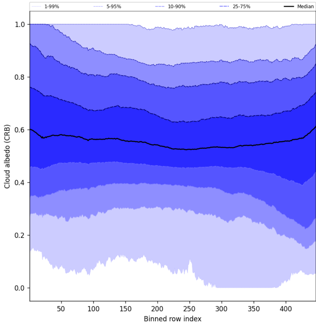
Figure 60: Along track statistics of “Cloud albedo (CRB)” for 2025-08-06 to 2025-08-08
