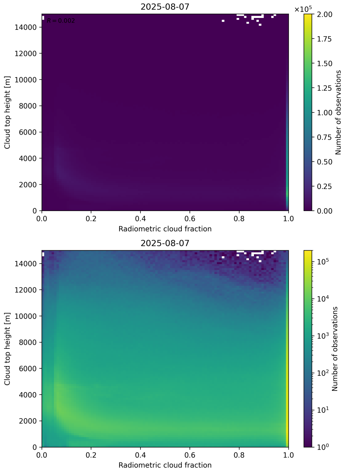
Figure 76: Scatter density plot of “Radiometric cloud fraction” against “Cloud top height” for 2025-08-06 to 2025-08-08.
