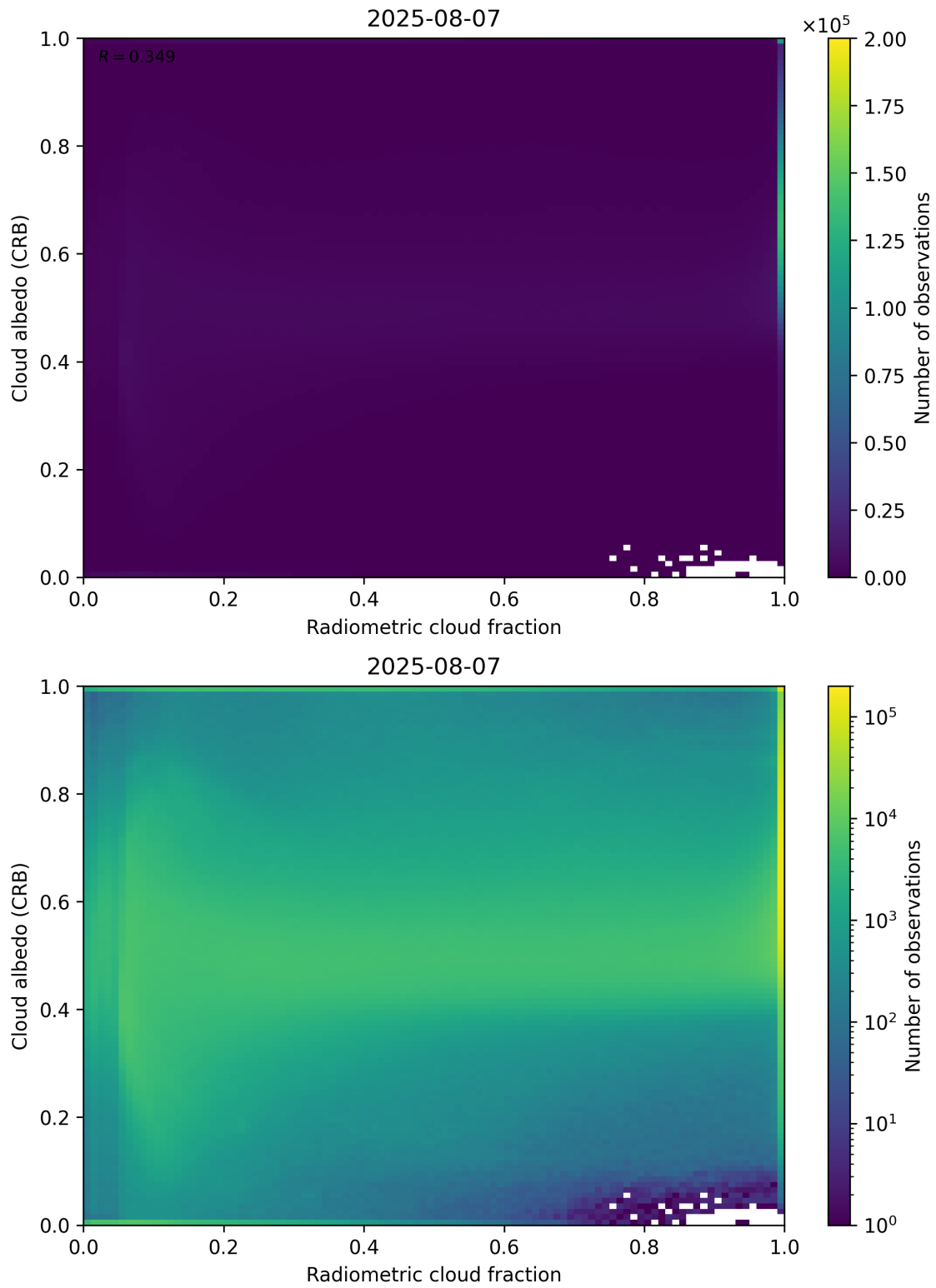
Figure 71: Scatter density plot of “Radiometric cloud fraction” against “Cloud albedo (CRB)” for 2025-08-06 to 2025-08-08.
