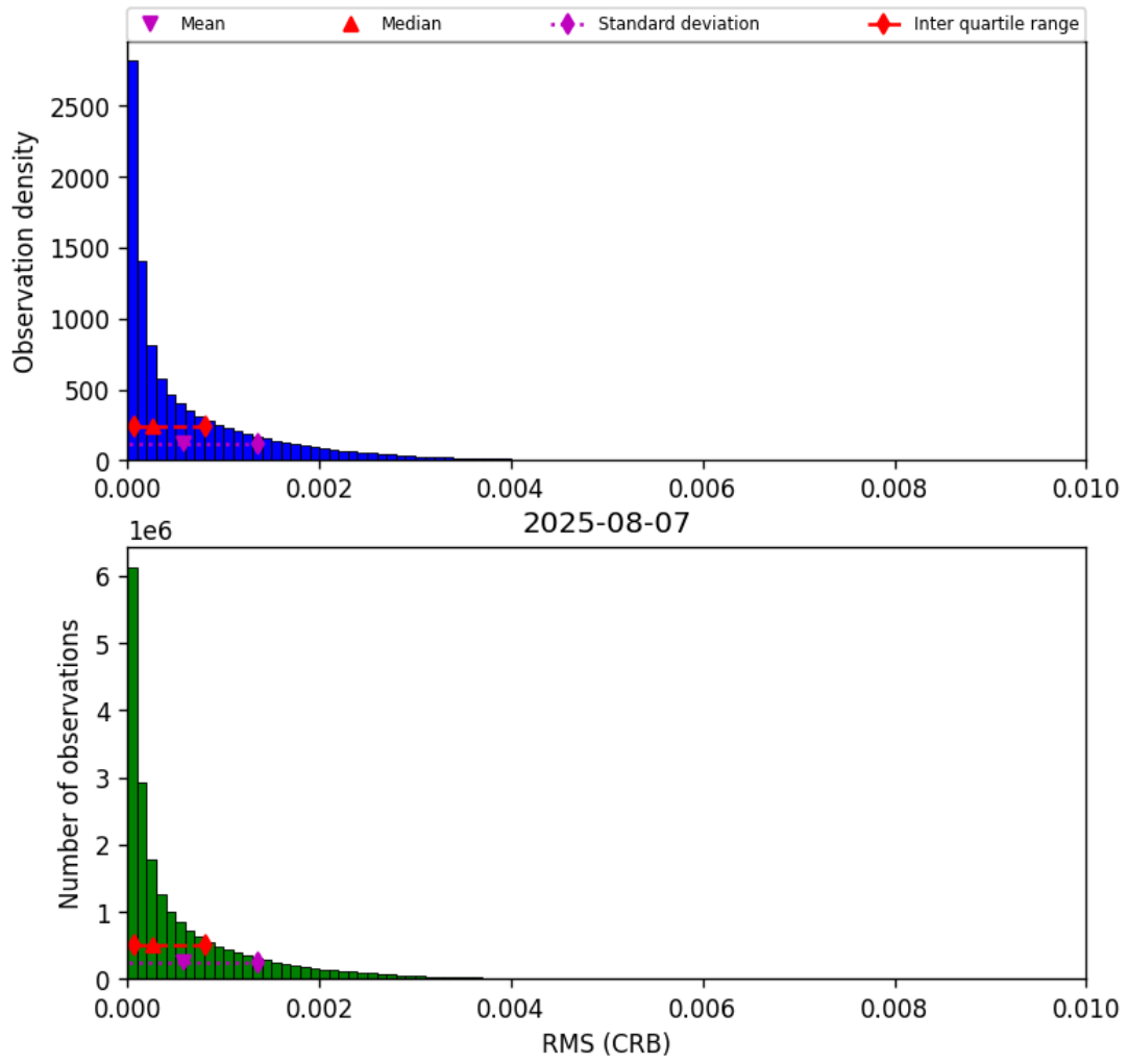
Figure 48: Histogram of “RMS (CRB)” for 2025-08-06 to 2025-08-08
