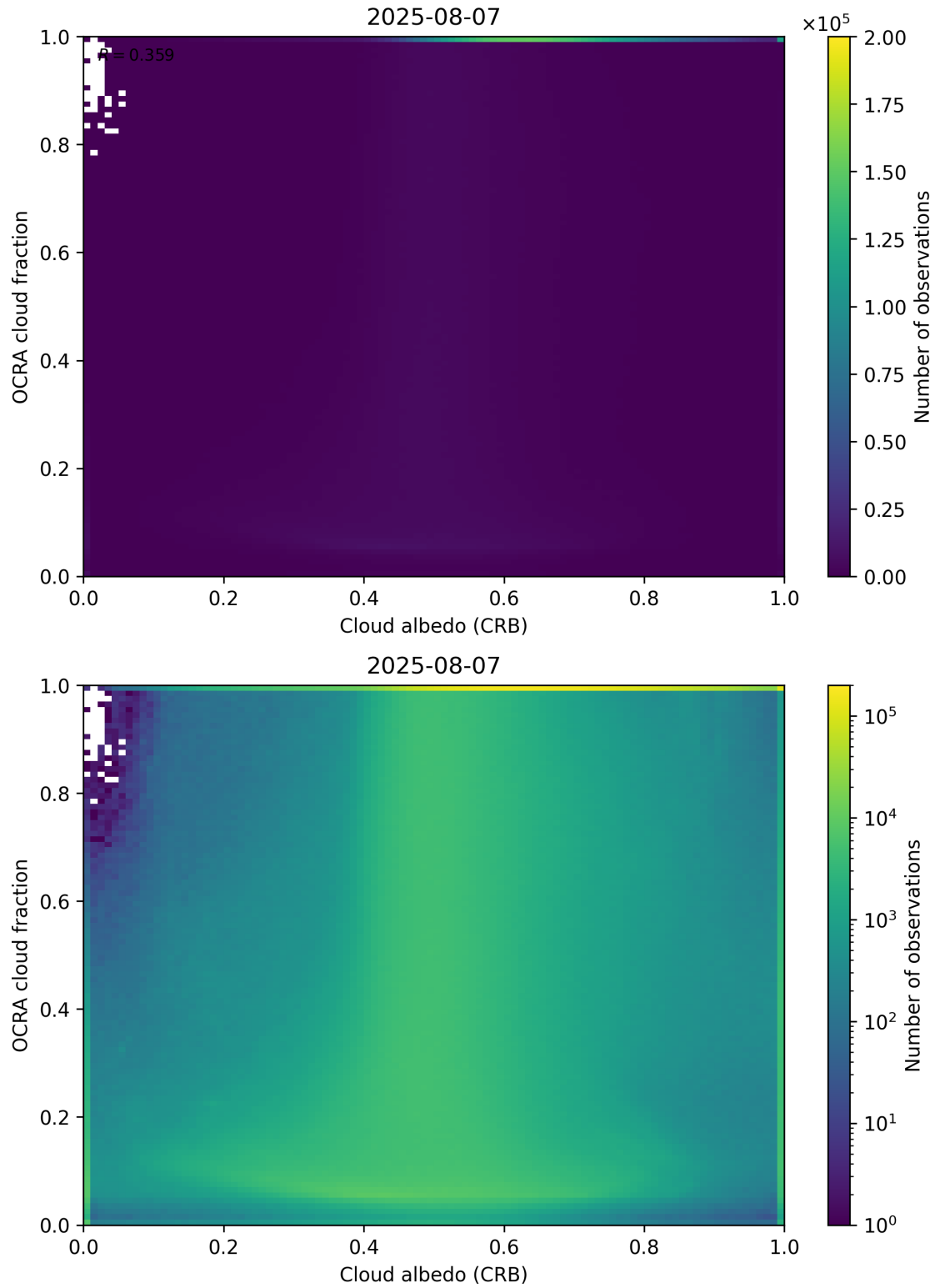
Figure 70: Scatter density plot of “Cloud albedo (CRB)” against “OCRA cloud fraction” for 2025-08-06 to 2025-08-08.
