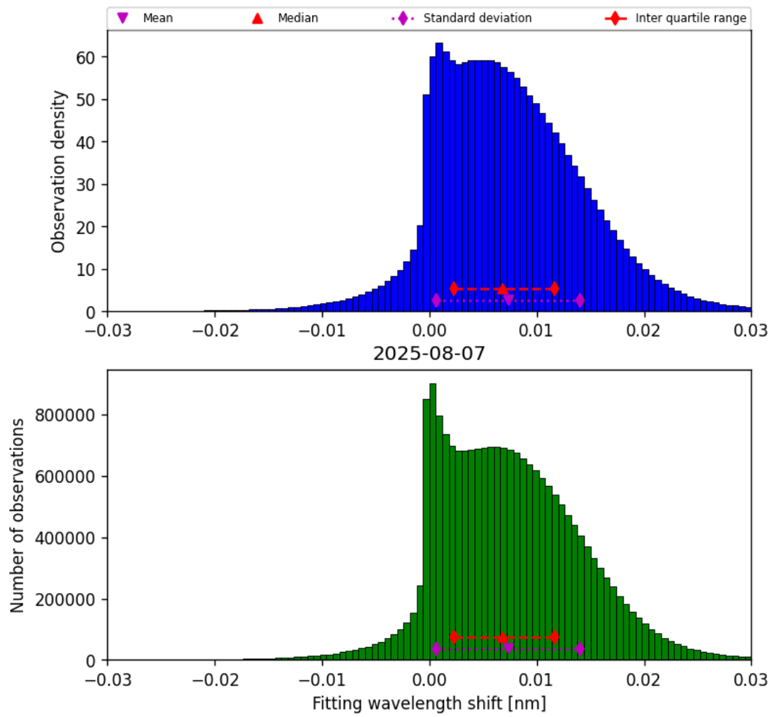
Figure 49: Histogram of “Fitting wavelength shift” for 2025-08-06 to 2025-08-08
