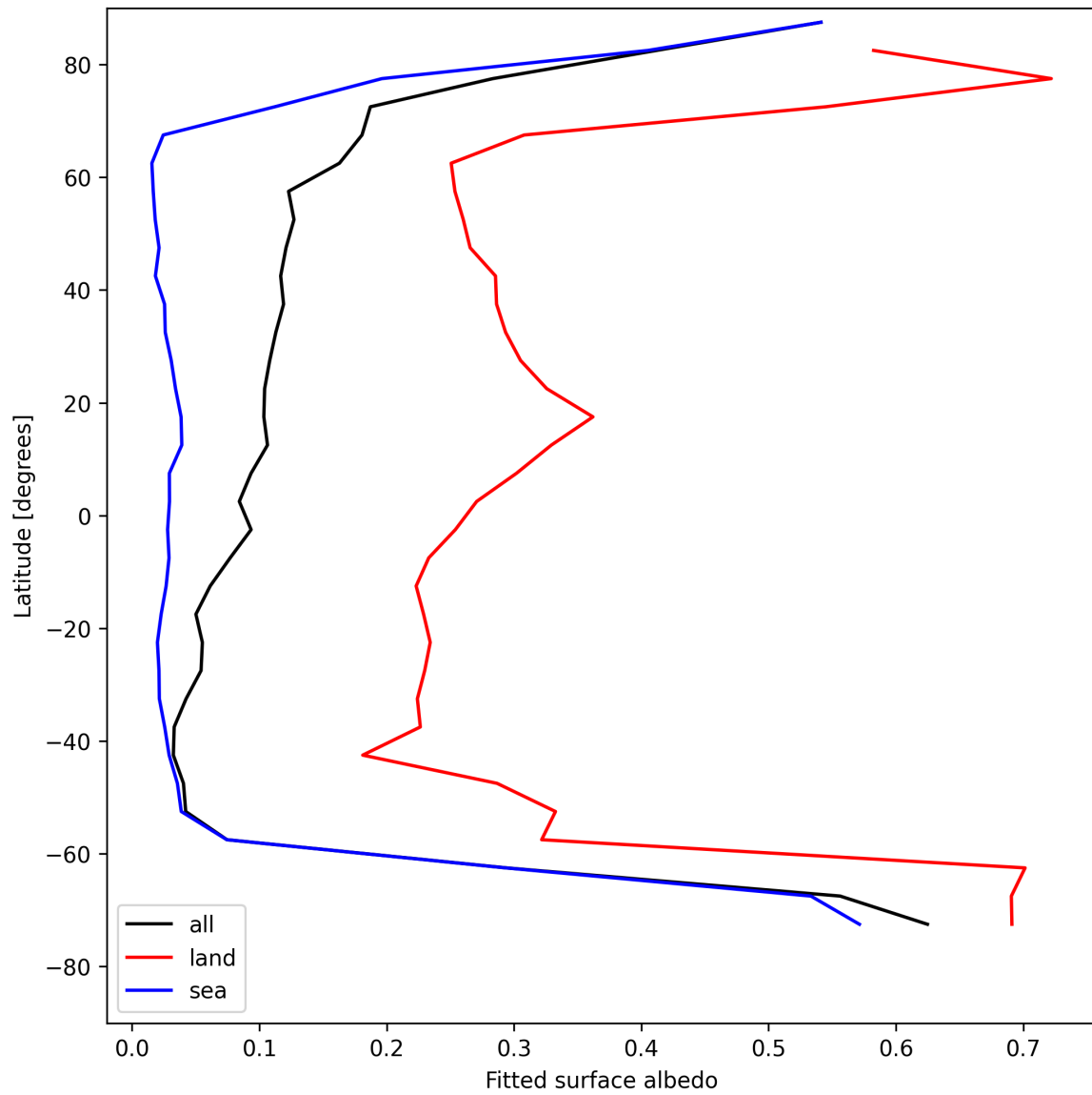
Figure 29: Zonal average of “Fitted surface albedo” for 2025-08-06 to 2025-08-08.
