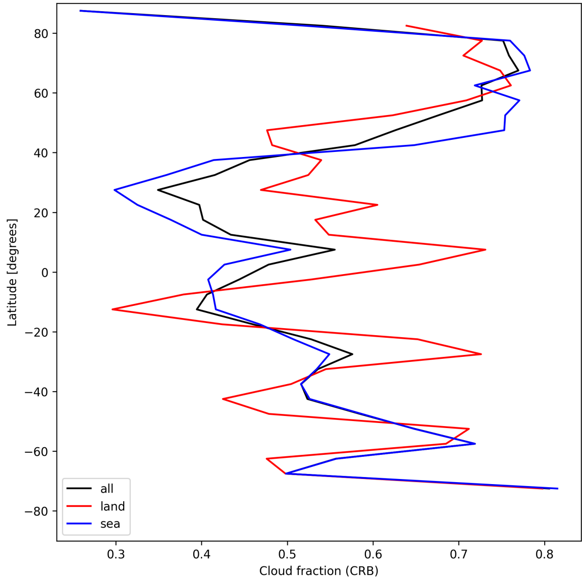
Figure 26: Zonal average of “Cloud fraction (CRB)” for 2025-08-06 to 2025-08-08.
