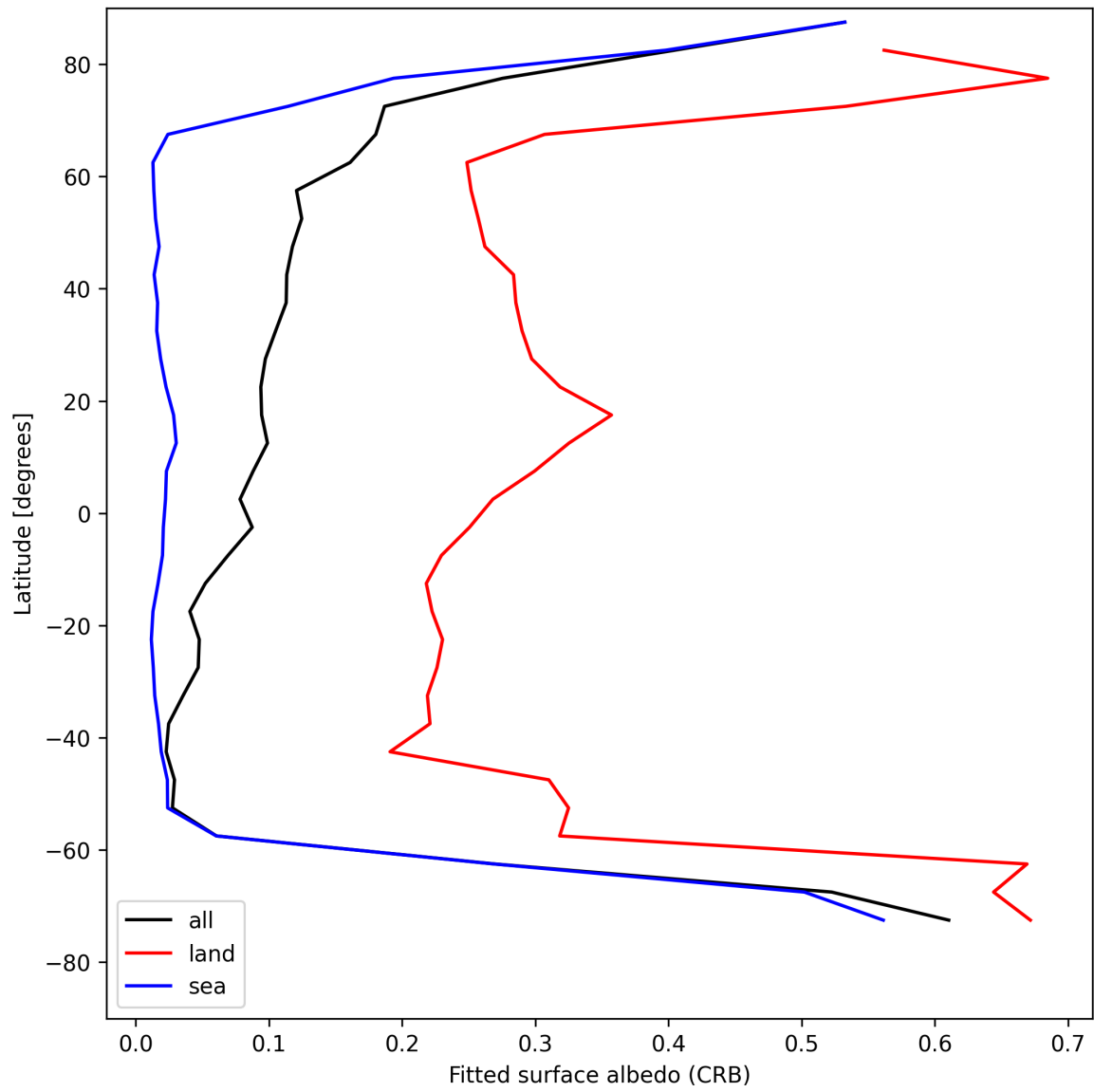
Figure 30: Zonal average of “Fitted surface albedo (CRB)” for 2025-08-06 to 2025-08-08.
