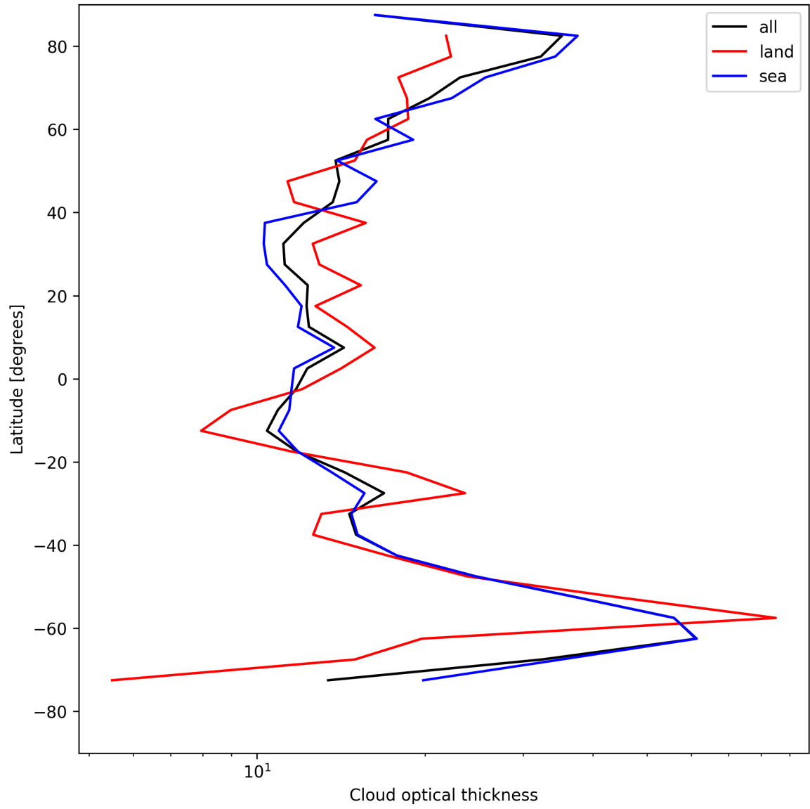
Figure 25: Zonal average of “Cloud optical thickness” for 2025-08-06 to 2025-08-08.
