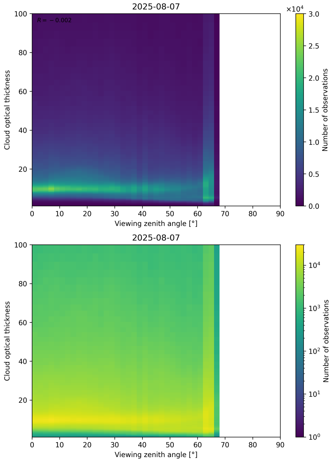
Figure 111: Scatter density plot of “Viewing zenith angle” against “Cloud optical thickness” for 2025-08-06 to 2025-08-08.
