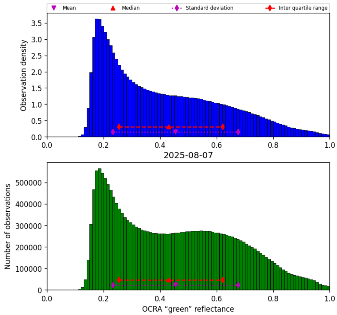
Figure 52: Histogram of “OCRA “green” reflectance” for 2025-08-06 to 2025-08-08
