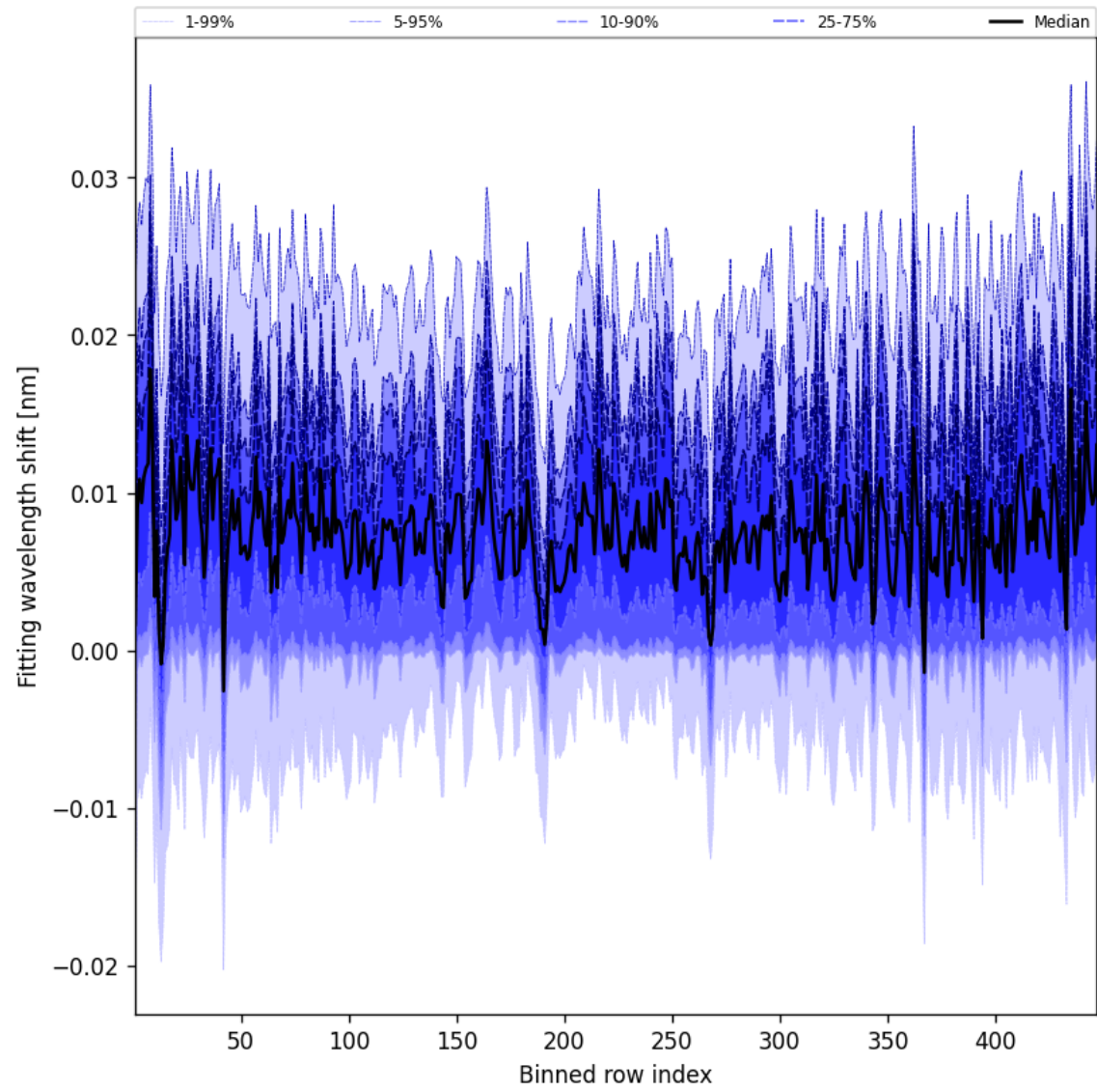
Figure 65: Along track statistics of “Fitting wavelength shift” for 2025-08-06 to 2025-08-08
