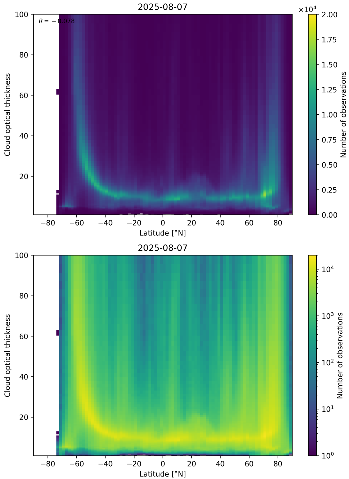
Figure 96: Scatter density plot of “Latitude” against “Cloud optical thickness” for 2025-08-06 to 2025-08-08.
