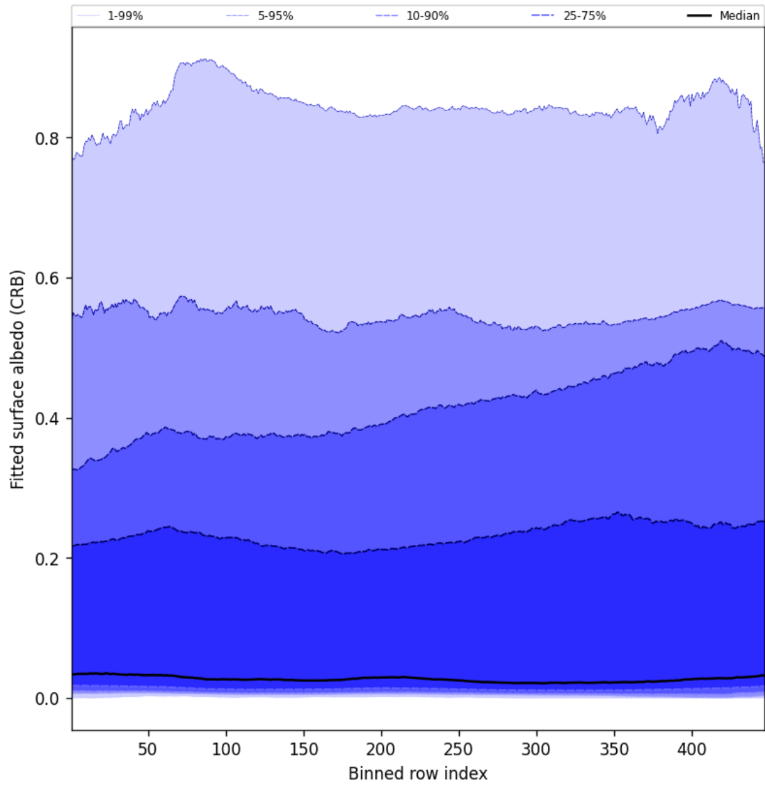
Figure 62: Along track statistics of “Fitted surface albedo (CRB)” for 2025-08-06 to 2025-08-08
