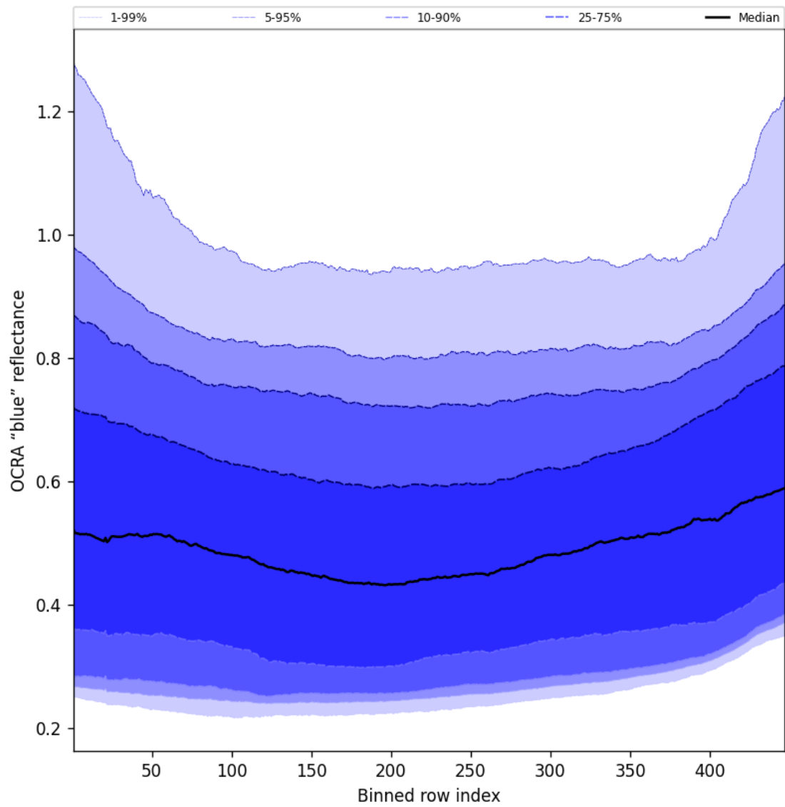
Figure 67: Along track statistics of “OCRA “blue” reflectance” for 2025-08-06 to 2025-08-08
