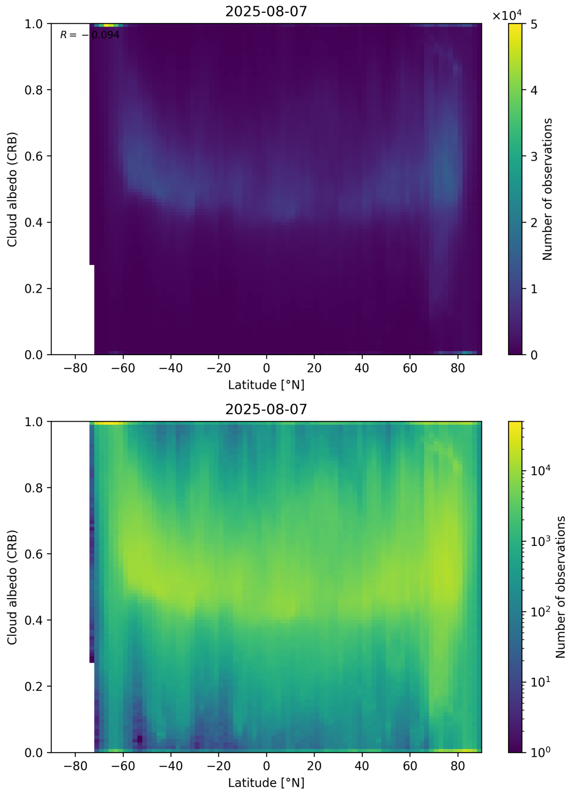
Figure 91: Scatter density plot of “Latitude” against “Cloud albedo (CRB)” for 2025-08-06 to 2025-08-08.
