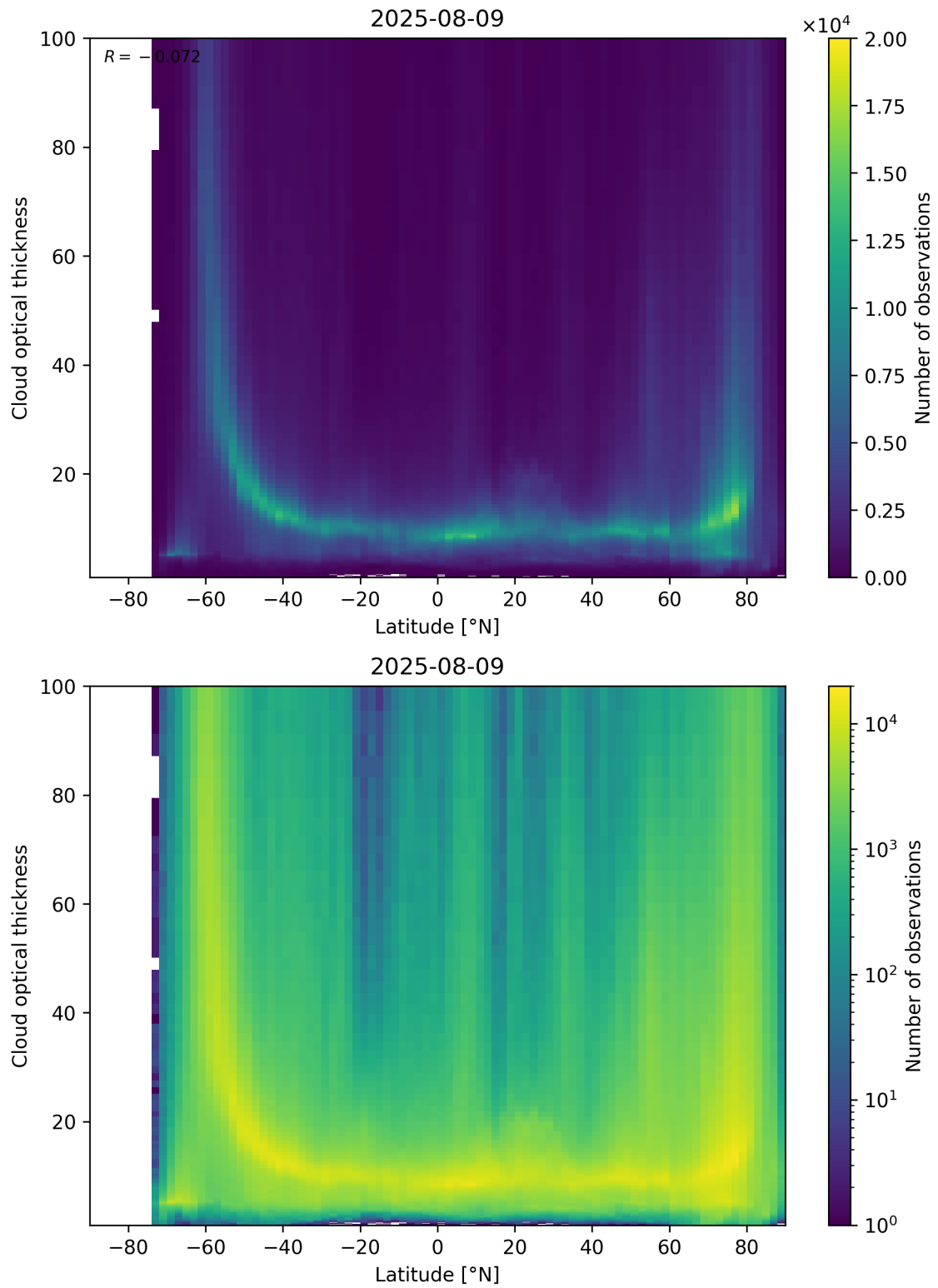
Figure 96: Scatter density plot of “Latitude” against “Cloud optical thickness” for 2025-08-09 to 2025-08-10.
