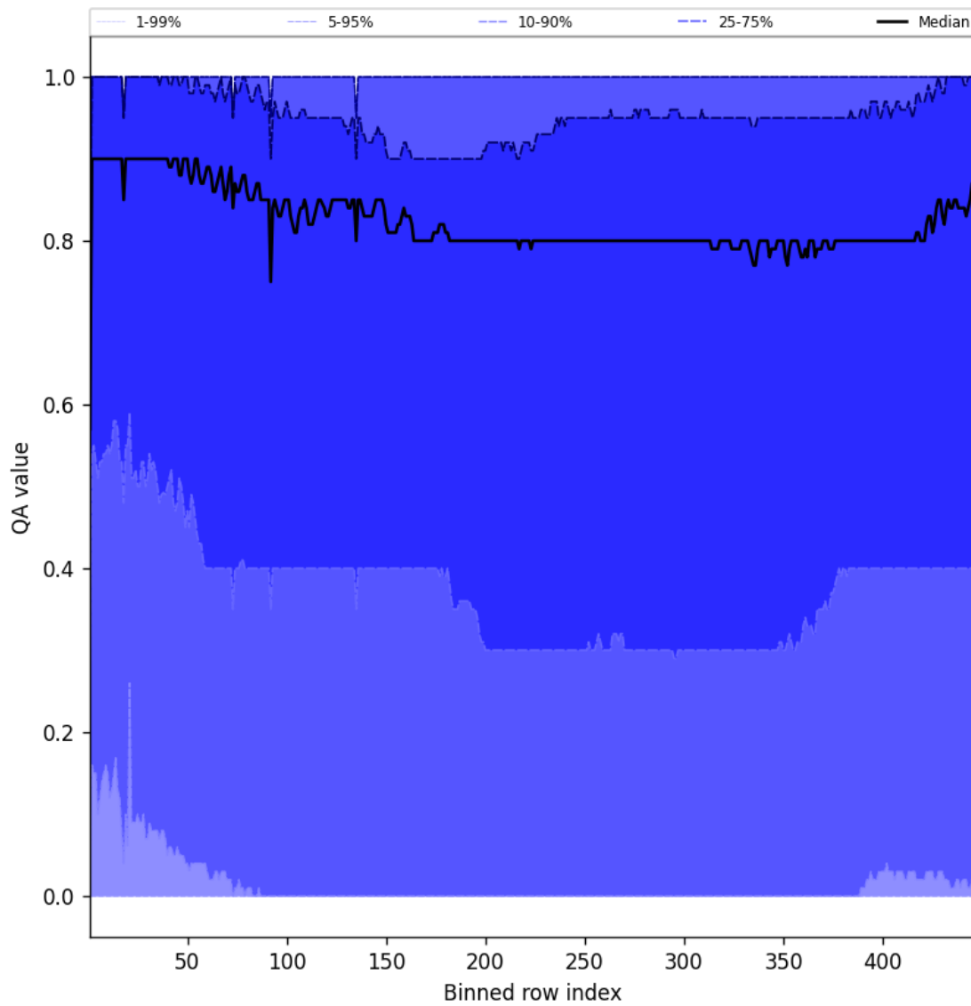
Figure 54: Along track statistics of “QA value” for 2025-08-09 to 2025-08-10
