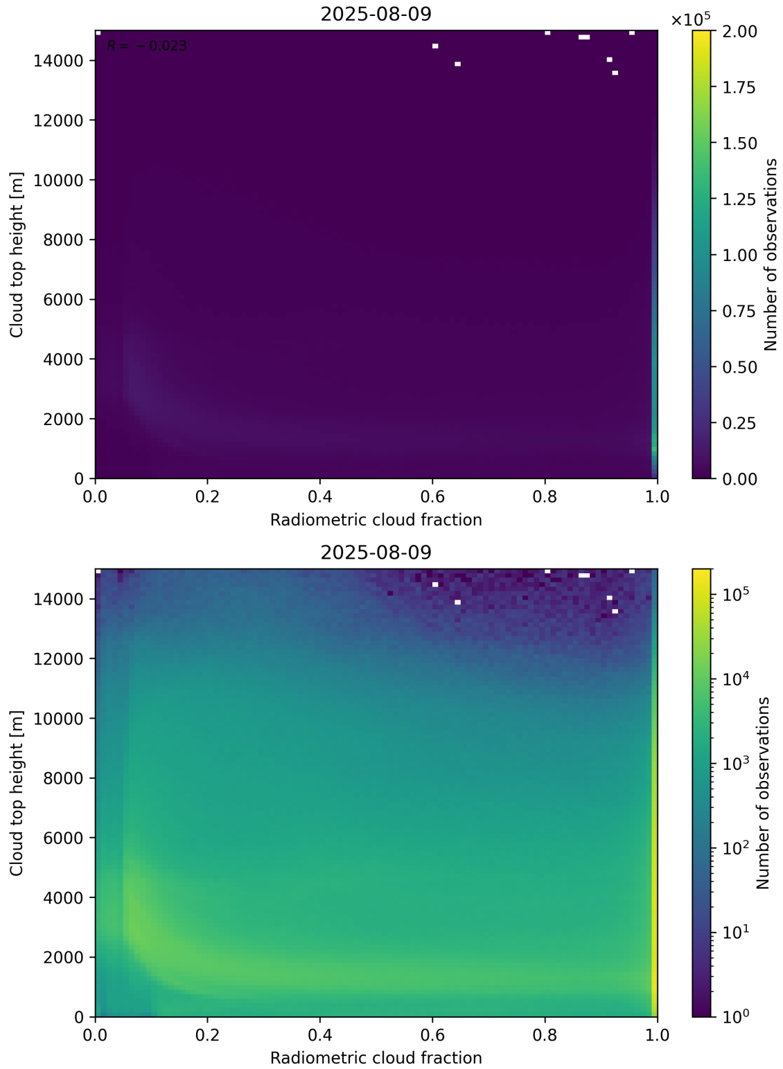
Figure 76: Scatter density plot of “Radiometric cloud fraction” against “Cloud top height” for 2025-08-09 to 2025-08-10.
