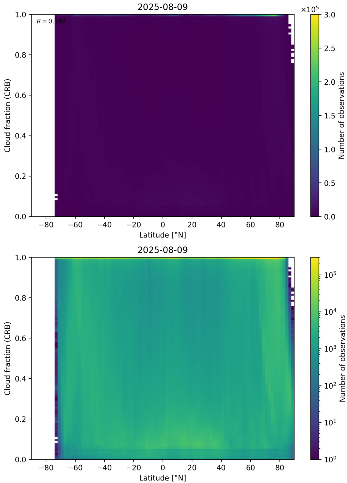
Figure 94: Scatter density plot of “Latitude” against “Cloud fraction (CRB)” for 2025-08-09 to 2025-08-10.
