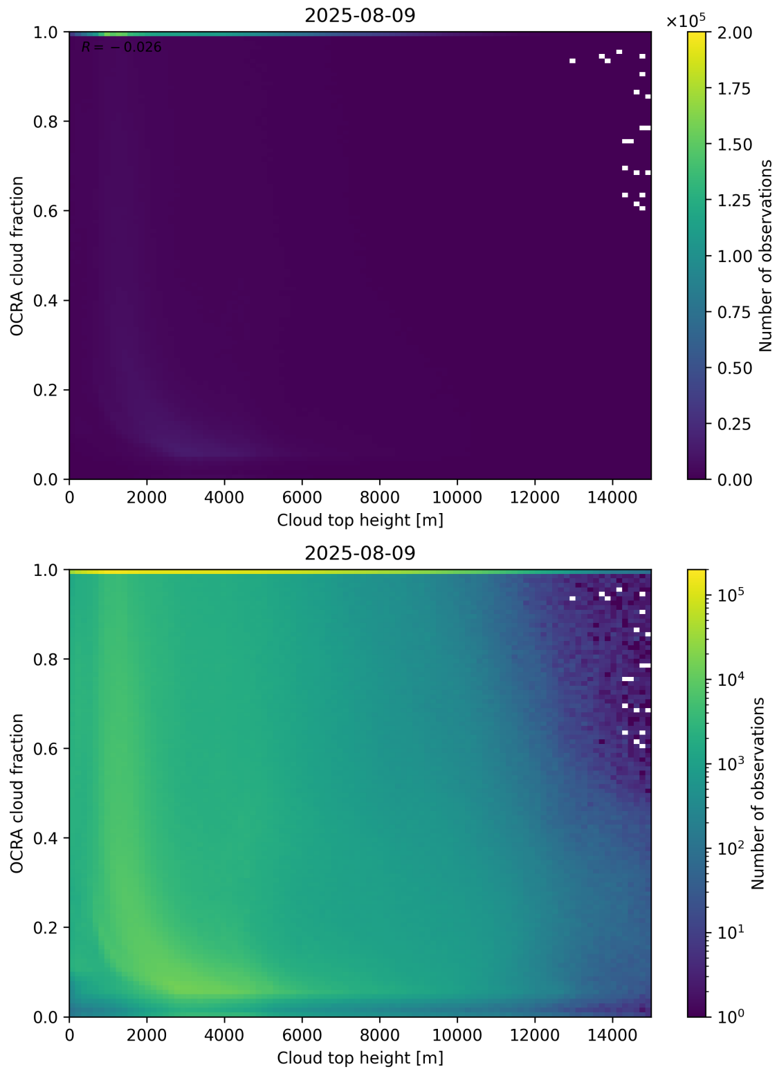
Figure 87: Scatter density plot of “Cloud top height” against “OCRA cloud fraction” for 2025-08-09 to 2025-08-10.
