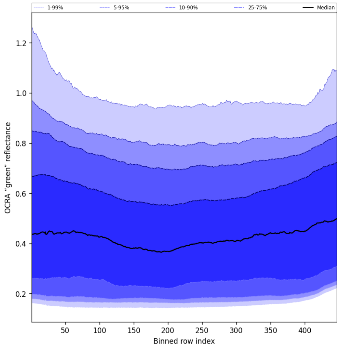
Figure 68: Along track statistics of “OCRA “green” reflectance” for 2025-08-09 to 2025-08-10
