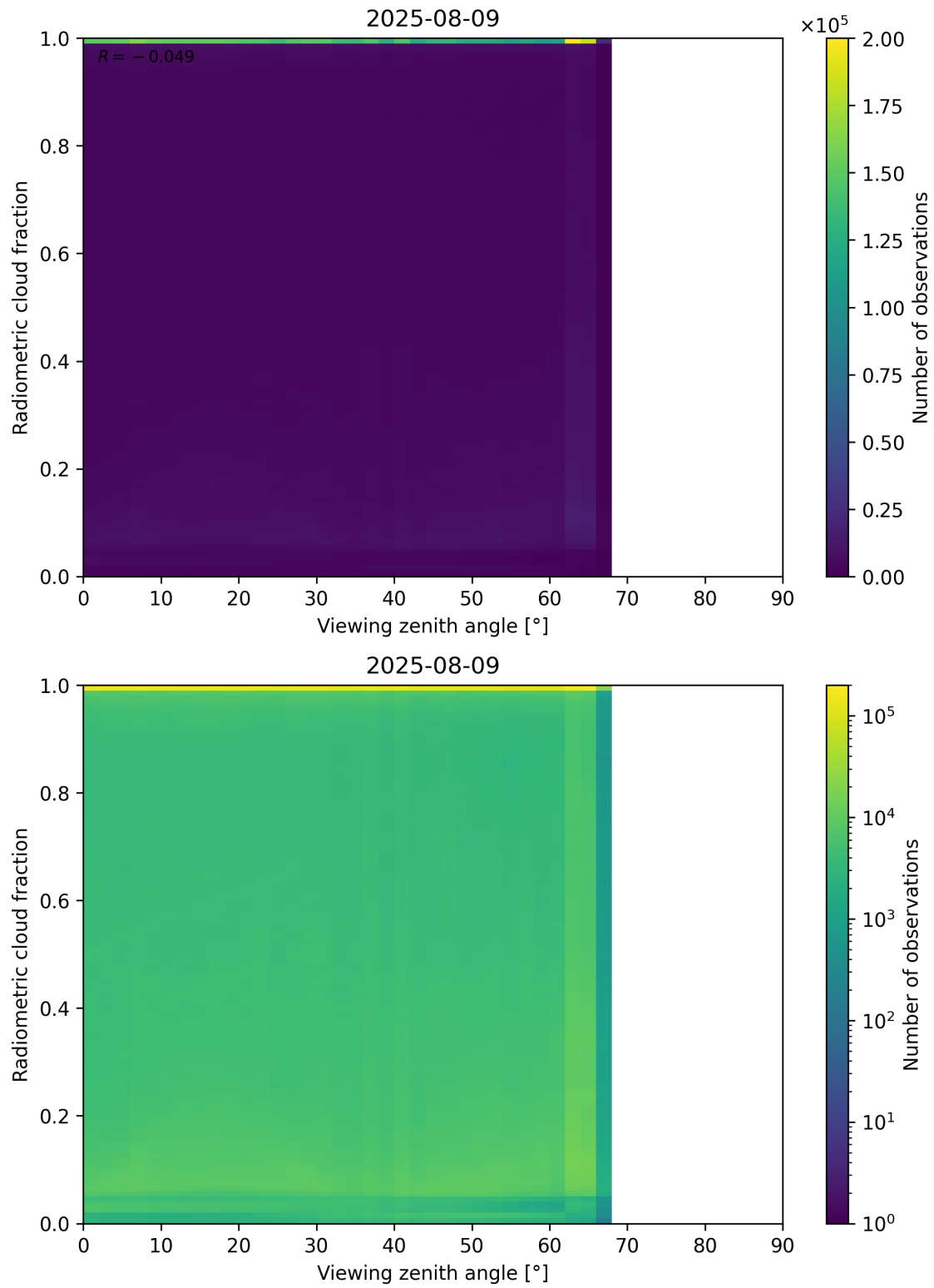
Figure 107: Scatter density plot of “Viewing zenith angle” against “Radiometric cloud fraction” for 2025-08-09 to 2025-08-10.
