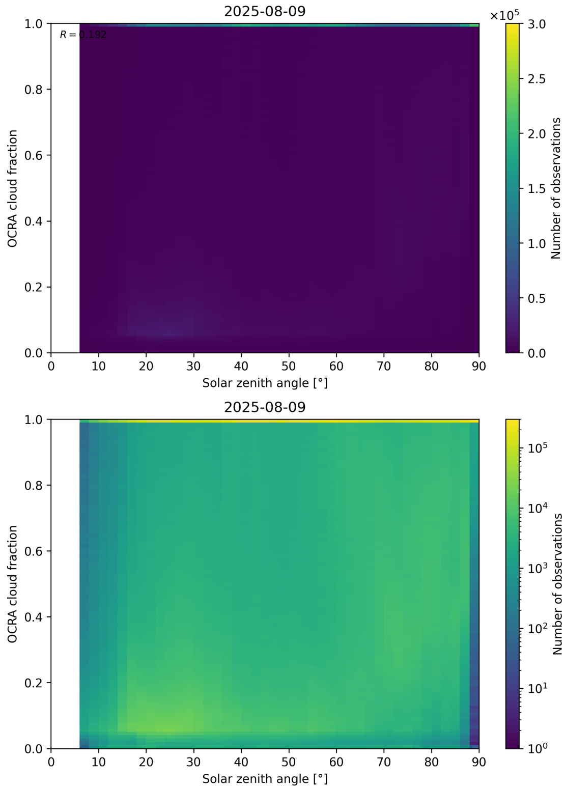
Figure 100: Scatter density plot of “Solar zenith angle” against “OCRA cloud fraction” for 2025-08-09 to 2025-08-10.
