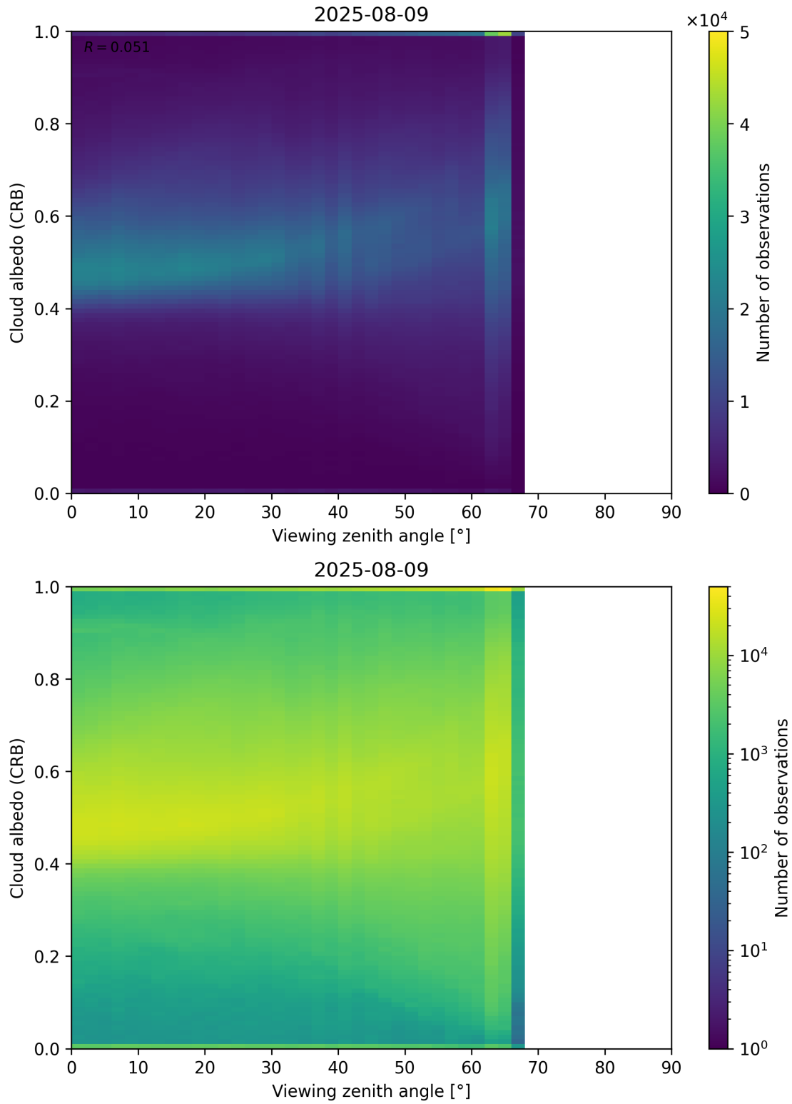
Figure 106: Scatter density plot of “Viewing zenith angle” against “Cloud albedo (CRB)” for 2025-08-09 to 2025-08-10.
