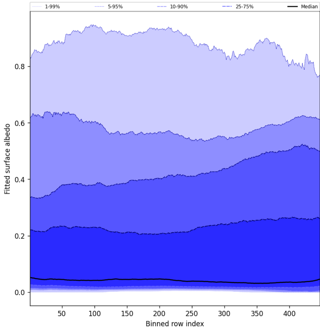
Figure 61: Along track statistics of “Fitted surface albedo” for 2025-08-09 to 2025-08-10
