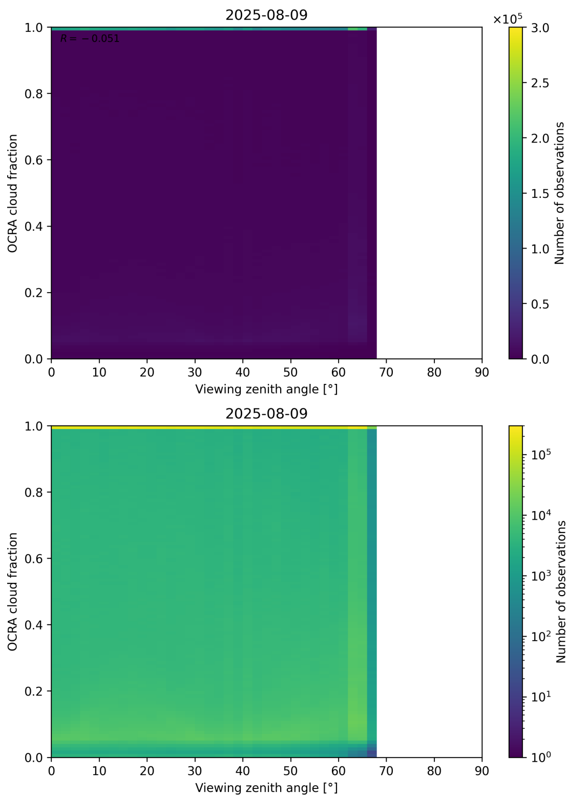
Figure 108: Scatter density plot of “Viewing zenith angle” against “OCRA cloud fraction” for 2025-08-09 to 2025-08-10.
