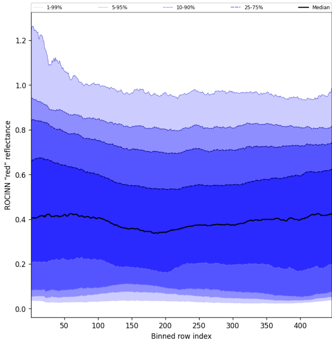
Figure 69: Along track statistics of “ROCINN “red” reflectance” for 2025-08-09 to 2025-08-10
