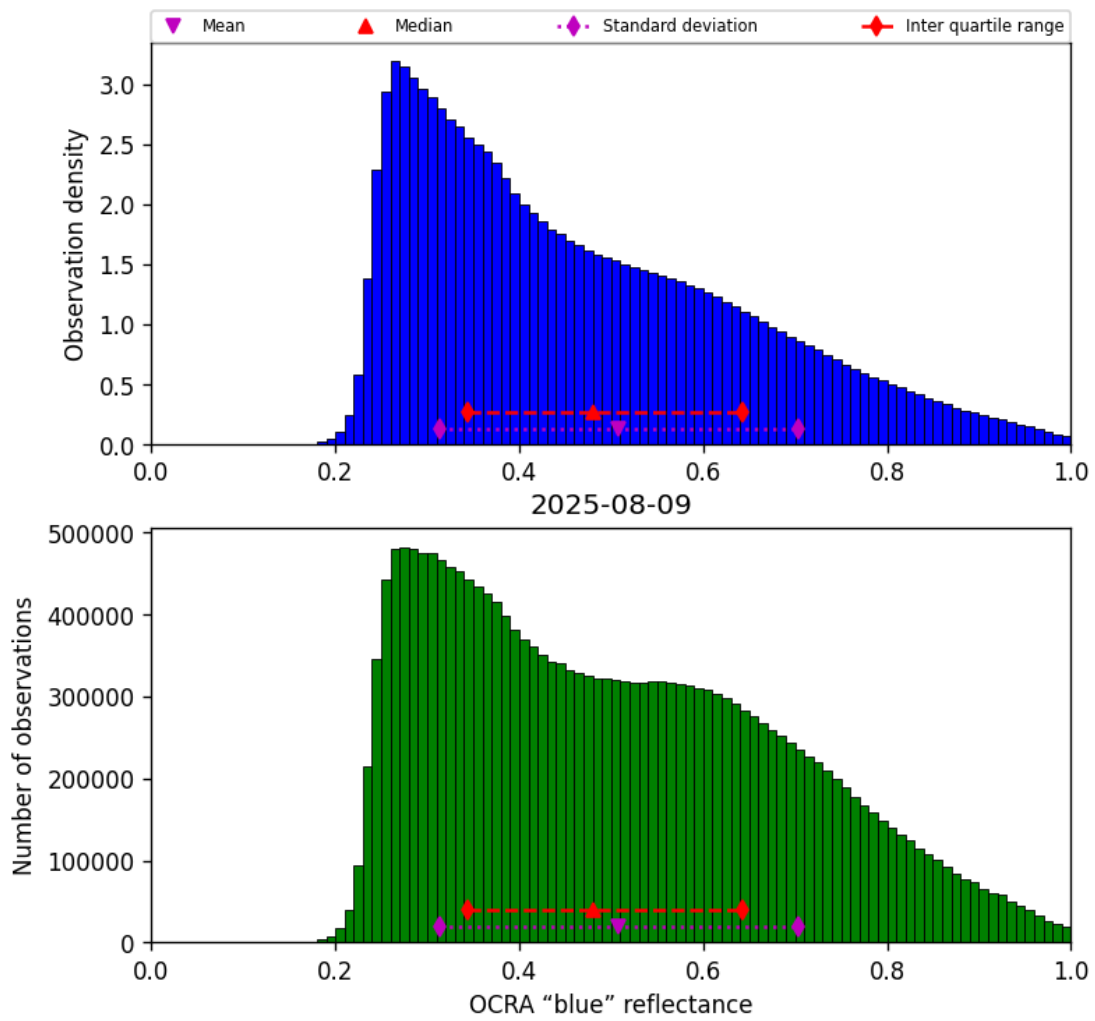
Figure 51: Histogram of “OCRA “blue” reflectance” for 2025-08-09 to 2025-08-10
