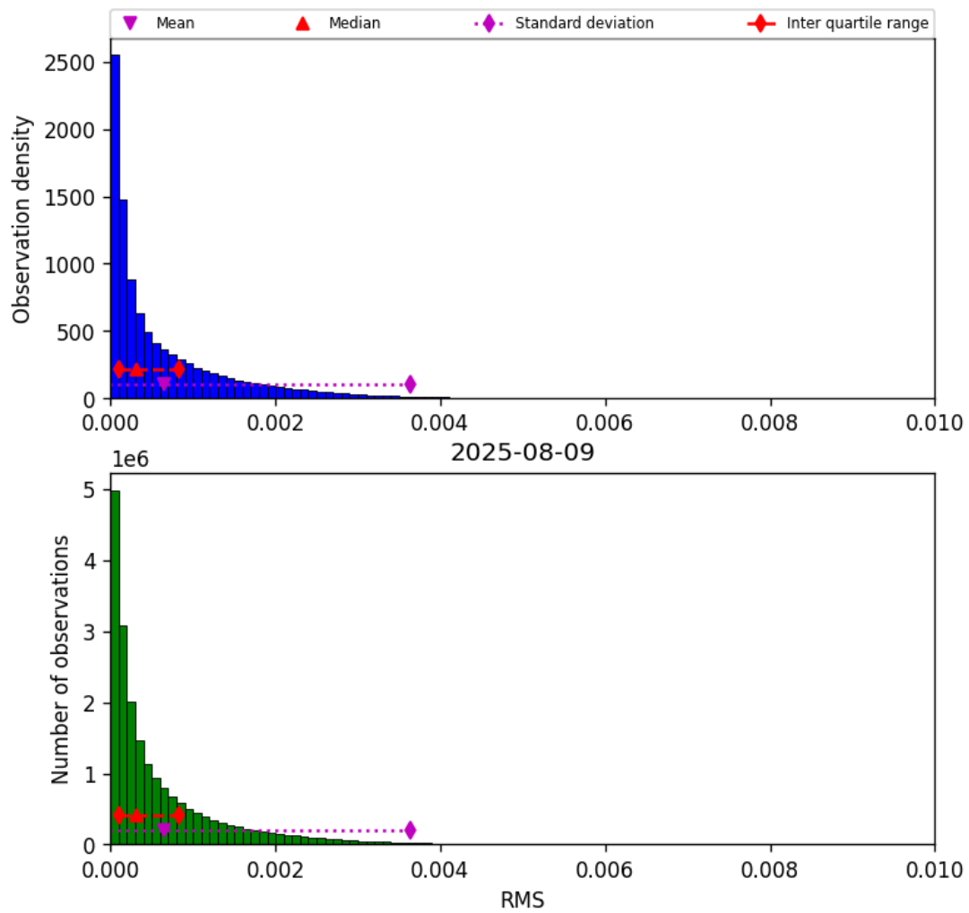
Figure 47: Histogram of “RMS” for 2025-08-09 to 2025-08-10
