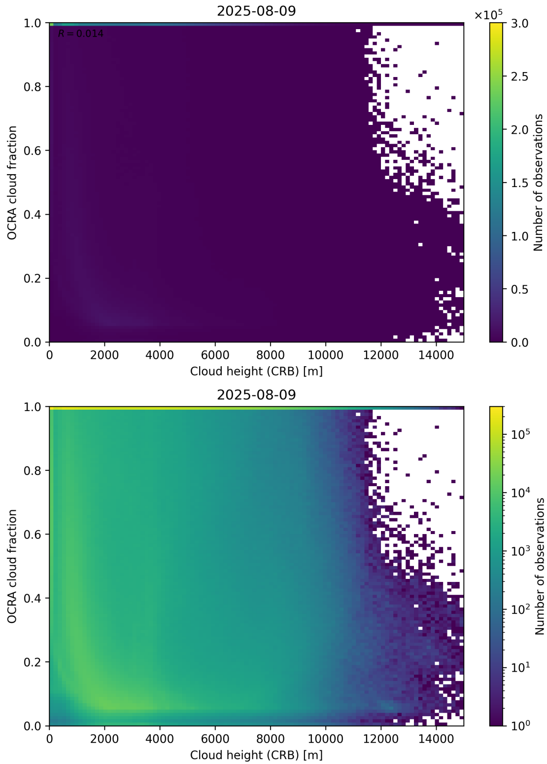
Figure 81: Scatter density plot of “Cloud height (CRB)” against “OCRA cloud fraction” for 2025-08-09 to 2025-08-10.
