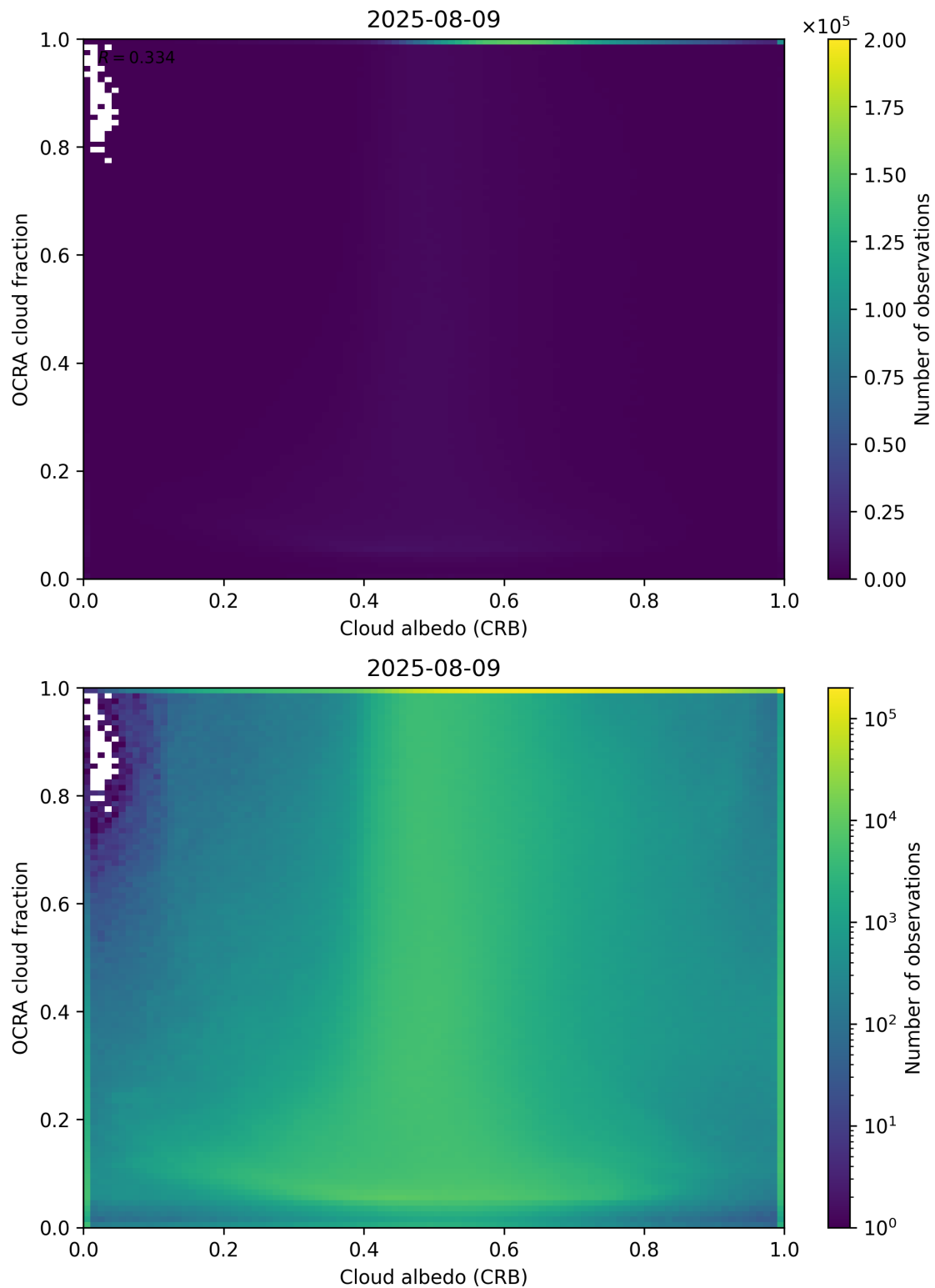
Figure 70: Scatter density plot of “Cloud albedo (CRB)” against “OCRA cloud fraction” for 2025-08-09 to 2025-08-10.
