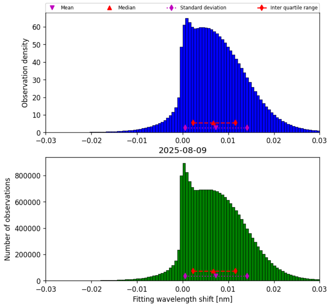
Figure 49: Histogram of “Fitting wavelength shift” for 2025-08-09 to 2025-08-10
