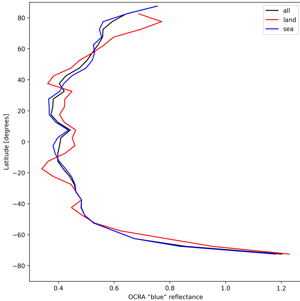
Figure 35: Zonal average of "OCRA "blue" reflectance" for 2025-08-09 to 2025-08-10.
