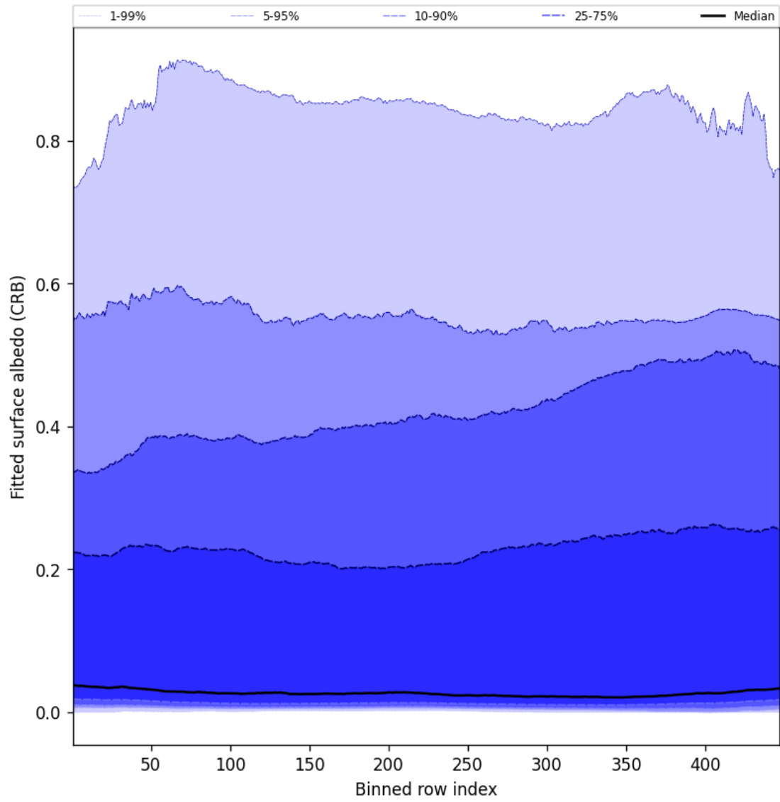
Figure 62: Along track statistics of “Fitted surface albedo (CRB)” for 2025-08-09 to 2025-08-10
