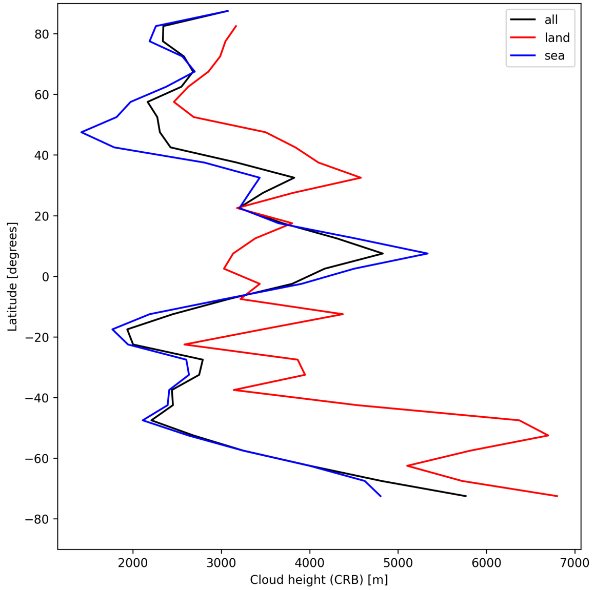
Figure 27: Zonal average of “Cloud height (CRB)” for 2025-08-09 to 2025-08-10.
