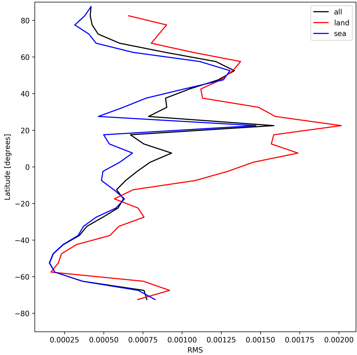
Figure 31: Zonal average of “RMS” for 2025-08-09 to 2025-08-10.
