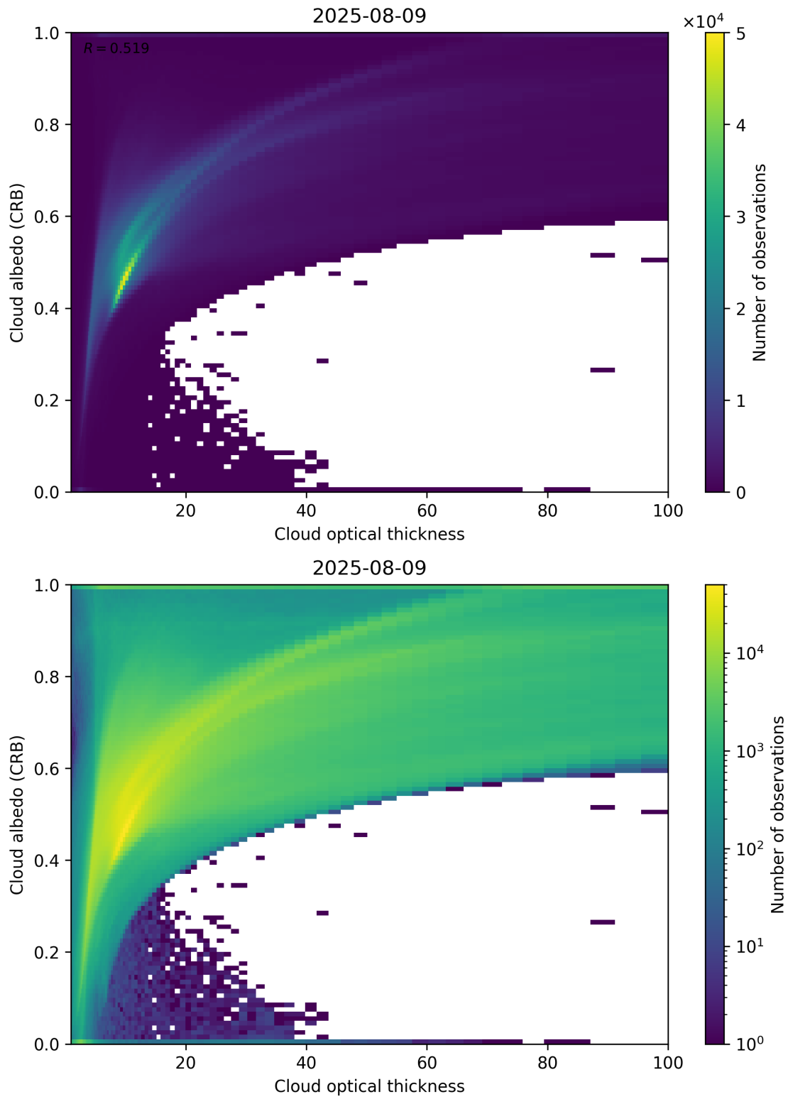
Figure 82: Scatter density plot of “Cloud optical thickness” against “Cloud albedo (CRB)” for 2025-08-09 to 2025-08-10.
