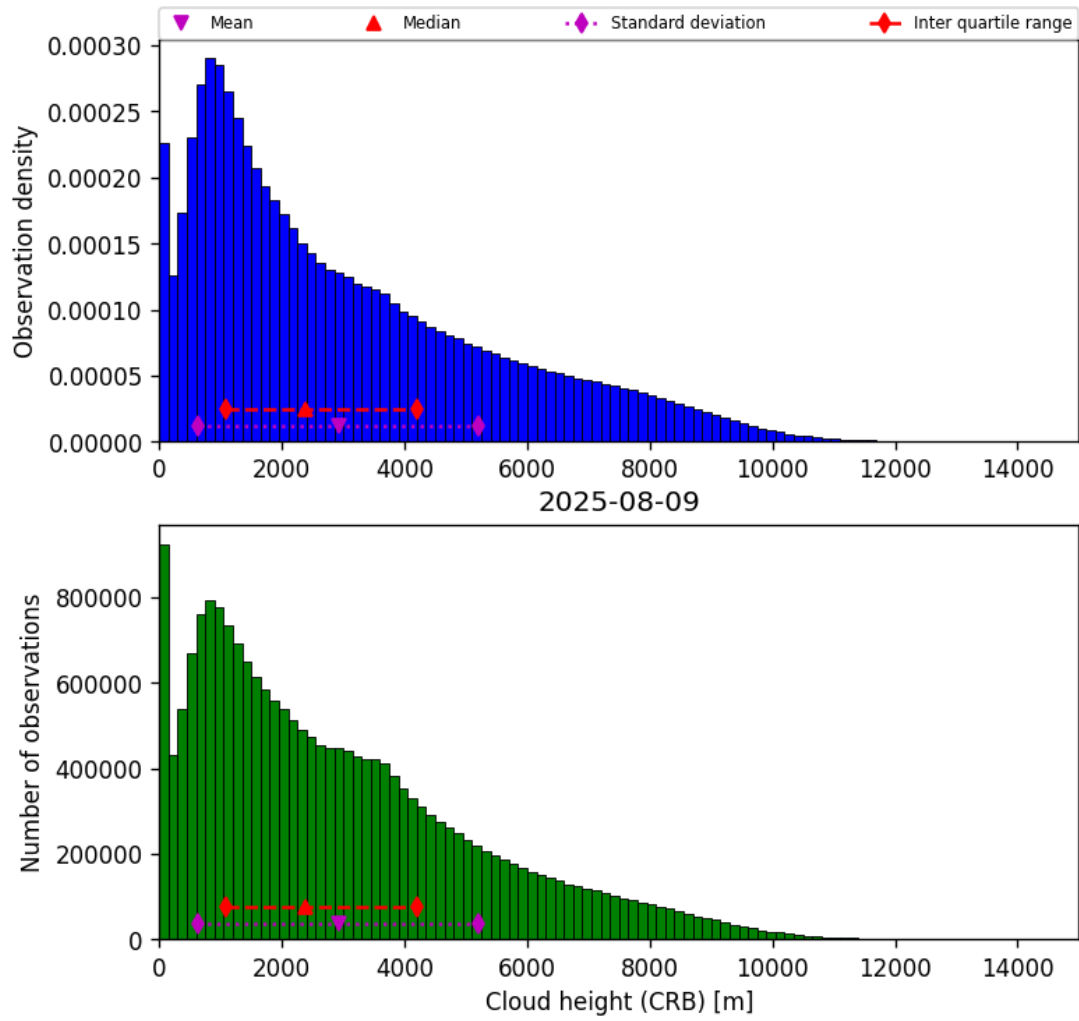
Figure 43: Histogram of “Cloud height (CRB)” for 2025-08-09 to 2025-08-10
