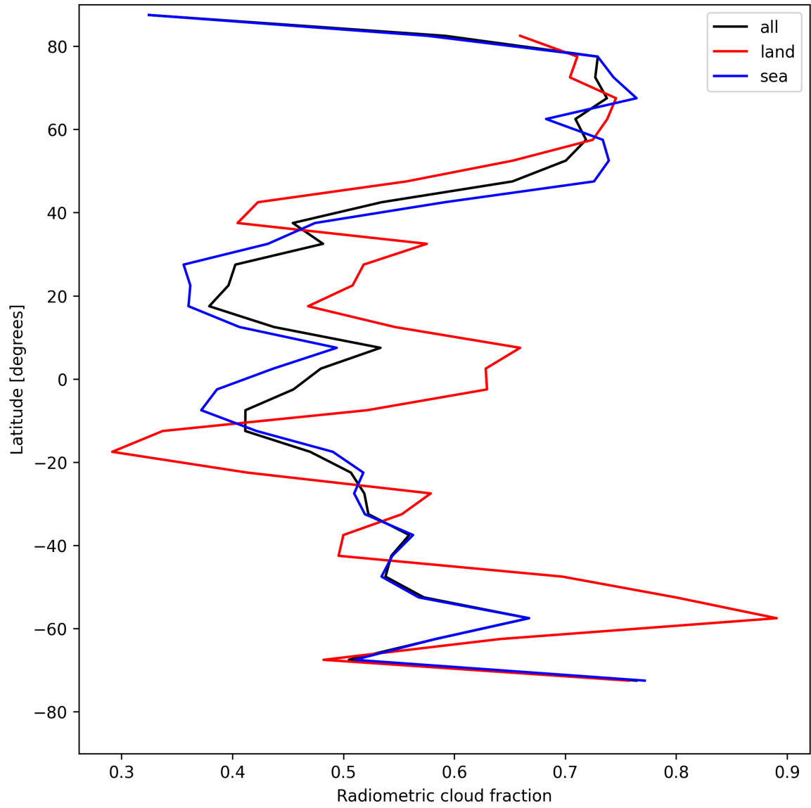
Figure 23: Zonal average of “Radiometric cloud fraction” for 2025-08-09 to 2025-08-10.
