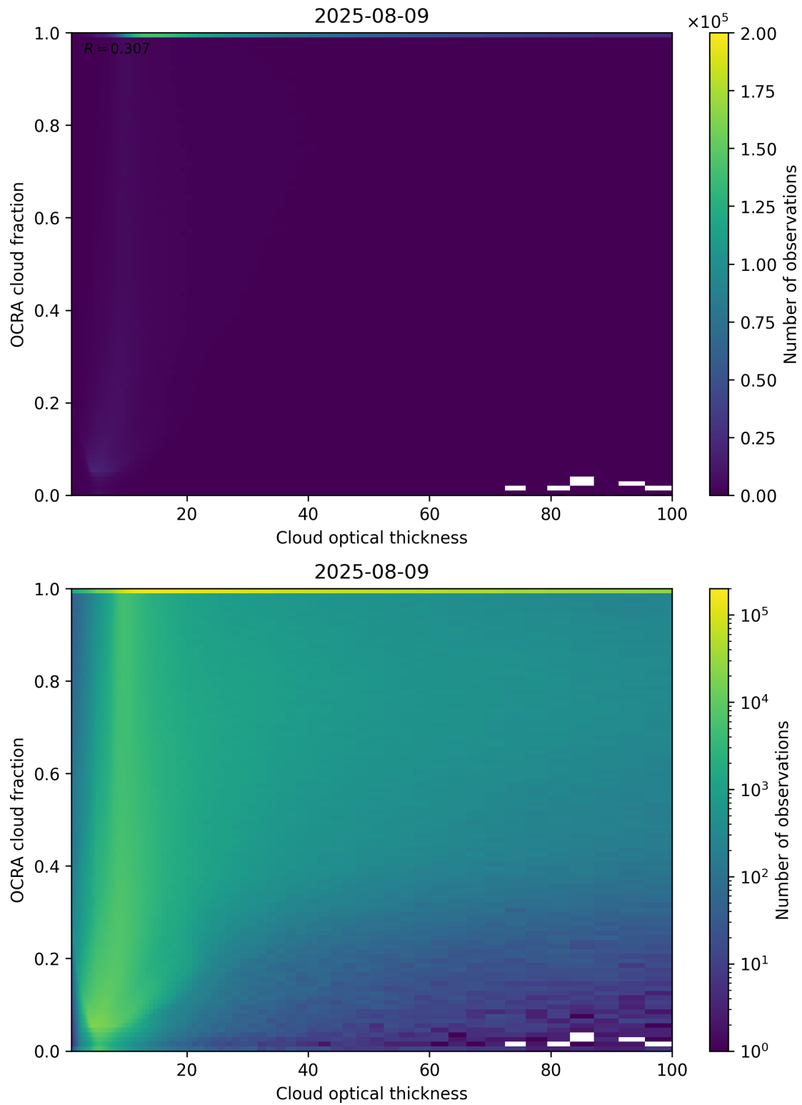
Figure 83: Scatter density plot of “Cloud optical thickness” against “OCRA cloud fraction” for 2025-08-09 to 2025-08-10.
