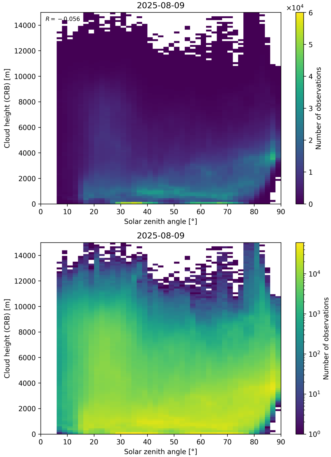
Figure 102: Scatter density plot of “Solar zenith angle” against “Cloud height (CRB)” for 2025-08-09 to 2025-08-10.
