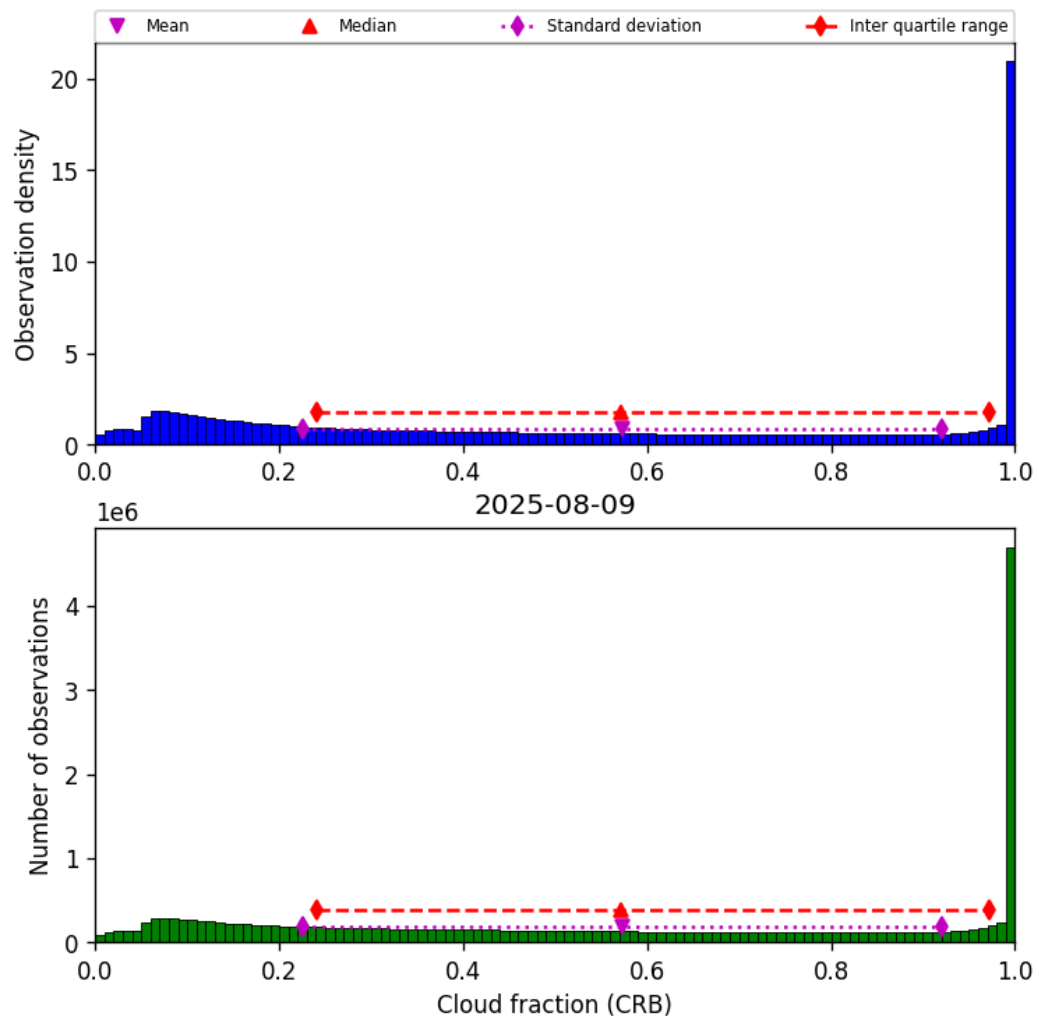
Figure 42: Histogram of “Cloud fraction (CRB)” for 2025-08-09 to 2025-08-10
