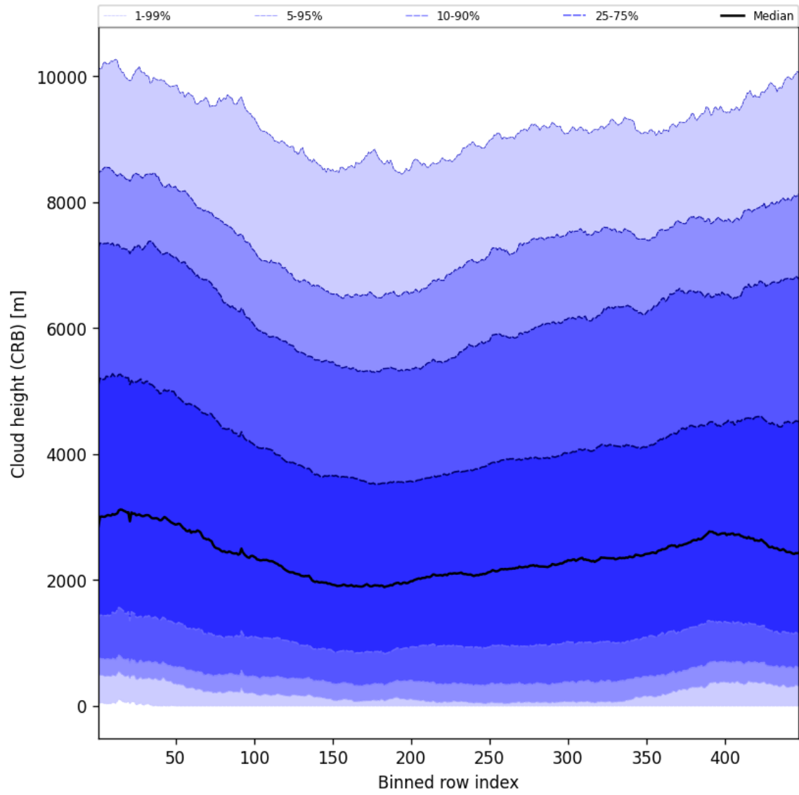
Figure 59: Along track statistics of “Cloud height (CRB)” for 2025-08-09 to 2025-08-10
