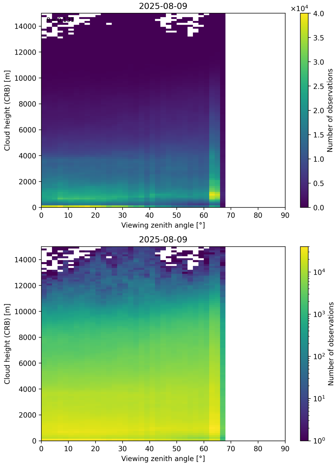
Figure 110: Scatter density plot of “Viewing zenith angle” against “Cloud height (CRB)” for 2025-08-09 to 2025-08-10.
