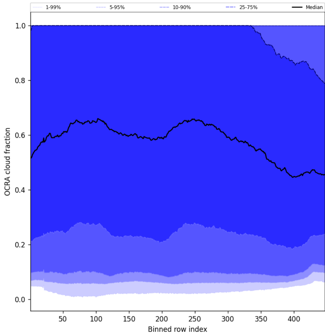
Figure 66: Along track statistics of “OCRA cloud fraction” for 2025-08-09 to 2025-08-10
