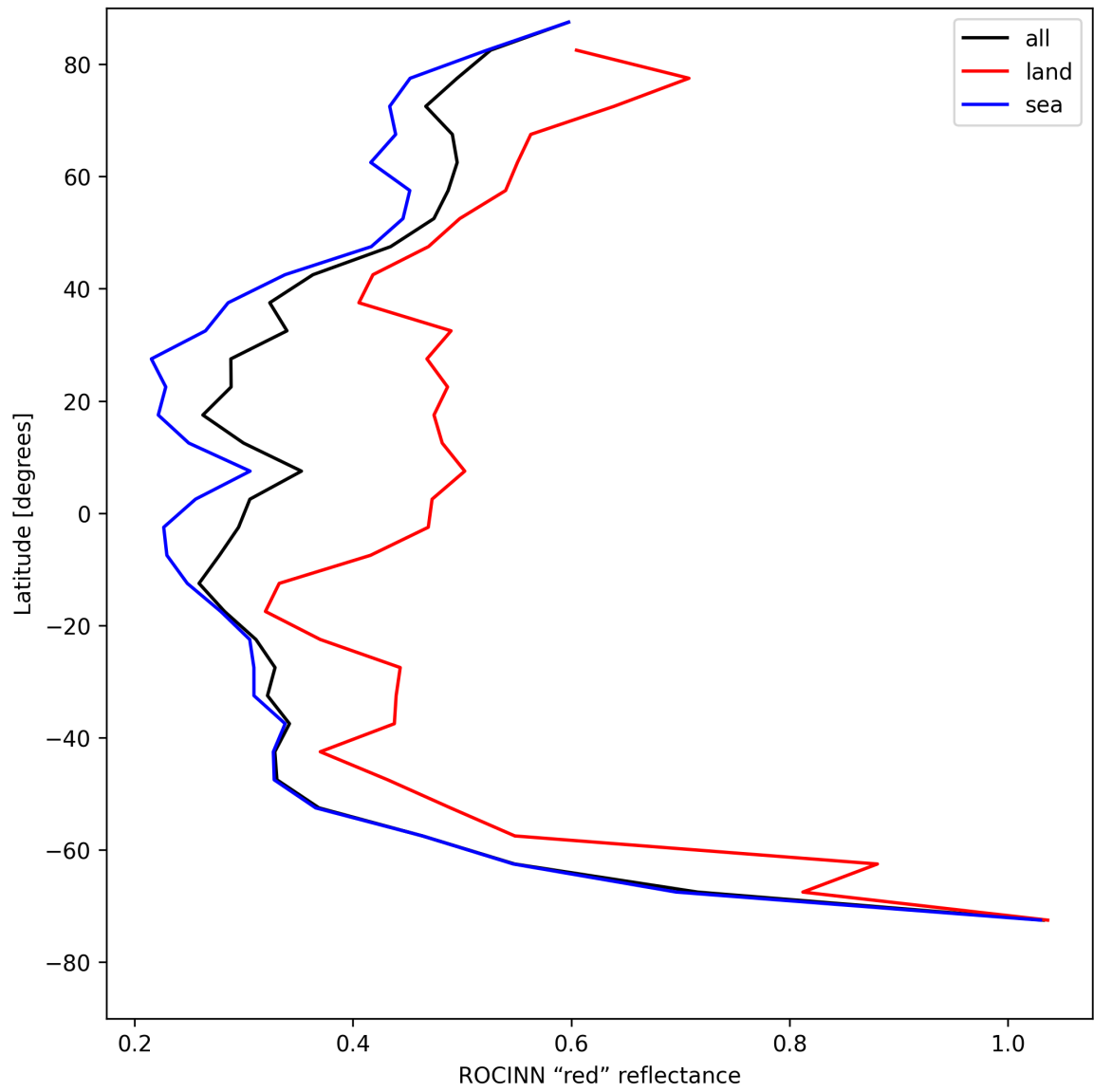
Figure 37: Zonal average of “ROCINN “red” reflectance” for 2025-08-09 to 2025-08-10.
