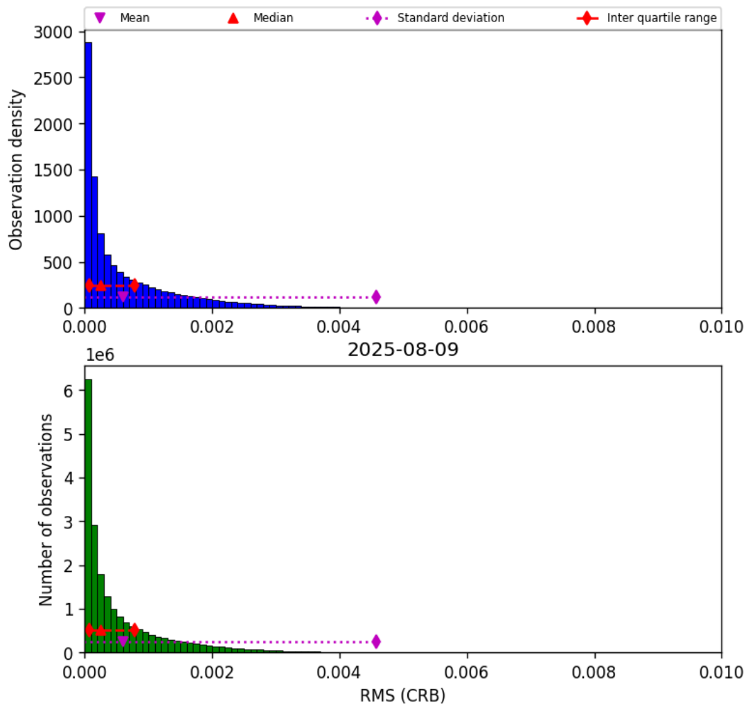
Figure 48: Histogram of “RMS (CRB)” for 2025-08-09 to 2025-08-10
