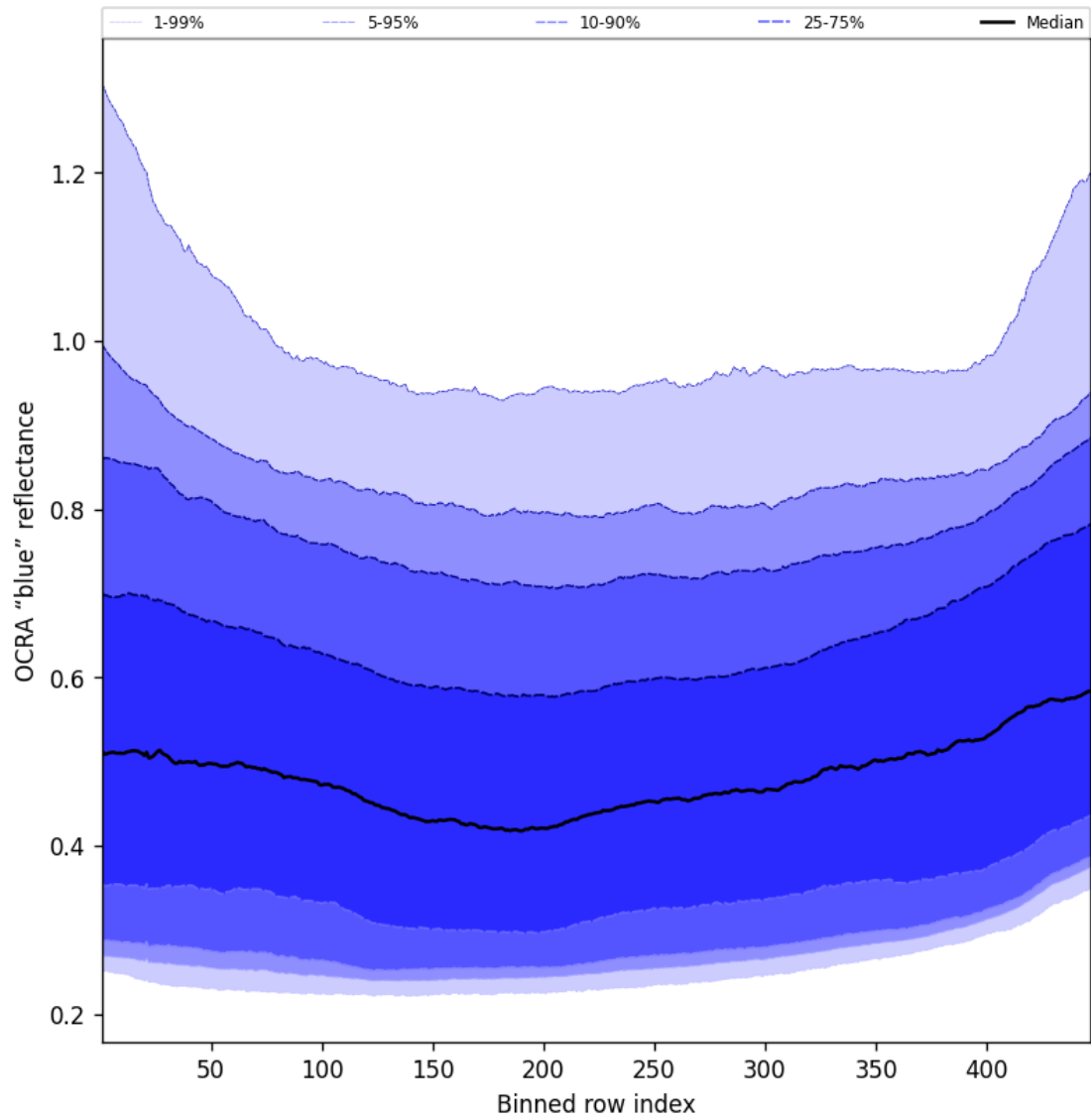
Figure 67: Along track statistics of “OCRA “blue” reflectance” for 2025-08-09 to 2025-08-10
