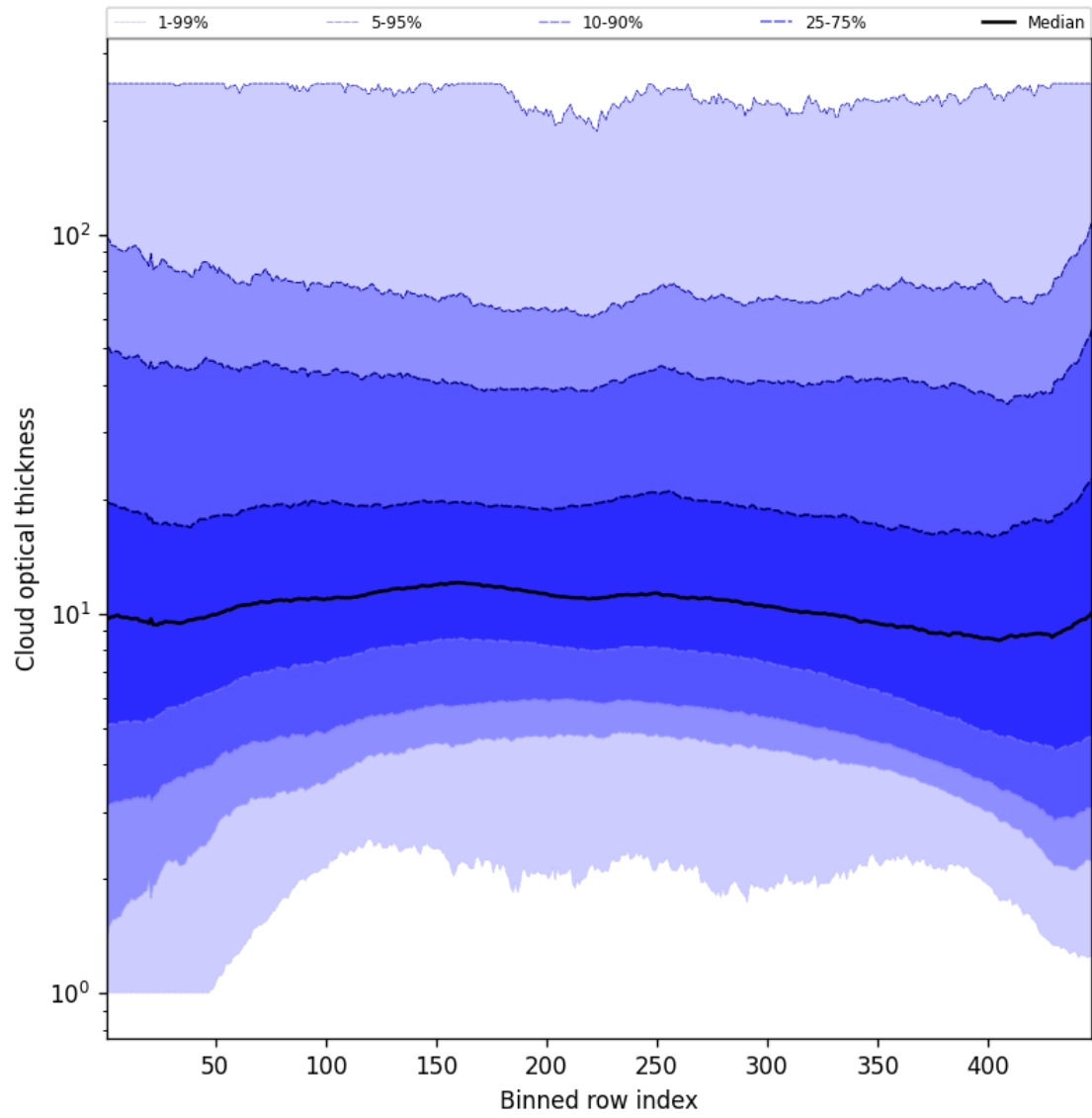
Figure 57: Along track statistics of “Cloud optical thickness” for 2025-08-09 to 2025-08-10
