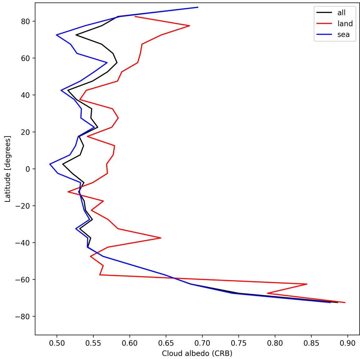
Figure 28: Zonal average of “Cloud albedo (CRB)” for 2025-08-09 to 2025-08-10.
