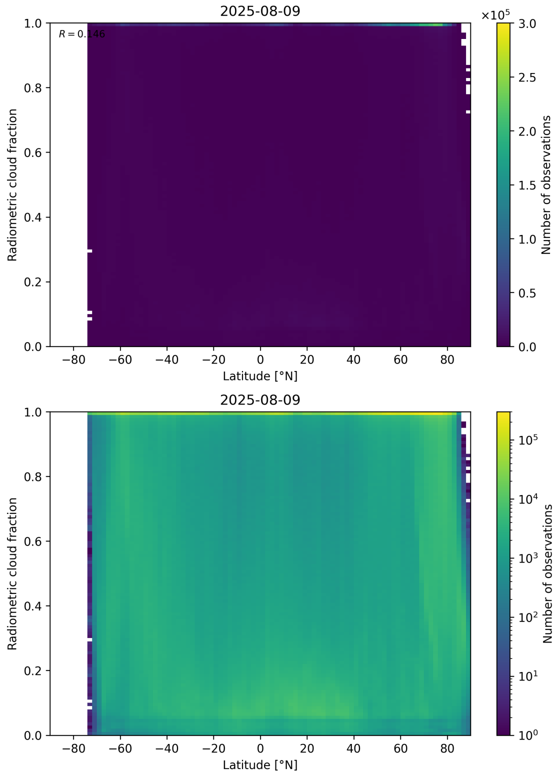
Figure 92: Scatter density plot of “Latitude” against “Radiometric cloud fraction” for 2025-08-09 to 2025-08-10.
