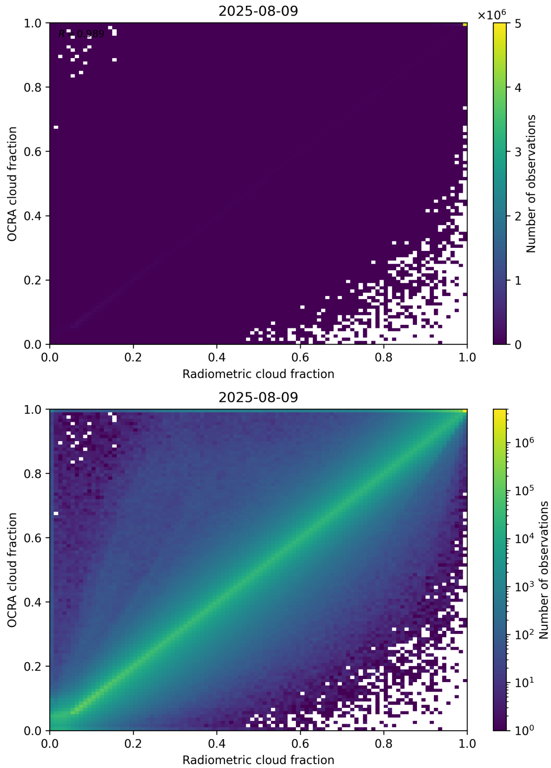
Figure 72: Scatter density plot of “Radiometric cloud fraction” against “OCRA cloud fraction” for 2025-08-09 to 2025-08-10.
