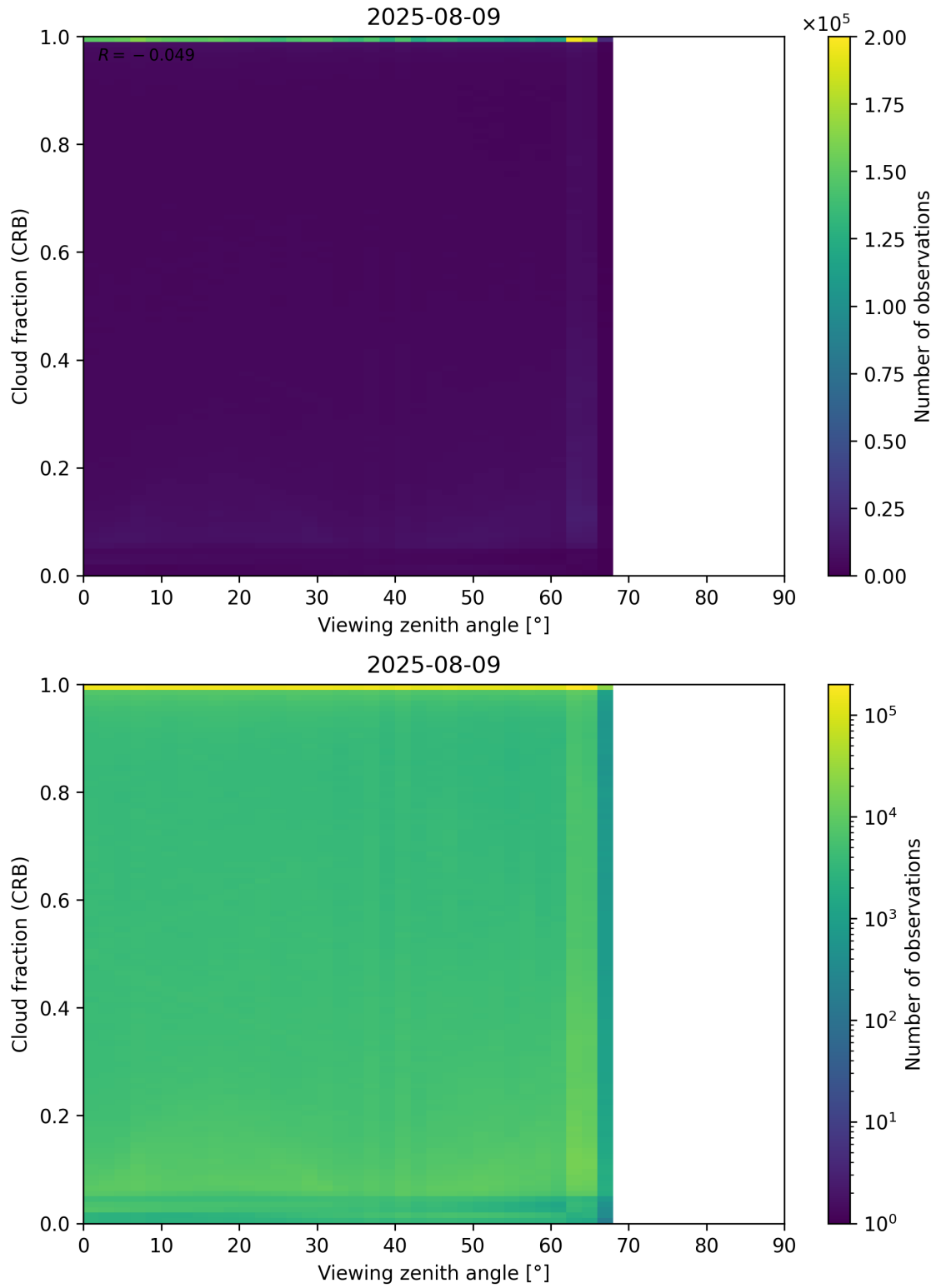
Figure 109: Scatter density plot of “Viewing zenith angle” against “Cloud fraction (CRB)” for 2025-08-09 to 2025-08-10.
