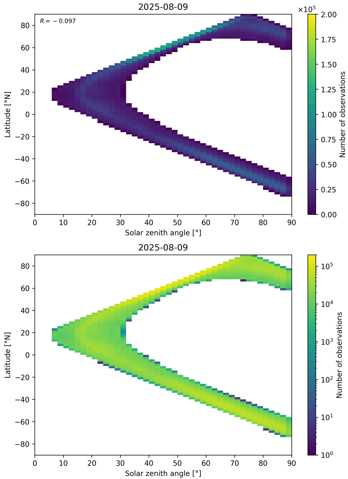
Figure 105: Scatter density plot of “Solar zenith angle” against “Latitude” for 2025-08-09 to 2025-08-10.
