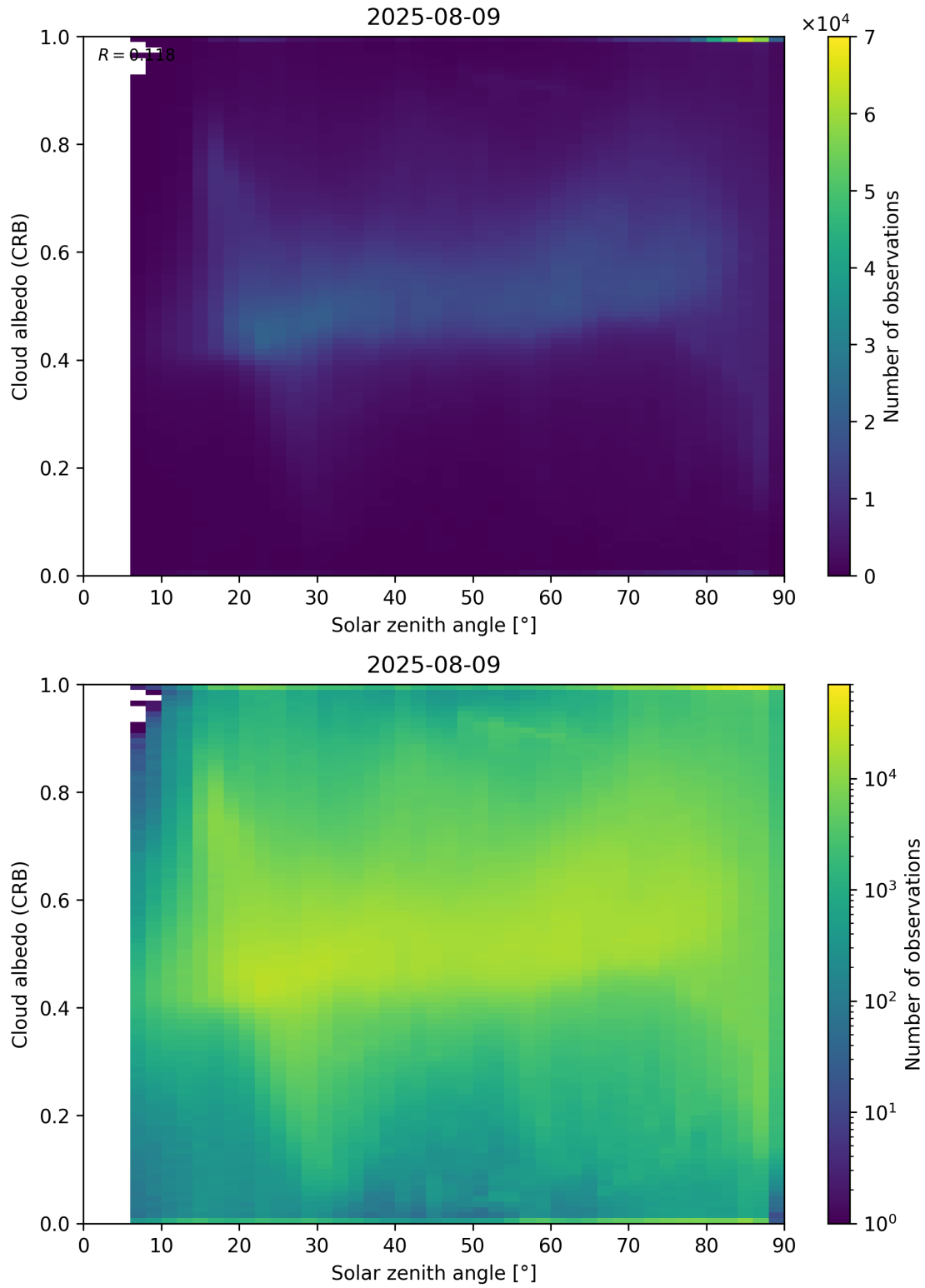
Figure 98: Scatter density plot of “Solar zenith angle” against “Cloud albedo (CRB)” for 2025-08-09 to 2025-08-10.
