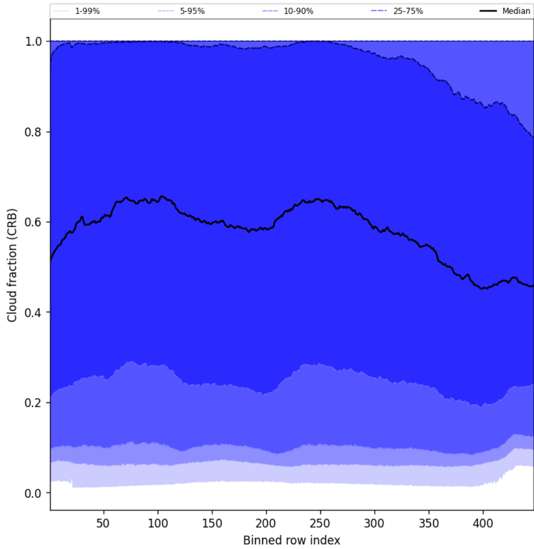
Figure 58: Along track statistics of “Cloud fraction (CRB)” for 2025-08-09 to 2025-08-10
