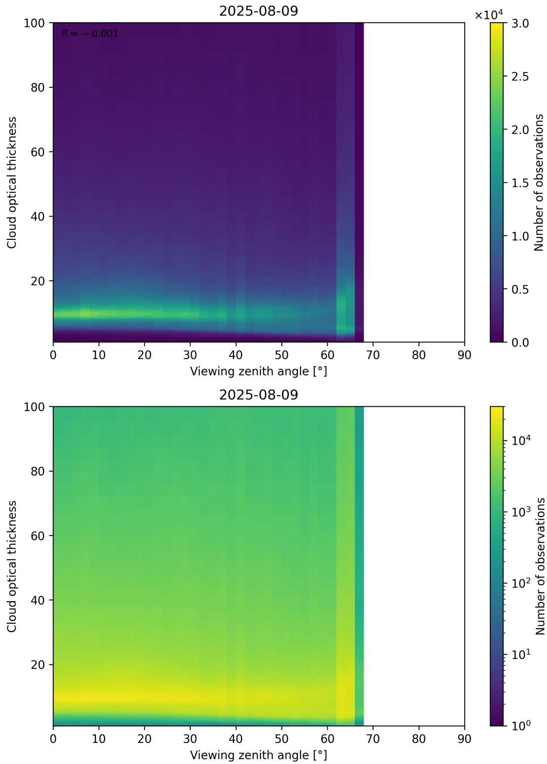
Figure 111: Scatter density plot of “Viewing zenith angle” against “Cloud optical thickness” for 2025-08-09 to 2025-08-10.
