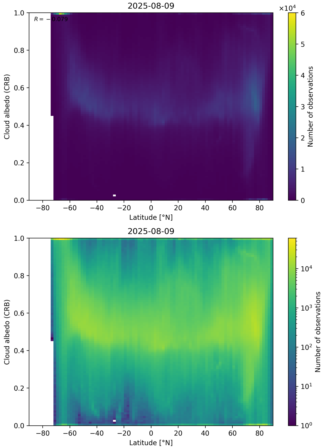
Figure 91: Scatter density plot of “Latitude” against “Cloud albedo (CRB)” for 2025-08-09 to 2025-08-10.
