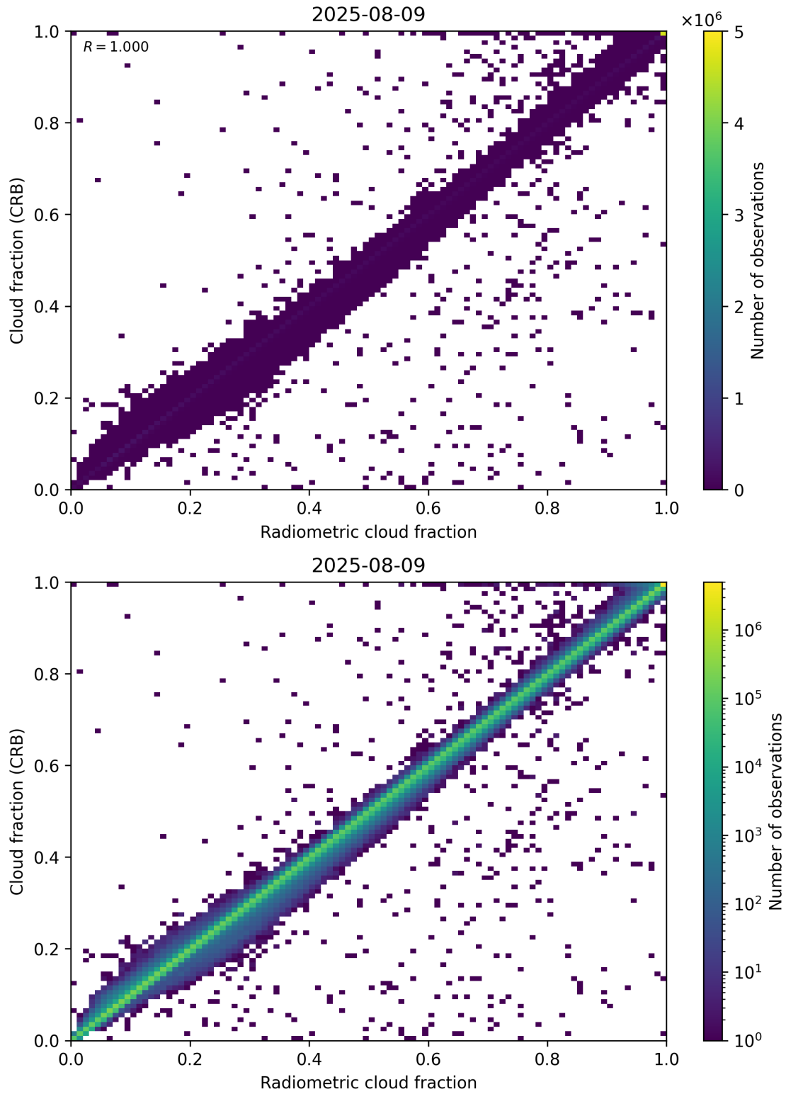
Figure 73: Scatter density plot of “Radiometric cloud fraction” against “Cloud fraction (CRB)” for 2025-08-09 to 2025-08-10.
