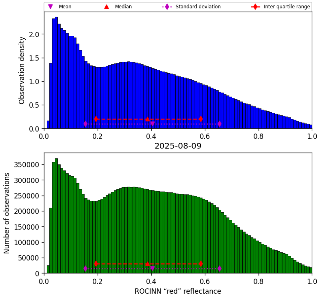
Figure 53: Histogram of “ROCINN “red” reflectance” for 2025-08-09 to 2025-08-10
