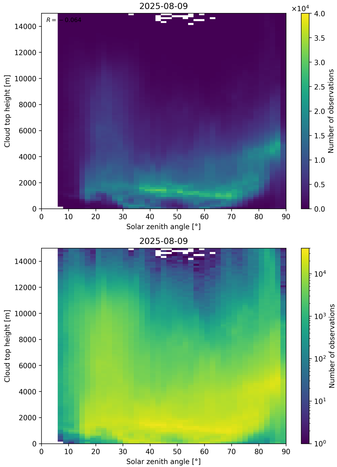
Figure 104: Scatter density plot of “Solar zenith angle” against “Cloud top height” for 2025-08-09 to 2025-08-10.
