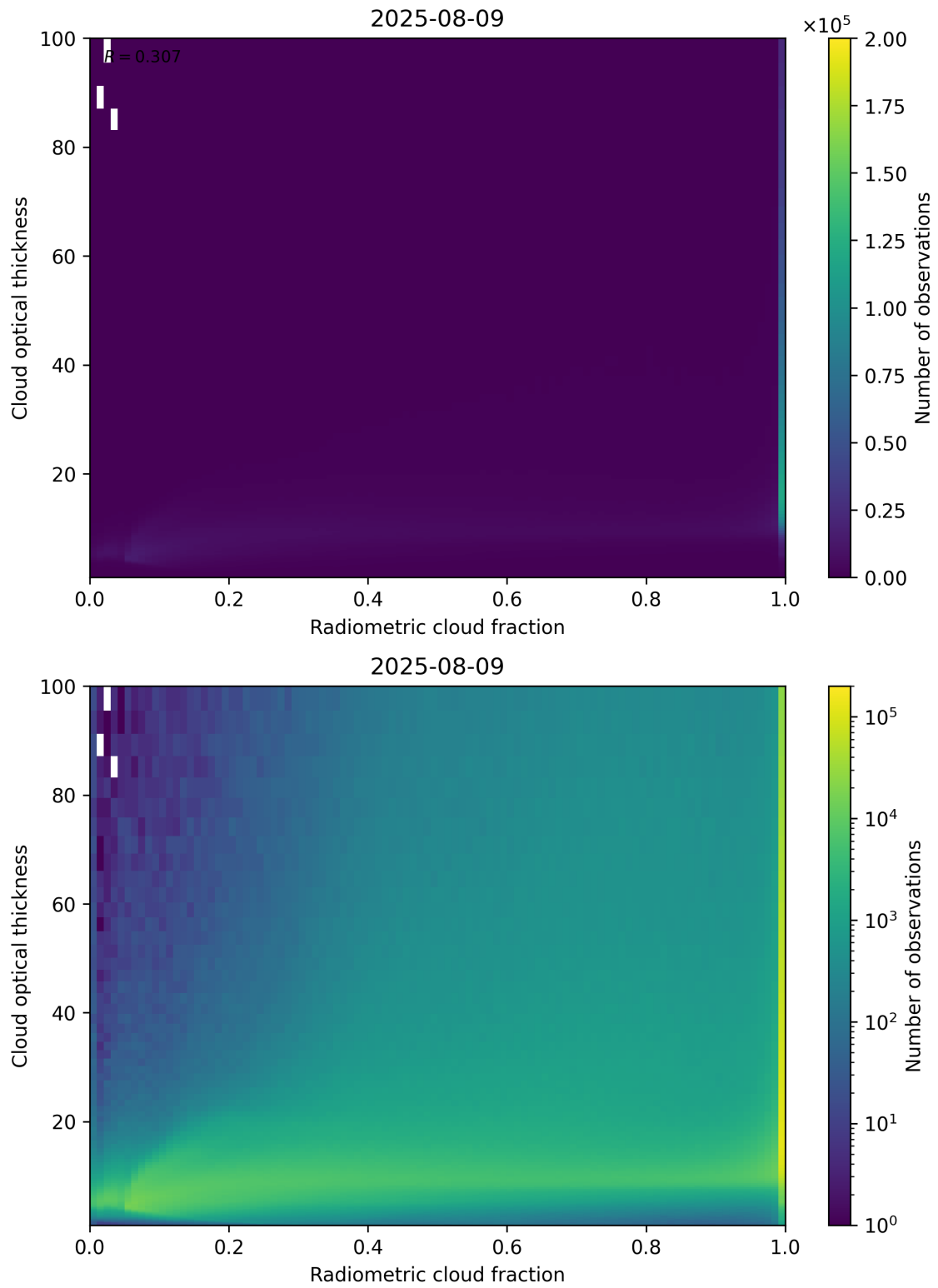
Figure 75: Scatter density plot of “Radiometric cloud fraction” against “Cloud optical thickness” for 2025-08-09 to 2025-08-10.
