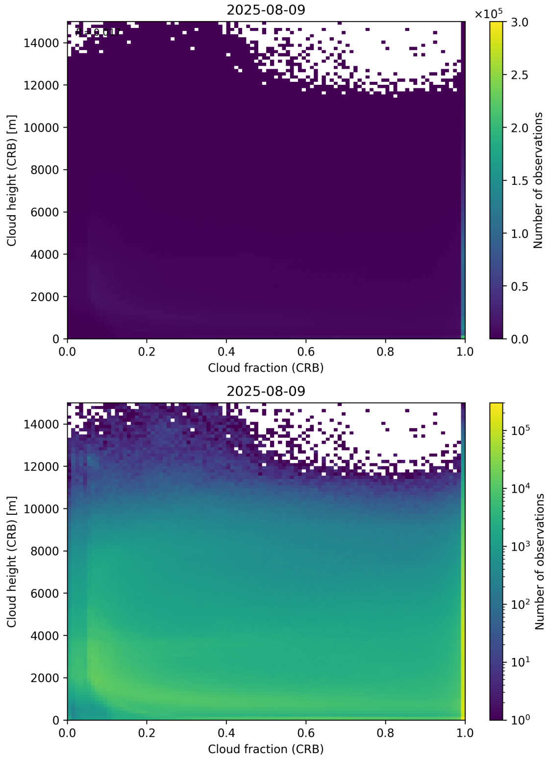
Figure 79: Scatter density plot of “Cloud fraction (CRB)” against “Cloud height (CRB)” for 2025-08-09 to 2025-08-10.
