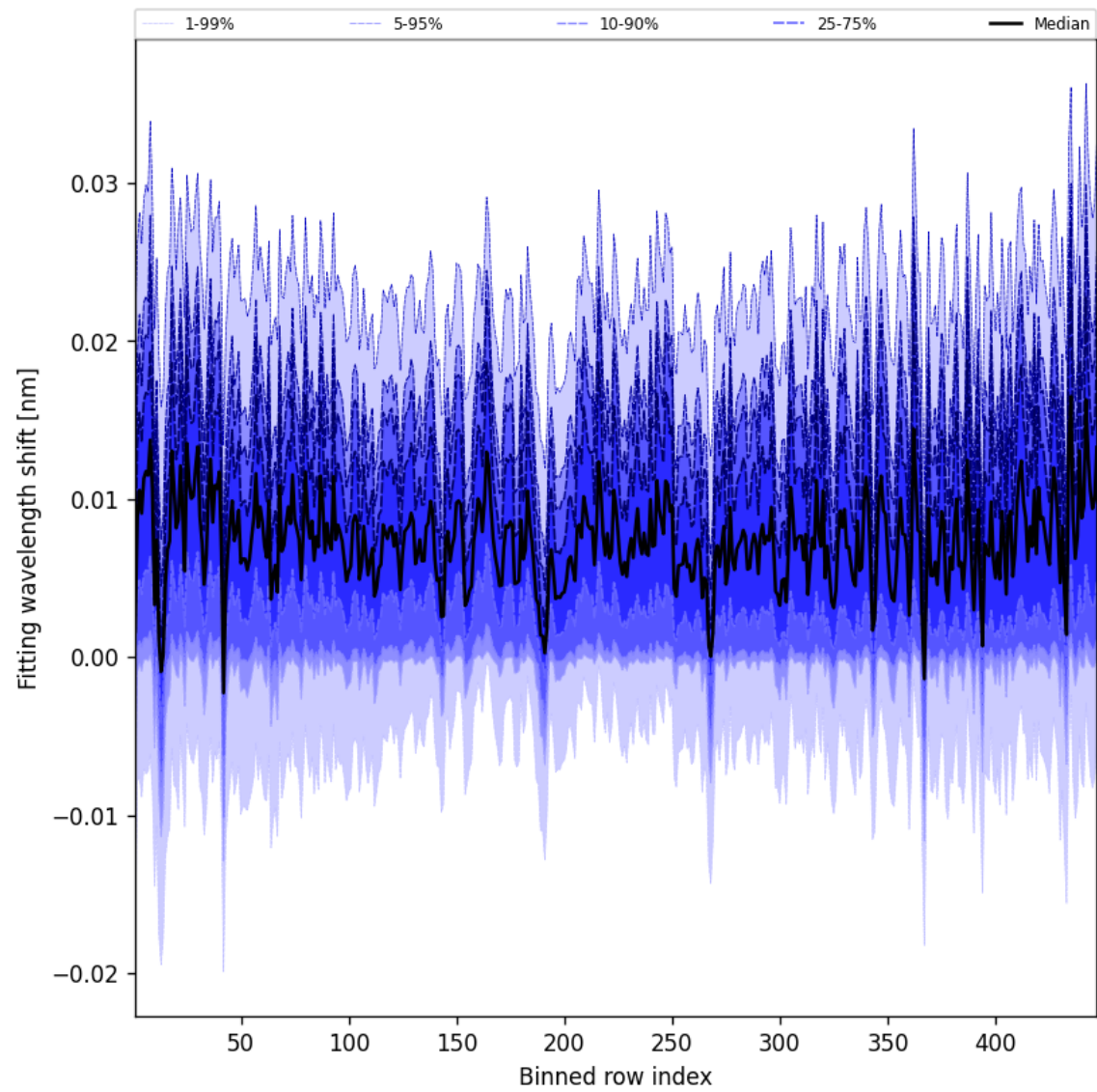
Figure 65: Along track statistics of “Fitting wavelength shift” for 2025-08-09 to 2025-08-10
