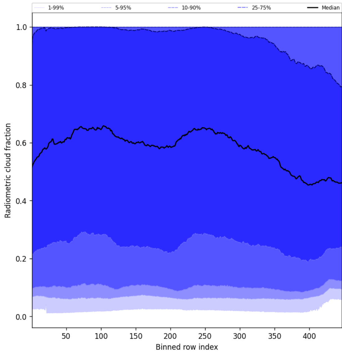
Figure 55: Along track statistics of “Radiometric cloud fraction” for 2025-08-09 to 2025-08-10
