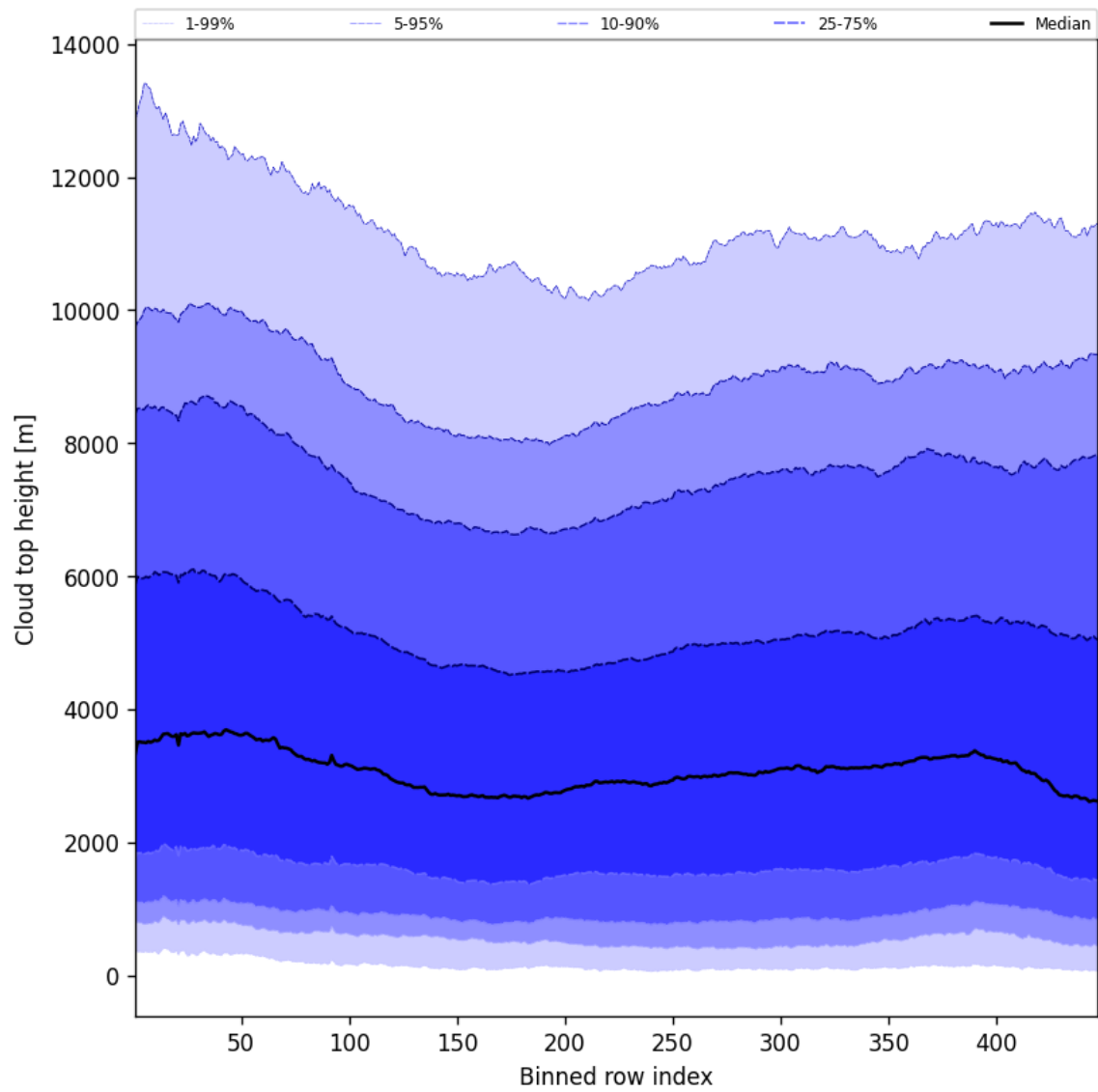
Figure 56: Along track statistics of “Cloud top height” for 2025-08-09 to 2025-08-10
