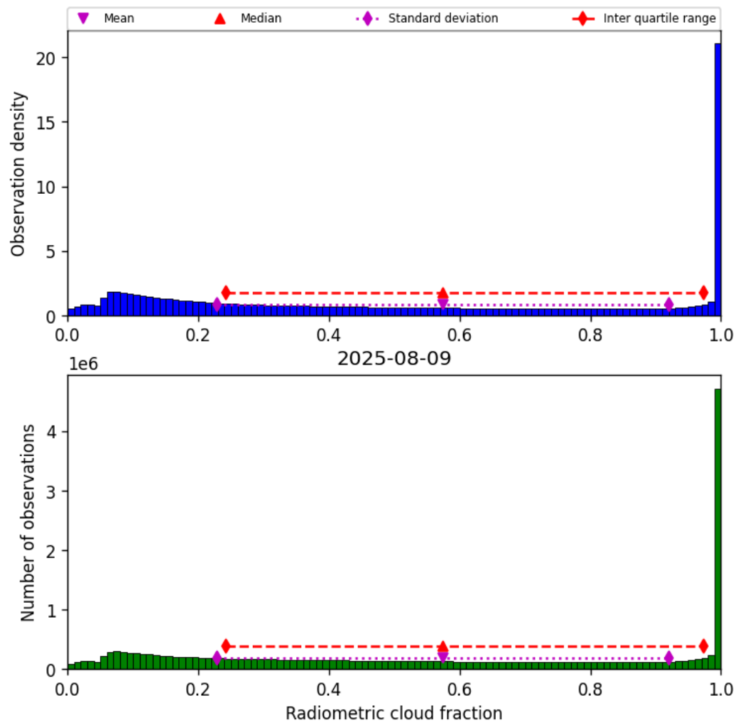
Figure 39: Histogram of “Radiometric cloud fraction” for 2025-08-09 to 2025-08-10
