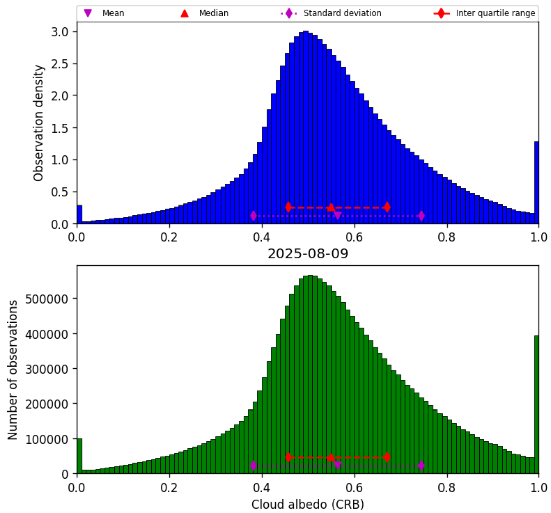
Figure 44: Histogram of “Cloud albedo (CRB)” for 2025-08-09 to 2025-08-10
