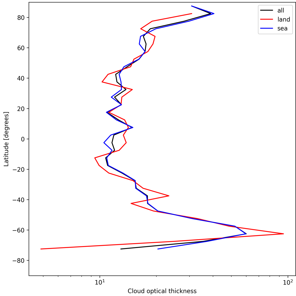
Figure 25: Zonal average of “Cloud optical thickness” for 2025-08-09 to 2025-08-10.
