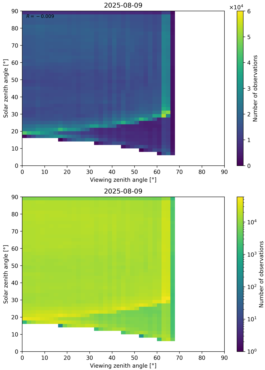
Figure 114: Scatter density plot of “Viewing zenith angle” against “Solar zenith angle” for 2025-08-09 to 2025-08-10.
