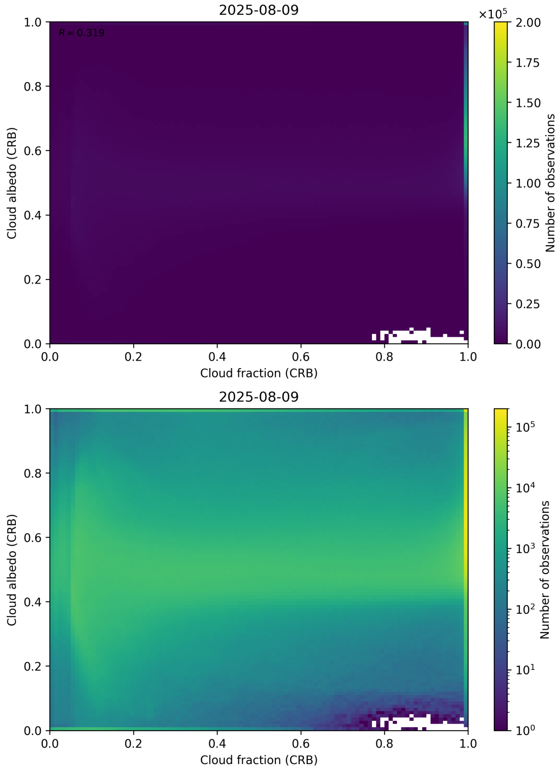
Figure 77: Scatter density plot of “Cloud fraction (CRB)” against “Cloud albedo (CRB)” for 2025-08-09 to 2025-08-10.
