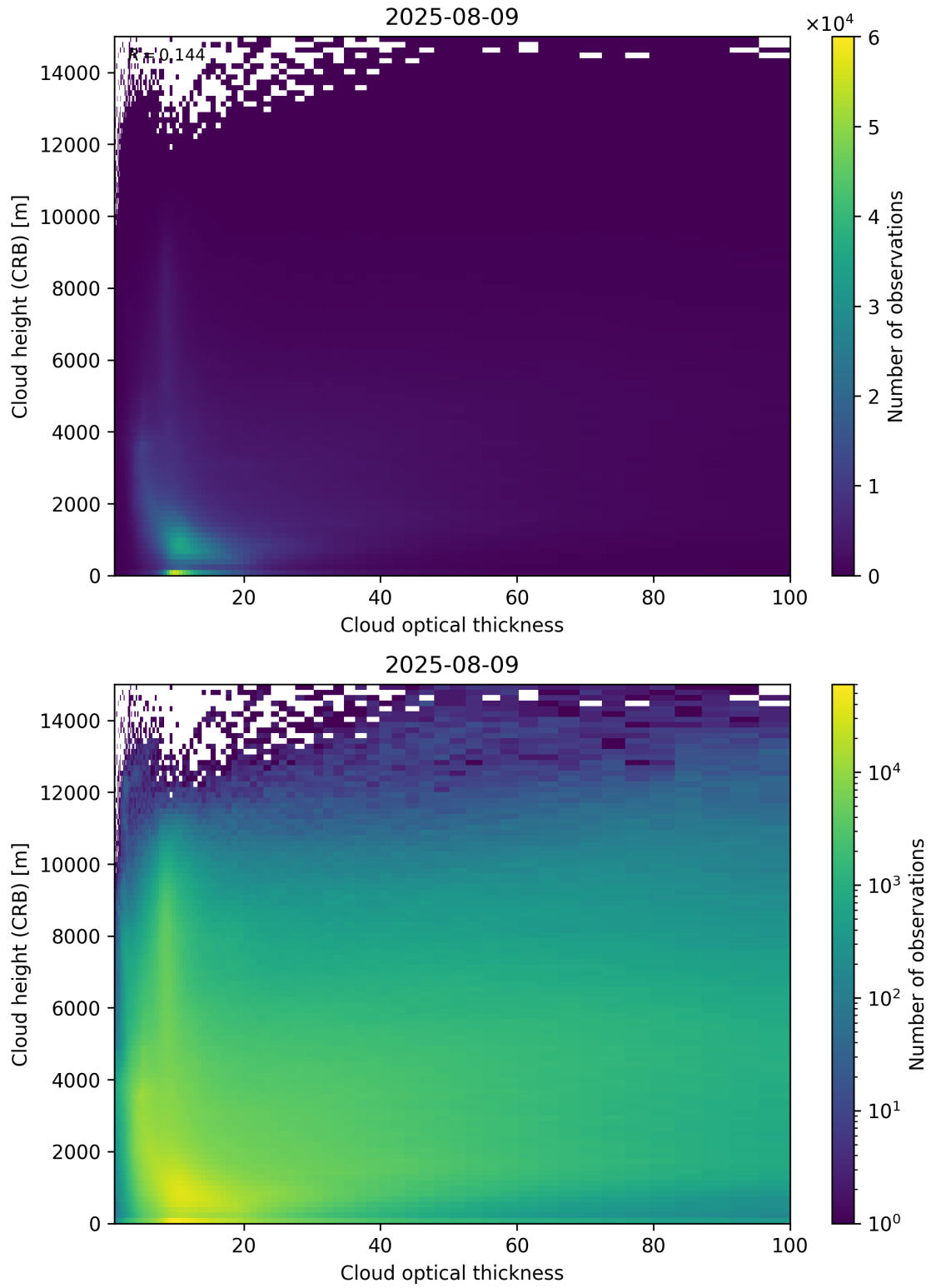
Figure 85: Scatter density plot of “Cloud optical thickness” against “Cloud height (CRB)” for 2025-08-09 to 2025-08-10.
