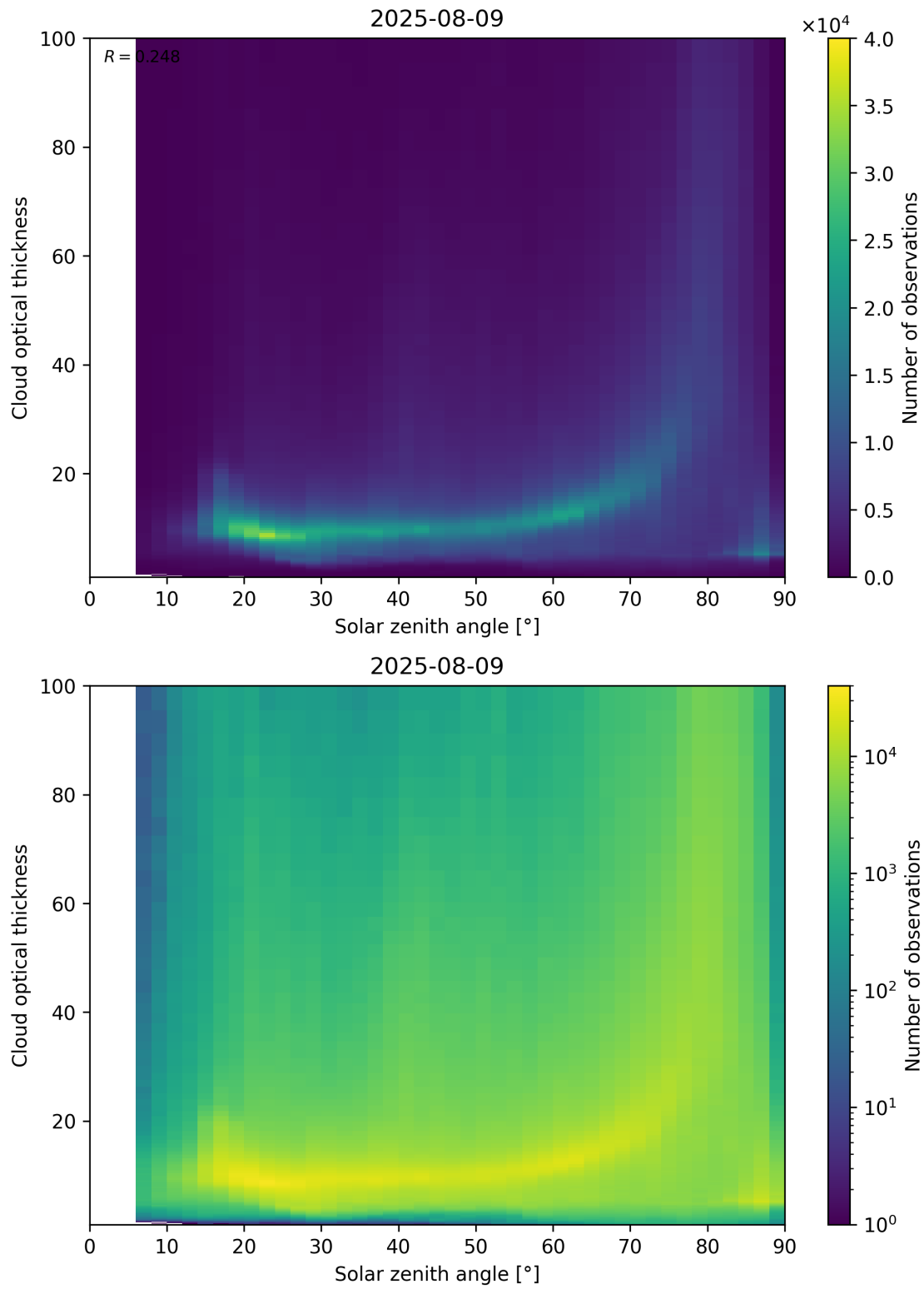
Figure 103: Scatter density plot of “Solar zenith angle” against “Cloud optical thickness” for 2025-08-09 to 2025-08-10.
