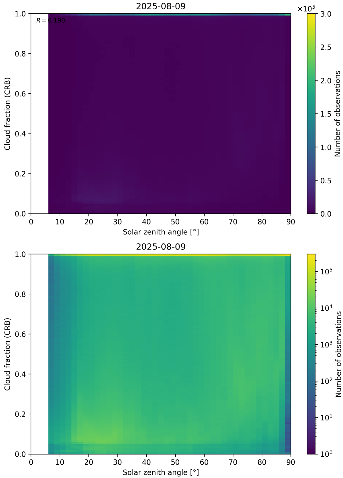
Figure 101: Scatter density plot of “Solar zenith angle” against “Cloud fraction (CRB)” for 2025-08-09 to 2025-08-10.
