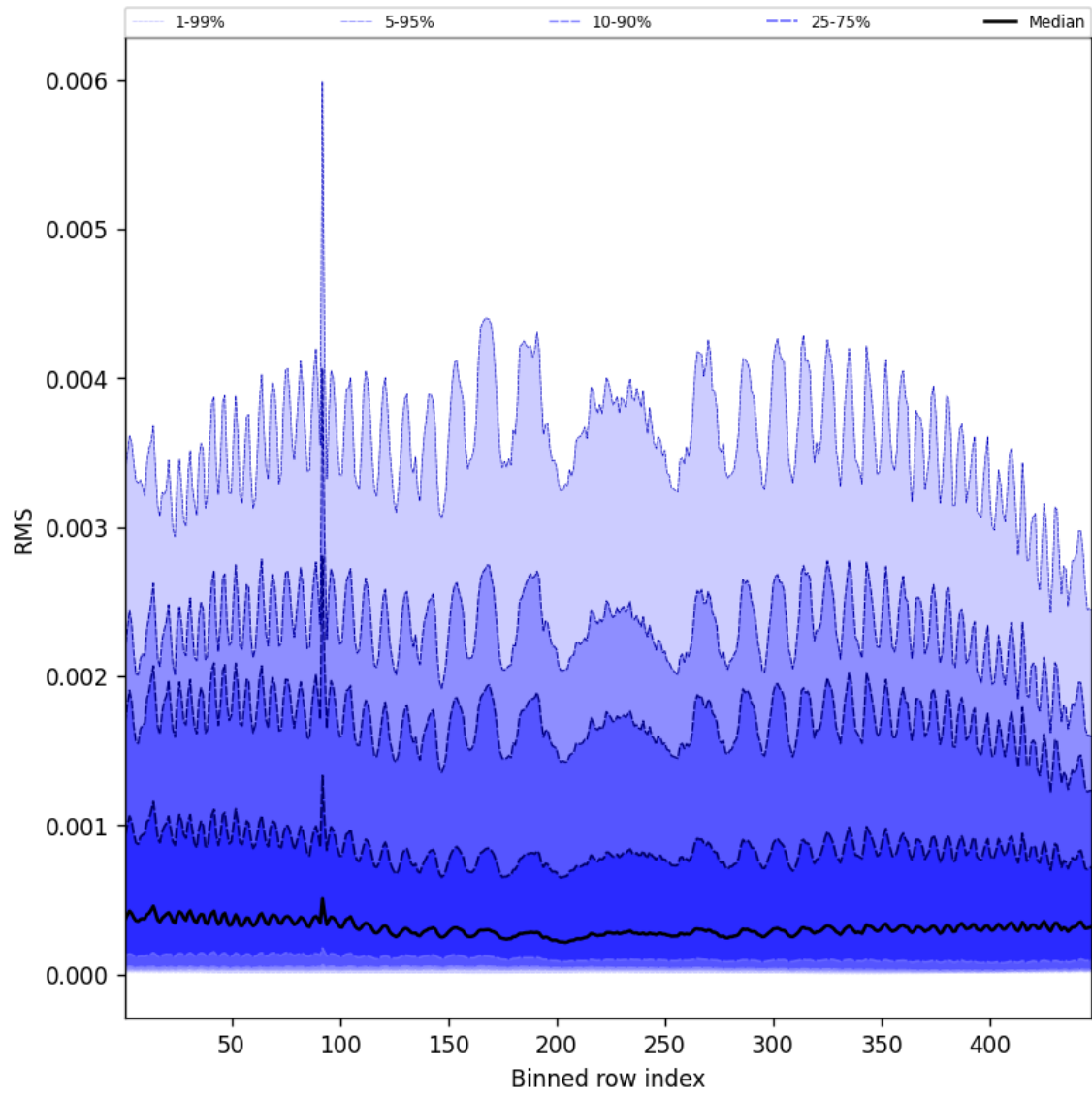
Figure 63: Along track statistics of “RMS” for 2025-08-09 to 2025-08-10
