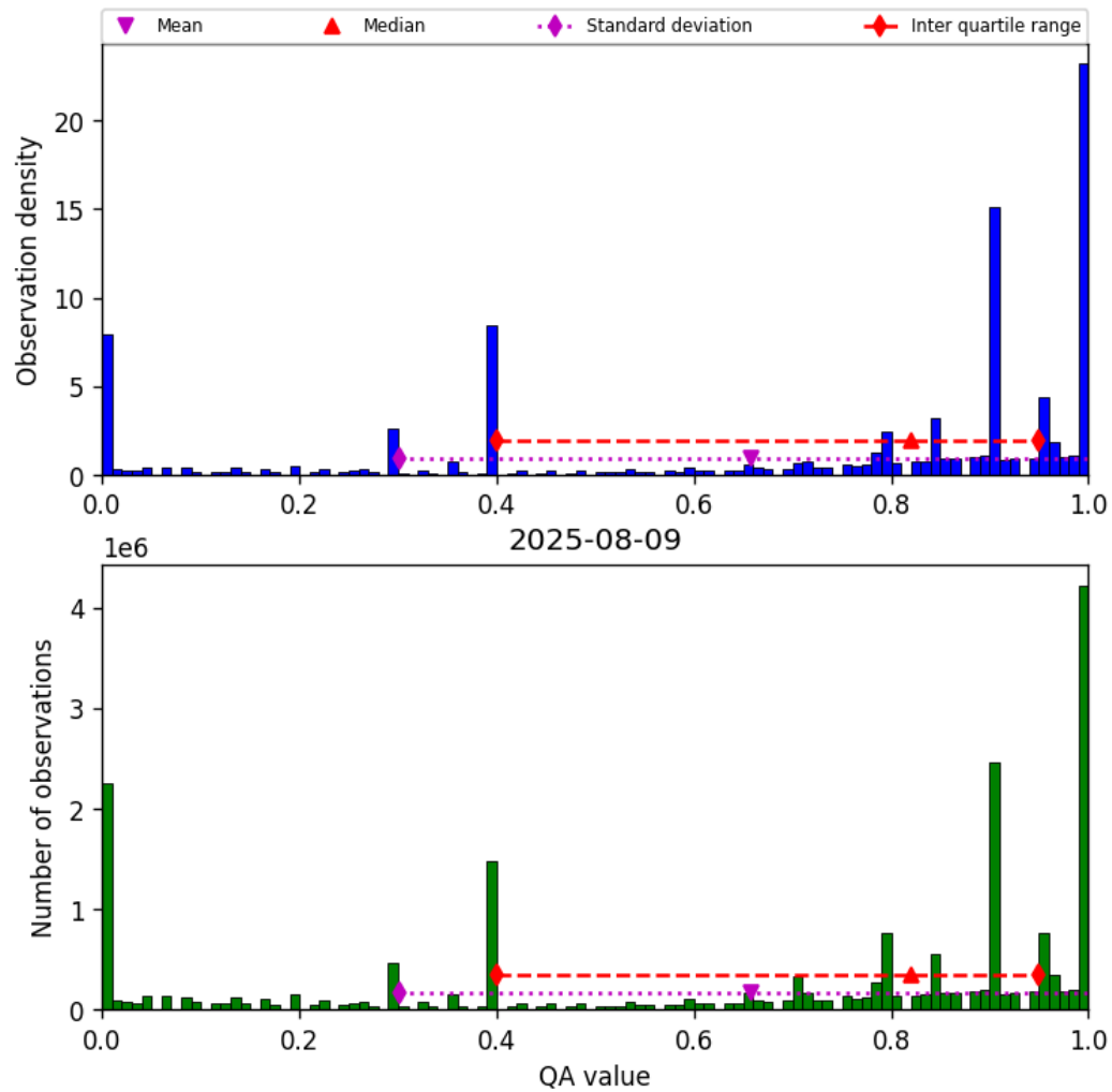
Figure 38: Histogram of “QA value” for 2025-08-09 to 2025-08-10
