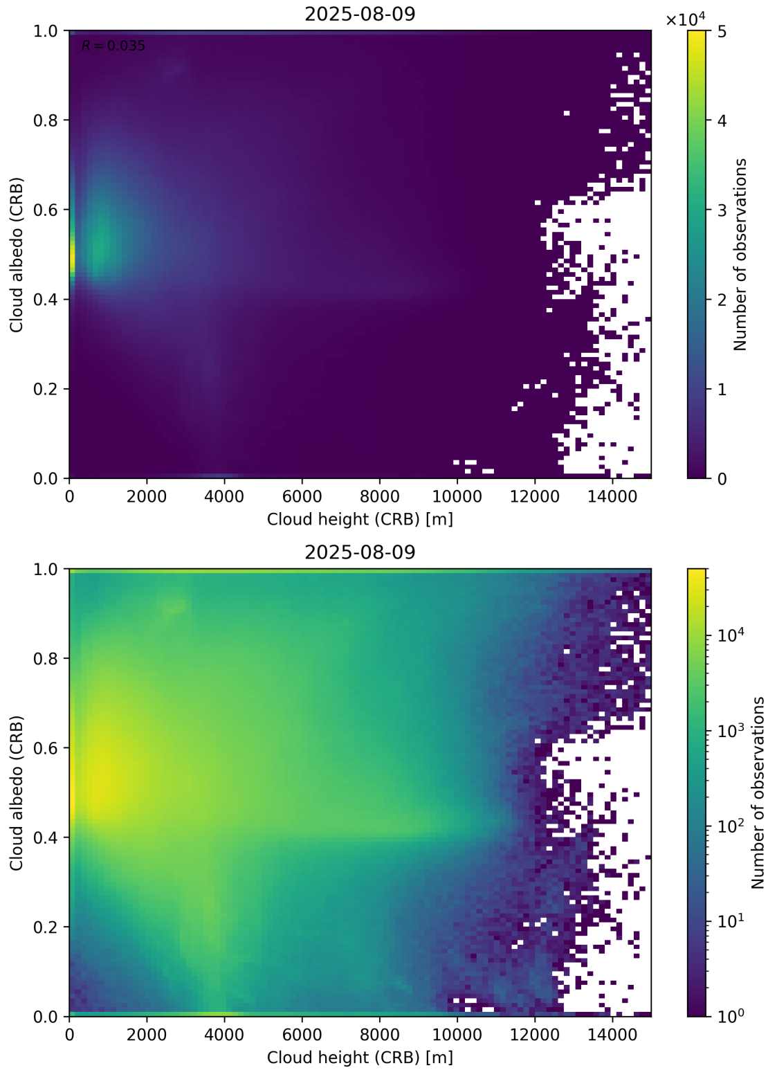
Figure 80: Scatter density plot of “Cloud height (CRB)” against “Cloud albedo (CRB)” for 2025-08-09 to 2025-08-10.
