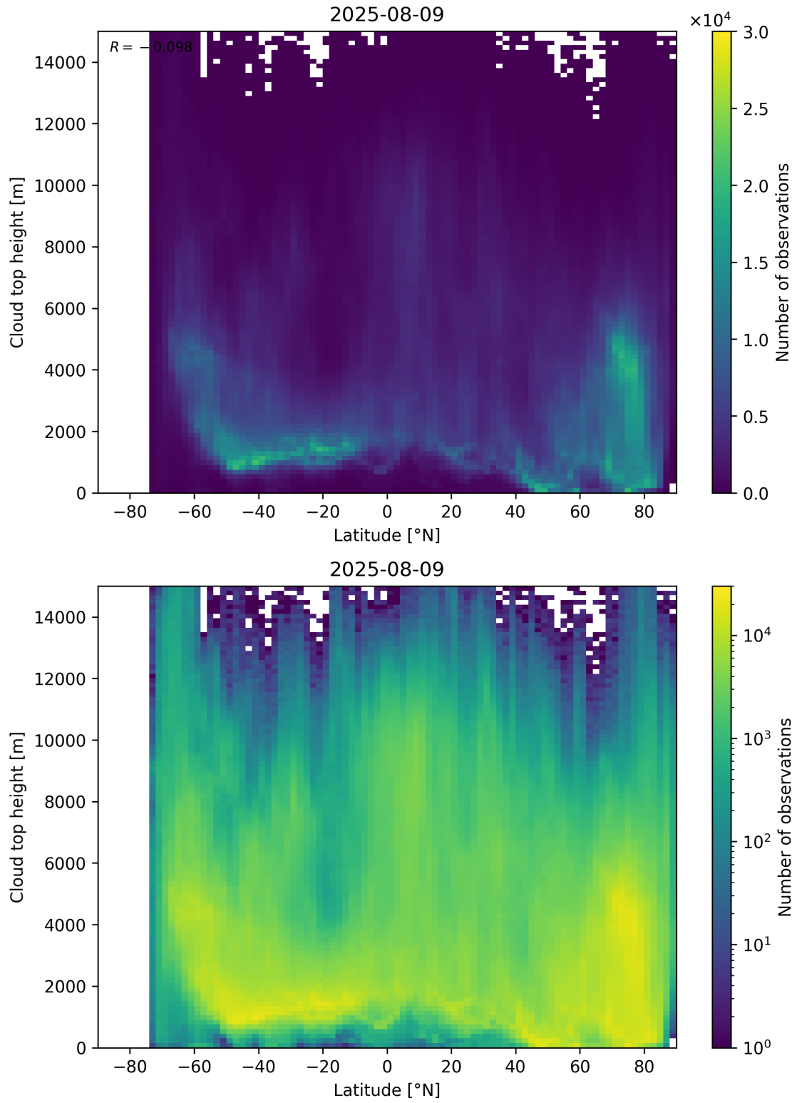
Figure 97: Scatter density plot of “Latitude” against “Cloud top height” for 2025-08-09 to 2025-08-10.
