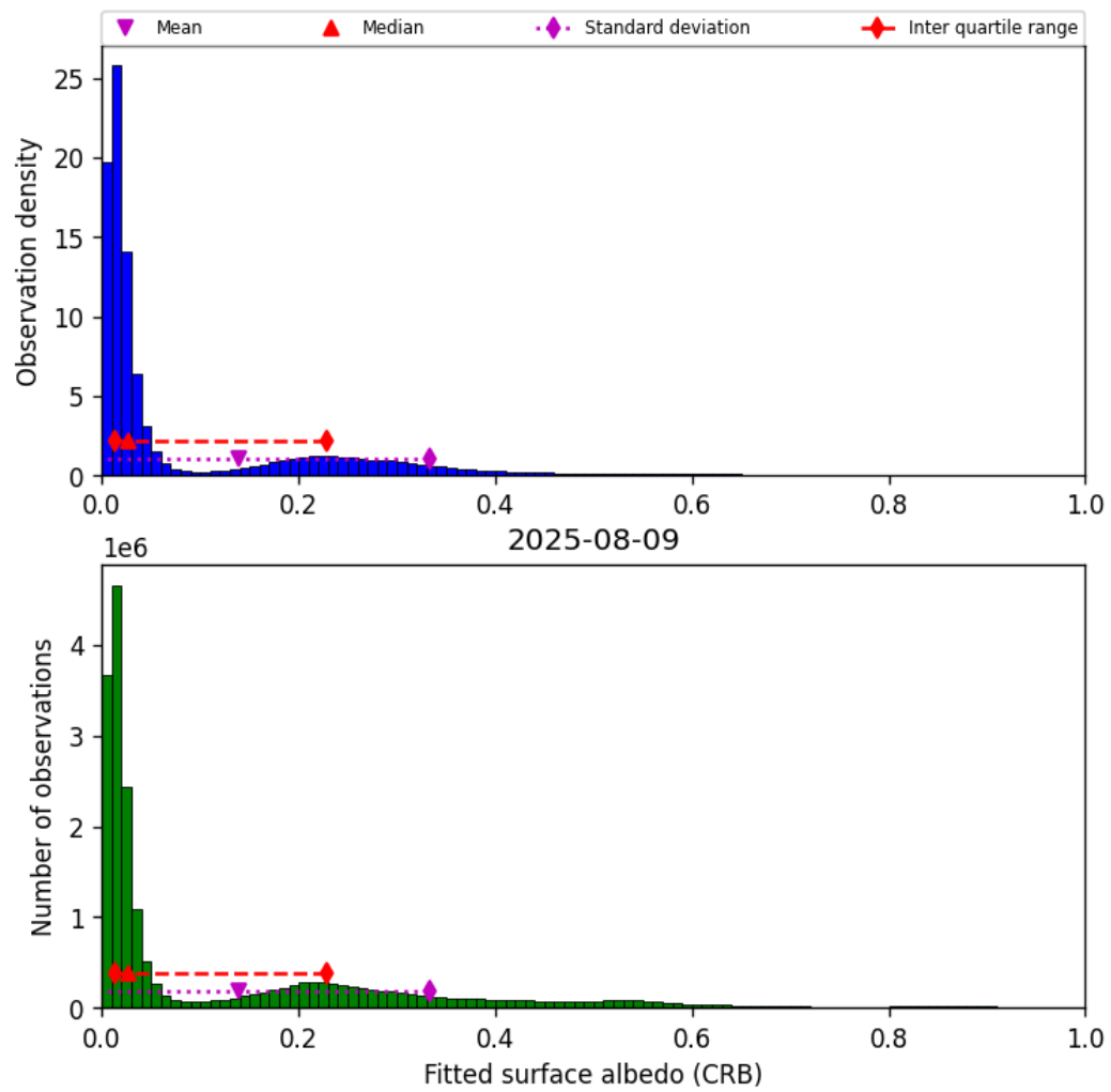
Figure 46: Histogram of “Fitted surface albedo (CRB)” for 2025-08-09 to 2025-08-10
