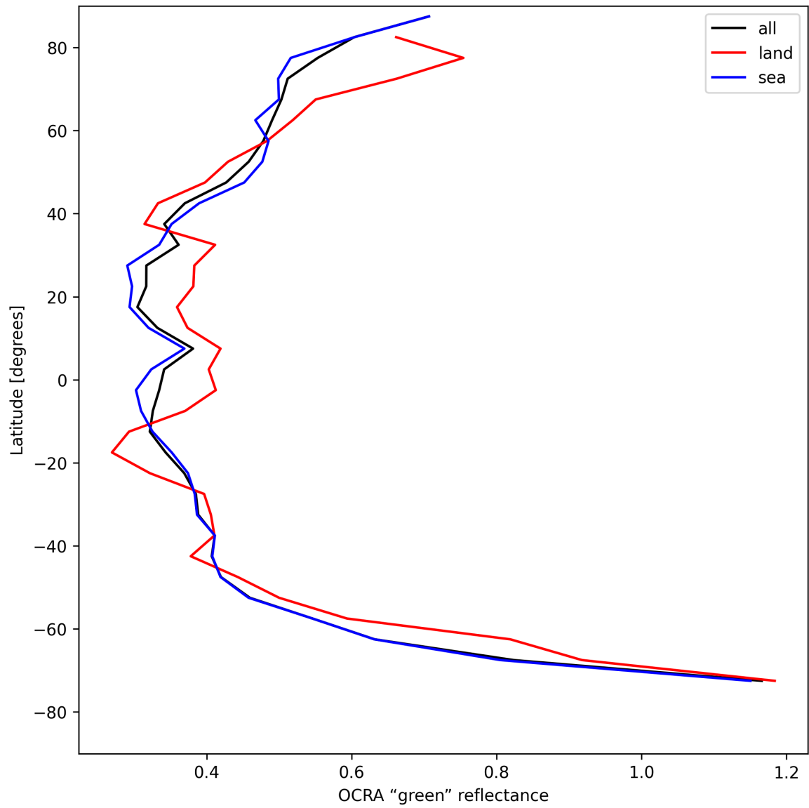
Figure 36: Zonal average of “OCRA “green” reflectance” for 2025-08-09 to 2025-08-10.
