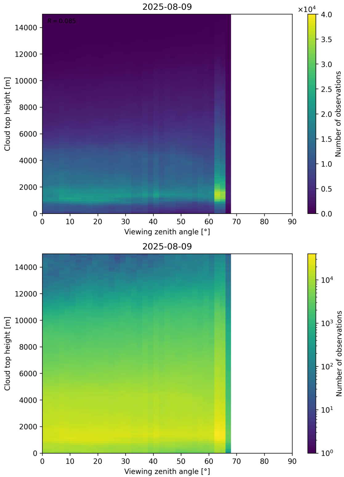
Figure 112: Scatter density plot of “Viewing zenith angle” against “Cloud top height” for 2025-08-09 to 2025-08-10.
