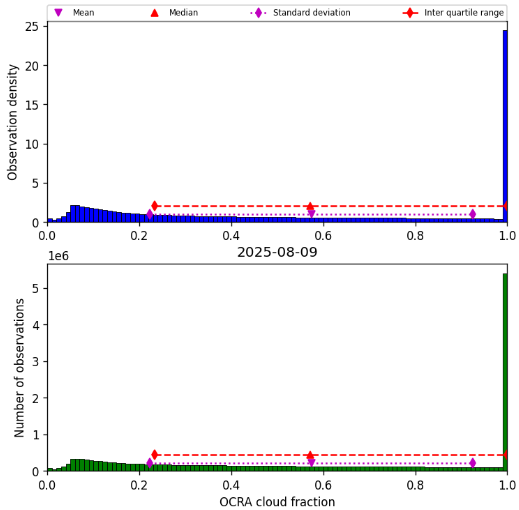
Figure 50: Histogram of “OCRA cloud fraction” for 2025-08-09 to 2025-08-10
