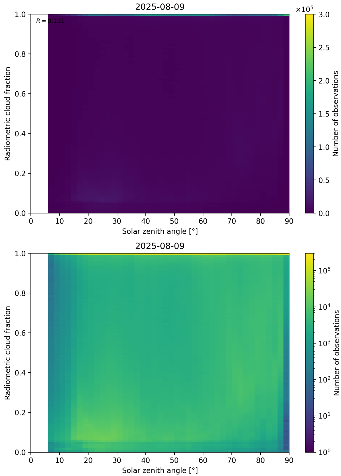
Figure 99: Scatter density plot of “Solar zenith angle” against “Radiometric cloud fraction” for 2025-08-09 to 2025-08-10.
