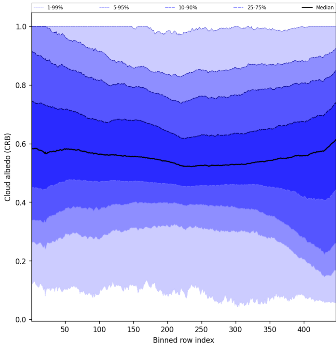
Figure 60: Along track statistics of “Cloud albedo (CRB)” for 2025-08-09 to 2025-08-10
