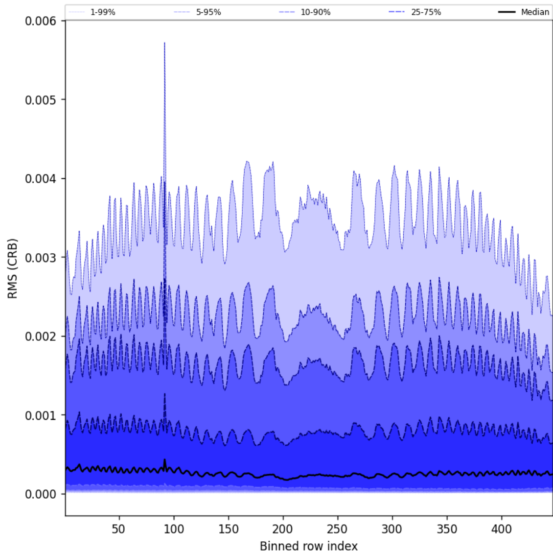
Figure 64: Along track statistics of “RMS (CRB)” for 2025-08-09 to 2025-08-10
