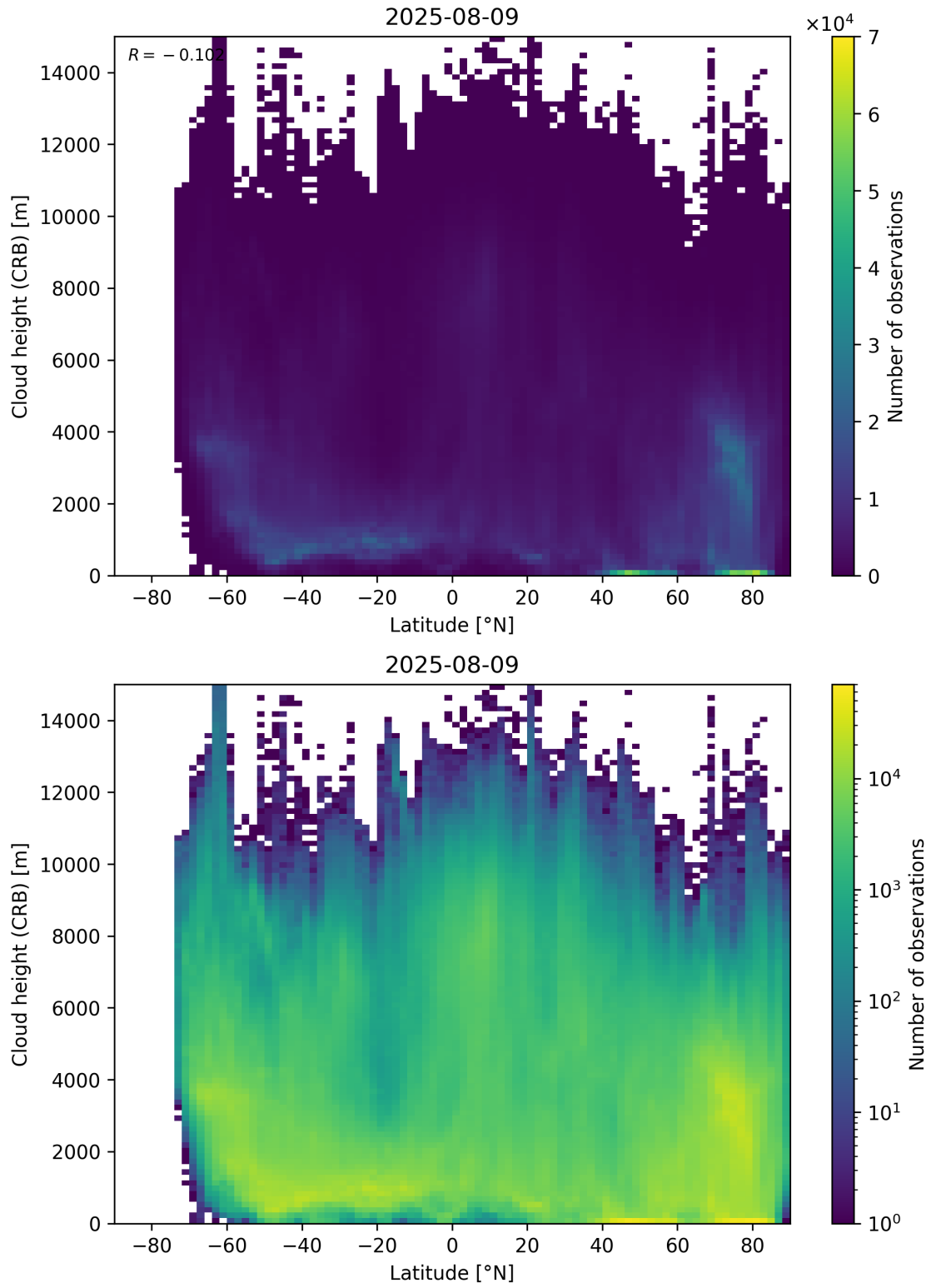
Figure 95: Scatter density plot of “Latitude” against “Cloud height (CRB)” for 2025-08-09 to 2025-08-10.
