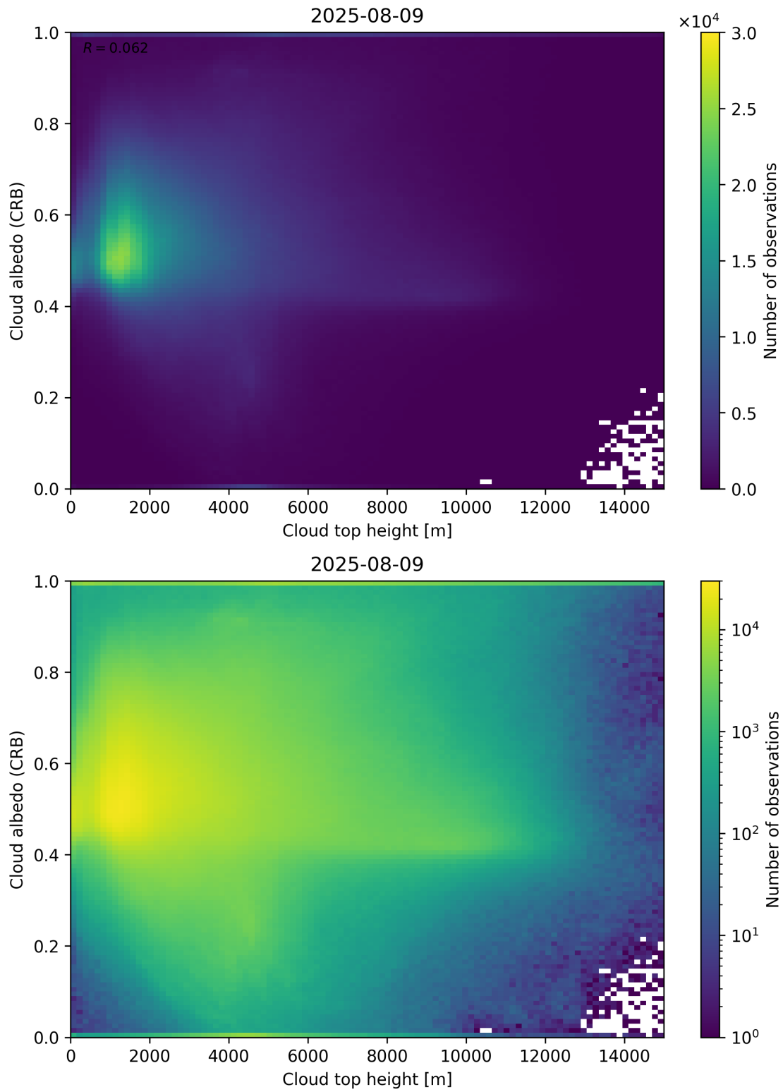
Figure 86: Scatter density plot of “Cloud top height” against “Cloud albedo (CRB)” for 2025-08-09 to 2025-08-10.
