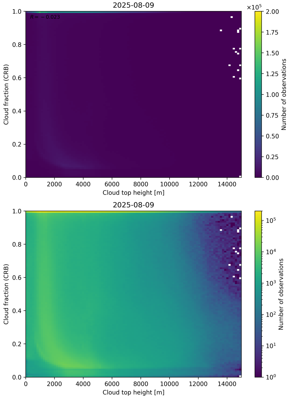
Figure 88: Scatter density plot of “Cloud top height” against “Cloud fraction (CRB)” for 2025-08-09 to 2025-08-10.
