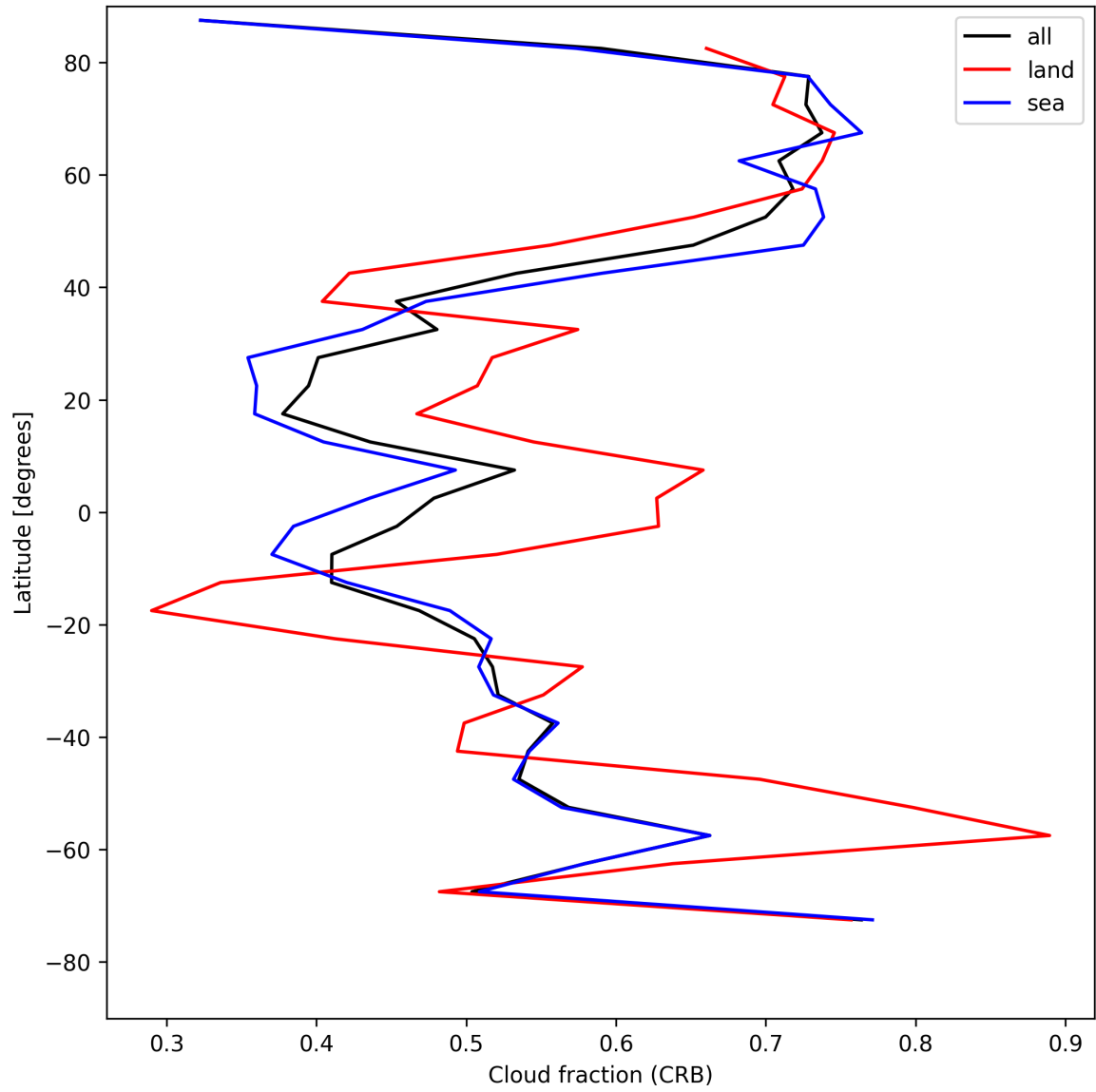
Figure 26: Zonal average of “Cloud fraction (CRB)” for 2025-08-09 to 2025-08-10.
