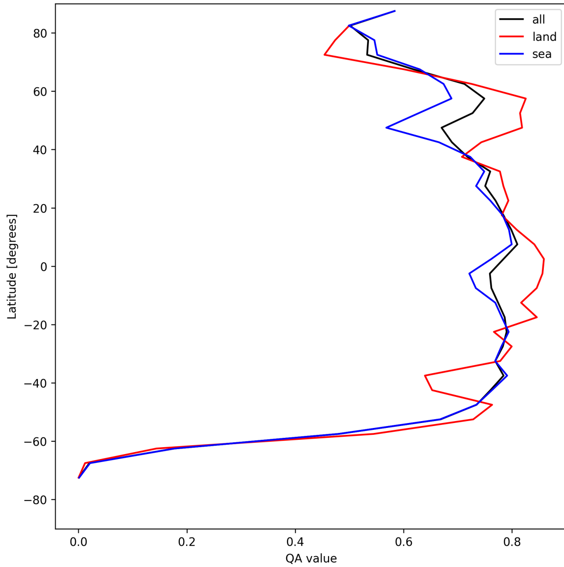
Figure 22: Zonal average of “QA value” for 2025-08-09 to 2025-08-10.
