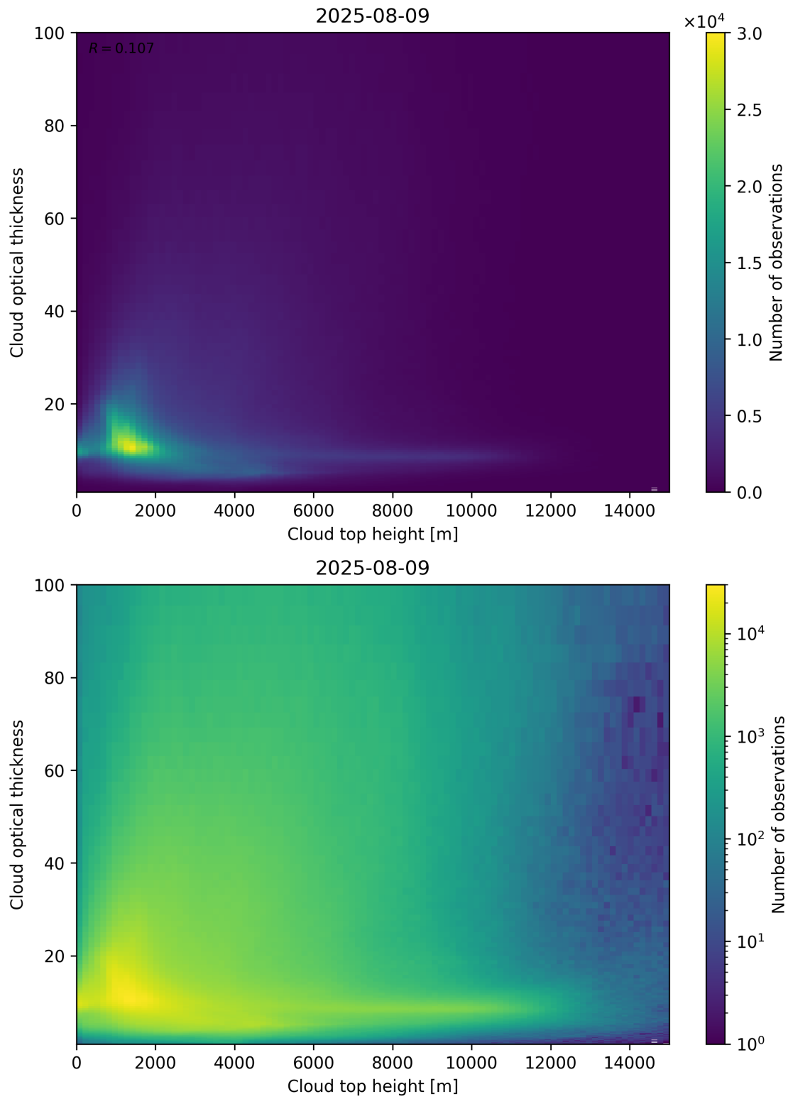
Figure 90: Scatter density plot of “Cloud top height” against “Cloud optical thickness” for 2025-08-09 to 2025-08-10.
