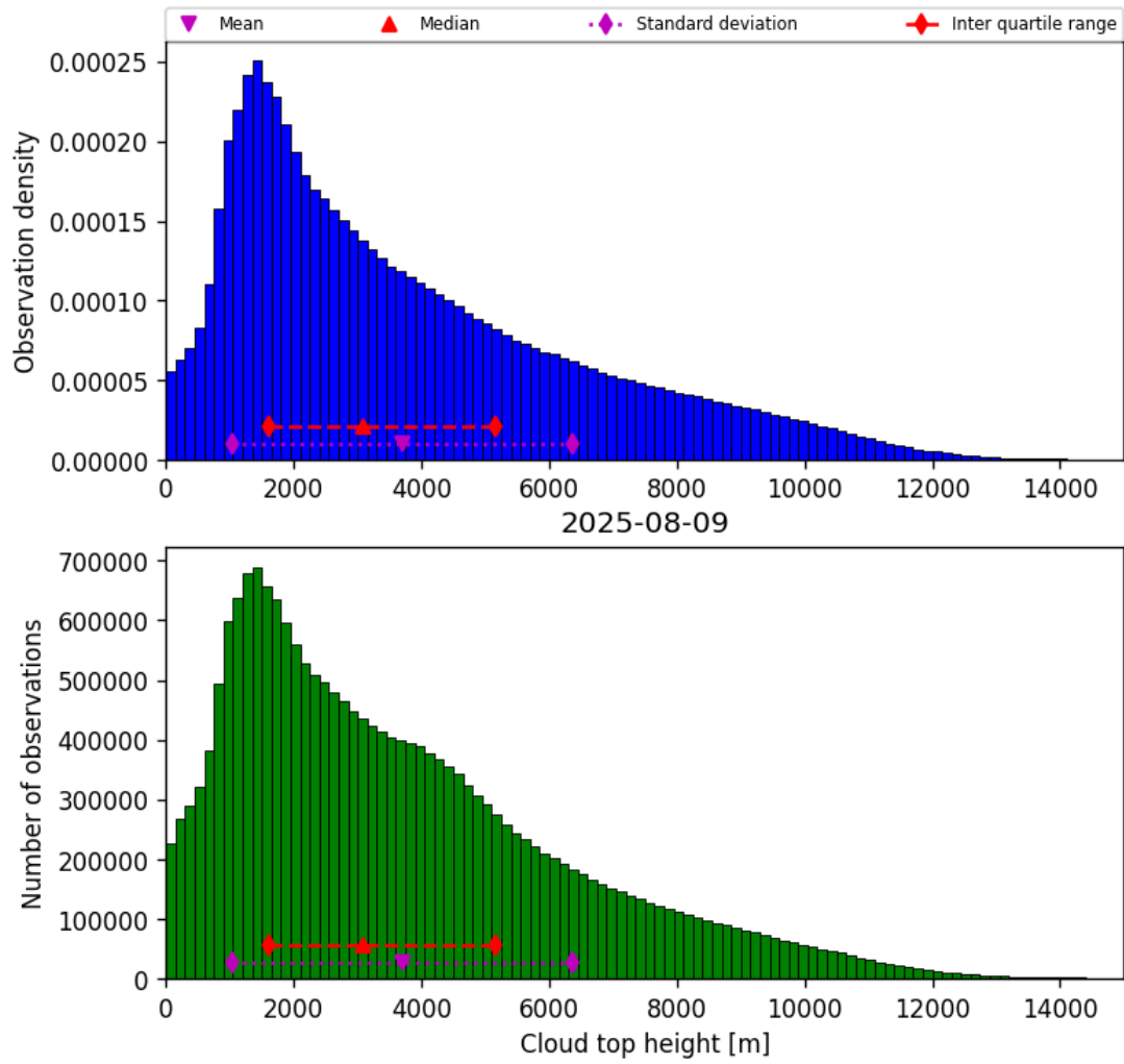
Figure 40: Histogram of “Cloud top height” for 2025-08-09 to 2025-08-10
