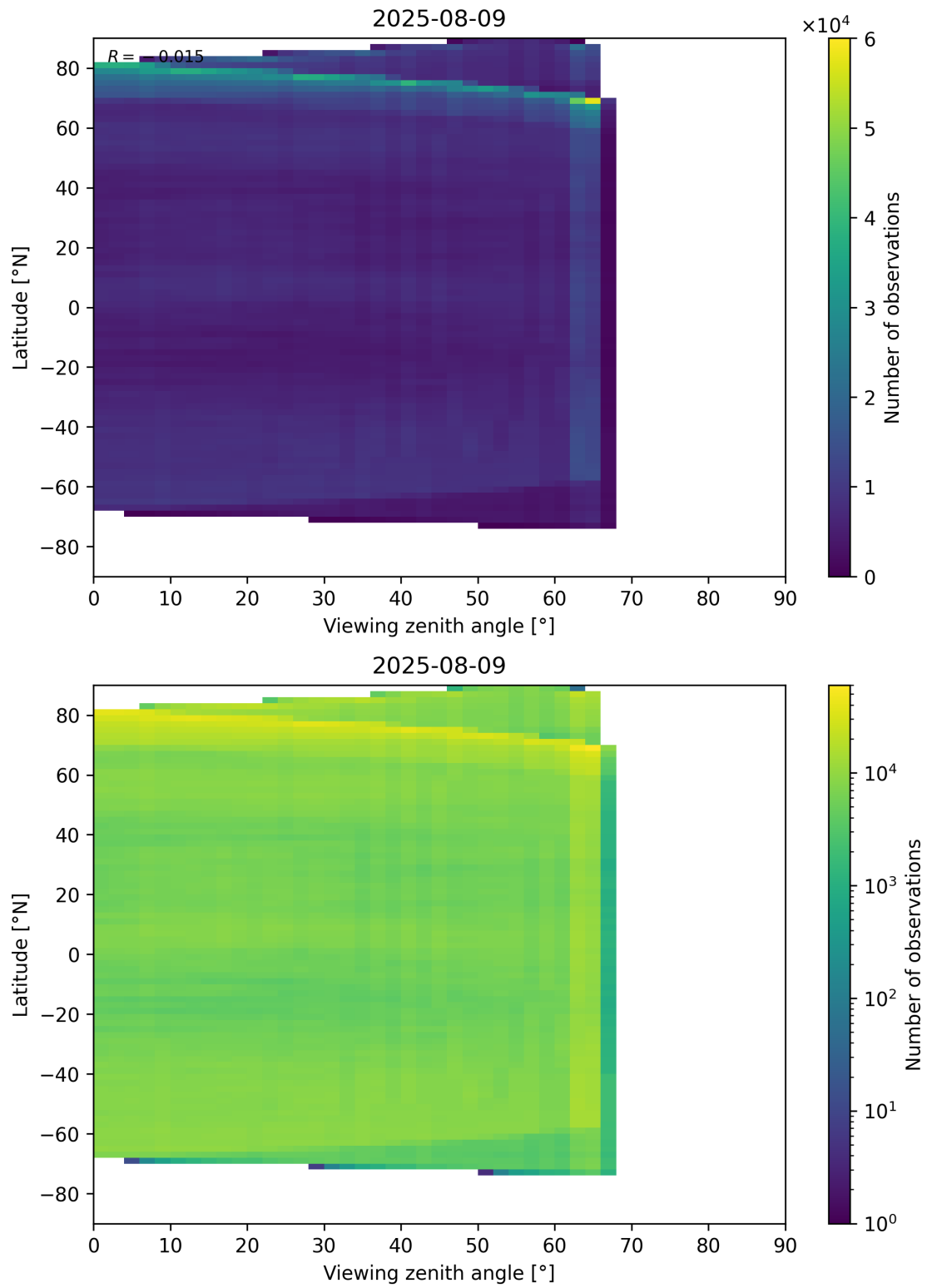
Figure 113: Scatter density plot of “Viewing zenith angle” against “Latitude” for 2025-08-09 to 2025-08-10.
