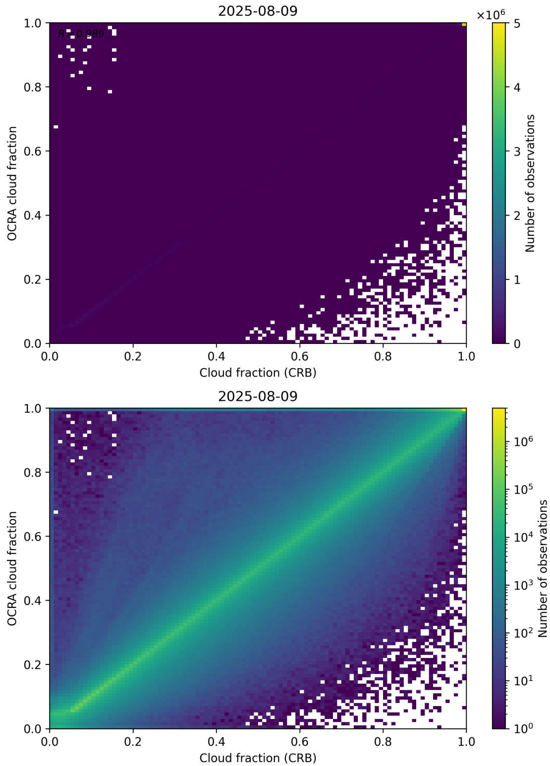
Figure 78: Scatter density plot of “Cloud fraction (CRB)” against “OCRA cloud fraction” for 2025-08-09 to 2025-08-10.
