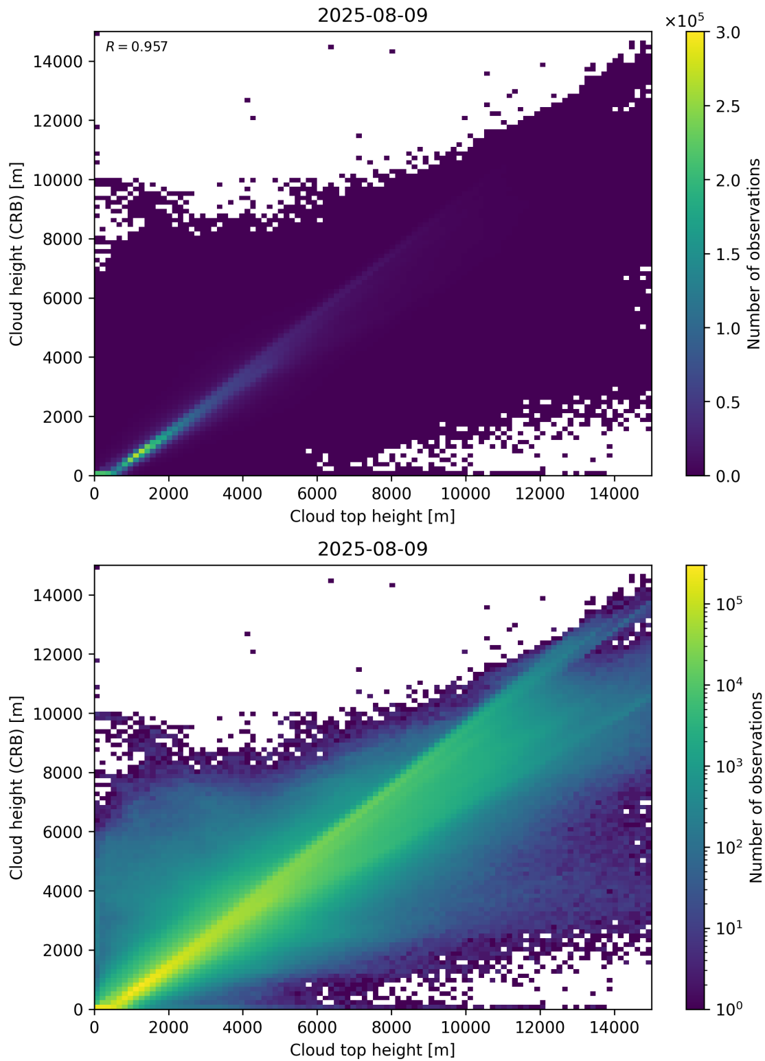
Figure 89: Scatter density plot of “Cloud top height” against “Cloud height (CRB)” for 2025-08-09 to 2025-08-10.
