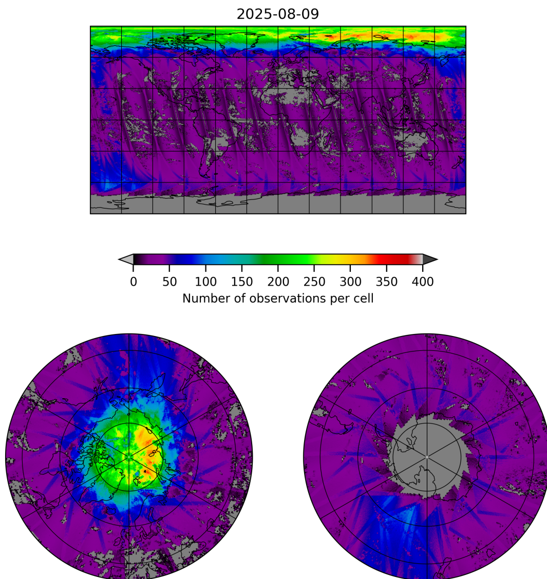
Figure 21: Map of the number of observations for 2025-08-09 to 2025-08-10
