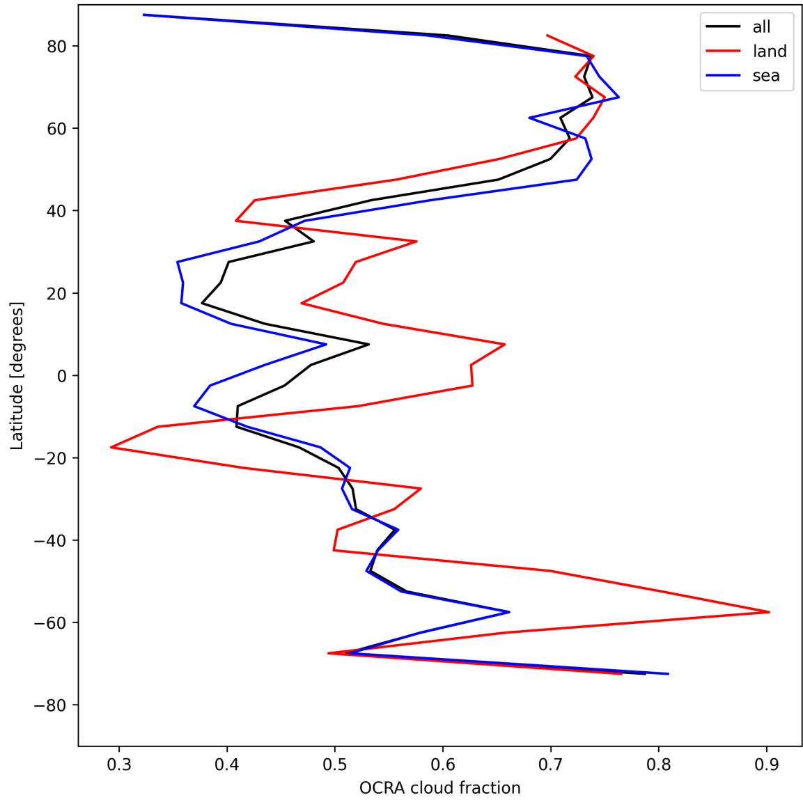
Figure 34: Zonal average of “OCRA cloud fraction” for 2025-08-09 to 2025-08-10.
