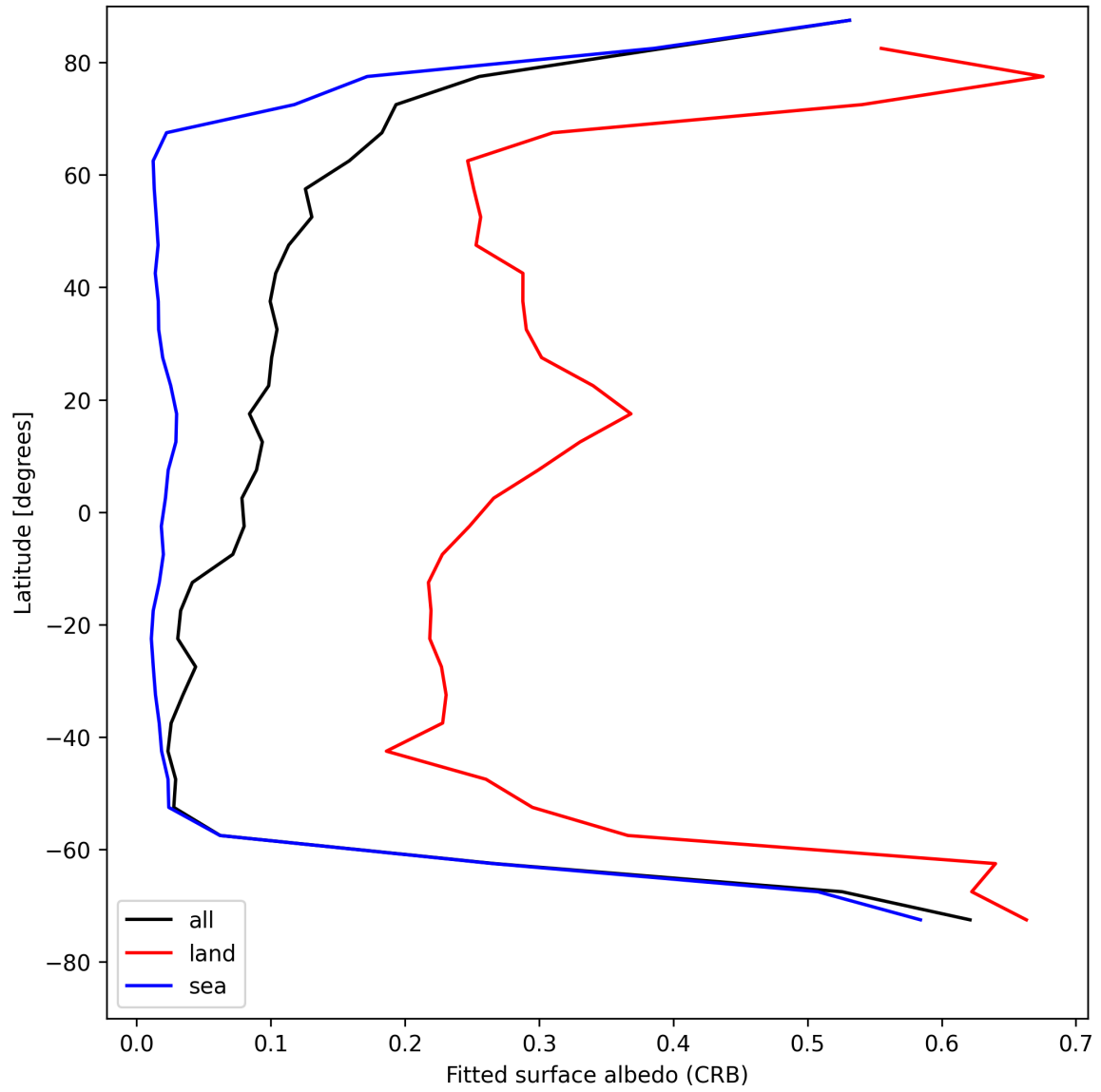
Figure 30: Zonal average of “Fitted surface albedo (CRB)” for 2025-08-09 to 2025-08-10.
