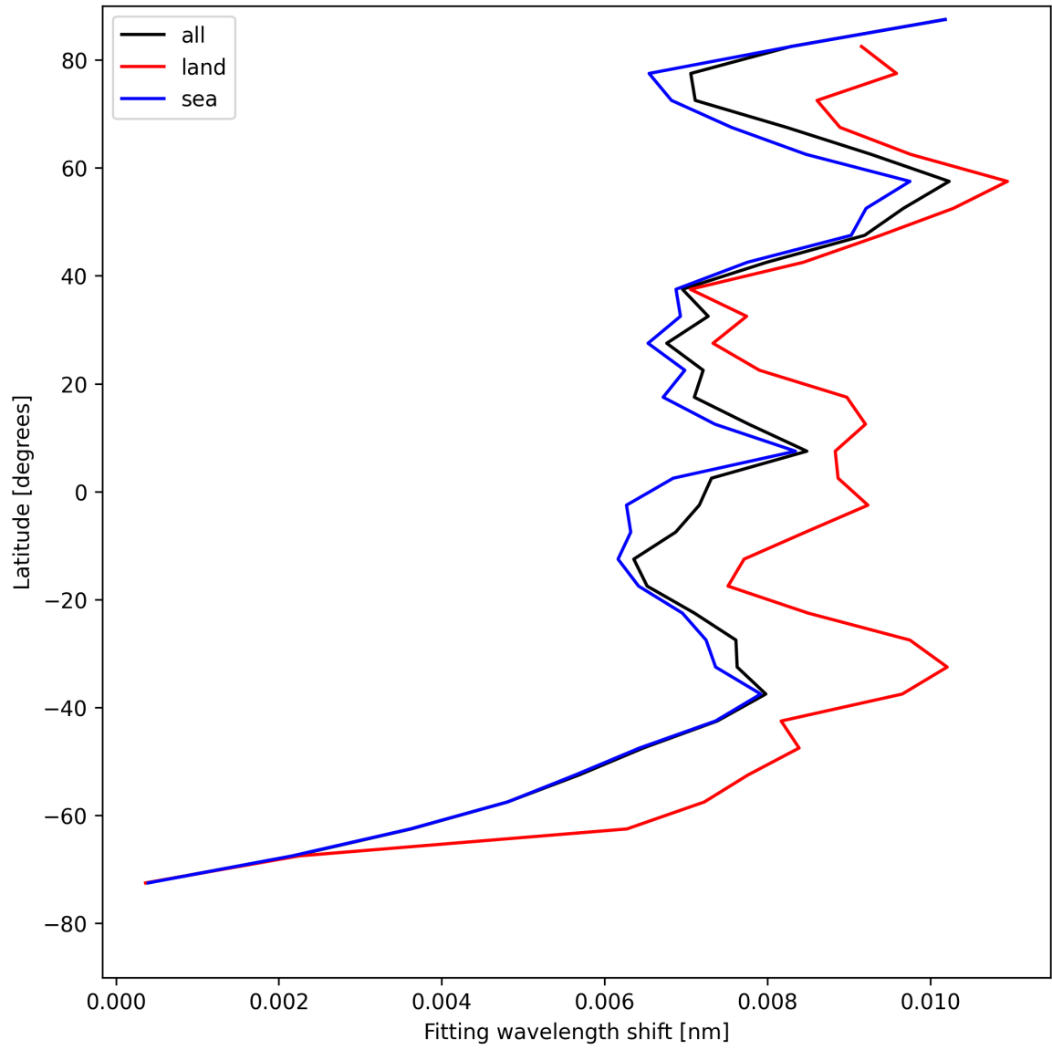
Figure 33: Zonal average of “Fitting wavelength shift” for 2025-08-09 to 2025-08-10.
