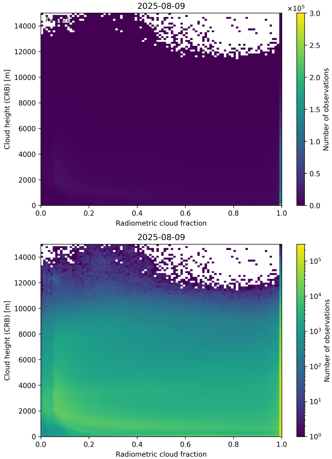
Figure 74: Scatter density plot of “Radiometric cloud fraction” against “Cloud height (CRB)” for 2025-08-09 to 2025-08-10.
