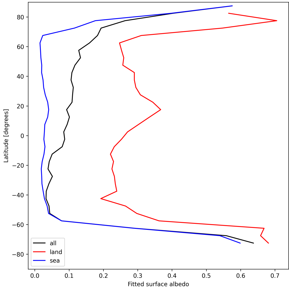
Figure 29: Zonal average of “Fitted surface albedo” for 2025-08-09 to 2025-08-10.
