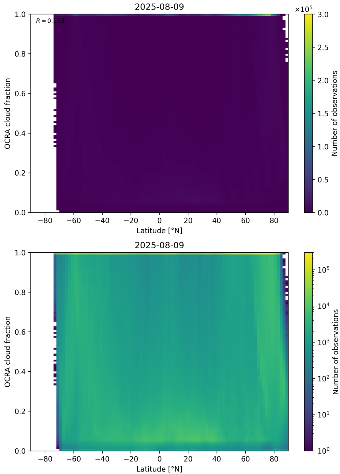
Figure 93: Scatter density plot of “Latitude” against “OCRA cloud fraction” for 2025-08-09 to 2025-08-10.
