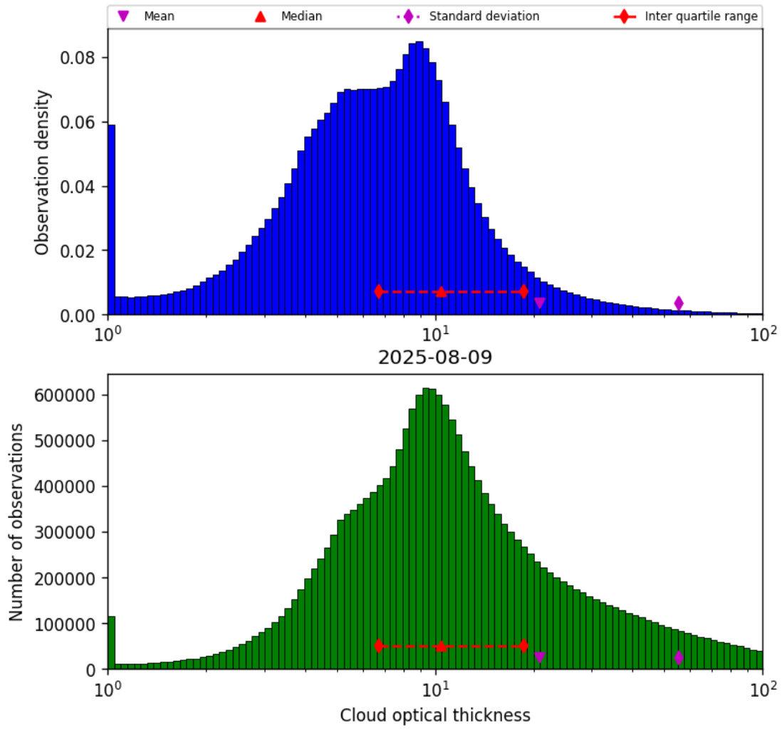
Figure 41: Histogram of “Cloud optical thickness” for 2025-08-09 to 2025-08-10
