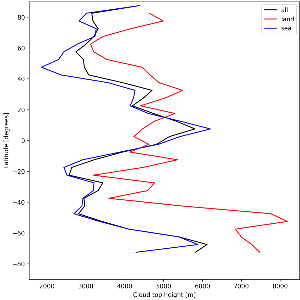
Figure 24: Zonal average of “Cloud top height” for 2025-08-09 to 2025-08-10.
