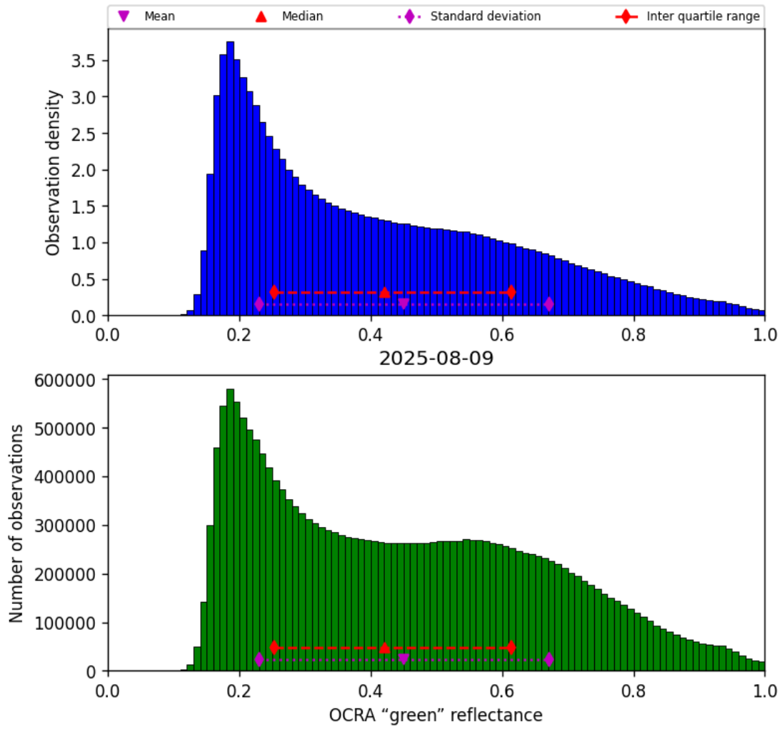
Figure 52: Histogram of “OCRA “green” reflectance” for 2025-08-09 to 2025-08-10
