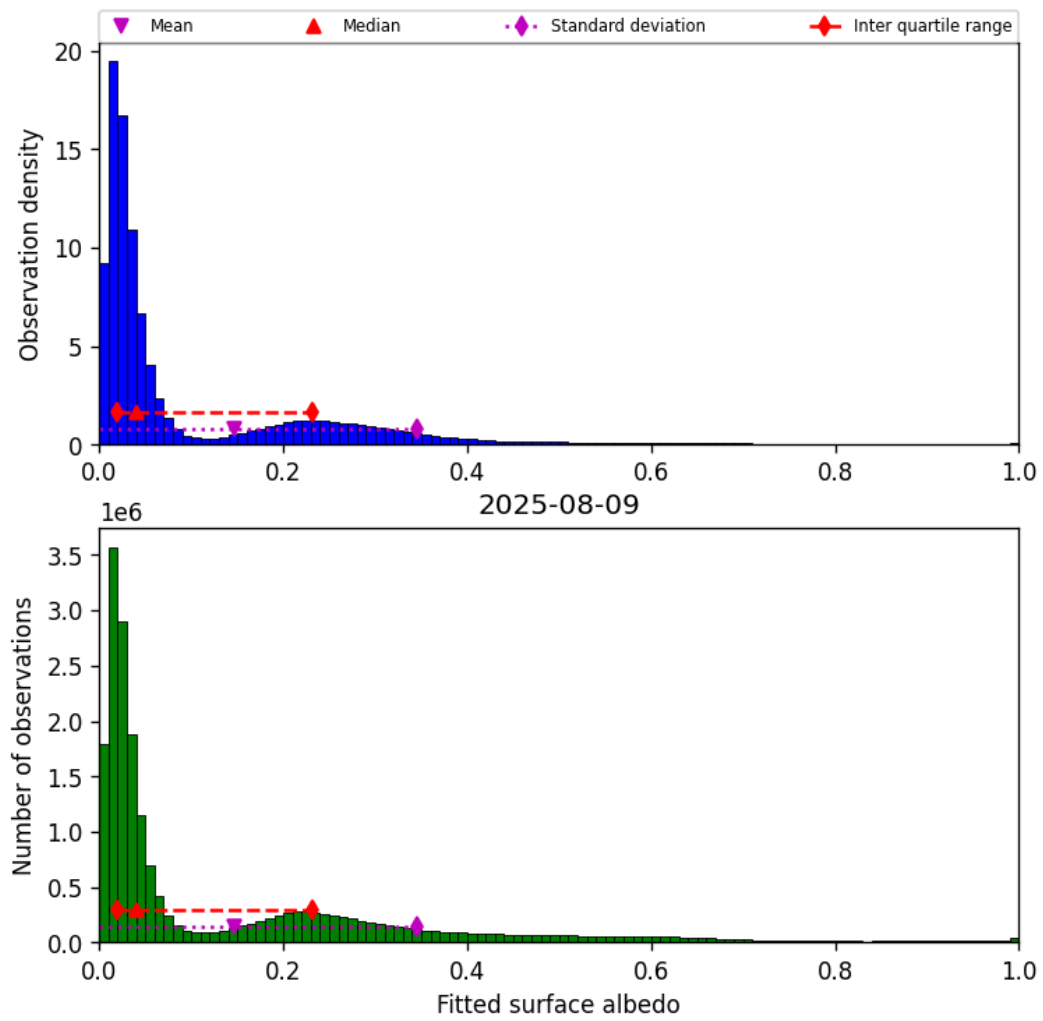
Figure 45: Histogram of “Fitted surface albedo” for 2025-08-09 to 2025-08-10
