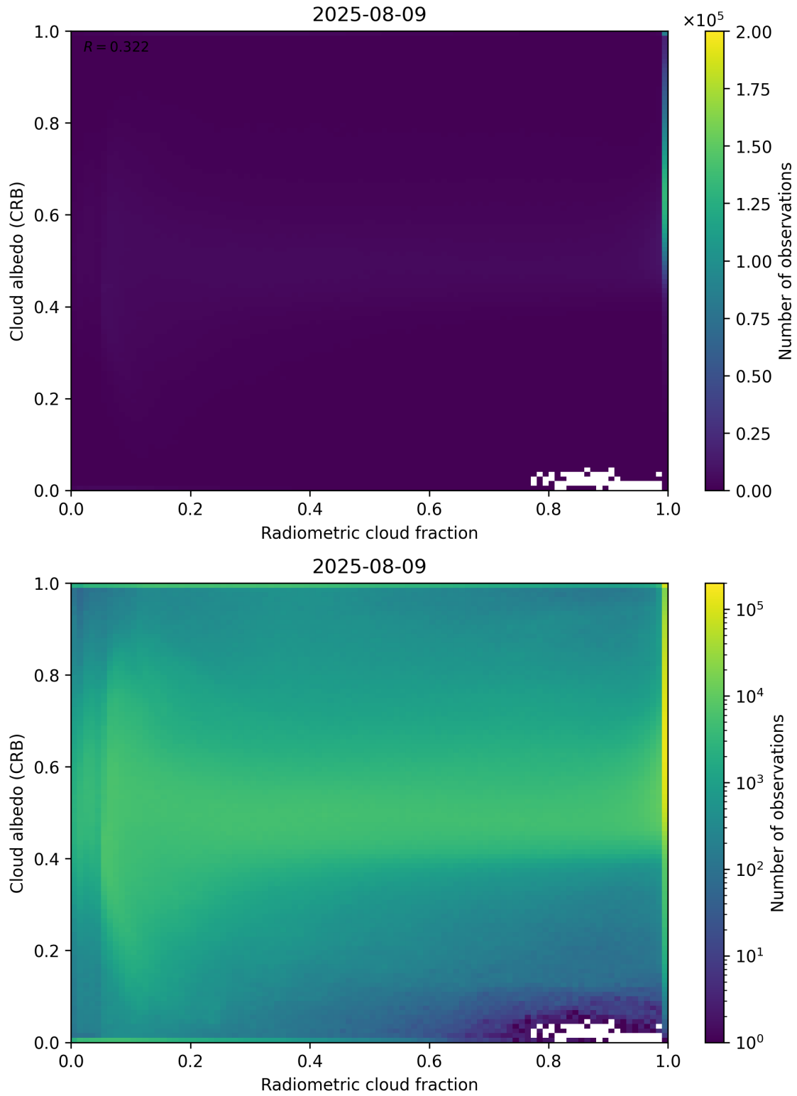
Figure 71: Scatter density plot of “Radiometric cloud fraction” against “Cloud albedo (CRB)” for 2025-08-09 to 2025-08-10.
