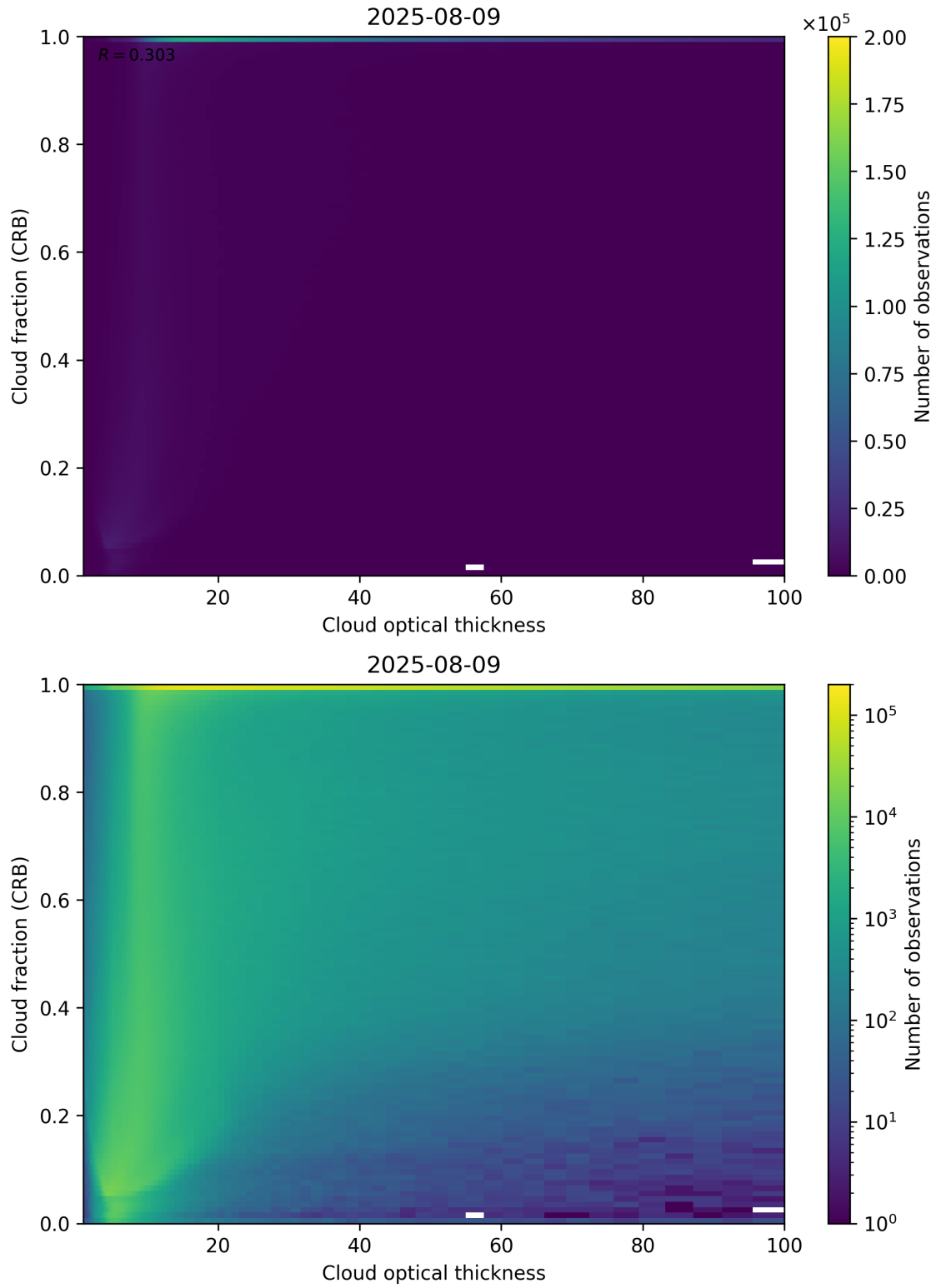
Figure 84: Scatter density plot of “Cloud optical thickness” against “Cloud fraction (CRB)” for 2025-08-09 to 2025-08-10.
