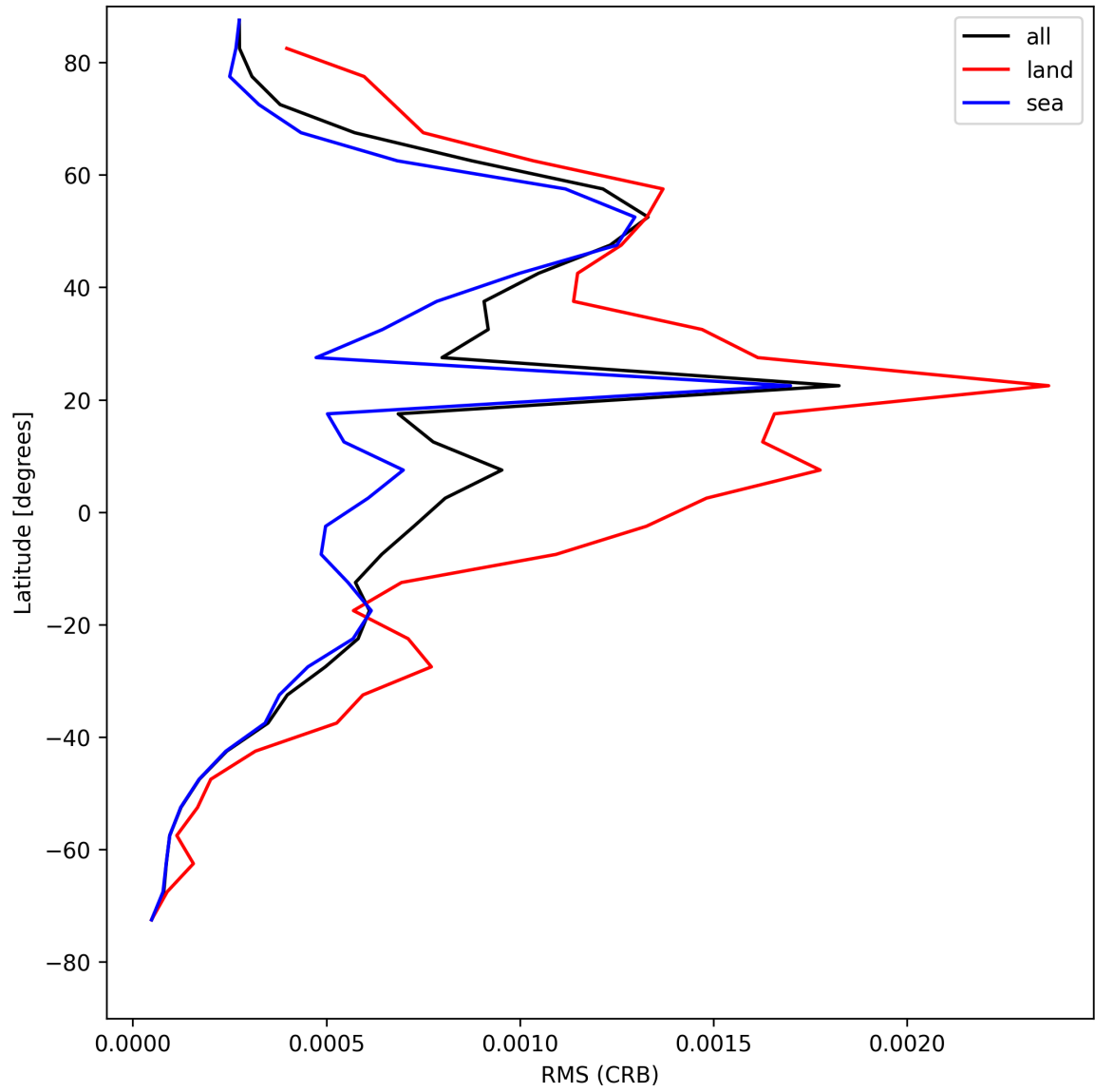
Figure 32: Zonal average of “RMS (CRB)” for 2025-08-09 to 2025-08-10.
