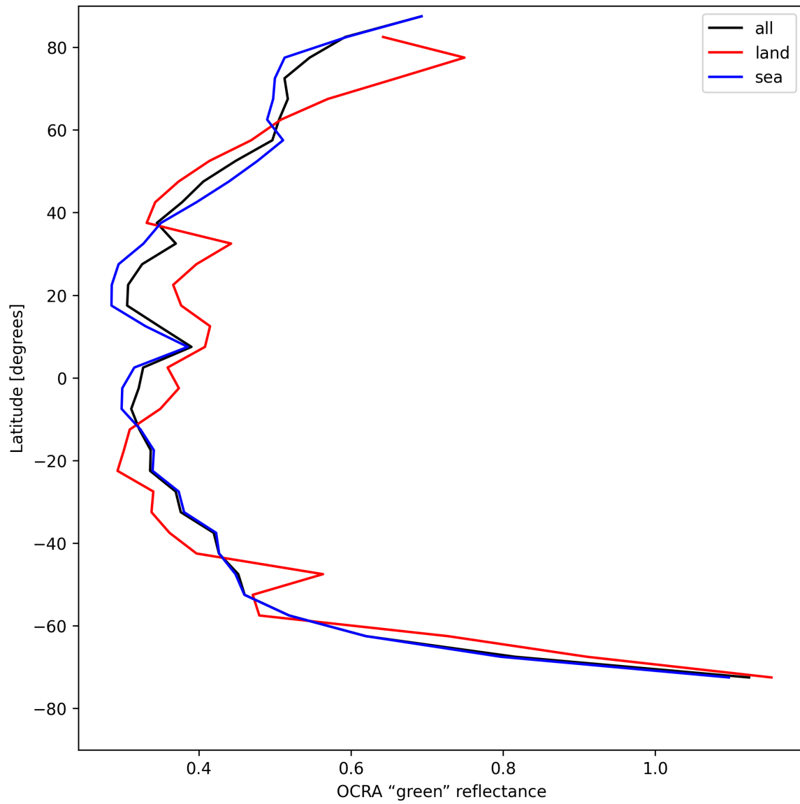
Figure 36: Zonal average of “OCRA “green” reflectance” for 2025-08-09 to 2025-08-11.
