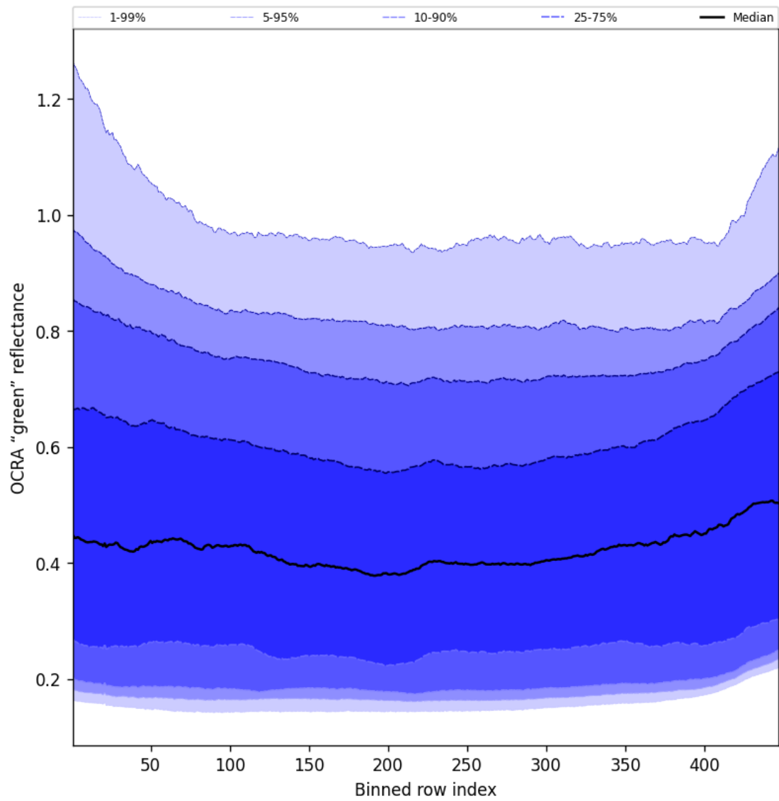
Figure 68: Along track statistics of "OCRA "green" reflectance" for 2025-08-09 to 2025-08-11
