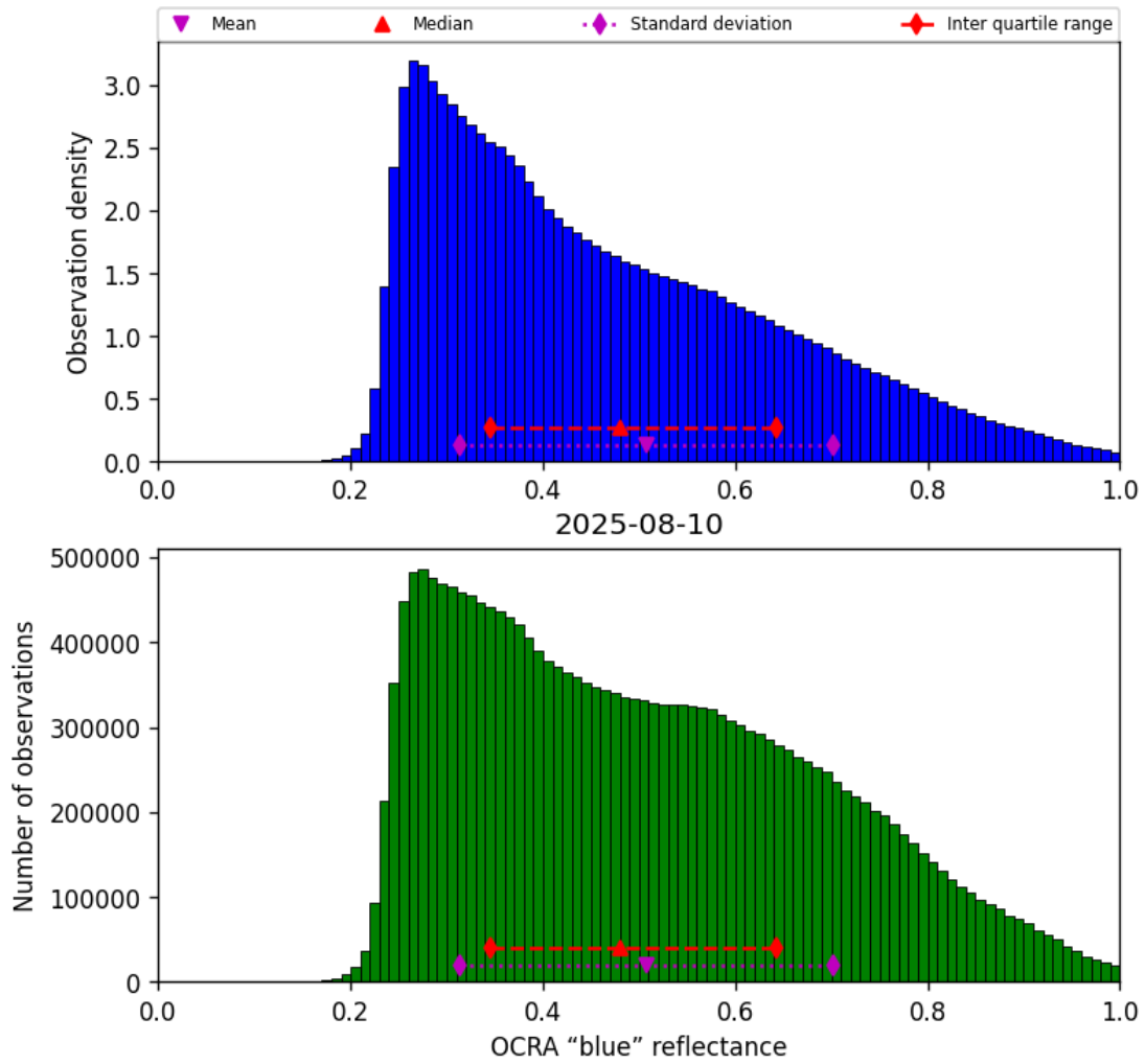
Figure 51: Histogram of “OCRA “blue” reflectance” for 2025-08-09 to 2025-08-11
