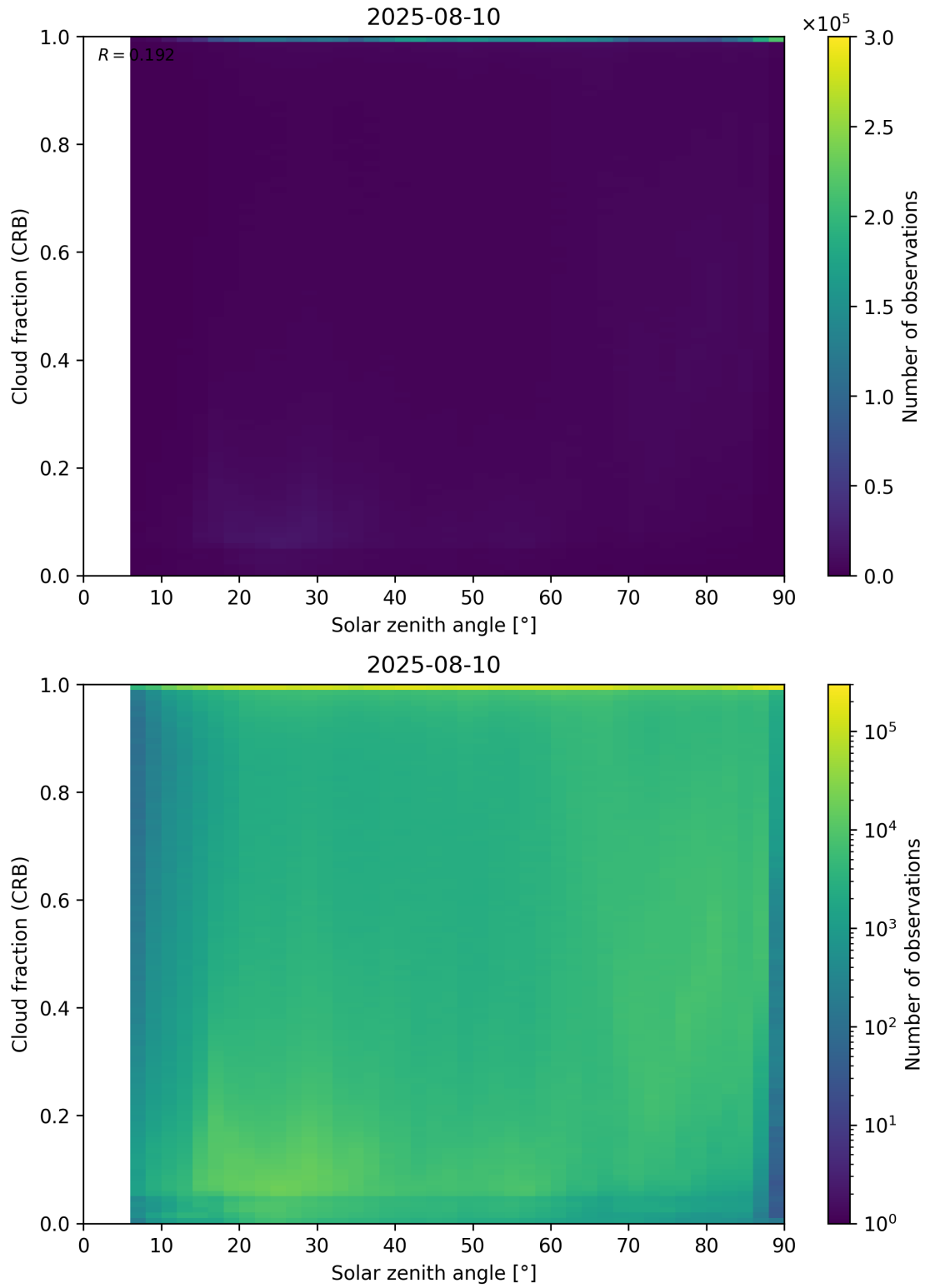
Figure 101: Scatter density plot of “Solar zenith angle” against “Cloud fraction (CRB)” for 2025-08-09 to 2025-08-11.
