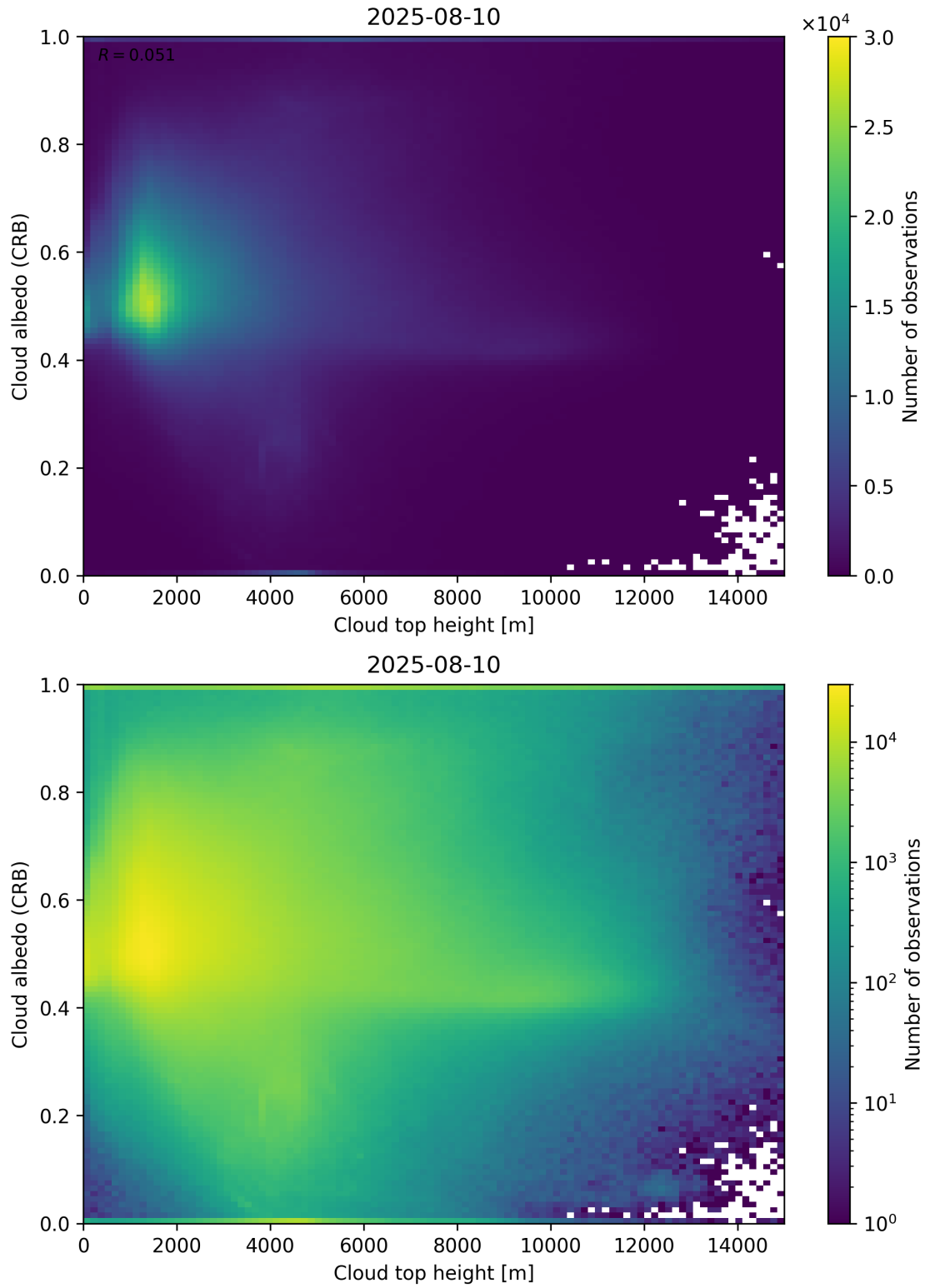
Figure 86: Scatter density plot of “Cloud top height” against “Cloud albedo (CRB)” for 2025-08-09 to 2025-08-11.
