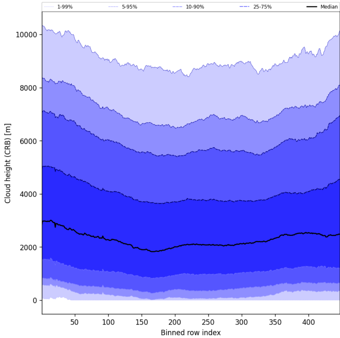
Figure 59: Along track statistics of “Cloud height (CRB)” for 2025-08-09 to 2025-08-11
