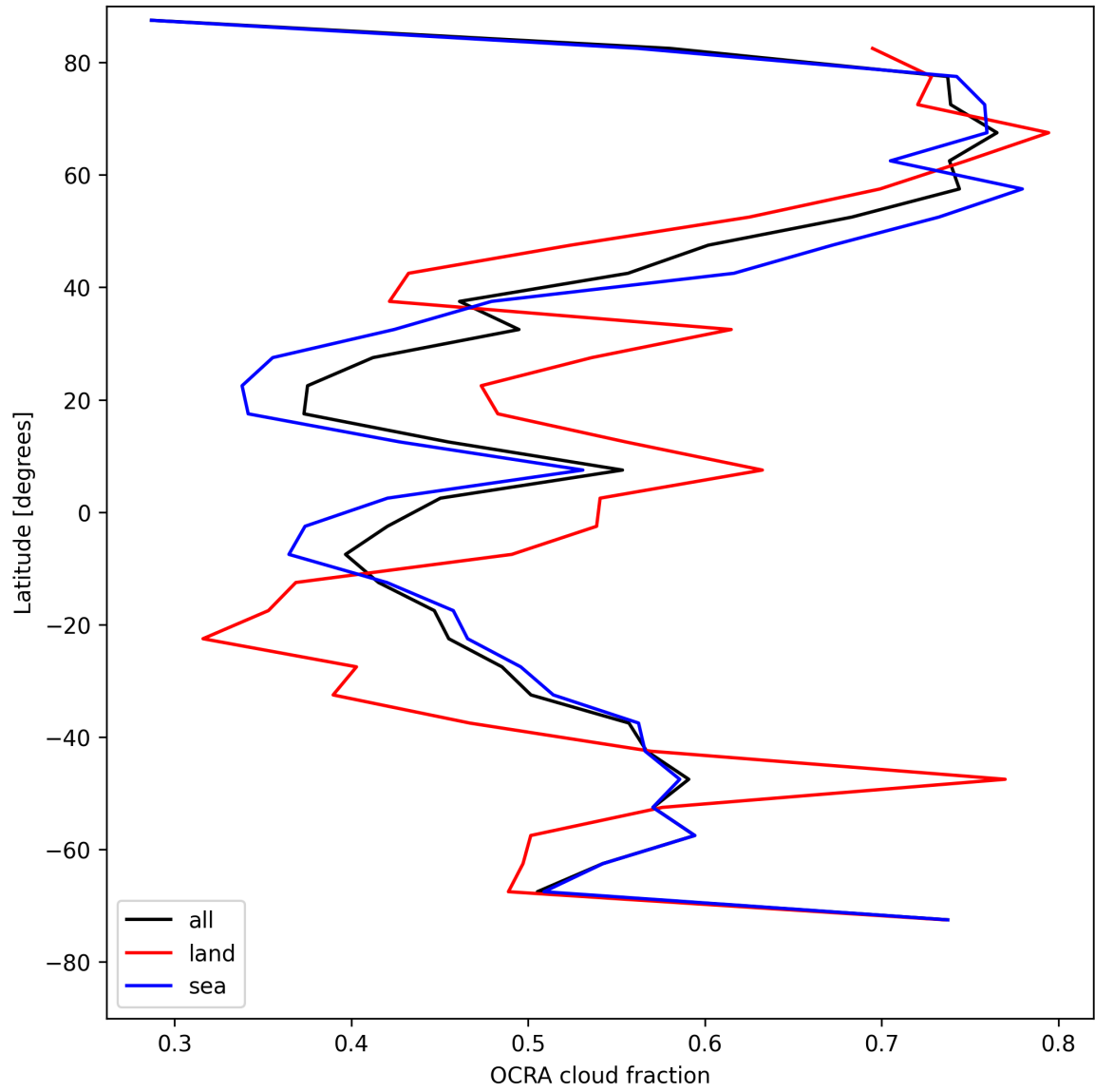
Figure 34: Zonal average of “OCRA cloud fraction” for 2025-08-09 to 2025-08-11.
