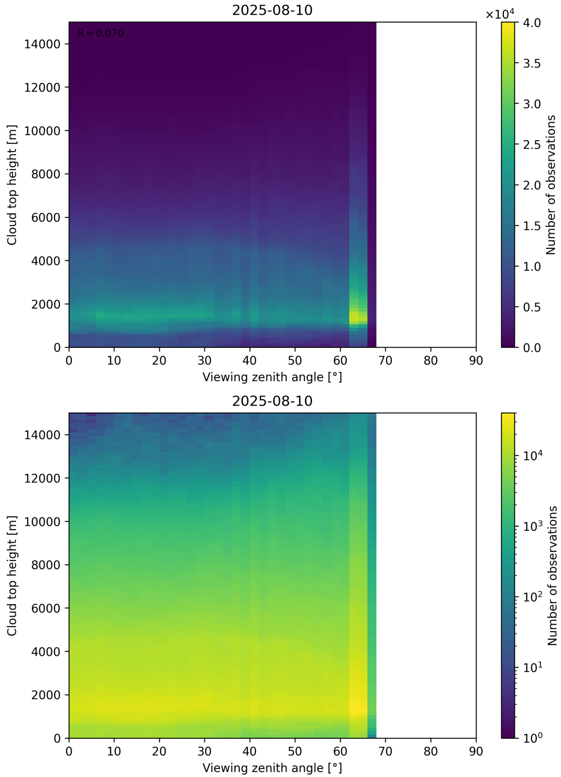
Figure 112: Scatter density plot of “Viewing zenith angle” against “Cloud top height” for 2025-08-09 to 2025-08-11.
