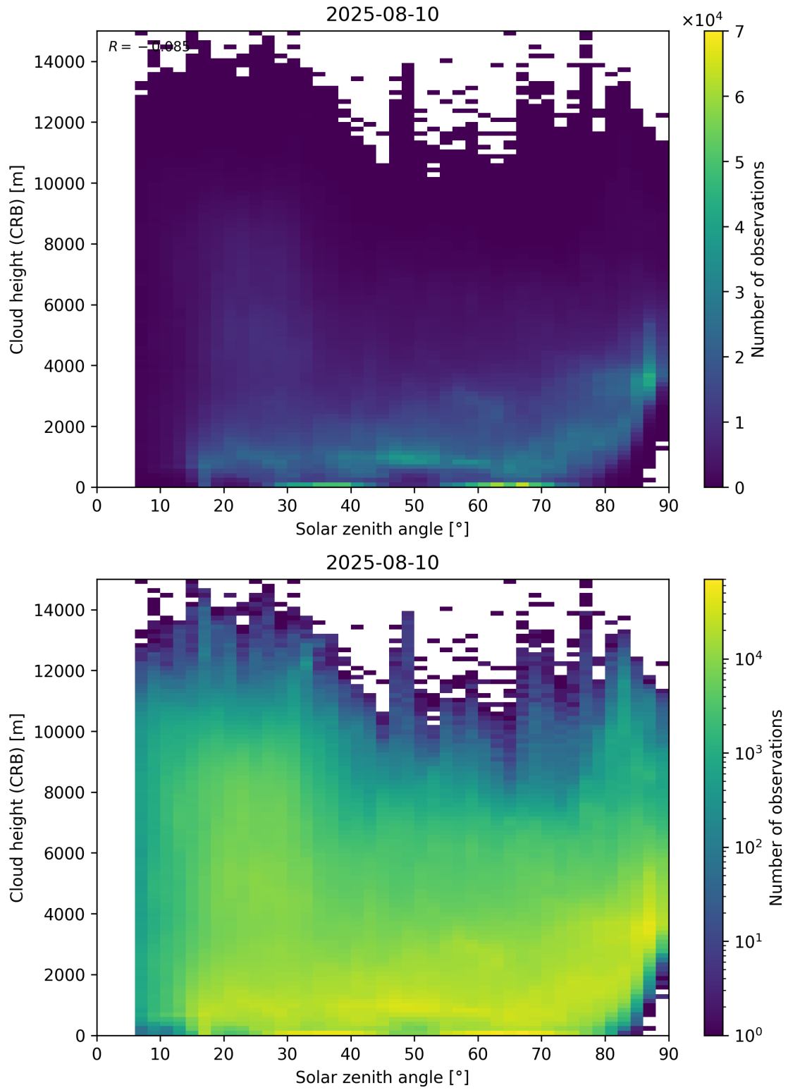
Figure 102: Scatter density plot of “Solar zenith angle” against “Cloud height (CRB)” for 2025-08-09 to 2025-08-11.
