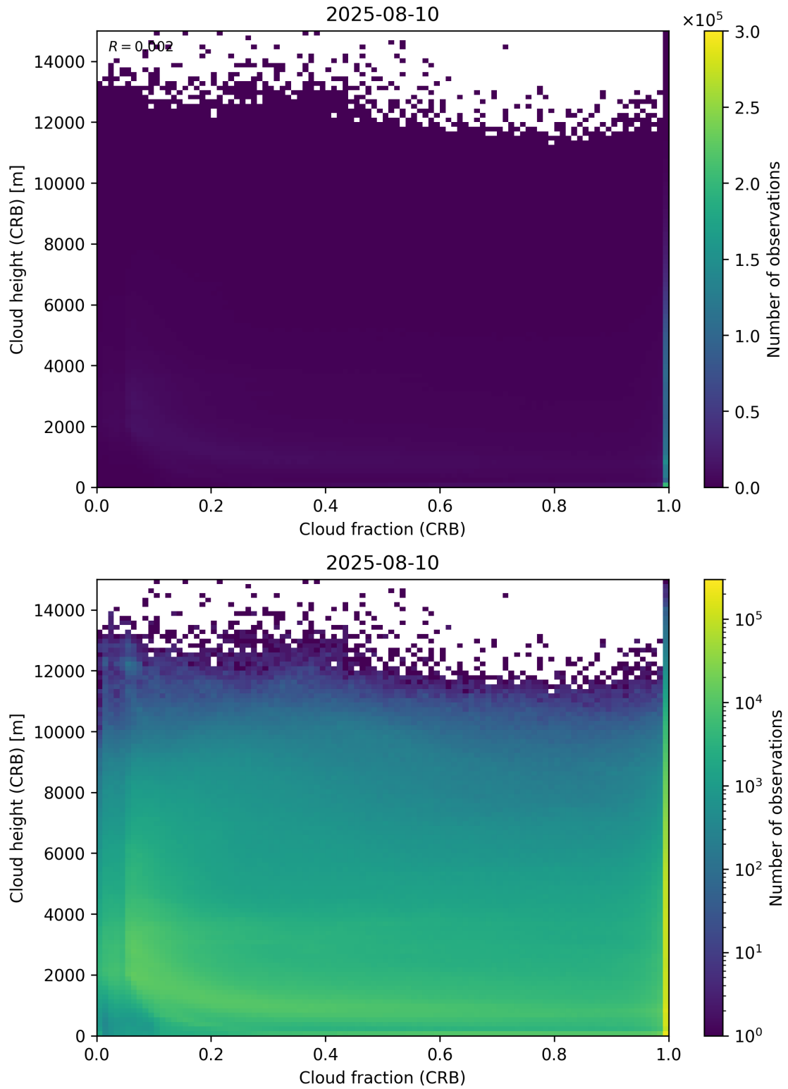
Figure 79: Scatter density plot of “Cloud fraction (CRB)” against “Cloud height (CRB)” for 2025-08-09 to 2025-08-11.
