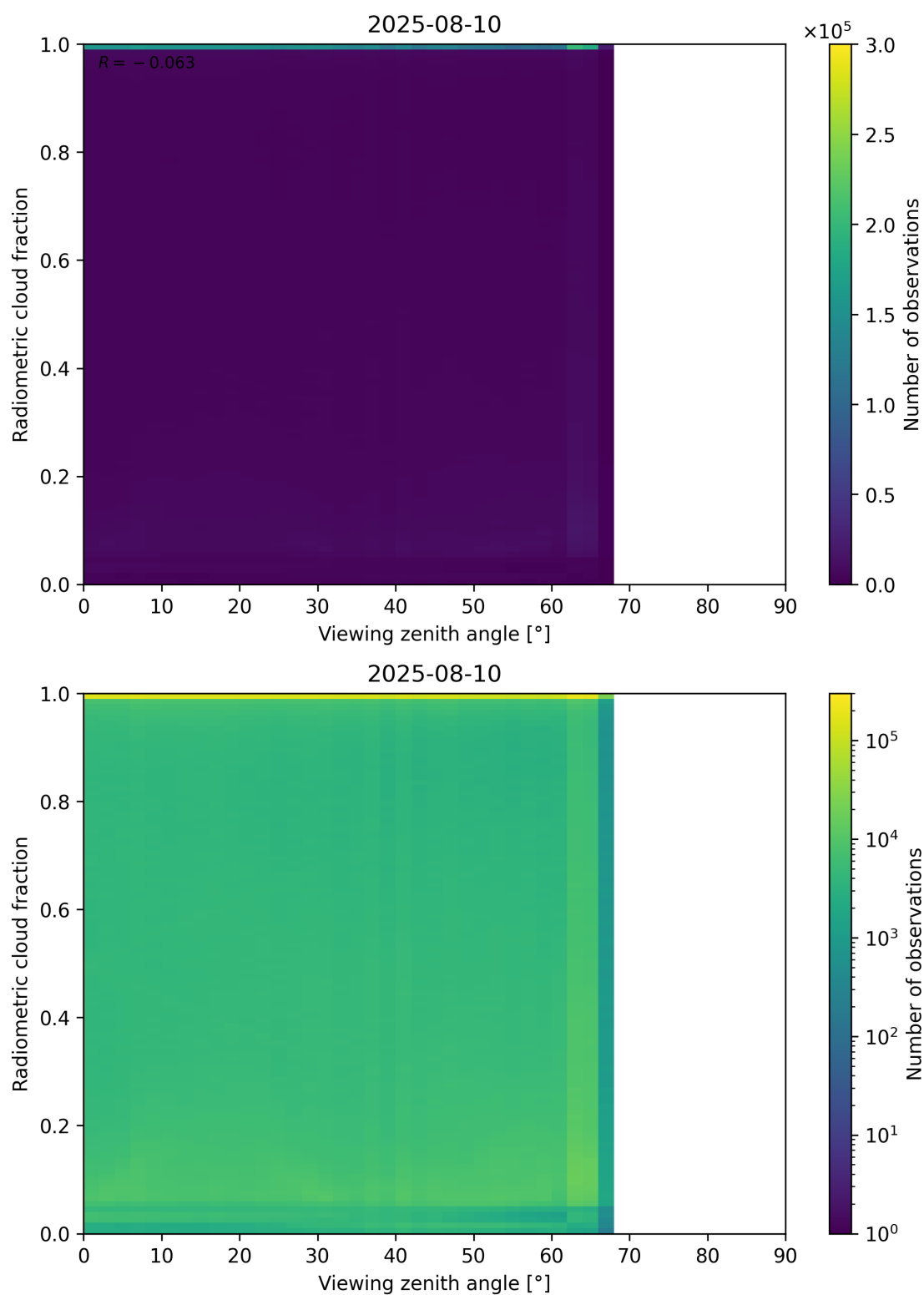
Figure 107: Scatter density plot of “Viewing zenith angle” against “Radiometric cloud fraction” for 2025-08-09 to 2025-08-11.
