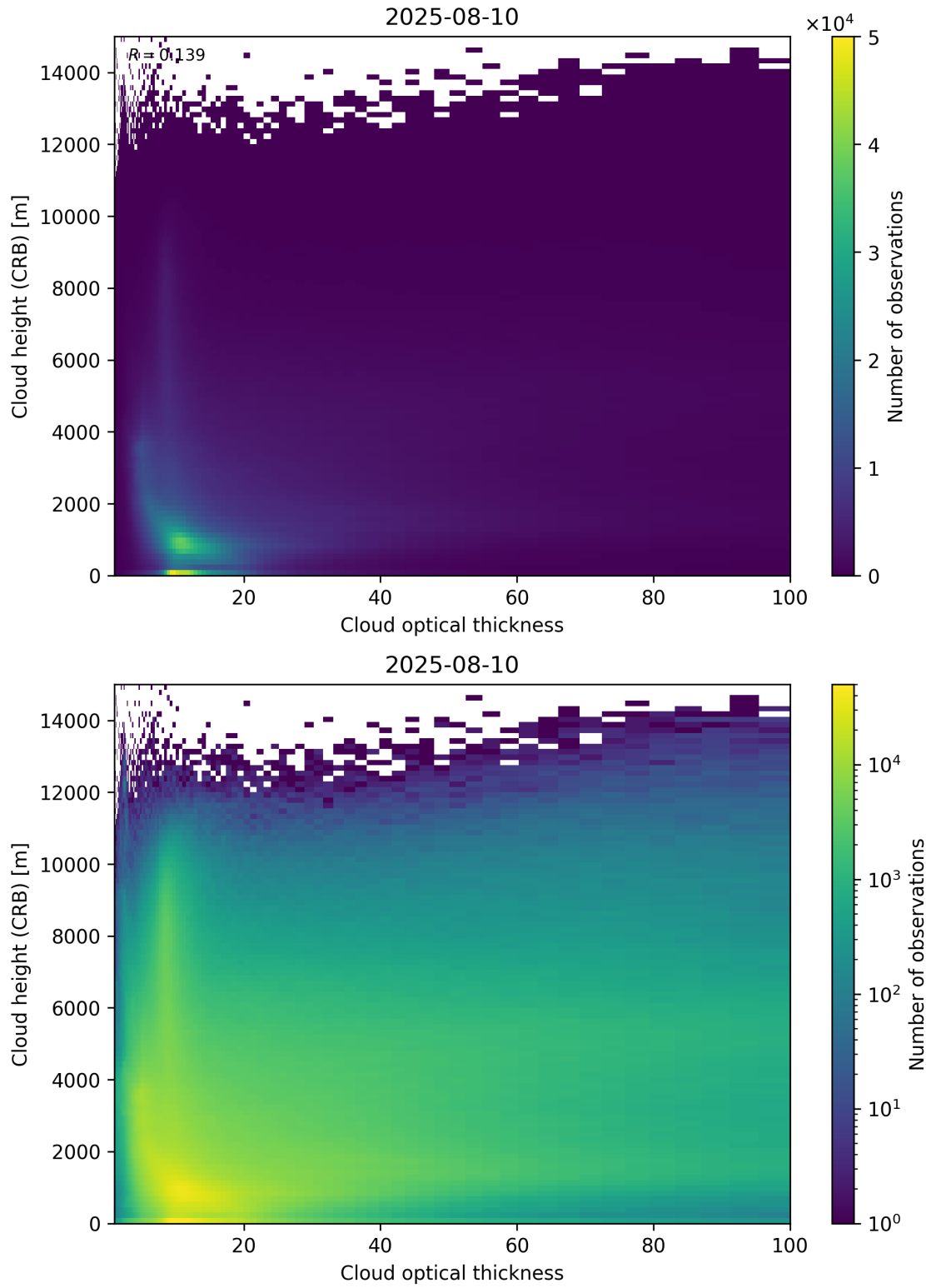
Figure 85: Scatter density plot of “Cloud optical thickness” against “Cloud height (CRB)” for 2025-08-09 to 2025-08-11.
