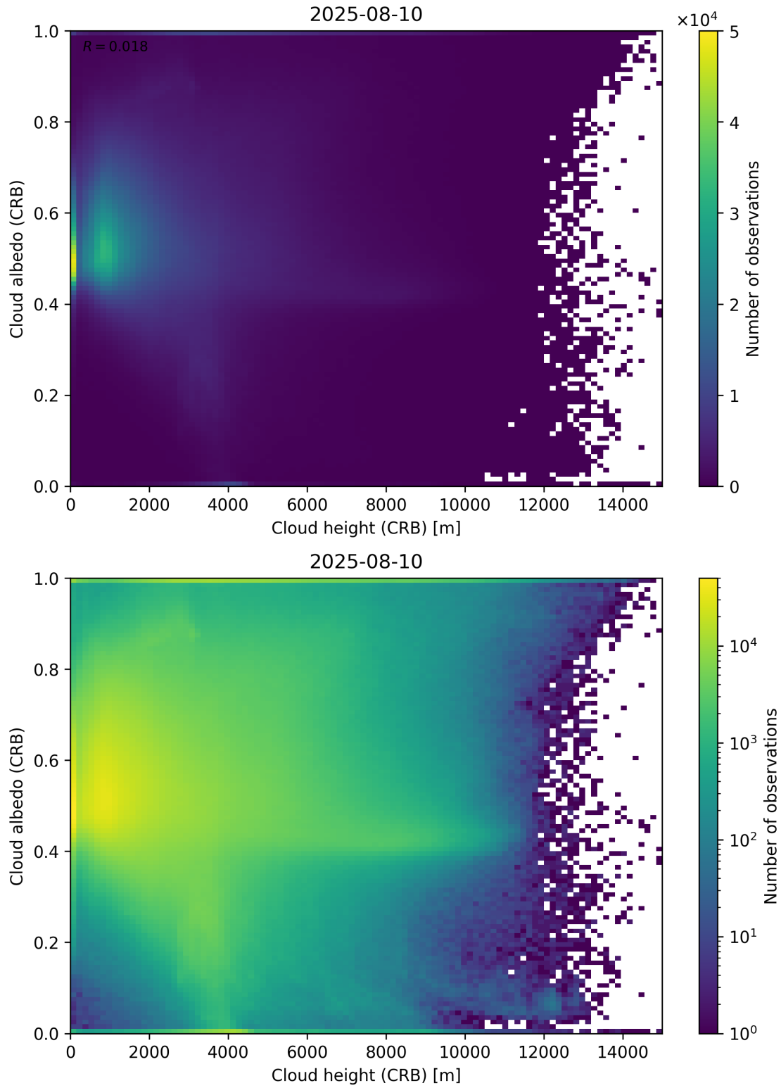
Figure 80: Scatter density plot of “Cloud height (CRB)” against “Cloud albedo (CRB)” for 2025-08-09 to 2025-08-11.
