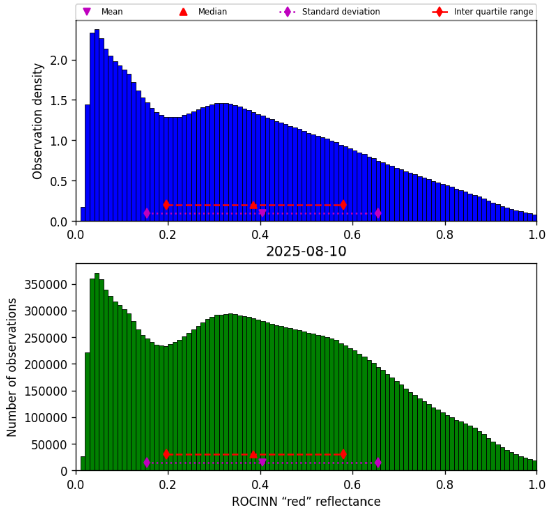
Figure 53: Histogram of “ROCINN “red” reflectance” for 2025-08-09 to 2025-08-11
