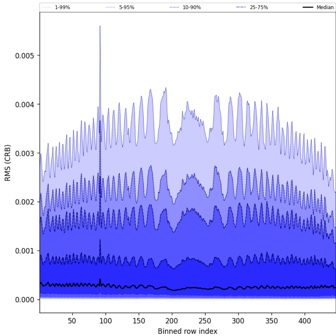
Figure 64: Along track statistics of “RMS (CRB)” for 2025-08-09 to 2025-08-11
