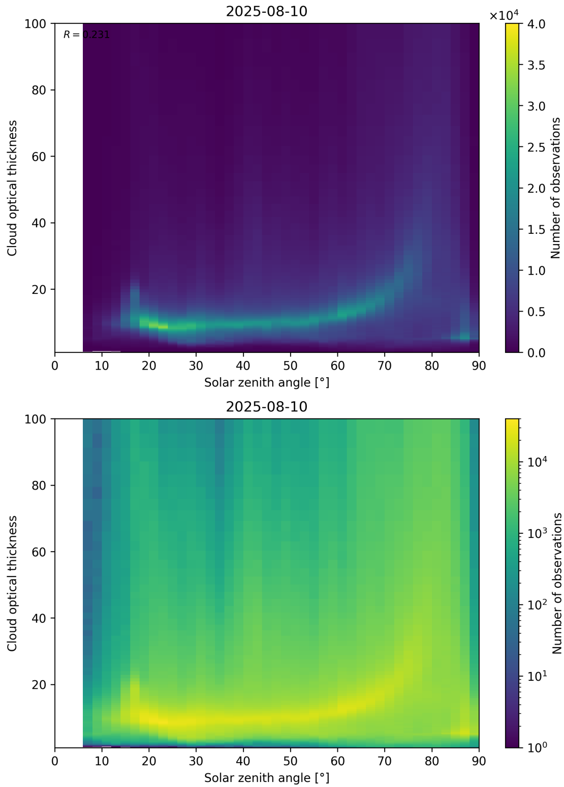
Figure 103: Scatter density plot of “Solar zenith angle” against “Cloud optical thickness” for 2025-08-09 to 2025-08-11.
