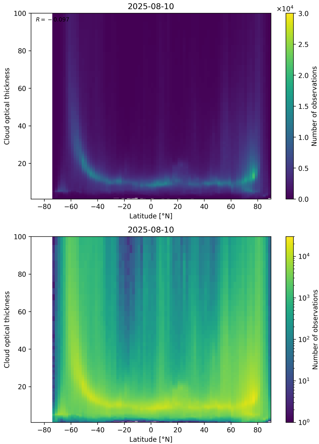
Figure 96: Scatter density plot of “Latitude” against “Cloud optical thickness” for 2025-08-09 to 2025-08-11.
