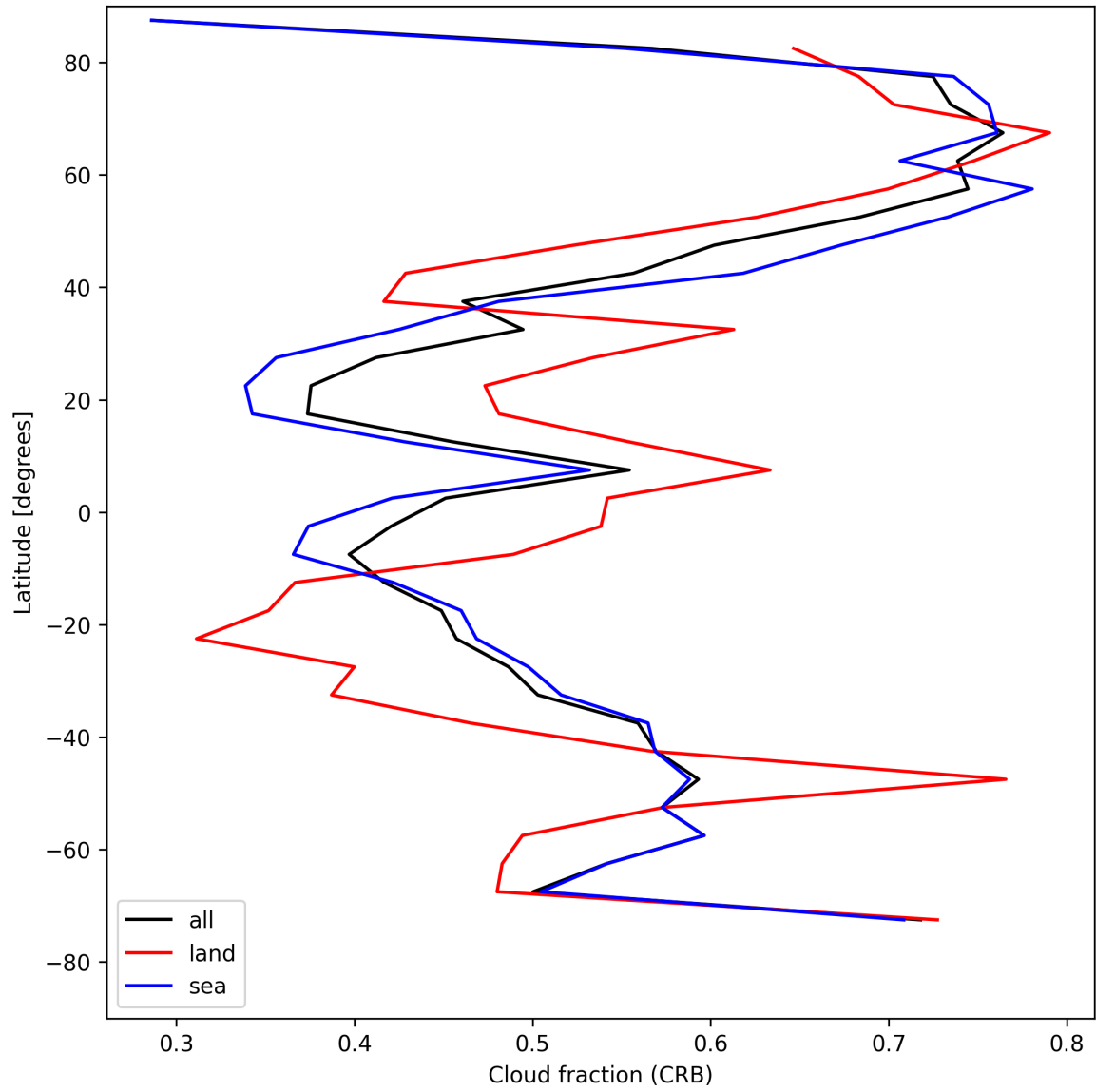
Figure 26: Zonal average of “Cloud fraction (CRB)” for 2025-08-09 to 2025-08-11.
