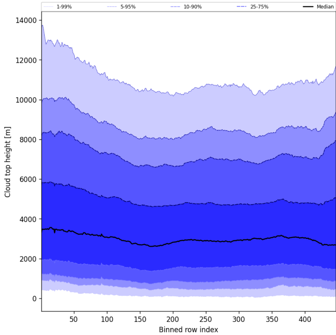
Figure 56: Along track statistics of “Cloud top height” for 2025-08-09 to 2025-08-11
