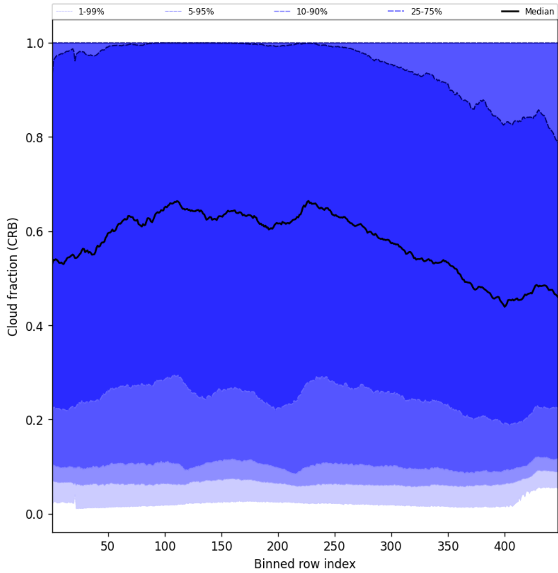
Figure 58: Along track statistics of “Cloud fraction (CRB)” for 2025-08-09 to 2025-08-11
