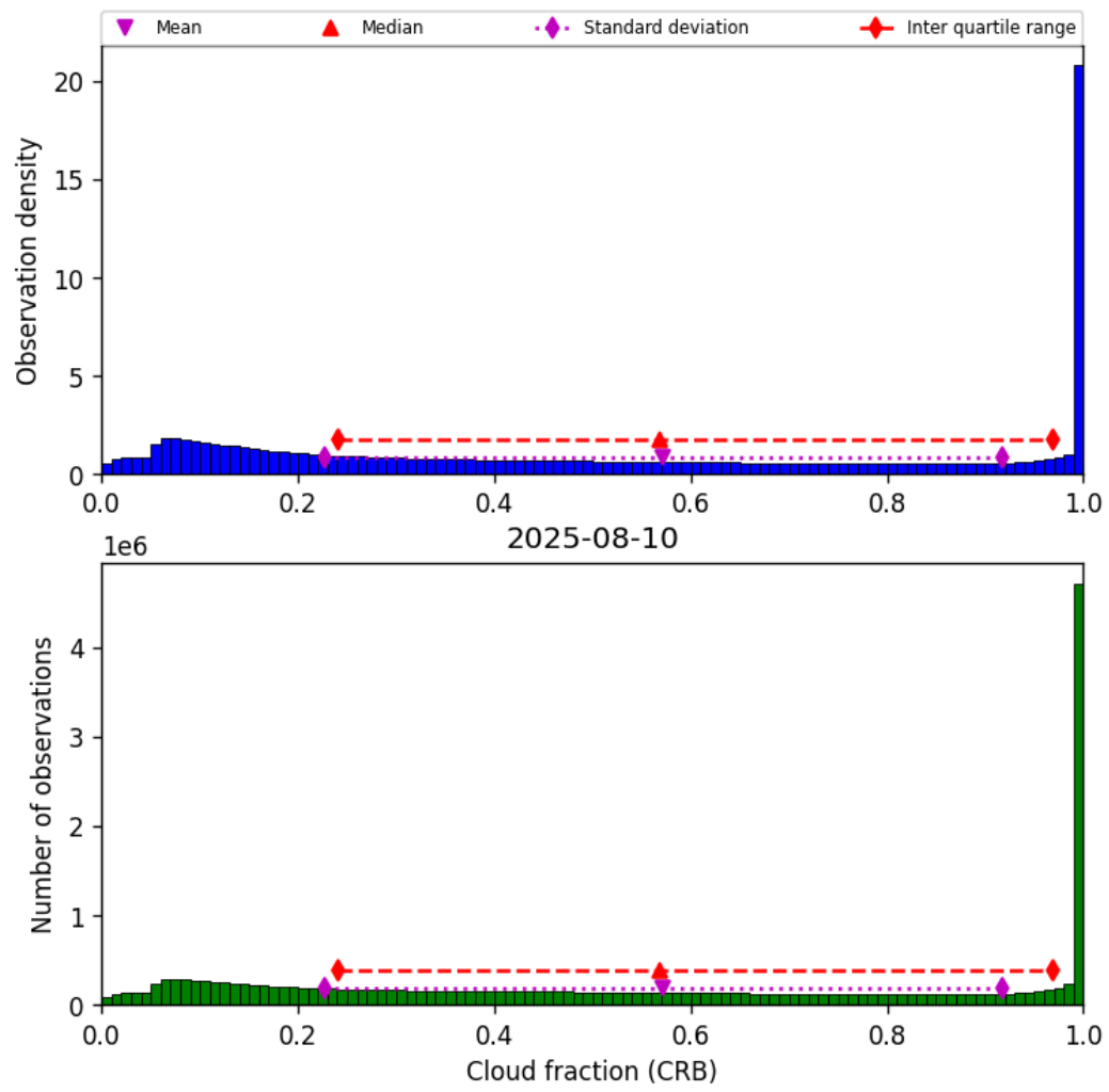
Figure 42: Histogram of “Cloud fraction (CRB)” for 2025-08-09 to 2025-08-11
