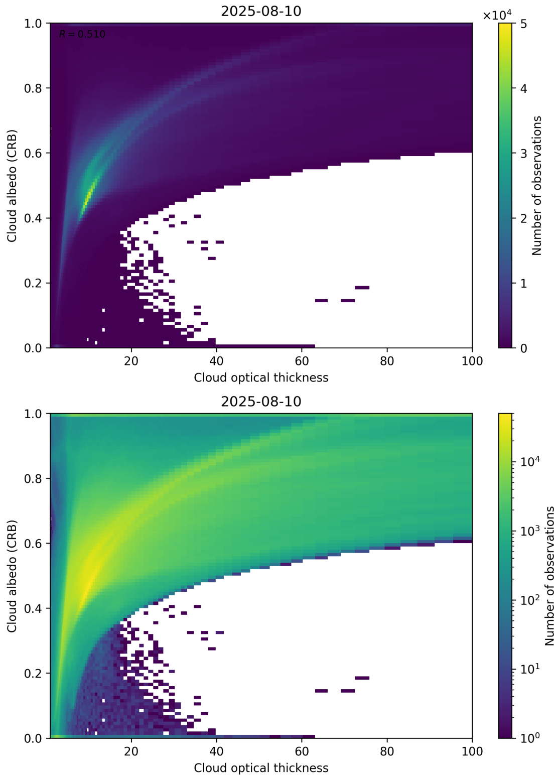
Figure 82: Scatter density plot of “Cloud optical thickness” against “Cloud albedo (CRB)” for 2025-08-09 to 2025-08-11.
