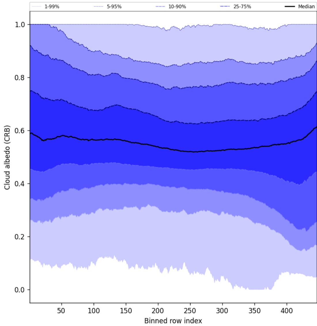
Figure 60: Along track statistics of “Cloud albedo (CRB)” for 2025-08-09 to 2025-08-11
