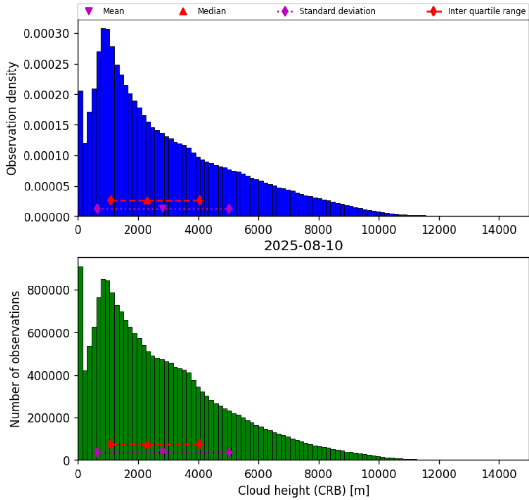
Figure 43: Histogram of “Cloud height (CRB)” for 2025-08-09 to 2025-08-11
