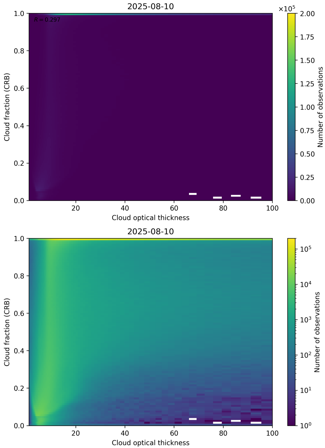
Figure 84: Scatter density plot of “Cloud optical thickness” against “Cloud fraction (CRB)” for 2025-08-09 to 2025-08-11.
