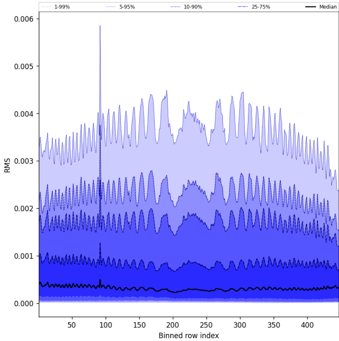
Figure 63: Along track statistics of “RMS” for 2025-08-09 to 2025-08-11
