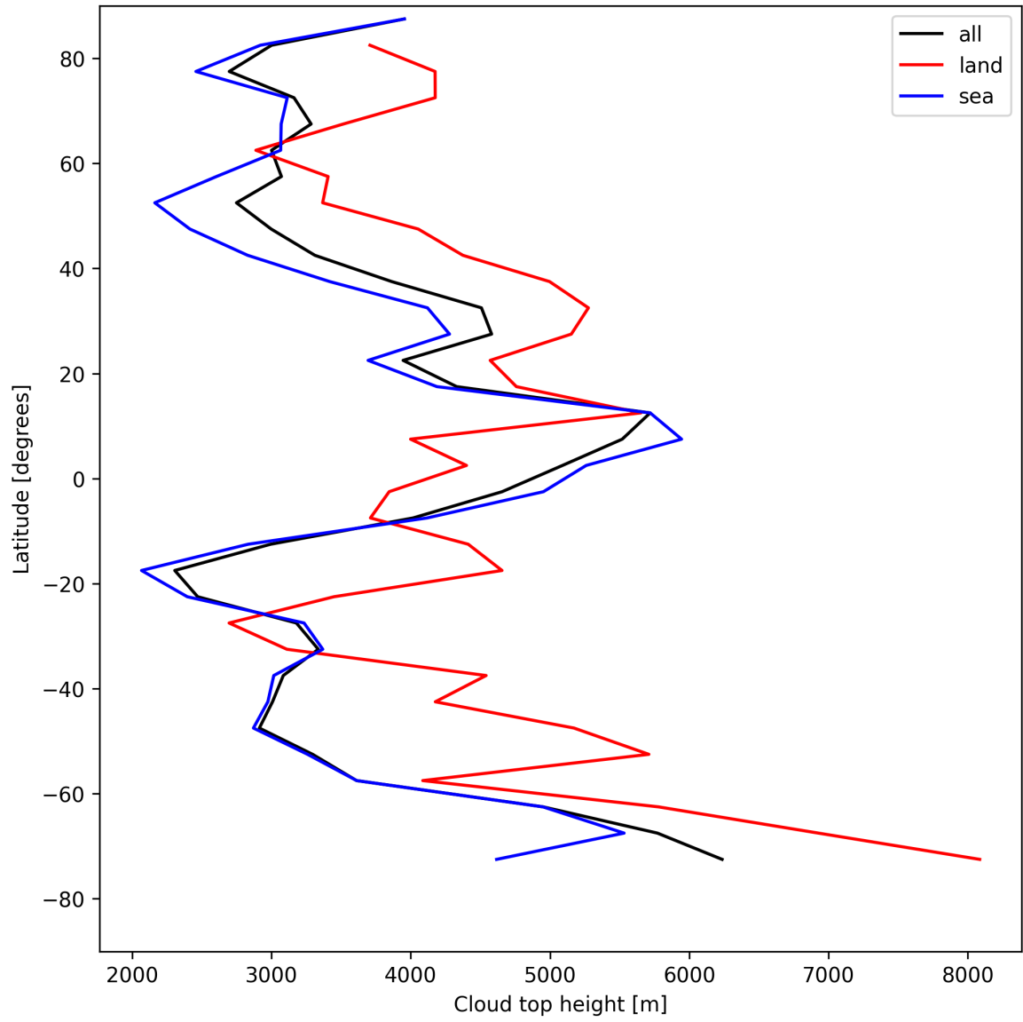
Figure 24: Zonal average of “Cloud top height” for 2025-08-09 to 2025-08-11.
