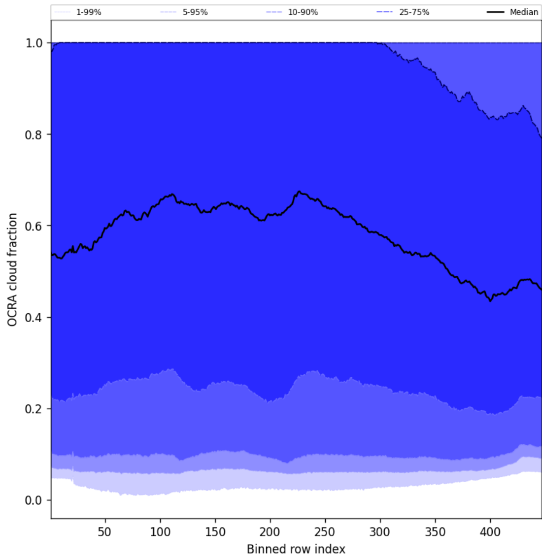
Figure 66: Along track statistics of “OCRA cloud fraction” for 2025-08-09 to 2025-08-11
