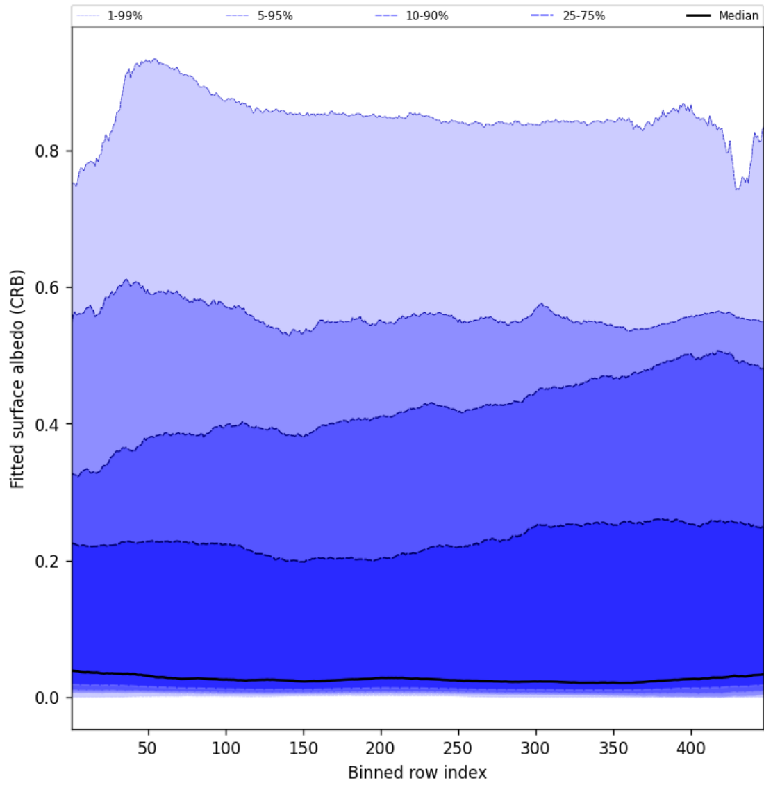
Figure 62: Along track statistics of “Fitted surface albedo (CRB)” for 2025-08-09 to 2025-08-11
