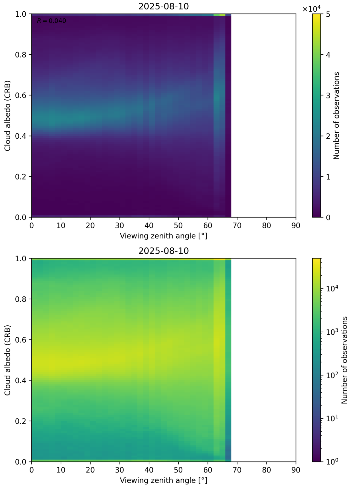
Figure 106: Scatter density plot of “Viewing zenith angle” against “Cloud albedo (CRB)” for 2025-08-09 to 2025-08-11.
