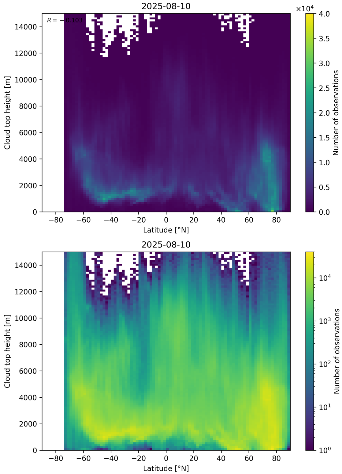
Figure 97: Scatter density plot of “Latitude” against “Cloud top height” for 2025-08-09 to 2025-08-11.
