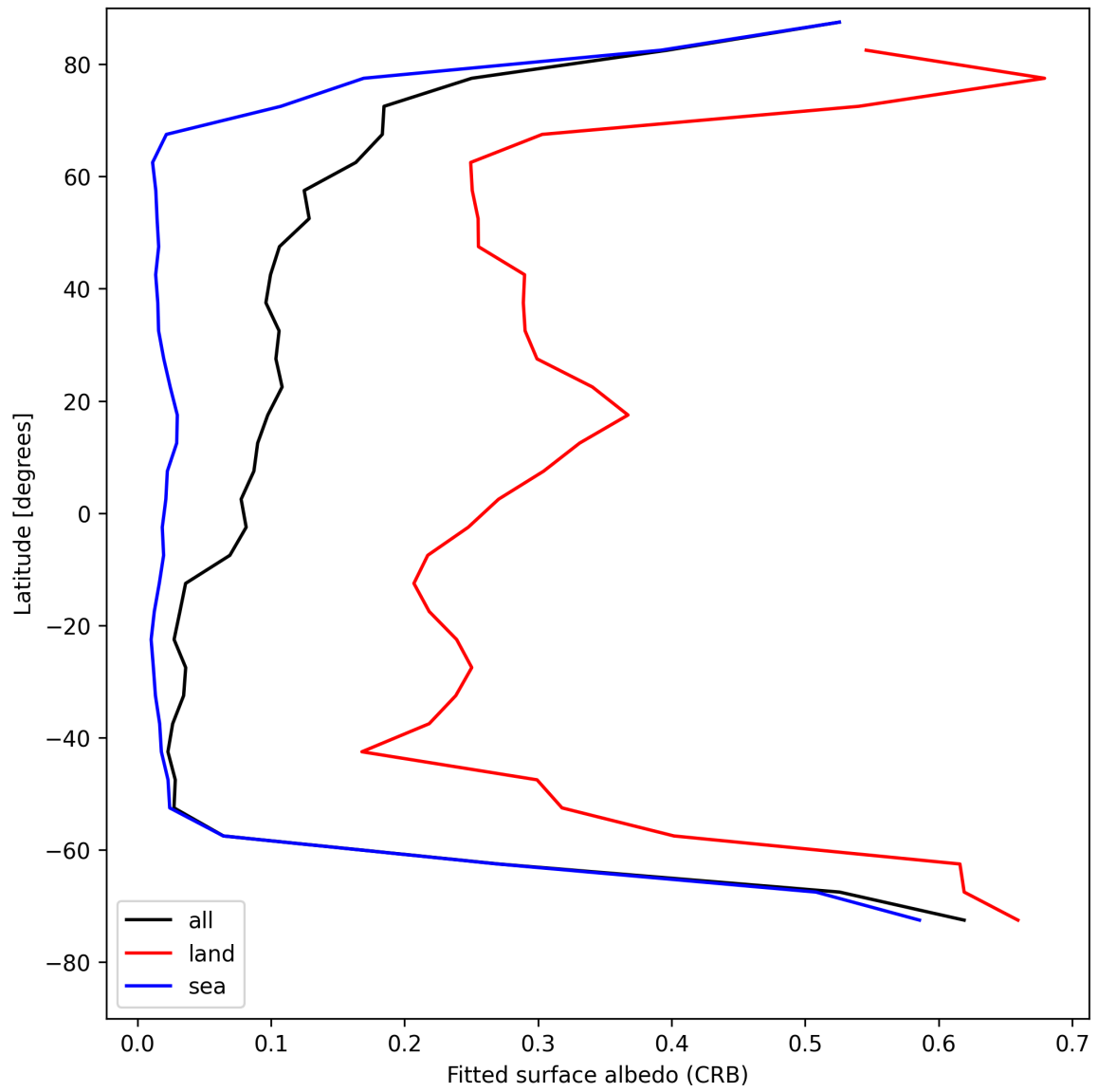
Figure 30: Zonal average of “Fitted surface albedo (CRB)” for 2025-08-09 to 2025-08-11.
