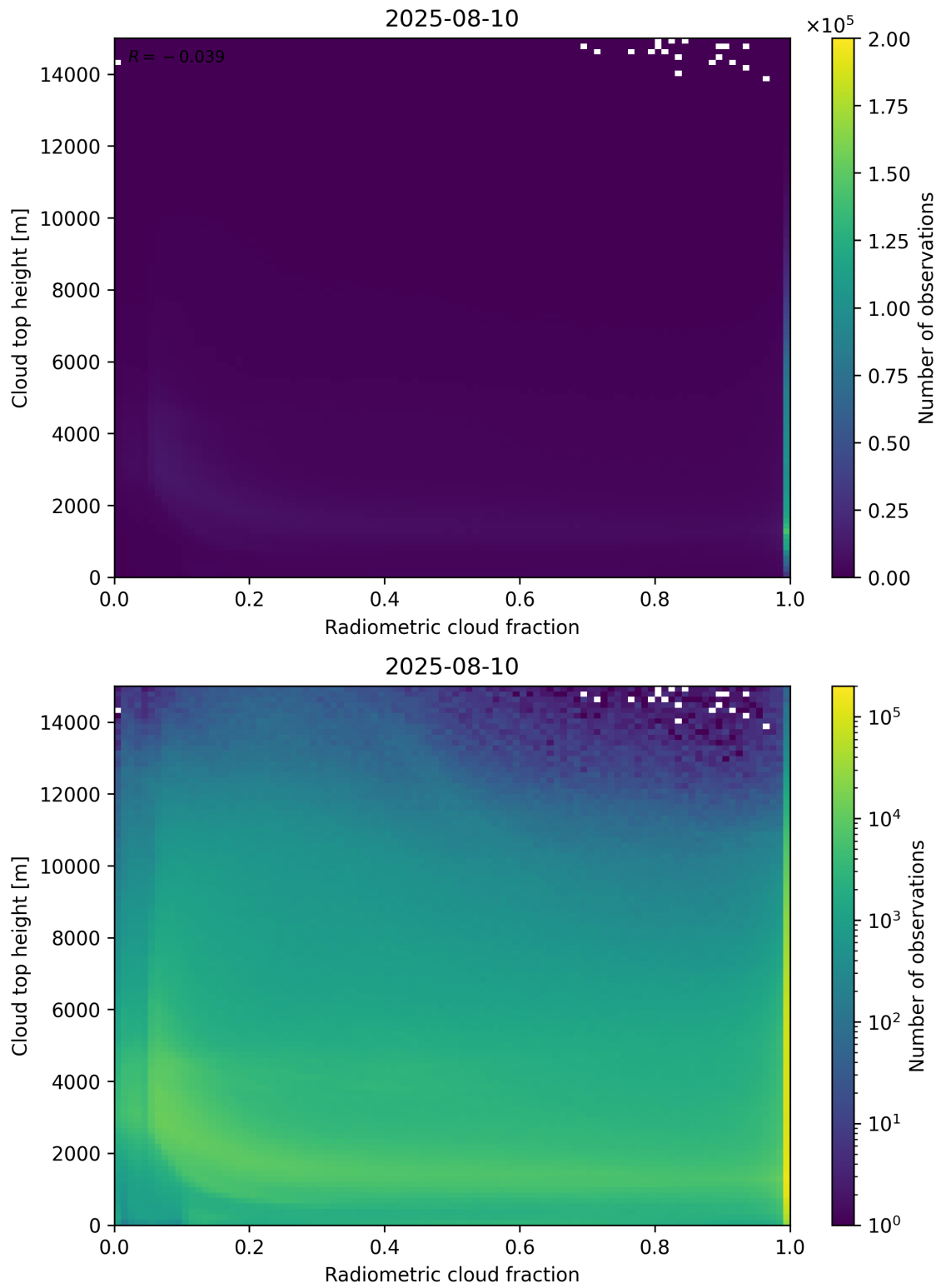
Figure 76: Scatter density plot of “Radiometric cloud fraction” against “Cloud top height” for 2025-08-09 to 2025-08-11.
