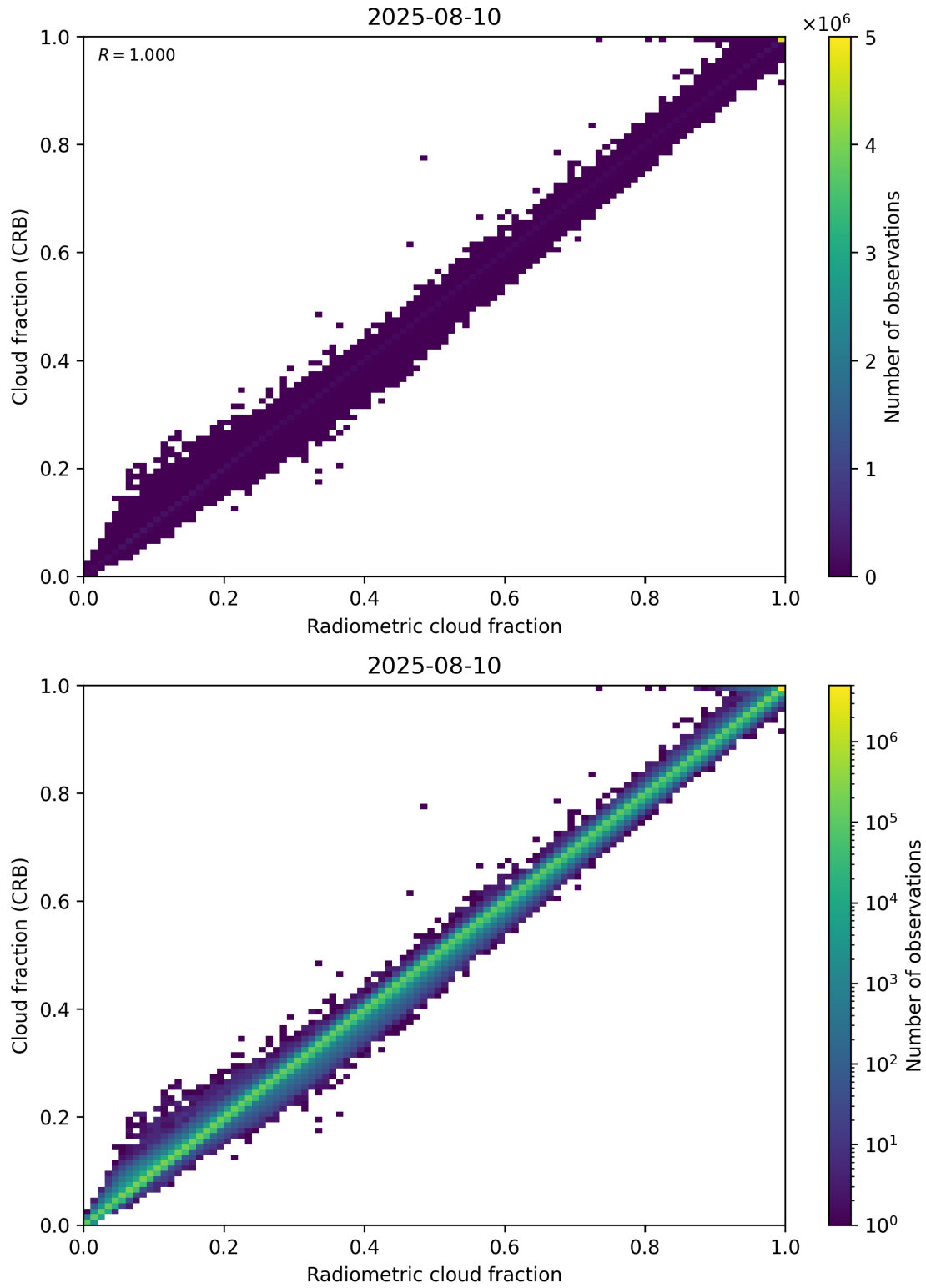
Figure 73: Scatter density plot of “Radiometric cloud fraction” against “Cloud fraction (CRB)” for 2025-08-09 to 2025-08-11.
