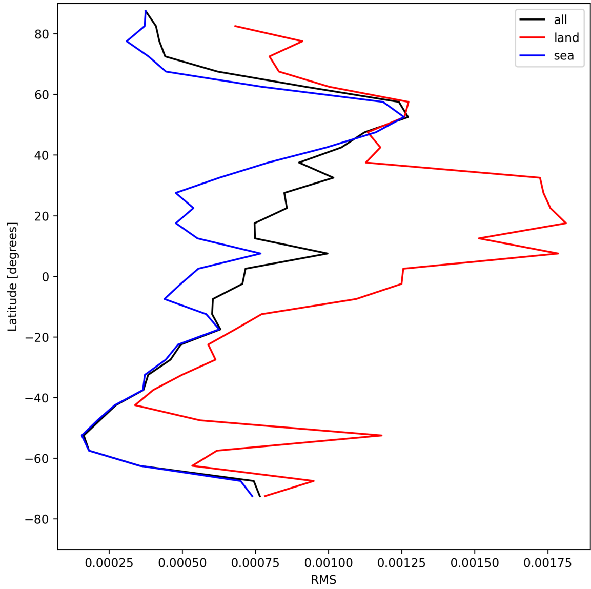
Figure 31: Zonal average of “RMS” for 2025-08-09 to 2025-08-11.
