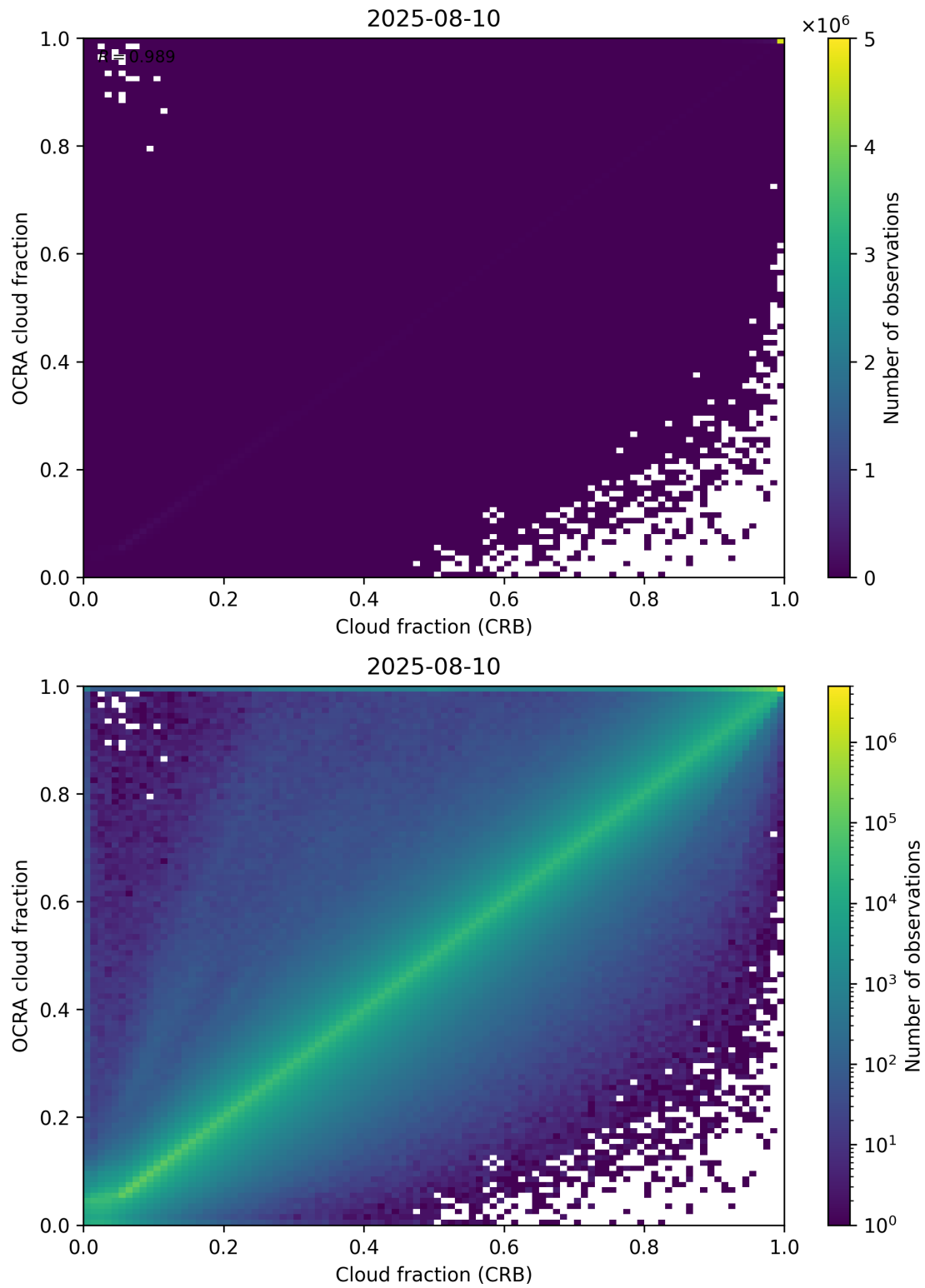
Figure 78: Scatter density plot of “Cloud fraction (CRB)” against “OCRA cloud fraction” for 2025-08-09 to 2025-08-11.
