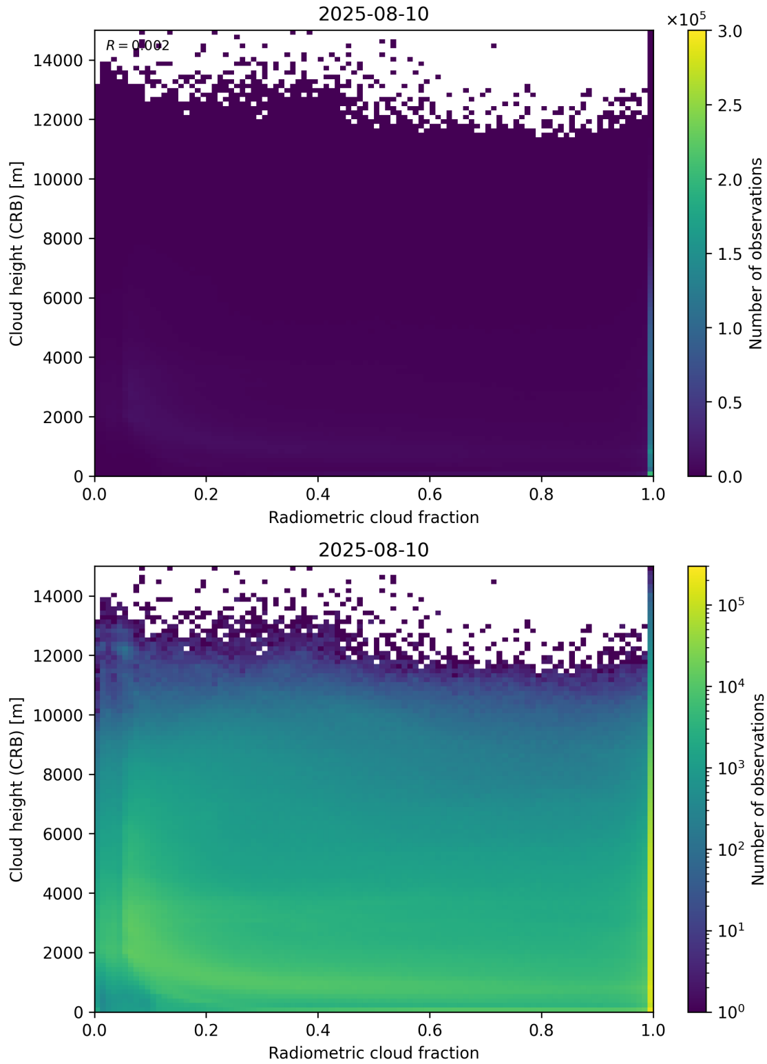
Figure 74: Scatter density plot of “Radiometric cloud fraction” against “Cloud height (CRB)” for 2025-08-09 to 2025-08-11.
