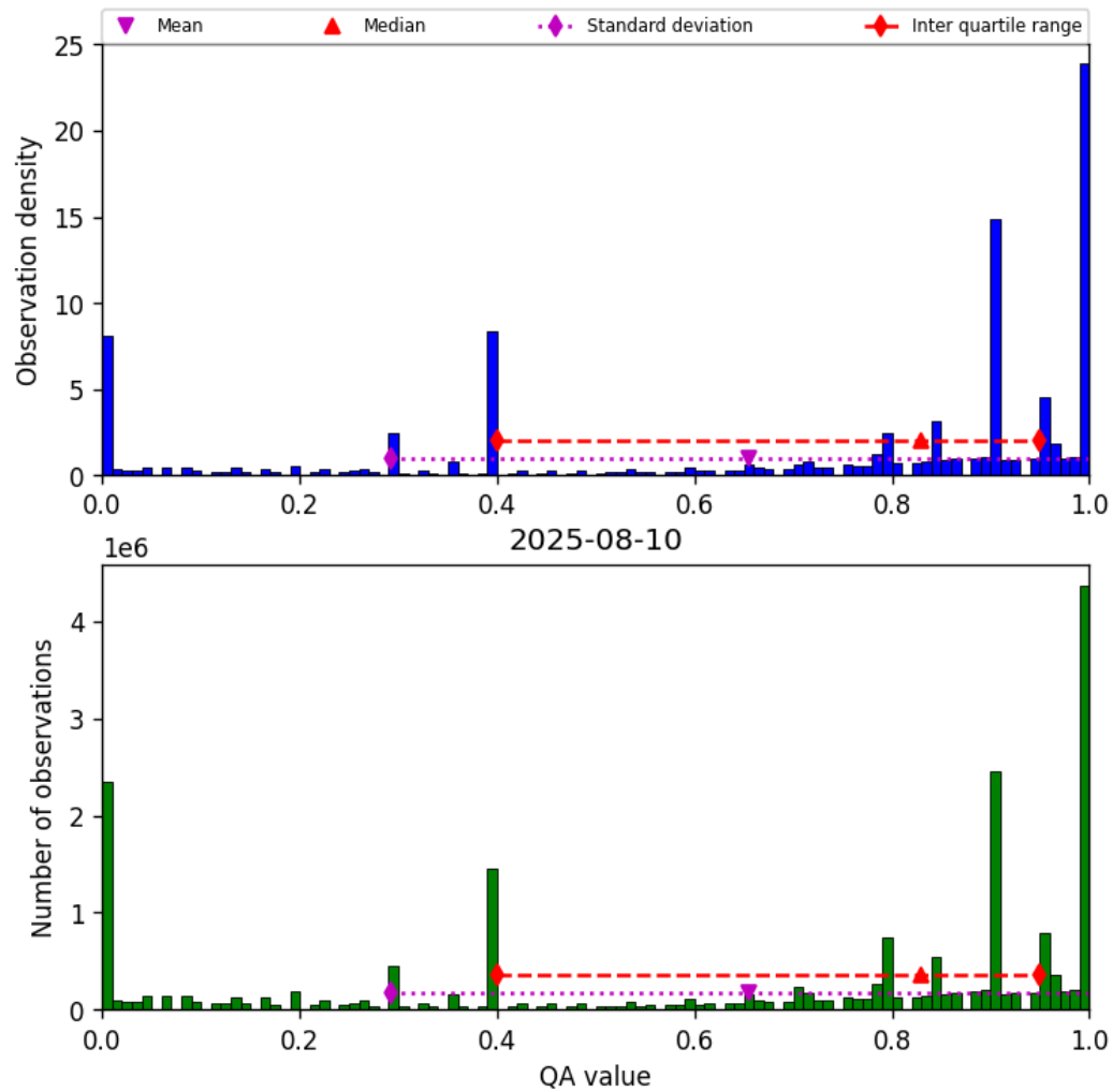
Figure 38: Histogram of “QA value” for 2025-08-09 to 2025-08-11
