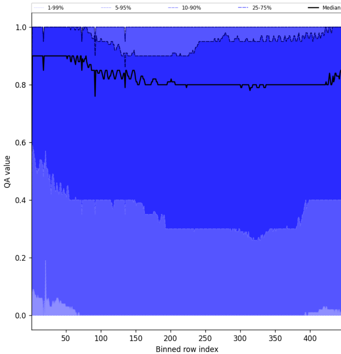
Figure 54: Along track statistics of “QA value” for 2025-08-09 to 2025-08-11
