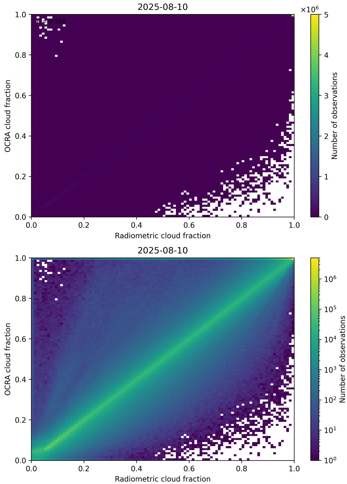
Figure 72: Scatter density plot of “Radiometric cloud fraction” against “OCRA cloud fraction” for 2025-08-09 to 2025-08-11.
