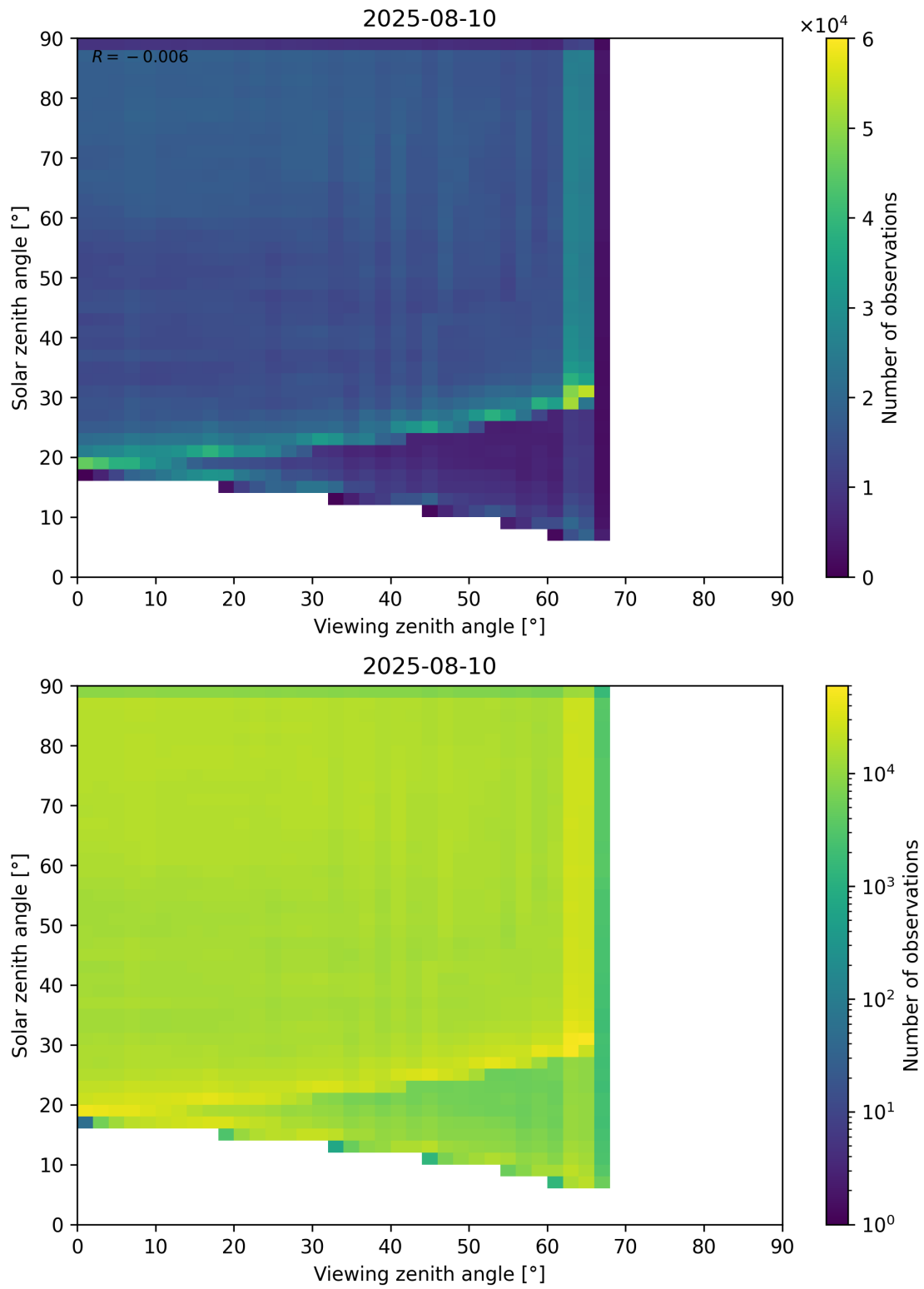
Figure 114: Scatter density plot of “Viewing zenith angle” against “Solar zenith angle” for 2025-08-09 to 2025-08-11.
