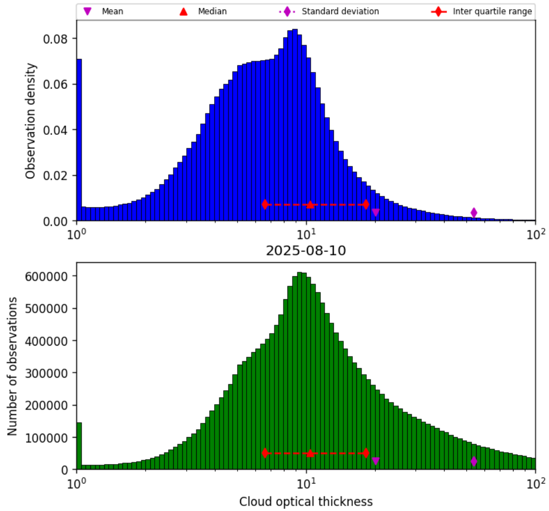
Figure 41: Histogram of “Cloud optical thickness” for 2025-08-09 to 2025-08-11
