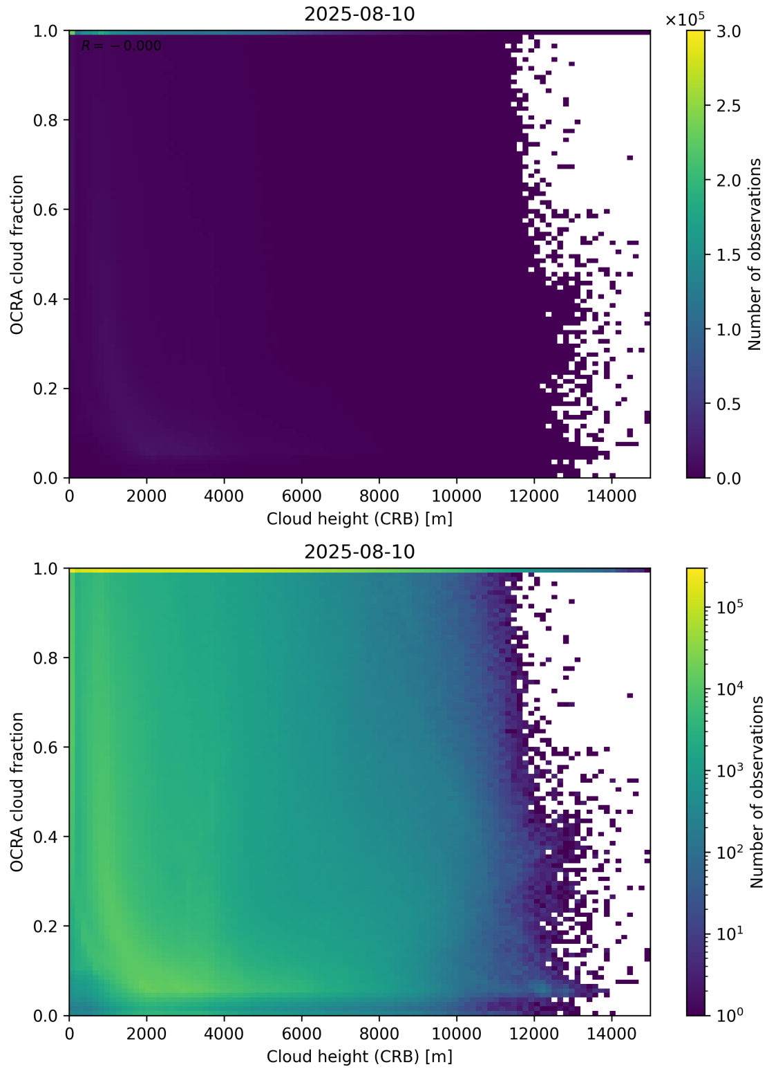
Figure 81: Scatter density plot of “Cloud height (CRB)” against “OCRA cloud fraction” for 2025-08-09 to 2025-08-11.
