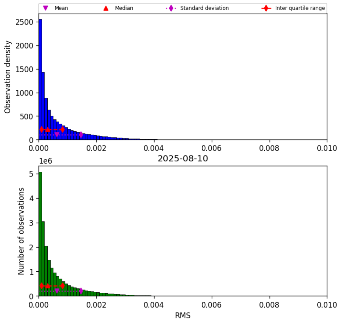
Figure 47: Histogram of “RMS” for 2025-08-09 to 2025-08-11
