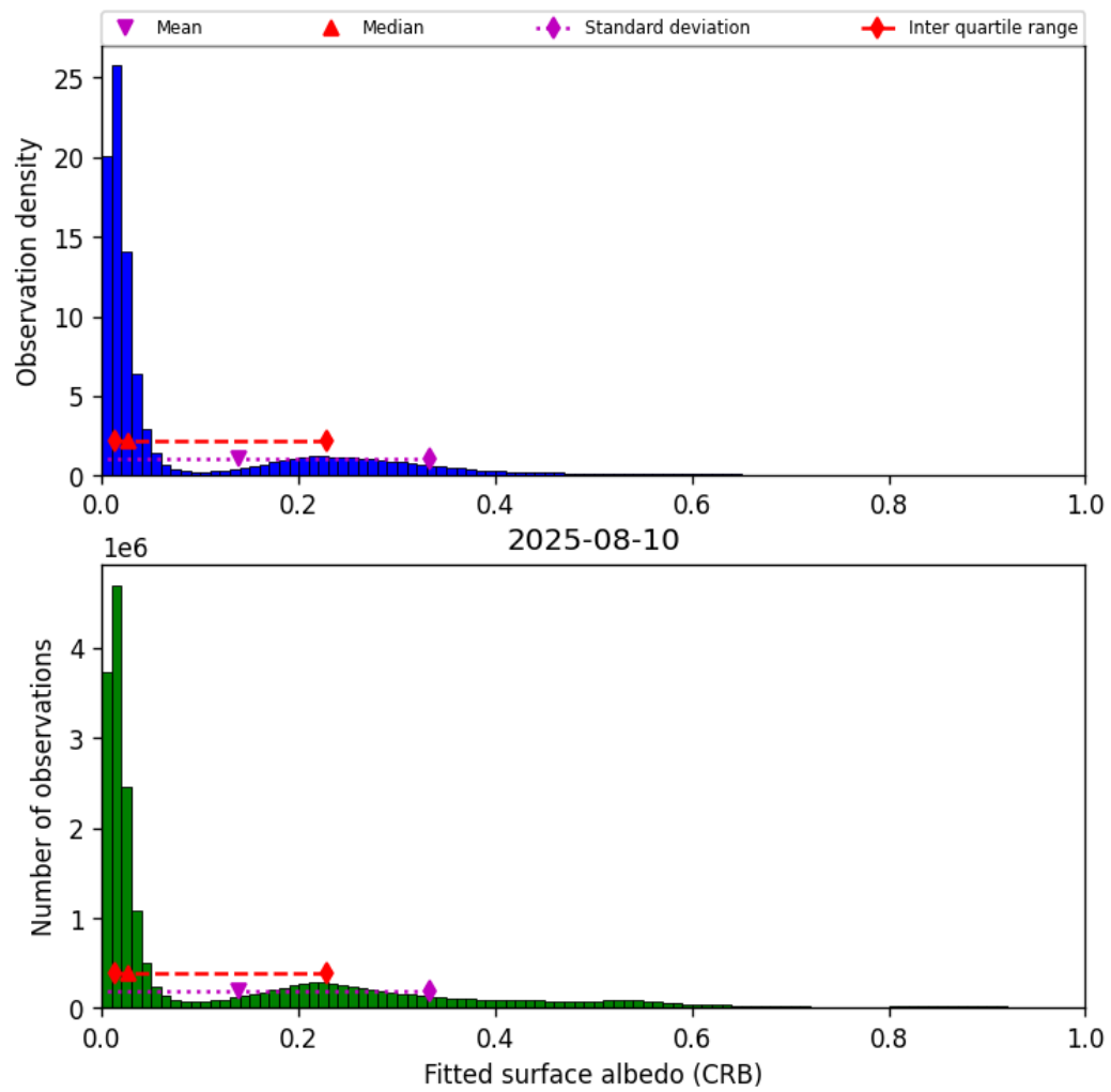
Figure 46: Histogram of “Fitted surface albedo (CRB)” for 2025-08-09 to 2025-08-11
