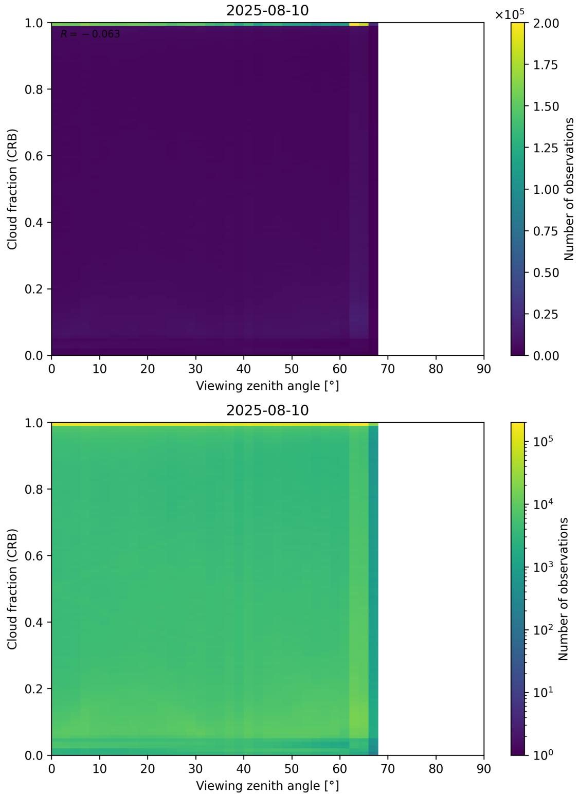
Figure 109: Scatter density plot of “Viewing zenith angle” against “Cloud fraction (CRB)” for 2025-08-09 to 2025-08-11.
