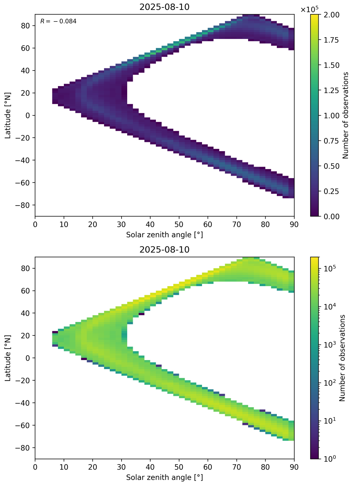
Figure 105: Scatter density plot of “Solar zenith angle” against “Latitude” for 2025-08-09 to 2025-08-11.
