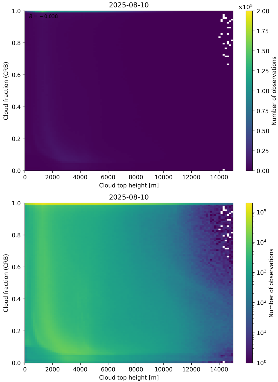
Figure 88: Scatter density plot of “Cloud top height” against “Cloud fraction (CRB)” for 2025-08-09 to 2025-08-11.
