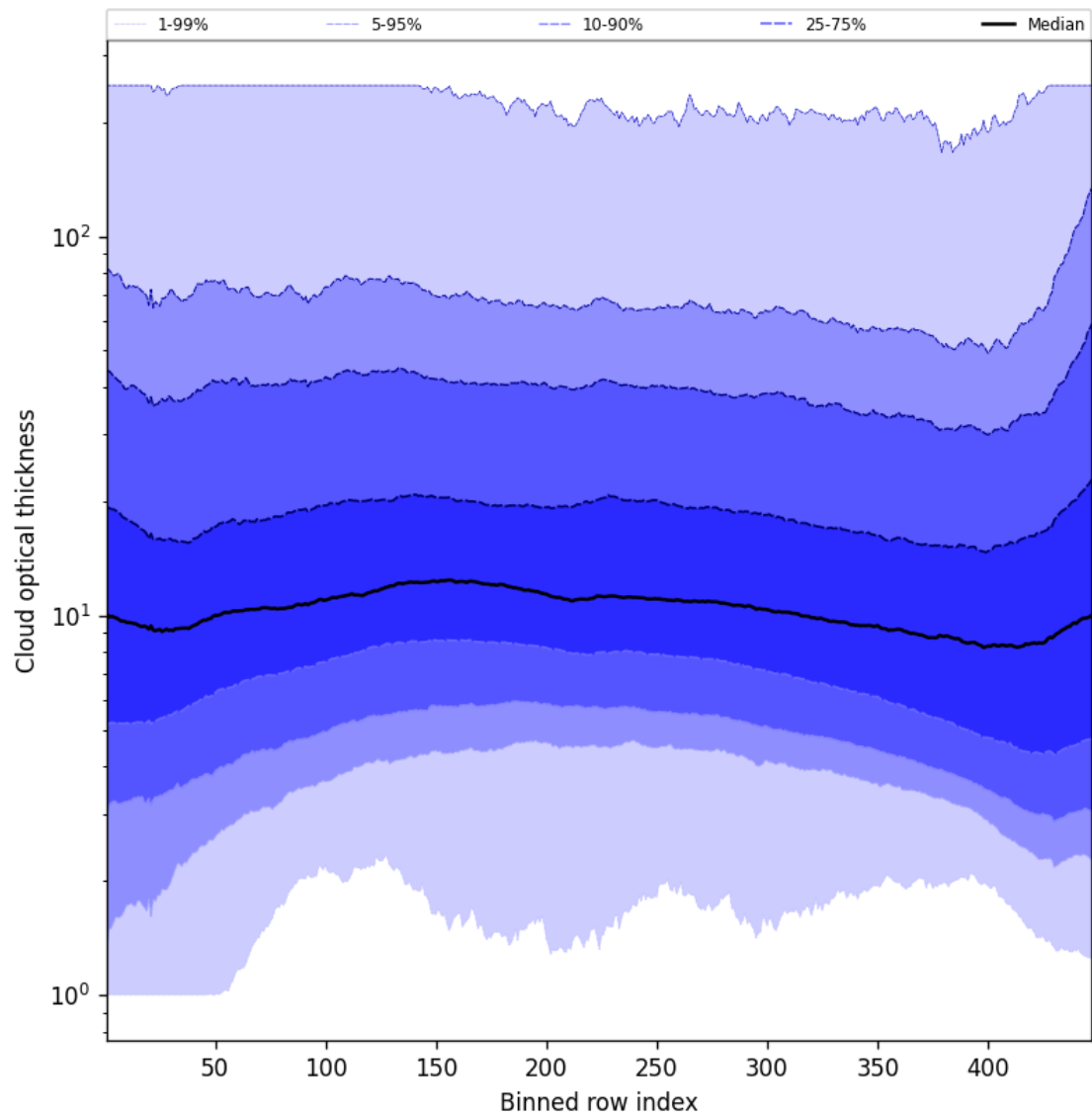
Figure 57: Along track statistics of “Cloud optical thickness” for 2025-08-09 to 2025-08-11
