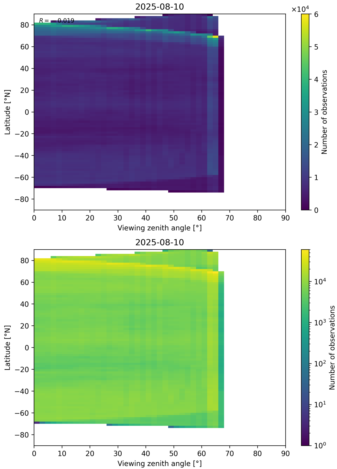
Figure 113: Scatter density plot of “Viewing zenith angle” against “Latitude” for 2025-08-09 to 2025-08-11.
