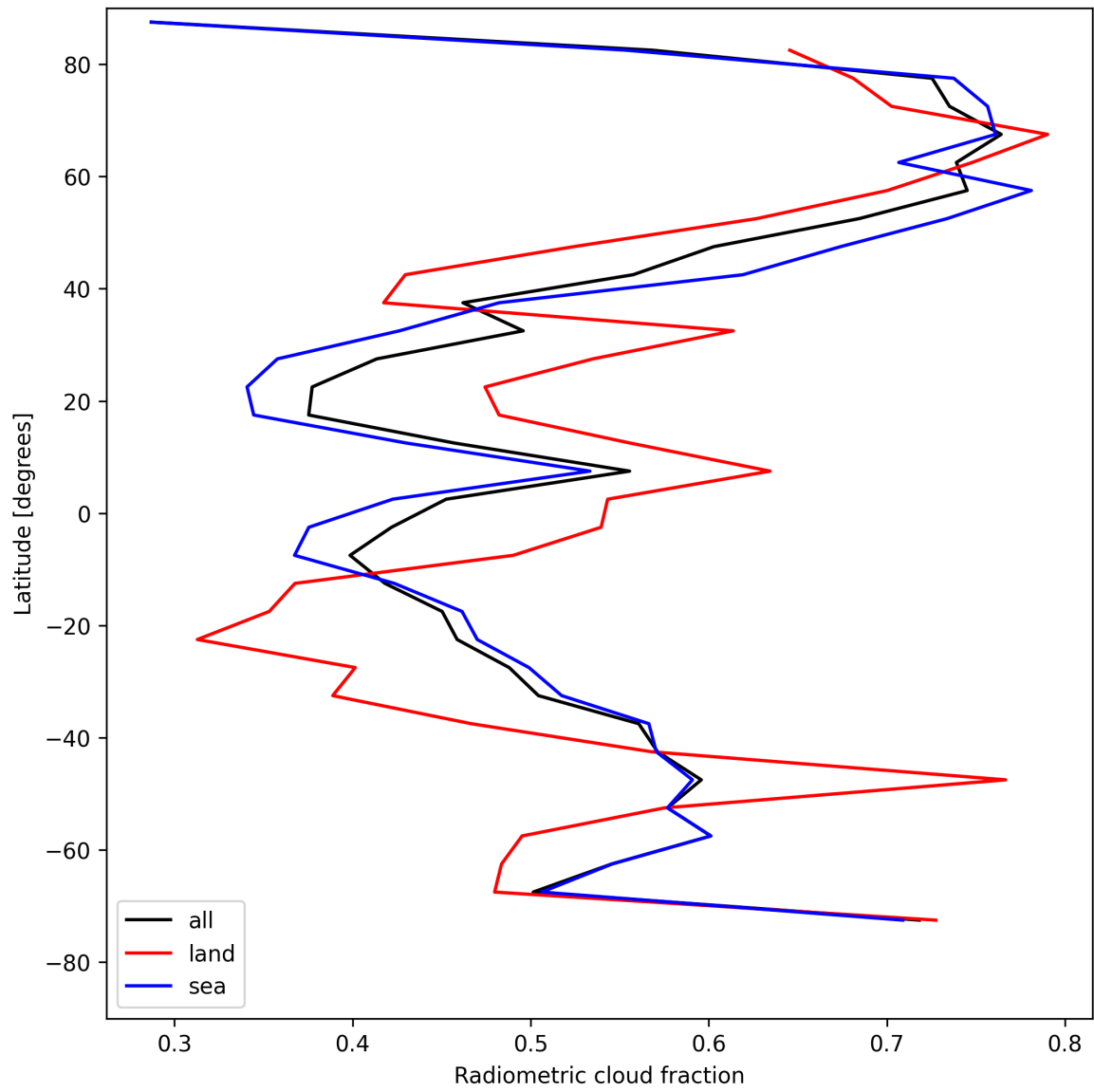
Figure 23: Zonal average of “Radiometric cloud fraction” for 2025-08-09 to 2025-08-11.
