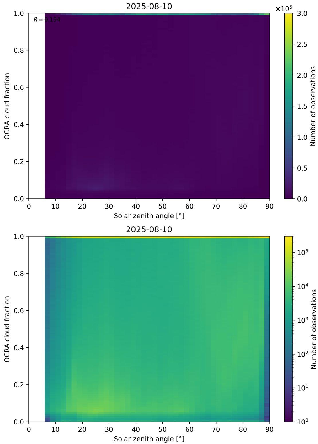
Figure 100: Scatter density plot of “Solar zenith angle” against “OCRA cloud fraction” for 2025-08-09 to 2025-08-11.
