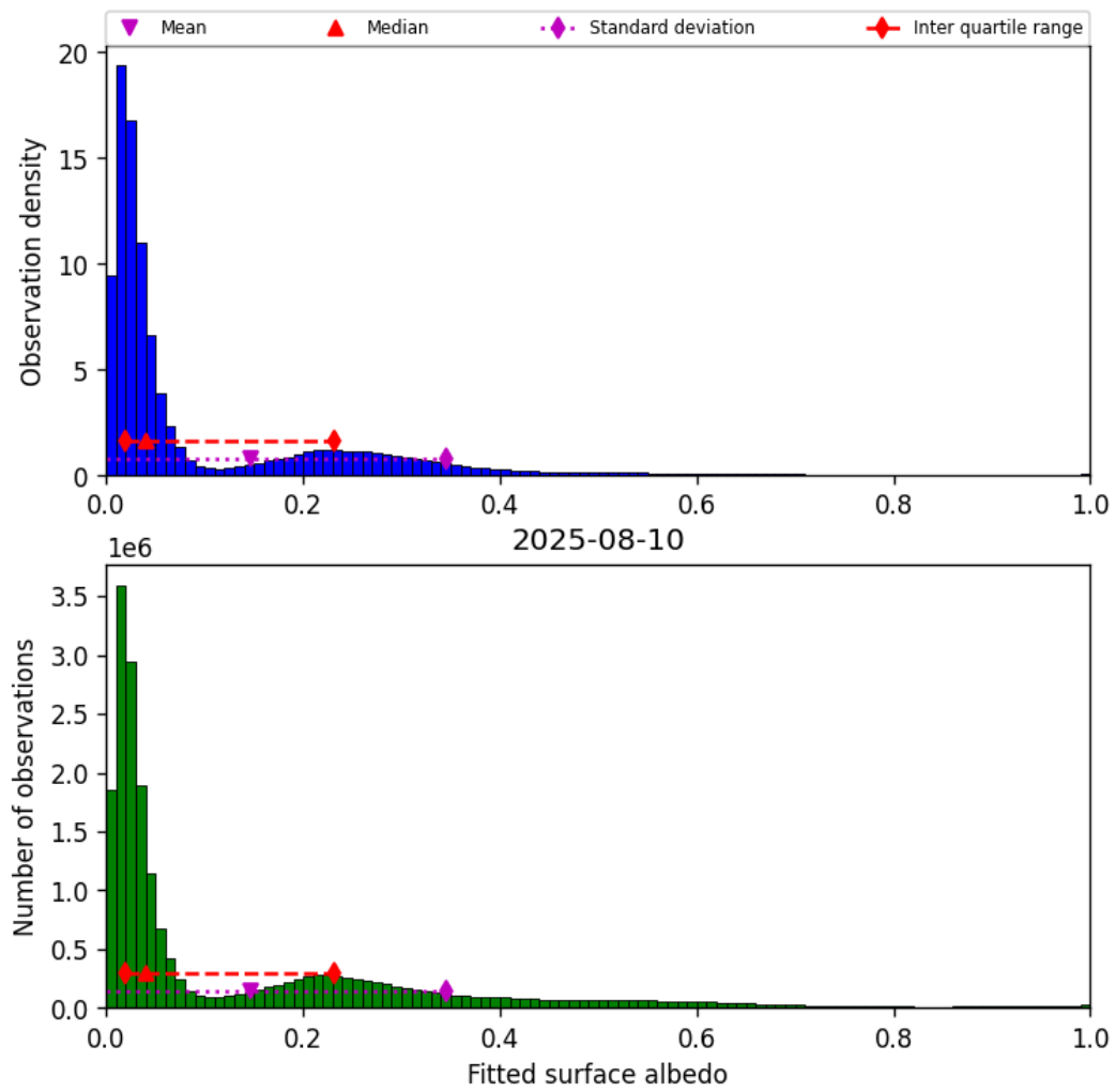
Figure 45: Histogram of “Fitted surface albedo” for 2025-08-09 to 2025-08-11
