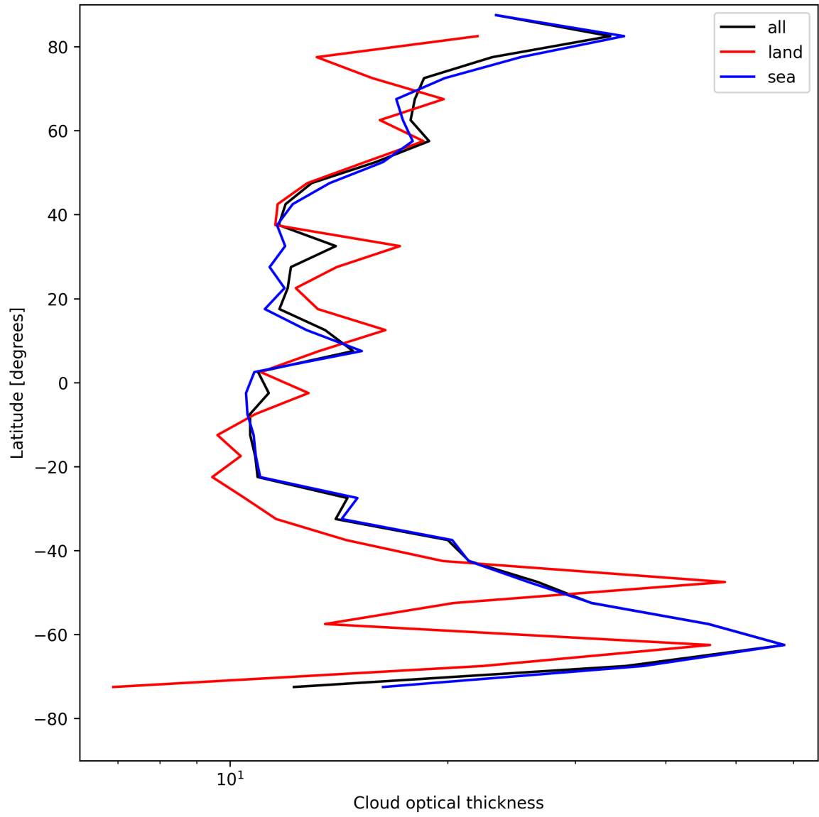
Figure 25: Zonal average of “Cloud optical thickness” for 2025-08-09 to 2025-08-11.
