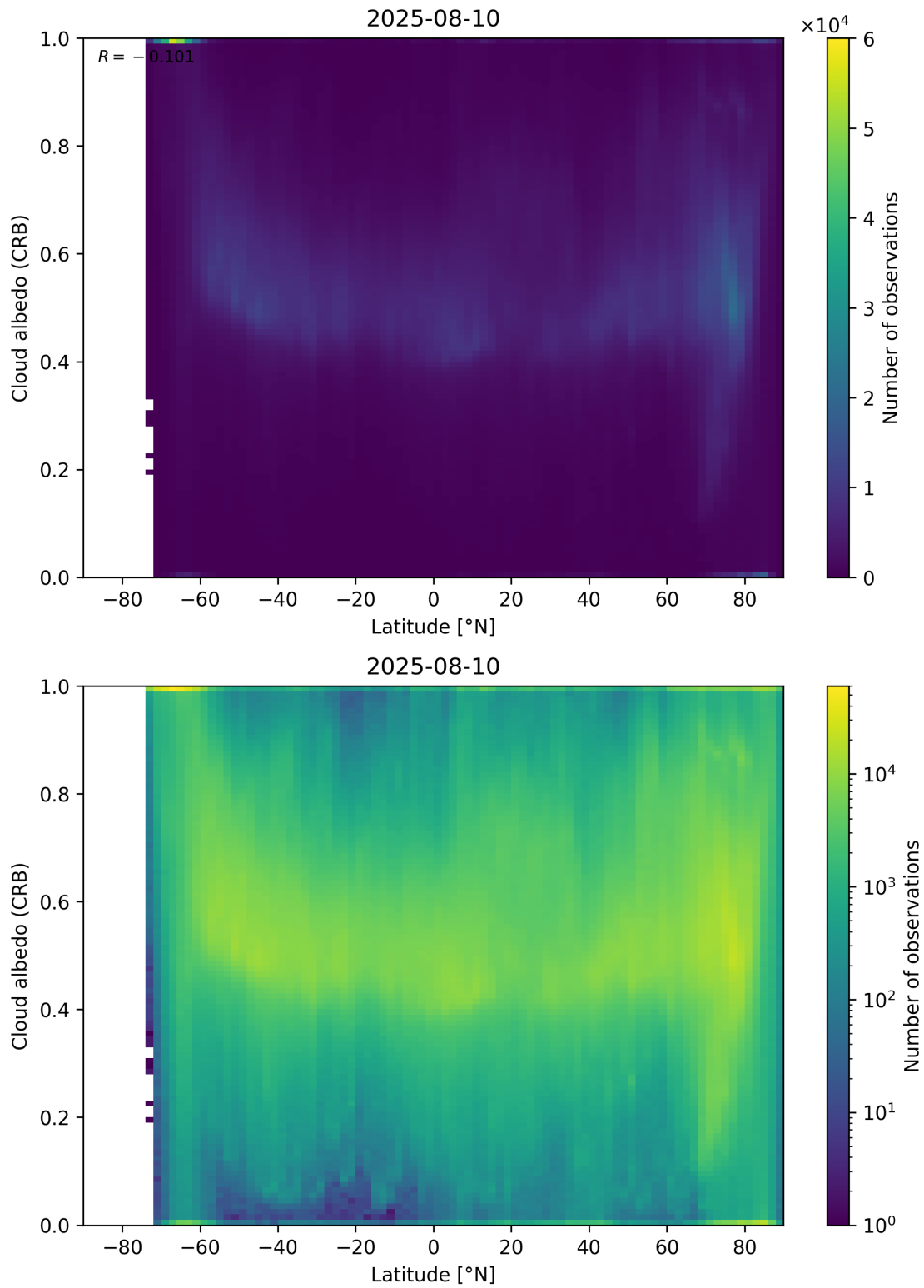
Figure 91: Scatter density plot of “Latitude” against “Cloud albedo (CRB)” for 2025-08-09 to 2025-08-11.
