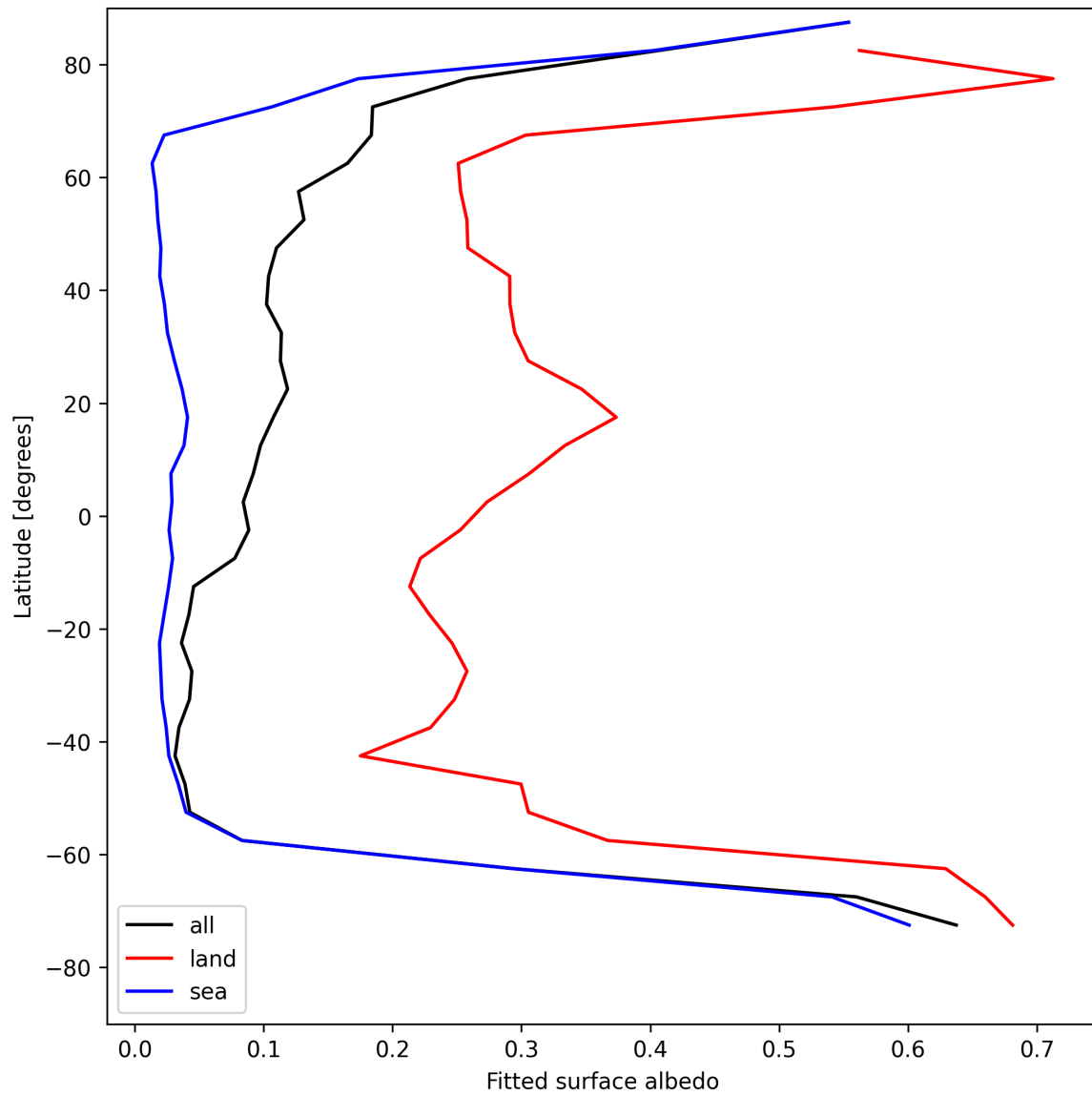
Figure 29: Zonal average of “Fitted surface albedo” for 2025-08-09 to 2025-08-11.
