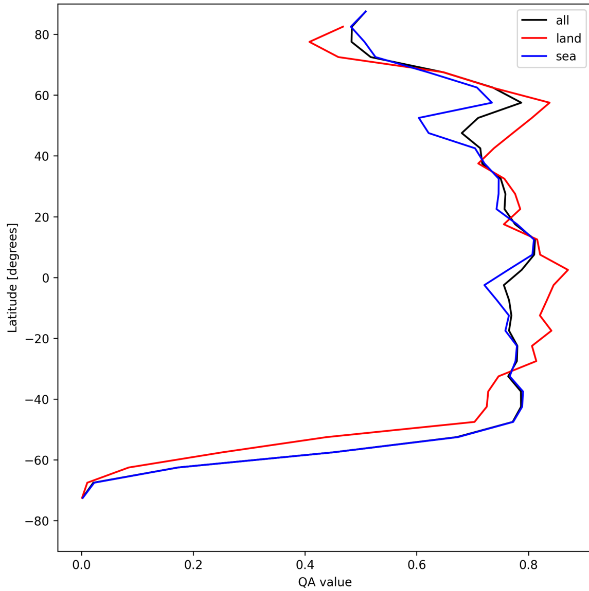
Figure 22: Zonal average of “QA value” for 2025-08-09 to 2025-08-11.
