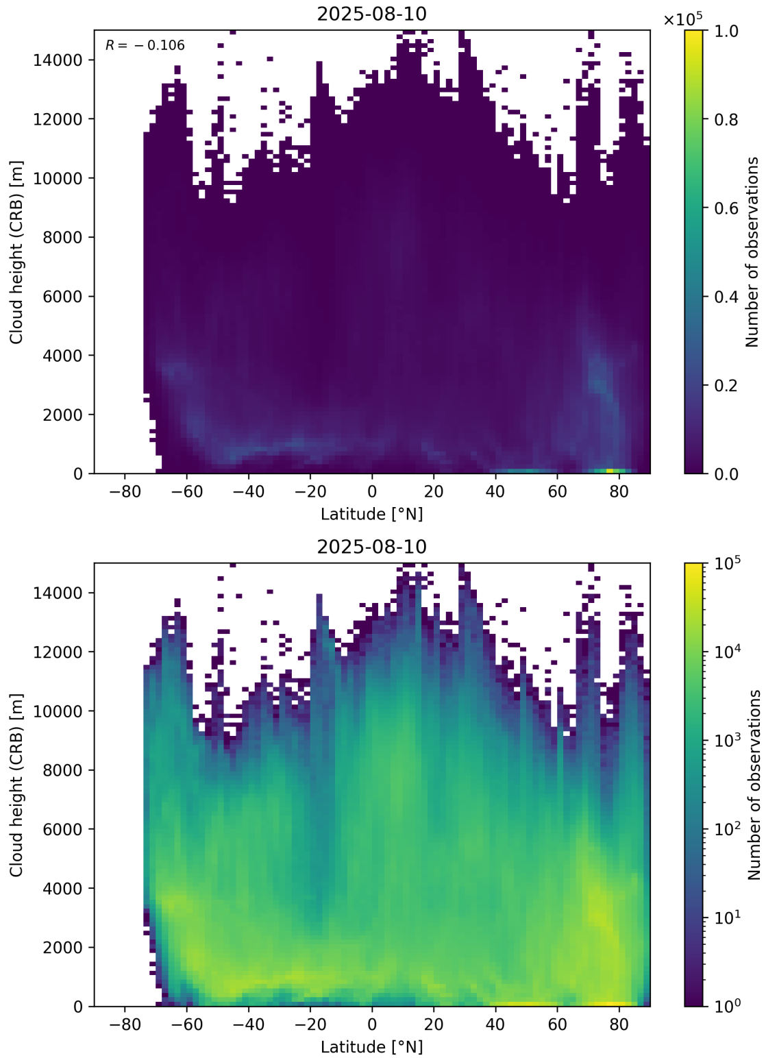
Figure 95: Scatter density plot of “Latitude” against “Cloud height (CRB)” for 2025-08-09 to 2025-08-11.
