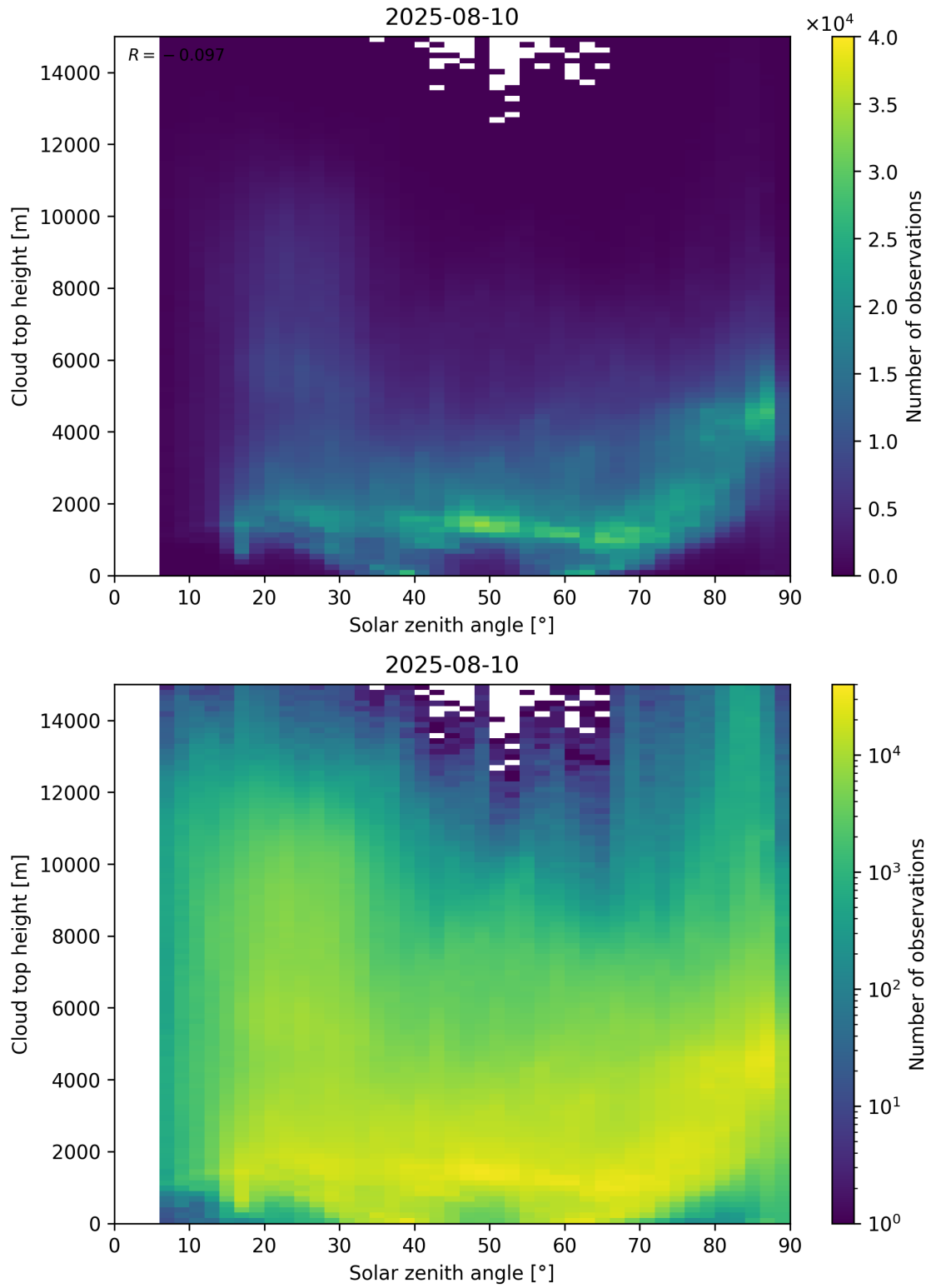
Figure 104: Scatter density plot of “Solar zenith angle” against “Cloud top height” for 2025-08-09 to 2025-08-11.
