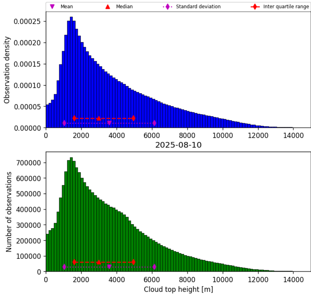
Figure 40: Histogram of “Cloud top height” for 2025-08-09 to 2025-08-11
