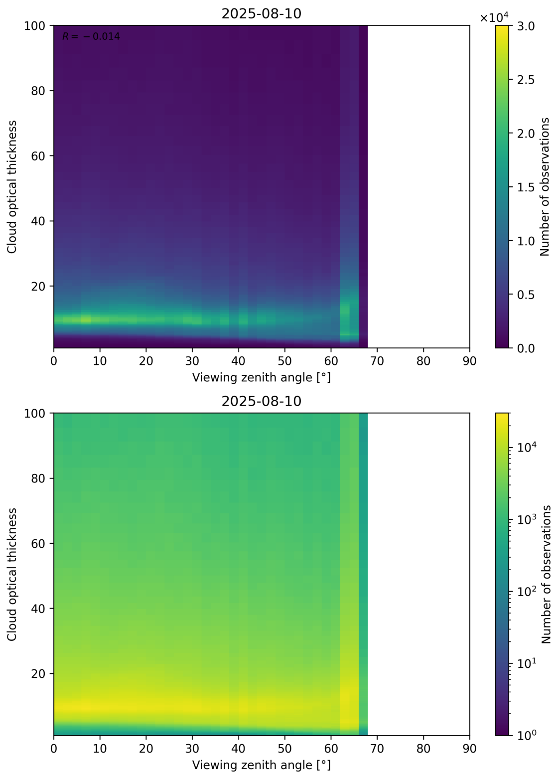
Figure 111: Scatter density plot of “Viewing zenith angle” against “Cloud optical thickness” for 2025-08-09 to 2025-08-11.
