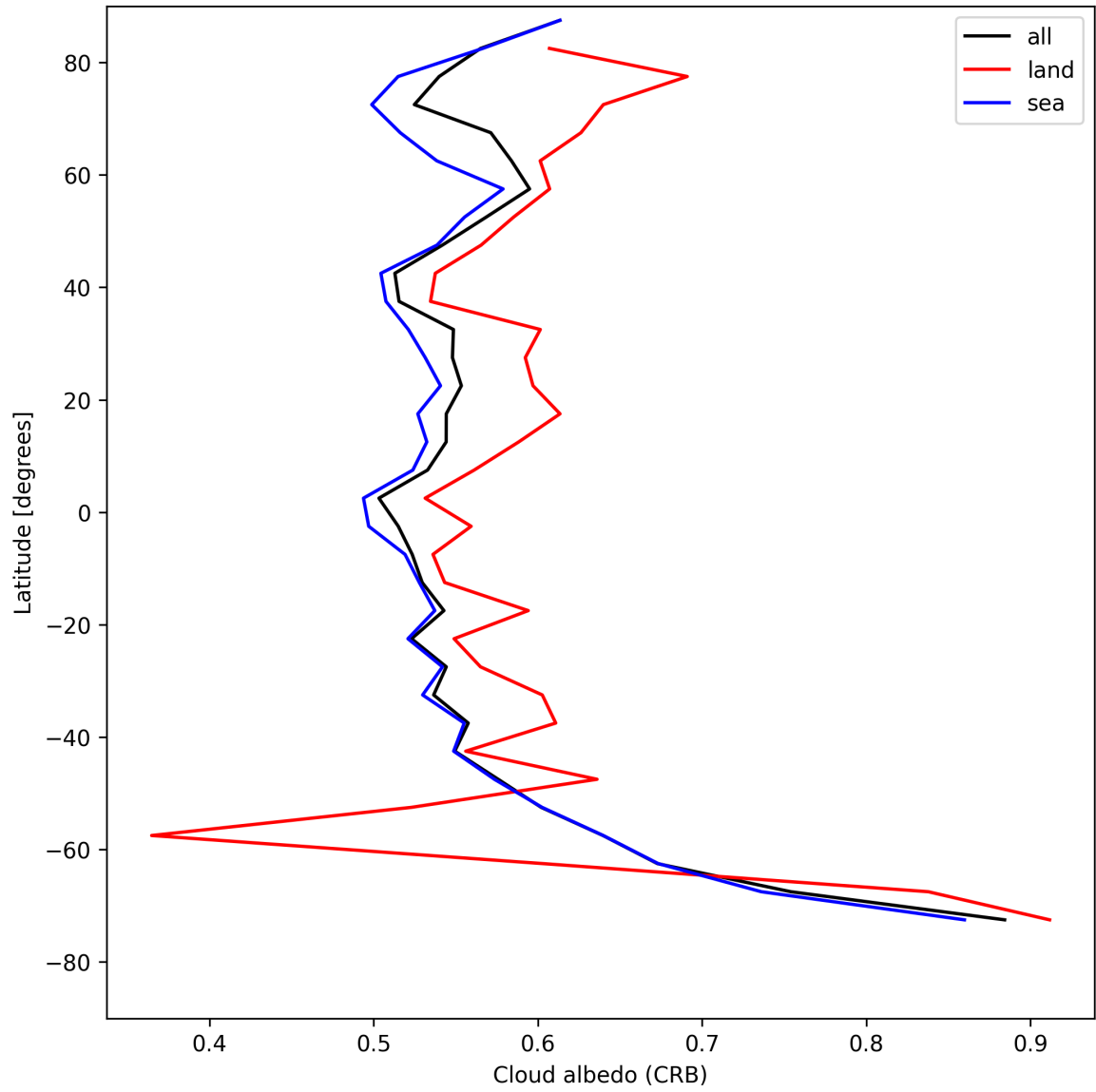
Figure 28: Zonal average of “Cloud albedo (CRB)” for 2025-08-09 to 2025-08-11.
