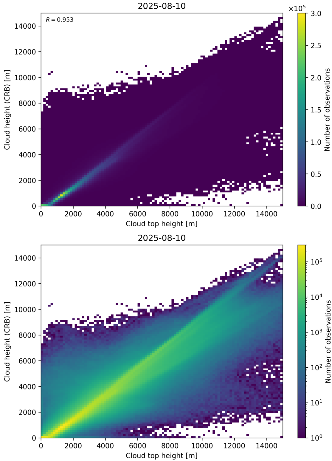
Figure 89: Scatter density plot of “Cloud top height” against “Cloud height (CRB)” for 2025-08-09 to 2025-08-11.
