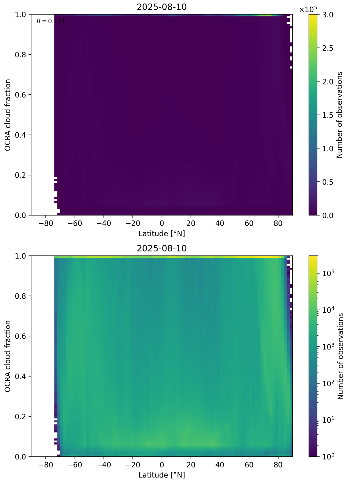
Figure 93: Scatter density plot of “Latitude” against “OCRA cloud fraction” for 2025-08-09 to 2025-08-11.
