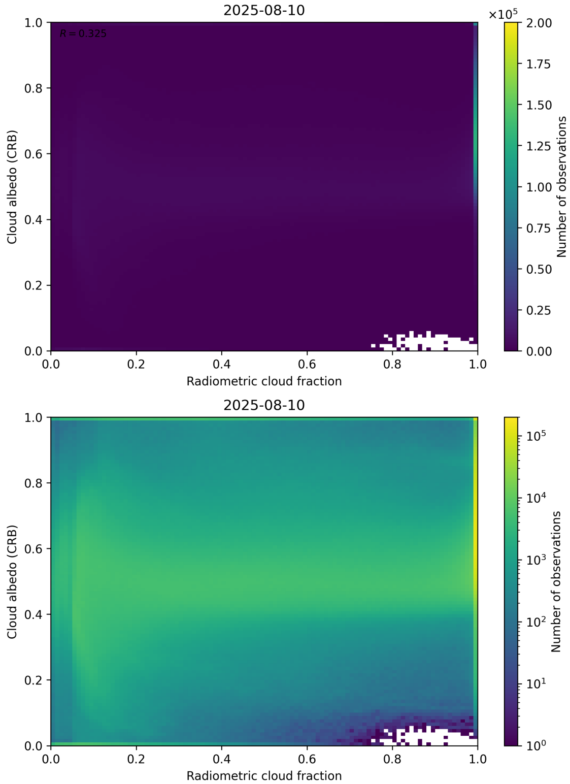
Figure 71: Scatter density plot of “Radiometric cloud fraction” against “Cloud albedo (CRB)” for 2025-08-09 to 2025-08-11.
