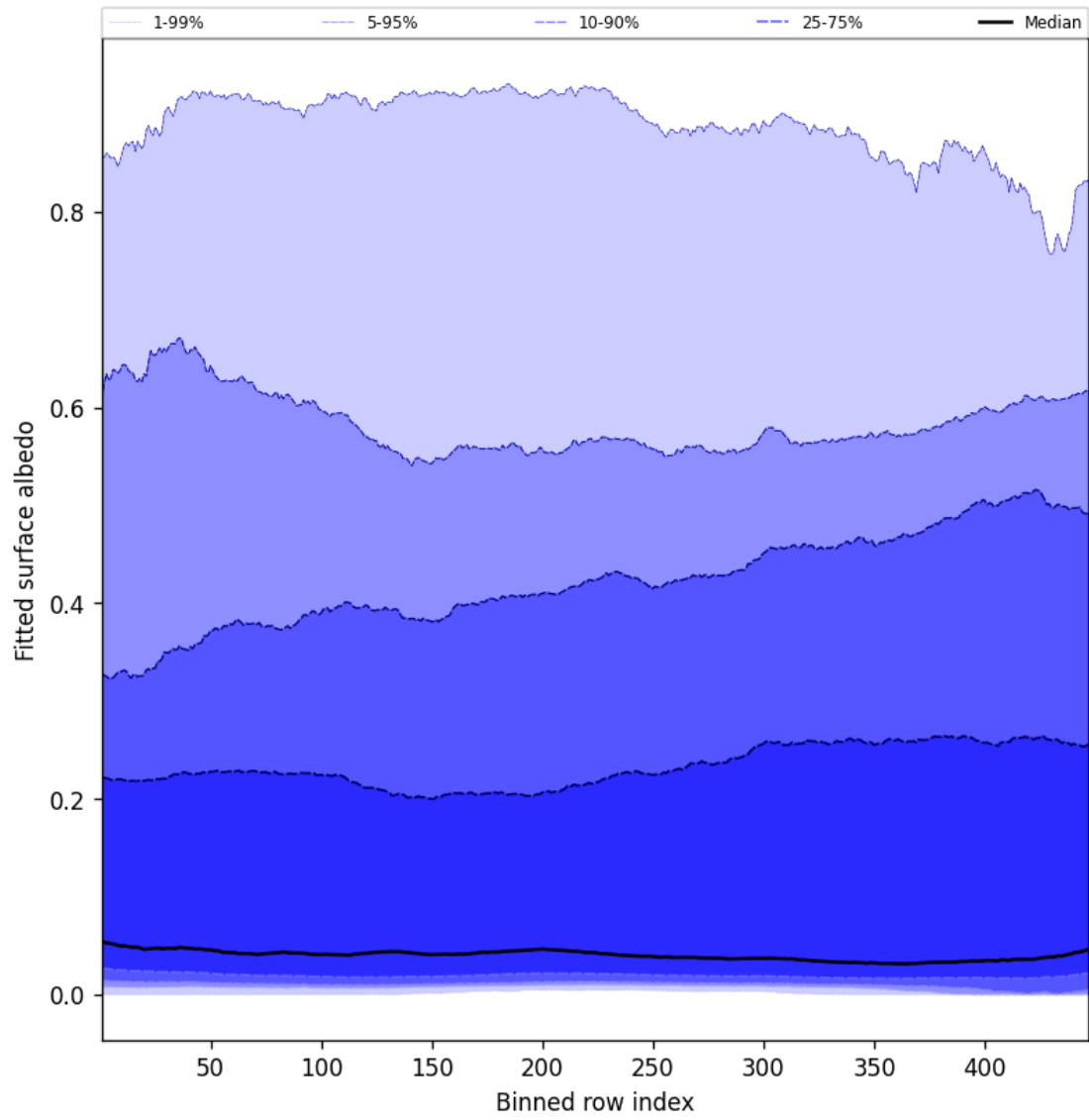
Figure 61: Along track statistics of “Fitted surface albedo” for 2025-08-09 to 2025-08-11
