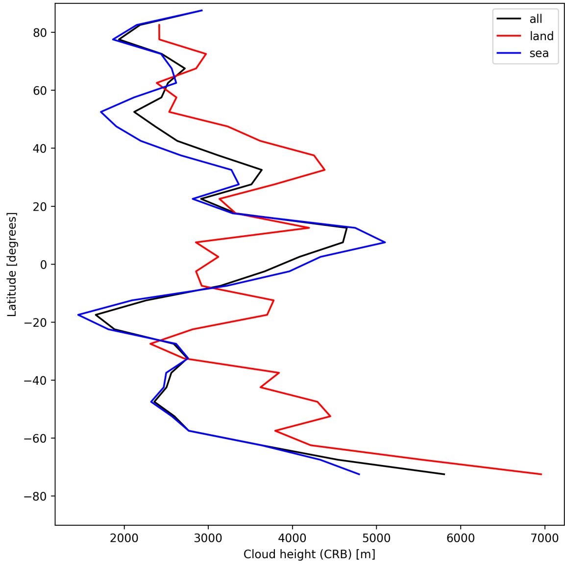
Figure 27: Zonal average of “Cloud height (CRB)” for 2025-08-09 to 2025-08-11.
