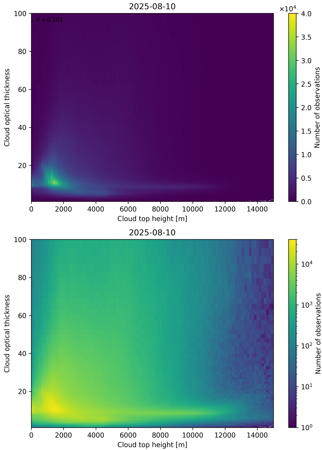
Figure 90: Scatter density plot of “Cloud top height” against “Cloud optical thickness” for 2025-08-09 to 2025-08-11.
