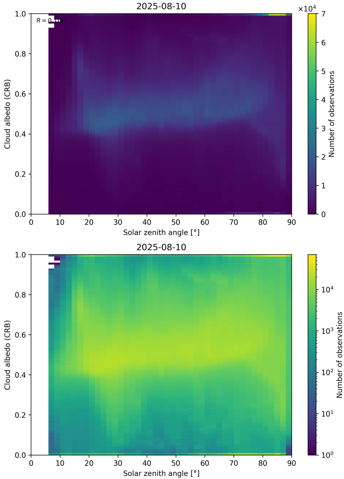
Figure 98: Scatter density plot of “Solar zenith angle” against “Cloud albedo (CRB)” for 2025-08-09 to 2025-08-11.
