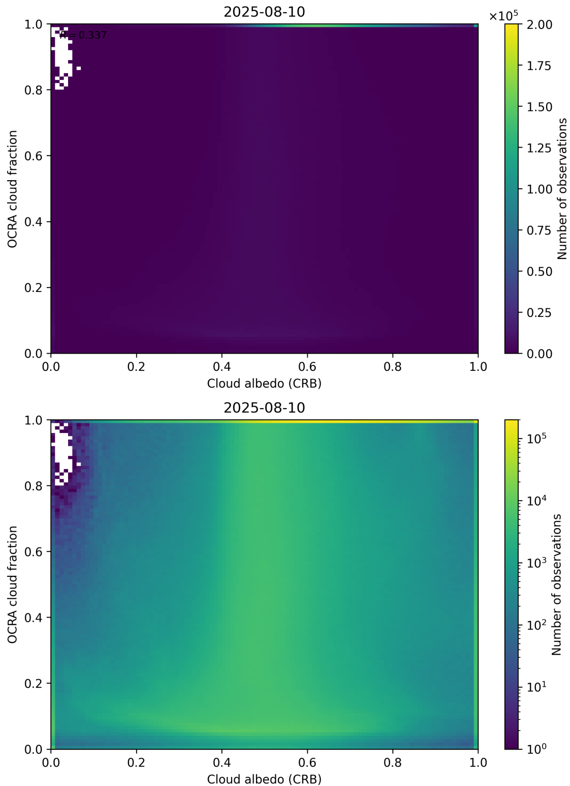
Figure 70: Scatter density plot of “Cloud albedo (CRB)” against “OCRA cloud fraction” for 2025-08-09 to 2025-08-11.
