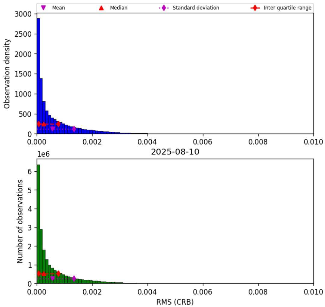
Figure 48: Histogram of “RMS (CRB)” for 2025-08-09 to 2025-08-11
