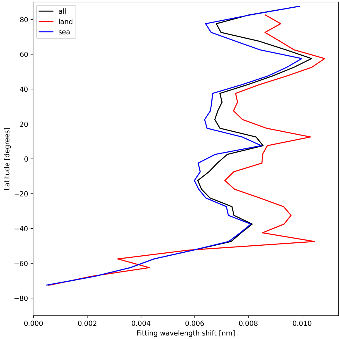
Figure 33: Zonal average of “Fitting wavelength shift” for 2025-08-09 to 2025-08-11.
