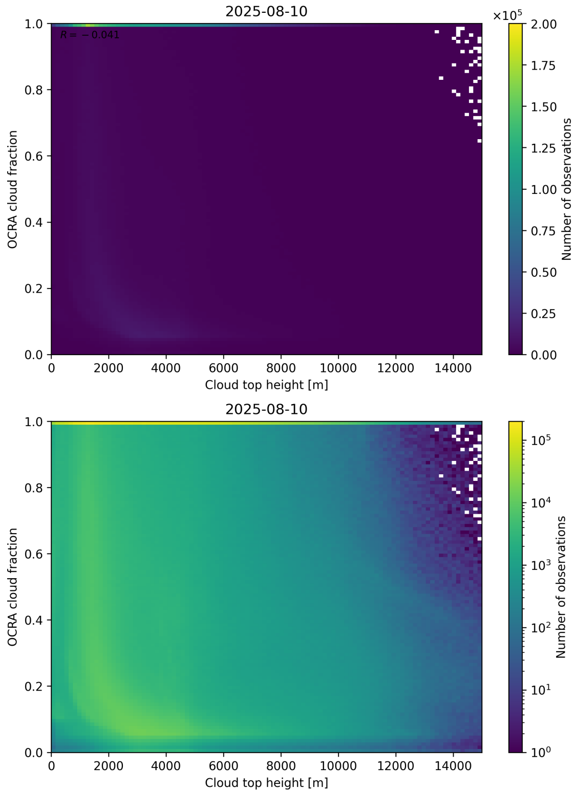
Figure 87: Scatter density plot of “Cloud top height” against “OCRA cloud fraction” for 2025-08-09 to 2025-08-11.
