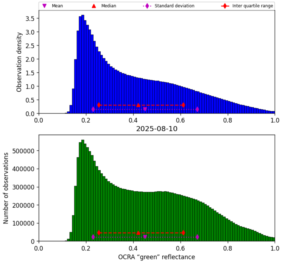
Figure 52: Histogram of “OCRA “green” reflectance” for 2025-08-09 to 2025-08-11
