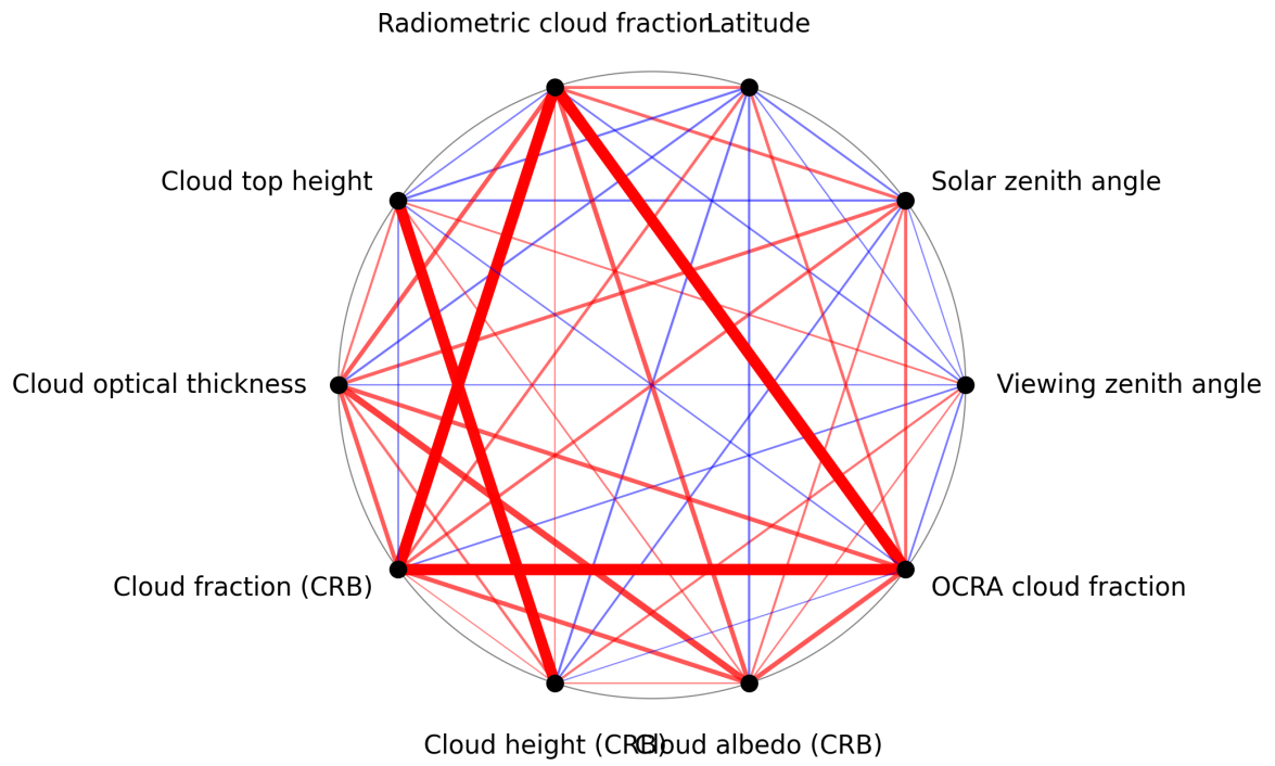
Figure 1: Map of correlation graph for 2025-08-09 to 2025-08-11.
