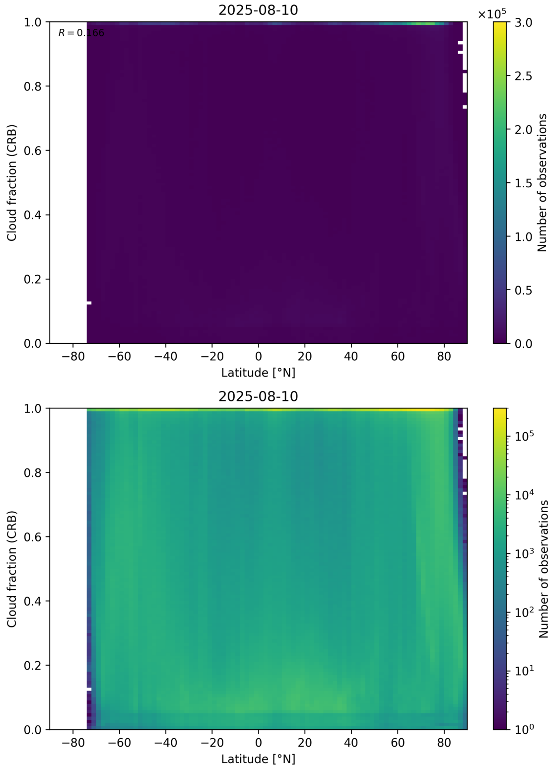
Figure 94: Scatter density plot of “Latitude” against “Cloud fraction (CRB)” for 2025-08-09 to 2025-08-11.
