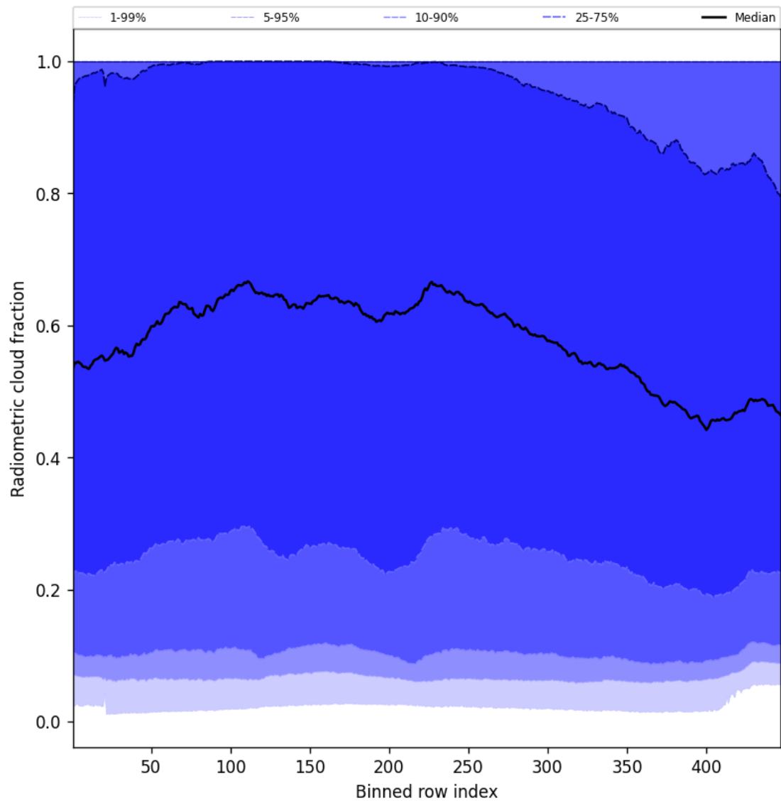
Figure 55: Along track statistics of “Radiometric cloud fraction” for 2025-08-09 to 2025-08-11
