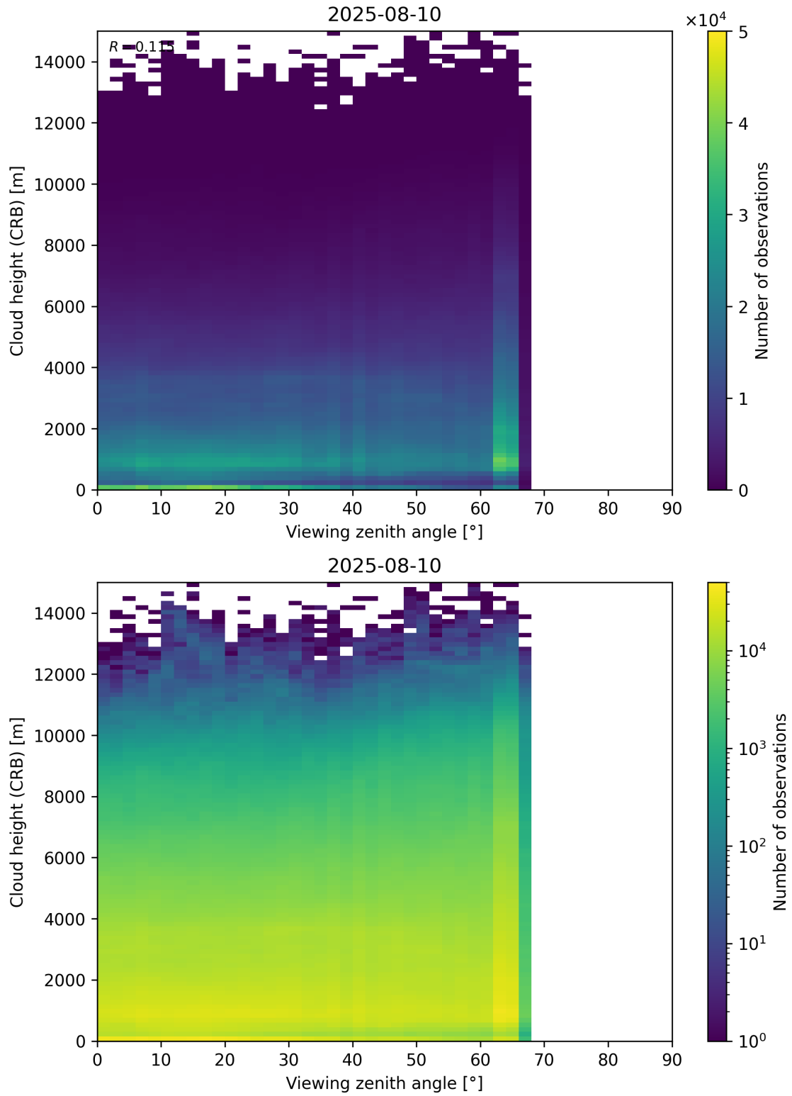
Figure 110: Scatter density plot of “Viewing zenith angle” against “Cloud height (CRB)” for 2025-08-09 to 2025-08-11.
