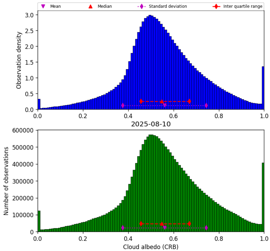
Figure 44: Histogram of “Cloud albedo (CRB)” for 2025-08-09 to 2025-08-11
