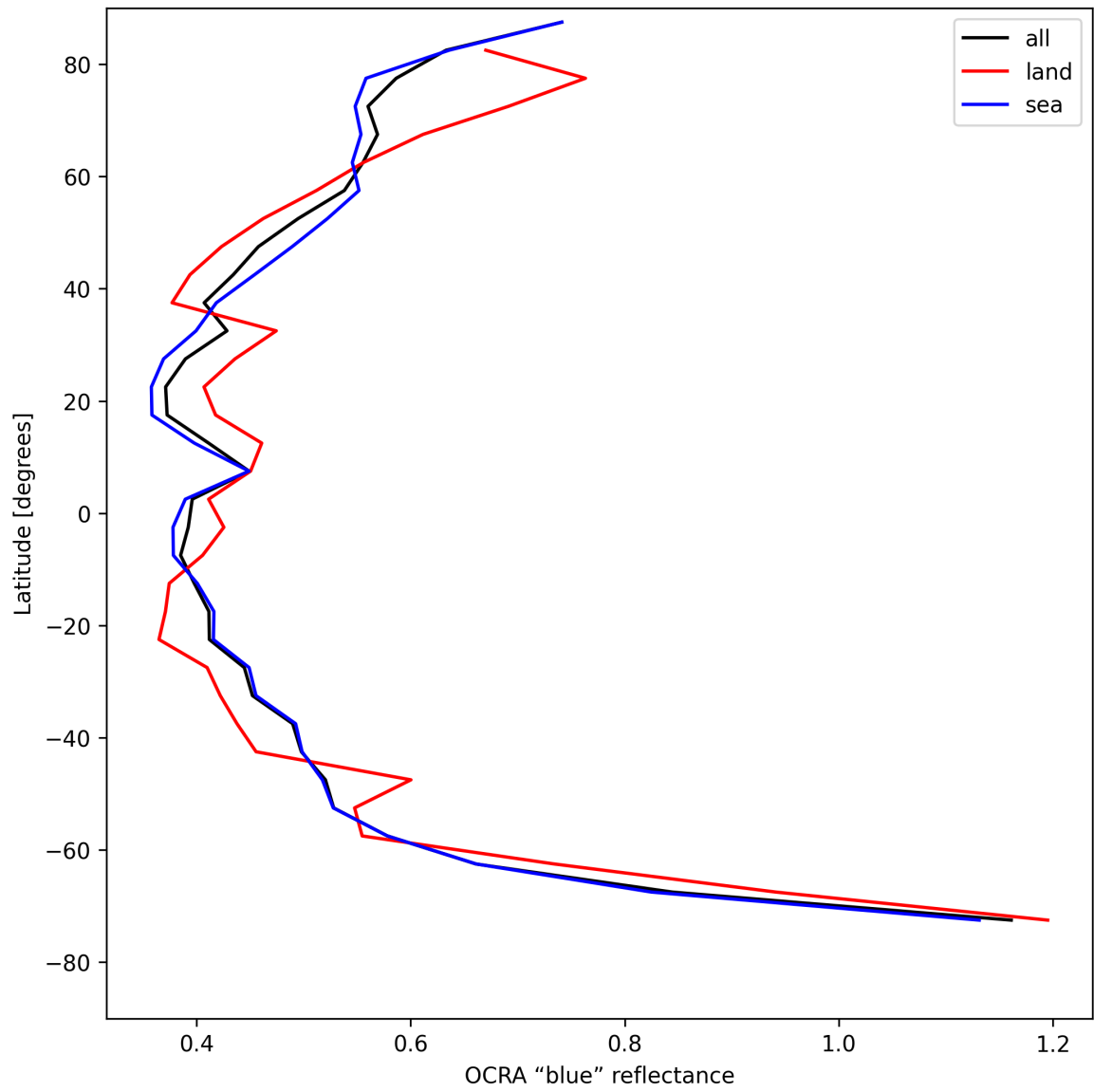
Figure 35: Zonal average of “OCRA “blue” reflectance” for 2025-08-09 to 2025-08-11.
