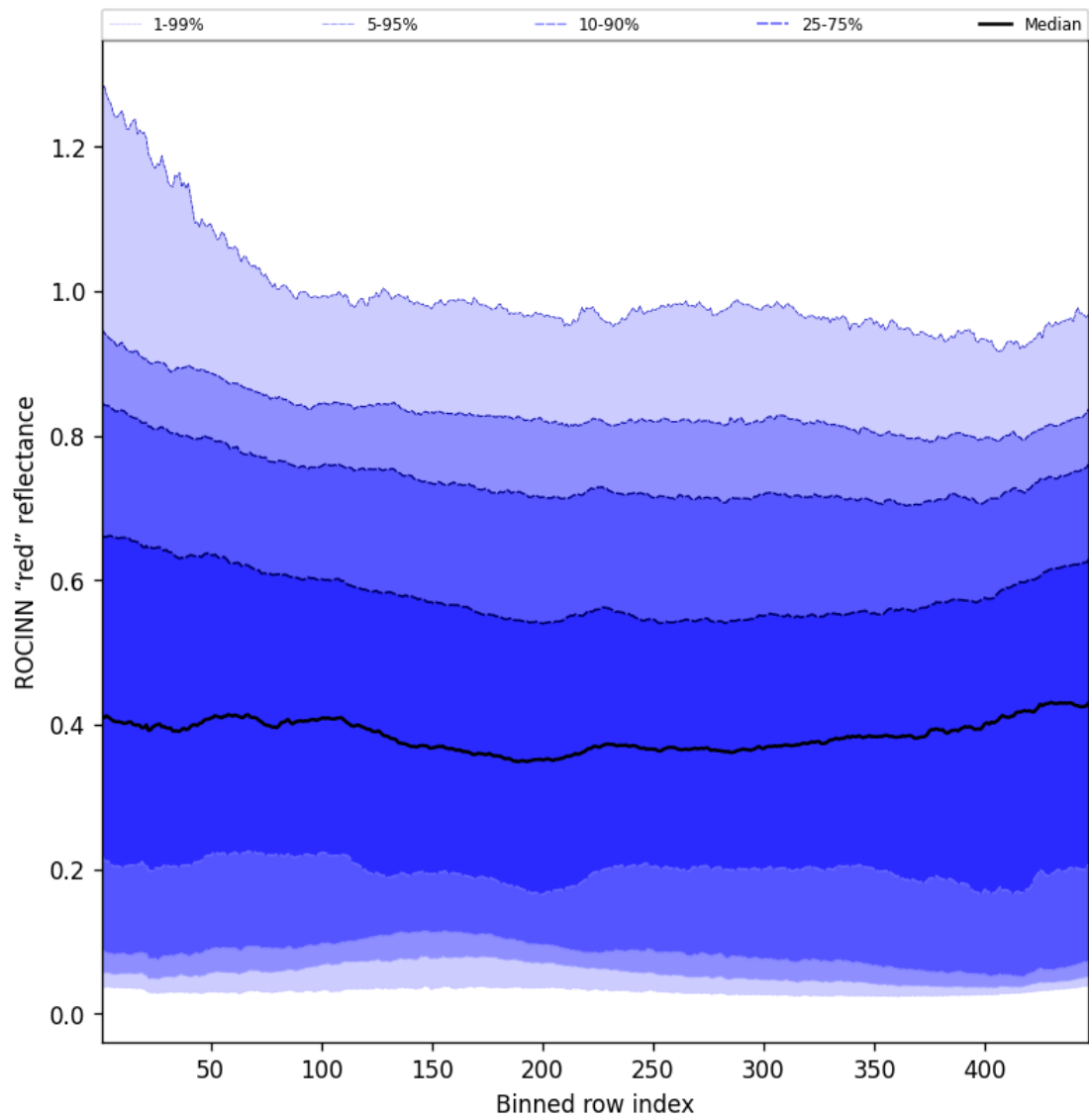
Figure 69: Along track statistics of "ROCINN "red" reflectance" for 2025-08-09 to 2025-08-11
