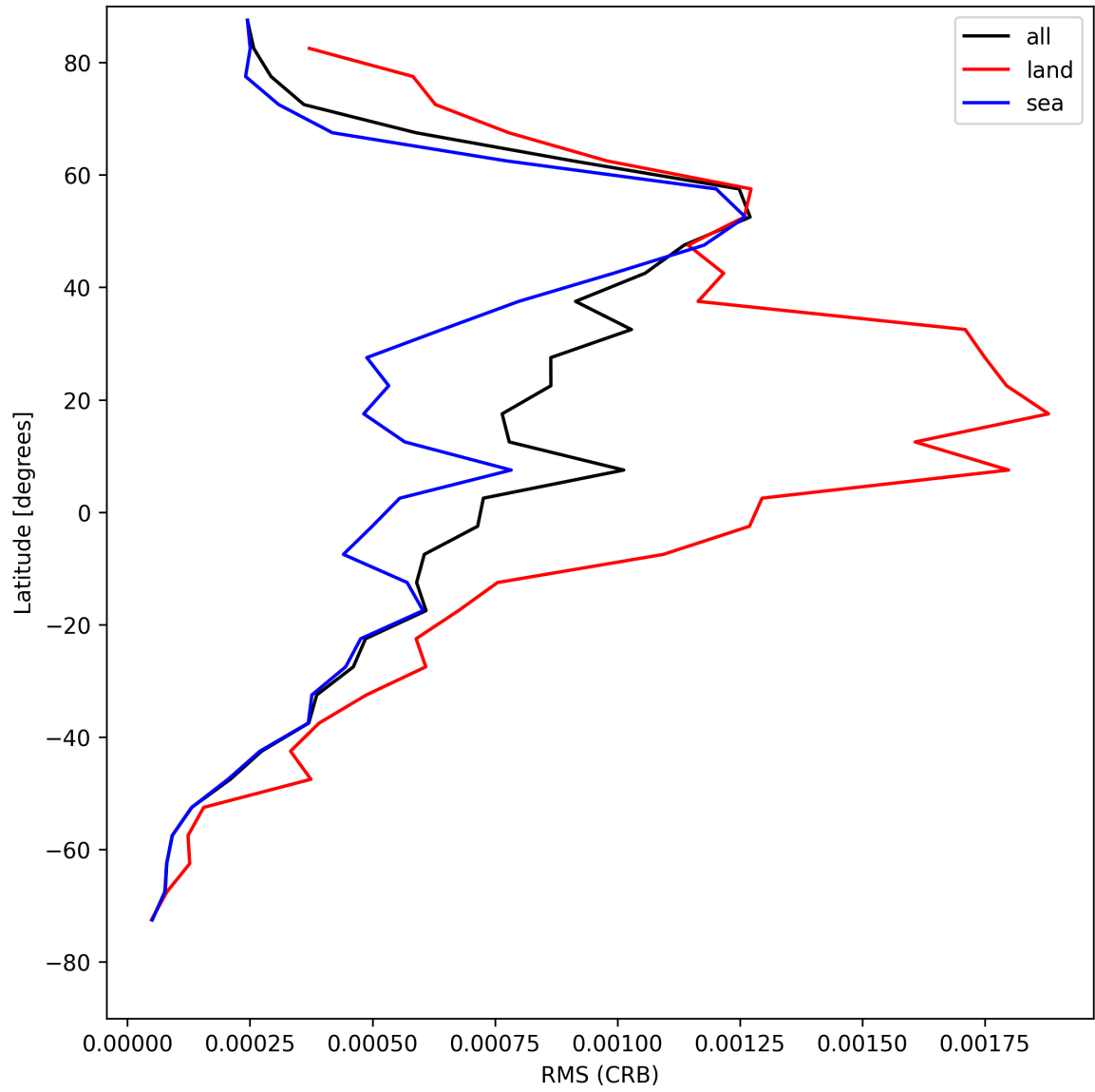
Figure 32: Zonal average of “RMS (CRB)” for 2025-08-09 to 2025-08-11.
