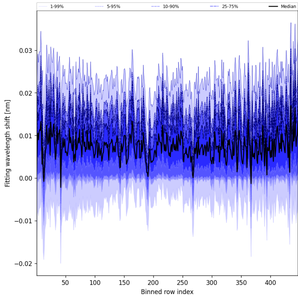
Figure 65: Along track statistics of “Fitting wavelength shift” for 2025-08-09 to 2025-08-11
