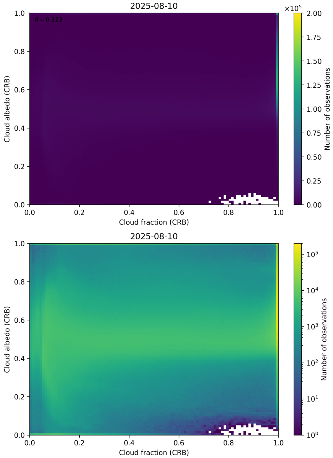
Figure 77: Scatter density plot of “Cloud fraction (CRB)” against “Cloud albedo (CRB)” for 2025-08-09 to 2025-08-11.
