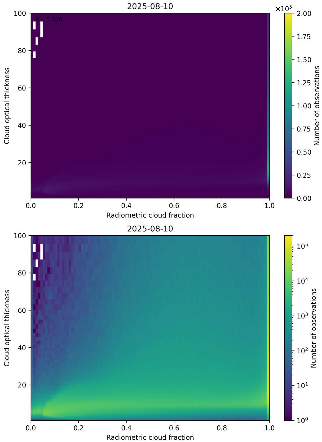
Figure 75: Scatter density plot of “Radiometric cloud fraction” against “Cloud optical thickness” for 2025-08-09 to 2025-08-11.
