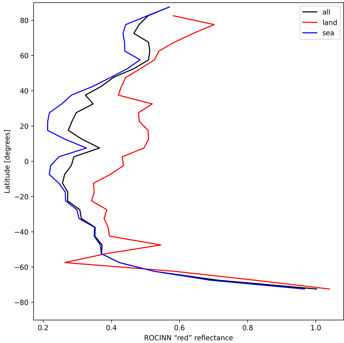
Figure 37: Zonal average of “ROCINN “red” reflectance” for 2025-08-09 to 2025-08-11.
