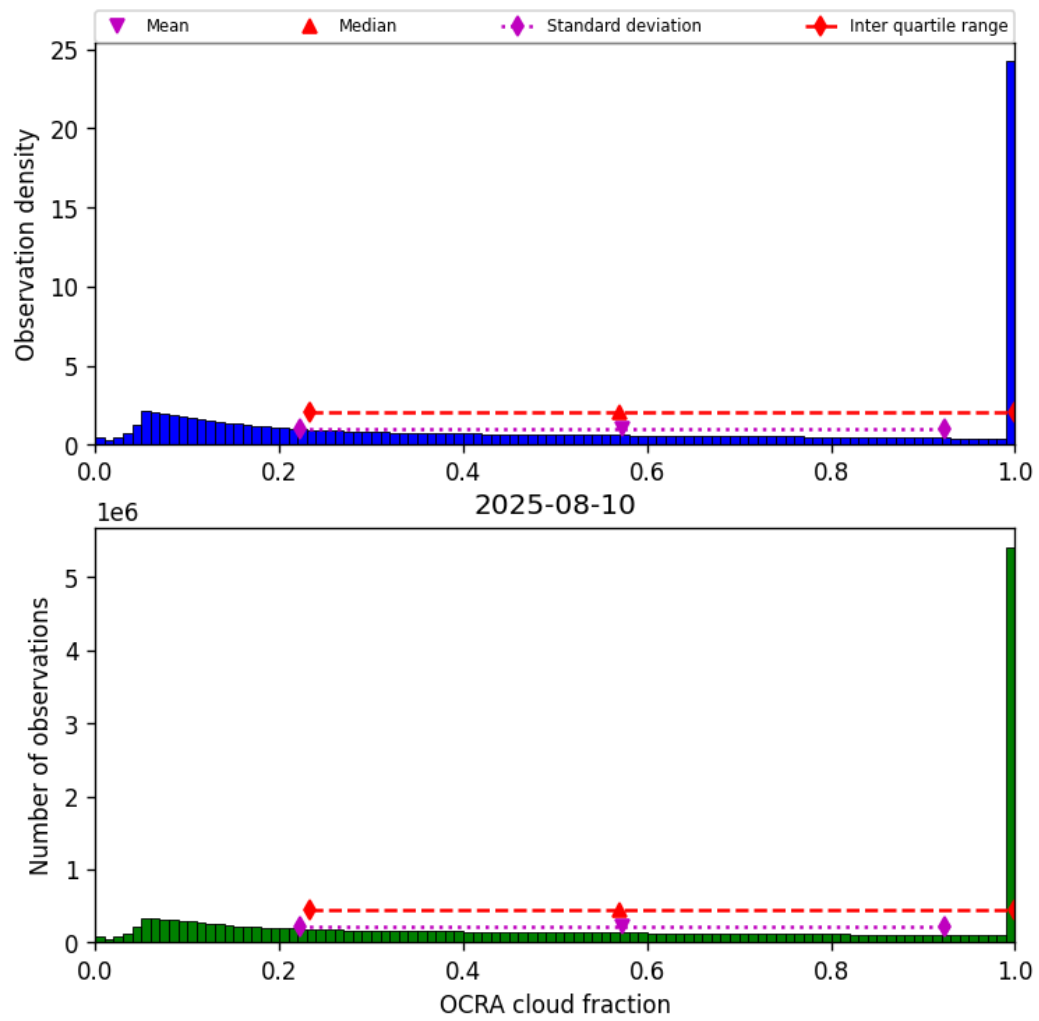
Figure 50: Histogram of “OCRA cloud fraction” for 2025-08-09 to 2025-08-11
