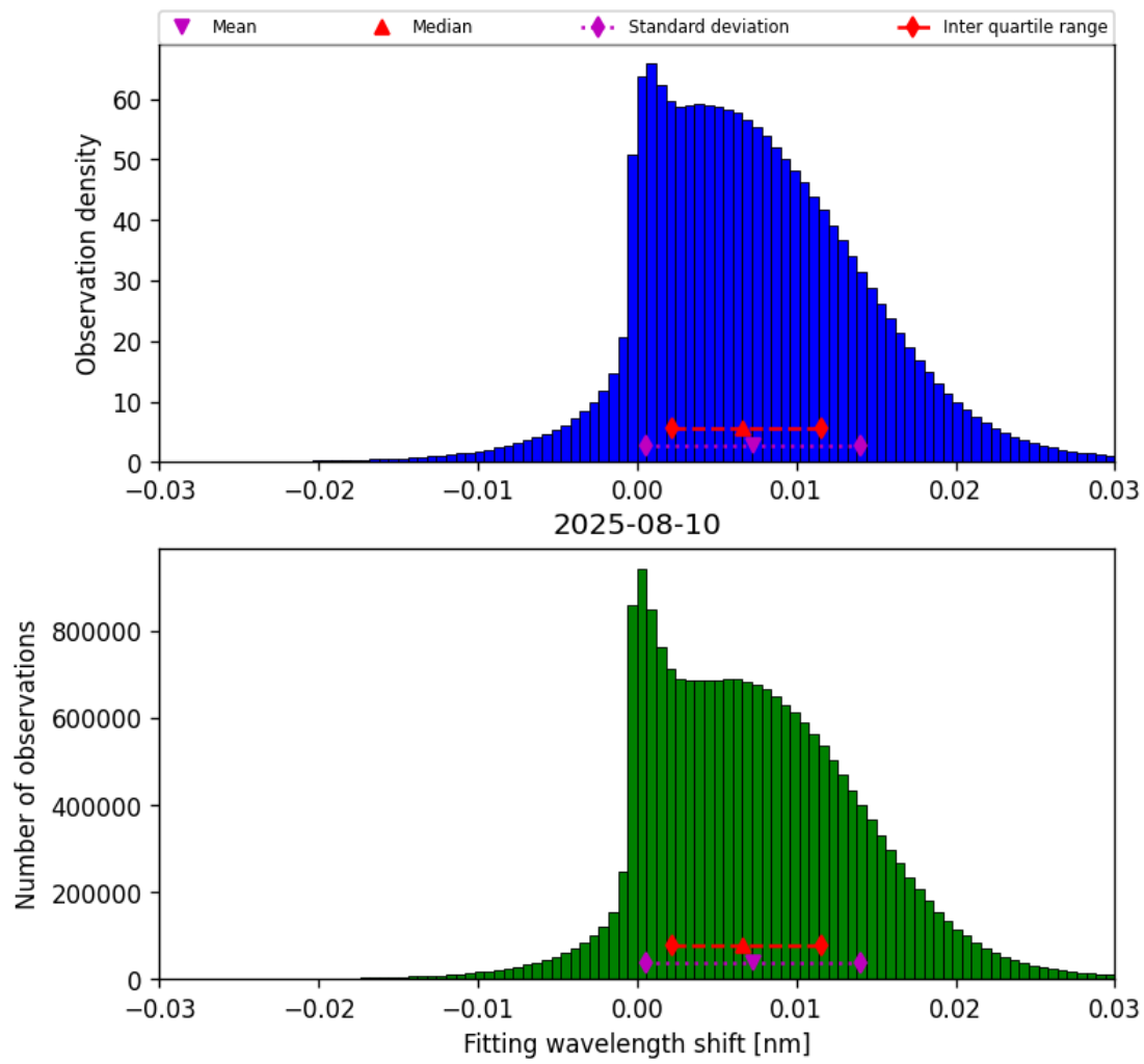
Figure 49: Histogram of “Fitting wavelength shift” for 2025-08-09 to 2025-08-11
