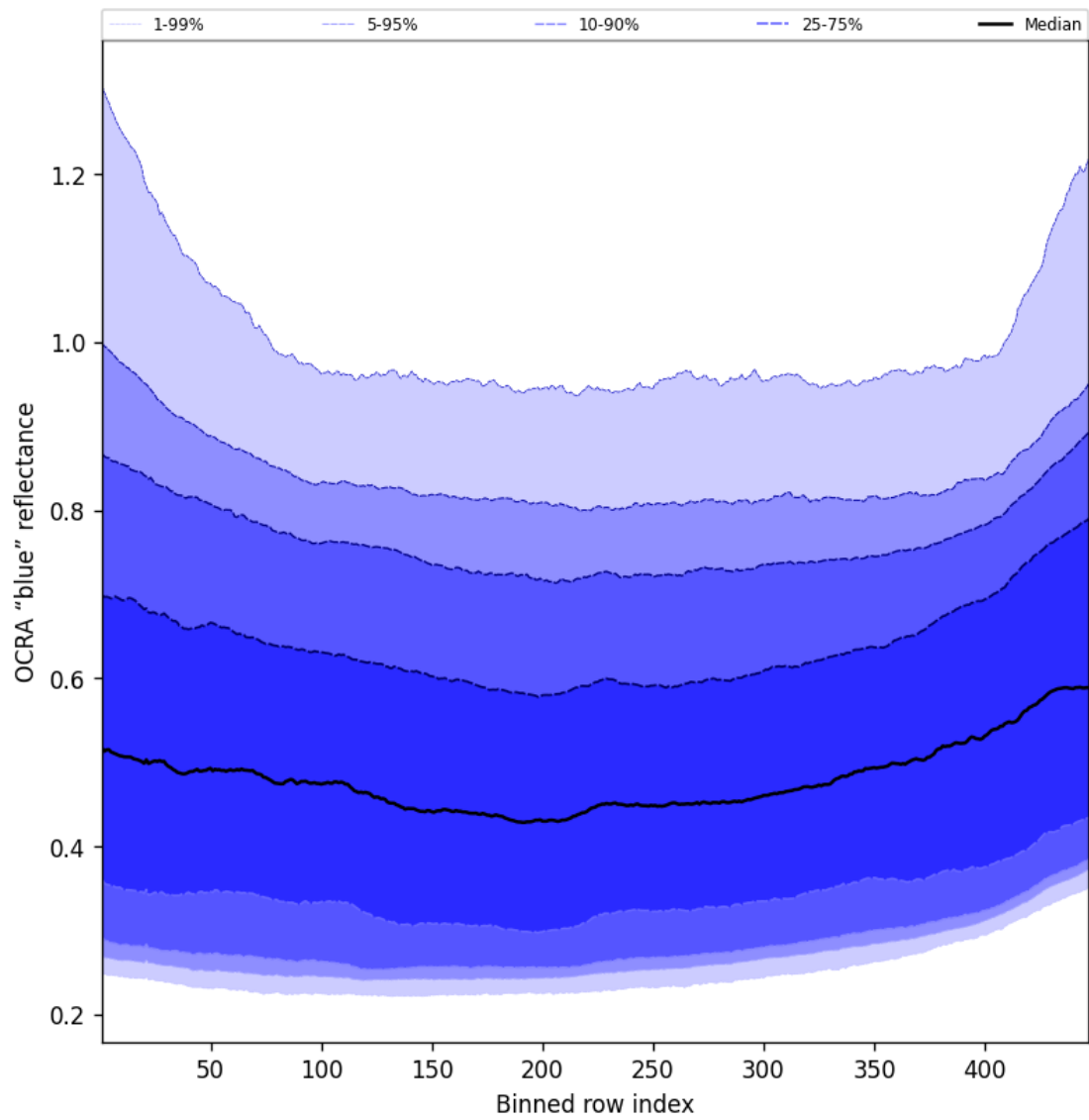
Figure 67: Along track statistics of “OCRA “blue” reflectance” for 2025-08-09 to 2025-08-11
