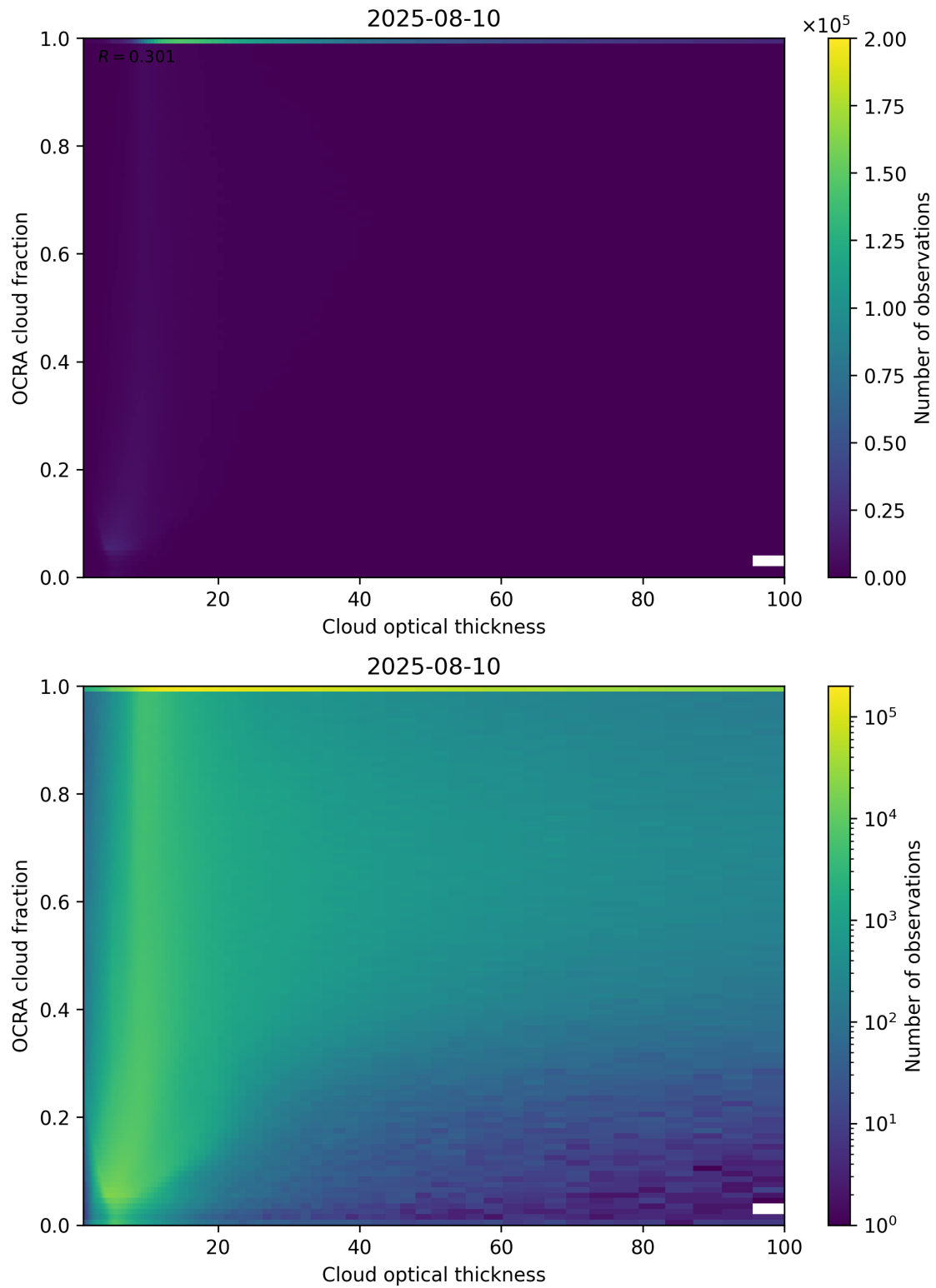
Figure 83: Scatter density plot of “Cloud optical thickness” against “OCRA cloud fraction” for 2025-08-09 to 2025-08-11.
