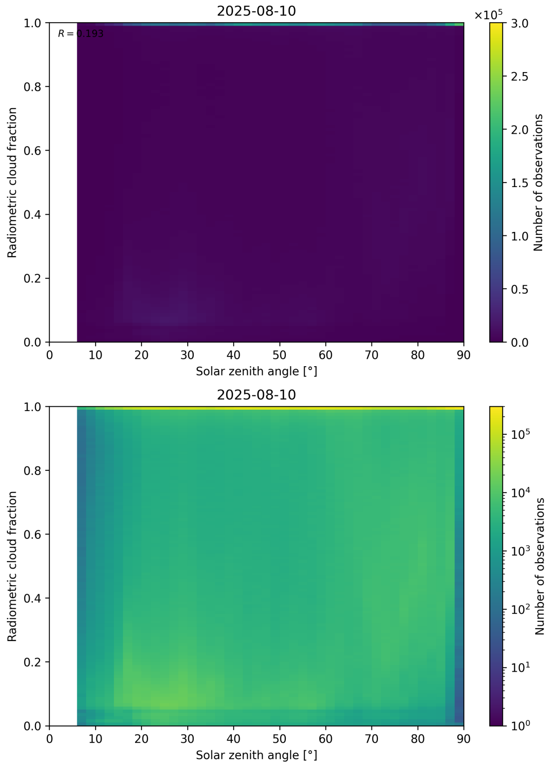
Figure 99: Scatter density plot of “Solar zenith angle” against “Radiometric cloud fraction” for 2025-08-09 to 2025-08-11.
