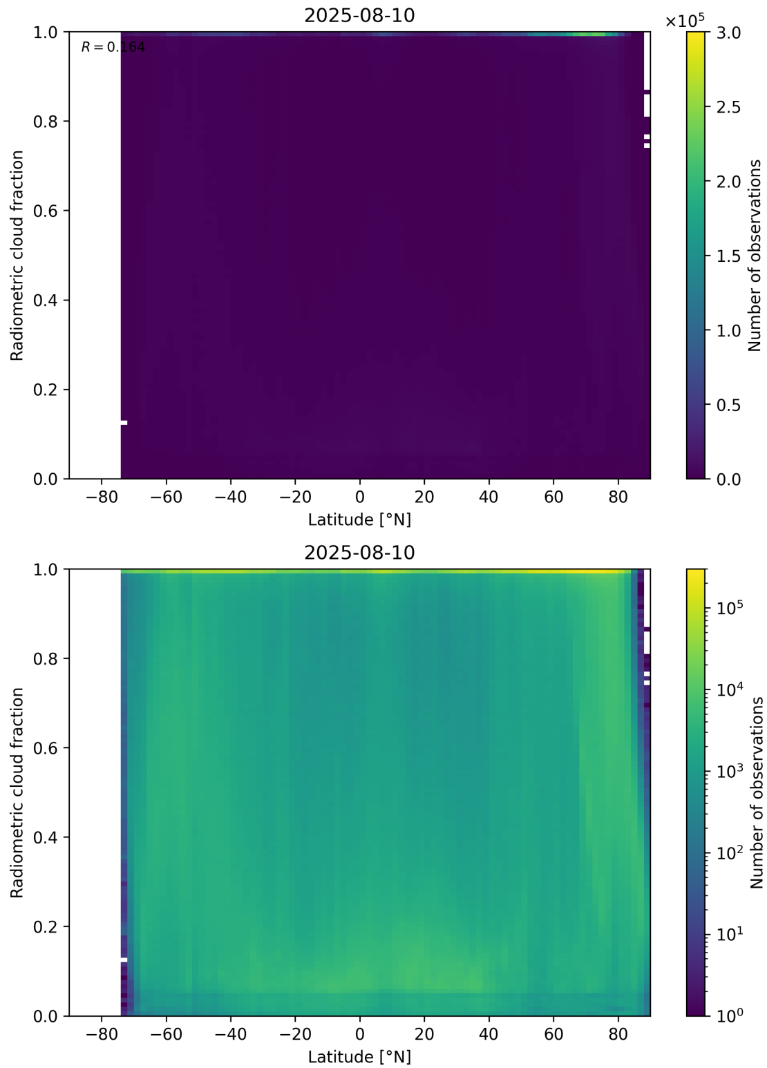
Figure 92: Scatter density plot of “Latitude” against “Radiometric cloud fraction” for 2025-08-09 to 2025-08-11.
