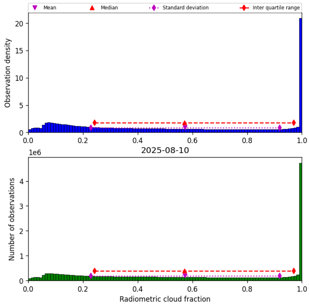
Figure 39: Histogram of “Radiometric cloud fraction” for 2025-08-09 to 2025-08-11
