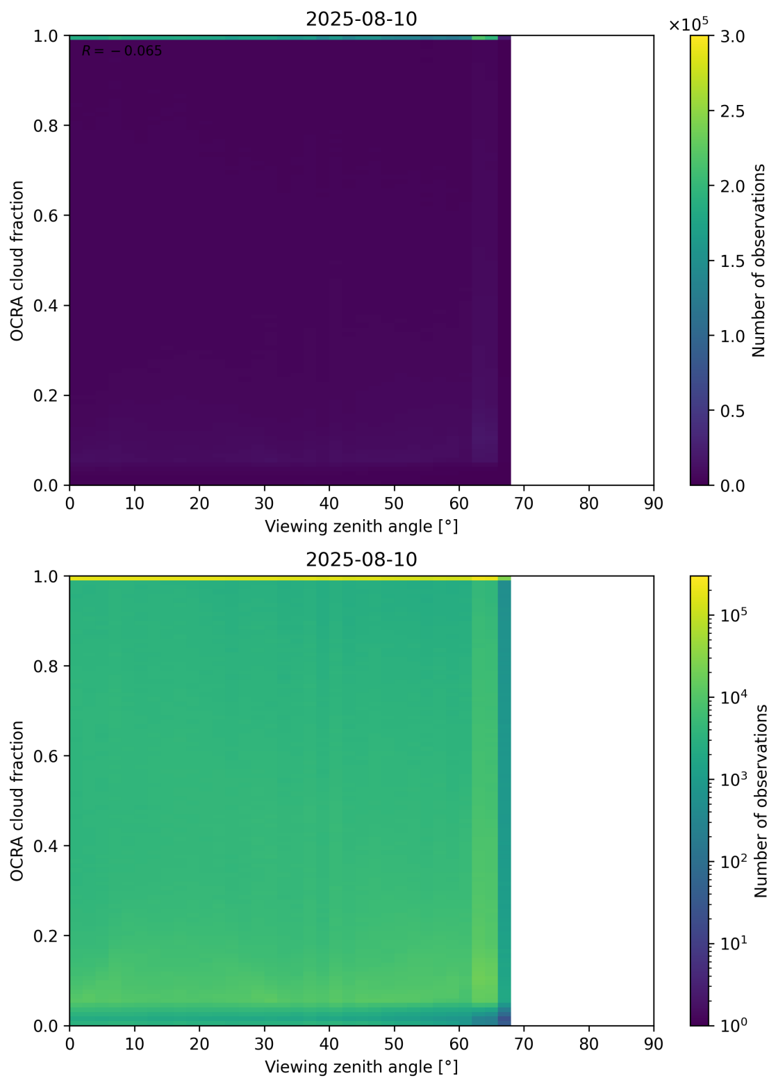
Figure 108: Scatter density plot of “Viewing zenith angle” against “OCRA cloud fraction” for 2025-08-09 to 2025-08-11.
