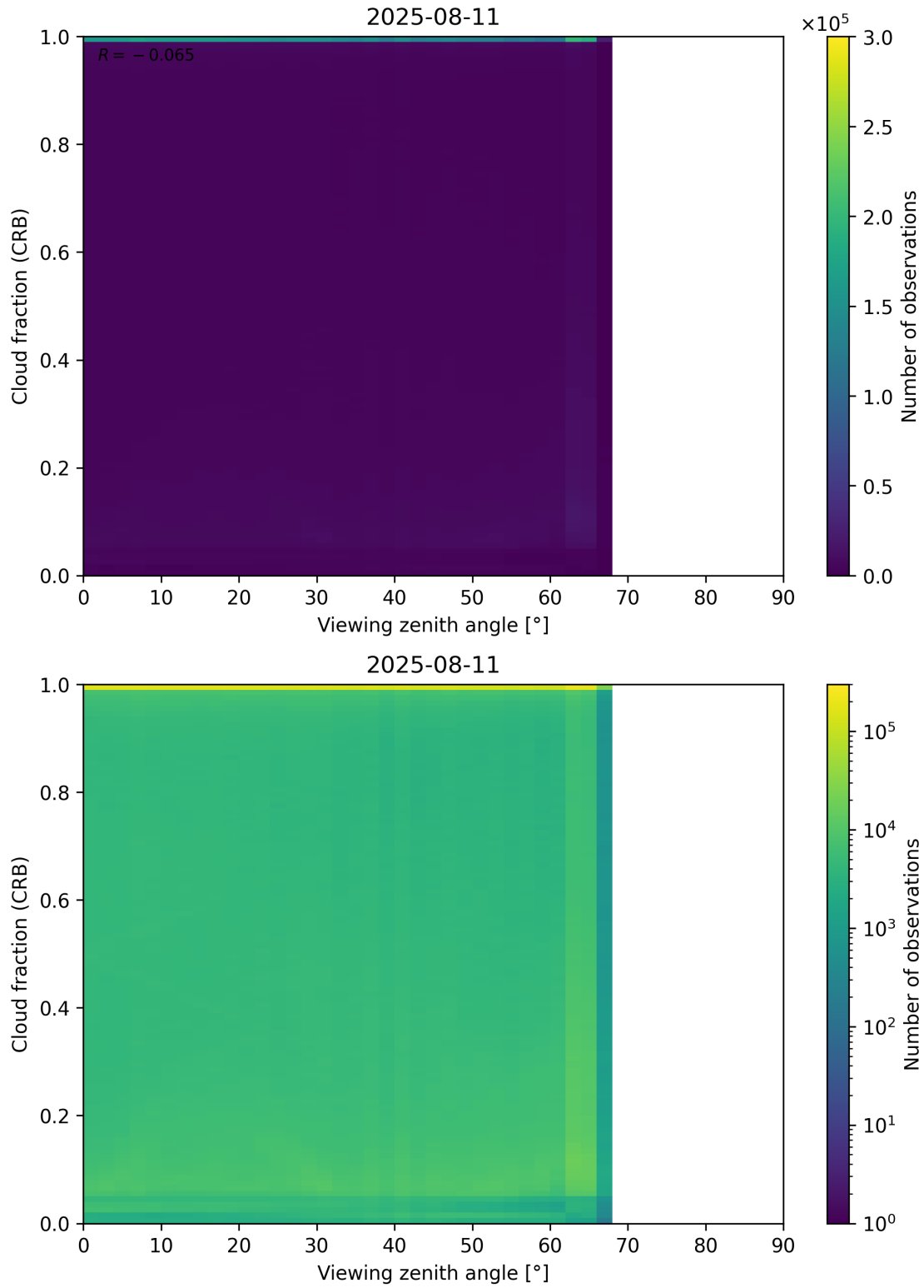
Figure 109: Scatter density plot of “Viewing zenith angle” against “Cloud fraction (CRB)” for 2025-08-10 to 2025-08-12.
