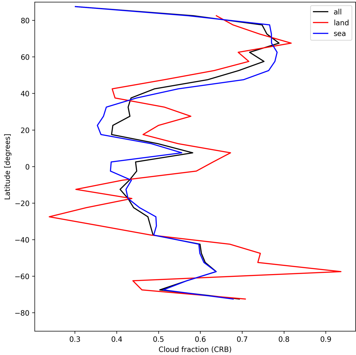
Figure 26: Zonal average of “Cloud fraction (CRB)” for 2025-08-10 to 2025-08-12.
