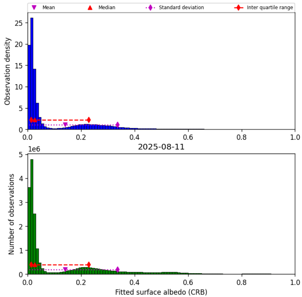
Figure 46: Histogram of “Fitted surface albedo (CRB)” for 2025-08-10 to 2025-08-12
