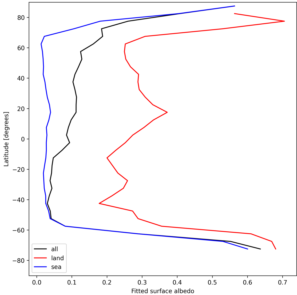
Figure 29: Zonal average of “Fitted surface albedo” for 2025-08-10 to 2025-08-12.
