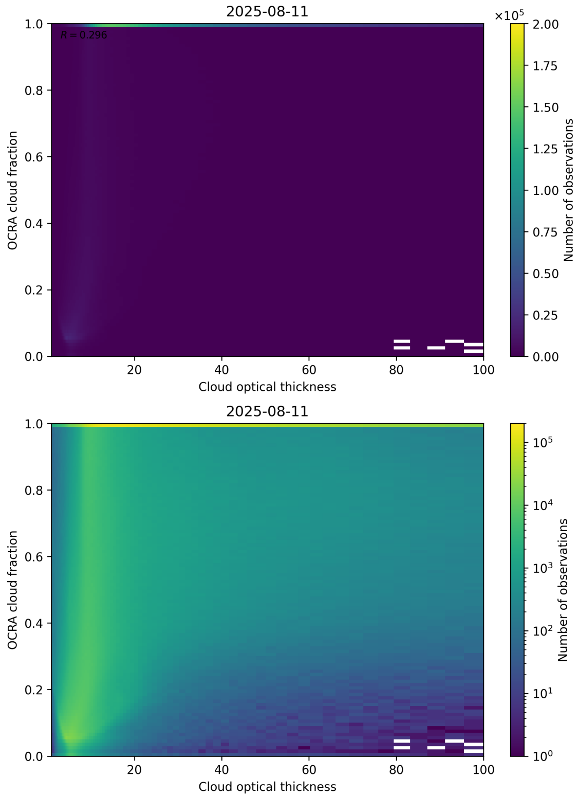
Figure 83: Scatter density plot of “Cloud optical thickness” against “OCRA cloud fraction” for 2025-08-10 to 2025-08-12.
