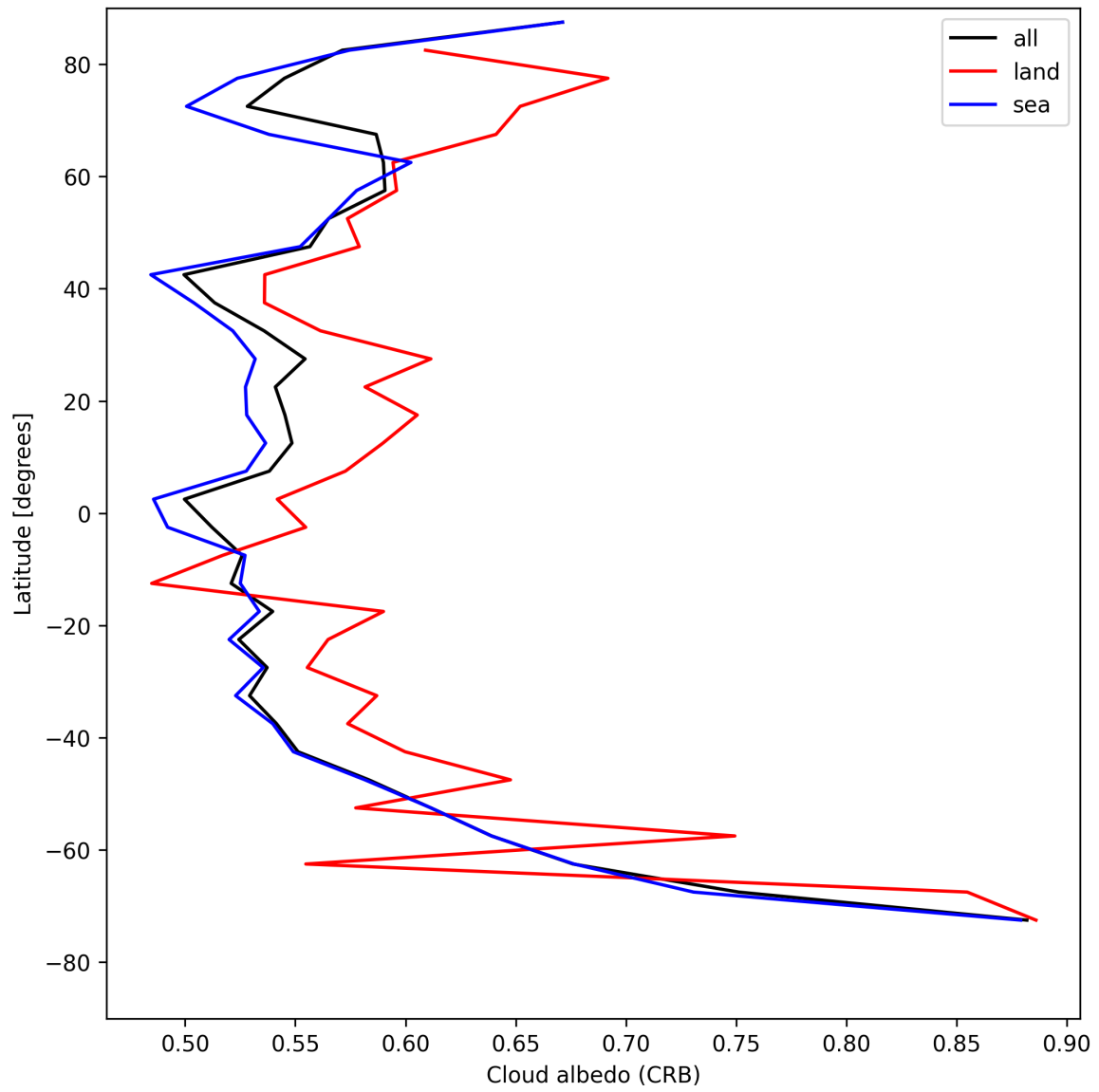
Figure 28: Zonal average of “Cloud albedo (CRB)” for 2025-08-10 to 2025-08-12.
