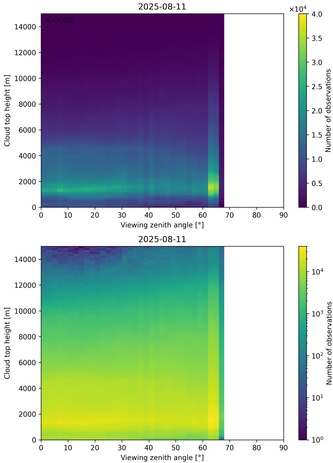
Figure 112: Scatter density plot of “Viewing zenith angle” against “Cloud top height” for 2025-08-10 to 2025-08-12.
