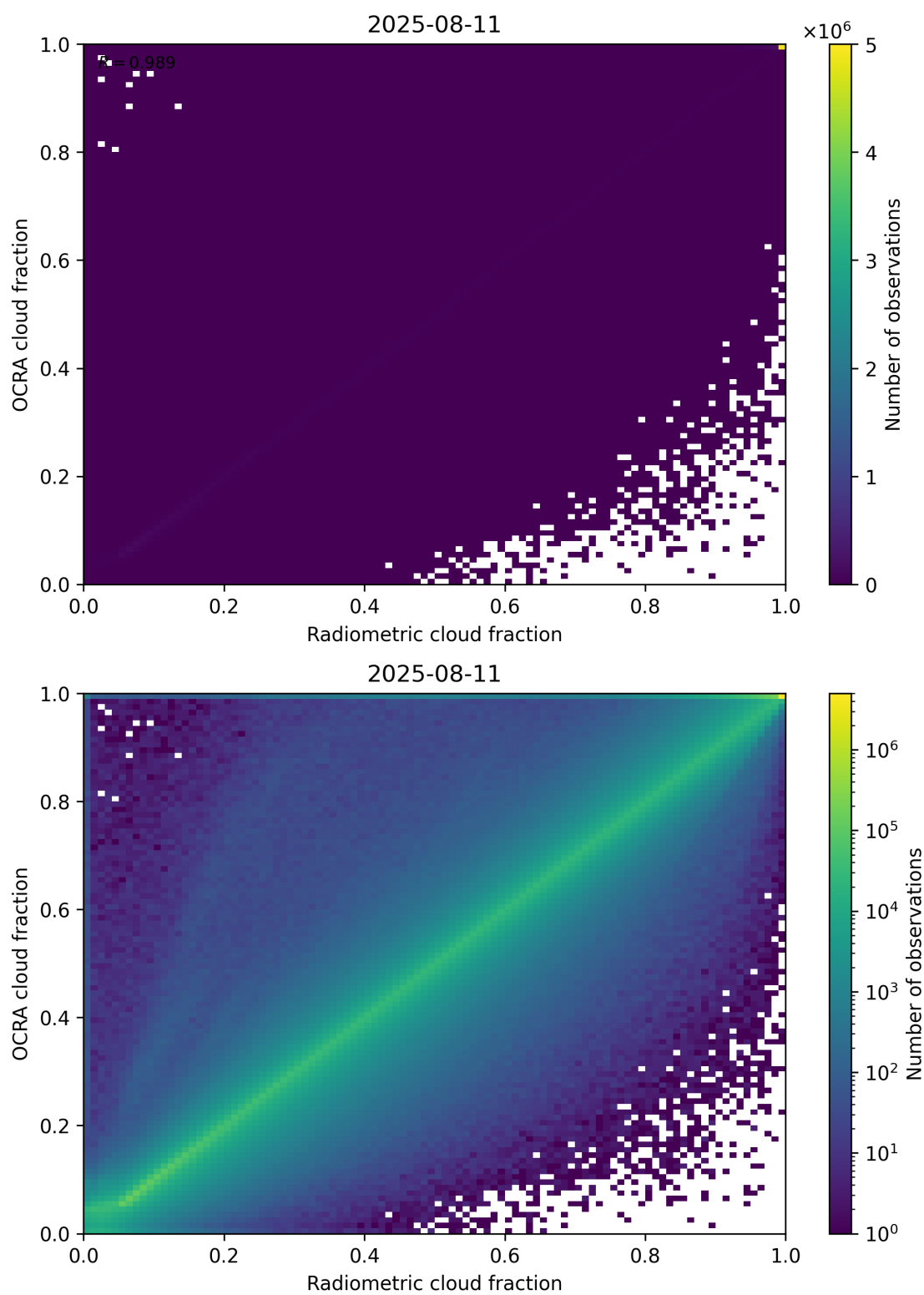
Figure 72: Scatter density plot of “Radiometric cloud fraction” against “OCRA cloud fraction” for 2025-08-10 to 2025-08-12.
