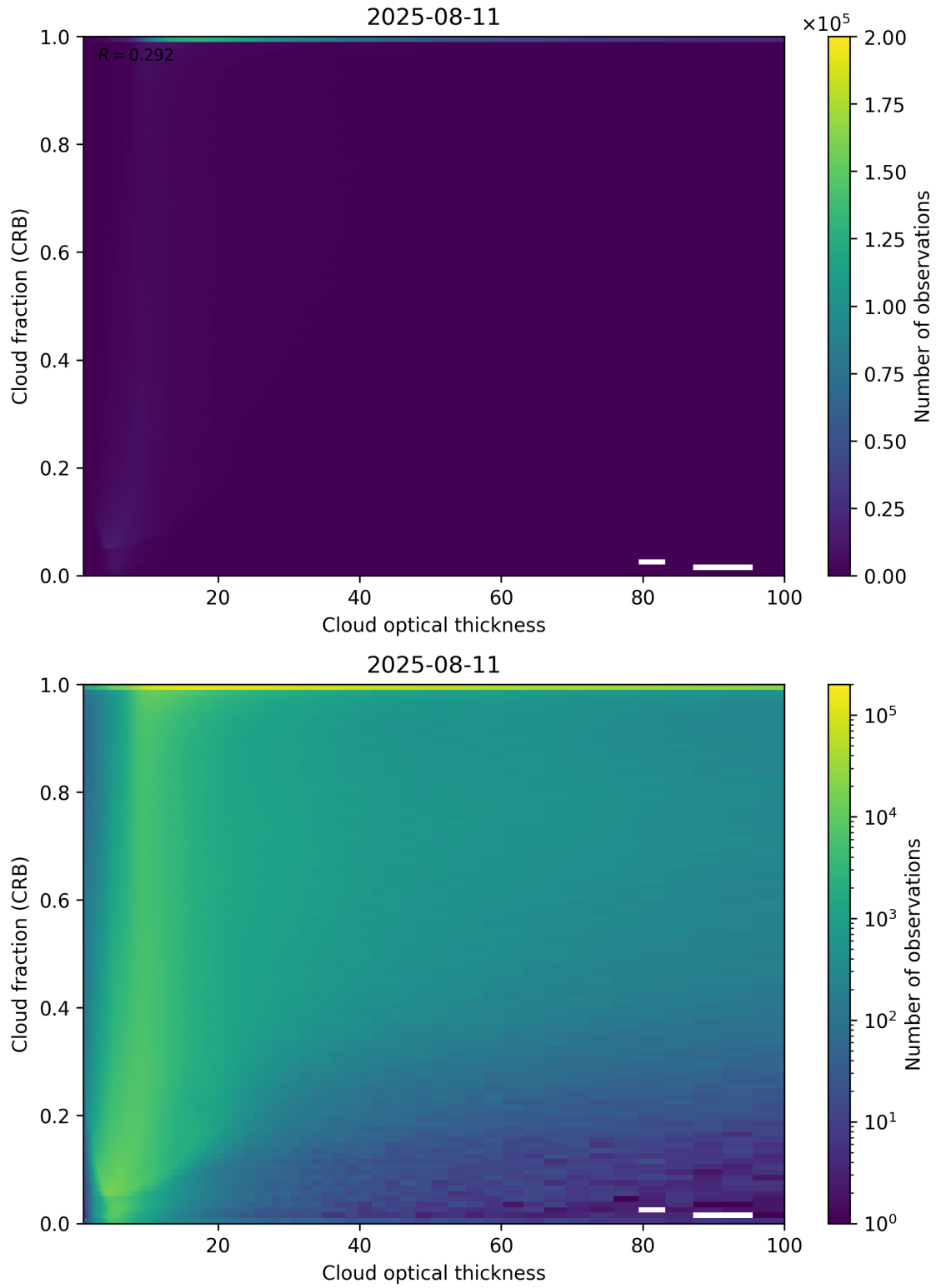
Figure 84: Scatter density plot of “Cloud optical thickness” against “Cloud fraction (CRB)” for 2025-08-10 to 2025-08-12.
