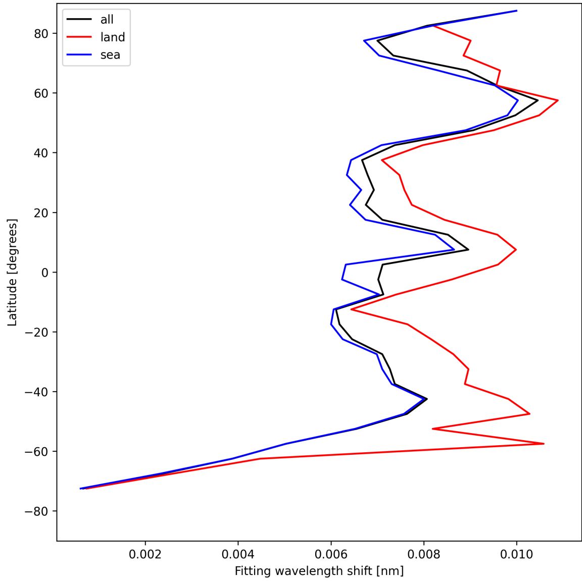
Figure 33: Zonal average of “Fitting wavelength shift” for 2025-08-10 to 2025-08-12.
