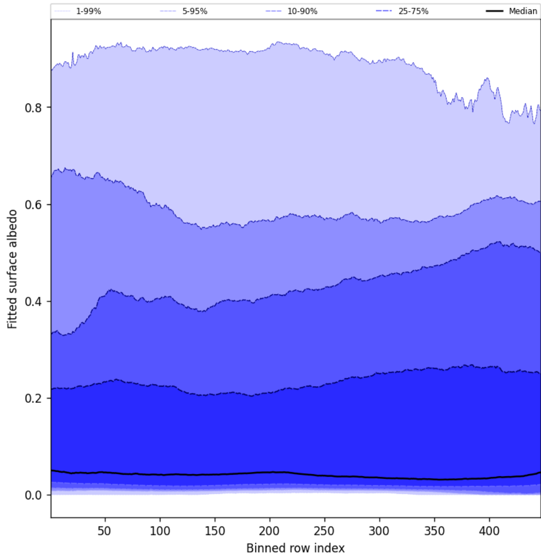
Figure 61: Along track statistics of “Fitted surface albedo” for 2025-08-10 to 2025-08-12
