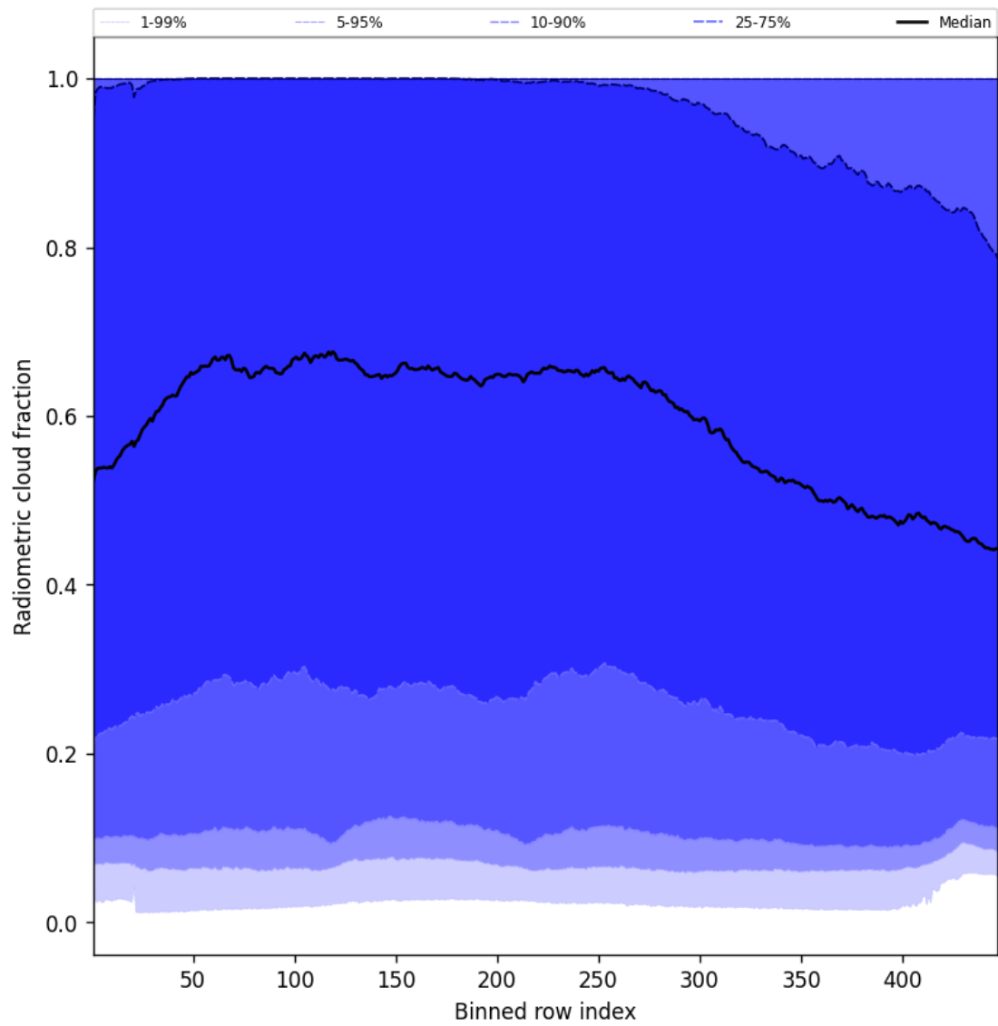
Figure 55: Along track statistics of “Radiometric cloud fraction” for 2025-08-10 to 2025-08-12
