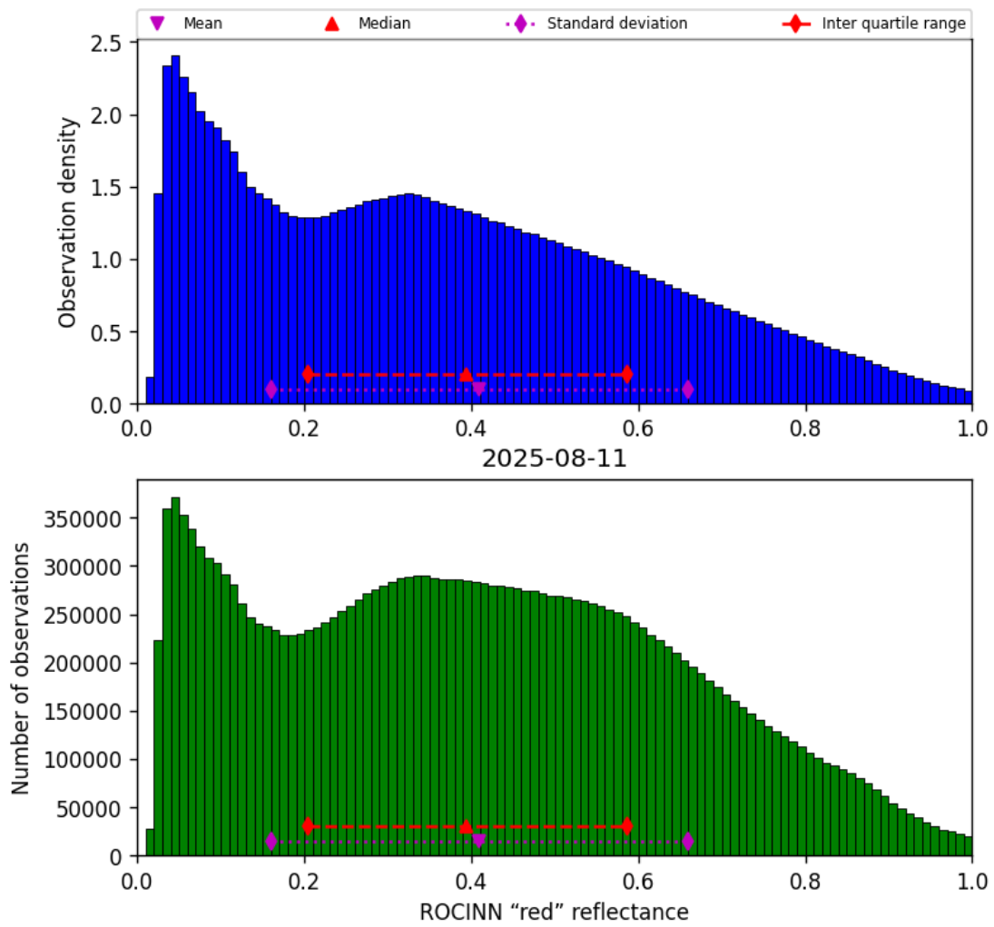
Figure 53: Histogram of “ROCINN “red” reflectance” for 2025-08-10 to 2025-08-12
