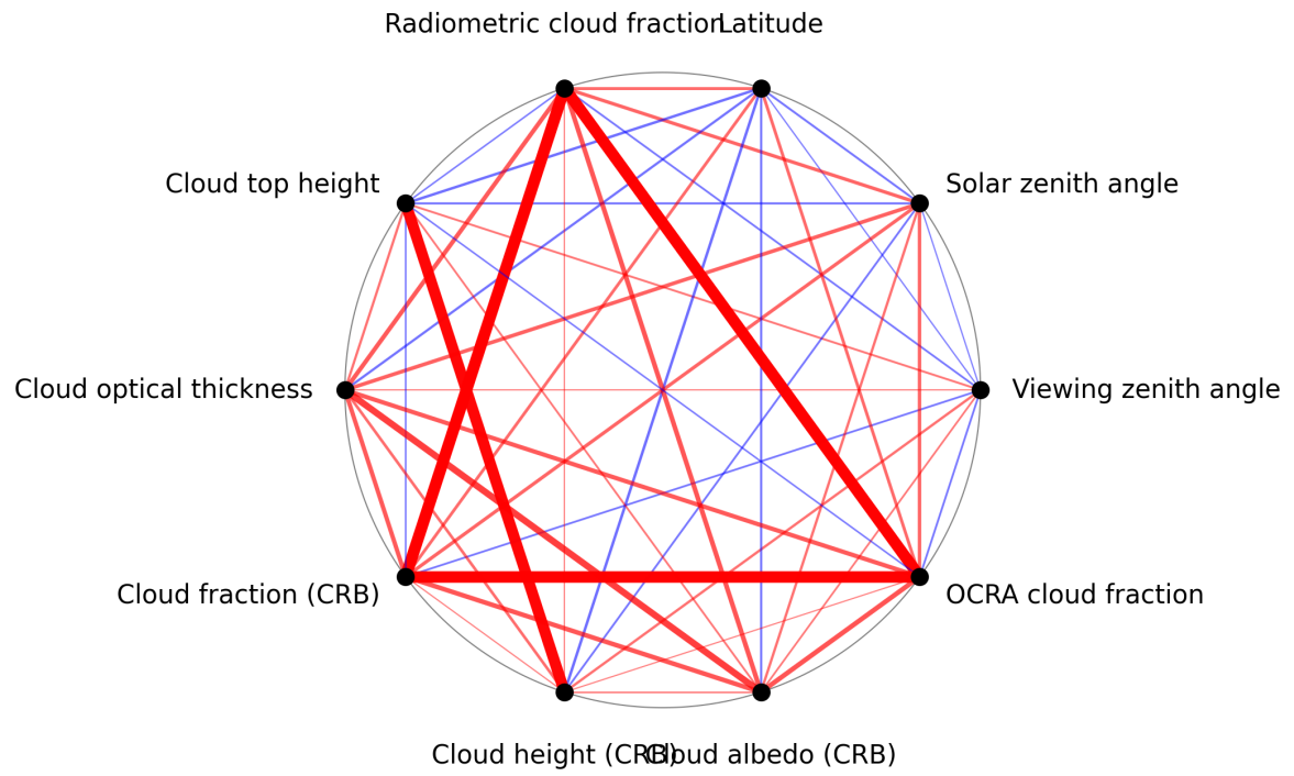
Figure 1: Map of correlation graph for 2025-08-10 to 2025-08-12.
