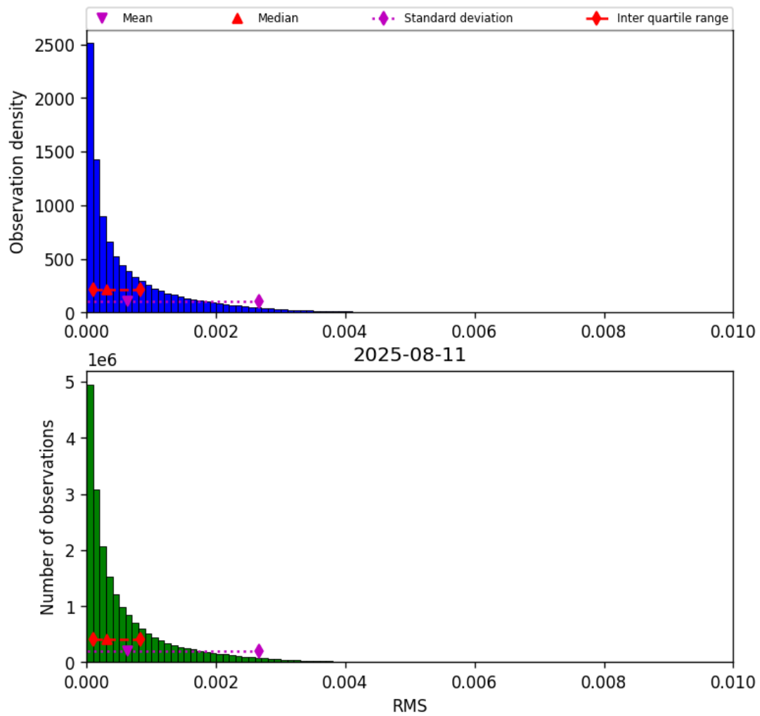
Figure 47: Histogram of “RMS” for 2025-08-10 to 2025-08-12
