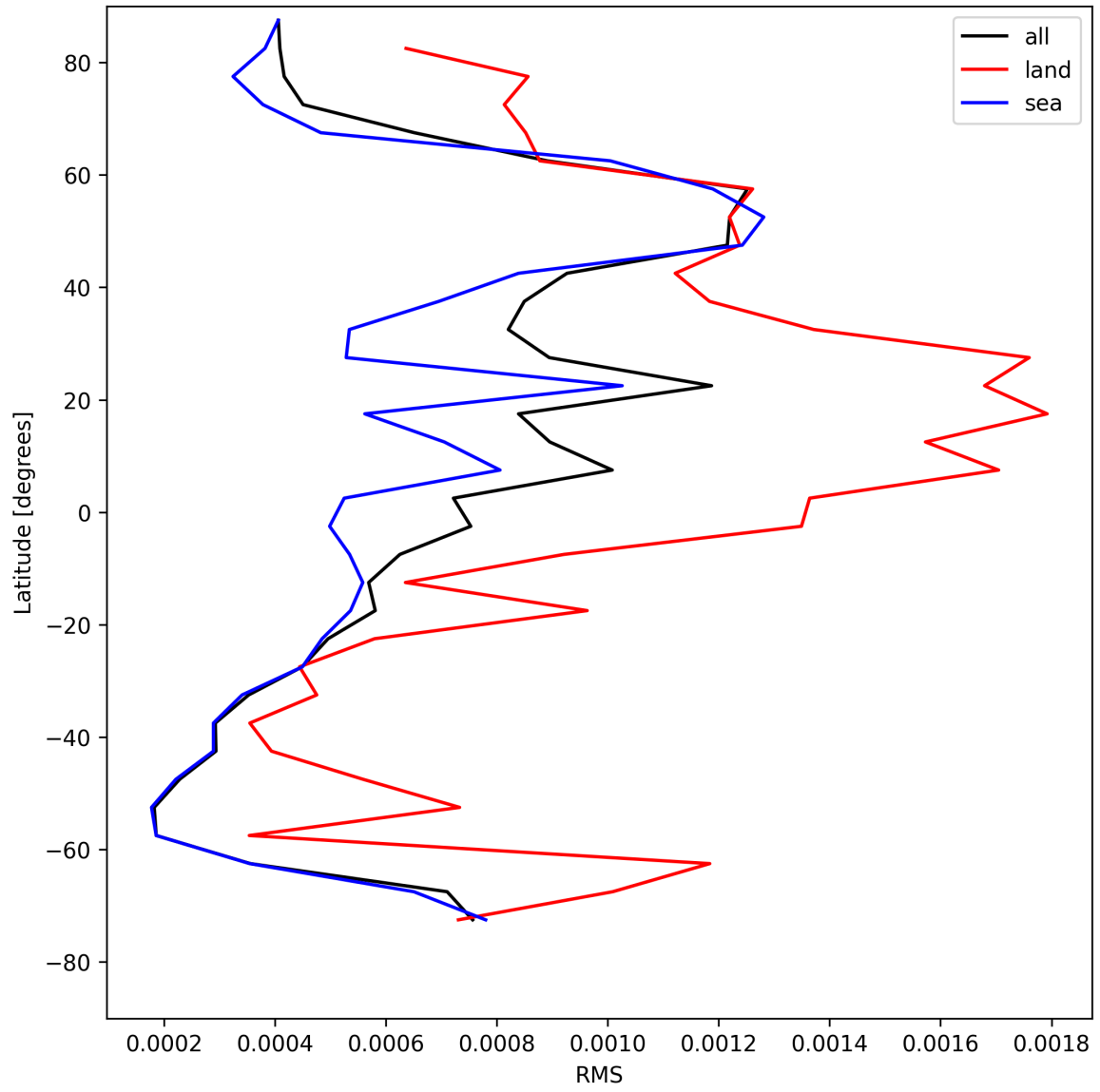
Figure 31: Zonal average of “RMS” for 2025-08-10 to 2025-08-12.
