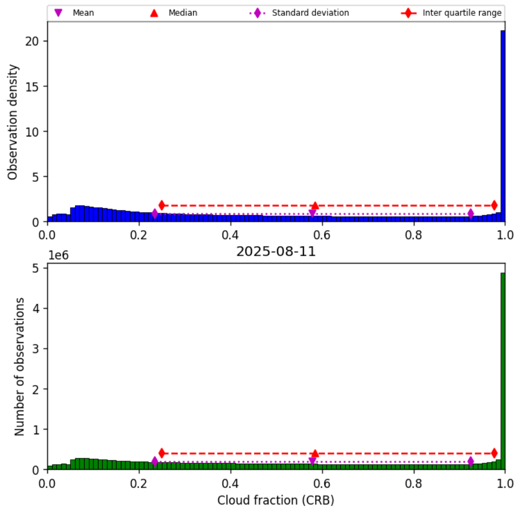
Figure 42: Histogram of “Cloud fraction (CRB)” for 2025-08-10 to 2025-08-12
