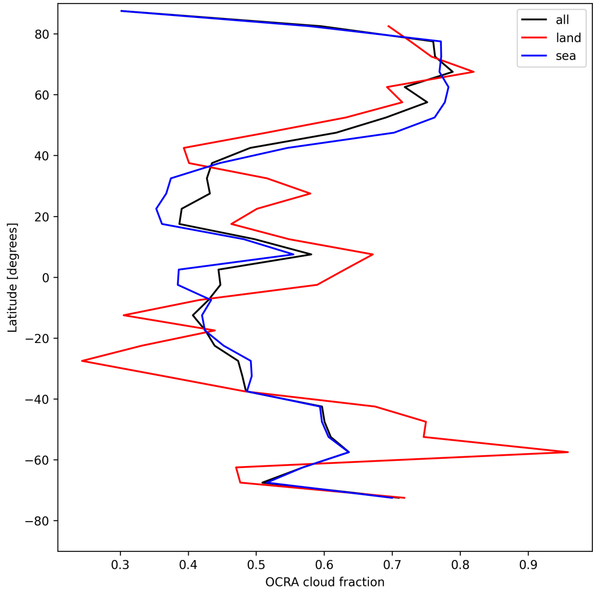
Figure 34: Zonal average of “OCRA cloud fraction” for 2025-08-10 to 2025-08-12.
