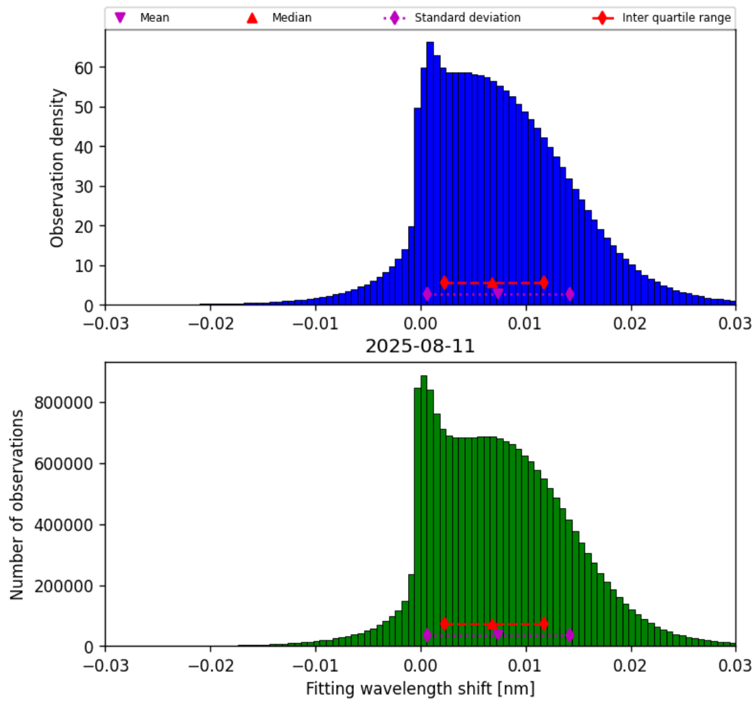
Figure 49: Histogram of “Fitting wavelength shift” for 2025-08-10 to 2025-08-12
