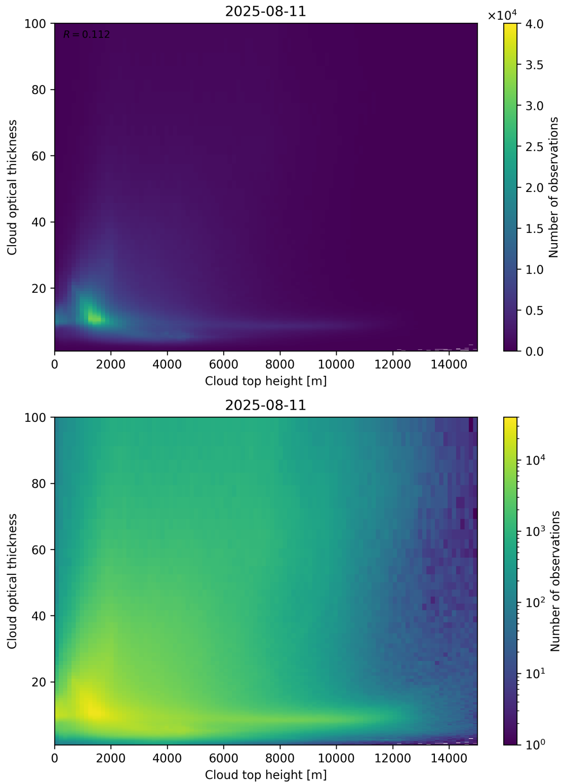
Figure 90: Scatter density plot of “Cloud top height” against “Cloud optical thickness” for 2025-08-10 to 2025-08-12.
