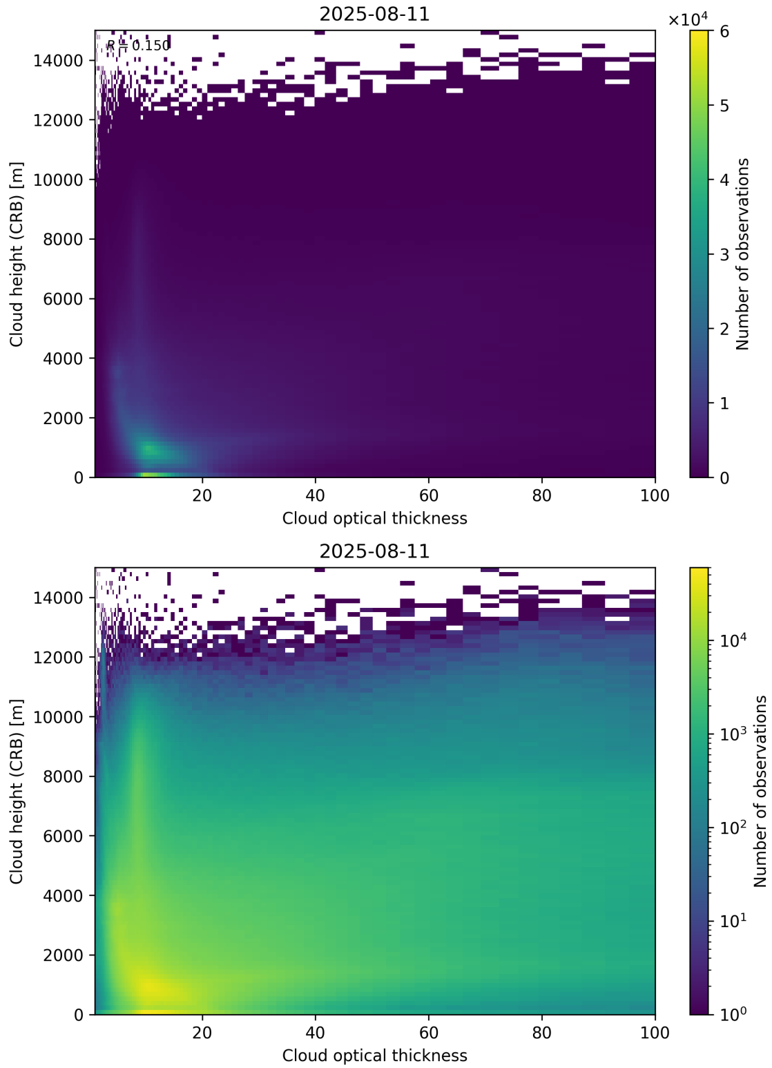
Figure 85: Scatter density plot of “Cloud optical thickness” against “Cloud height (CRB)” for 2025-08-10 to 2025-08-12.
