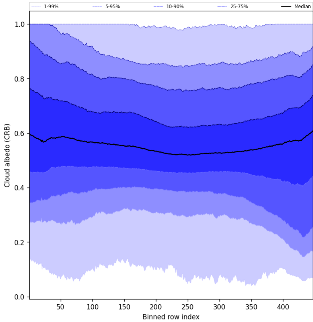
Figure 60: Along track statistics of “Cloud albedo (CRB)” for 2025-08-10 to 2025-08-12
