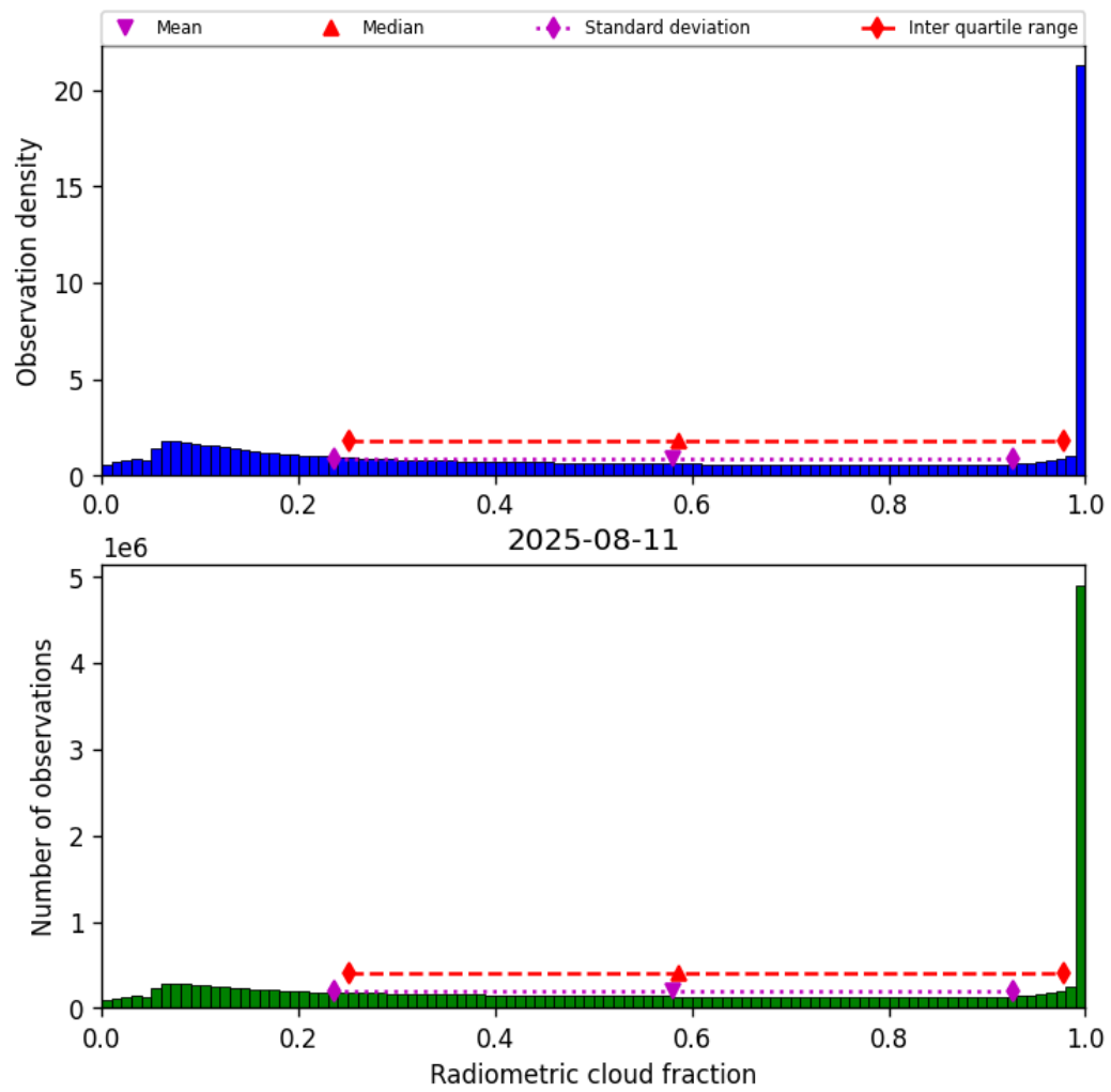
Figure 39: Histogram of “Radiometric cloud fraction” for 2025-08-10 to 2025-08-12
