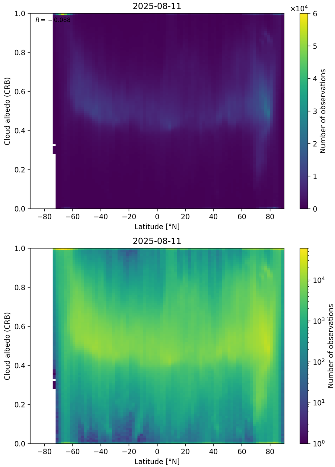
Figure 91: Scatter density plot of “Latitude” against “Cloud albedo (CRB)” for 2025-08-10 to 2025-08-12.
