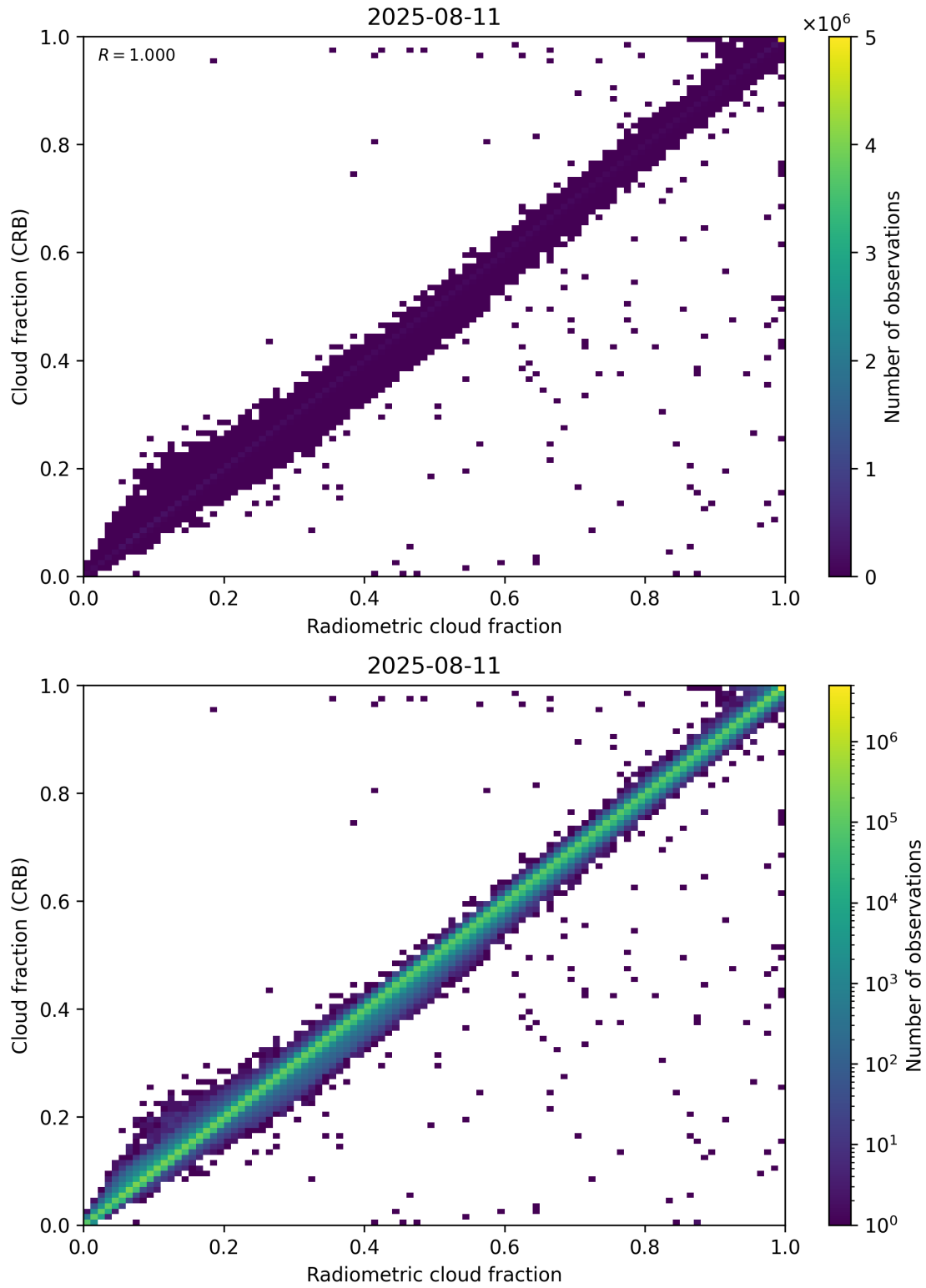
Figure 73: Scatter density plot of “Radiometric cloud fraction” against “Cloud fraction (CRB)” for 2025-08-10 to 2025-08-12.
