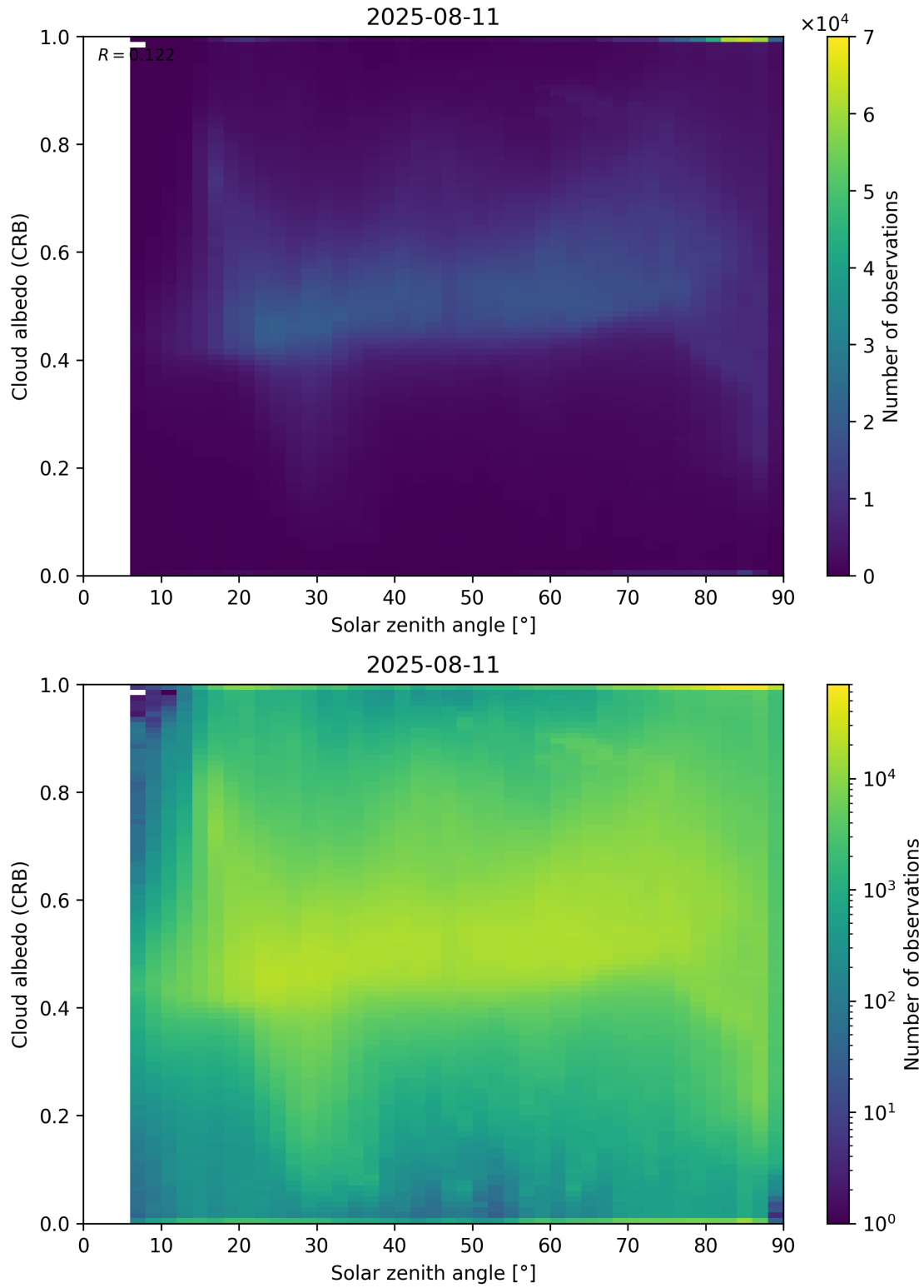
Figure 98: Scatter density plot of “Solar zenith angle” against “Cloud albedo (CRB)” for 2025-08-10 to 2025-08-12.
