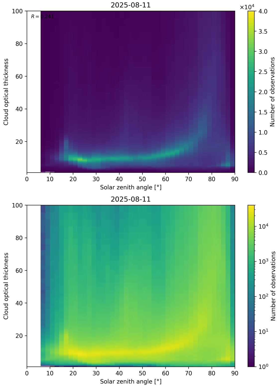
Figure 103: Scatter density plot of “Solar zenith angle” against “Cloud optical thickness” for 2025-08-10 to 2025-08-12.
