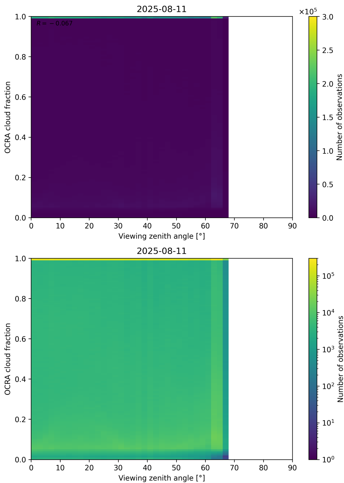
Figure 108: Scatter density plot of “Viewing zenith angle” against “OCRA cloud fraction” for 2025-08-10 to 2025-08-12.
