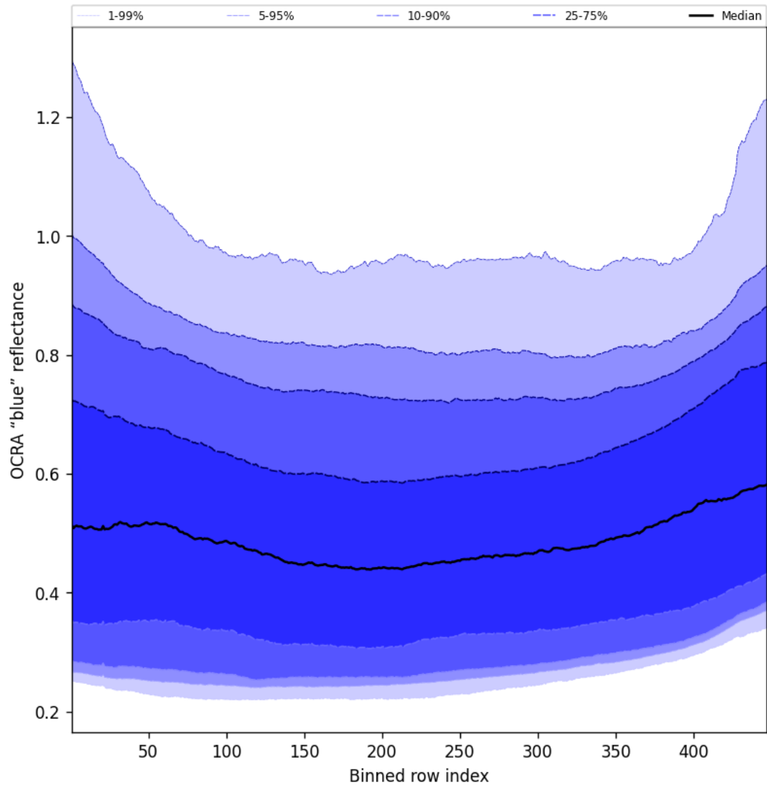
Figure 67: Along track statistics of “OCRA “blue” reflectance” for 2025-08-10 to 2025-08-12
