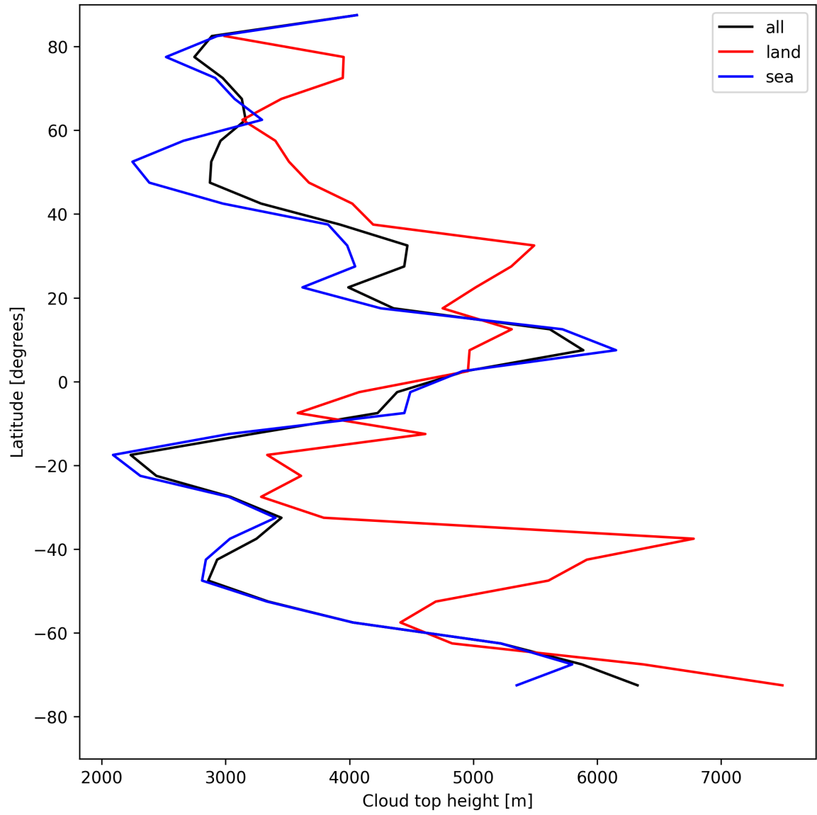
Figure 24: Zonal average of “Cloud top height” for 2025-08-10 to 2025-08-12.
