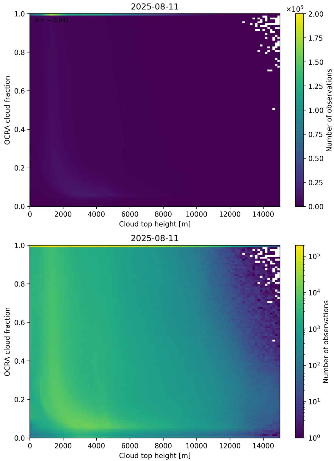
Figure 87: Scatter density plot of “Cloud top height” against “OCRA cloud fraction” for 2025-08-10 to 2025-08-12.
