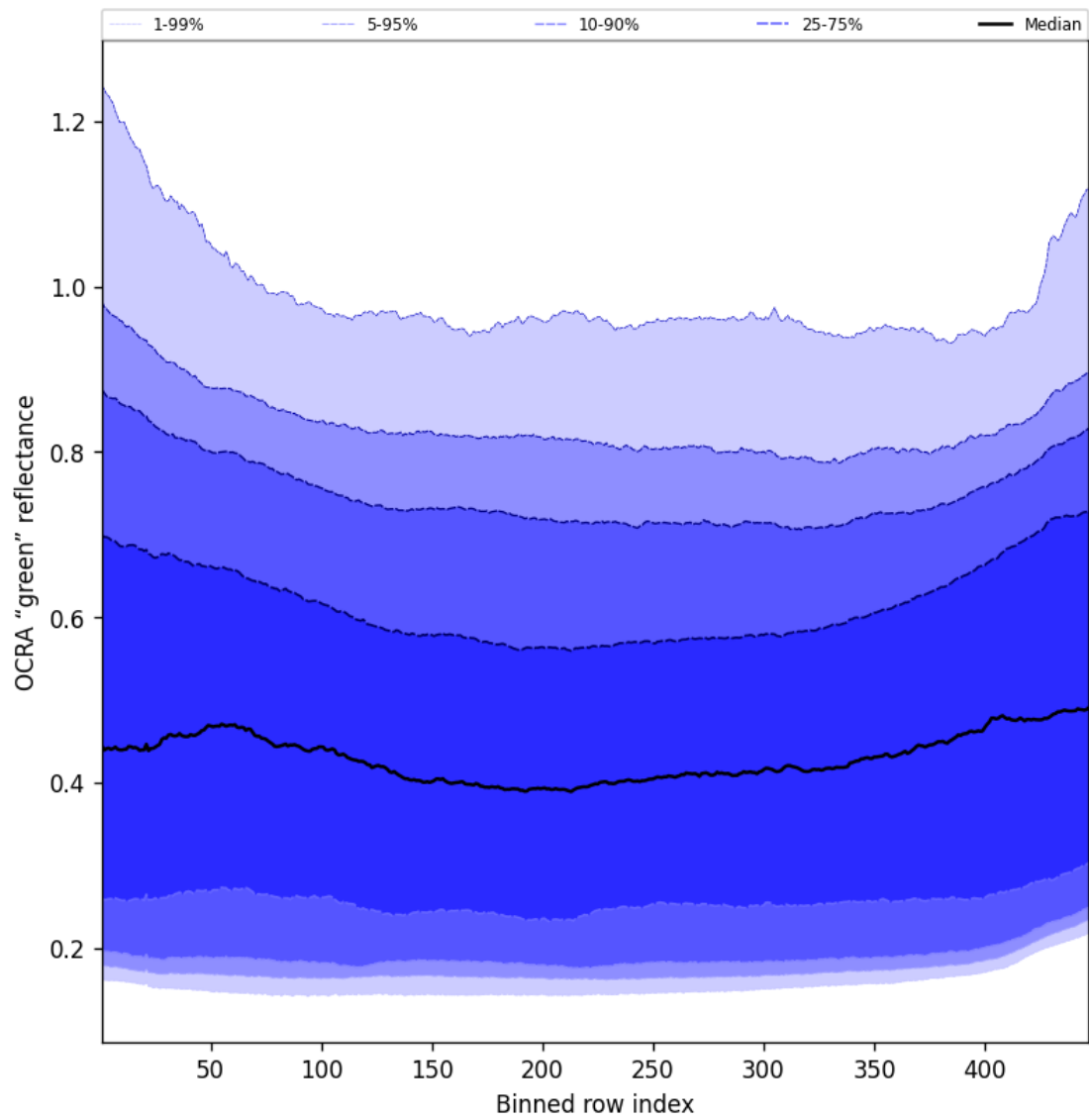
Figure 68: Along track statistics of "OCRA "green" reflectance" for 2025-08-10 to 2025-08-12
