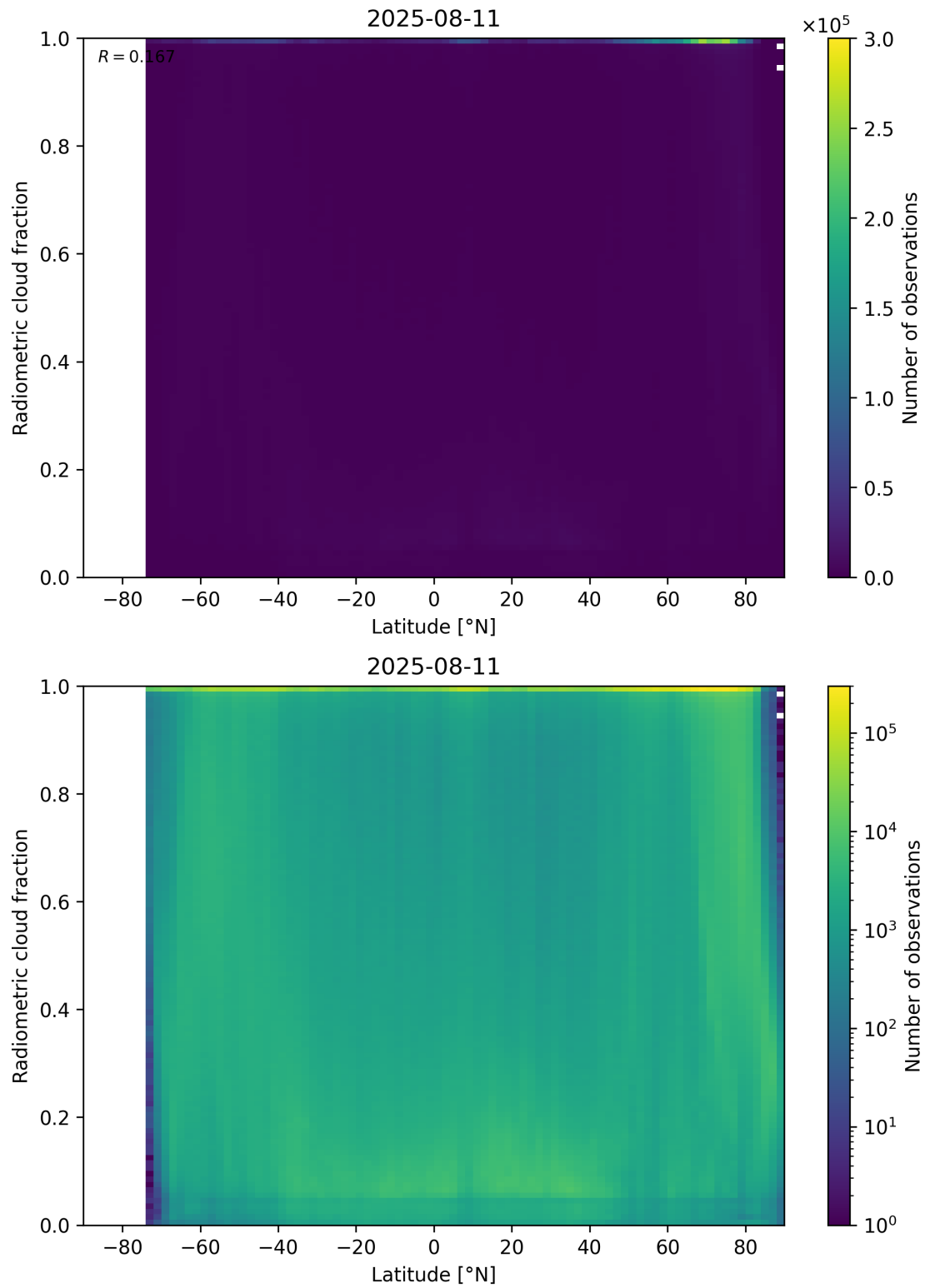
Figure 92: Scatter density plot of “Latitude” against “Radiometric cloud fraction” for 2025-08-10 to 2025-08-12.
