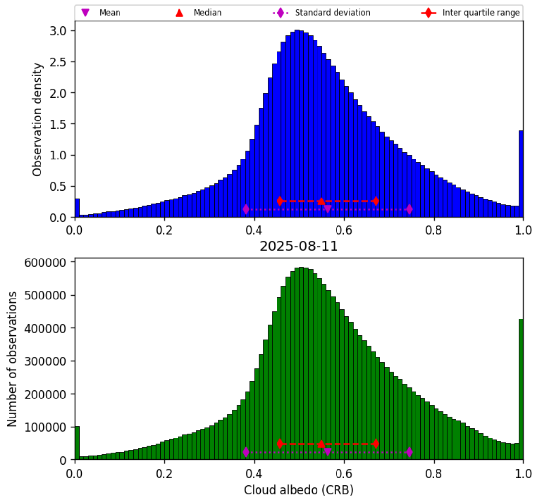
Figure 44: Histogram of “Cloud albedo (CRB)” for 2025-08-10 to 2025-08-12
