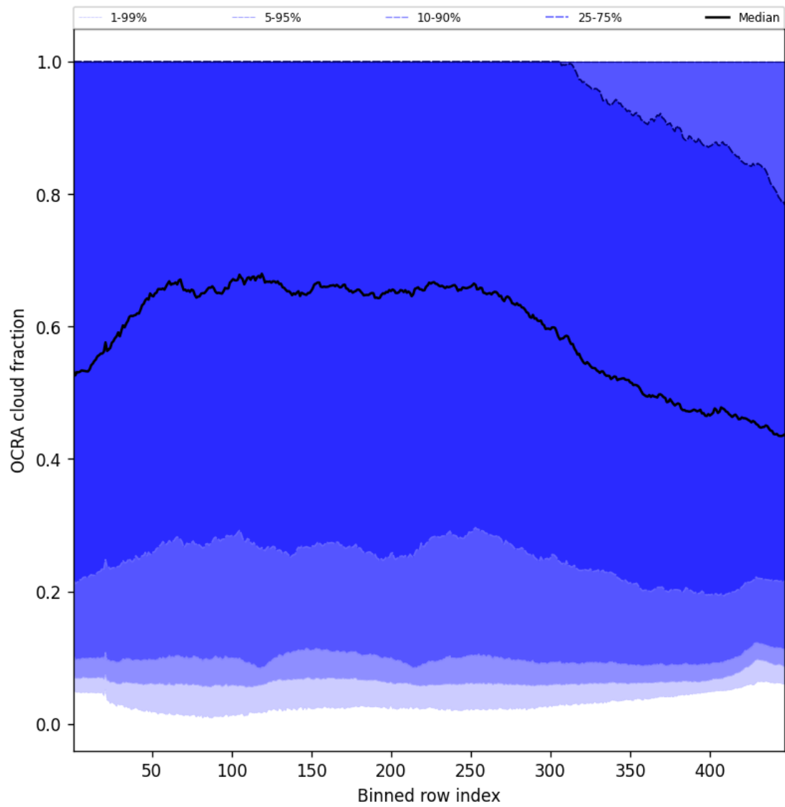
Figure 66: Along track statistics of “OCRA cloud fraction” for 2025-08-10 to 2025-08-12
