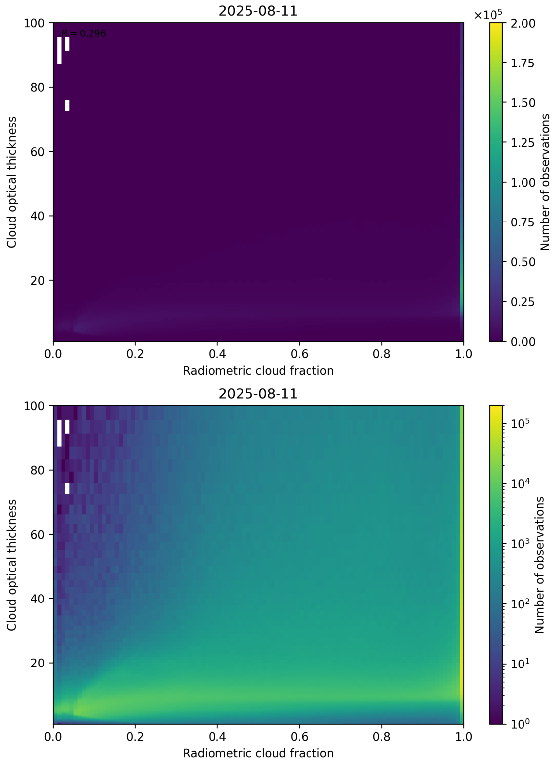
Figure 75: Scatter density plot of “Radiometric cloud fraction” against “Cloud optical thickness” for 2025-08-10 to 2025-08-12.
