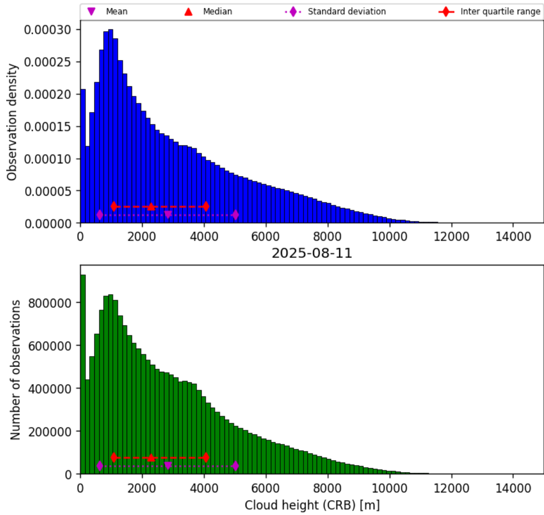
Figure 43: Histogram of “Cloud height (CRB)” for 2025-08-10 to 2025-08-12
