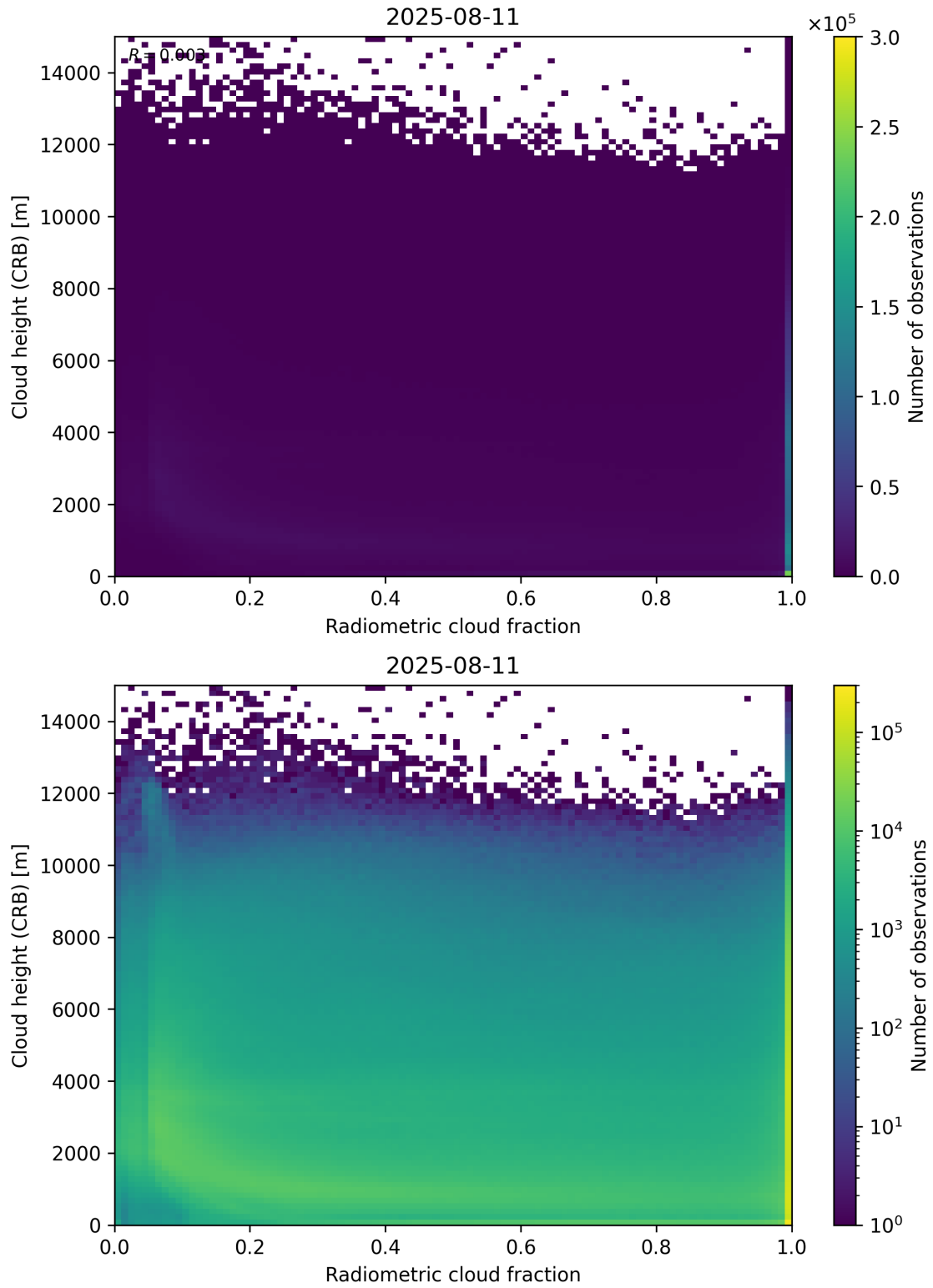
Figure 74: Scatter density plot of “Radiometric cloud fraction” against “Cloud height (CRB)” for 2025-08-10 to 2025-08-12.
