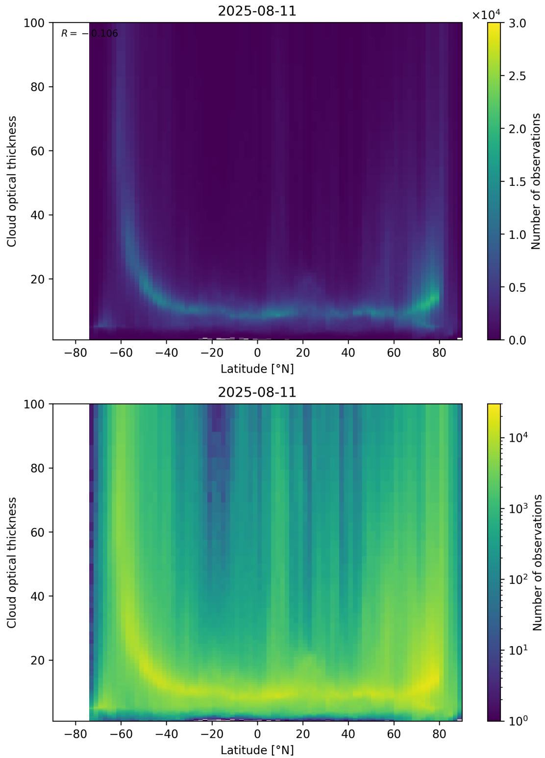
Figure 96: Scatter density plot of “Latitude” against “Cloud optical thickness” for 2025-08-10 to 2025-08-12.
