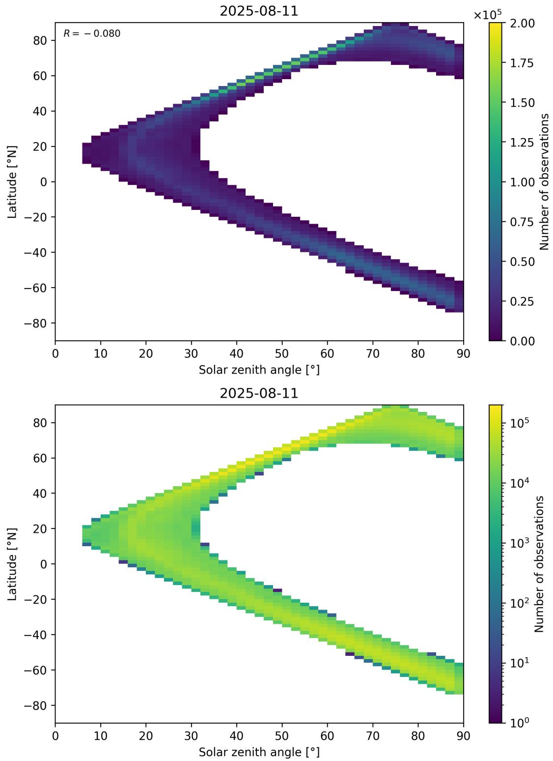
Figure 105: Scatter density plot of “Solar zenith angle” against “Latitude” for 2025-08-10 to 2025-08-12.
