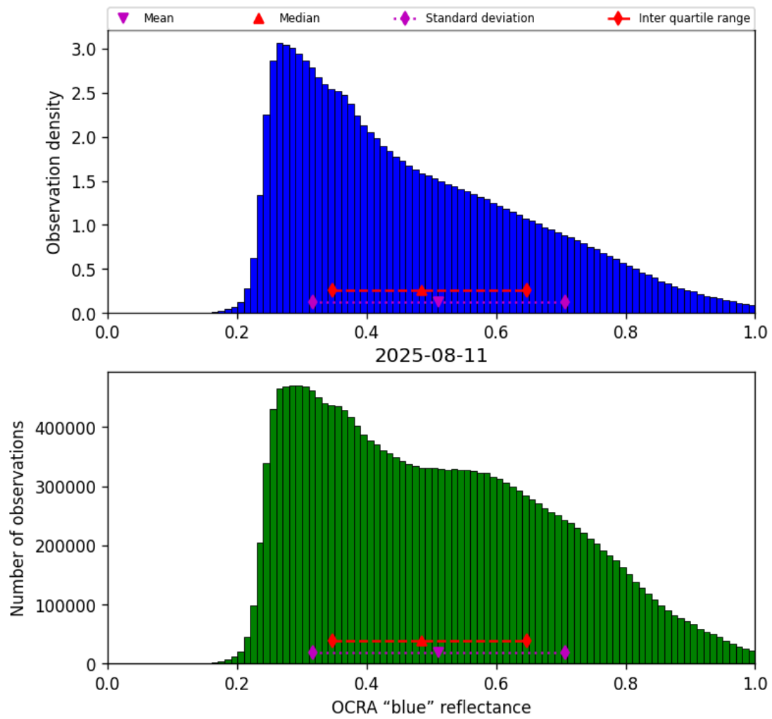
Figure 51: Histogram of “OCRA “blue” reflectance” for 2025-08-10 to 2025-08-12
