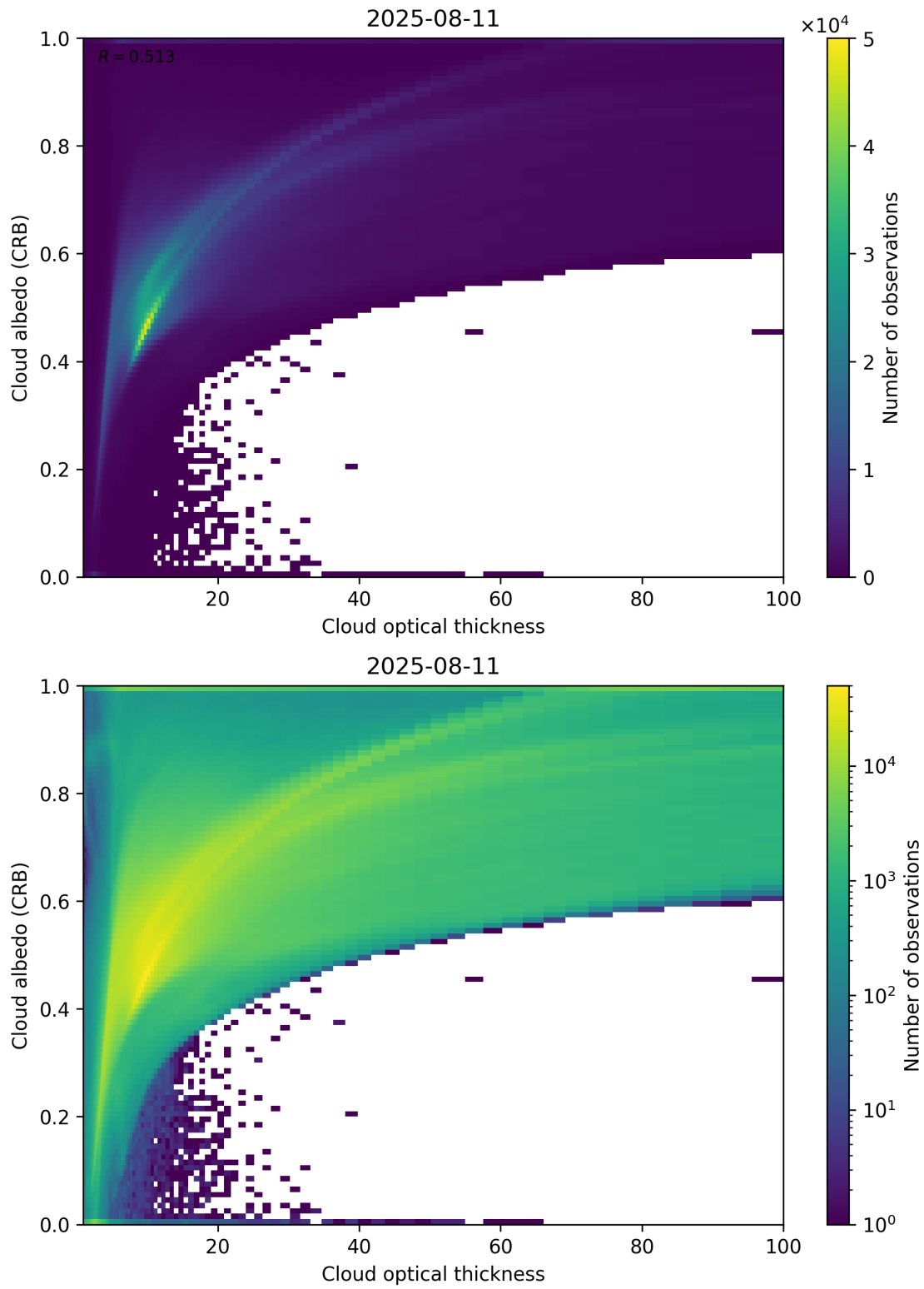
Figure 82: Scatter density plot of “Cloud optical thickness” against “Cloud albedo (CRB)” for 2025-08-10 to 2025-08-12.
