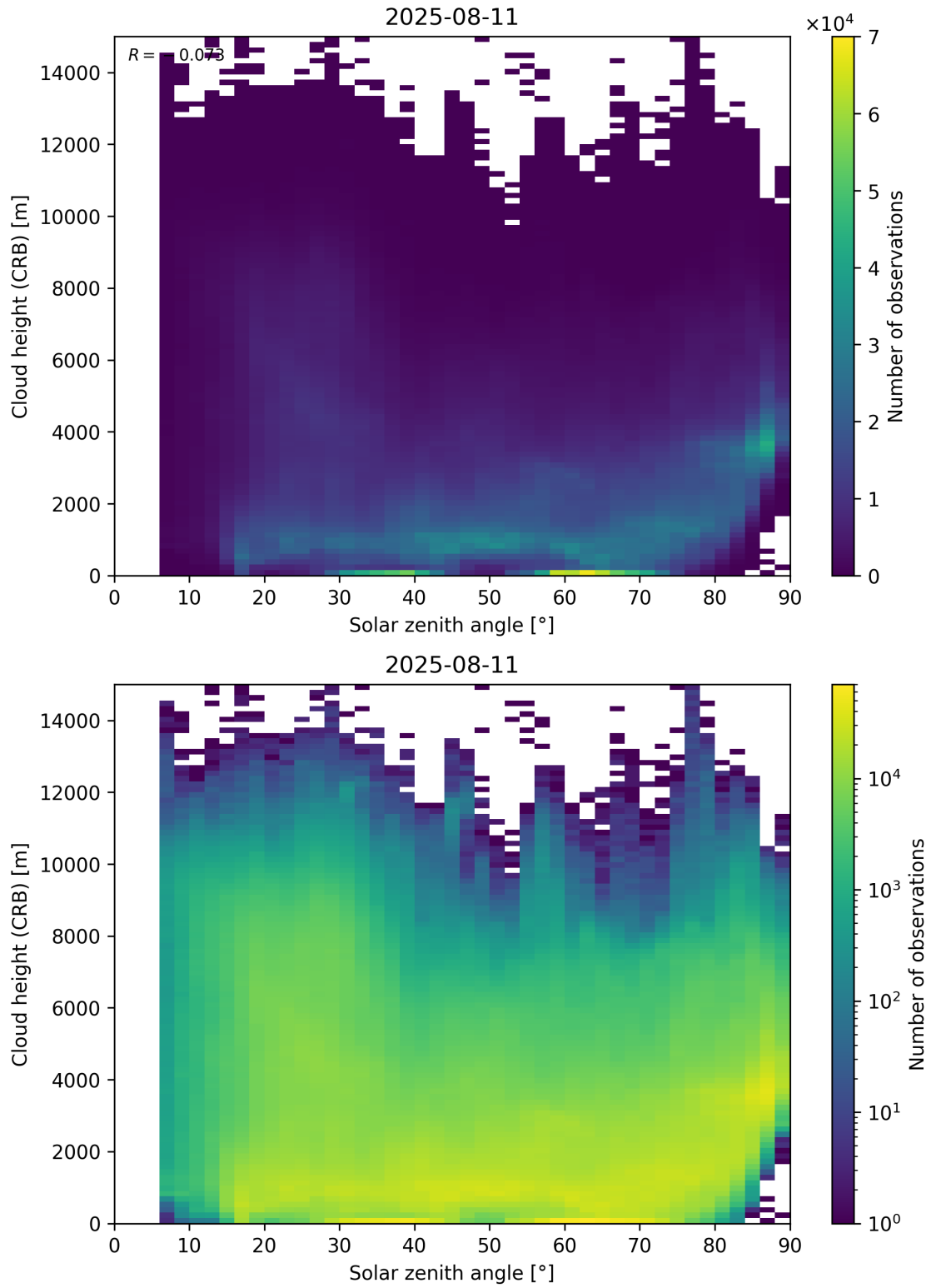
Figure 102: Scatter density plot of “Solar zenith angle” against “Cloud height (CRB)” for 2025-08-10 to 2025-08-12.
