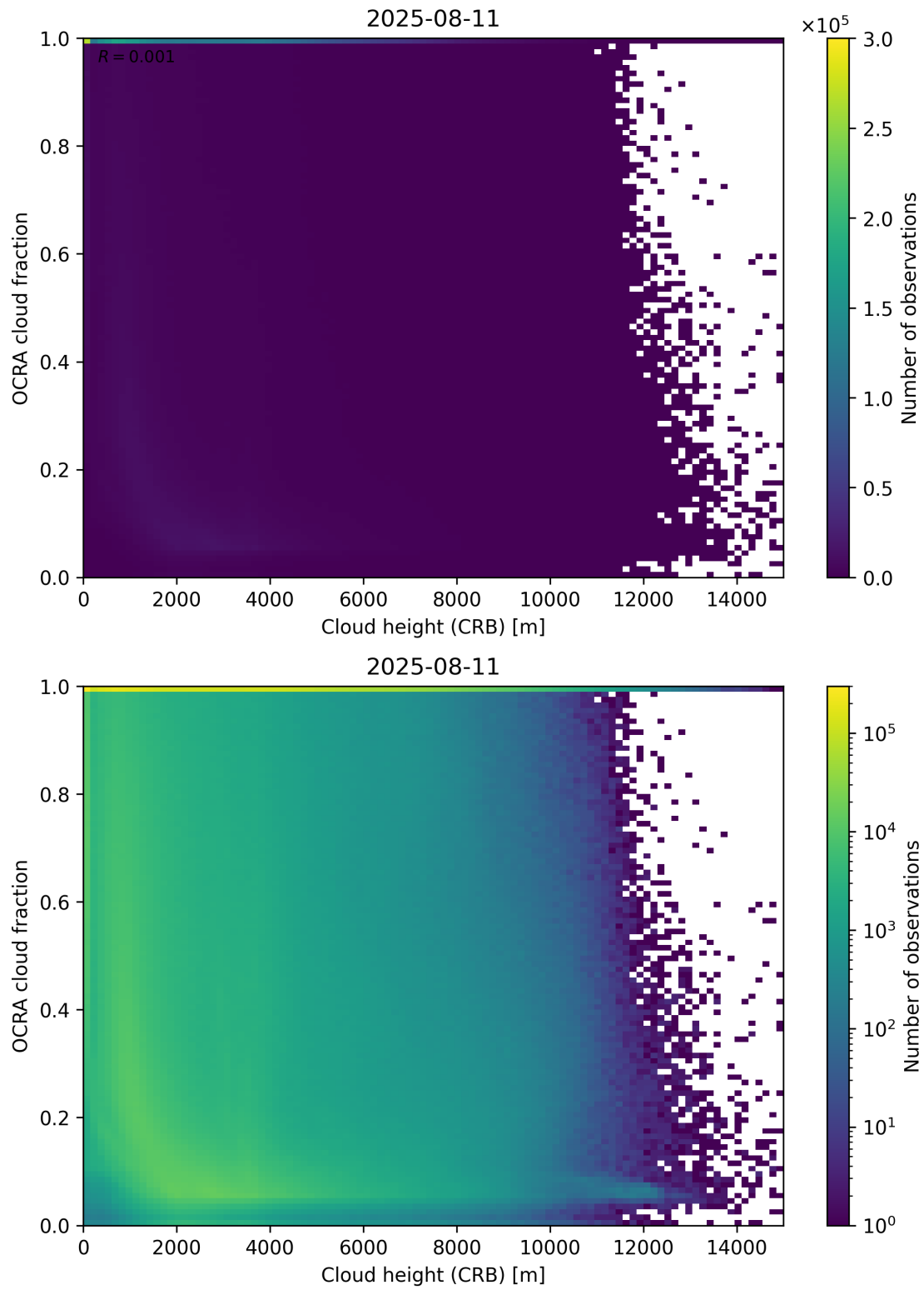
Figure 81: Scatter density plot of “Cloud height (CRB)” against “OCRA cloud fraction” for 2025-08-10 to 2025-08-12.
