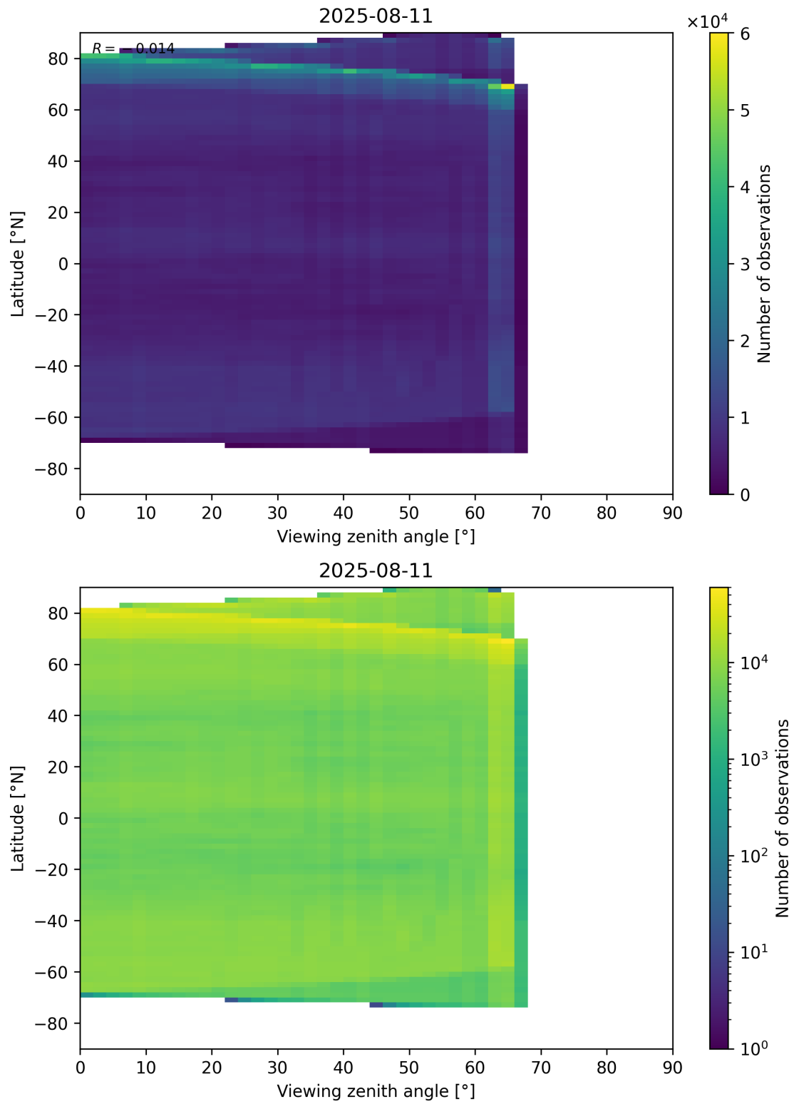
Figure 113: Scatter density plot of “Viewing zenith angle” against “Latitude” for 2025-08-10 to 2025-08-12.
