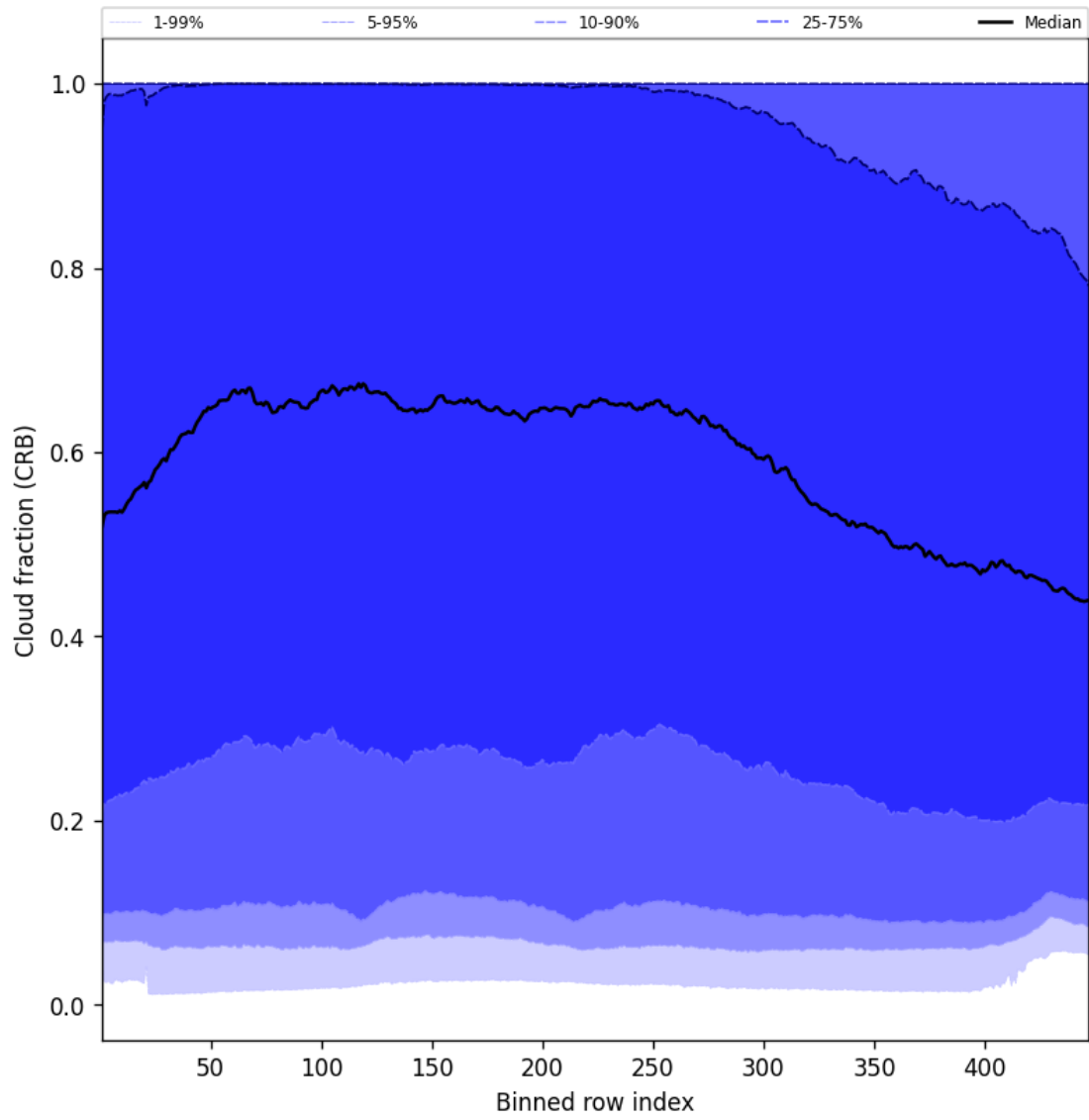
Figure 58: Along track statistics of “Cloud fraction (CRB)” for 2025-08-10 to 2025-08-12
