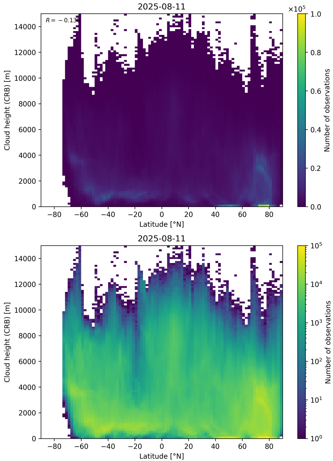
Figure 95: Scatter density plot of “Latitude” against “Cloud height (CRB)” for 2025-08-10 to 2025-08-12.
