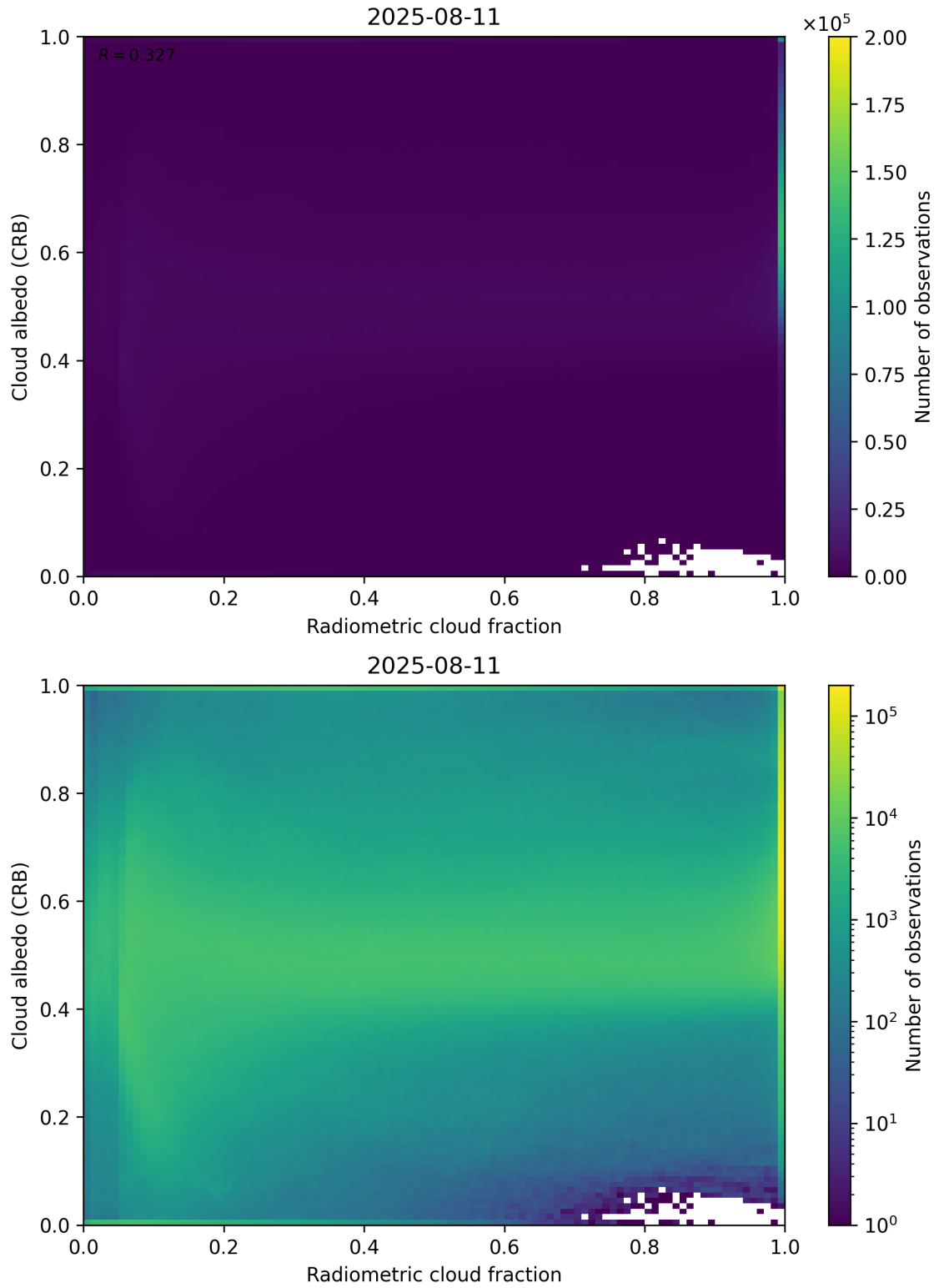
Figure 71: Scatter density plot of “Radiometric cloud fraction” against “Cloud albedo (CRB)” for 2025-08-10 to 2025-08-12.
