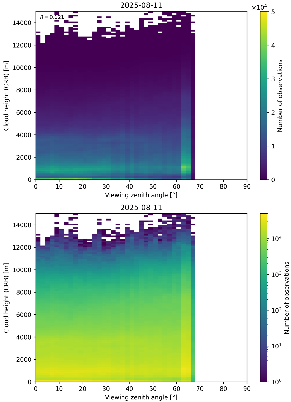
Figure 110: Scatter density plot of “Viewing zenith angle” against “Cloud height (CRB)” for 2025-08-10 to 2025-08-12.
