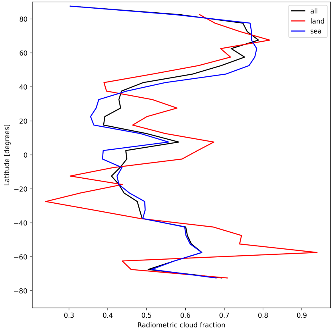
Figure 23: Zonal average of “Radiometric cloud fraction” for 2025-08-10 to 2025-08-12.
