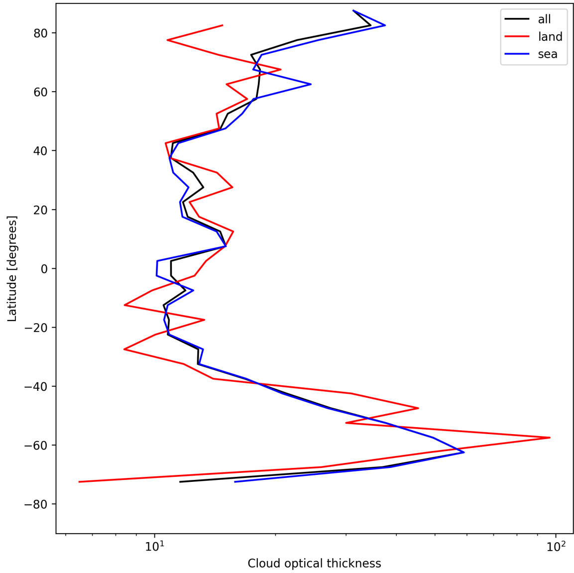
Figure 25: Zonal average of “Cloud optical thickness” for 2025-08-10 to 2025-08-12.
