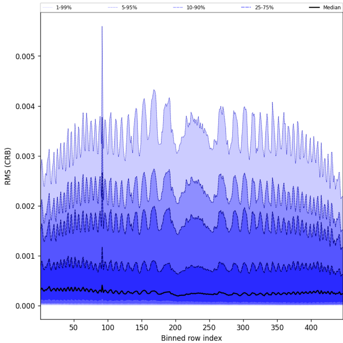
Figure 64: Along track statistics of “RMS (CRB)” for 2025-08-10 to 2025-08-12
