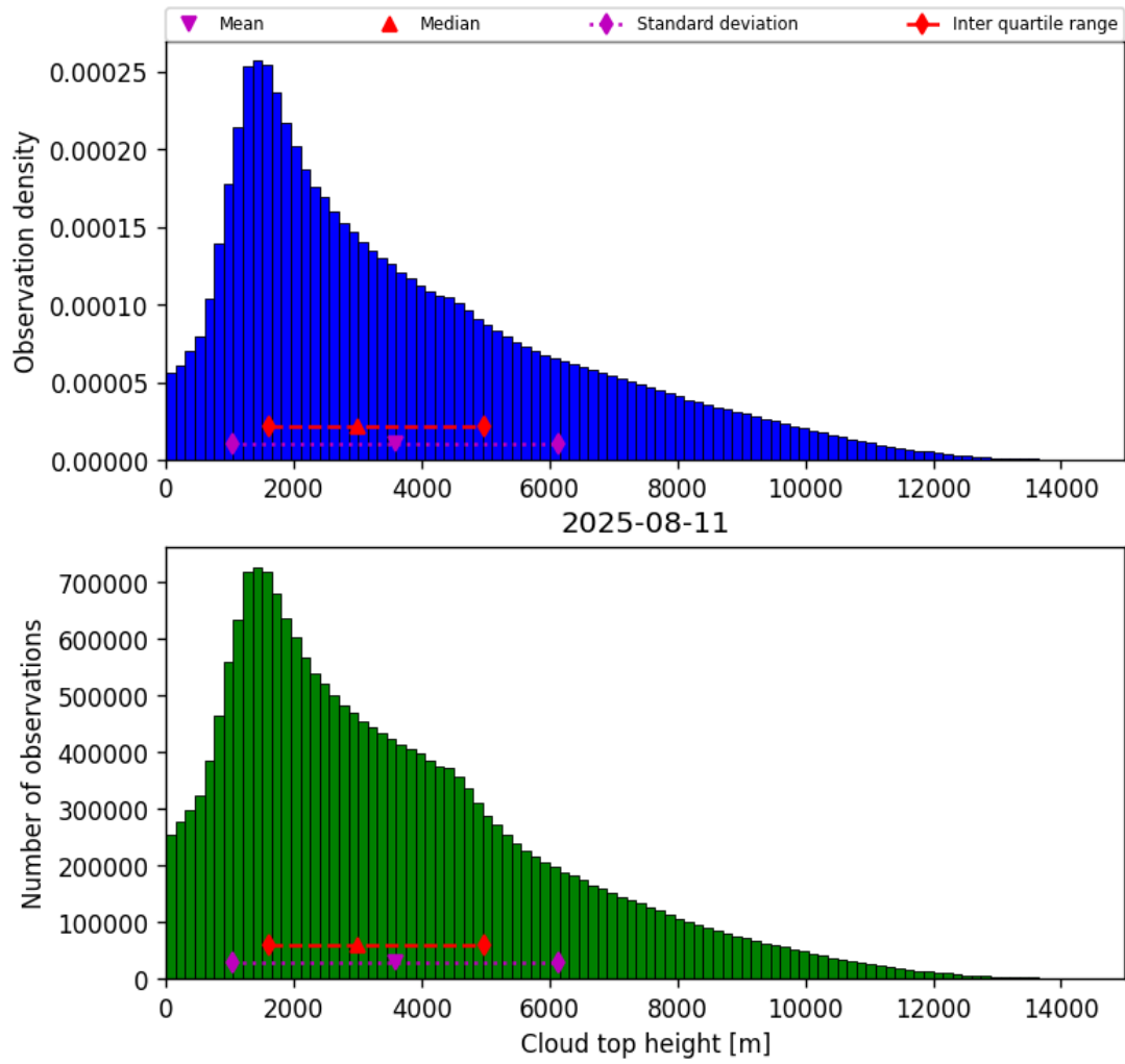
Figure 40: Histogram of “Cloud top height” for 2025-08-10 to 2025-08-12
