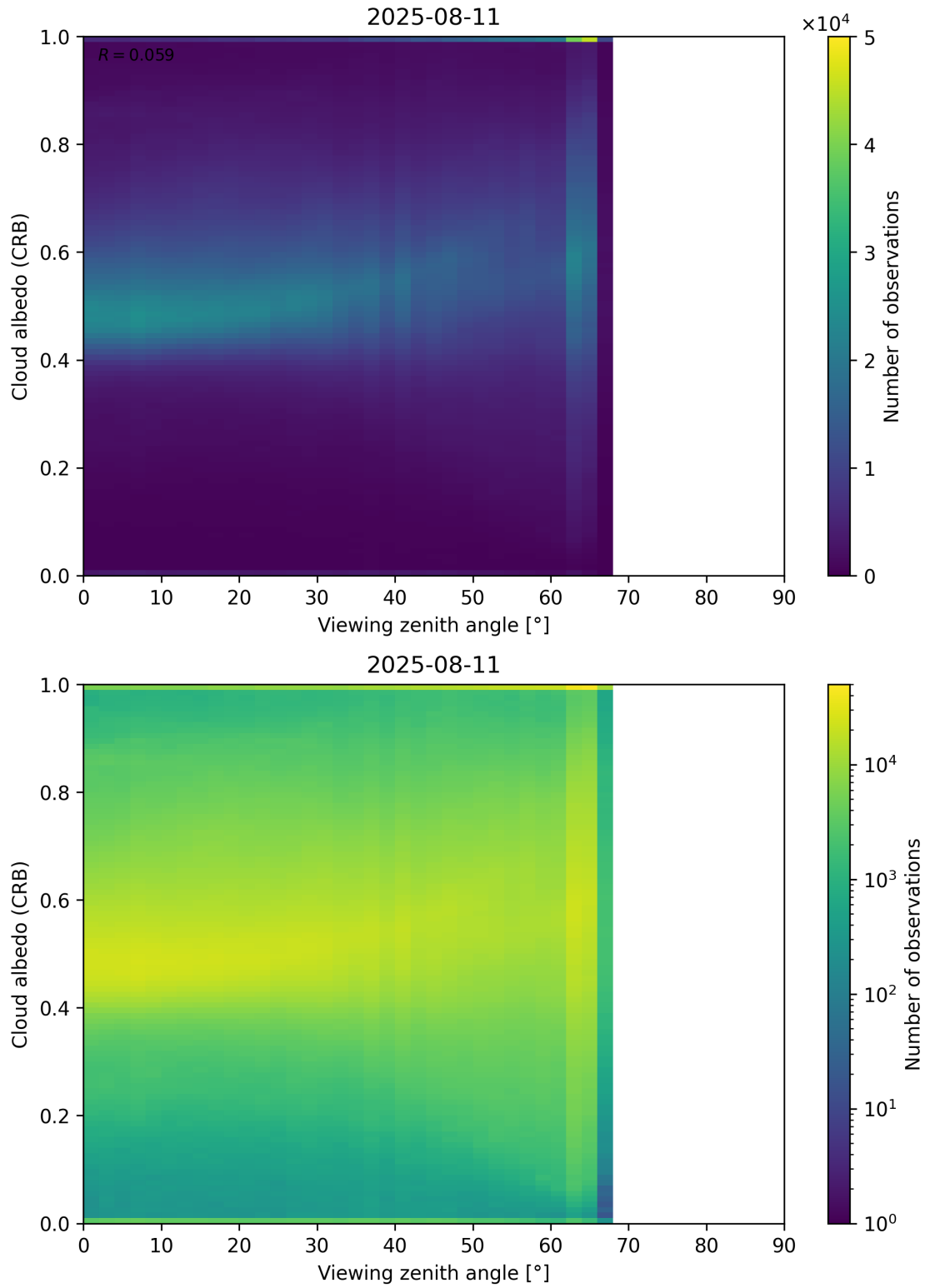
Figure 106: Scatter density plot of “Viewing zenith angle” against “Cloud albedo (CRB)” for 2025-08-10 to 2025-08-12.
