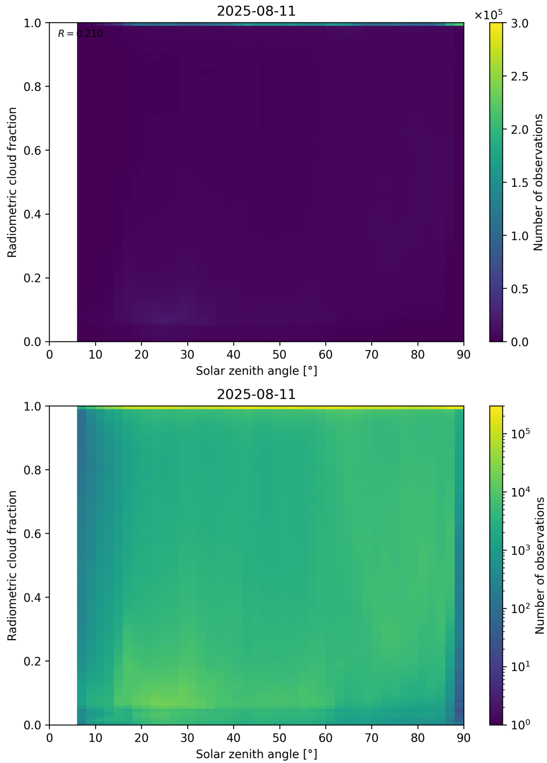
Figure 99: Scatter density plot of “Solar zenith angle” against “Radiometric cloud fraction” for 2025-08-10 to 2025-08-12.
