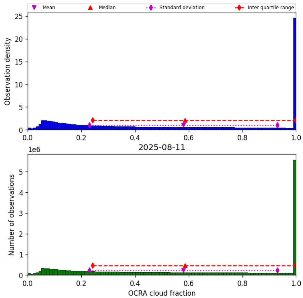
Figure 50: Histogram of “OCRA cloud fraction” for 2025-08-10 to 2025-08-12
