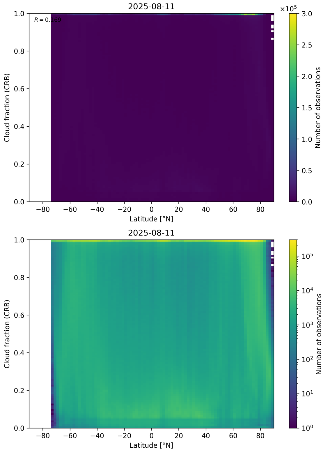
Figure 94: Scatter density plot of “Latitude” against “Cloud fraction (CRB)” for 2025-08-10 to 2025-08-12.
