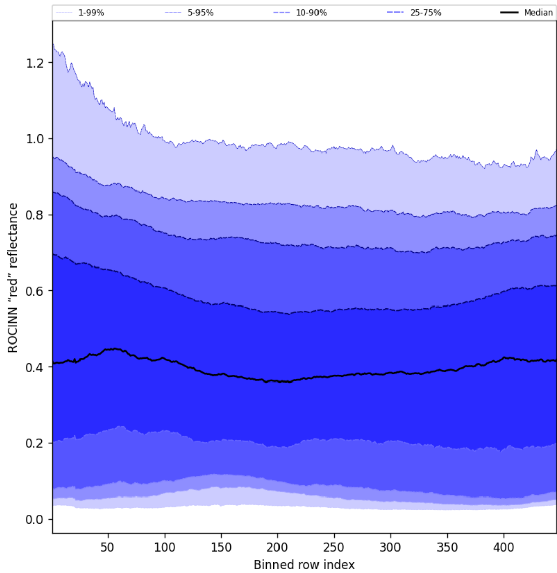
Figure 69: Along track statistics of “ROCINN “red” reflectance” for 2025-08-10 to 2025-08-12
