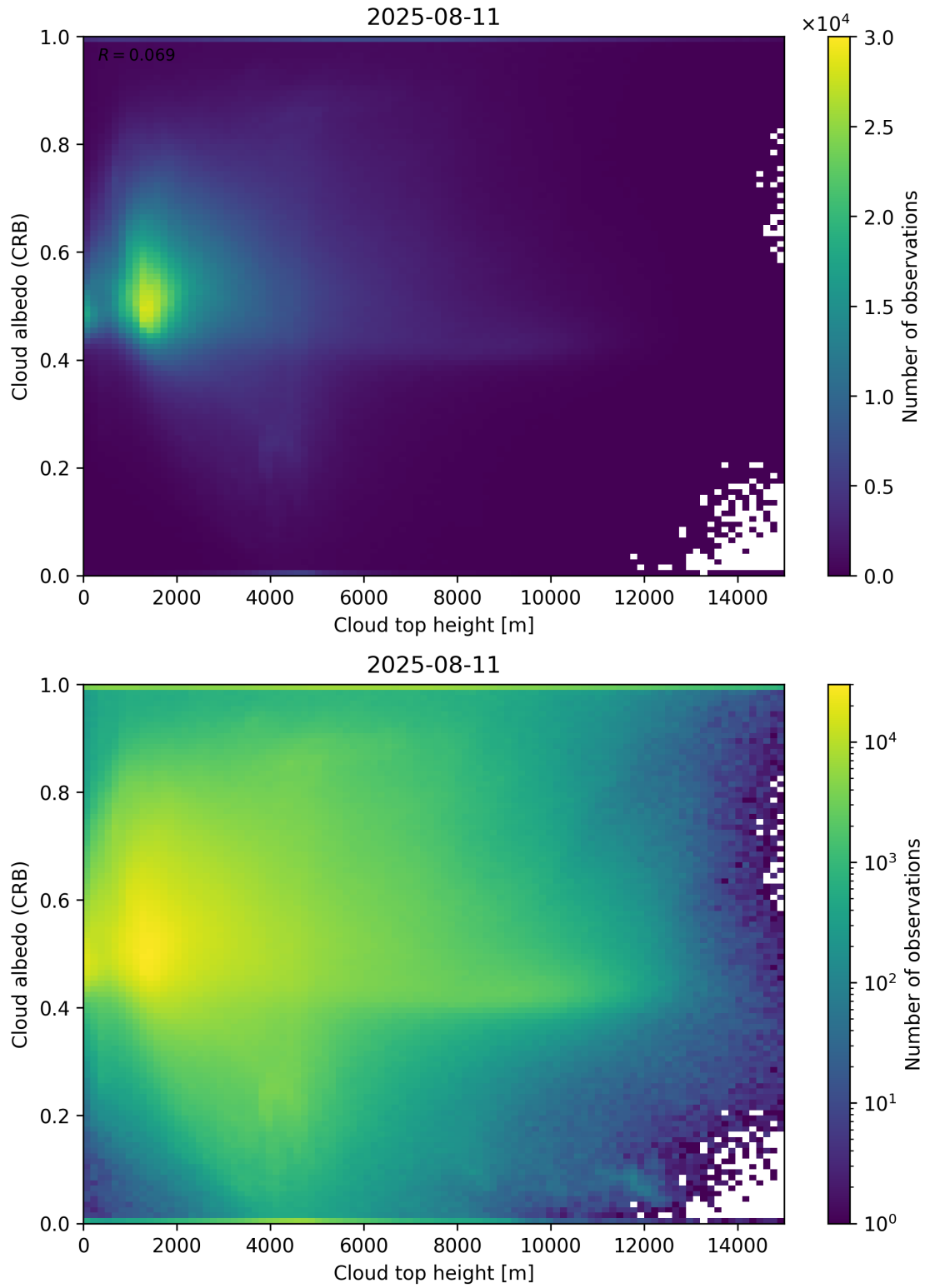
Figure 86: Scatter density plot of “Cloud top height” against “Cloud albedo (CRB)” for 2025-08-10 to 2025-08-12.
