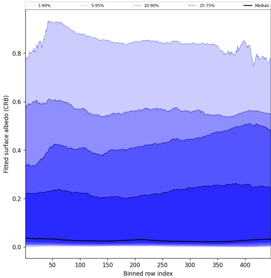
Figure 62: Along track statistics of “Fitted surface albedo (CRB)” for 2025-08-10 to 2025-08-12
