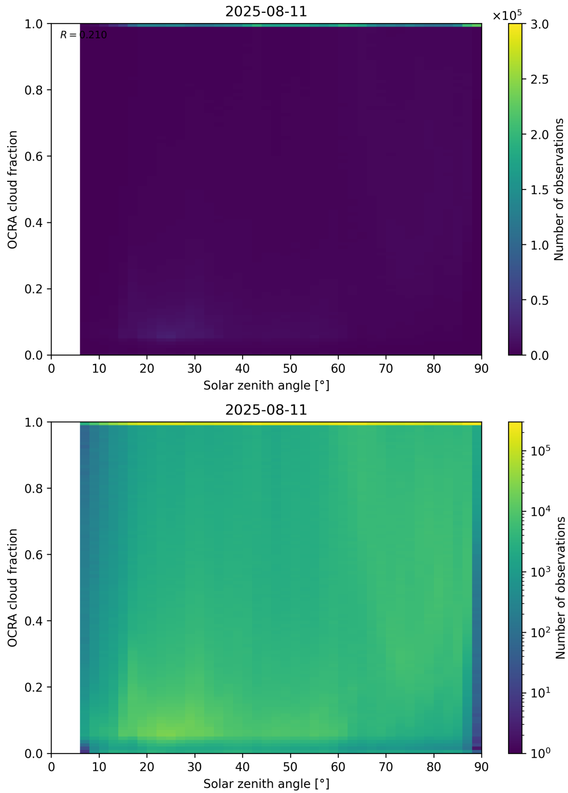
Figure 100: Scatter density plot of “Solar zenith angle” against “OCRA cloud fraction” for 2025-08-10 to 2025-08-12.
