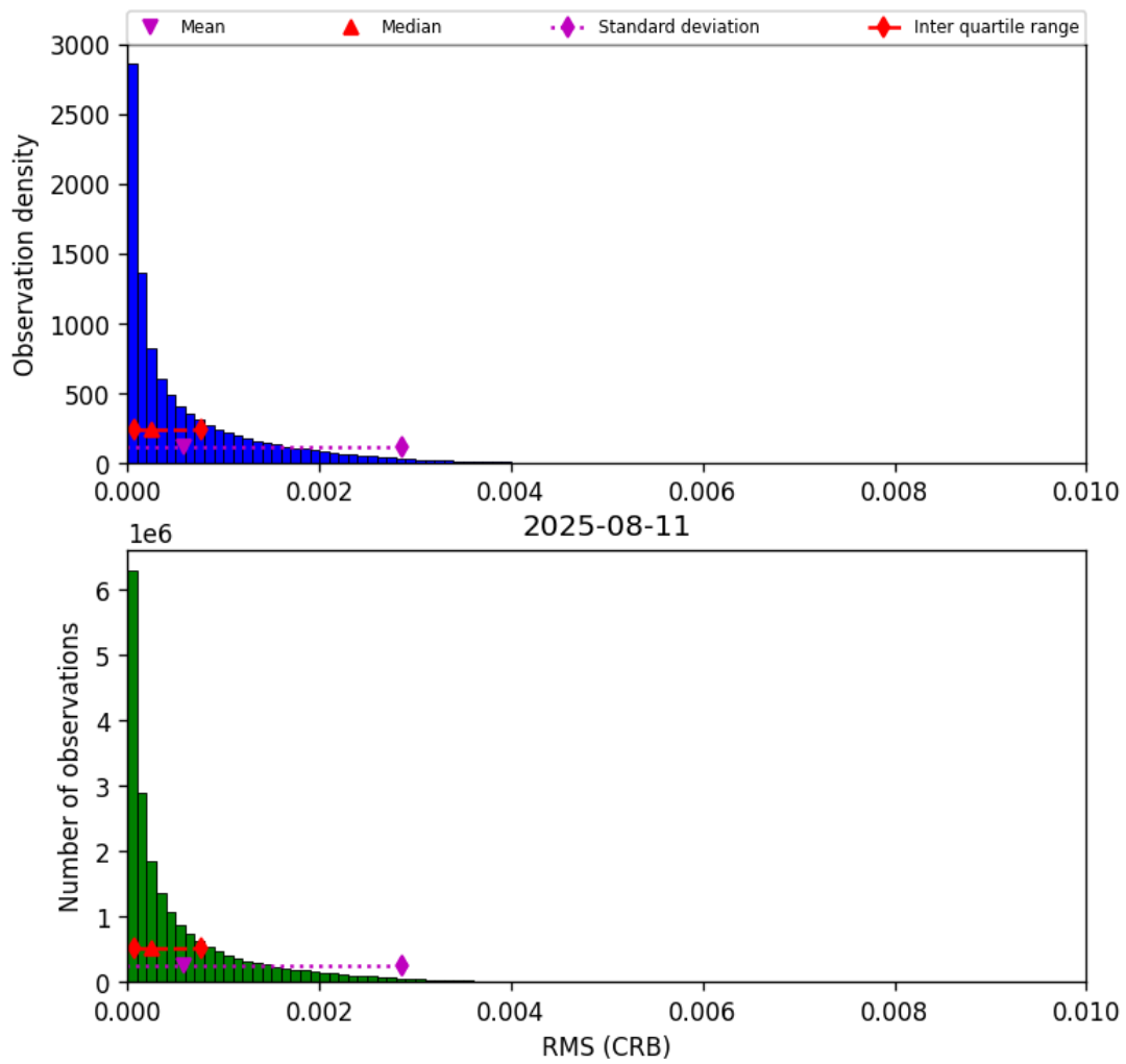
Figure 48: Histogram of “RMS (CRB)” for 2025-08-10 to 2025-08-12
