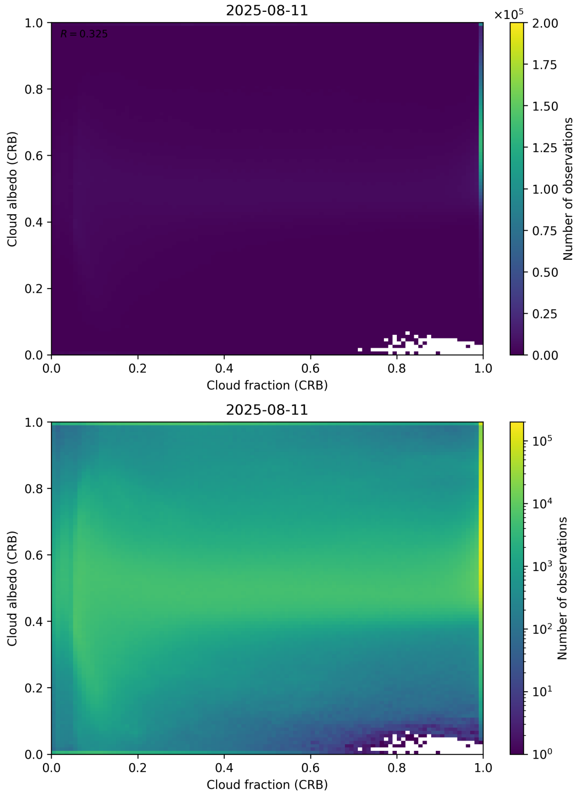
Figure 77: Scatter density plot of “Cloud fraction (CRB)” against “Cloud albedo (CRB)” for 2025-08-10 to 2025-08-12.
