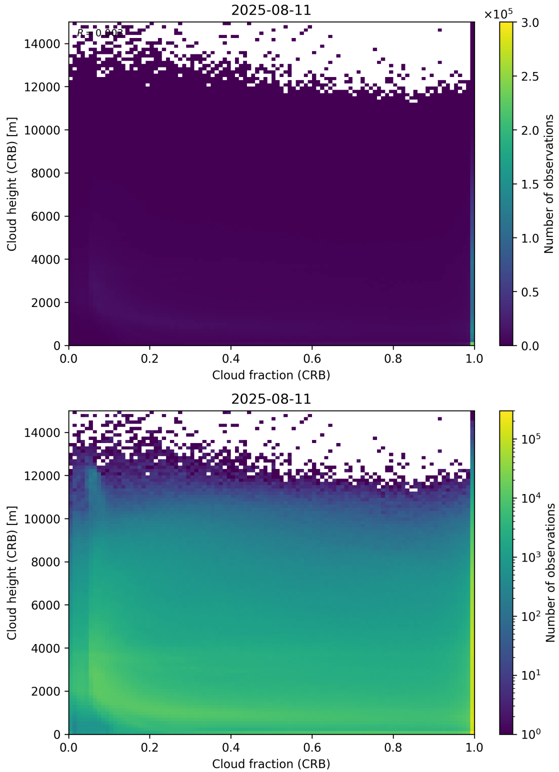
Figure 79: Scatter density plot of “Cloud fraction (CRB)” against “Cloud height (CRB)” for 2025-08-10 to 2025-08-12.
