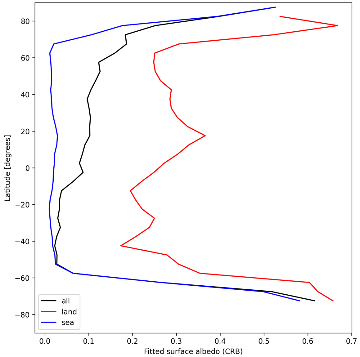
Figure 30: Zonal average of “Fitted surface albedo (CRB)” for 2025-08-10 to 2025-08-12.
