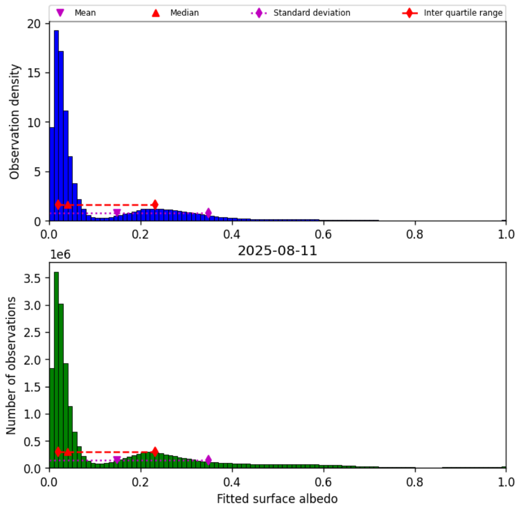
Figure 45: Histogram of “Fitted surface albedo” for 2025-08-10 to 2025-08-12
