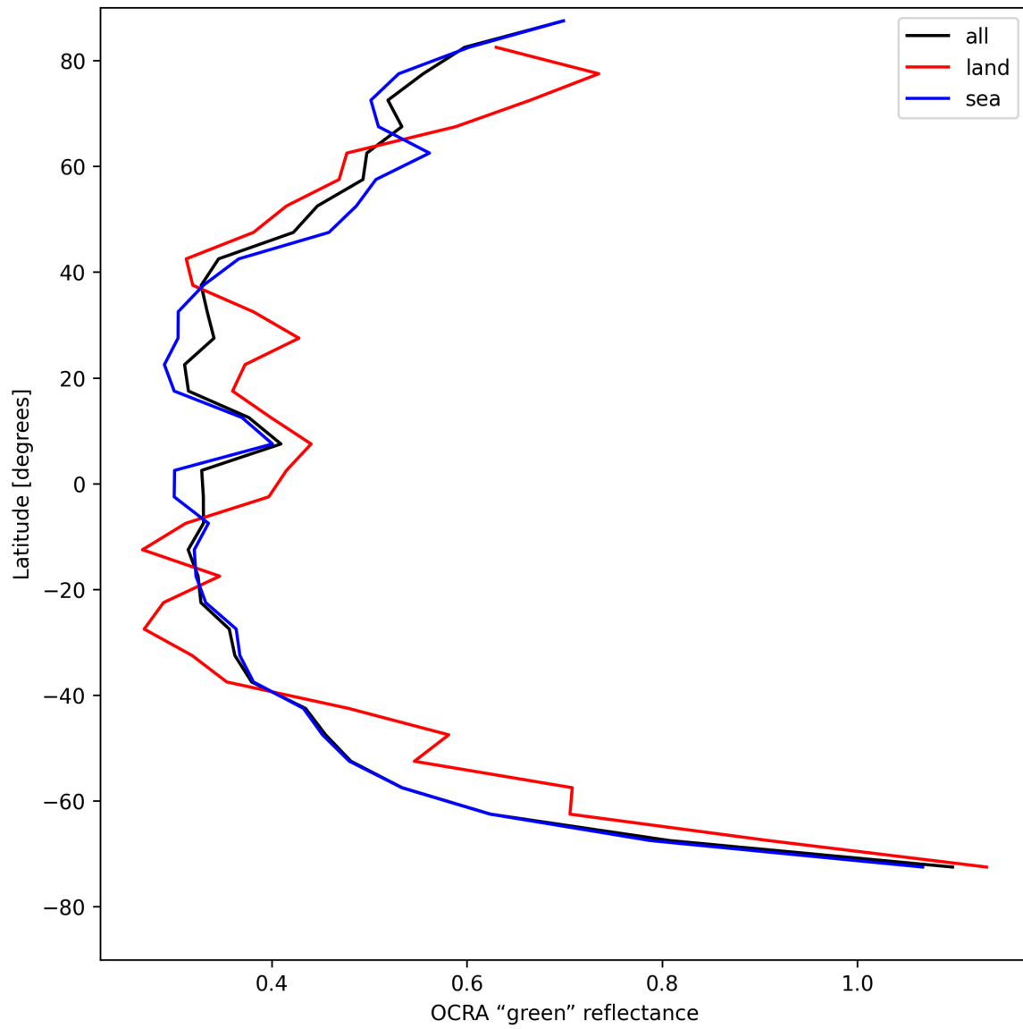
Figure 36: Zonal average of “OCRA “green” reflectance” for 2025-08-10 to 2025-08-12.
