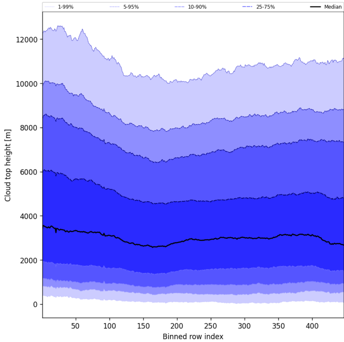
Figure 56: Along track statistics of “Cloud top height” for 2025-08-10 to 2025-08-12
