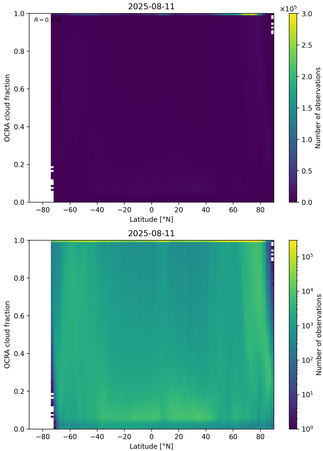
Figure 93: Scatter density plot of “Latitude” against “OCRA cloud fraction” for 2025-08-10 to 2025-08-12.
