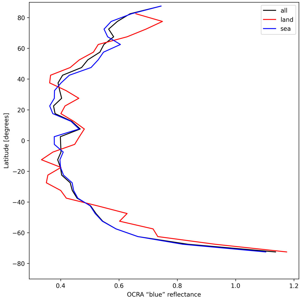
Figure 35: Zonal average of “OCRA “blue” reflectance” for 2025-08-10 to 2025-08-12.
