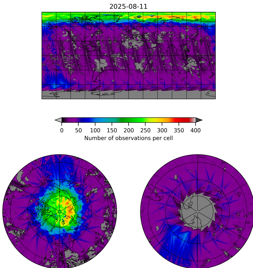
Figure 21: Map of the number of observations for 2025-08-10 to 2025-08-12
