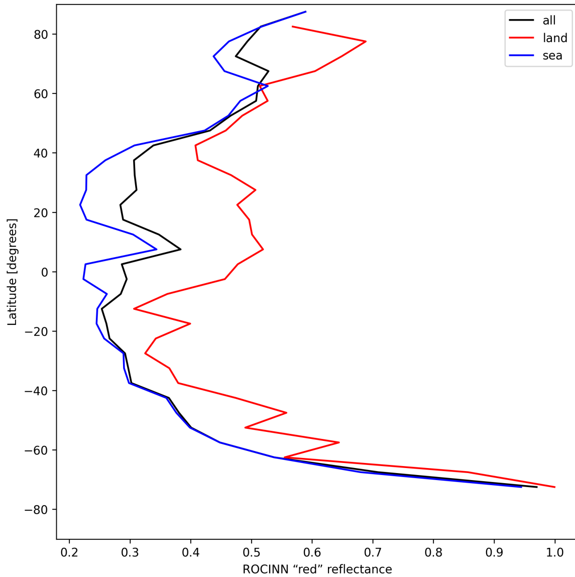
Figure 37: Zonal average of “ROCINN “red” reflectance” for 2025-08-10 to 2025-08-12.
