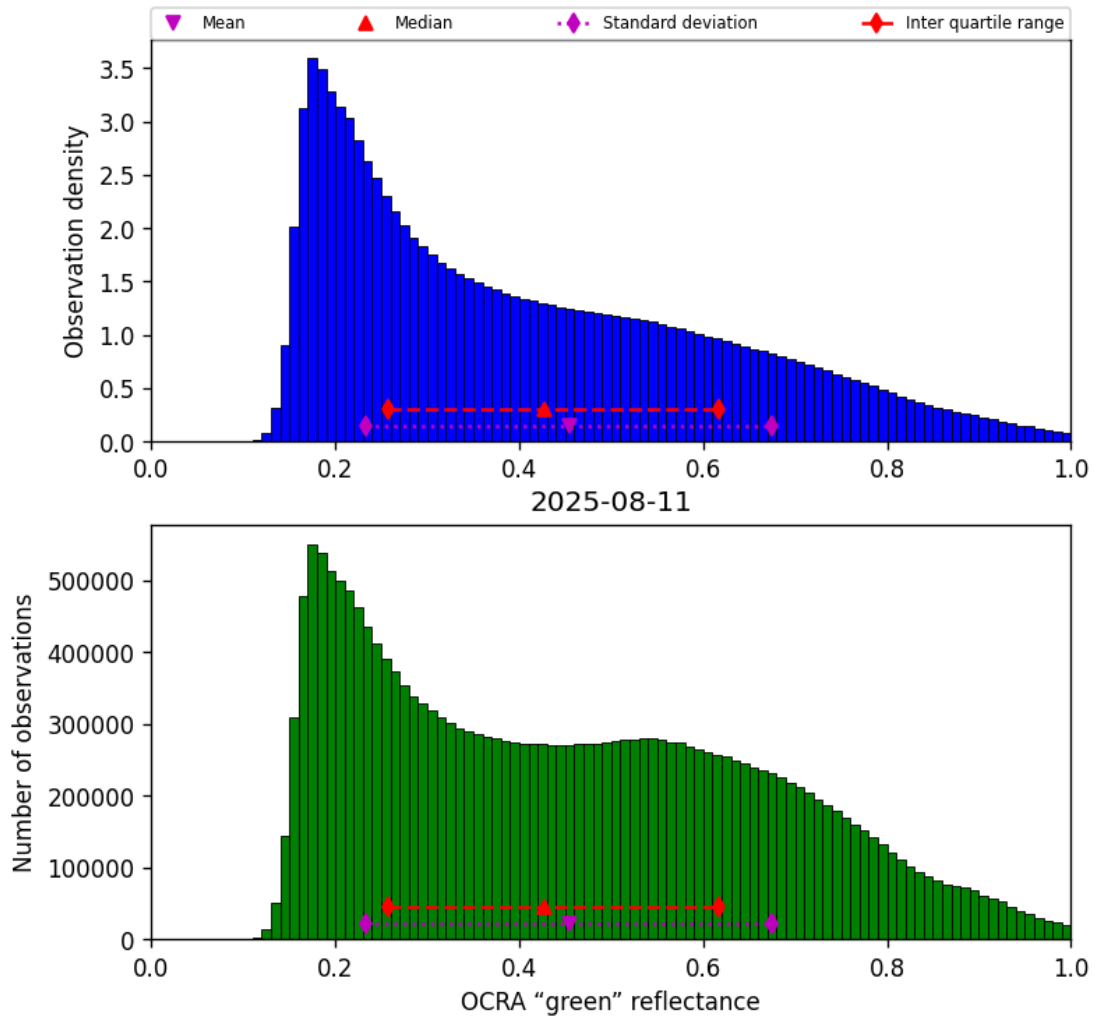
Figure 52: Histogram of “OCRA “green” reflectance” for 2025-08-10 to 2025-08-12
