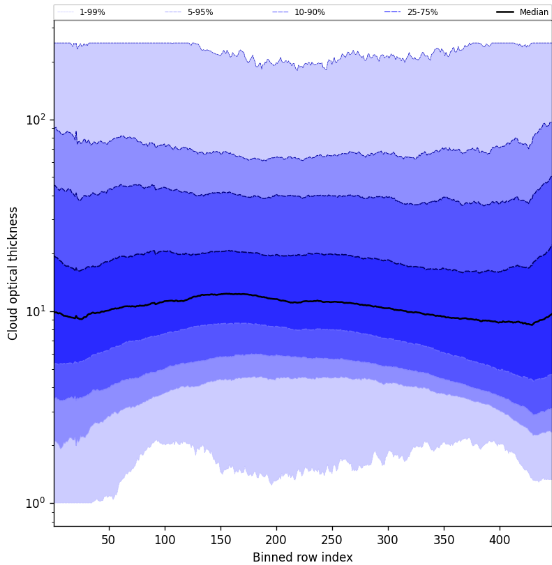
Figure 57: Along track statistics of “Cloud optical thickness” for 2025-08-10 to 2025-08-12
