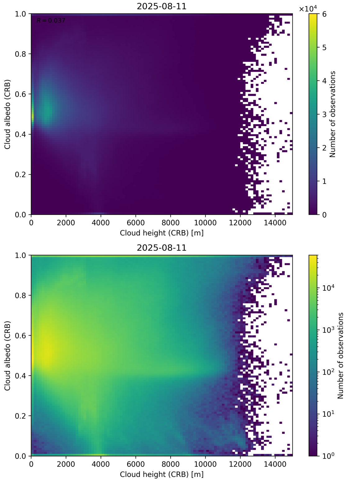
Figure 80: Scatter density plot of “Cloud height (CRB)” against “Cloud albedo (CRB)” for 2025-08-10 to 2025-08-12.
