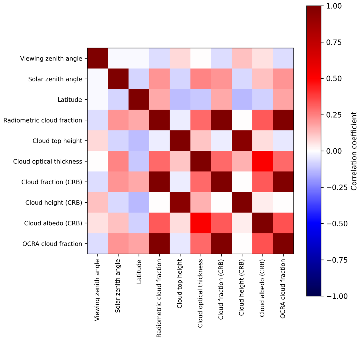
Figure 2: Map of correlation matrix for 2025-08-10 to 2025-08-12.
