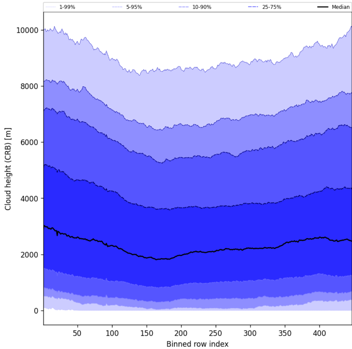
Figure 59: Along track statistics of “Cloud height (CRB)” for 2025-08-10 to 2025-08-12
