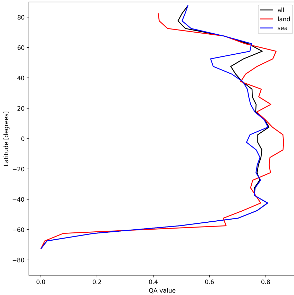
Figure 22: Zonal average of “QA value” for 2025-08-10 to 2025-08-12.
