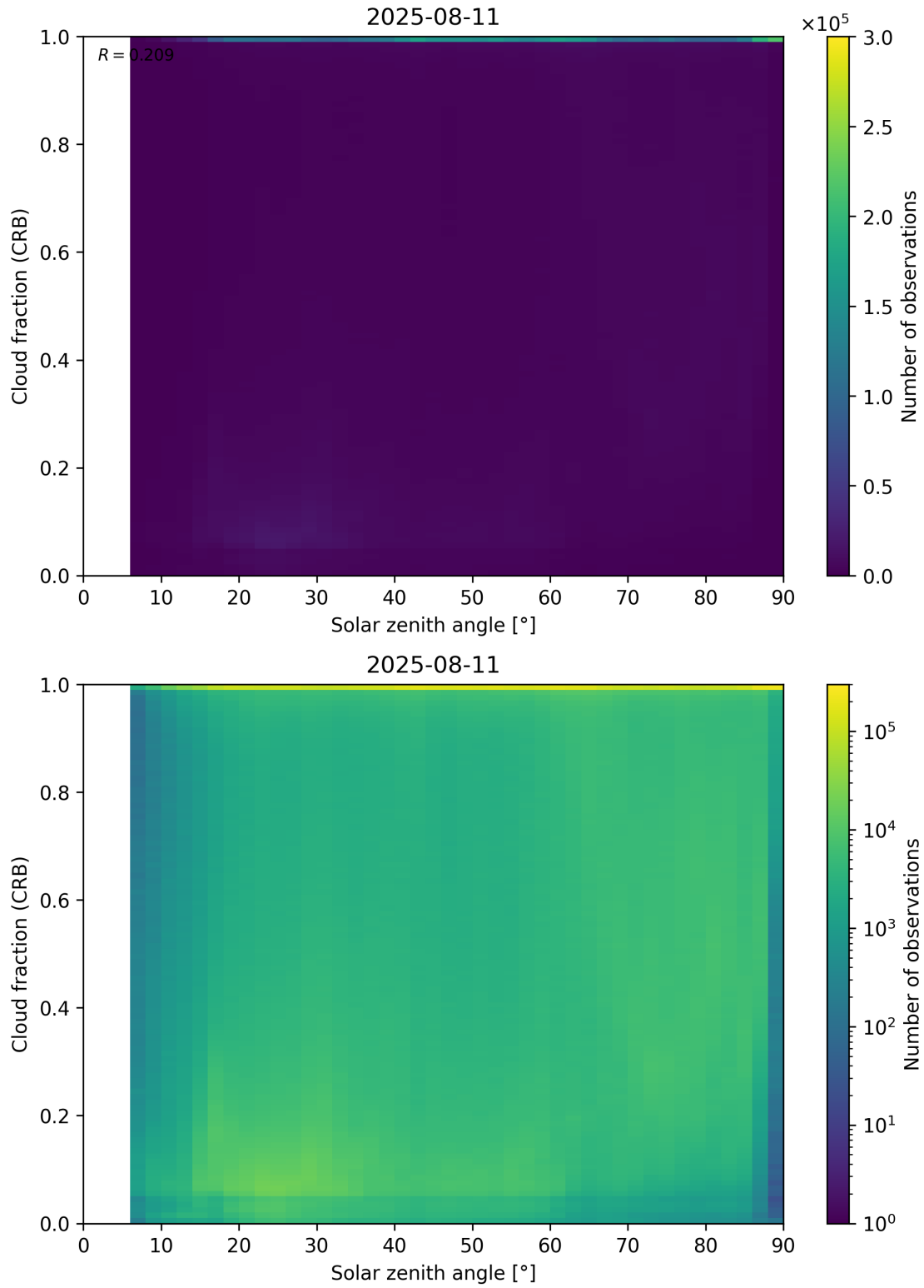
Figure 101: Scatter density plot of “Solar zenith angle” against “Cloud fraction (CRB)” for 2025-08-10 to 2025-08-12.
