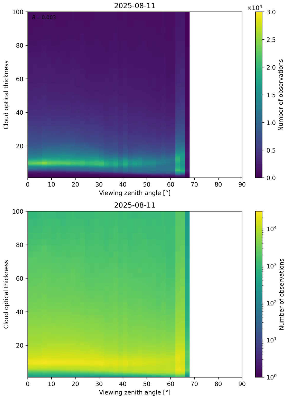
Figure 111: Scatter density plot of “Viewing zenith angle” against “Cloud optical thickness” for 2025-08-10 to 2025-08-12.
