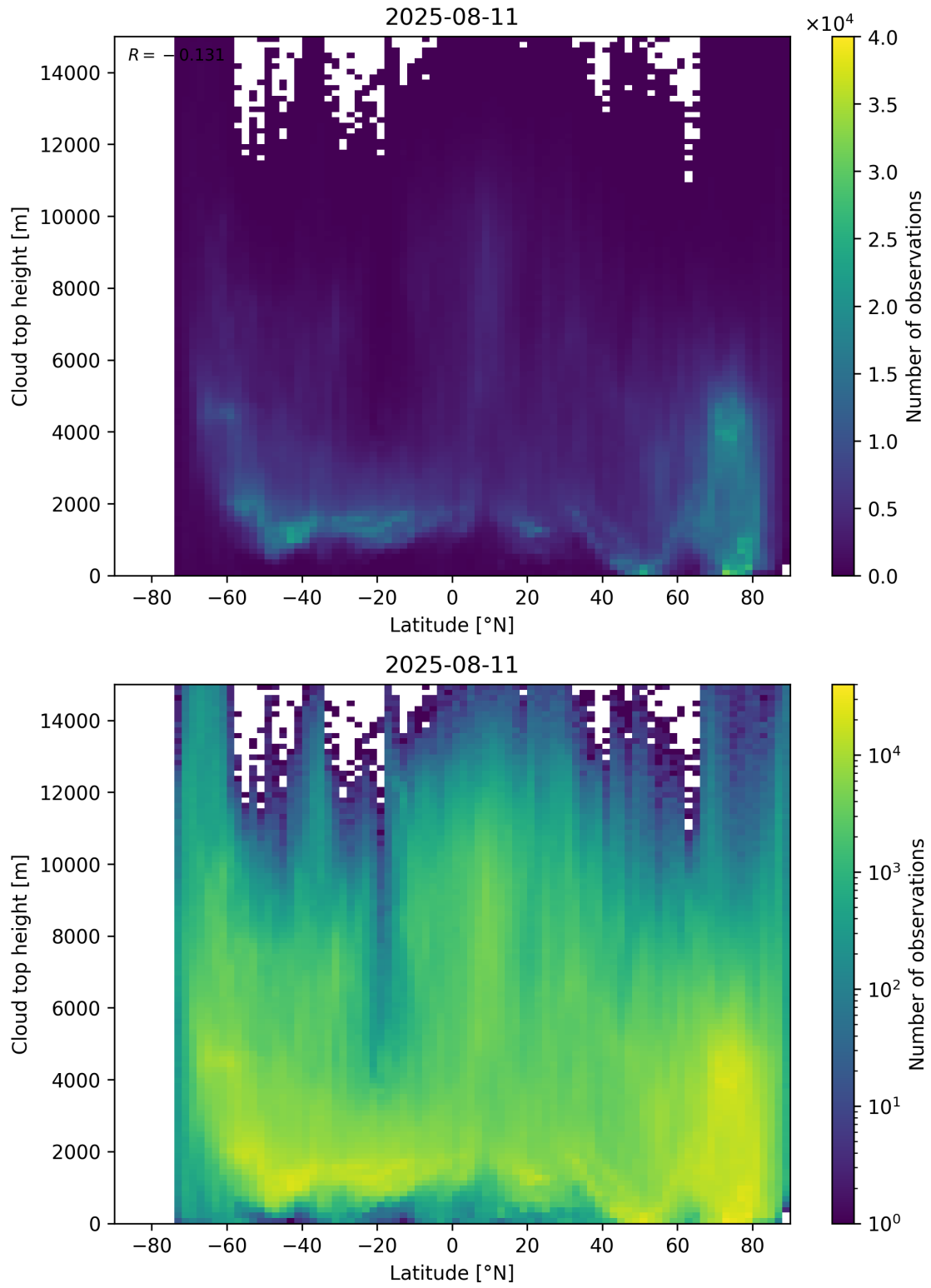
Figure 97: Scatter density plot of “Latitude” against “Cloud top height” for 2025-08-10 to 2025-08-12.
