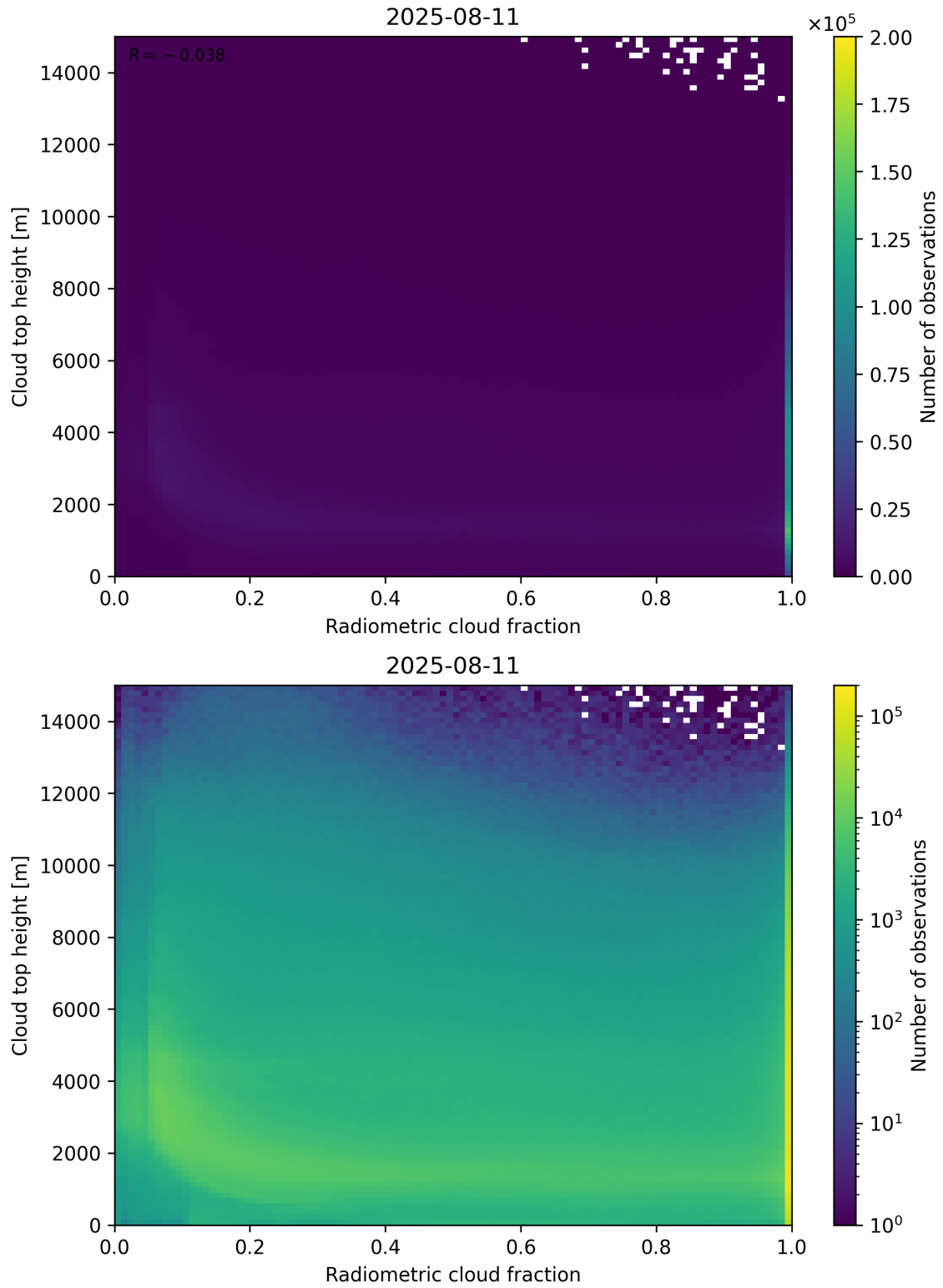
Figure 76: Scatter density plot of “Radiometric cloud fraction” against “Cloud top height” for 2025-08-10 to 2025-08-12.
