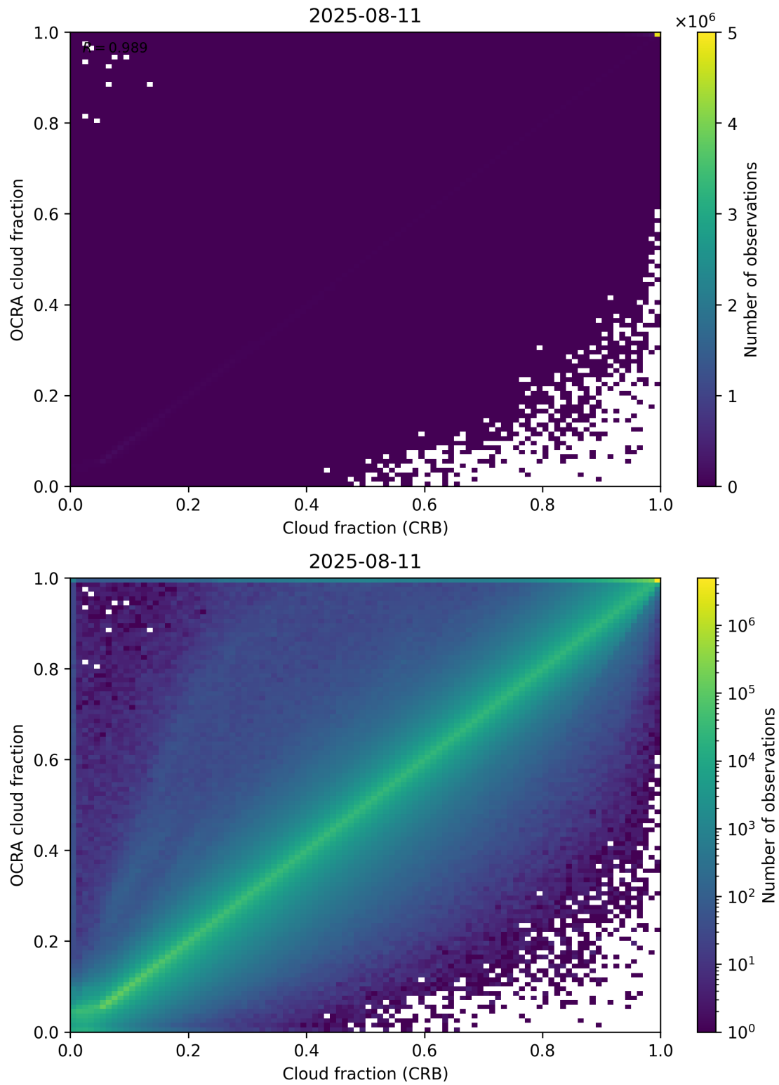
Figure 78: Scatter density plot of “Cloud fraction (CRB)” against “OCRA cloud fraction” for 2025-08-10 to 2025-08-12.
