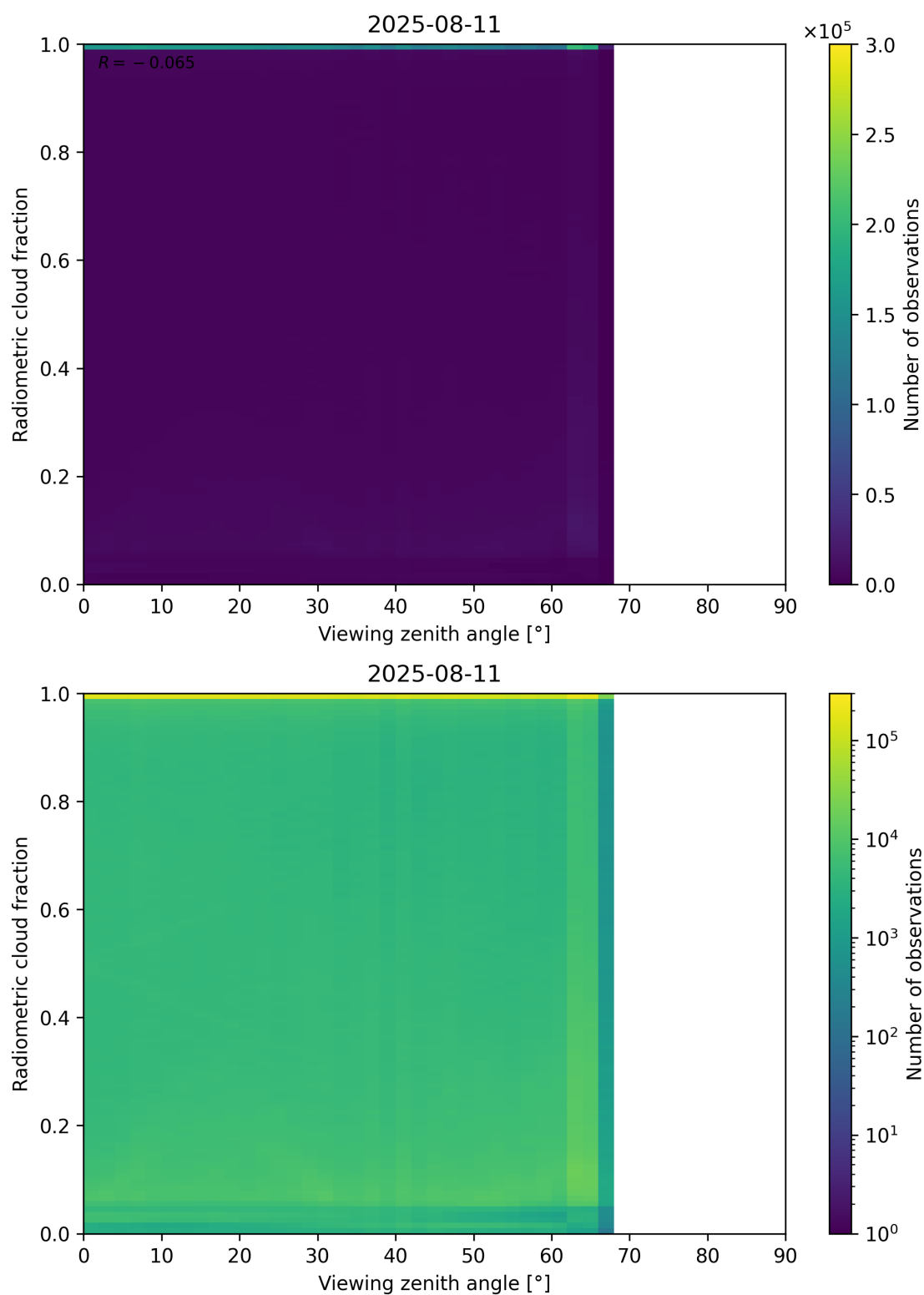
Figure 107: Scatter density plot of “Viewing zenith angle” against “Radiometric cloud fraction” for 2025-08-10 to 2025-08-12.
