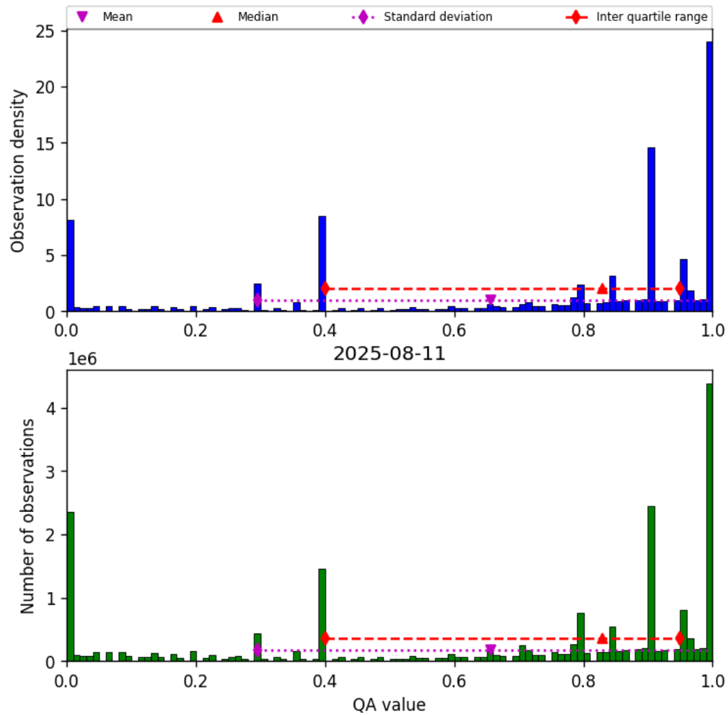
Figure 38: Histogram of “QA value” for 2025-08-10 to 2025-08-12
