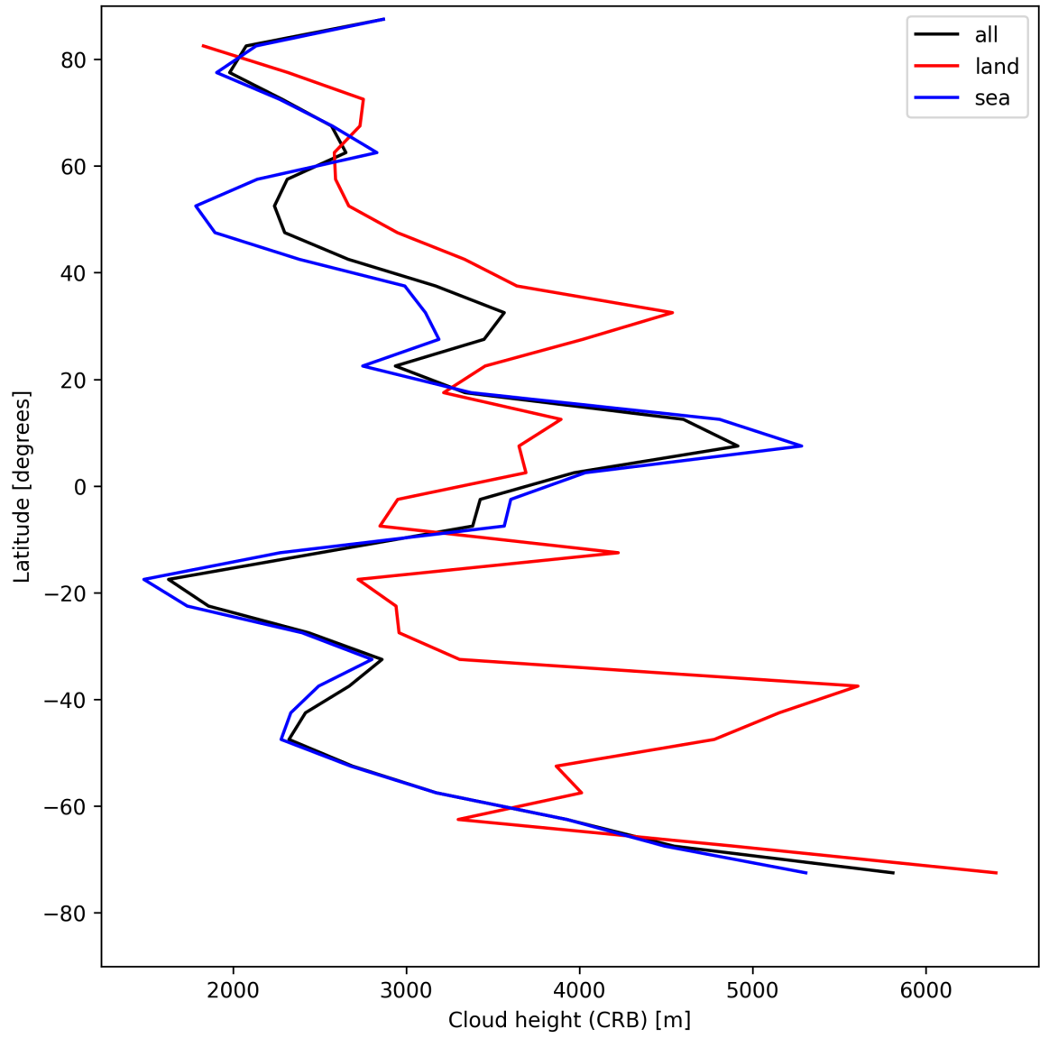
Figure 27: Zonal average of “Cloud height (CRB)” for 2025-08-10 to 2025-08-12.
