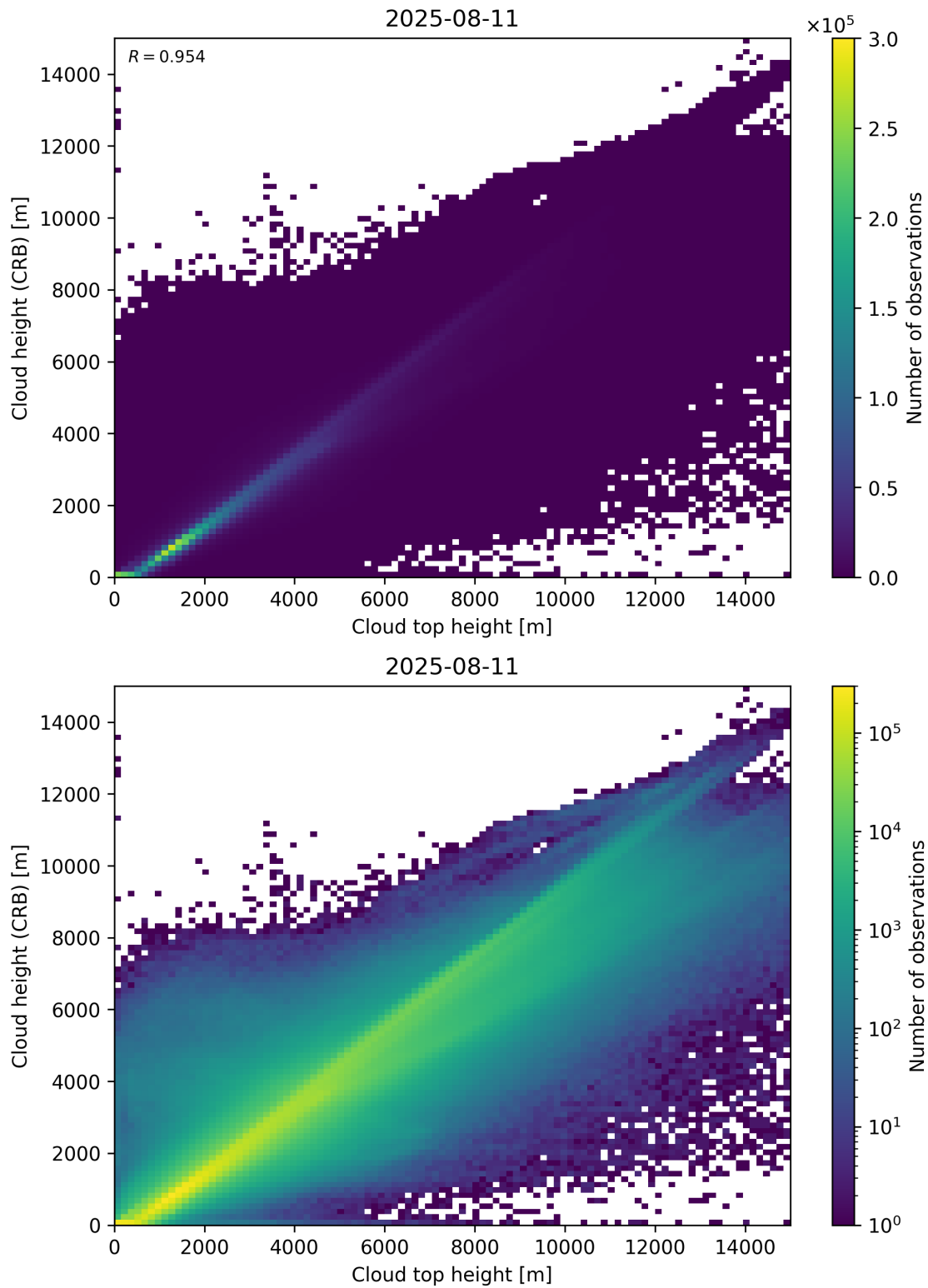
Figure 89: Scatter density plot of “Cloud top height” against “Cloud height (CRB)” for 2025-08-10 to 2025-08-12.
