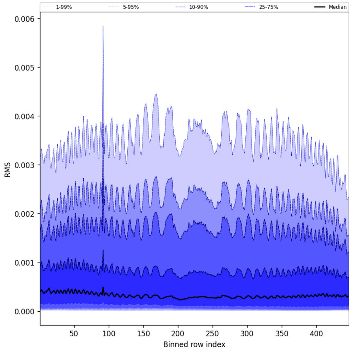
Figure 63: Along track statistics of “RMS” for 2025-08-10 to 2025-08-12
