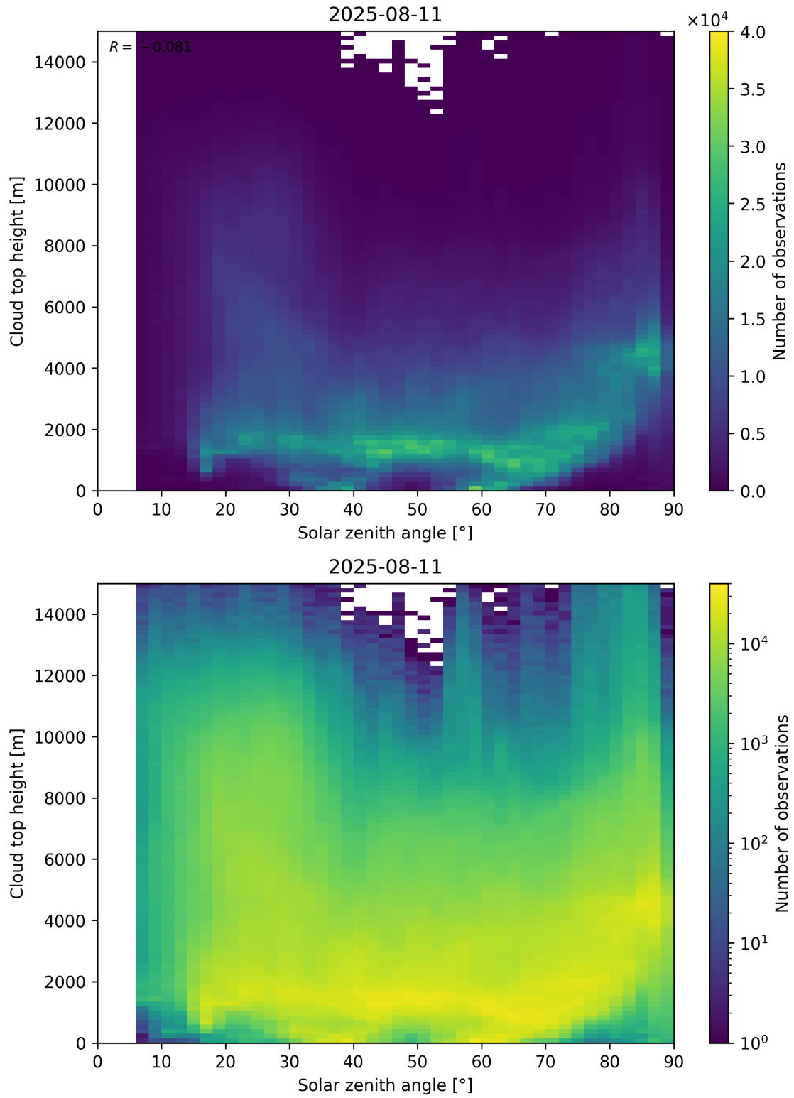
Figure 104: Scatter density plot of “Solar zenith angle” against “Cloud top height” for 2025-08-10 to 2025-08-12.
