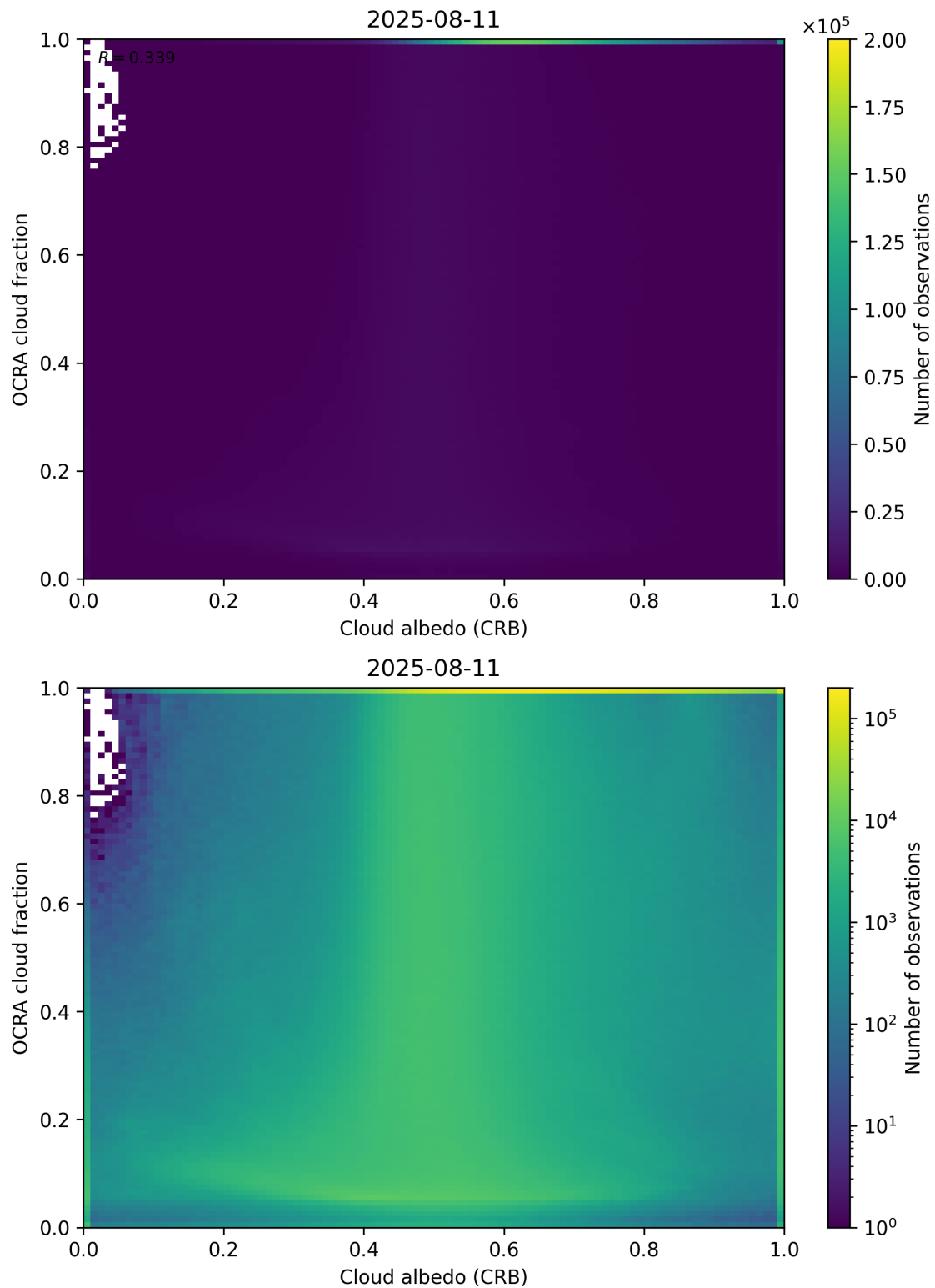
Figure 70: Scatter density plot of “Cloud albedo (CRB)” against “OCRA cloud fraction” for 2025-08-10 to 2025-08-12.
