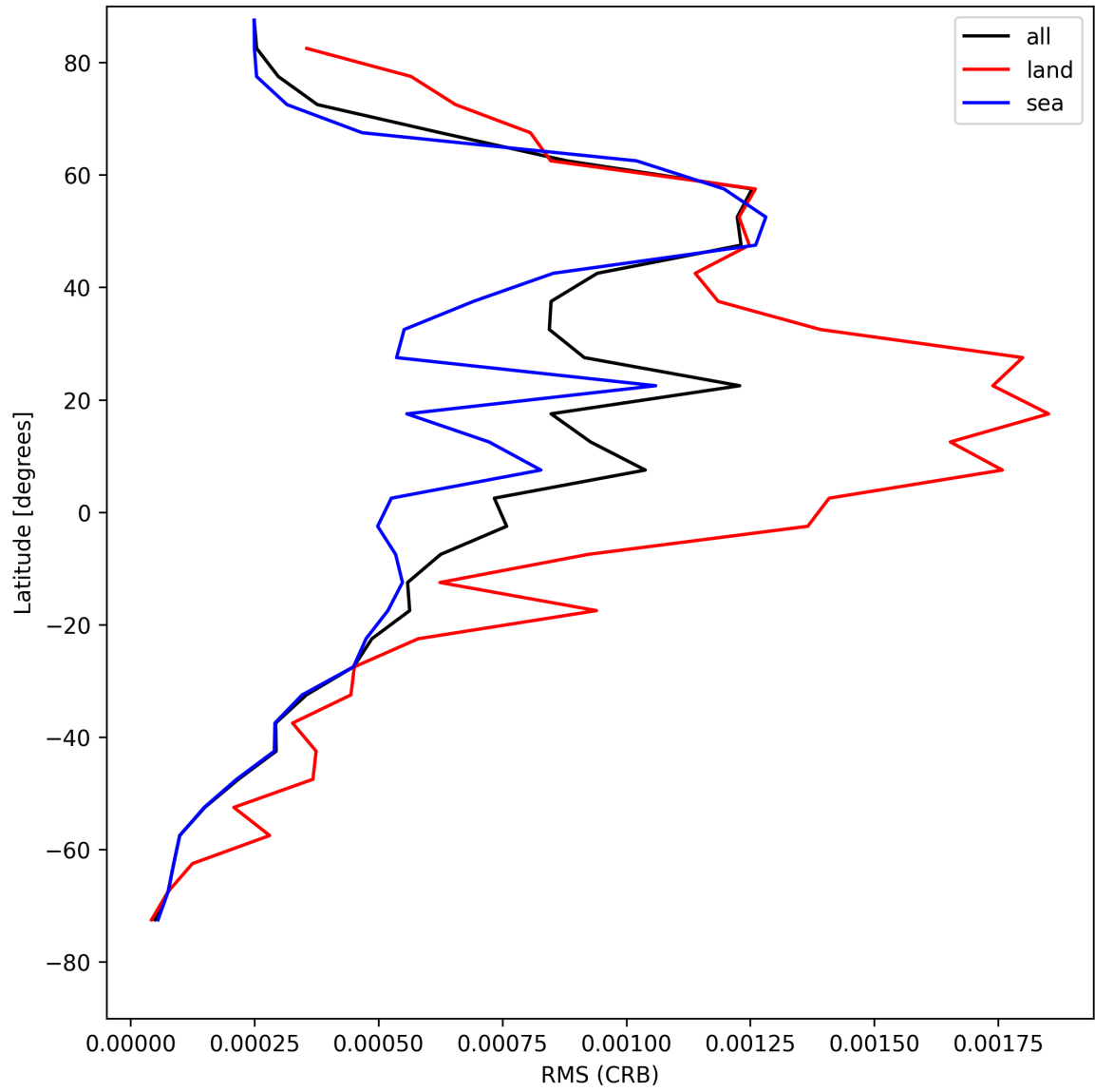
Figure 32: Zonal average of “RMS (CRB)” for 2025-08-10 to 2025-08-12.
