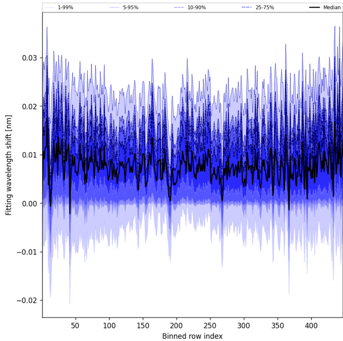
Figure 65: Along track statistics of “Fitting wavelength shift” for 2025-08-10 to 2025-08-12
