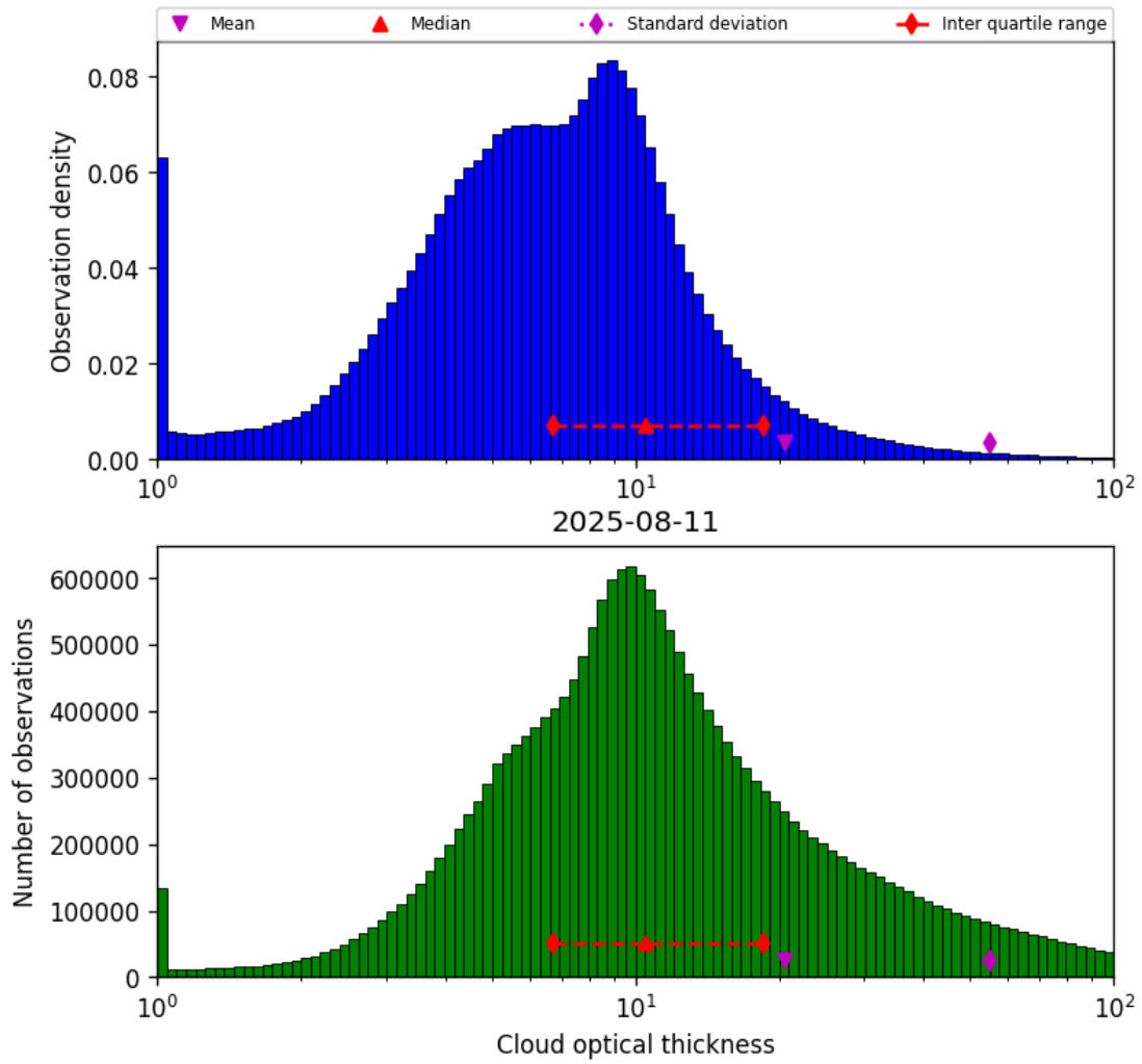
Figure 41: Histogram of “Cloud optical thickness” for 2025-08-10 to 2025-08-12
