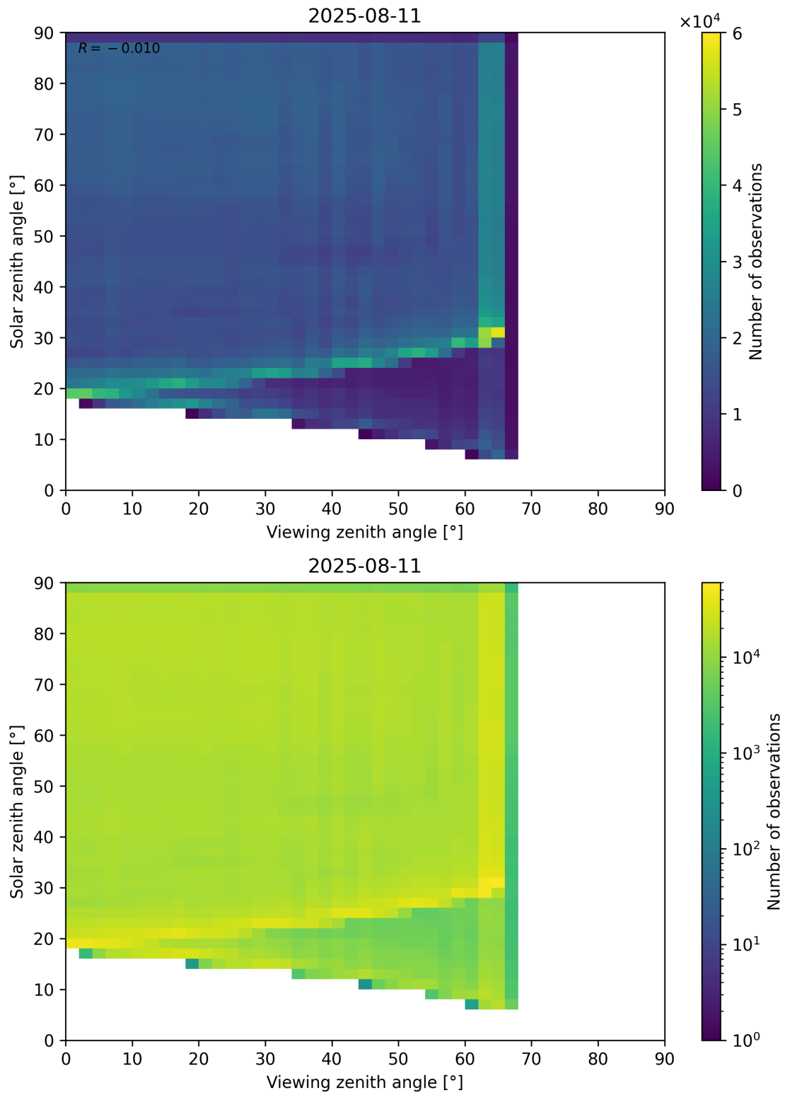
Figure 114: Scatter density plot of “Viewing zenith angle” against “Solar zenith angle” for 2025-08-10 to 2025-08-12.
