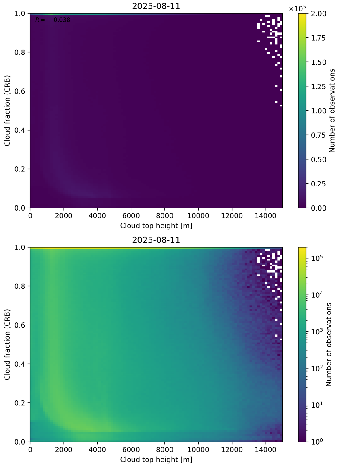
Figure 88: Scatter density plot of “Cloud top height” against “Cloud fraction (CRB)” for 2025-08-10 to 2025-08-12.
