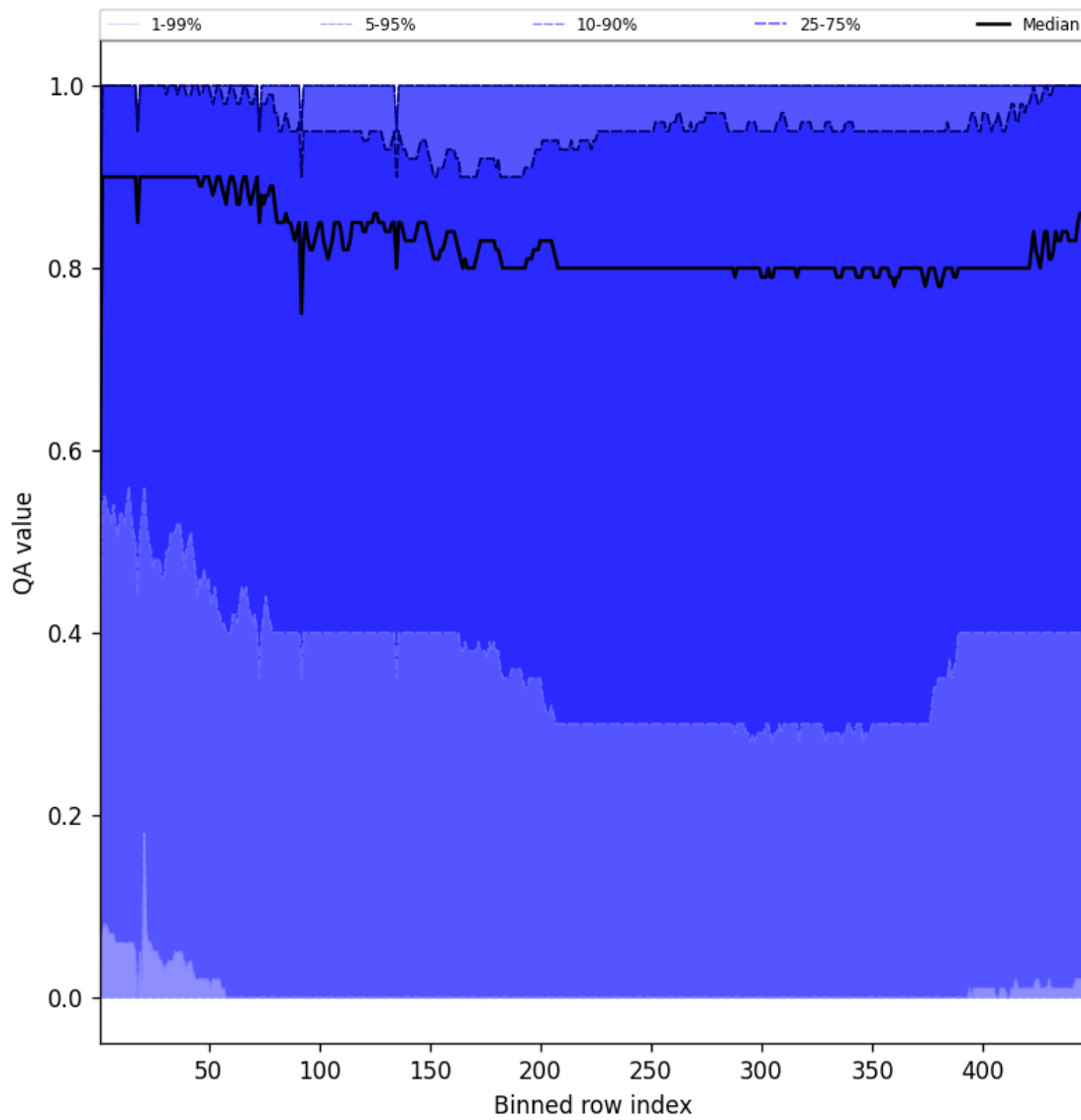
Figure 54: Along track statistics of “QA value” for 2025-08-10 to 2025-08-12
