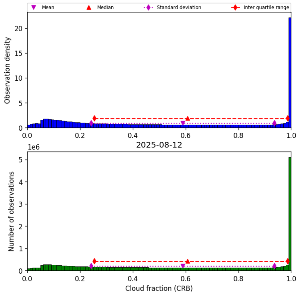
Figure 42: Histogram of “Cloud fraction (CRB)” for 2025-08-11 to 2025-08-13
