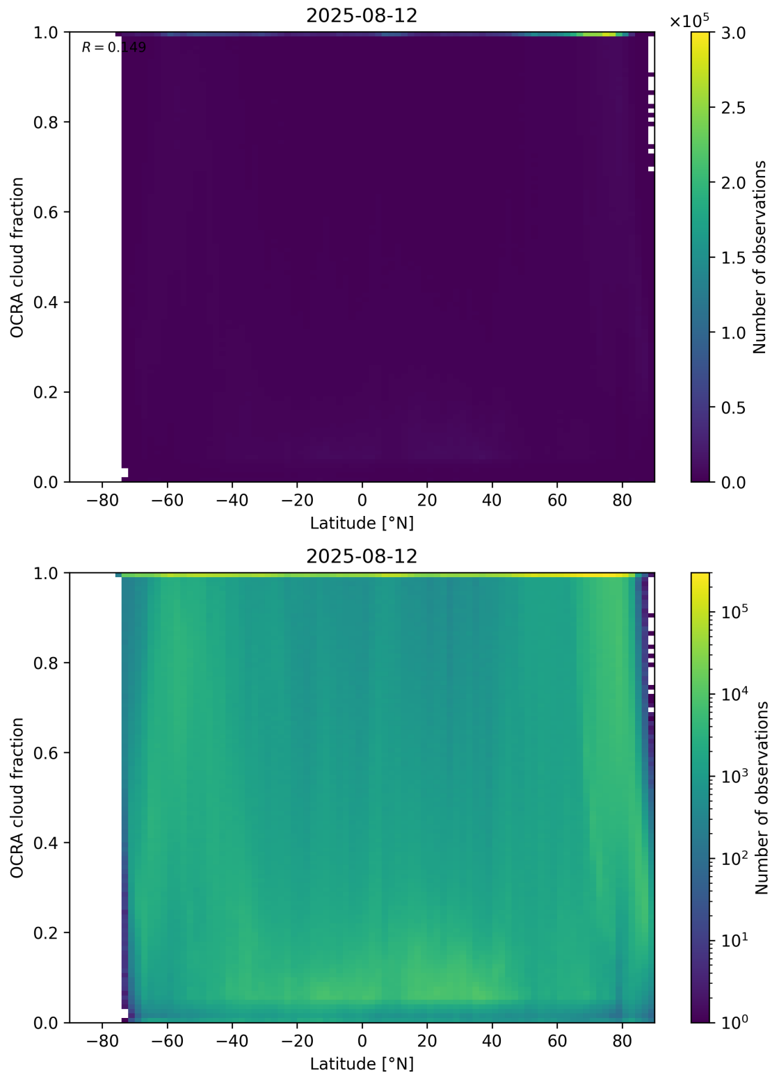
Figure 93: Scatter density plot of “Latitude” against “OCRA cloud fraction” for 2025-08-11 to 2025-08-13.
