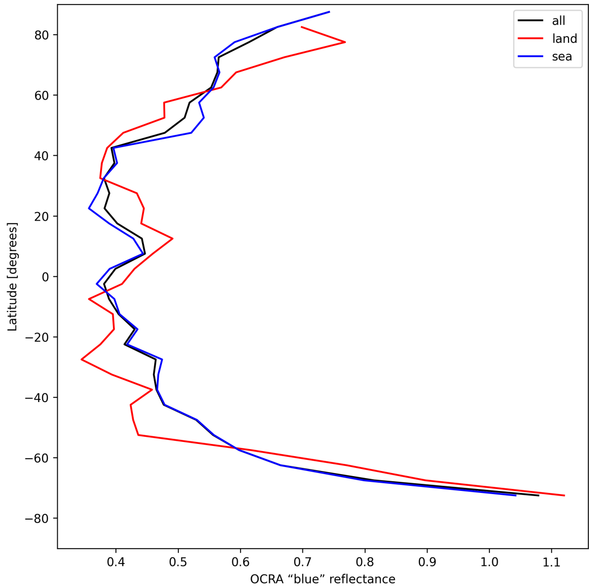
Figure 35: Zonal average of “OCRA “blue” reflectance” for 2025-08-12 to 2025-08-14.
