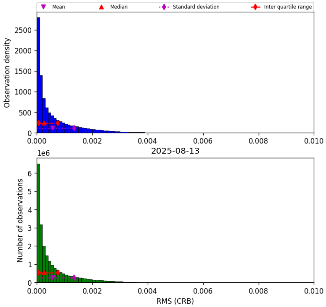
Figure 48: Histogram of “RMS (CRB)” for 2025-08-12 to 2025-08-14
