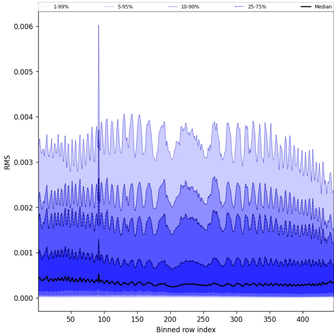
Figure 63: Along track statistics of “RMS” for 2025-08-12 to 2025-08-14
