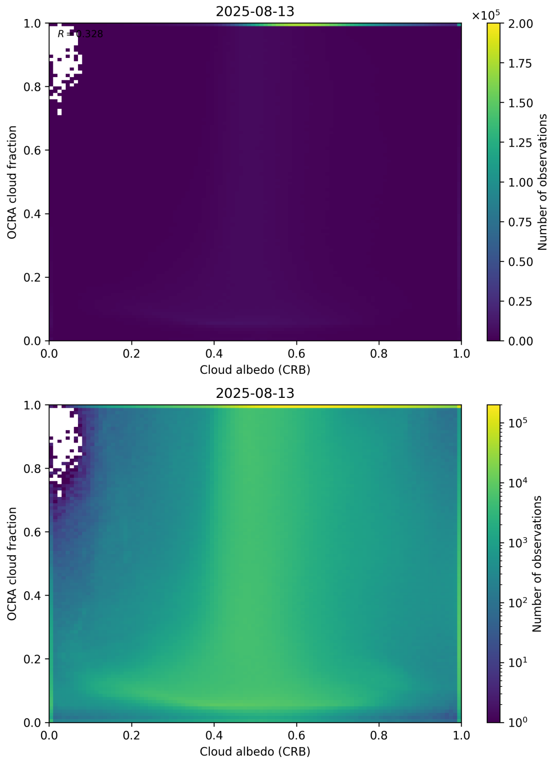
Figure 70: Scatter density plot of “Cloud albedo (CRB)” against “OCRA cloud fraction” for 2025-08-12 to 2025-08-14.
