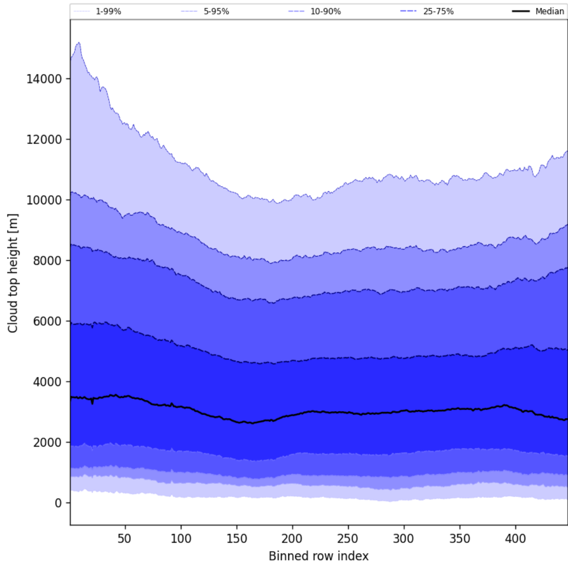
Figure 56: Along track statistics of “Cloud top height” for 2025-08-12 to 2025-08-14
