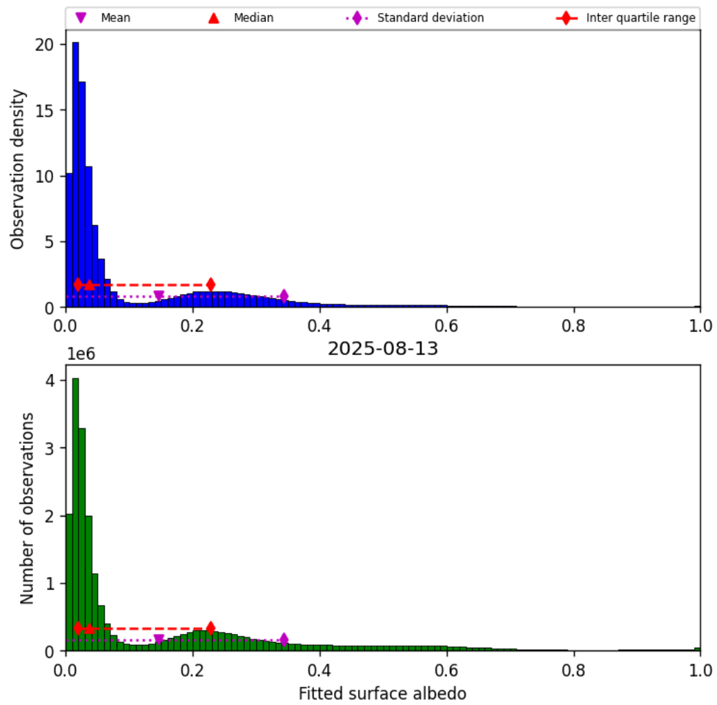
Figure 45: Histogram of “Fitted surface albedo” for 2025-08-12 to 2025-08-14
