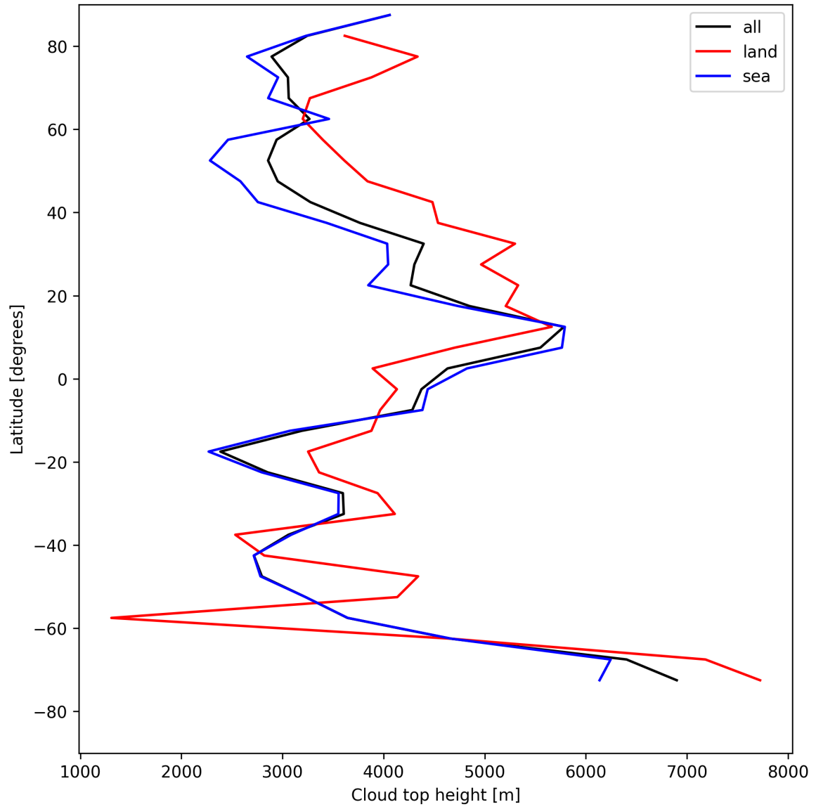
Figure 24: Zonal average of “Cloud top height” for 2025-08-12 to 2025-08-14.
