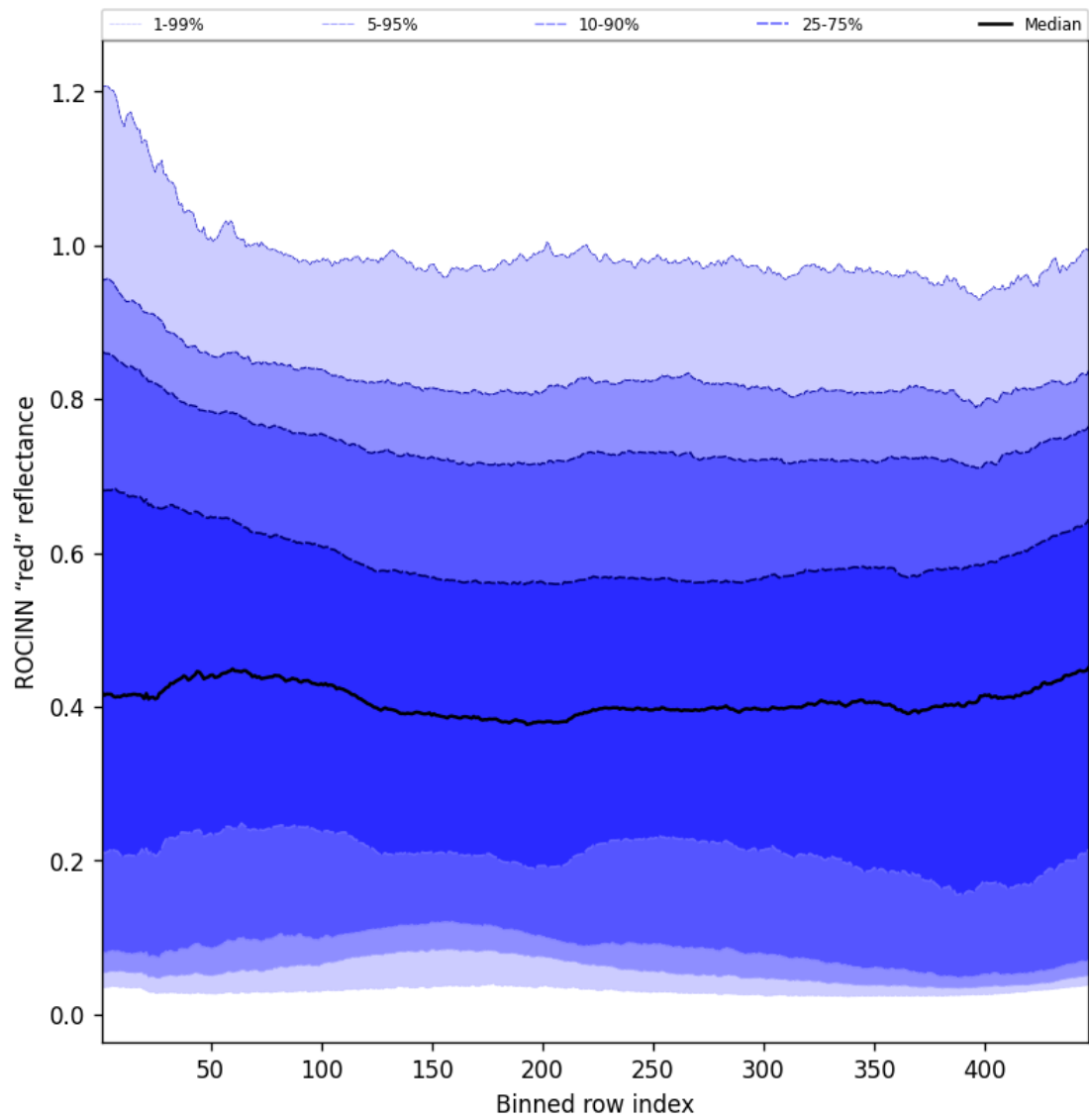
Figure 69: Along track statistics of "ROCINN "red" reflectance" for 2025-08-12 to 2025-08-14
