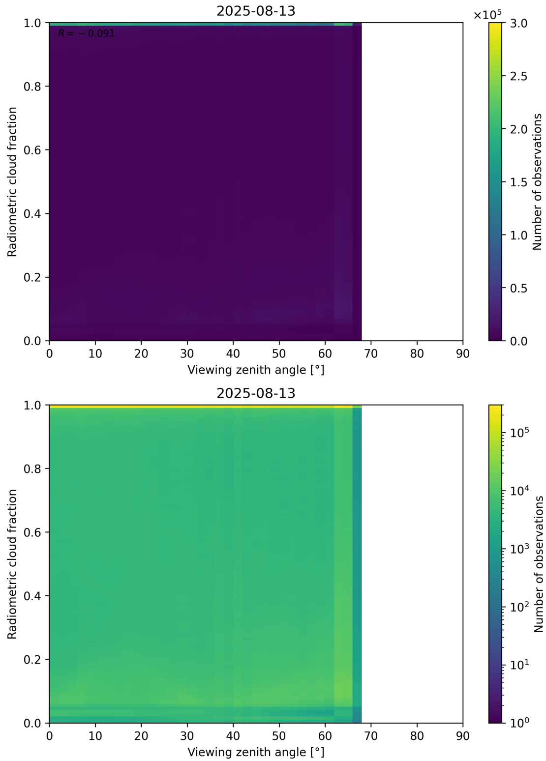
Figure 107: Scatter density plot of “Viewing zenith angle” against “Radiometric cloud fraction” for 2025-08-12 to 2025-08-14.
