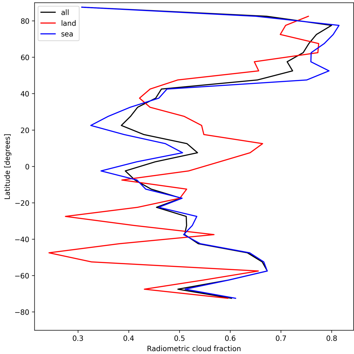
Figure 23: Zonal average of “Radiometric cloud fraction” for 2025-08-12 to 2025-08-14.
