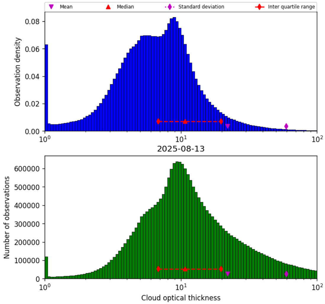
Figure 41: Histogram of “Cloud optical thickness” for 2025-08-12 to 2025-08-14
