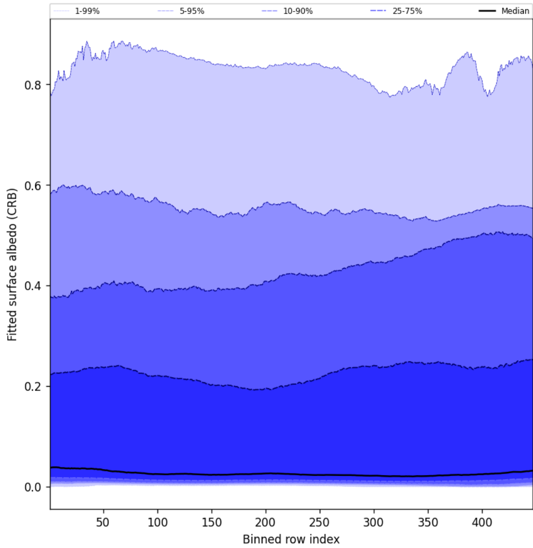
Figure 62: Along track statistics of “Fitted surface albedo (CRB)” for 2025-08-12 to 2025-08-14
