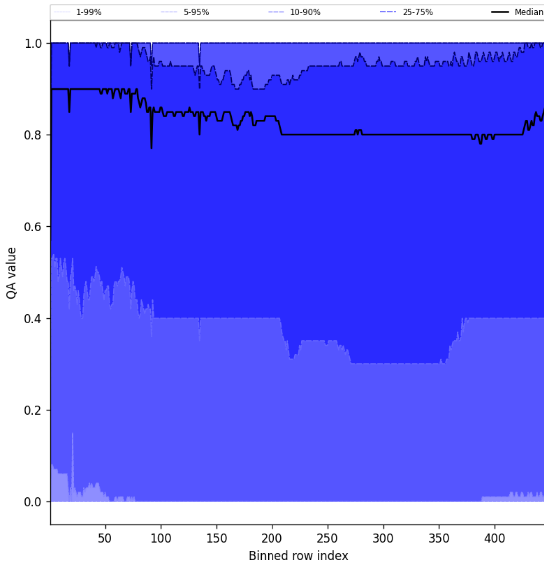
Figure 54: Along track statistics of “QA value” for 2025-08-12 to 2025-08-14
