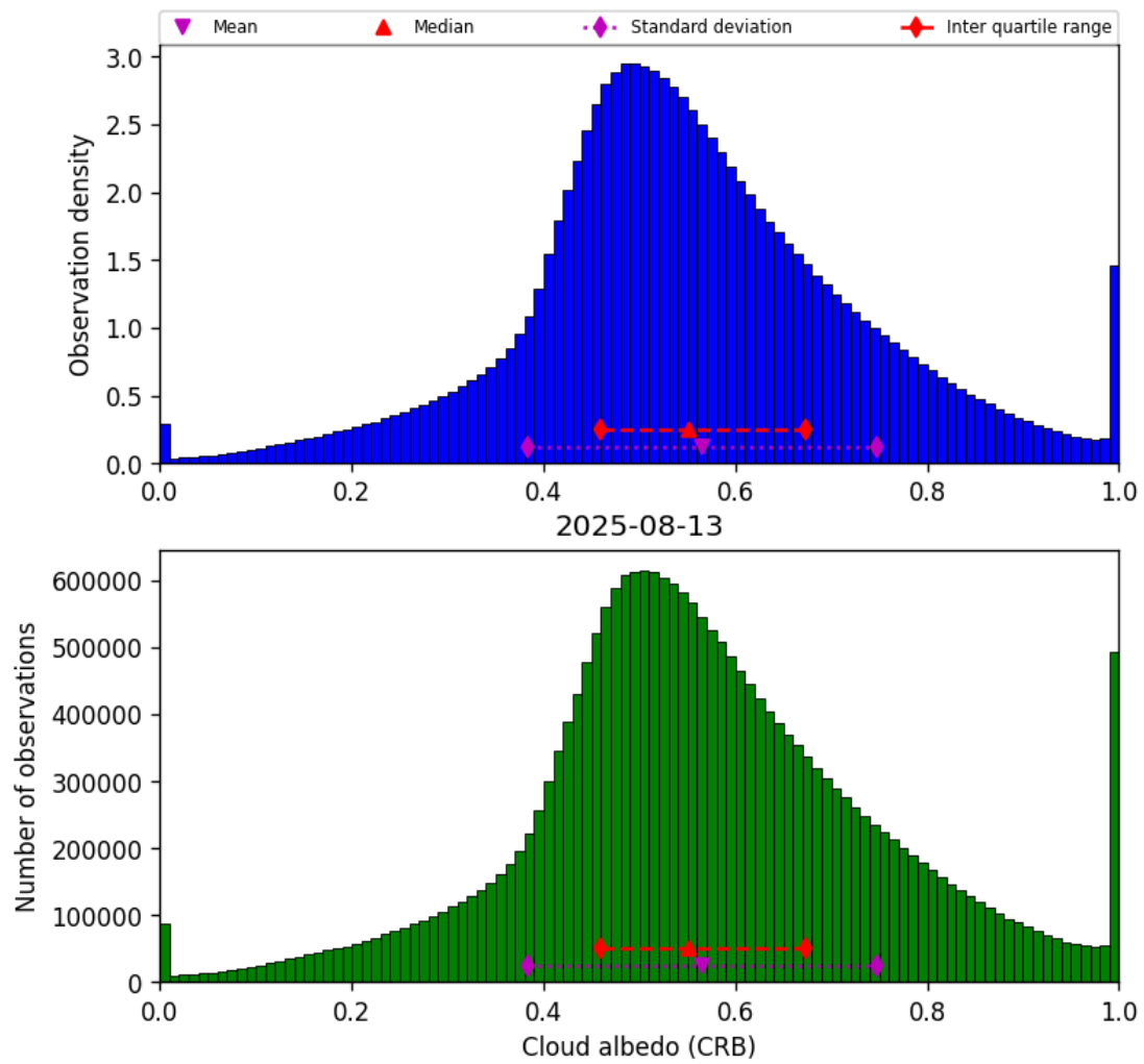
Figure 44: Histogram of “Cloud albedo (CRB)” for 2025-08-12 to 2025-08-14
