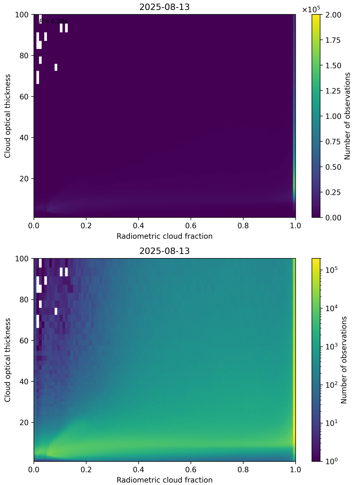
Figure 75: Scatter density plot of “Radiometric cloud fraction” against “Cloud optical thickness” for 2025-08-12 to 2025-08-14.
