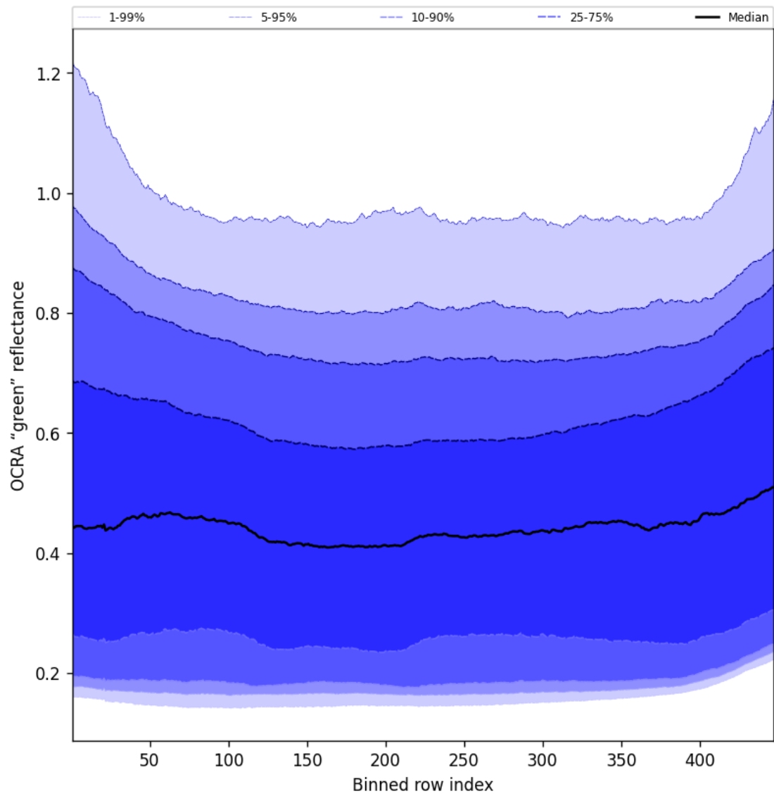
Figure 68: Along track statistics of “OCRA “green” reflectance” for 2025-08-12 to 2025-08-14
