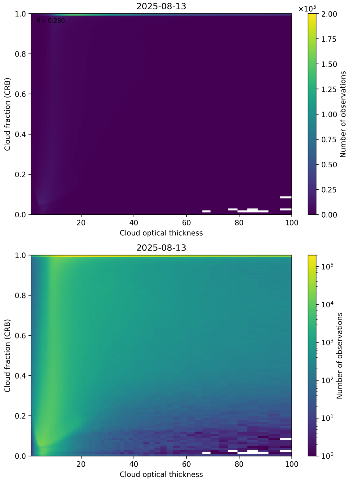
Figure 84: Scatter density plot of “Cloud optical thickness” against “Cloud fraction (CRB)” for 2025-08-12 to 2025-08-14.
