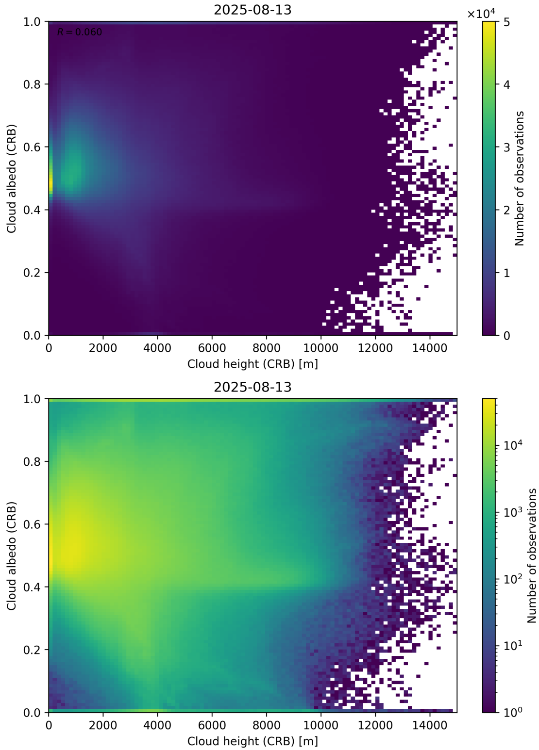
Figure 80: Scatter density plot of “Cloud height (CRB)” against “Cloud albedo (CRB)” for 2025-08-12 to 2025-08-14.
