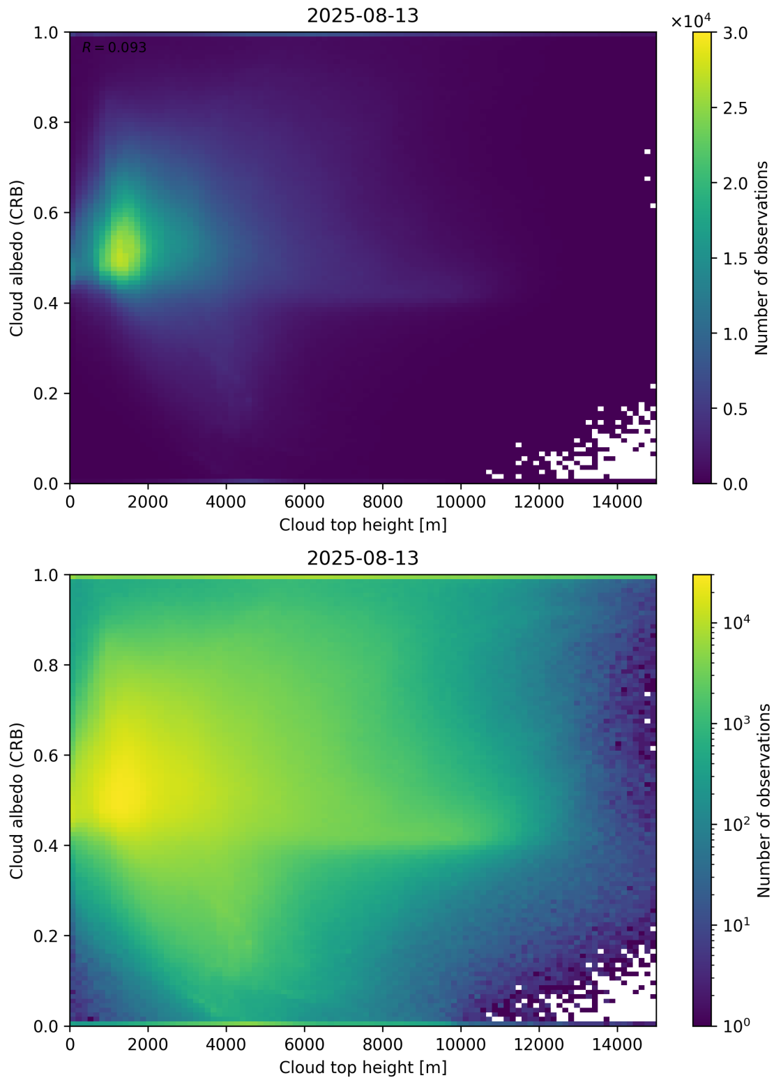
Figure 86: Scatter density plot of “Cloud top height” against “Cloud albedo (CRB)” for 2025-08-12 to 2025-08-14.
