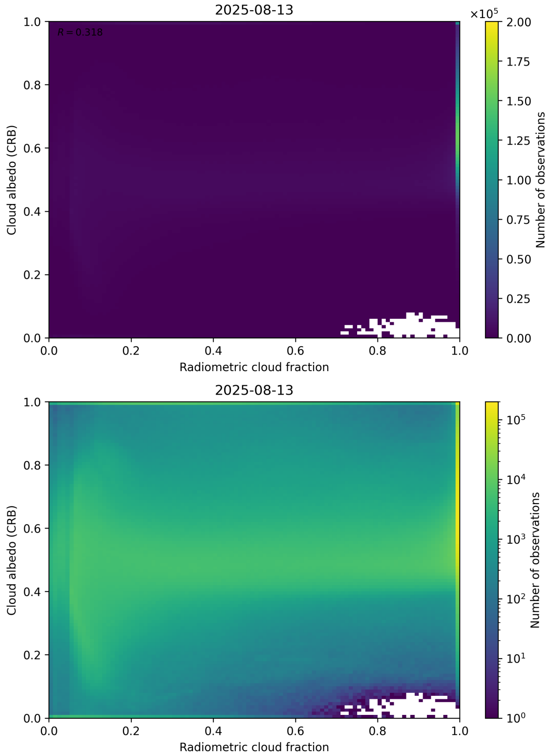
Figure 71: Scatter density plot of “Radiometric cloud fraction” against “Cloud albedo (CRB)” for 2025-08-12 to 2025-08-14.
