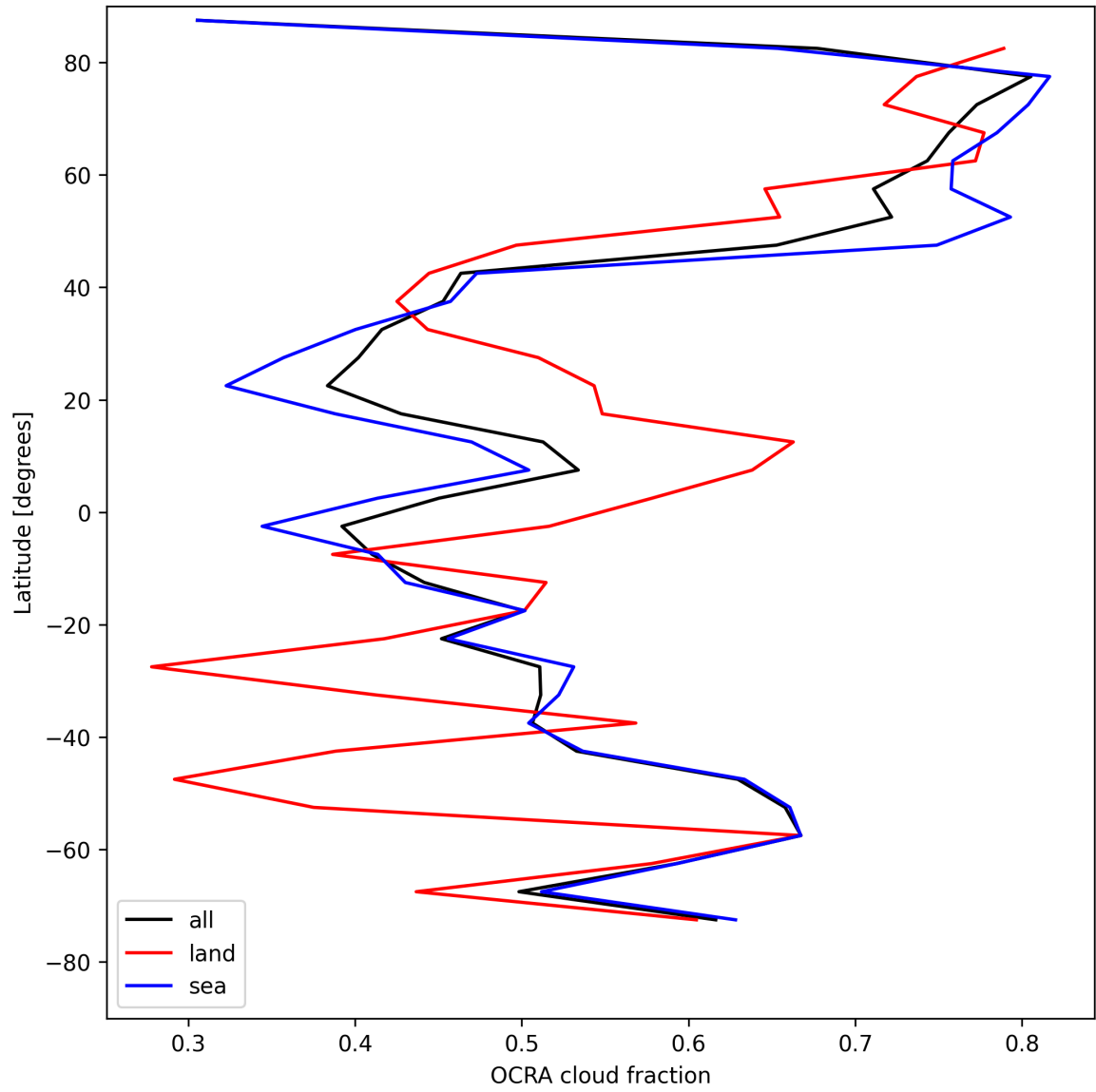
Figure 34: Zonal average of “OCRA cloud fraction” for 2025-08-12 to 2025-08-14.
