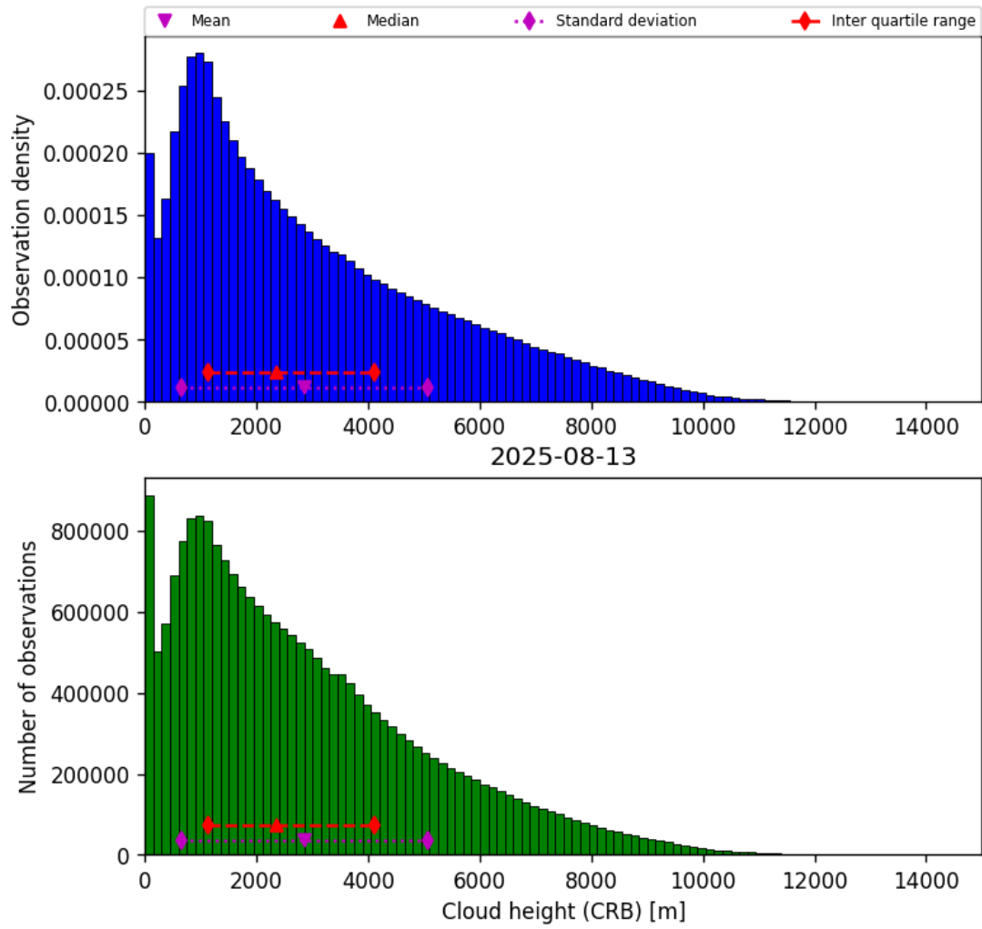
Figure 43: Histogram of “Cloud height (CRB)” for 2025-08-12 to 2025-08-14
