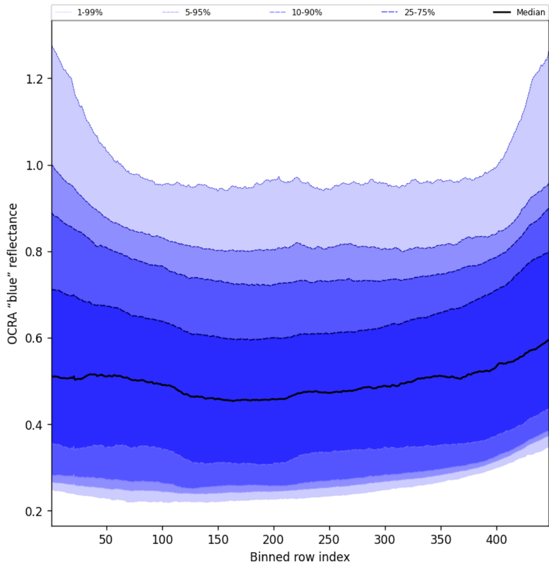
Figure 67: Along track statistics of "OCRA "blue" reflectance" for 2025-08-12 to 2025-08-14
