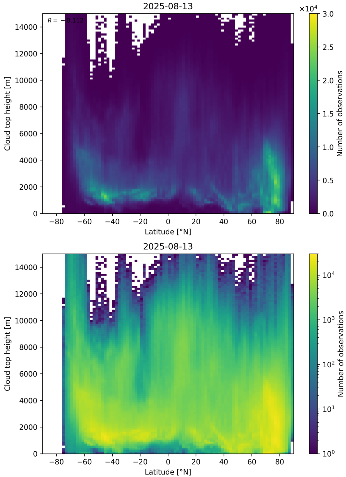
Figure 97: Scatter density plot of “Latitude” against “Cloud top height” for 2025-08-12 to 2025-08-14.
