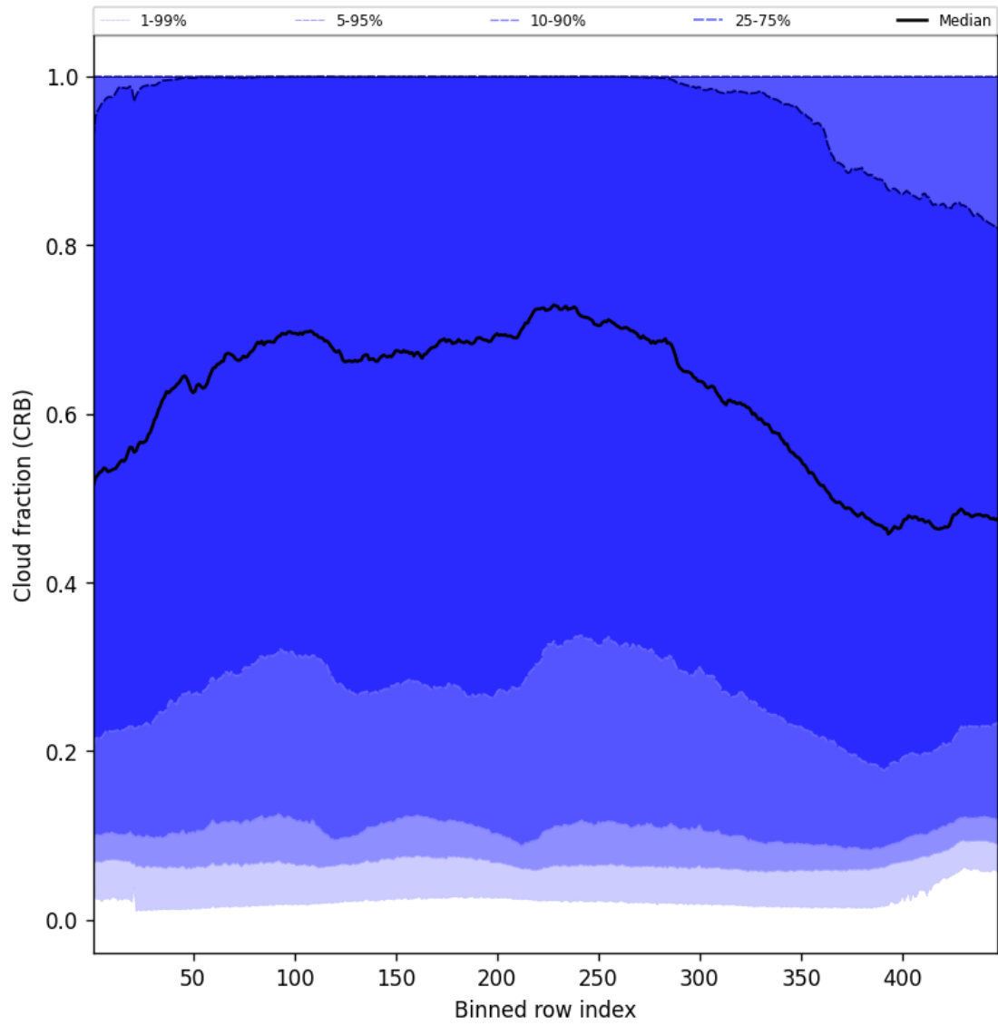
Figure 58: Along track statistics of “Cloud fraction (CRB)” for 2025-08-12 to 2025-08-14
