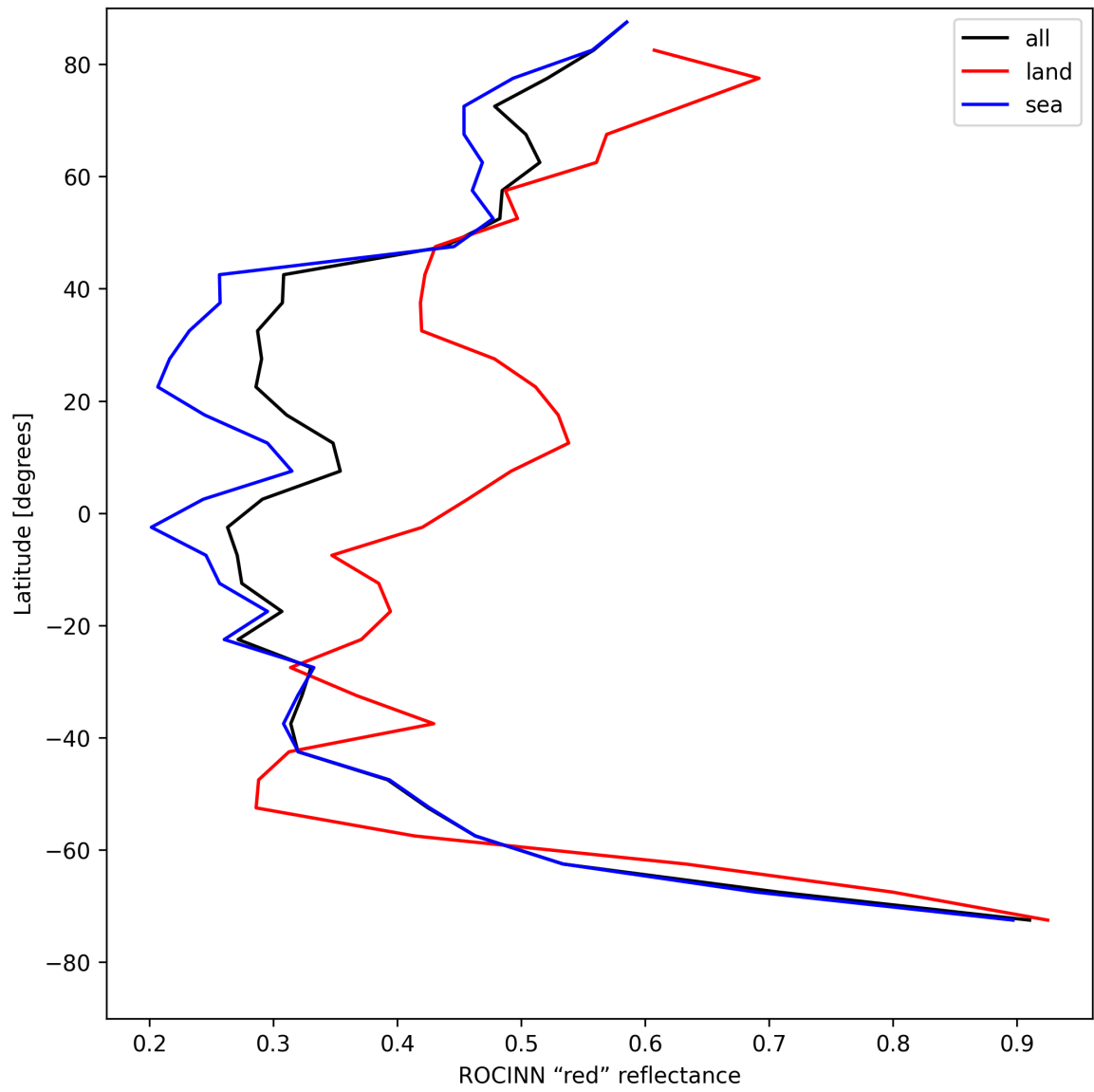
Figure 37: Zonal average of "ROCINN "red" reflectance" for 2025-08-12 to 2025-08-14.
