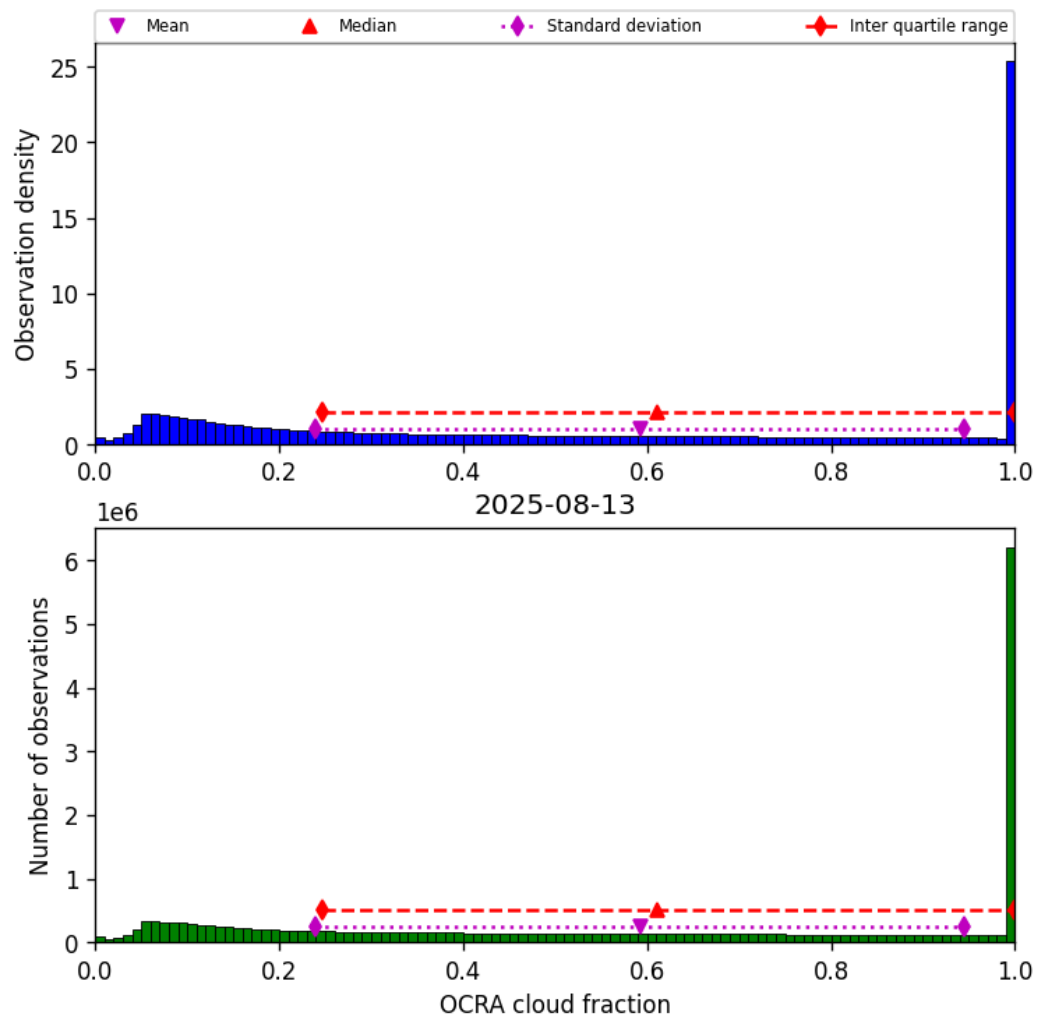
Figure 50: Histogram of “OCRA cloud fraction” for 2025-08-12 to 2025-08-14
