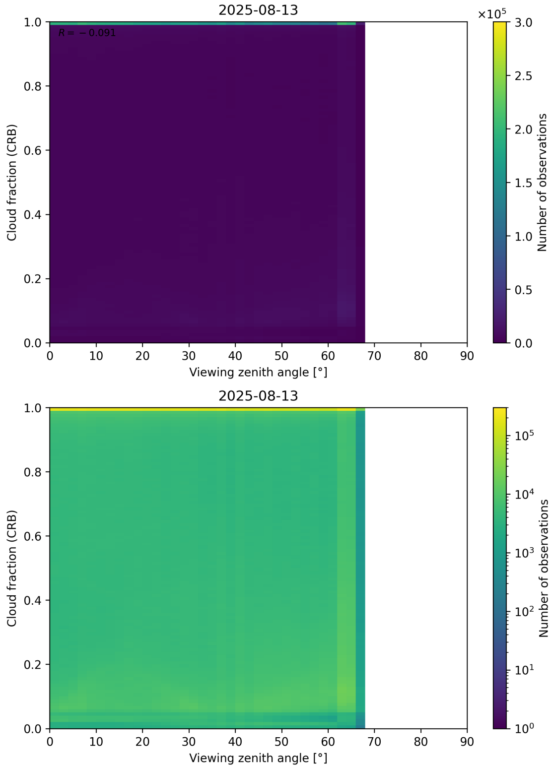
Figure 109: Scatter density plot of “Viewing zenith angle” against “Cloud fraction (CRB)” for 2025-08-12 to 2025-08-14.
