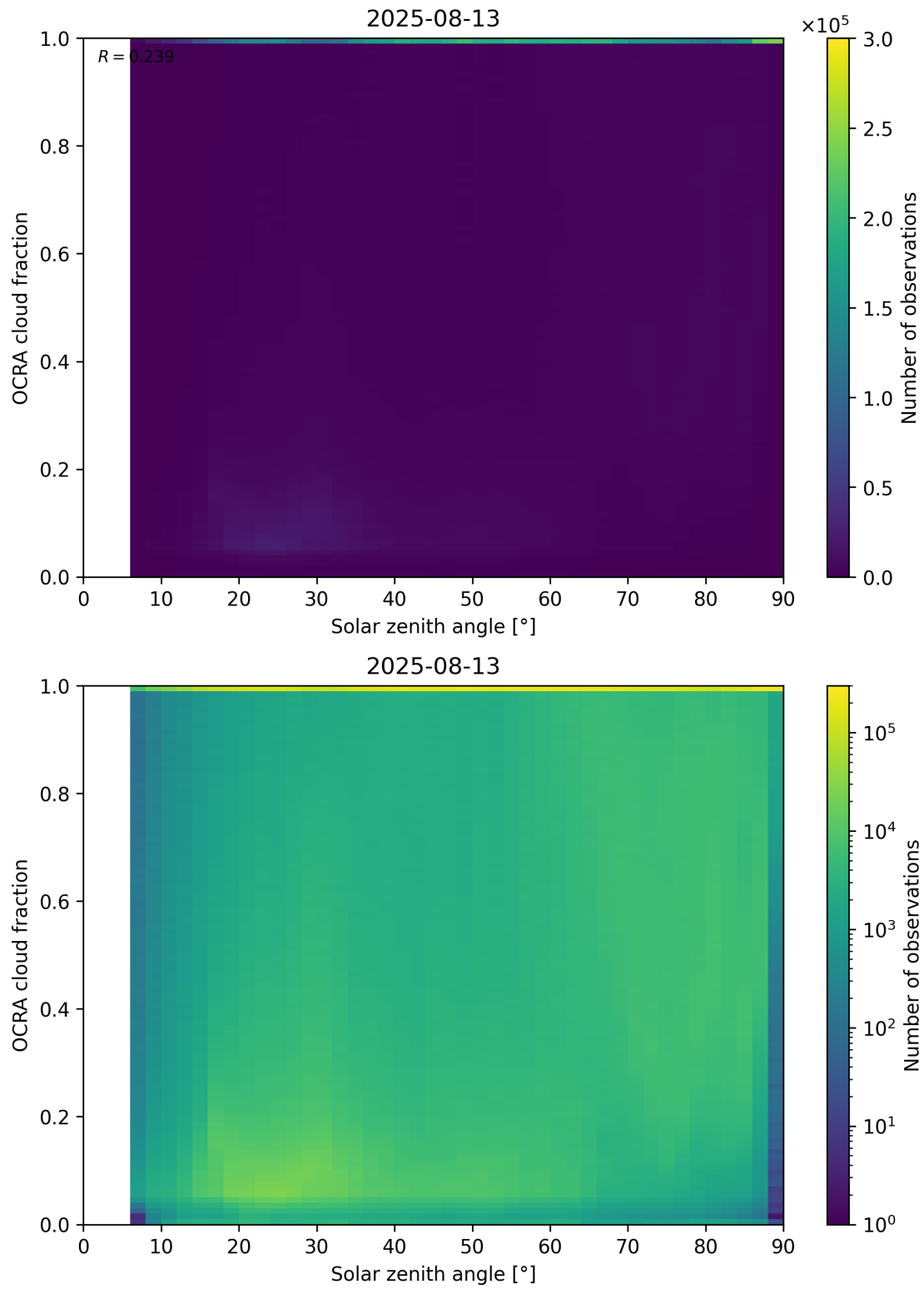
Figure 100: Scatter density plot of “Solar zenith angle” against “OCRA cloud fraction” for 2025-08-12 to 2025-08-14.
