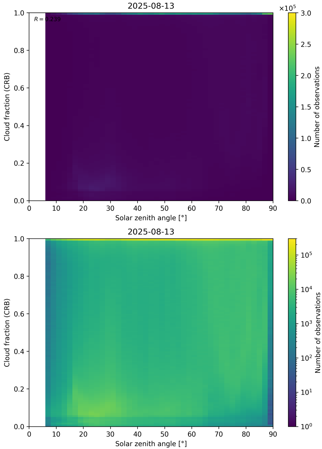
Figure 101: Scatter density plot of “Solar zenith angle” against “Cloud fraction (CRB)” for 2025-08-12 to 2025-08-14.
