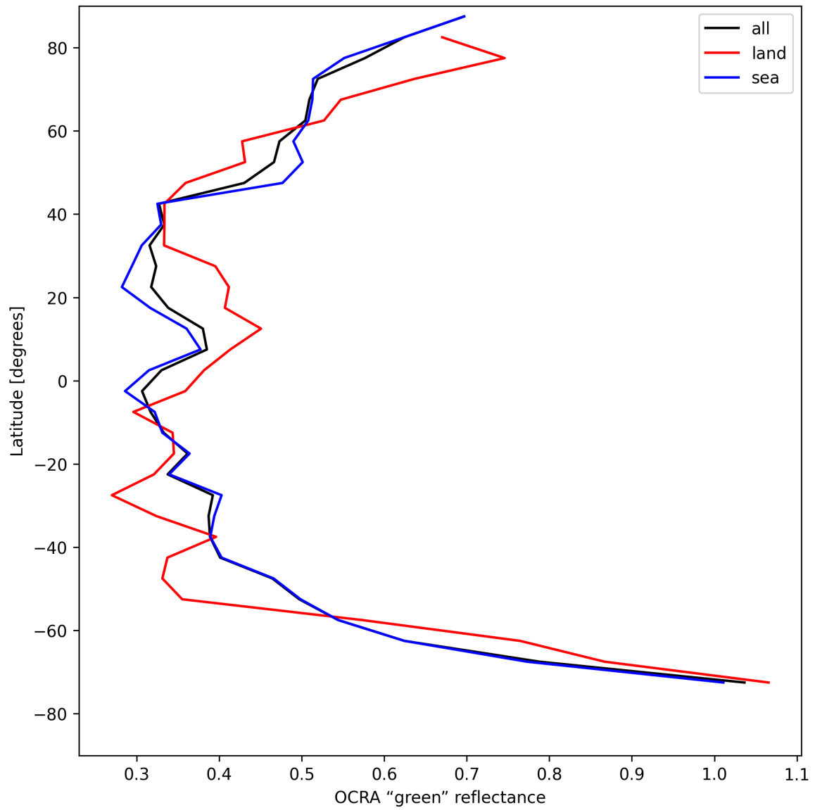
Figure 36: Zonal average of “OCRA “green” reflectance” for 2025-08-12 to 2025-08-14.
