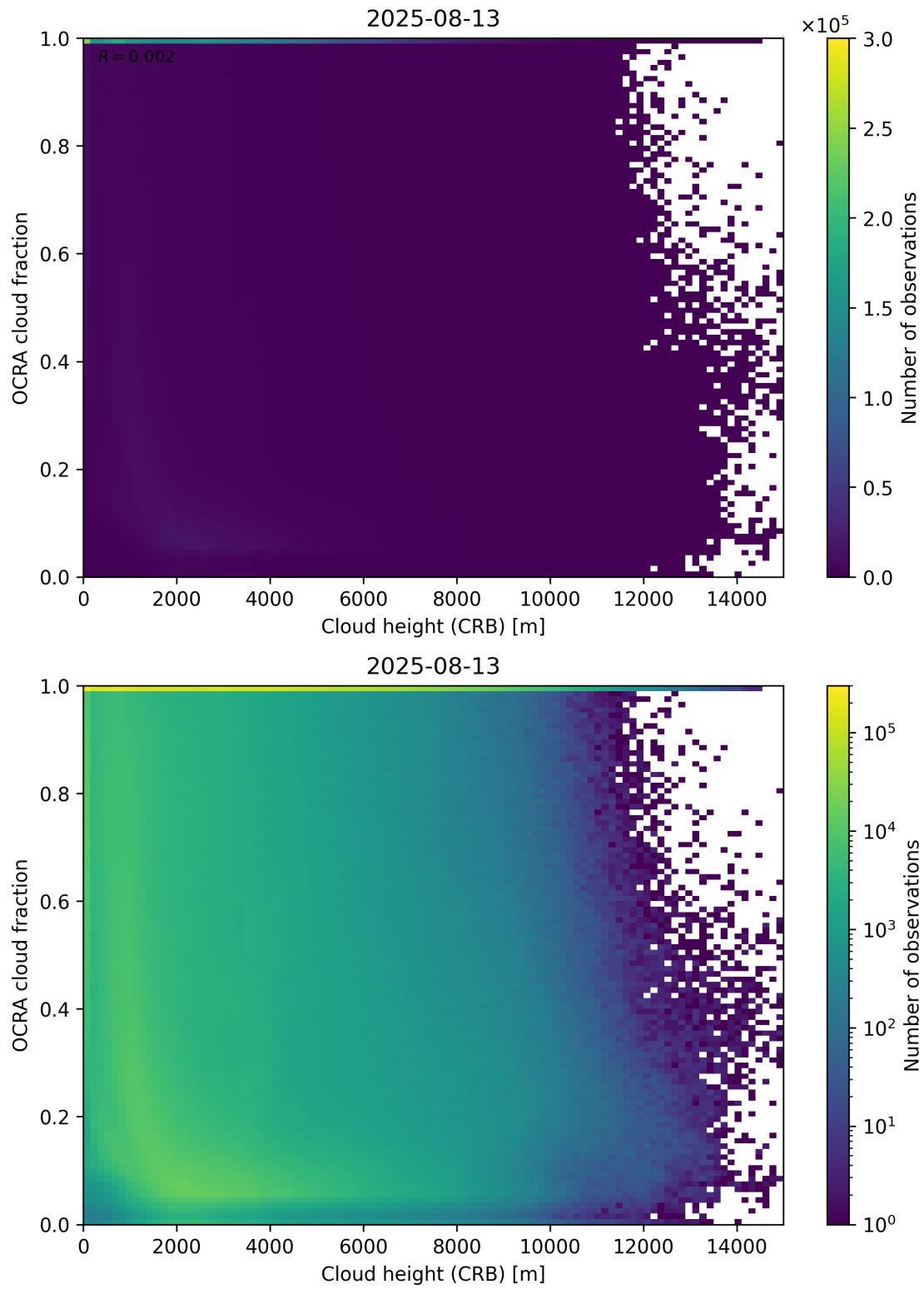
Figure 81: Scatter density plot of “Cloud height (CRB)” against “OCRA cloud fraction” for 2025-08-12 to 2025-08-14.
