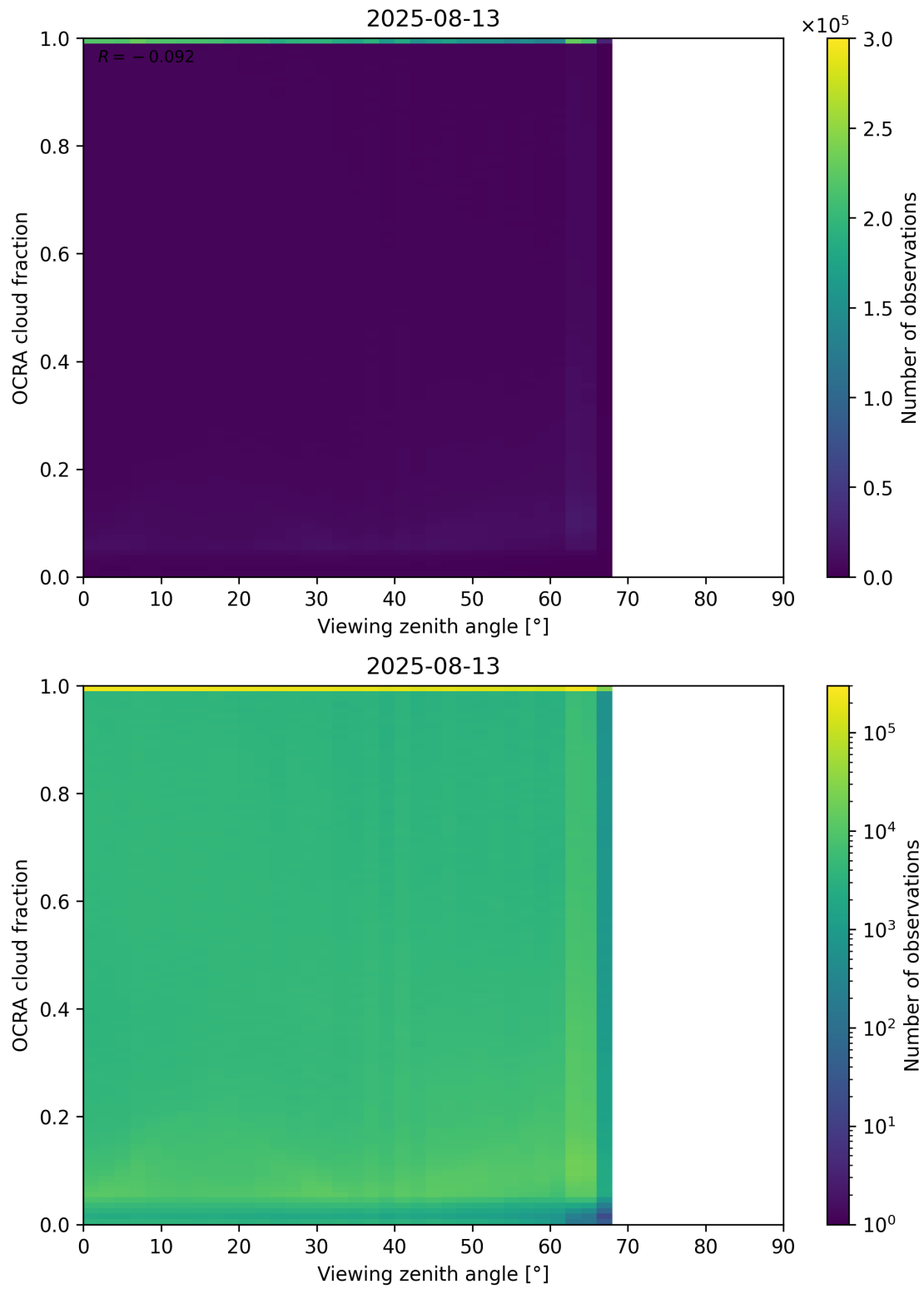
Figure 108: Scatter density plot of “Viewing zenith angle” against “OCRA cloud fraction” for 2025-08-12 to 2025-08-14.
