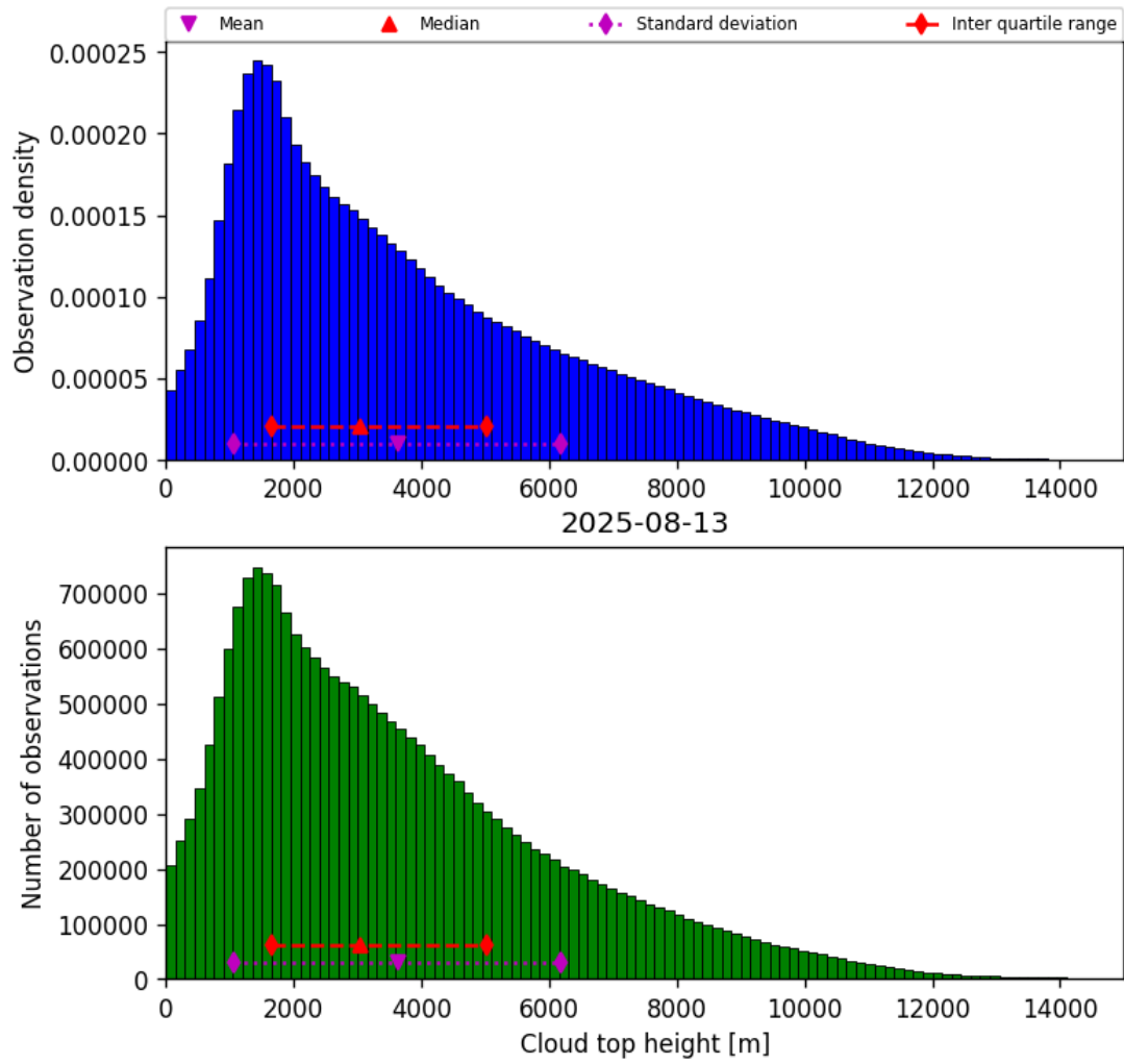
Figure 40: Histogram of “Cloud top height” for 2025-08-12 to 2025-08-14
