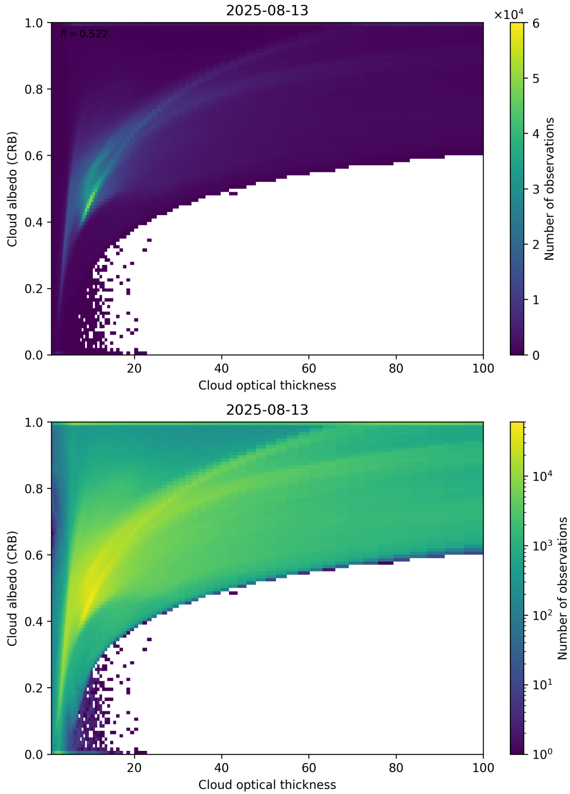
Figure 82: Scatter density plot of “Cloud optical thickness” against “Cloud albedo (CRB)” for 2025-08-12 to 2025-08-14.
