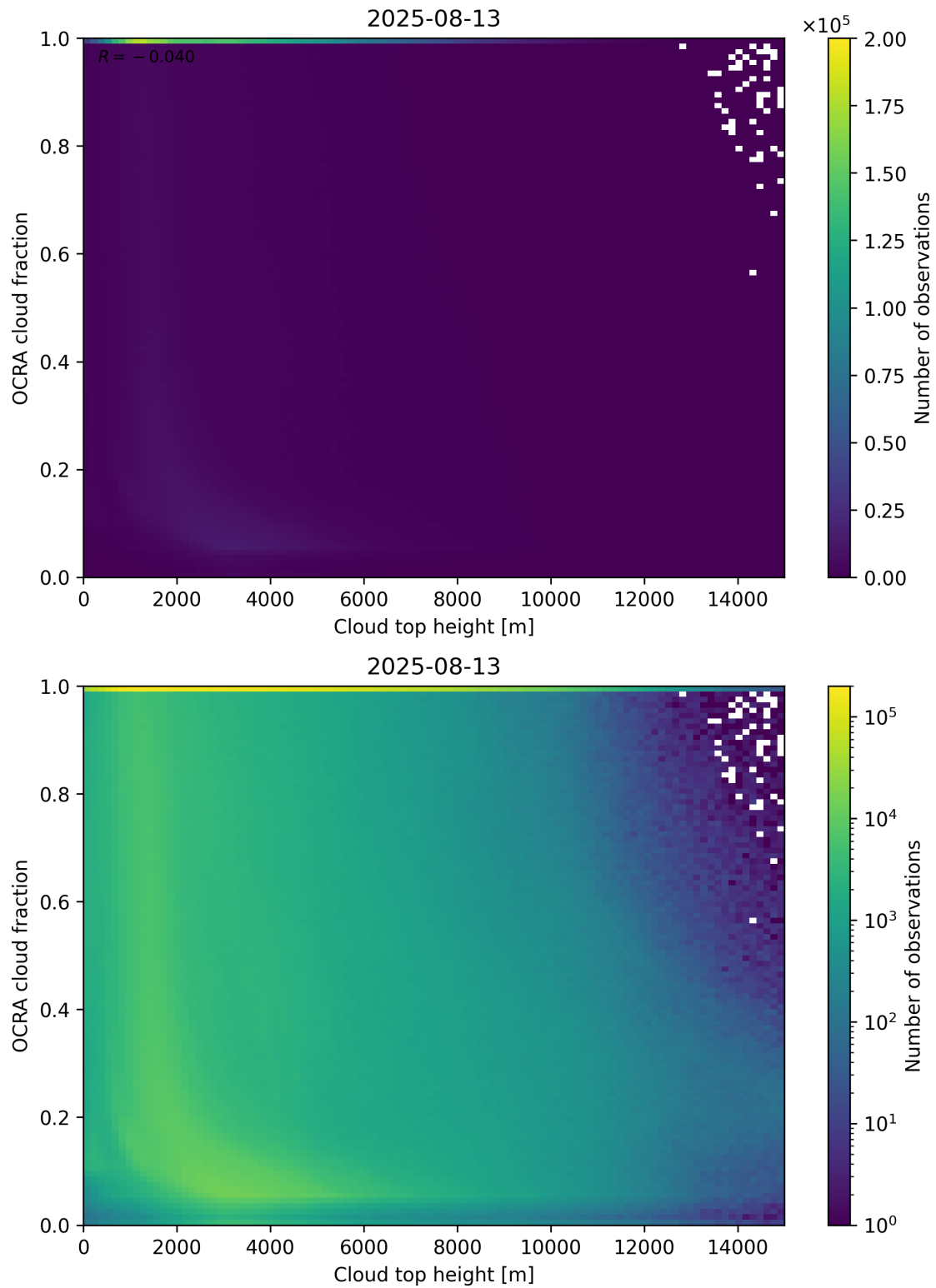
Figure 87: Scatter density plot of “Cloud top height” against “OCRA cloud fraction” for 2025-08-12 to 2025-08-14.
