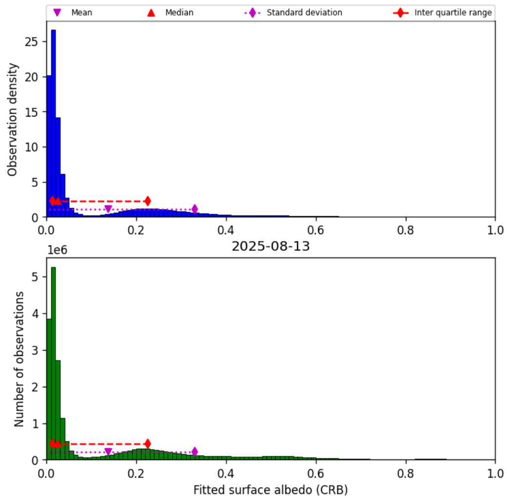
Figure 46: Histogram of “Fitted surface albedo (CRB)” for 2025-08-12 to 2025-08-14
