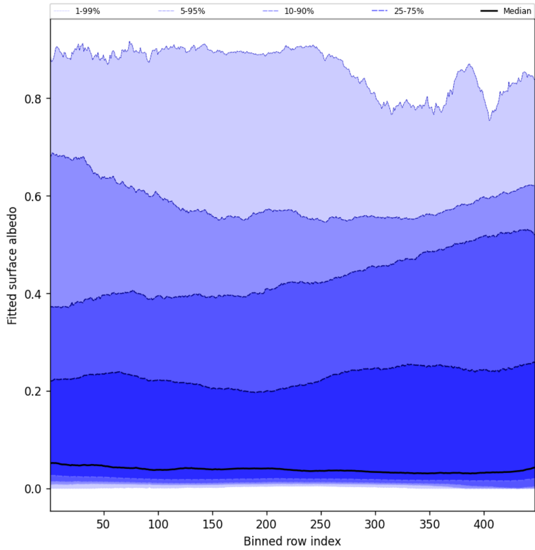
Figure 61: Along track statistics of “Fitted surface albedo” for 2025-08-12 to 2025-08-14
