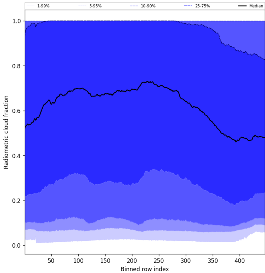
Figure 55: Along track statistics of “Radiometric cloud fraction” for 2025-08-12 to 2025-08-14
