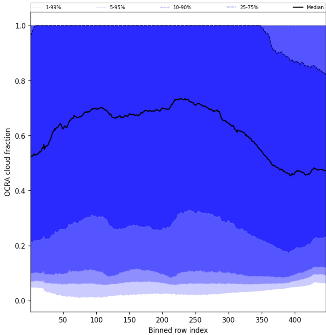
Figure 66: Along track statistics of “OCRA cloud fraction” for 2025-08-12 to 2025-08-14
