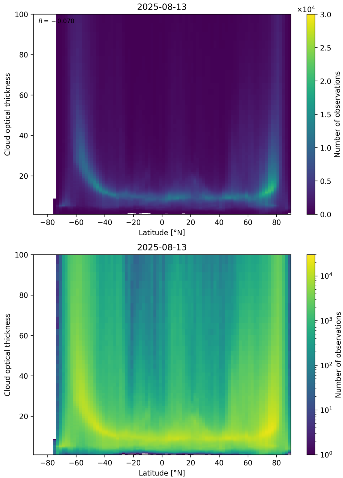
Figure 96: Scatter density plot of “Latitude” against “Cloud optical thickness” for 2025-08-12 to 2025-08-14.
