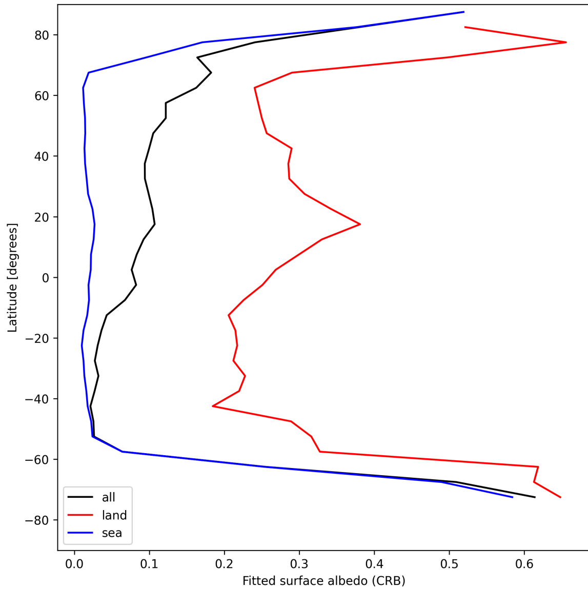
Figure 30: Zonal average of “Fitted surface albedo (CRB)” for 2025-08-12 to 2025-08-14.
