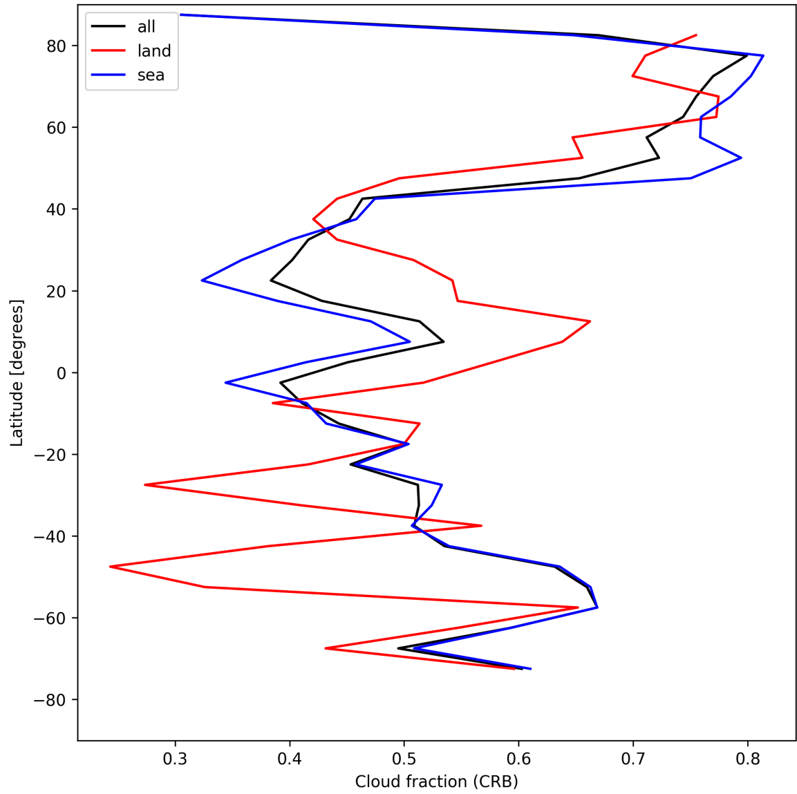
Figure 26: Zonal average of “Cloud fraction (CRB)” for 2025-08-12 to 2025-08-14.
