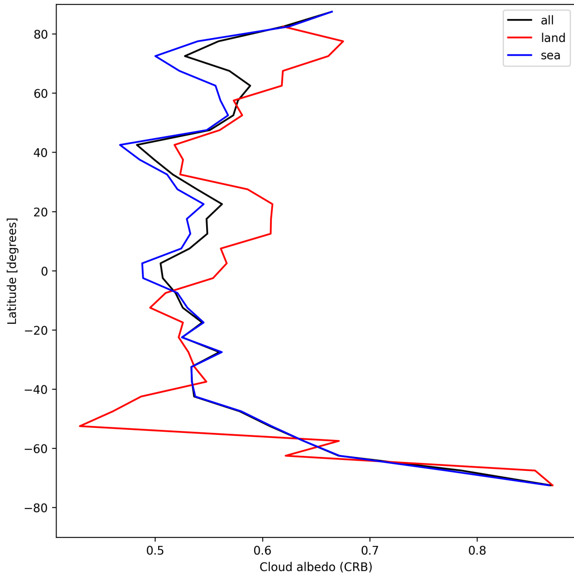
Figure 28: Zonal average of “Cloud albedo (CRB)” for 2025-08-12 to 2025-08-14.
