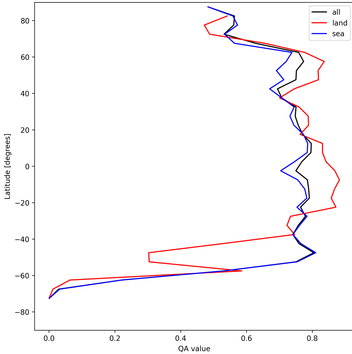
Figure 22: Zonal average of “QA value” for 2025-08-12 to 2025-08-14.
