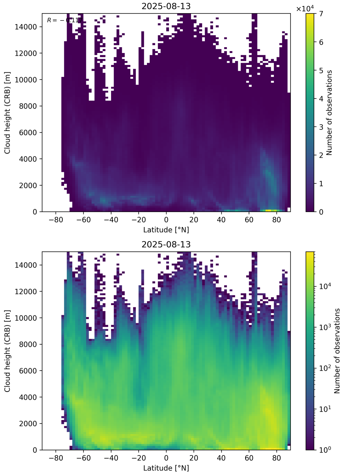
Figure 95: Scatter density plot of “Latitude” against “Cloud height (CRB)” for 2025-08-12 to 2025-08-14.
