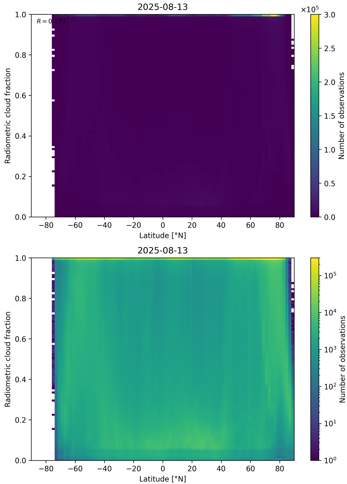
Figure 92: Scatter density plot of “Latitude” against “Radiometric cloud fraction” for 2025-08-12 to 2025-08-14.
