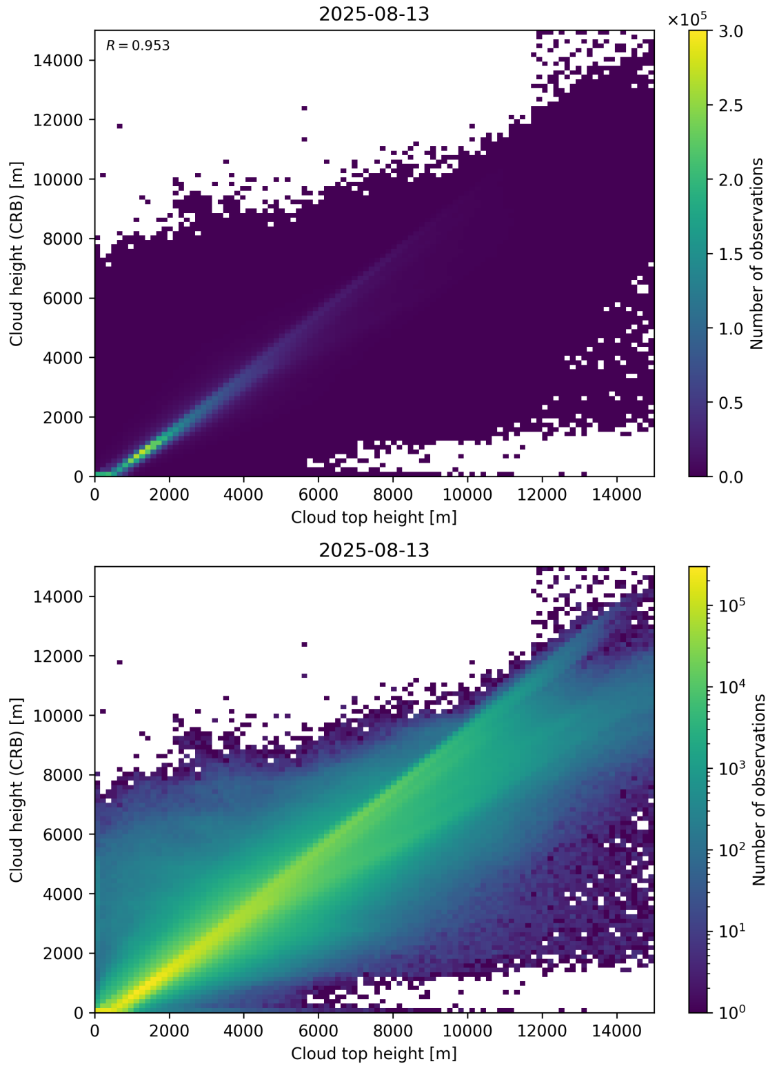
Figure 89: Scatter density plot of “Cloud top height” against “Cloud height (CRB)” for 2025-08-12 to 2025-08-14.
