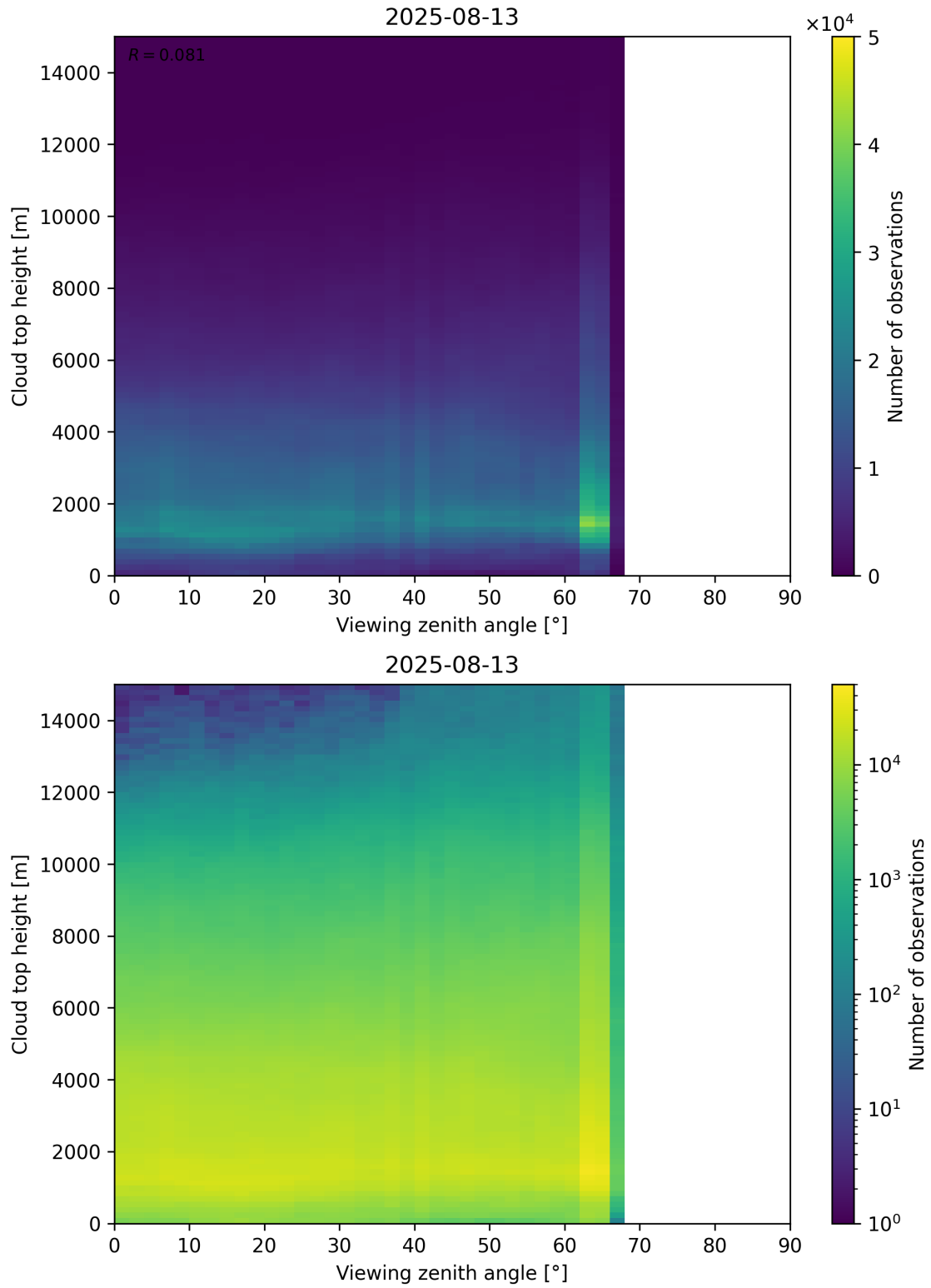
Figure 112: Scatter density plot of “Viewing zenith angle” against “Cloud top height” for 2025-08-12 to 2025-08-14.
