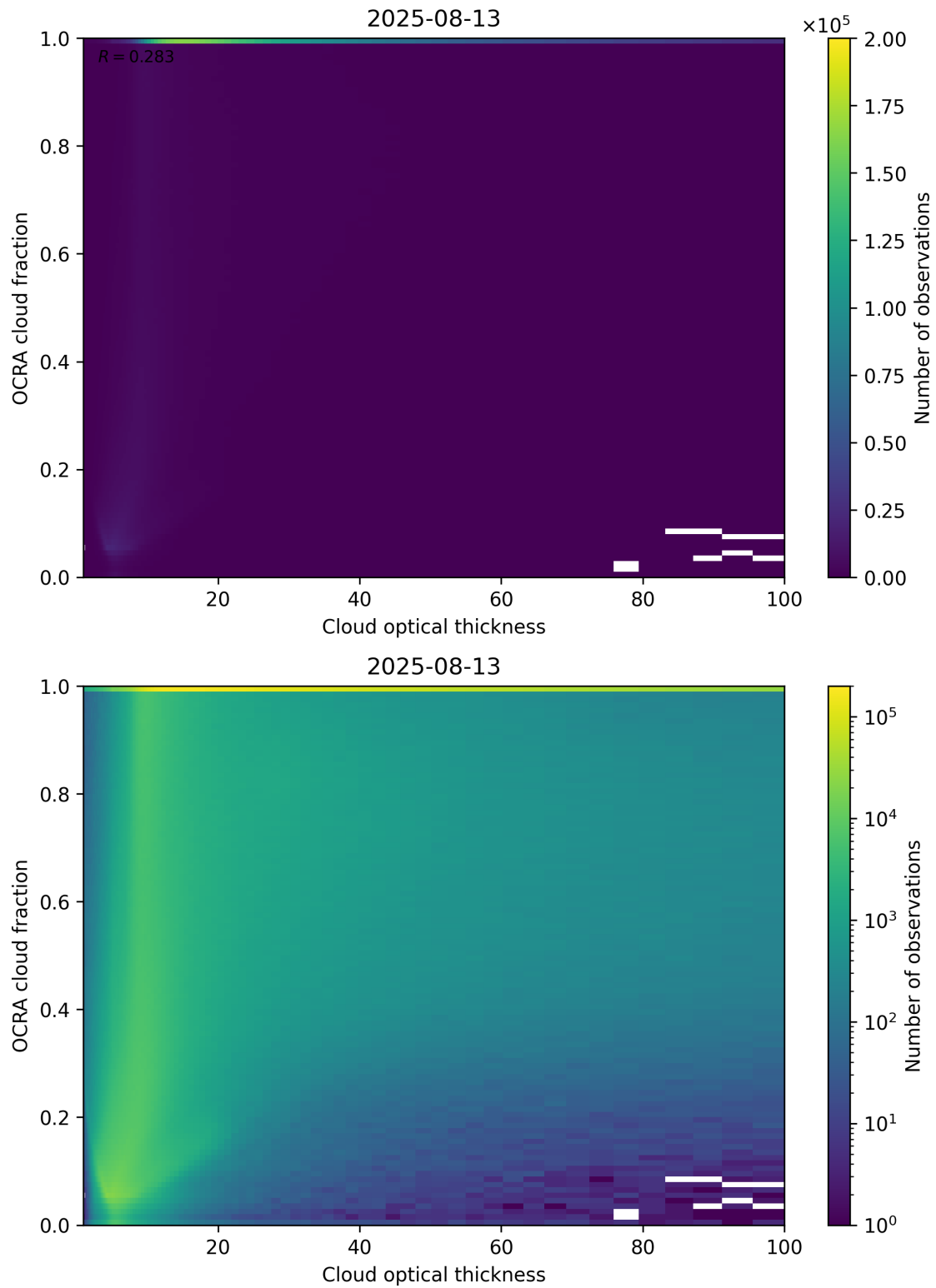
Figure 83: Scatter density plot of “Cloud optical thickness” against “OCRA cloud fraction” for 2025-08-12 to 2025-08-14.
