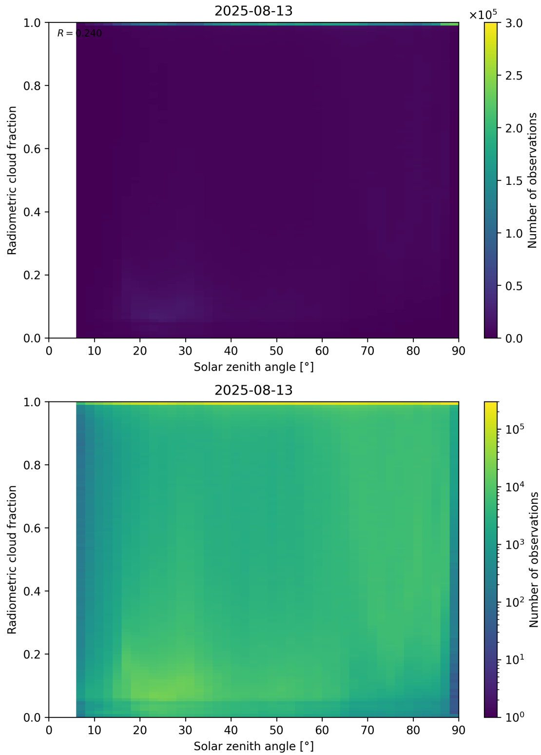
Figure 99: Scatter density plot of “Solar zenith angle” against “Radiometric cloud fraction” for 2025-08-12 to 2025-08-14.
