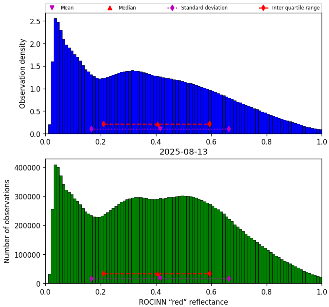
Figure 53: Histogram of “ROCINN “red” reflectance” for 2025-08-12 to 2025-08-14
