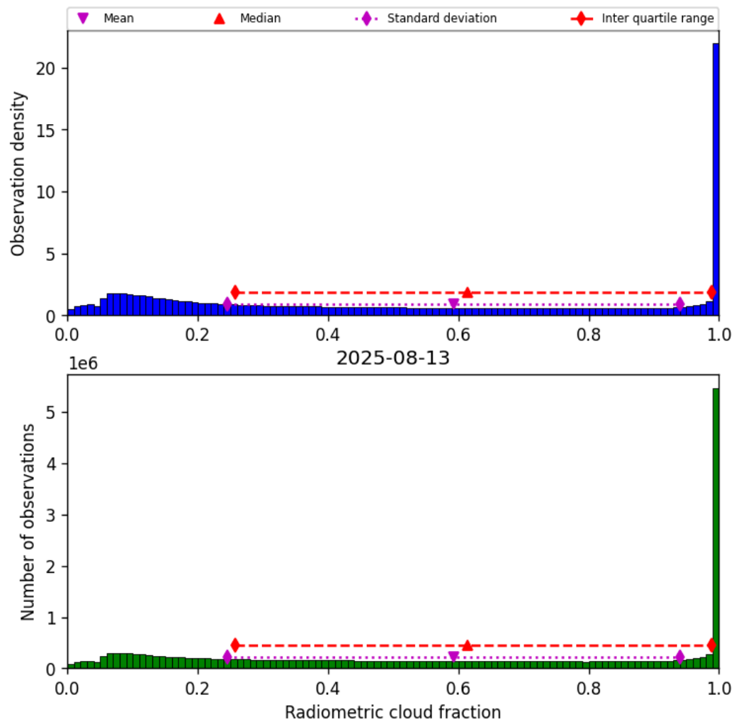
Figure 39: Histogram of “Radiometric cloud fraction” for 2025-08-12 to 2025-08-14
