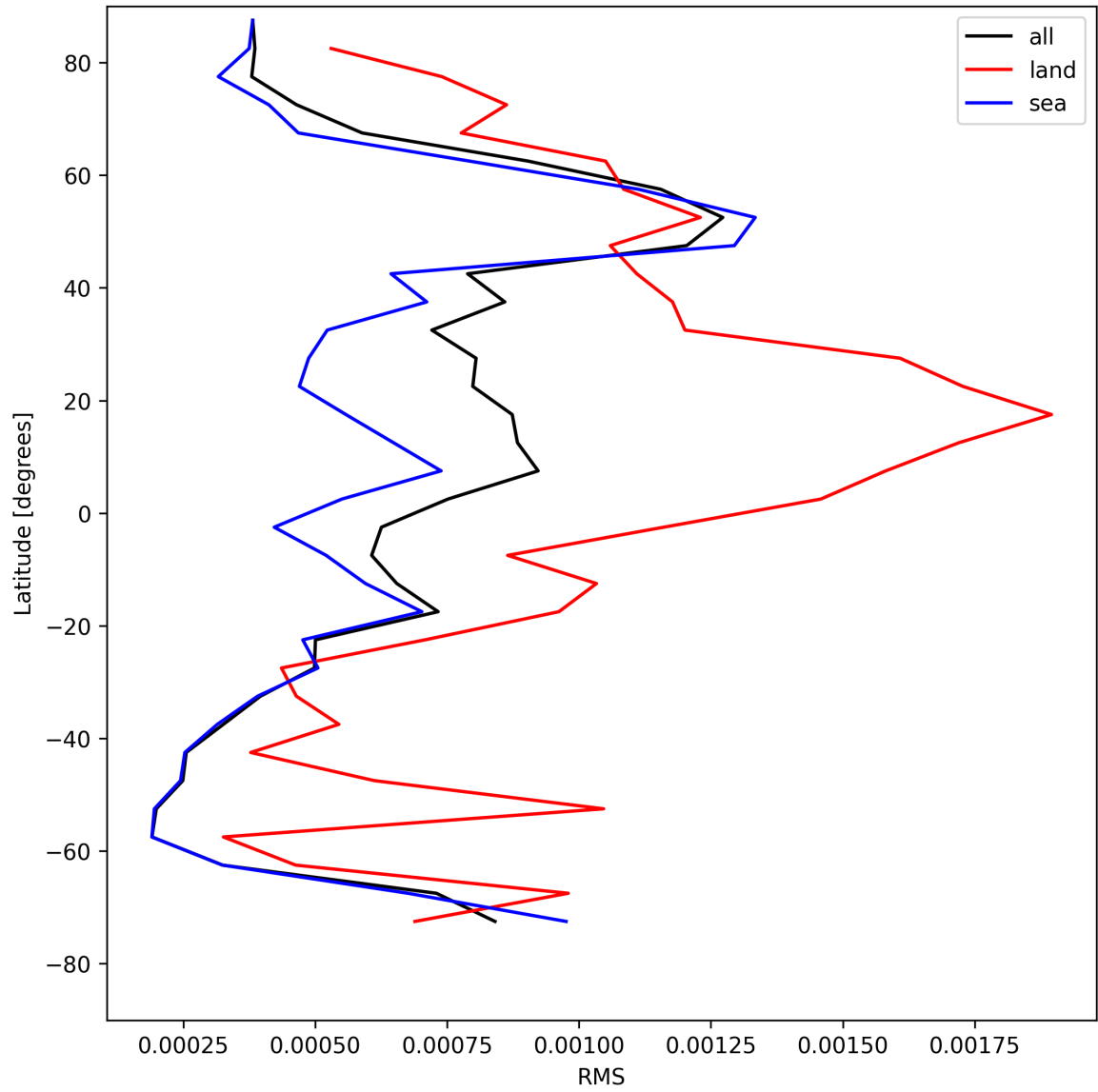
Figure 31: Zonal average of “RMS” for 2025-08-12 to 2025-08-14.
