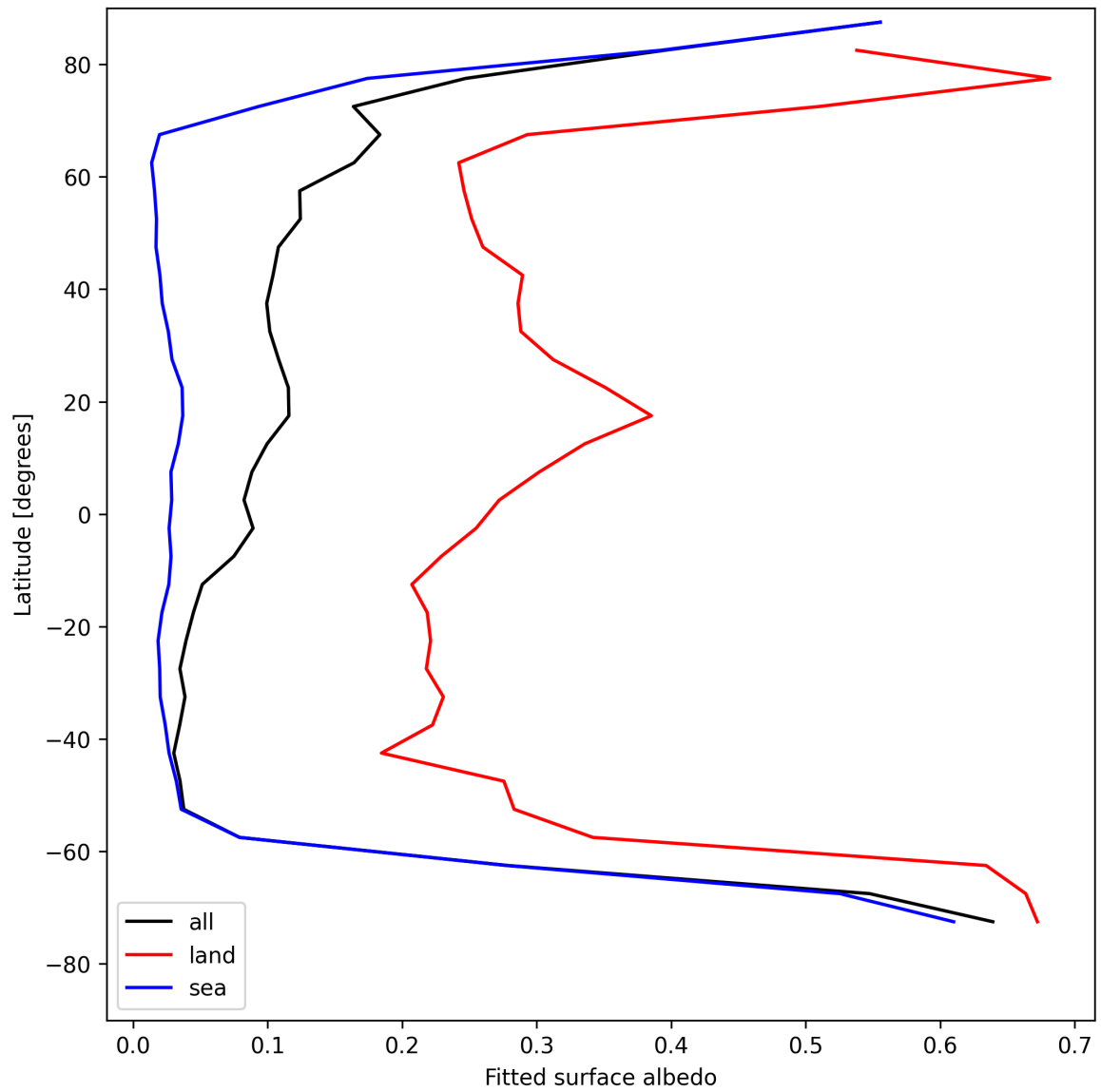
Figure 29: Zonal average of “Fitted surface albedo” for 2025-08-12 to 2025-08-14.
