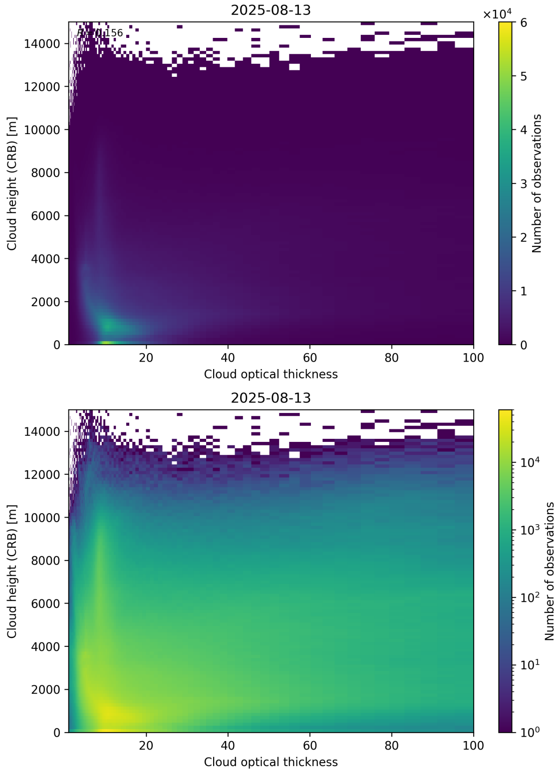
Figure 85: Scatter density plot of “Cloud optical thickness” against “Cloud height (CRB)” for 2025-08-12 to 2025-08-14.
