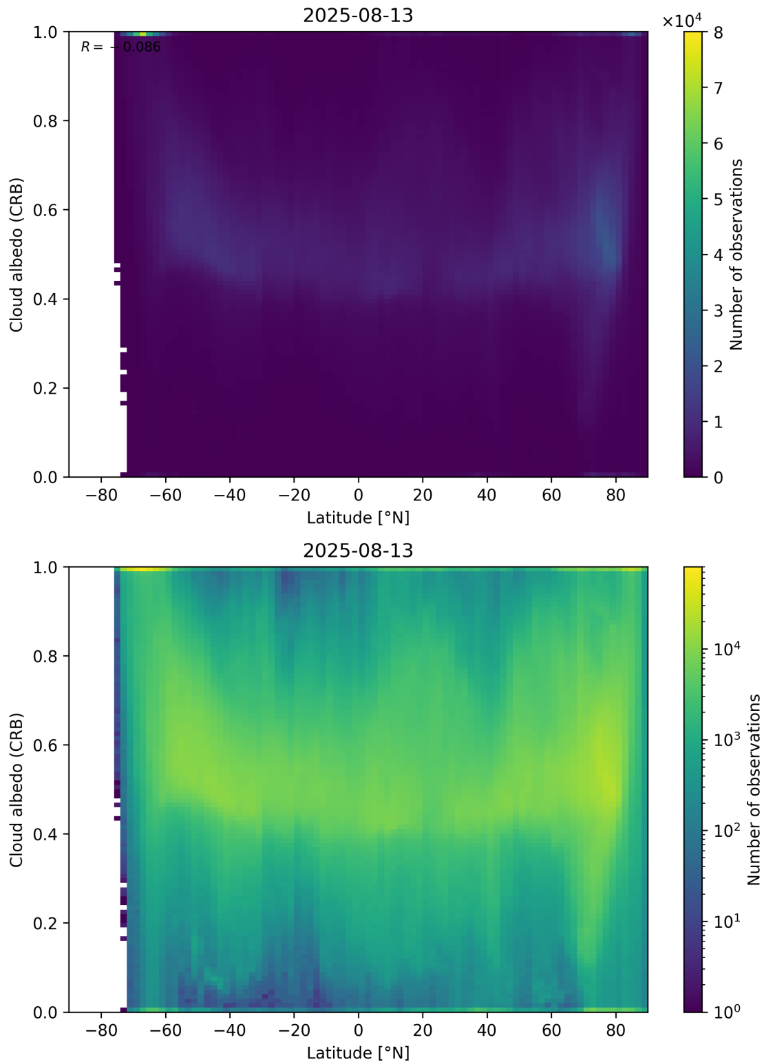
Figure 91: Scatter density plot of “Latitude” against “Cloud albedo (CRB)” for 2025-08-12 to 2025-08-14.
