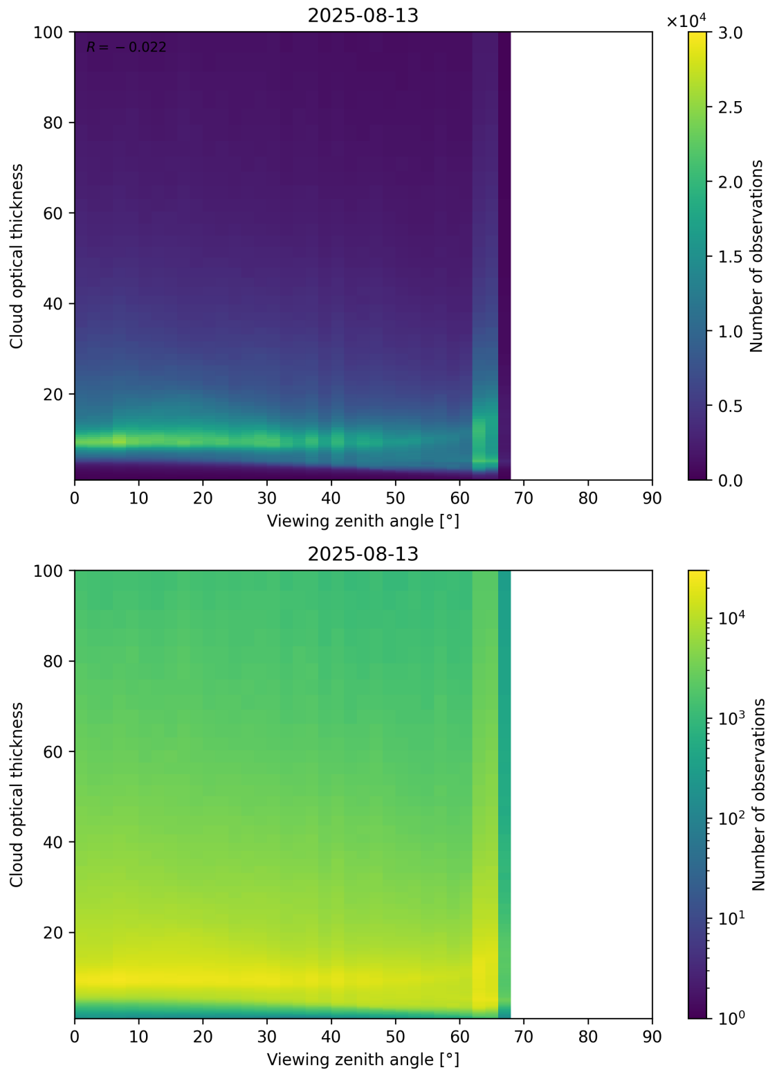
Figure 111: Scatter density plot of “Viewing zenith angle” against “Cloud optical thickness” for 2025-08-12 to 2025-08-14.
