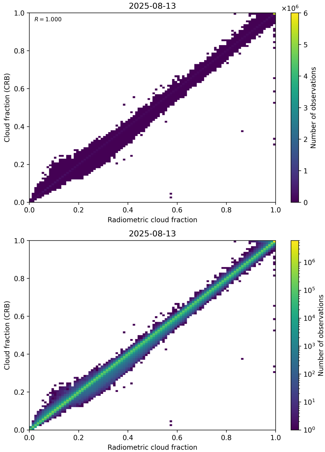
Figure 73: Scatter density plot of “Radiometric cloud fraction” against “Cloud fraction (CRB)” for 2025-08-12 to 2025-08-14.
