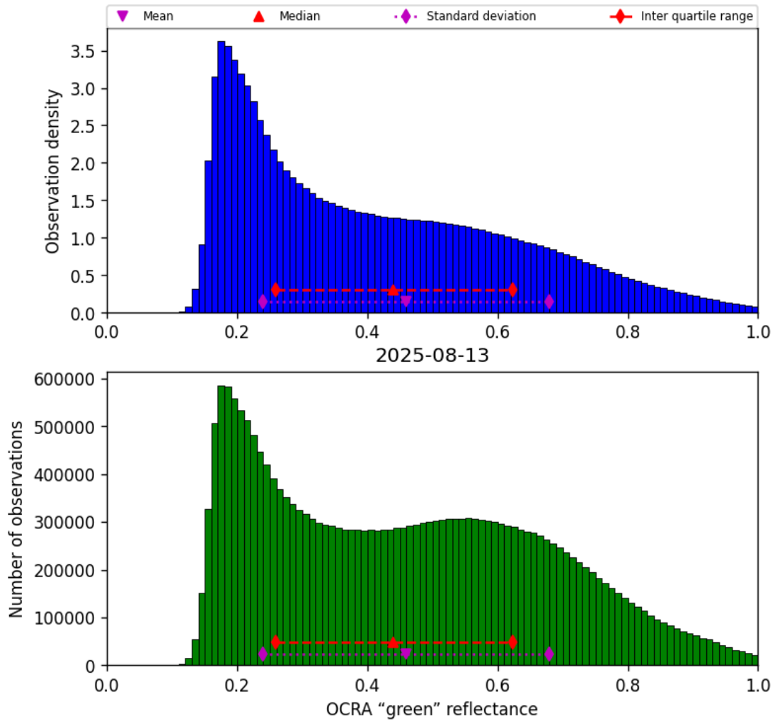
Figure 52: Histogram of “OCRA “green” reflectance” for 2025-08-12 to 2025-08-14
