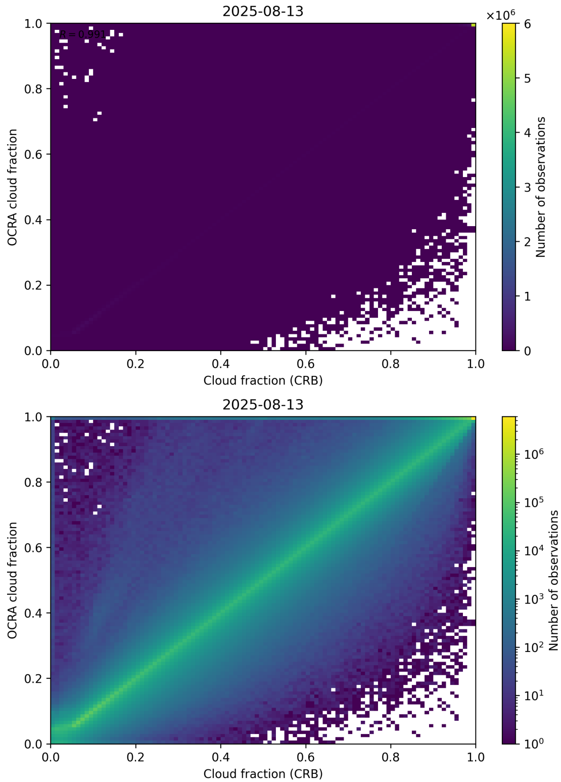
Figure 78: Scatter density plot of “Cloud fraction (CRB)” against “OCRA cloud fraction” for 2025-08-12 to 2025-08-14.
