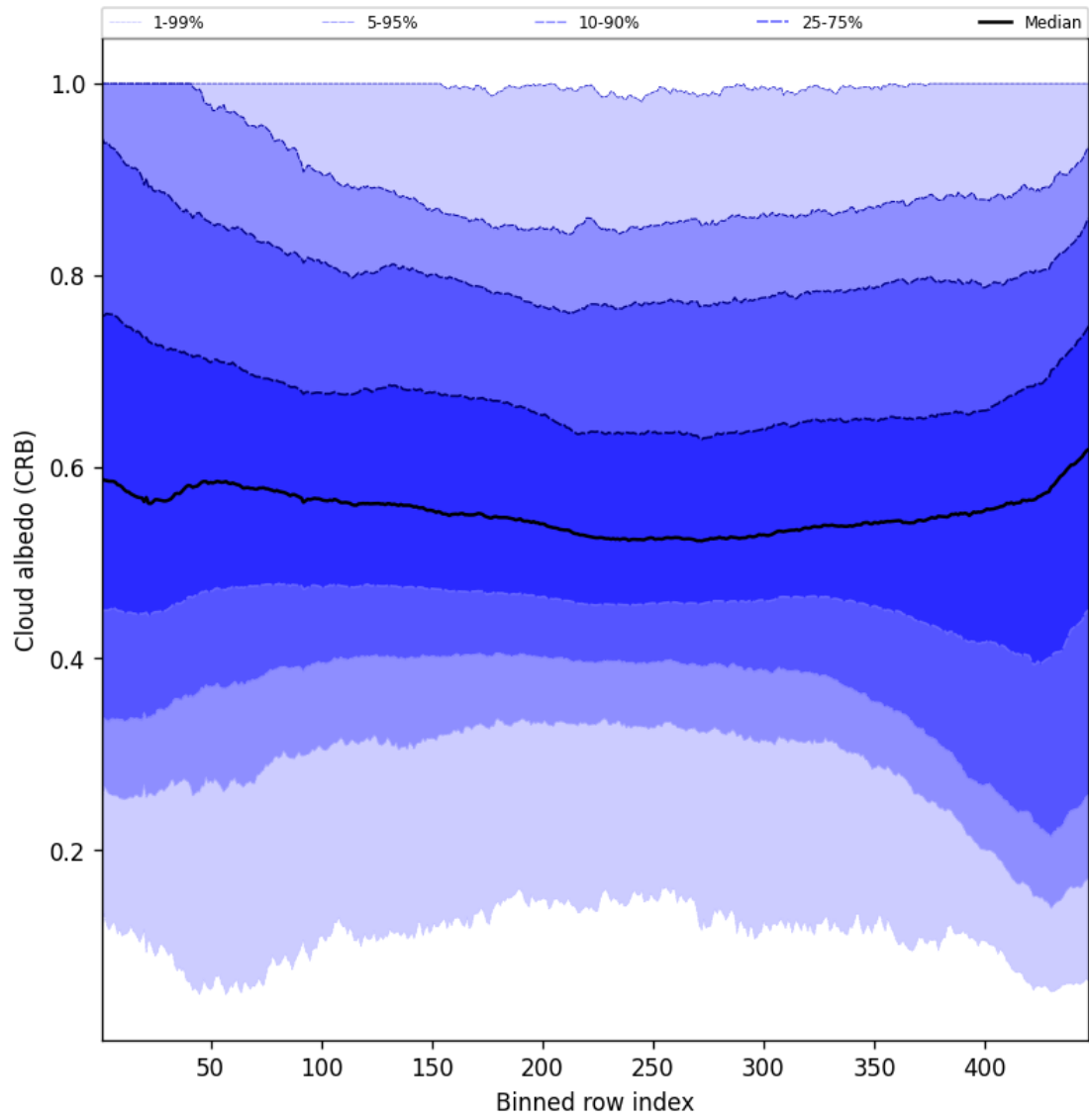
Figure 60: Along track statistics of “Cloud albedo (CRB)” for 2025-08-12 to 2025-08-14
