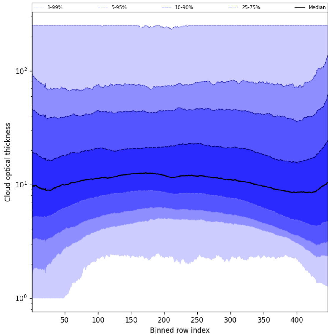
Figure 57: Along track statistics of “Cloud optical thickness” for 2025-08-12 to 2025-08-14
