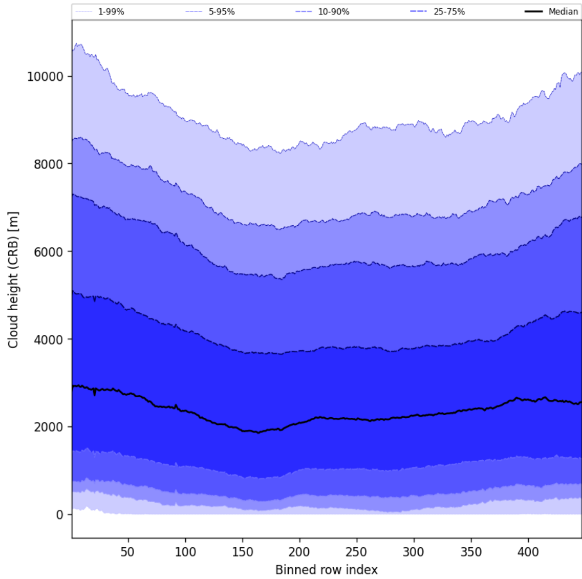
Figure 59: Along track statistics of “Cloud height (CRB)” for 2025-08-12 to 2025-08-14
