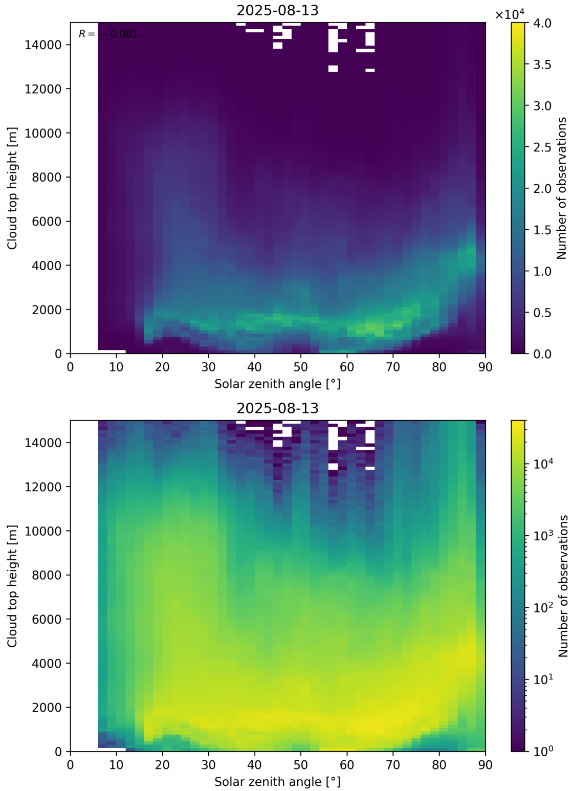
Figure 104: Scatter density plot of “Solar zenith angle” against “Cloud top height” for 2025-08-12 to 2025-08-14.
