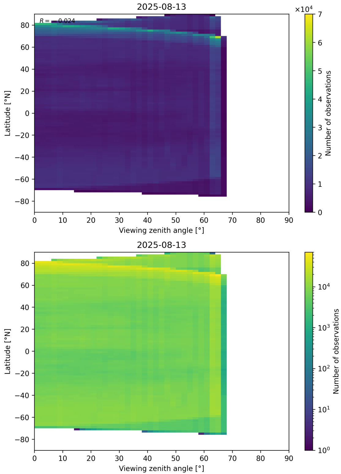
Figure 113: Scatter density plot of “Viewing zenith angle” against “Latitude” for 2025-08-12 to 2025-08-14.
