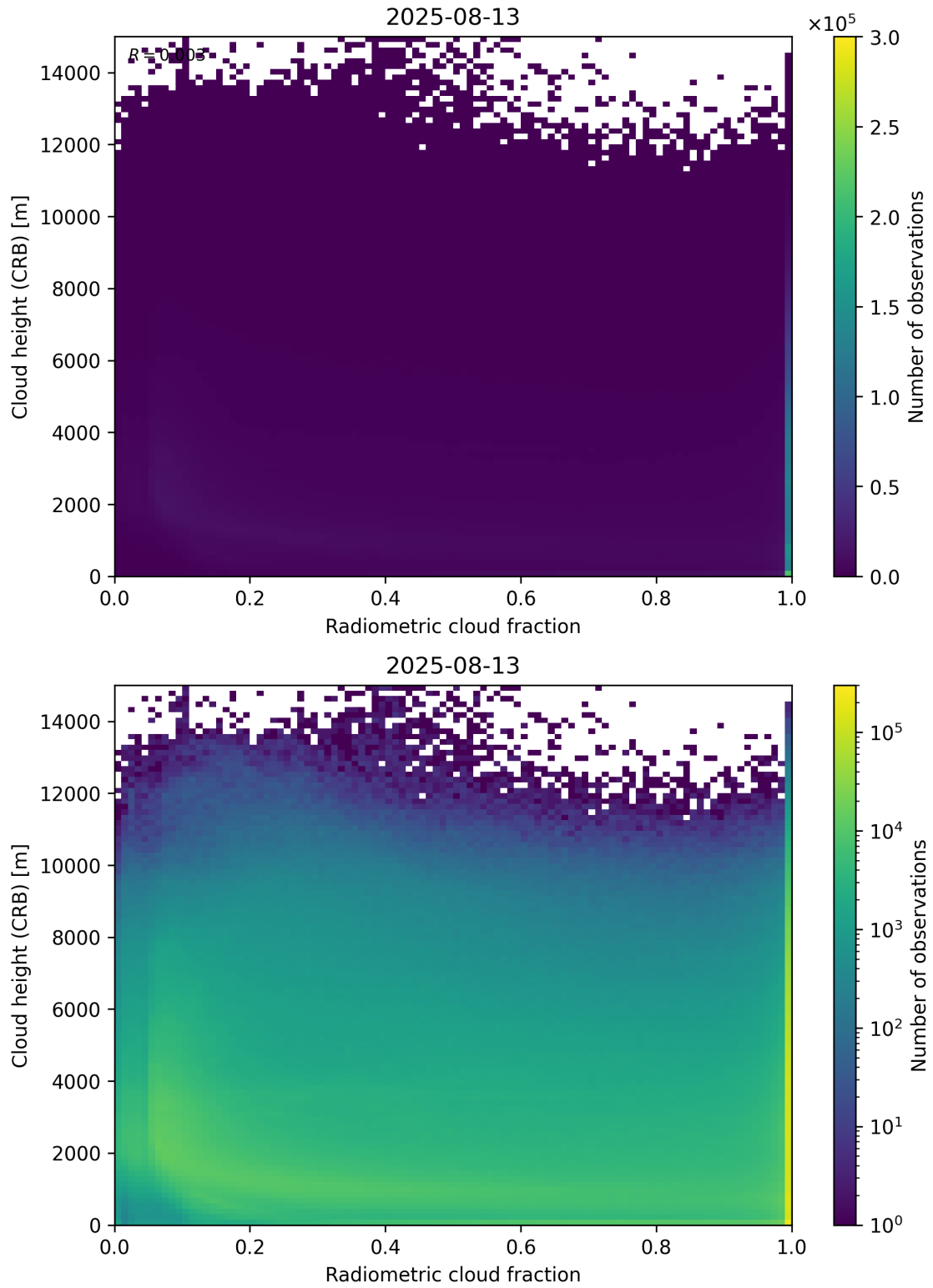
Figure 74: Scatter density plot of “Radiometric cloud fraction” against “Cloud height (CRB)” for 2025-08-12 to 2025-08-14.
