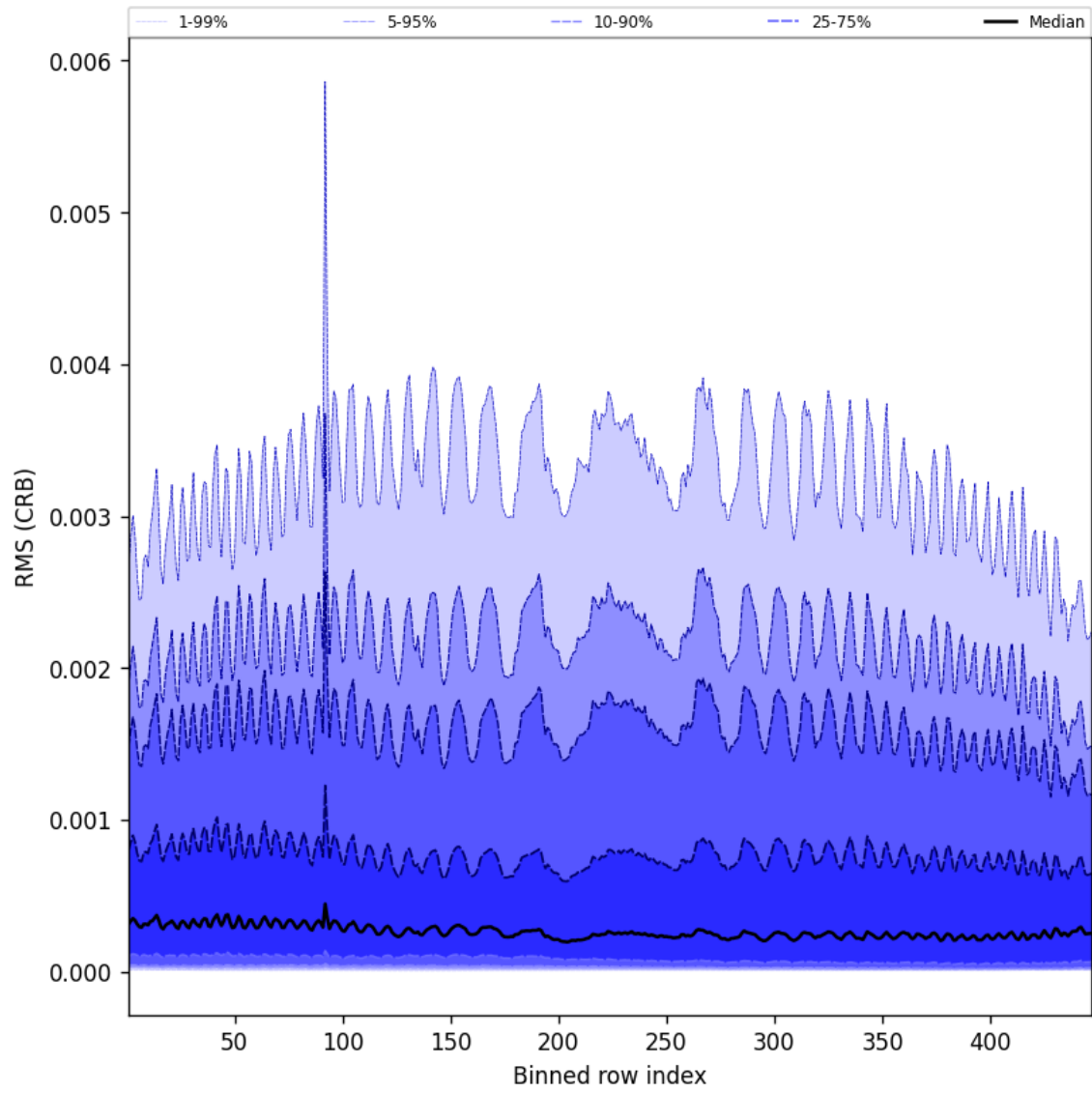
Figure 64: Along track statistics of “RMS (CRB)” for 2025-08-12 to 2025-08-14
