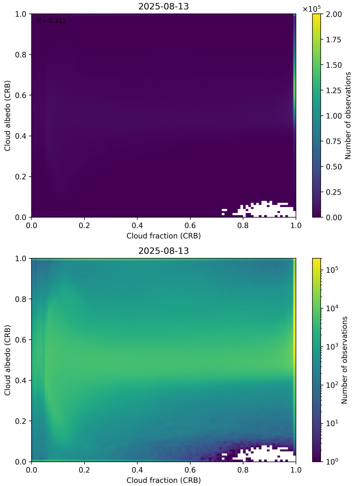
Figure 77: Scatter density plot of “Cloud fraction (CRB)” against “Cloud albedo (CRB)” for 2025-08-12 to 2025-08-14.
