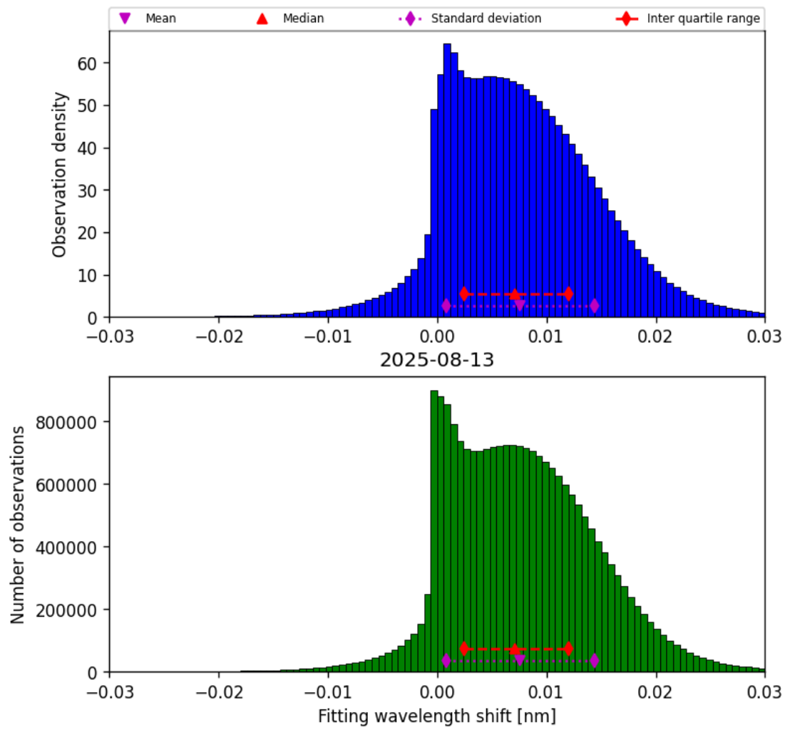
Figure 49: Histogram of “Fitting wavelength shift” for 2025-08-12 to 2025-08-14
