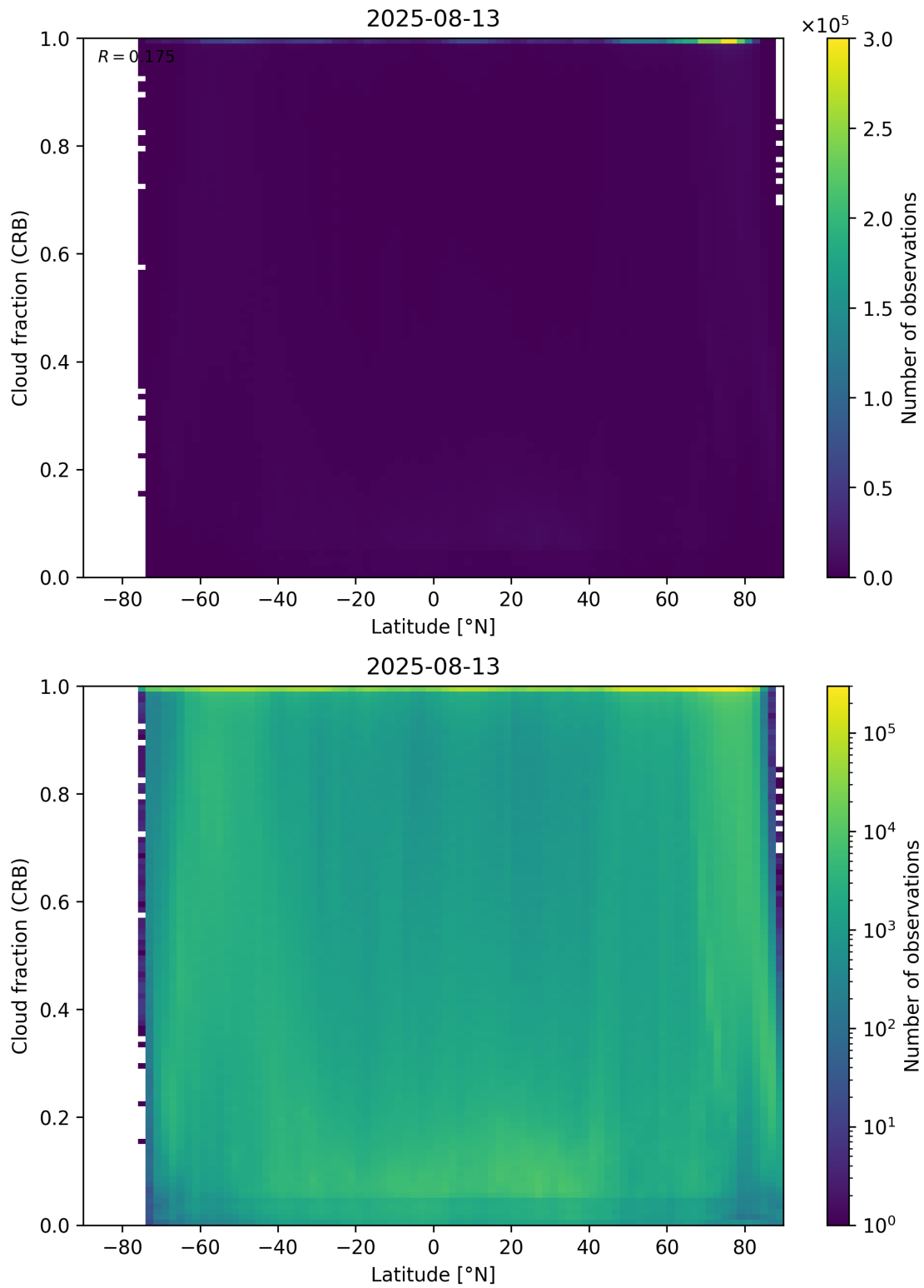
Figure 94: Scatter density plot of “Latitude” against “Cloud fraction (CRB)” for 2025-08-12 to 2025-08-14.
