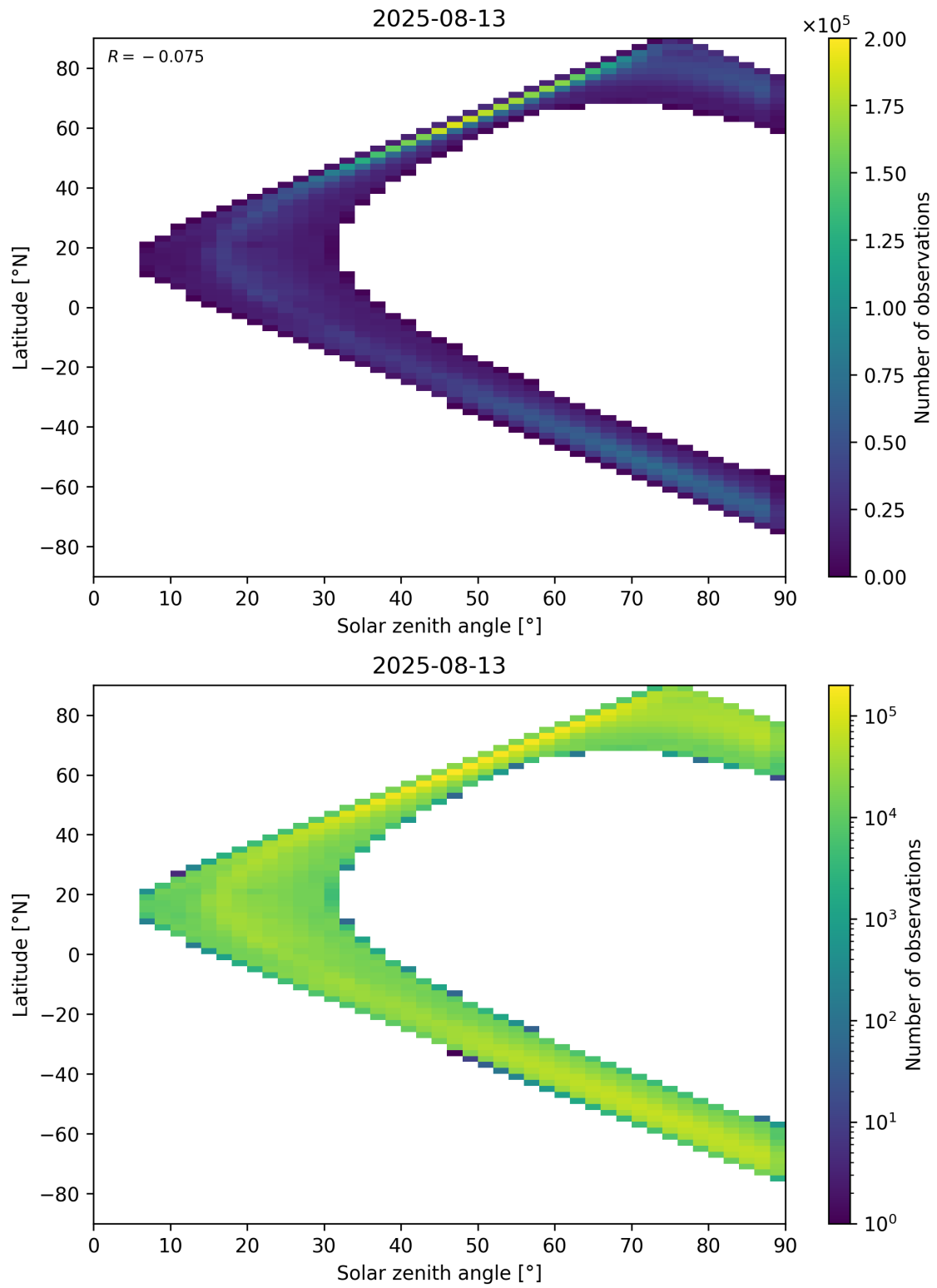
Figure 105: Scatter density plot of “Solar zenith angle” against “Latitude” for 2025-08-12 to 2025-08-14.
