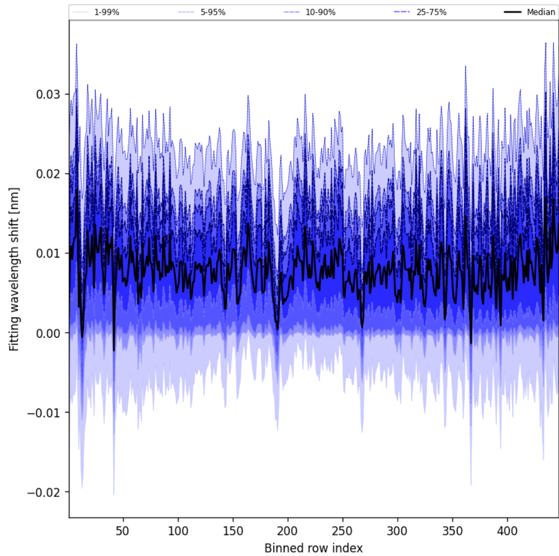
Figure 65: Along track statistics of “Fitting wavelength shift” for 2025-08-12 to 2025-08-14
