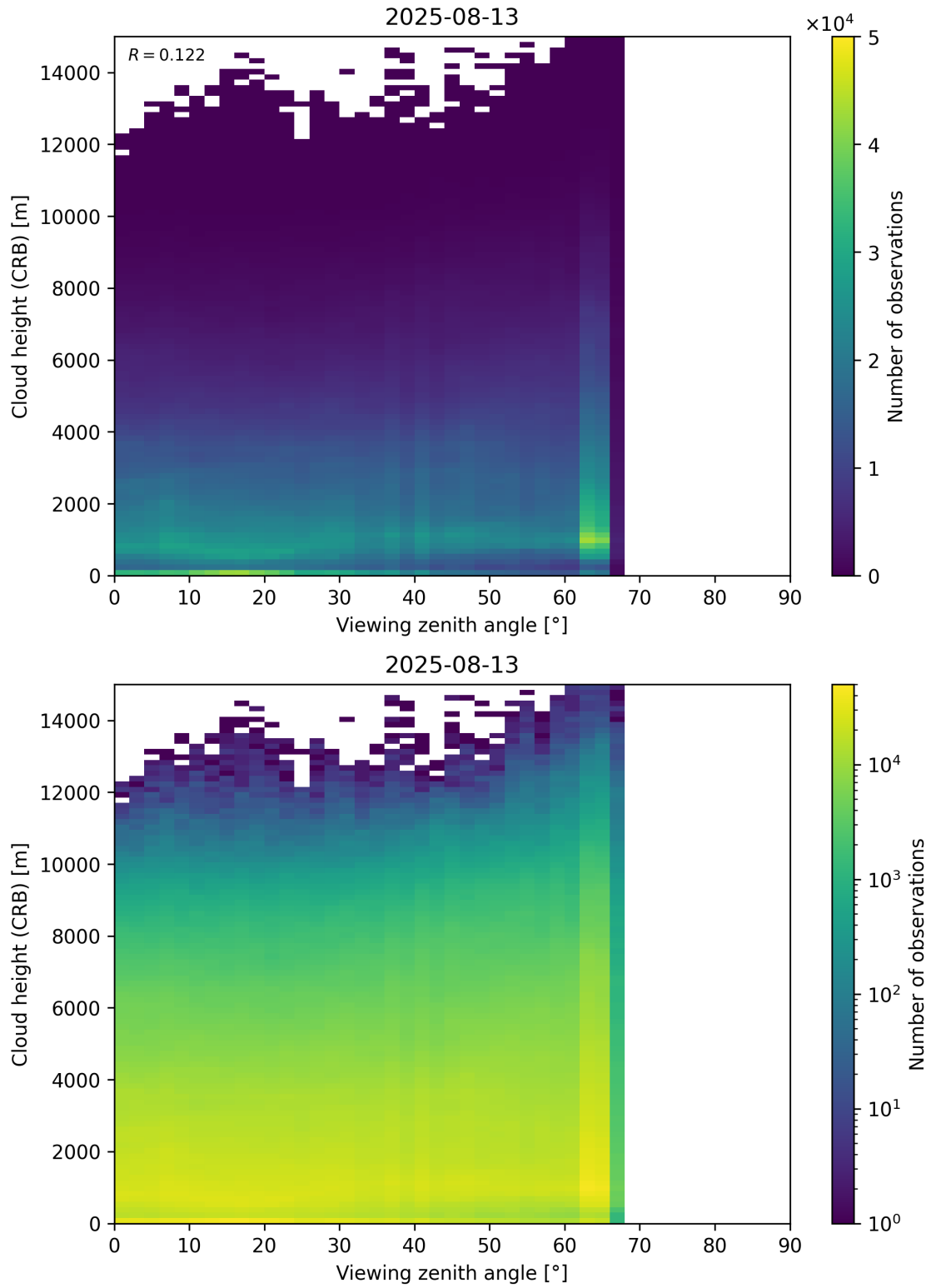
Figure 110: Scatter density plot of “Viewing zenith angle” against “Cloud height (CRB)” for 2025-08-12 to 2025-08-14.
