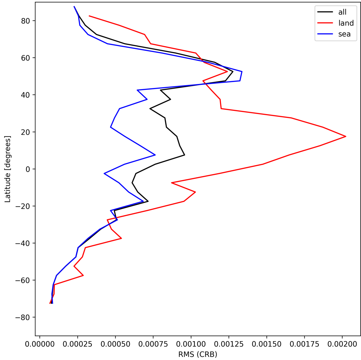
Figure 32: Zonal average of “RMS (CRB)” for 2025-08-12 to 2025-08-14.
