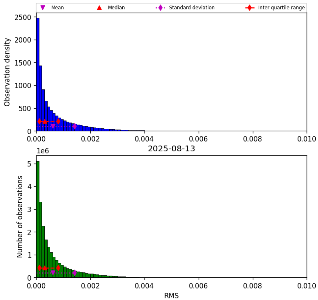
Figure 47: Histogram of “RMS” for 2025-08-12 to 2025-08-14
