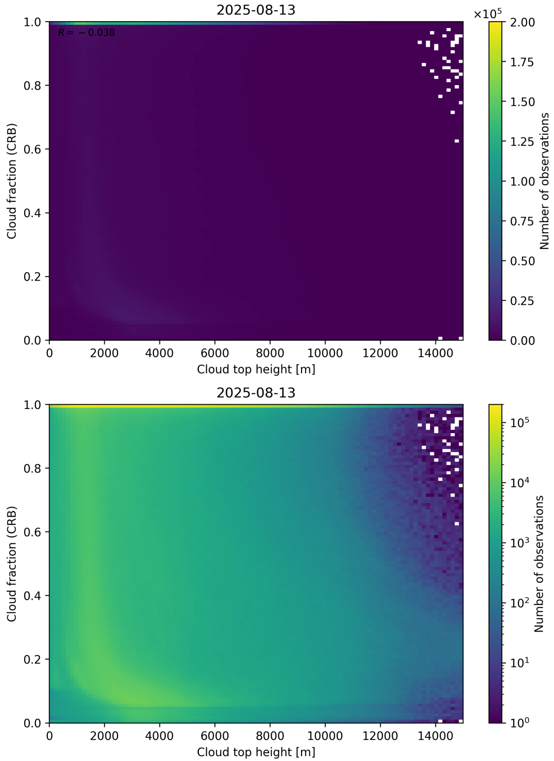
Figure 88: Scatter density plot of “Cloud top height” against “Cloud fraction (CRB)” for 2025-08-12 to 2025-08-14.
