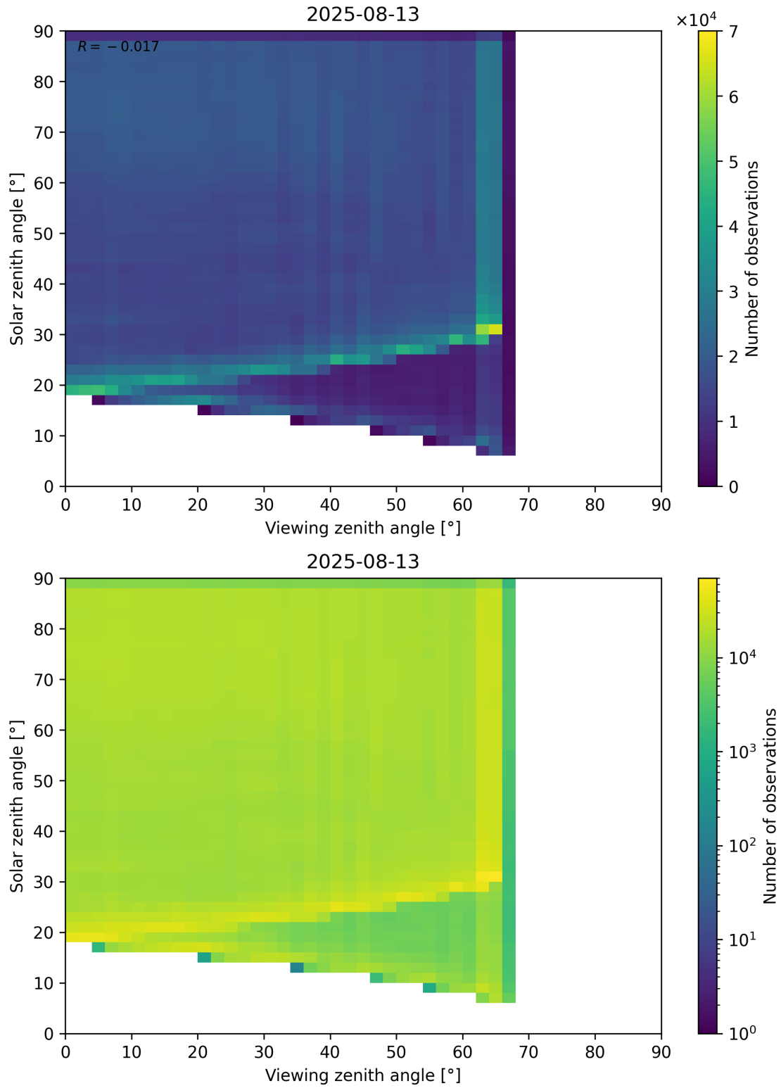
Figure 114: Scatter density plot of “Viewing zenith angle” against “Solar zenith angle” for 2025-08-12 to 2025-08-14.
