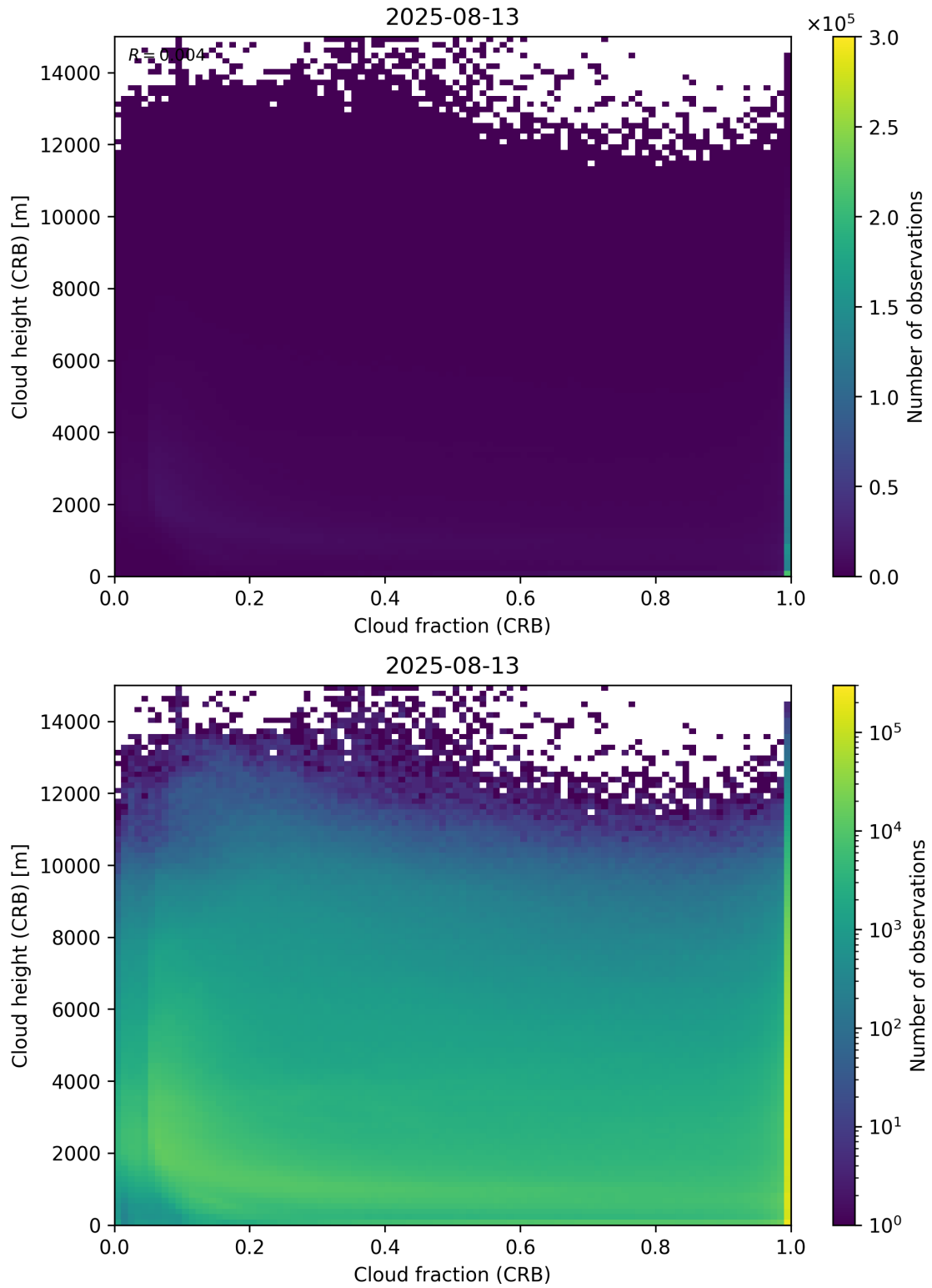
Figure 79: Scatter density plot of “Cloud fraction (CRB)” against “Cloud height (CRB)” for 2025-08-12 to 2025-08-14.
