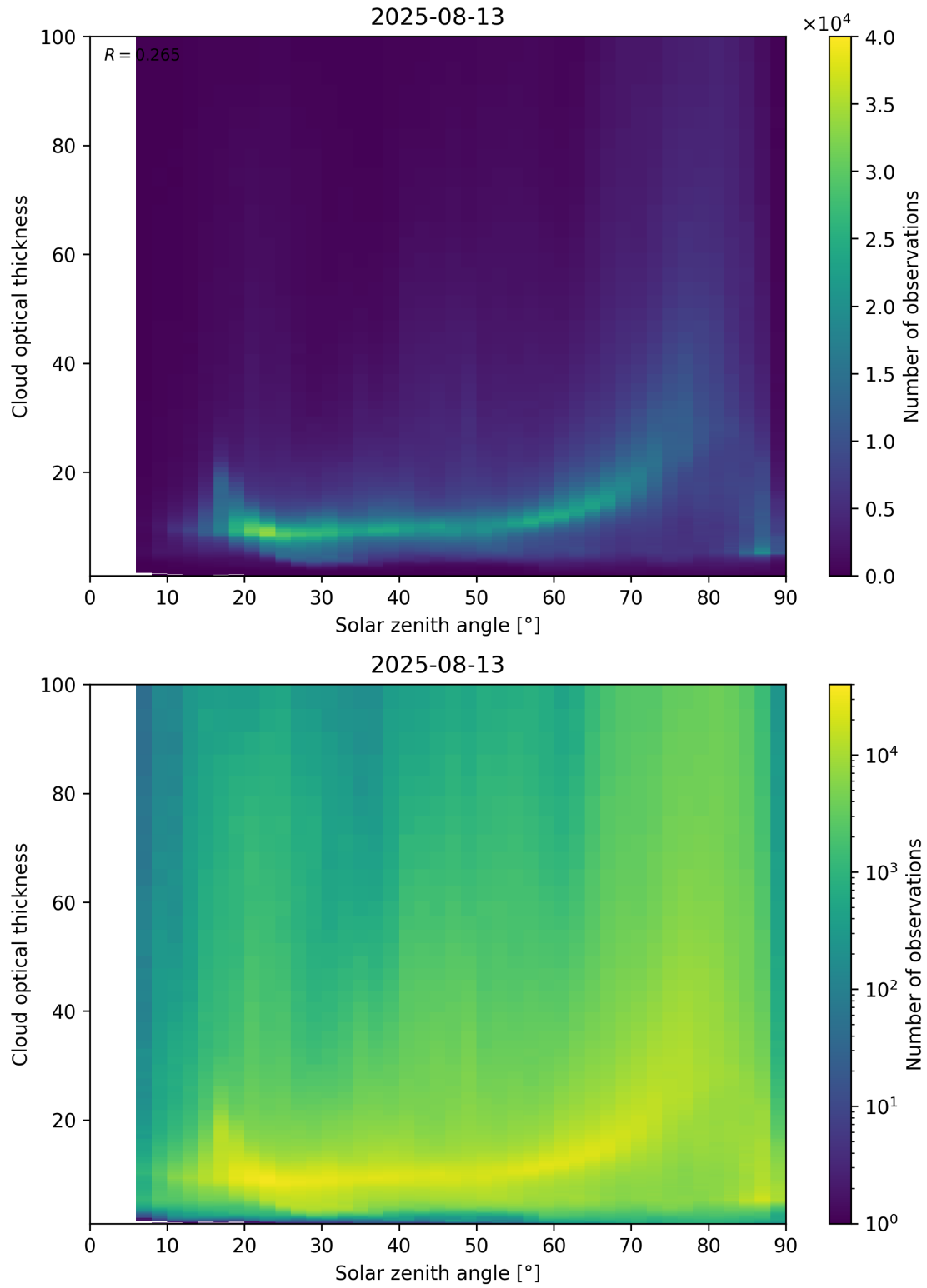
Figure 103: Scatter density plot of “Solar zenith angle” against “Cloud optical thickness” for 2025-08-12 to 2025-08-14.
