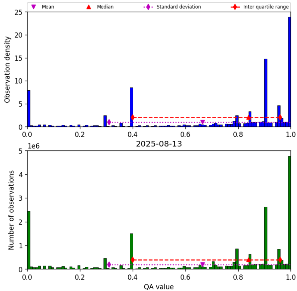
Figure 38: Histogram of “QA value” for 2025-08-12 to 2025-08-14
