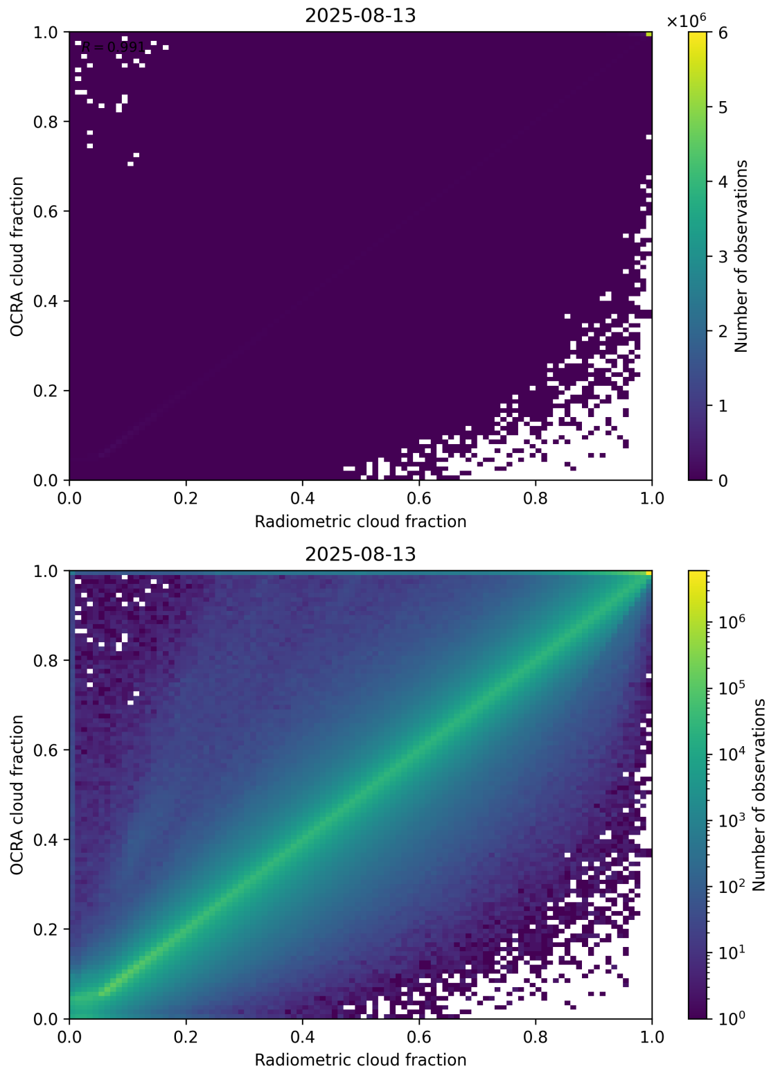
Figure 72: Scatter density plot of “Radiometric cloud fraction” against “OCRA cloud fraction” for 2025-08-12 to 2025-08-14.
