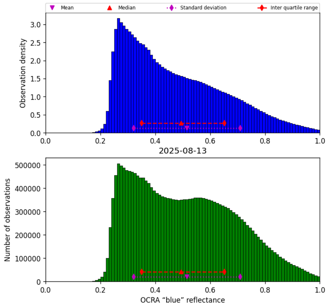
Figure 51: Histogram of “OCRA “blue” reflectance” for 2025-08-12 to 2025-08-14
