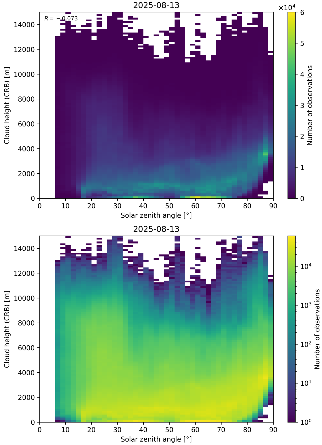
Figure 102: Scatter density plot of “Solar zenith angle” against “Cloud height (CRB)” for 2025-08-12 to 2025-08-14.
