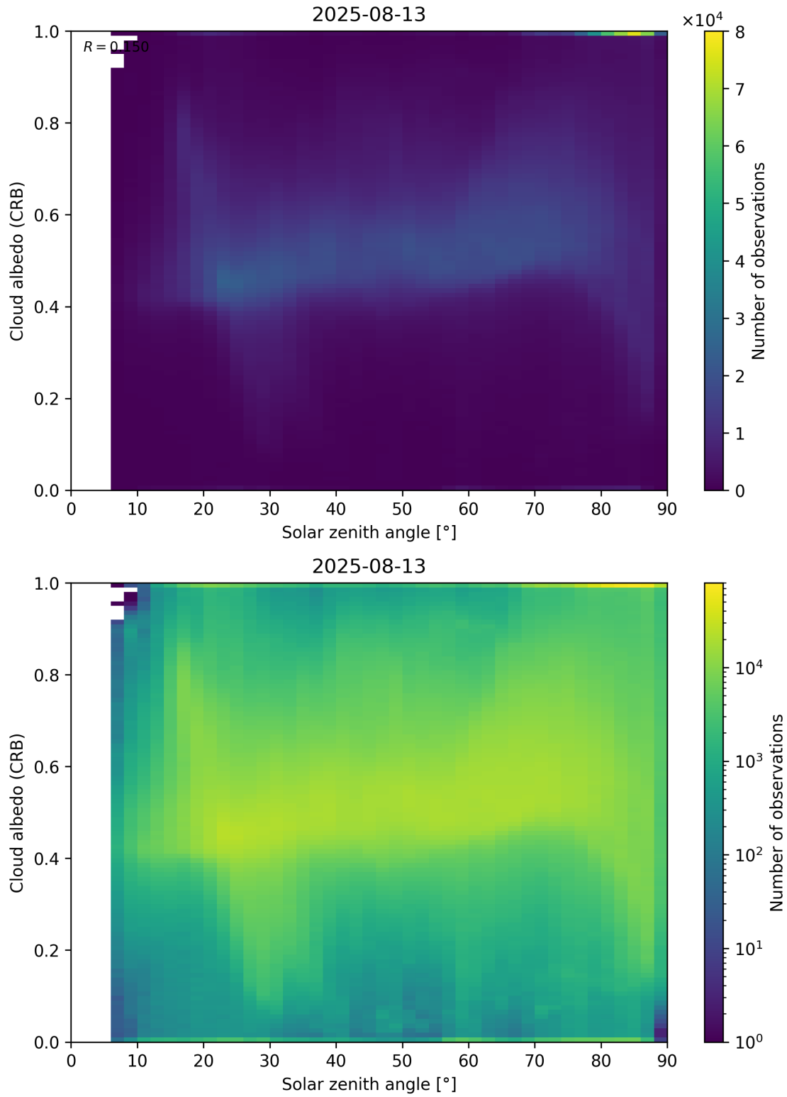
Figure 98: Scatter density plot of “Solar zenith angle” against “Cloud albedo (CRB)” for 2025-08-12 to 2025-08-14.
