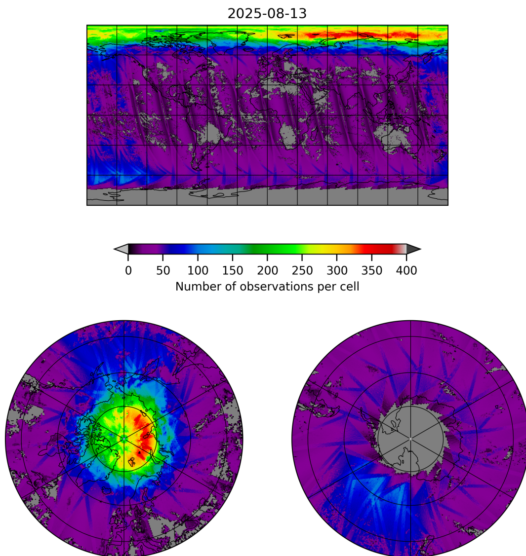
Figure 21: Map of the number of observations for 2025-08-12 to 2025-08-14
