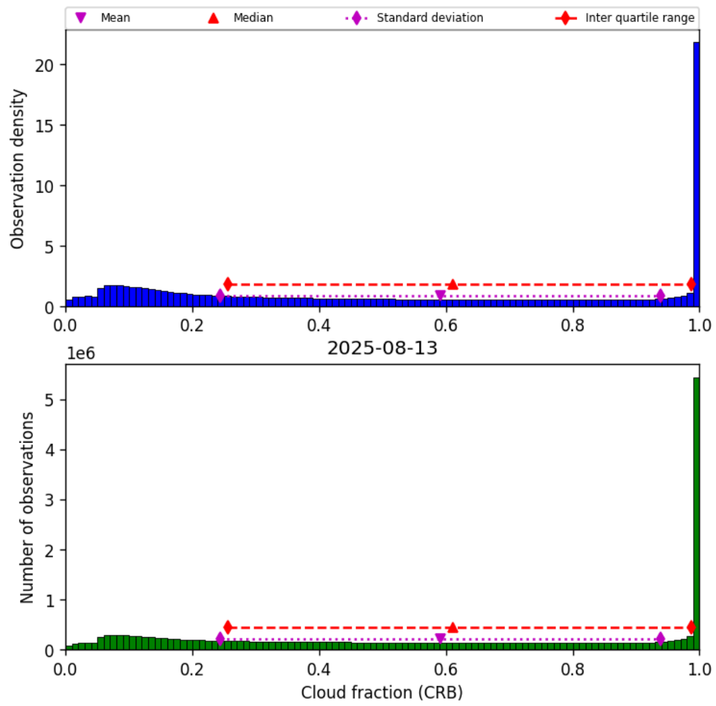
Figure 42: Histogram of “Cloud fraction (CRB)” for 2025-08-12 to 2025-08-14
