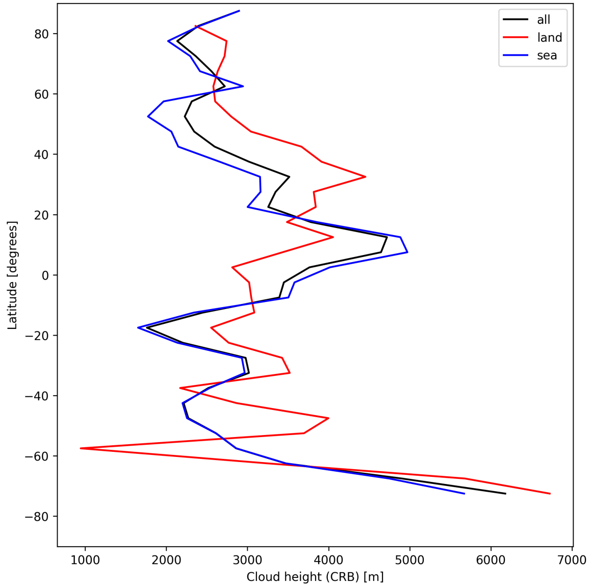
Figure 27: Zonal average of “Cloud height (CRB)” for 2025-08-12 to 2025-08-14.
