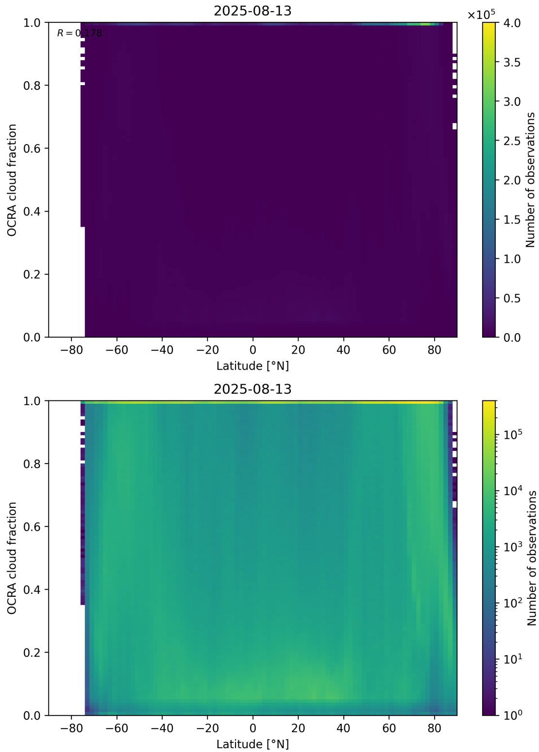
Figure 93: Scatter density plot of “Latitude” against “OCRA cloud fraction” for 2025-08-12 to 2025-08-14.
