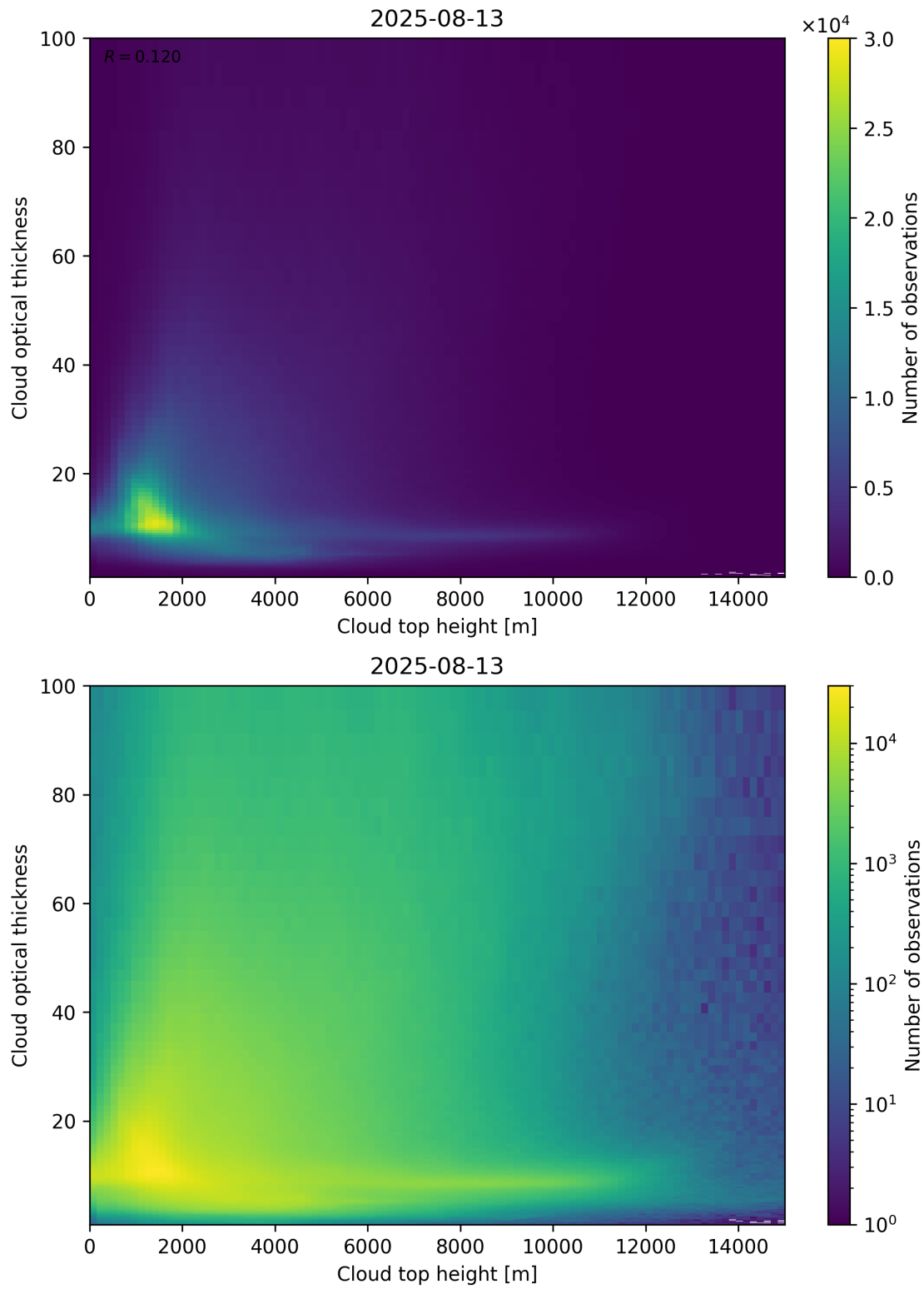
Figure 90: Scatter density plot of “Cloud top height” against “Cloud optical thickness” for 2025-08-12 to 2025-08-14.
