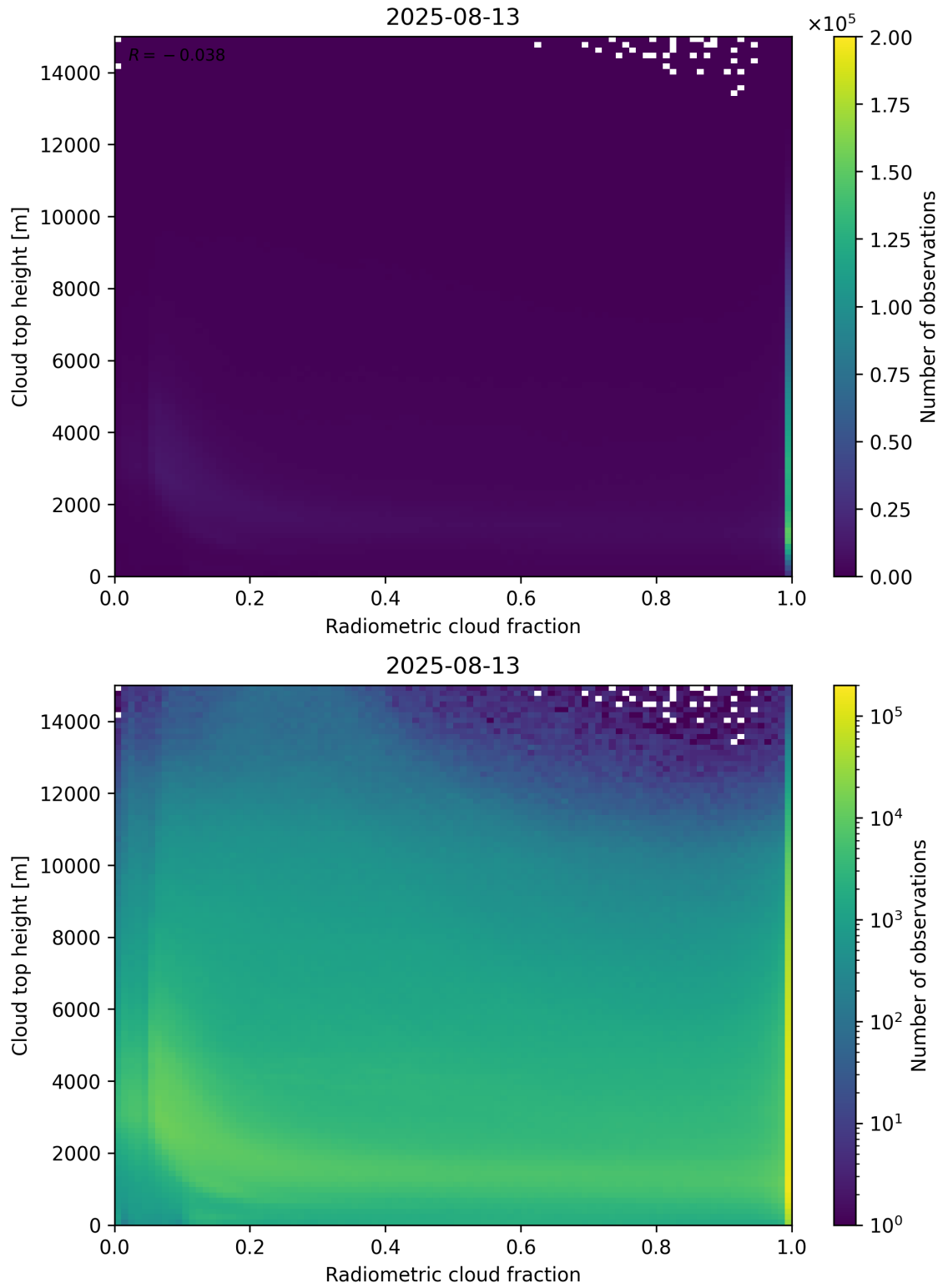
Figure 76: Scatter density plot of “Radiometric cloud fraction” against “Cloud top height” for 2025-08-12 to 2025-08-14.
