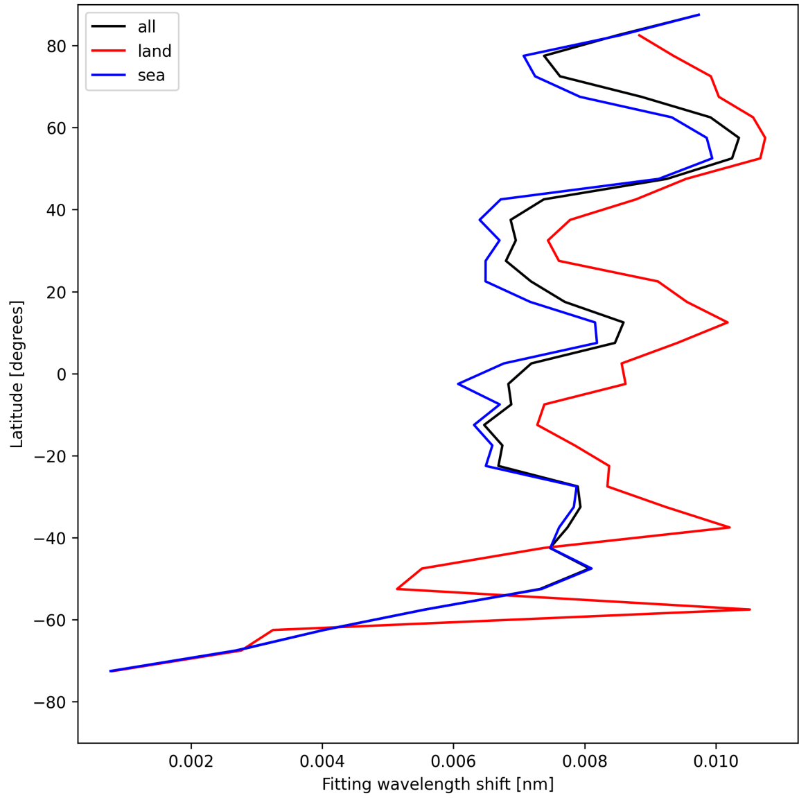
Figure 33: Zonal average of “Fitting wavelength shift” for 2025-08-12 to 2025-08-14.
