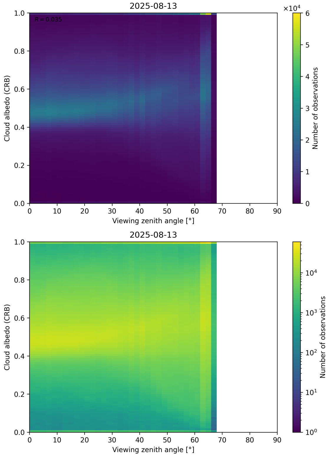
Figure 106: Scatter density plot of “Viewing zenith angle” against “Cloud albedo (CRB)” for 2025-08-12 to 2025-08-14.
