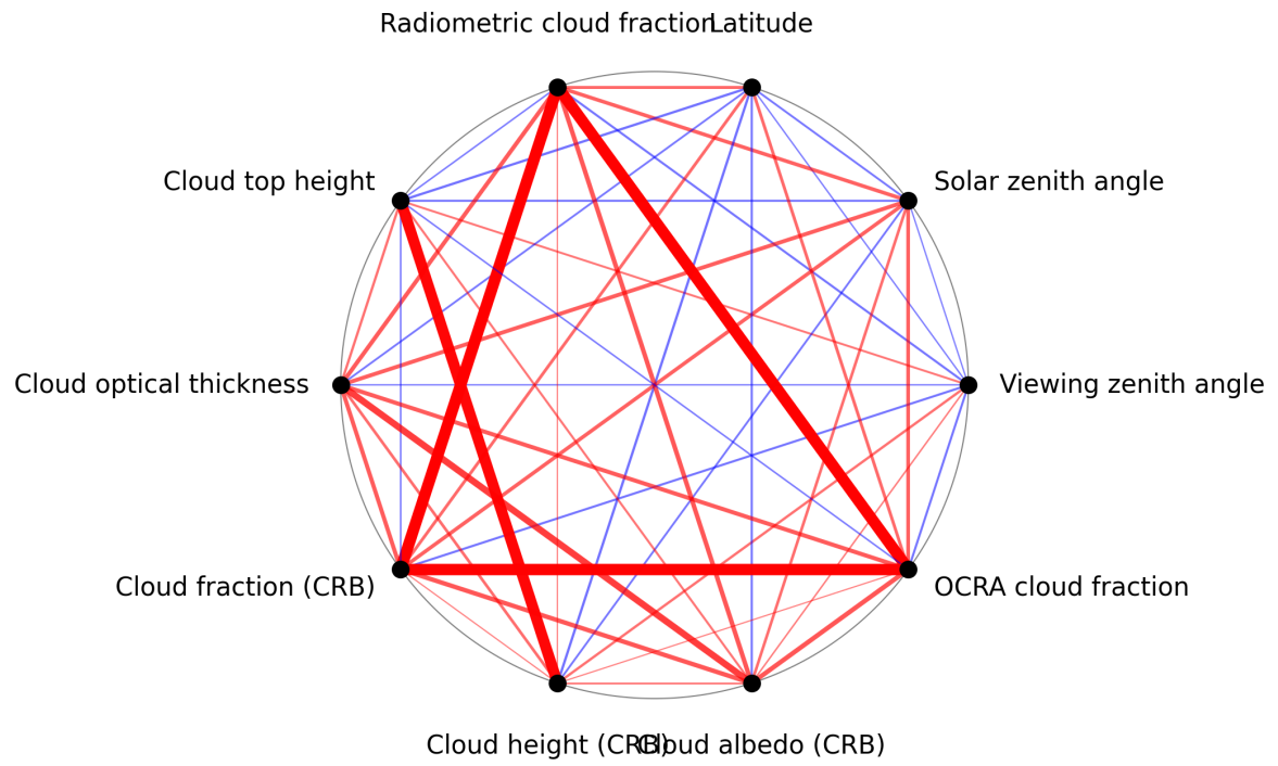
Figure 1: Map of correlation graph for 2025-08-12 to 2025-08-14.
