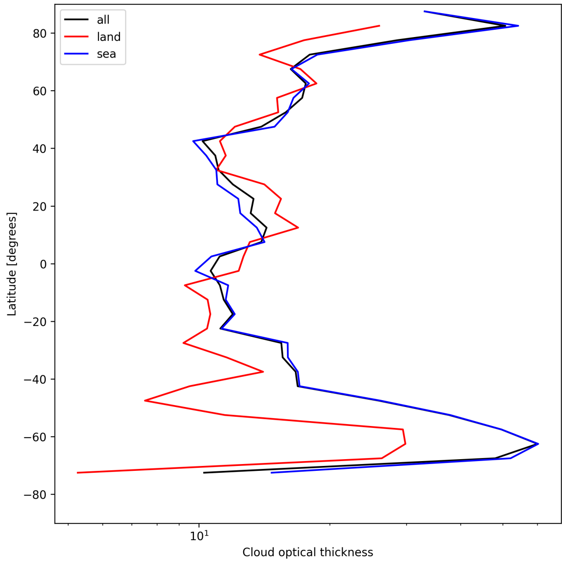
Figure 25: Zonal average of “Cloud optical thickness” for 2025-08-12 to 2025-08-14.
