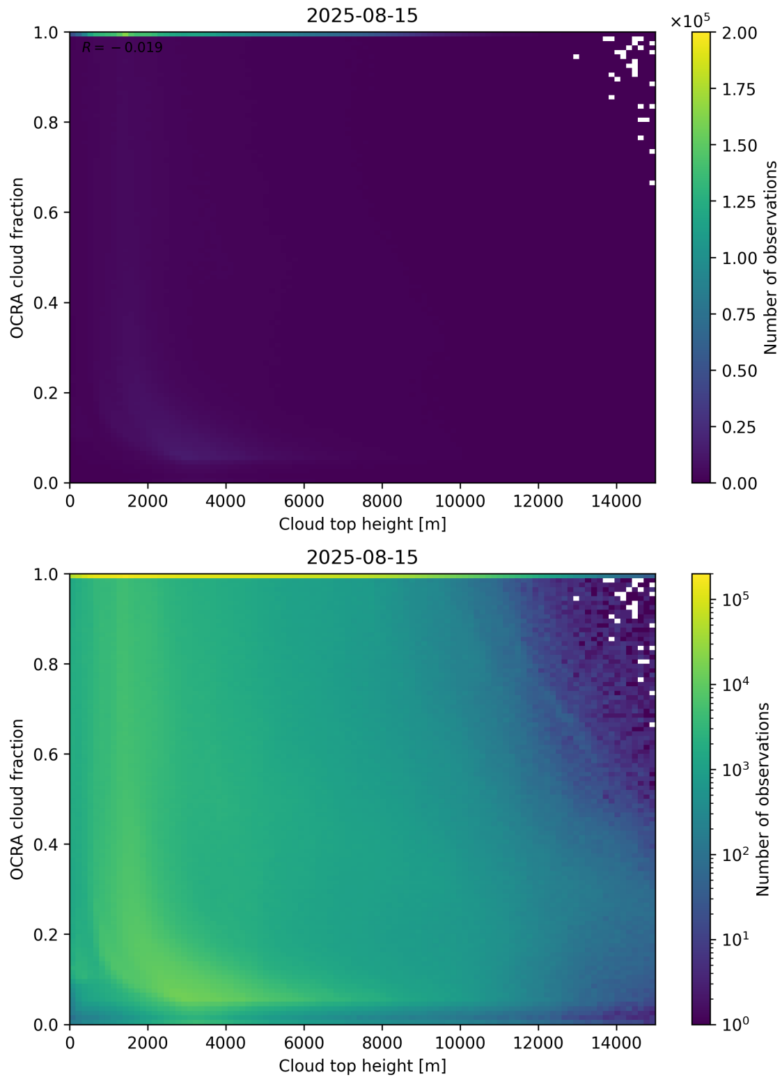
Figure 87: Scatter density plot of “Cloud top height” against “OCRA cloud fraction” for 2025-08-14 to 2025-08-16.
