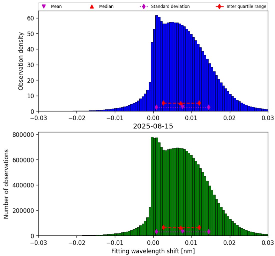
Figure 49: Histogram of “Fitting wavelength shift” for 2025-08-14 to 2025-08-16
