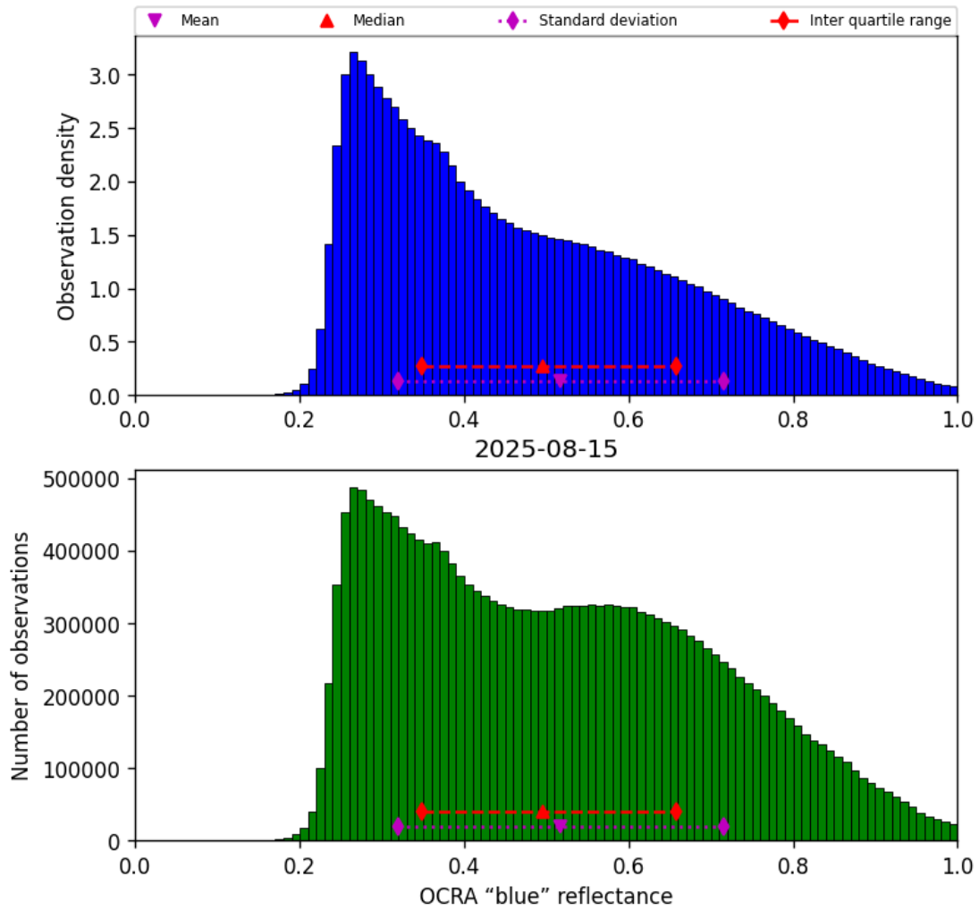
Figure 51: Histogram of “OCRA “blue” reflectance” for 2025-08-14 to 2025-08-16
