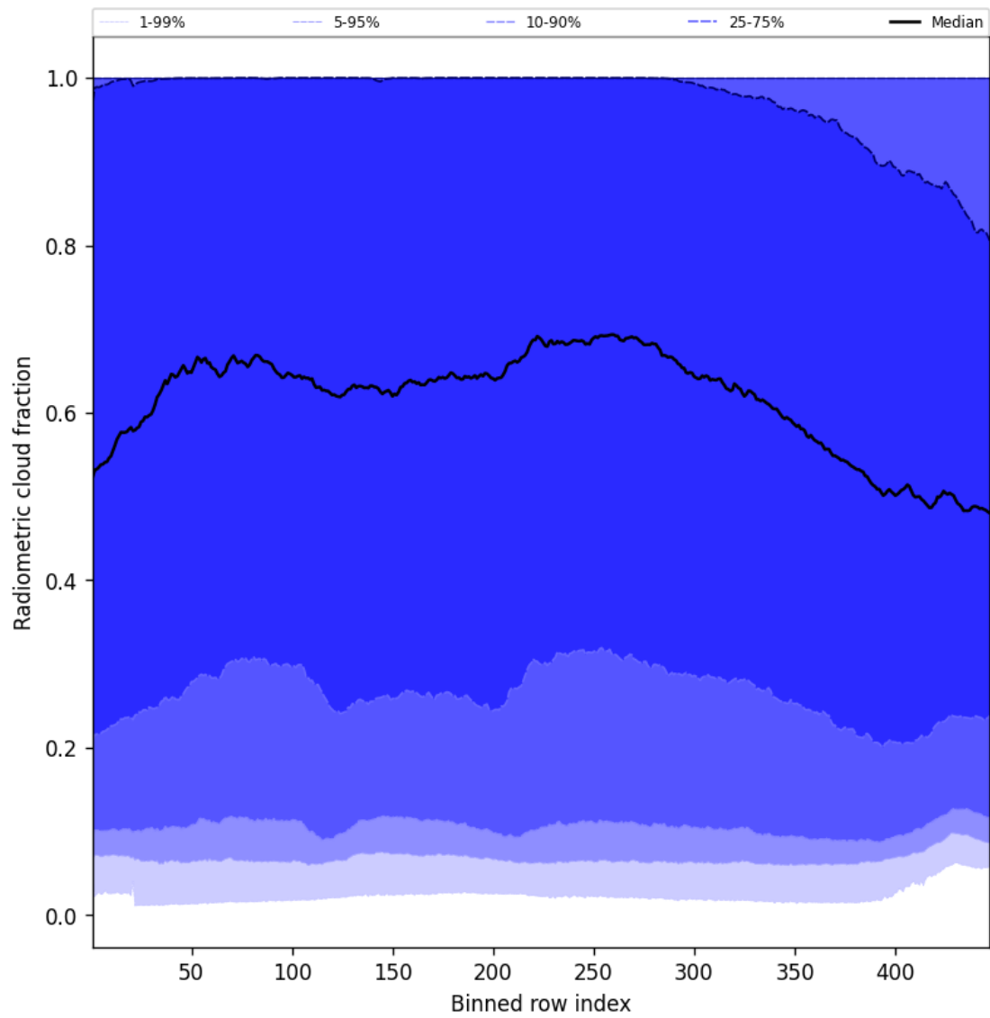
Figure 55: Along track statistics of “Radiometric cloud fraction” for 2025-08-14 to 2025-08-16
