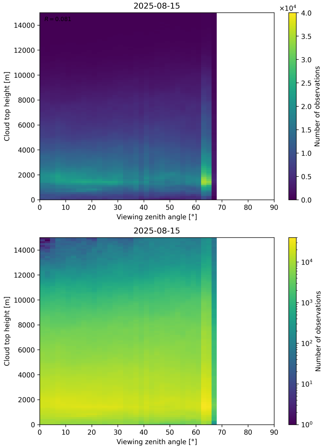
Figure 112: Scatter density plot of “Viewing zenith angle” against “Cloud top height” for 2025-08-14 to 2025-08-16.
