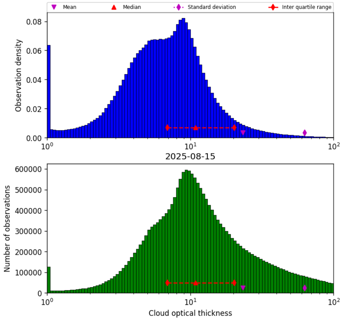
Figure 41: Histogram of “Cloud optical thickness” for 2025-08-14 to 2025-08-16
