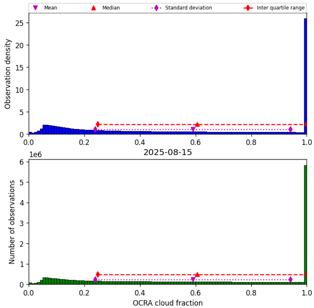
Figure 50: Histogram of “OCRA cloud fraction” for 2025-08-14 to 2025-08-16
