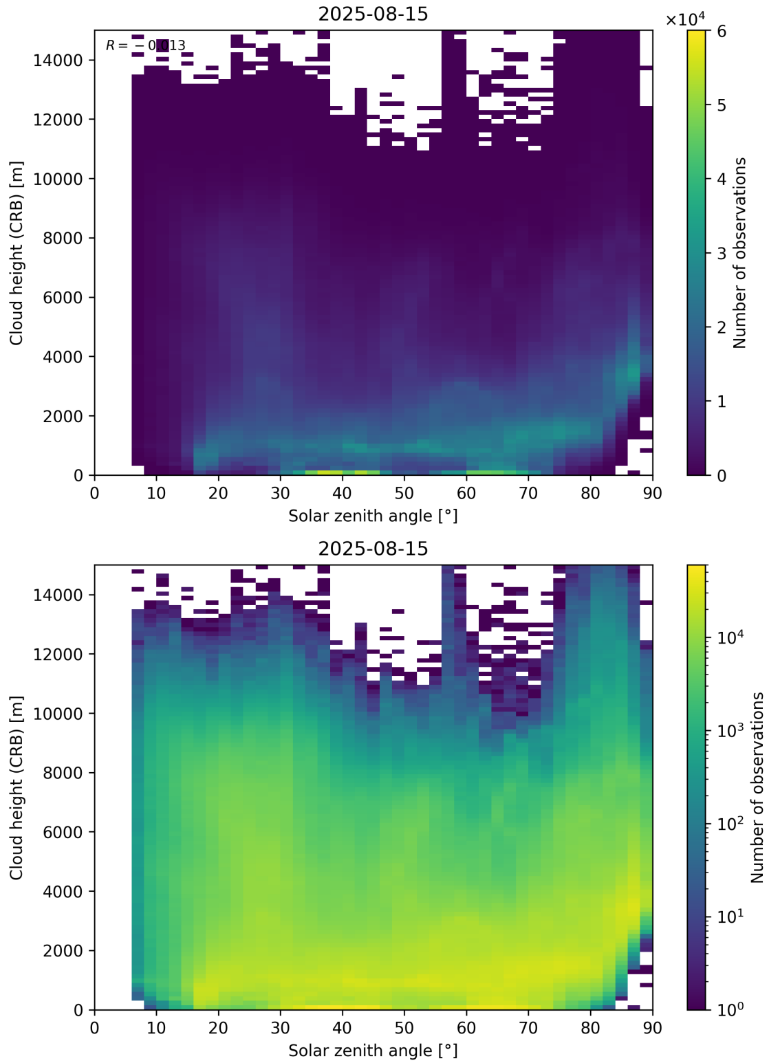
Figure 102: Scatter density plot of “Solar zenith angle” against “Cloud height (CRB)” for 2025-08-14 to 2025-08-16.
