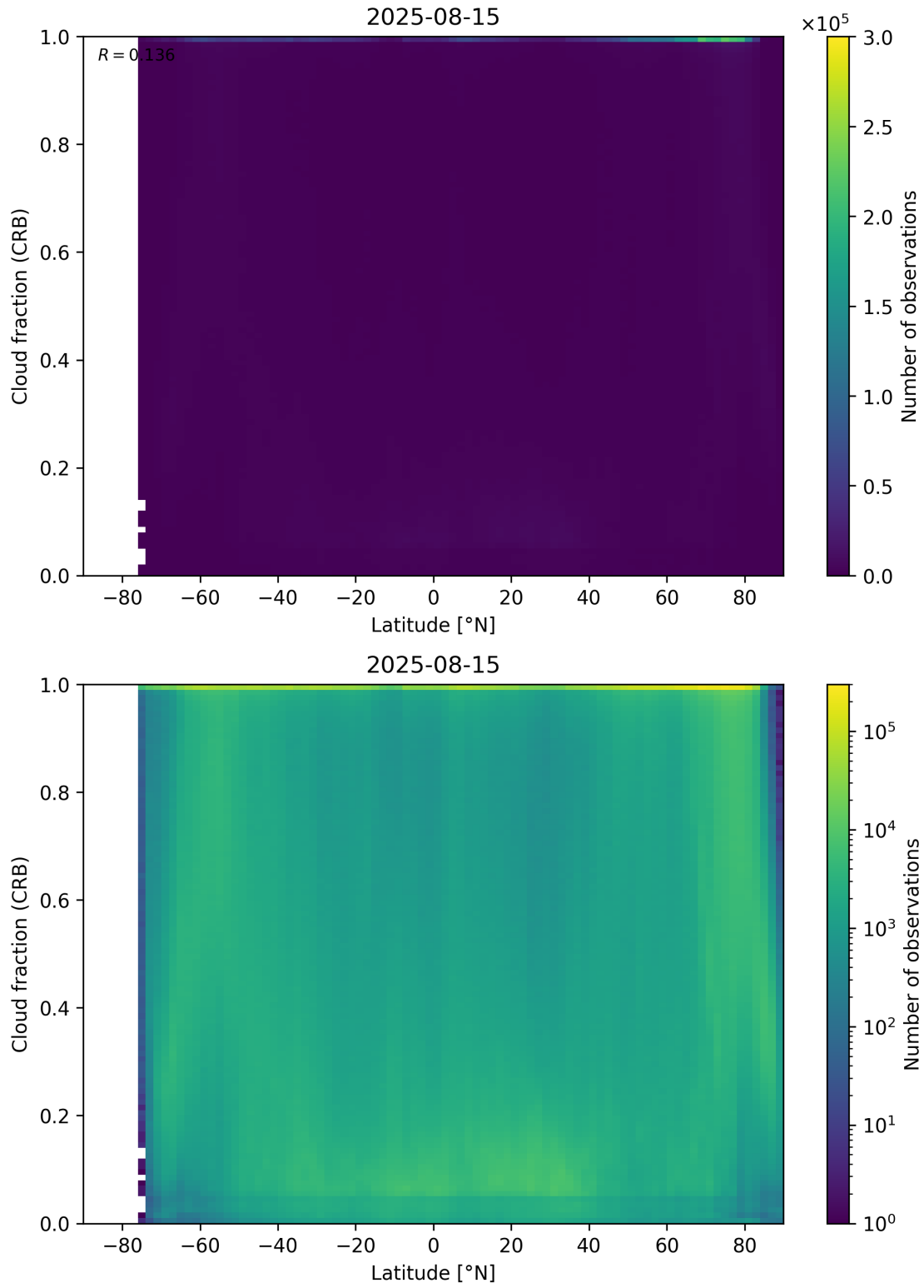
Figure 94: Scatter density plot of “Latitude” against “Cloud fraction (CRB)” for 2025-08-14 to 2025-08-16.
