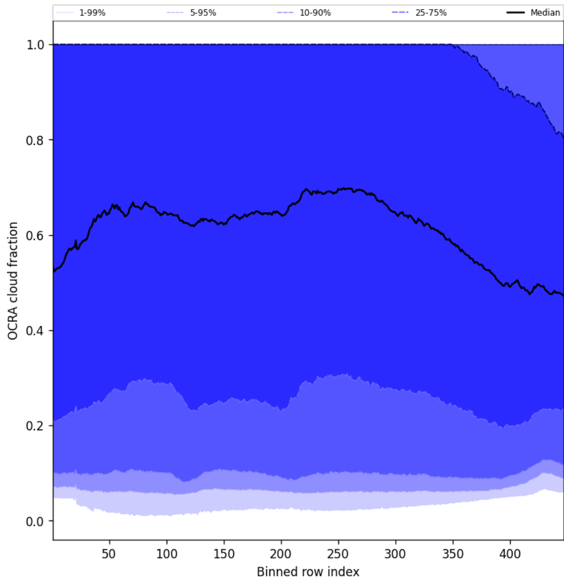
Figure 66: Along track statistics of “OCRA cloud fraction” for 2025-08-14 to 2025-08-16
