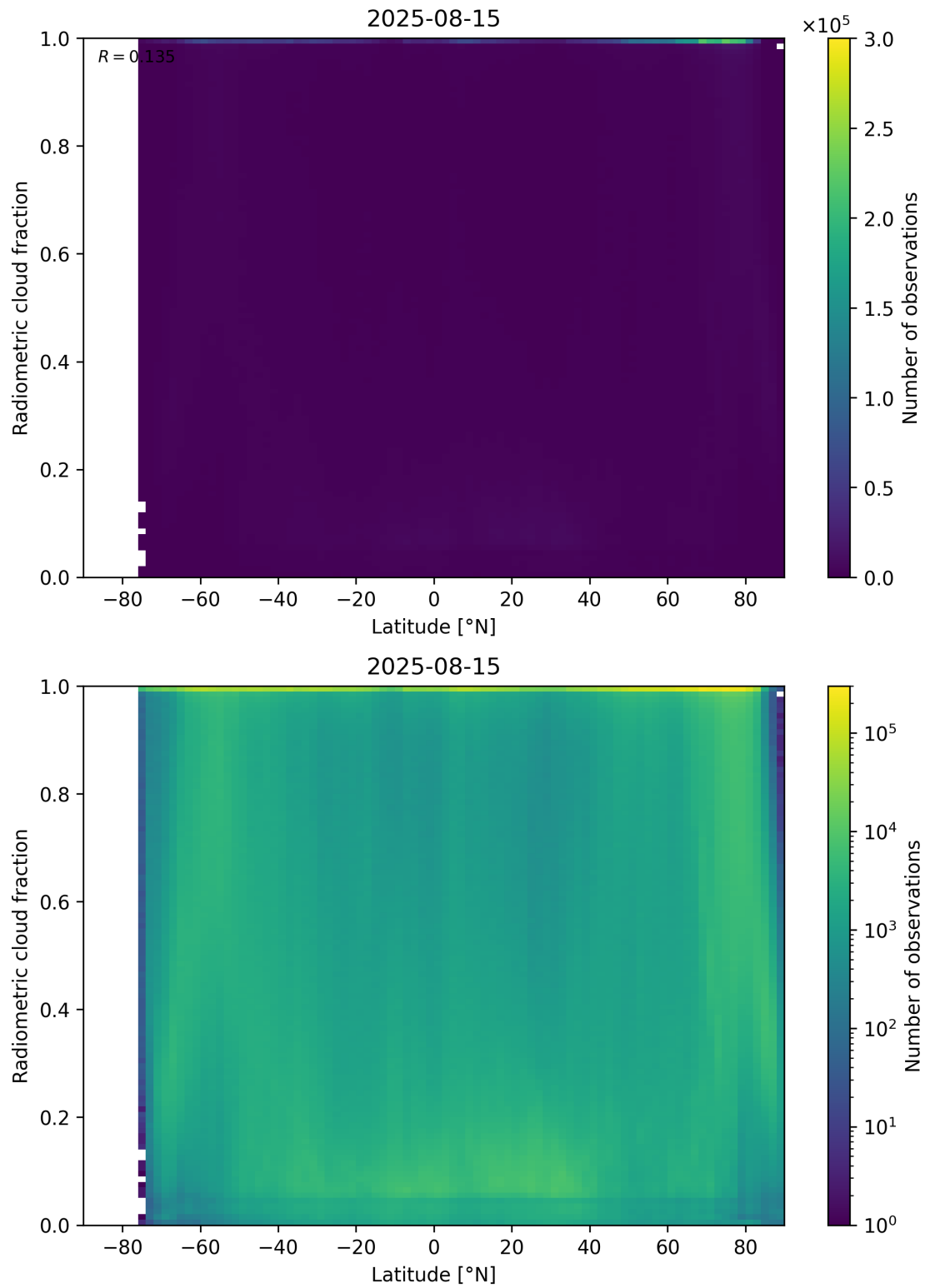
Figure 92: Scatter density plot of “Latitude” against “Radiometric cloud fraction” for 2025-08-14 to 2025-08-16.
