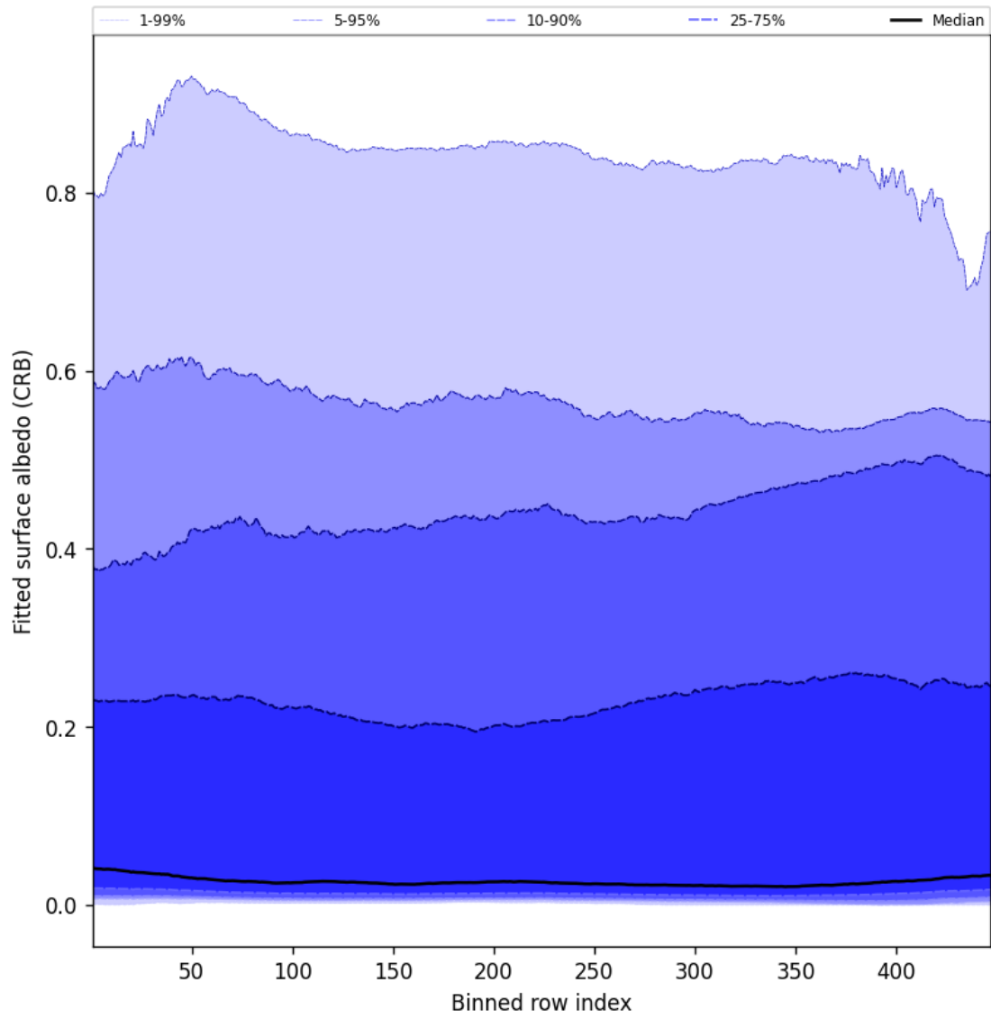
Figure 62: Along track statistics of “Fitted surface albedo (CRB)” for 2025-08-14 to 2025-08-16
