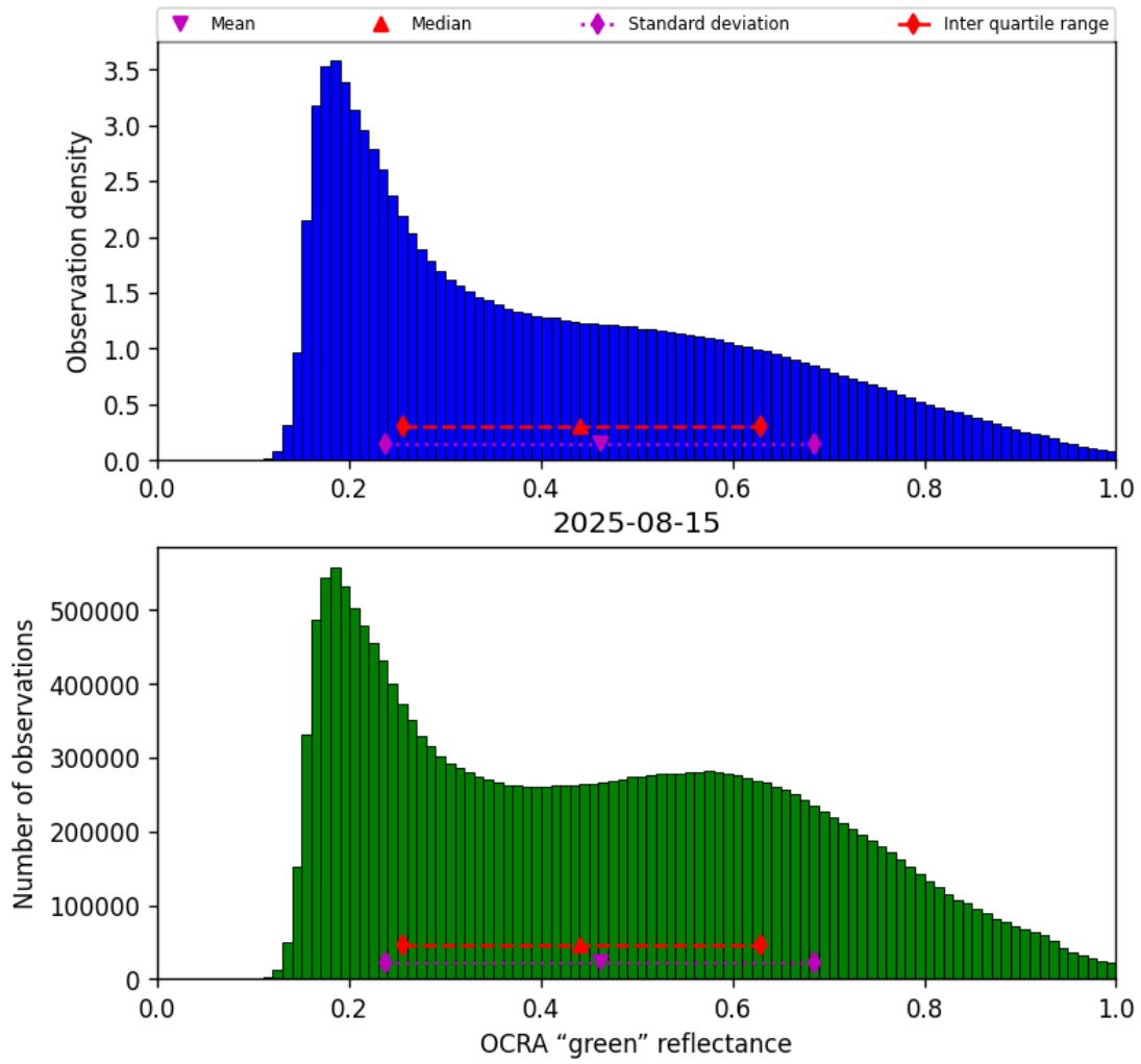
Figure 52: Histogram of “OCRA “green” reflectance” for 2025-08-14 to 2025-08-16
