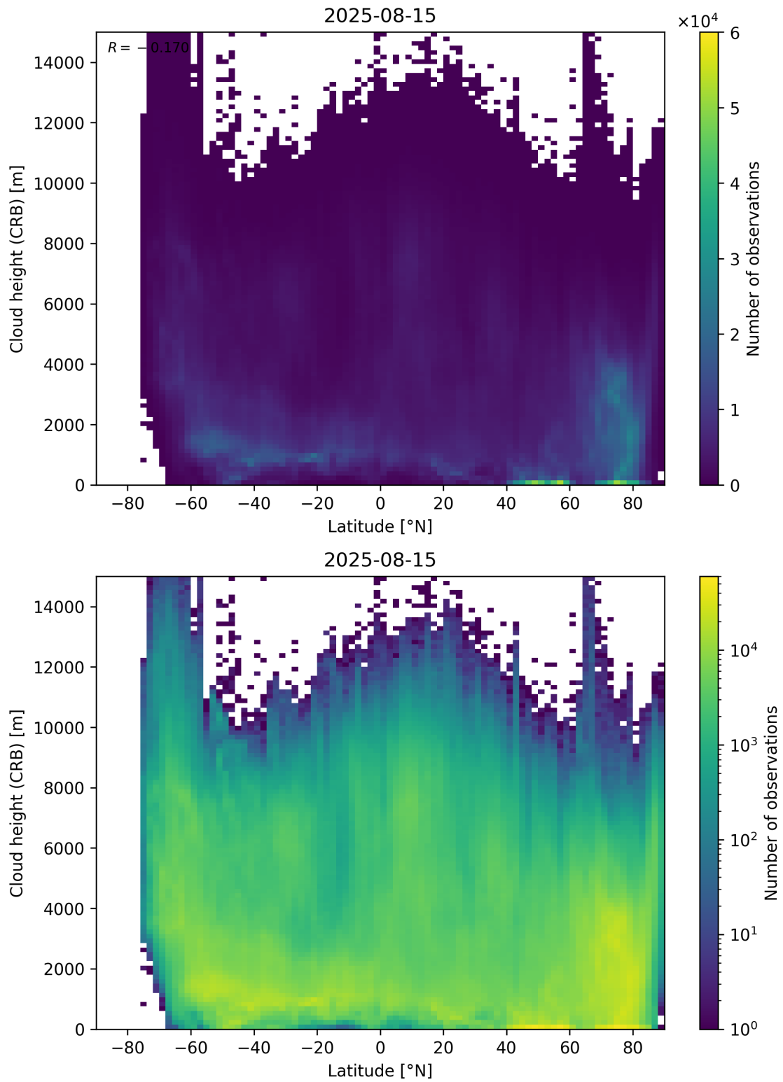
Figure 95: Scatter density plot of “Latitude” against “Cloud height (CRB)” for 2025-08-14 to 2025-08-16.
