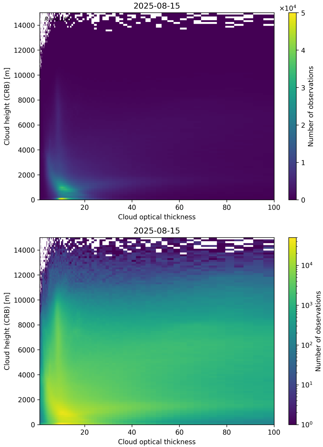
Figure 85: Scatter density plot of “Cloud optical thickness” against “Cloud height (CRB)” for 2025-08-14 to 2025-08-16.
