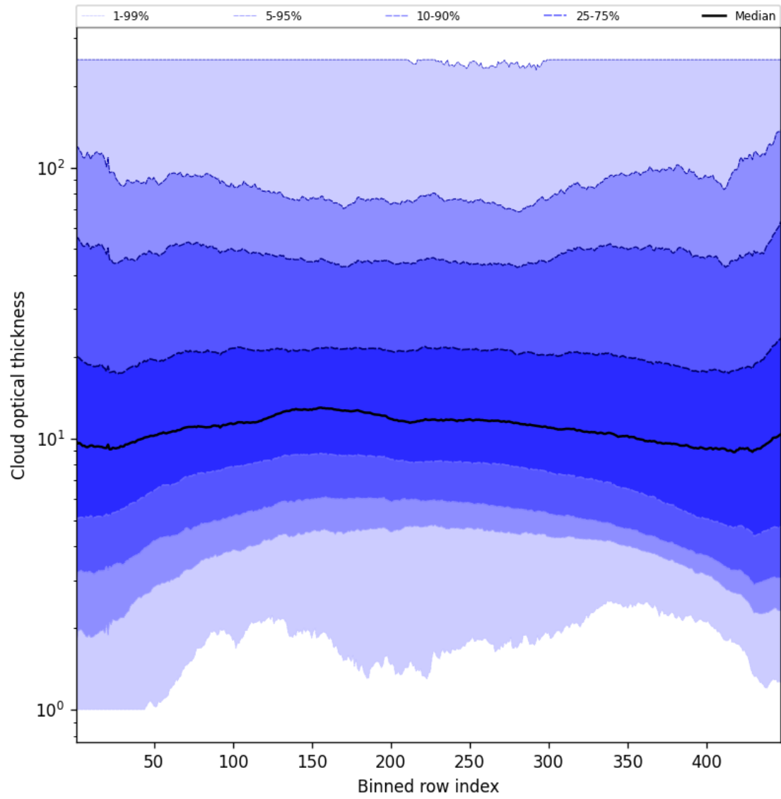
Figure 57: Along track statistics of “Cloud optical thickness” for 2025-08-14 to 2025-08-16
