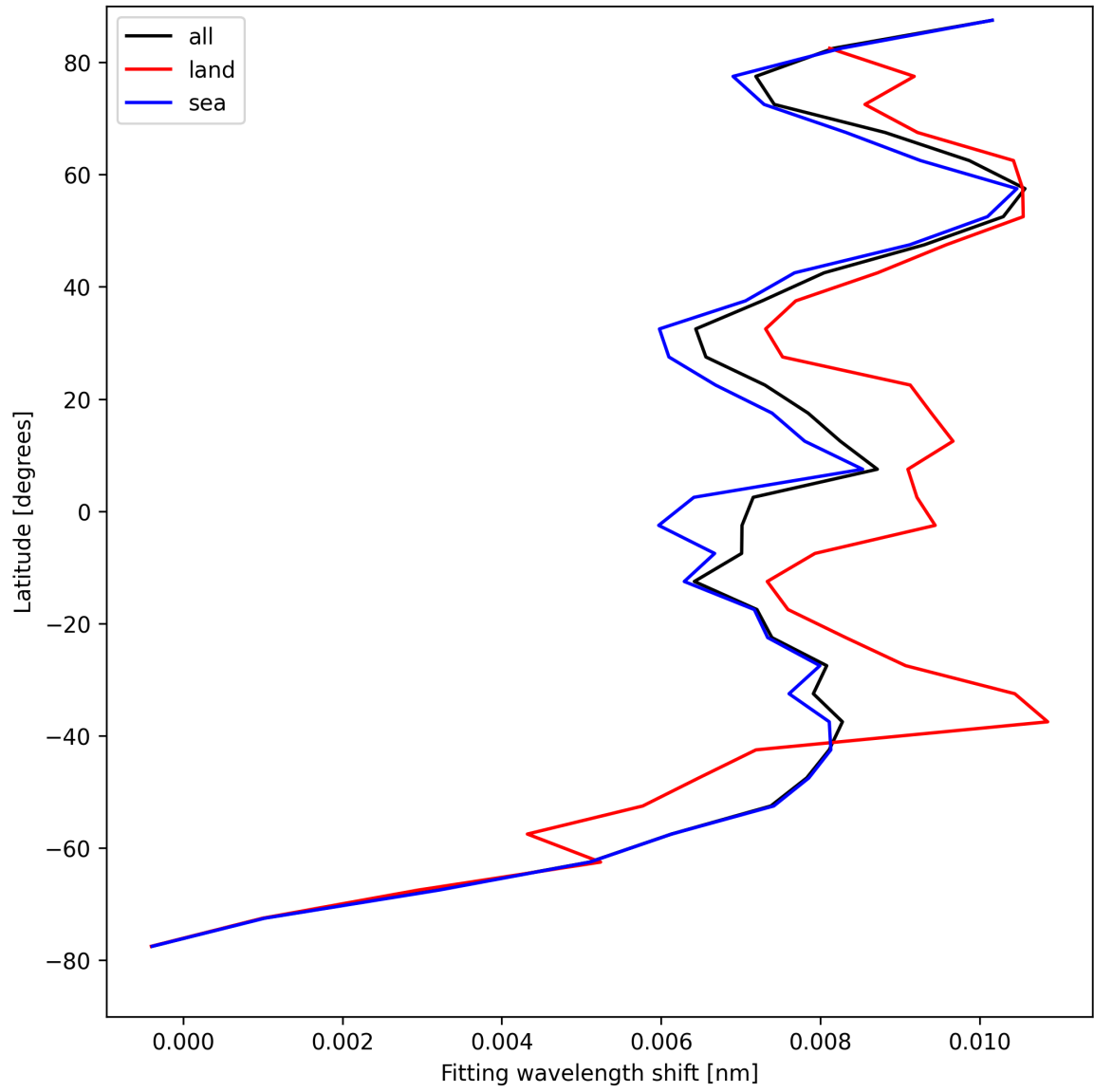
Figure 33: Zonal average of “Fitting wavelength shift” for 2025-08-14 to 2025-08-16.
