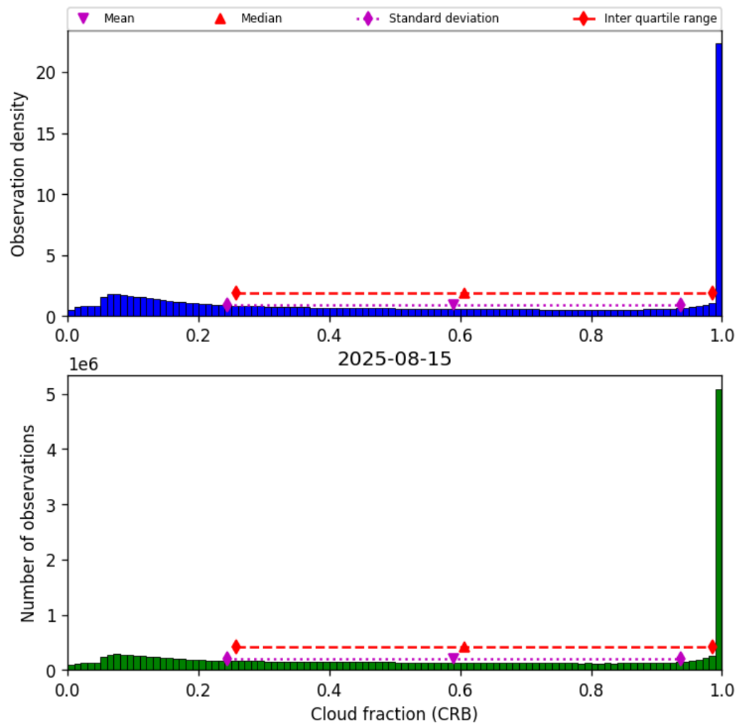
Figure 42: Histogram of “Cloud fraction (CRB)” for 2025-08-14 to 2025-08-16
