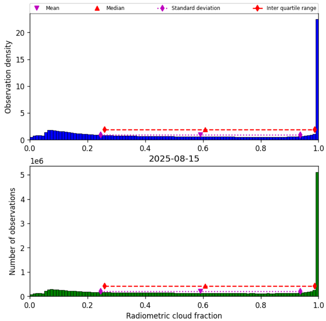
Figure 39: Histogram of “Radiometric cloud fraction” for 2025-08-14 to 2025-08-16
