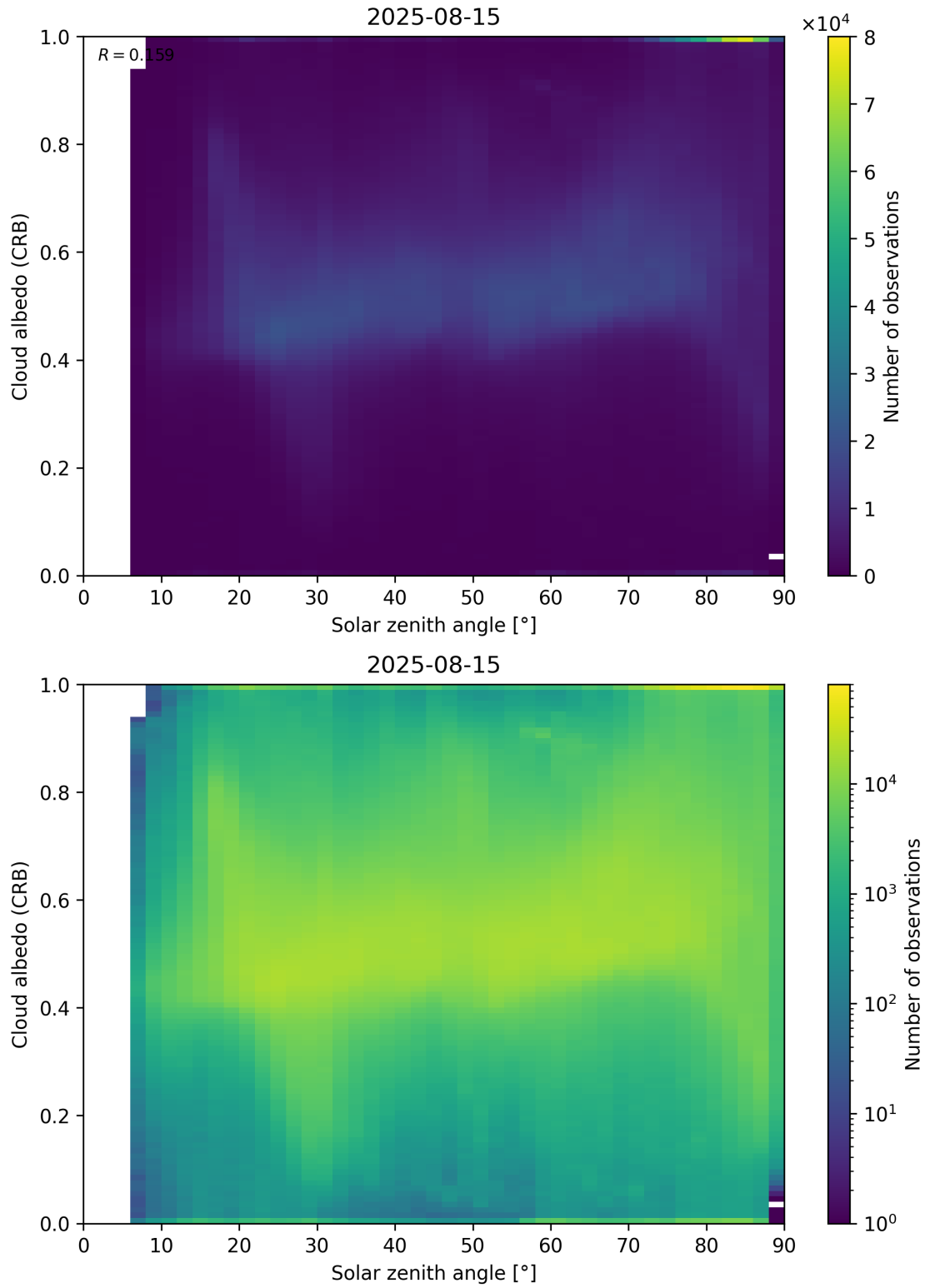
Figure 98: Scatter density plot of “Solar zenith angle” against “Cloud albedo (CRB)” for 2025-08-14 to 2025-08-16.
