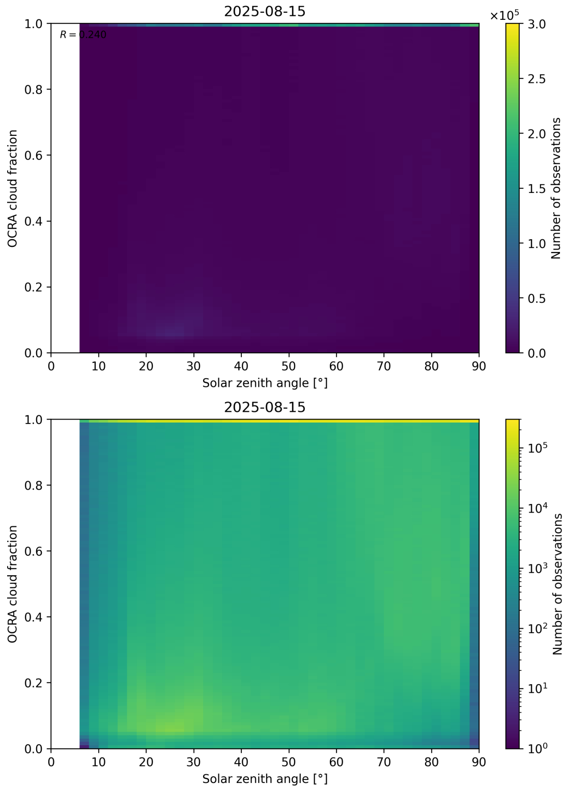
Figure 100: Scatter density plot of “Solar zenith angle” against “OCRA cloud fraction” for 2025-08-14 to 2025-08-16.
