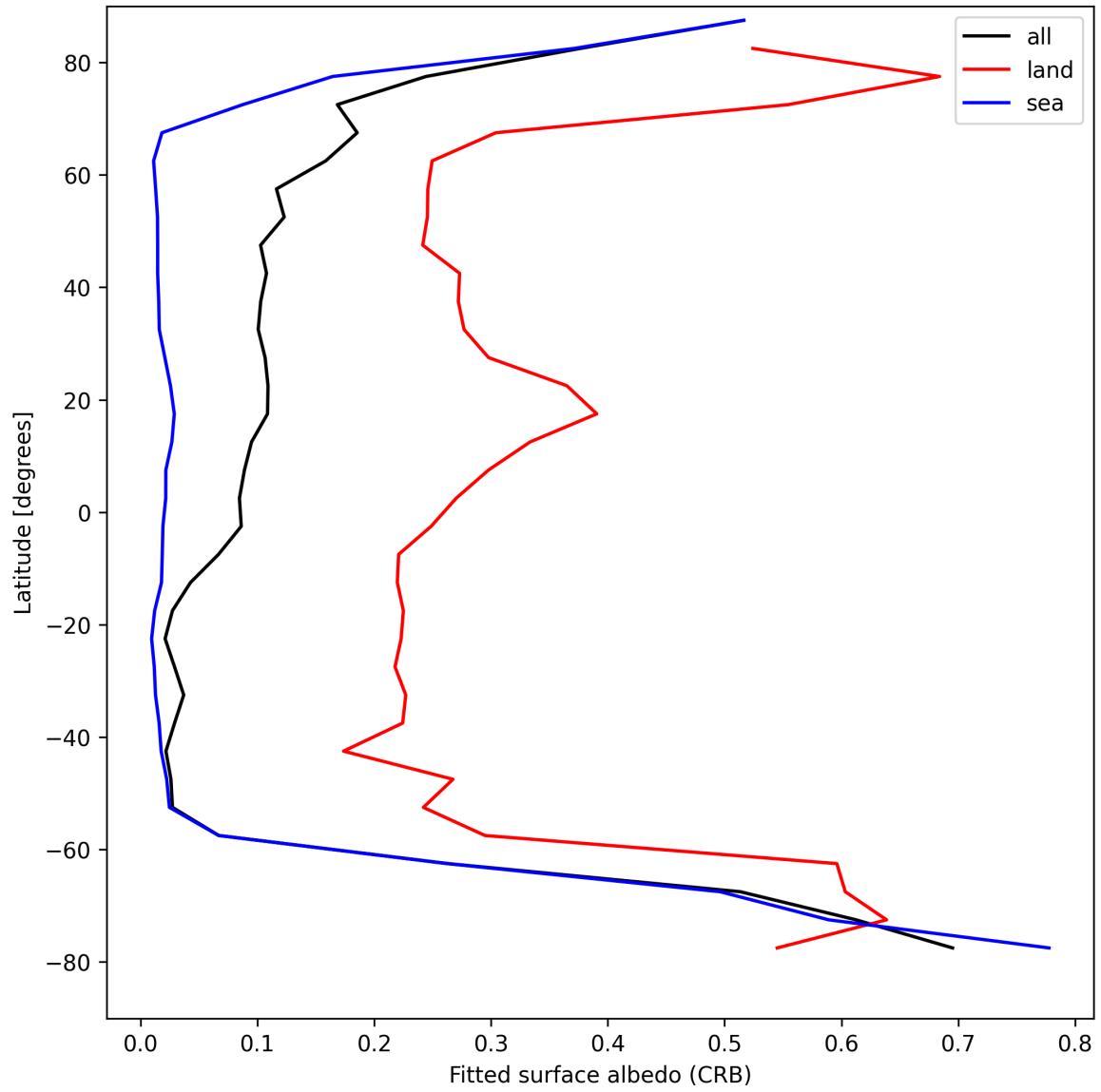
Figure 30: Zonal average of “Fitted surface albedo (CRB)” for 2025-08-14 to 2025-08-16.
