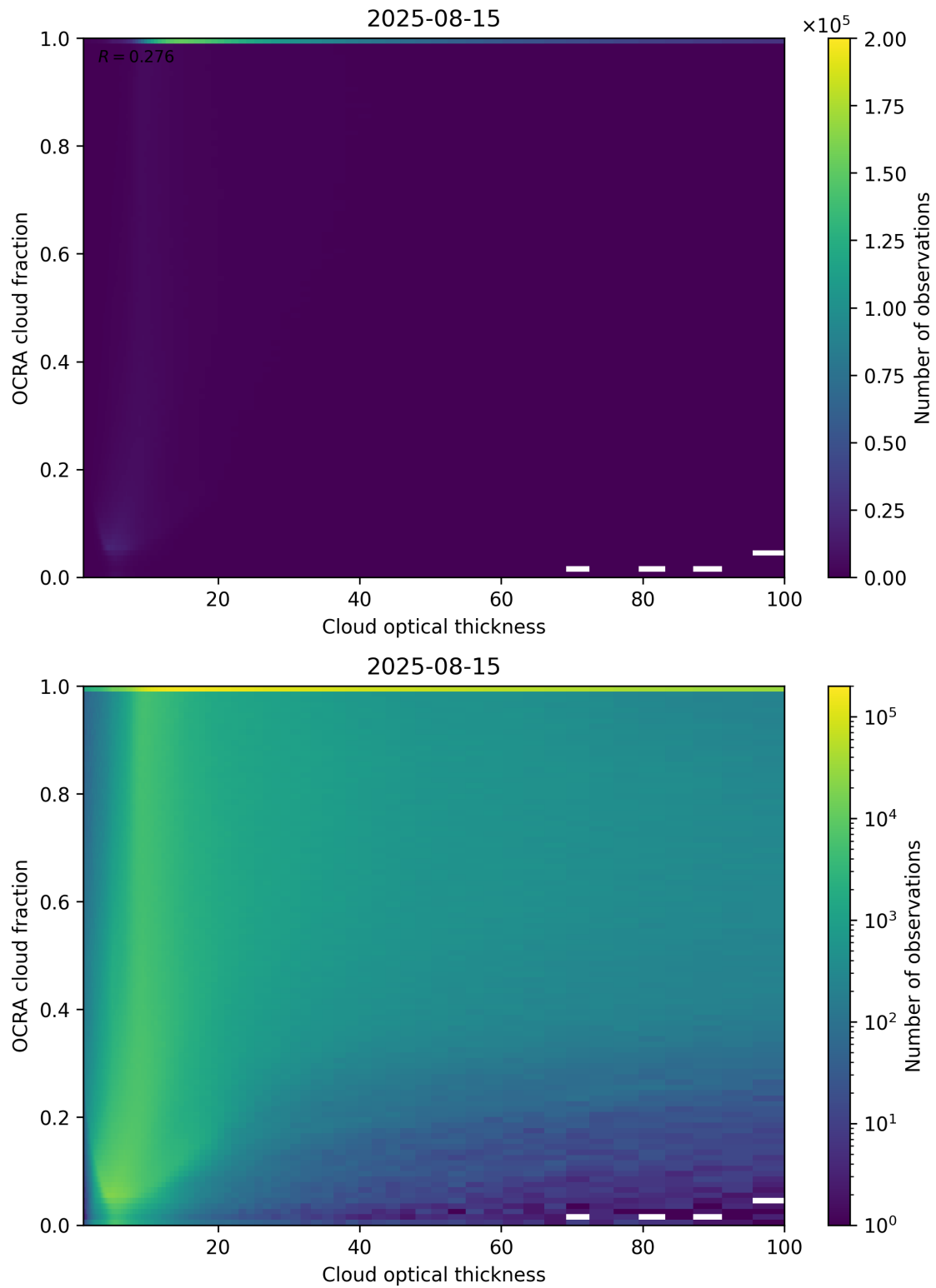
Figure 83: Scatter density plot of “Cloud optical thickness” against “OCRA cloud fraction” for 2025-08-14 to 2025-08-16.
