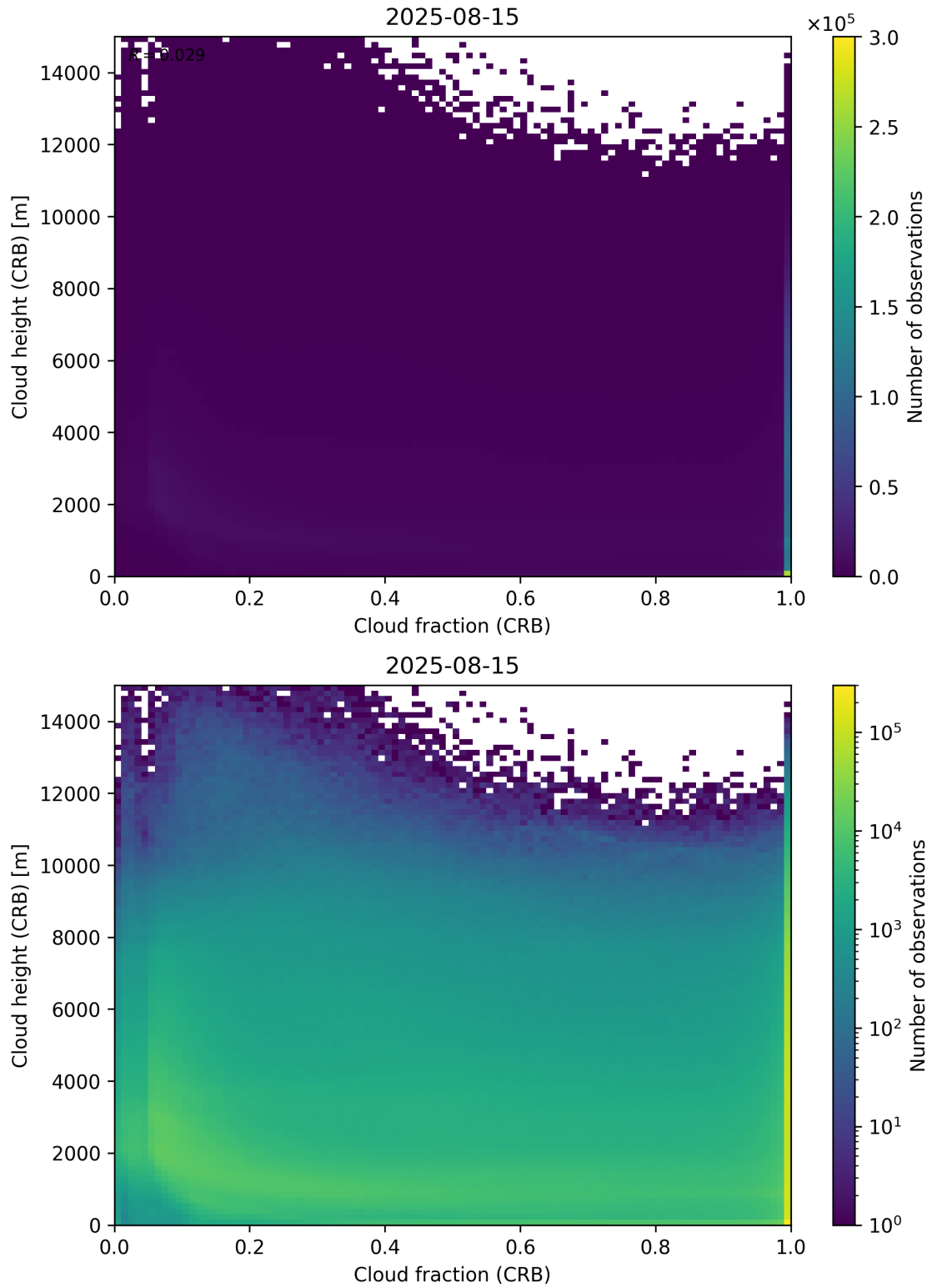
Figure 79: Scatter density plot of “Cloud fraction (CRB)” against “Cloud height (CRB)” for 2025-08-14 to 2025-08-16.
