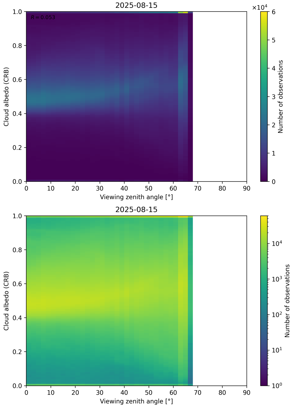
Figure 106: Scatter density plot of “Viewing zenith angle” against “Cloud albedo (CRB)” for 2025-08-14 to 2025-08-16.
