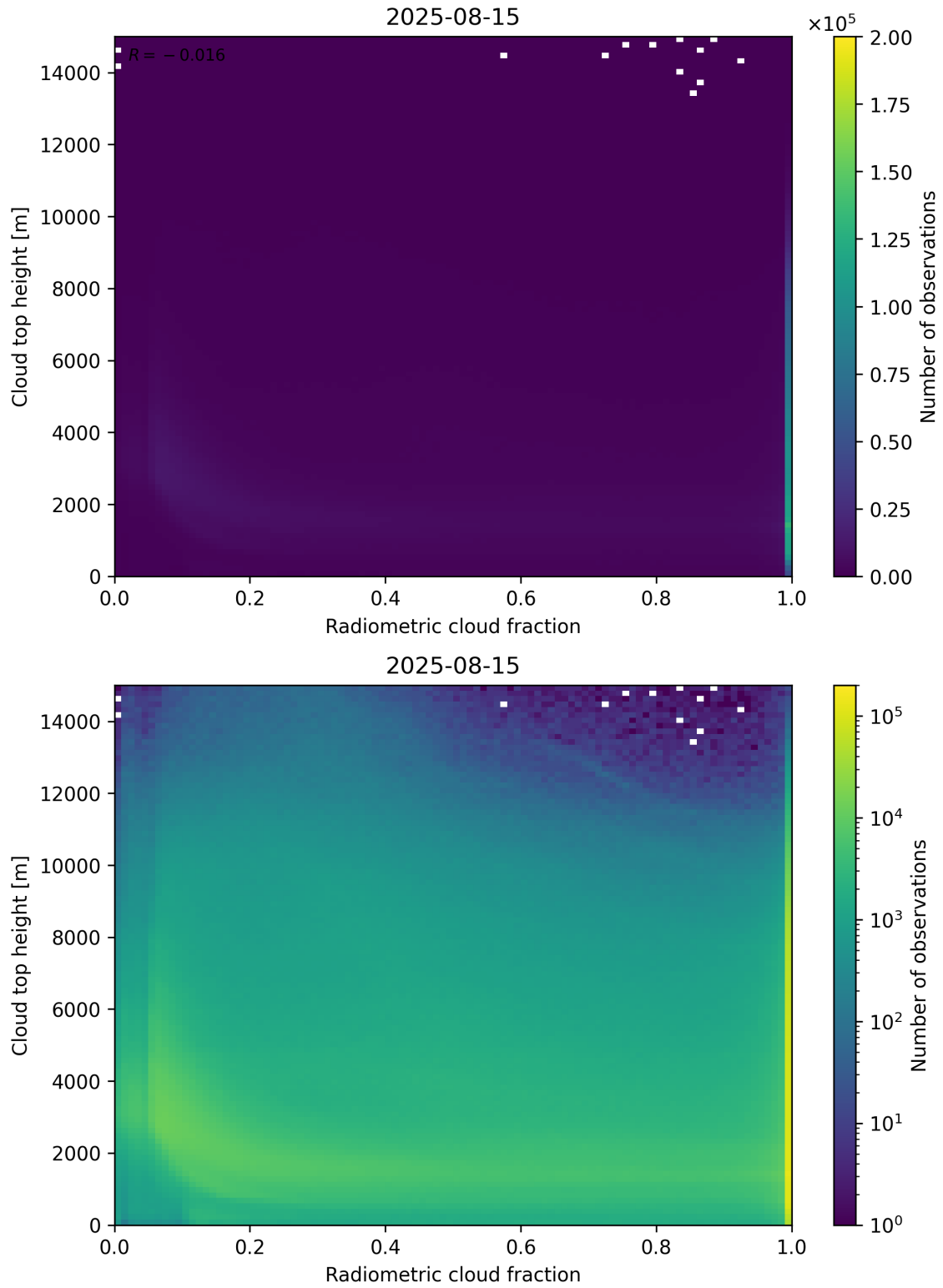
Figure 76: Scatter density plot of “Radiometric cloud fraction” against “Cloud top height” for 2025-08-14 to 2025-08-16.
