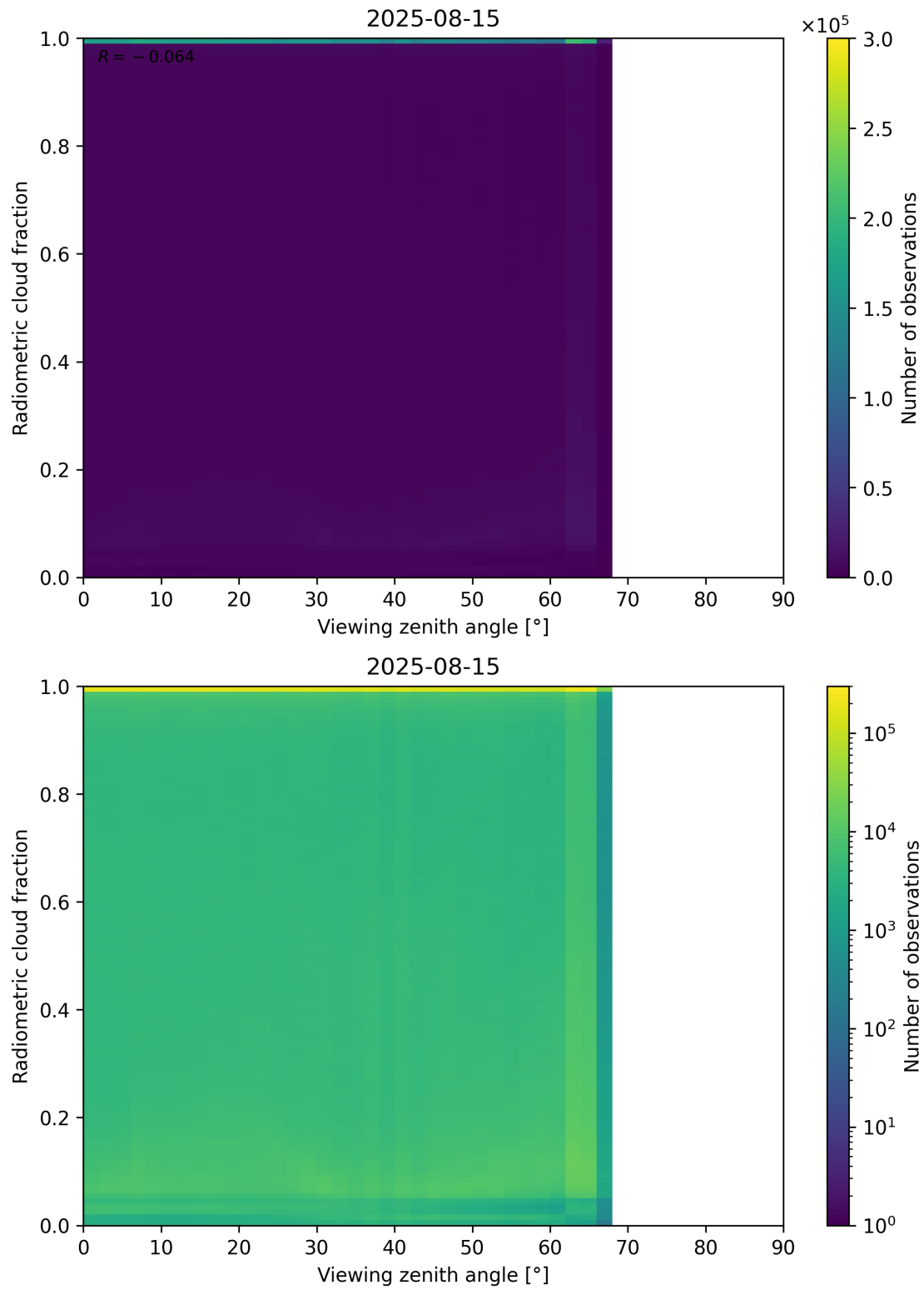
Figure 107: Scatter density plot of “Viewing zenith angle” against “Radiometric cloud fraction” for 2025-08-14 to 2025-08-16.
