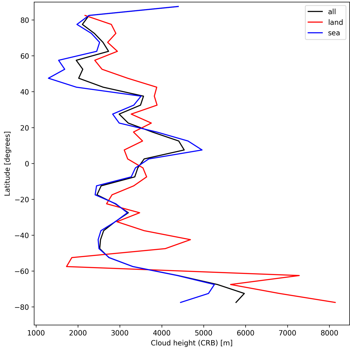
Figure 27: Zonal average of “Cloud height (CRB)” for 2025-08-14 to 2025-08-16.
