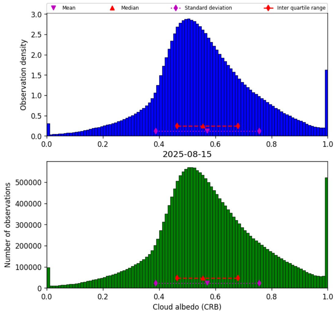
Figure 44: Histogram of “Cloud albedo (CRB)” for 2025-08-14 to 2025-08-16
