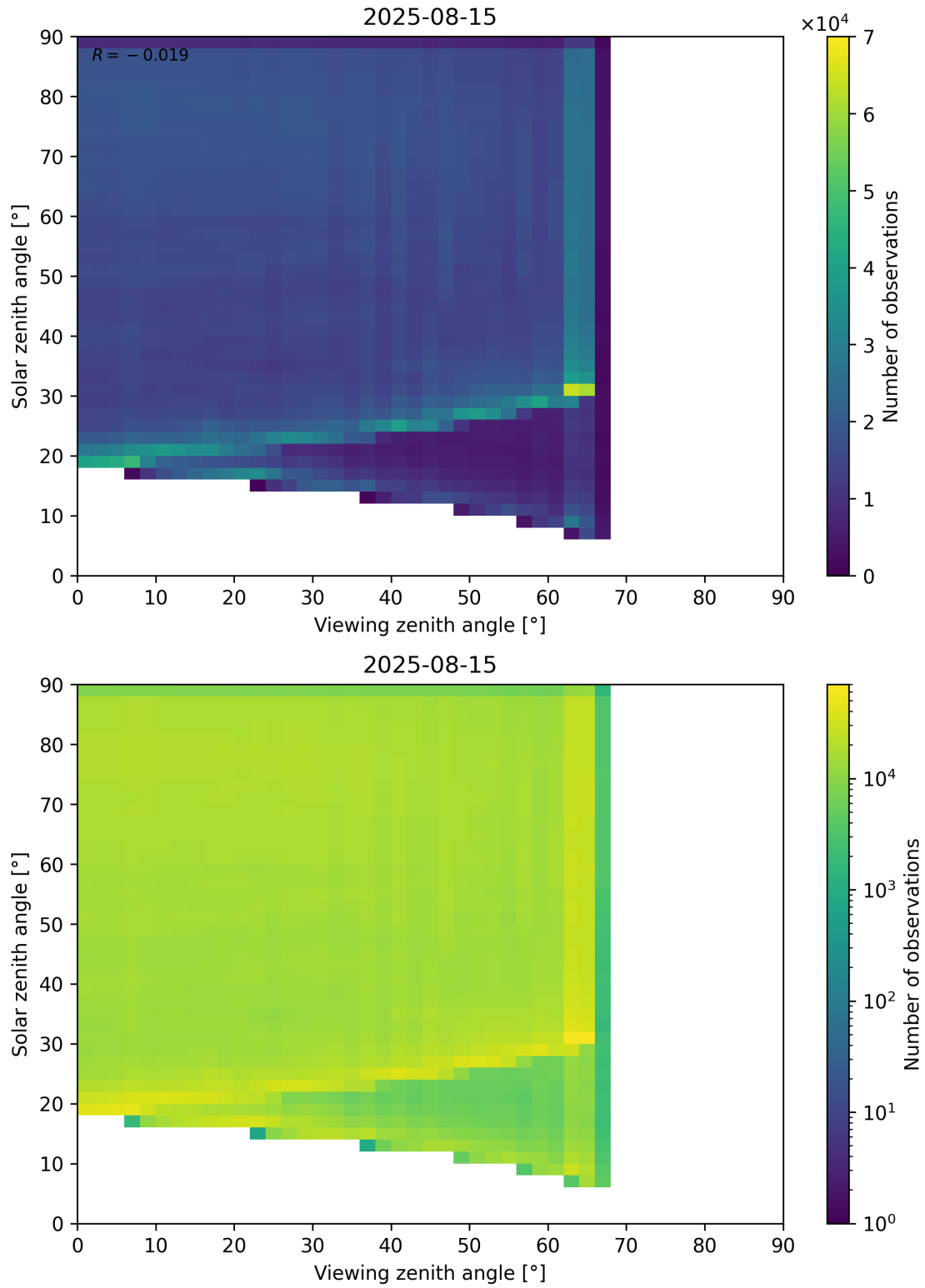
Figure 114: Scatter density plot of “Viewing zenith angle” against “Solar zenith angle” for 2025-08-14 to 2025-08-16.
