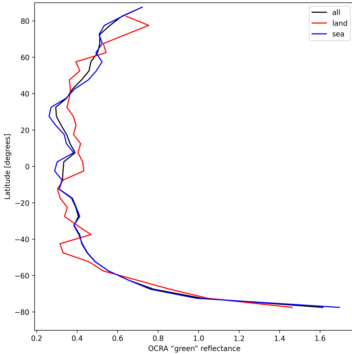
Figure 36: Zonal average of “OCRA “green” reflectance” for 2025-08-14 to 2025-08-16.
