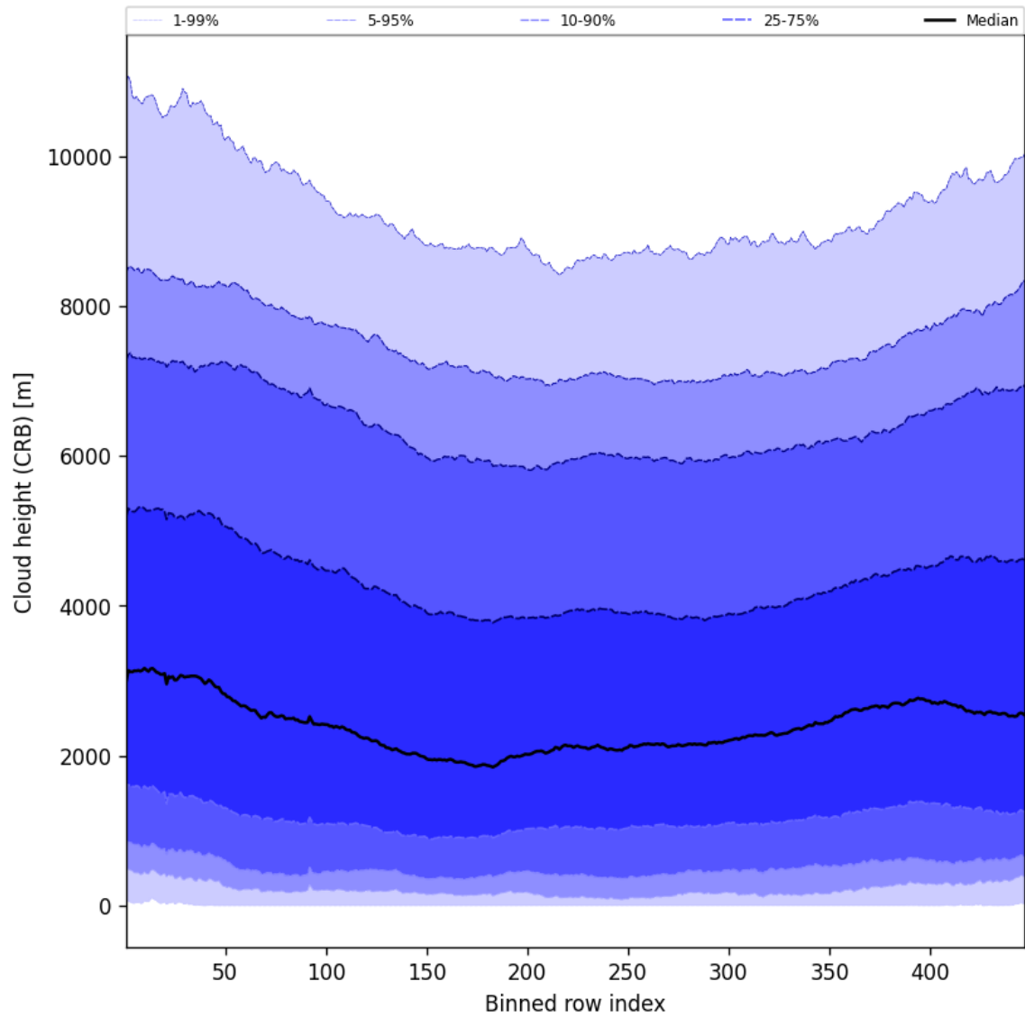
Figure 59: Along track statistics of “Cloud height (CRB)” for 2025-08-14 to 2025-08-16
