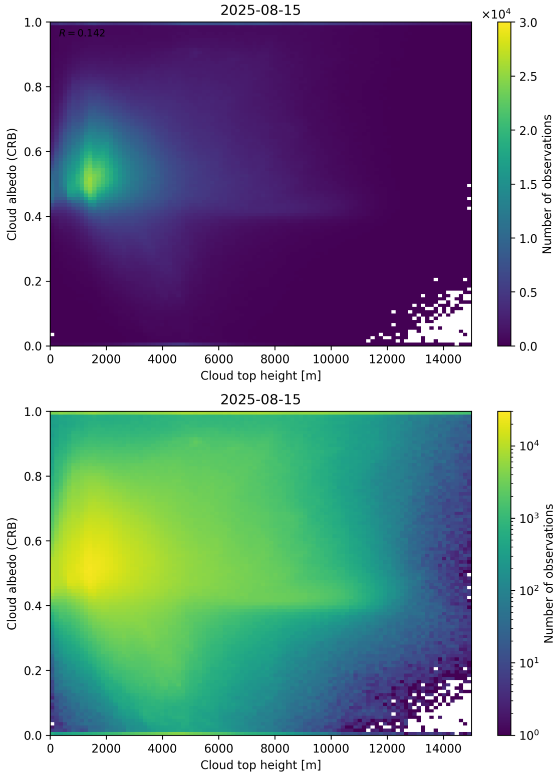
Figure 86: Scatter density plot of “Cloud top height” against “Cloud albedo (CRB)” for 2025-08-14 to 2025-08-16.
