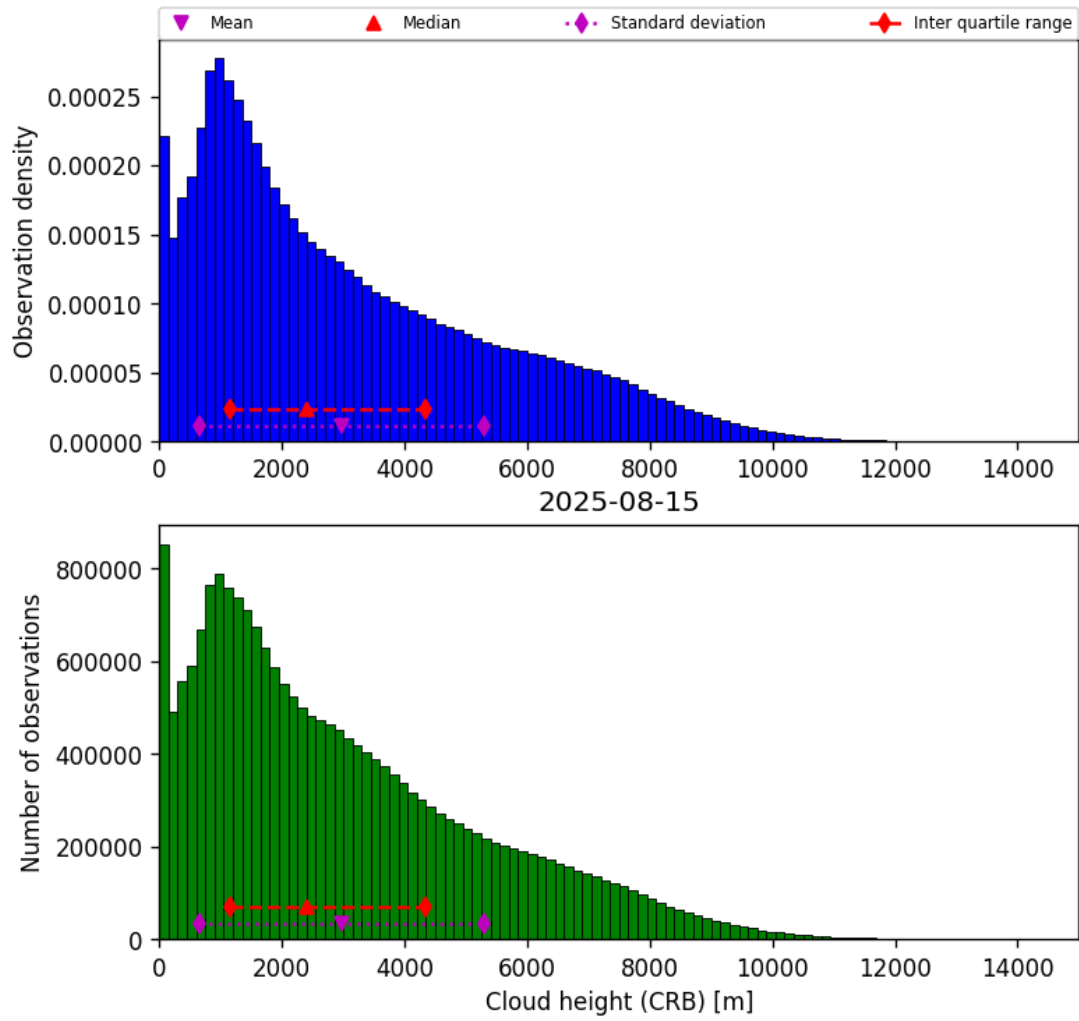
Figure 43: Histogram of “Cloud height (CRB)” for 2025-08-14 to 2025-08-16
