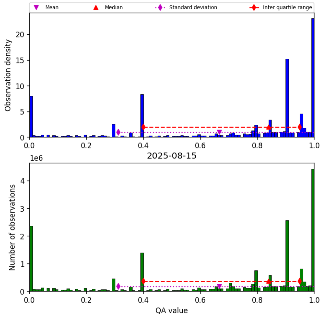
Figure 38: Histogram of “QA value” for 2025-08-14 to 2025-08-16
