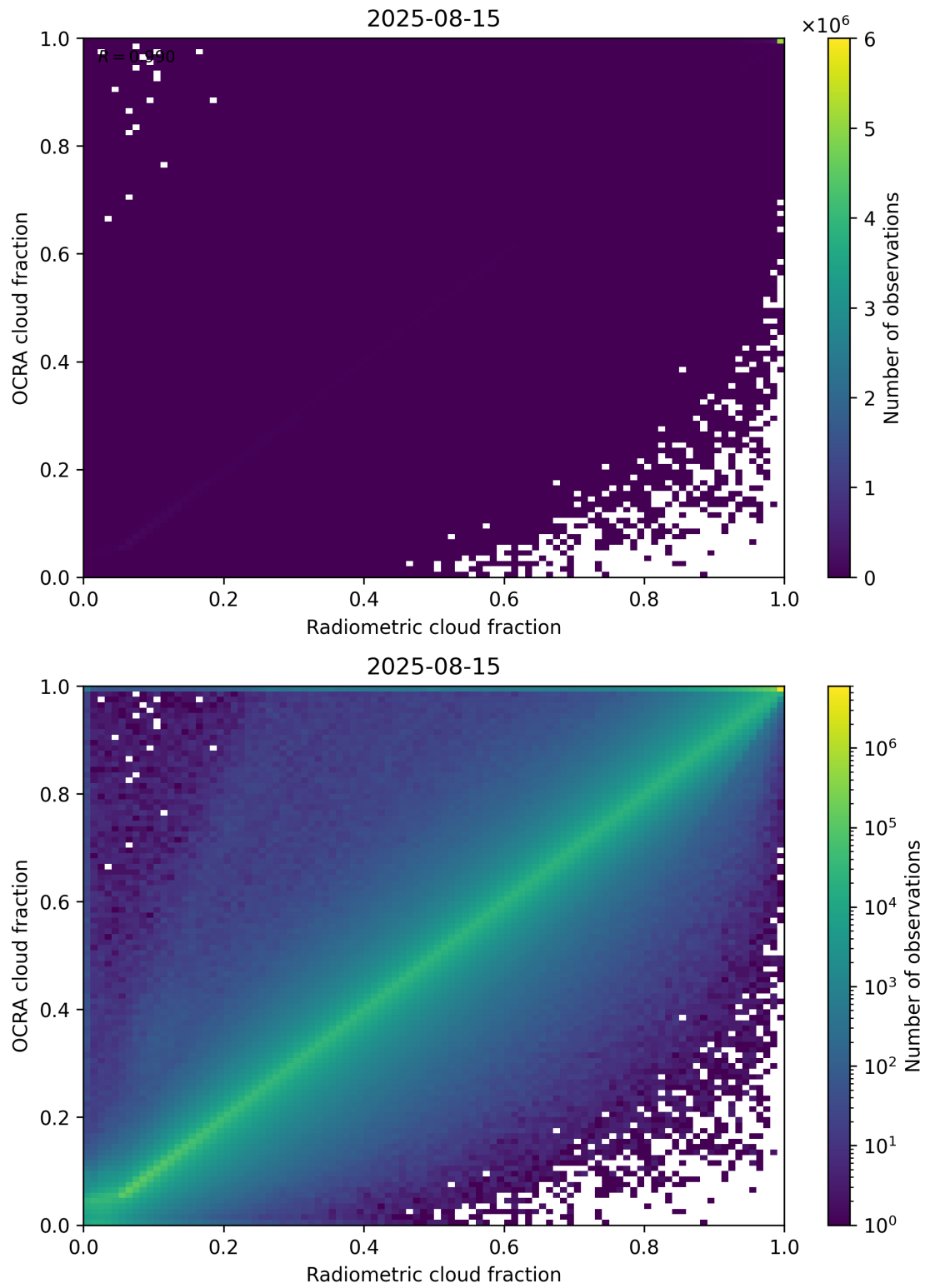
Figure 72: Scatter density plot of “Radiometric cloud fraction” against “OCRA cloud fraction” for 2025-08-14 to 2025-08-16.
