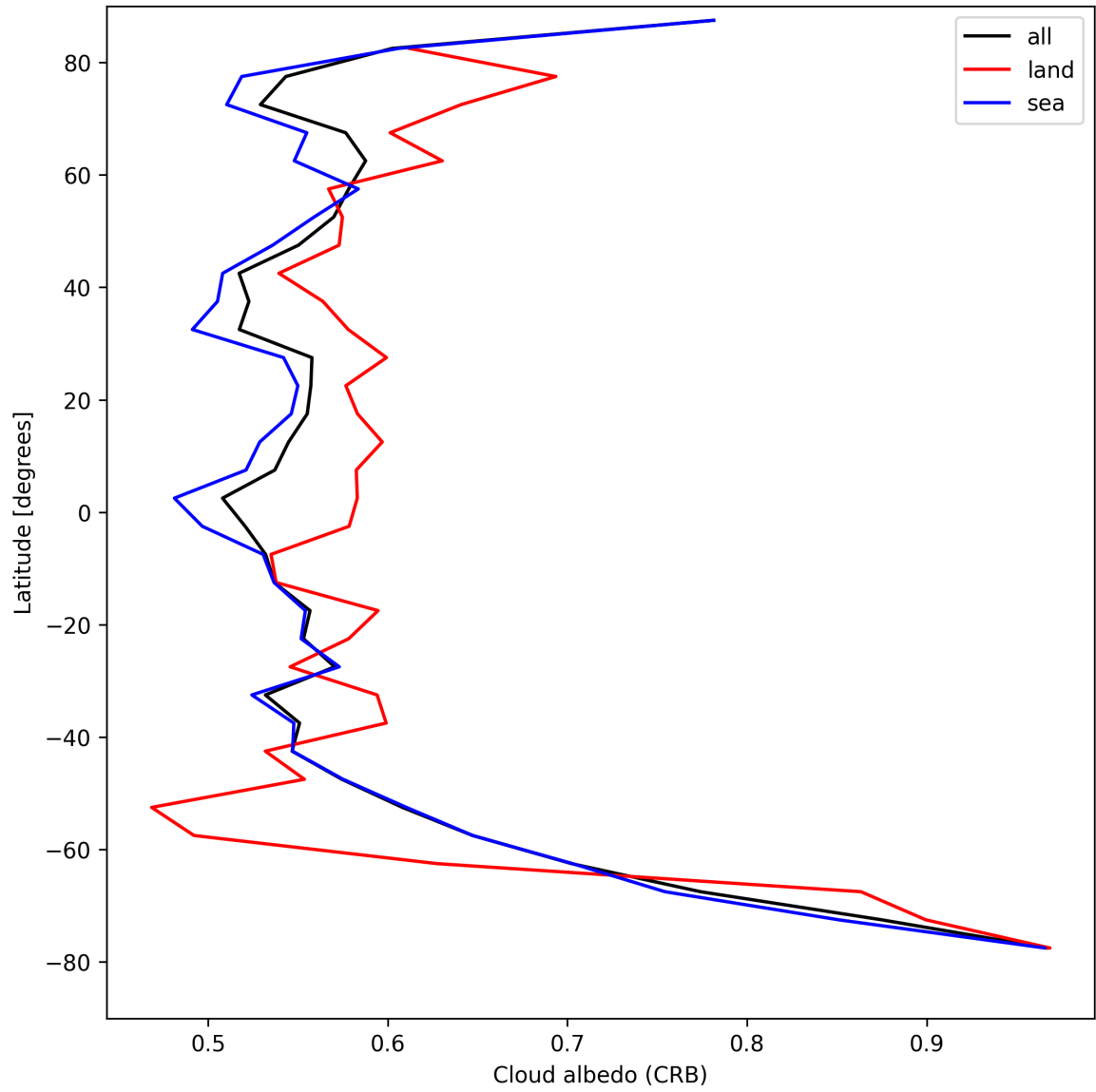
Figure 28: Zonal average of “Cloud albedo (CRB)” for 2025-08-14 to 2025-08-16.
