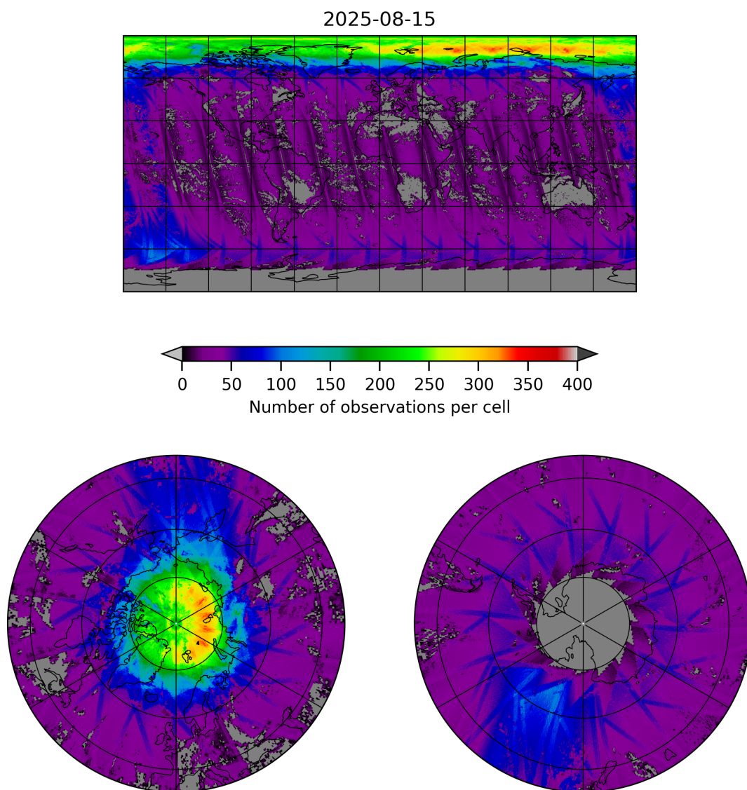
Figure 21: Map of the number of observations for 2025-08-14 to 2025-08-16
