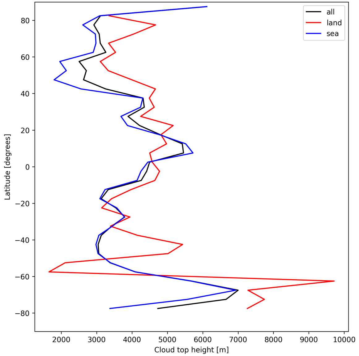
Figure 24: Zonal average of “Cloud top height” for 2025-08-14 to 2025-08-16.
