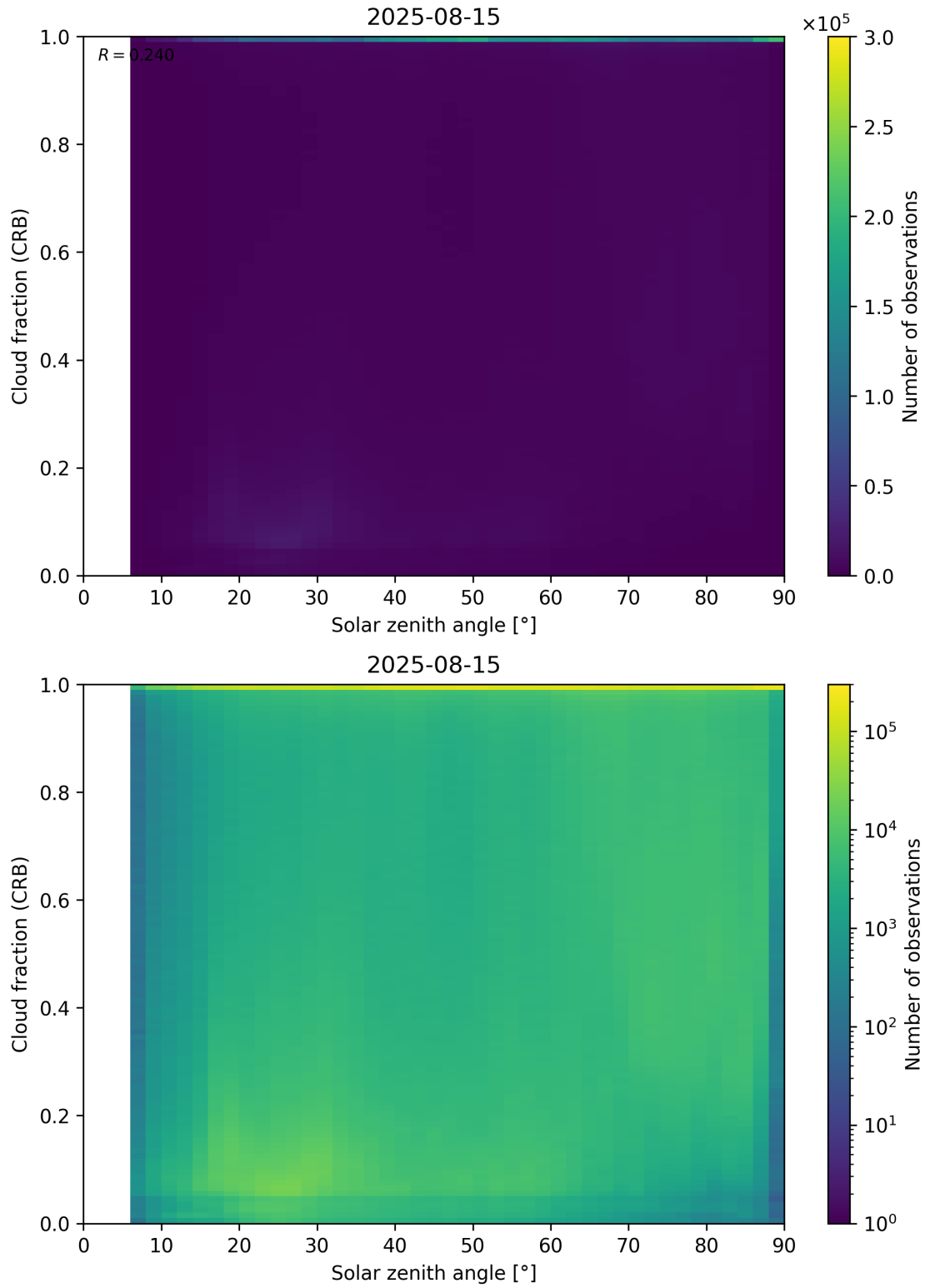
Figure 101: Scatter density plot of “Solar zenith angle” against “Cloud fraction (CRB)” for 2025-08-14 to 2025-08-16.
