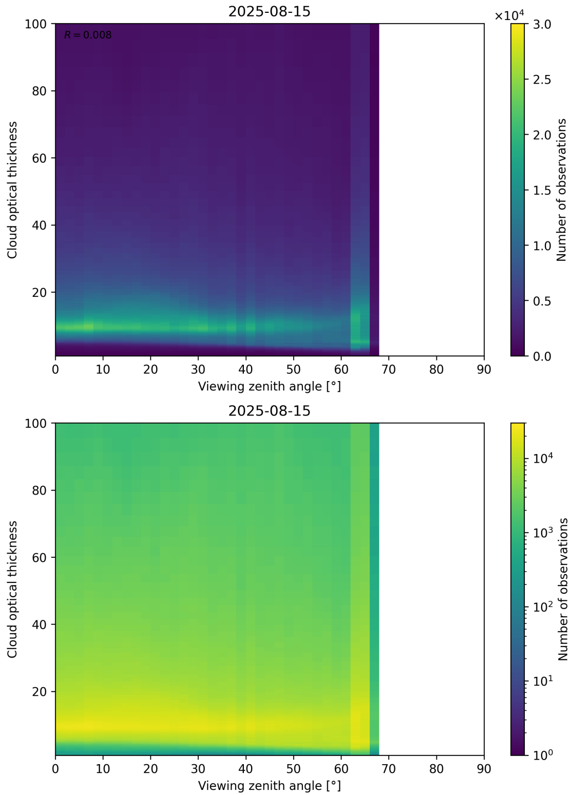
Figure 111: Scatter density plot of “Viewing zenith angle” against “Cloud optical thickness” for 2025-08-14 to 2025-08-16.
