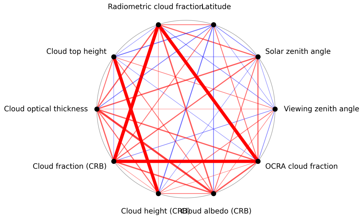
Figure 1: Map of correlation graph for 2025-08-14 to 2025-08-16.
