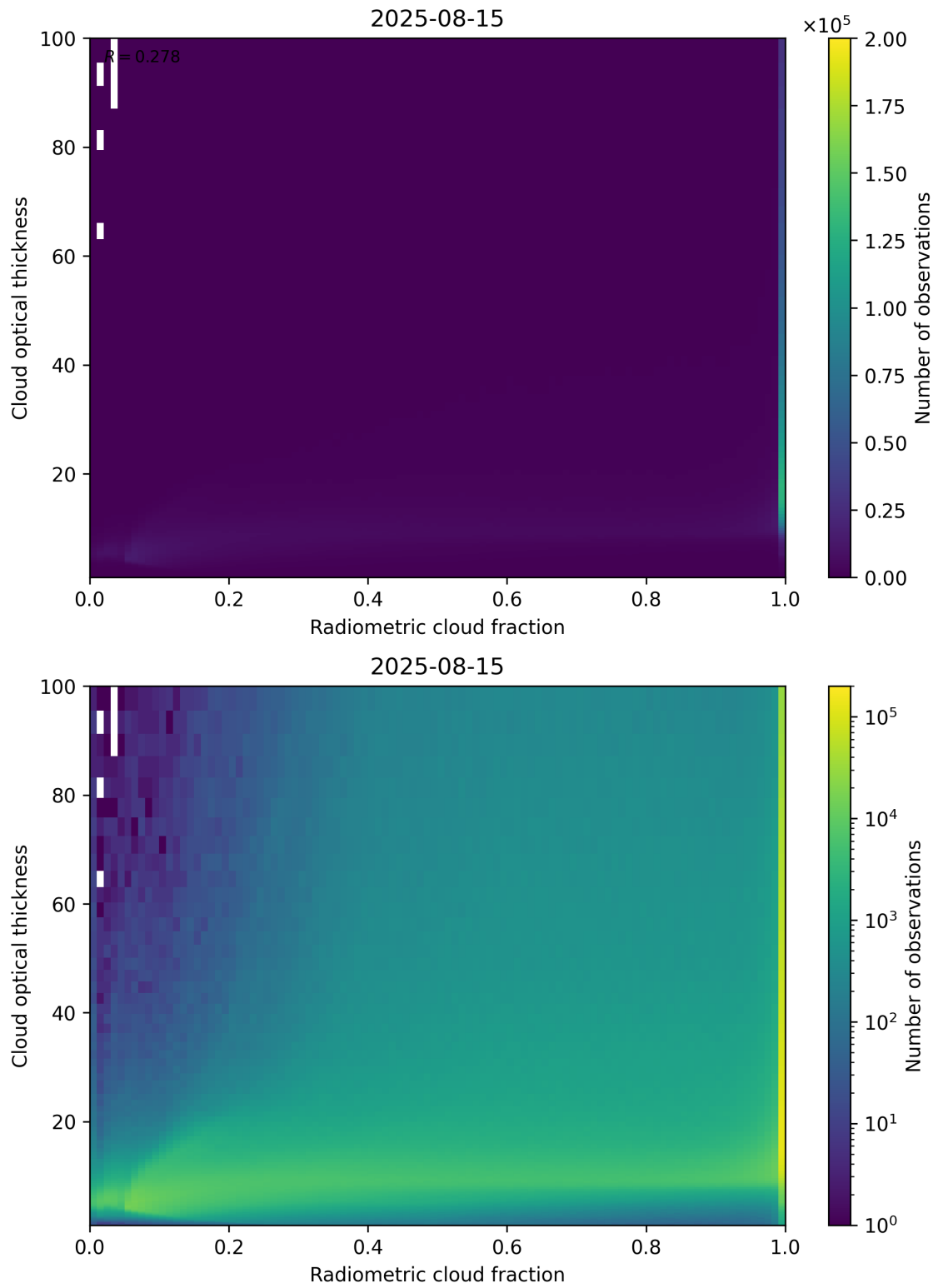
Figure 75: Scatter density plot of “Radiometric cloud fraction” against “Cloud optical thickness” for 2025-08-14 to 2025-08-16.
