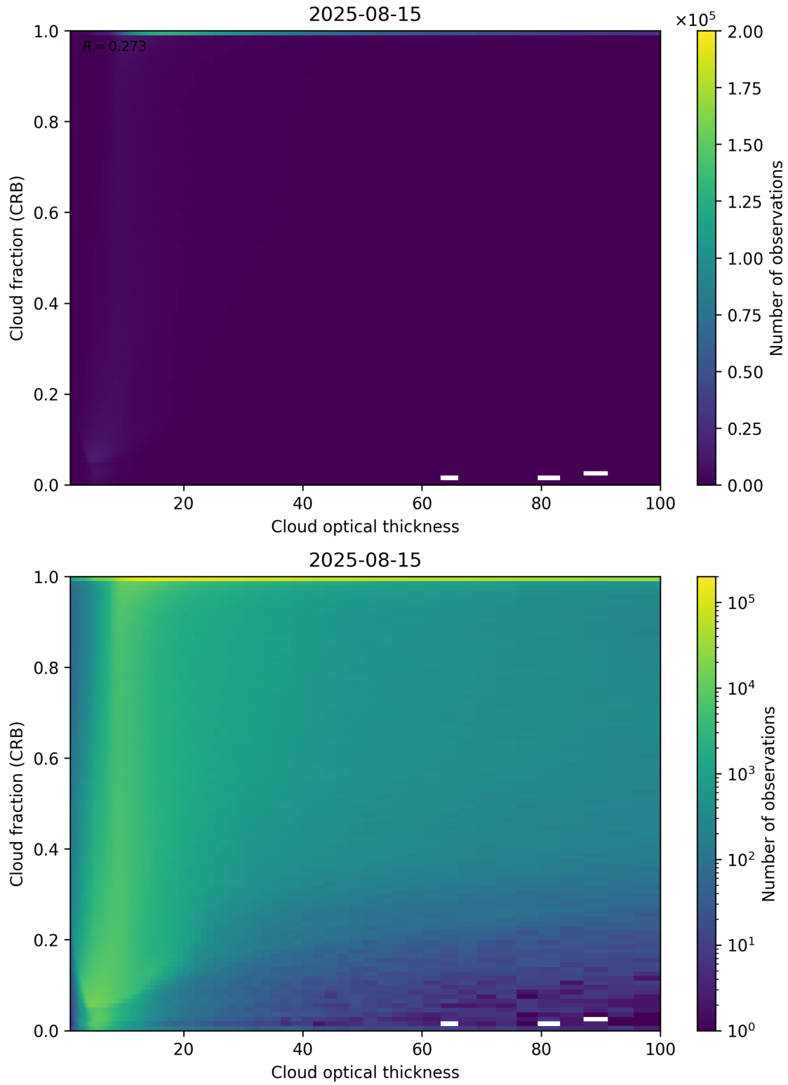
Figure 84: Scatter density plot of “Cloud optical thickness” against “Cloud fraction (CRB)” for 2025-08-14 to 2025-08-16.
