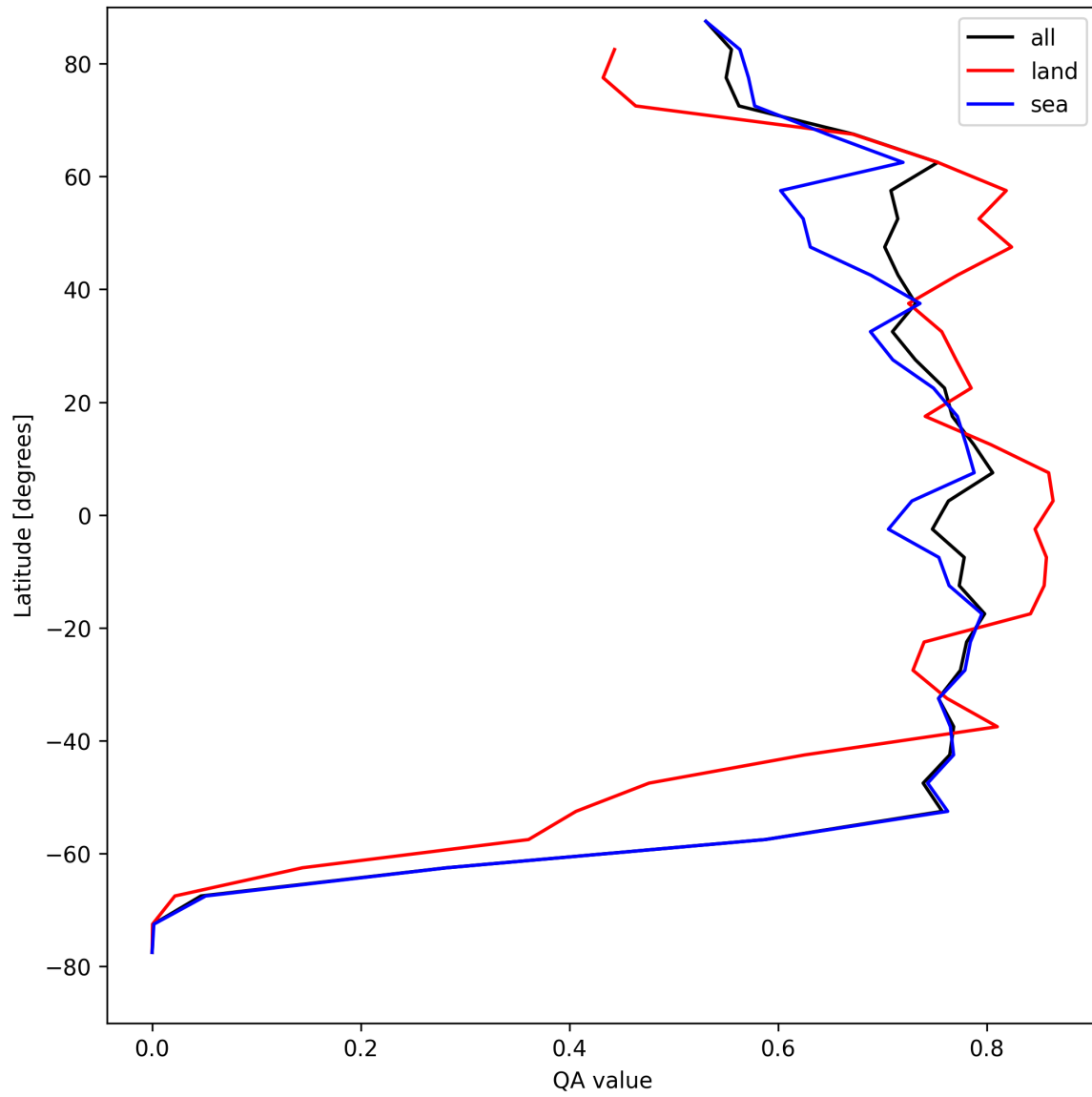
Figure 22: Zonal average of “QA value” for 2025-08-14 to 2025-08-16.
