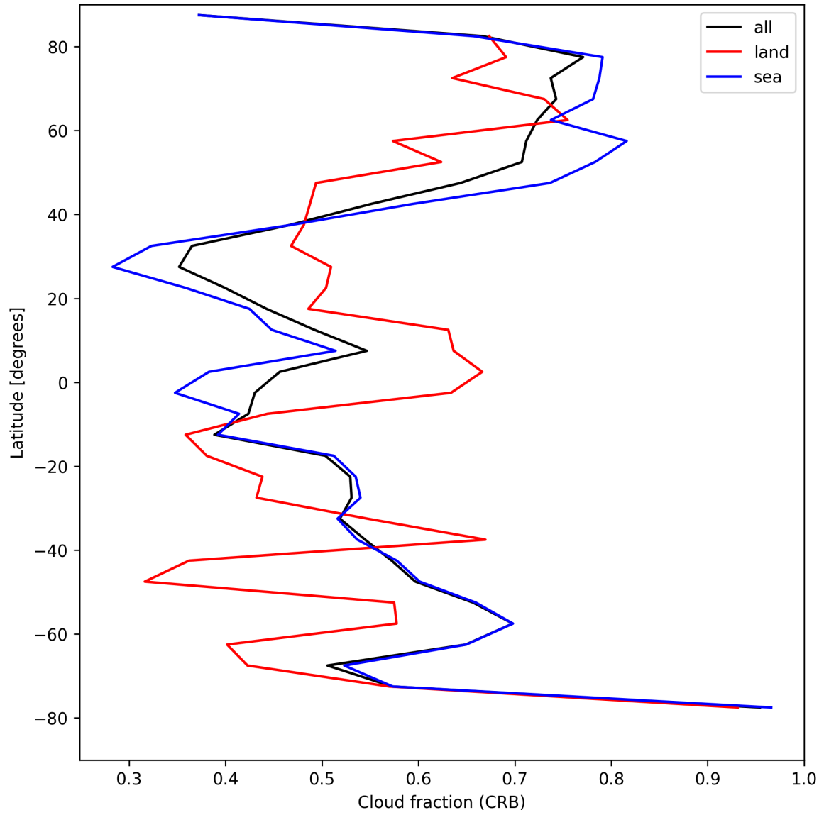
Figure 26: Zonal average of “Cloud fraction (CRB)” for 2025-08-14 to 2025-08-16.
