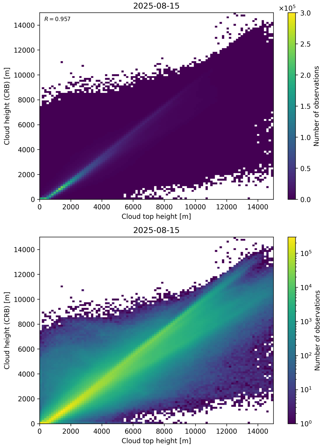
Figure 89: Scatter density plot of “Cloud top height” against “Cloud height (CRB)” for 2025-08-14 to 2025-08-16.
