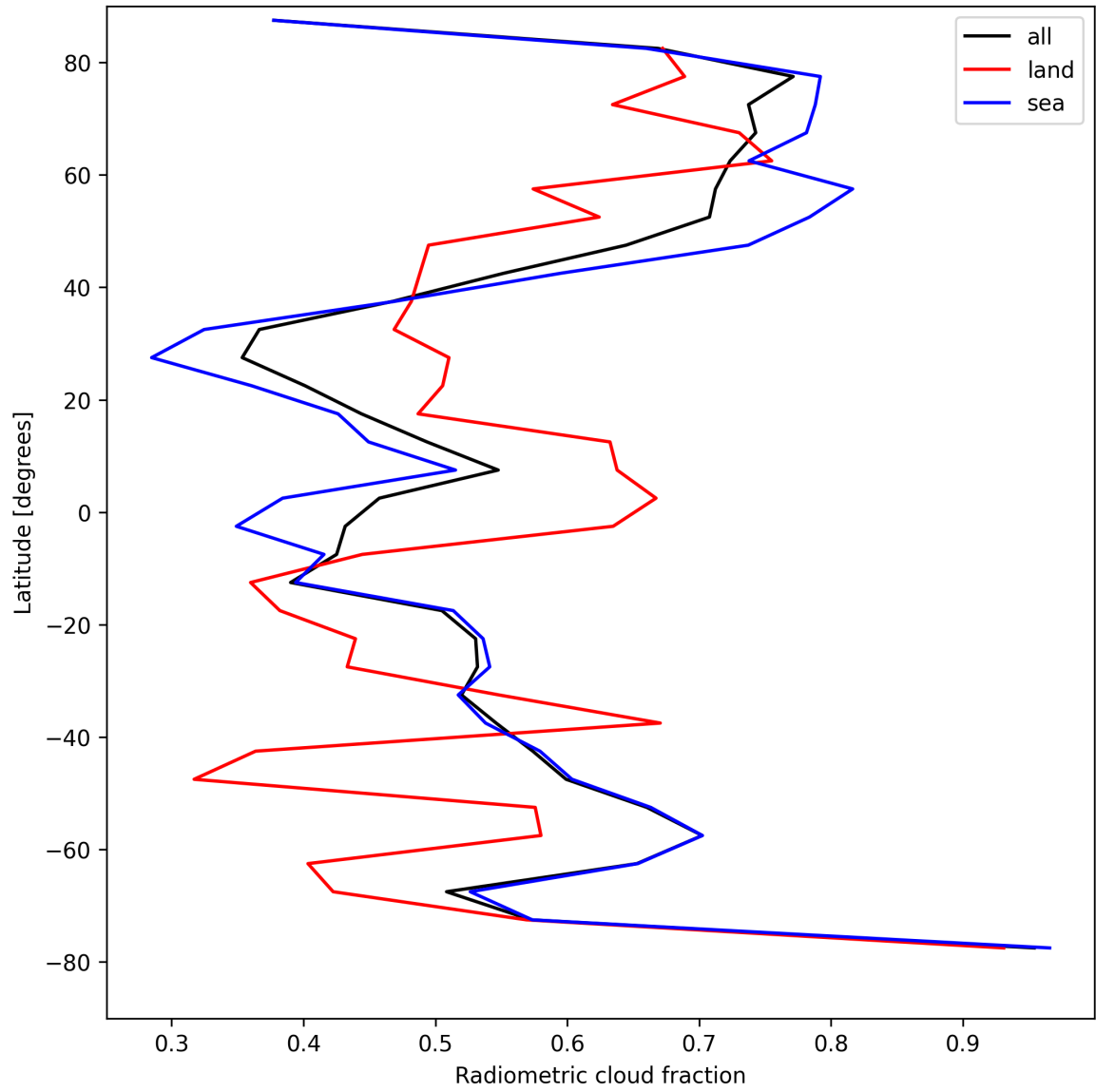
Figure 23: Zonal average of “Radiometric cloud fraction” for 2025-08-14 to 2025-08-16.
