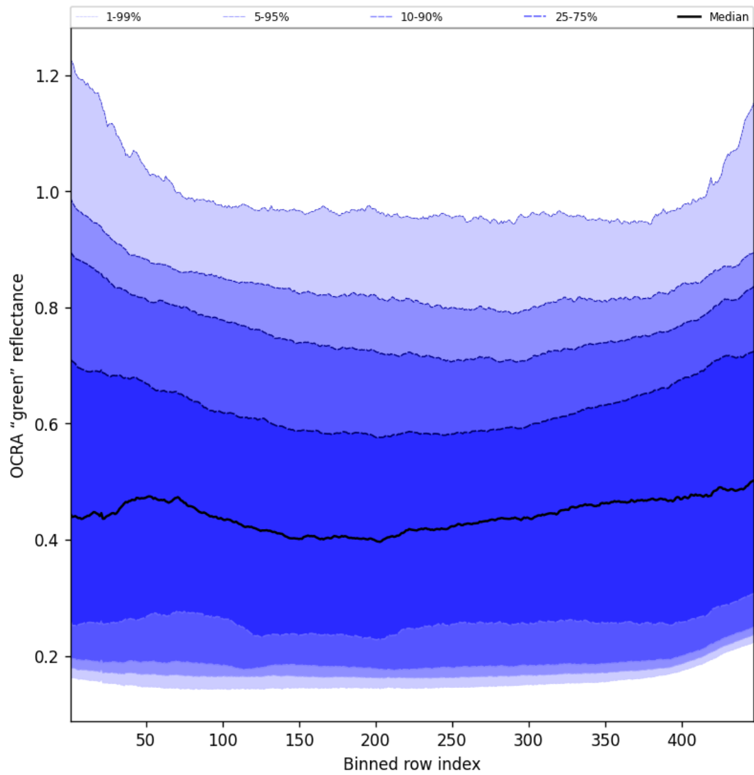
Figure 68: Along track statistics of "OCRA "green" reflectance" for 2025-08-14 to 2025-08-16
