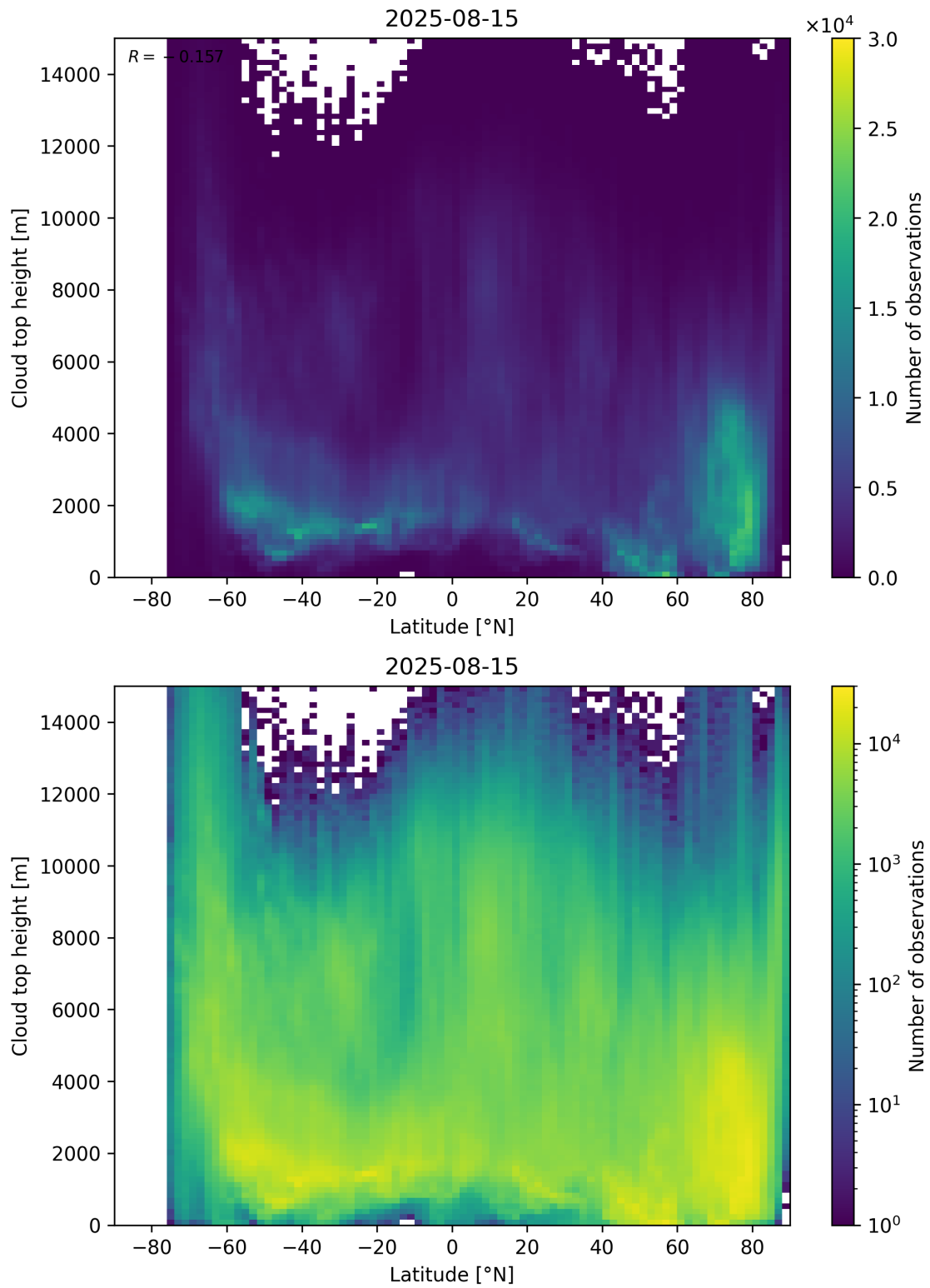
Figure 97: Scatter density plot of “Latitude” against “Cloud top height” for 2025-08-14 to 2025-08-16.
