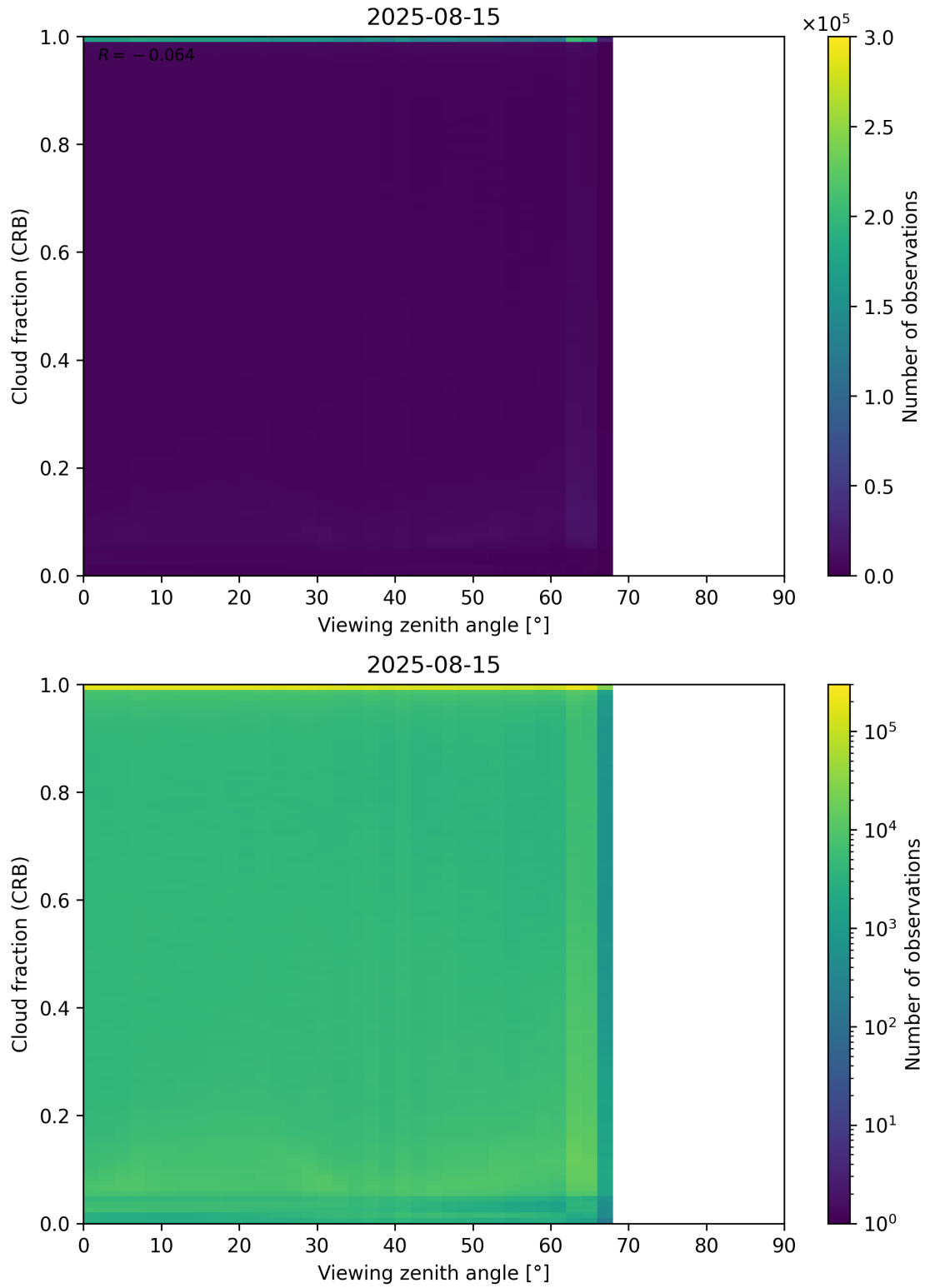
Figure 109: Scatter density plot of “Viewing zenith angle” against “Cloud fraction (CRB)” for 2025-08-14 to 2025-08-16.
