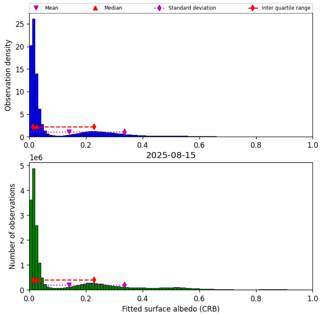
Figure 46: Histogram of “Fitted surface albedo (CRB)” for 2025-08-14 to 2025-08-16
