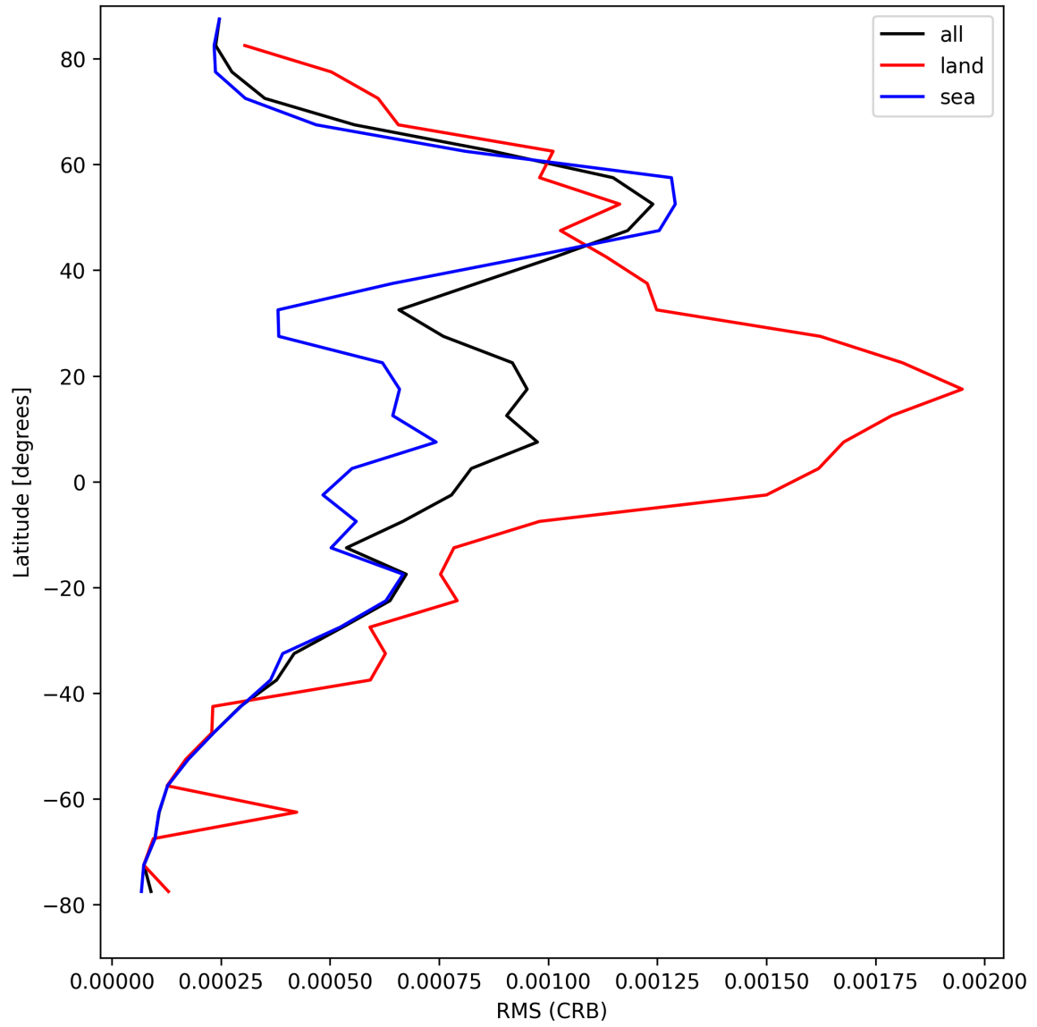
Figure 32: Zonal average of “RMS (CRB)” for 2025-08-14 to 2025-08-16.
