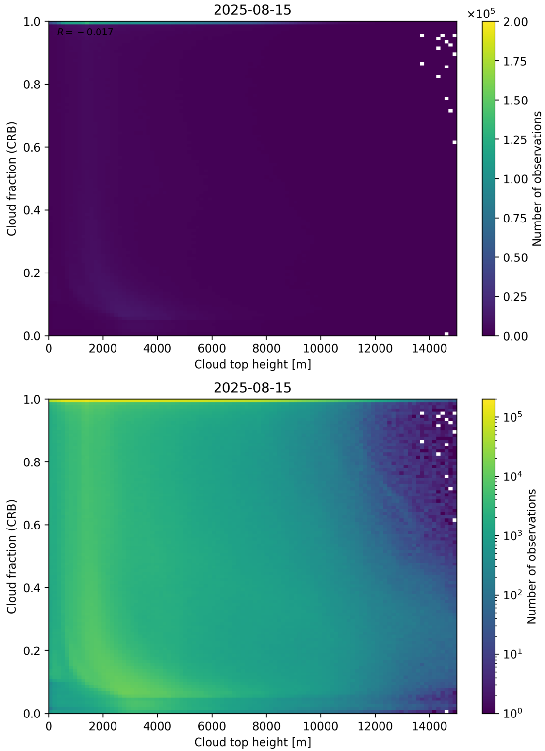
Figure 88: Scatter density plot of “Cloud top height” against “Cloud fraction (CRB)” for 2025-08-14 to 2025-08-16.
