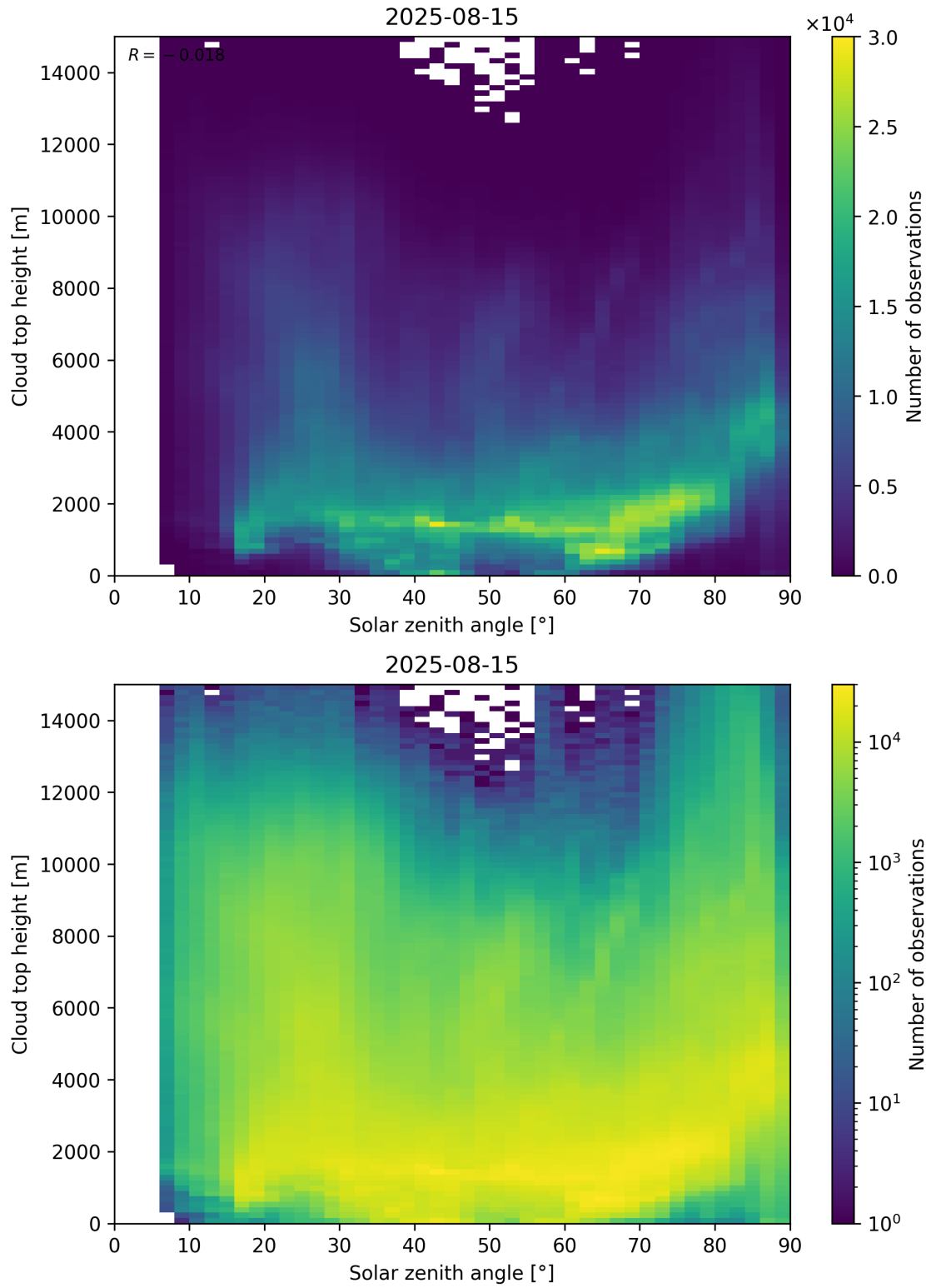
Figure 104: Scatter density plot of “Solar zenith angle” against “Cloud top height” for 2025-08-14 to 2025-08-16.
