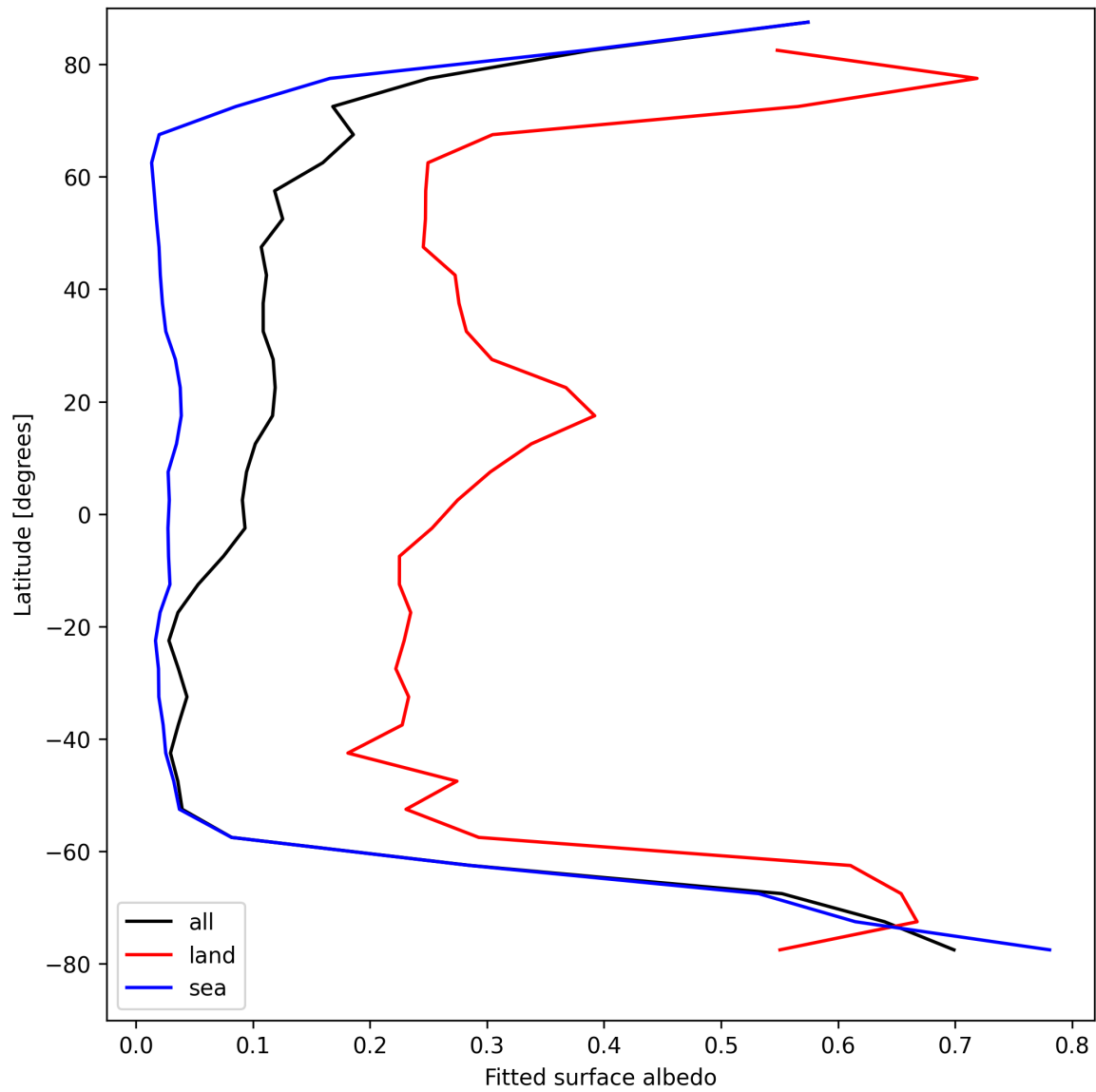
Figure 29: Zonal average of “Fitted surface albedo” for 2025-08-14 to 2025-08-16.
