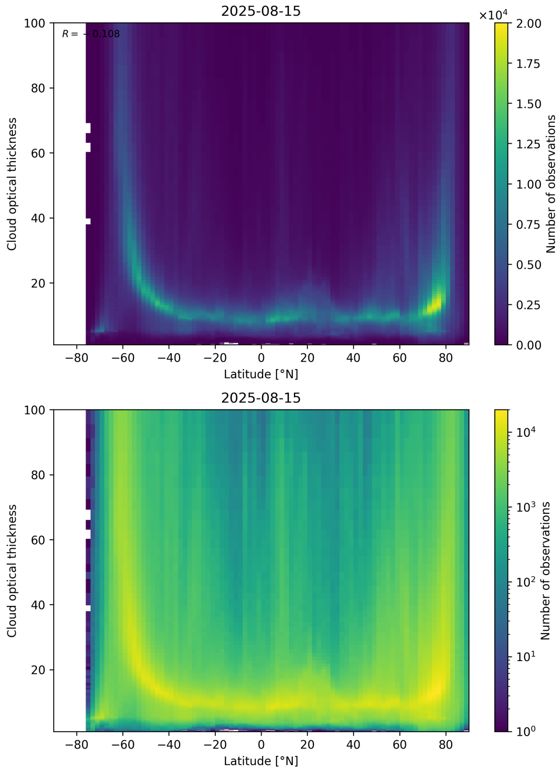
Figure 96: Scatter density plot of “Latitude” against “Cloud optical thickness” for 2025-08-14 to 2025-08-16.
