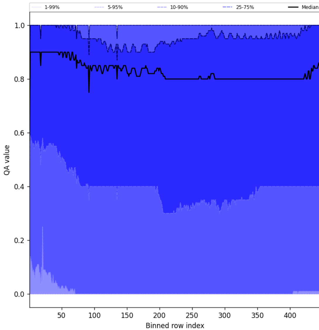
Figure 54: Along track statistics of “QA value” for 2025-08-14 to 2025-08-16
