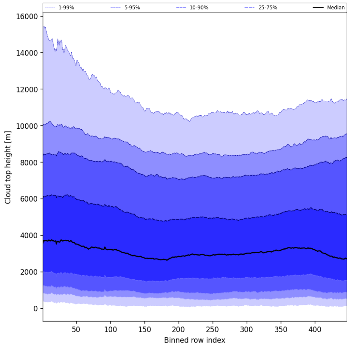
Figure 56: Along track statistics of “Cloud top height” for 2025-08-14 to 2025-08-16
