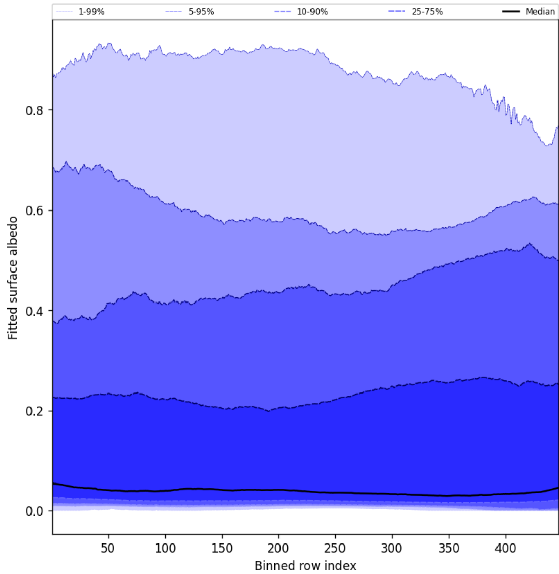
Figure 61: Along track statistics of “Fitted surface albedo” for 2025-08-14 to 2025-08-16
