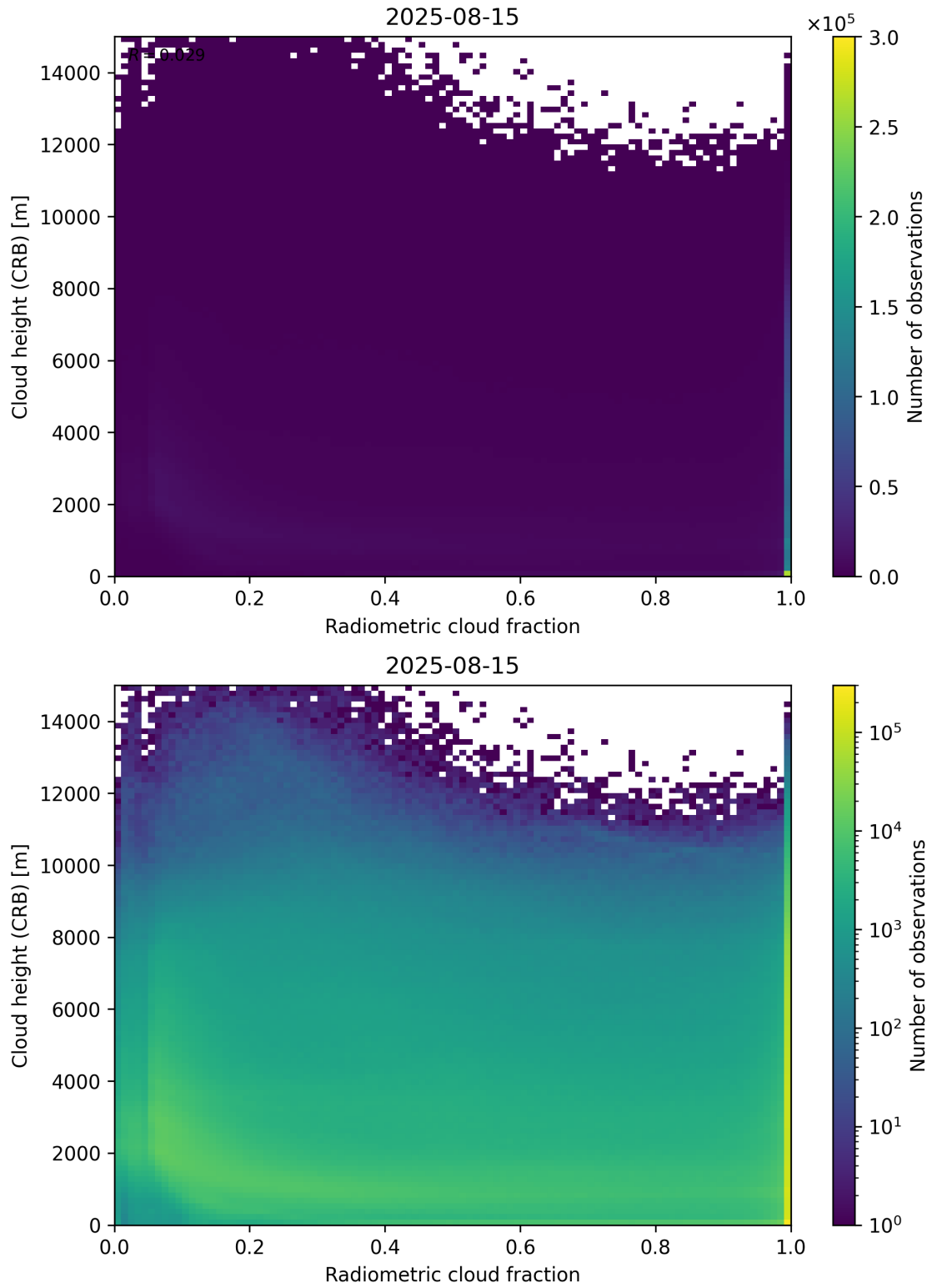
Figure 74: Scatter density plot of “Radiometric cloud fraction” against “Cloud height (CRB)” for 2025-08-14 to 2025-08-16.
