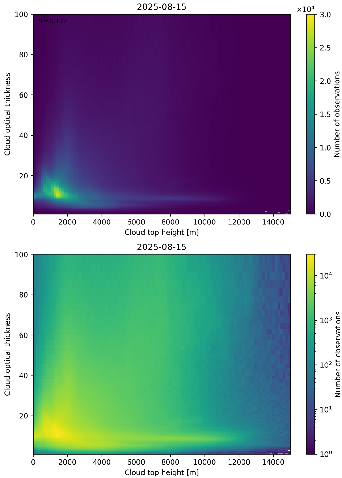
Figure 90: Scatter density plot of “Cloud top height” against “Cloud optical thickness” for 2025-08-14 to 2025-08-16.
