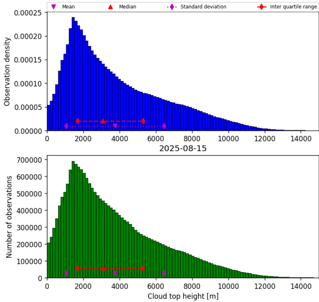
Figure 40: Histogram of “Cloud top height” for 2025-08-14 to 2025-08-16
