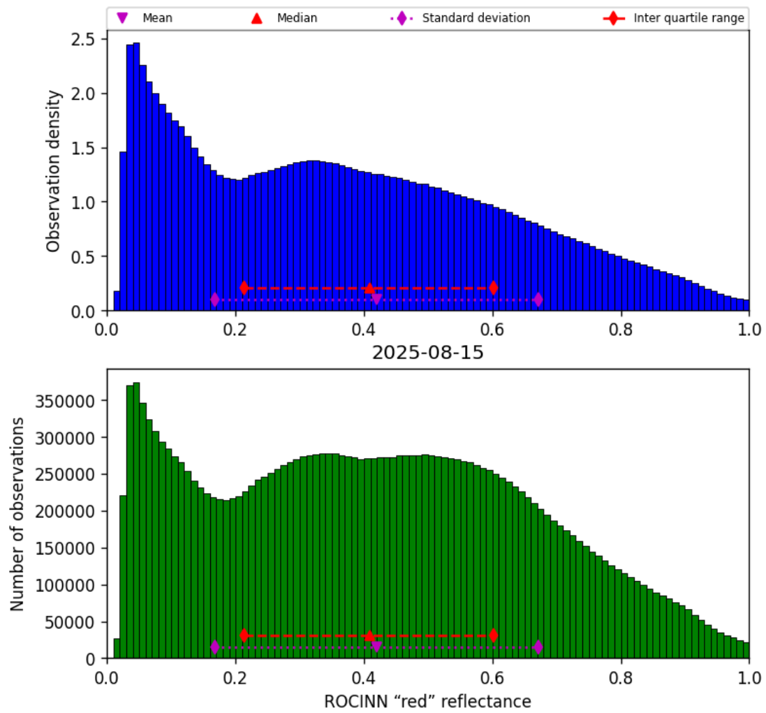
Figure 53: Histogram of “ROCINN “red” reflectance” for 2025-08-14 to 2025-08-16
