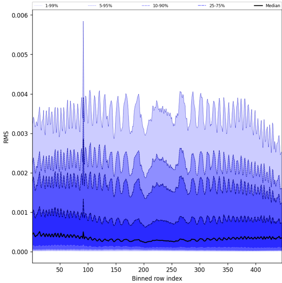
Figure 63: Along track statistics of “RMS” for 2025-08-14 to 2025-08-16
