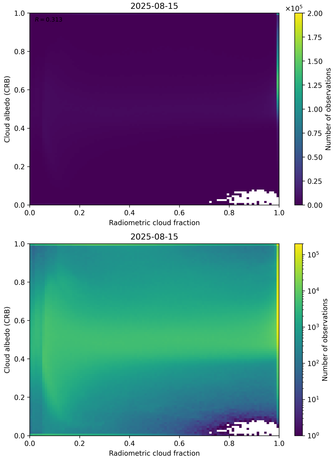
Figure 71: Scatter density plot of “Radiometric cloud fraction” against “Cloud albedo (CRB)” for 2025-08-14 to 2025-08-16.
