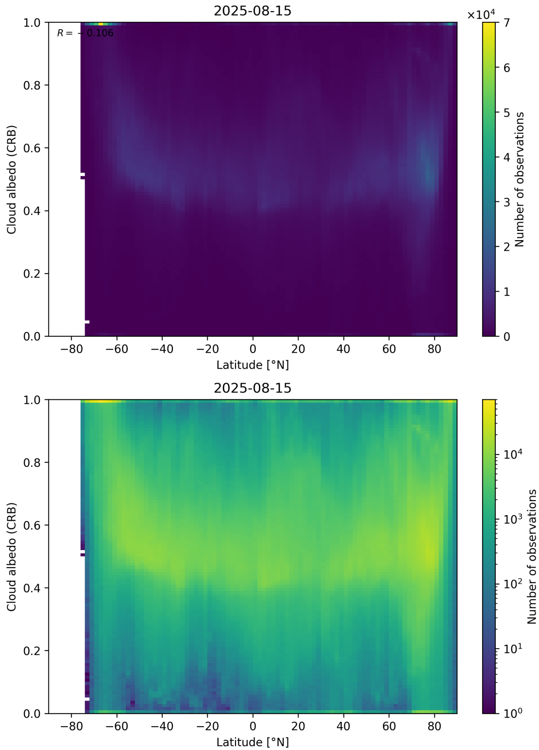
Figure 91: Scatter density plot of “Latitude” against “Cloud albedo (CRB)” for 2025-08-14 to 2025-08-16.
