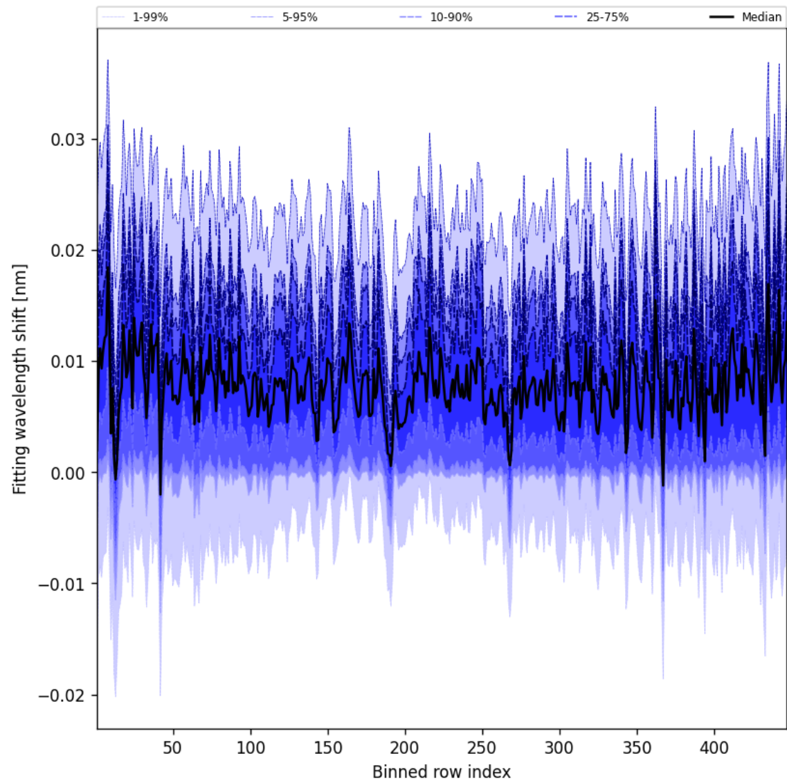
Figure 65: Along track statistics of “Fitting wavelength shift” for 2025-08-14 to 2025-08-16
