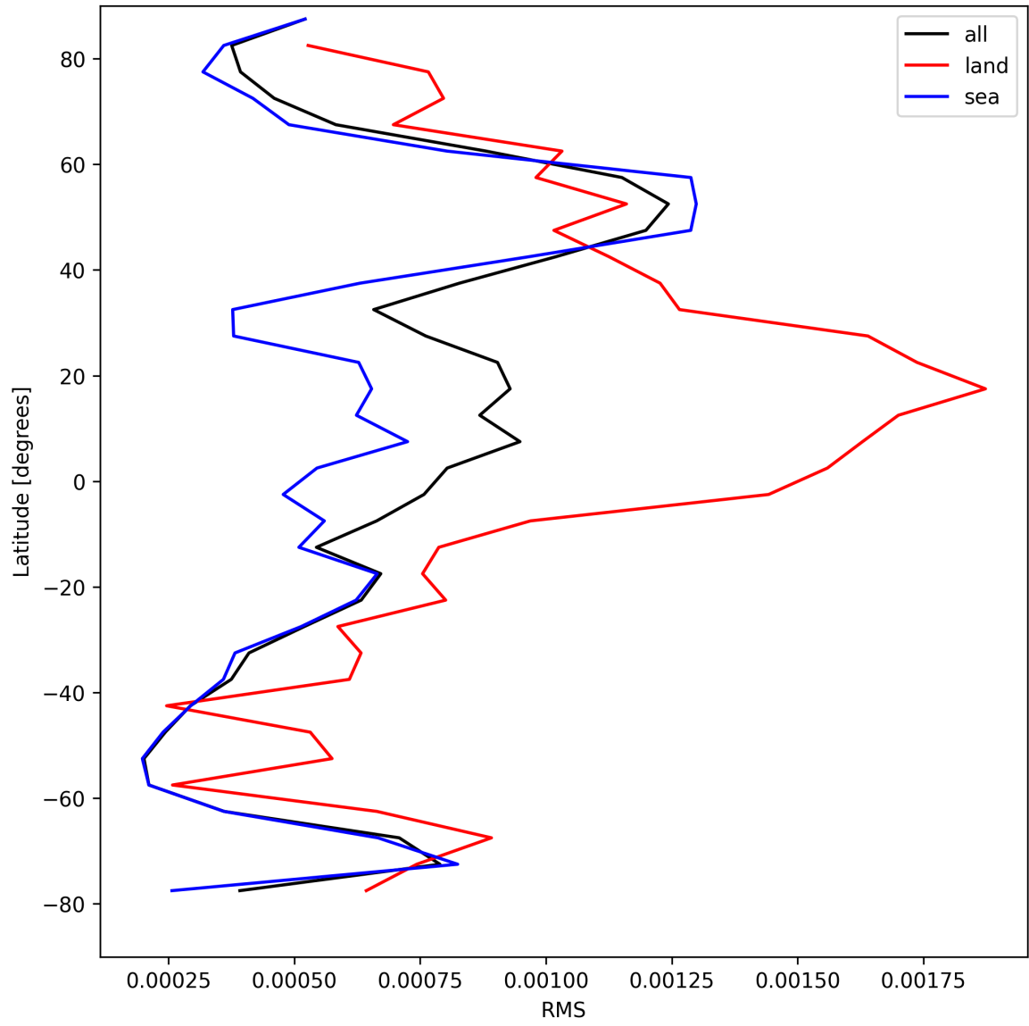
Figure 31: Zonal average of “RMS” for 2025-08-14 to 2025-08-16.
