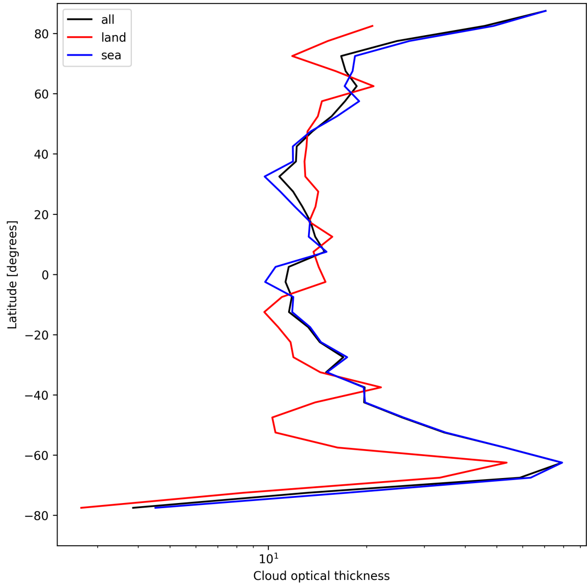
Figure 25: Zonal average of “Cloud optical thickness” for 2025-08-14 to 2025-08-16.
