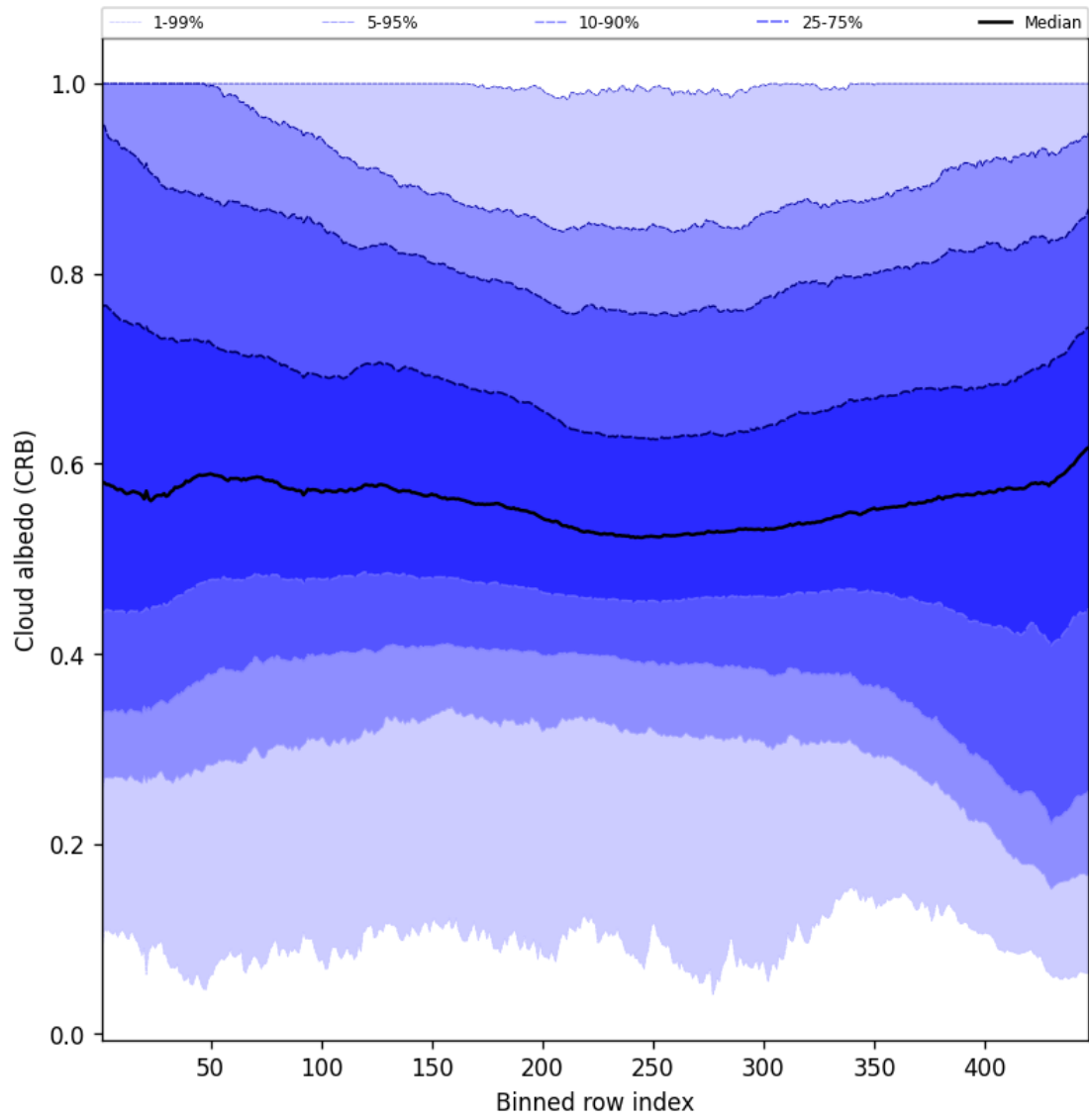
Figure 60: Along track statistics of “Cloud albedo (CRB)” for 2025-08-14 to 2025-08-16
