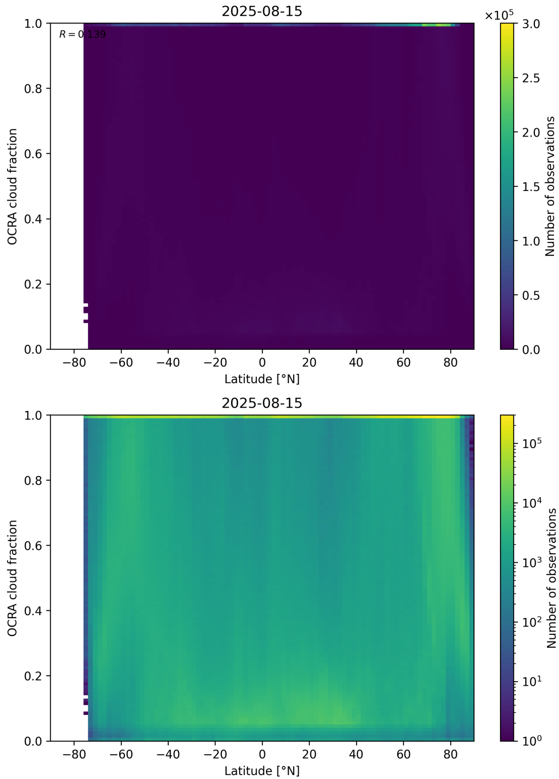
Figure 93: Scatter density plot of “Latitude” against “OCRA cloud fraction” for 2025-08-14 to 2025-08-16.
