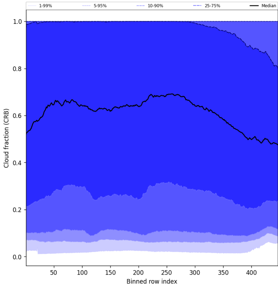
Figure 58: Along track statistics of “Cloud fraction (CRB)” for 2025-08-14 to 2025-08-16
