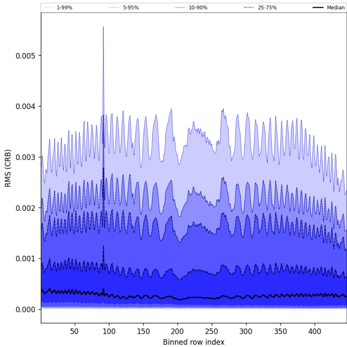
Figure 64: Along track statistics of “RMS (CRB)” for 2025-08-14 to 2025-08-16
