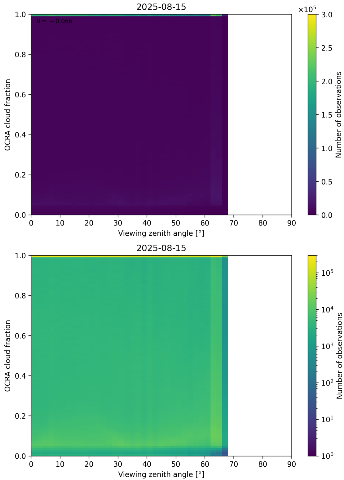
Figure 108: Scatter density plot of “Viewing zenith angle” against “OCRA cloud fraction” for 2025-08-14 to 2025-08-16.
