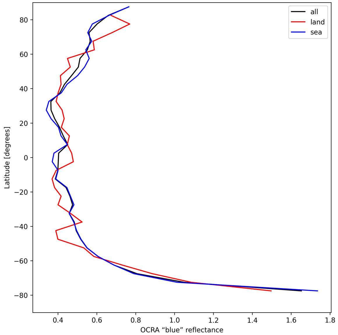
Figure 35: Zonal average of “OCRA “blue” reflectance” for 2025-08-14 to 2025-08-16.
