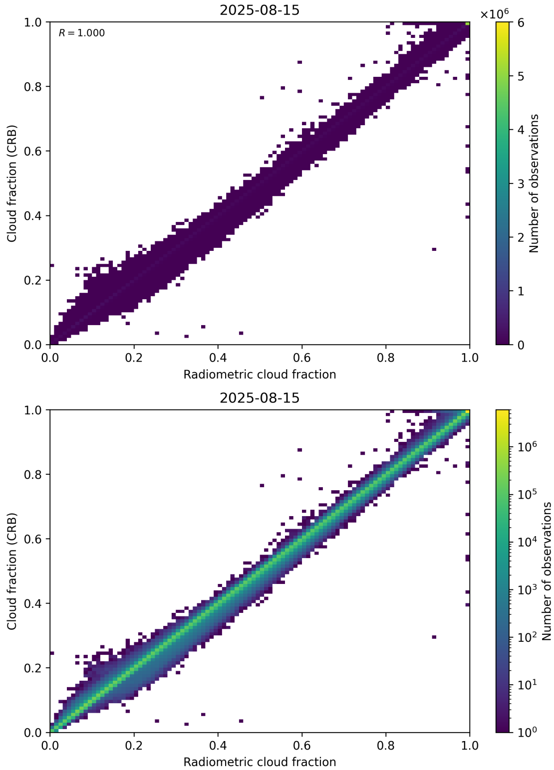
Figure 73: Scatter density plot of “Radiometric cloud fraction” against “Cloud fraction (CRB)” for 2025-08-14 to 2025-08-16.
