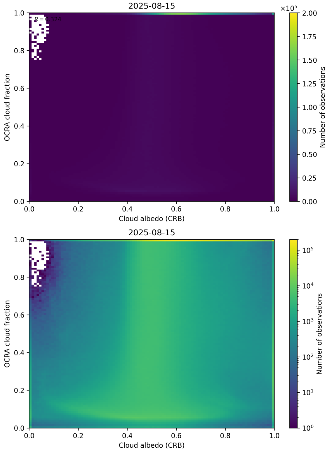
Figure 70: Scatter density plot of “Cloud albedo (CRB)” against “OCRA cloud fraction” for 2025-08-14 to 2025-08-16.
