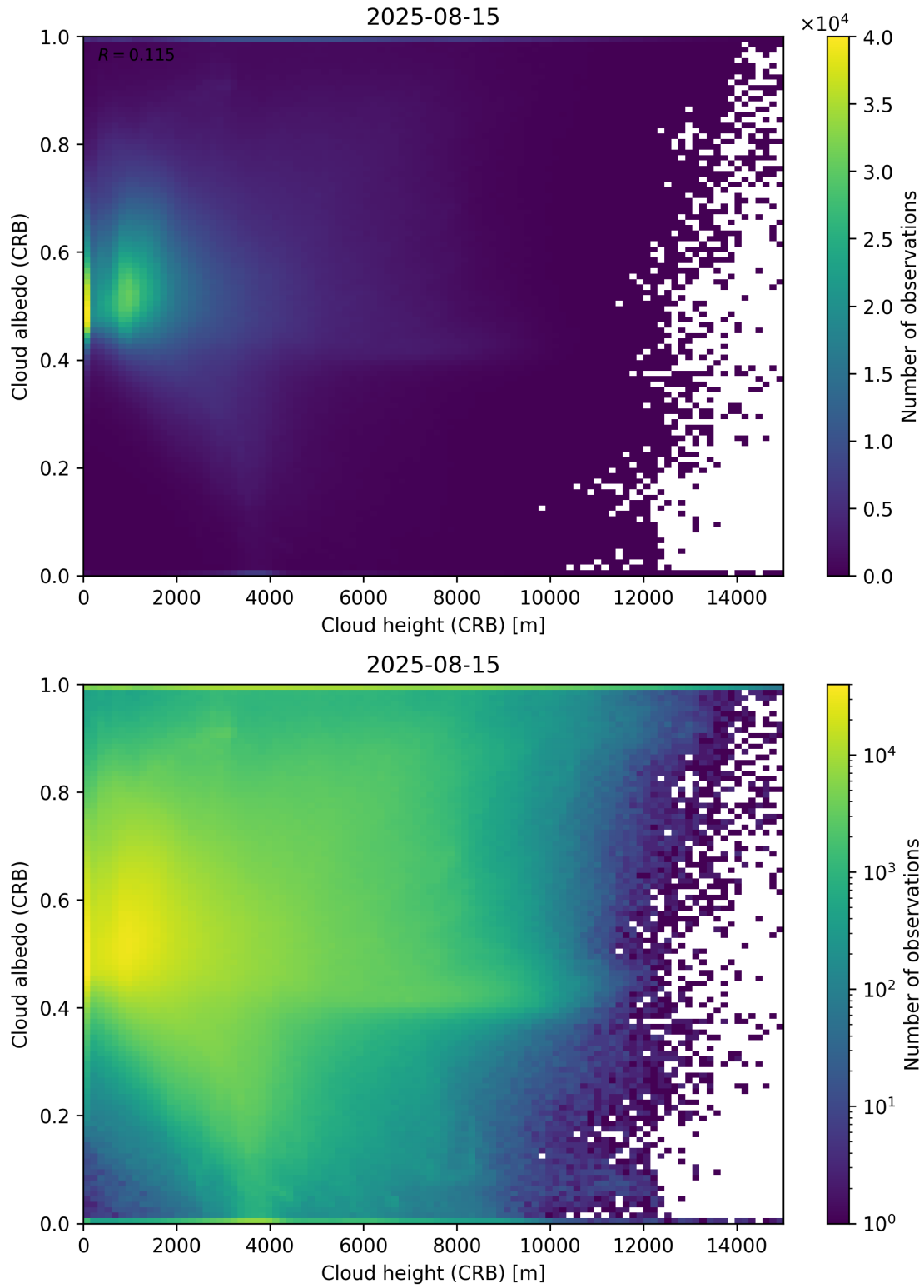
Figure 80: Scatter density plot of “Cloud height (CRB)” against “Cloud albedo (CRB)” for 2025-08-14 to 2025-08-16.
