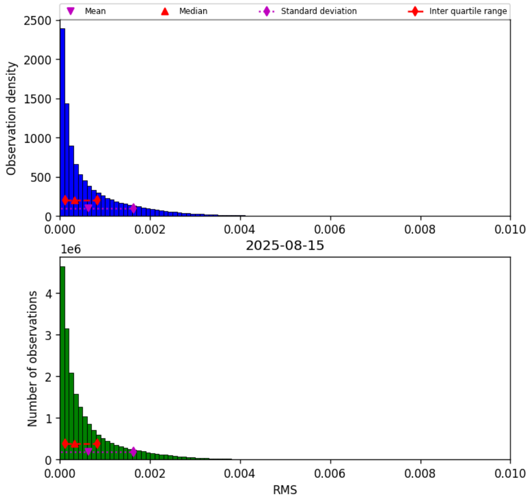
Figure 47: Histogram of “RMS” for 2025-08-14 to 2025-08-16
