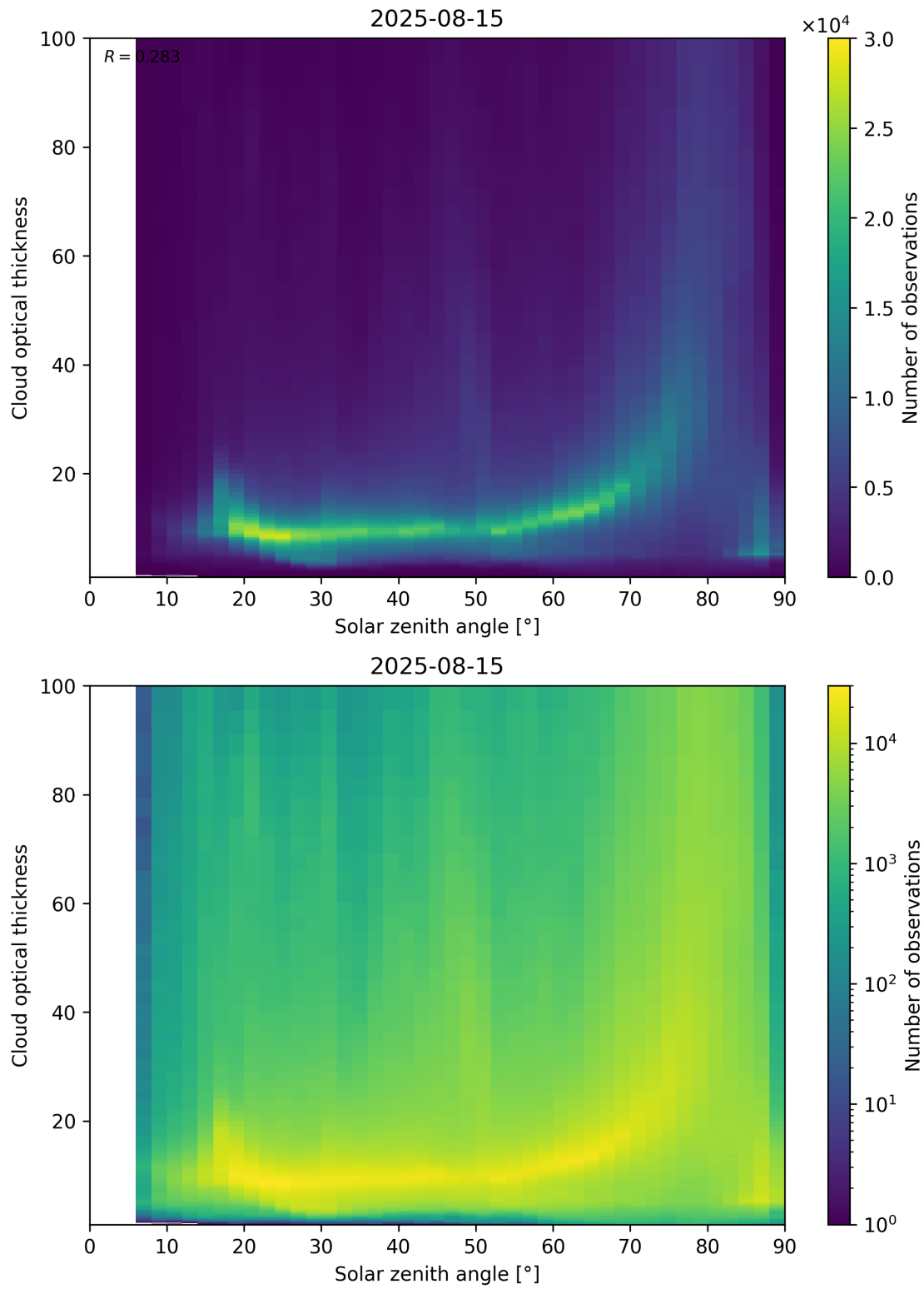
Figure 103: Scatter density plot of “Solar zenith angle” against “Cloud optical thickness” for 2025-08-14 to 2025-08-16.
