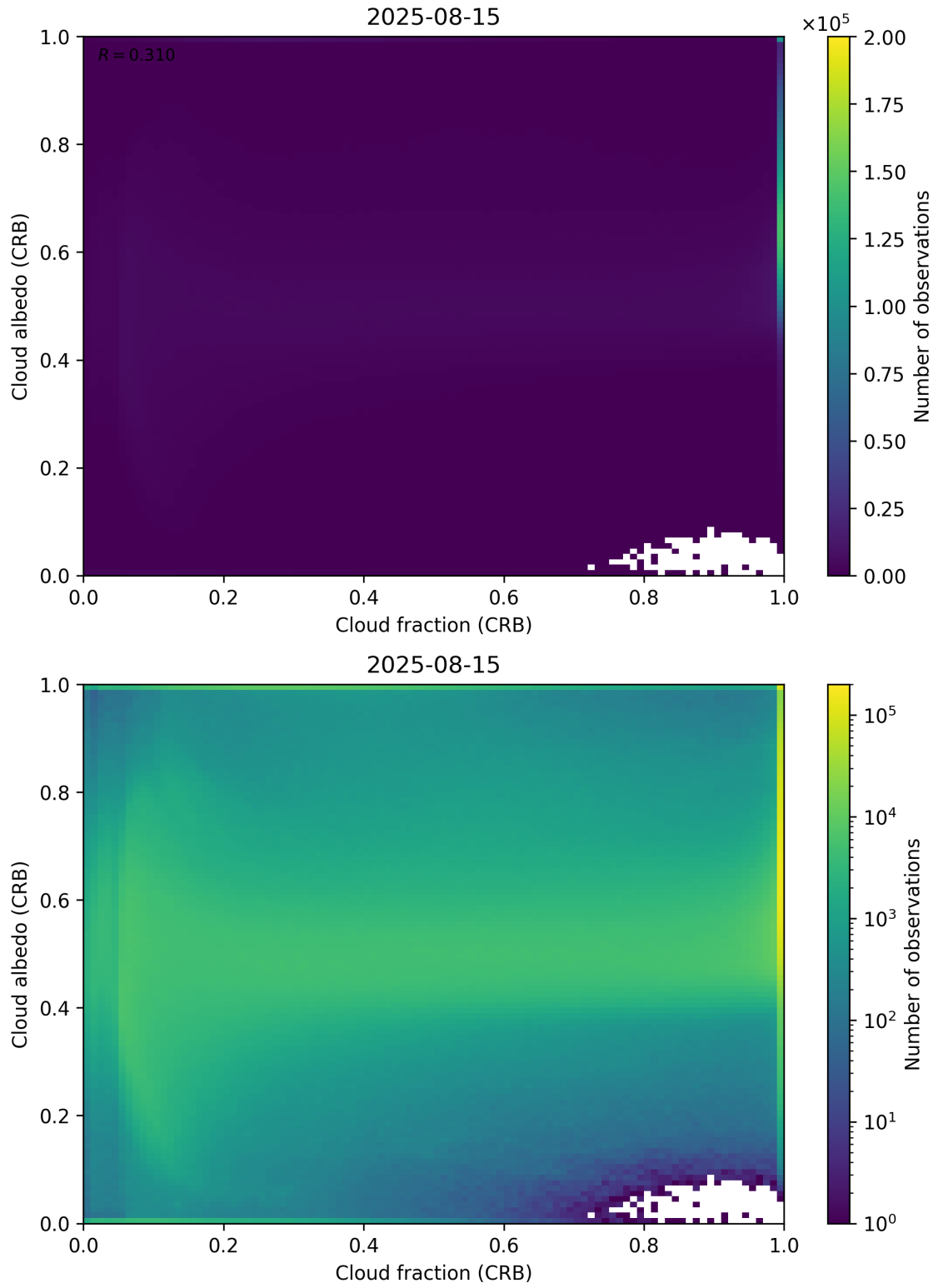
Figure 77: Scatter density plot of “Cloud fraction (CRB)” against “Cloud albedo (CRB)” for 2025-08-14 to 2025-08-16.
