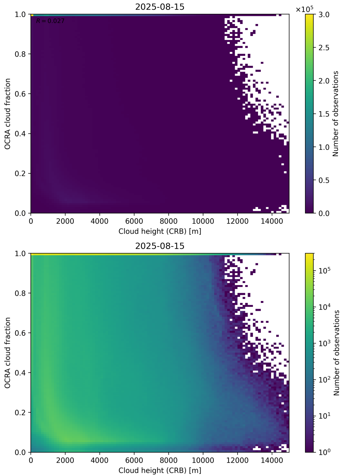
Figure 81: Scatter density plot of “Cloud height (CRB)” against “OCRA cloud fraction” for 2025-08-14 to 2025-08-16.
