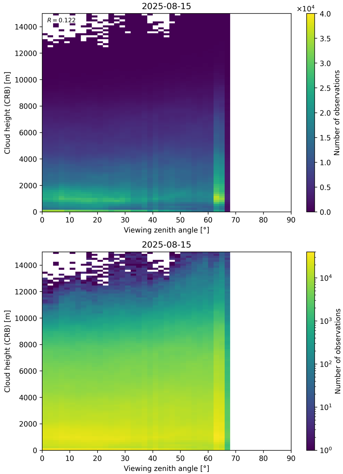
Figure 110: Scatter density plot of “Viewing zenith angle” against “Cloud height (CRB)” for 2025-08-14 to 2025-08-16.
