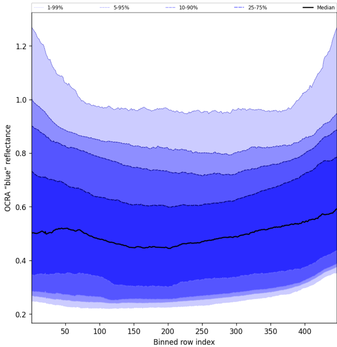
Figure 67: Along track statistics of “OCRA “blue” reflectance” for 2025-08-14 to 2025-08-16
