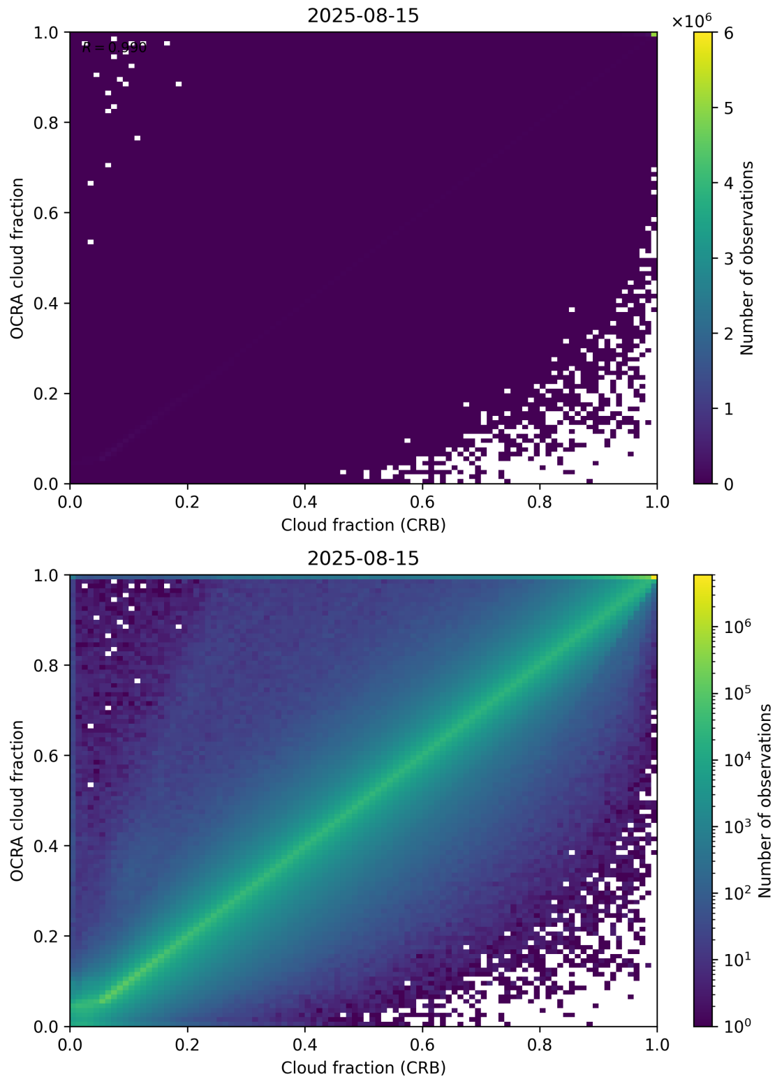
Figure 78: Scatter density plot of “Cloud fraction (CRB)” against “OCRA cloud fraction” for 2025-08-14 to 2025-08-16.
