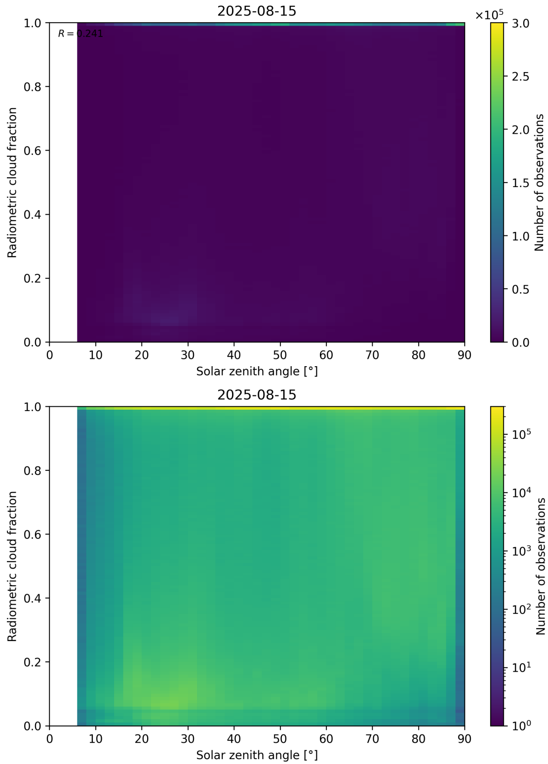
Figure 99: Scatter density plot of “Solar zenith angle” against “Radiometric cloud fraction” for 2025-08-14 to 2025-08-16.
