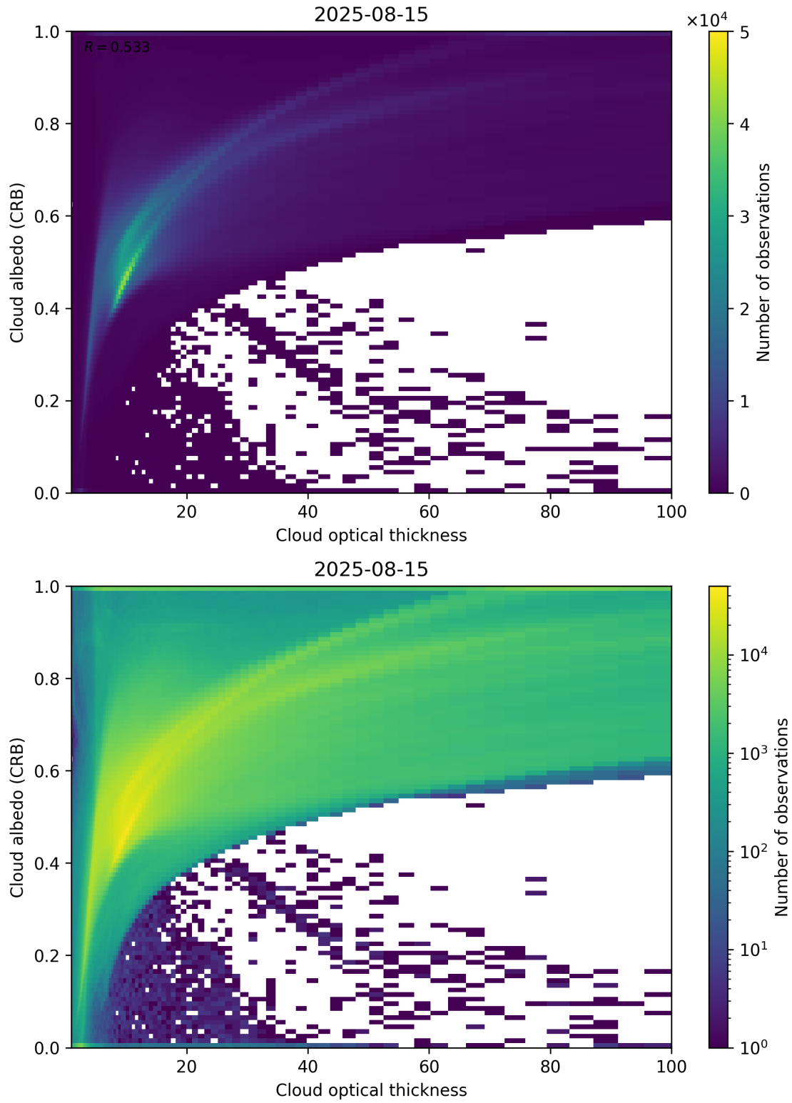
Figure 82: Scatter density plot of “Cloud optical thickness” against “Cloud albedo (CRB)” for 2025-08-14 to 2025-08-16.
