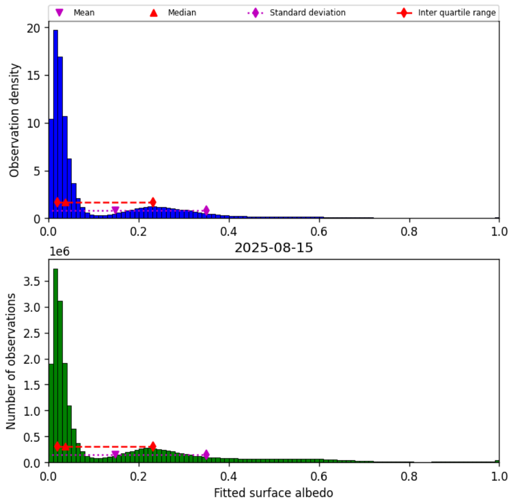
Figure 45: Histogram of “Fitted surface albedo” for 2025-08-14 to 2025-08-16
