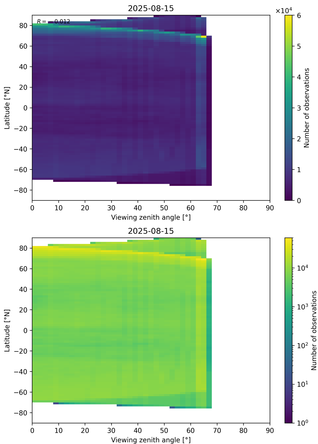
Figure 113: Scatter density plot of “Viewing zenith angle” against “Latitude” for 2025-08-14 to 2025-08-16.
