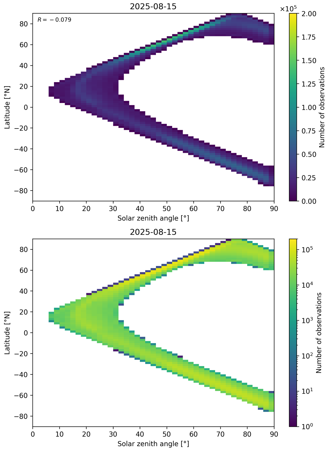
Figure 105: Scatter density plot of “Solar zenith angle” against “Latitude” for 2025-08-14 to 2025-08-16.
