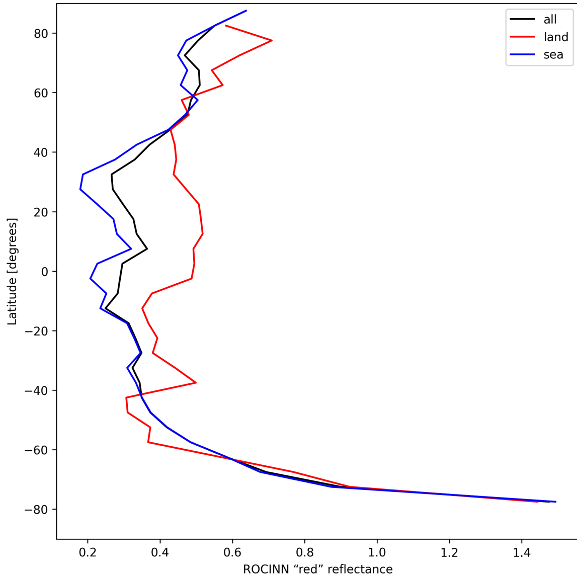
Figure 37: Zonal average of “ROCINN “red” reflectance” for 2025-08-14 to 2025-08-16.
