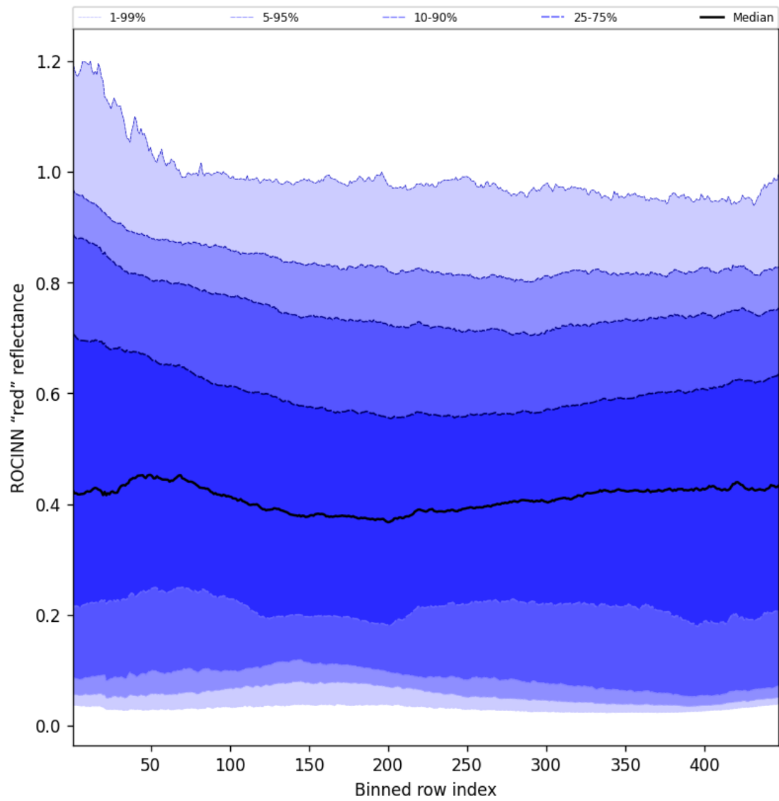
Figure 69: Along track statistics of “ROCINN “red” reflectance” for 2025-08-14 to 2025-08-16
