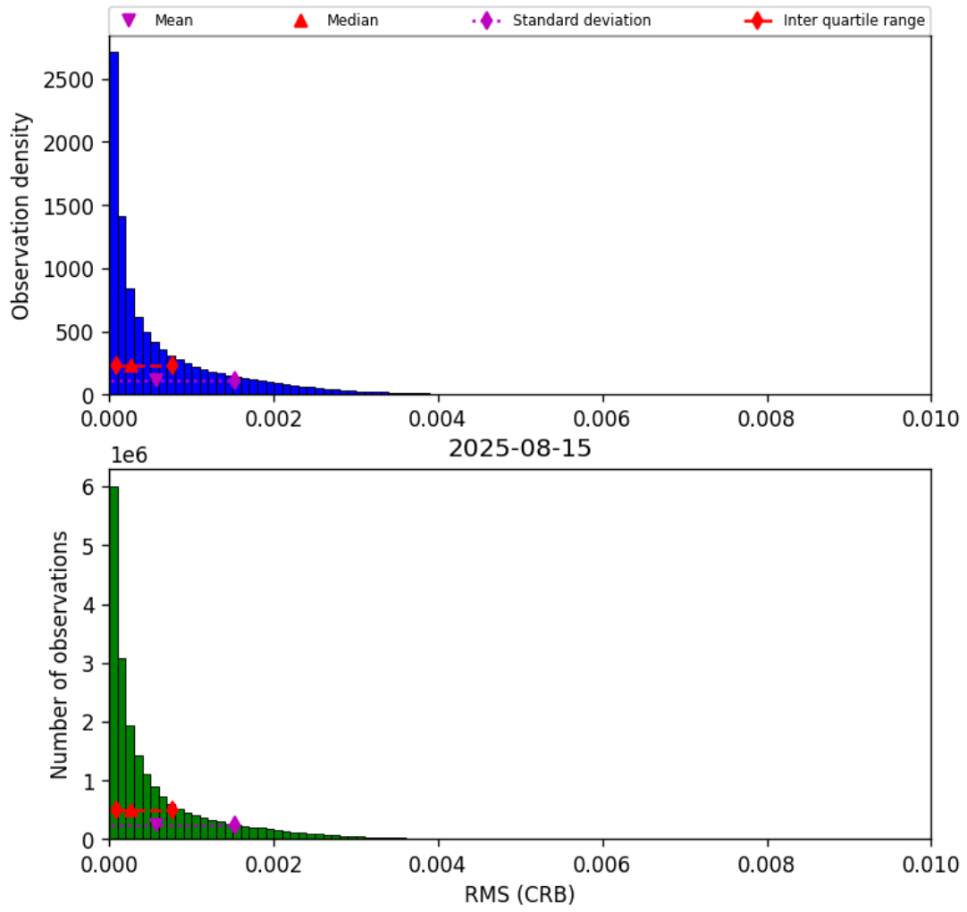
Figure 48: Histogram of “RMS (CRB)” for 2025-08-14 to 2025-08-16
