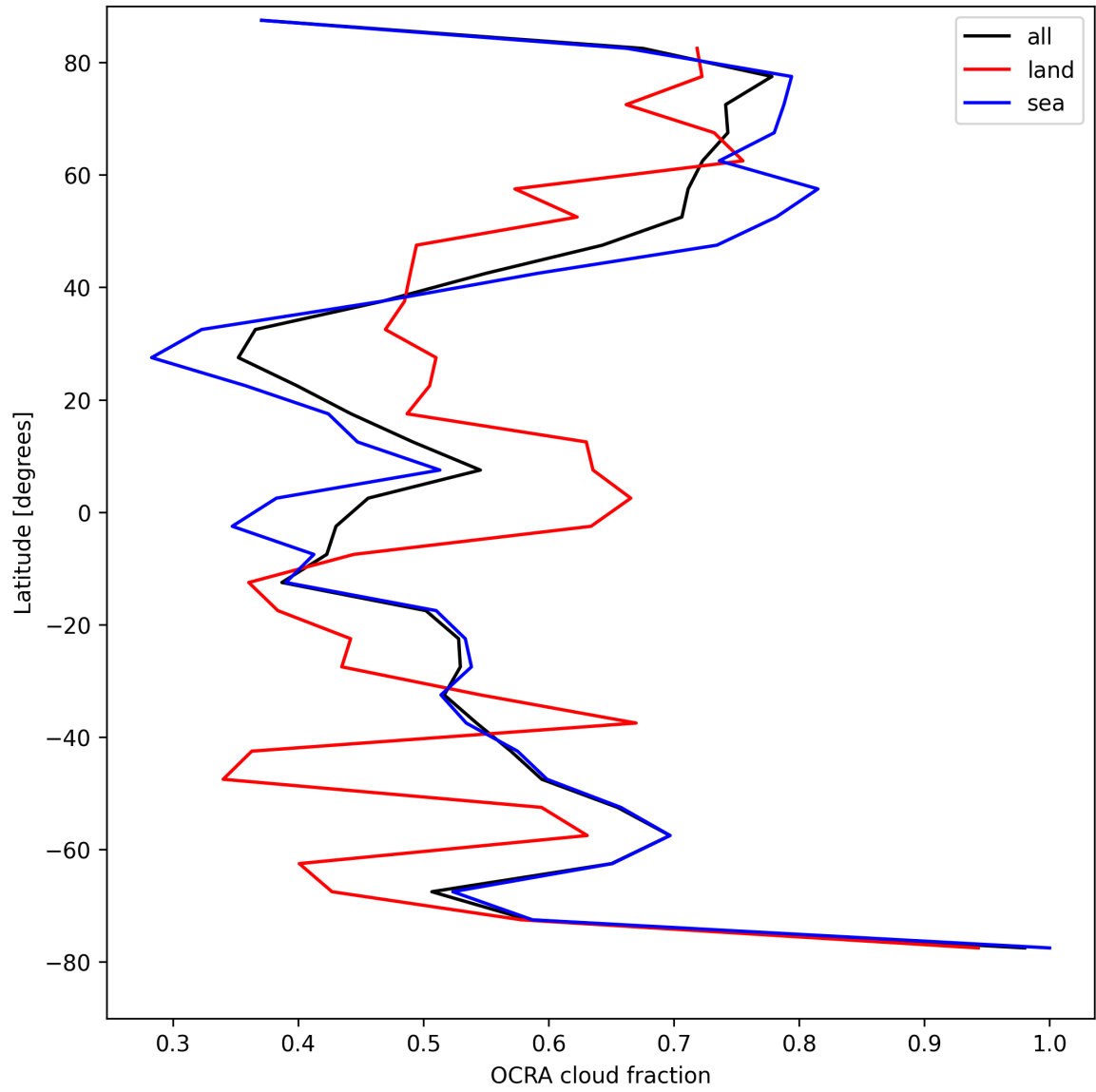
Figure 34: Zonal average of “OCRA cloud fraction” for 2025-08-14 to 2025-08-16.
