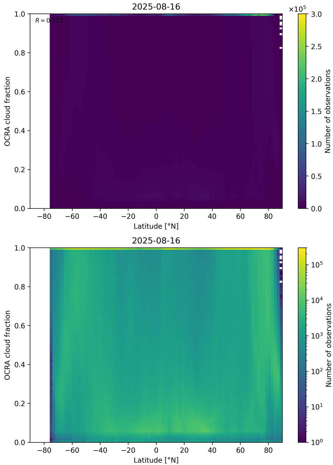
Figure 93: Scatter density plot of “Latitude” against “OCRA cloud fraction” for 2025-08-15 to 2025-08-17.
