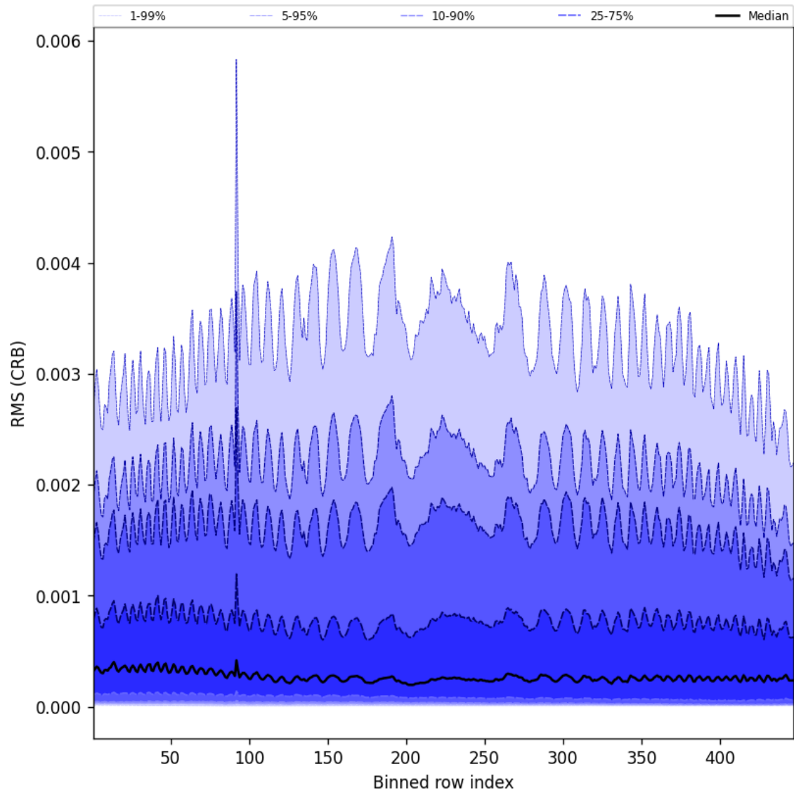
Figure 64: Along track statistics of “RMS (CRB)” for 2025-08-15 to 2025-08-17
