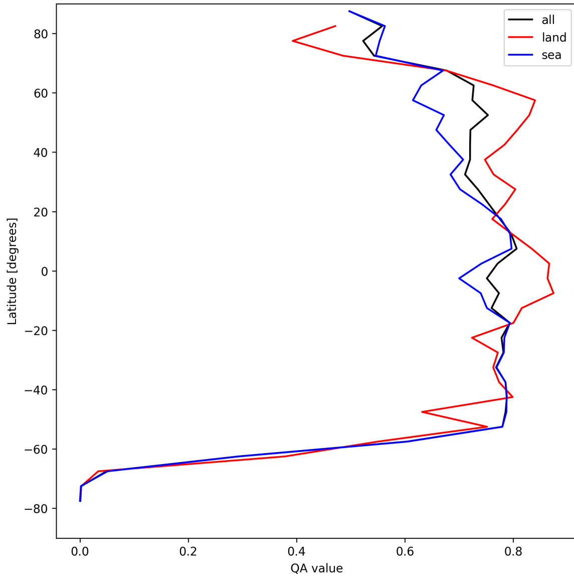
Figure 22: Zonal average of “QA value” for 2025-08-15 to 2025-08-17.
