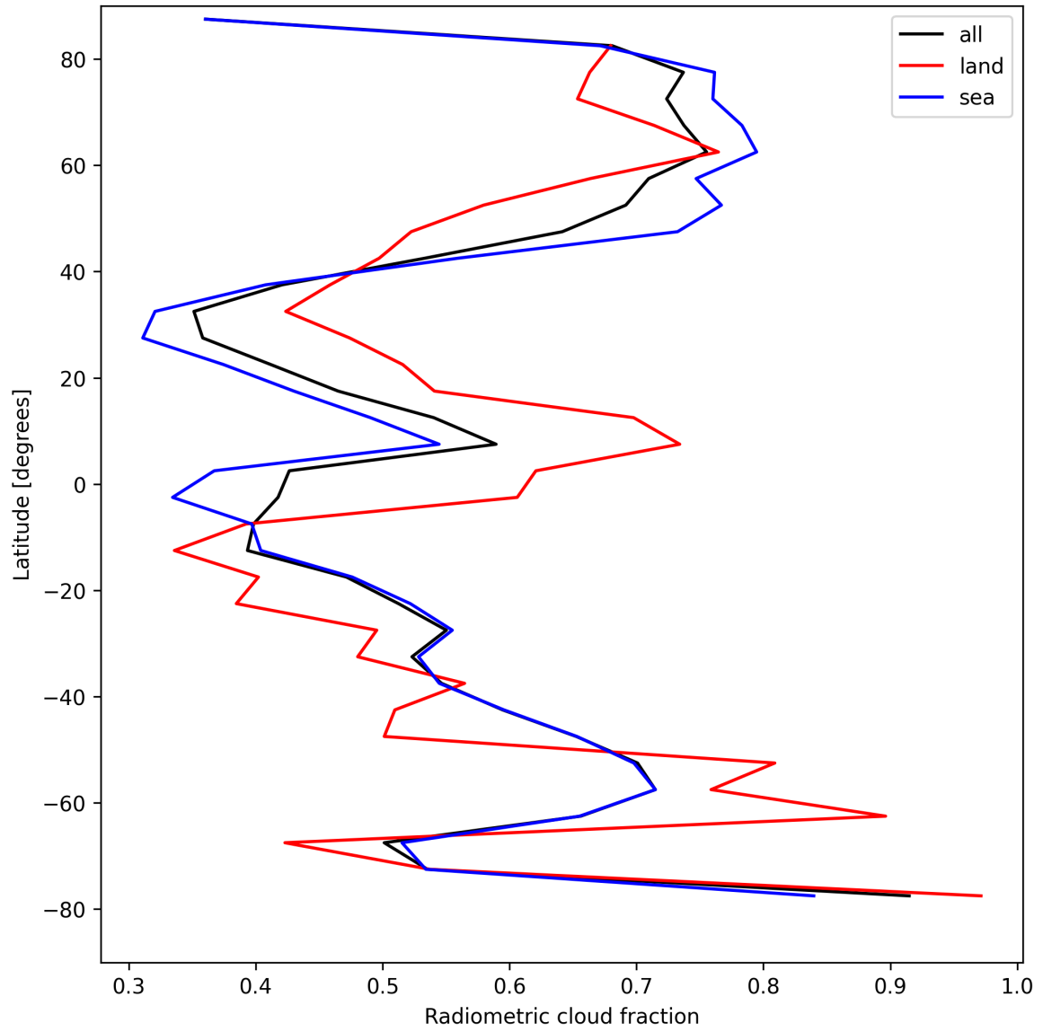
Figure 23: Zonal average of “Radiometric cloud fraction” for 2025-08-15 to 2025-08-17.
