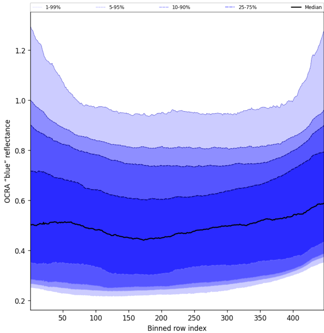
Figure 67: Along track statistics of “OCRA “blue” reflectance” for 2025-08-15 to 2025-08-17
