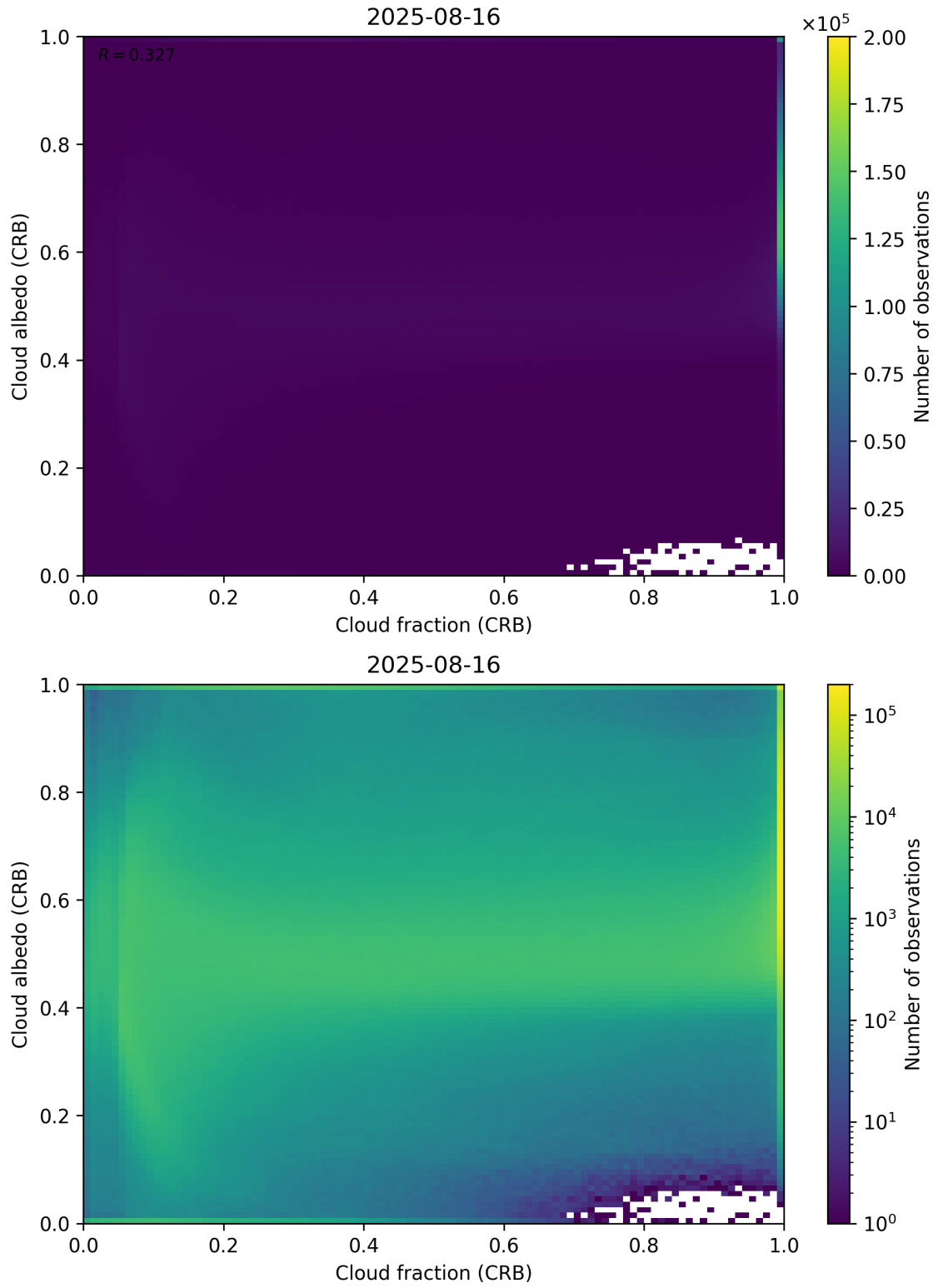
Figure 77: Scatter density plot of “Cloud fraction (CRB)” against “Cloud albedo (CRB)” for 2025-08-15 to 2025-08-17.
