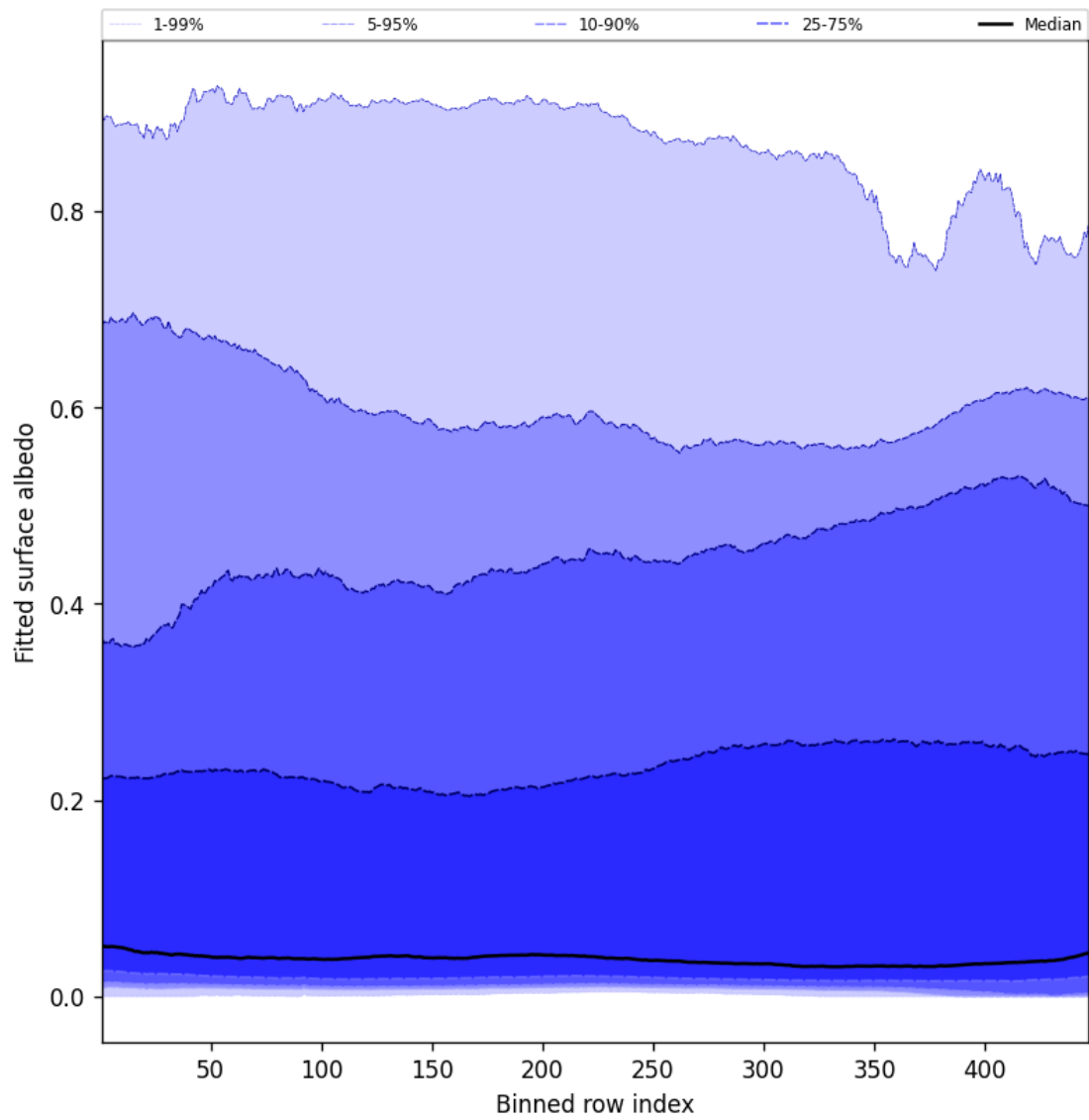
Figure 61: Along track statistics of “Fitted surface albedo” for 2025-08-15 to 2025-08-17
