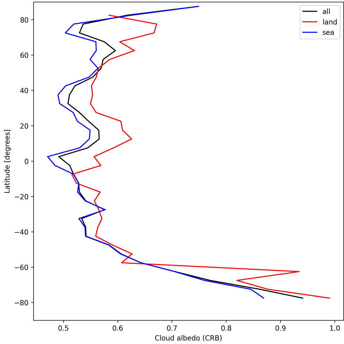
Figure 28: Zonal average of “Cloud albedo (CRB)” for 2025-08-15 to 2025-08-17.
