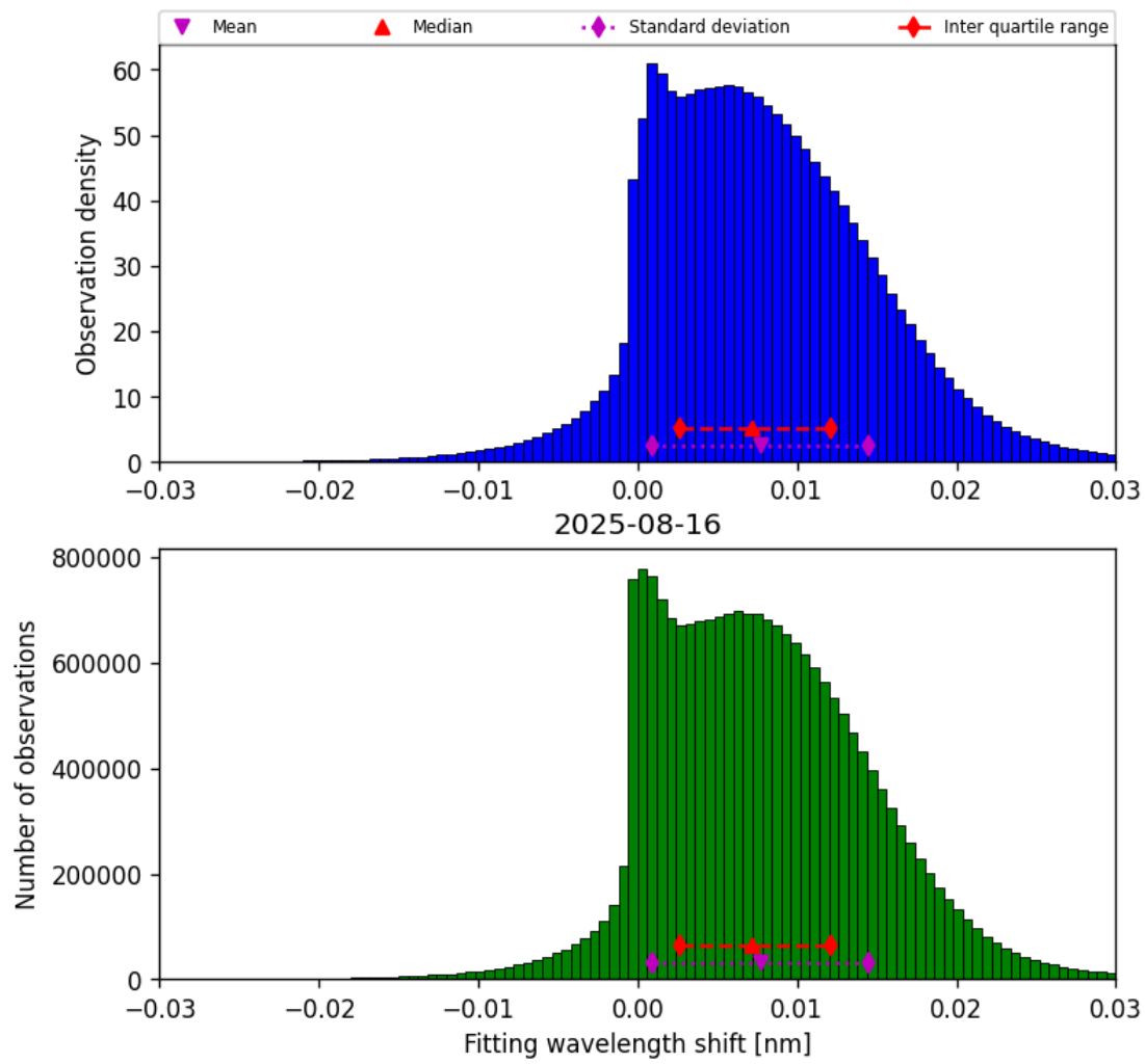
Figure 49: Histogram of “Fitting wavelength shift” for 2025-08-15 to 2025-08-17
