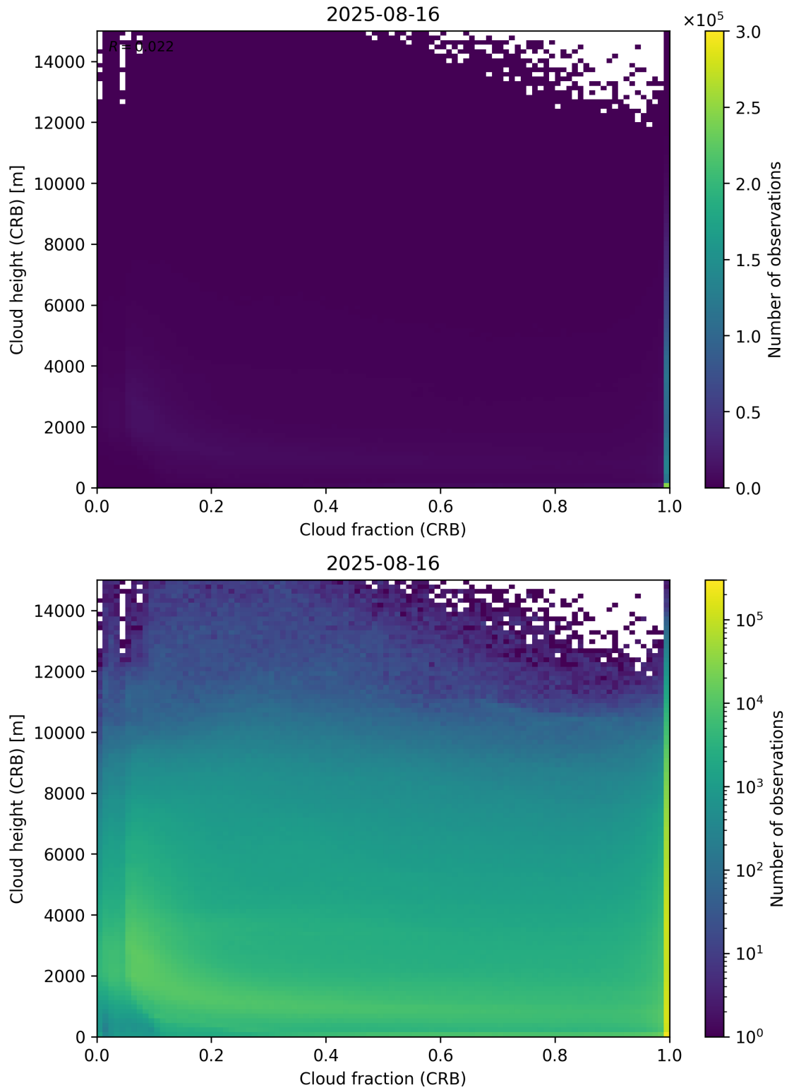
Figure 79: Scatter density plot of “Cloud fraction (CRB)” against “Cloud height (CRB)” for 2025-08-15 to 2025-08-17.
