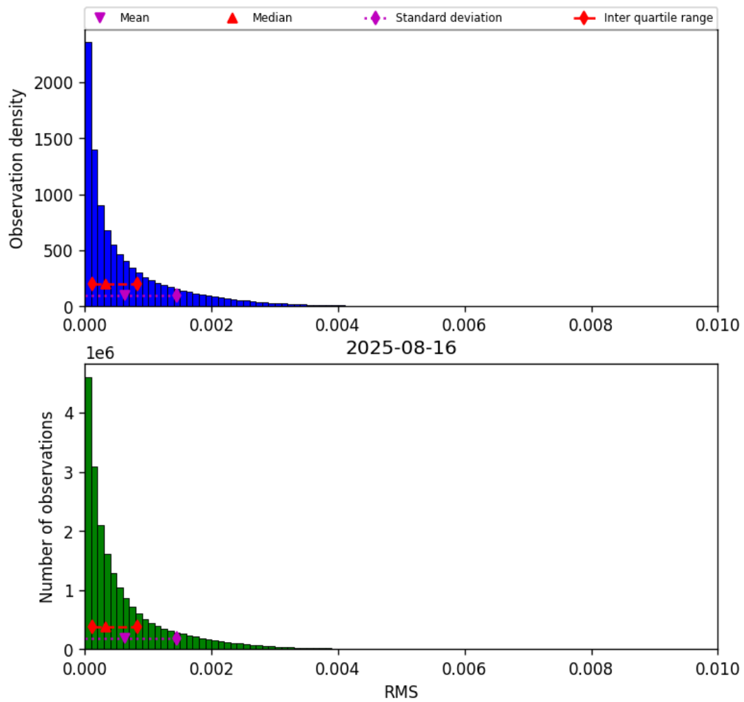
Figure 47: Histogram of “RMS” for 2025-08-15 to 2025-08-17
