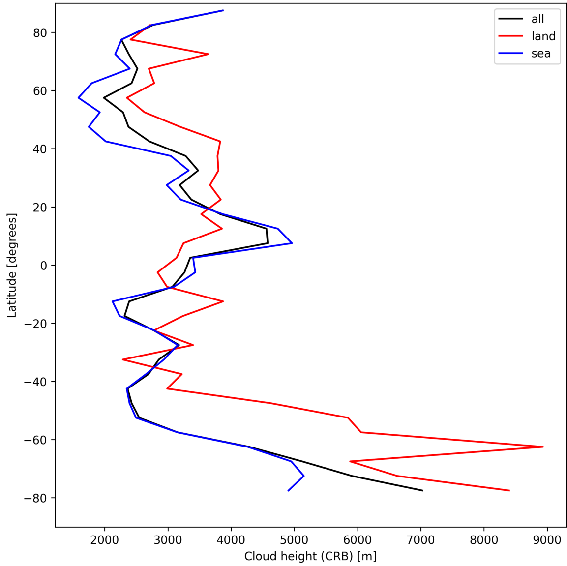
Figure 27: Zonal average of “Cloud height (CRB)” for 2025-08-15 to 2025-08-17.
