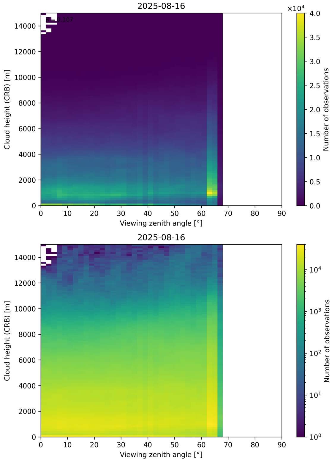
Figure 110: Scatter density plot of “Viewing zenith angle” against “Cloud height (CRB)” for 2025-08-15 to 2025-08-17.
