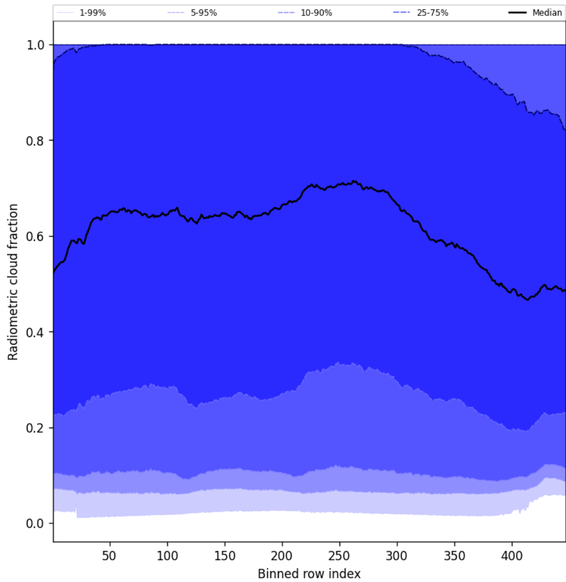
Figure 55: Along track statistics of “Radiometric cloud fraction” for 2025-08-15 to 2025-08-17
