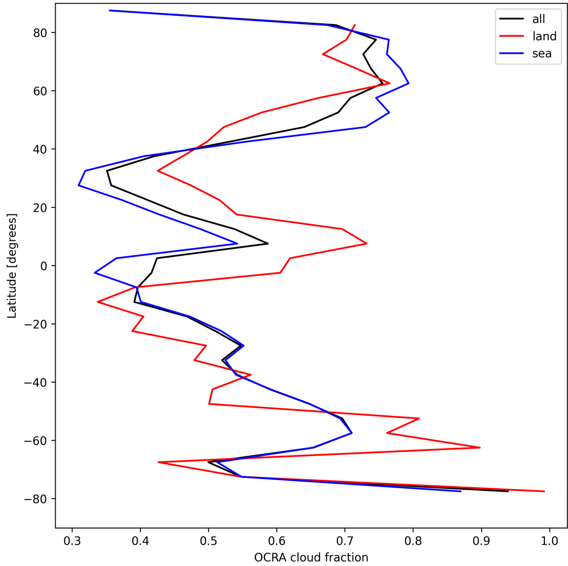
Figure 34: Zonal average of “OCRA cloud fraction” for 2025-08-15 to 2025-08-17.
