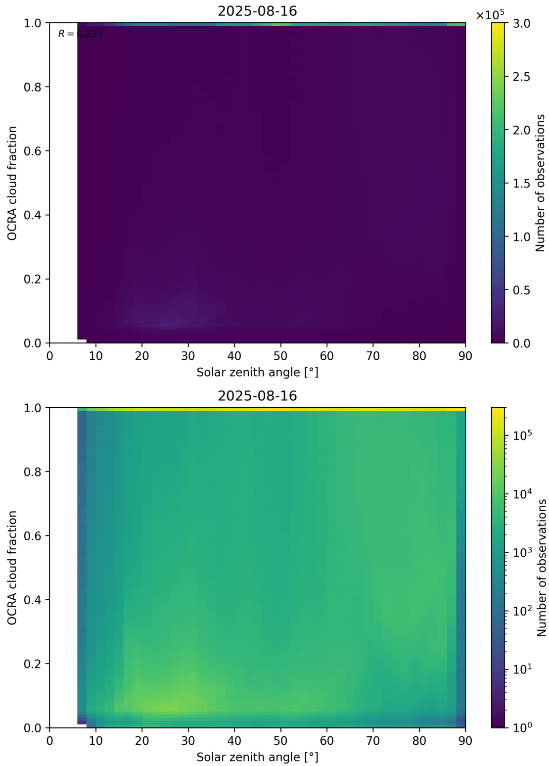
Figure 100: Scatter density plot of “Solar zenith angle” against “OCRA cloud fraction” for 2025-08-15 to 2025-08-17.
