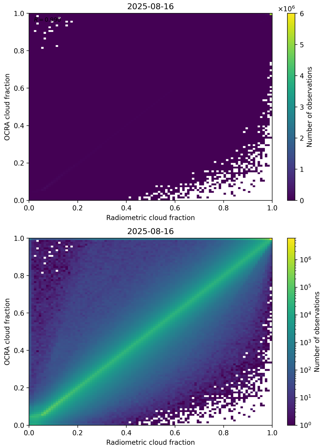
Figure 72: Scatter density plot of “Radiometric cloud fraction” against “OCRA cloud fraction” for 2025-08-15 to 2025-08-17.
