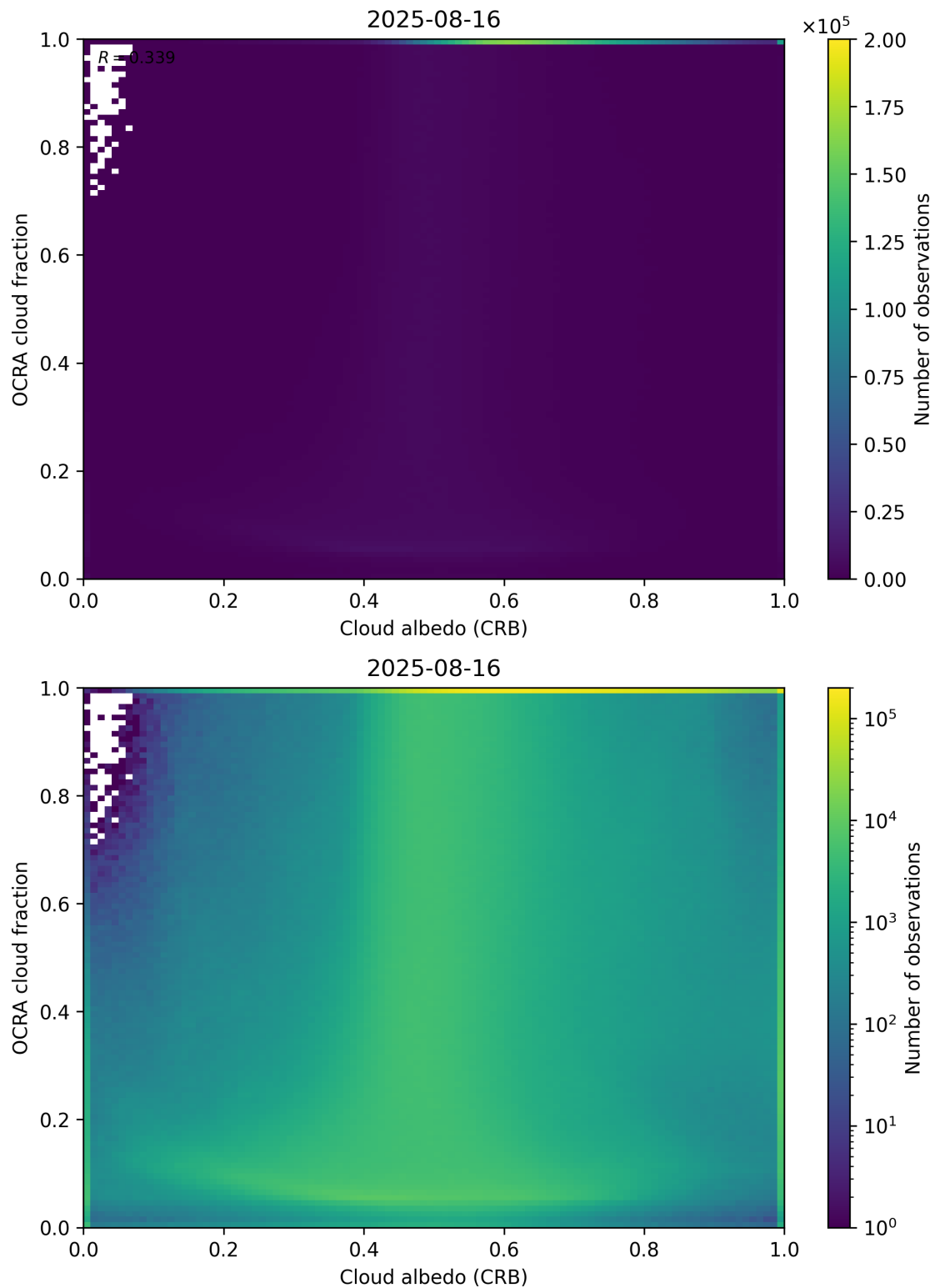
Figure 70: Scatter density plot of “Cloud albedo (CRB)” against “OCRA cloud fraction” for 2025-08-15 to 2025-08-17.
