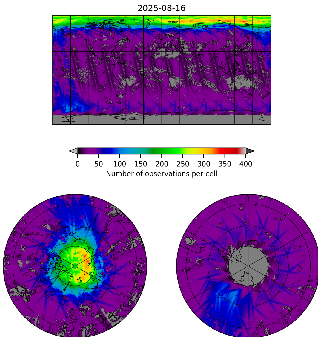
Figure 21: Map of the number of observations for 2025-08-15 to 2025-08-17
