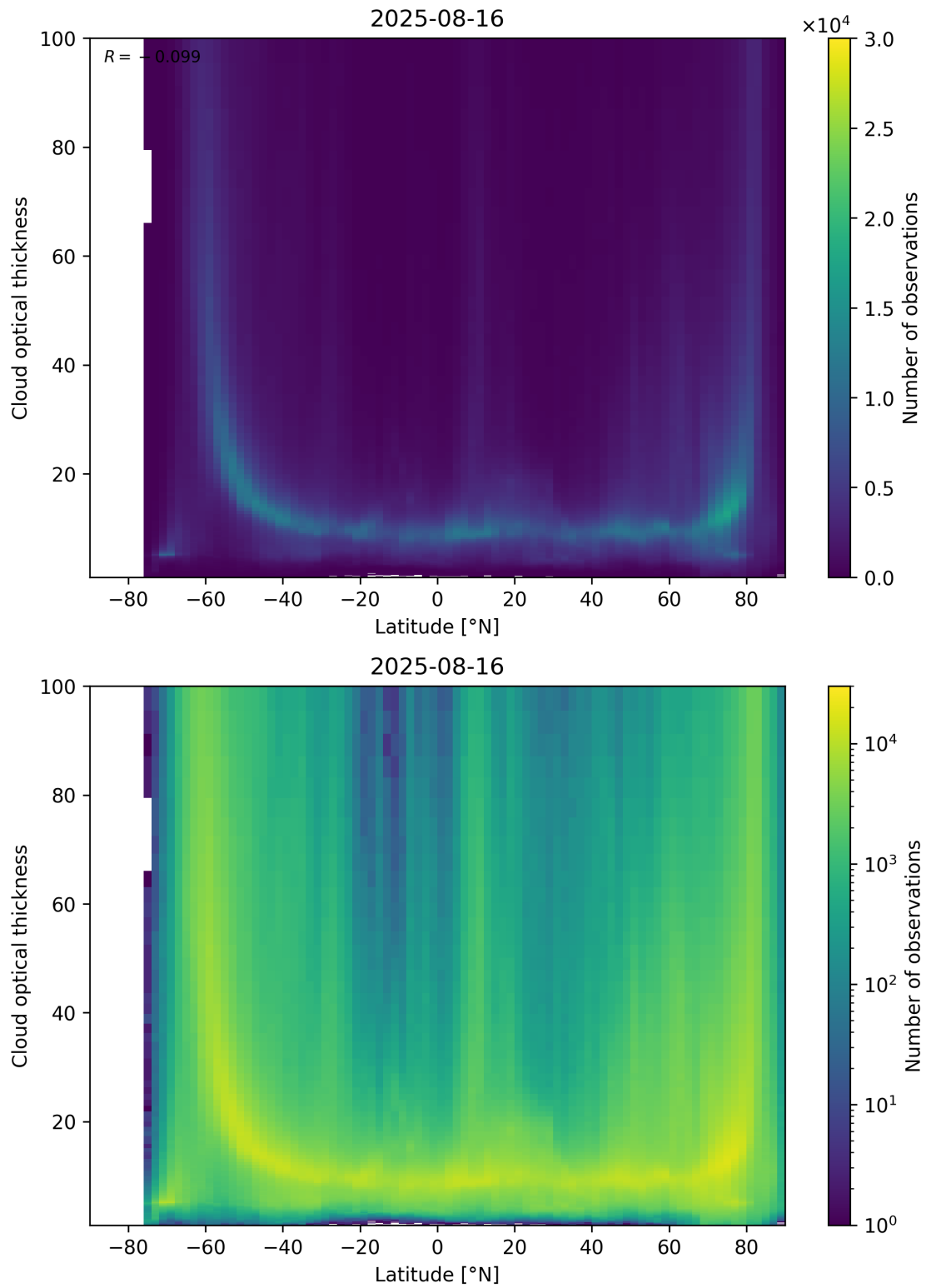
Figure 96: Scatter density plot of “Latitude” against “Cloud optical thickness” for 2025-08-15 to 2025-08-17.
