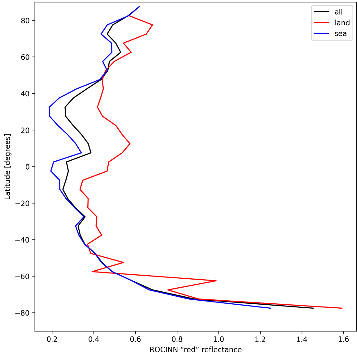
Figure 37: Zonal average of “ROCINN “red” reflectance” for 2025-08-15 to 2025-08-17.
