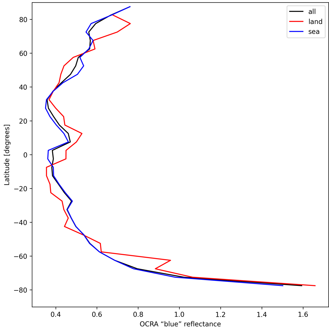
Figure 35: Zonal average of “OCRA “blue” reflectance” for 2025-08-15 to 2025-08-17.
