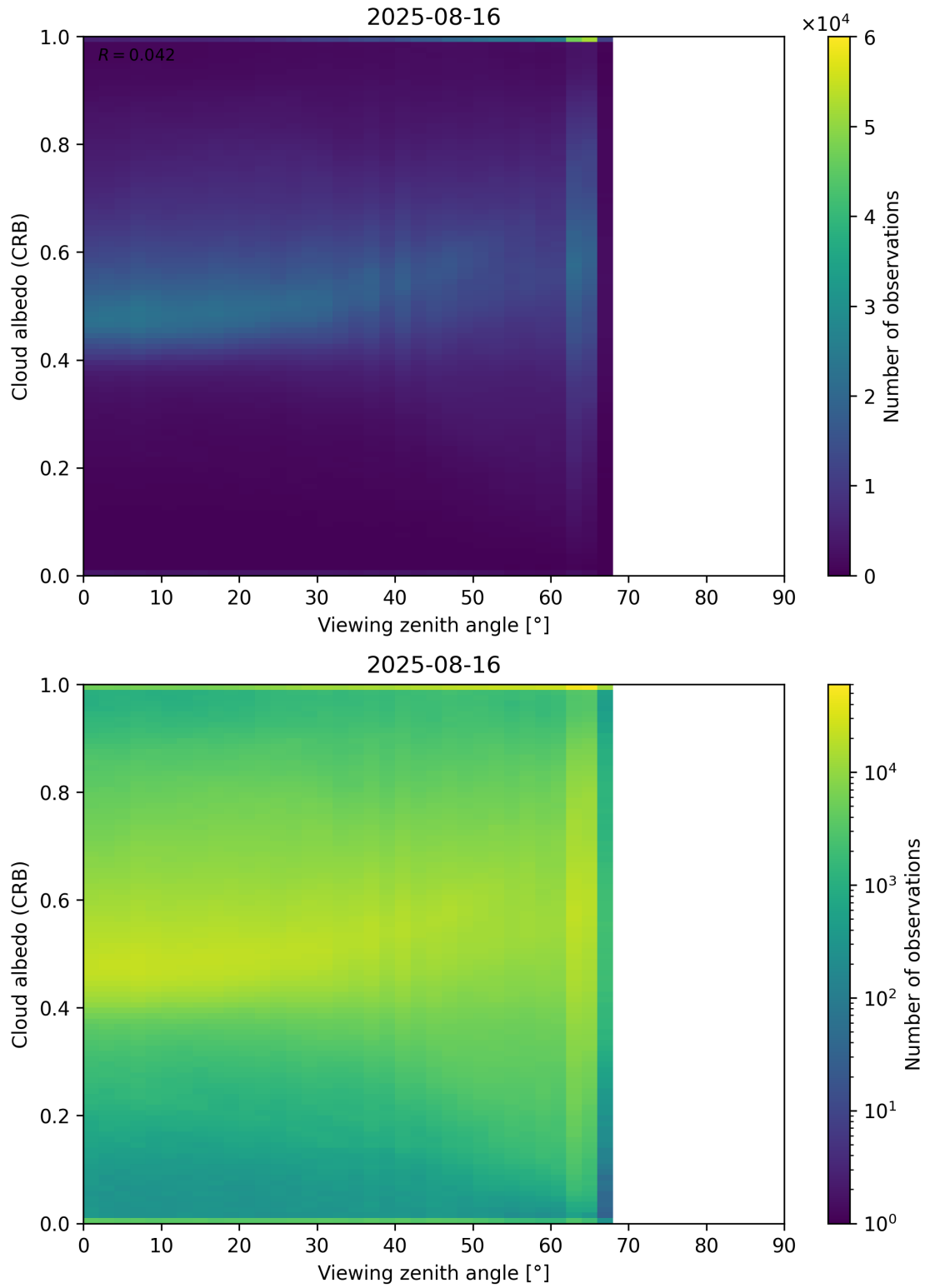
Figure 106: Scatter density plot of “Viewing zenith angle” against “Cloud albedo (CRB)” for 2025-08-15 to 2025-08-17.
