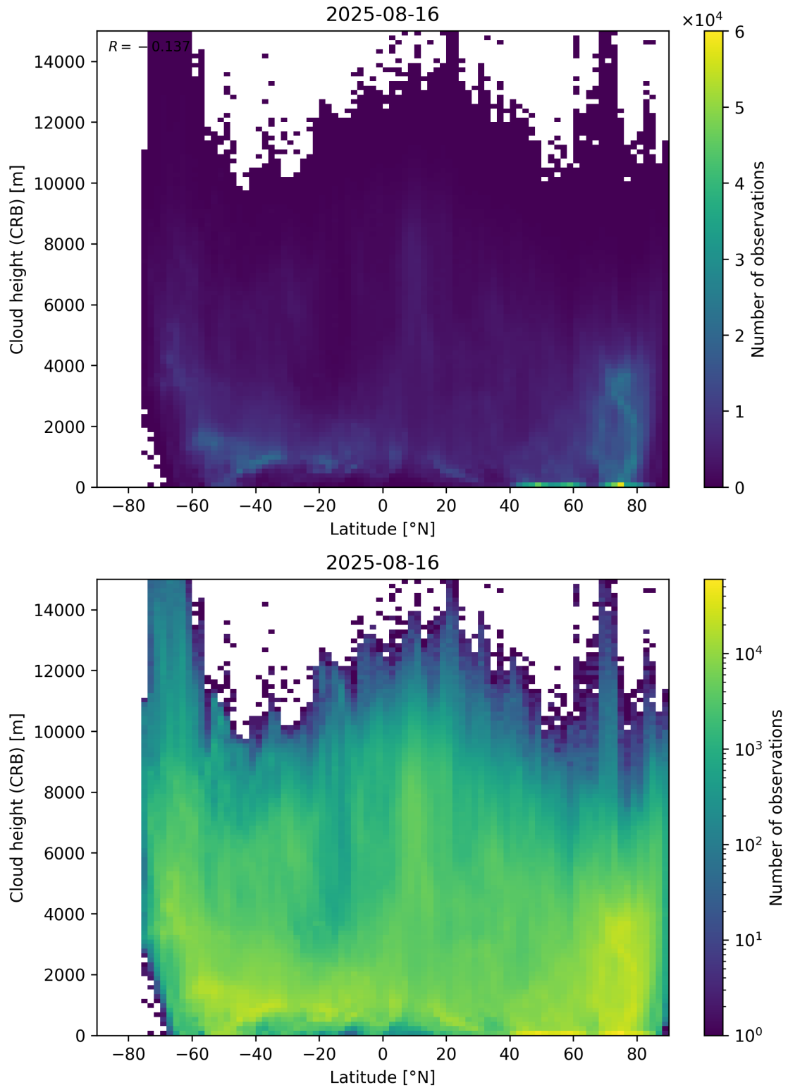
Figure 95: Scatter density plot of “Latitude” against “Cloud height (CRB)” for 2025-08-15 to 2025-08-17.
