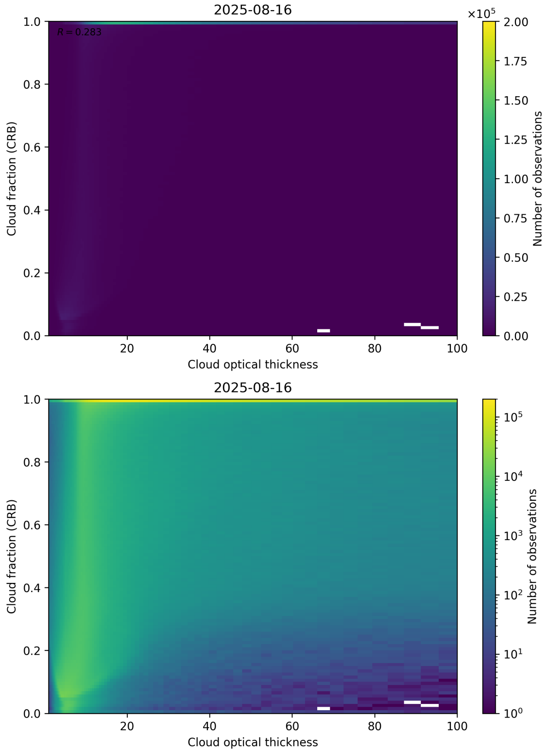
Figure 84: Scatter density plot of “Cloud optical thickness” against “Cloud fraction (CRB)” for 2025-08-15 to 2025-08-17.
