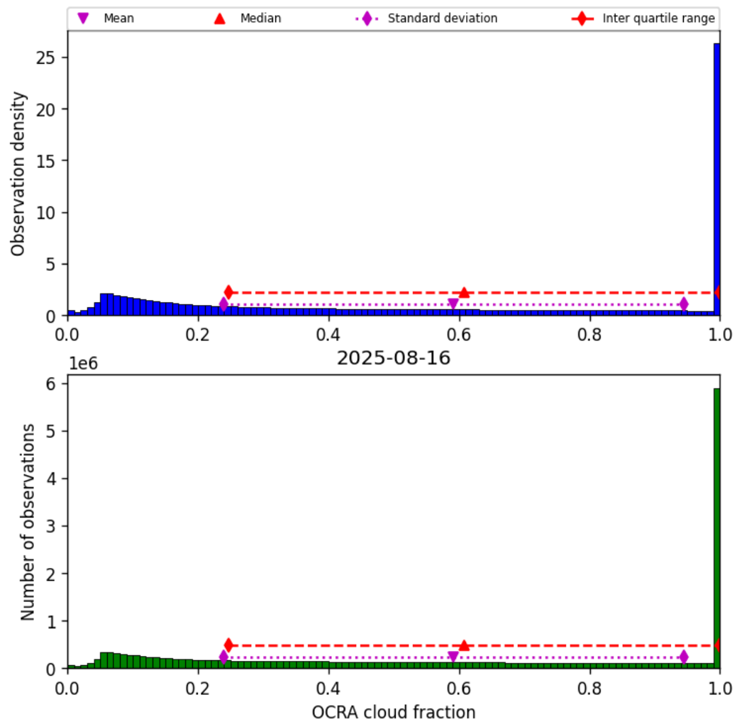
Figure 50: Histogram of “OCRA cloud fraction” for 2025-08-15 to 2025-08-17
