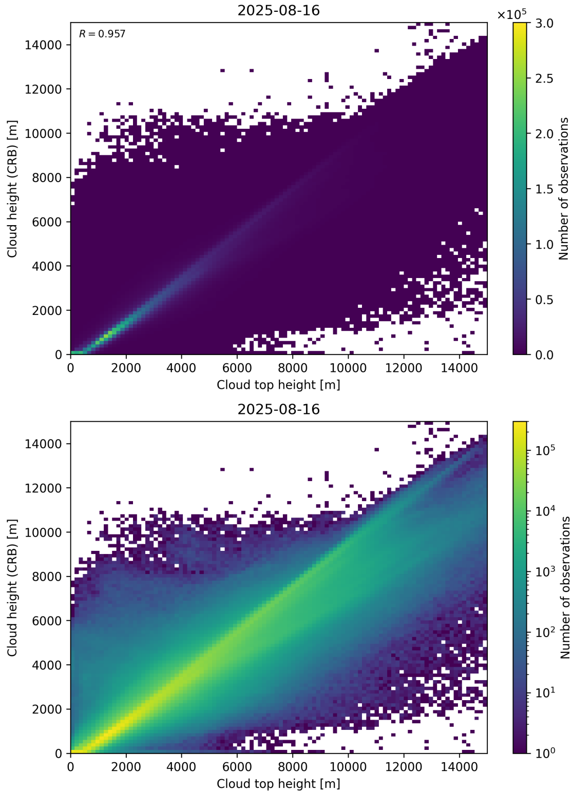
Figure 89: Scatter density plot of “Cloud top height” against “Cloud height (CRB)” for 2025-08-15 to 2025-08-17.
