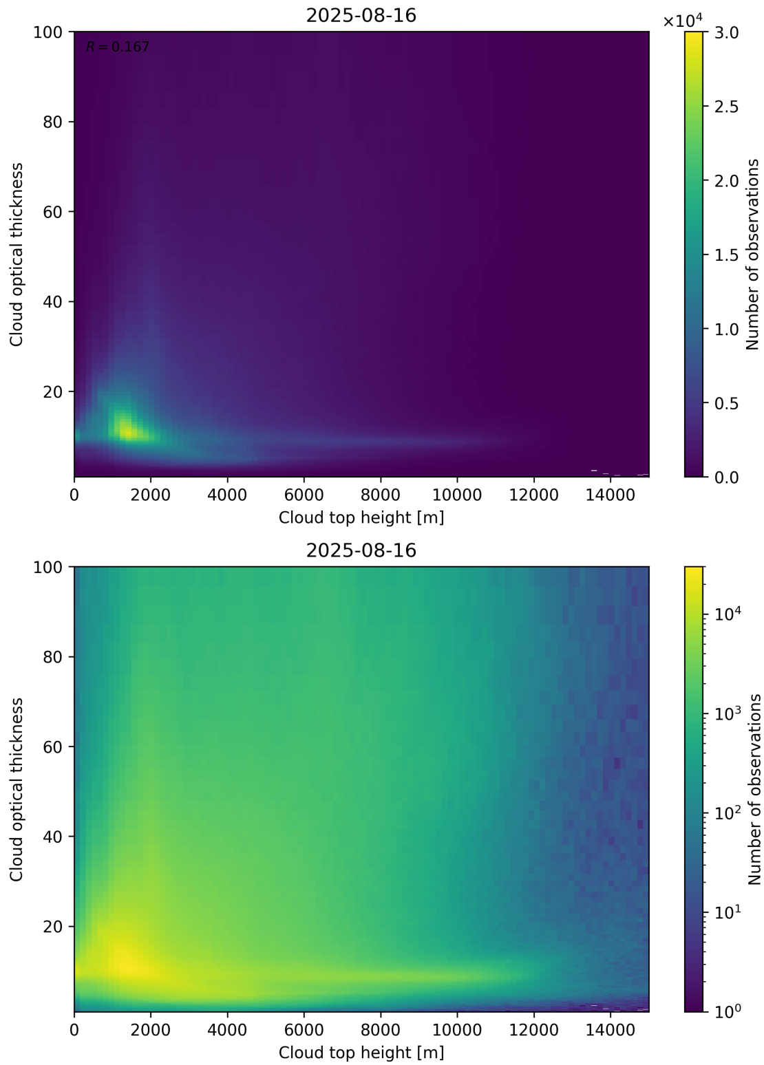
Figure 90: Scatter density plot of “Cloud top height” against “Cloud optical thickness” for 2025-08-15 to 2025-08-17.
