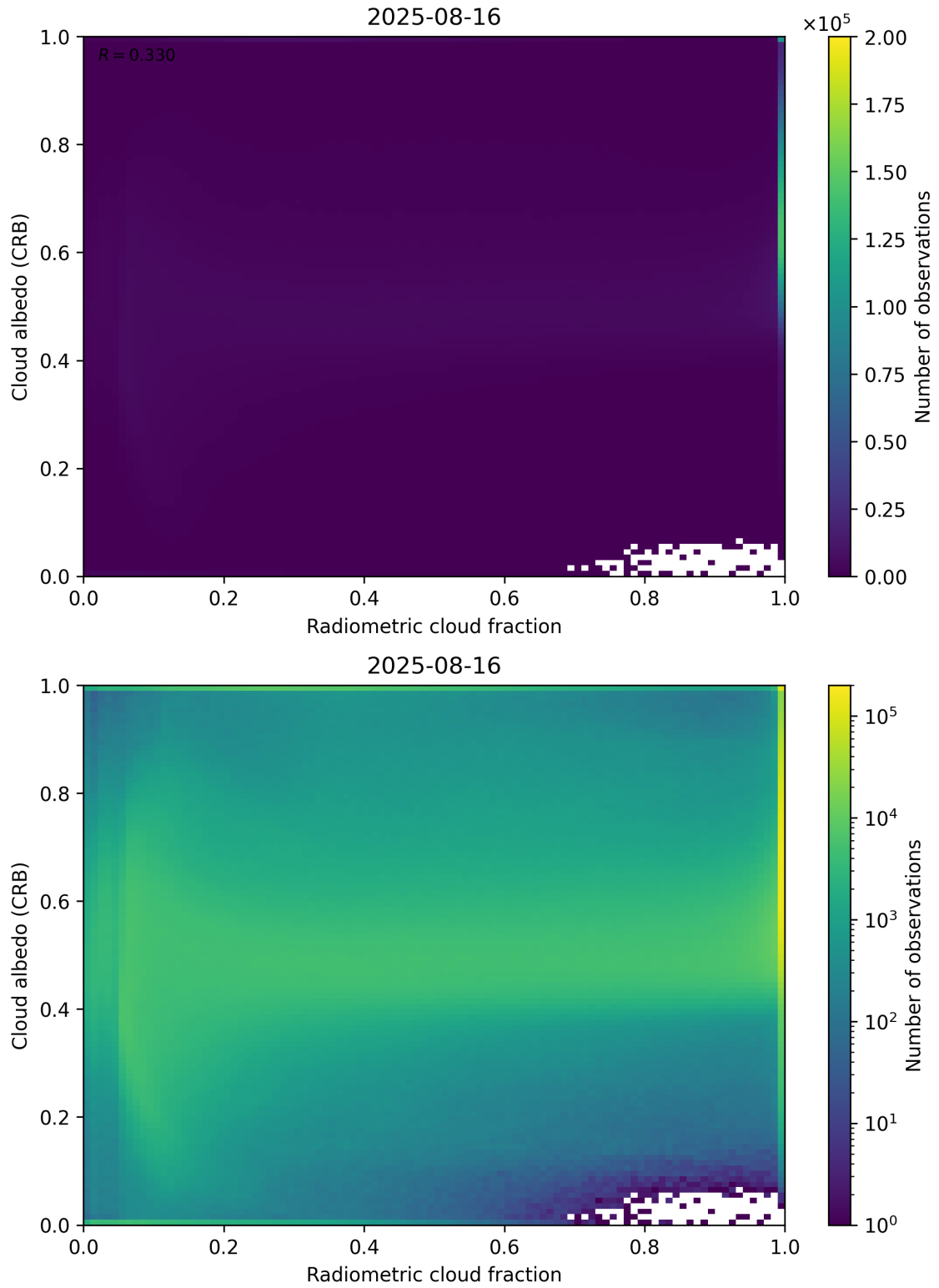
Figure 71: Scatter density plot of “Radiometric cloud fraction” against “Cloud albedo (CRB)” for 2025-08-15 to 2025-08-17.
