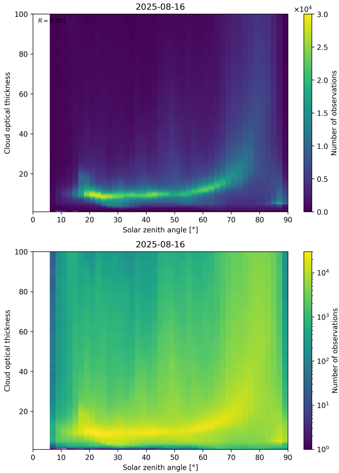
Figure 103: Scatter density plot of “Solar zenith angle” against “Cloud optical thickness” for 2025-08-15 to 2025-08-17.
