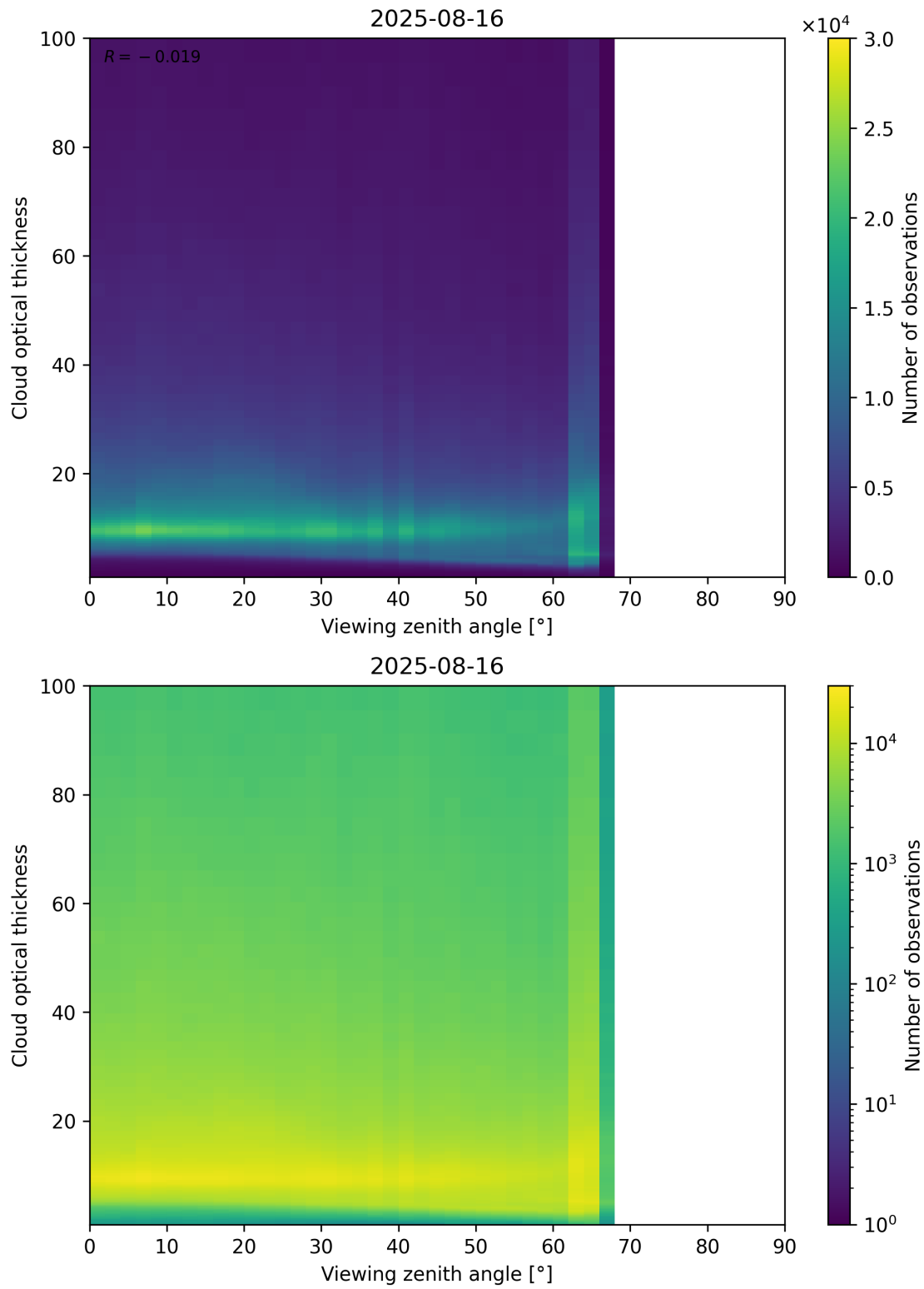
Figure 111: Scatter density plot of “Viewing zenith angle” against “Cloud optical thickness” for 2025-08-15 to 2025-08-17.
