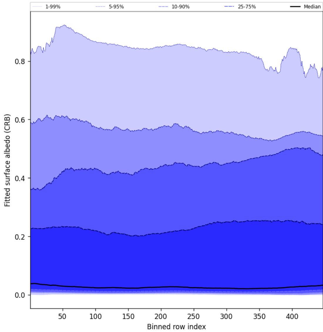
Figure 62: Along track statistics of “Fitted surface albedo (CRB)” for 2025-08-15 to 2025-08-17
