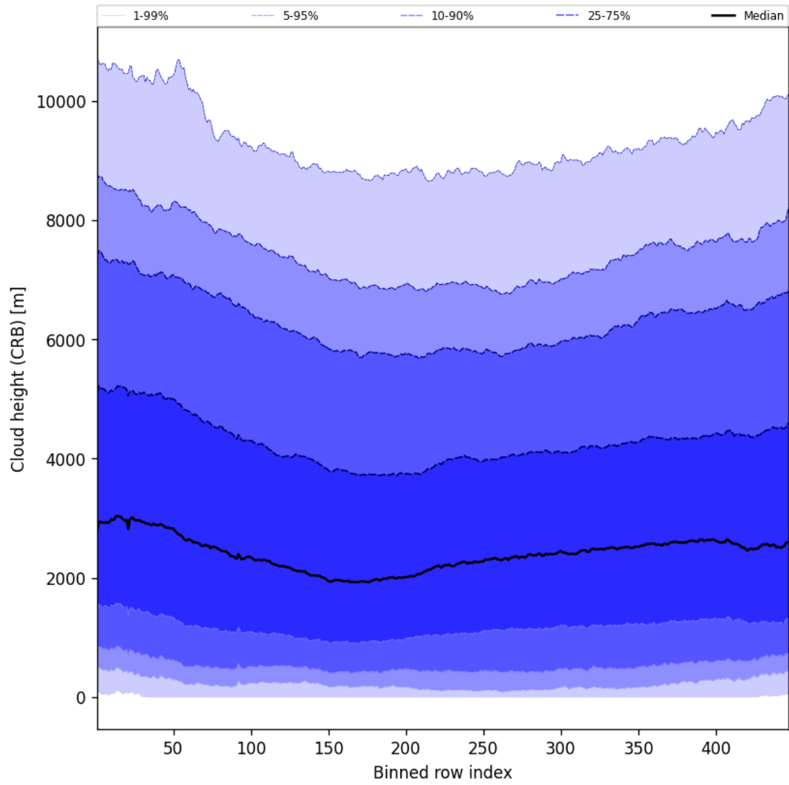
Figure 59: Along track statistics of “Cloud height (CRB)” for 2025-08-15 to 2025-08-17
