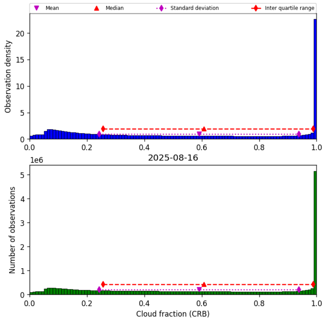
Figure 42: Histogram of “Cloud fraction (CRB)” for 2025-08-15 to 2025-08-17
