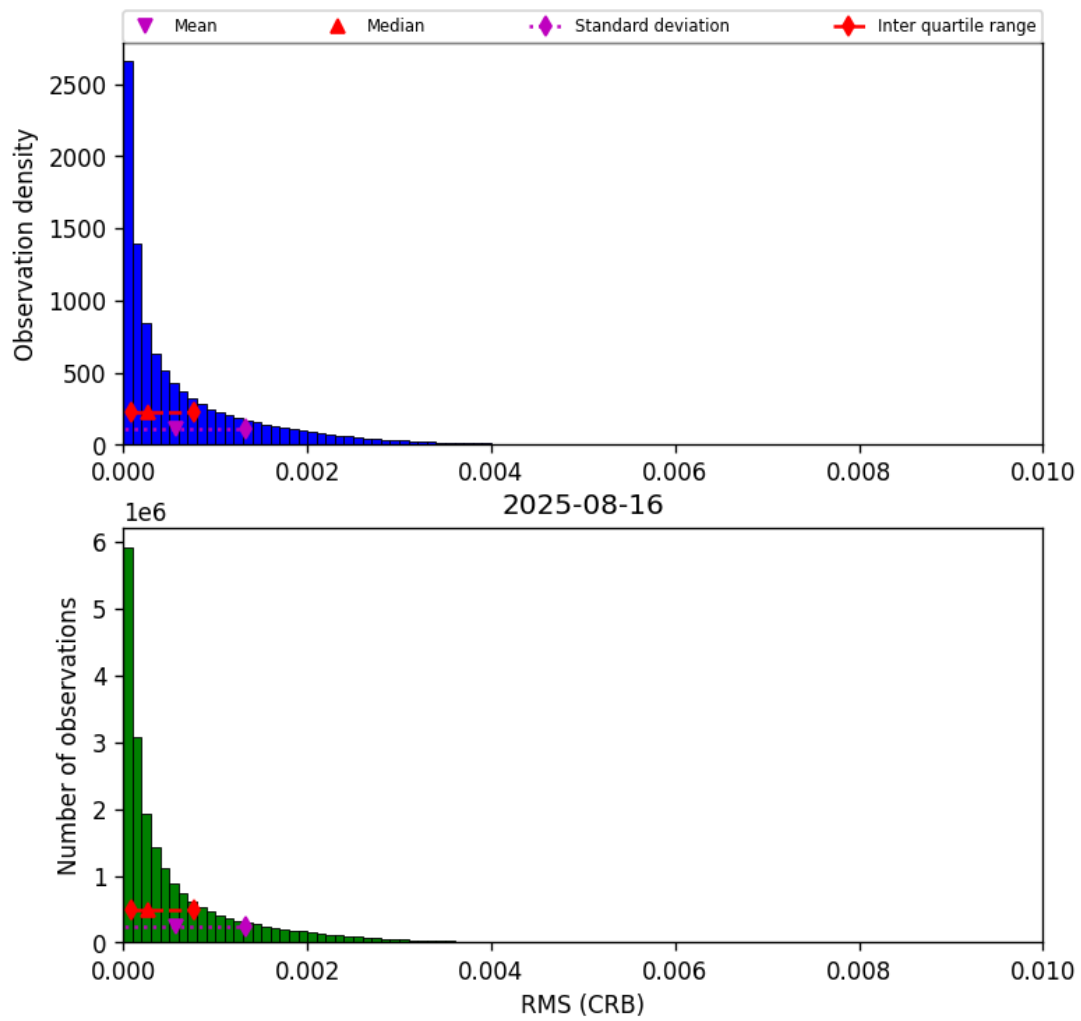
Figure 48: Histogram of “RMS (CRB)” for 2025-08-15 to 2025-08-17
