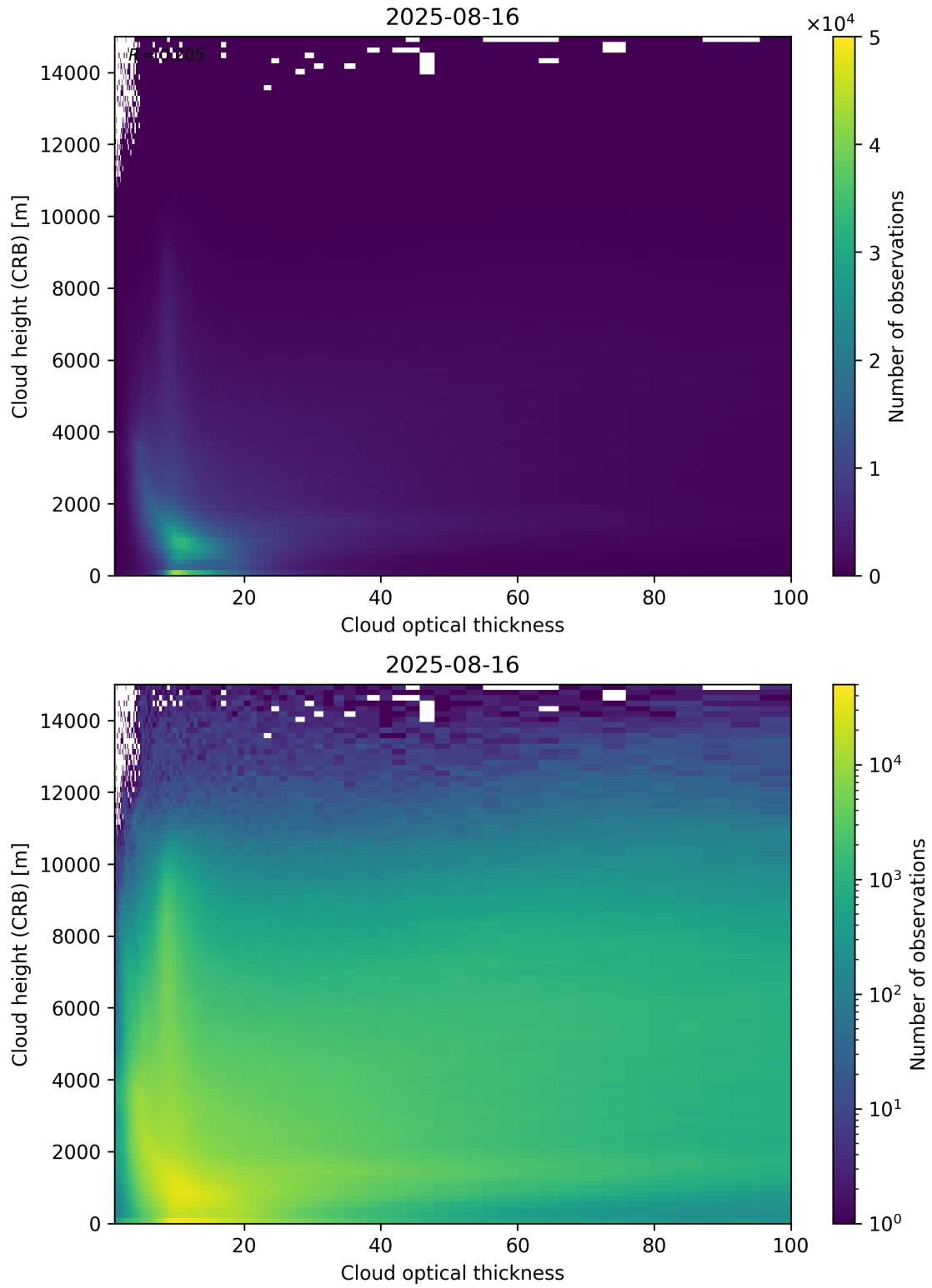
Figure 85: Scatter density plot of “Cloud optical thickness” against “Cloud height (CRB)” for 2025-08-15 to 2025-08-17.
