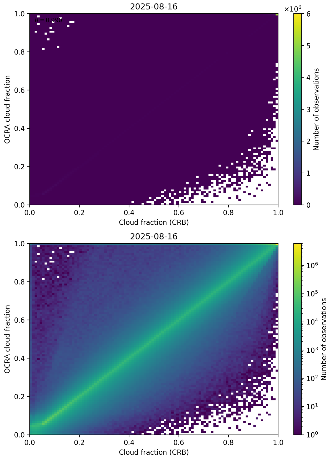
Figure 78: Scatter density plot of “Cloud fraction (CRB)” against “OCRA cloud fraction” for 2025-08-15 to 2025-08-17.
