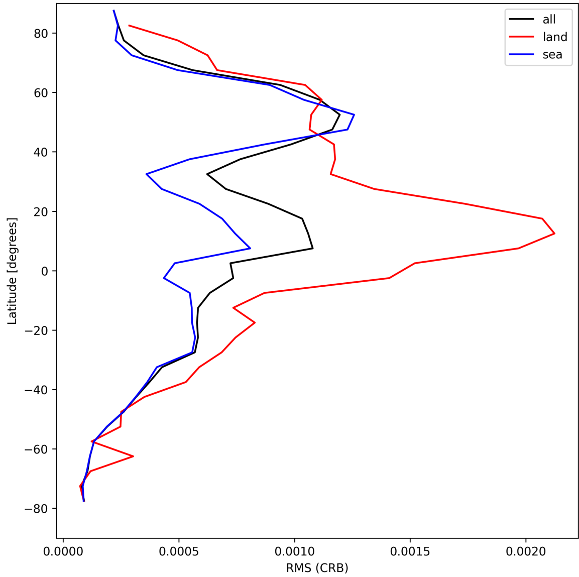
Figure 32: Zonal average of “RMS (CRB)” for 2025-08-15 to 2025-08-17.
