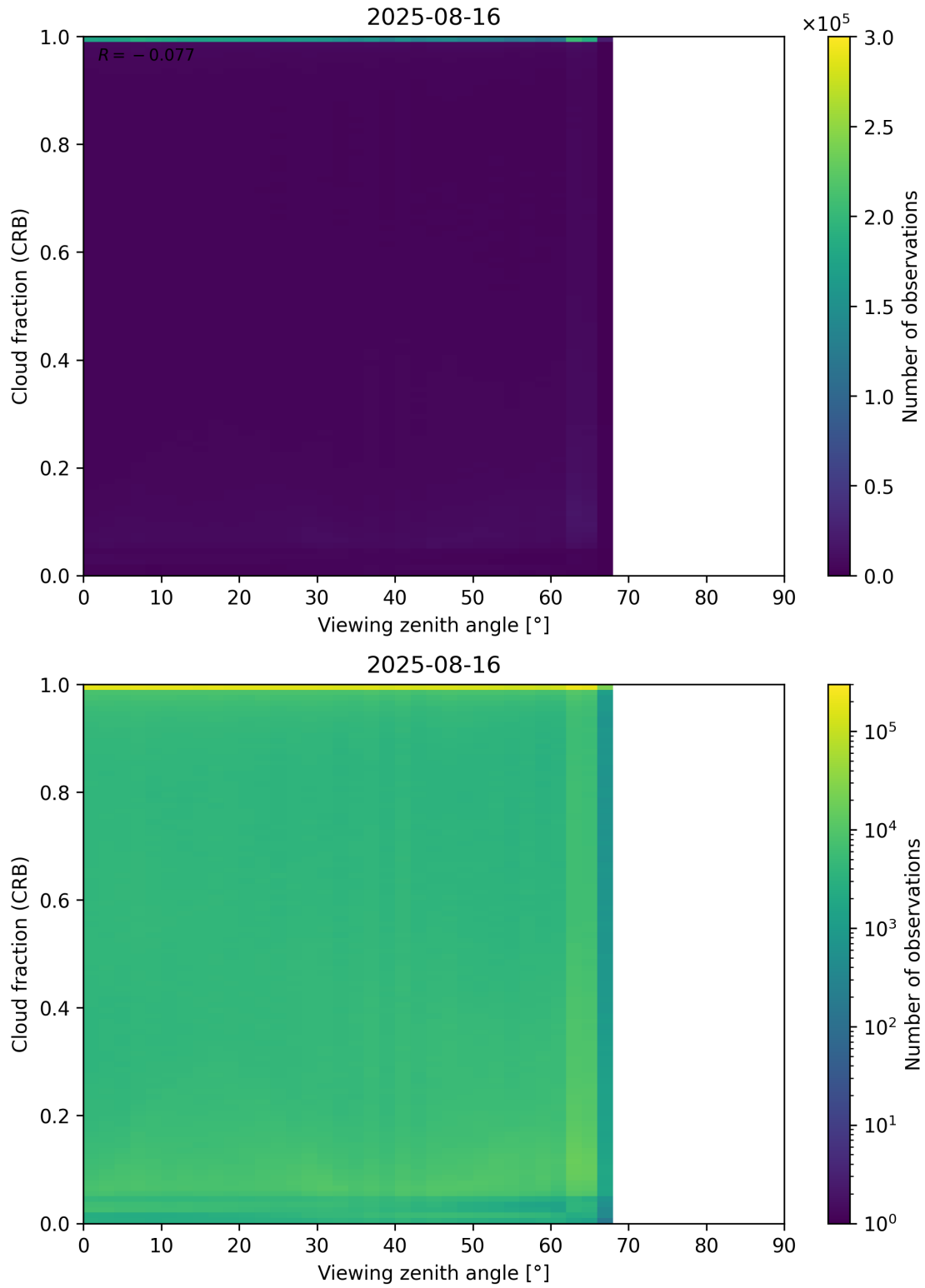
Figure 109: Scatter density plot of “Viewing zenith angle” against “Cloud fraction (CRB)” for 2025-08-15 to 2025-08-17.
