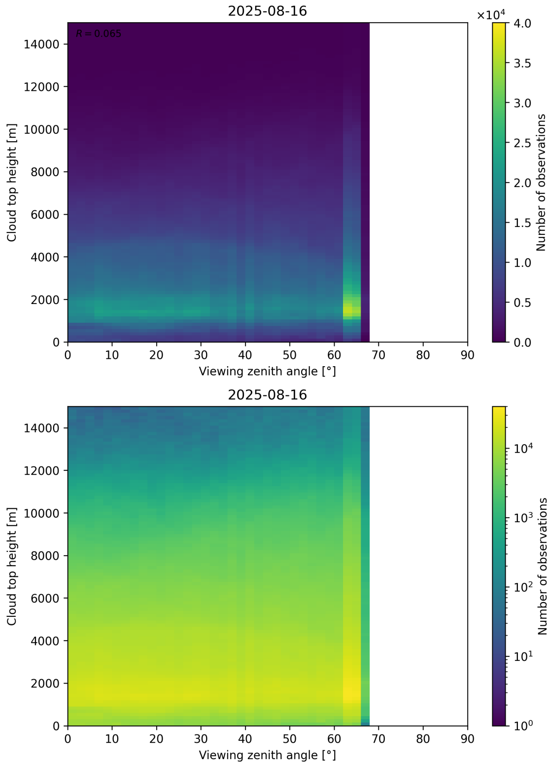
Figure 112: Scatter density plot of “Viewing zenith angle” against “Cloud top height” for 2025-08-15 to 2025-08-17.
