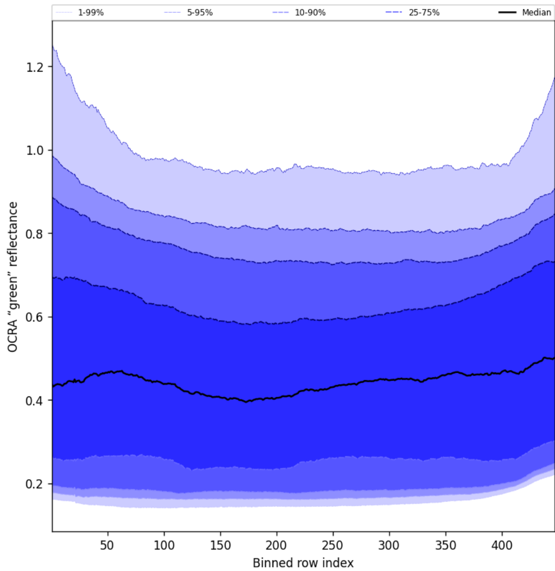
Figure 68: Along track statistics of “OCRA “green” reflectance” for 2025-08-15 to 2025-08-17
