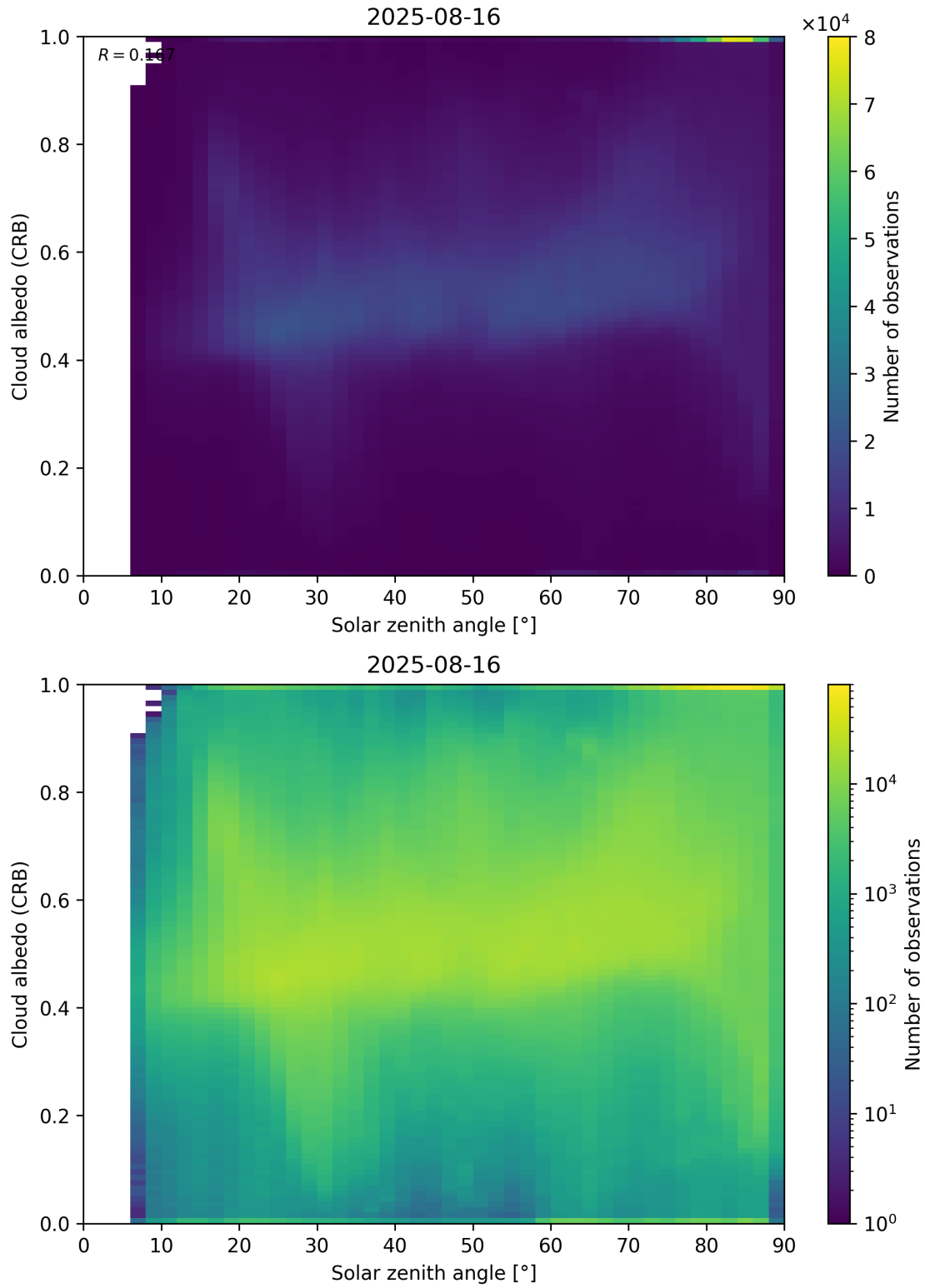
Figure 98: Scatter density plot of “Solar zenith angle” against “Cloud albedo (CRB)” for 2025-08-15 to 2025-08-17.
