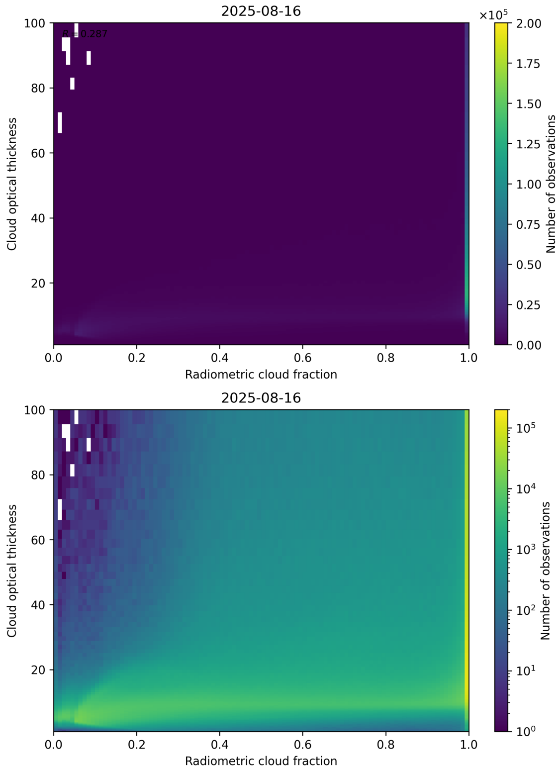
Figure 75: Scatter density plot of “Radiometric cloud fraction” against “Cloud optical thickness” for 2025-08-15 to 2025-08-17.
