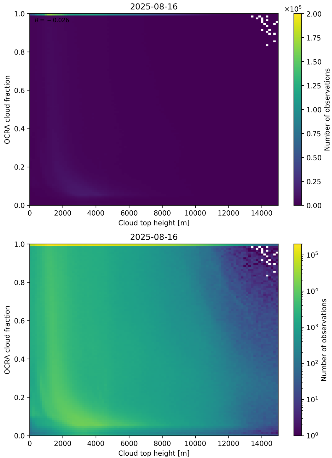
Figure 87: Scatter density plot of “Cloud top height” against “OCRA cloud fraction” for 2025-08-15 to 2025-08-17.
