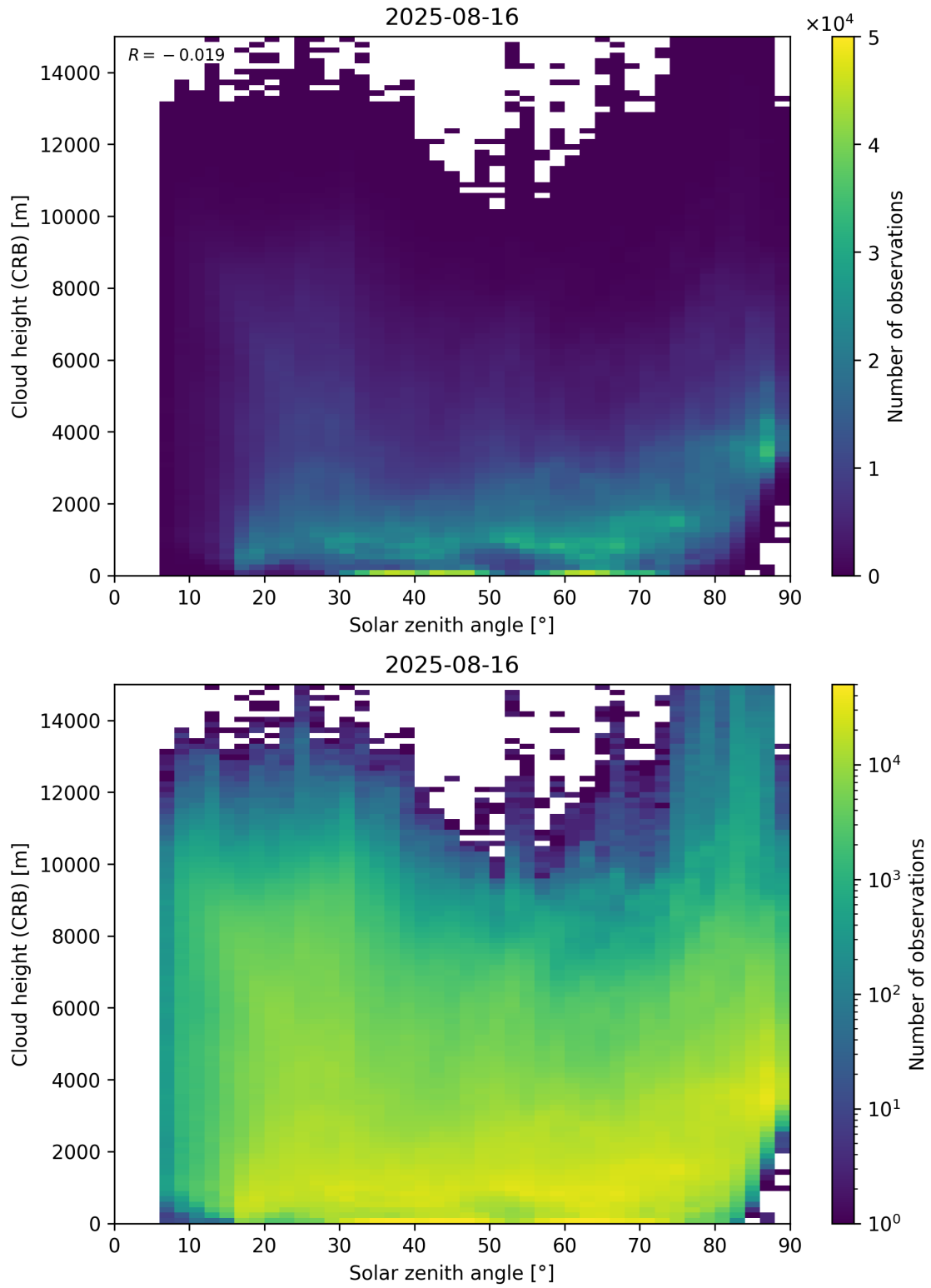
Figure 102: Scatter density plot of “Solar zenith angle” against “Cloud height (CRB)” for 2025-08-15 to 2025-08-17.
