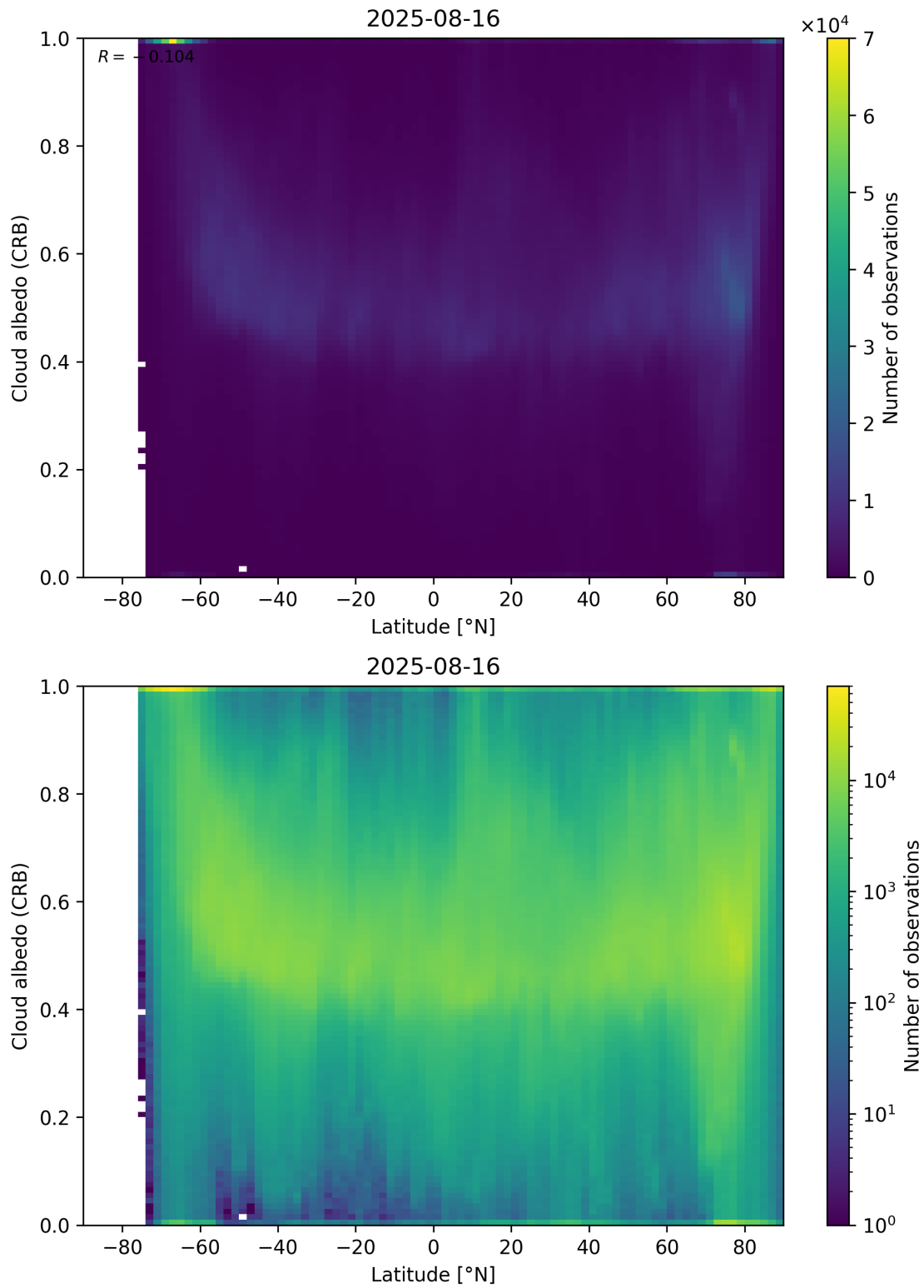
Figure 91: Scatter density plot of “Latitude” against “Cloud albedo (CRB)” for 2025-08-15 to 2025-08-17.
