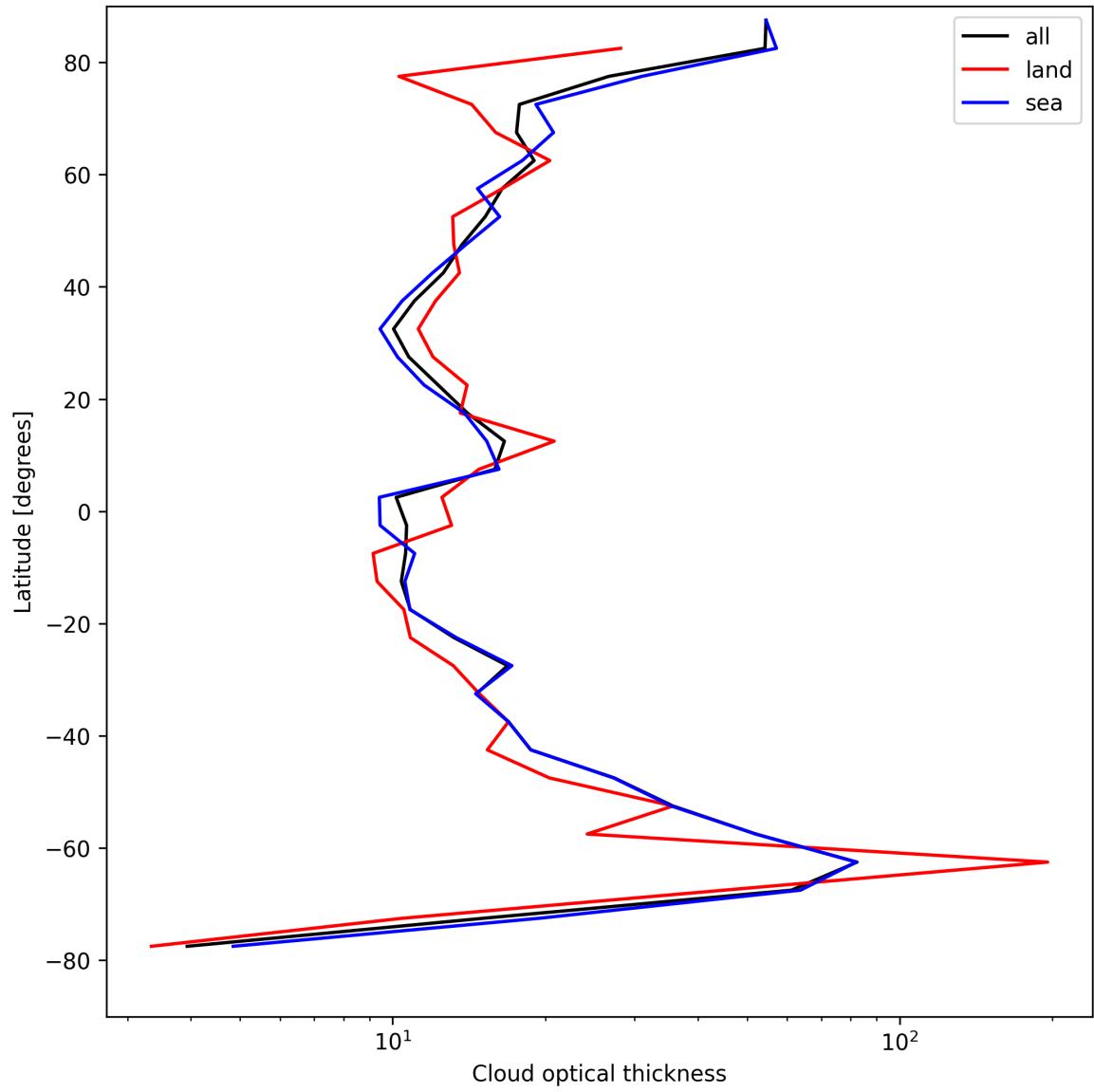
Figure 25: Zonal average of “Cloud optical thickness” for 2025-08-15 to 2025-08-17.
