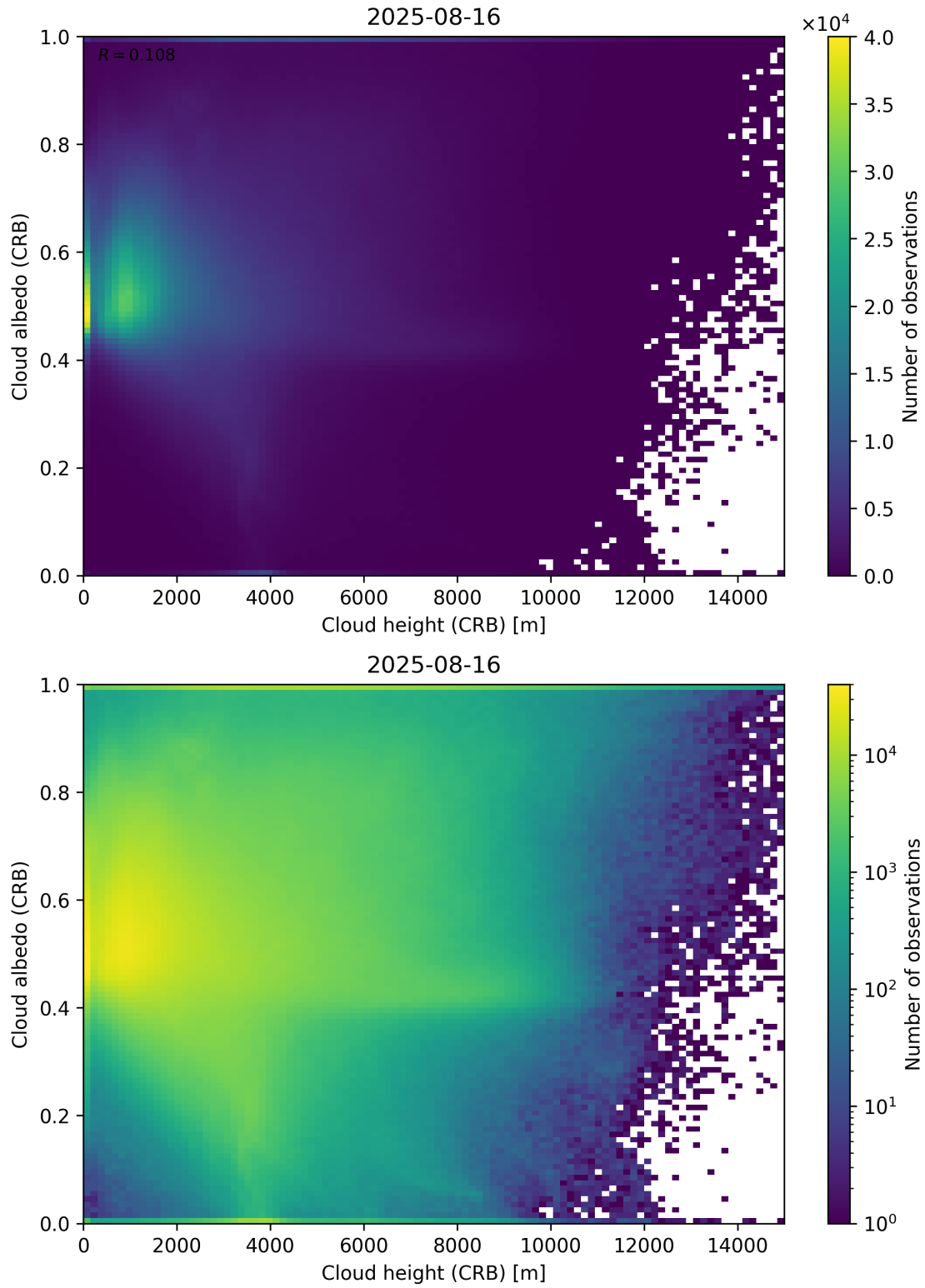
Figure 80: Scatter density plot of “Cloud height (CRB)” against “Cloud albedo (CRB)” for 2025-08-15 to 2025-08-17.
