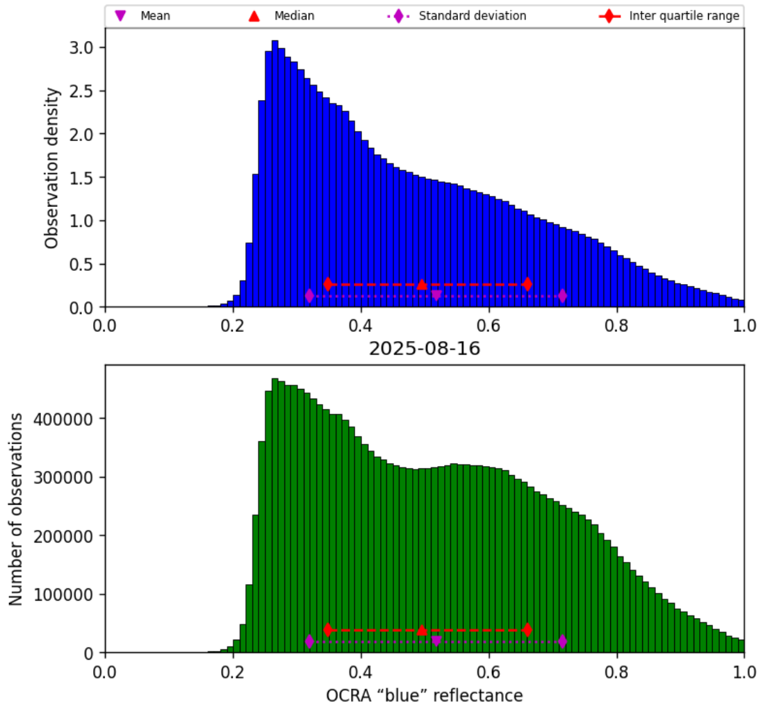
Figure 51: Histogram of “OCRA “blue” reflectance” for 2025-08-15 to 2025-08-17
