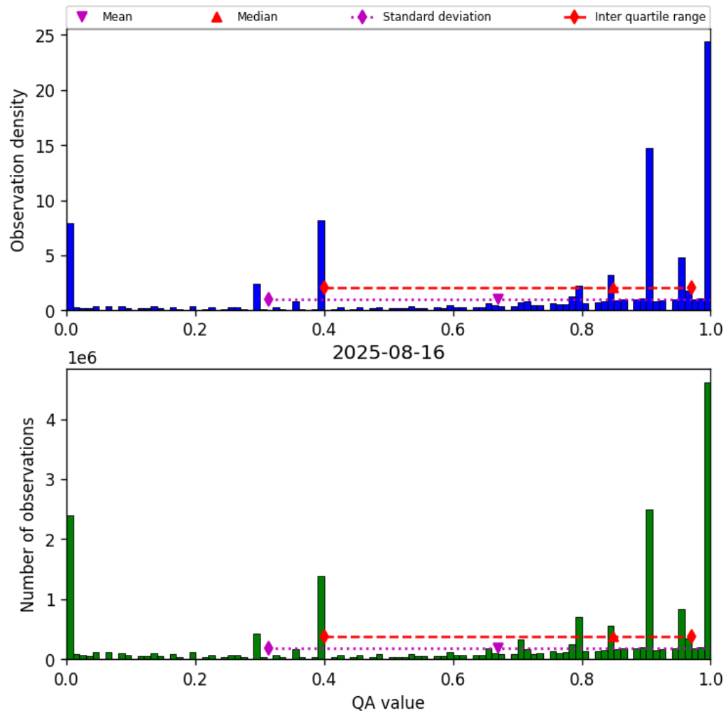
Figure 38: Histogram of “QA value” for 2025-08-15 to 2025-08-17
