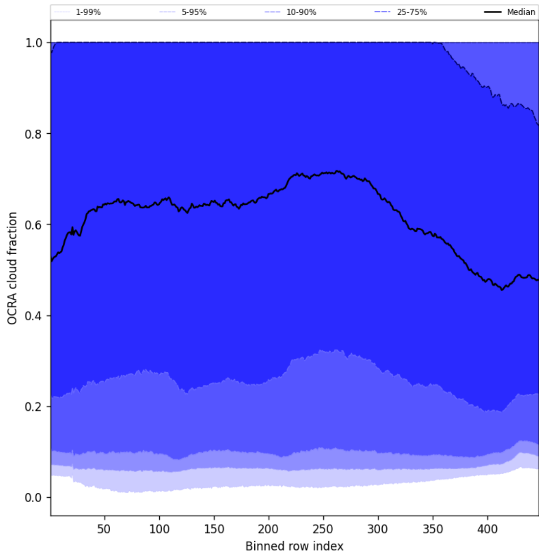
Figure 66: Along track statistics of “OCRA cloud fraction” for 2025-08-15 to 2025-08-17
