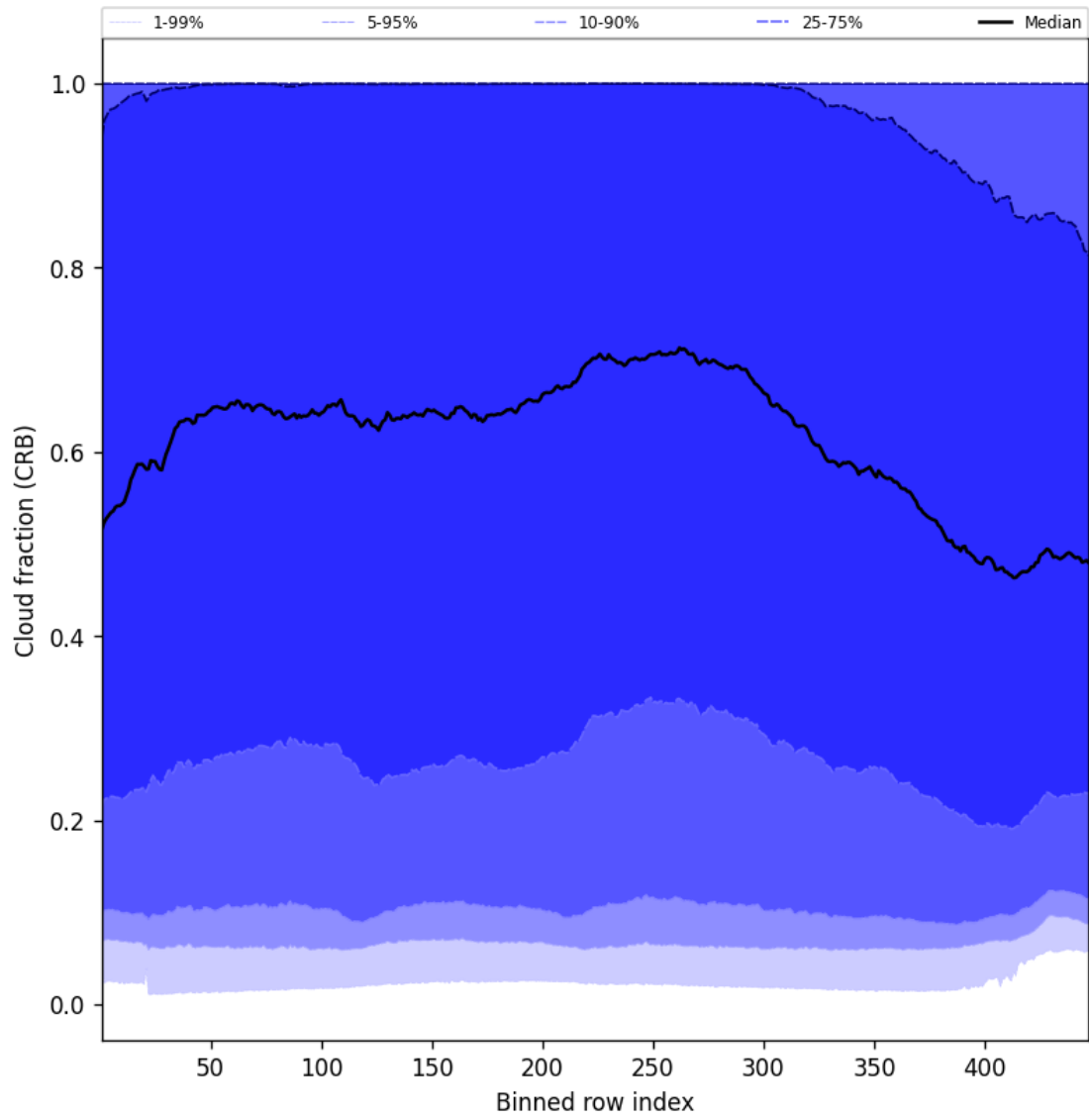
Figure 58: Along track statistics of “Cloud fraction (CRB)” for 2025-08-15 to 2025-08-17
