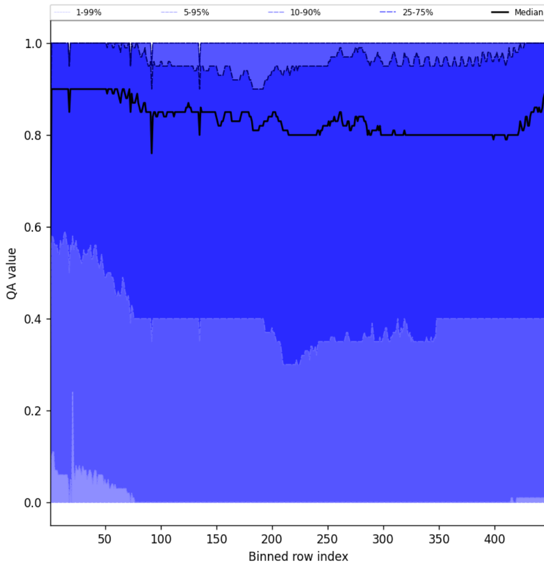
Figure 54: Along track statistics of “QA value” for 2025-08-15 to 2025-08-17
