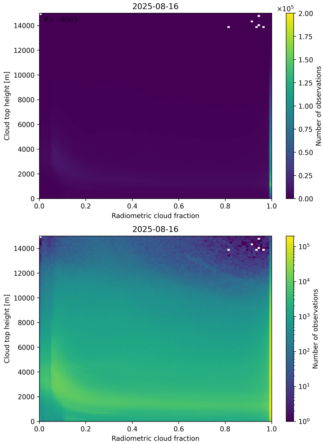
Figure 76: Scatter density plot of “Radiometric cloud fraction” against “Cloud top height” for 2025-08-15 to 2025-08-17.
