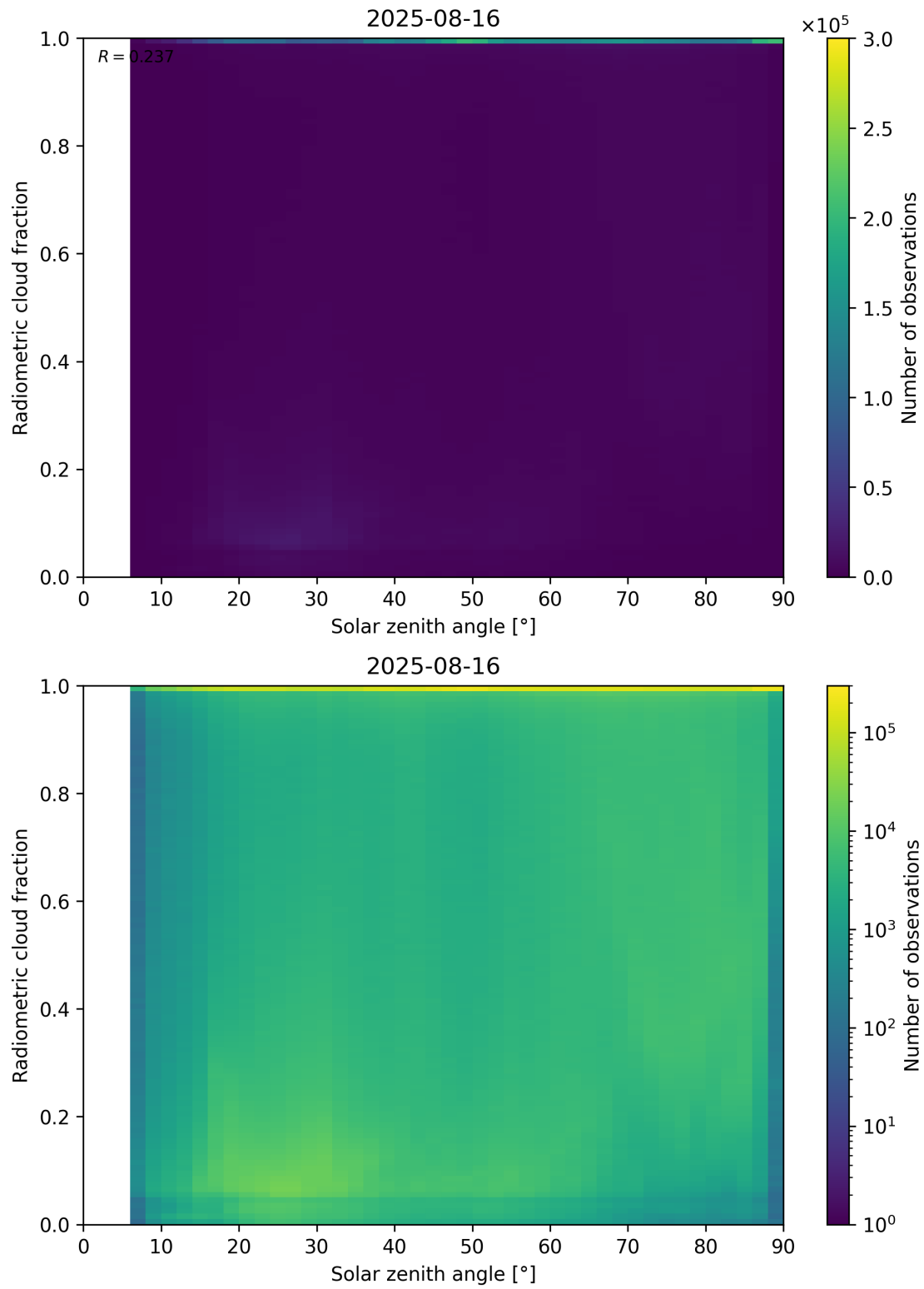
Figure 99: Scatter density plot of “Solar zenith angle” against “Radiometric cloud fraction” for 2025-08-15 to 2025-08-17.
