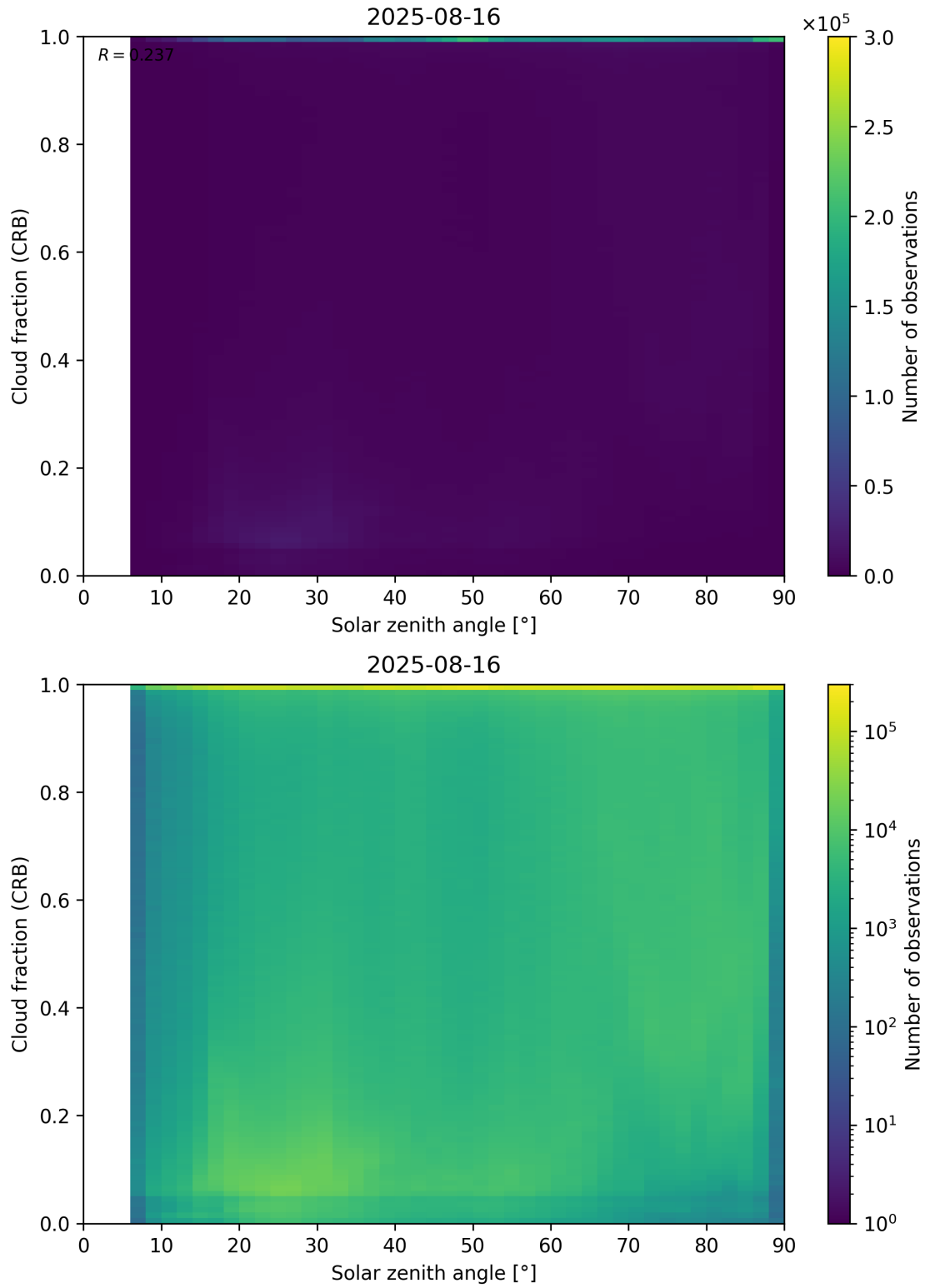
Figure 101: Scatter density plot of “Solar zenith angle” against “Cloud fraction (CRB)” for 2025-08-15 to 2025-08-17.
