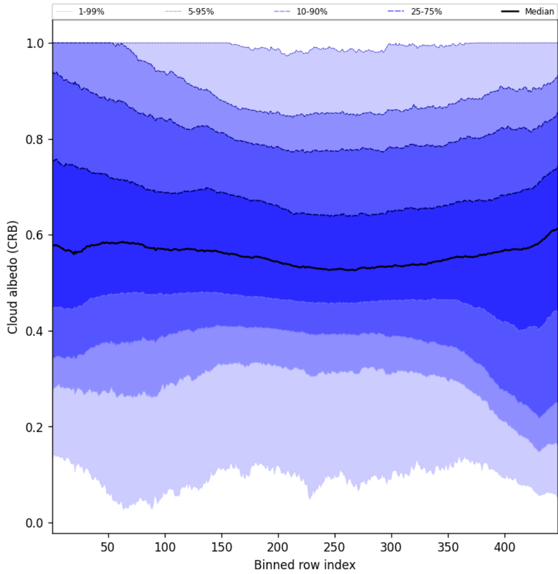
Figure 60: Along track statistics of “Cloud albedo (CRB)” for 2025-08-15 to 2025-08-17
