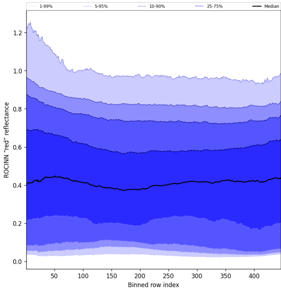
Figure 69: Along track statistics of "ROCINN "red" reflectance" for 2025-08-15 to 2025-08-17
