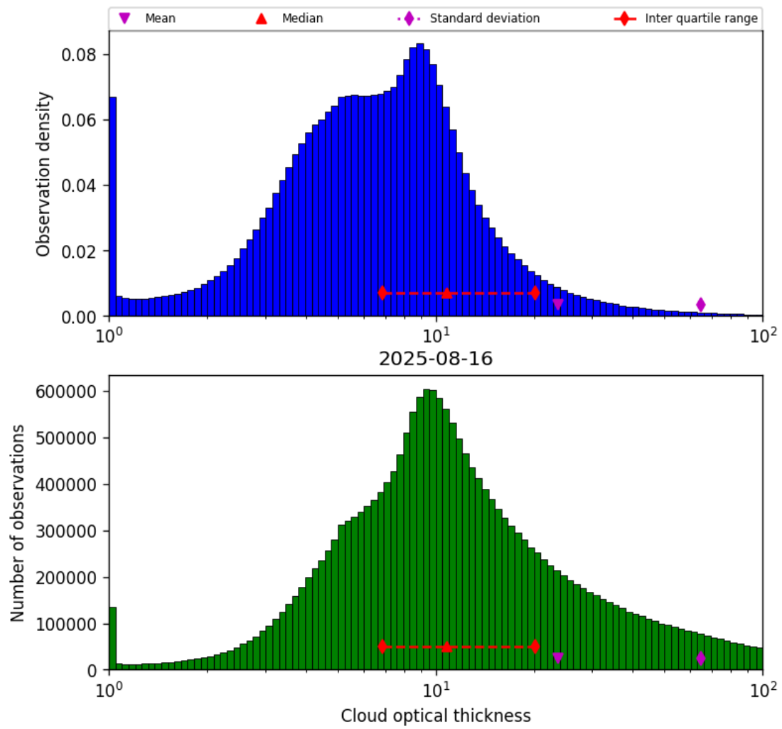
Figure 41: Histogram of “Cloud optical thickness” for 2025-08-15 to 2025-08-17
