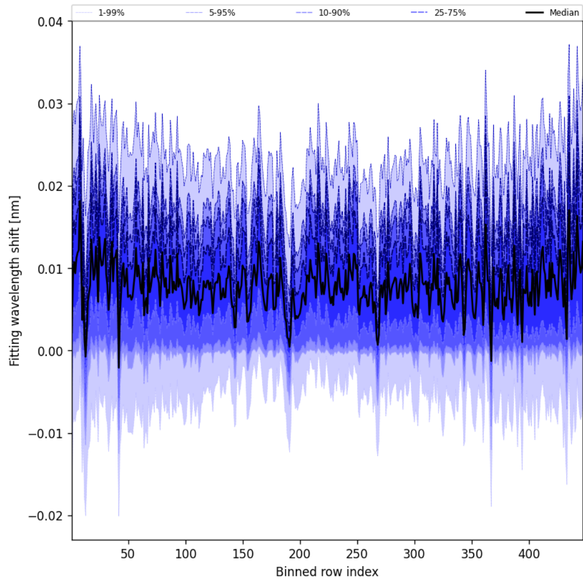
Figure 65: Along track statistics of “Fitting wavelength shift” for 2025-08-15 to 2025-08-17
