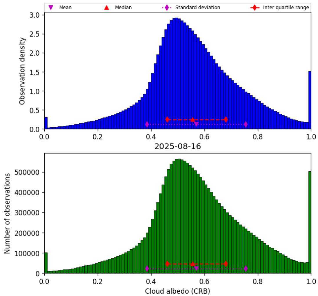
Figure 44: Histogram of “Cloud albedo (CRB)” for 2025-08-15 to 2025-08-17
