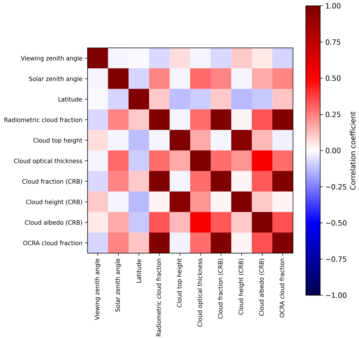
Figure 2: Map of correlation matrix for 2025-08-15 to 2025-08-17.
