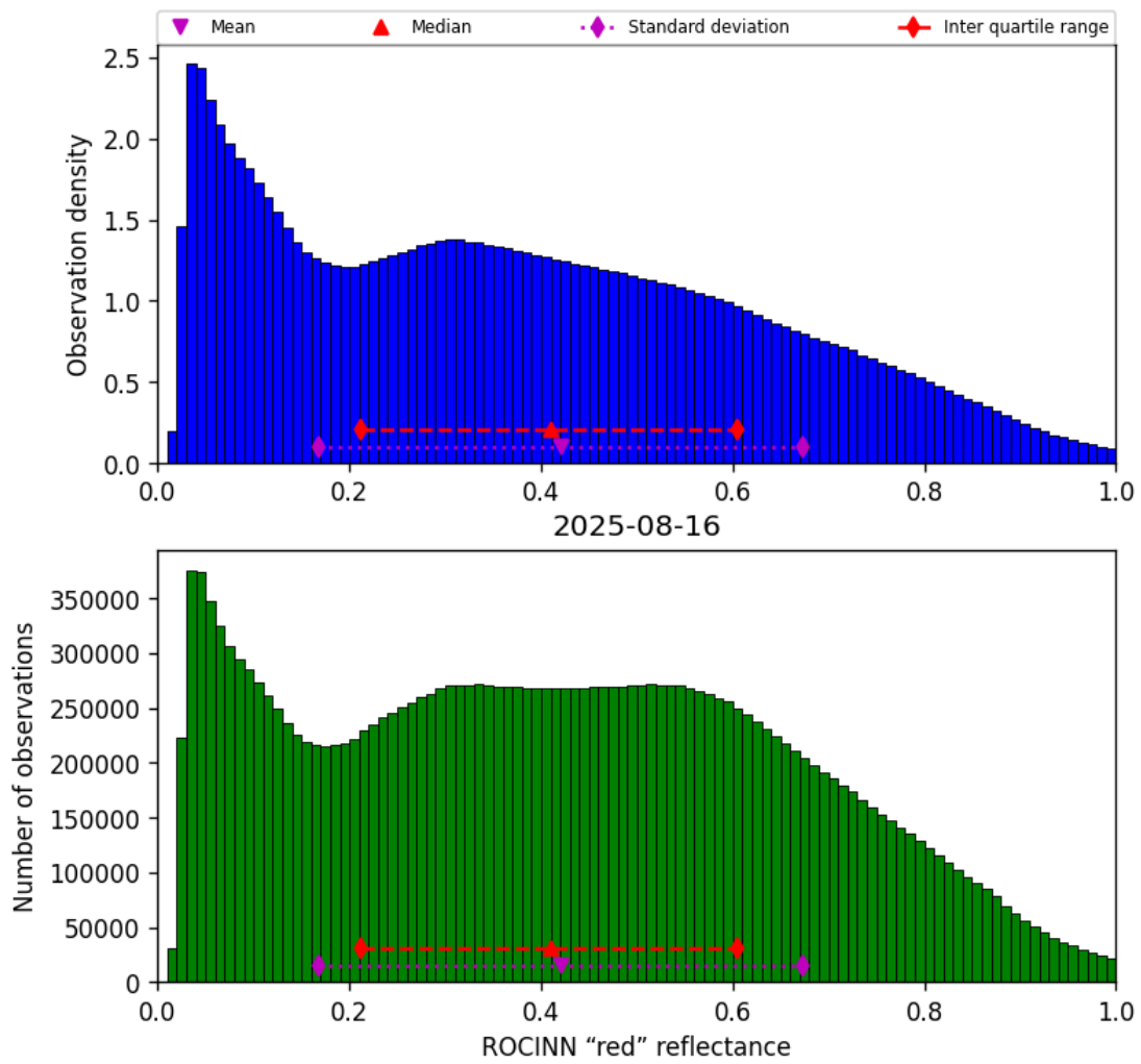
Figure 53: Histogram of “ROCINN “red” reflectance” for 2025-08-15 to 2025-08-17
