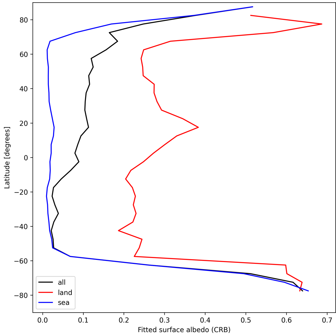
Figure 30: Zonal average of “Fitted surface albedo (CRB)” for 2025-08-15 to 2025-08-17.
