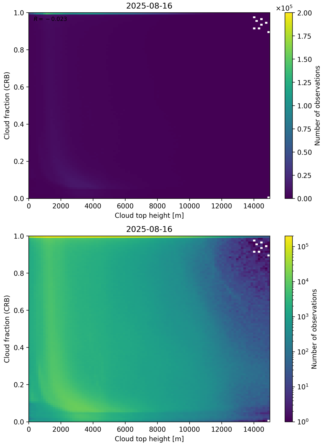
Figure 88: Scatter density plot of “Cloud top height” against “Cloud fraction (CRB)” for 2025-08-15 to 2025-08-17.
