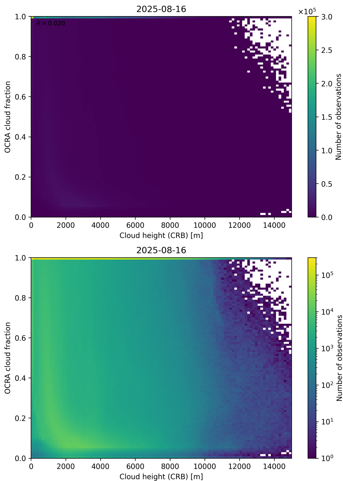
Figure 81: Scatter density plot of “Cloud height (CRB)” against “OCRA cloud fraction” for 2025-08-15 to 2025-08-17.
