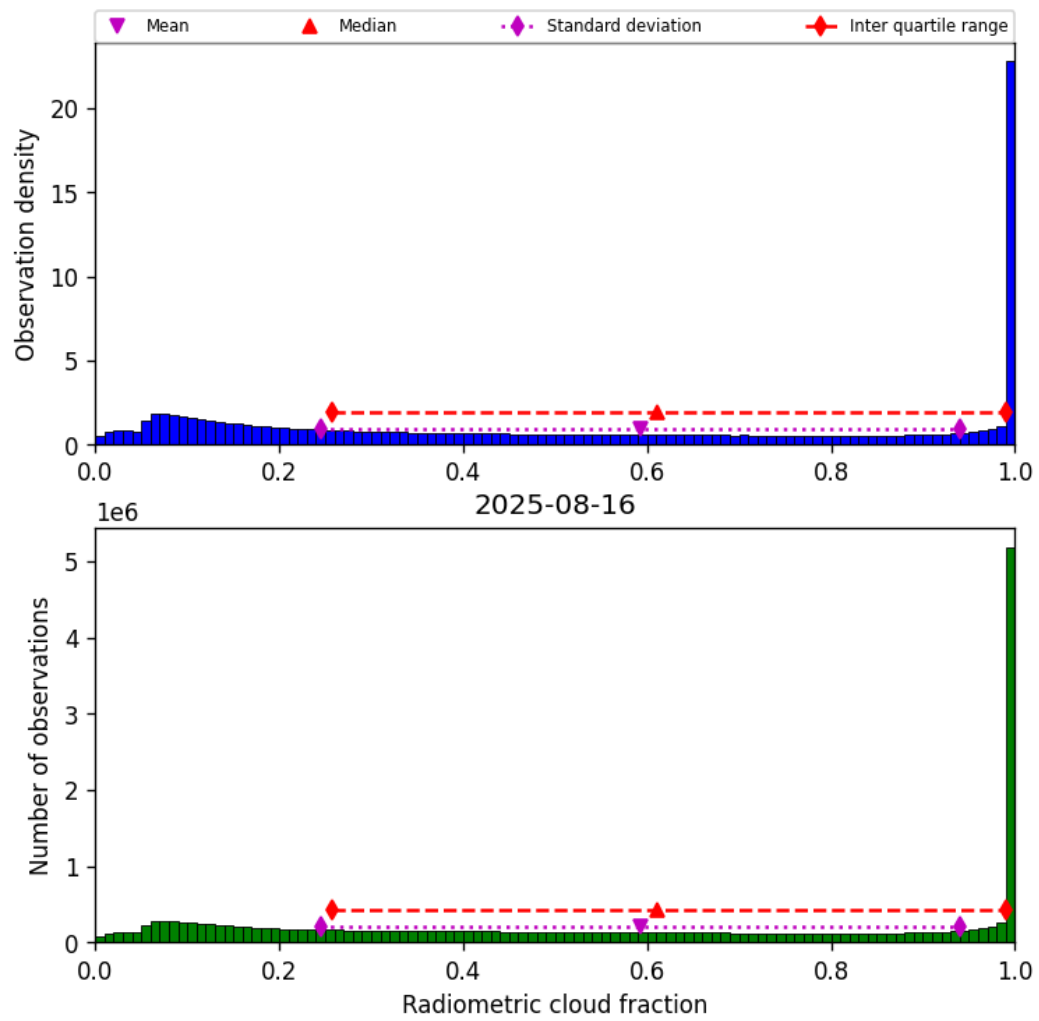
Figure 39: Histogram of “Radiometric cloud fraction” for 2025-08-15 to 2025-08-17
