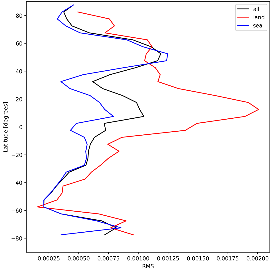
Figure 31: Zonal average of “RMS” for 2025-08-15 to 2025-08-17.
