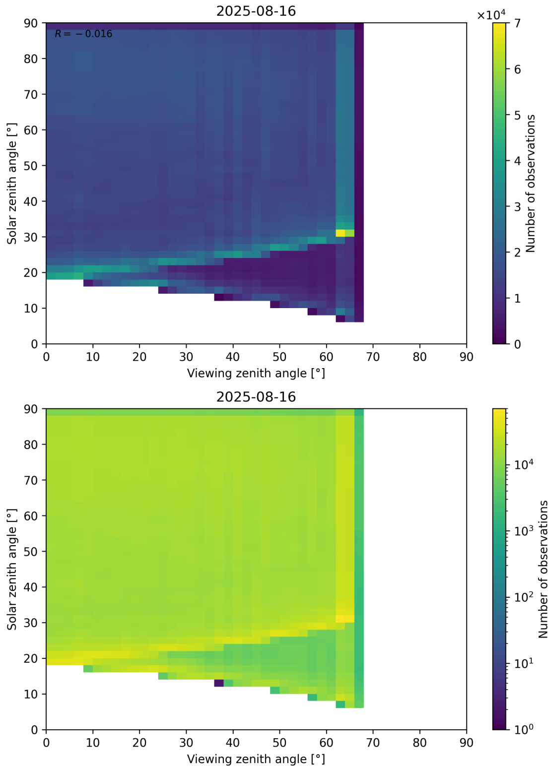
Figure 114: Scatter density plot of “Viewing zenith angle” against “Solar zenith angle” for 2025-08-15 to 2025-08-17.
