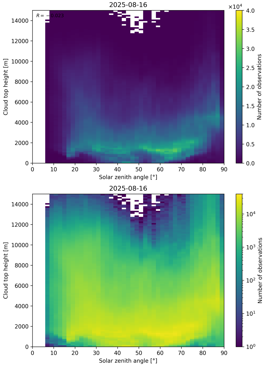
Figure 104: Scatter density plot of “Solar zenith angle” against “Cloud top height” for 2025-08-15 to 2025-08-17.
