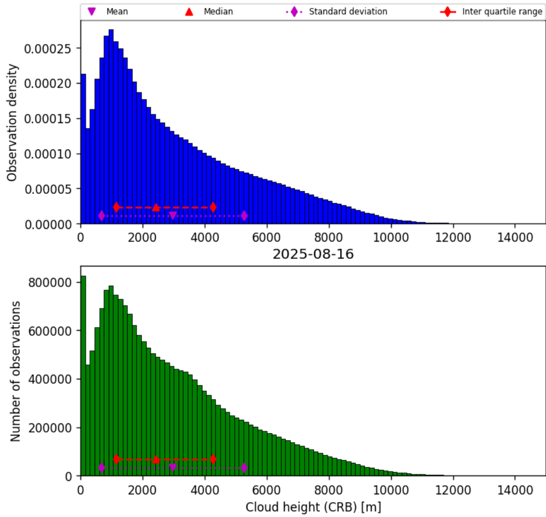
Figure 43: Histogram of “Cloud height (CRB)” for 2025-08-15 to 2025-08-17
