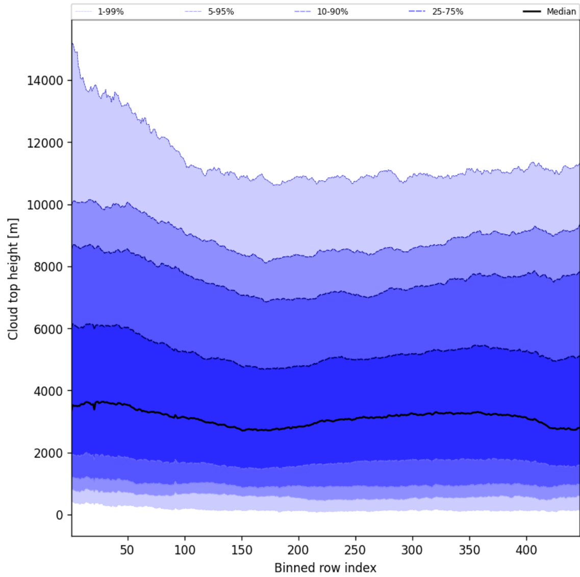
Figure 56: Along track statistics of “Cloud top height” for 2025-08-15 to 2025-08-17
