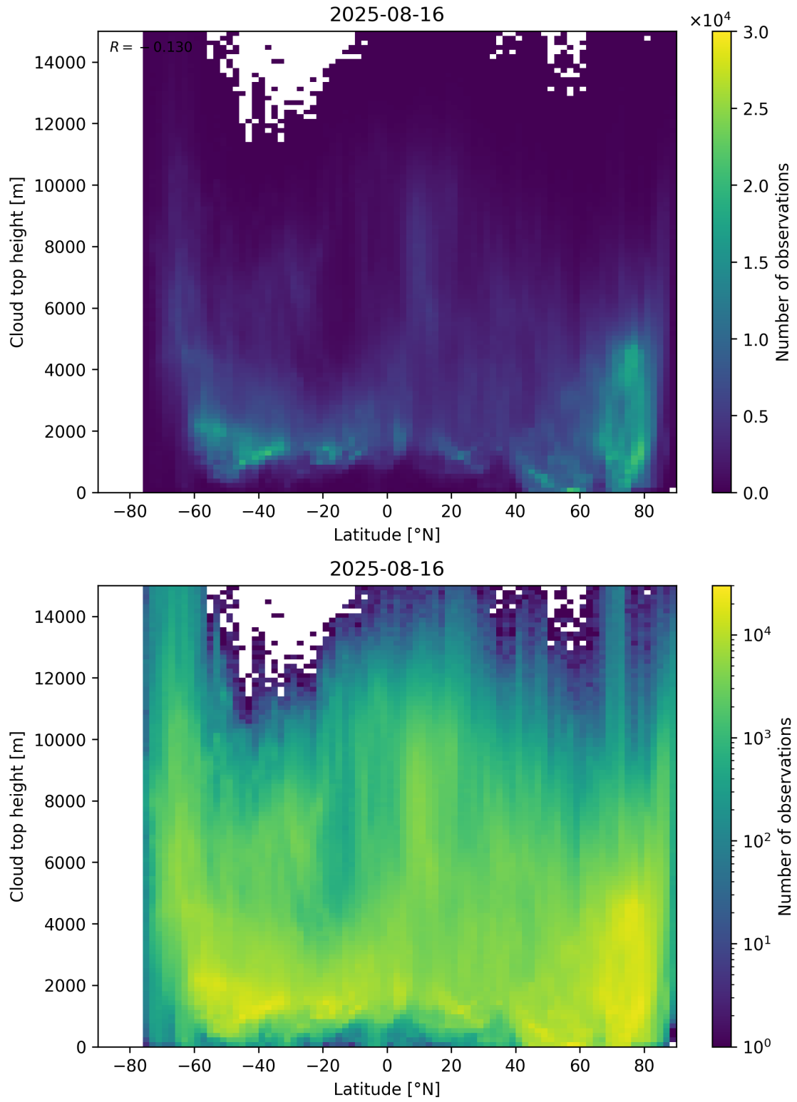
Figure 97: Scatter density plot of “Latitude” against “Cloud top height” for 2025-08-15 to 2025-08-17.
