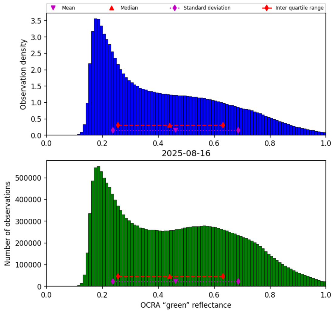
Figure 52: Histogram of “OCRA “green” reflectance” for 2025-08-15 to 2025-08-17
