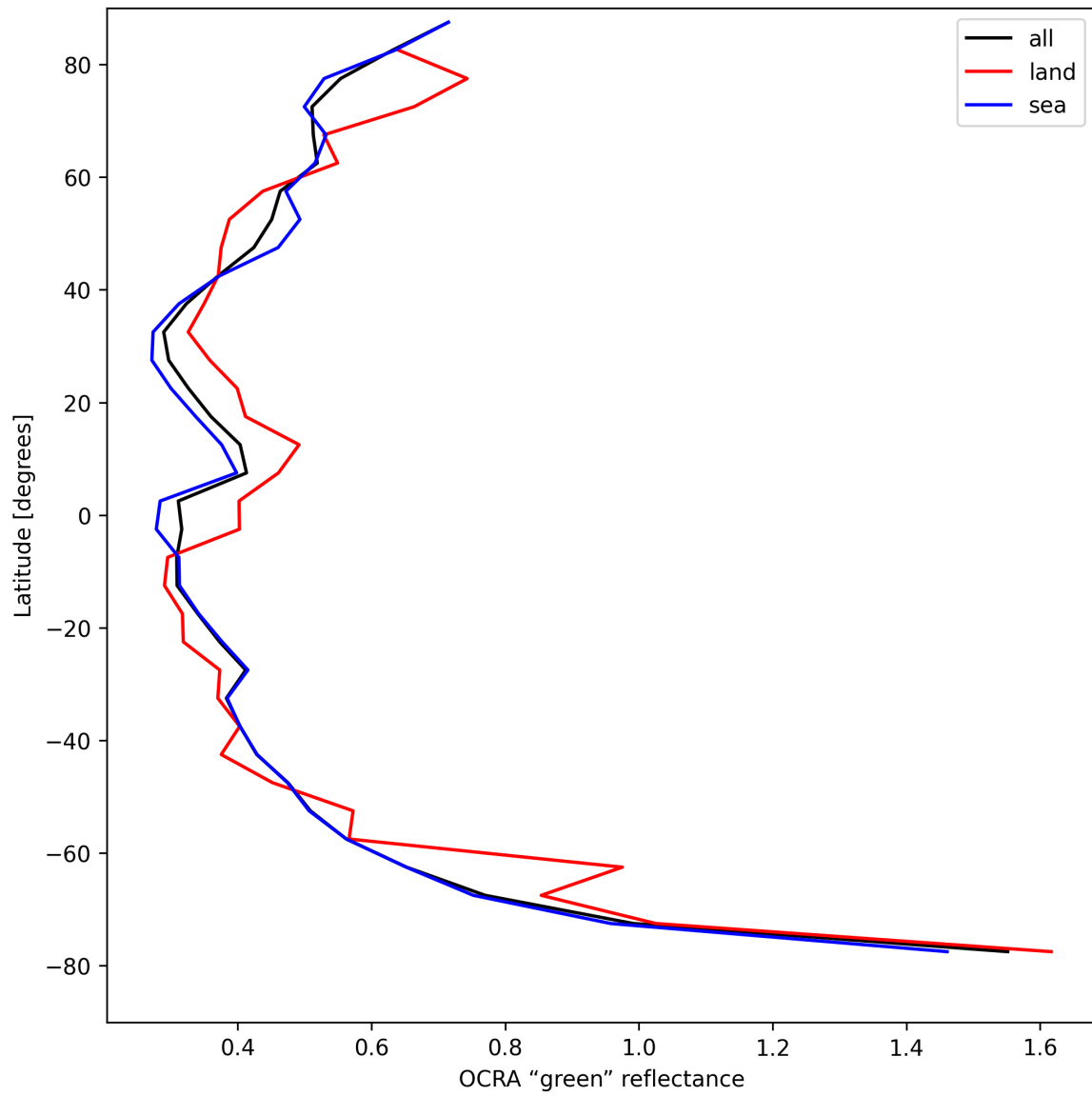
Figure 36: Zonal average of “OCRA “green” reflectance” for 2025-08-15 to 2025-08-17.
