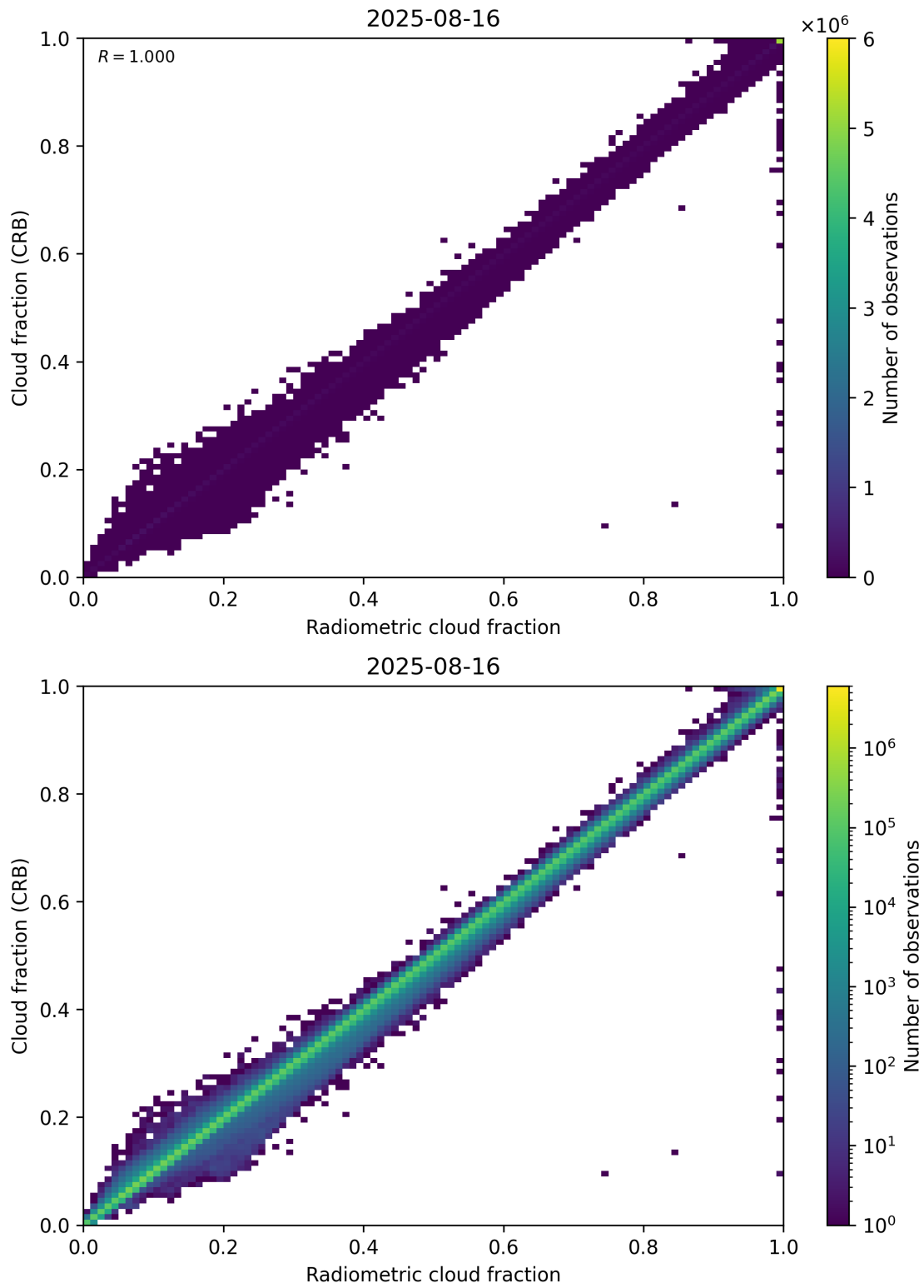
Figure 73: Scatter density plot of “Radiometric cloud fraction” against “Cloud fraction (CRB)” for 2025-08-15 to 2025-08-17.
