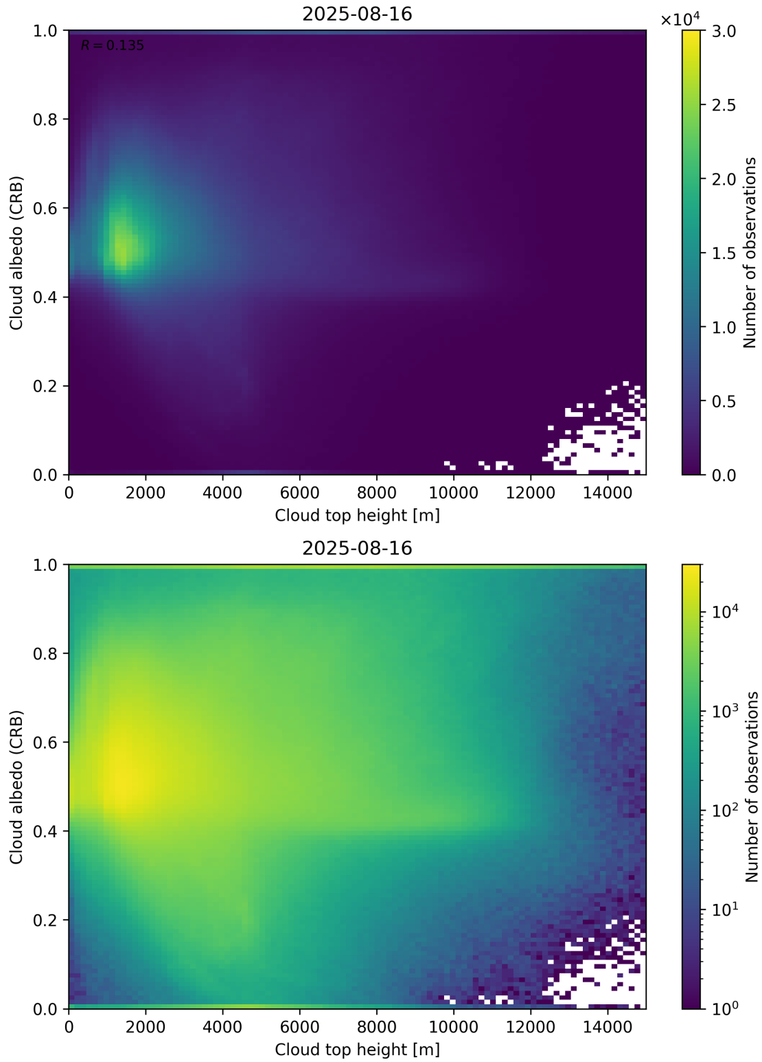
Figure 86: Scatter density plot of “Cloud top height” against “Cloud albedo (CRB)” for 2025-08-15 to 2025-08-17.
