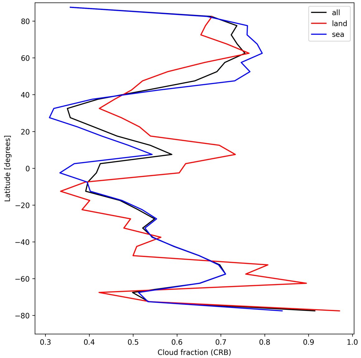
Figure 26: Zonal average of “Cloud fraction (CRB)” for 2025-08-15 to 2025-08-17.
