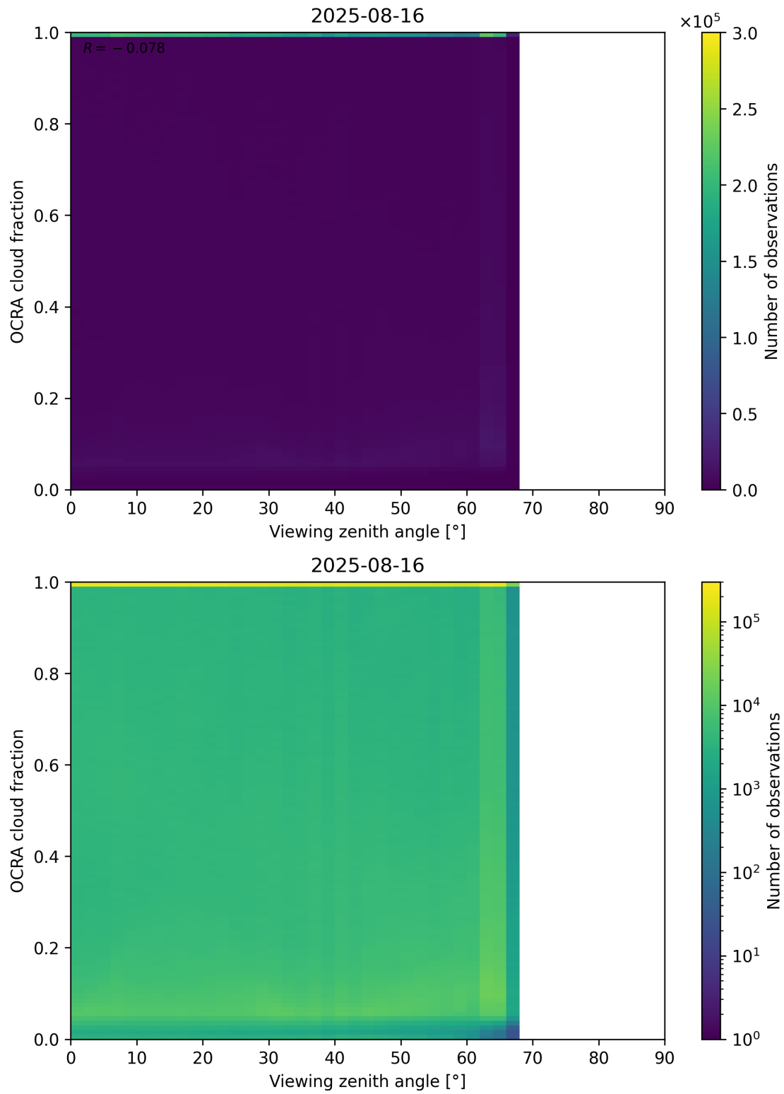
Figure 108: Scatter density plot of “Viewing zenith angle” against “OCRA cloud fraction” for 2025-08-15 to 2025-08-17.
