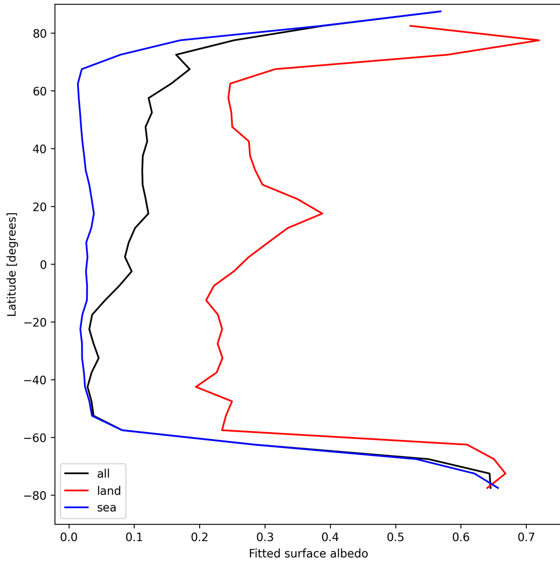
Figure 29: Zonal average of “Fitted surface albedo” for 2025-08-15 to 2025-08-17.
