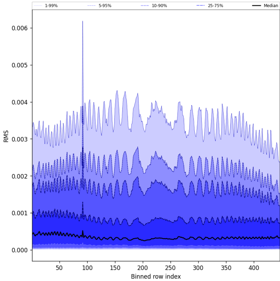
Figure 63: Along track statistics of “RMS” for 2025-08-15 to 2025-08-17
