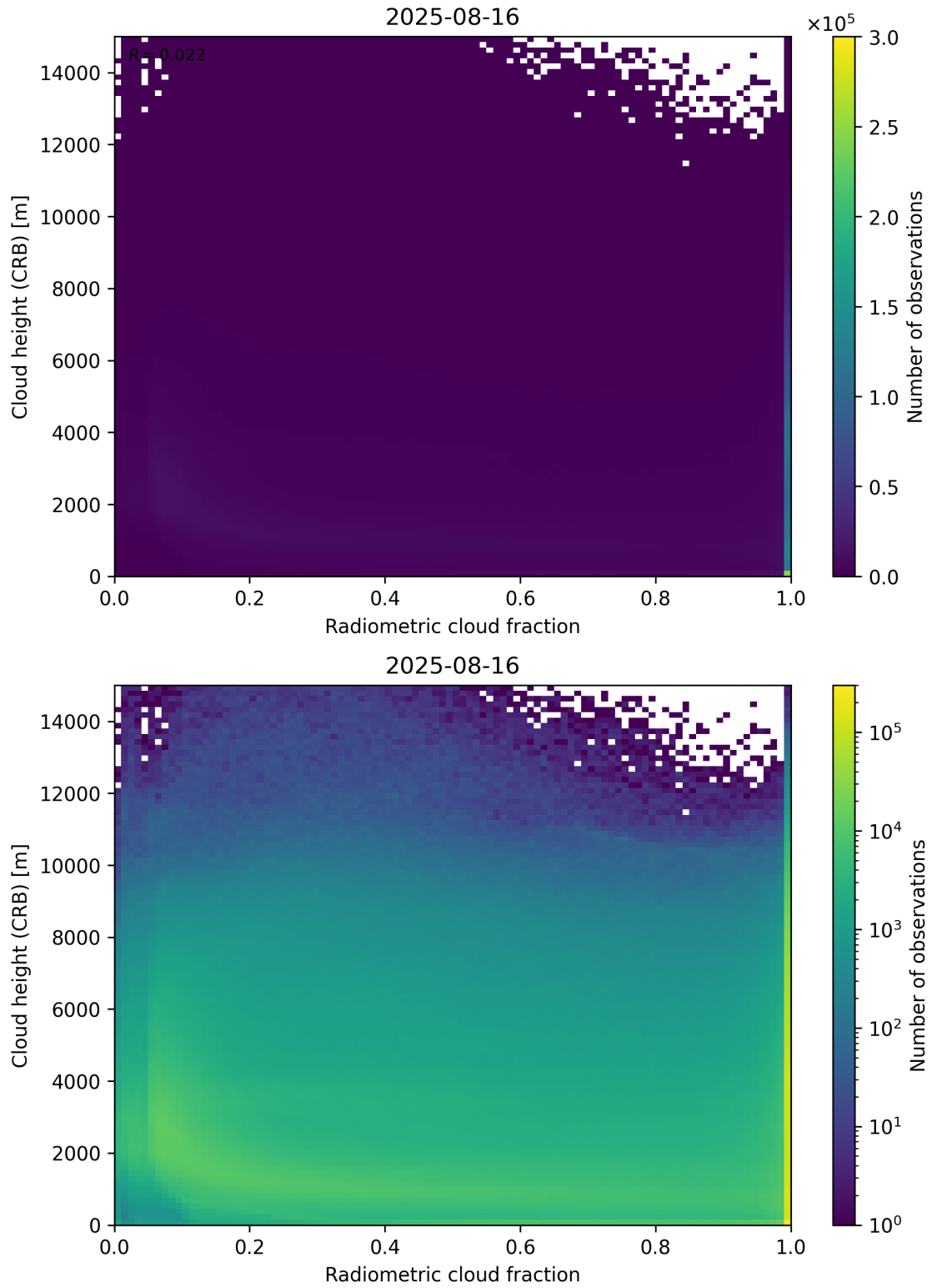
Figure 74: Scatter density plot of “Radiometric cloud fraction” against “Cloud height (CRB)” for 2025-08-15 to 2025-08-17.
