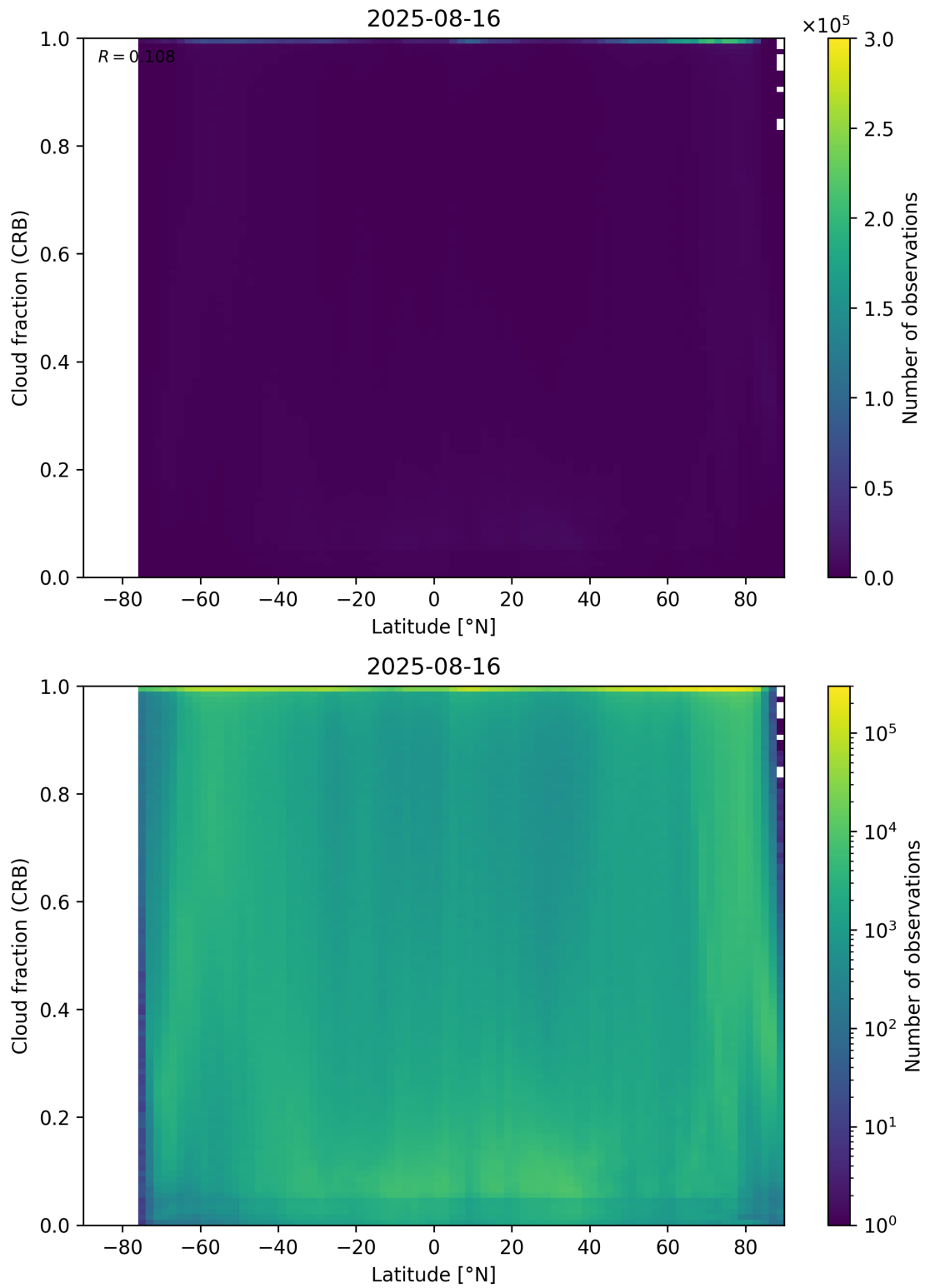
Figure 94: Scatter density plot of “Latitude” against “Cloud fraction (CRB)” for 2025-08-15 to 2025-08-17.
