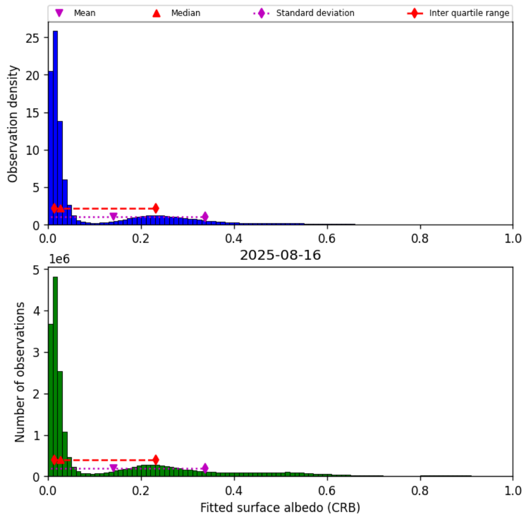
Figure 46: Histogram of “Fitted surface albedo (CRB)” for 2025-08-15 to 2025-08-17
