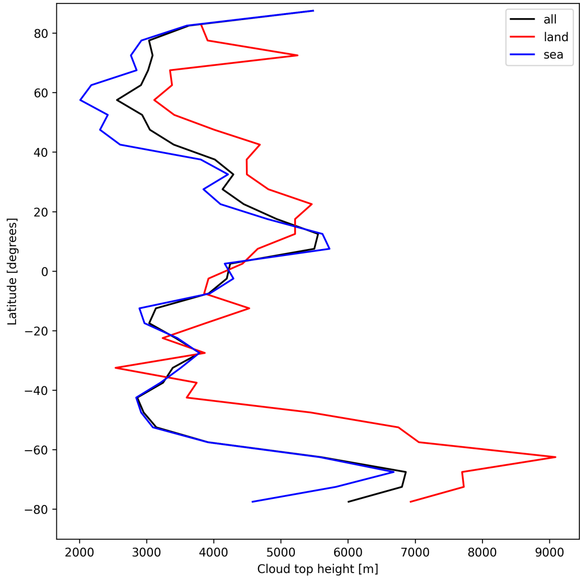
Figure 24: Zonal average of “Cloud top height” for 2025-08-15 to 2025-08-17.
