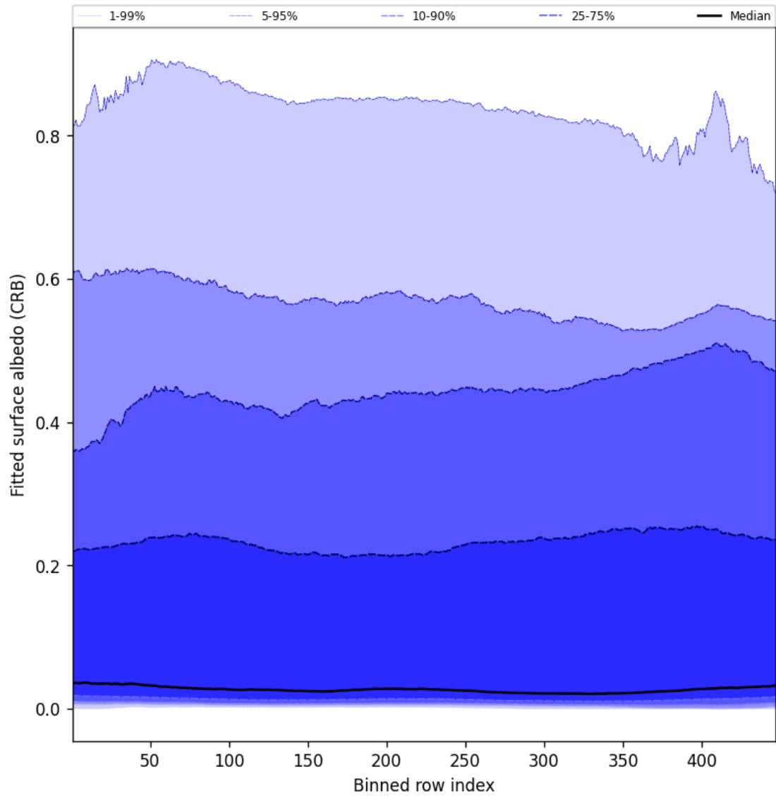
Figure 62: Along track statistics of “Fitted surface albedo (CRB)” for 2025-08-16 to 2025-08-18
