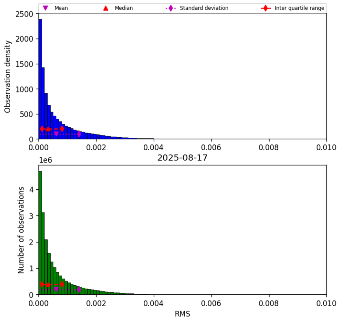
Figure 47: Histogram of “RMS” for 2025-08-16 to 2025-08-18
