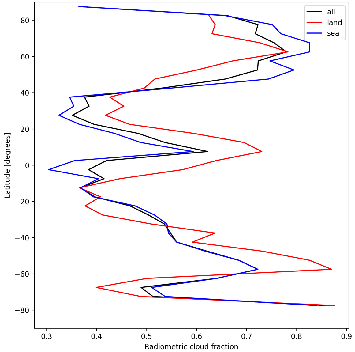
Figure 23: Zonal average of “Radiometric cloud fraction” for 2025-08-16 to 2025-08-18.
