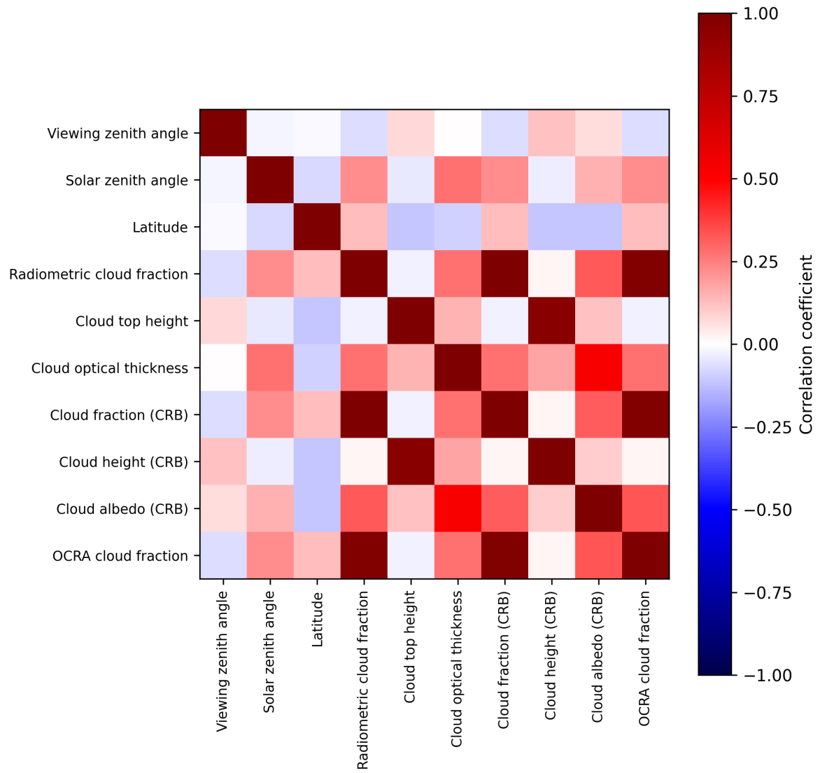
Figure 2: Map of correlation matrix for 2025-08-16 to 2025-08-18.
