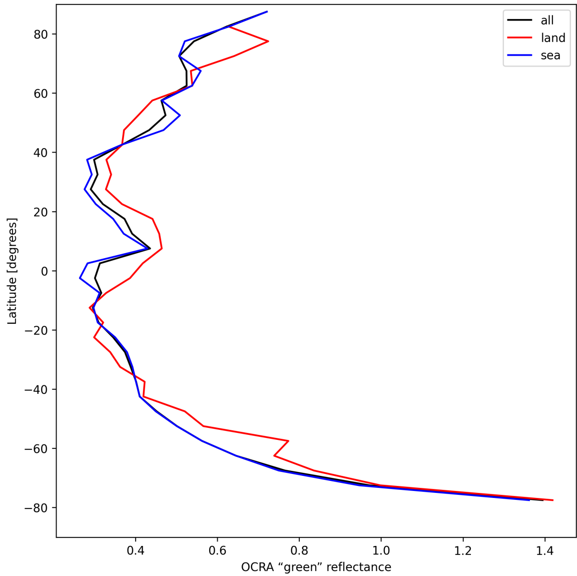
Figure 36: Zonal average of “OCRA “green” reflectance” for 2025-08-16 to 2025-08-18.
