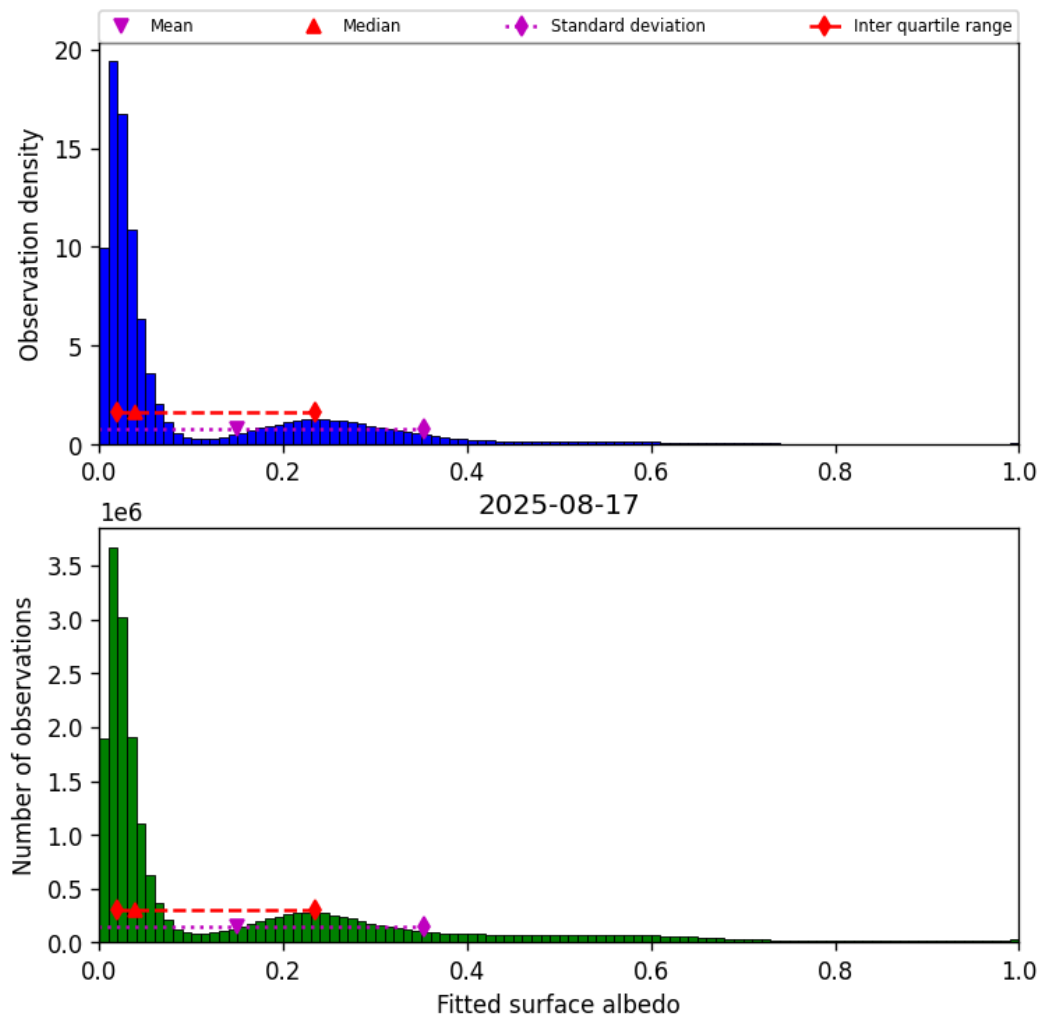
Figure 45: Histogram of “Fitted surface albedo” for 2025-08-16 to 2025-08-18
