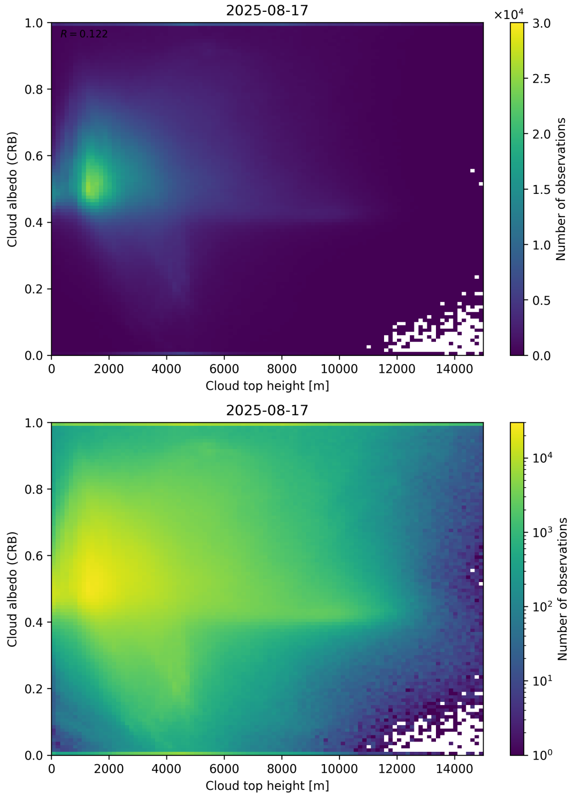
Figure 86: Scatter density plot of “Cloud top height” against “Cloud albedo (CRB)” for 2025-08-16 to 2025-08-18.
