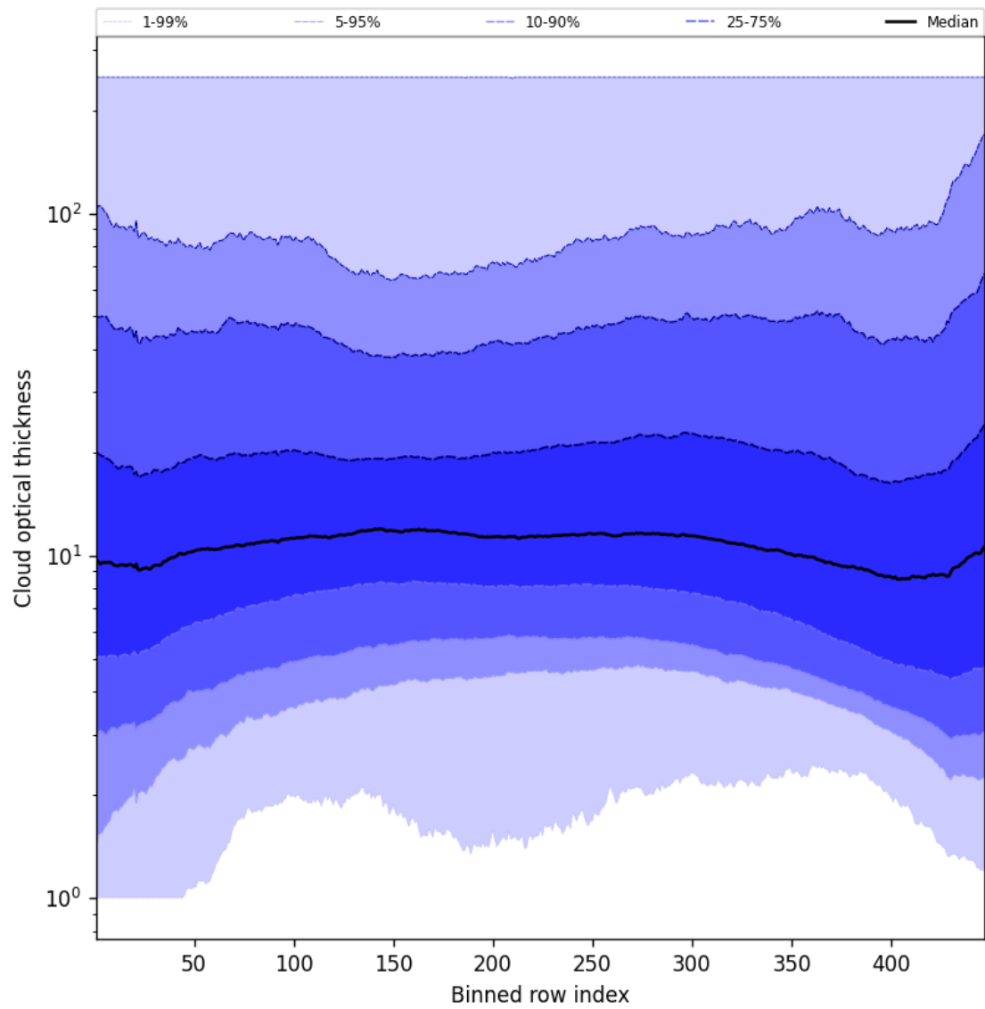
Figure 57: Along track statistics of “Cloud optical thickness” for 2025-08-16 to 2025-08-18
