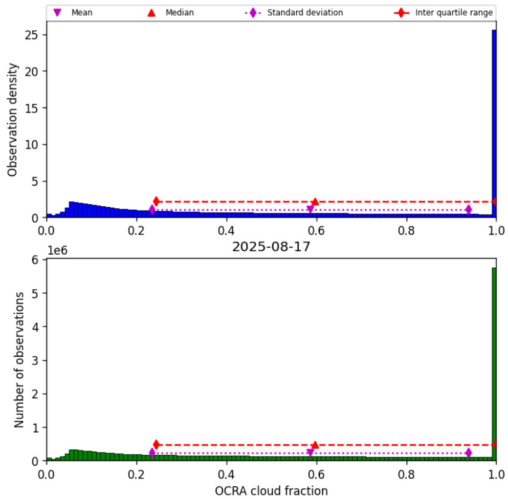
Figure 50: Histogram of “OCRA cloud fraction” for 2025-08-16 to 2025-08-18
