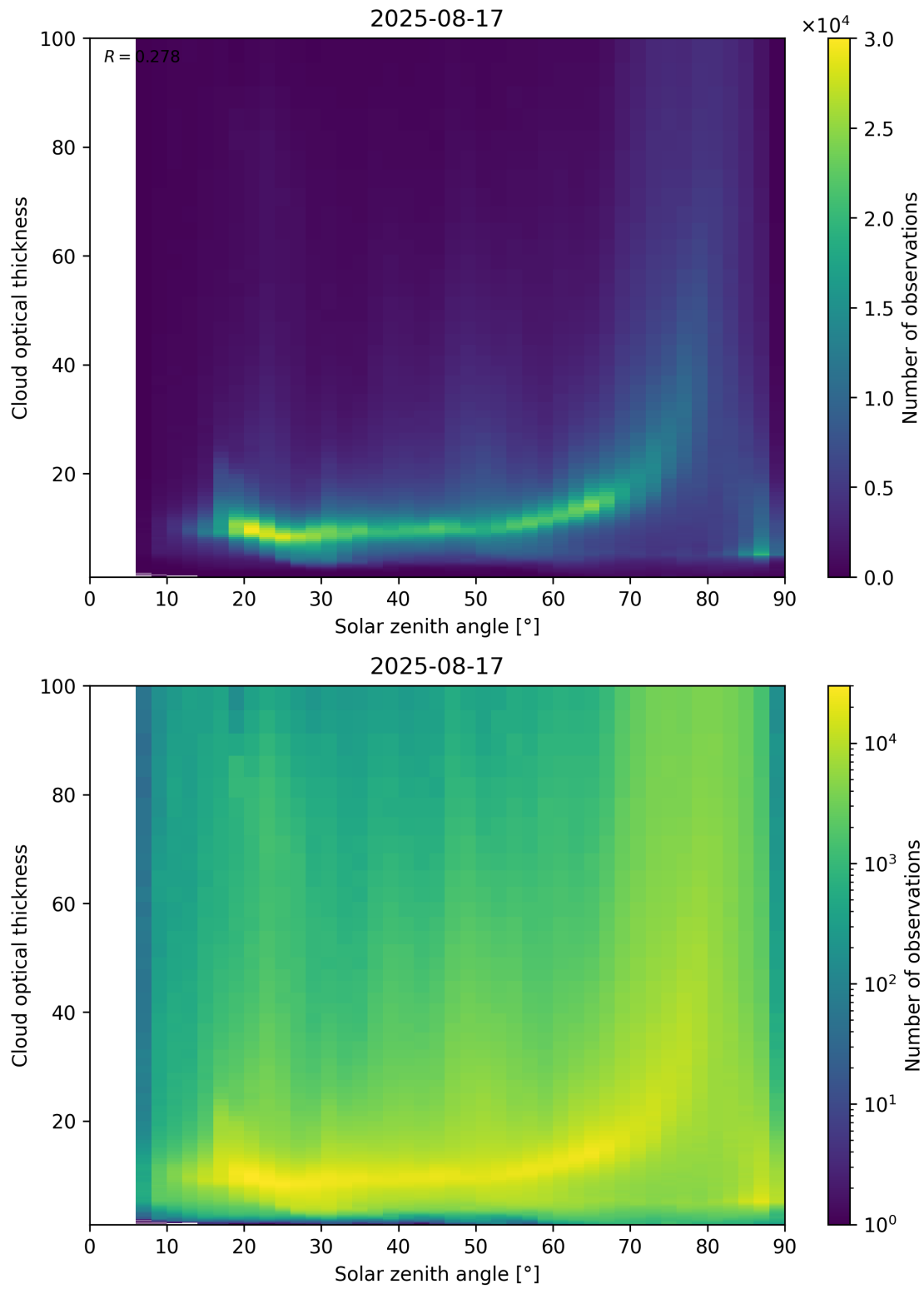
Figure 103: Scatter density plot of “Solar zenith angle” against “Cloud optical thickness” for 2025-08-16 to 2025-08-18.
