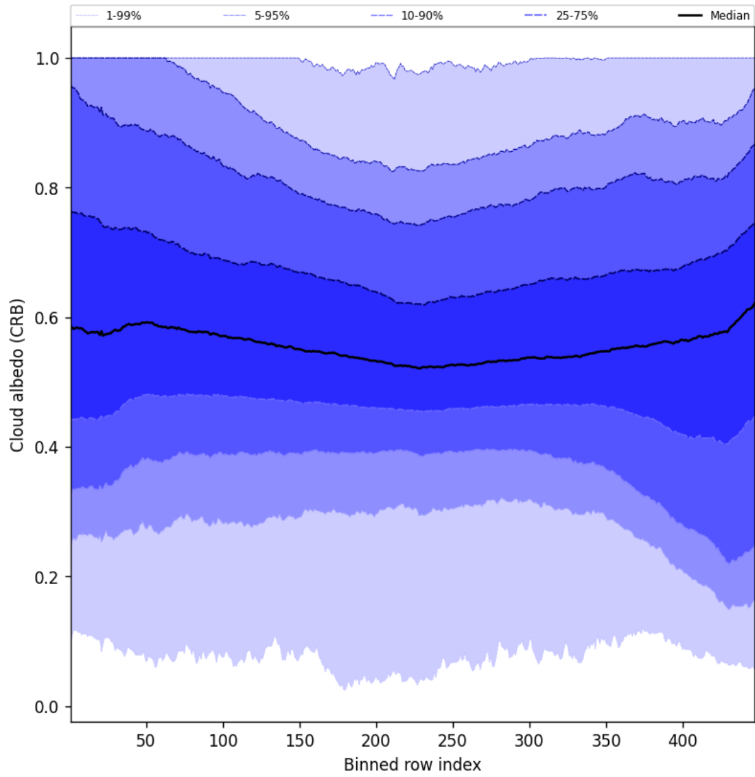
Figure 60: Along track statistics of “Cloud albedo (CRB)” for 2025-08-16 to 2025-08-18
