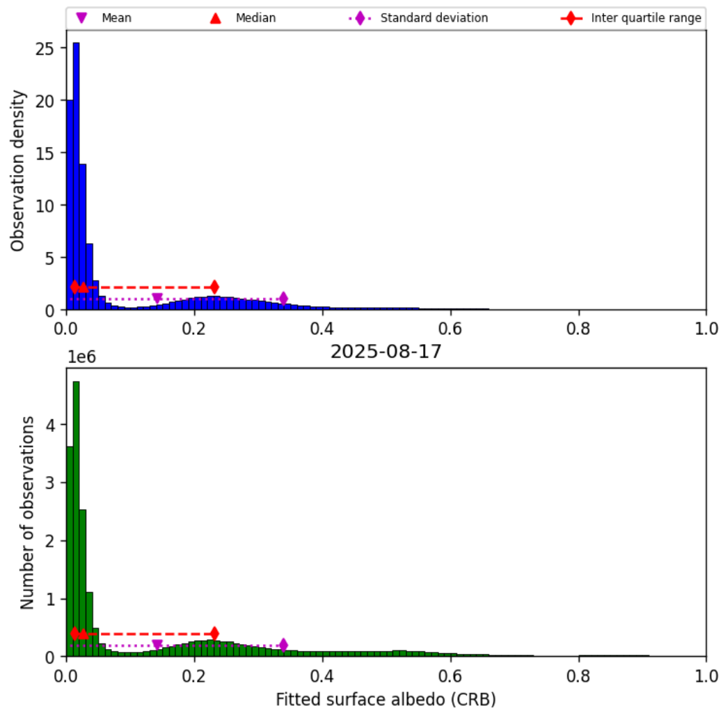
Figure 46: Histogram of “Fitted surface albedo (CRB)” for 2025-08-16 to 2025-08-18
