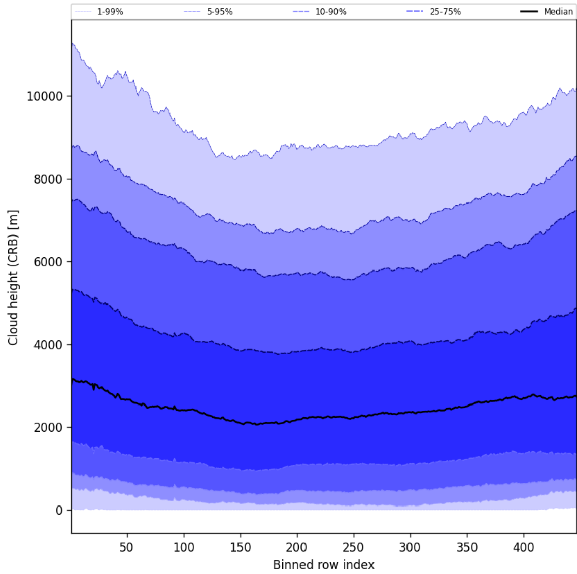
Figure 59: Along track statistics of “Cloud height (CRB)” for 2025-08-16 to 2025-08-18
