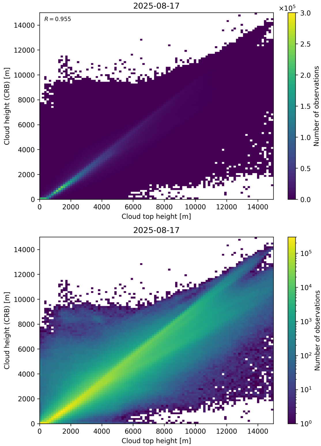
Figure 89: Scatter density plot of “Cloud top height” against “Cloud height (CRB)” for 2025-08-16 to 2025-08-18.
