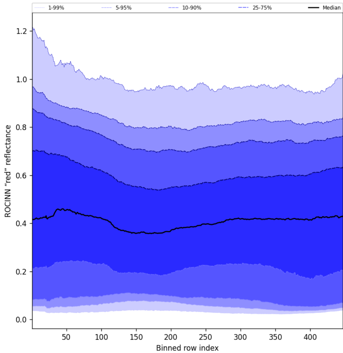
Figure 69: Along track statistics of “ROCINN “red” reflectance” for 2025-08-16 to 2025-08-18
