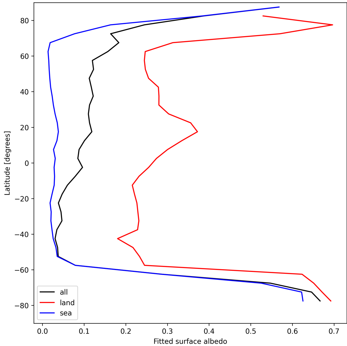
Figure 29: Zonal average of “Fitted surface albedo” for 2025-08-16 to 2025-08-18.
