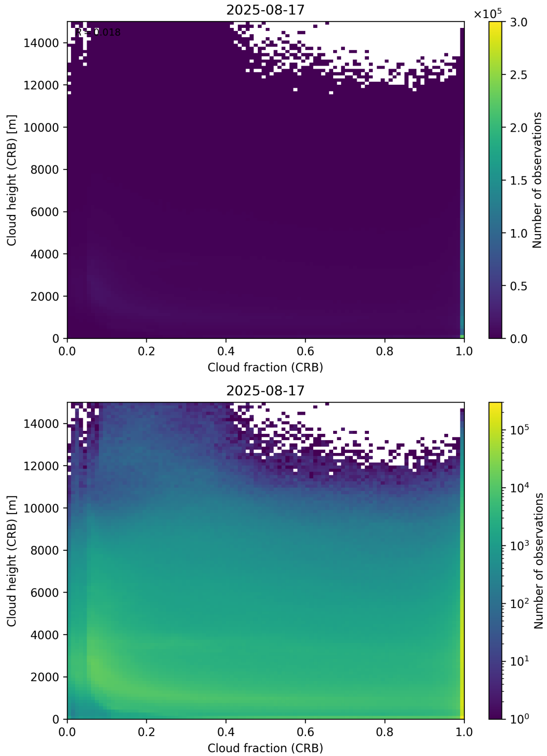
Figure 79: Scatter density plot of “Cloud fraction (CRB)” against “Cloud height (CRB)” for 2025-08-16 to 2025-08-18.
