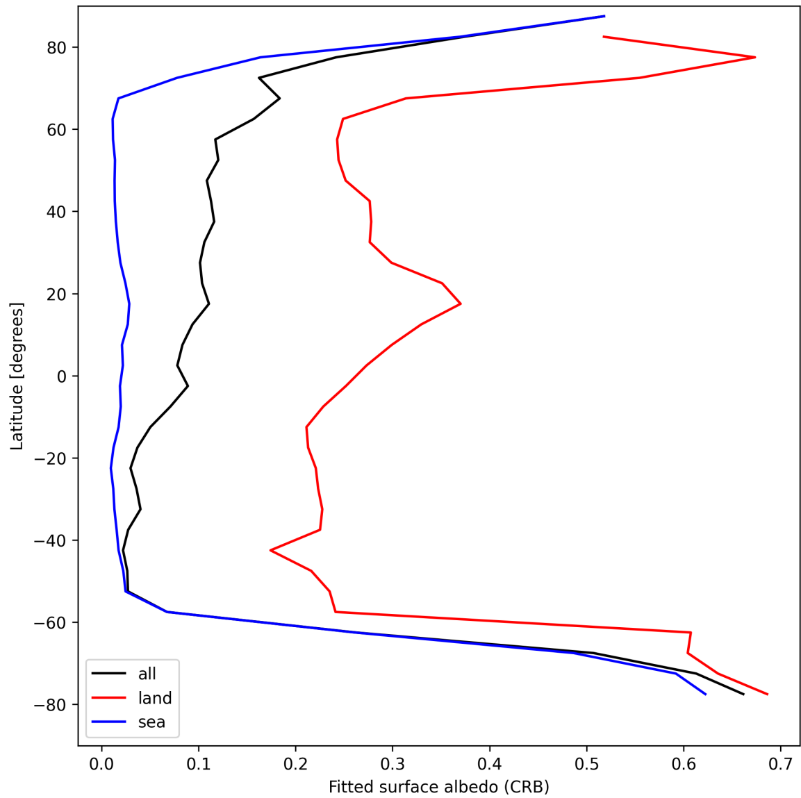
Figure 30: Zonal average of “Fitted surface albedo (CRB)” for 2025-08-16 to 2025-08-18.
