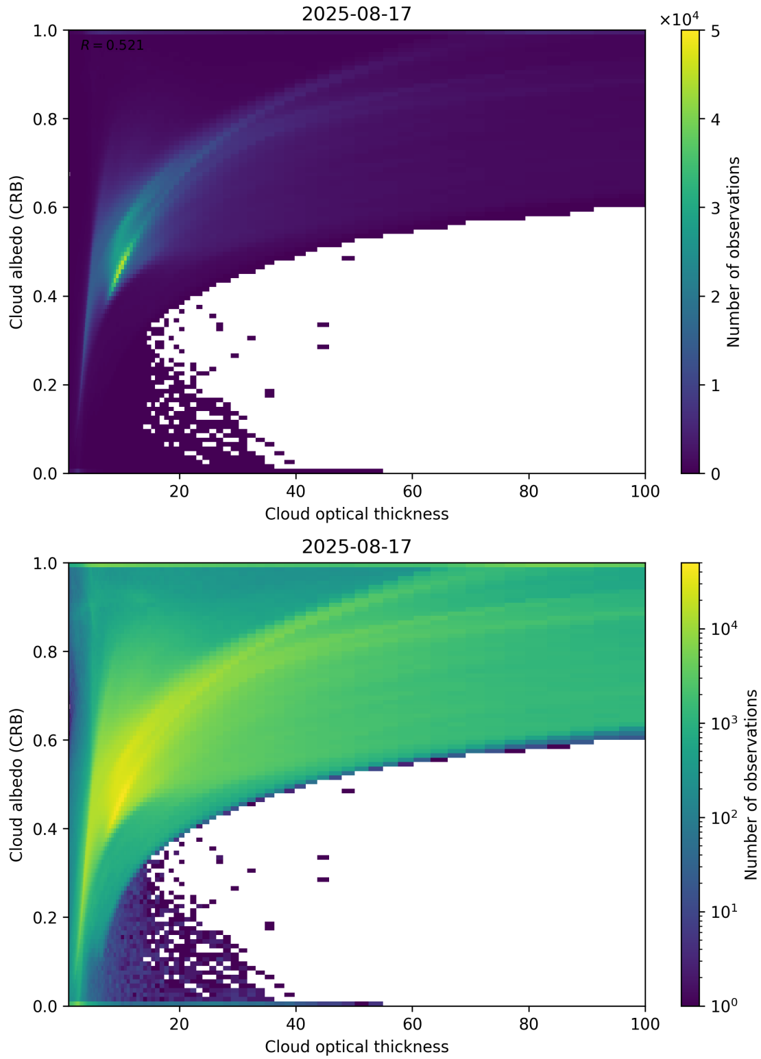
Figure 82: Scatter density plot of “Cloud optical thickness” against “Cloud albedo (CRB)” for 2025-08-16 to 2025-08-18.
