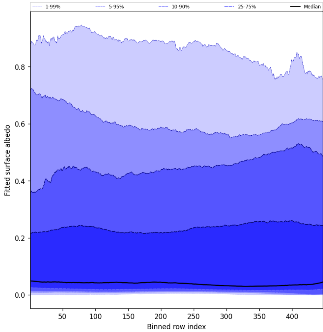
Figure 61: Along track statistics of “Fitted surface albedo” for 2025-08-16 to 2025-08-18
