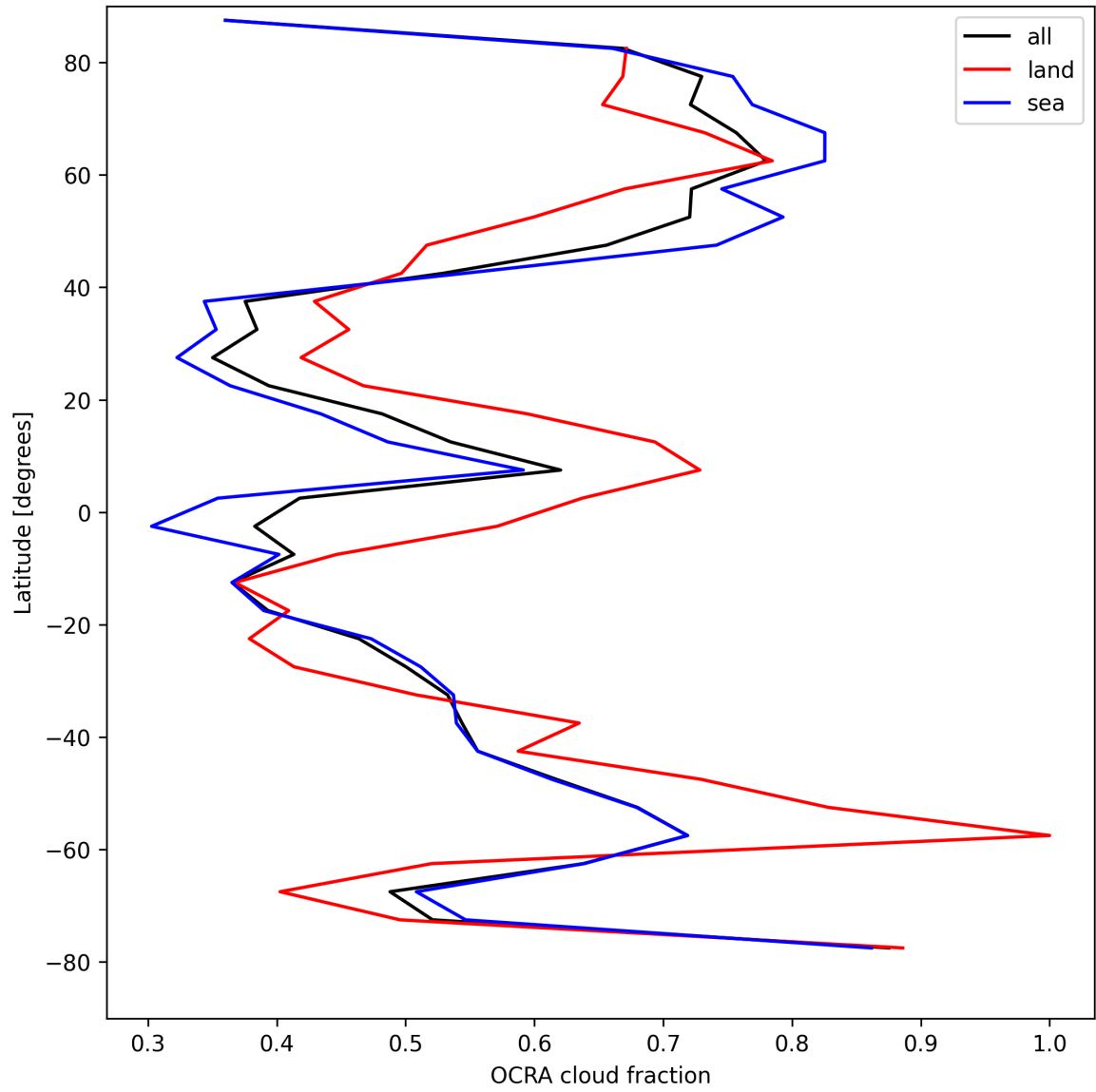
Figure 34: Zonal average of “OCRA cloud fraction” for 2025-08-16 to 2025-08-18.
