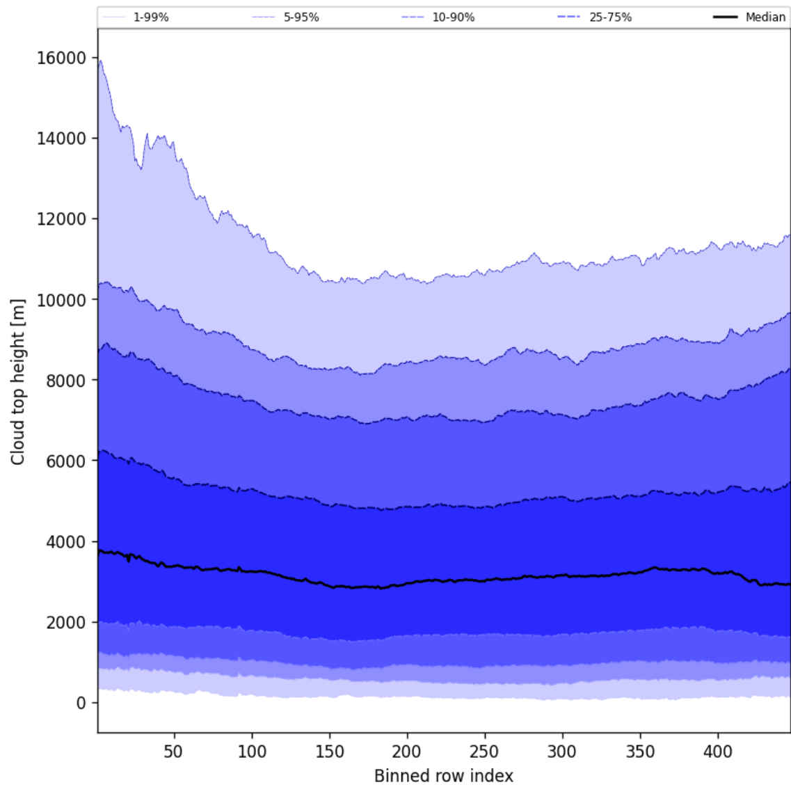
Figure 56: Along track statistics of “Cloud top height” for 2025-08-16 to 2025-08-18
