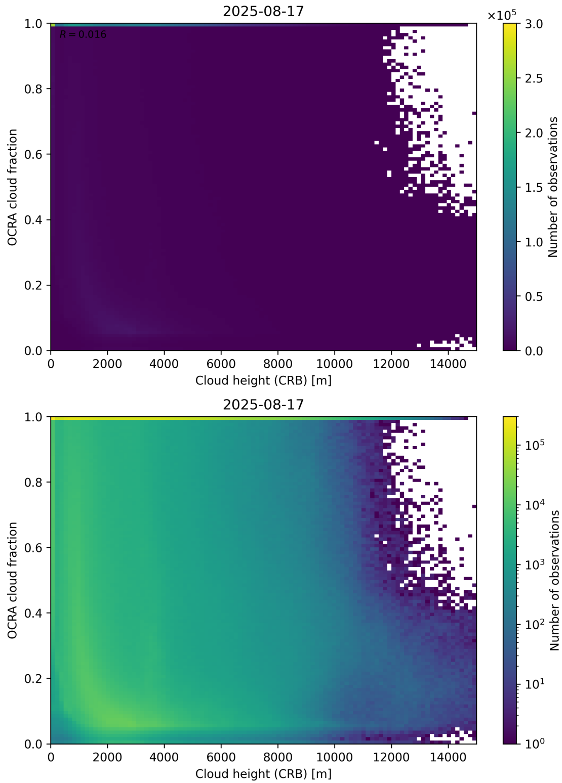
Figure 81: Scatter density plot of “Cloud height (CRB)” against “OCRA cloud fraction” for 2025-08-16 to 2025-08-18.
