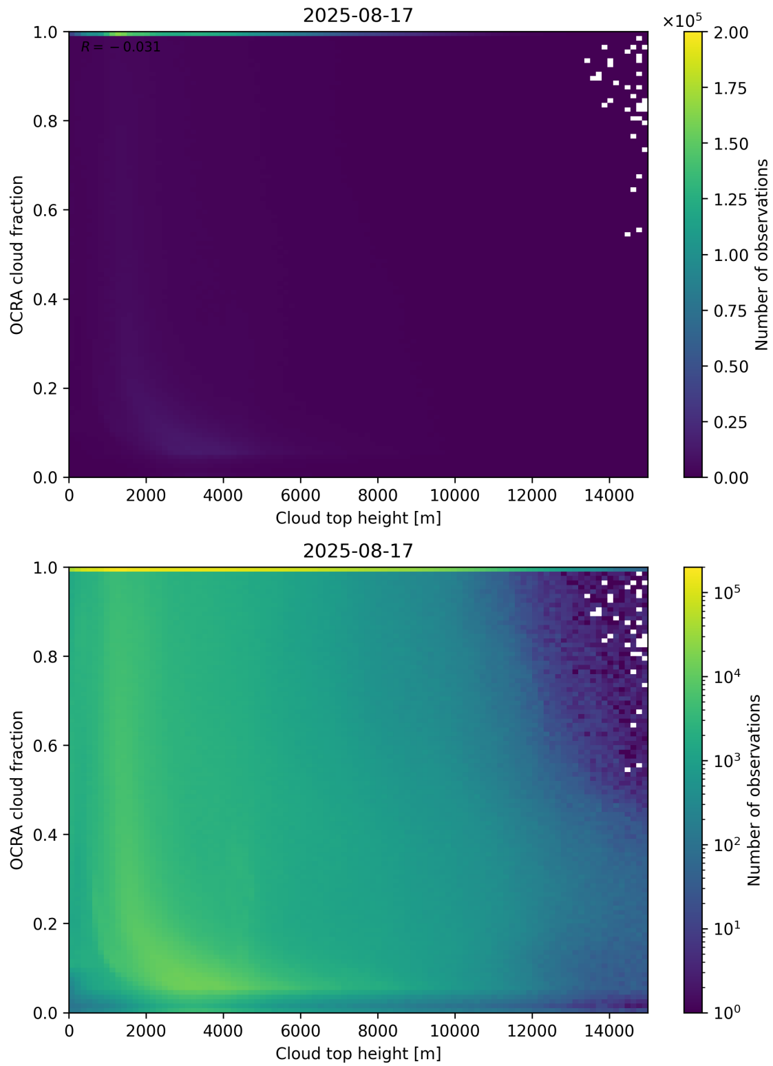
Figure 87: Scatter density plot of “Cloud top height” against “OCRA cloud fraction” for 2025-08-16 to 2025-08-18.
