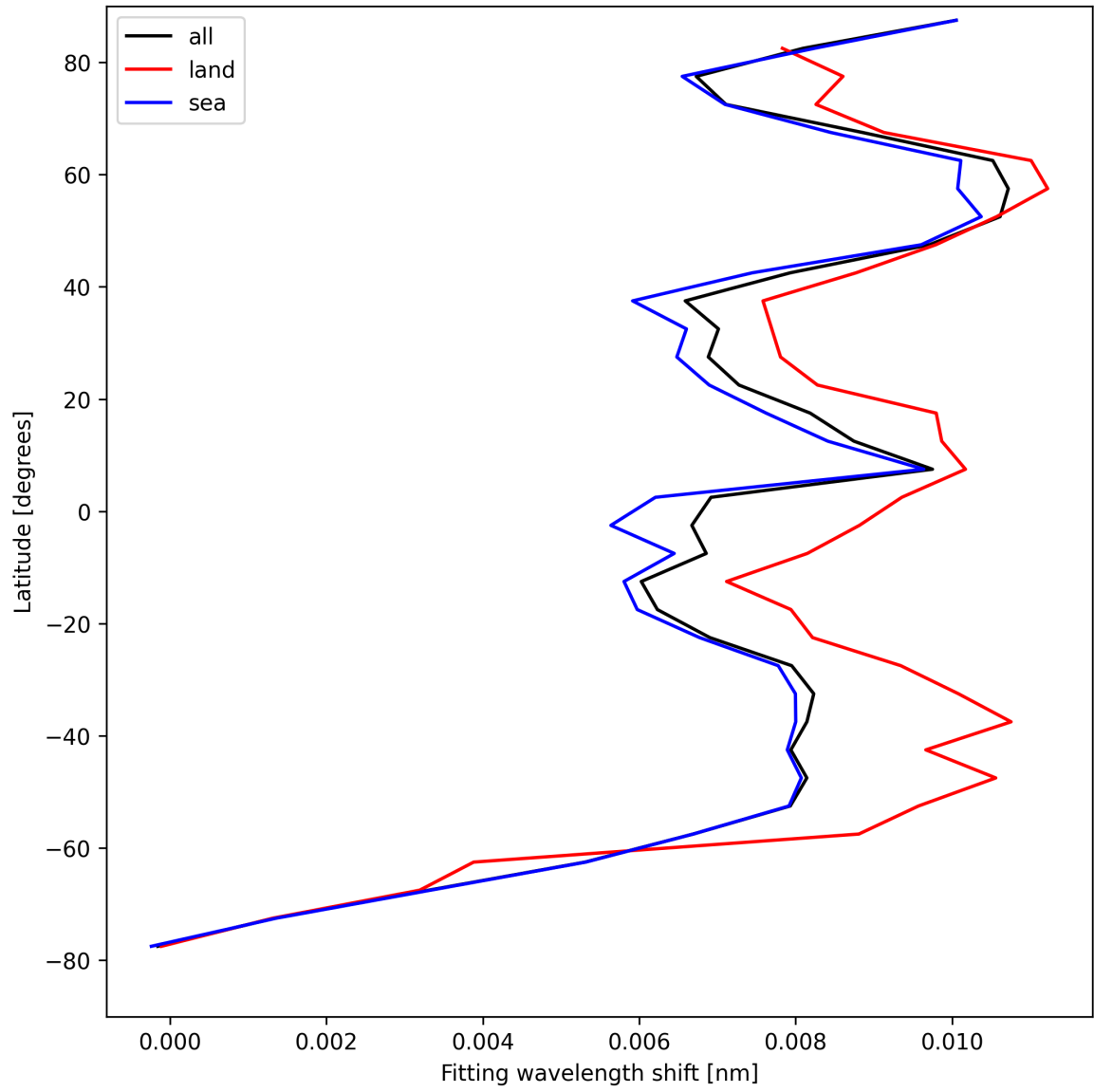
Figure 33: Zonal average of “Fitting wavelength shift” for 2025-08-16 to 2025-08-18.
