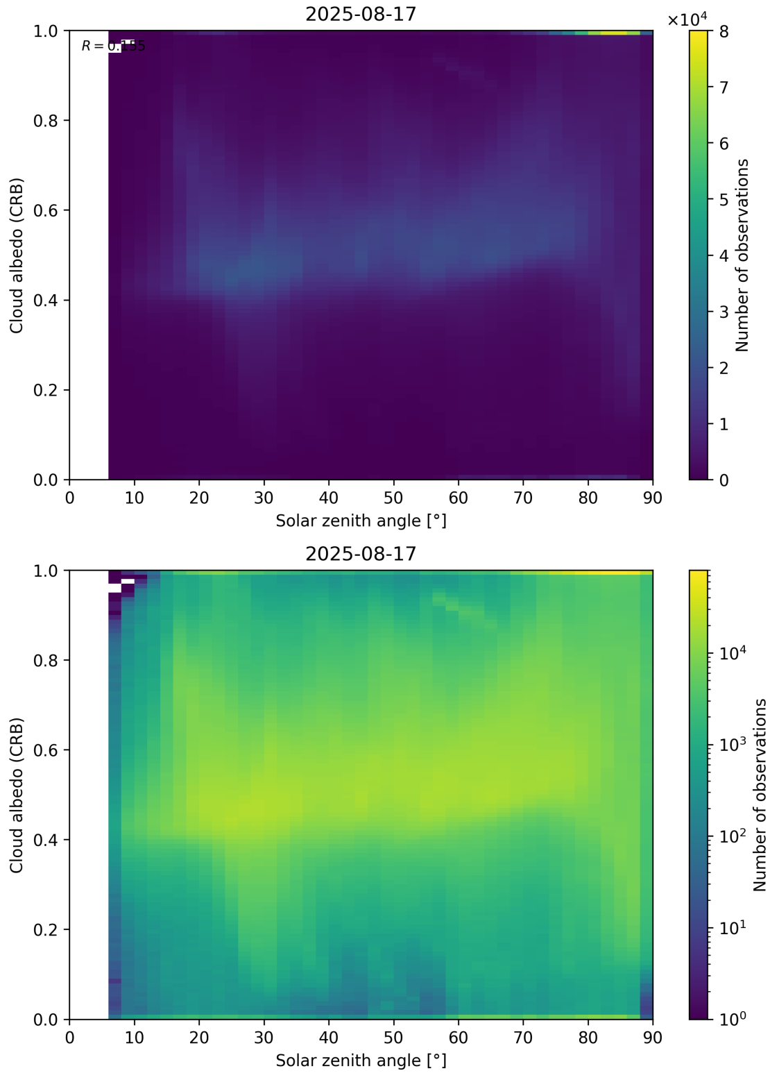
Figure 98: Scatter density plot of “Solar zenith angle” against “Cloud albedo (CRB)” for 2025-08-16 to 2025-08-18.
