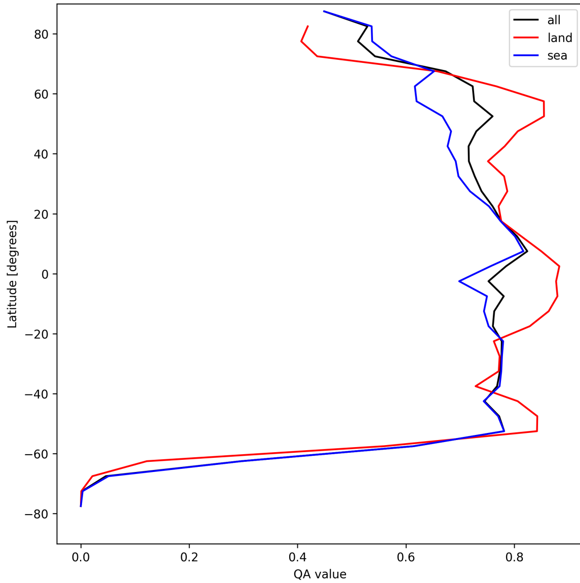
Figure 22: Zonal average of “QA value” for 2025-08-16 to 2025-08-18.
