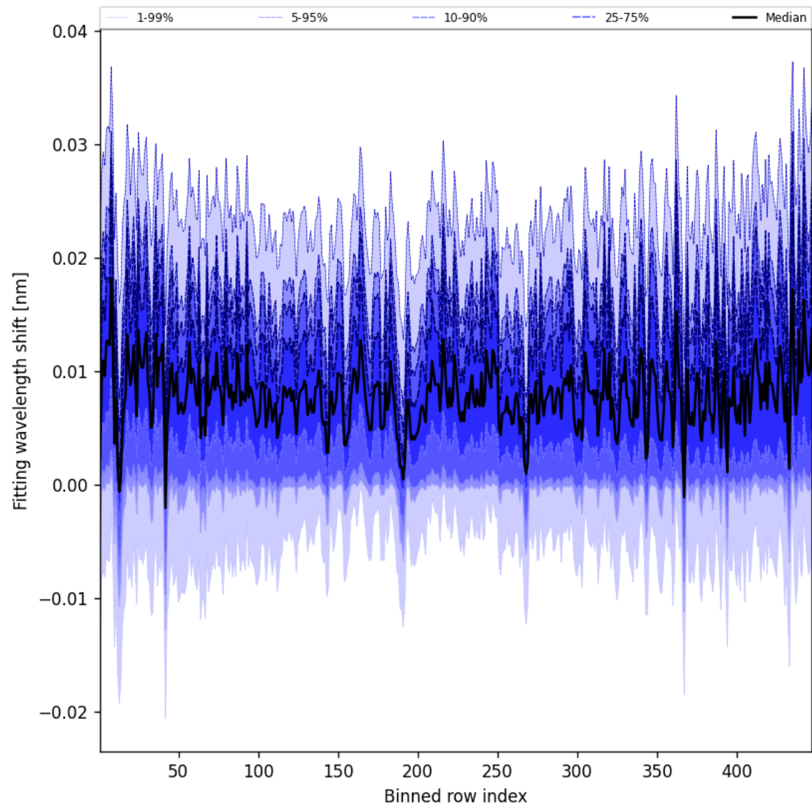
Figure 65: Along track statistics of “Fitting wavelength shift” for 2025-08-16 to 2025-08-18
