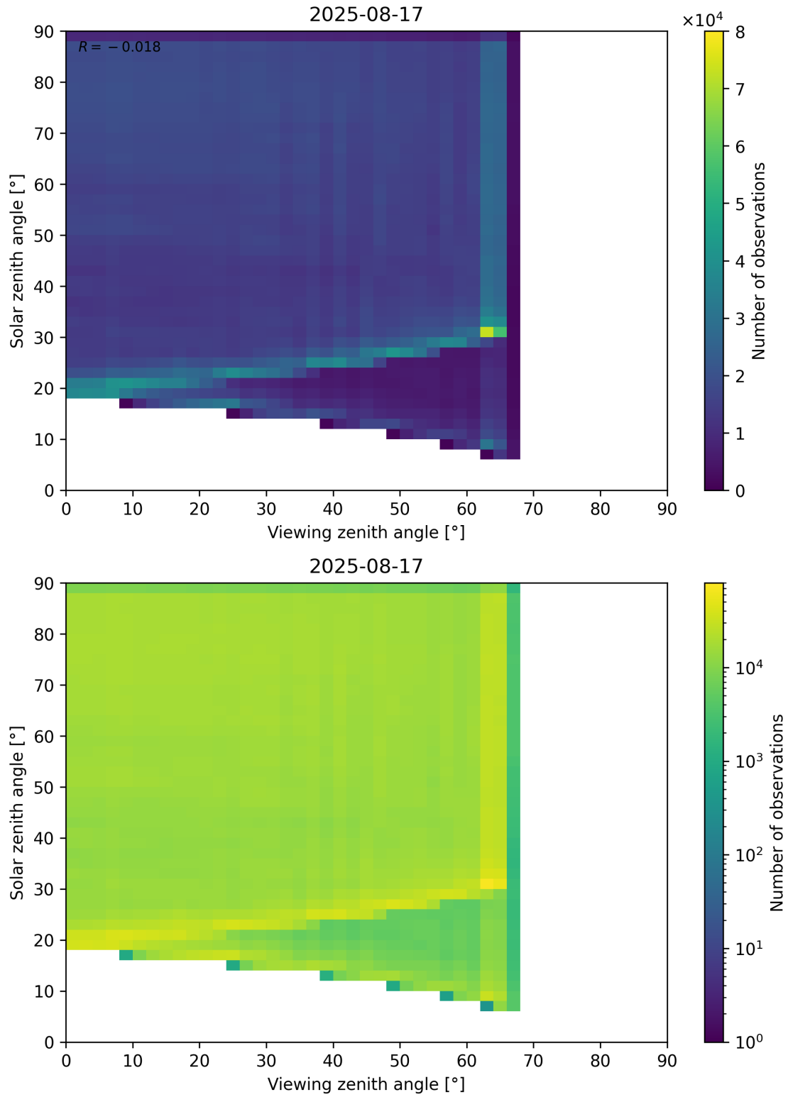
Figure 114: Scatter density plot of “Viewing zenith angle” against “Solar zenith angle” for 2025-08-16 to 2025-08-18.
