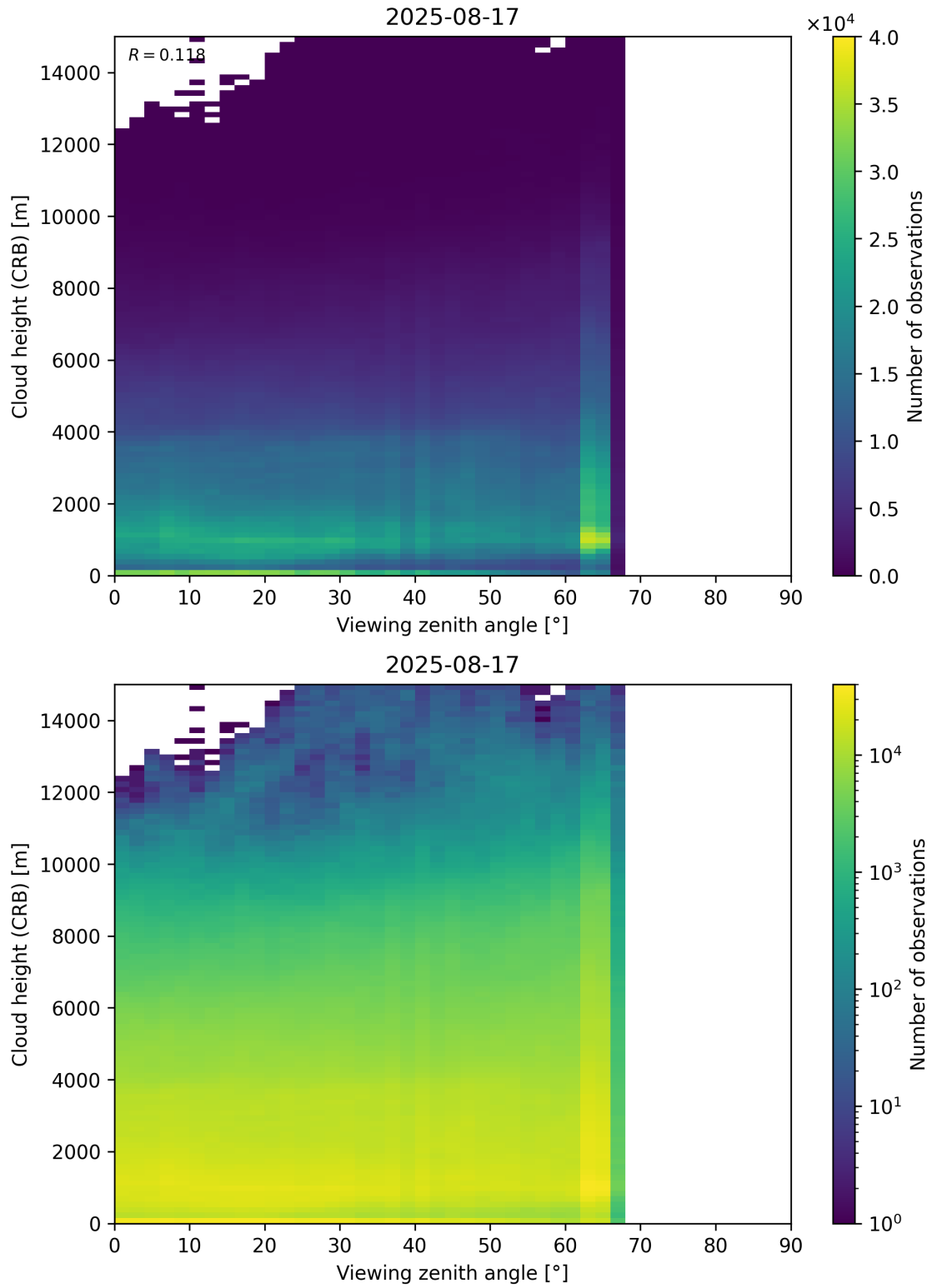
Figure 110: Scatter density plot of “Viewing zenith angle” against “Cloud height (CRB)” for 2025-08-16 to 2025-08-18.
