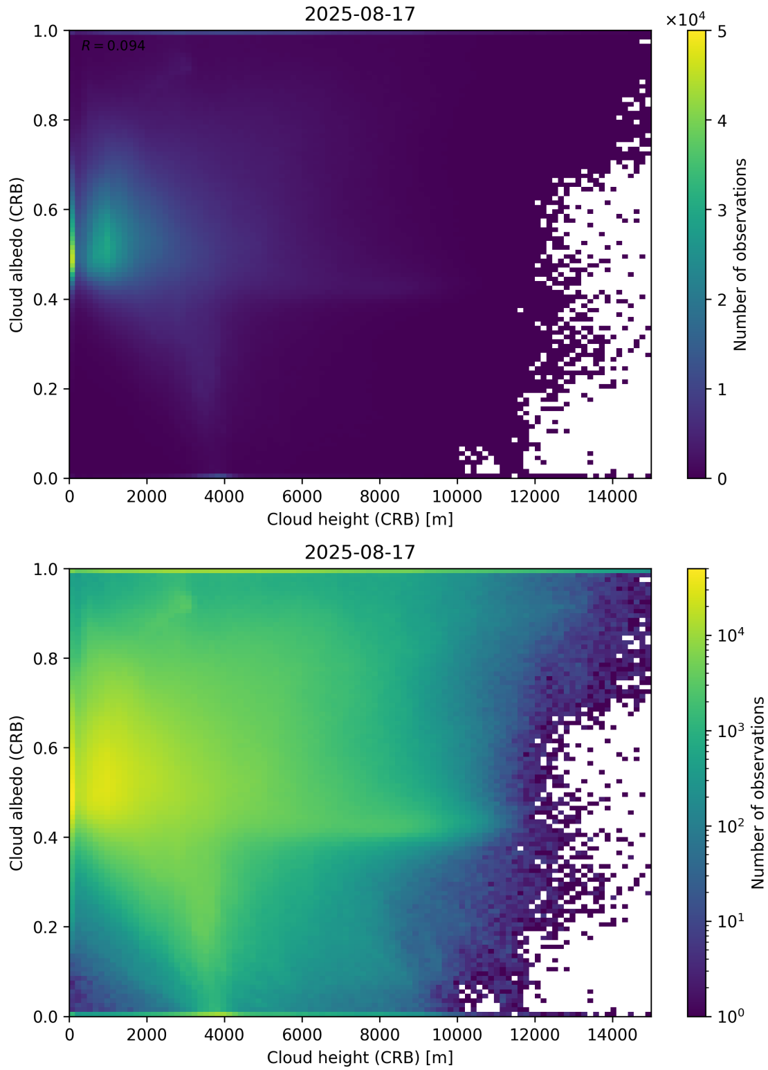
Figure 80: Scatter density plot of “Cloud height (CRB)” against “Cloud albedo (CRB)” for 2025-08-16 to 2025-08-18.
