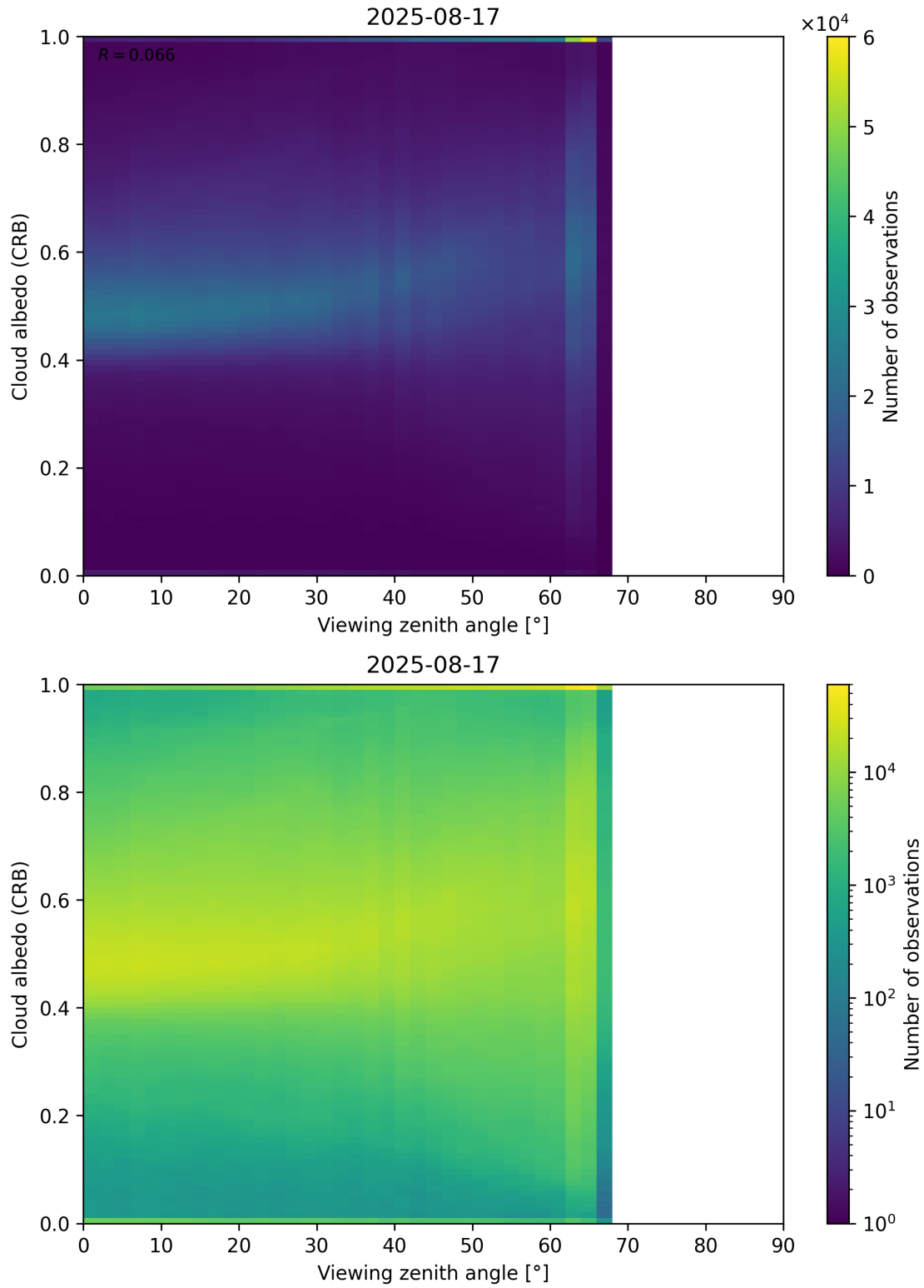
Figure 106: Scatter density plot of “Viewing zenith angle” against “Cloud albedo (CRB)” for 2025-08-16 to 2025-08-18.
