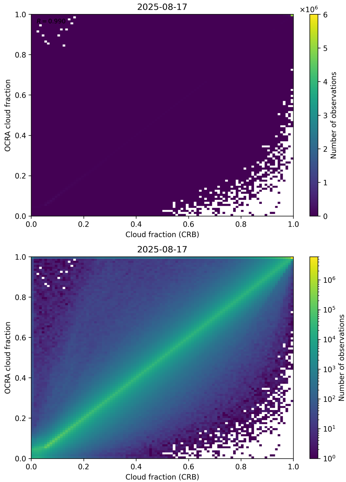
Figure 78: Scatter density plot of “Cloud fraction (CRB)” against “OCRA cloud fraction” for 2025-08-16 to 2025-08-18.
