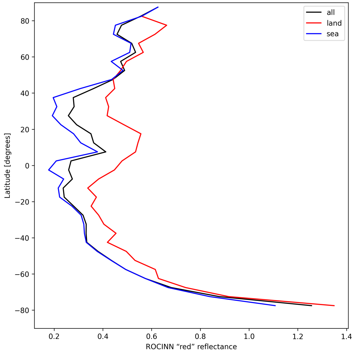
Figure 37: Zonal average of “ROCINN “red” reflectance” for 2025-08-16 to 2025-08-18.
