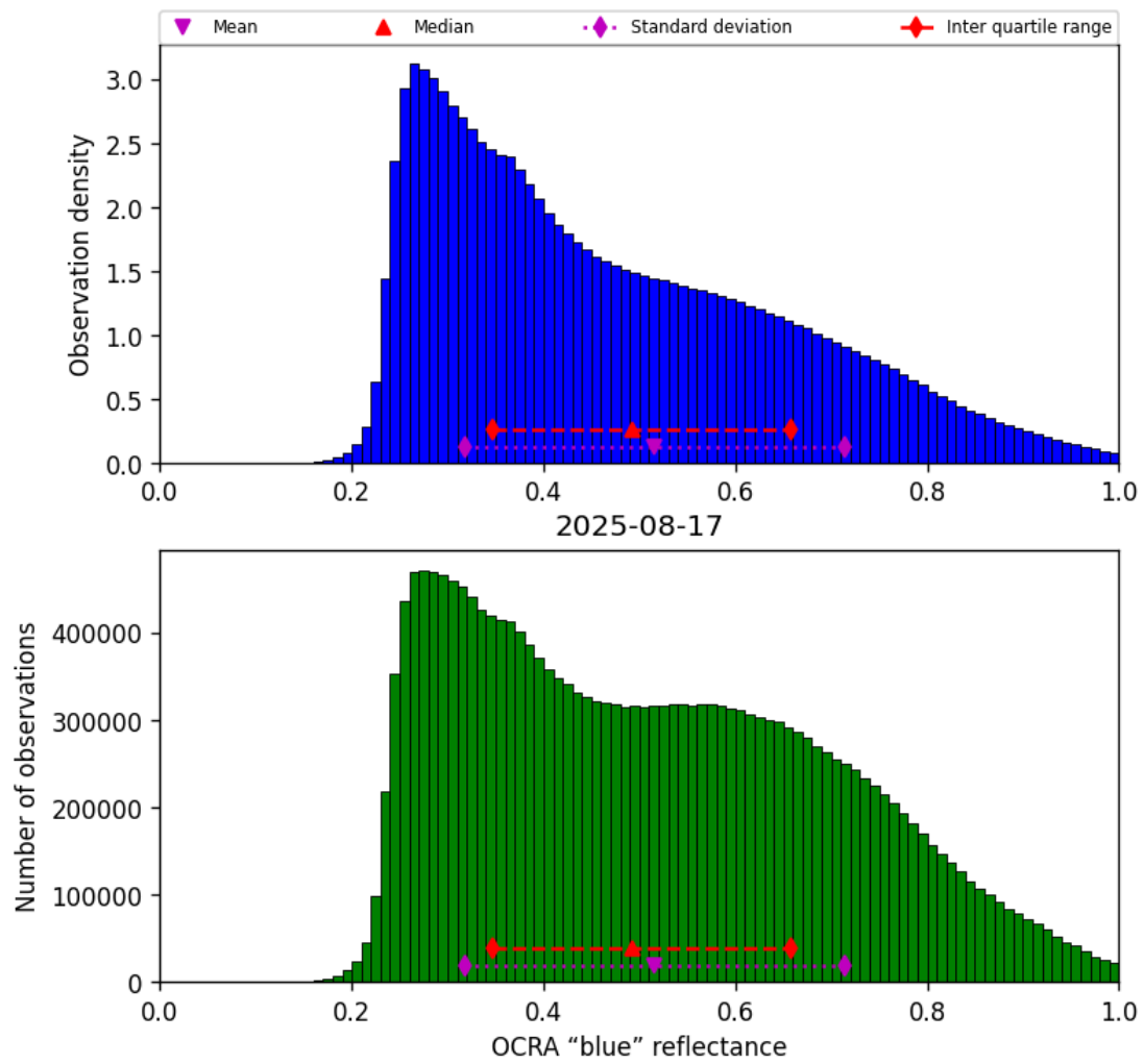
Figure 51: Histogram of “OCRA “blue” reflectance” for 2025-08-16 to 2025-08-18
