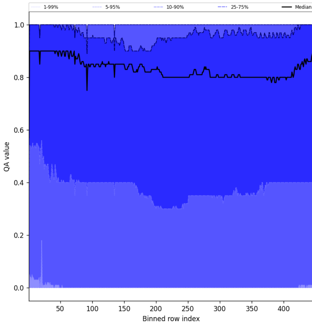
Figure 54: Along track statistics of “QA value” for 2025-08-16 to 2025-08-18
