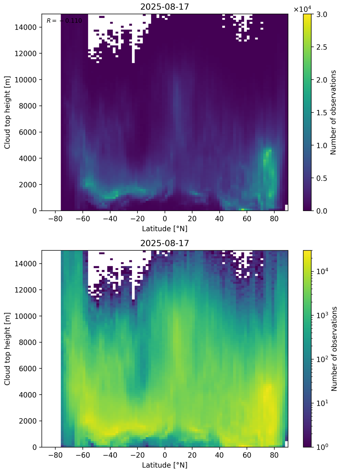
Figure 97: Scatter density plot of “Latitude” against “Cloud top height” for 2025-08-16 to 2025-08-18.
