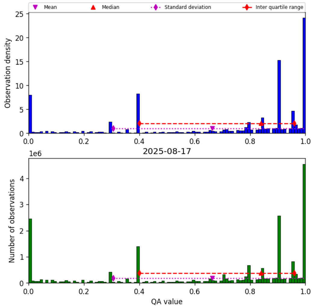
Figure 38: Histogram of “QA value” for 2025-08-16 to 2025-08-18
