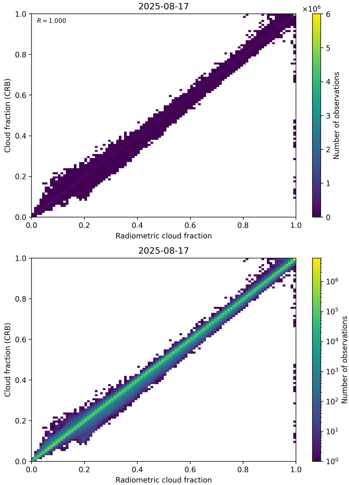
Figure 73: Scatter density plot of “Radiometric cloud fraction” against “Cloud fraction (CRB)” for 2025-08-16 to 2025-08-18.
