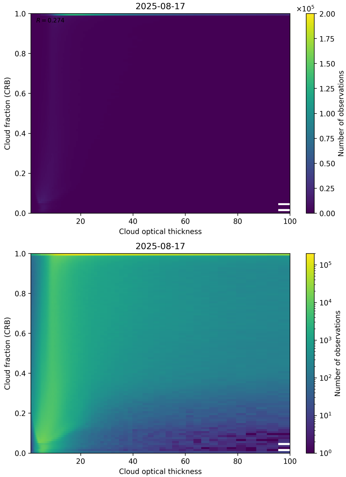
Figure 84: Scatter density plot of “Cloud optical thickness” against “Cloud fraction (CRB)” for 2025-08-16 to 2025-08-18.
