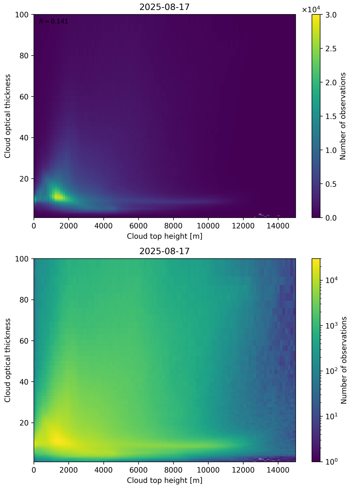
Figure 90: Scatter density plot of “Cloud top height” against “Cloud optical thickness” for 2025-08-16 to 2025-08-18.
