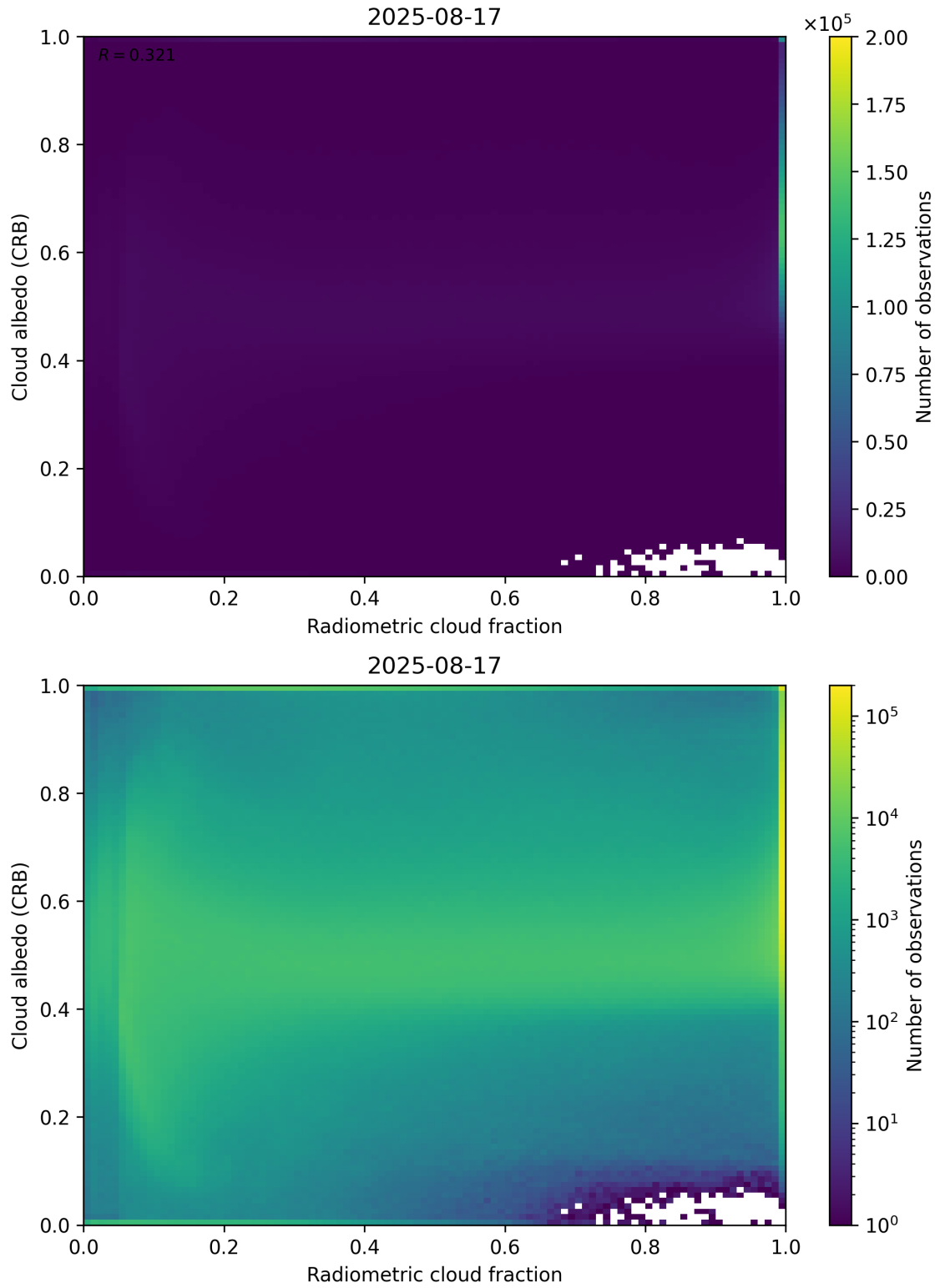
Figure 71: Scatter density plot of “Radiometric cloud fraction” against “Cloud albedo (CRB)” for 2025-08-16 to 2025-08-18.
