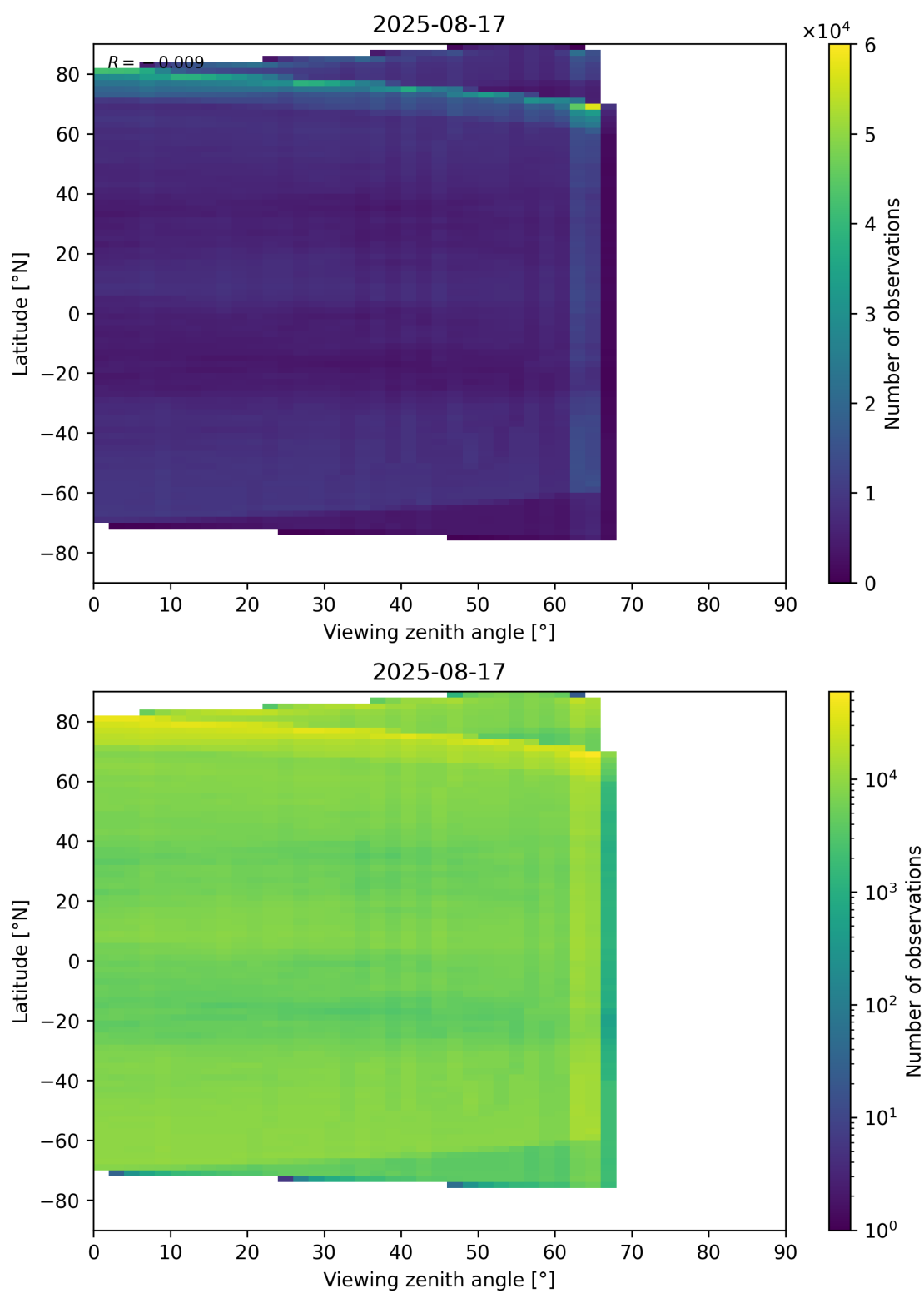
Figure 113: Scatter density plot of “Viewing zenith angle” against “Latitude” for 2025-08-16 to 2025-08-18.
