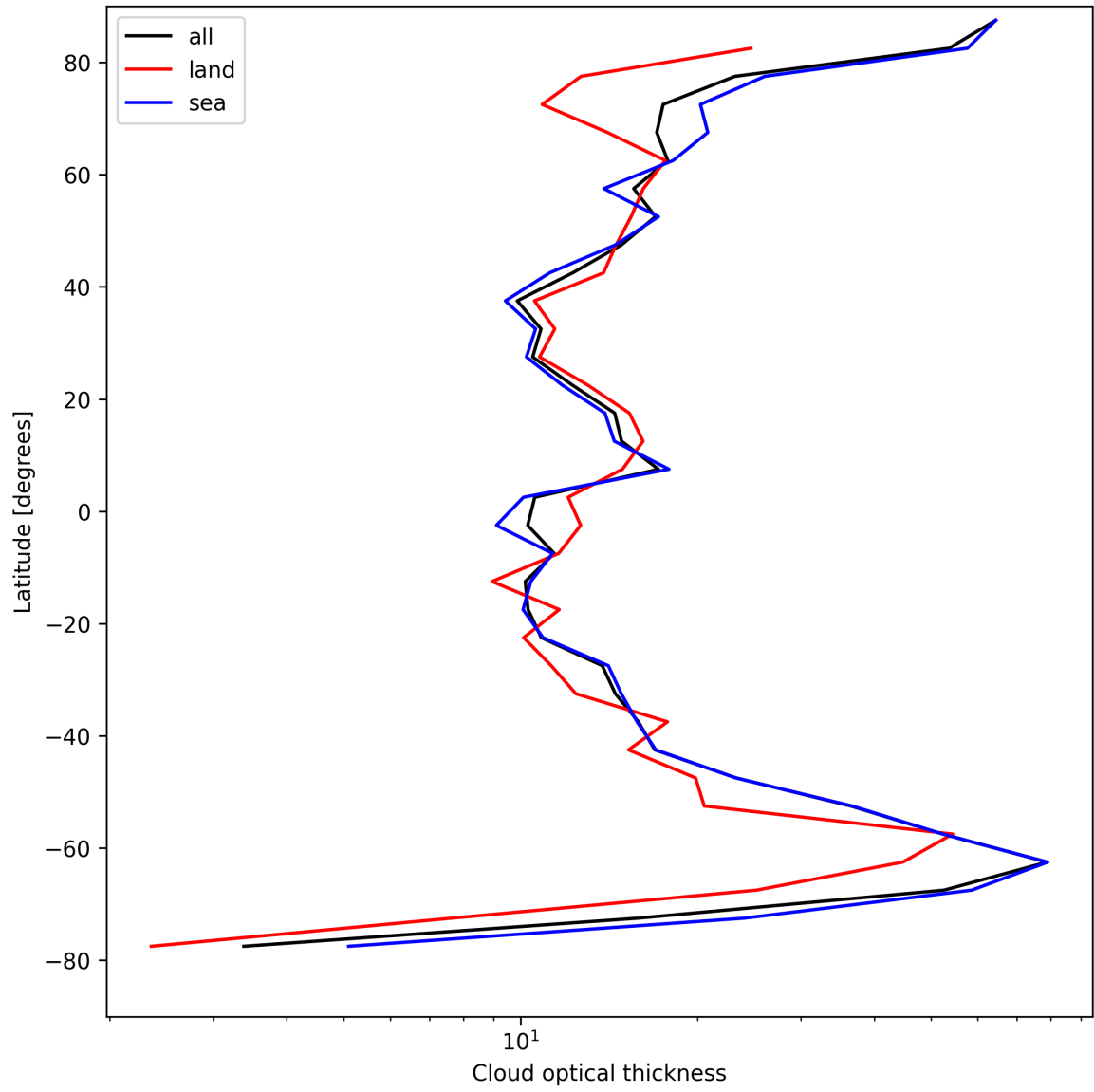
Figure 25: Zonal average of “Cloud optical thickness” for 2025-08-16 to 2025-08-18.
