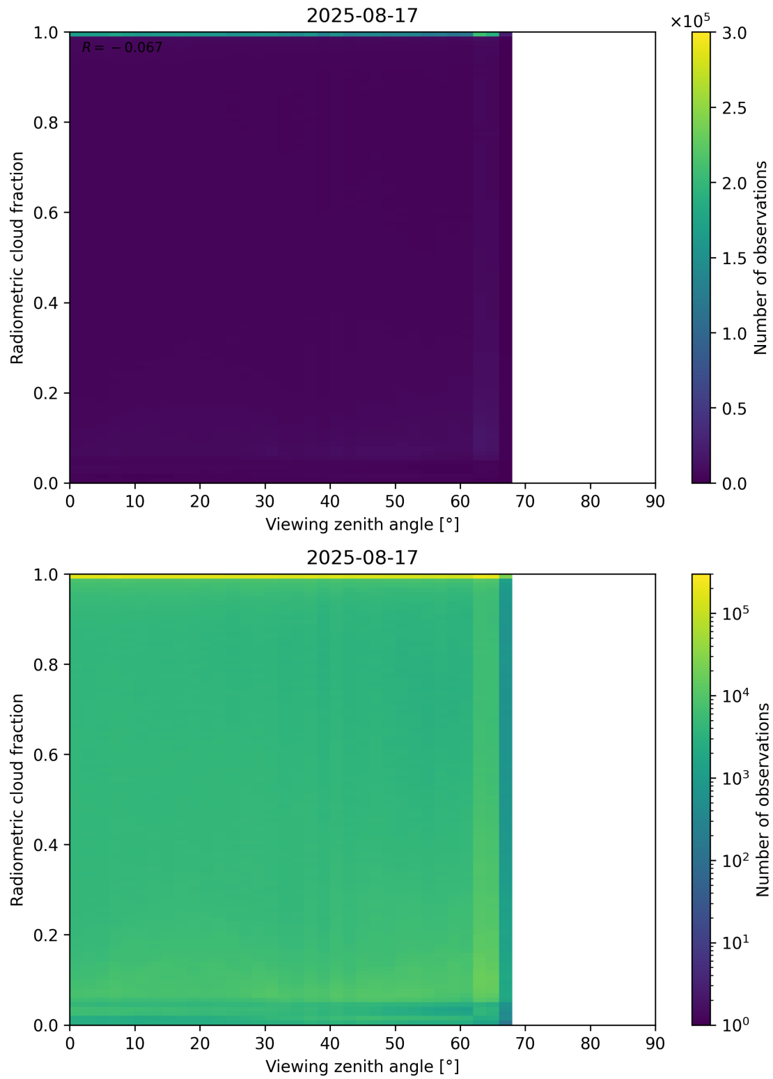
Figure 107: Scatter density plot of “Viewing zenith angle” against “Radiometric cloud fraction” for 2025-08-16 to 2025-08-18.
