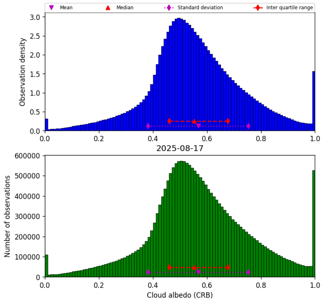
Figure 44: Histogram of “Cloud albedo (CRB)” for 2025-08-16 to 2025-08-18
