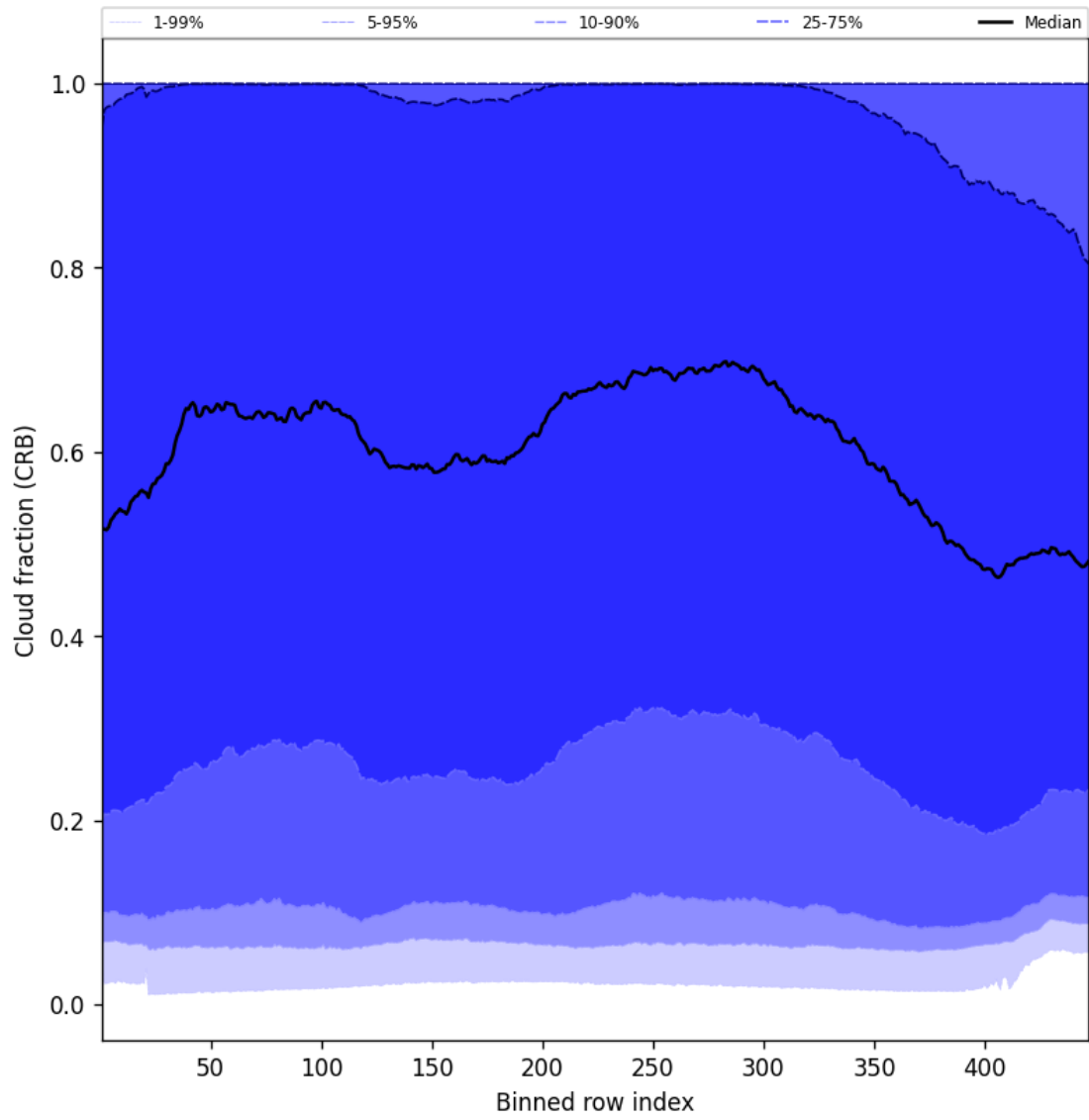
Figure 58: Along track statistics of “Cloud fraction (CRB)” for 2025-08-16 to 2025-08-18
