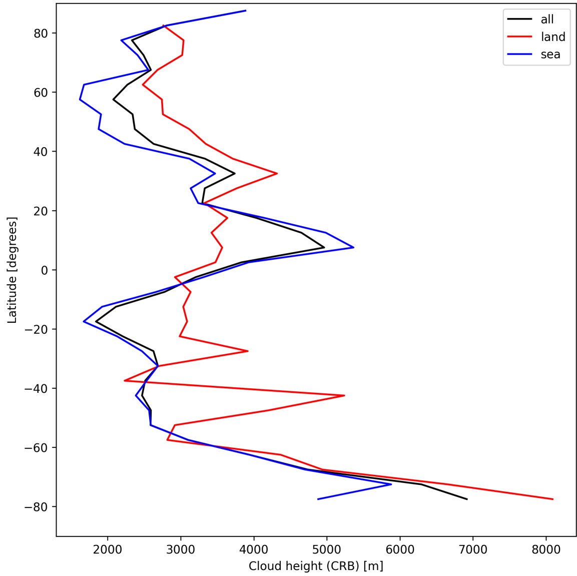
Figure 27: Zonal average of “Cloud height (CRB)” for 2025-08-16 to 2025-08-18.
