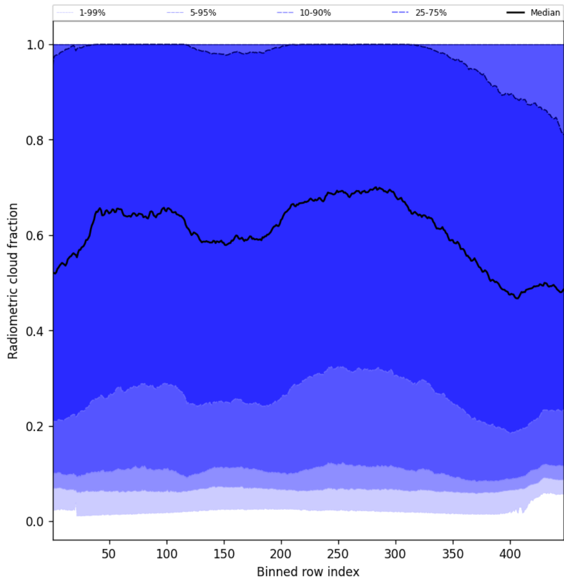
Figure 55: Along track statistics of “Radiometric cloud fraction” for 2025-08-16 to 2025-08-18
