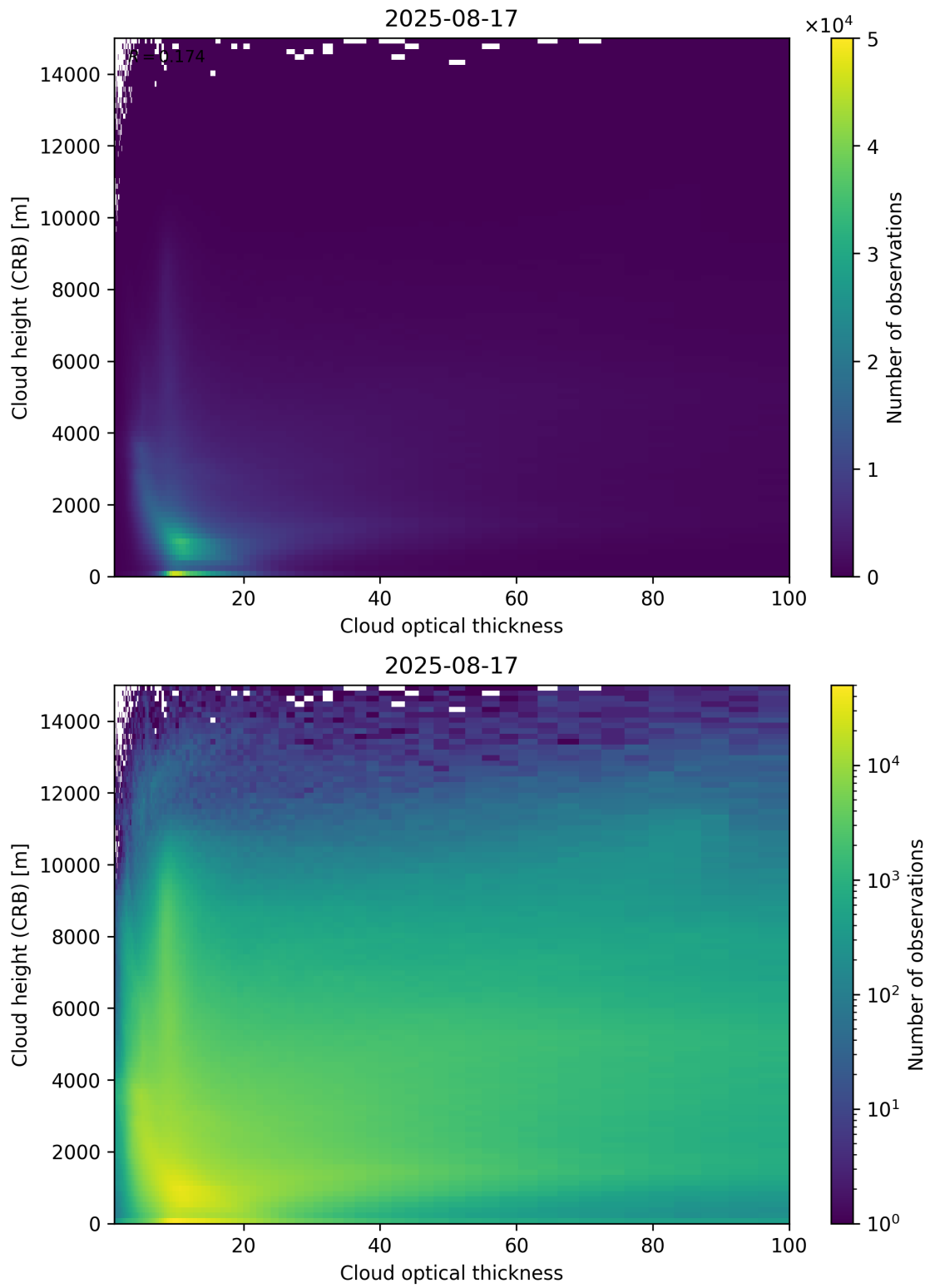
Figure 85: Scatter density plot of “Cloud optical thickness” against “Cloud height (CRB)” for 2025-08-16 to 2025-08-18.
