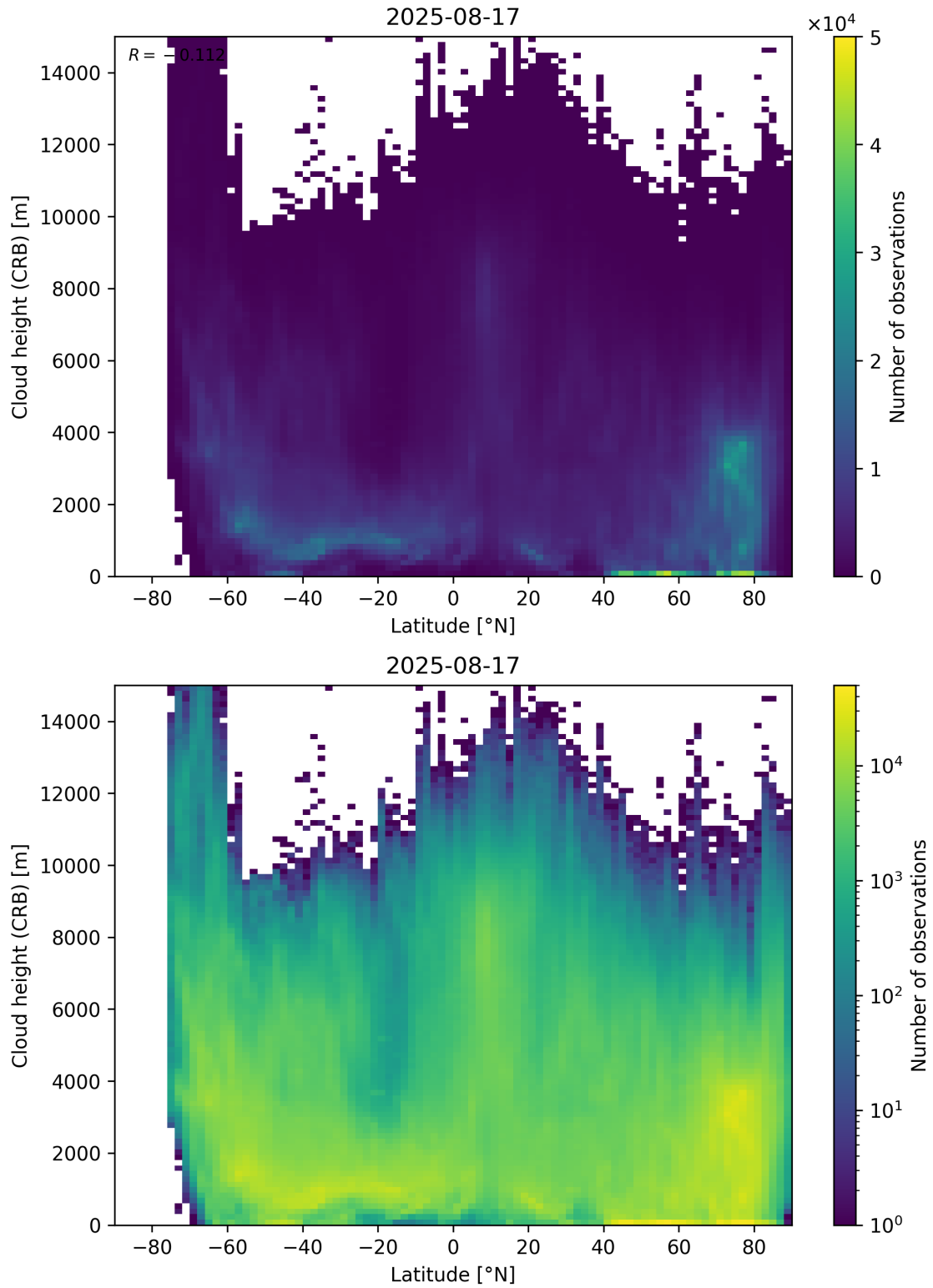
Figure 95: Scatter density plot of “Latitude” against “Cloud height (CRB)” for 2025-08-16 to 2025-08-18.
