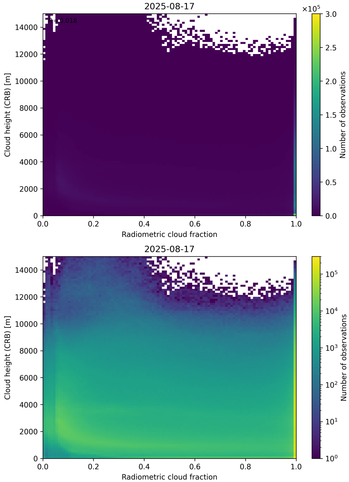
Figure 74: Scatter density plot of “Radiometric cloud fraction” against “Cloud height (CRB)” for 2025-08-16 to 2025-08-18.
