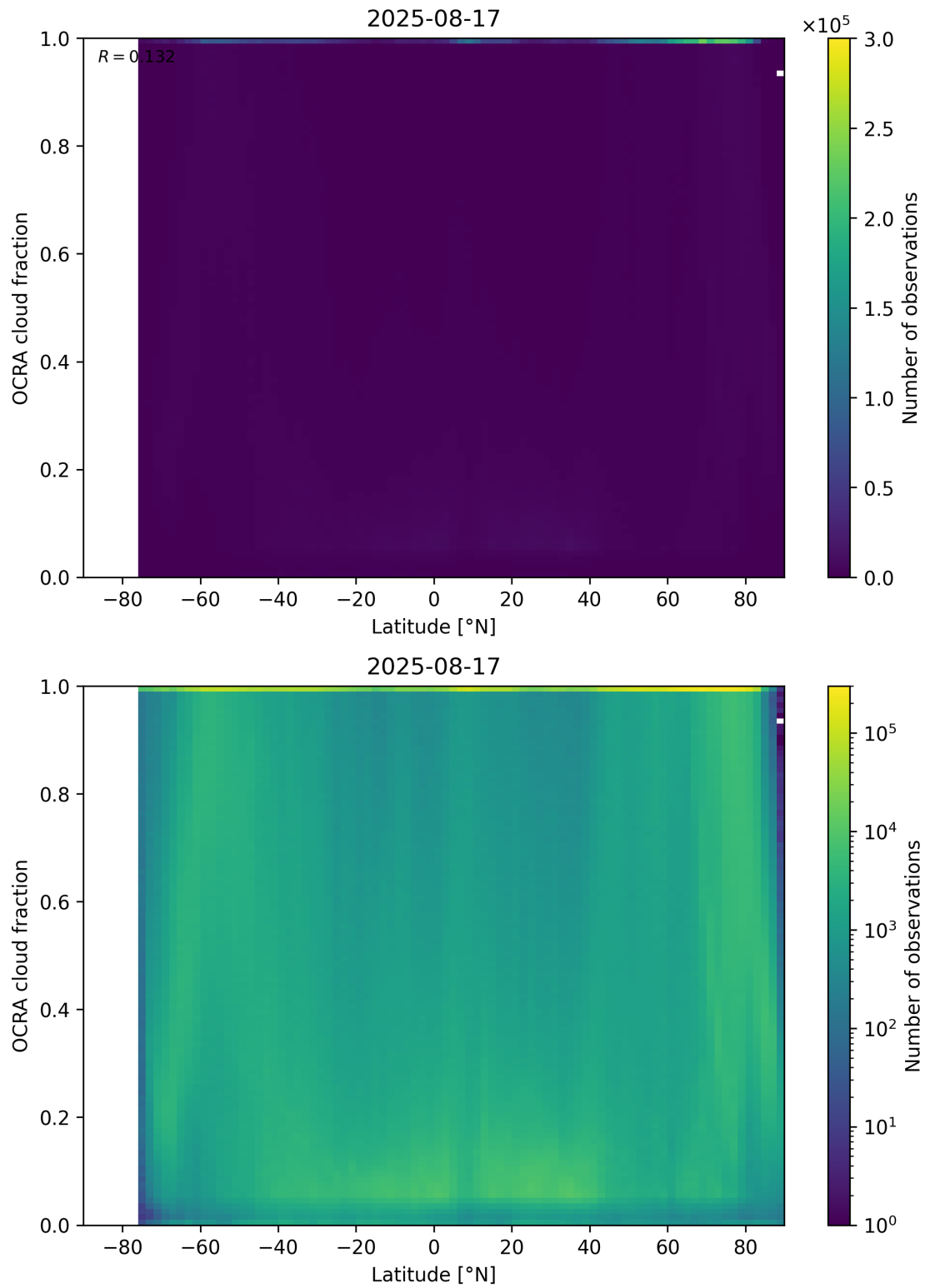
Figure 93: Scatter density plot of “Latitude” against “OCRA cloud fraction” for 2025-08-16 to 2025-08-18.
