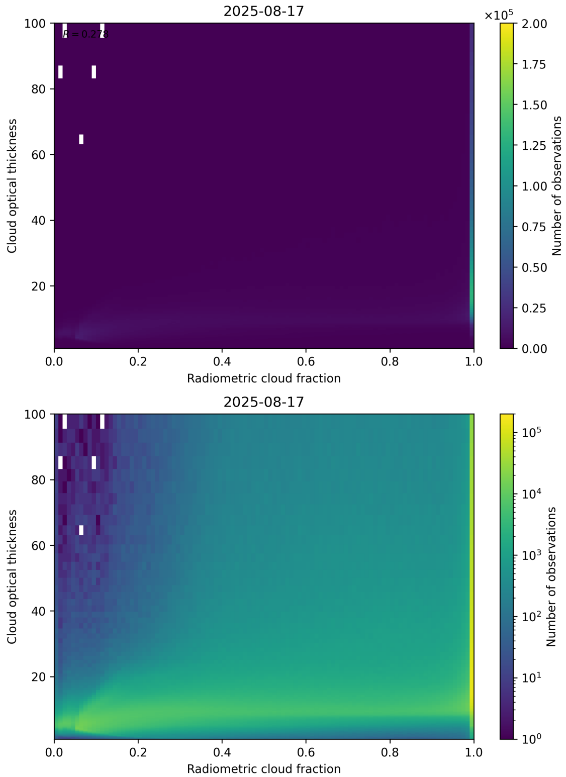
Figure 75: Scatter density plot of “Radiometric cloud fraction” against “Cloud optical thickness” for 2025-08-16 to 2025-08-18.
