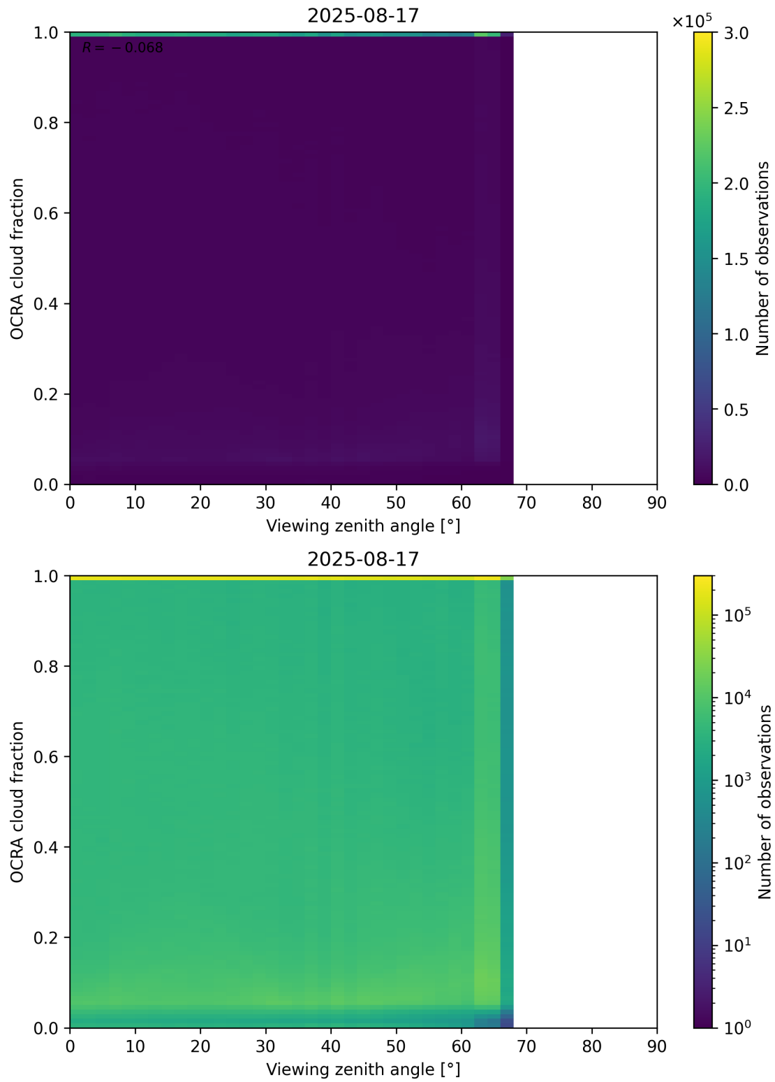
Figure 108: Scatter density plot of “Viewing zenith angle” against “OCRA cloud fraction” for 2025-08-16 to 2025-08-18.
