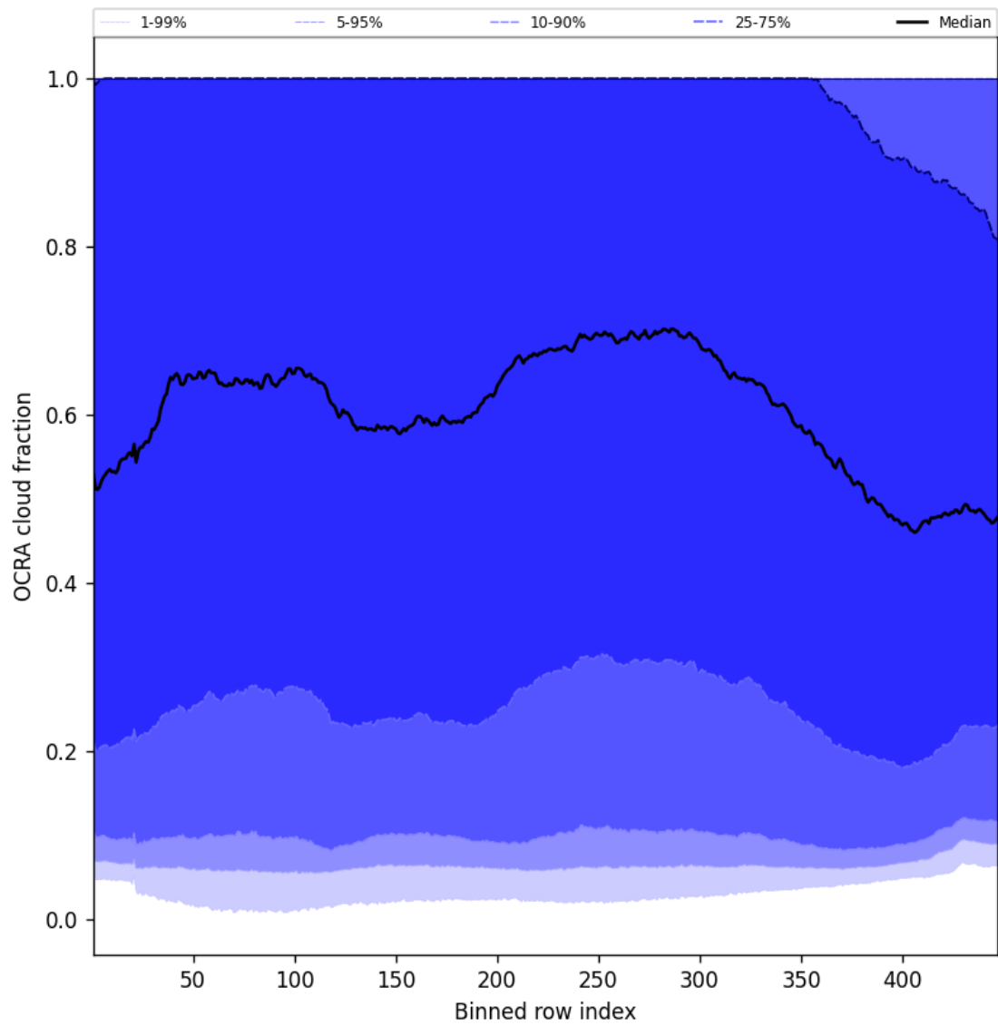
Figure 66: Along track statistics of “OCRA cloud fraction” for 2025-08-16 to 2025-08-18
