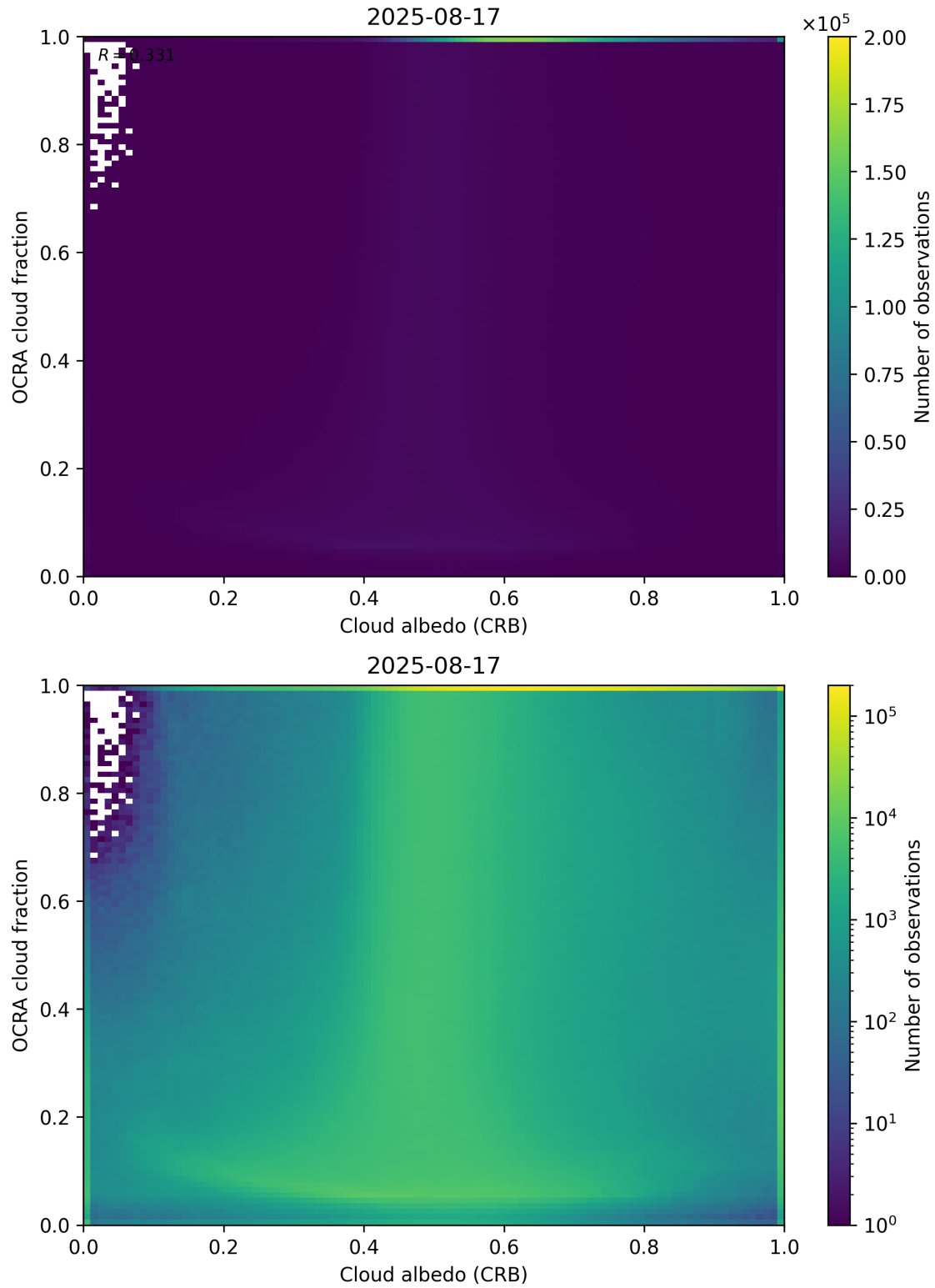
Figure 70: Scatter density plot of “Cloud albedo (CRB)” against “OCRA cloud fraction” for 2025-08-16 to 2025-08-18.
