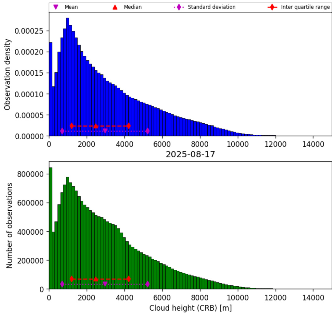
Figure 43: Histogram of “Cloud height (CRB)” for 2025-08-16 to 2025-08-18
