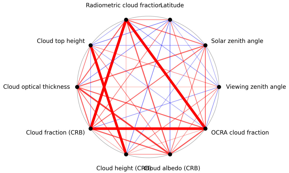
Figure 1: Map of correlation graph for 2025-08-16 to 2025-08-18.
