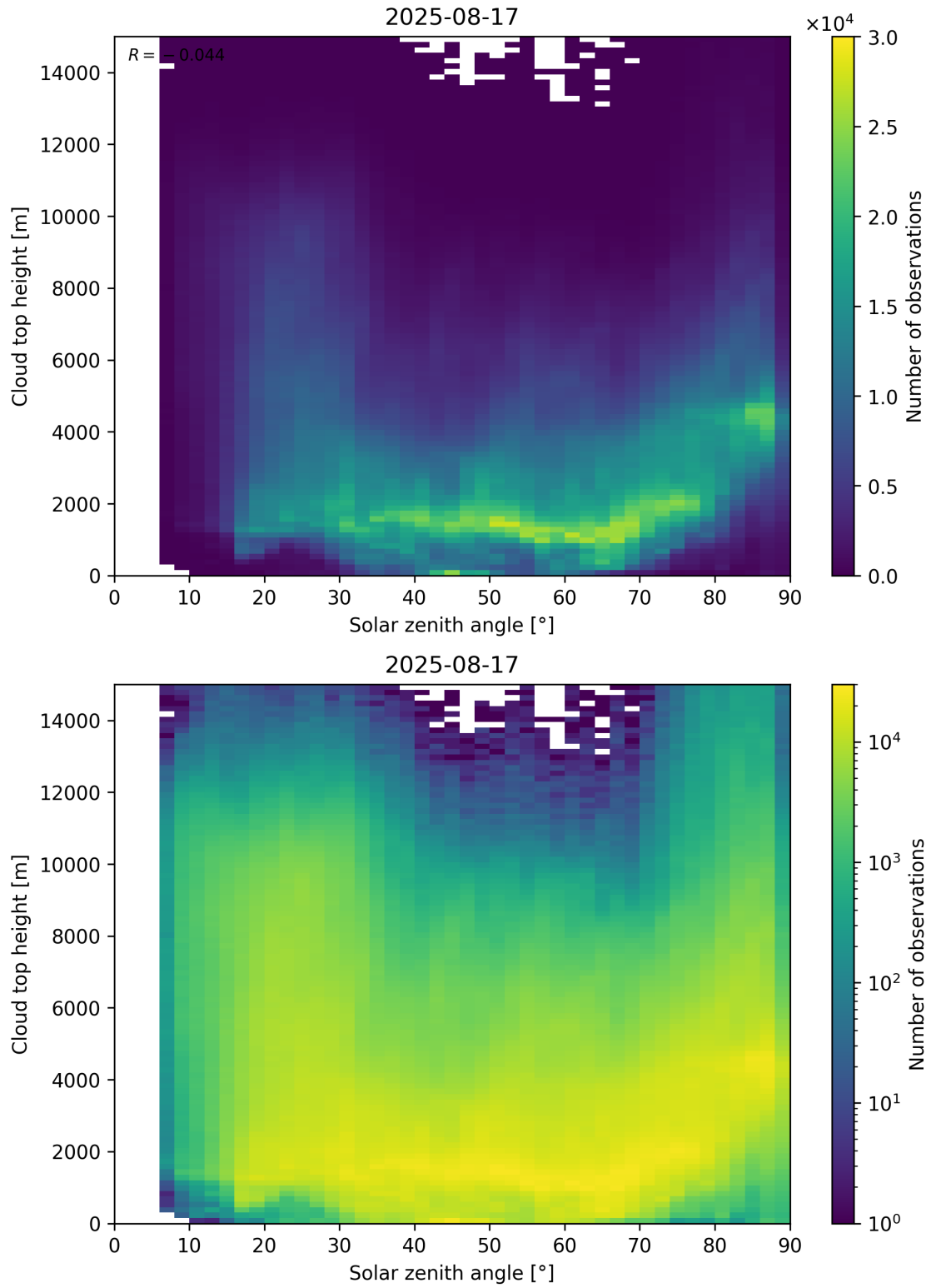
Figure 104: Scatter density plot of “Solar zenith angle” against “Cloud top height” for 2025-08-16 to 2025-08-18.
