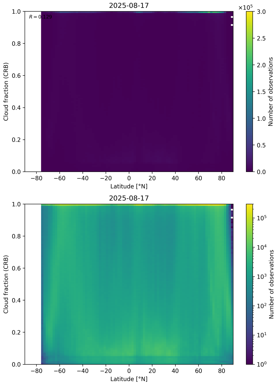
Figure 94: Scatter density plot of “Latitude” against “Cloud fraction (CRB)” for 2025-08-16 to 2025-08-18.
