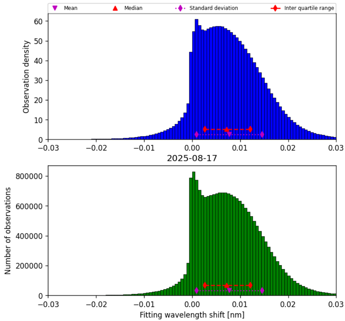
Figure 49: Histogram of “Fitting wavelength shift” for 2025-08-16 to 2025-08-18
