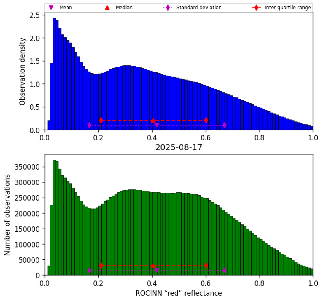
Figure 53: Histogram of “ROCINN “red” reflectance” for 2025-08-16 to 2025-08-18
