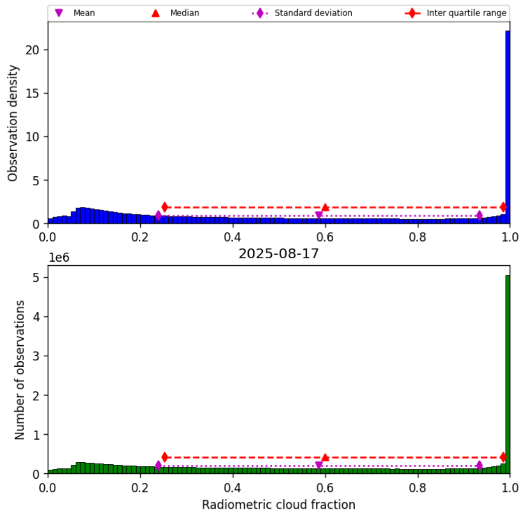
Figure 39: Histogram of “Radiometric cloud fraction” for 2025-08-16 to 2025-08-18
