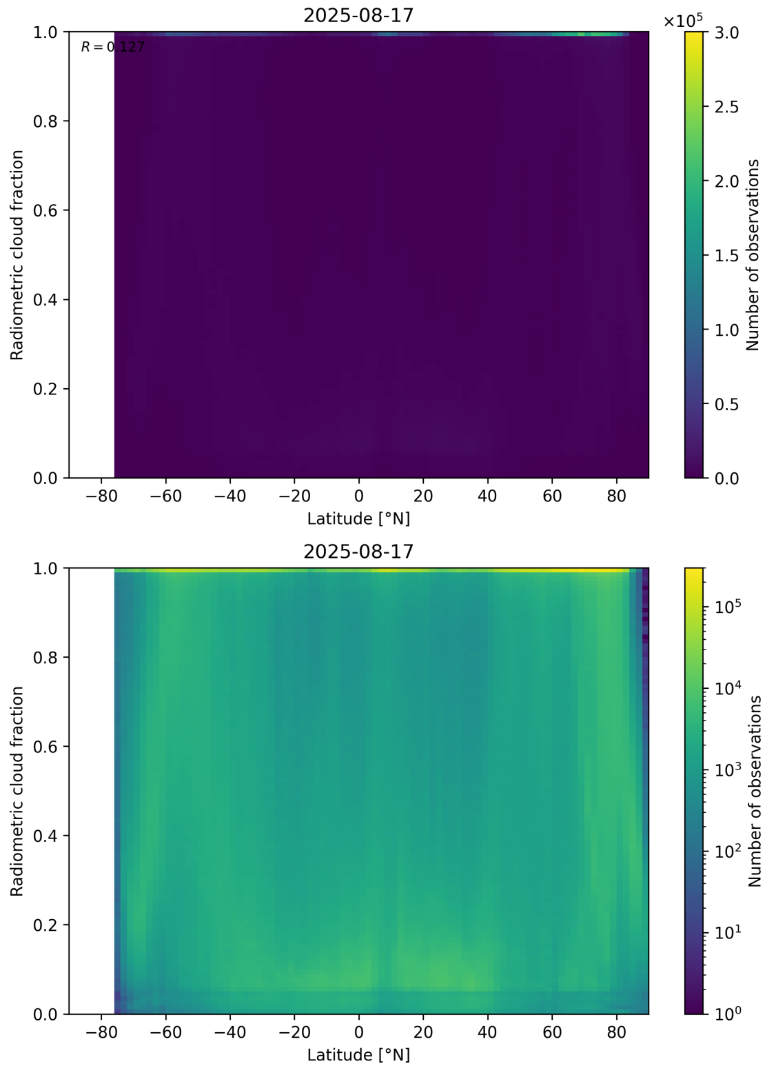
Figure 92: Scatter density plot of “Latitude” against “Radiometric cloud fraction” for 2025-08-16 to 2025-08-18.
