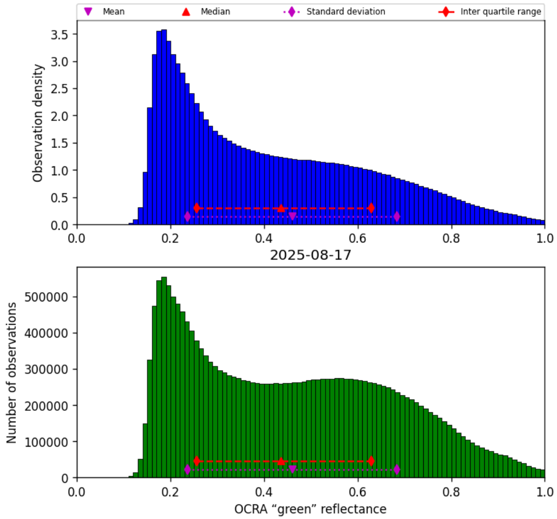
Figure 52: Histogram of “OCRA “green” reflectance” for 2025-08-16 to 2025-08-18
