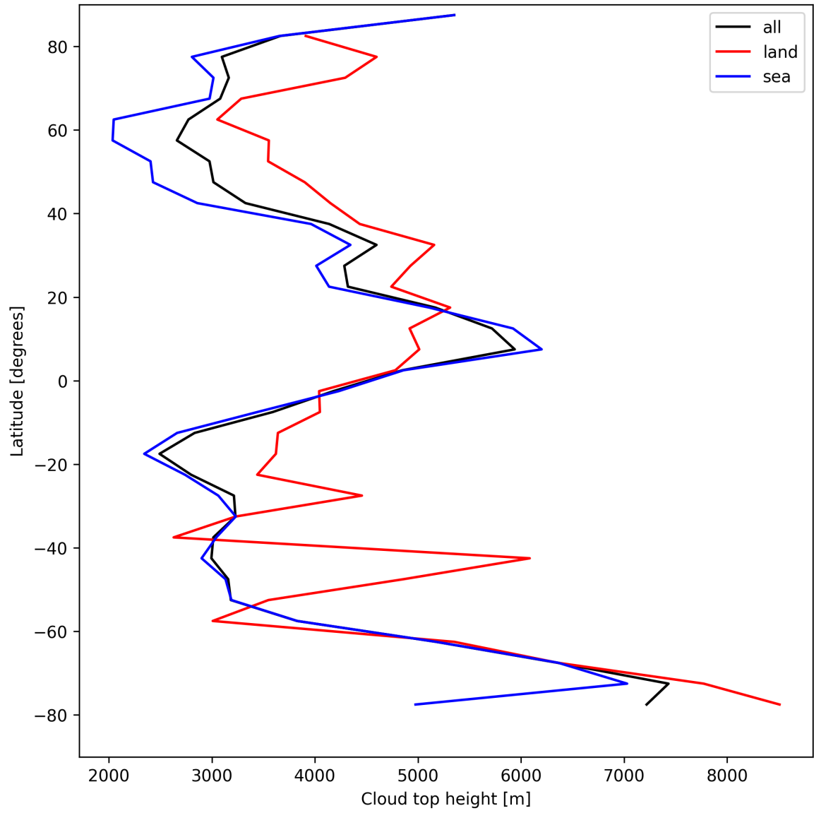
Figure 24: Zonal average of “Cloud top height” for 2025-08-16 to 2025-08-18.
