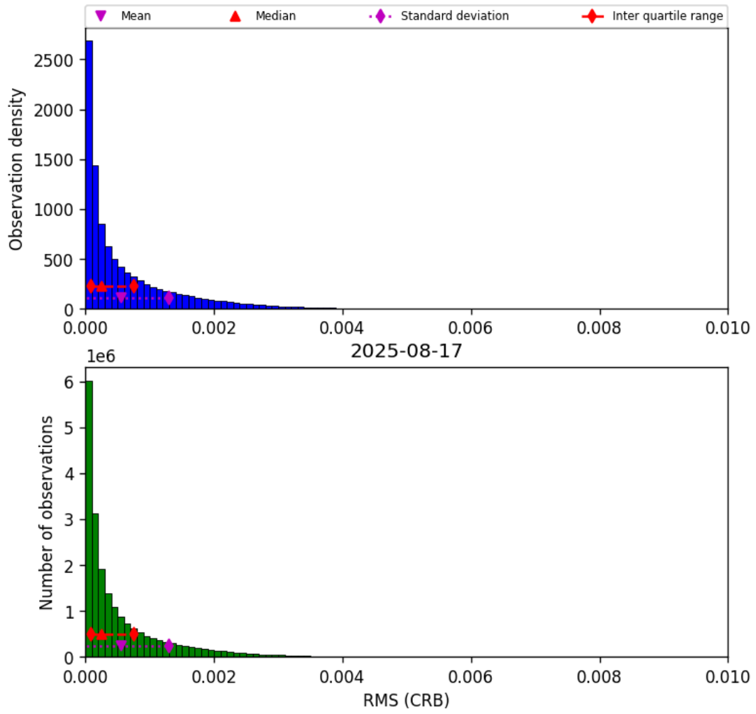
Figure 48: Histogram of “RMS (CRB)” for 2025-08-16 to 2025-08-18
