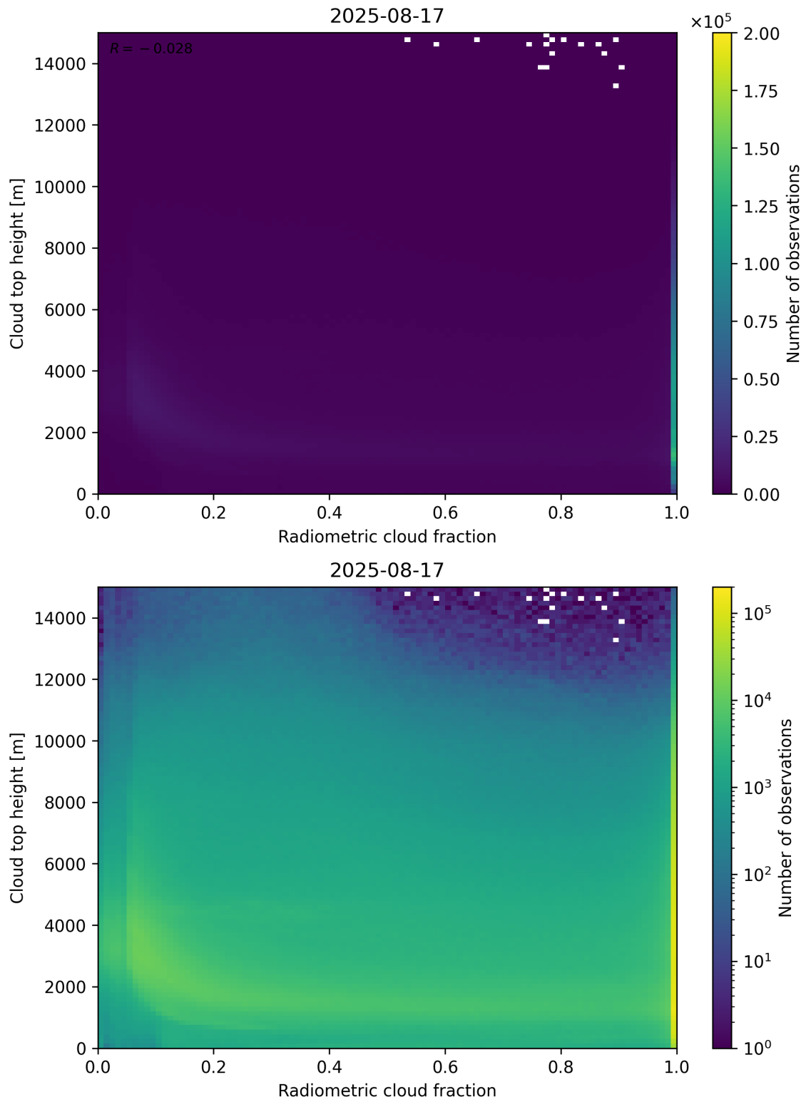
Figure 76: Scatter density plot of “Radiometric cloud fraction” against “Cloud top height” for 2025-08-16 to 2025-08-18.
