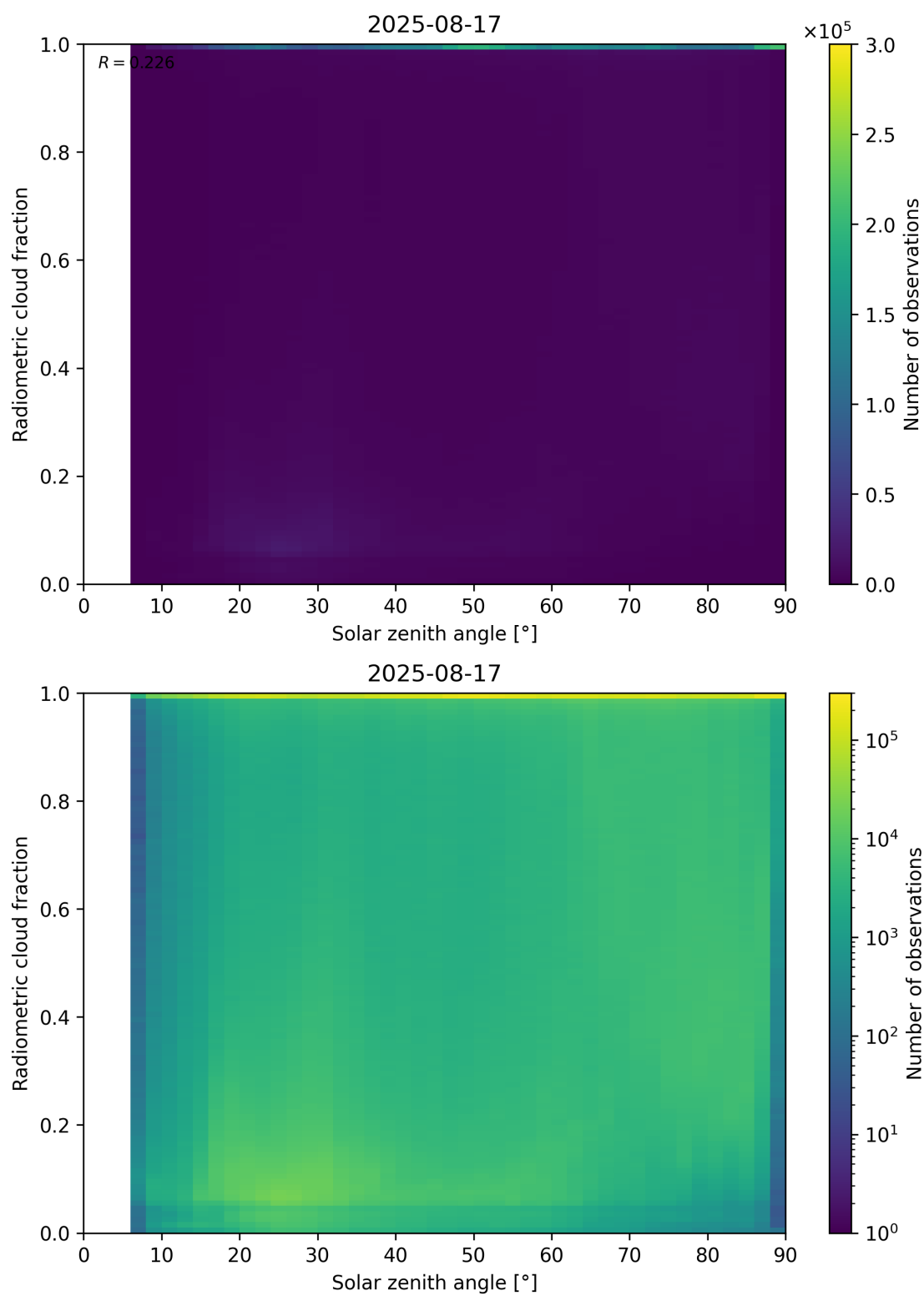
Figure 99: Scatter density plot of “Solar zenith angle” against “Radiometric cloud fraction” for 2025-08-16 to 2025-08-18.
