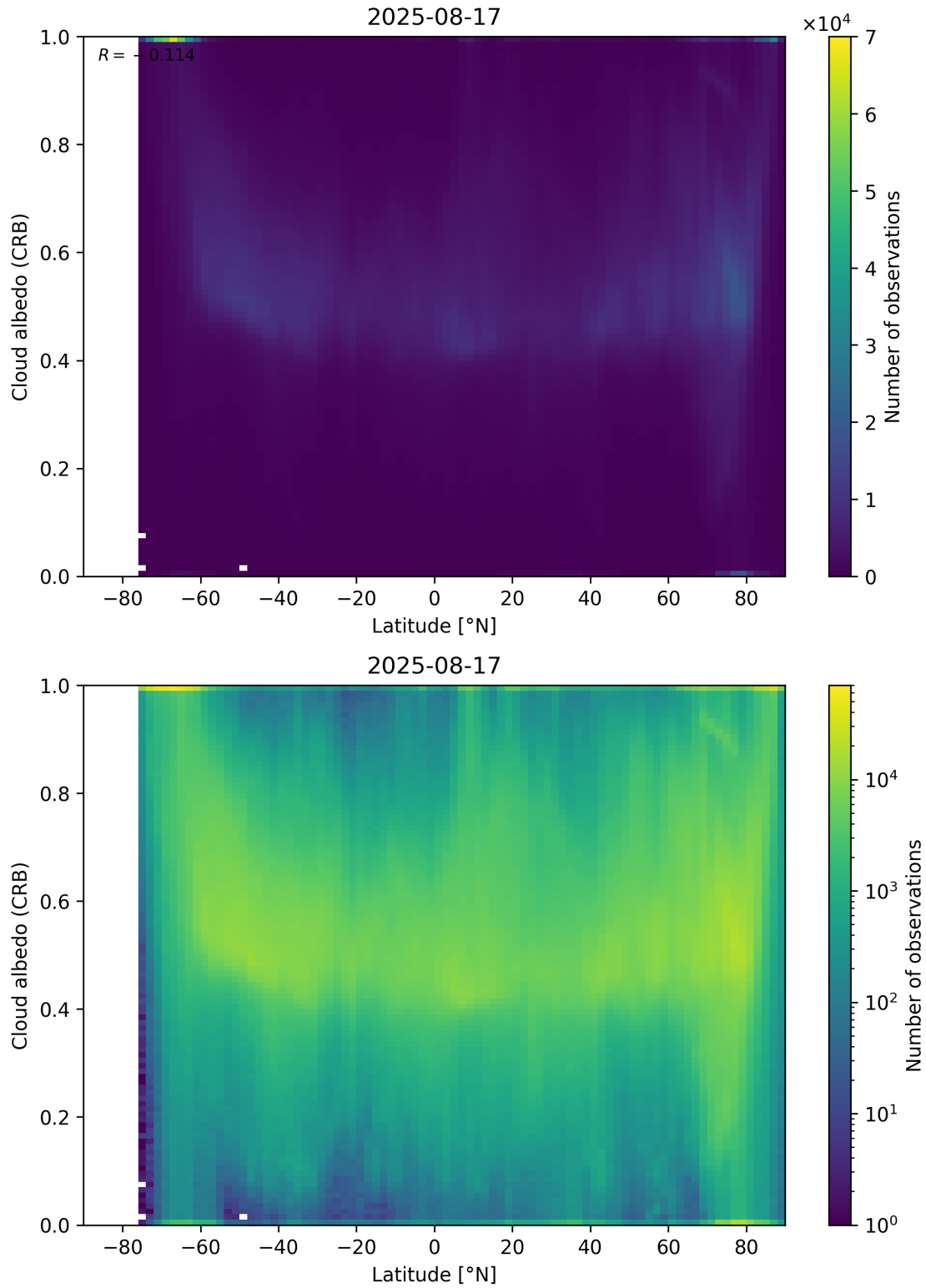
Figure 91: Scatter density plot of “Latitude” against “Cloud albedo (CRB)” for 2025-08-16 to 2025-08-18.
