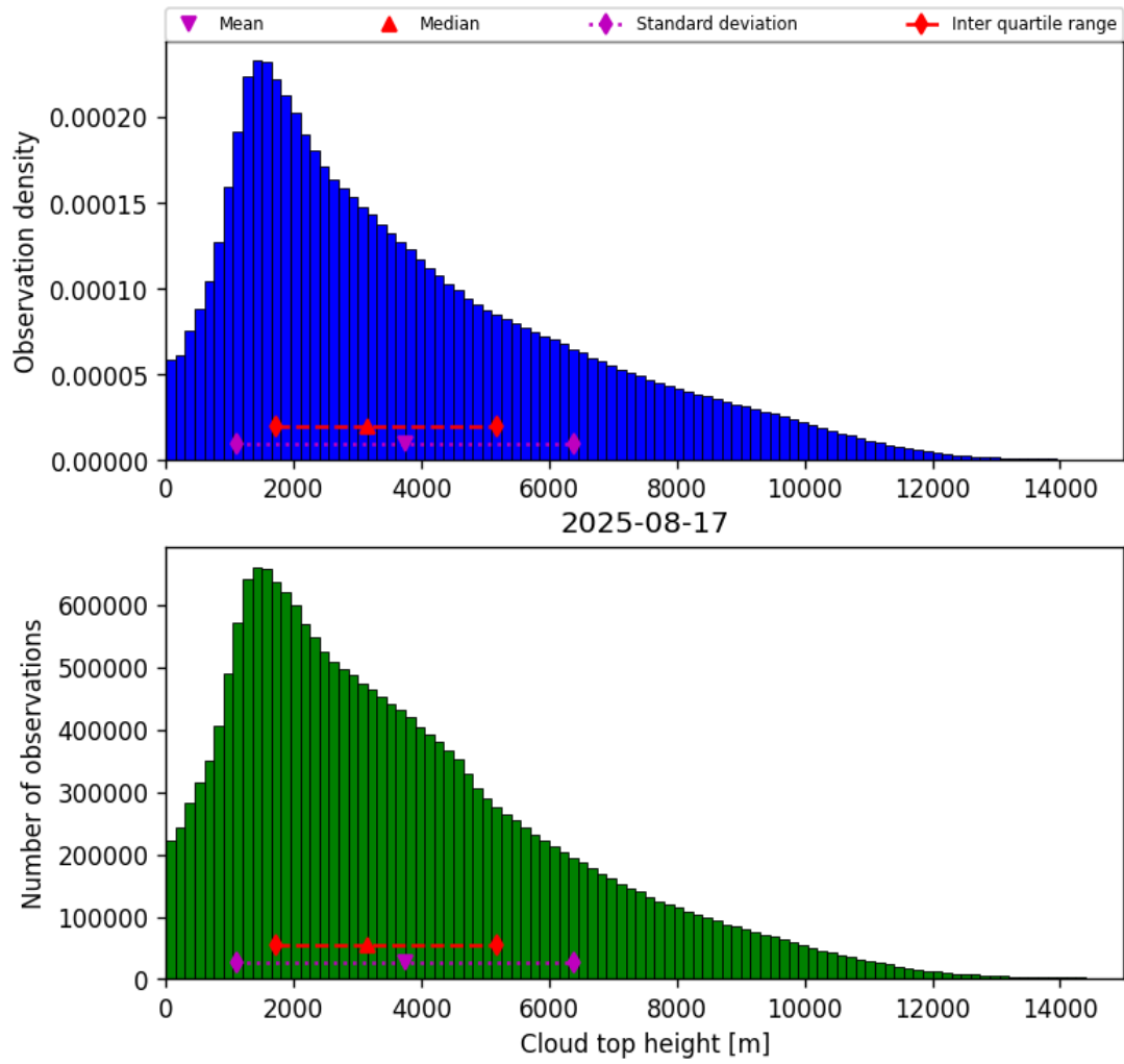
Figure 40: Histogram of “Cloud top height” for 2025-08-16 to 2025-08-18
