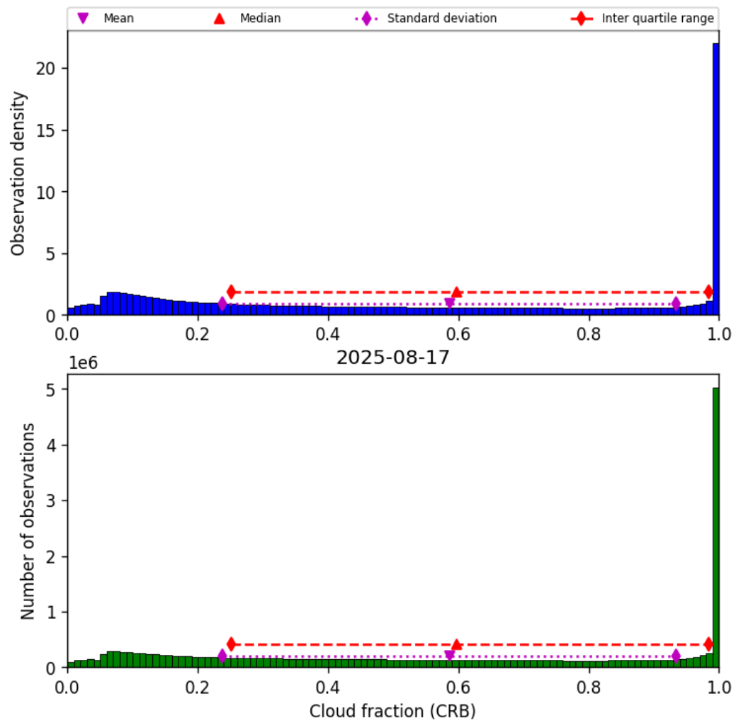
Figure 42: Histogram of “Cloud fraction (CRB)” for 2025-08-16 to 2025-08-18
