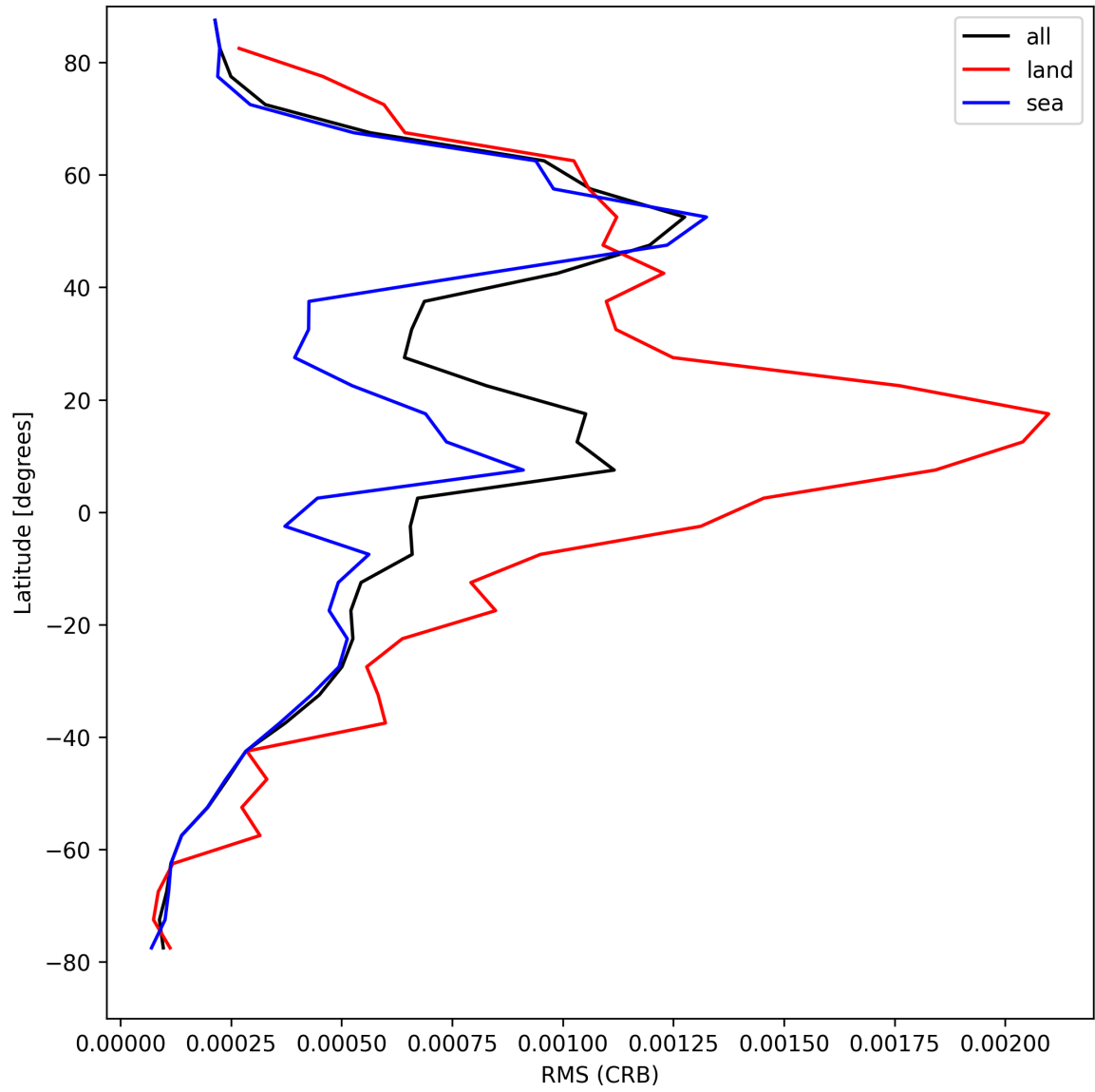
Figure 32: Zonal average of “RMS (CRB)” for 2025-08-16 to 2025-08-18.
