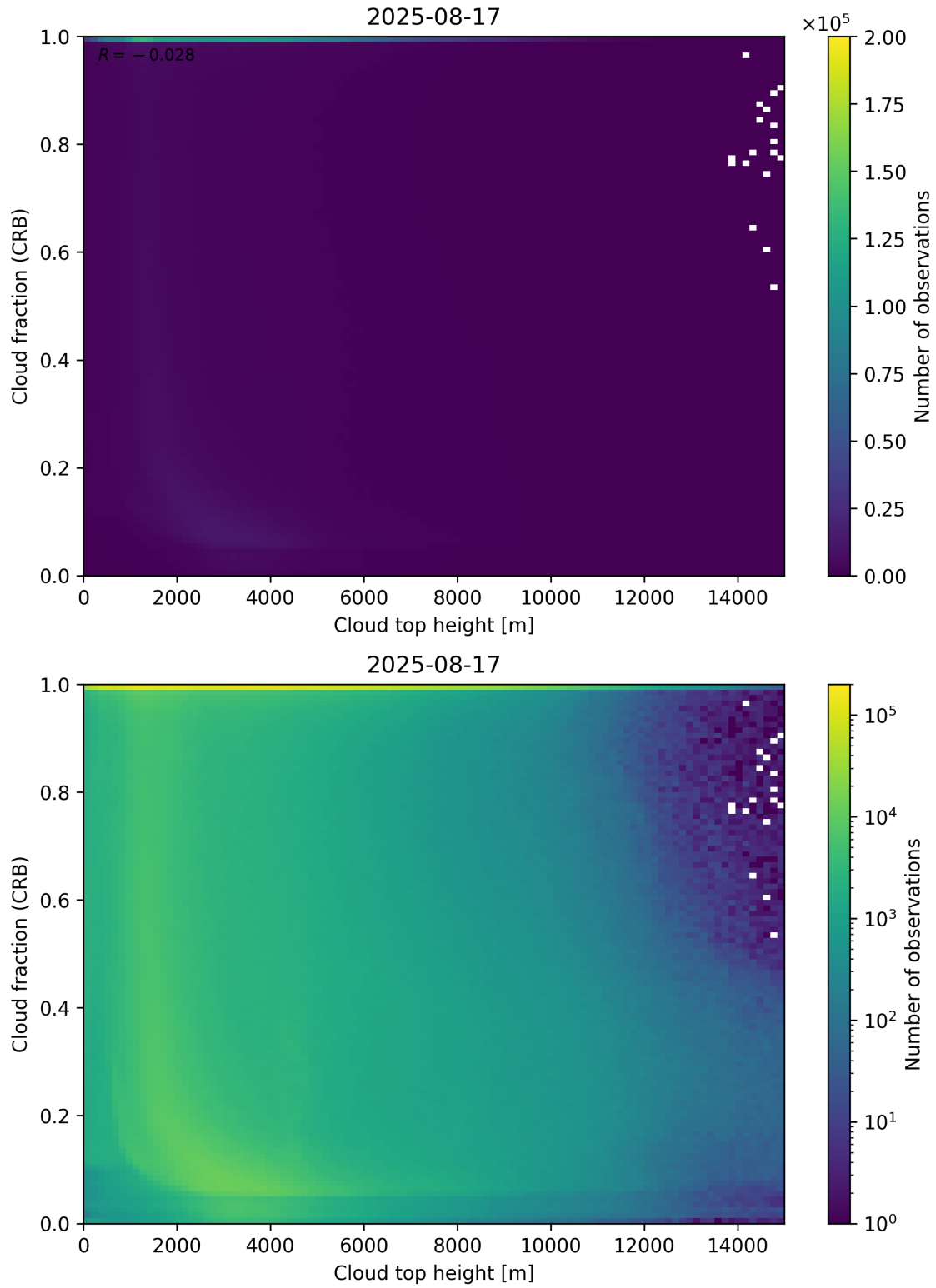
Figure 88: Scatter density plot of “Cloud top height” against “Cloud fraction (CRB)” for 2025-08-16 to 2025-08-18.
