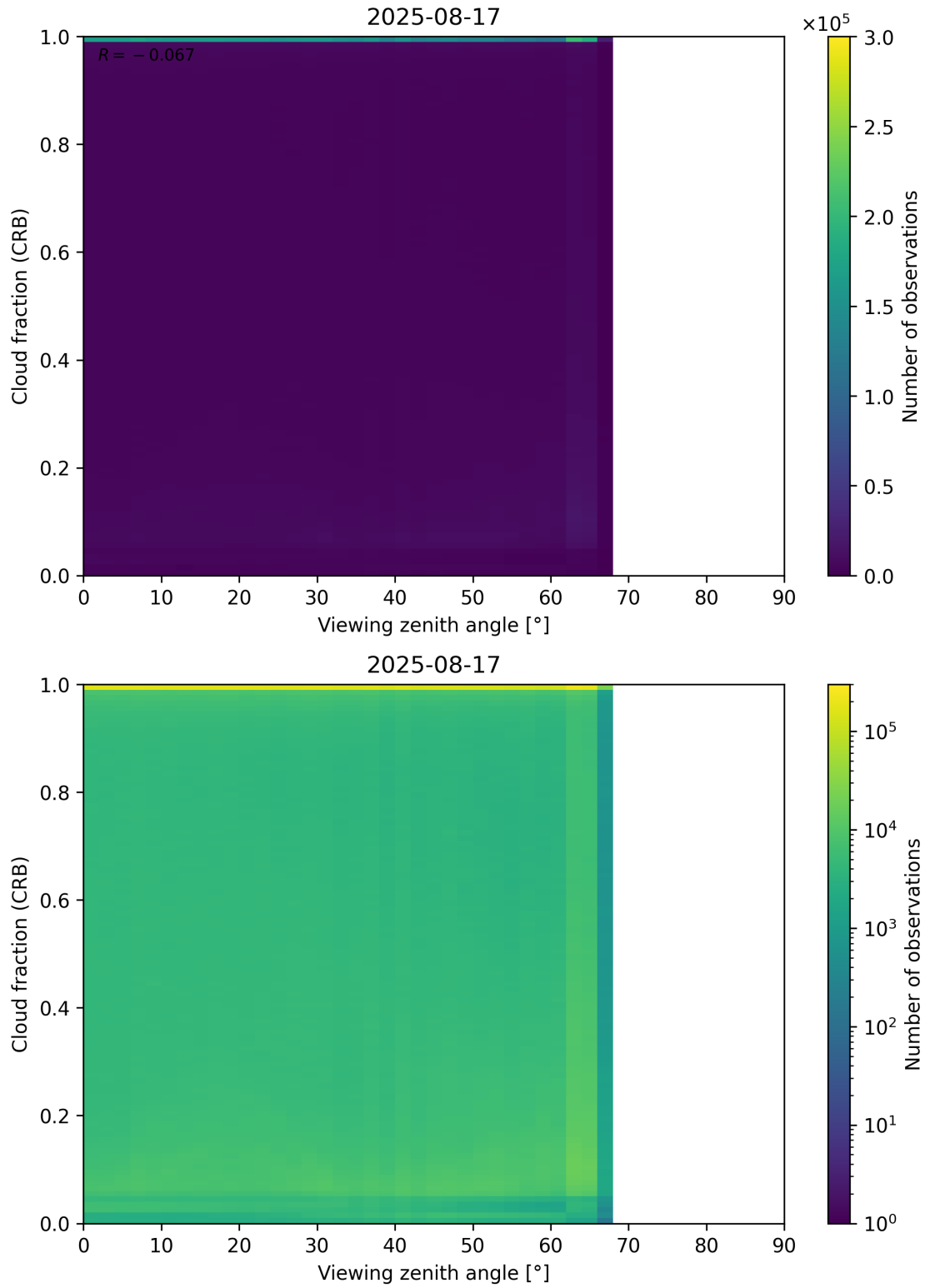
Figure 109: Scatter density plot of “Viewing zenith angle” against “Cloud fraction (CRB)” for 2025-08-16 to 2025-08-18.
