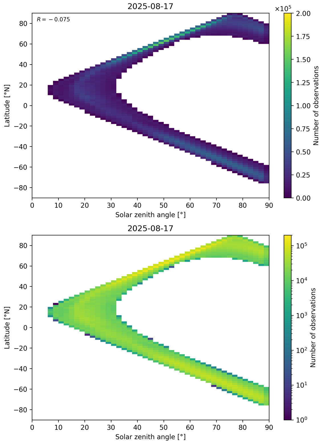
Figure 105: Scatter density plot of “Solar zenith angle” against “Latitude” for 2025-08-16 to 2025-08-18.
