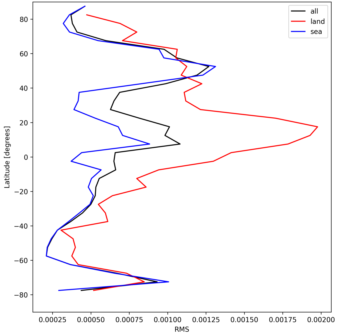
Figure 31: Zonal average of “RMS” for 2025-08-16 to 2025-08-18.
