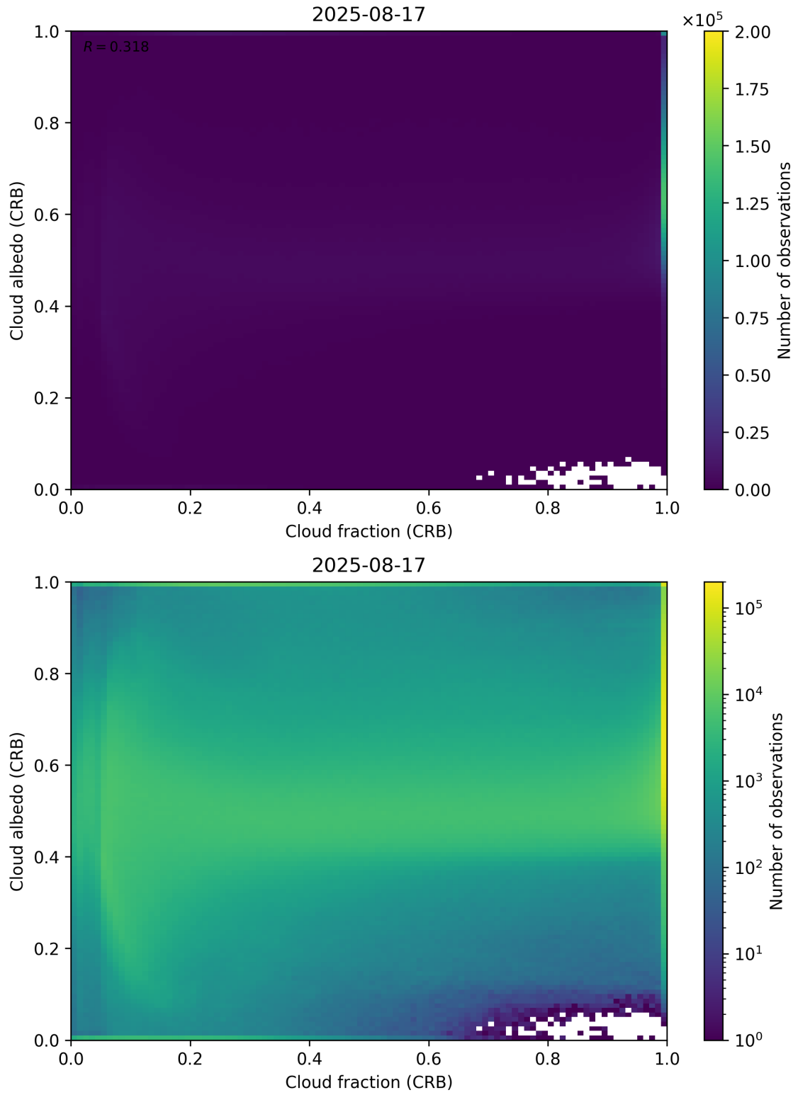
Figure 77: Scatter density plot of “Cloud fraction (CRB)” against “Cloud albedo (CRB)” for 2025-08-16 to 2025-08-18.
