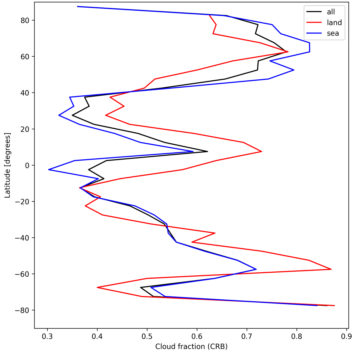
Figure 26: Zonal average of “Cloud fraction (CRB)” for 2025-08-16 to 2025-08-18.
