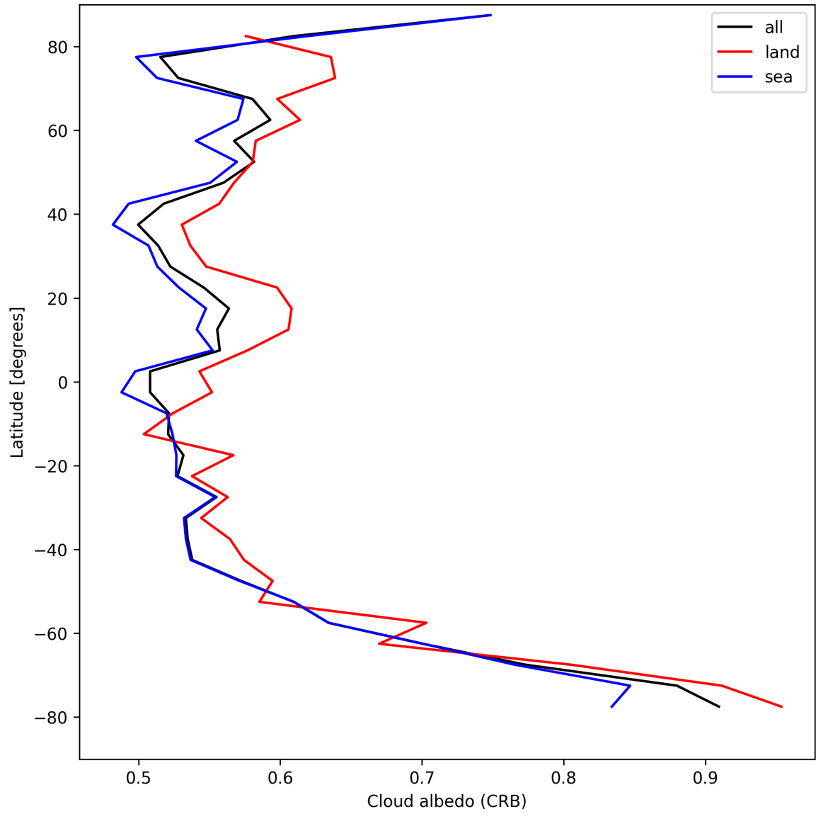
Figure 28: Zonal average of “Cloud albedo (CRB)” for 2025-08-16 to 2025-08-18.
