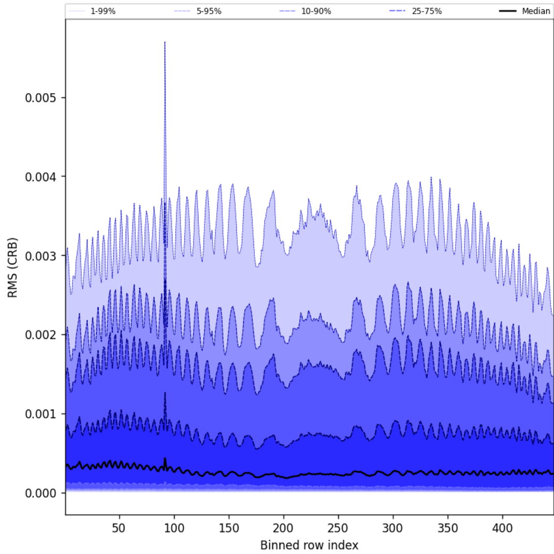
Figure 64: Along track statistics of “RMS (CRB)” for 2025-08-16 to 2025-08-18
