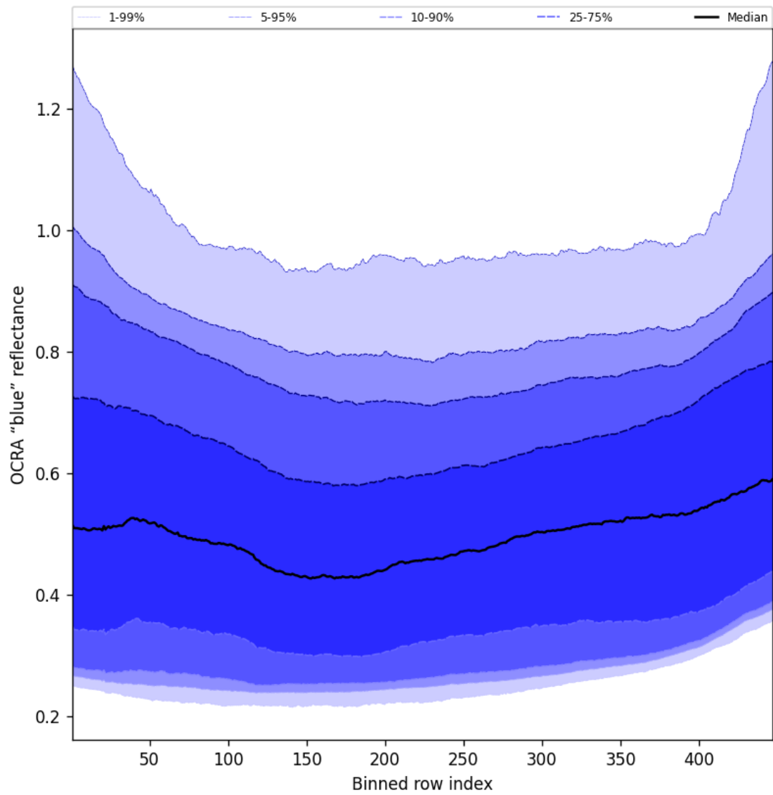
Figure 67: Along track statistics of "OCRA "blue" reflectance" for 2025-08-16 to 2025-08-18
