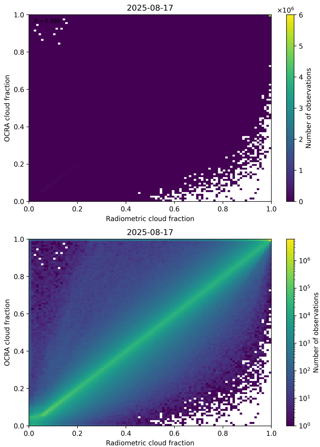
Figure 72: Scatter density plot of “Radiometric cloud fraction” against “OCRA cloud fraction” for 2025-08-16 to 2025-08-18.
