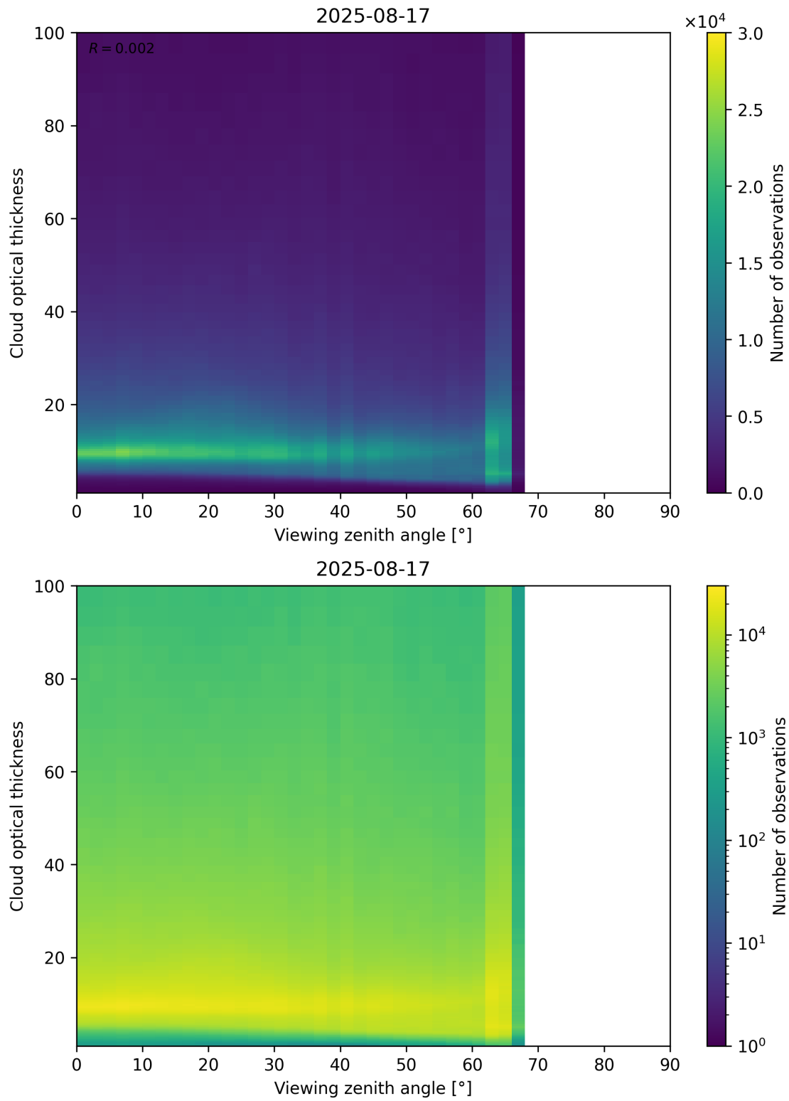
Figure 111: Scatter density plot of “Viewing zenith angle” against “Cloud optical thickness” for 2025-08-16 to 2025-08-18.
