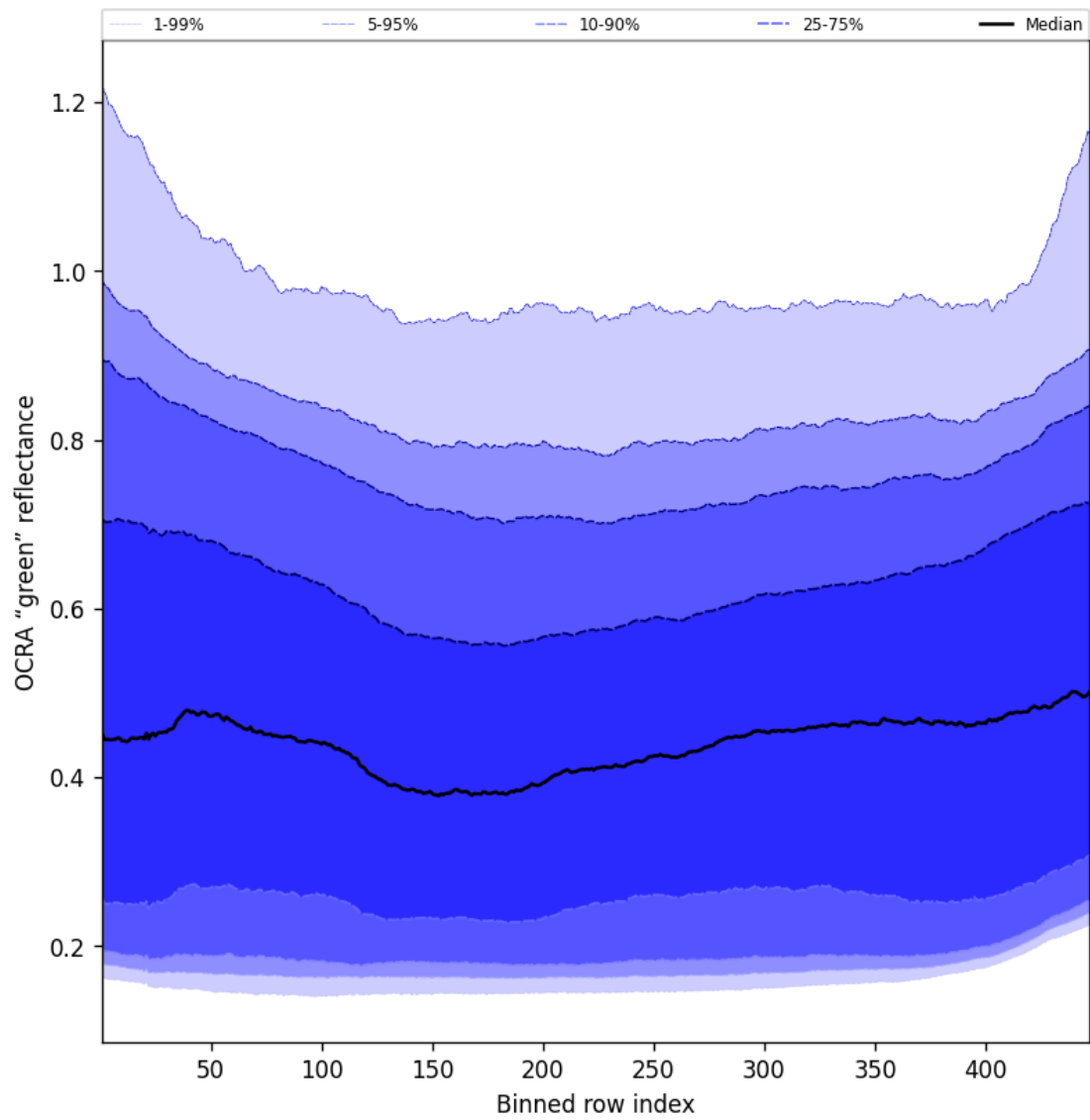
Figure 68: Along track statistics of "OCRA "green" reflectance" for 2025-08-16 to 2025-08-18
