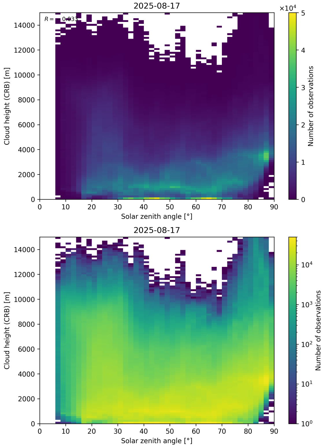
Figure 102: Scatter density plot of “Solar zenith angle” against “Cloud height (CRB)” for 2025-08-16 to 2025-08-18.
