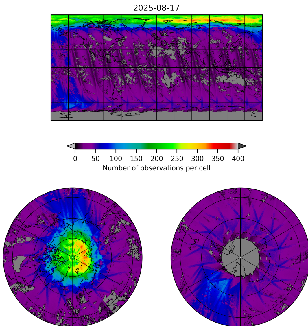
Figure 21: Map of the number of observations for 2025-08-16 to 2025-08-18
