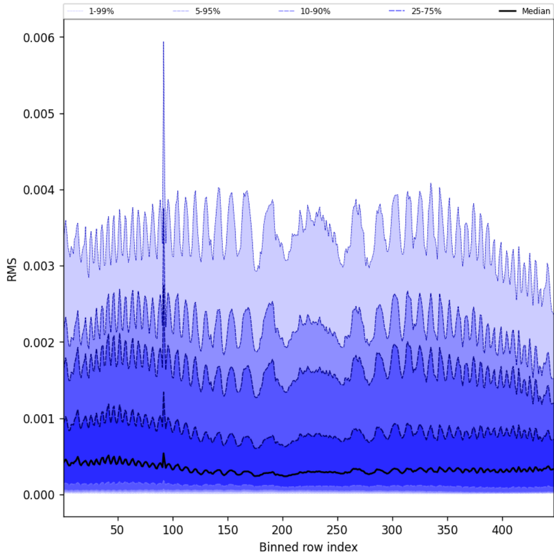
Figure 63: Along track statistics of “RMS” for 2025-08-16 to 2025-08-18
