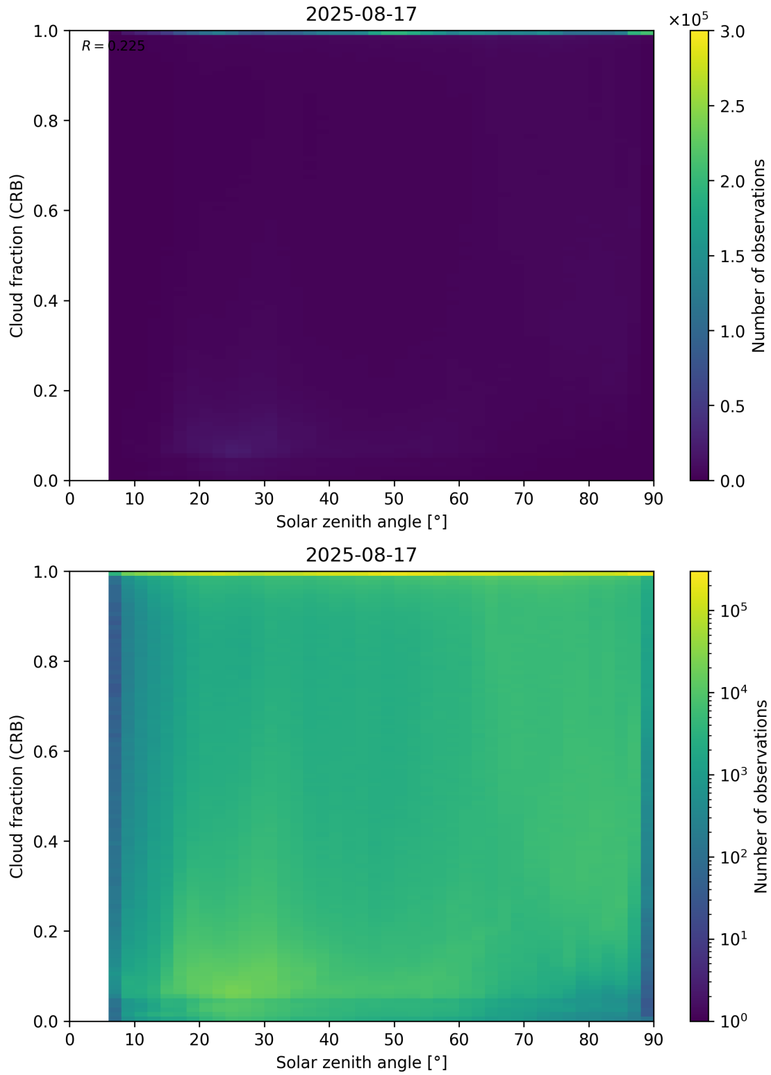
Figure 101: Scatter density plot of “Solar zenith angle” against “Cloud fraction (CRB)” for 2025-08-16 to 2025-08-18.
