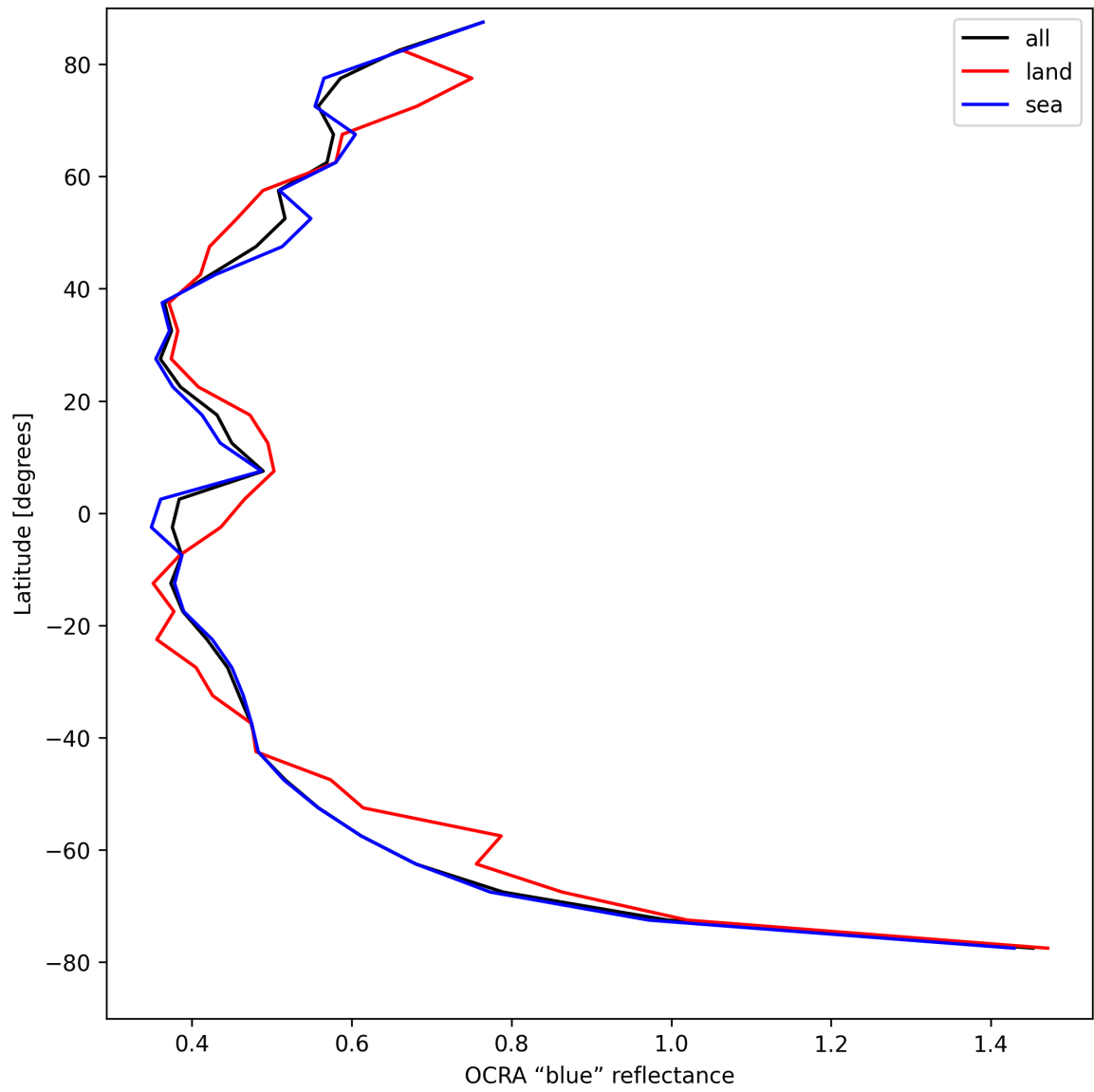
Figure 35: Zonal average of “OCRA “blue” reflectance” for 2025-08-16 to 2025-08-18.
