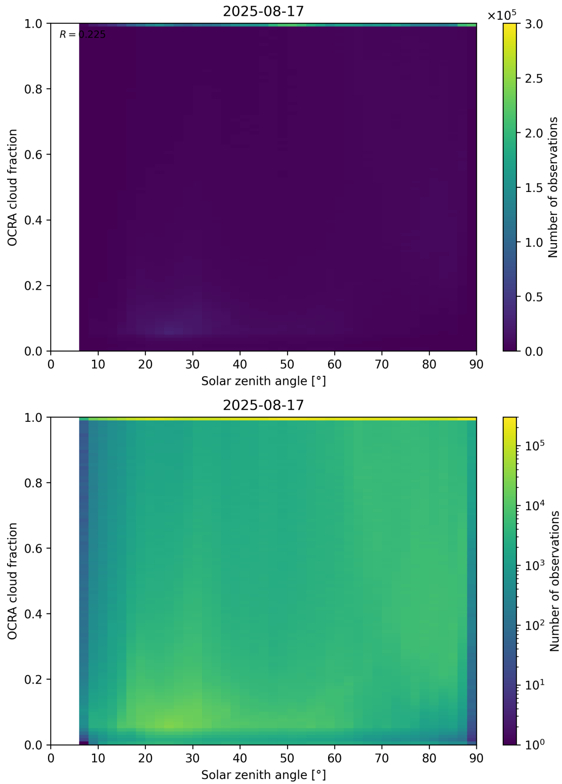
Figure 100: Scatter density plot of “Solar zenith angle” against “OCRA cloud fraction” for 2025-08-16 to 2025-08-18.
