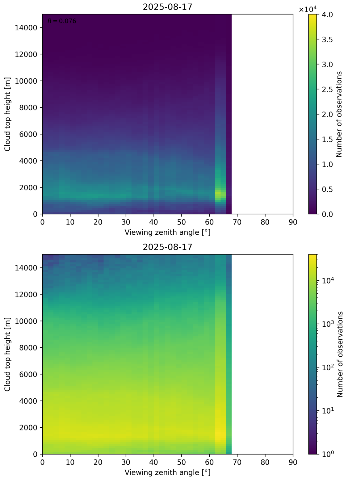
Figure 112: Scatter density plot of “Viewing zenith angle” against “Cloud top height” for 2025-08-16 to 2025-08-18.
