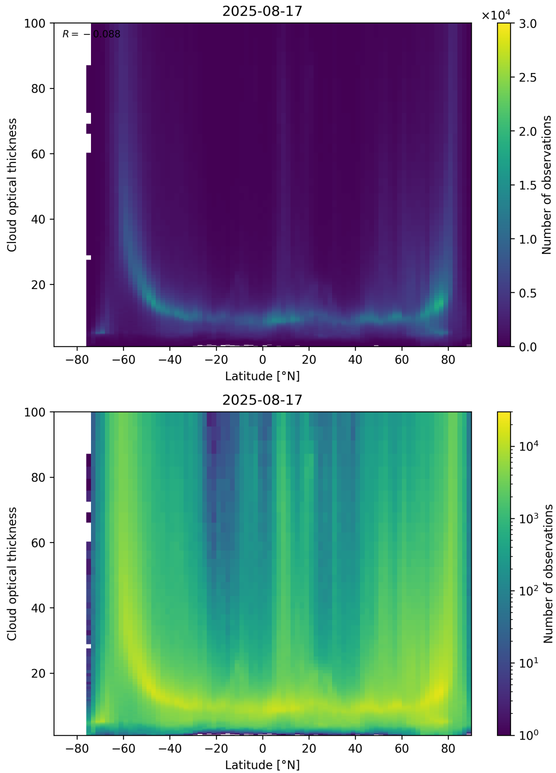
Figure 96: Scatter density plot of “Latitude” against “Cloud optical thickness” for 2025-08-16 to 2025-08-18.
