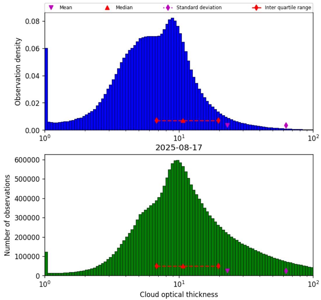
Figure 41: Histogram of “Cloud optical thickness” for 2025-08-16 to 2025-08-18
