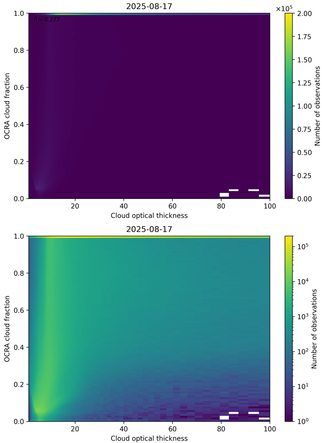
Figure 83: Scatter density plot of “Cloud optical thickness” against “OCRA cloud fraction” for 2025-08-16 to 2025-08-18.
