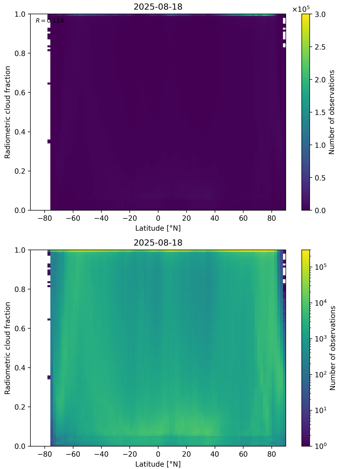
Figure 92: Scatter density plot of “Latitude” against “Radiometric cloud fraction” for 2025-08-17 to 2025-08-19.
