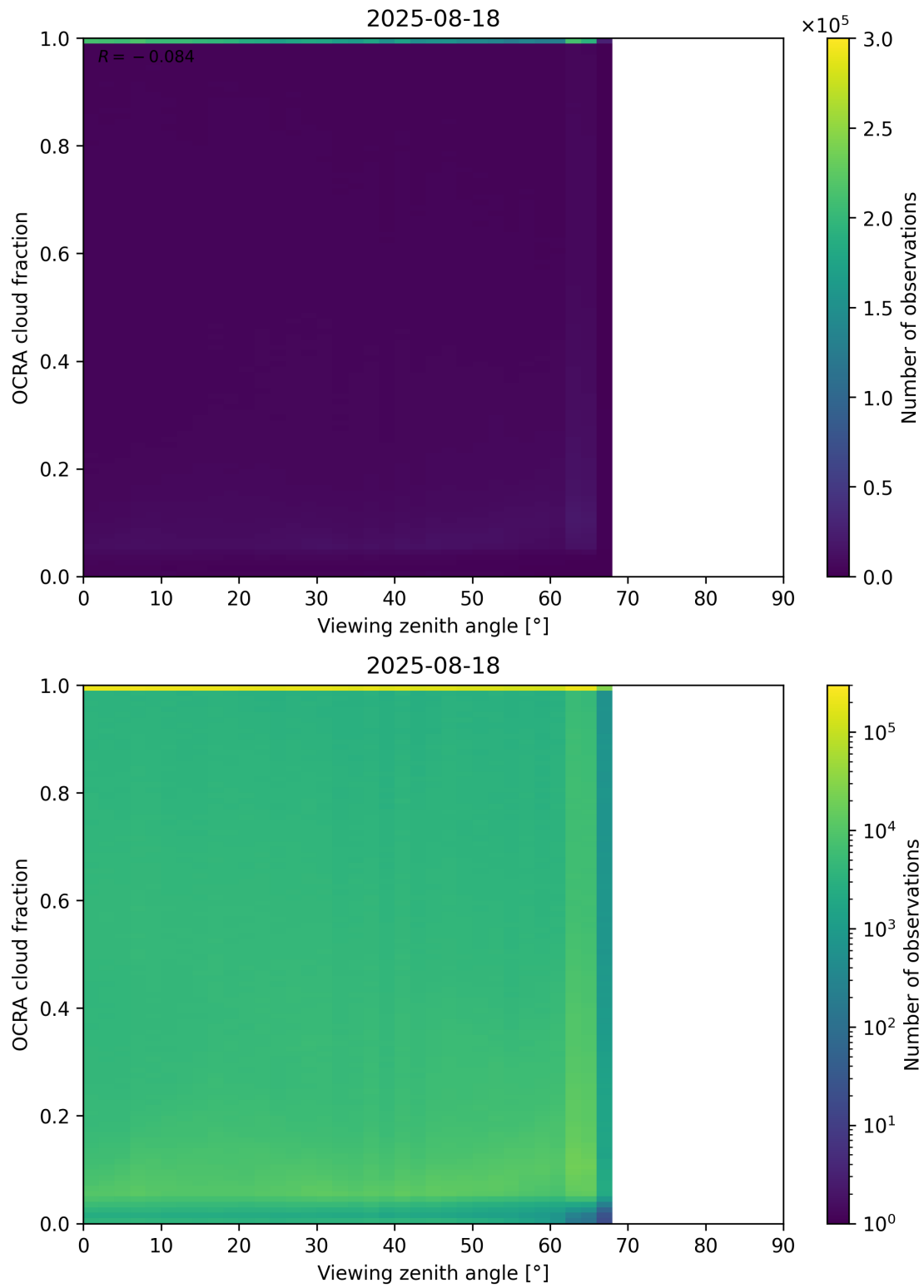
Figure 108: Scatter density plot of “Viewing zenith angle” against “OCRA cloud fraction” for 2025-08-17 to 2025-08-19.
