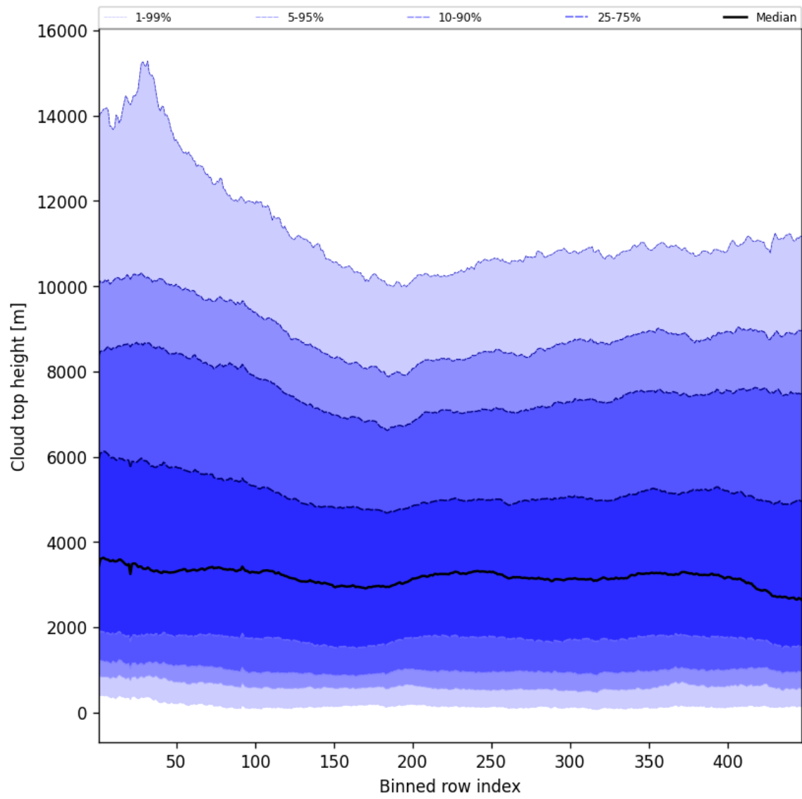
Figure 56: Along track statistics of “Cloud top height” for 2025-08-17 to 2025-08-19
