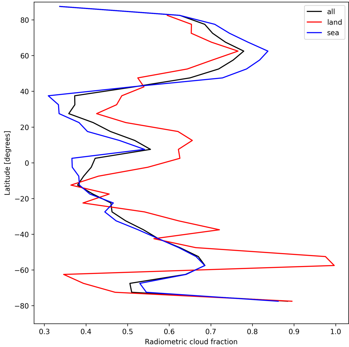
Figure 23: Zonal average of “Radiometric cloud fraction” for 2025-08-17 to 2025-08-19.
