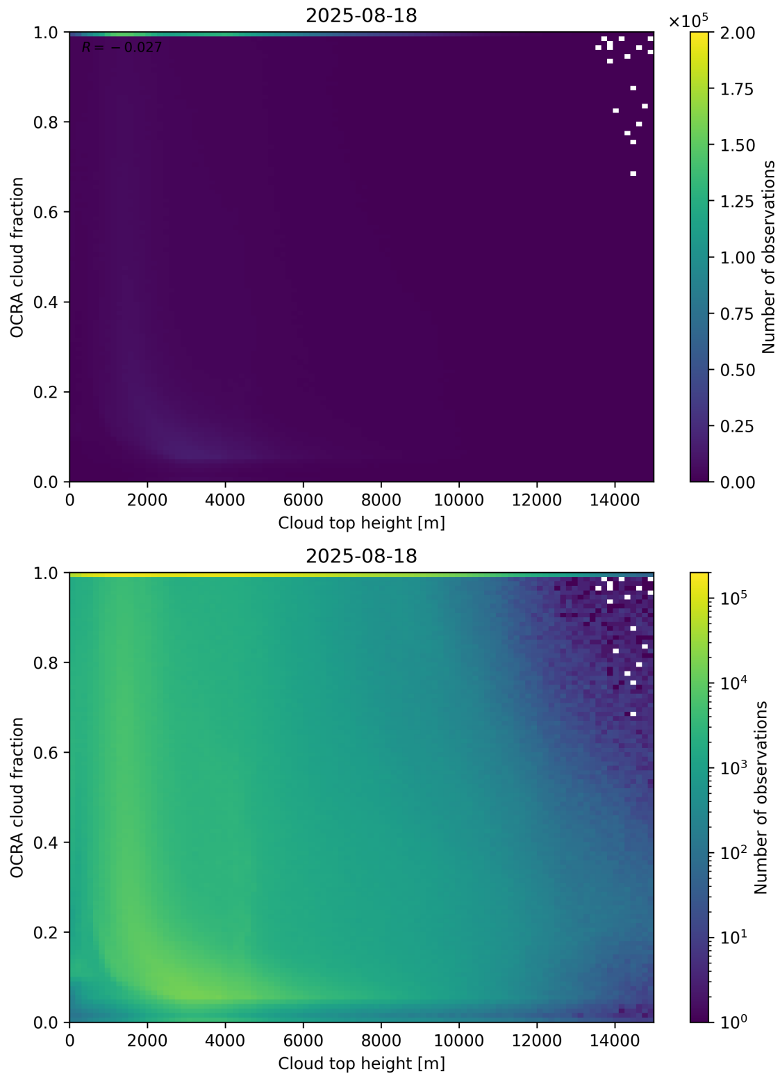
Figure 87: Scatter density plot of “Cloud top height” against “OCRA cloud fraction” for 2025-08-17 to 2025-08-19.
