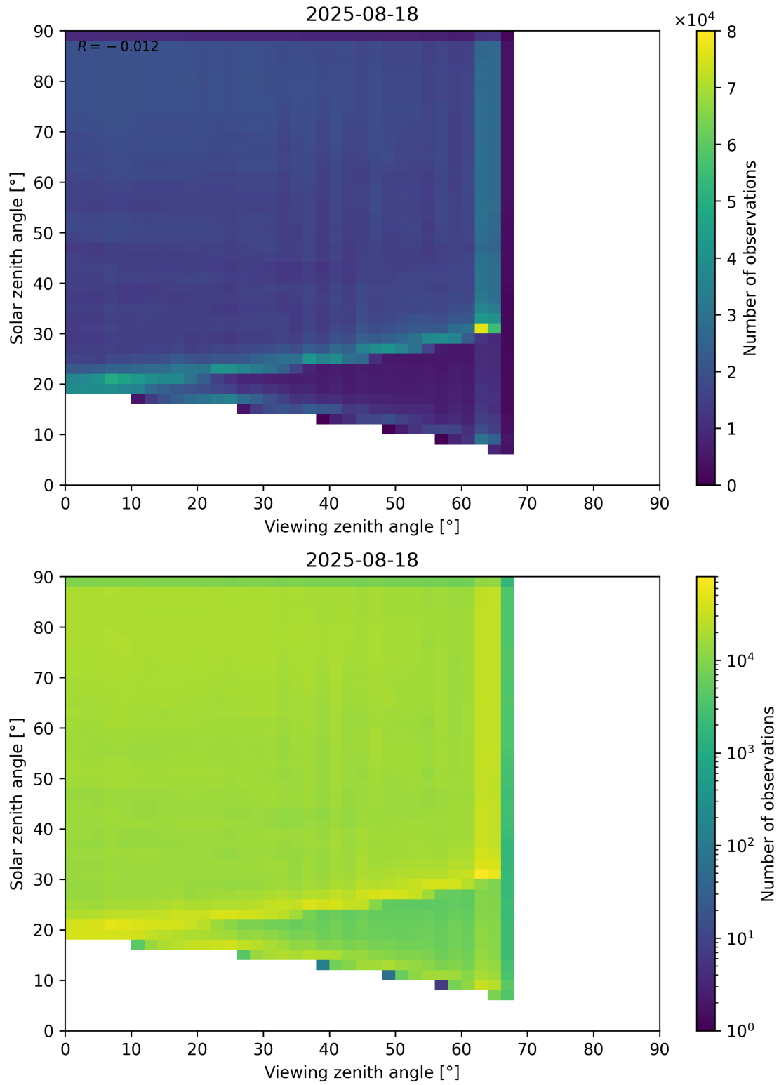
Figure 114: Scatter density plot of “Viewing zenith angle” against “Solar zenith angle” for 2025-08-17 to 2025-08-19.
