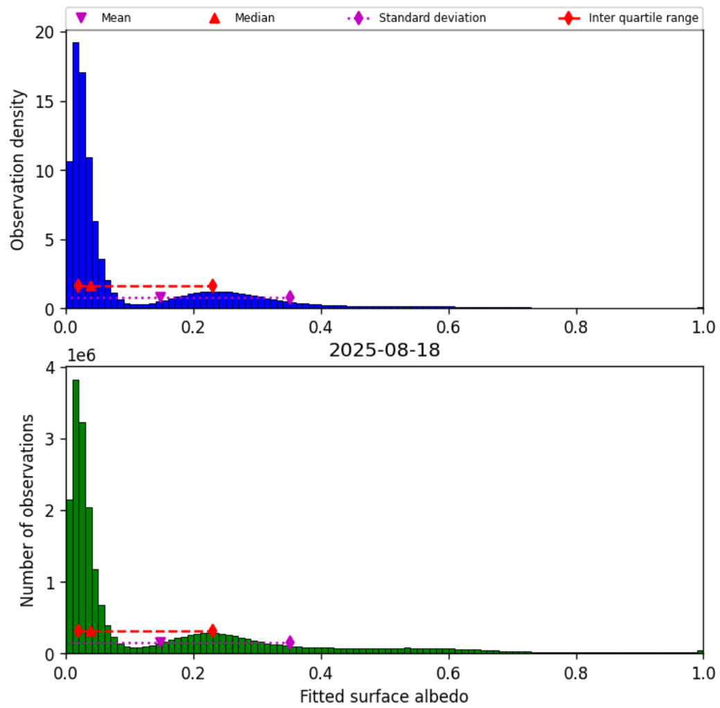
Figure 45: Histogram of “Fitted surface albedo” for 2025-08-17 to 2025-08-19
