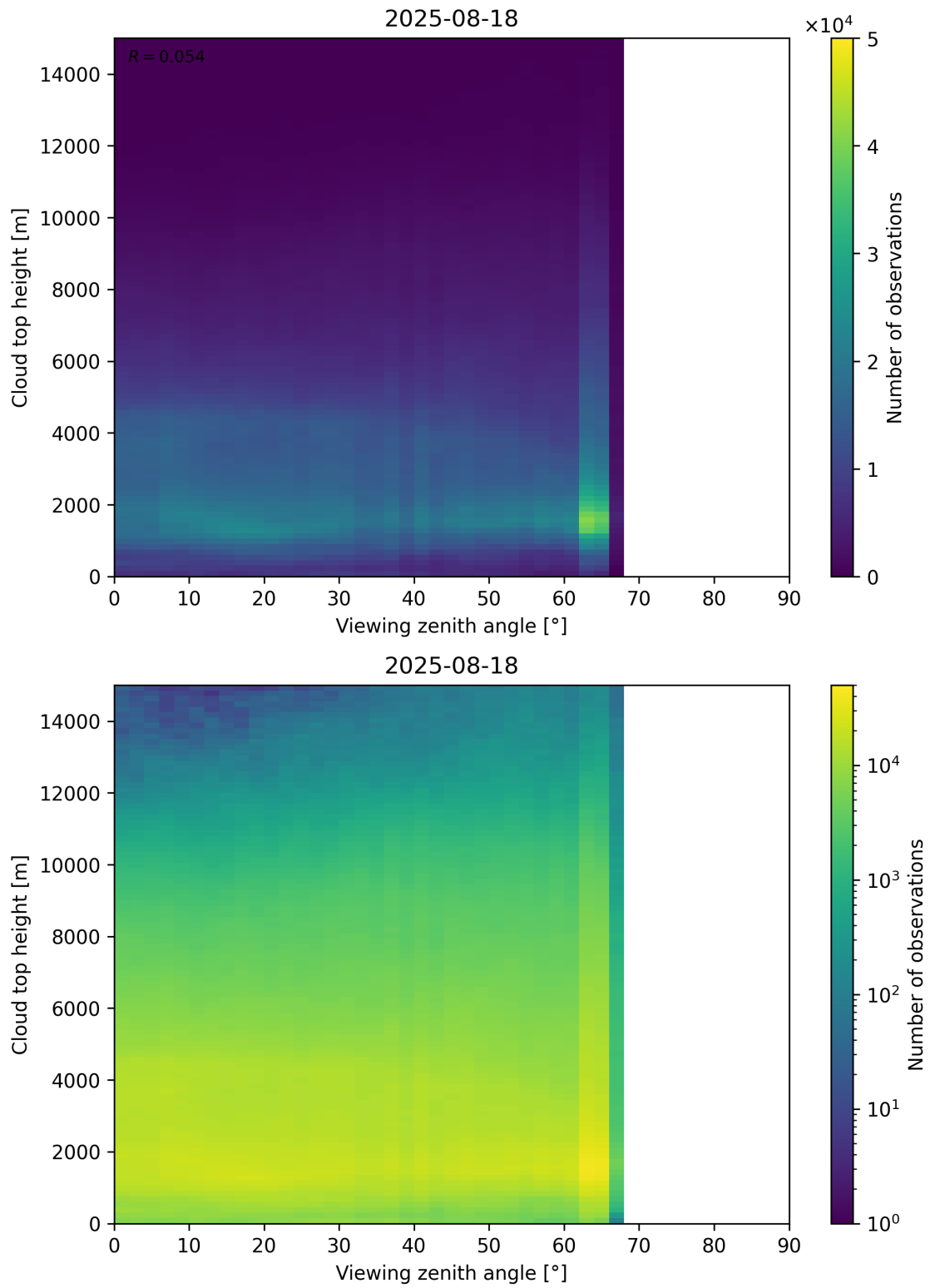
Figure 112: Scatter density plot of “Viewing zenith angle” against “Cloud top height” for 2025-08-17 to 2025-08-19.
