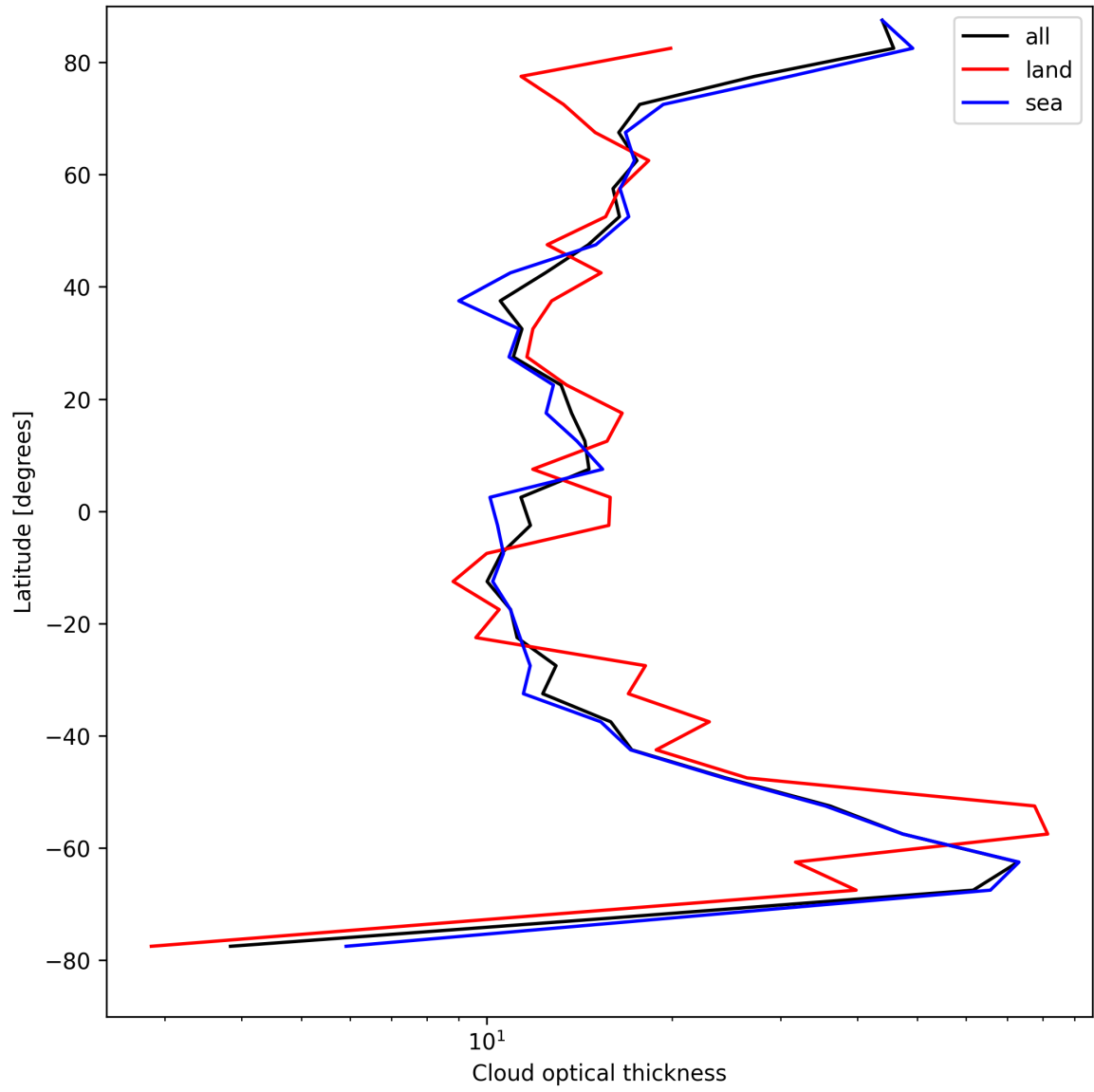
Figure 25: Zonal average of “Cloud optical thickness” for 2025-08-17 to 2025-08-19.
