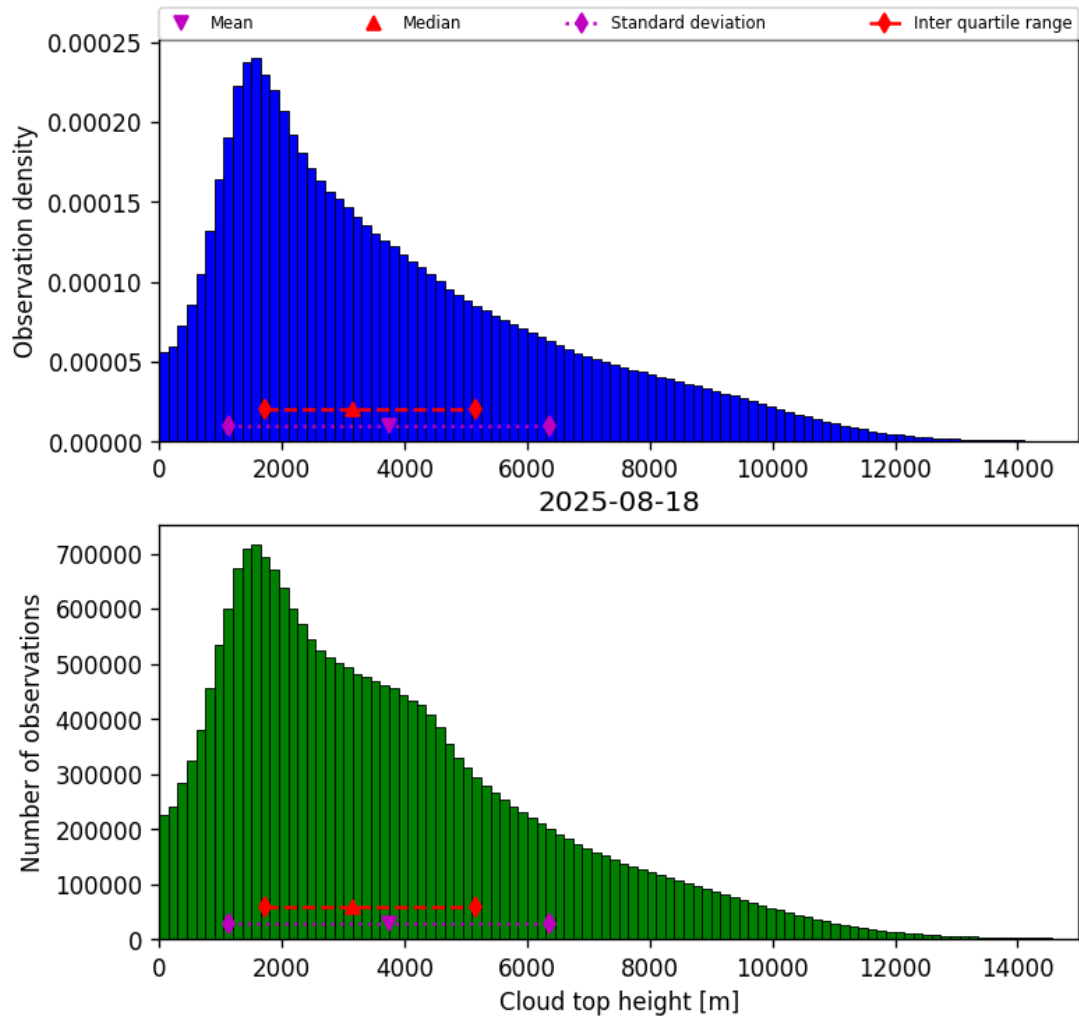
Figure 40: Histogram of “Cloud top height” for 2025-08-17 to 2025-08-19
