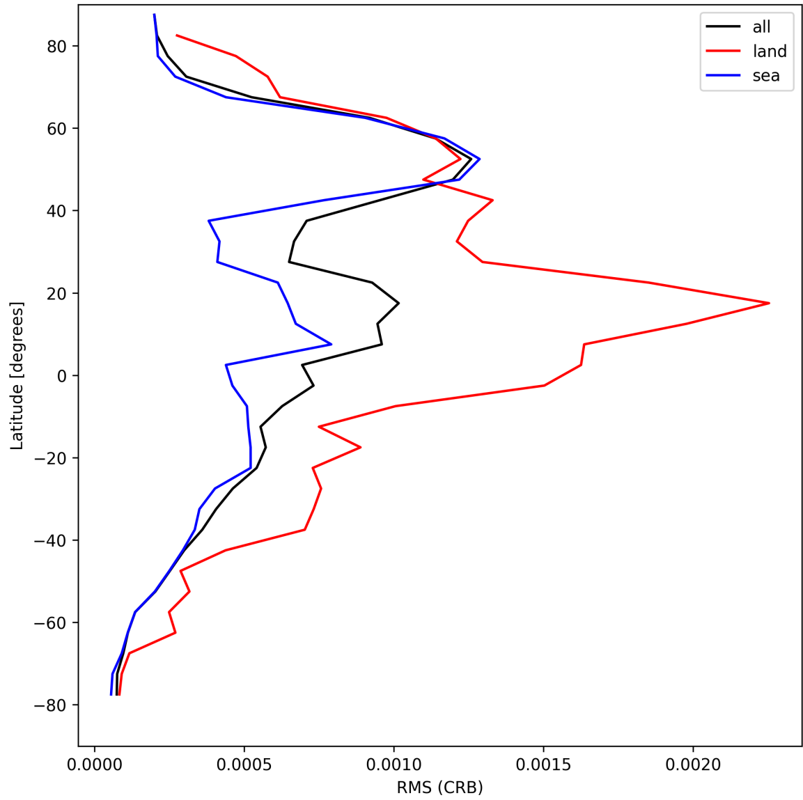
Figure 32: Zonal average of “RMS (CRB)” for 2025-08-17 to 2025-08-19.
