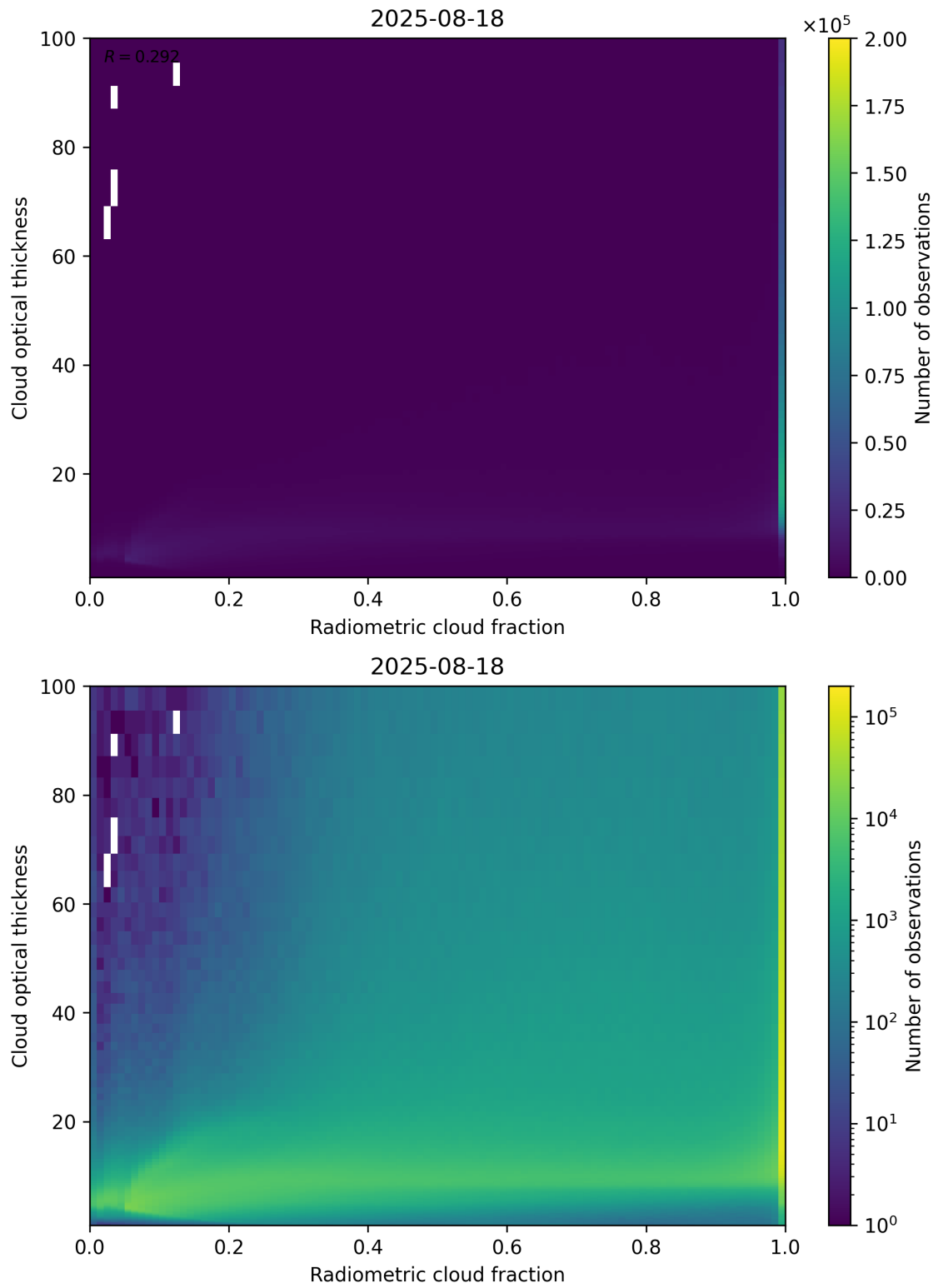
Figure 75: Scatter density plot of “Radiometric cloud fraction” against “Cloud optical thickness” for 2025-08-17 to 2025-08-19.
