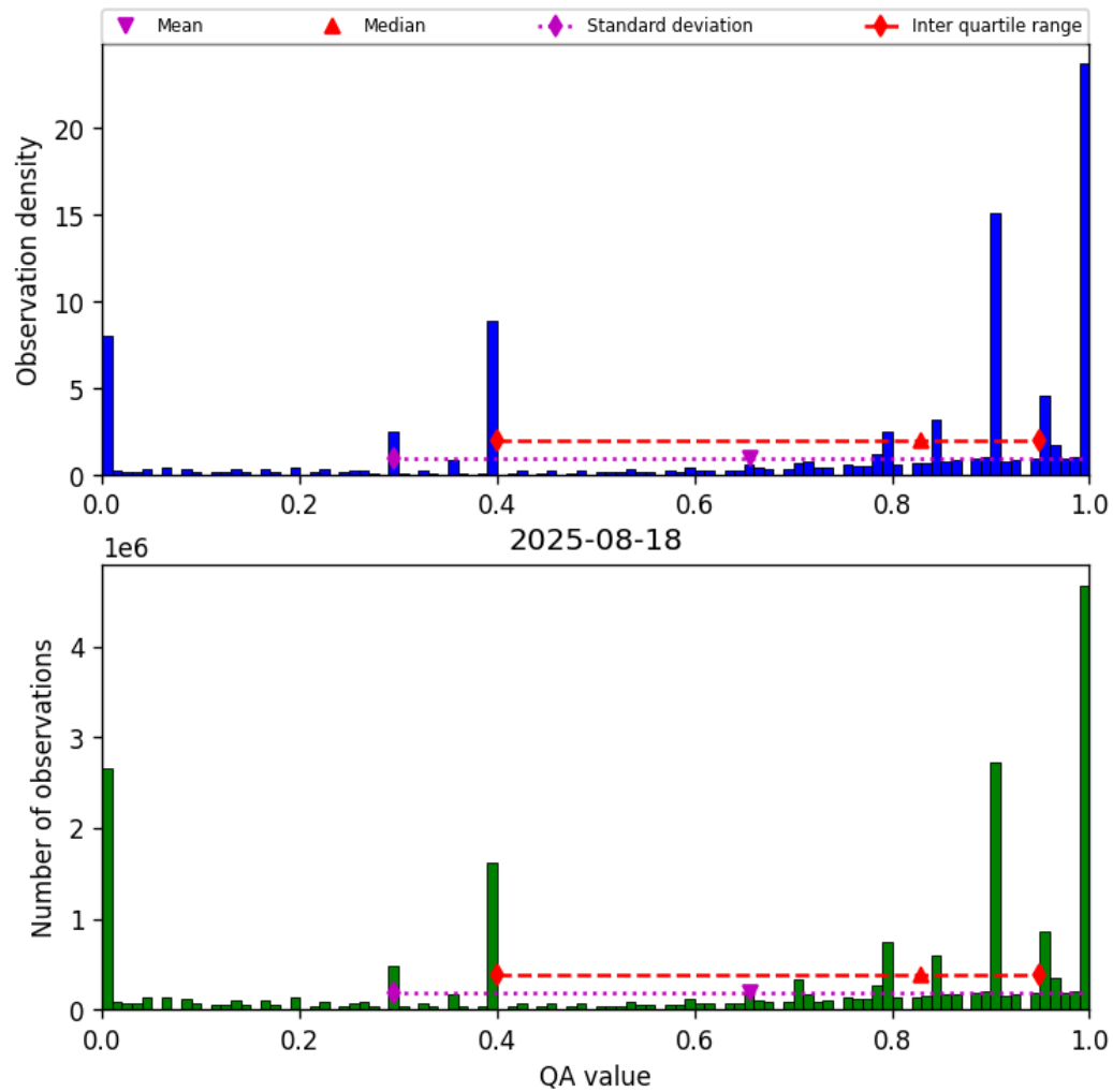
Figure 38: Histogram of “QA value” for 2025-08-17 to 2025-08-19
