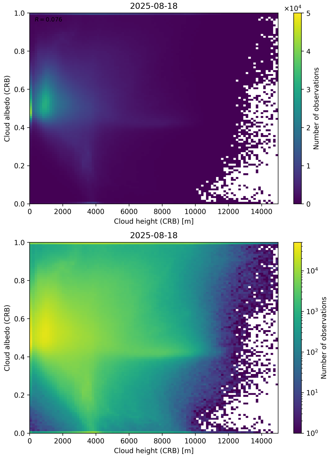
Figure 80: Scatter density plot of “Cloud height (CRB)” against “Cloud albedo (CRB)” for 2025-08-17 to 2025-08-19.
