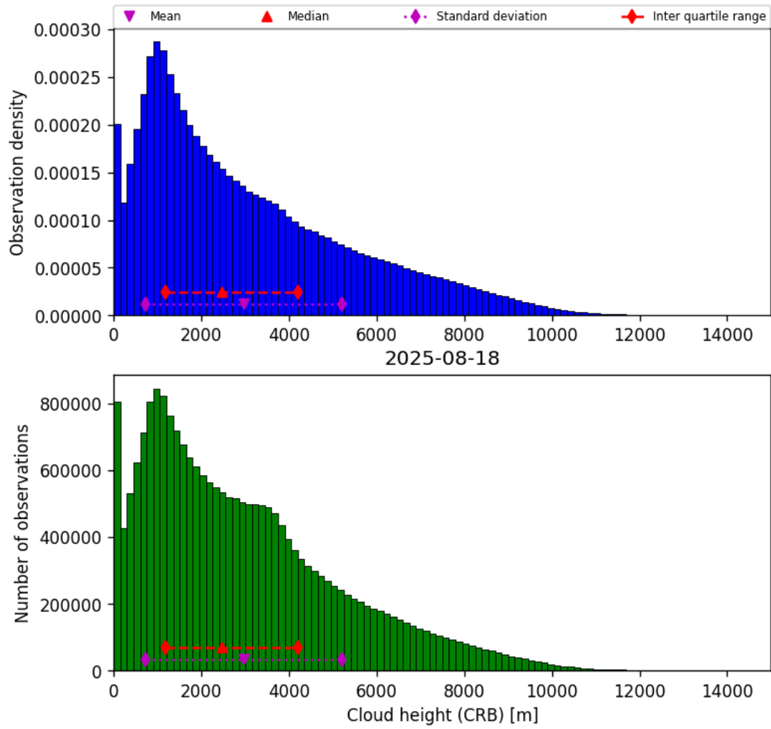
Figure 43: Histogram of “Cloud height (CRB)” for 2025-08-17 to 2025-08-19
