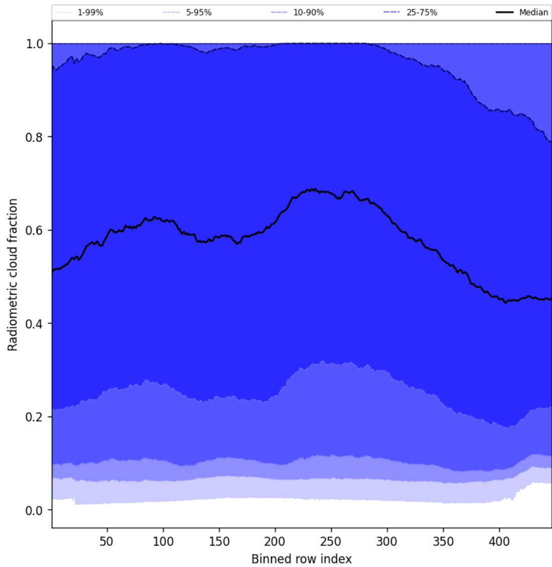
Figure 55: Along track statistics of “Radiometric cloud fraction” for 2025-08-17 to 2025-08-19
