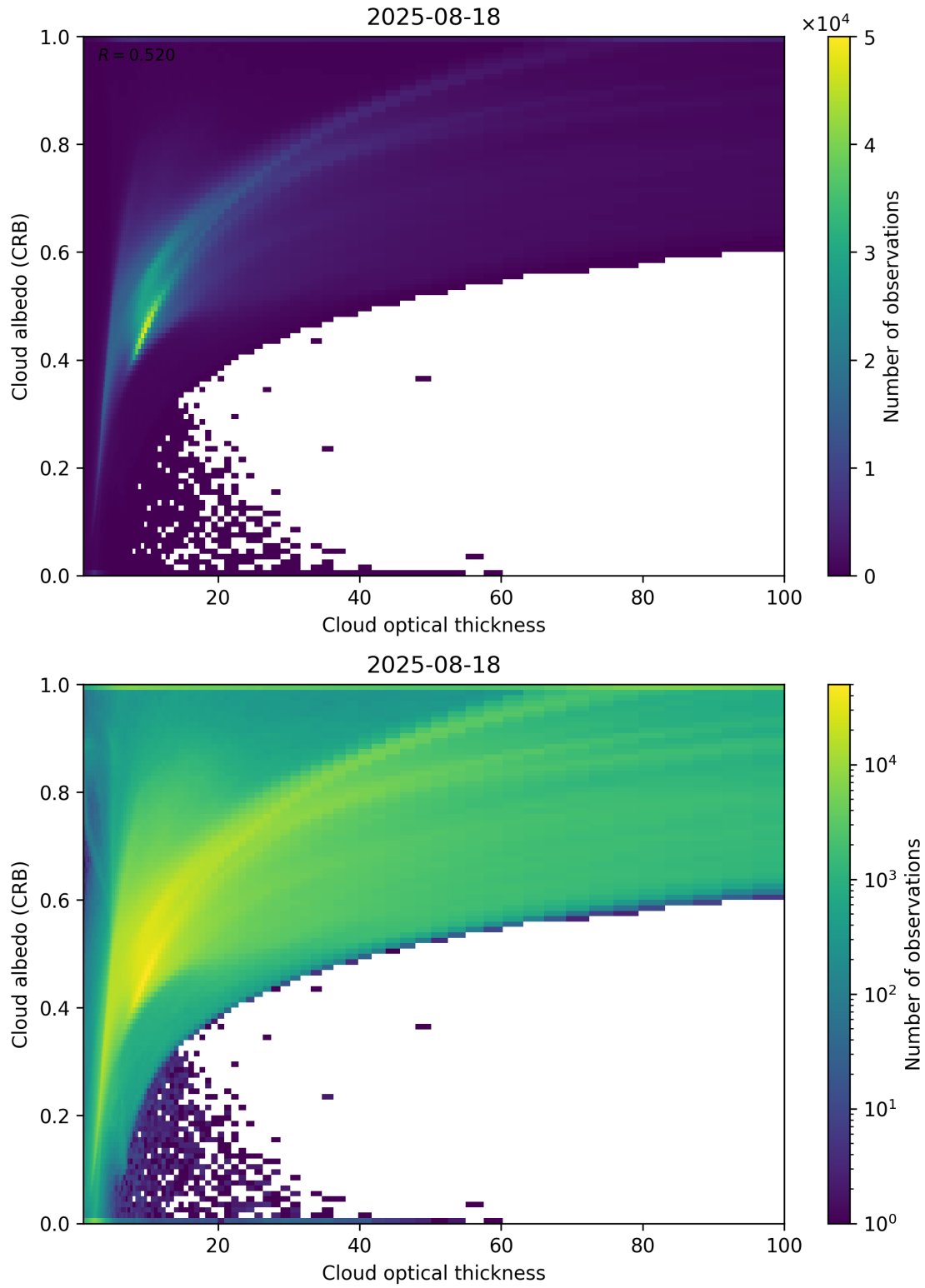
Figure 82: Scatter density plot of “Cloud optical thickness” against “Cloud albedo (CRB)” for 2025-08-17 to 2025-08-19.
