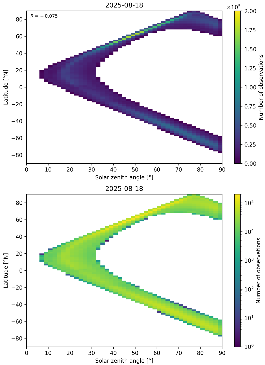
Figure 105: Scatter density plot of “Solar zenith angle” against “Latitude” for 2025-08-17 to 2025-08-19.
