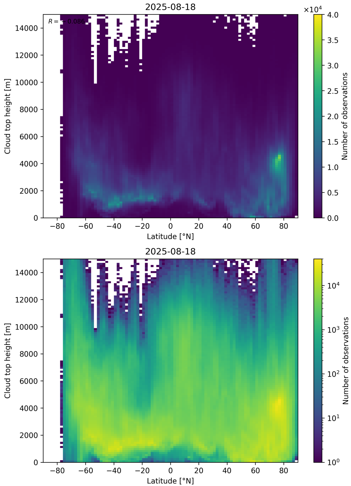
Figure 97: Scatter density plot of “Latitude” against “Cloud top height” for 2025-08-17 to 2025-08-19.
