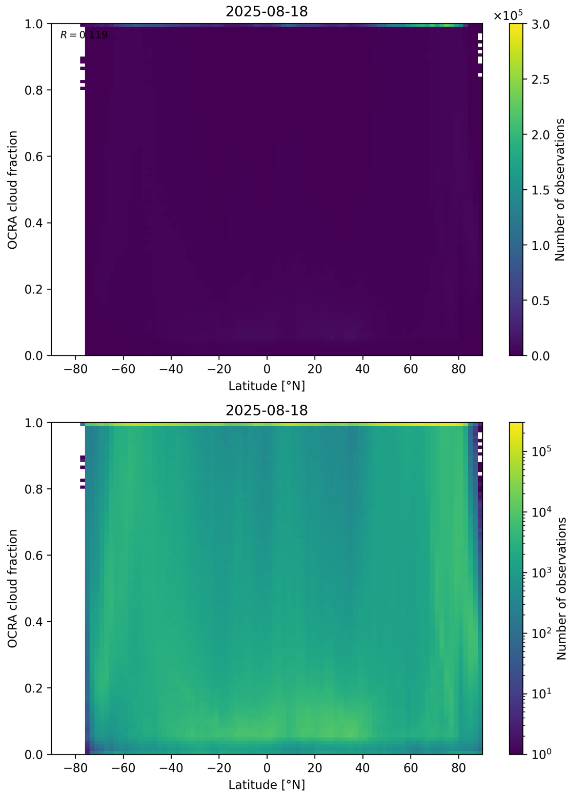
Figure 93: Scatter density plot of “Latitude” against “OCRA cloud fraction” for 2025-08-17 to 2025-08-19.
