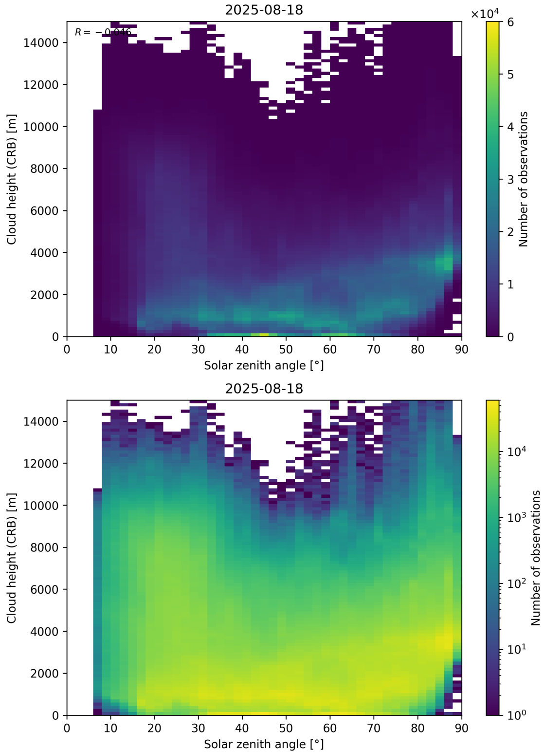
Figure 102: Scatter density plot of “Solar zenith angle” against “Cloud height (CRB)” for 2025-08-17 to 2025-08-19.
