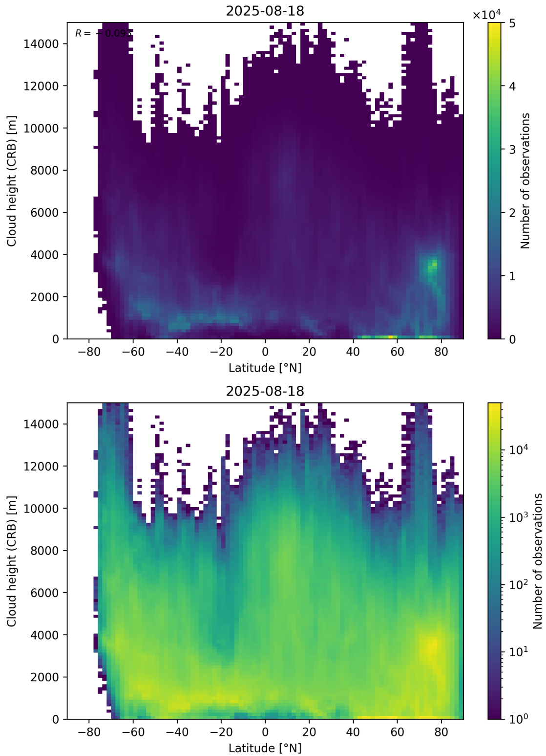
Figure 95: Scatter density plot of “Latitude” against “Cloud height (CRB)” for 2025-08-17 to 2025-08-19.
