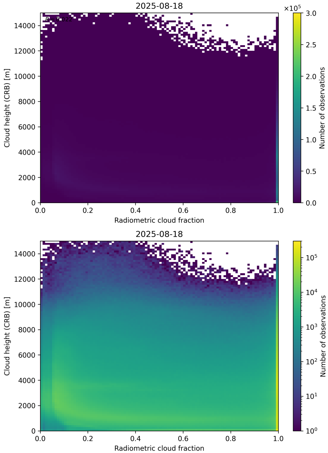
Figure 74: Scatter density plot of “Radiometric cloud fraction” against “Cloud height (CRB)” for 2025-08-17 to 2025-08-19.
