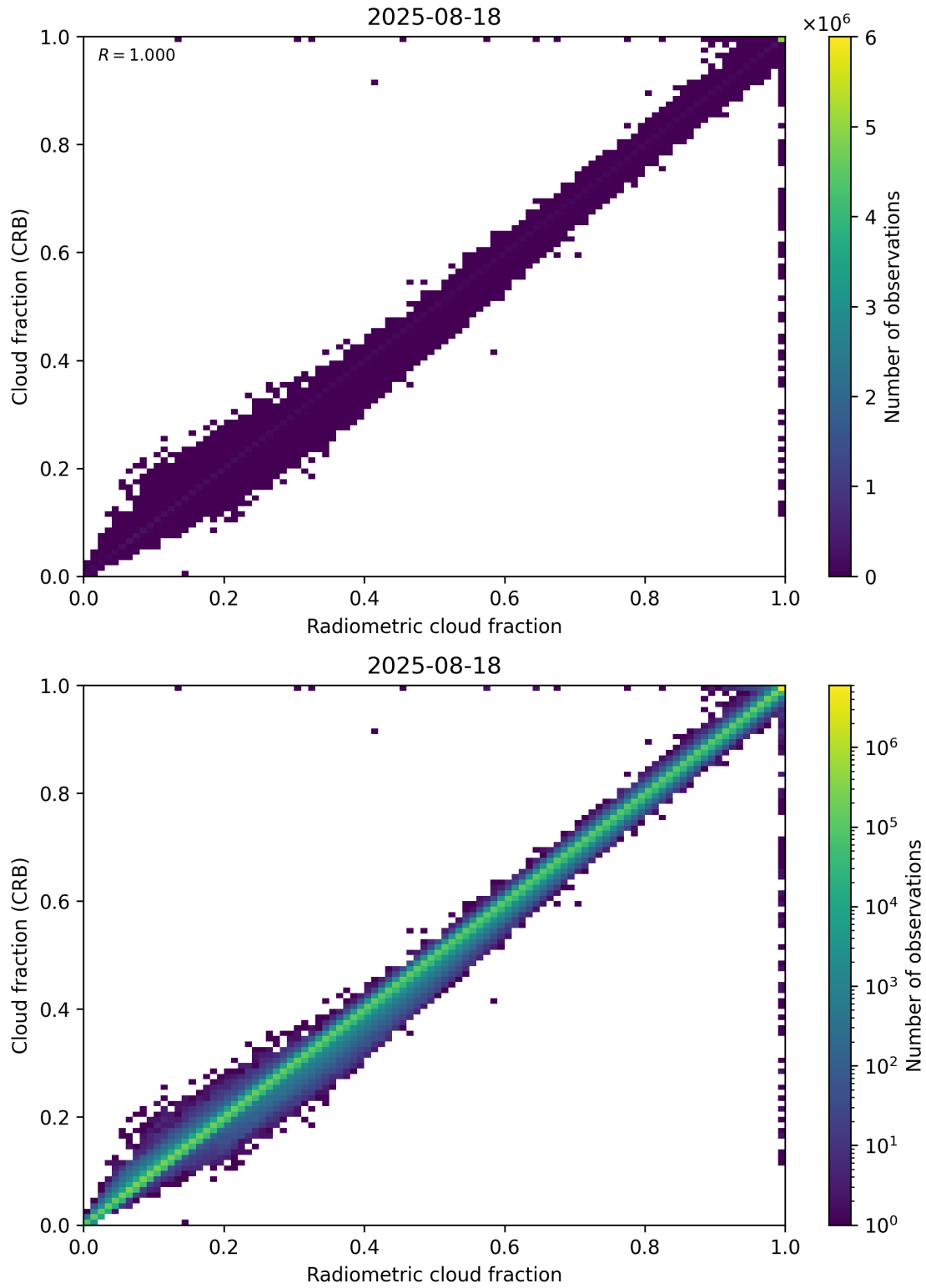
Figure 73: Scatter density plot of “Radiometric cloud fraction” against “Cloud fraction (CRB)” for 2025-08-17 to 2025-08-19.
