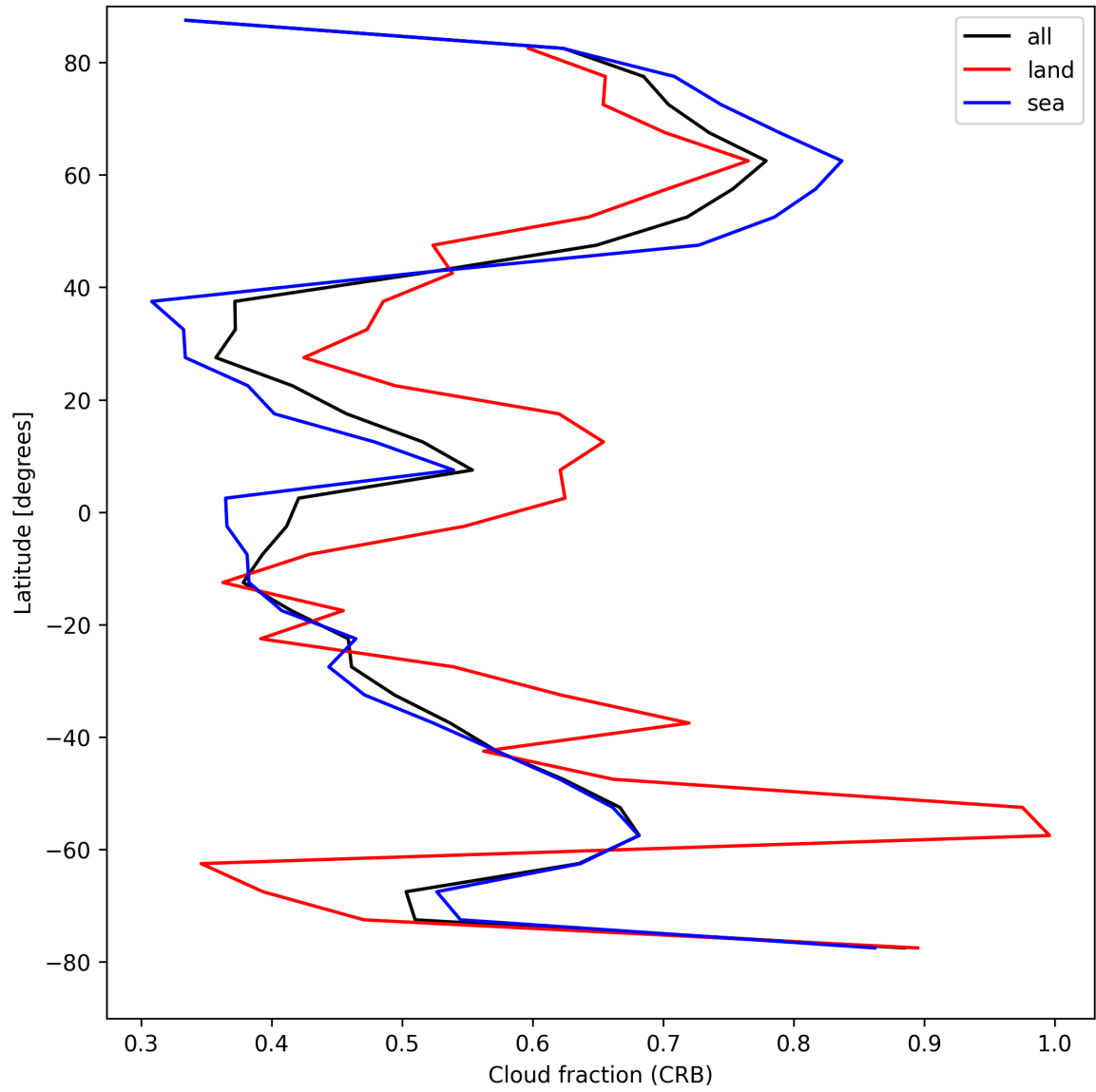
Figure 26: Zonal average of “Cloud fraction (CRB)” for 2025-08-17 to 2025-08-19.
