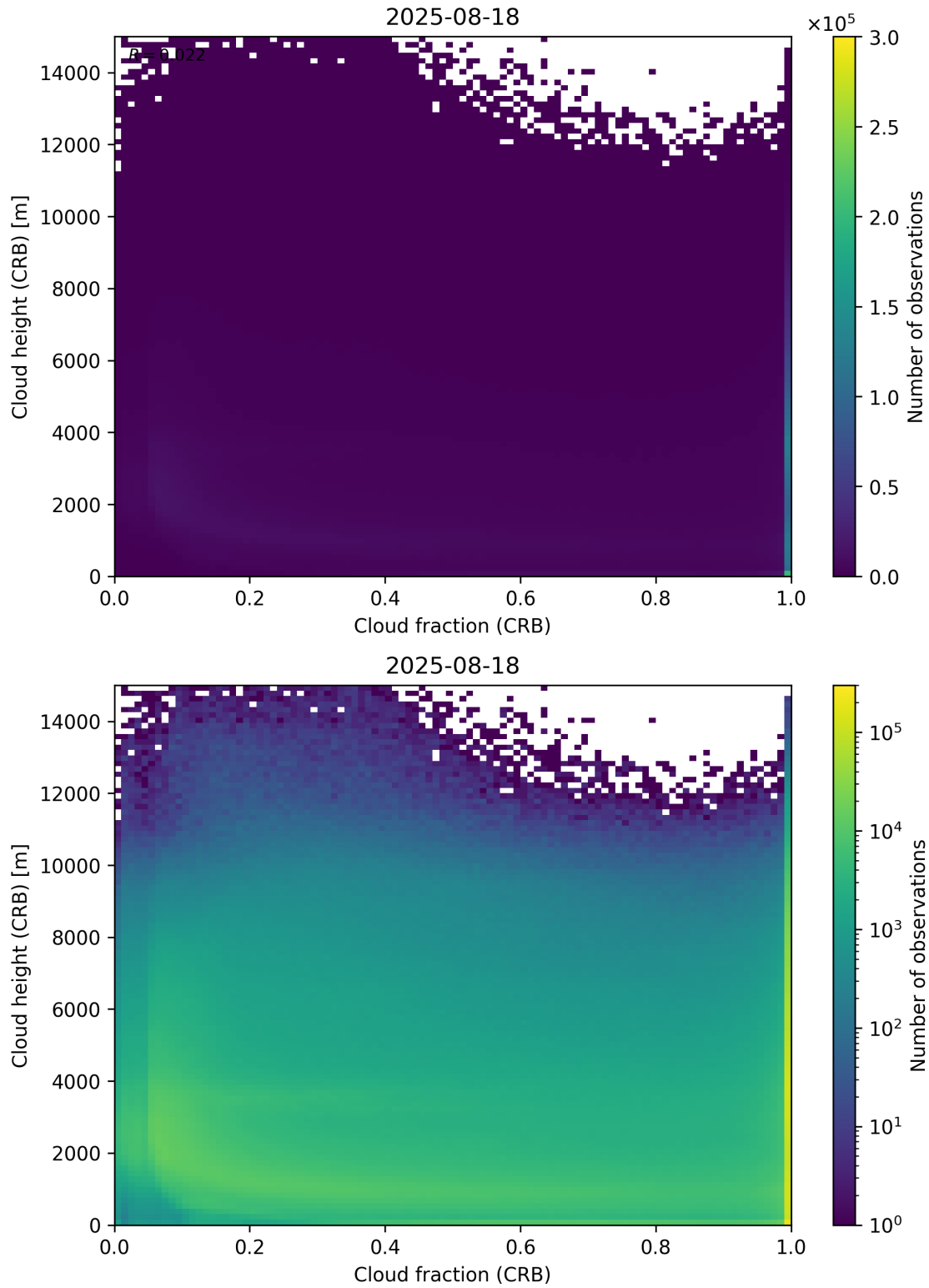
Figure 79: Scatter density plot of “Cloud fraction (CRB)” against “Cloud height (CRB)” for 2025-08-17 to 2025-08-19.
