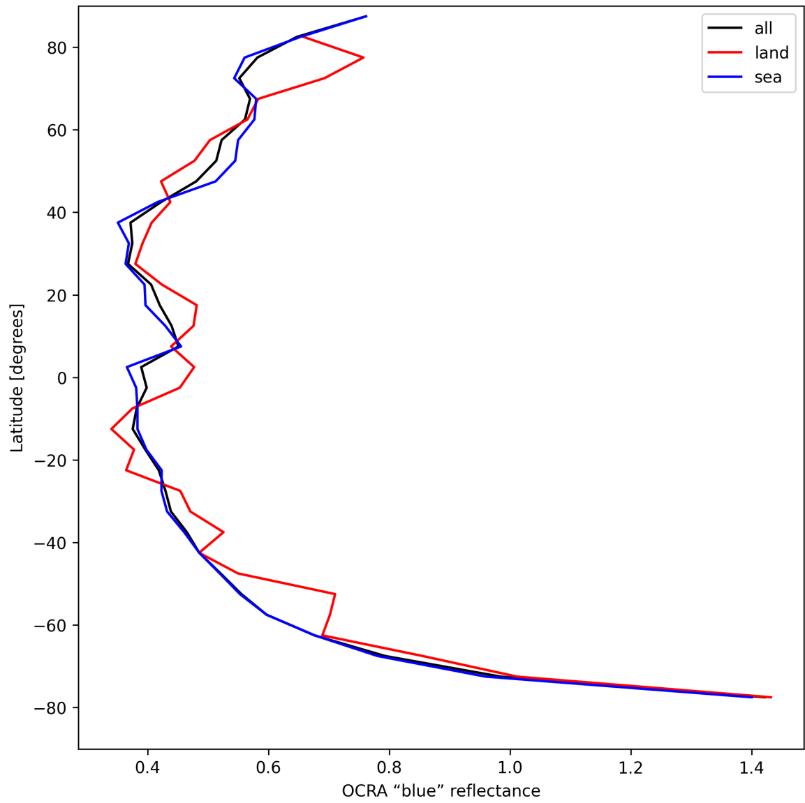
Figure 35: Zonal average of “OCRA “blue” reflectance” for 2025-08-17 to 2025-08-19.
