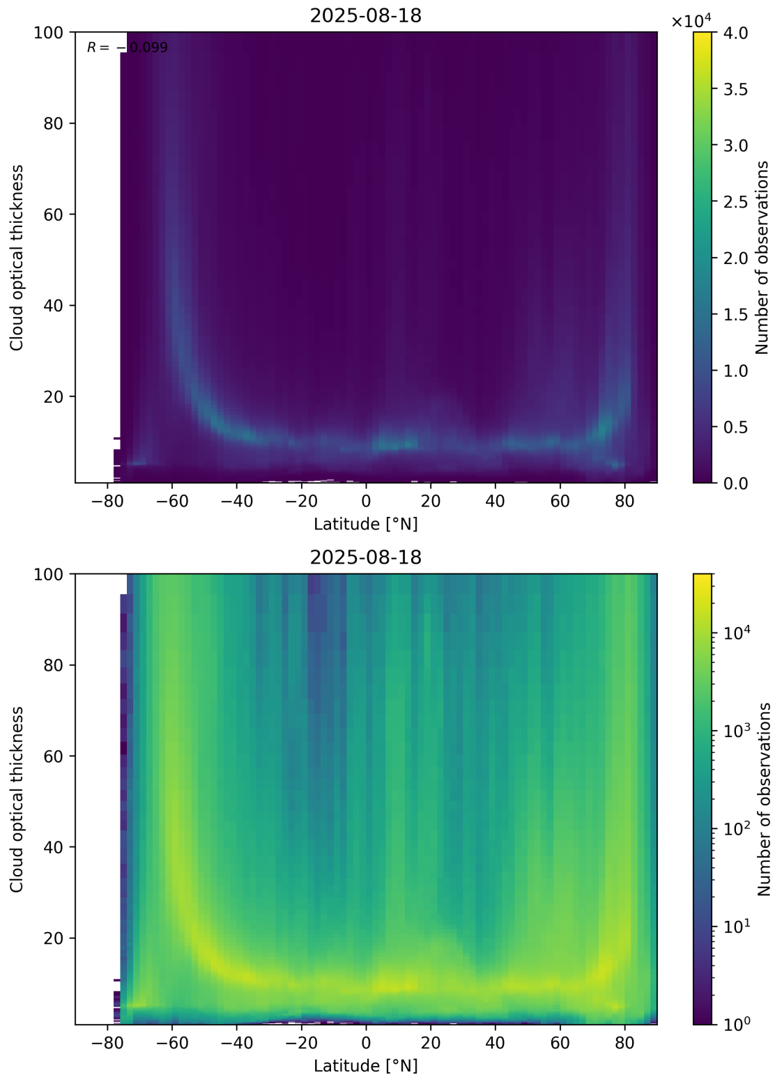
Figure 96: Scatter density plot of “Latitude” against “Cloud optical thickness” for 2025-08-17 to 2025-08-19.
