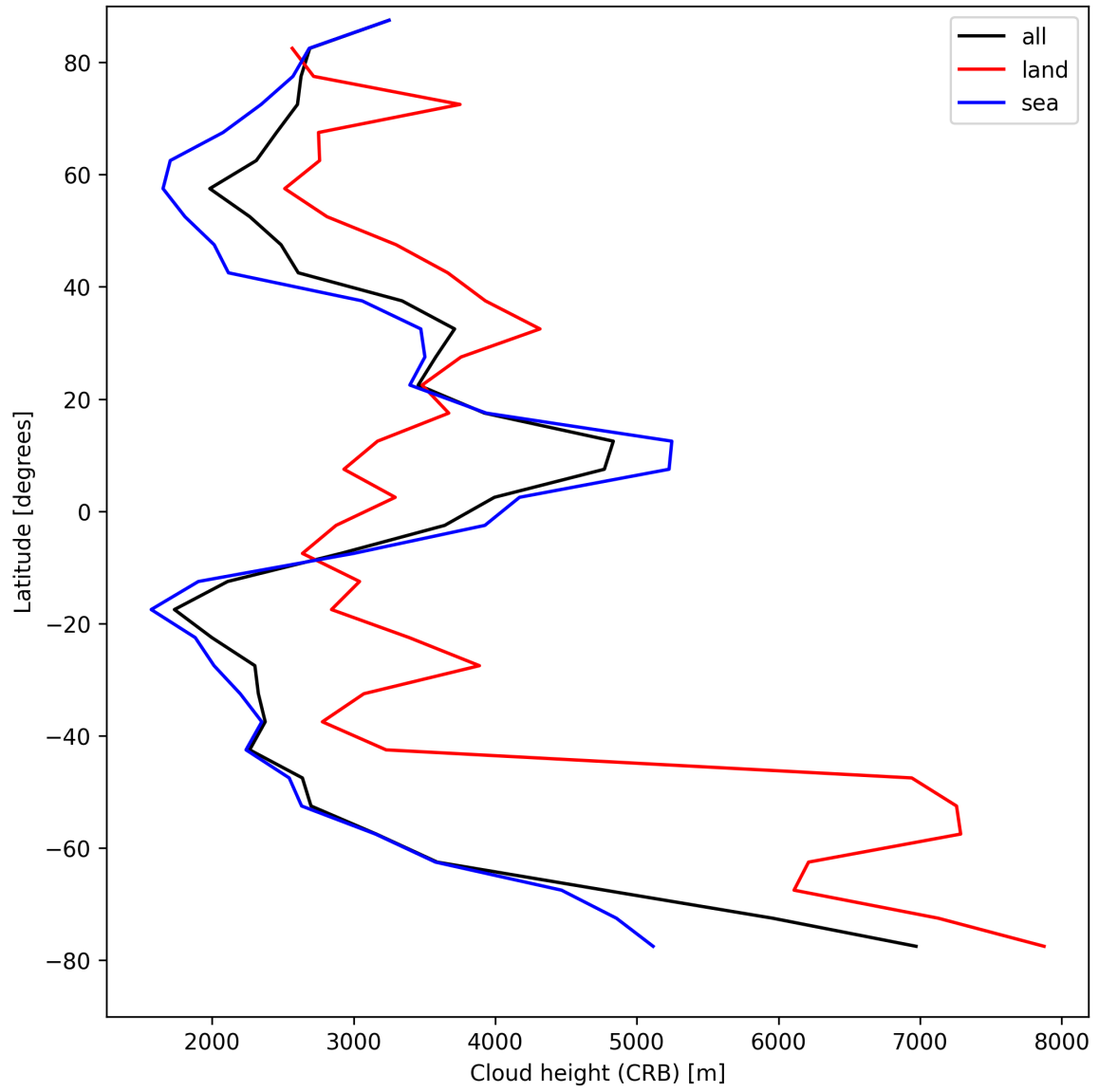
Figure 27: Zonal average of “Cloud height (CRB)” for 2025-08-17 to 2025-08-19.
