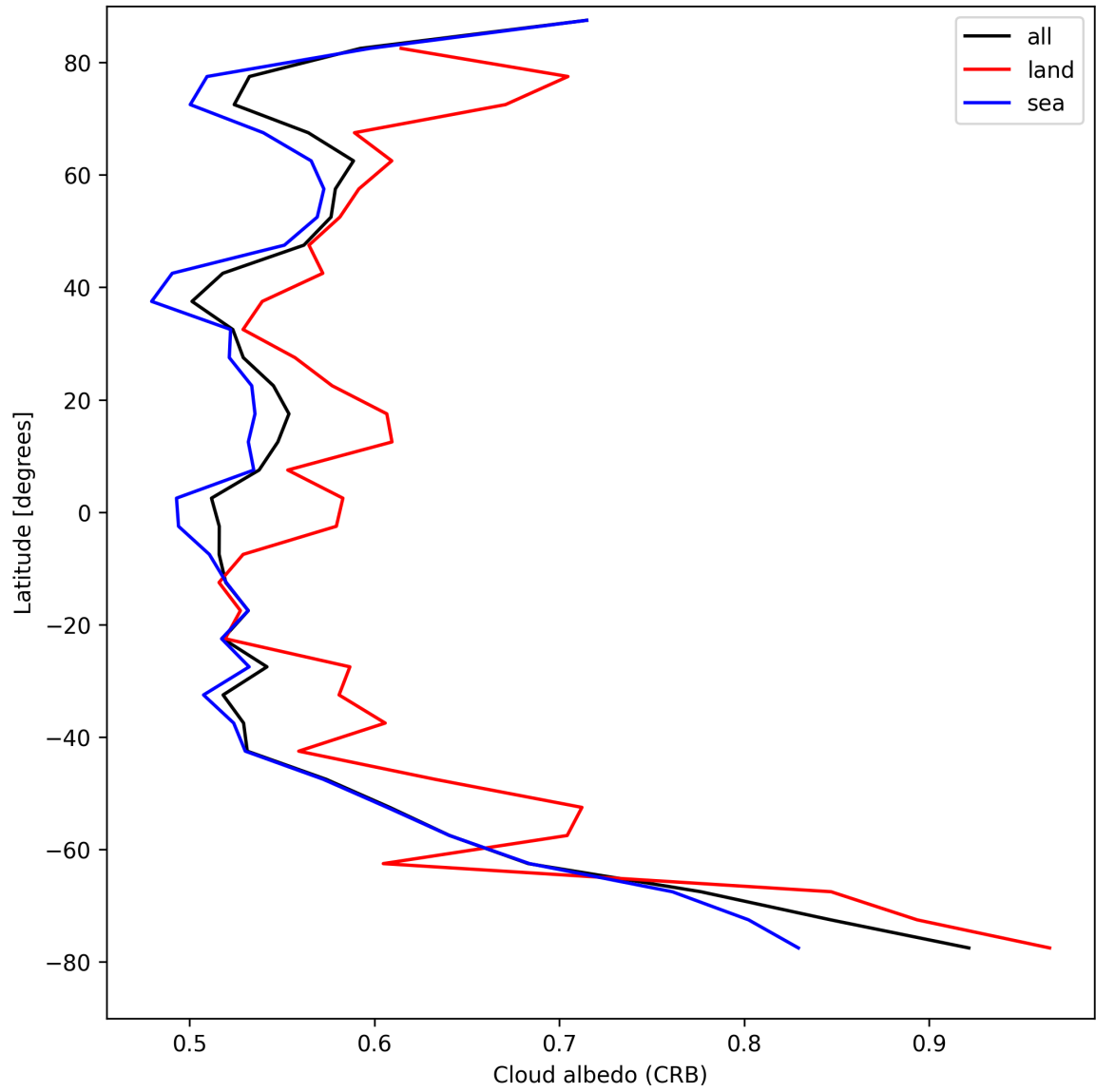
Figure 28: Zonal average of “Cloud albedo (CRB)” for 2025-08-17 to 2025-08-19.
