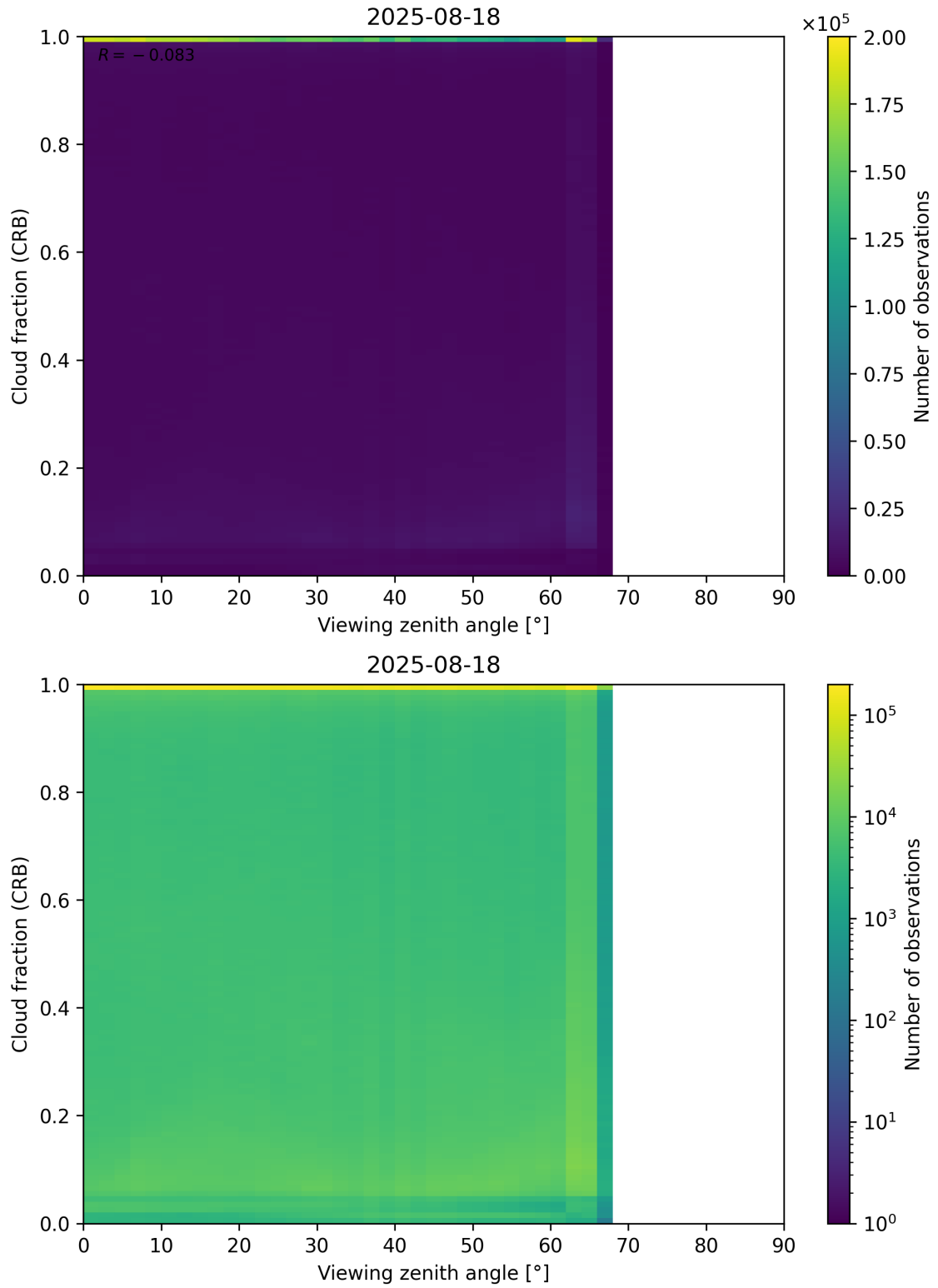
Figure 109: Scatter density plot of “Viewing zenith angle” against “Cloud fraction (CRB)” for 2025-08-17 to 2025-08-19.
