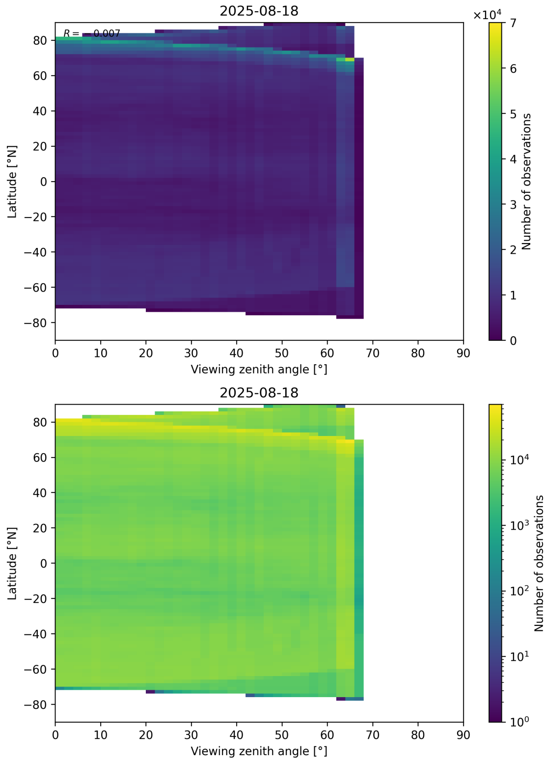
Figure 113: Scatter density plot of “Viewing zenith angle” against “Latitude” for 2025-08-17 to 2025-08-19.
