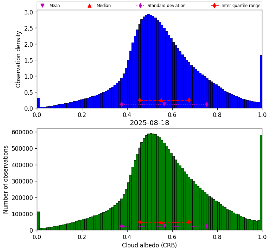
Figure 44: Histogram of “Cloud albedo (CRB)” for 2025-08-17 to 2025-08-19
