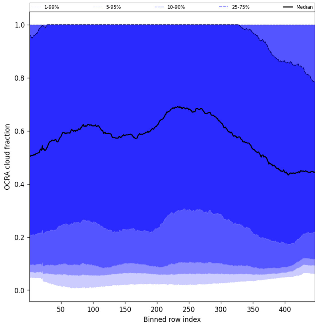
Figure 66: Along track statistics of “OCRA cloud fraction” for 2025-08-17 to 2025-08-19
