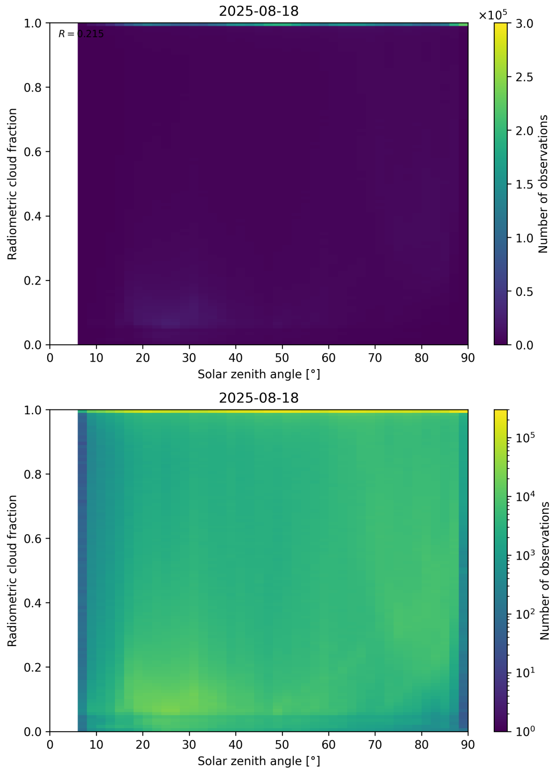
Figure 99: Scatter density plot of “Solar zenith angle” against “Radiometric cloud fraction” for 2025-08-17 to 2025-08-19.
