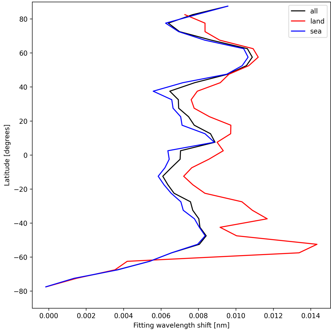
Figure 33: Zonal average of “Fitting wavelength shift” for 2025-08-17 to 2025-08-19.
