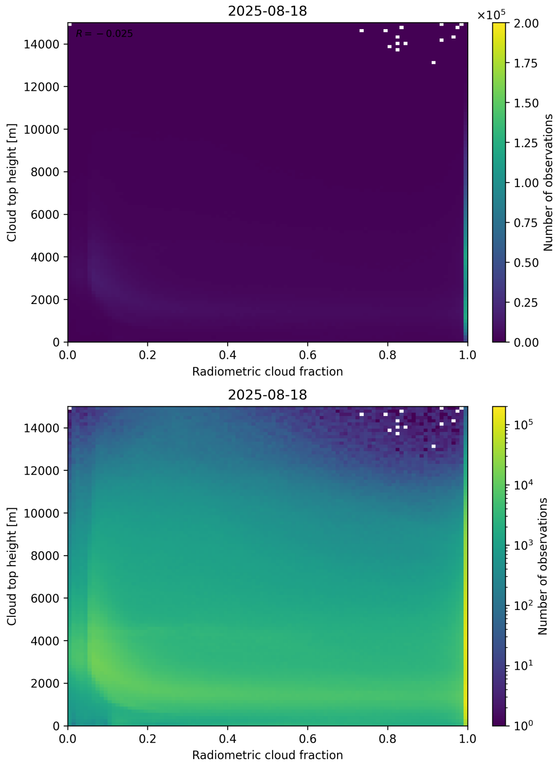
Figure 76: Scatter density plot of “Radiometric cloud fraction” against “Cloud top height” for 2025-08-17 to 2025-08-19.
