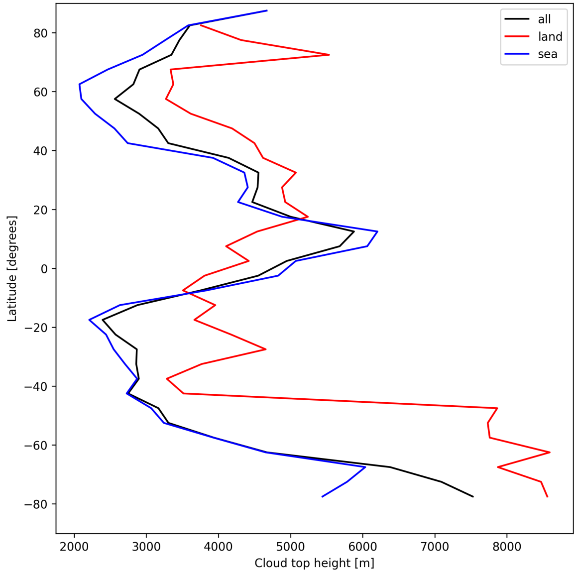
Figure 24: Zonal average of “Cloud top height” for 2025-08-17 to 2025-08-19.
