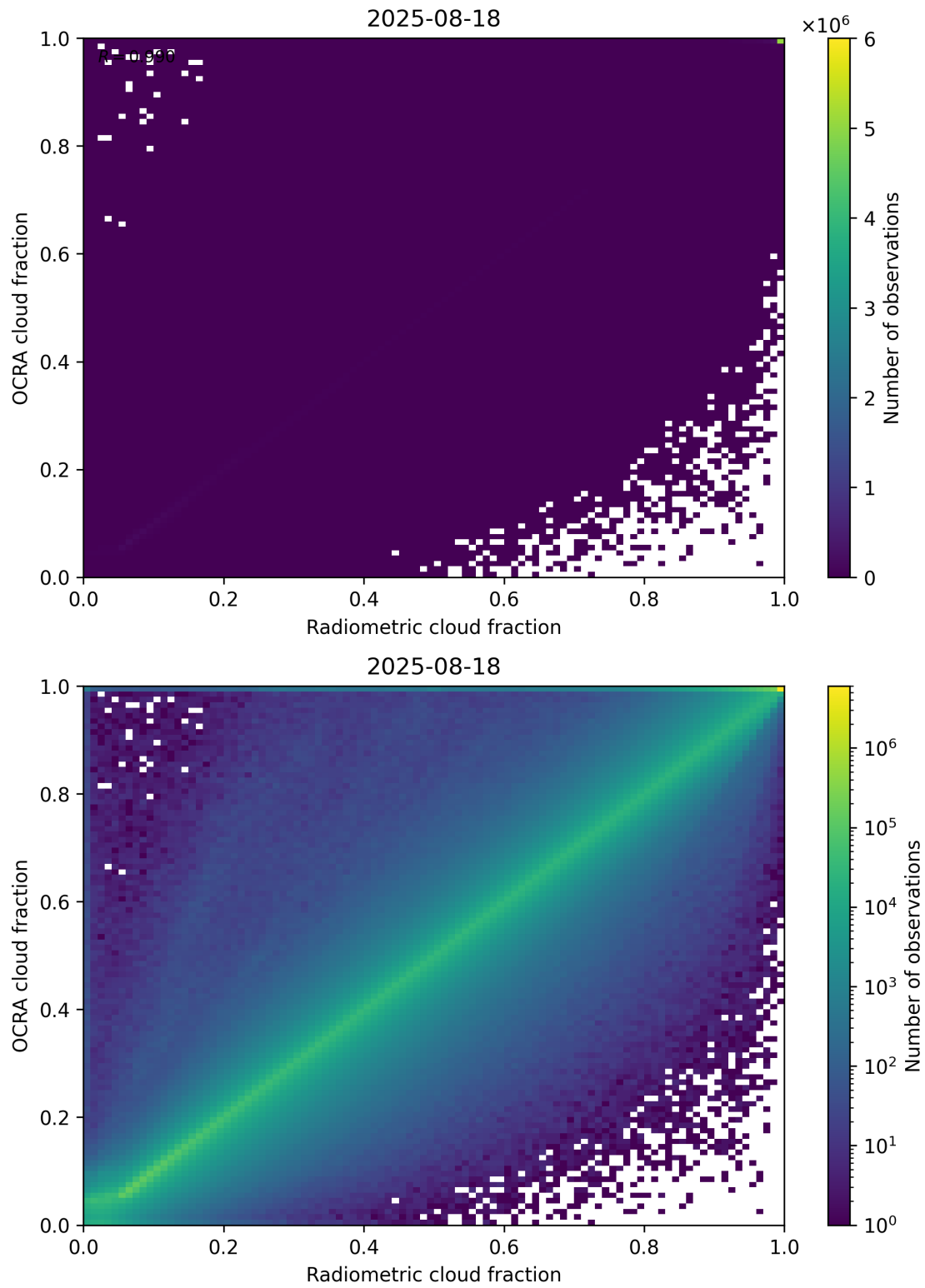
Figure 72: Scatter density plot of “Radiometric cloud fraction” against “OCRA cloud fraction” for 2025-08-17 to 2025-08-19.
