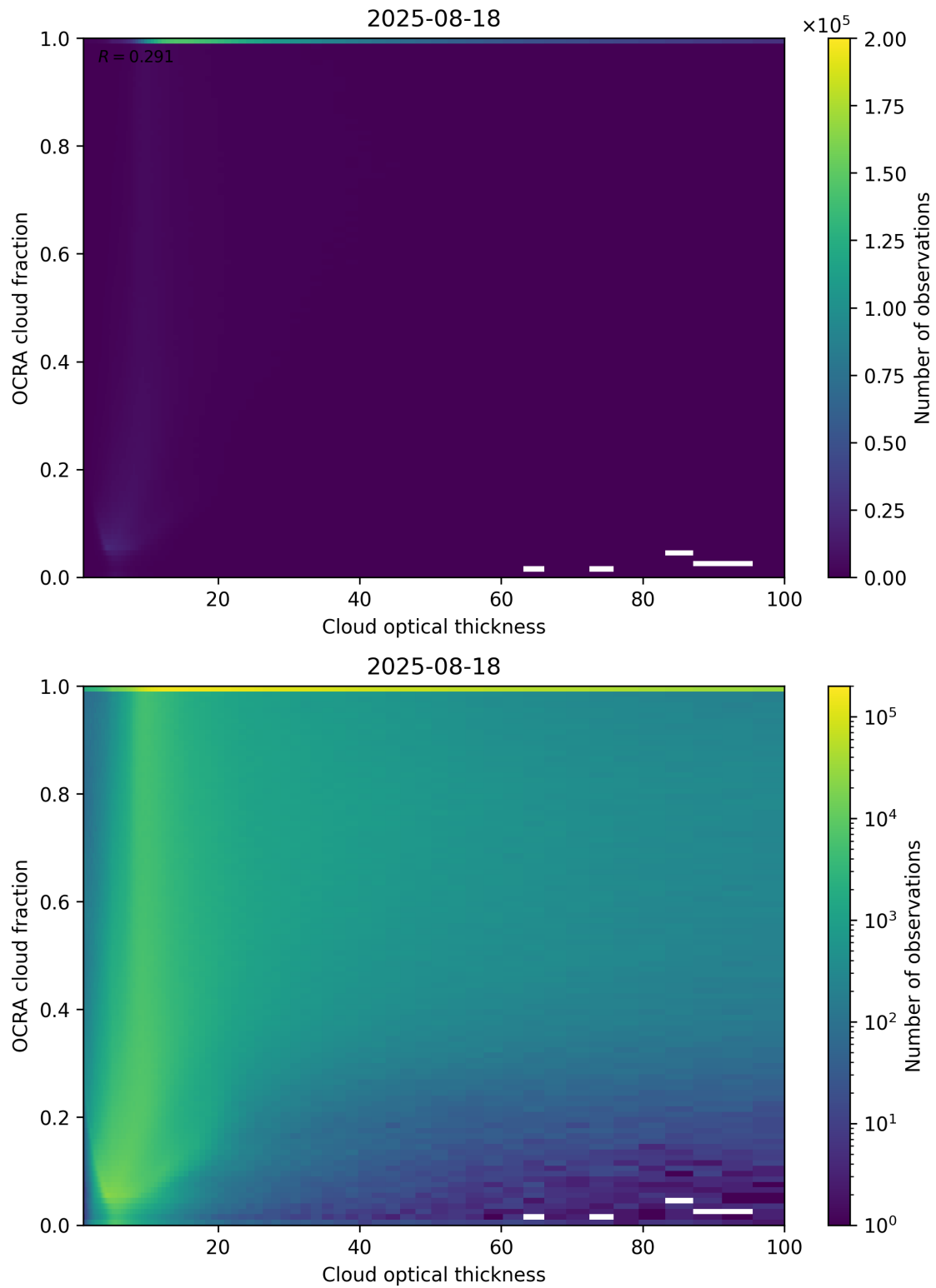
Figure 83: Scatter density plot of “Cloud optical thickness” against “OCRA cloud fraction” for 2025-08-17 to 2025-08-19.
