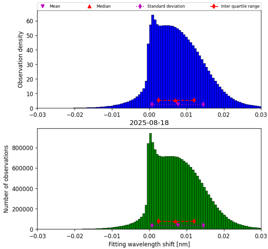
Figure 49: Histogram of “Fitting wavelength shift” for 2025-08-17 to 2025-08-19
