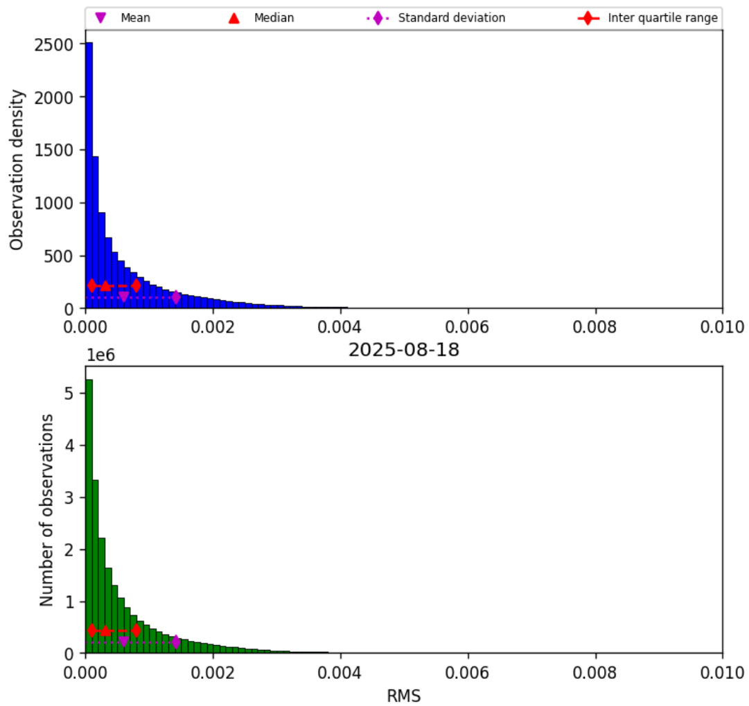
Figure 47: Histogram of “RMS” for 2025-08-17 to 2025-08-19
