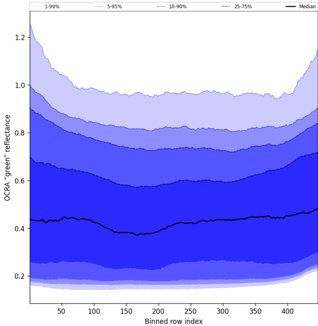
Figure 68: Along track statistics of “OCRA “green” reflectance” for 2025-08-17 to 2025-08-19
