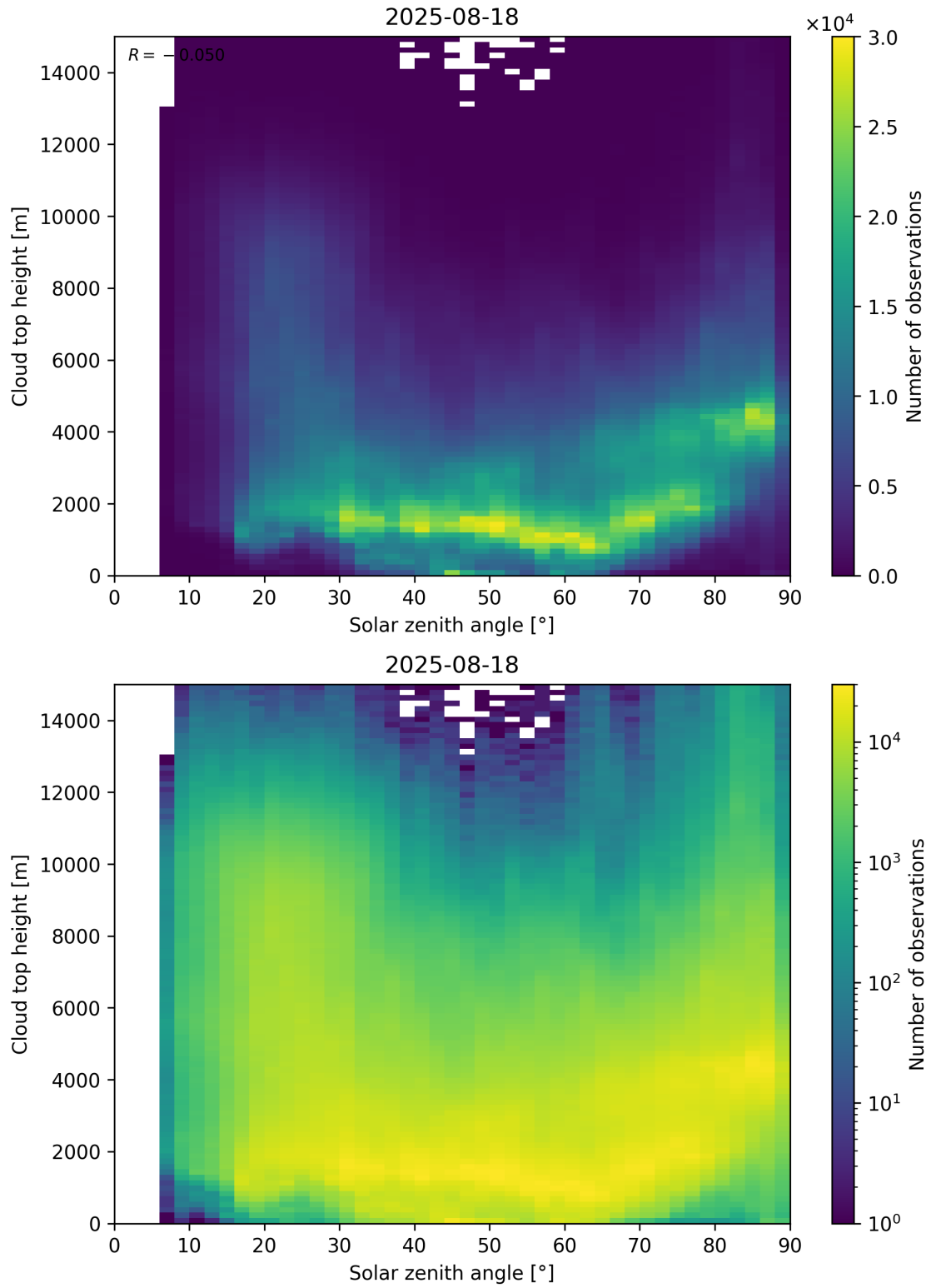
Figure 104: Scatter density plot of “Solar zenith angle” against “Cloud top height” for 2025-08-17 to 2025-08-19.
