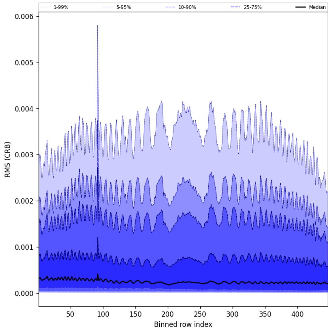
Figure 64: Along track statistics of “RMS (CRB)” for 2025-08-17 to 2025-08-19
