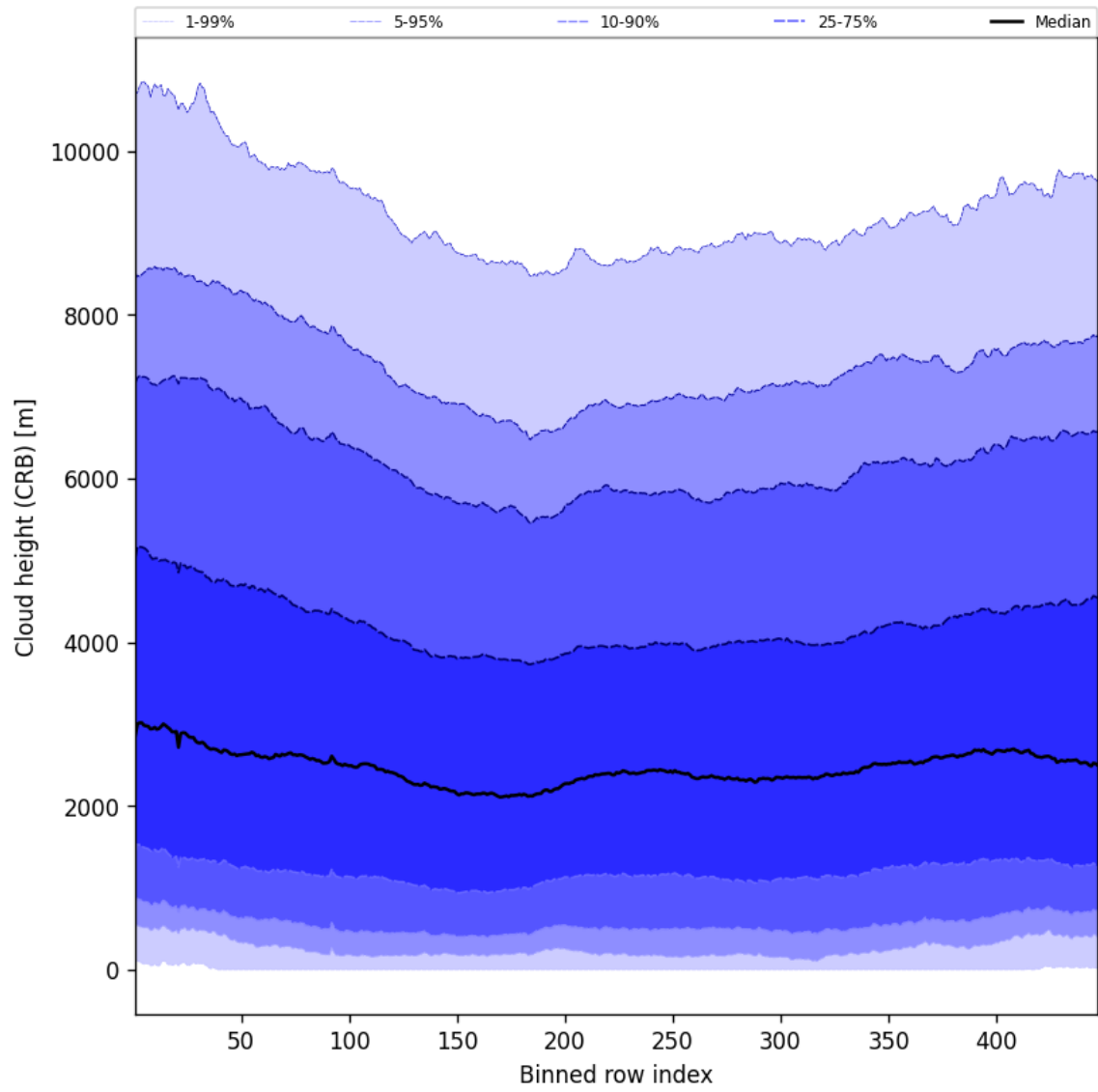
Figure 59: Along track statistics of “Cloud height (CRB)” for 2025-08-17 to 2025-08-19
