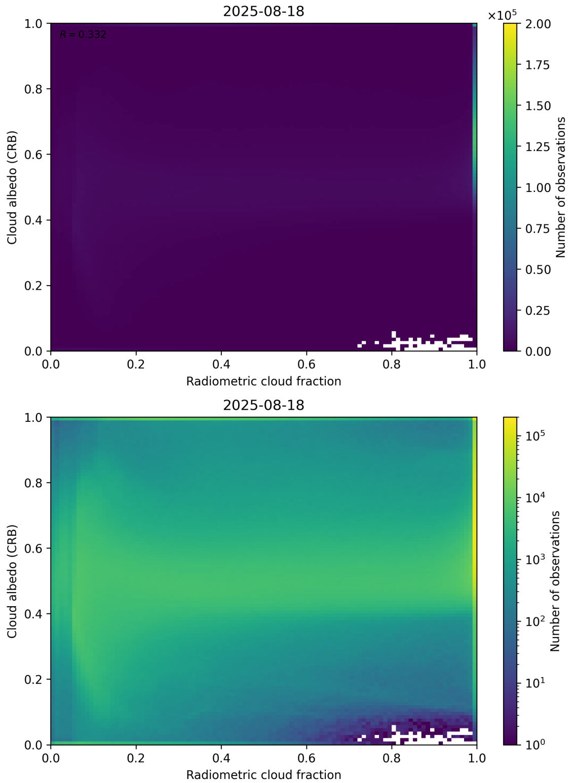
Figure 71: Scatter density plot of “Radiometric cloud fraction” against “Cloud albedo (CRB)” for 2025-08-17 to 2025-08-19.
