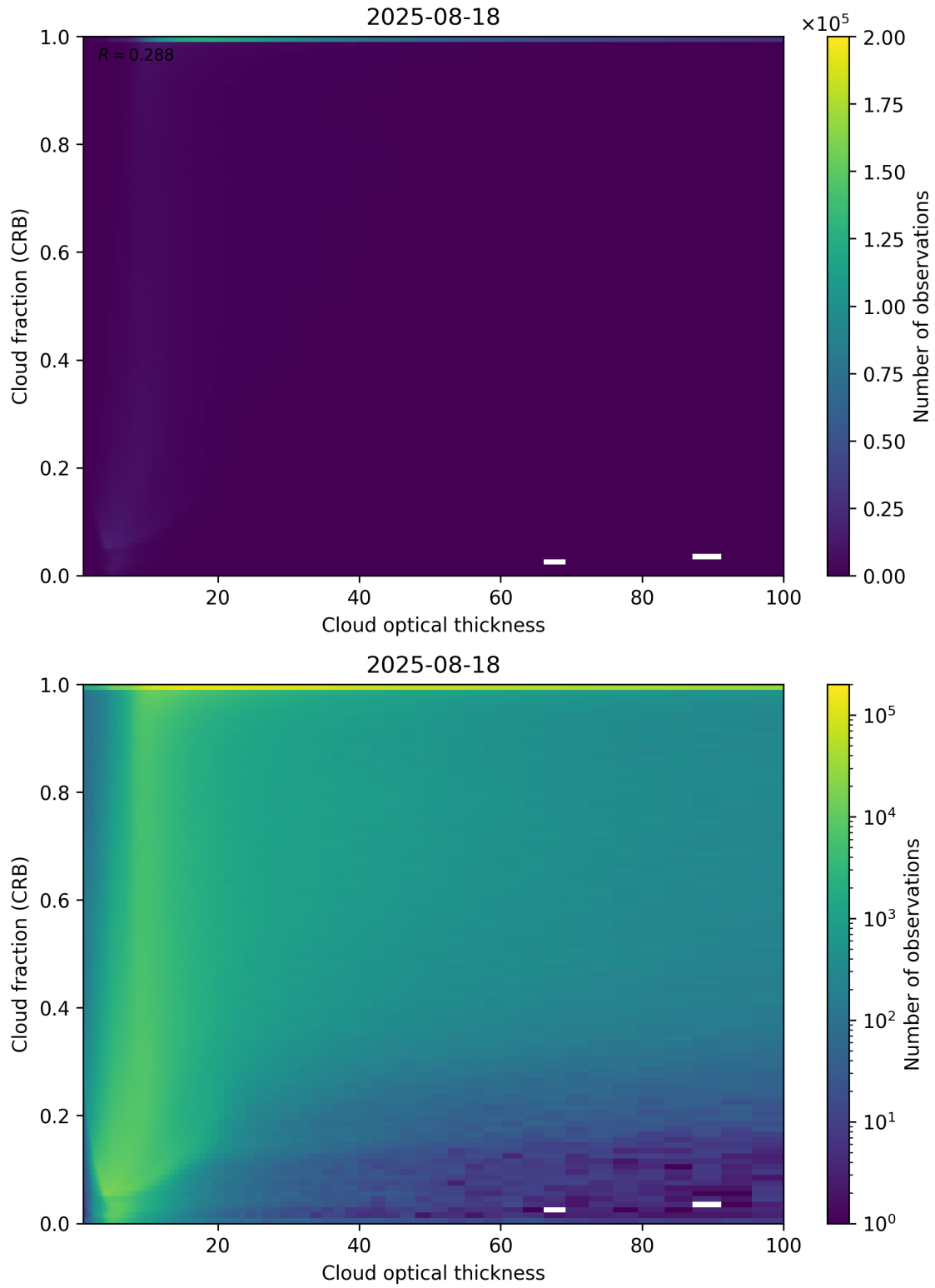
Figure 84: Scatter density plot of “Cloud optical thickness” against “Cloud fraction (CRB)” for 2025-08-17 to 2025-08-19.
