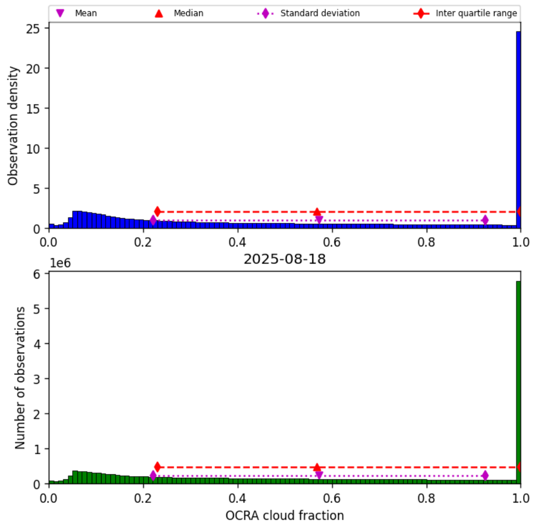
Figure 50: Histogram of “OCRA cloud fraction” for 2025-08-17 to 2025-08-19
