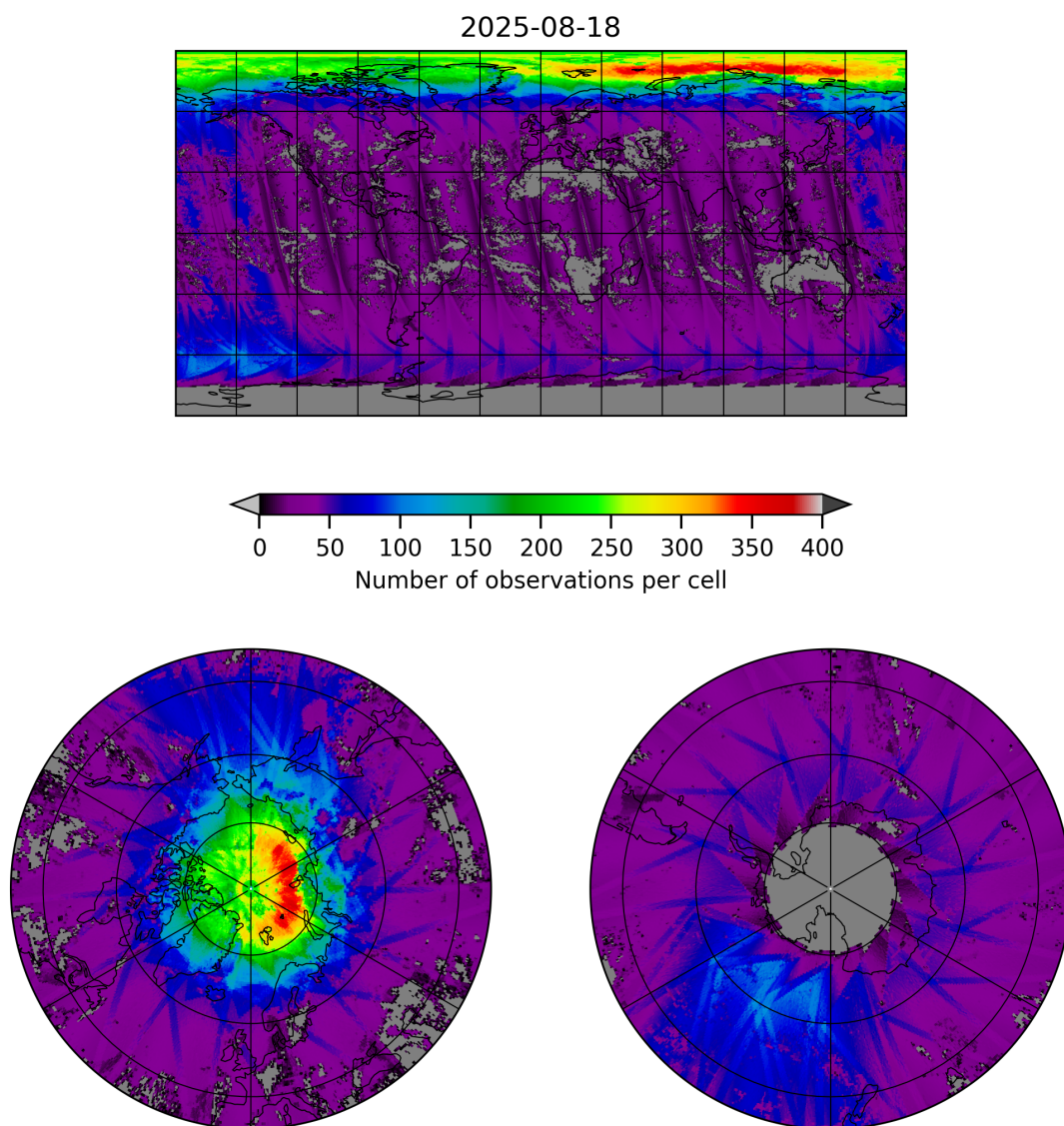
Figure 21: Map of the number of observations for 2025-08-17 to 2025-08-19
