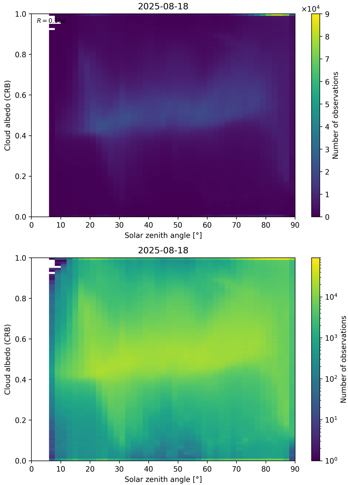
Figure 98: Scatter density plot of “Solar zenith angle” against “Cloud albedo (CRB)” for 2025-08-17 to 2025-08-19.
