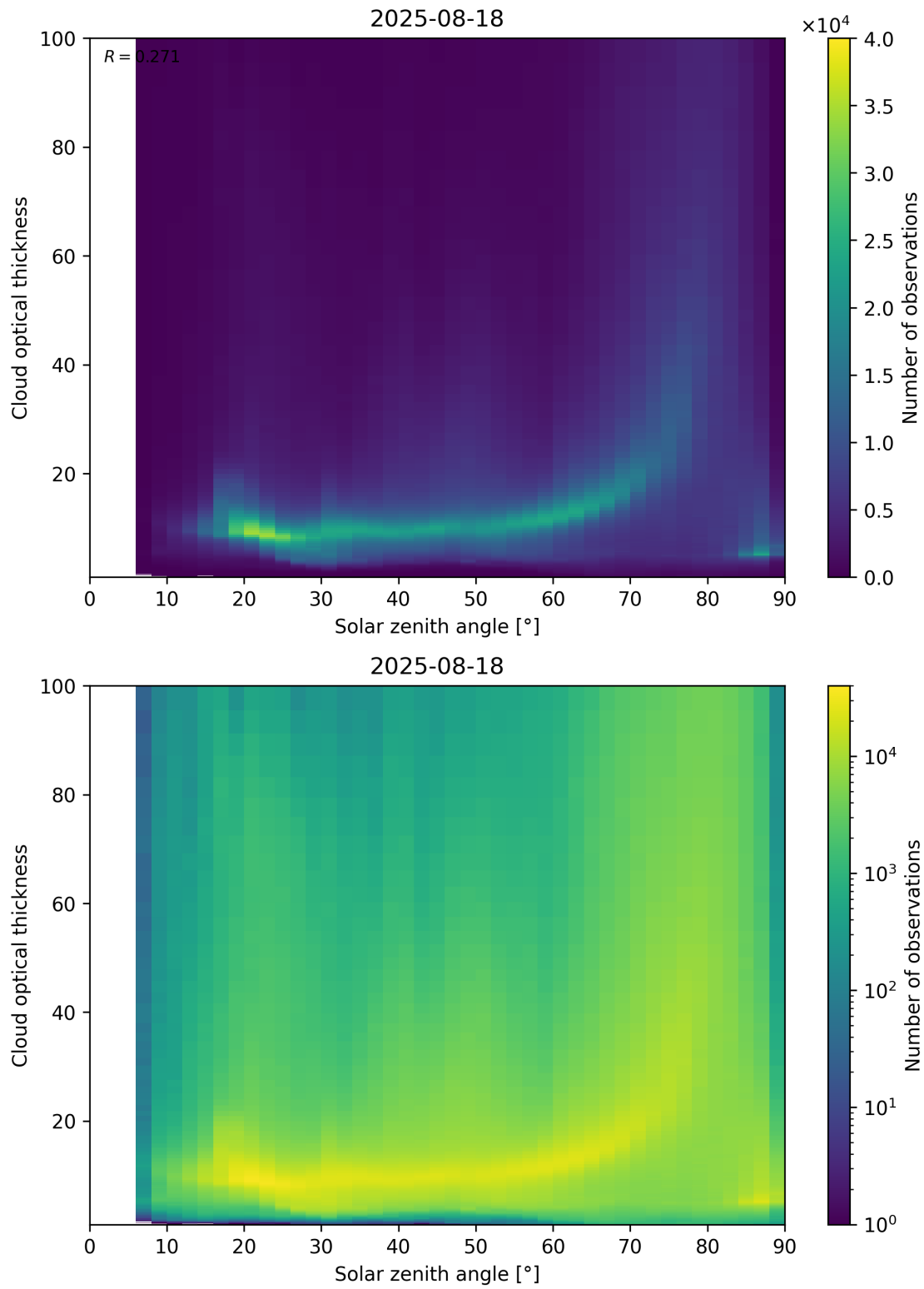
Figure 103: Scatter density plot of “Solar zenith angle” against “Cloud optical thickness” for 2025-08-17 to 2025-08-19.
