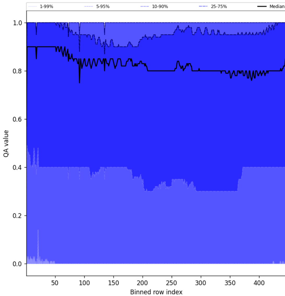
Figure 54: Along track statistics of “QA value” for 2025-08-17 to 2025-08-19
