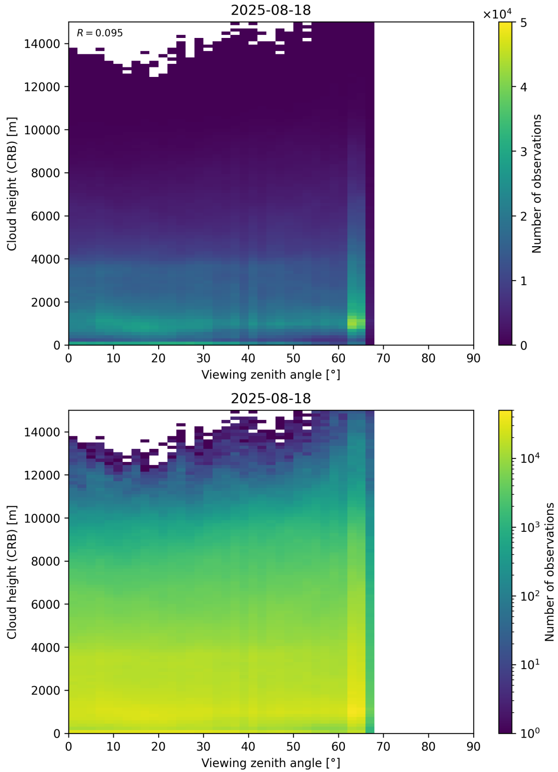
Figure 110: Scatter density plot of “Viewing zenith angle” against “Cloud height (CRB)” for 2025-08-17 to 2025-08-19.
