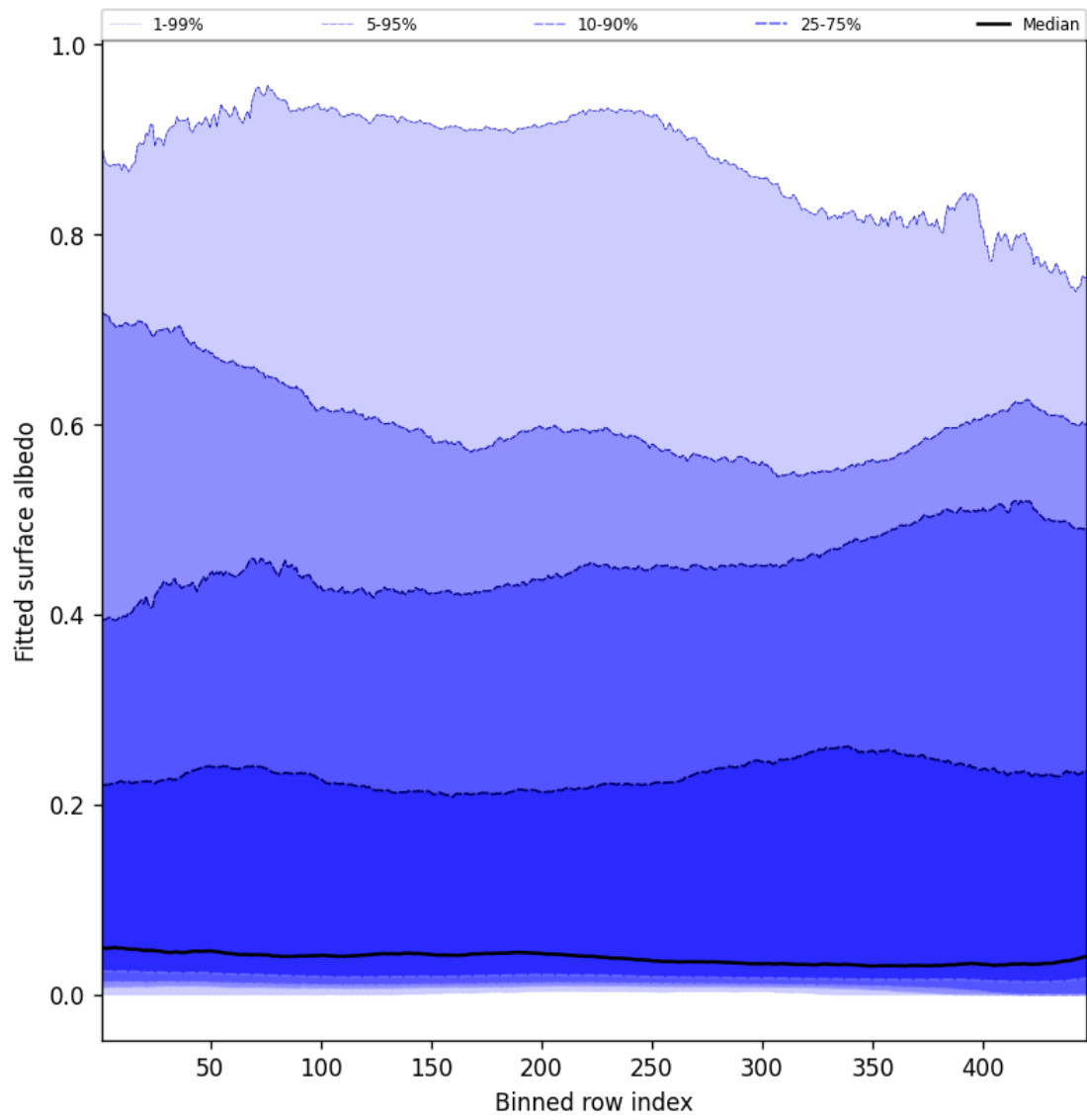
Figure 61: Along track statistics of “Fitted surface albedo” for 2025-08-17 to 2025-08-19
