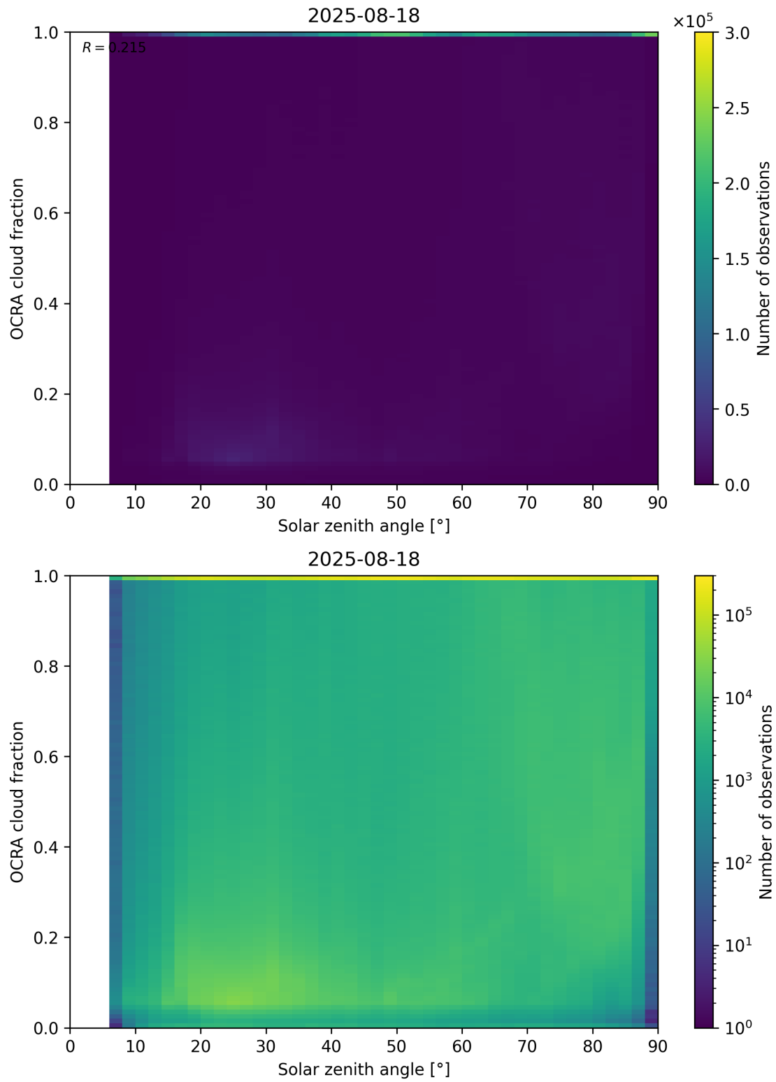
Figure 100: Scatter density plot of “Solar zenith angle” against “OCRA cloud fraction” for 2025-08-17 to 2025-08-19.
