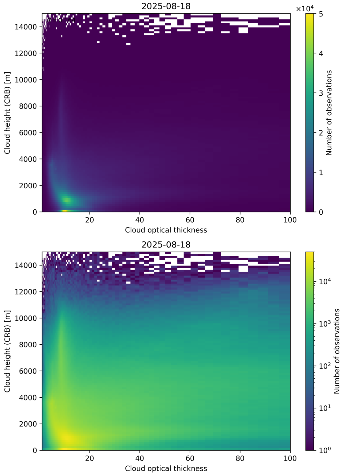
Figure 85: Scatter density plot of “Cloud optical thickness” against “Cloud height (CRB)” for 2025-08-17 to 2025-08-19.
