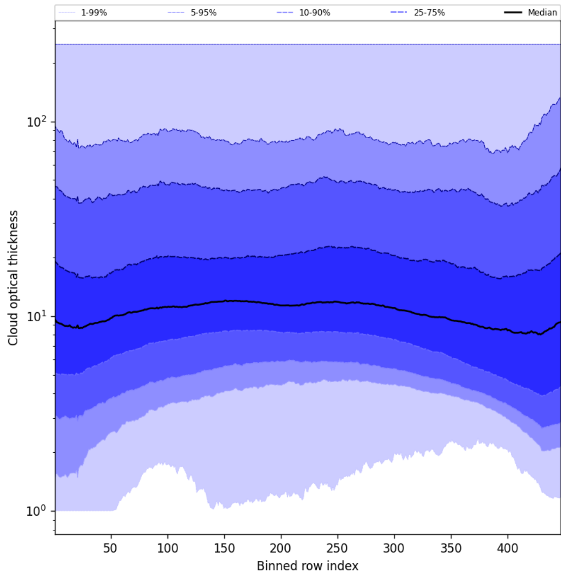
Figure 57: Along track statistics of “Cloud optical thickness” for 2025-08-17 to 2025-08-19
