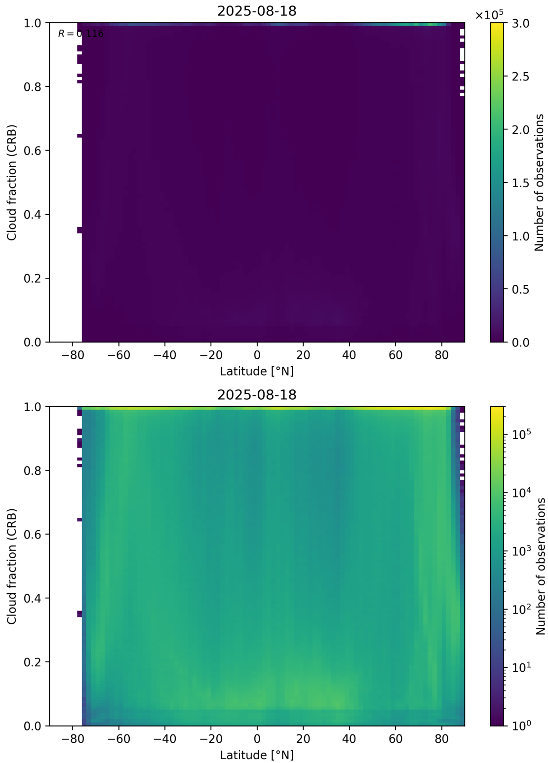
Figure 94: Scatter density plot of “Latitude” against “Cloud fraction (CRB)” for 2025-08-17 to 2025-08-19.
