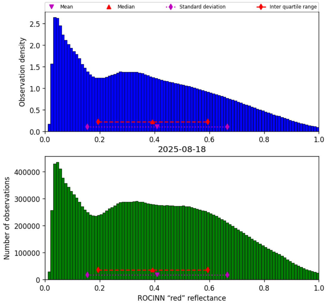
Figure 53: Histogram of “ROCINN “red” reflectance” for 2025-08-17 to 2025-08-19
