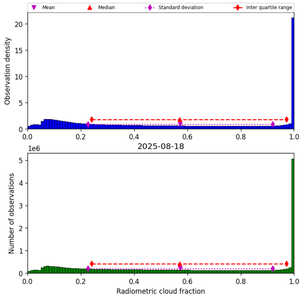
Figure 39: Histogram of “Radiometric cloud fraction” for 2025-08-17 to 2025-08-19
