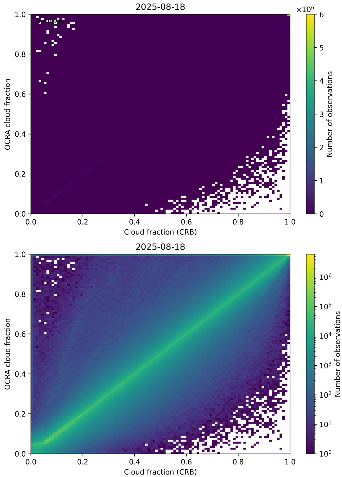
Figure 78: Scatter density plot of “Cloud fraction (CRB)” against “OCRA cloud fraction” for 2025-08-17 to 2025-08-19.
