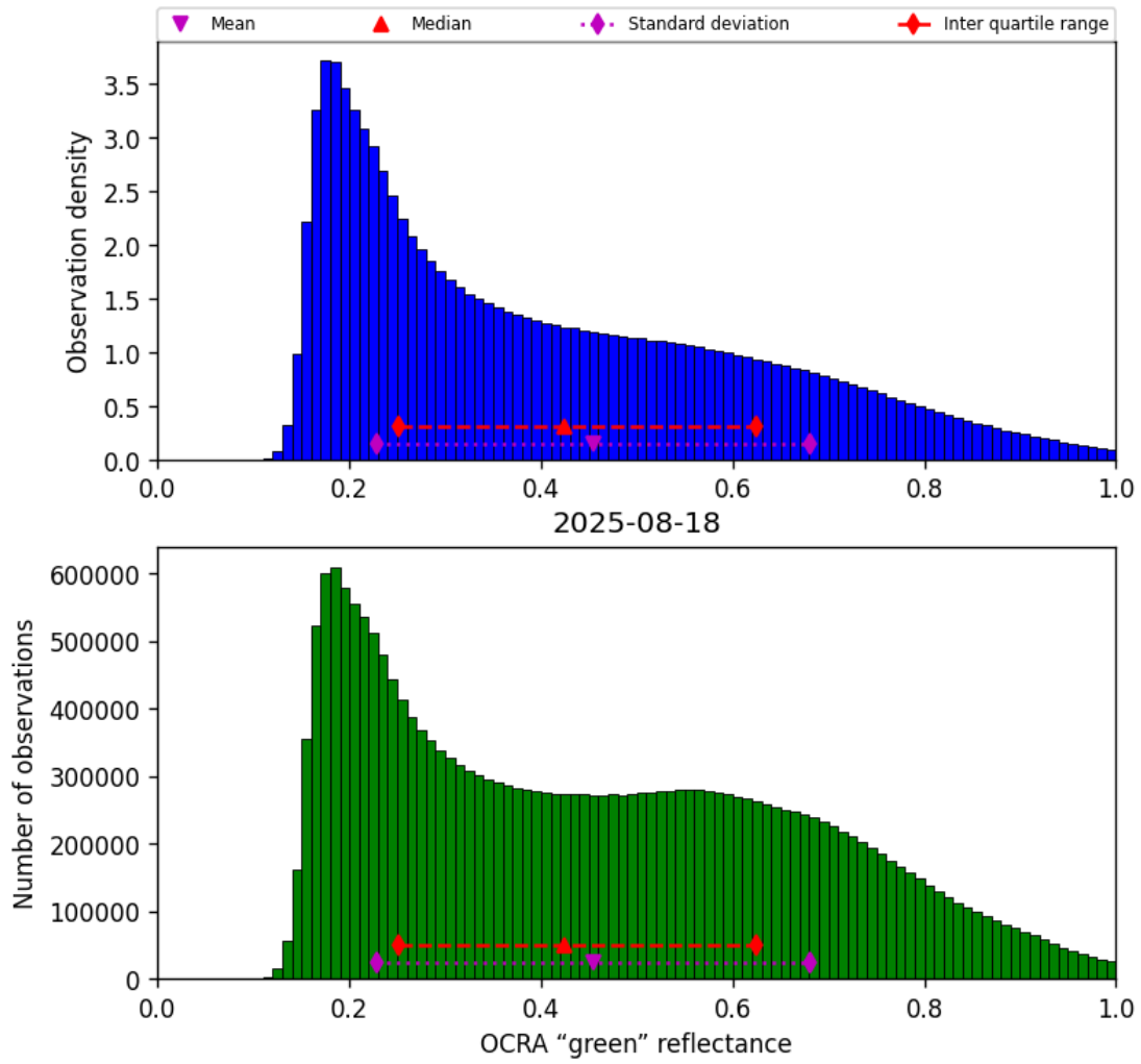
Figure 52: Histogram of “OCRA “green” reflectance” for 2025-08-17 to 2025-08-19
