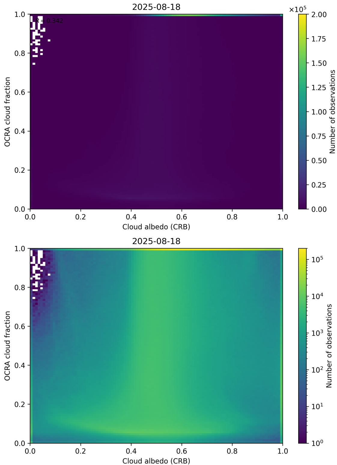
Figure 70: Scatter density plot of “Cloud albedo (CRB)” against “OCRA cloud fraction” for 2025-08-17 to 2025-08-19.
