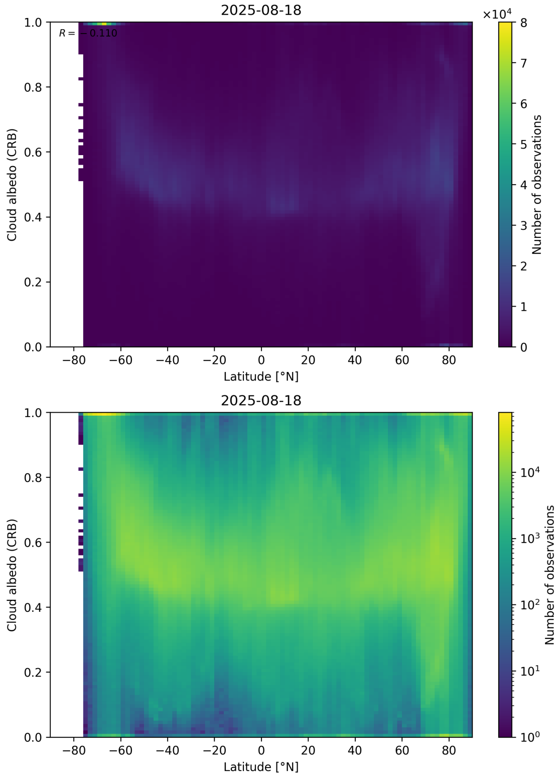
Figure 91: Scatter density plot of “Latitude” against “Cloud albedo (CRB)” for 2025-08-17 to 2025-08-19.
