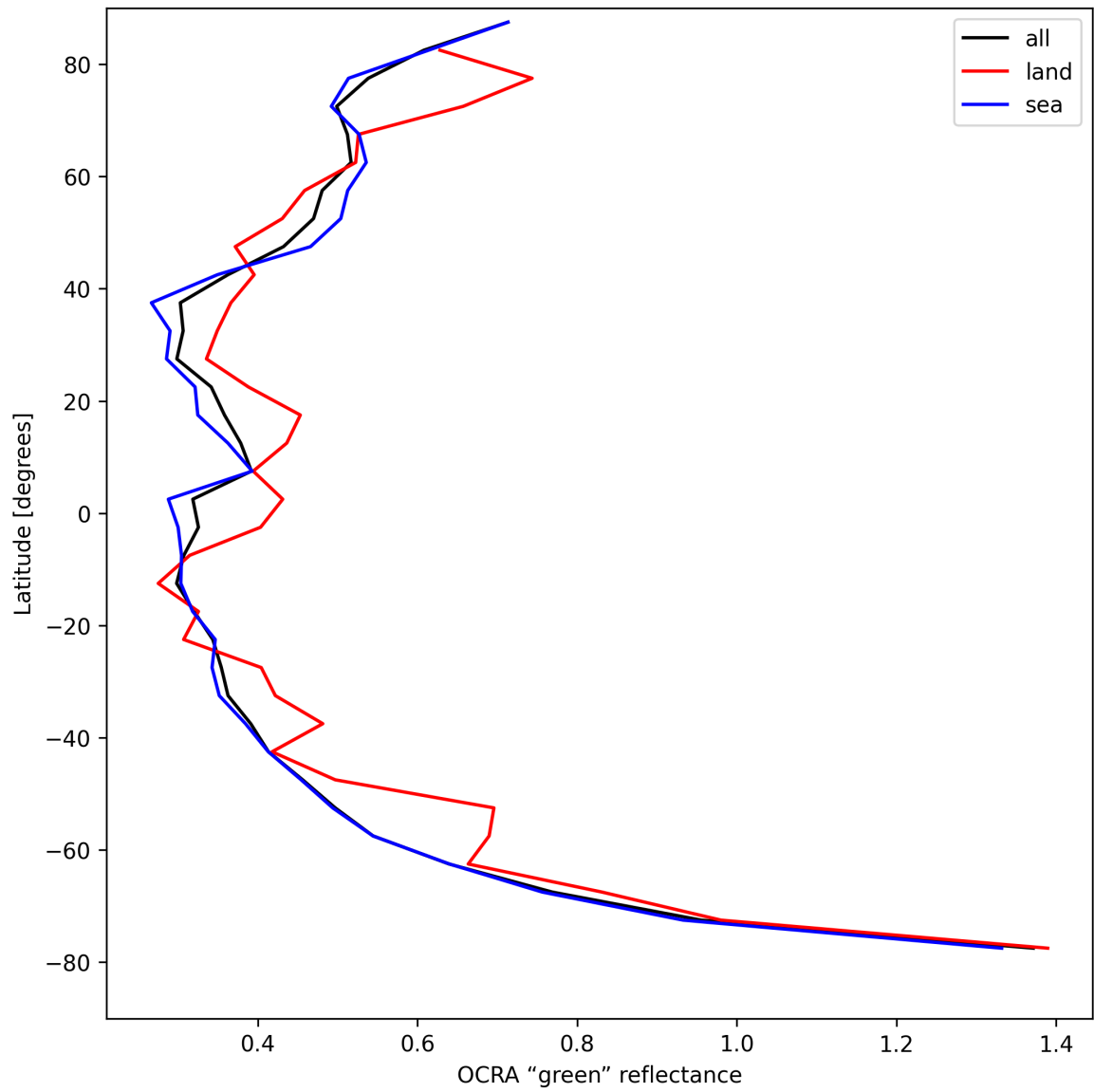
Figure 36: Zonal average of “OCRA “green” reflectance” for 2025-08-17 to 2025-08-19.
