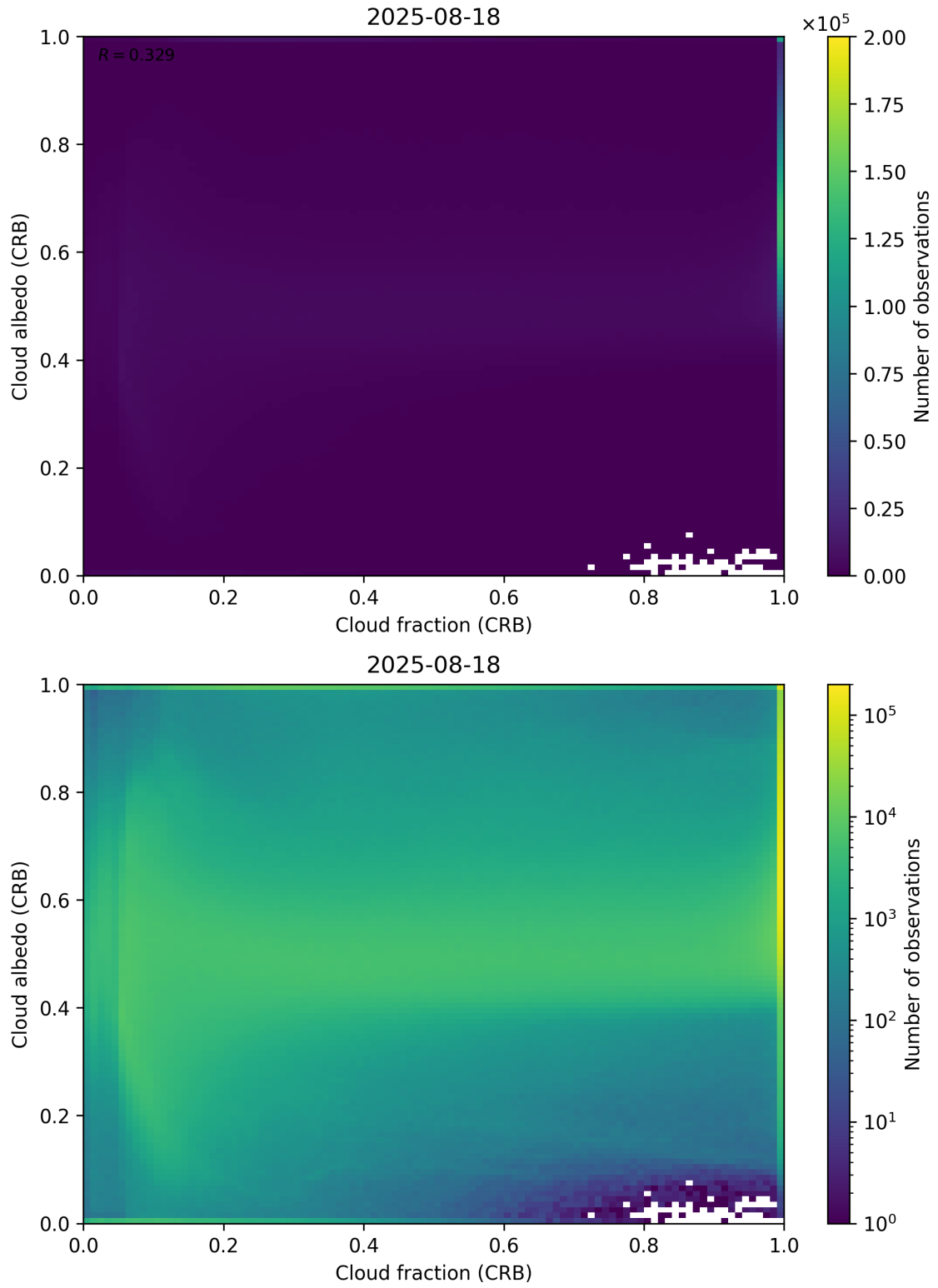
Figure 77: Scatter density plot of “Cloud fraction (CRB)” against “Cloud albedo (CRB)” for 2025-08-17 to 2025-08-19.
