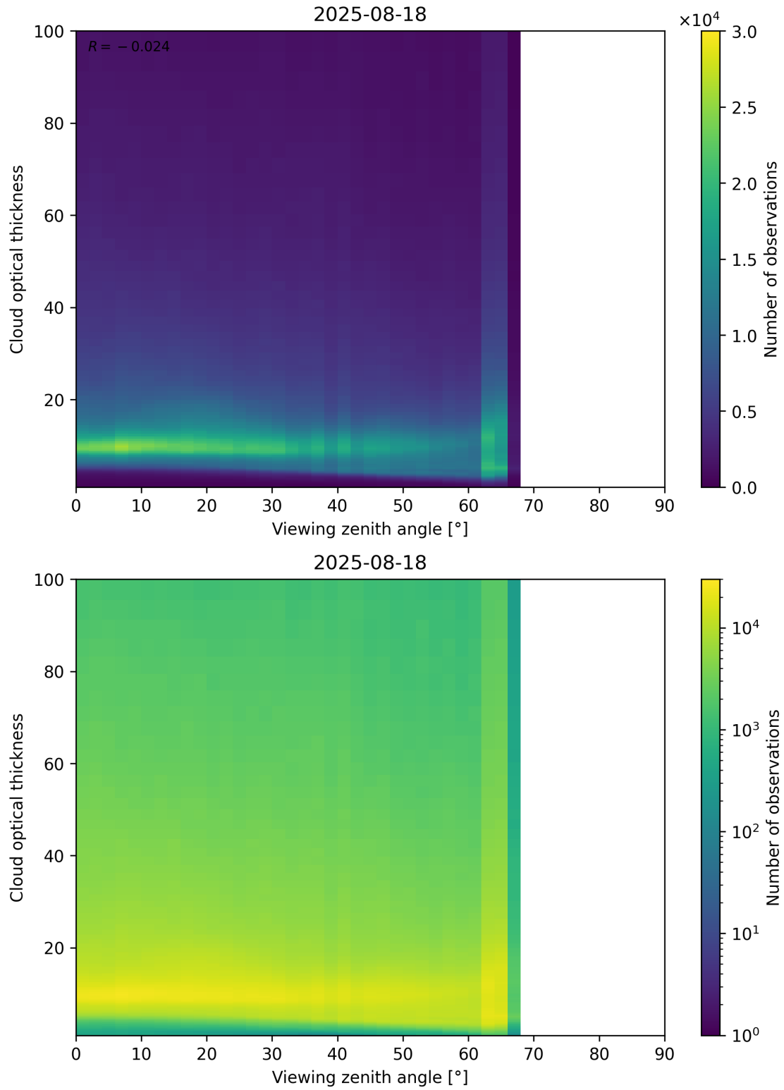
Figure 111: Scatter density plot of “Viewing zenith angle” against “Cloud optical thickness” for 2025-08-17 to 2025-08-19.
