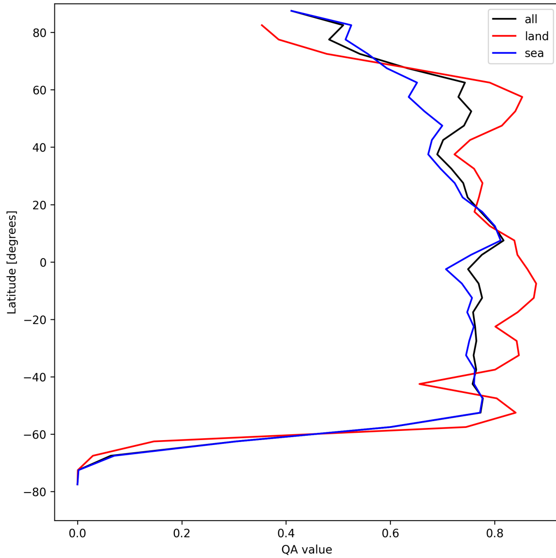
Figure 22: Zonal average of “QA value” for 2025-08-17 to 2025-08-19.
