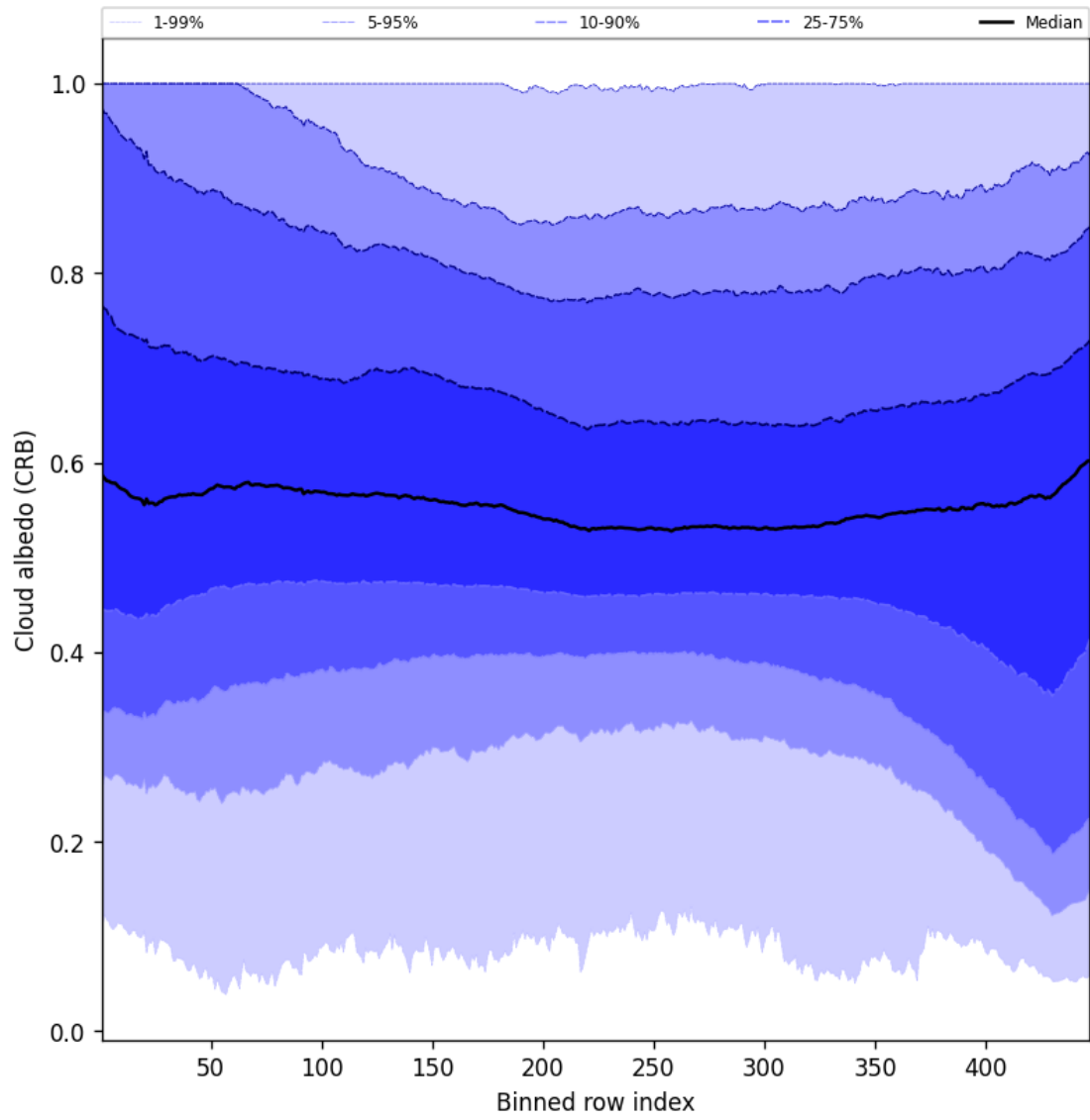
Figure 60: Along track statistics of “Cloud albedo (CRB)” for 2025-08-17 to 2025-08-19
