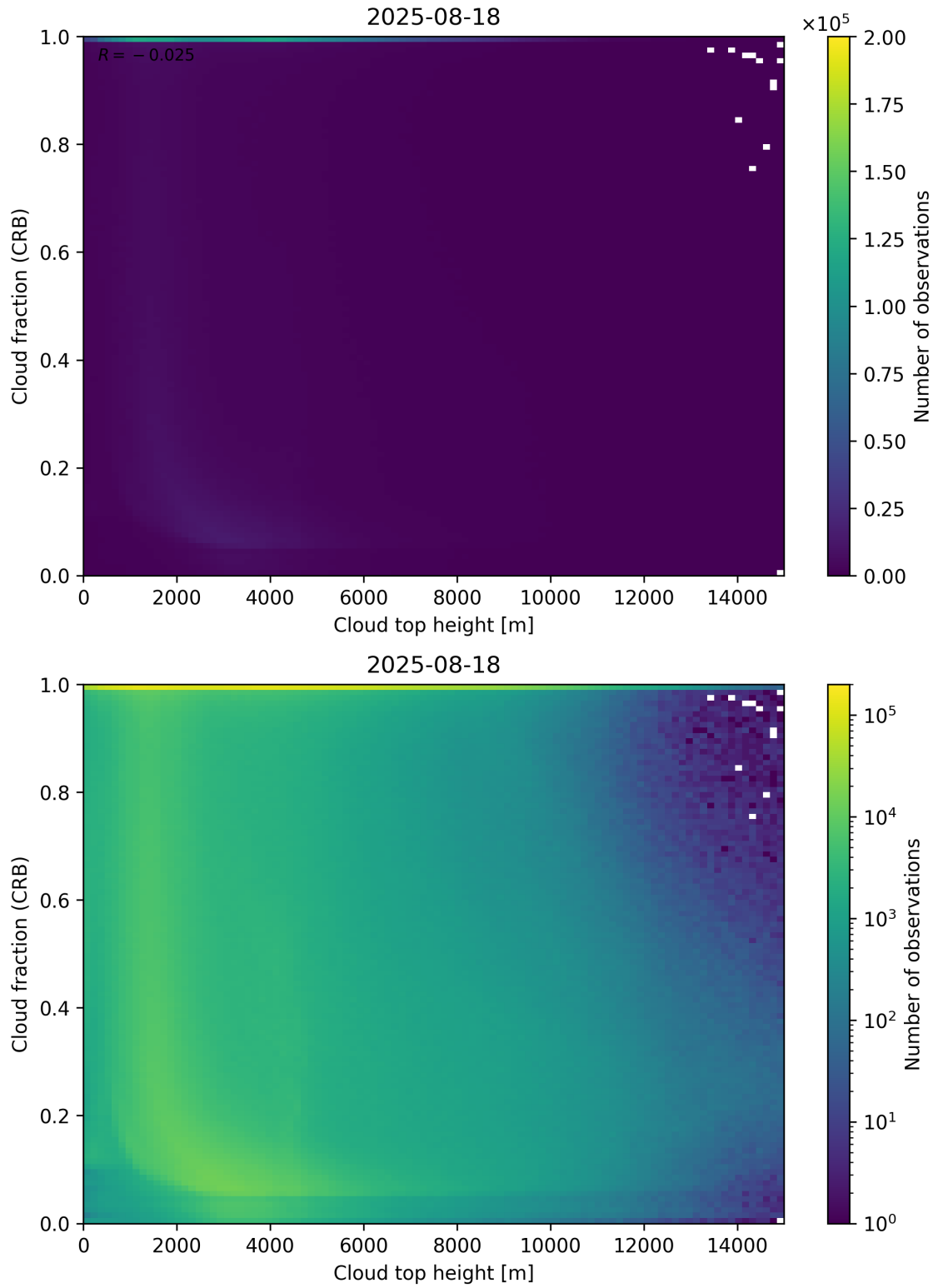
Figure 88: Scatter density plot of “Cloud top height” against “Cloud fraction (CRB)” for 2025-08-17 to 2025-08-19.
