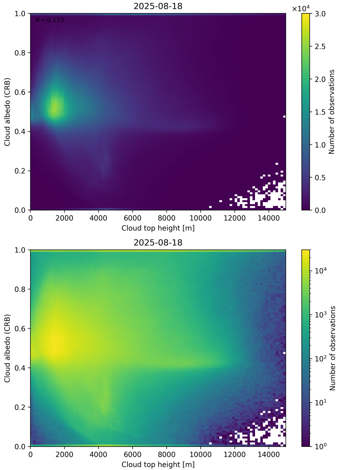
Figure 86: Scatter density plot of “Cloud top height” against “Cloud albedo (CRB)” for 2025-08-17 to 2025-08-19.
