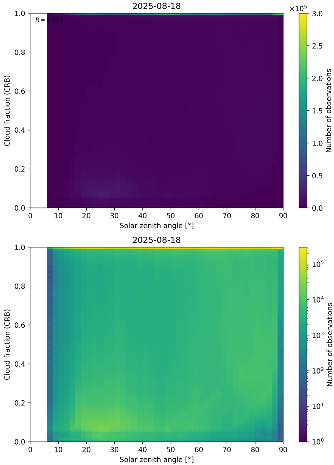
Figure 101: Scatter density plot of “Solar zenith angle” against “Cloud fraction (CRB)” for 2025-08-17 to 2025-08-19.
