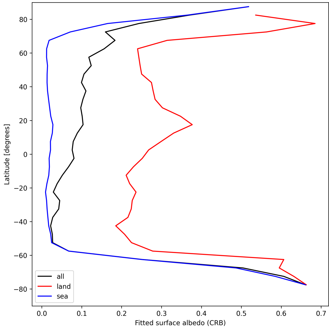
Figure 30: Zonal average of “Fitted surface albedo (CRB)” for 2025-08-17 to 2025-08-19.
