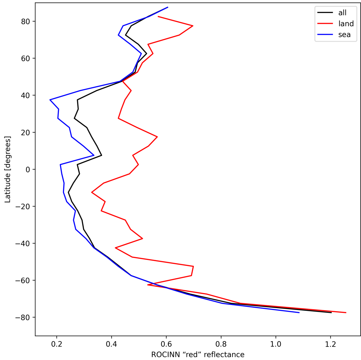
Figure 37: Zonal average of “ROCINN “red” reflectance” for 2025-08-17 to 2025-08-19.
