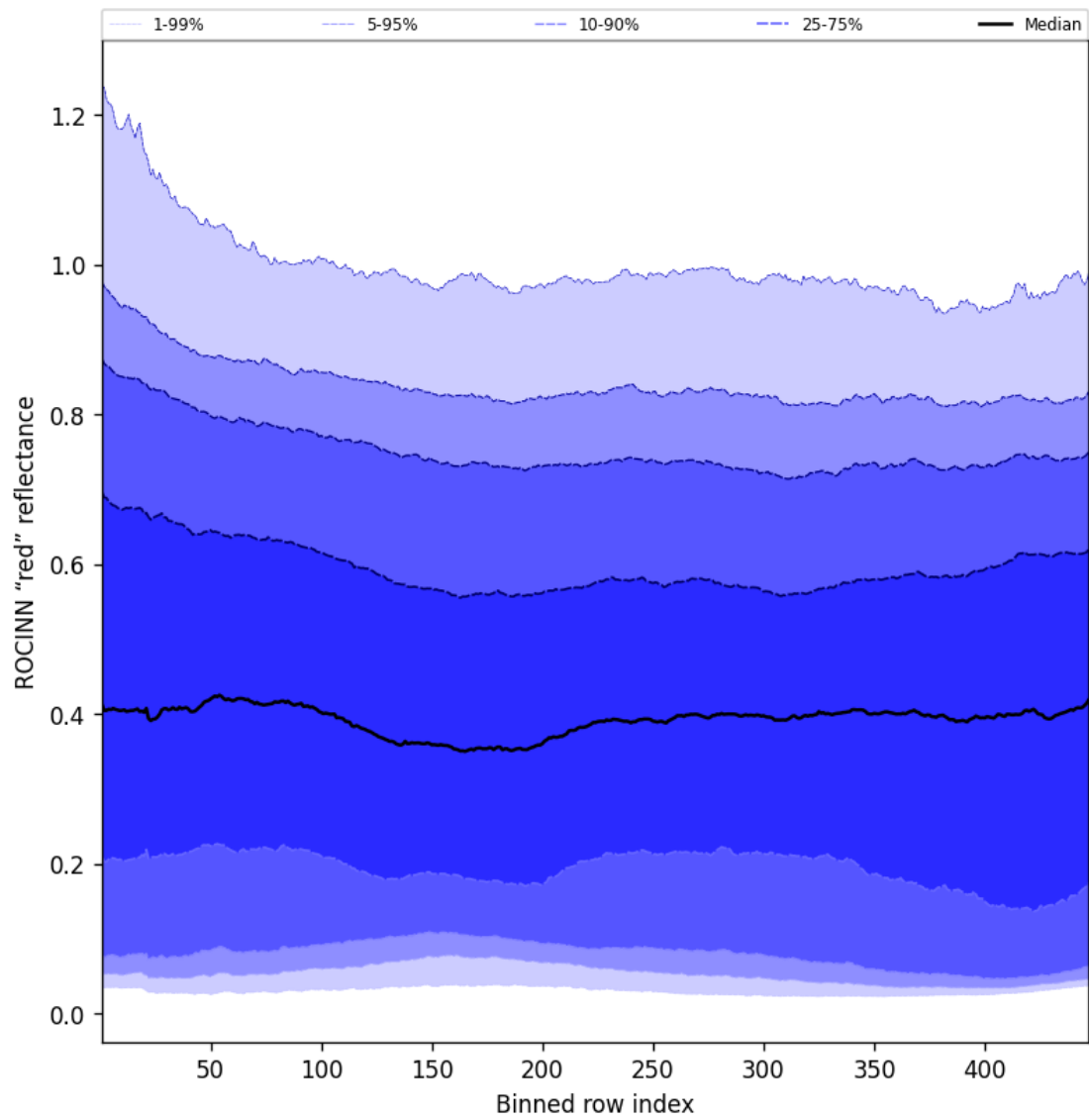
Figure 69: Along track statistics of “ROCINN “red” reflectance” for 2025-08-17 to 2025-08-19
