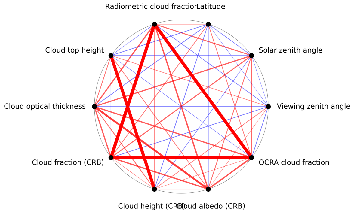
Figure 1: Map of correlation graph for 2025-08-17 to 2025-08-19.
