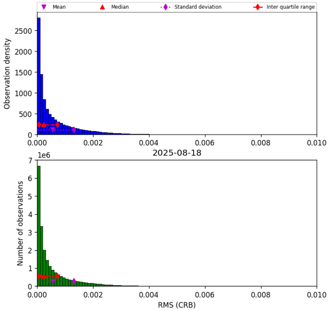
Figure 48: Histogram of “RMS (CRB)” for 2025-08-17 to 2025-08-19
