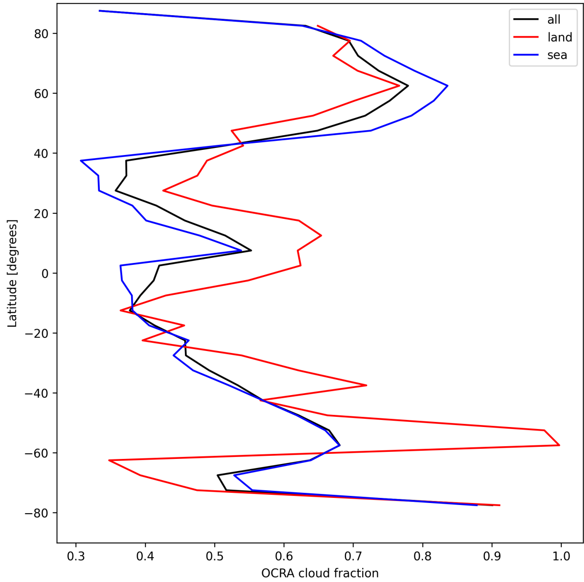
Figure 34: Zonal average of “OCRA cloud fraction” for 2025-08-17 to 2025-08-19.
