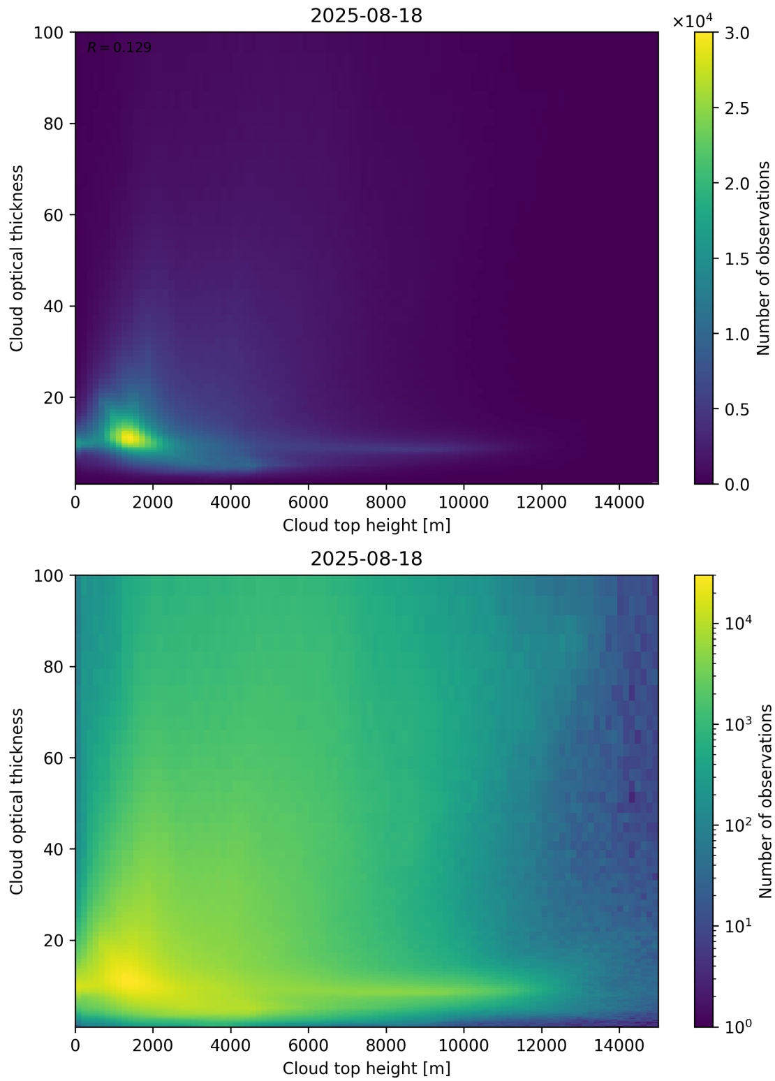
Figure 90: Scatter density plot of “Cloud top height” against “Cloud optical thickness” for 2025-08-17 to 2025-08-19.
