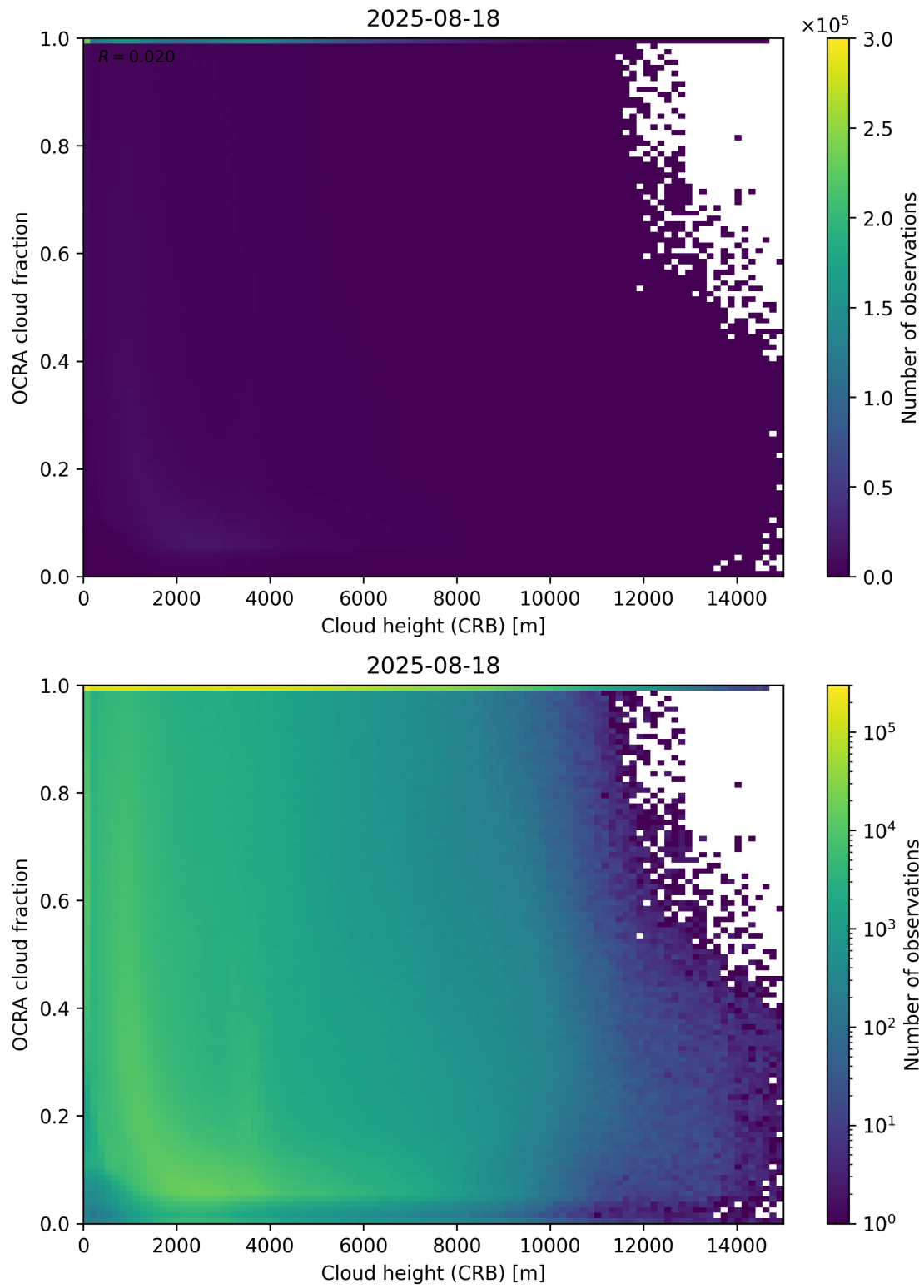
Figure 81: Scatter density plot of “Cloud height (CRB)” against “OCRA cloud fraction” for 2025-08-17 to 2025-08-19.
