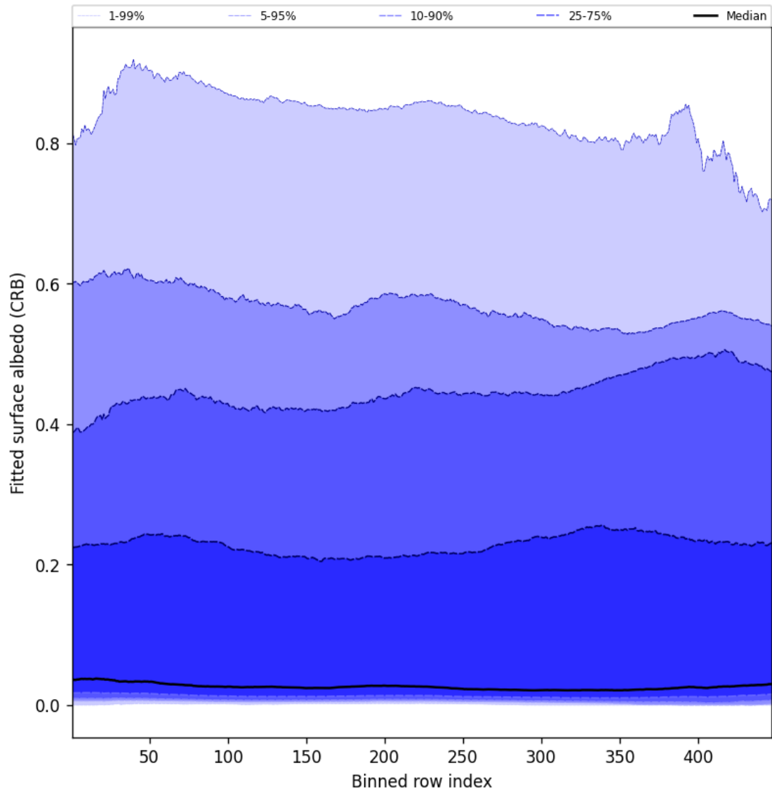
Figure 62: Along track statistics of “Fitted surface albedo (CRB)” for 2025-08-17 to 2025-08-19
