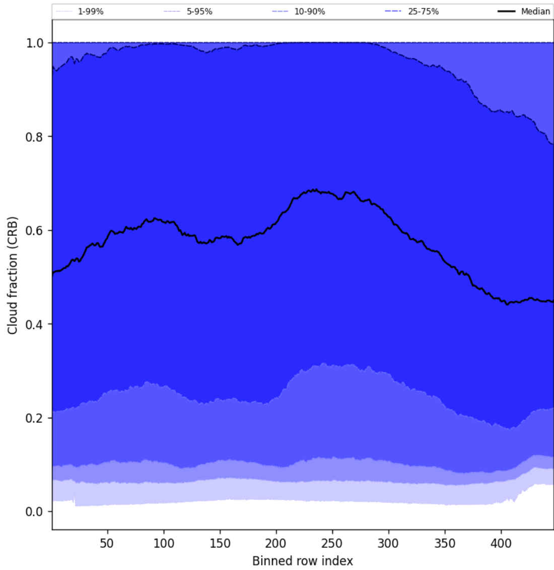
Figure 58: Along track statistics of “Cloud fraction (CRB)” for 2025-08-17 to 2025-08-19
