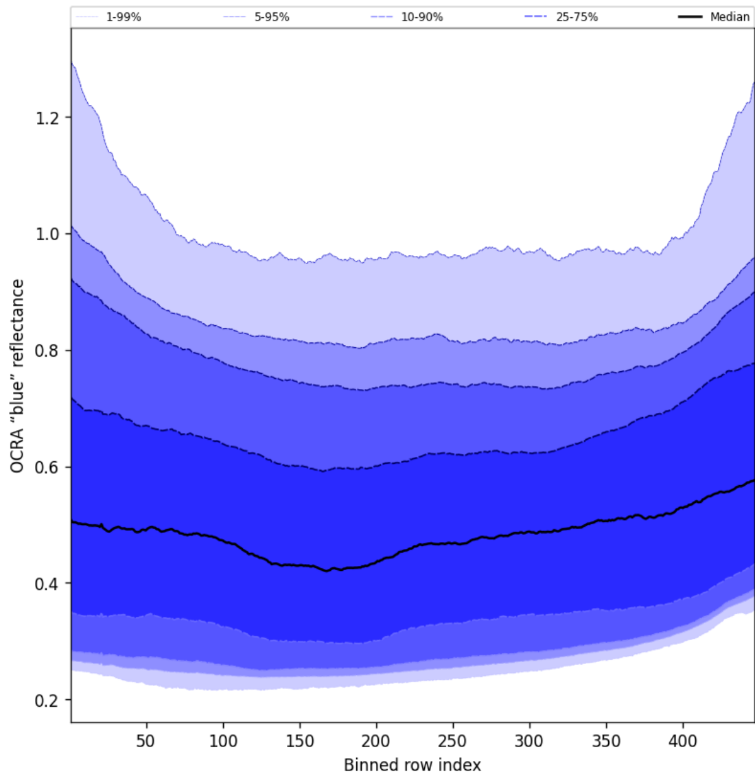
Figure 67: Along track statistics of “OCRA “blue” reflectance” for 2025-08-17 to 2025-08-19
