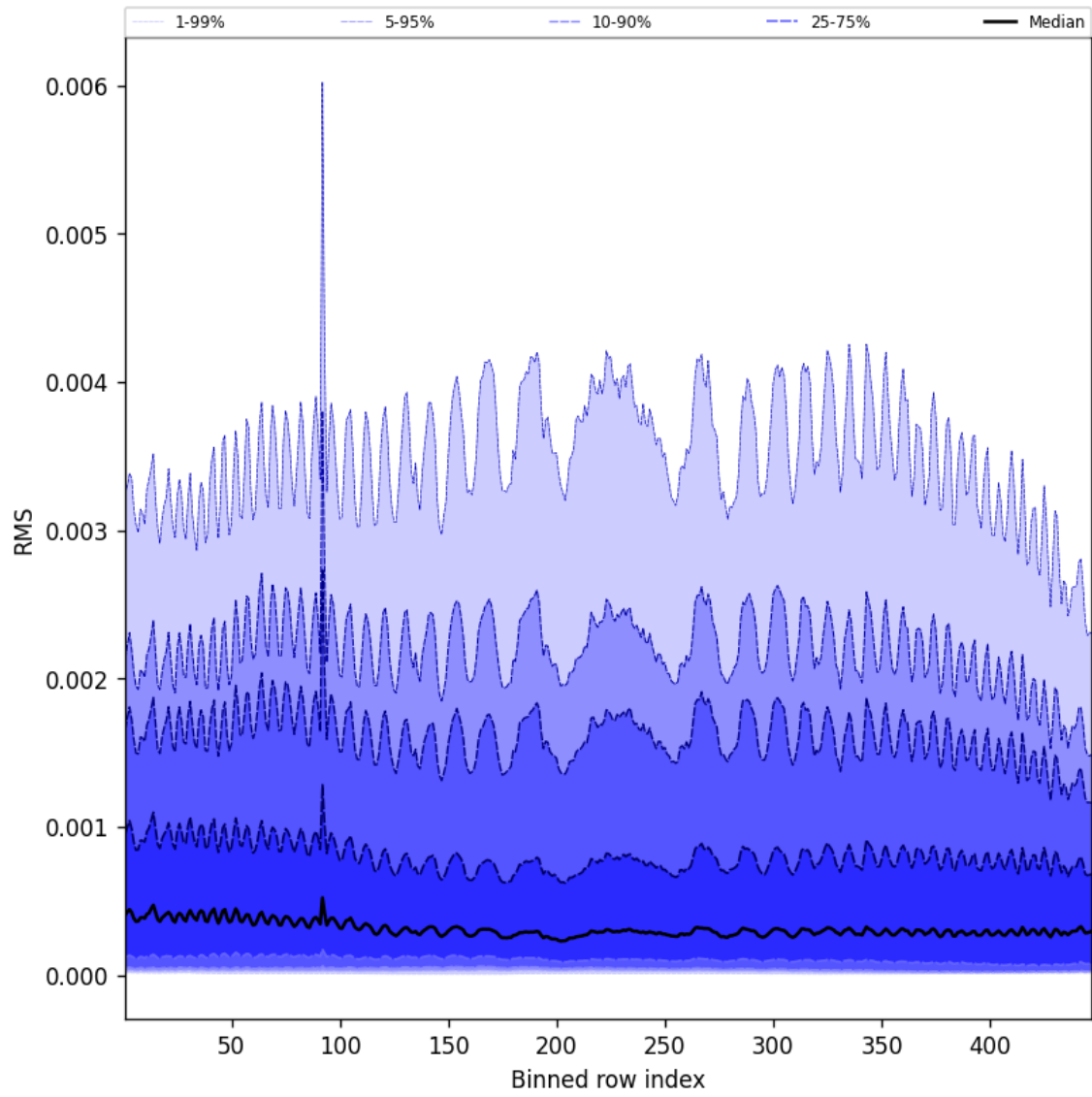
Figure 63: Along track statistics of “RMS” for 2025-08-17 to 2025-08-19
