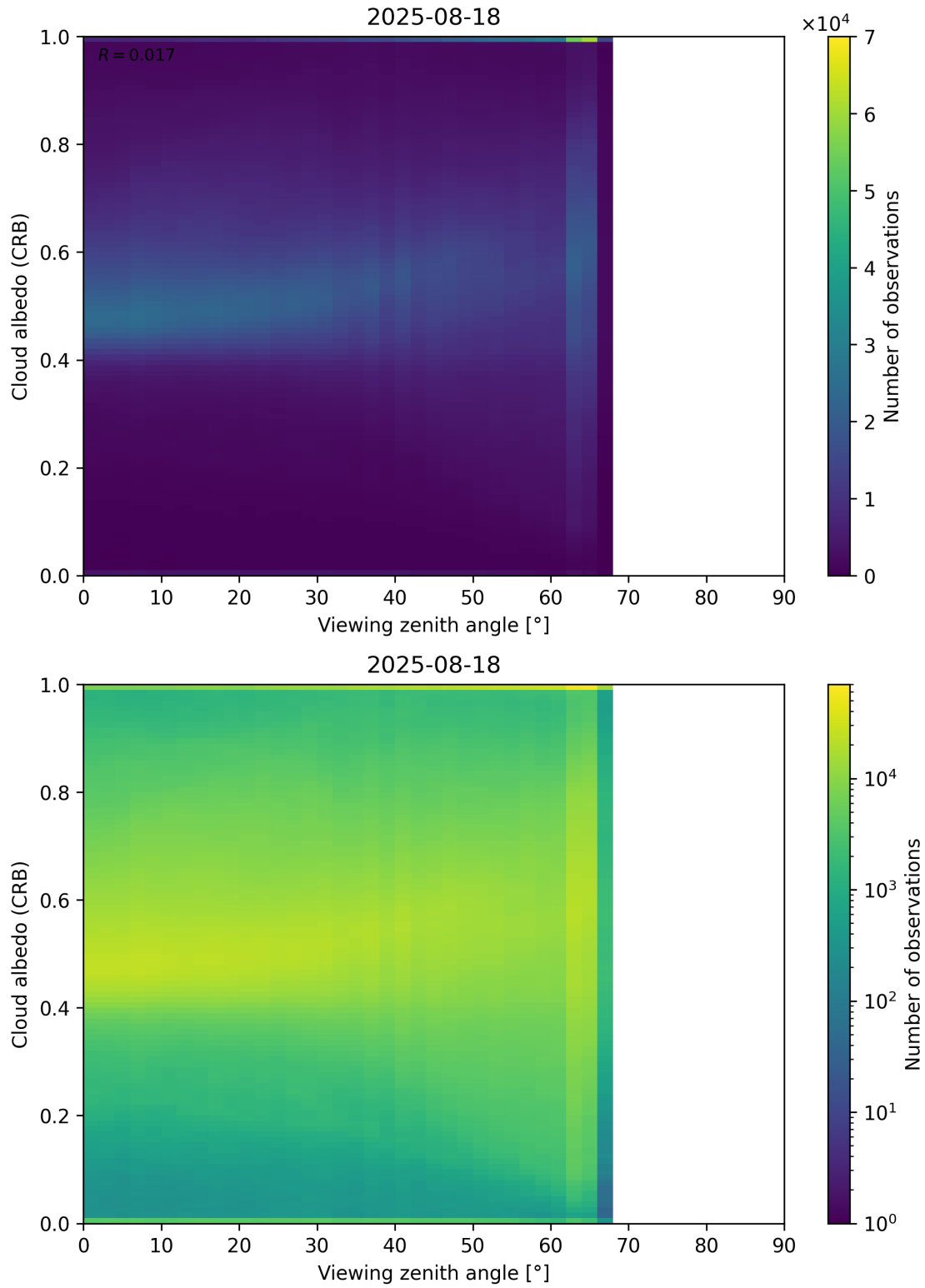
Figure 106: Scatter density plot of “Viewing zenith angle” against “Cloud albedo (CRB)” for 2025-08-17 to 2025-08-19.
