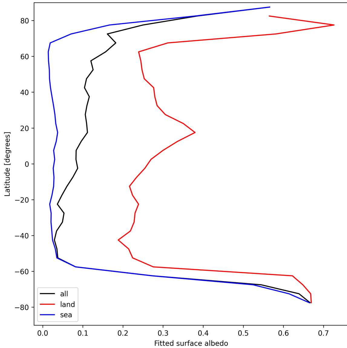
Figure 29: Zonal average of “Fitted surface albedo” for 2025-08-17 to 2025-08-19.
