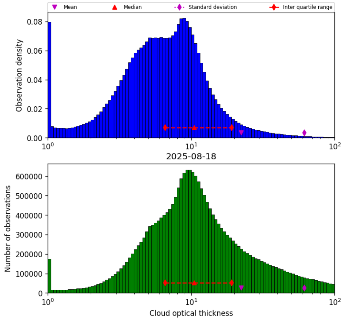
Figure 41: Histogram of “Cloud optical thickness” for 2025-08-17 to 2025-08-19
