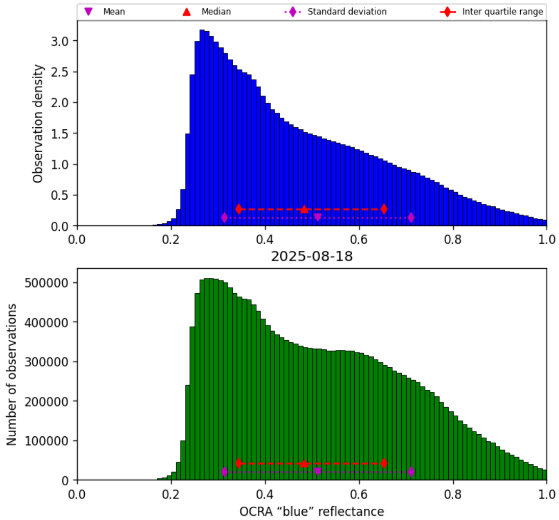
Figure 51: Histogram of “OCRA “blue” reflectance” for 2025-08-17 to 2025-08-19
