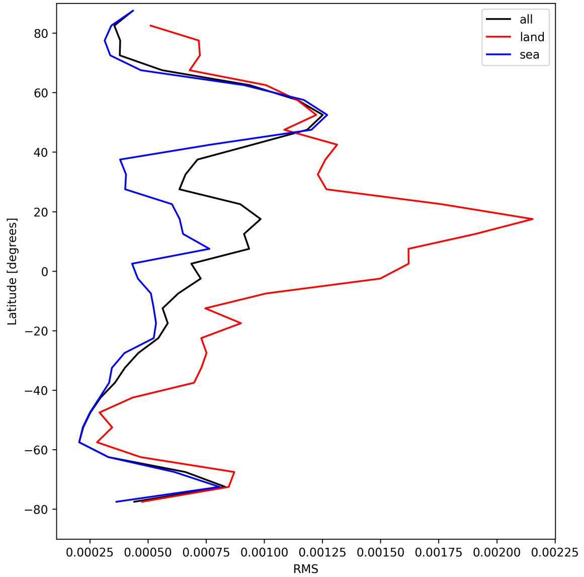
Figure 31: Zonal average of “RMS” for 2025-08-17 to 2025-08-19.
