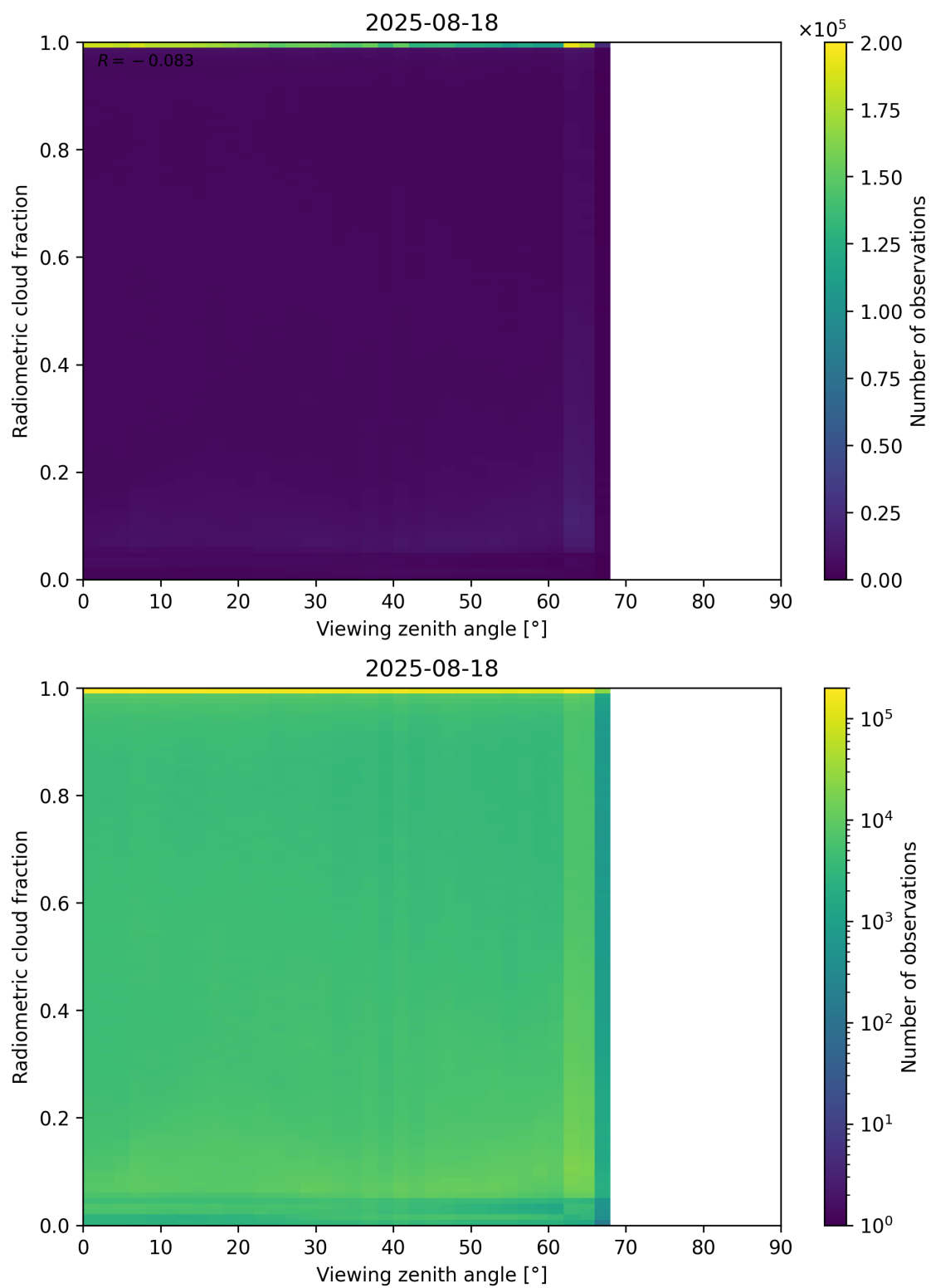
Figure 107: Scatter density plot of “Viewing zenith angle” against “Radiometric cloud fraction” for 2025-08-17 to 2025-08-19.
