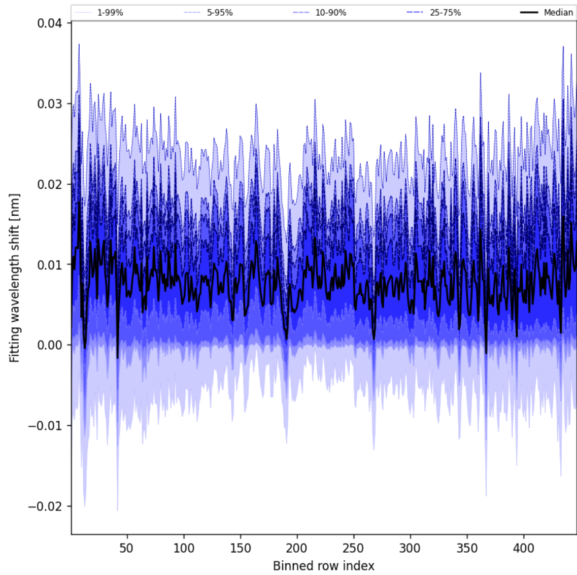
Figure 65: Along track statistics of “Fitting wavelength shift” for 2025-08-17 to 2025-08-19
