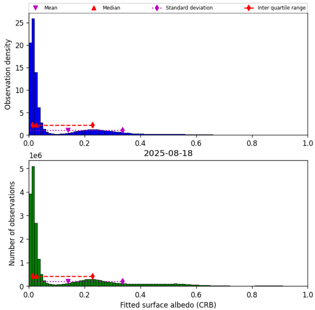
Figure 46: Histogram of “Fitted surface albedo (CRB)” for 2025-08-17 to 2025-08-19
