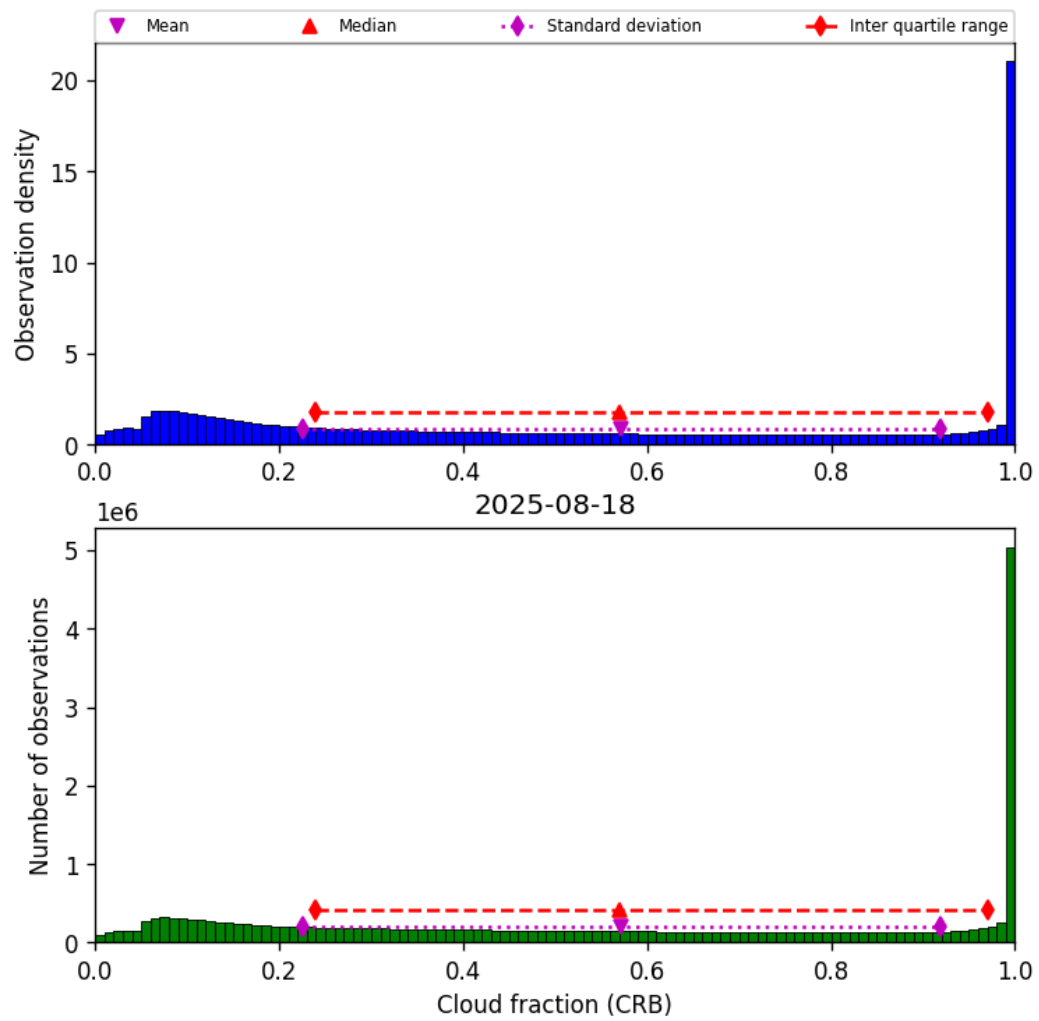
Figure 42: Histogram of “Cloud fraction (CRB)” for 2025-08-17 to 2025-08-19
