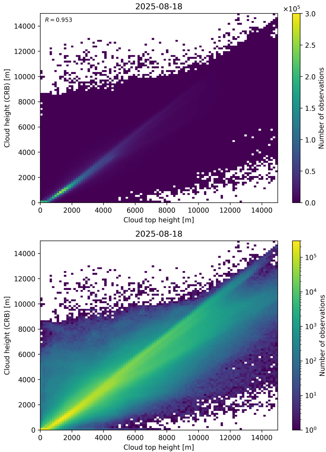
Figure 89: Scatter density plot of “Cloud top height” against “Cloud height (CRB)” for 2025-08-17 to 2025-08-19.
