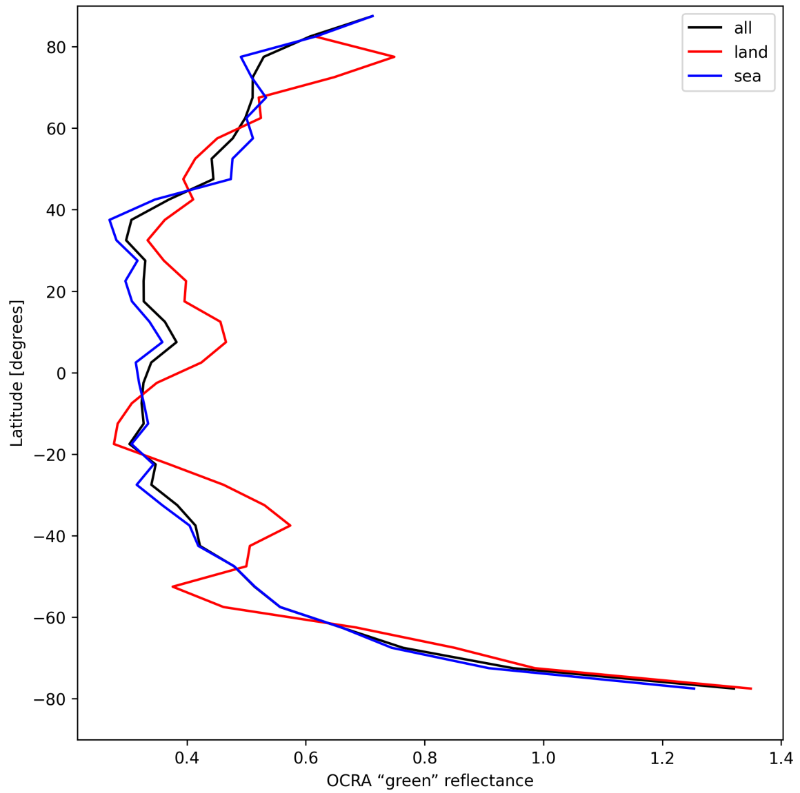
Figure 36: Zonal average of “OCRA “green” reflectance” for 2025-08-19 to 2025-08-20.
