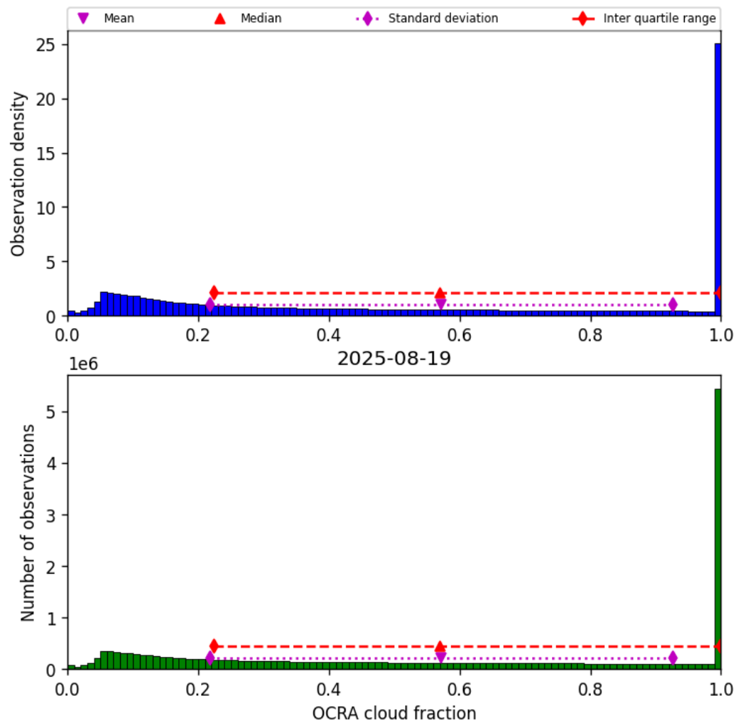
Figure 50: Histogram of “OCRA cloud fraction” for 2025-08-19 to 2025-08-20
