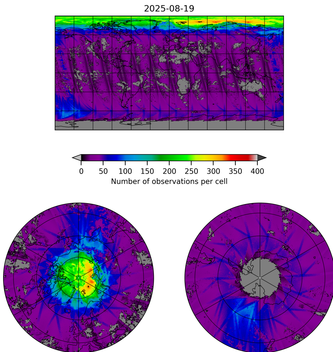
Figure 21: Map of the number of observations for 2025-08-19 to 2025-08-20
