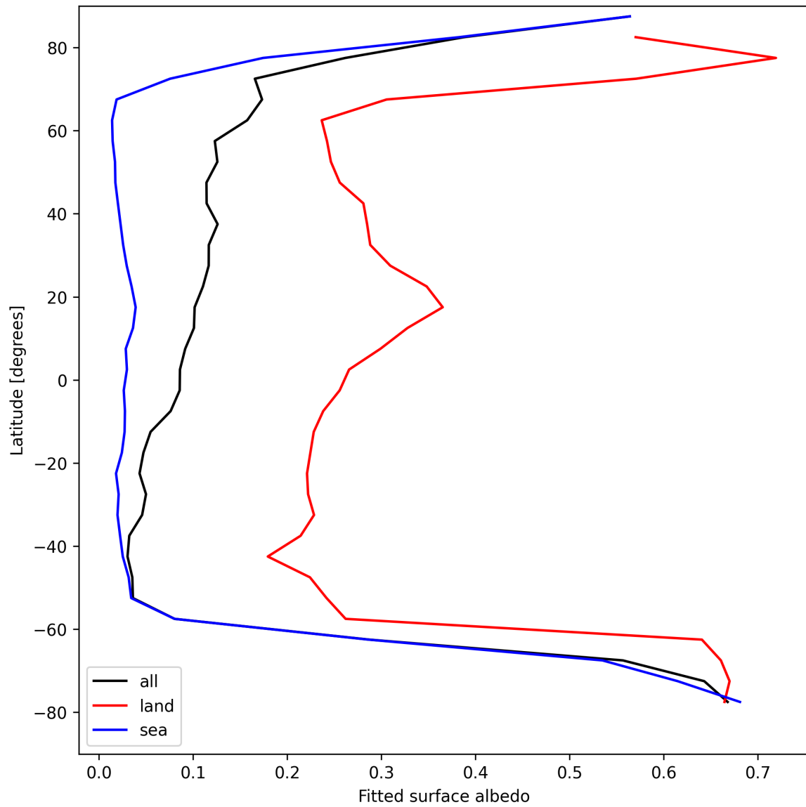
Figure 29: Zonal average of “Fitted surface albedo” for 2025-08-19 to 2025-08-20.
