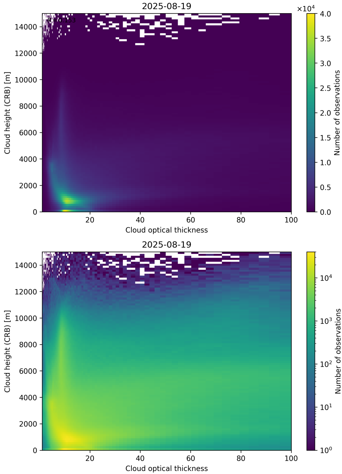
Figure 85: Scatter density plot of “Cloud optical thickness” against “Cloud height (CRB)” for 2025-08-19 to 2025-08-20.
