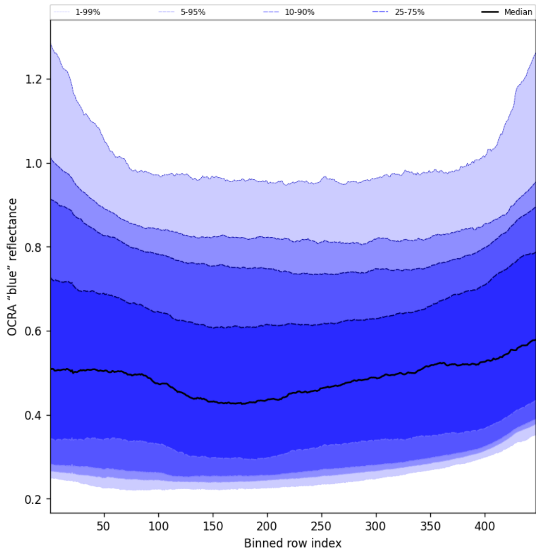
Figure 67: Along track statistics of “OCRA “blue” reflectance” for 2025-08-19 to 2025-08-20
