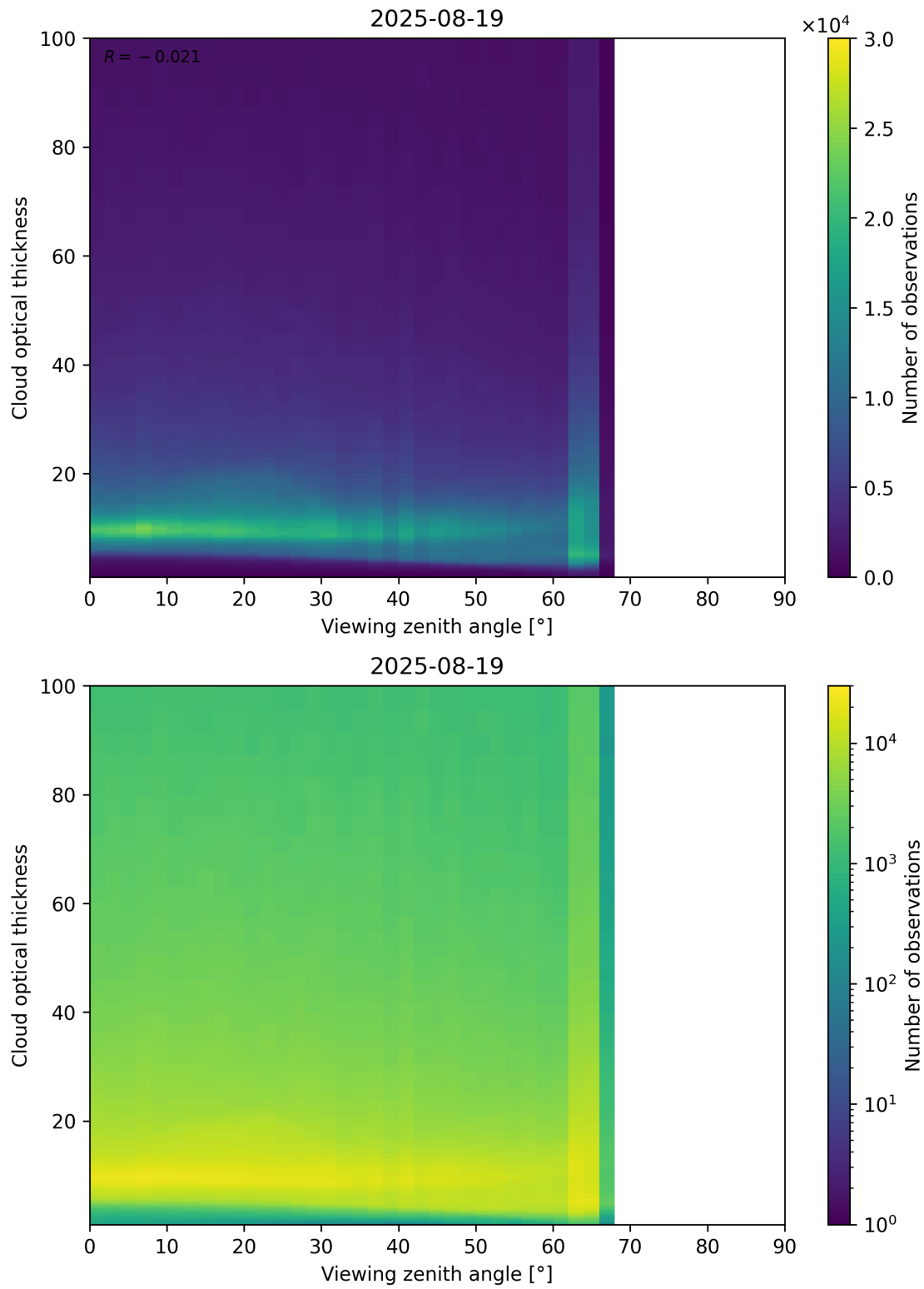
Figure 111: Scatter density plot of “Viewing zenith angle” against “Cloud optical thickness” for 2025-08-19 to 2025-08-20.
