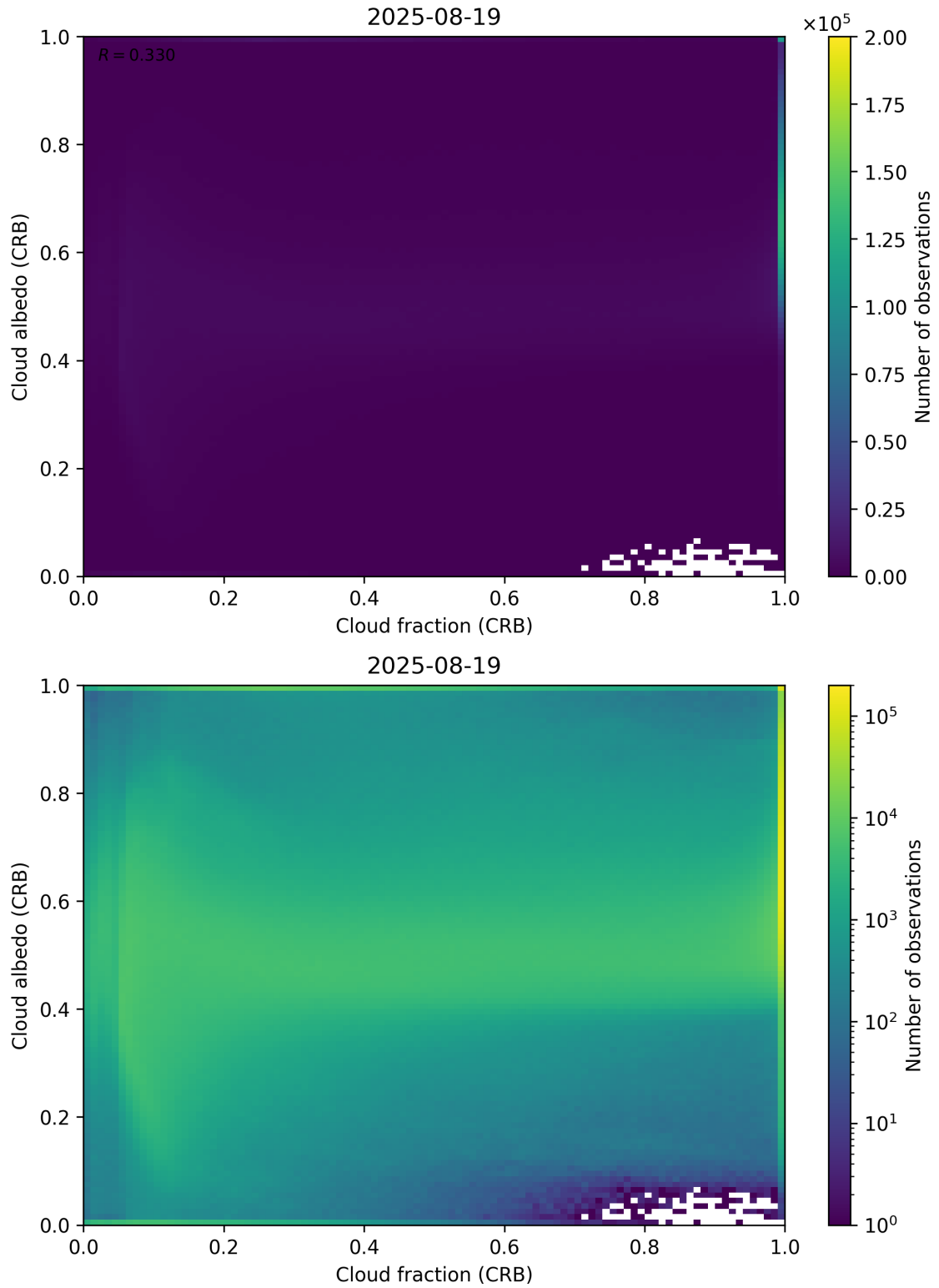
Figure 77: Scatter density plot of “Cloud fraction (CRB)” against “Cloud albedo (CRB)” for 2025-08-19 to 2025-08-20.
