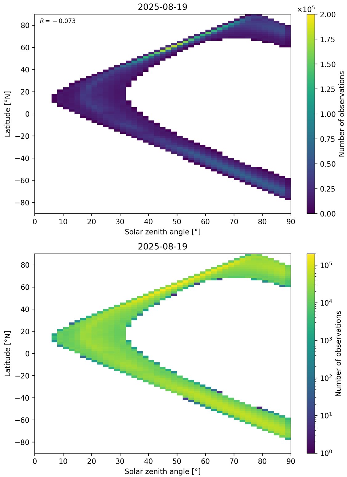
Figure 105: Scatter density plot of “Solar zenith angle” against “Latitude” for 2025-08-19 to 2025-08-20.
