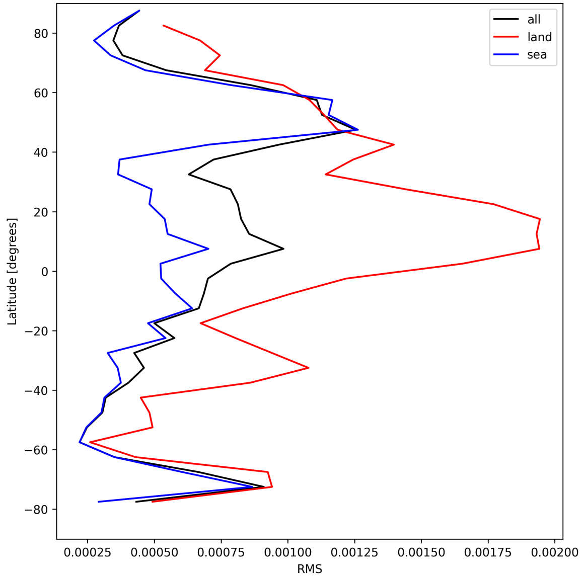
Figure 31: Zonal average of “RMS” for 2025-08-19 to 2025-08-20.
