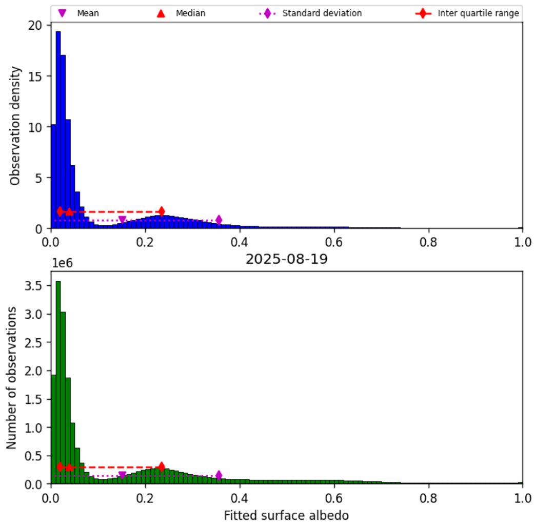
Figure 45: Histogram of “Fitted surface albedo” for 2025-08-19 to 2025-08-20
