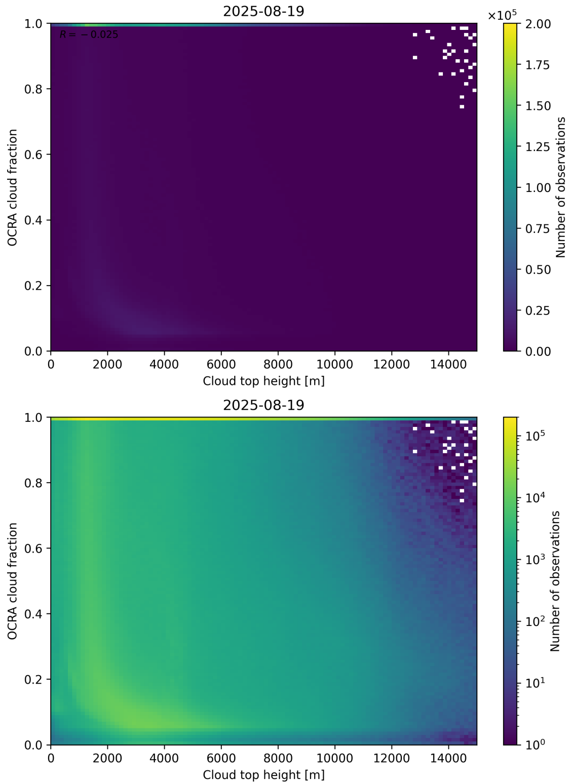
Figure 87: Scatter density plot of “Cloud top height” against “OCRA cloud fraction” for 2025-08-19 to 2025-08-20.
