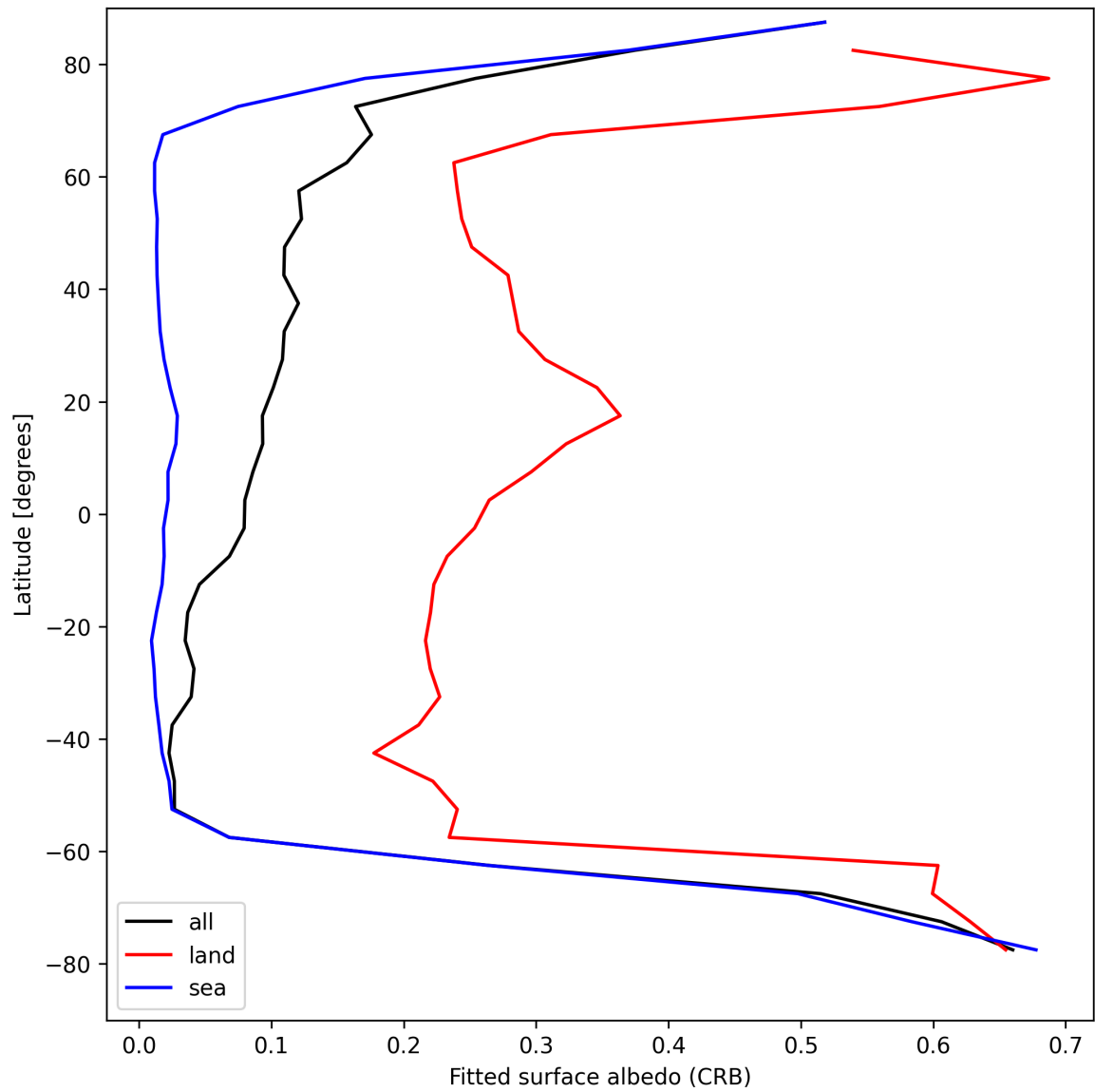
Figure 30: Zonal average of “Fitted surface albedo (CRB)” for 2025-08-19 to 2025-08-20.
