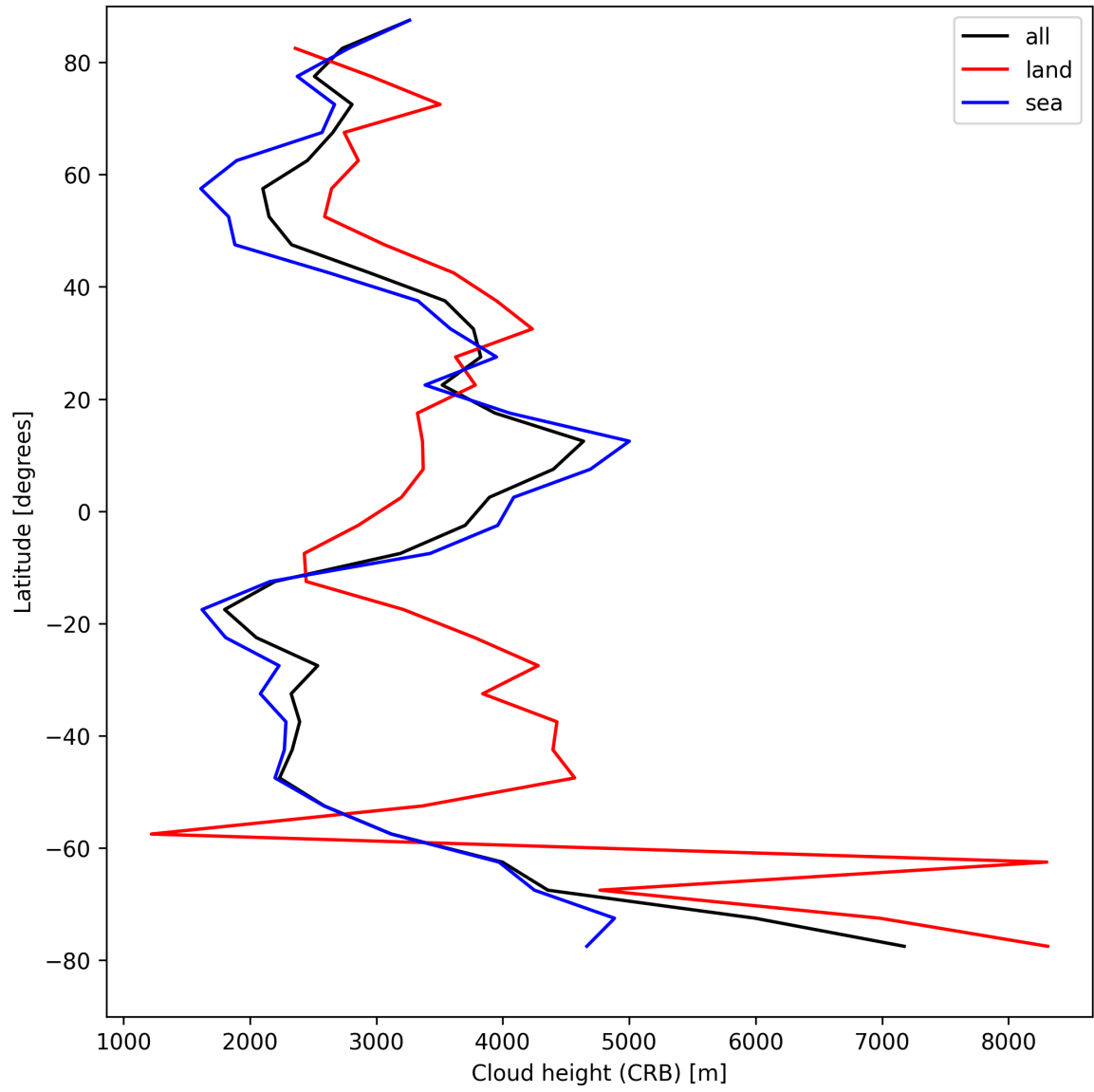
Figure 27: Zonal average of “Cloud height (CRB)” for 2025-08-19 to 2025-08-20.
