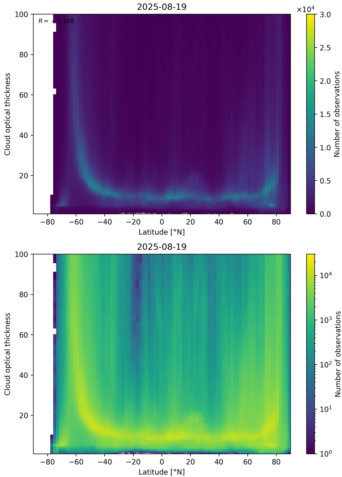
Figure 96: Scatter density plot of “Latitude” against “Cloud optical thickness” for 2025-08-19 to 2025-08-20.
