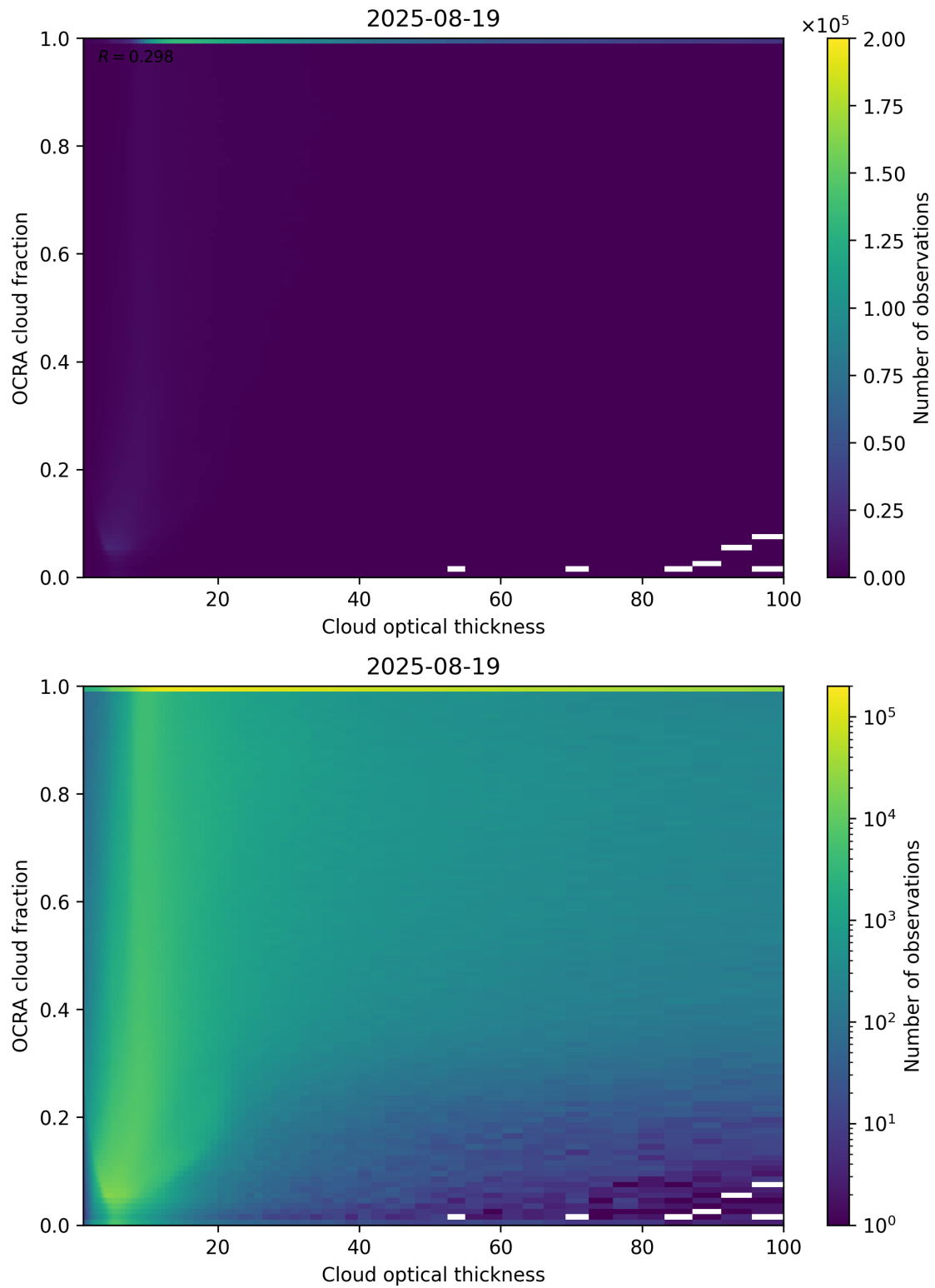
Figure 83: Scatter density plot of “Cloud optical thickness” against “OCRA cloud fraction” for 2025-08-19 to 2025-08-20.
