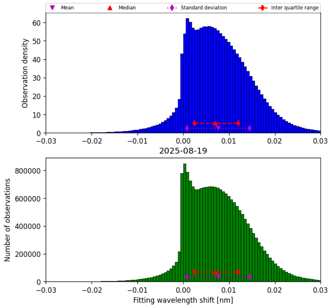
Figure 49: Histogram of “Fitting wavelength shift” for 2025-08-19 to 2025-08-20
