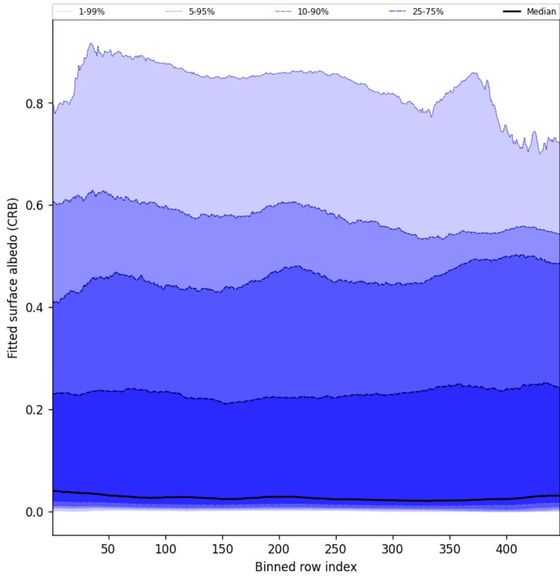
Figure 62: Along track statistics of “Fitted surface albedo (CRB)” for 2025-08-19 to 2025-08-20
