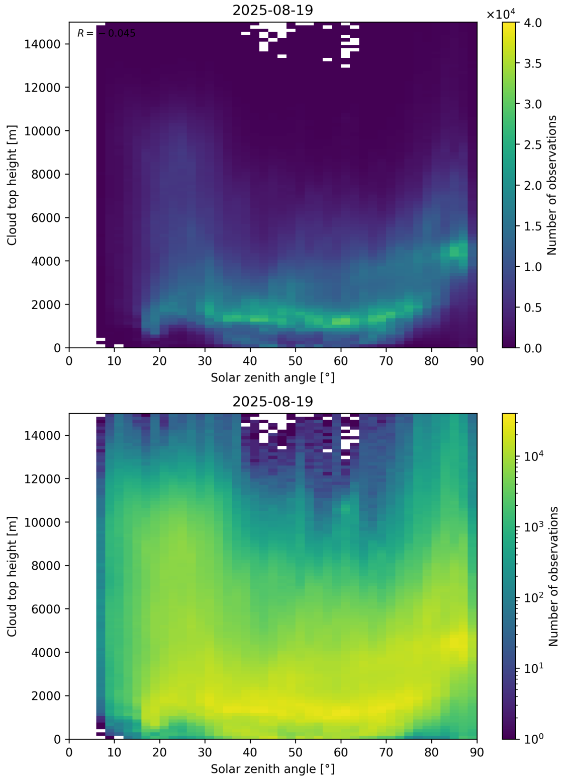
Figure 104: Scatter density plot of “Solar zenith angle” against “Cloud top height” for 2025-08-19 to 2025-08-20.
