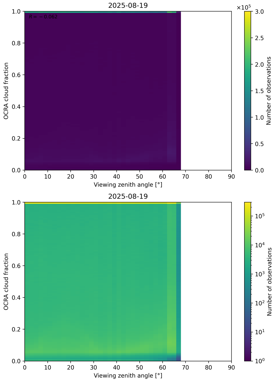
Figure 108: Scatter density plot of “Viewing zenith angle” against “OCRA cloud fraction” for 2025-08-19 to 2025-08-20.
