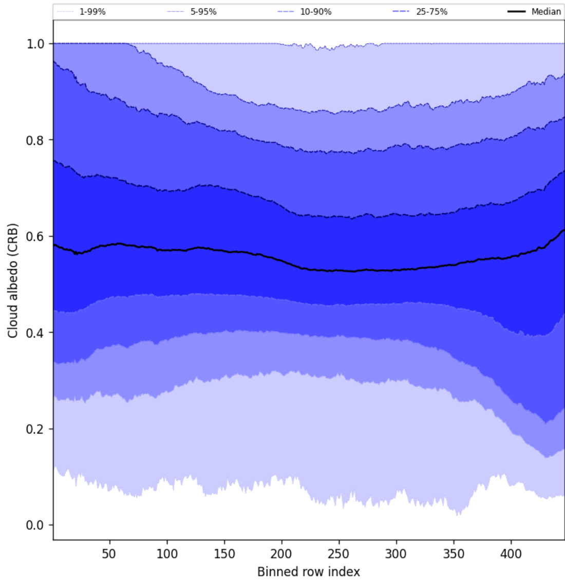
Figure 60: Along track statistics of “Cloud albedo (CRB)” for 2025-08-19 to 2025-08-20
