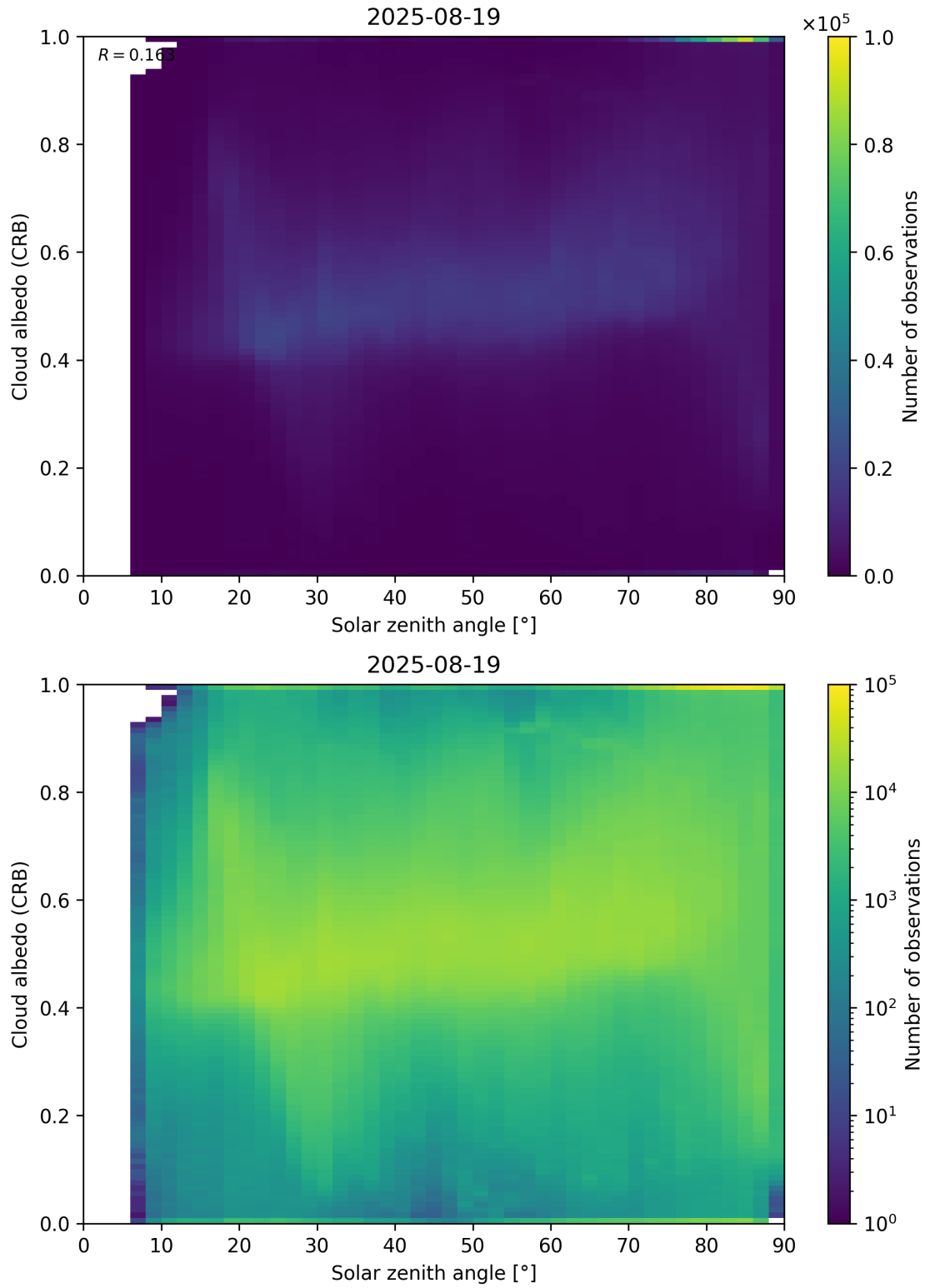
Figure 98: Scatter density plot of “Solar zenith angle” against “Cloud albedo (CRB)” for 2025-08-19 to 2025-08-20.
