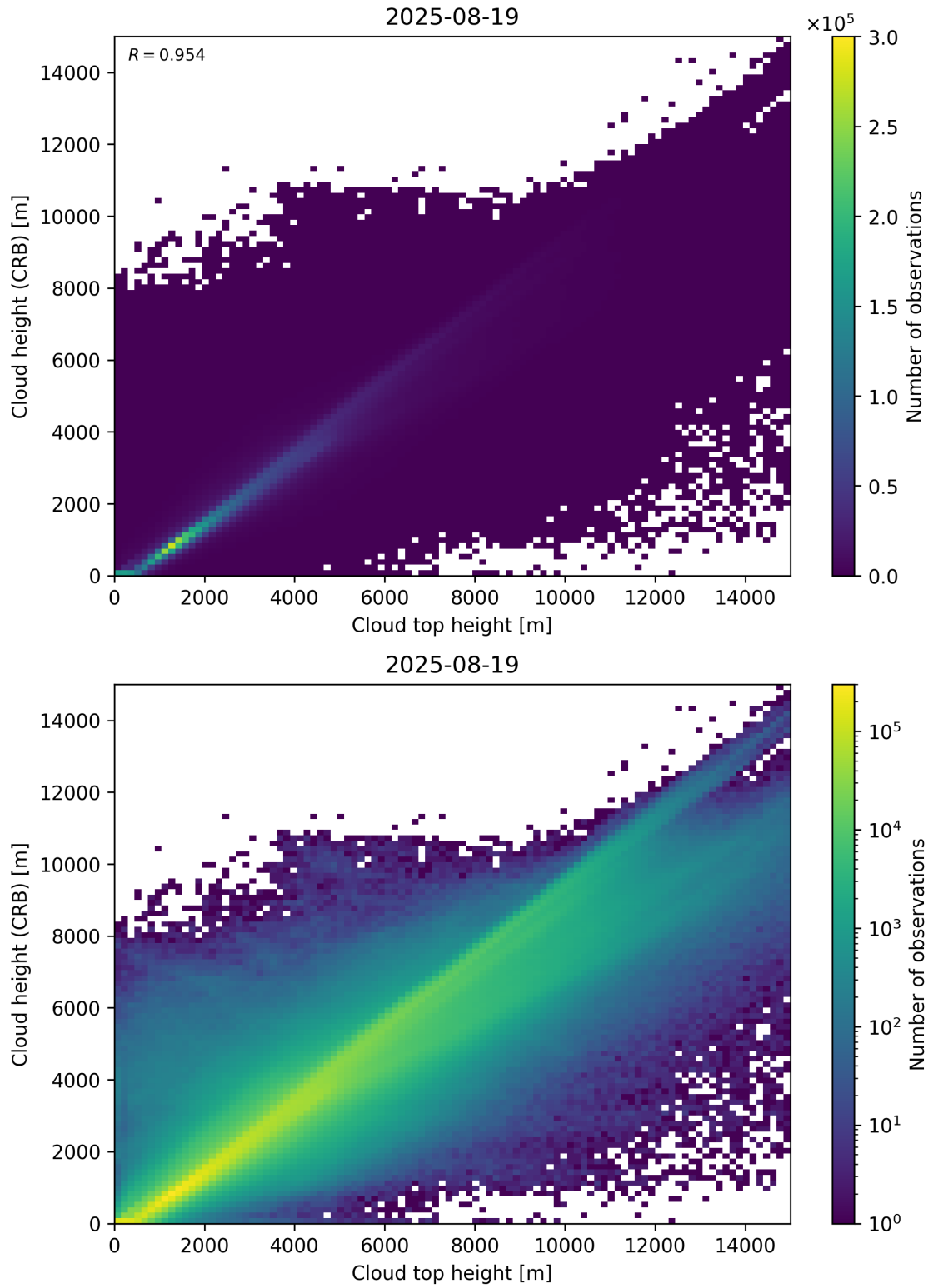
Figure 89: Scatter density plot of “Cloud top height” against “Cloud height (CRB)” for 2025-08-19 to 2025-08-20.
