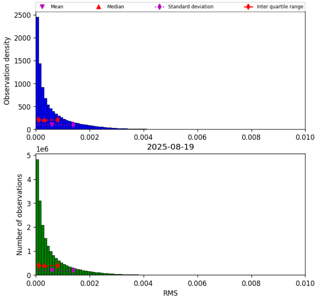
Figure 47: Histogram of “RMS” for 2025-08-19 to 2025-08-20
