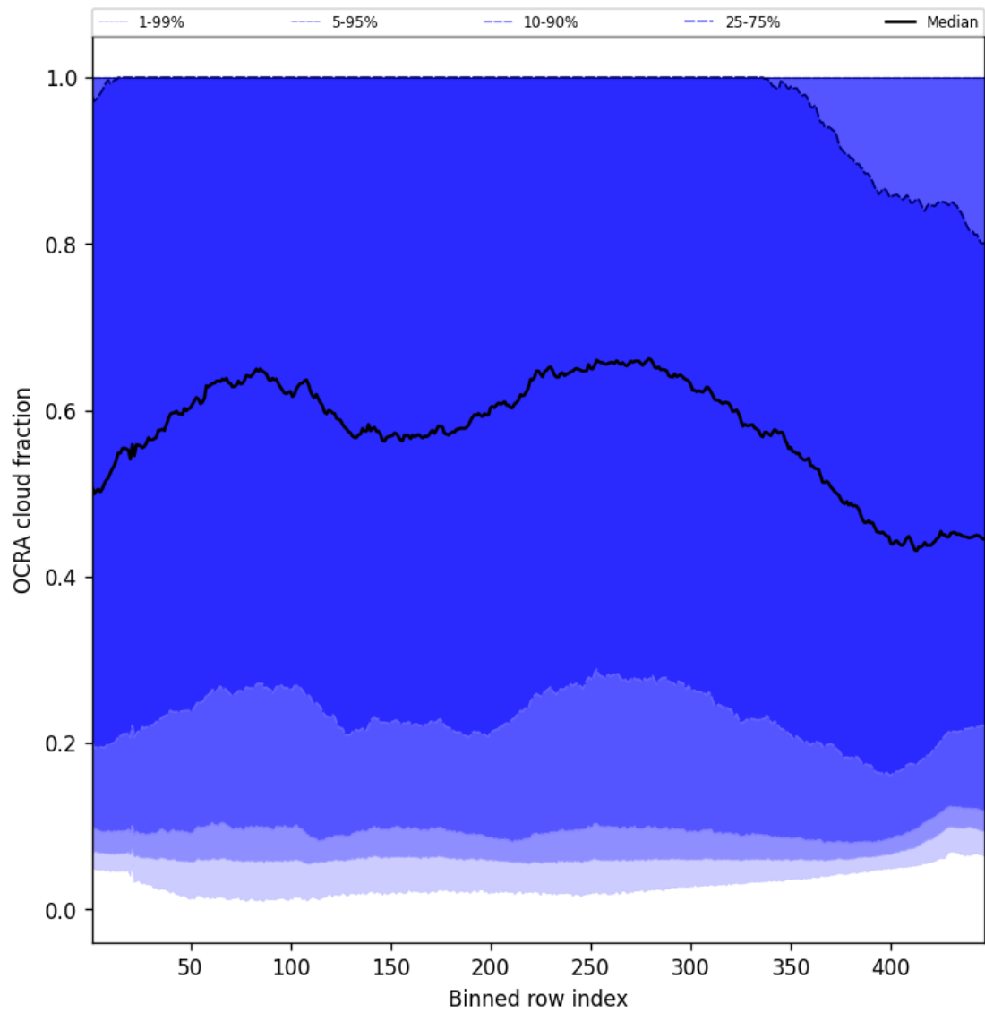
Figure 66: Along track statistics of “OCRA cloud fraction” for 2025-08-19 to 2025-08-20
