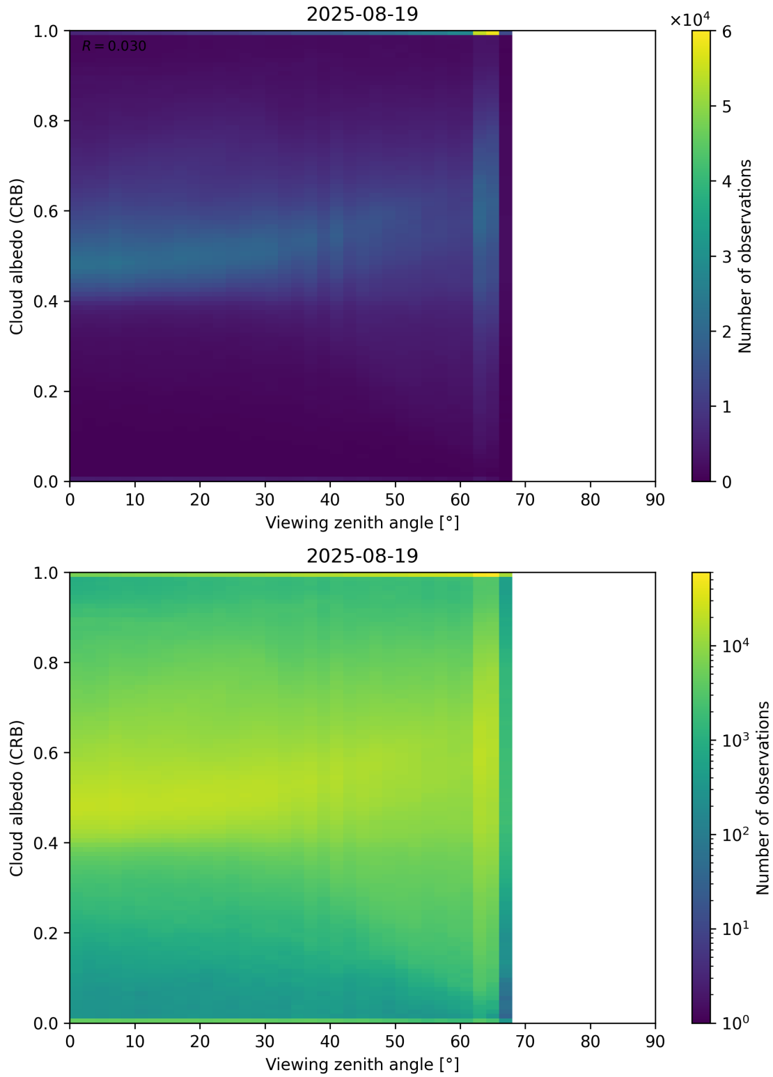
Figure 106: Scatter density plot of “Viewing zenith angle” against “Cloud albedo (CRB)” for 2025-08-19 to 2025-08-20.
