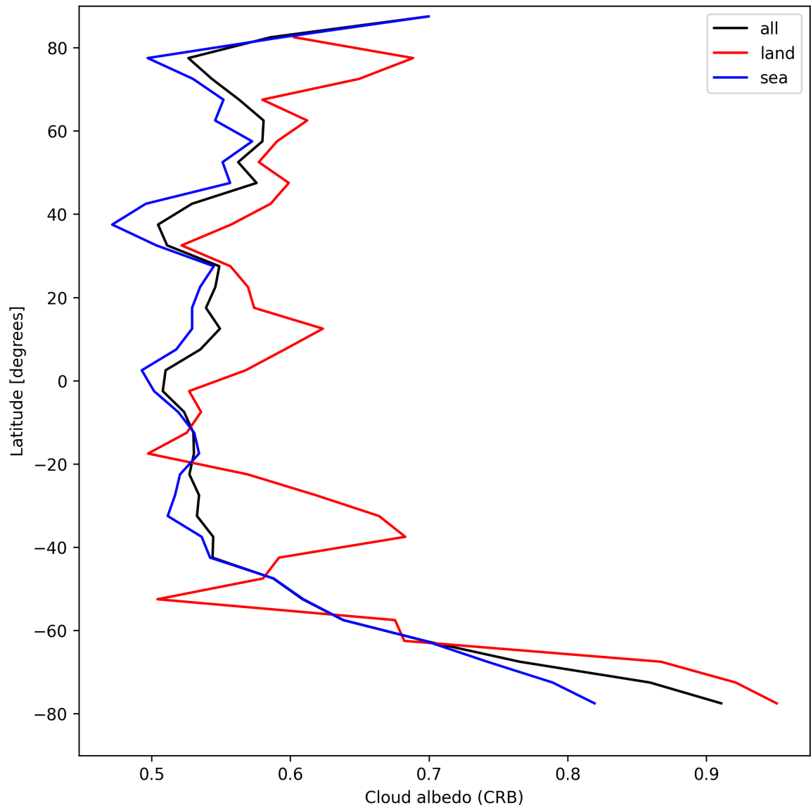
Figure 28: Zonal average of “Cloud albedo (CRB)” for 2025-08-19 to 2025-08-20.
