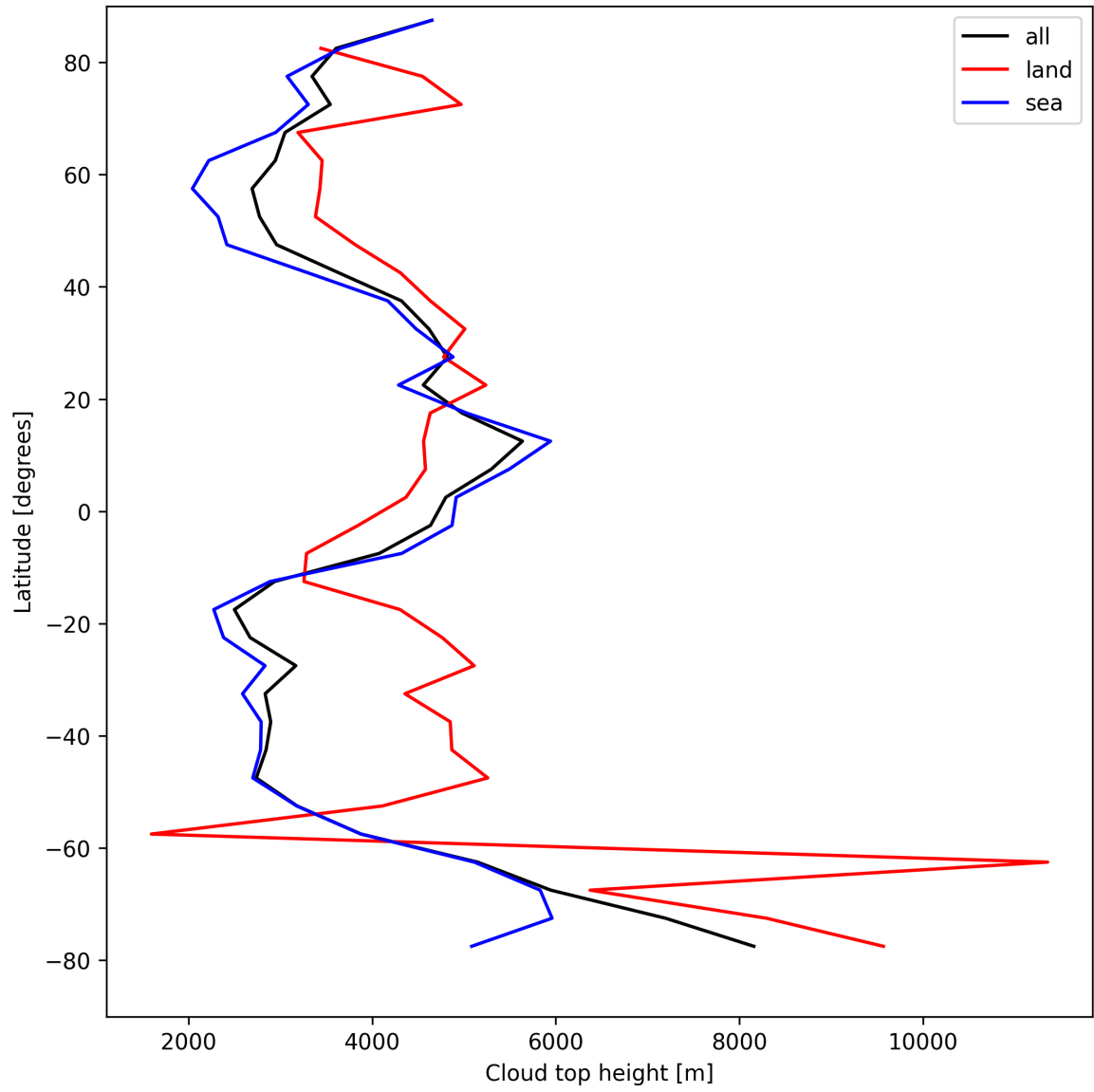
Figure 24: Zonal average of “Cloud top height” for 2025-08-19 to 2025-08-20.
