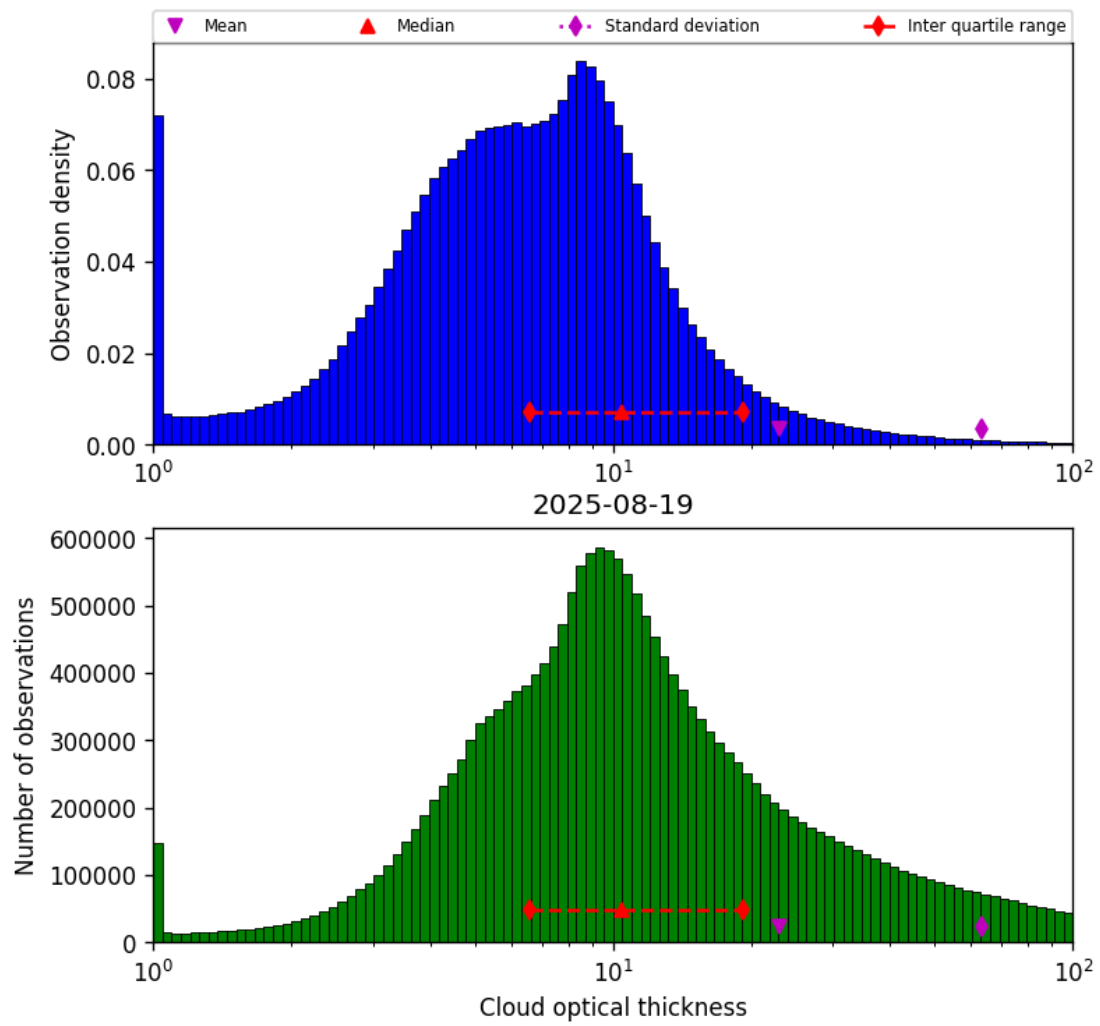
Figure 41: Histogram of “Cloud optical thickness” for 2025-08-19 to 2025-08-20
