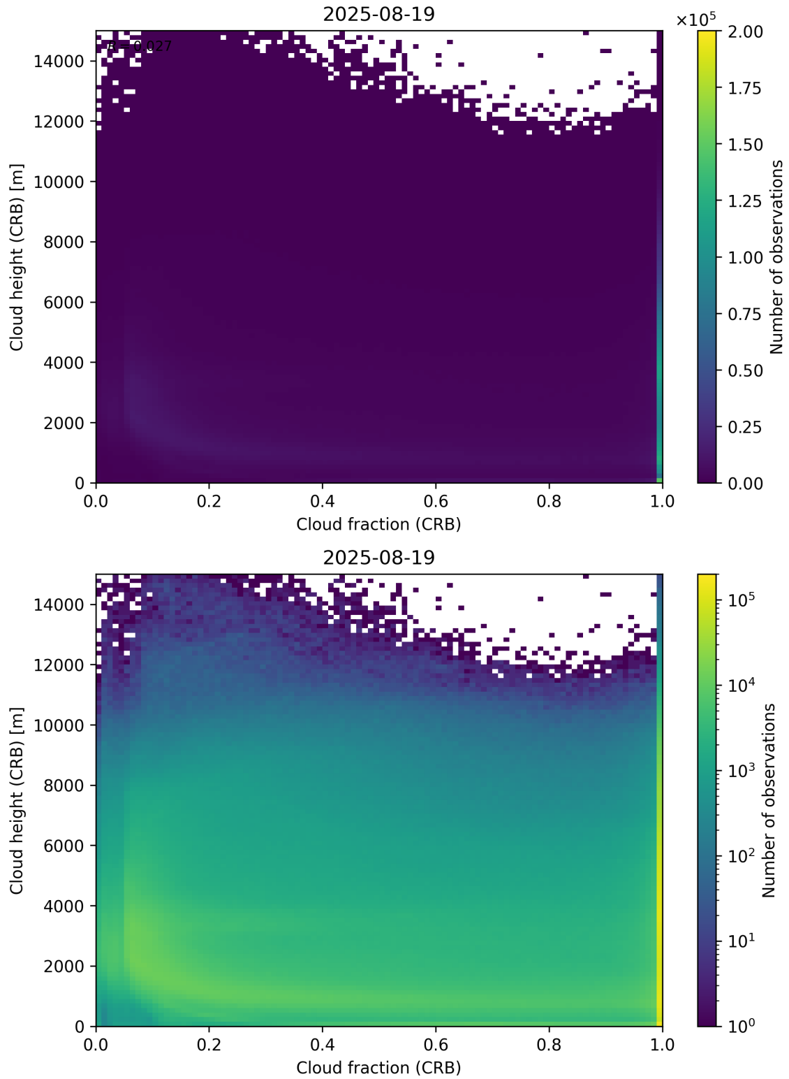
Figure 79: Scatter density plot of “Cloud fraction (CRB)” against “Cloud height (CRB)” for 2025-08-19 to 2025-08-20.
