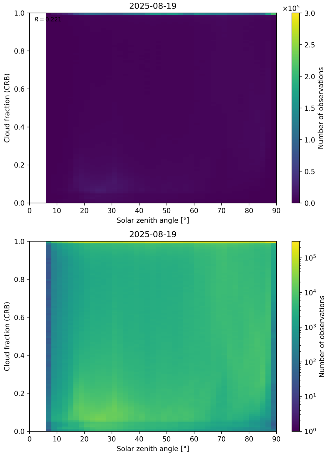
Figure 101: Scatter density plot of “Solar zenith angle” against “Cloud fraction (CRB)” for 2025-08-19 to 2025-08-20.
