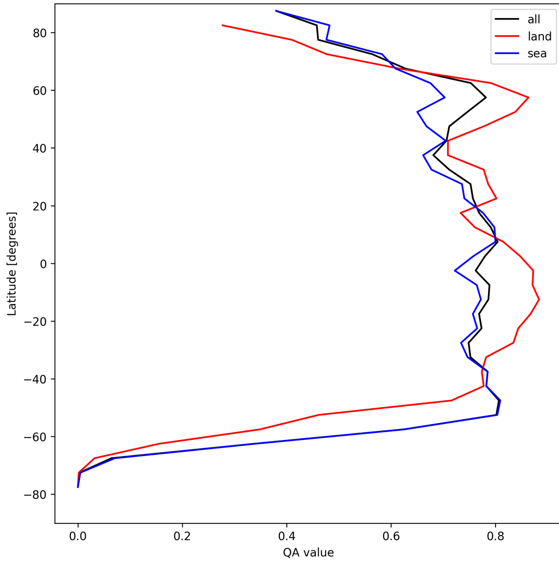
Figure 22: Zonal average of “QA value” for 2025-08-19 to 2025-08-20.
