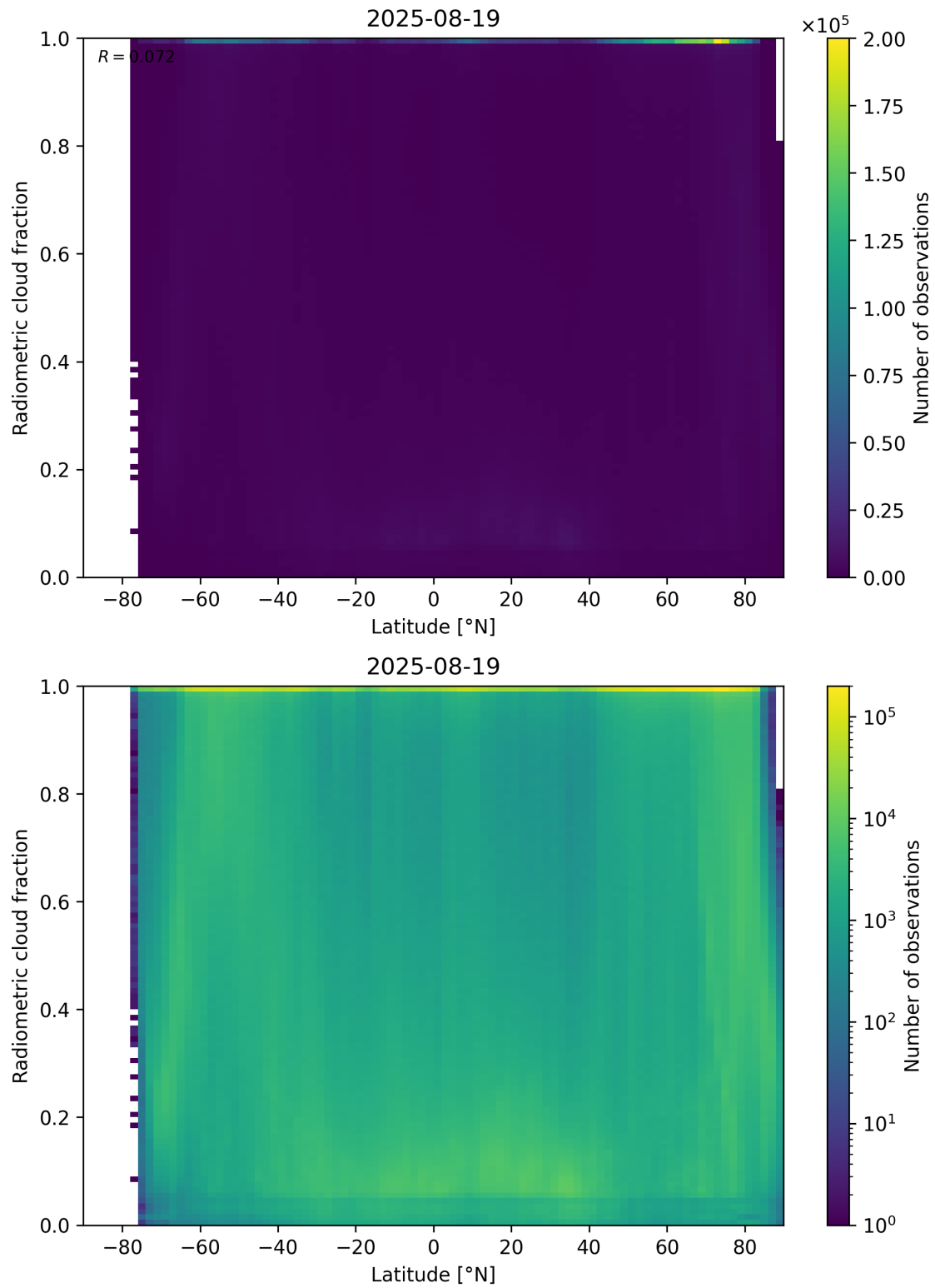
Figure 92: Scatter density plot of “Latitude” against “Radiometric cloud fraction” for 2025-08-19 to 2025-08-20.
