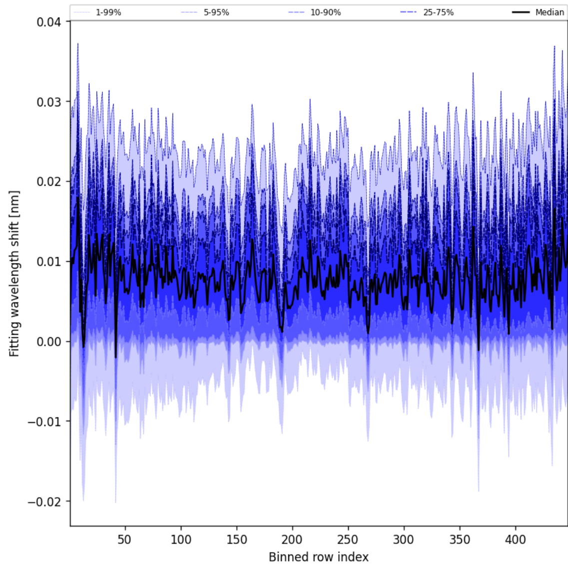
Figure 65: Along track statistics of “Fitting wavelength shift” for 2025-08-19 to 2025-08-20
