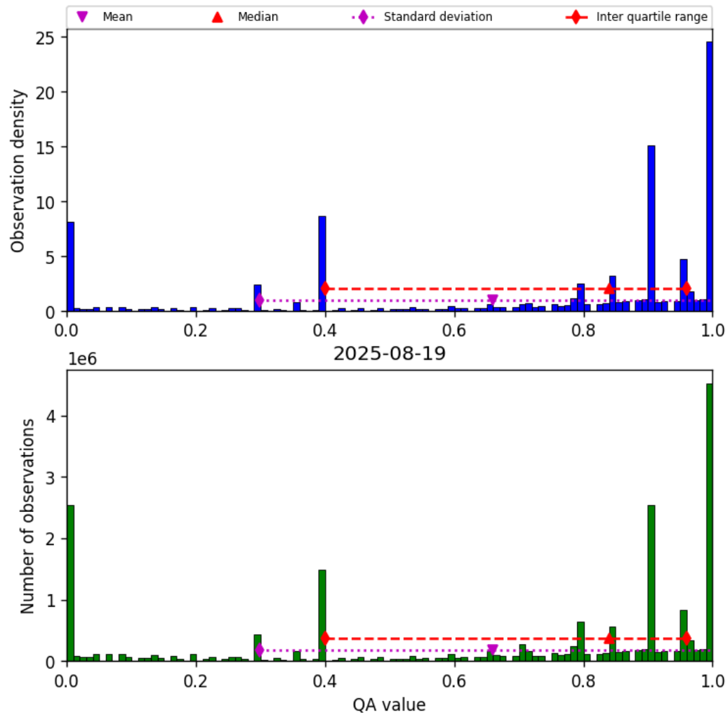
Figure 38: Histogram of “QA value” for 2025-08-19 to 2025-08-20
