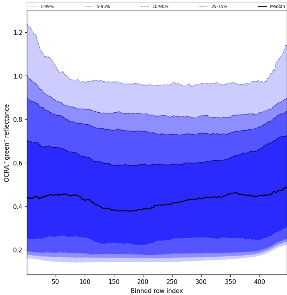
Figure 68: Along track statistics of “OCRA “green” reflectance” for 2025-08-19 to 2025-08-20
