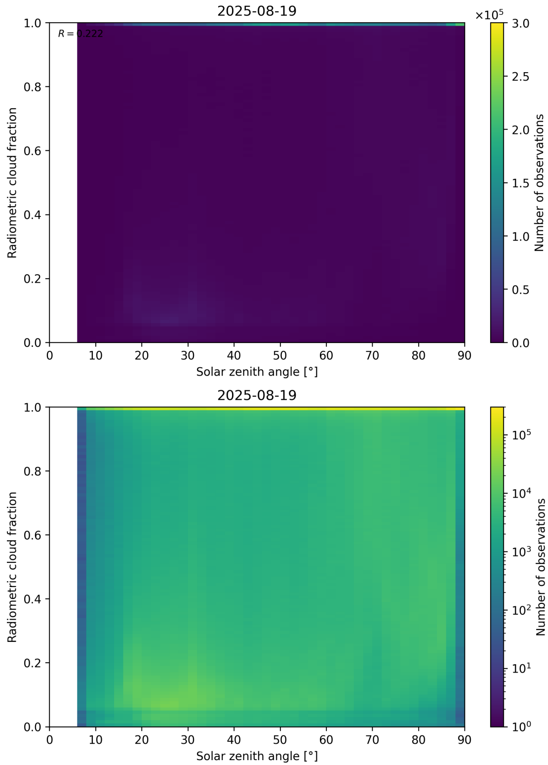
Figure 99: Scatter density plot of “Solar zenith angle” against “Radiometric cloud fraction” for 2025-08-19 to 2025-08-20.
