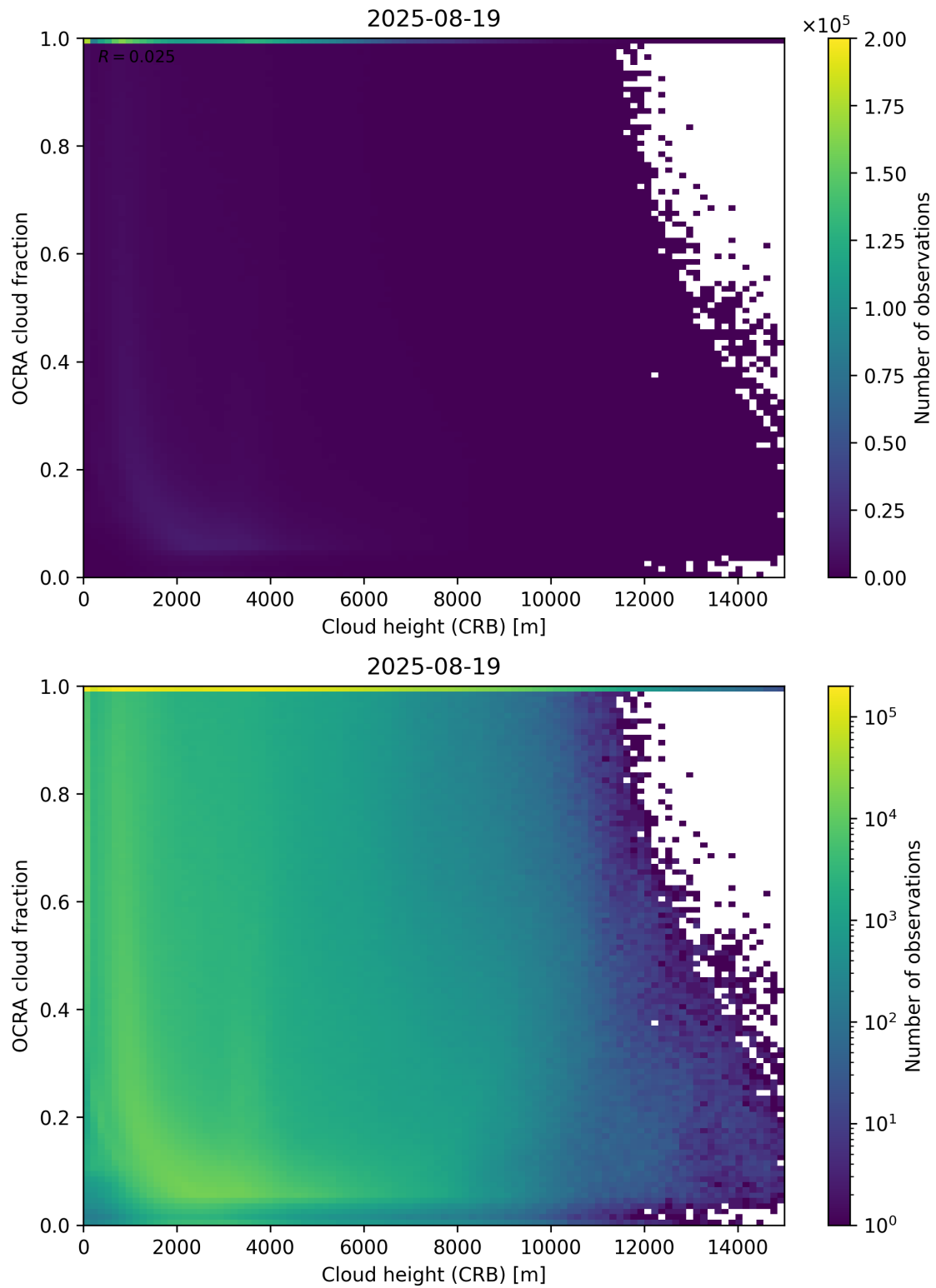
Figure 81: Scatter density plot of “Cloud height (CRB)” against “OCRA cloud fraction” for 2025-08-19 to 2025-08-20.
