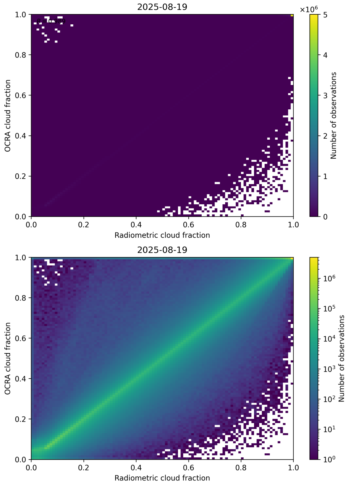
Figure 72: Scatter density plot of “Radiometric cloud fraction” against “OCRA cloud fraction” for 2025-08-19 to 2025-08-20.
