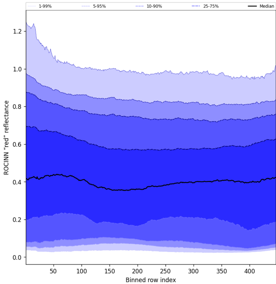
Figure 69: Along track statistics of "ROCINN "red" reflectance" for 2025-08-19 to 2025-08-20
