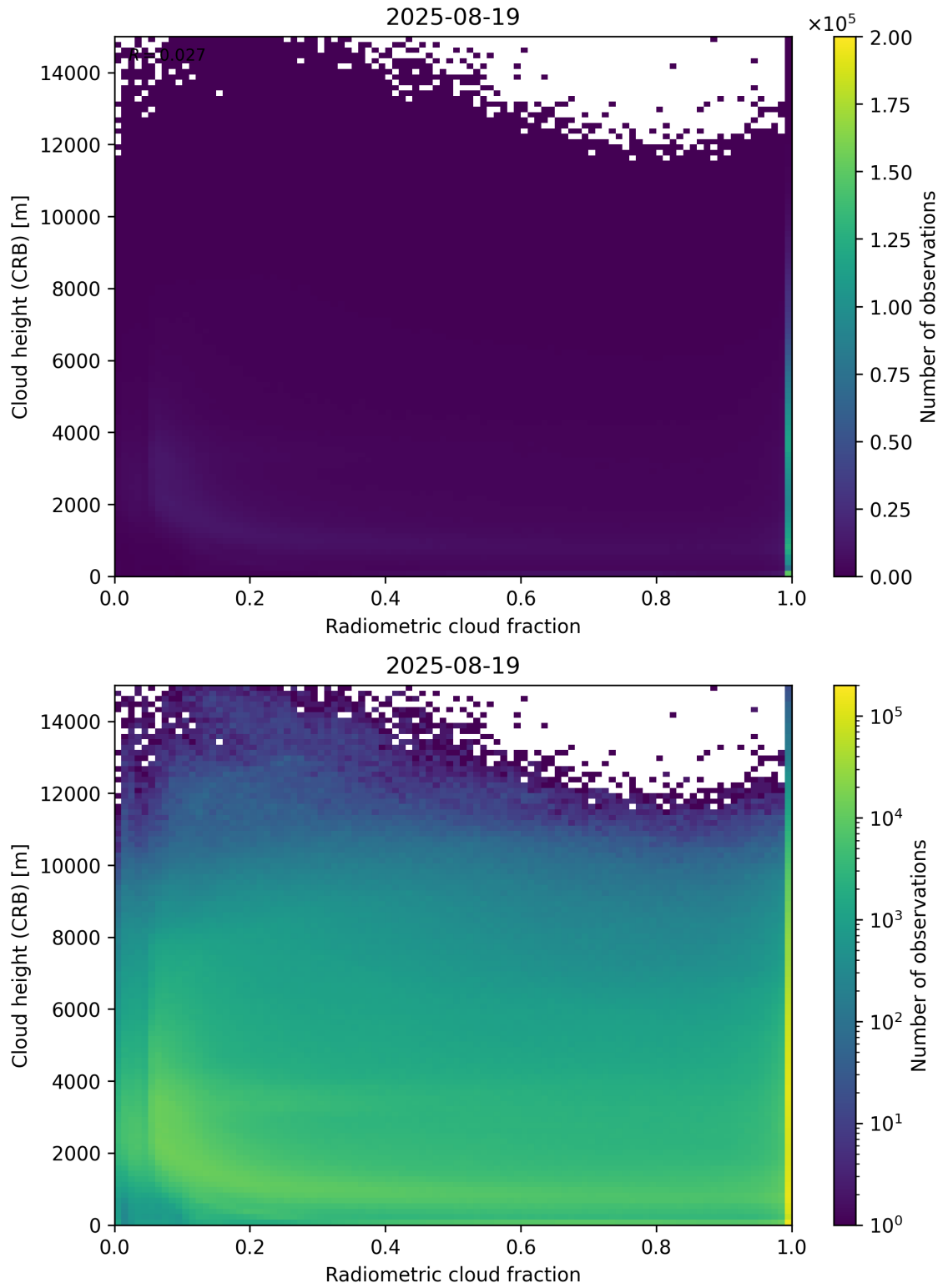
Figure 74: Scatter density plot of “Radiometric cloud fraction” against “Cloud height (CRB)” for 2025-08-19 to 2025-08-20.
