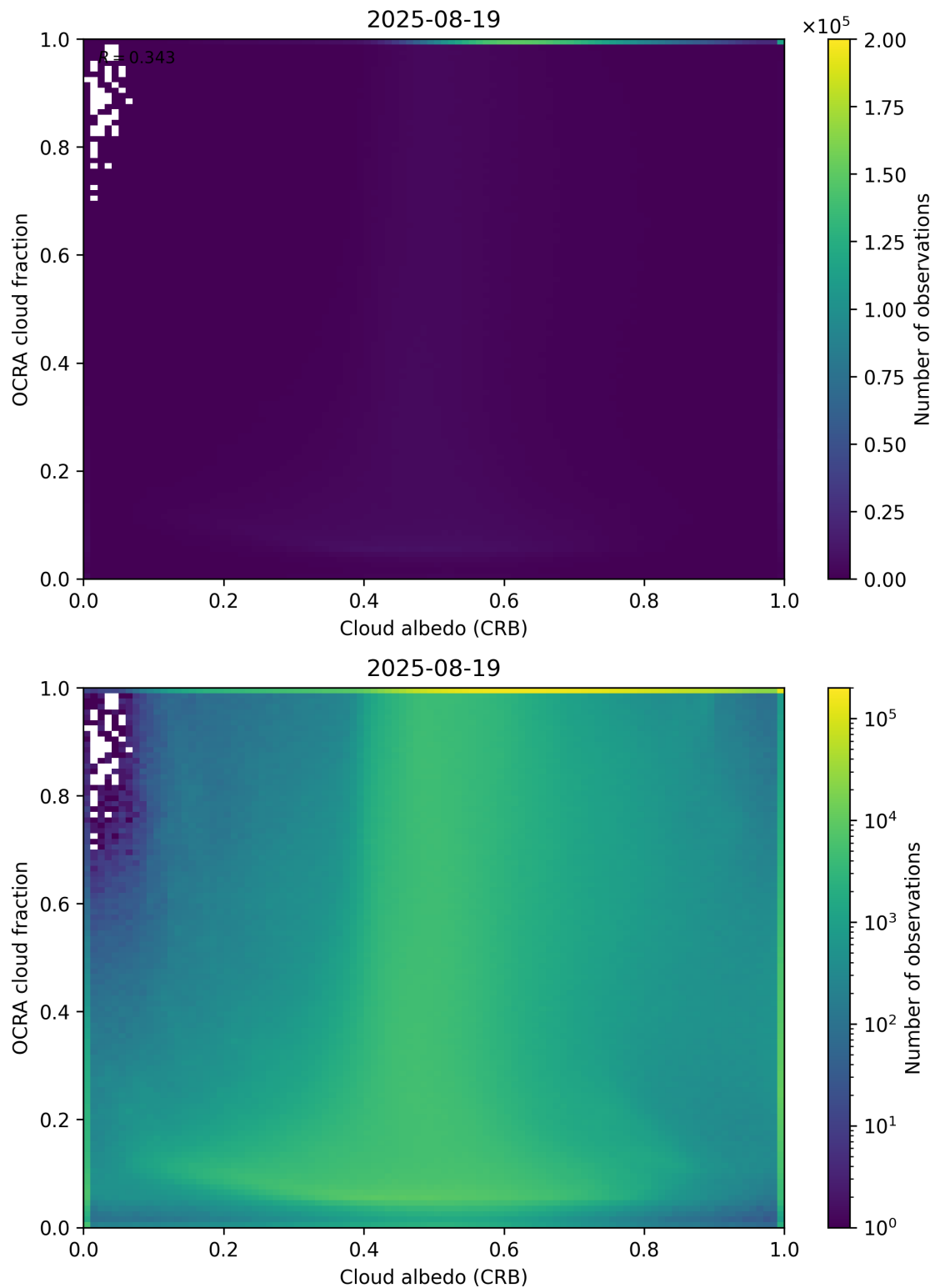
Figure 70: Scatter density plot of “Cloud albedo (CRB)” against “OCRA cloud fraction” for 2025-08-19 to 2025-08-20.
