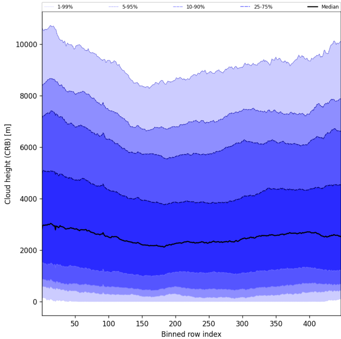
Figure 59: Along track statistics of “Cloud height (CRB)” for 2025-08-19 to 2025-08-20
