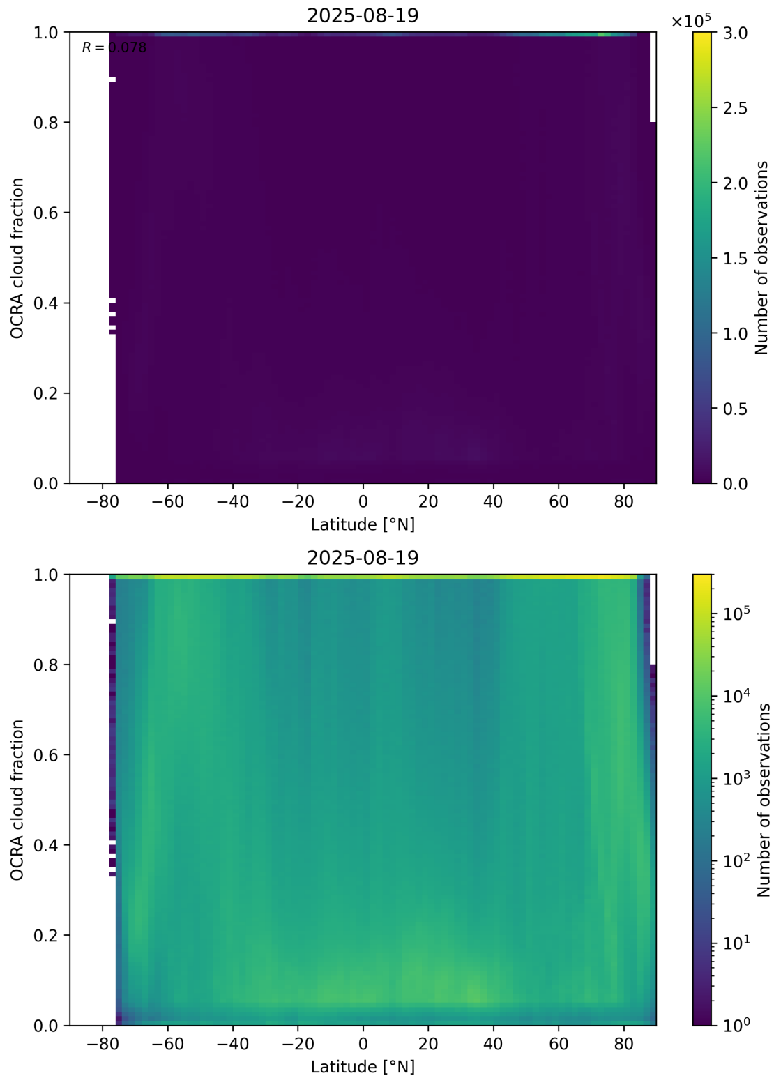
Figure 93: Scatter density plot of “Latitude” against “OCRA cloud fraction” for 2025-08-19 to 2025-08-20.
