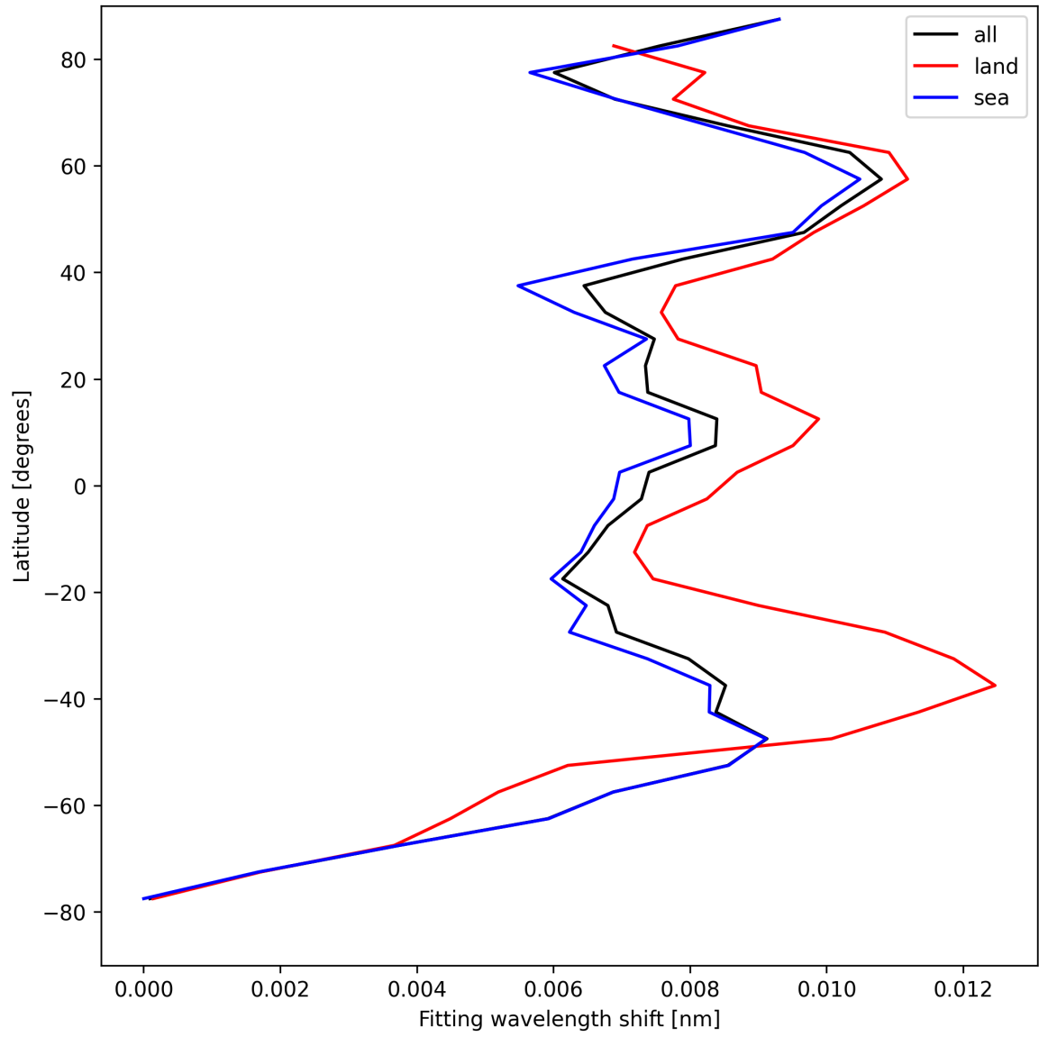
Figure 33: Zonal average of “Fitting wavelength shift” for 2025-08-19 to 2025-08-20.
