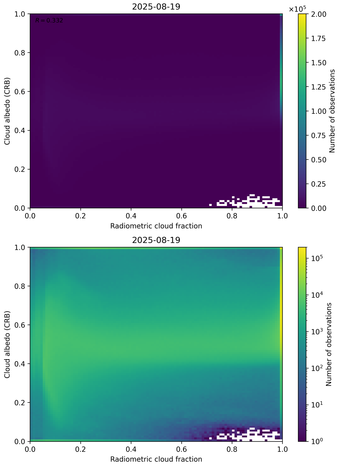
Figure 71: Scatter density plot of “Radiometric cloud fraction” against “Cloud albedo (CRB)” for 2025-08-19 to 2025-08-20.
