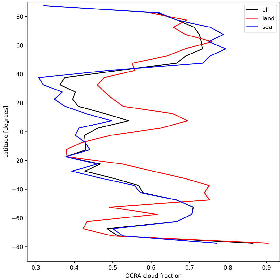
Figure 34: Zonal average of “OCRA cloud fraction” for 2025-08-19 to 2025-08-20.
