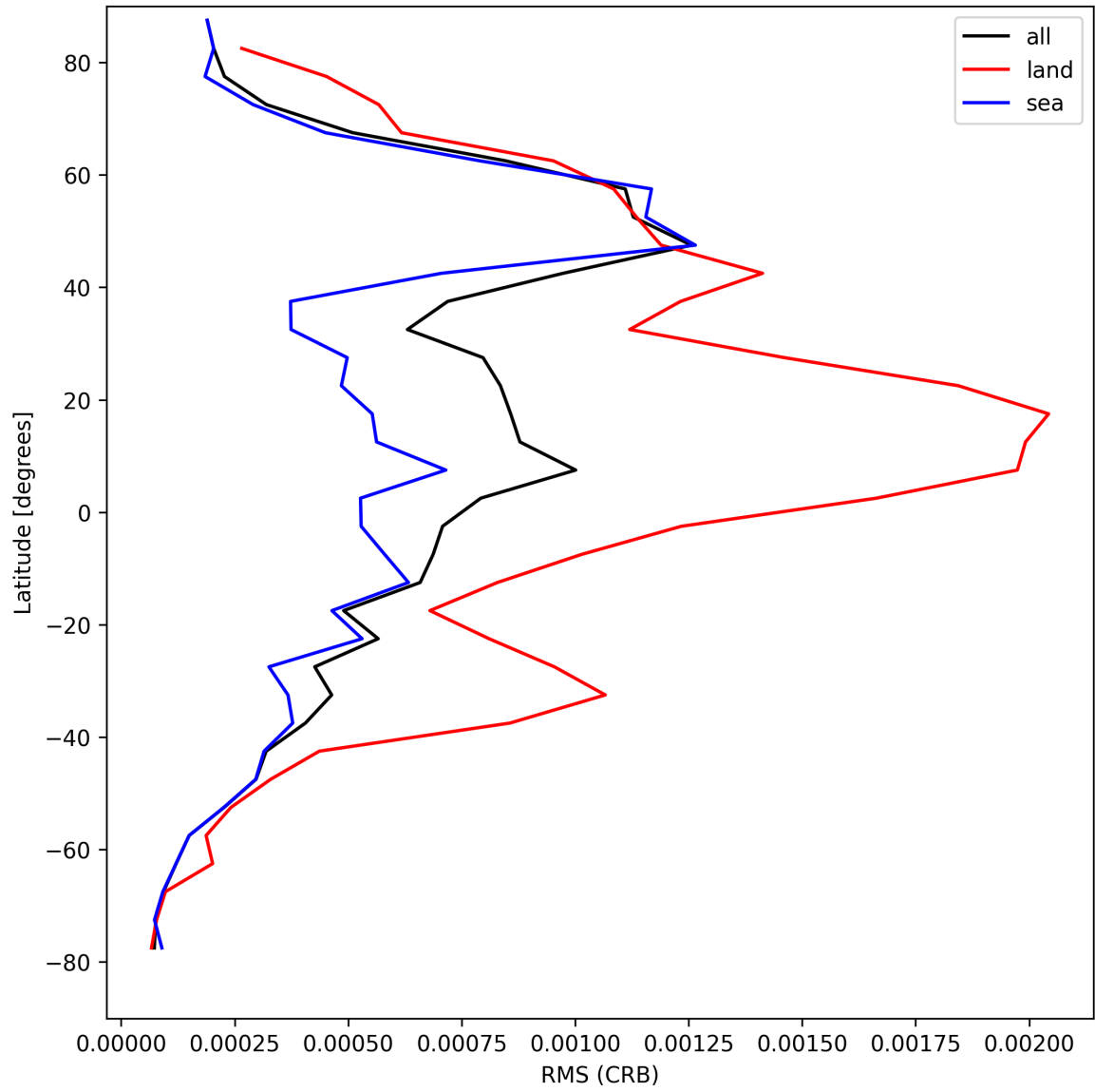
Figure 32: Zonal average of “RMS (CRB)” for 2025-08-19 to 2025-08-20.
