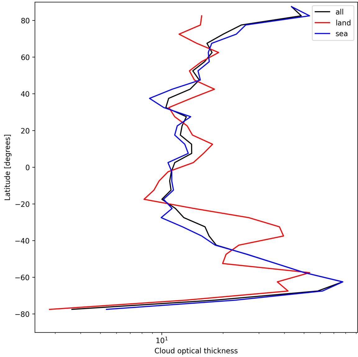
Figure 25: Zonal average of “Cloud optical thickness” for 2025-08-19 to 2025-08-20.
