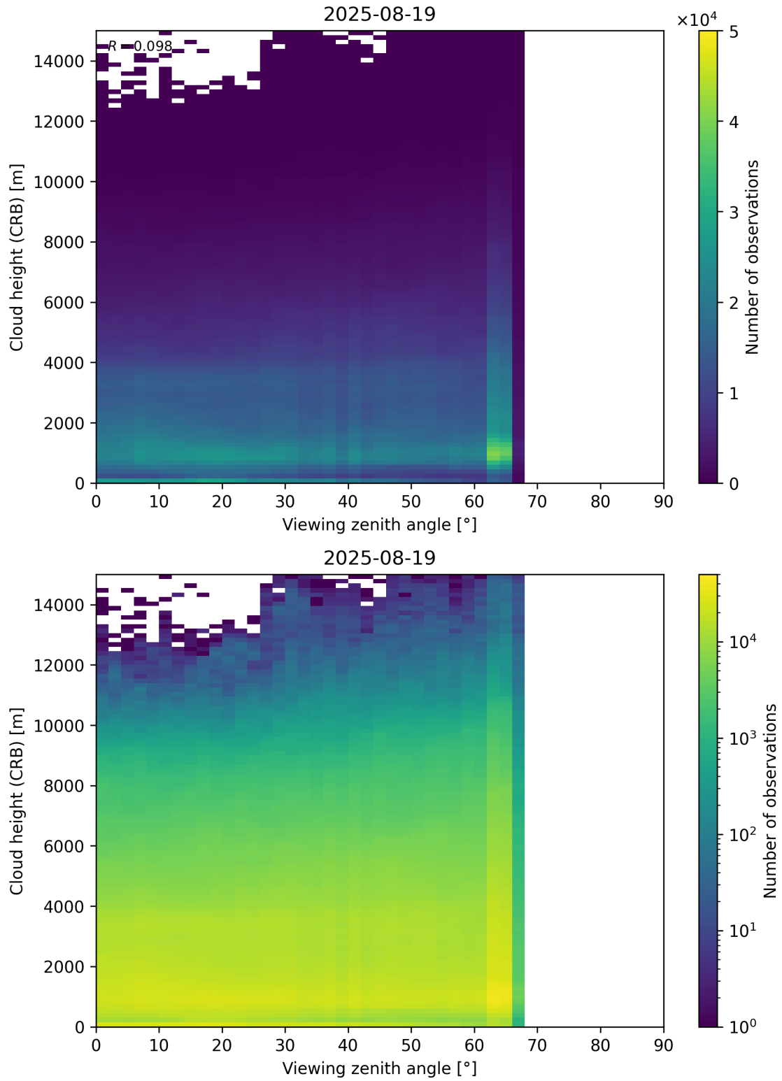
Figure 110: Scatter density plot of “Viewing zenith angle” against “Cloud height (CRB)” for 2025-08-19 to 2025-08-20.
