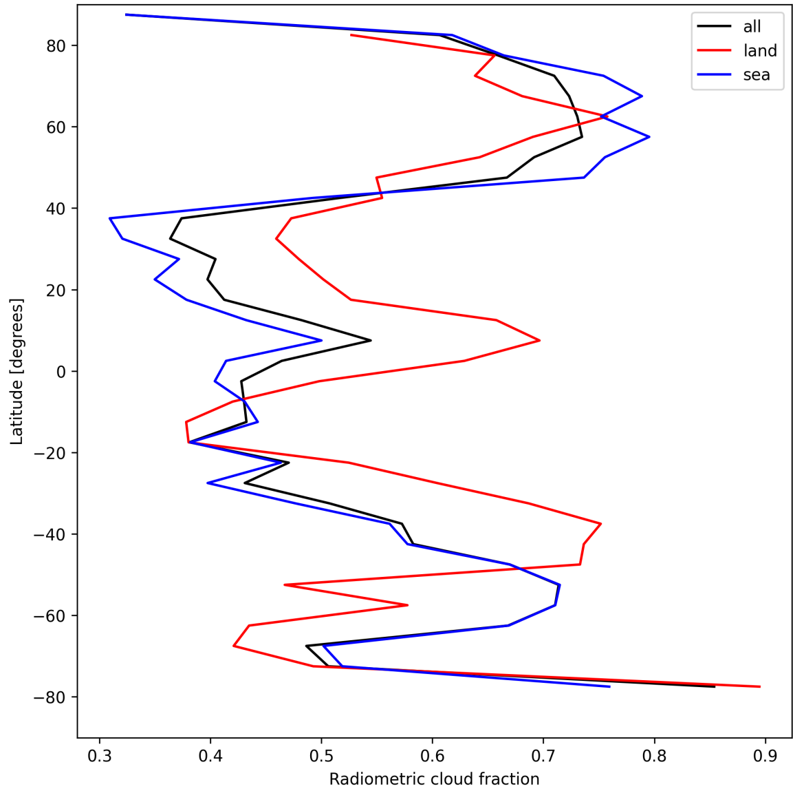
Figure 23: Zonal average of “Radiometric cloud fraction” for 2025-08-19 to 2025-08-20.
