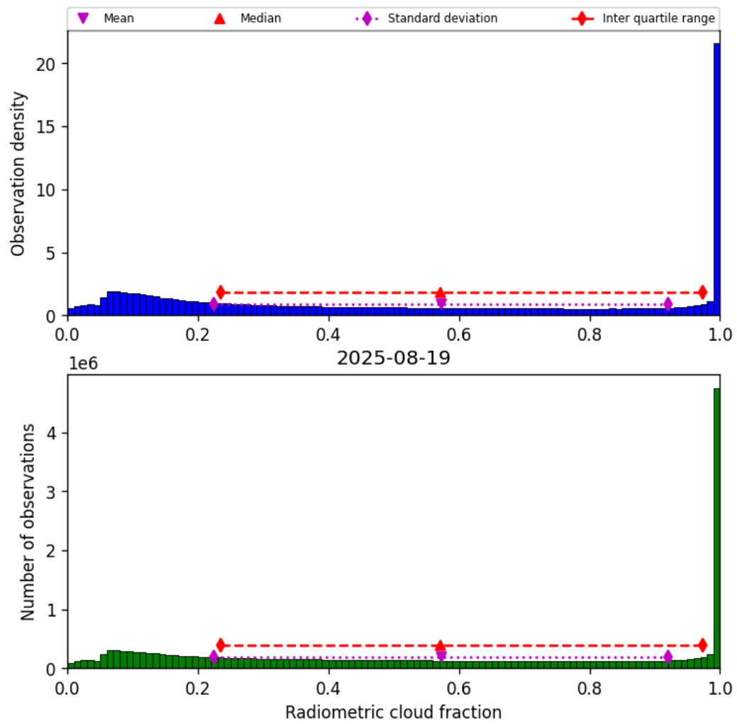
Figure 39: Histogram of “Radiometric cloud fraction” for 2025-08-19 to 2025-08-20
