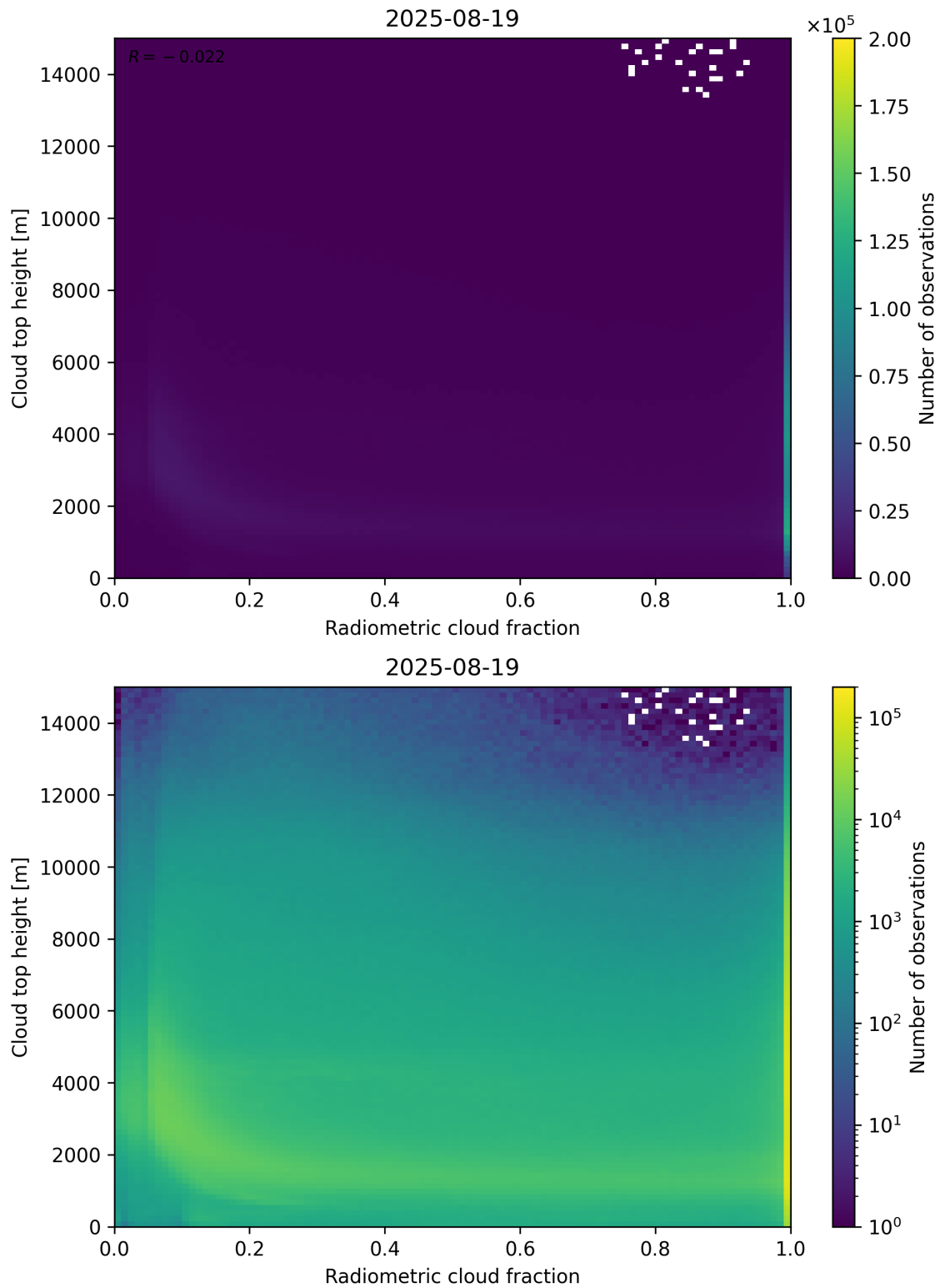
Figure 76: Scatter density plot of “Radiometric cloud fraction” against “Cloud top height” for 2025-08-19 to 2025-08-20.
