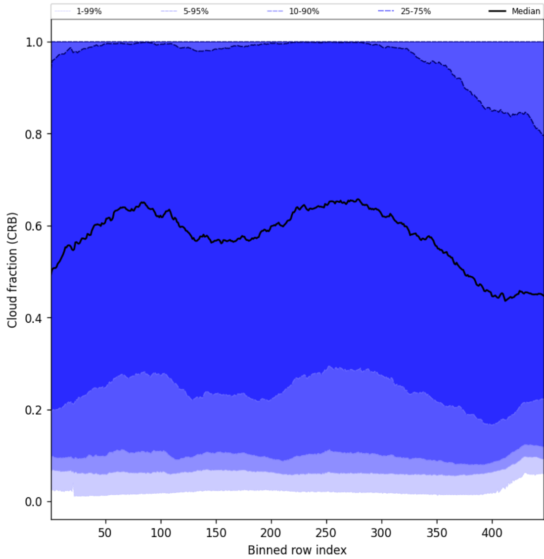
Figure 58: Along track statistics of “Cloud fraction (CRB)” for 2025-08-19 to 2025-08-20
