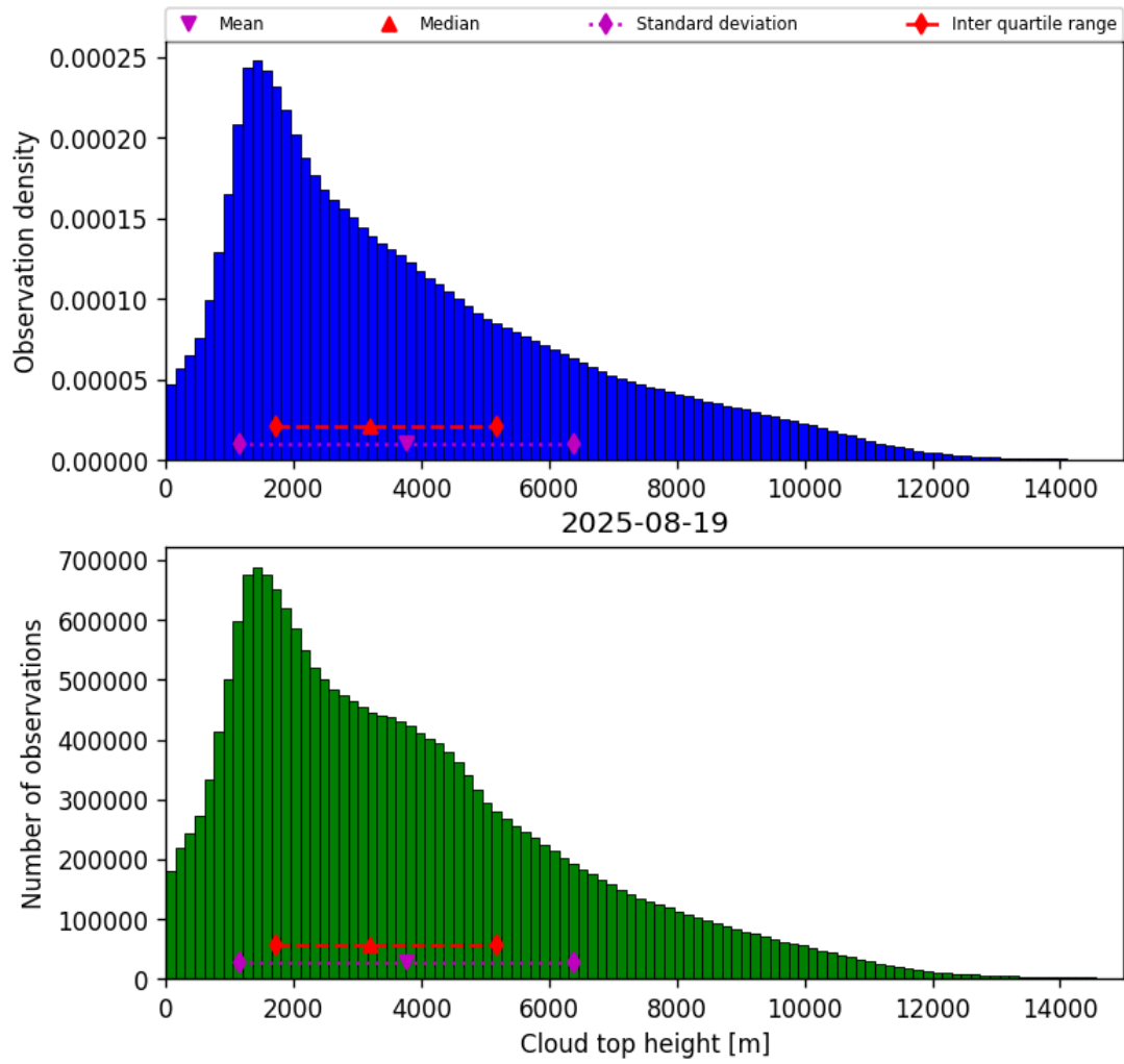
Figure 40: Histogram of “Cloud top height” for 2025-08-19 to 2025-08-20
