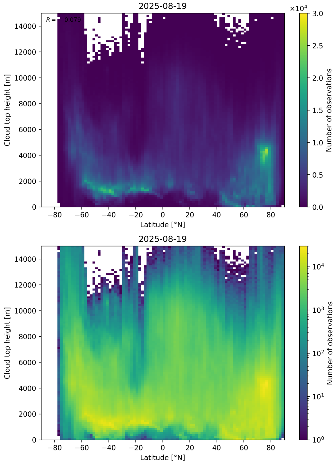
Figure 97: Scatter density plot of “Latitude” against “Cloud top height” for 2025-08-19 to 2025-08-20.
