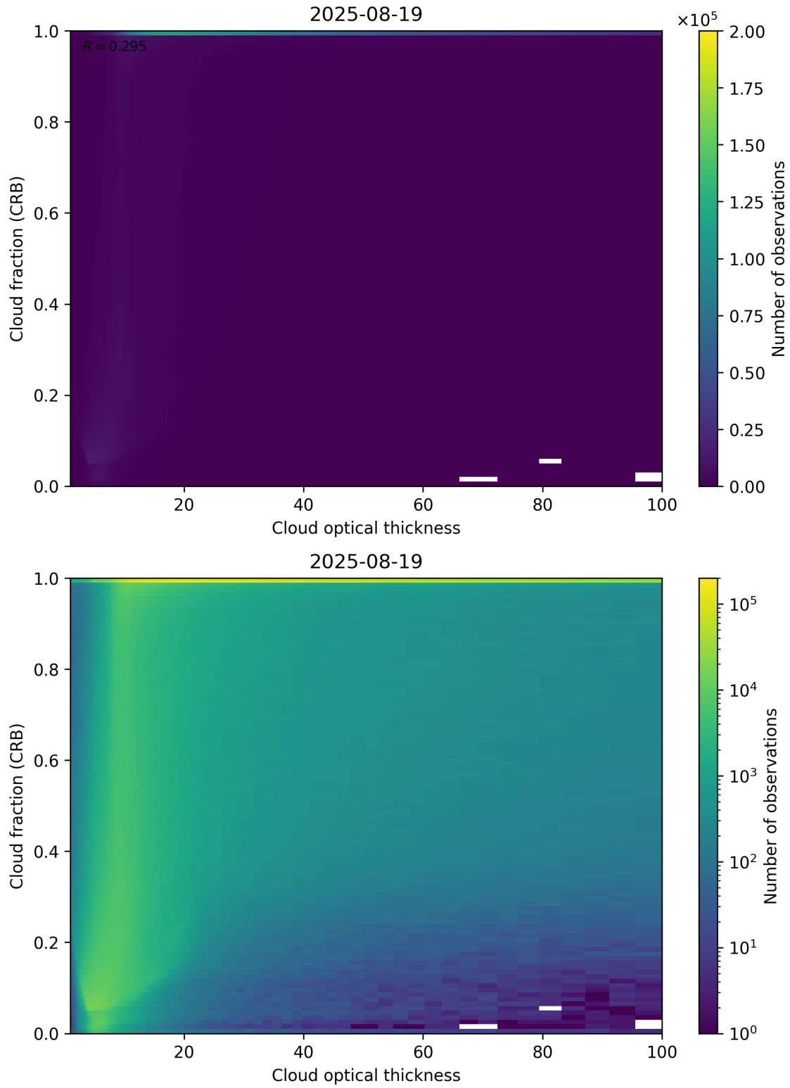
Figure 84: Scatter density plot of “Cloud optical thickness” against “Cloud fraction (CRB)” for 2025-08-19 to 2025-08-20.
