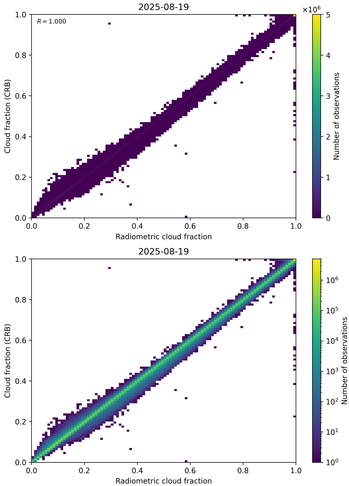
Figure 73: Scatter density plot of “Radiometric cloud fraction” against “Cloud fraction (CRB)” for 2025-08-19 to 2025-08-20.
