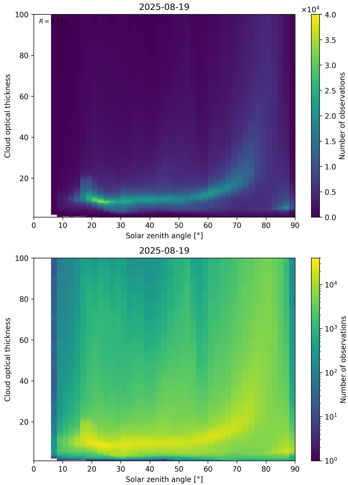
Figure 103: Scatter density plot of “Solar zenith angle” against “Cloud optical thickness” for 2025-08-19 to 2025-08-20.
