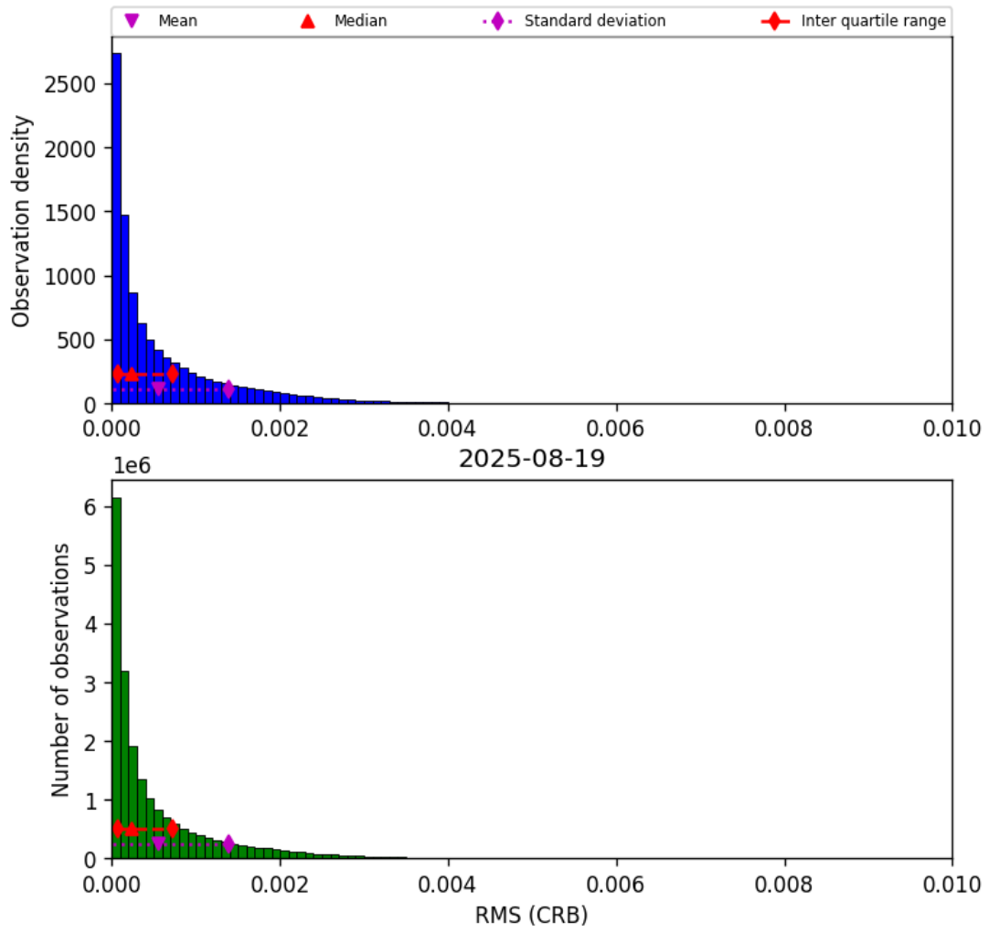
Figure 48: Histogram of “RMS (CRB)” for 2025-08-19 to 2025-08-20
