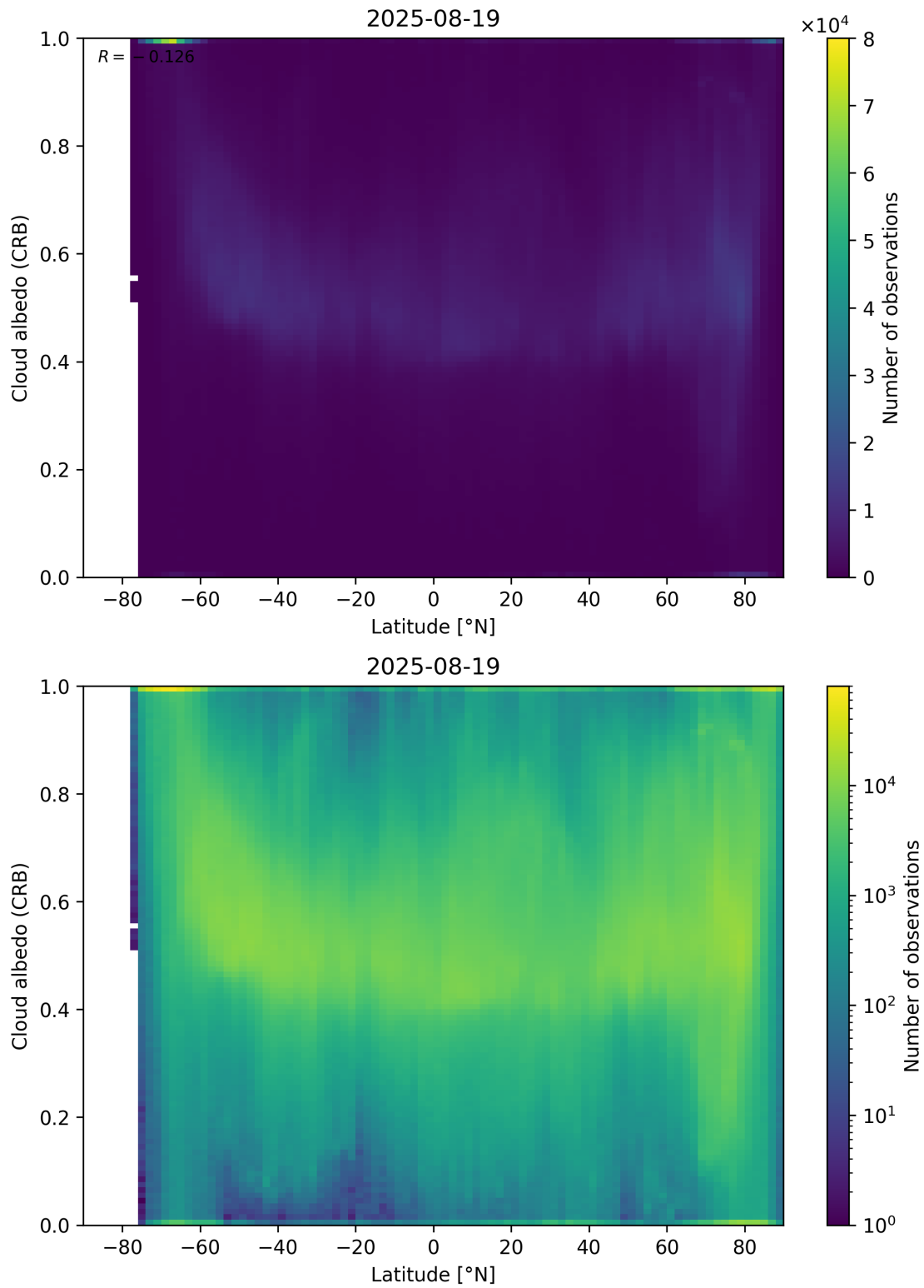
Figure 91: Scatter density plot of “Latitude” against “Cloud albedo (CRB)” for 2025-08-19 to 2025-08-20.
