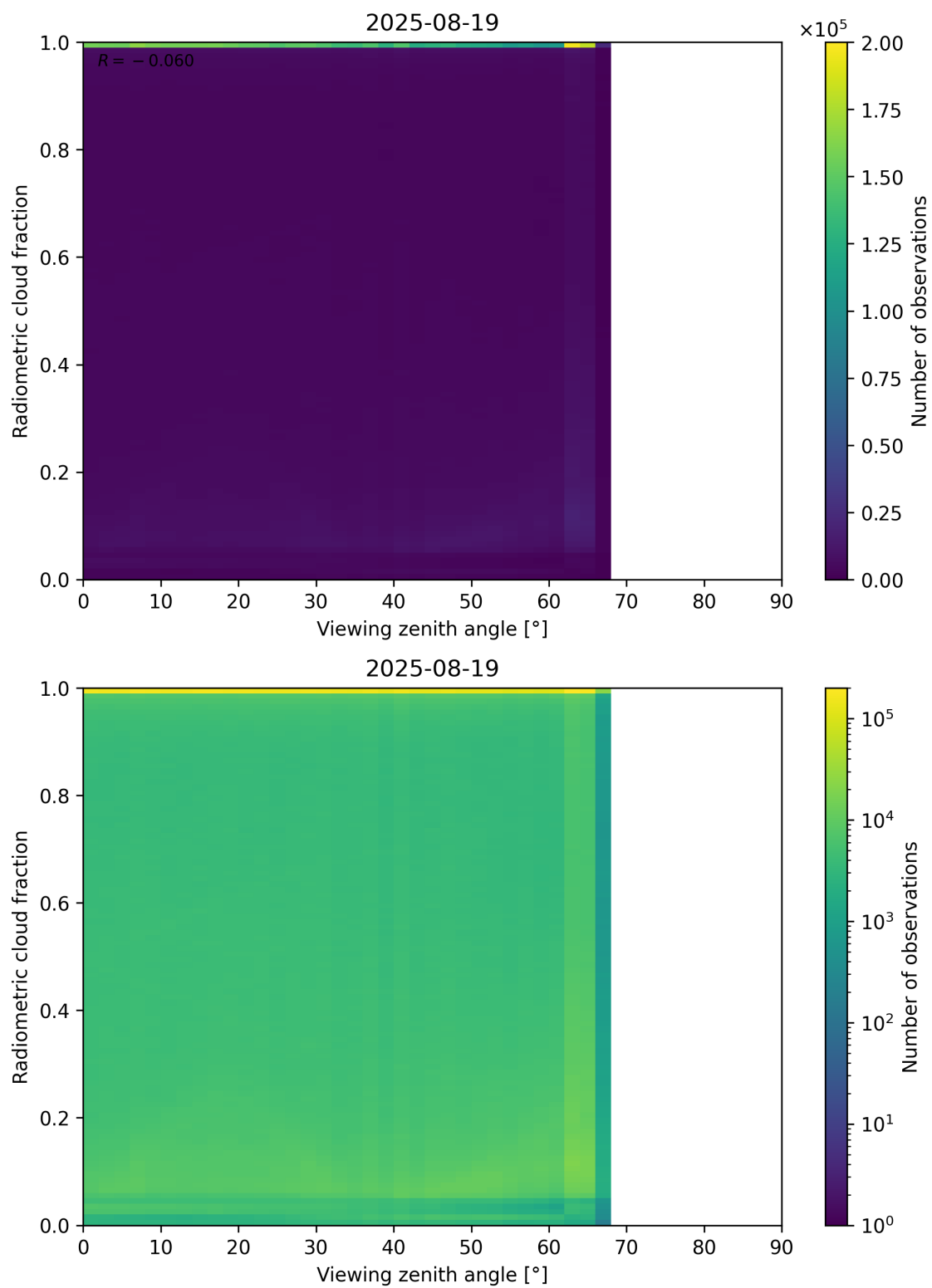
Figure 107: Scatter density plot of “Viewing zenith angle” against “Radiometric cloud fraction” for 2025-08-19 to 2025-08-20.
