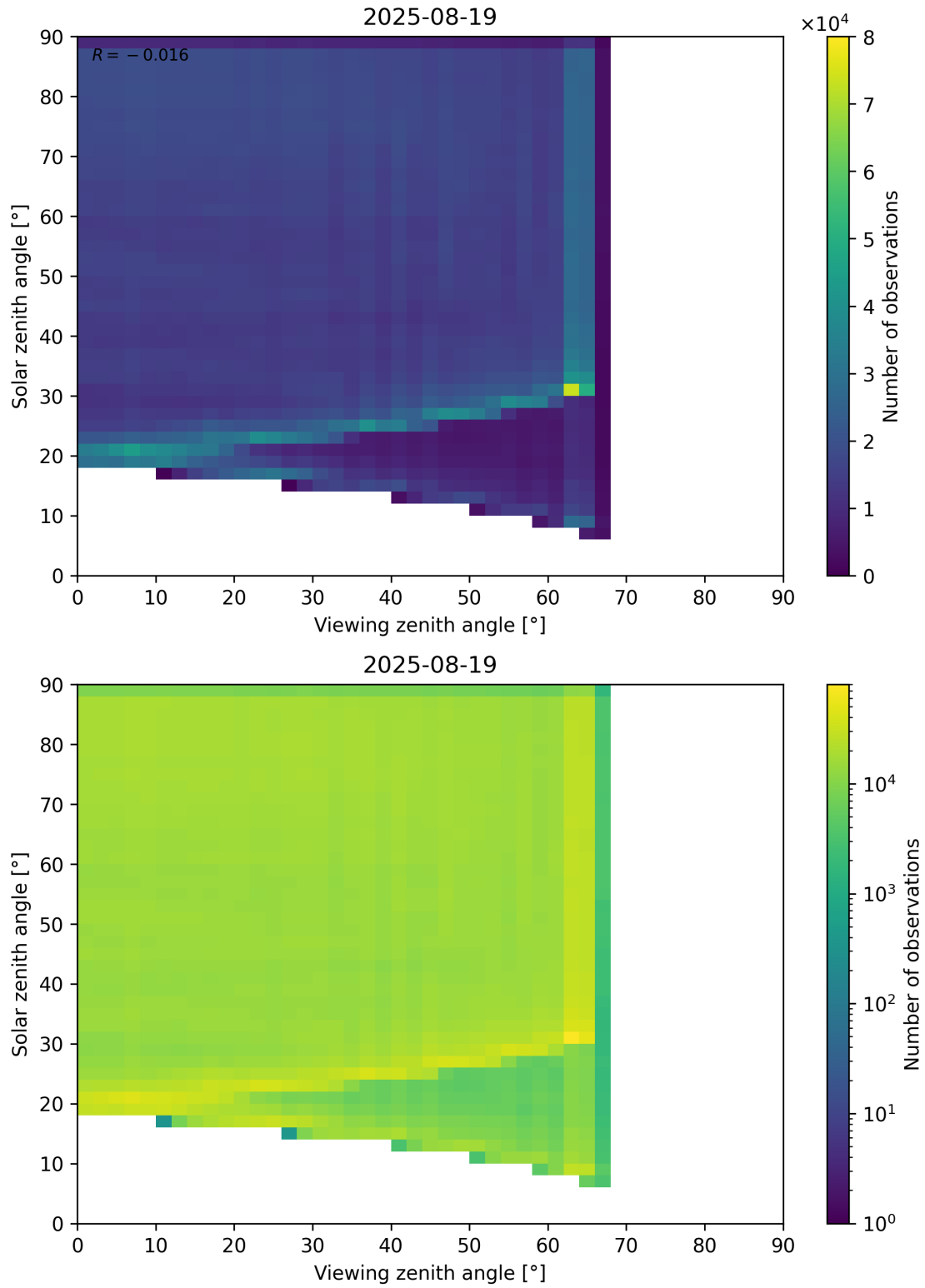
Figure 114: Scatter density plot of “Viewing zenith angle” against “Solar zenith angle” for 2025-08-19 to 2025-08-20.
