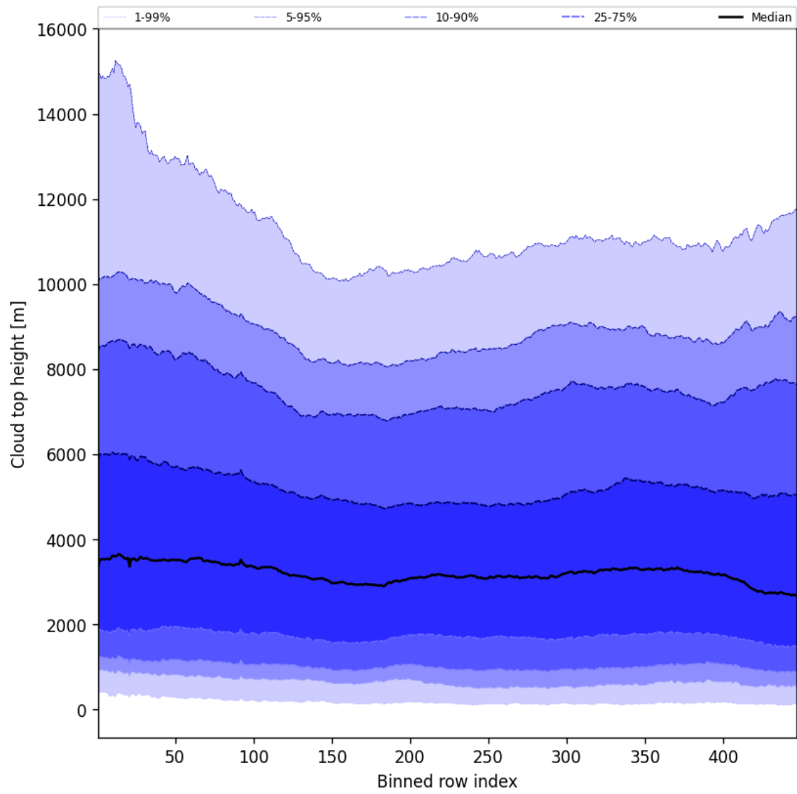
Figure 56: Along track statistics of “Cloud top height” for 2025-08-19 to 2025-08-20
