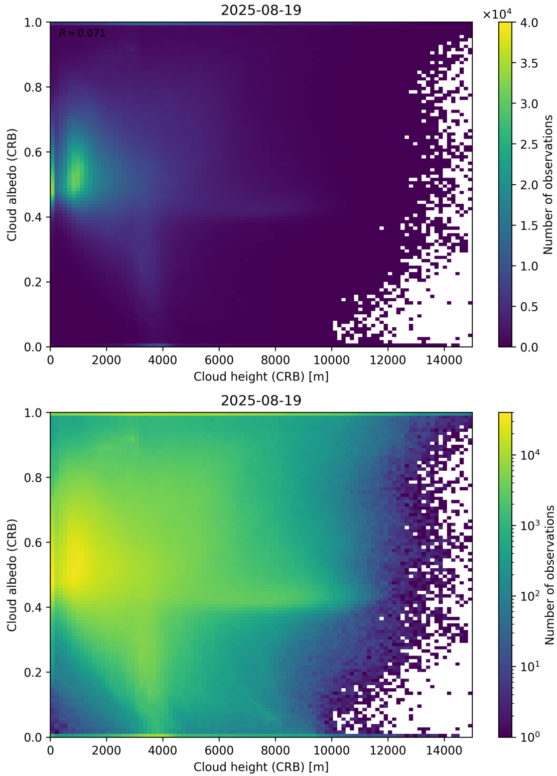
Figure 80: Scatter density plot of “Cloud height (CRB)” against “Cloud albedo (CRB)” for 2025-08-19 to 2025-08-20.
