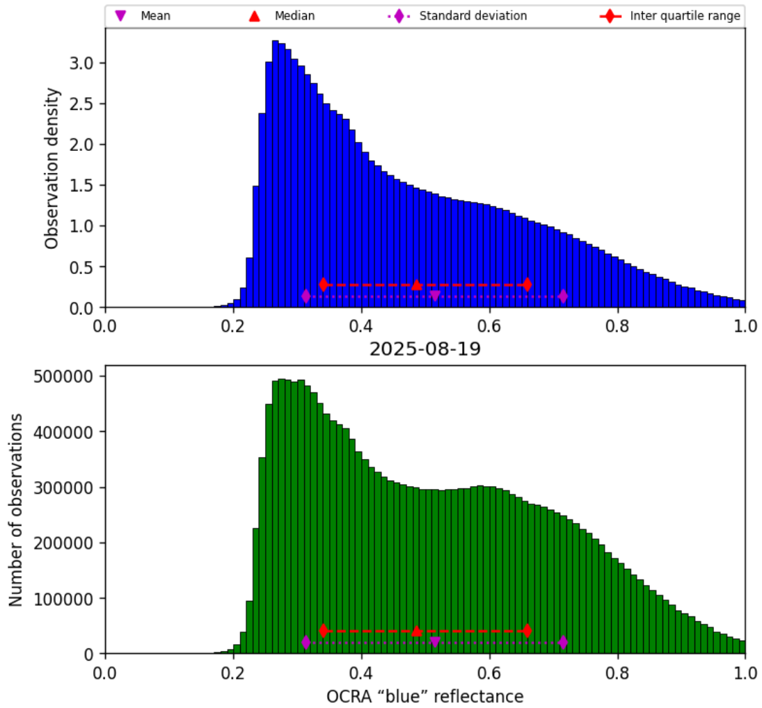
Figure 51: Histogram of “OCRA “blue” reflectance” for 2025-08-19 to 2025-08-20
