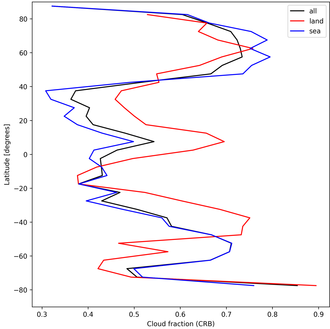
Figure 26: Zonal average of “Cloud fraction (CRB)” for 2025-08-19 to 2025-08-20.
