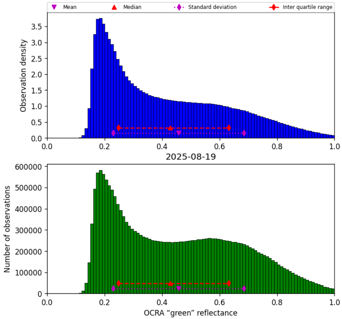
Figure 52: Histogram of “OCRA “green” reflectance” for 2025-08-19 to 2025-08-20
