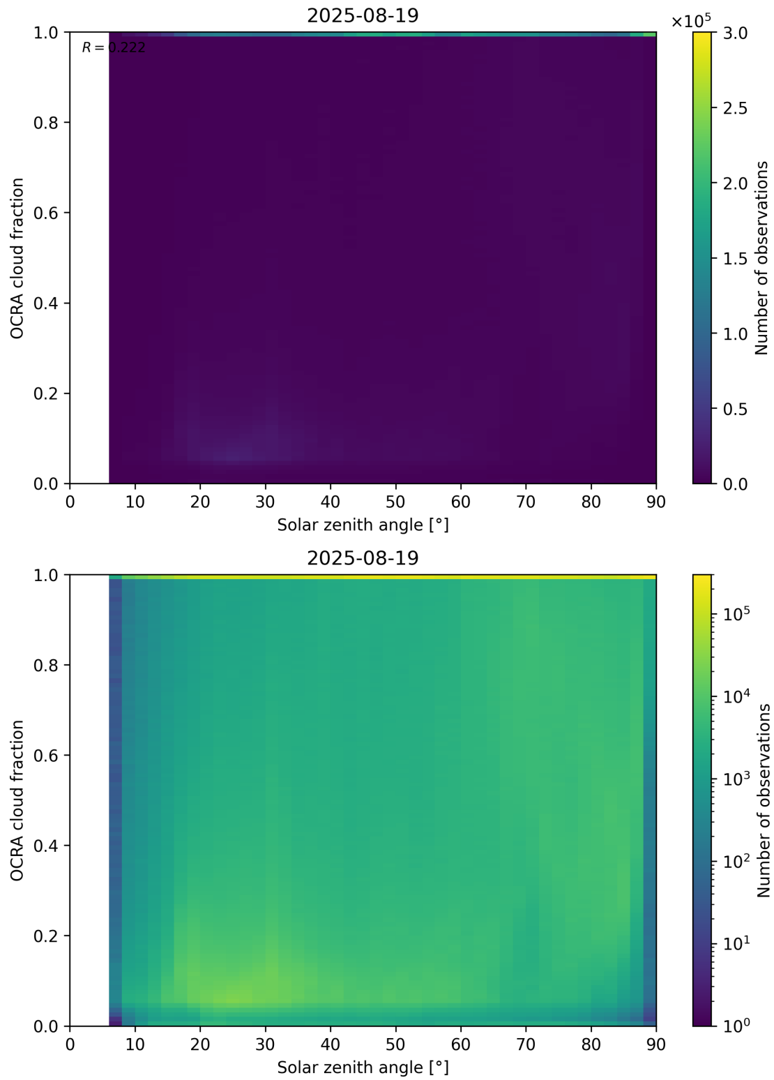
Figure 100: Scatter density plot of “Solar zenith angle” against “OCRA cloud fraction” for 2025-08-19 to 2025-08-20.
