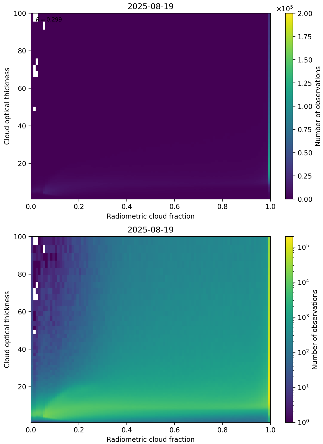
Figure 75: Scatter density plot of “Radiometric cloud fraction” against “Cloud optical thickness” for 2025-08-19 to 2025-08-20.
