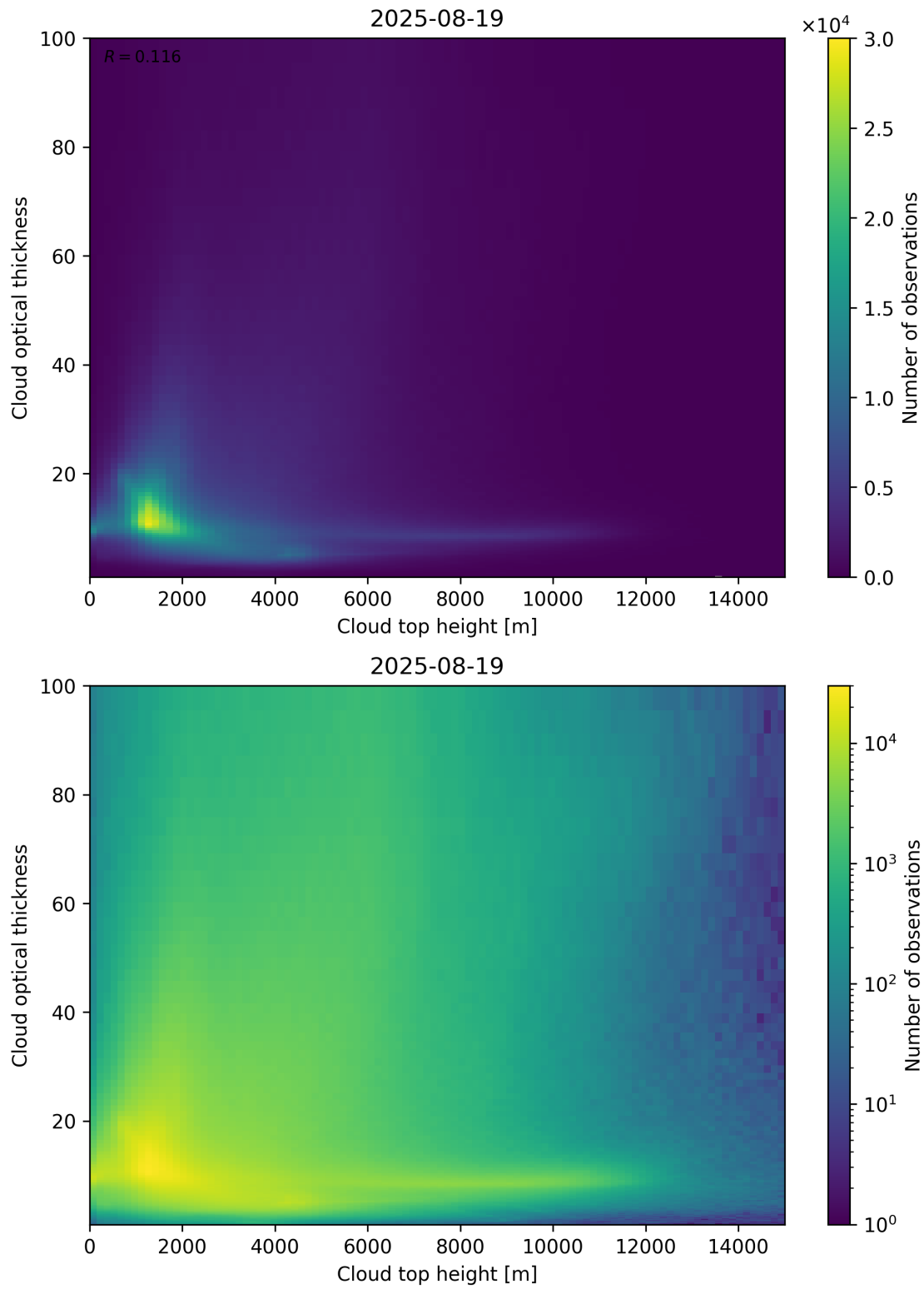
Figure 90: Scatter density plot of “Cloud top height” against “Cloud optical thickness” for 2025-08-19 to 2025-08-20.
