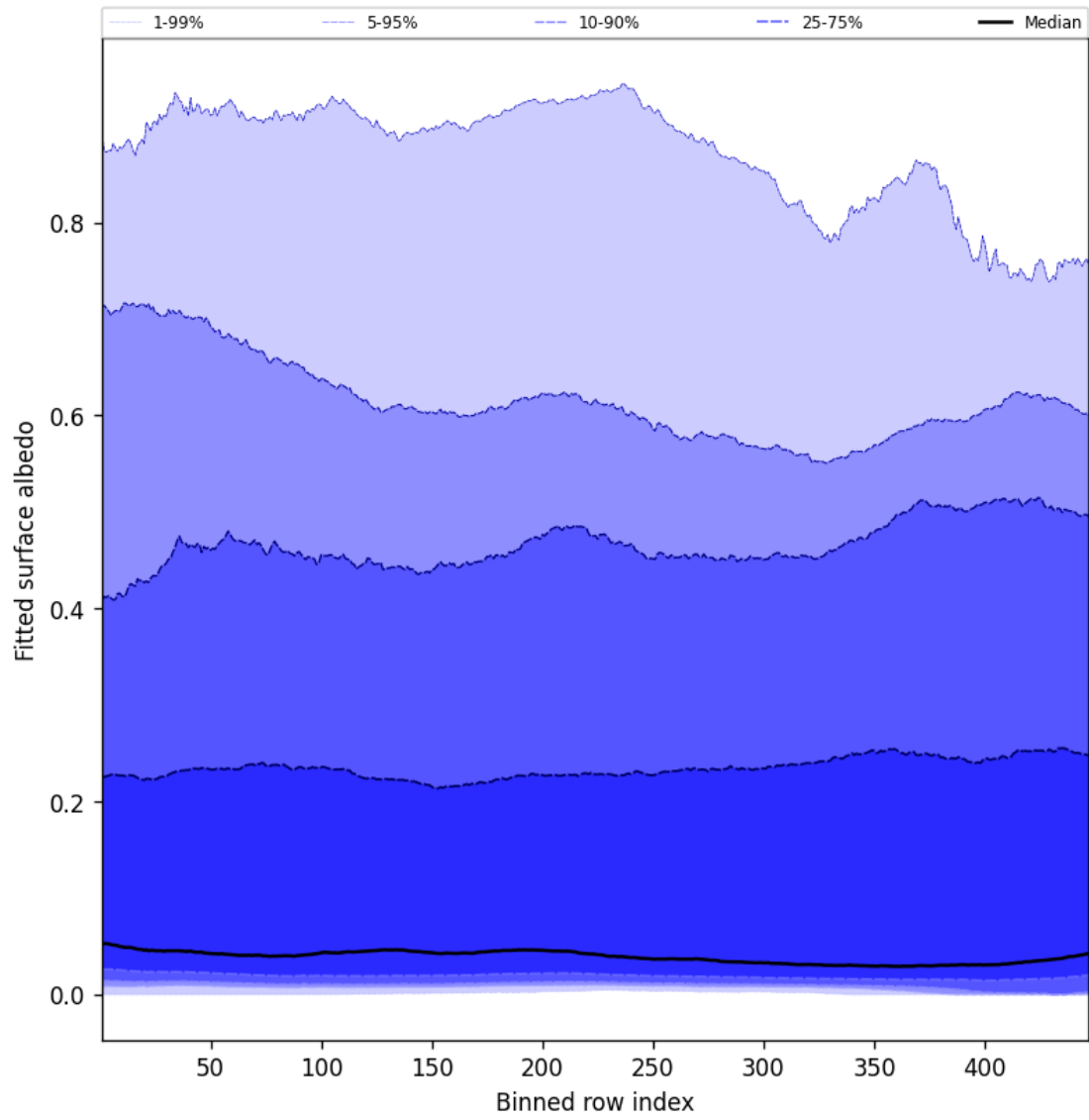
Figure 61: Along track statistics of “Fitted surface albedo” for 2025-08-19 to 2025-08-20
