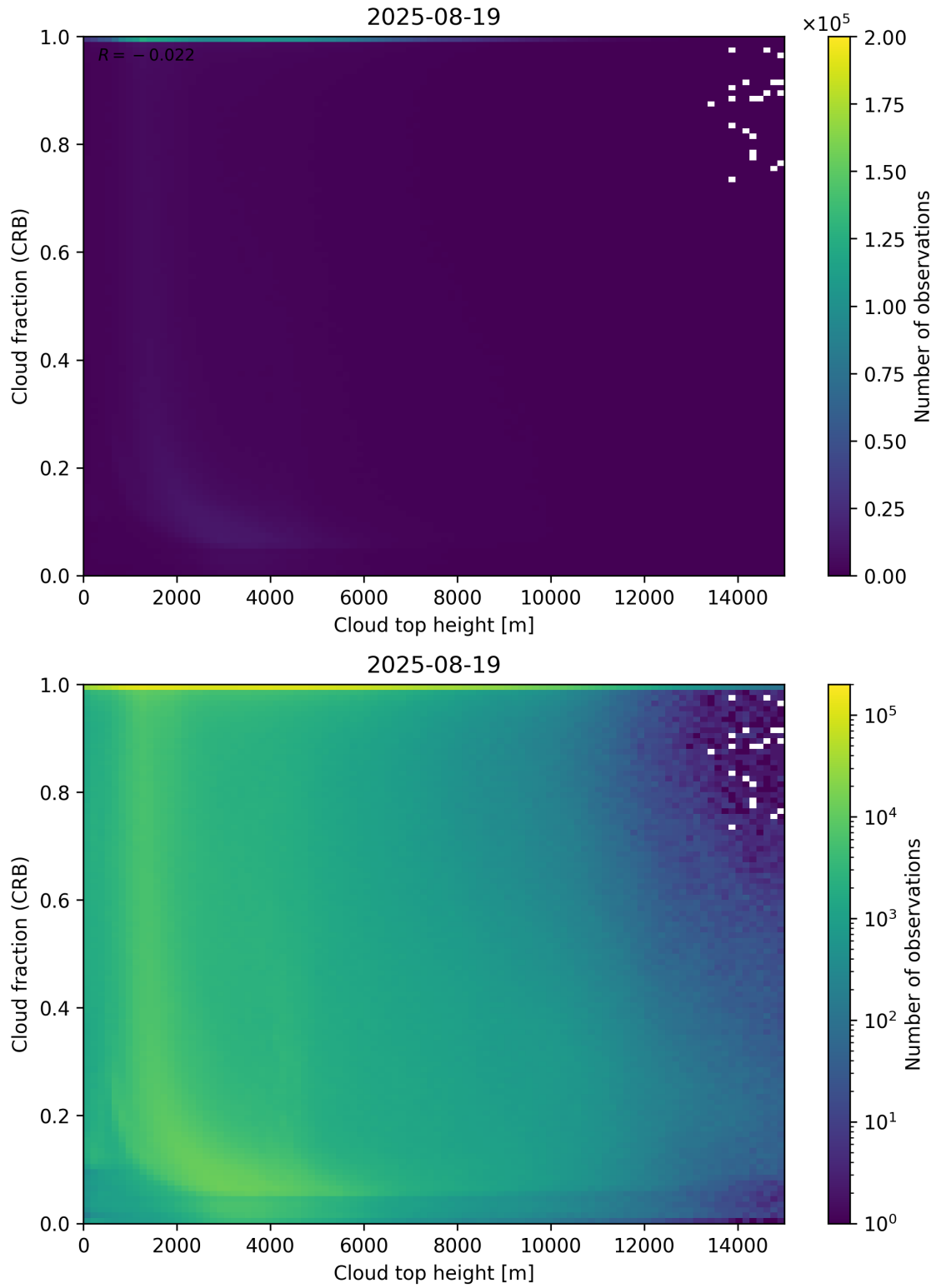
Figure 88: Scatter density plot of “Cloud top height” against “Cloud fraction (CRB)” for 2025-08-19 to 2025-08-20.
