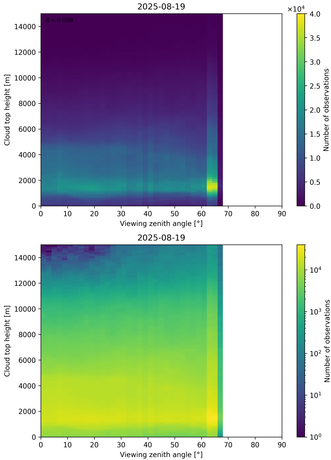
Figure 112: Scatter density plot of “Viewing zenith angle” against “Cloud top height” for 2025-08-19 to 2025-08-20.
