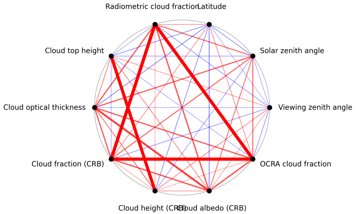
Figure 1: Map of correlation graph for 2025-08-19 to 2025-08-20.
