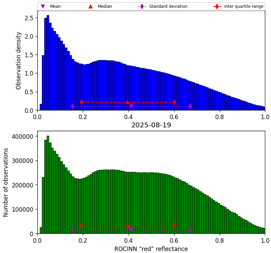
Figure 53: Histogram of “ROCINN “red” reflectance” for 2025-08-19 to 2025-08-20
