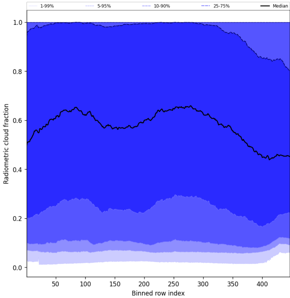
Figure 55: Along track statistics of “Radiometric cloud fraction” for 2025-08-19 to 2025-08-20
