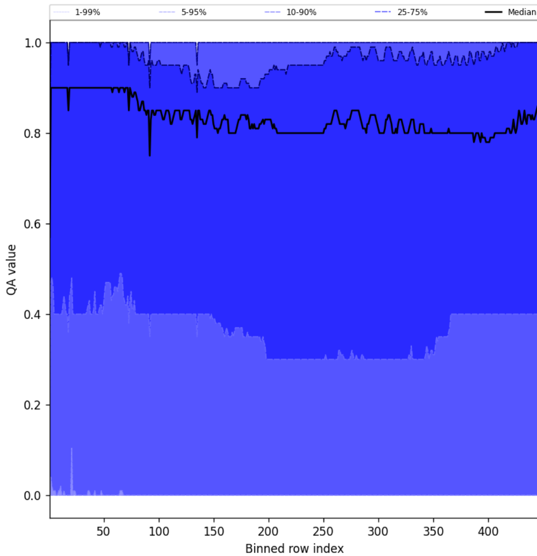
Figure 54: Along track statistics of “QA value” for 2025-08-19 to 2025-08-20
