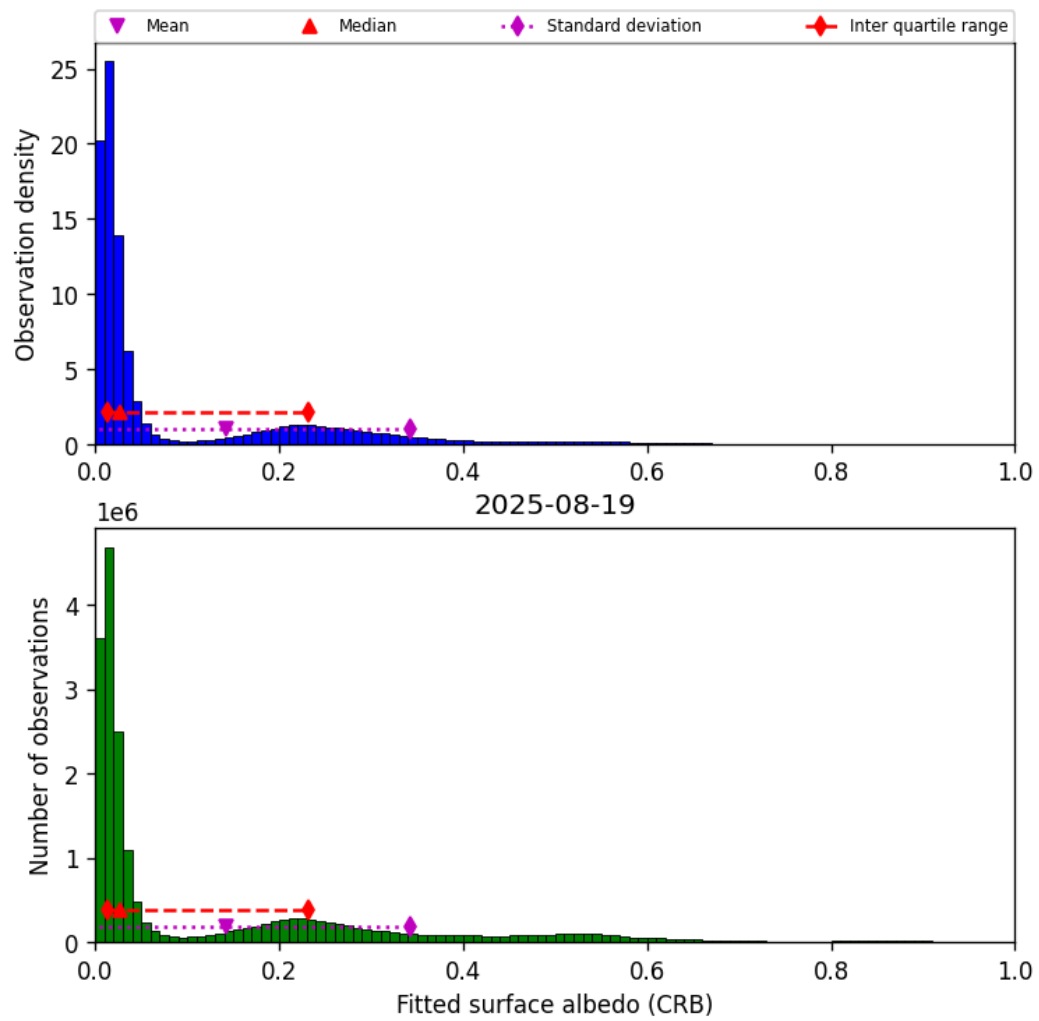
Figure 46: Histogram of “Fitted surface albedo (CRB)” for 2025-08-19 to 2025-08-20
