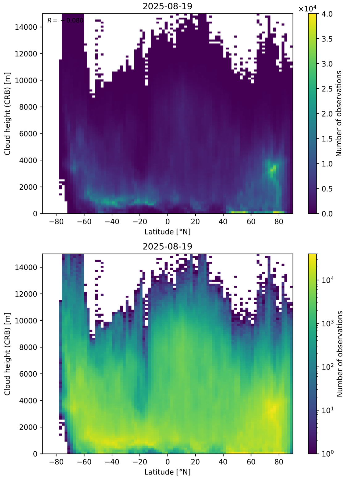
Figure 95: Scatter density plot of “Latitude” against “Cloud height (CRB)” for 2025-08-19 to 2025-08-20.
