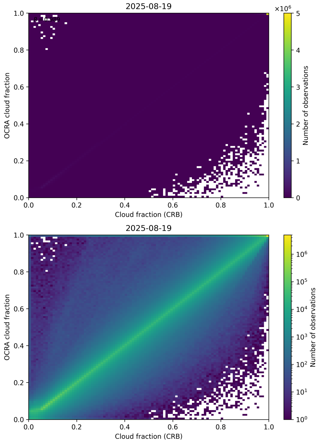
Figure 78: Scatter density plot of “Cloud fraction (CRB)” against “OCRA cloud fraction” for 2025-08-19 to 2025-08-20.
