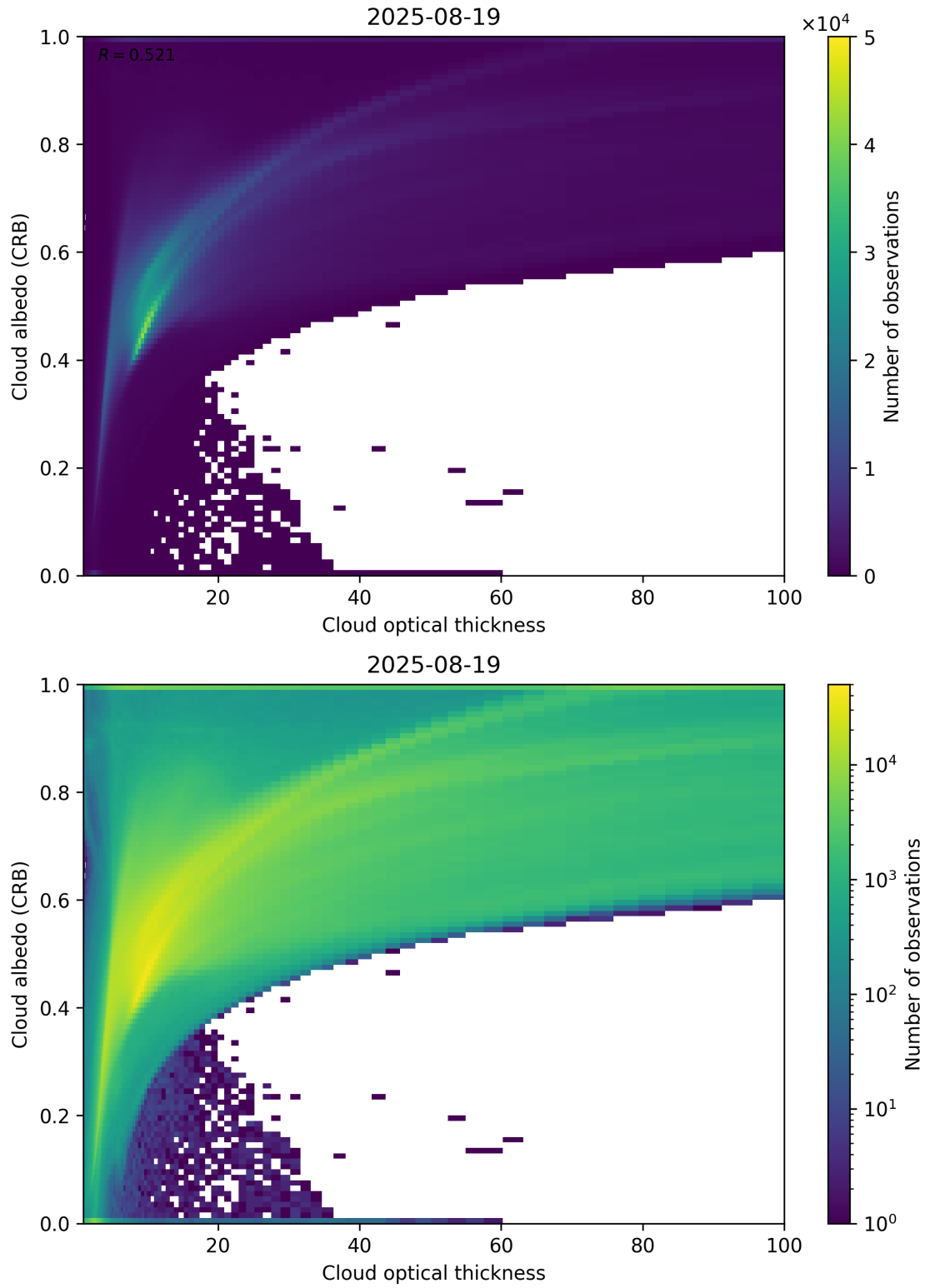
Figure 82: Scatter density plot of “Cloud optical thickness” against “Cloud albedo (CRB)” for 2025-08-19 to 2025-08-20.
