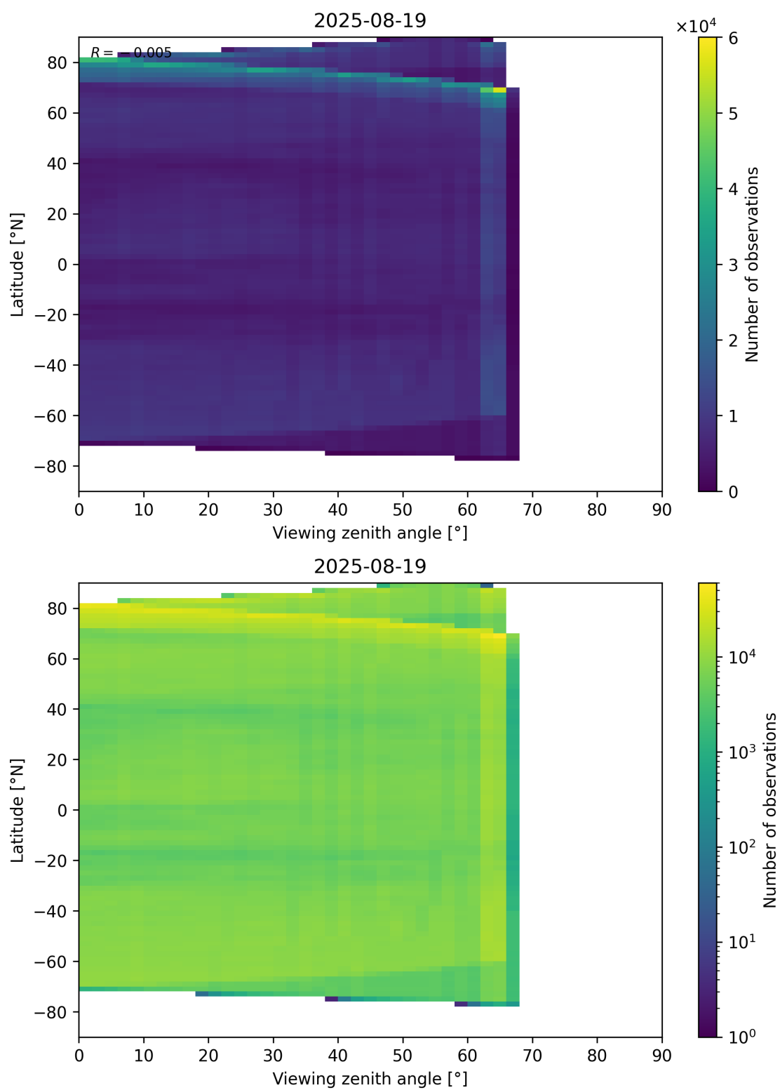
Figure 113: Scatter density plot of “Viewing zenith angle” against “Latitude” for 2025-08-19 to 2025-08-20.
