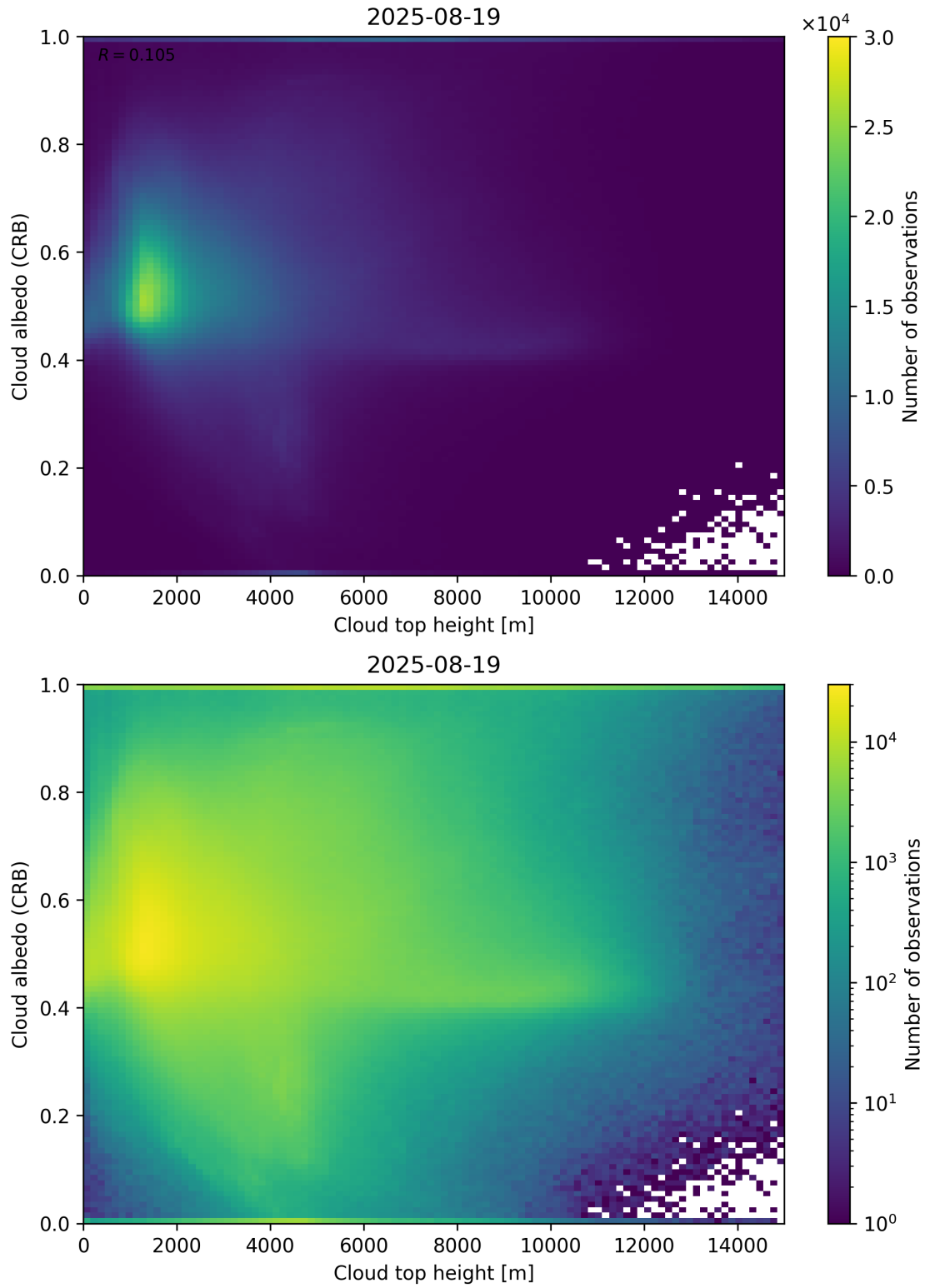
Figure 86: Scatter density plot of “Cloud top height” against “Cloud albedo (CRB)” for 2025-08-19 to 2025-08-20.
