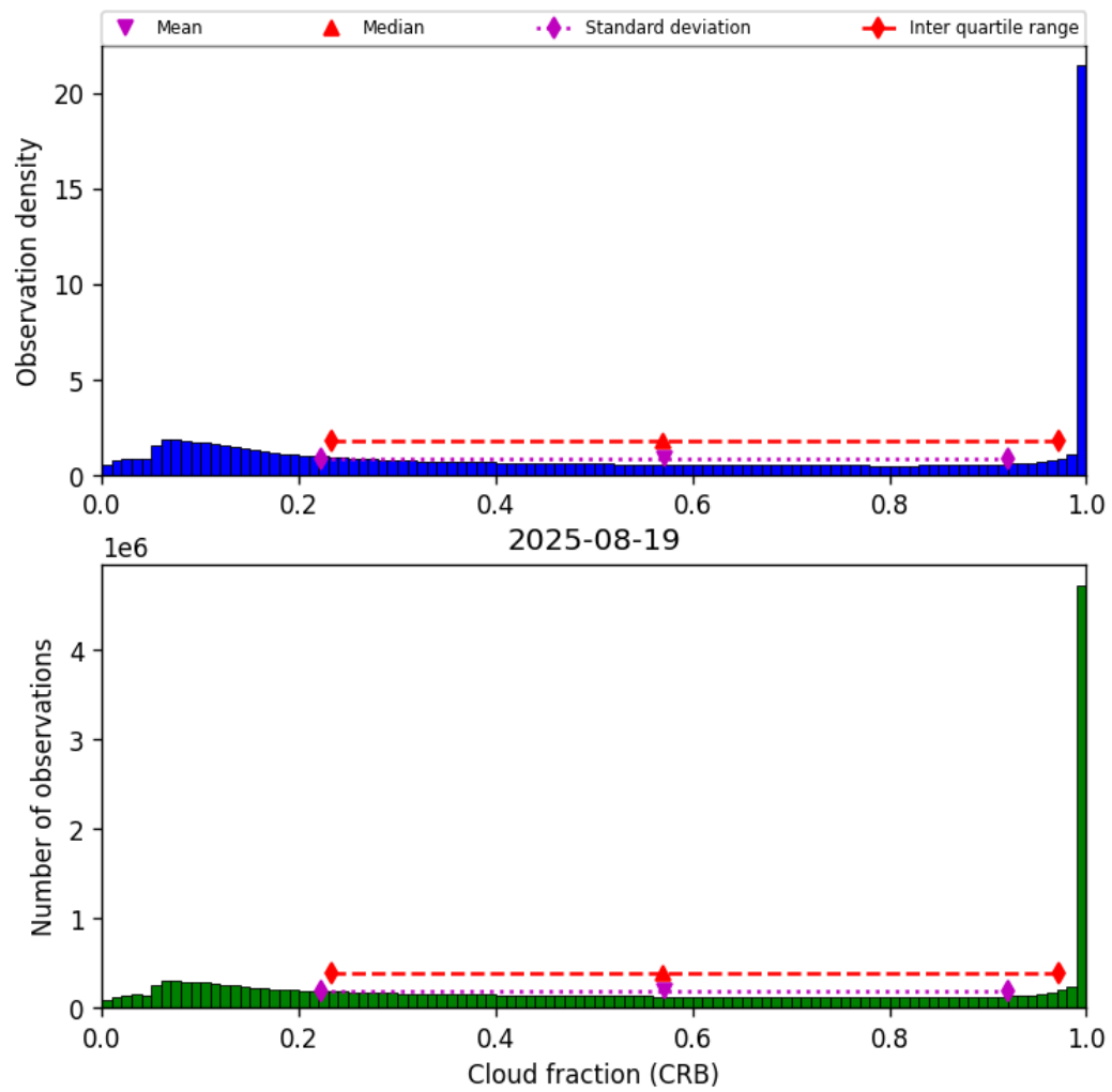
Figure 42: Histogram of “Cloud fraction (CRB)” for 2025-08-19 to 2025-08-20
