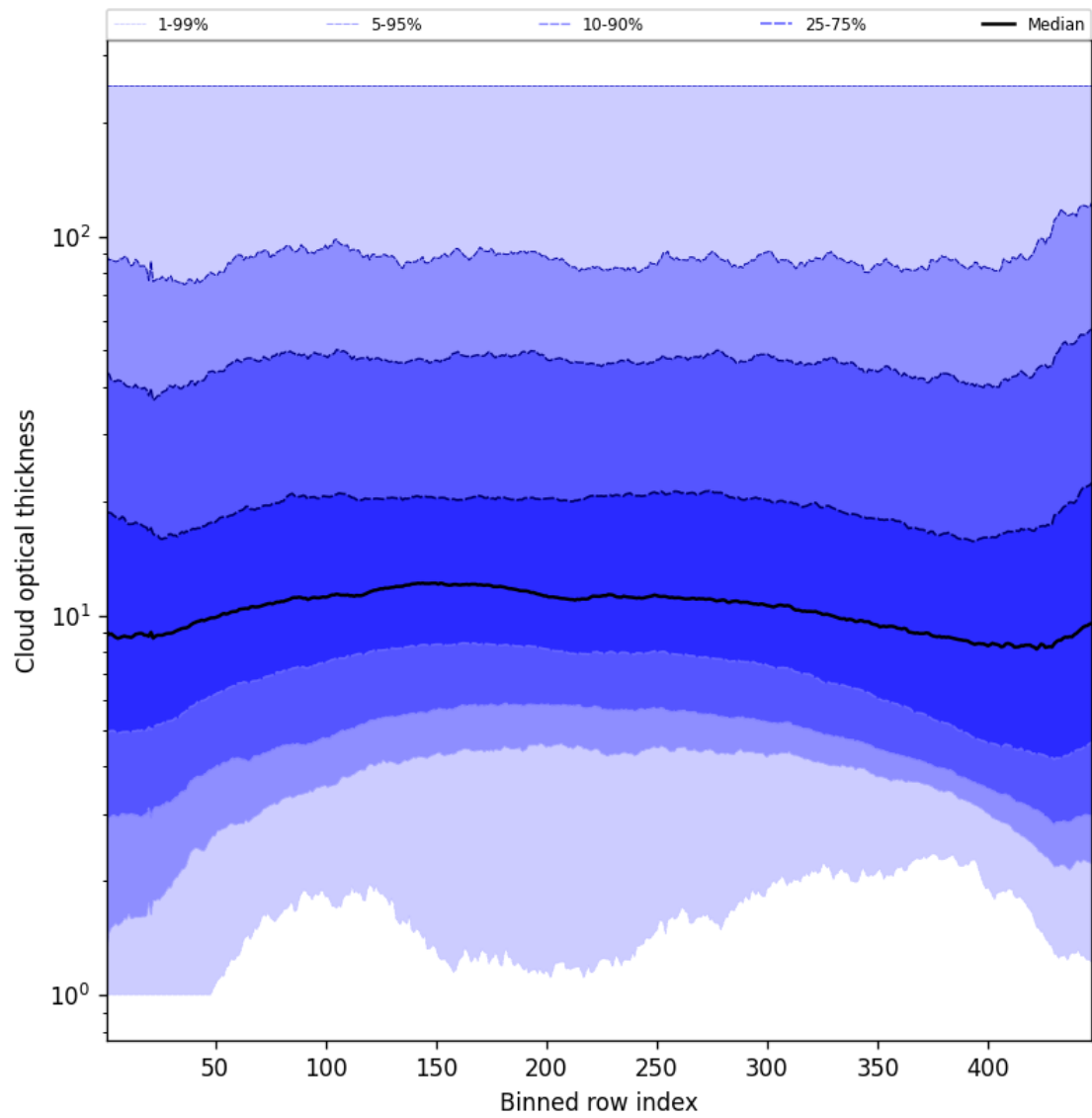
Figure 57: Along track statistics of “Cloud optical thickness” for 2025-08-19 to 2025-08-20
