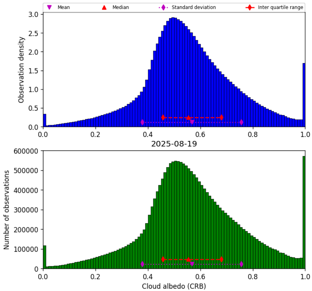
Figure 44: Histogram of “Cloud albedo (CRB)” for 2025-08-19 to 2025-08-20
