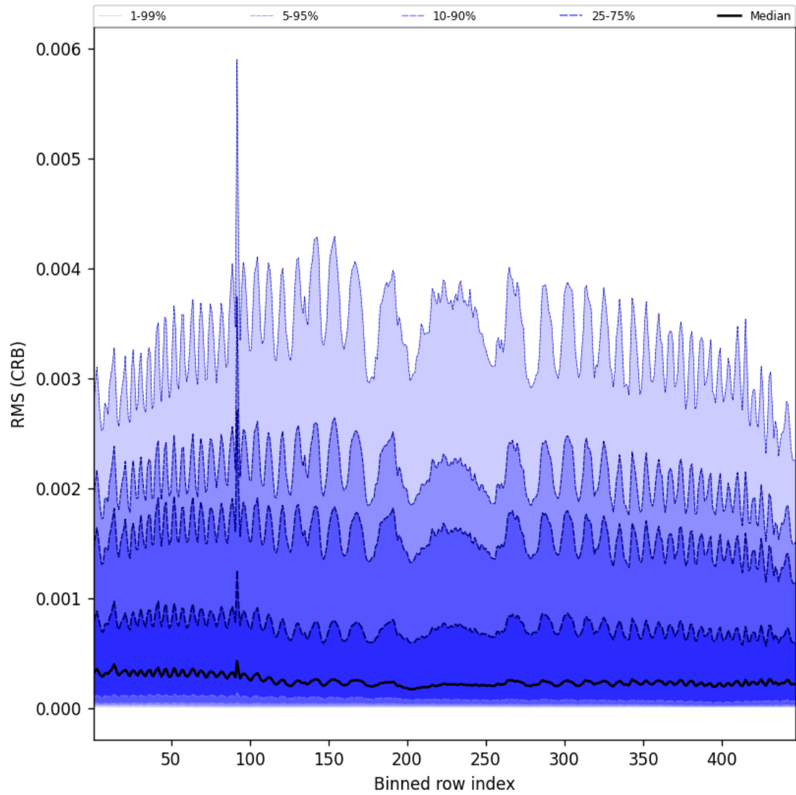
Figure 64: Along track statistics of “RMS (CRB)” for 2025-08-19 to 2025-08-20
