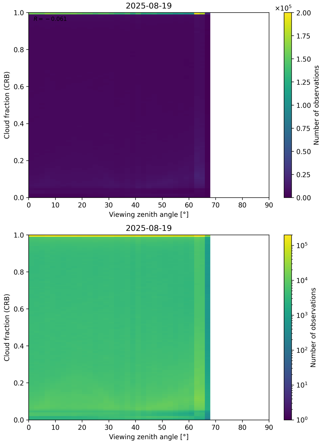
Figure 109: Scatter density plot of “Viewing zenith angle” against “Cloud fraction (CRB)” for 2025-08-19 to 2025-08-20.
