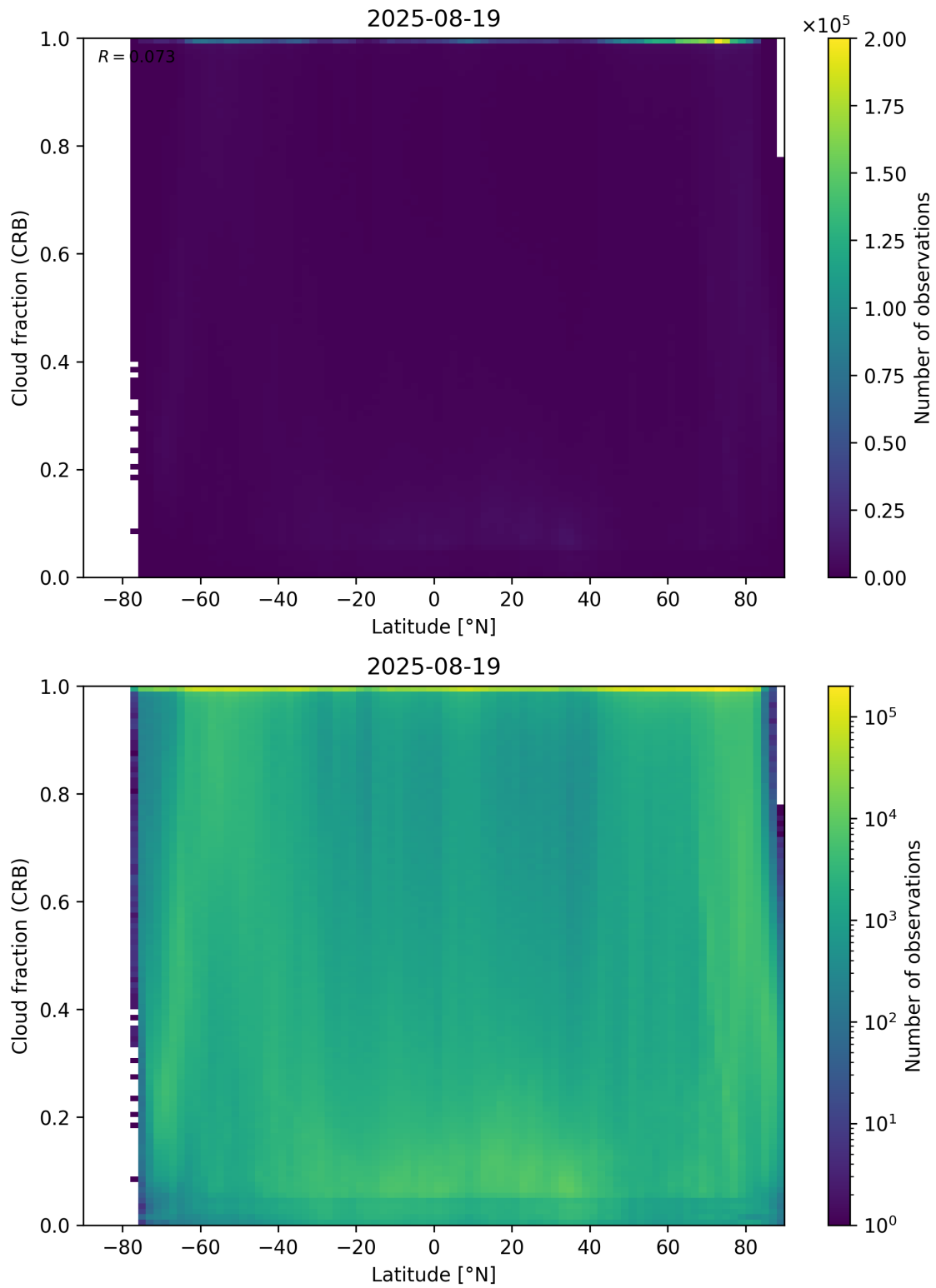
Figure 94: Scatter density plot of “Latitude” against “Cloud fraction (CRB)” for 2025-08-19 to 2025-08-20.
