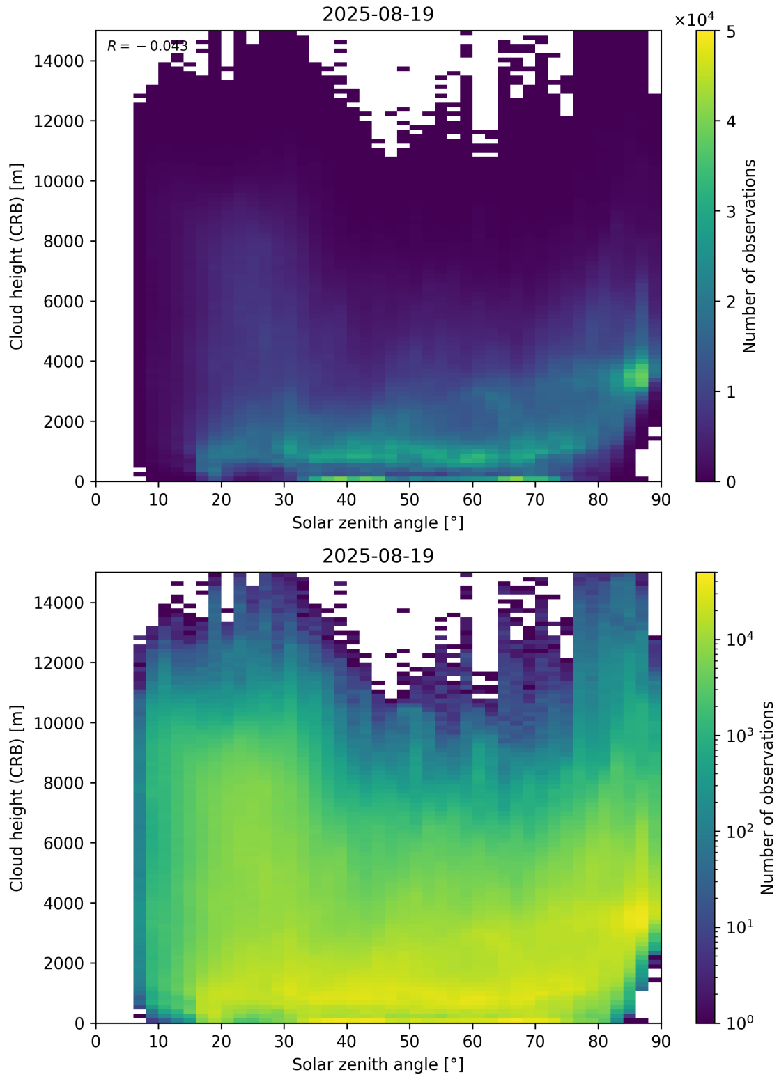
Figure 102: Scatter density plot of “Solar zenith angle” against “Cloud height (CRB)” for 2025-08-19 to 2025-08-20.
