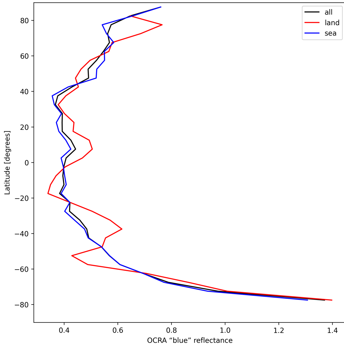
Figure 35: Zonal average of “OCRA “blue” reflectance” for 2025-08-19 to 2025-08-20.
