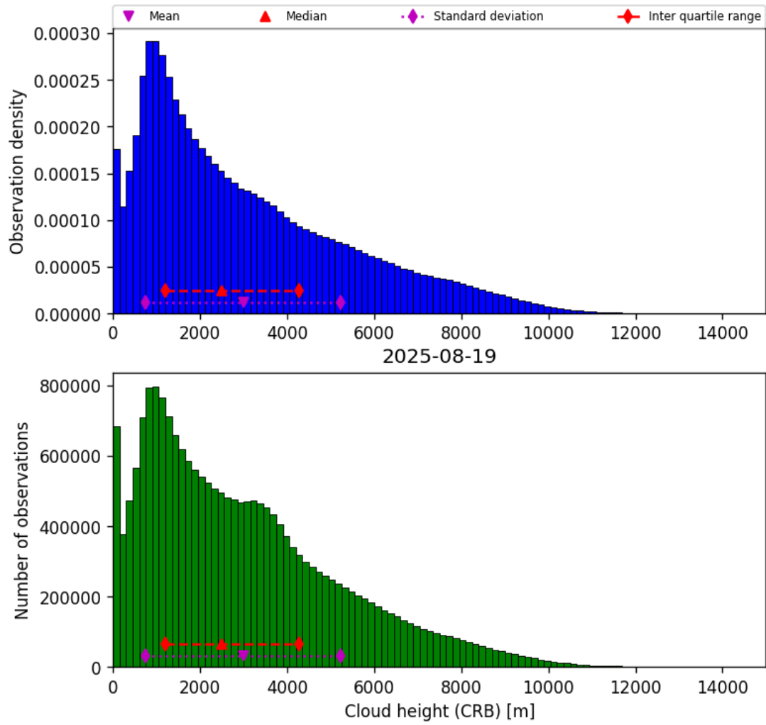
Figure 43: Histogram of “Cloud height (CRB)” for 2025-08-19 to 2025-08-20
