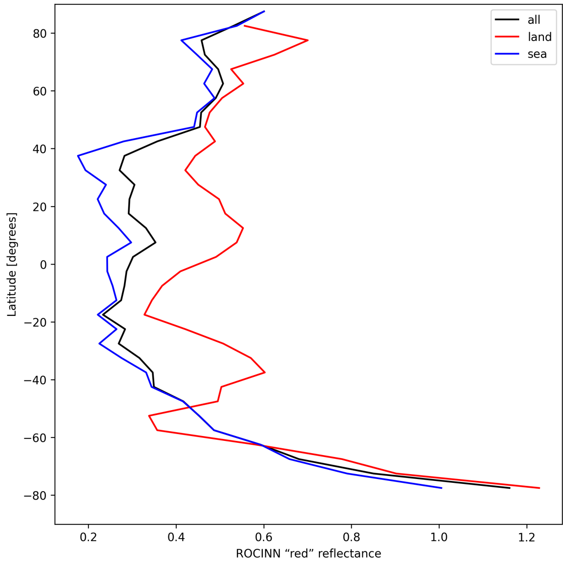
Figure 37: Zonal average of “ROCINN “red” reflectance” for 2025-08-19 to 2025-08-20.
