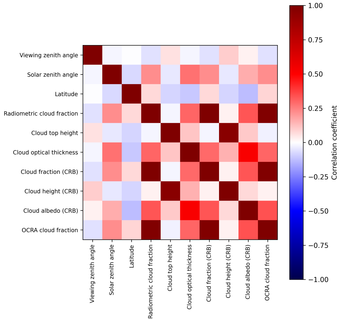
Figure 2: Map of correlation matrix for 2025-08-19 to 2025-08-20.
