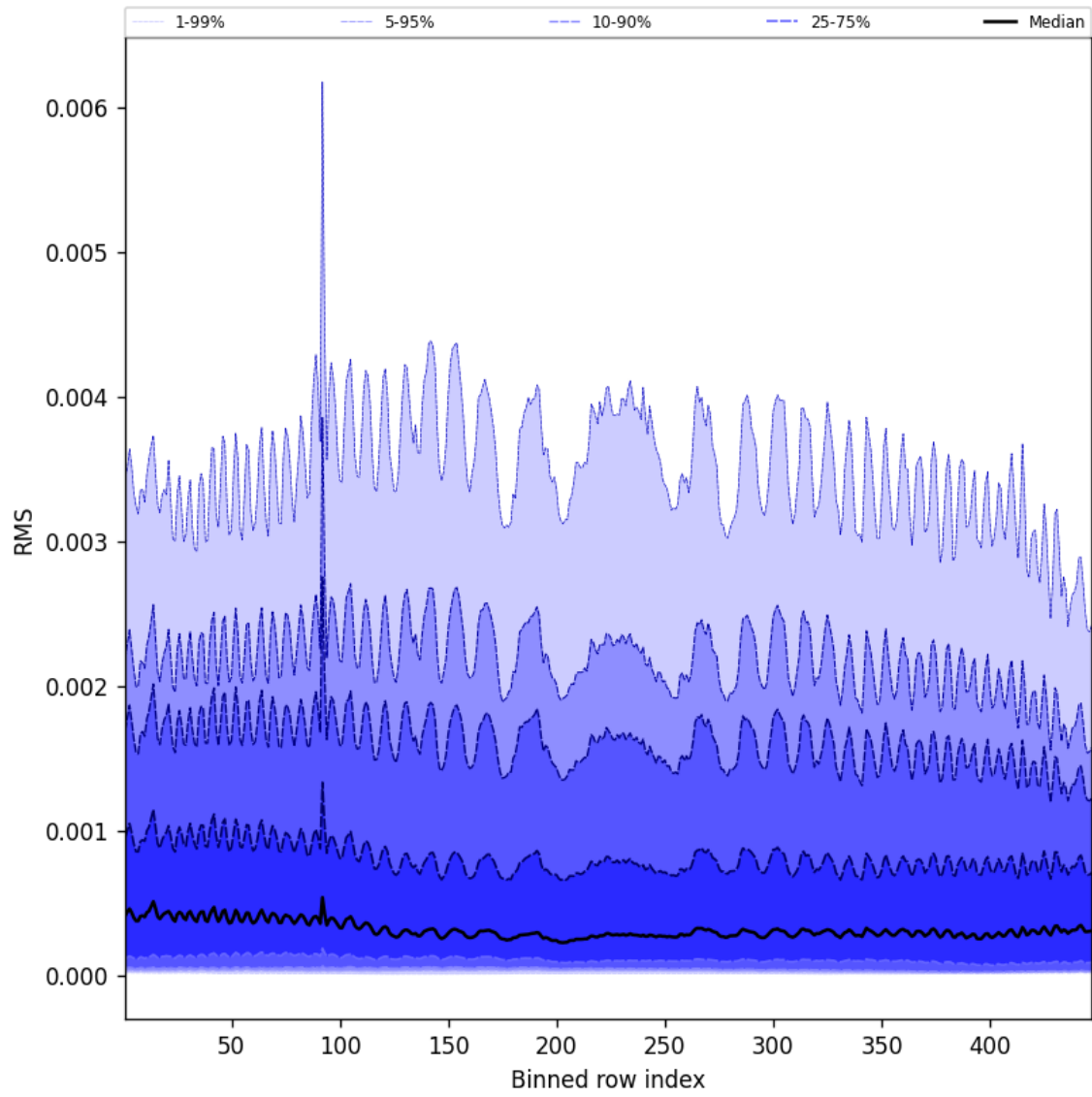
Figure 63: Along track statistics of “RMS” for 2025-08-19 to 2025-08-20
