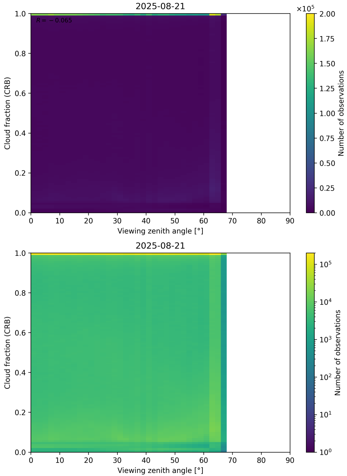
Figure 109: Scatter density plot of “Viewing zenith angle” against “Cloud fraction (CRB)” for 2025-08-20 to 2025-08-22.
