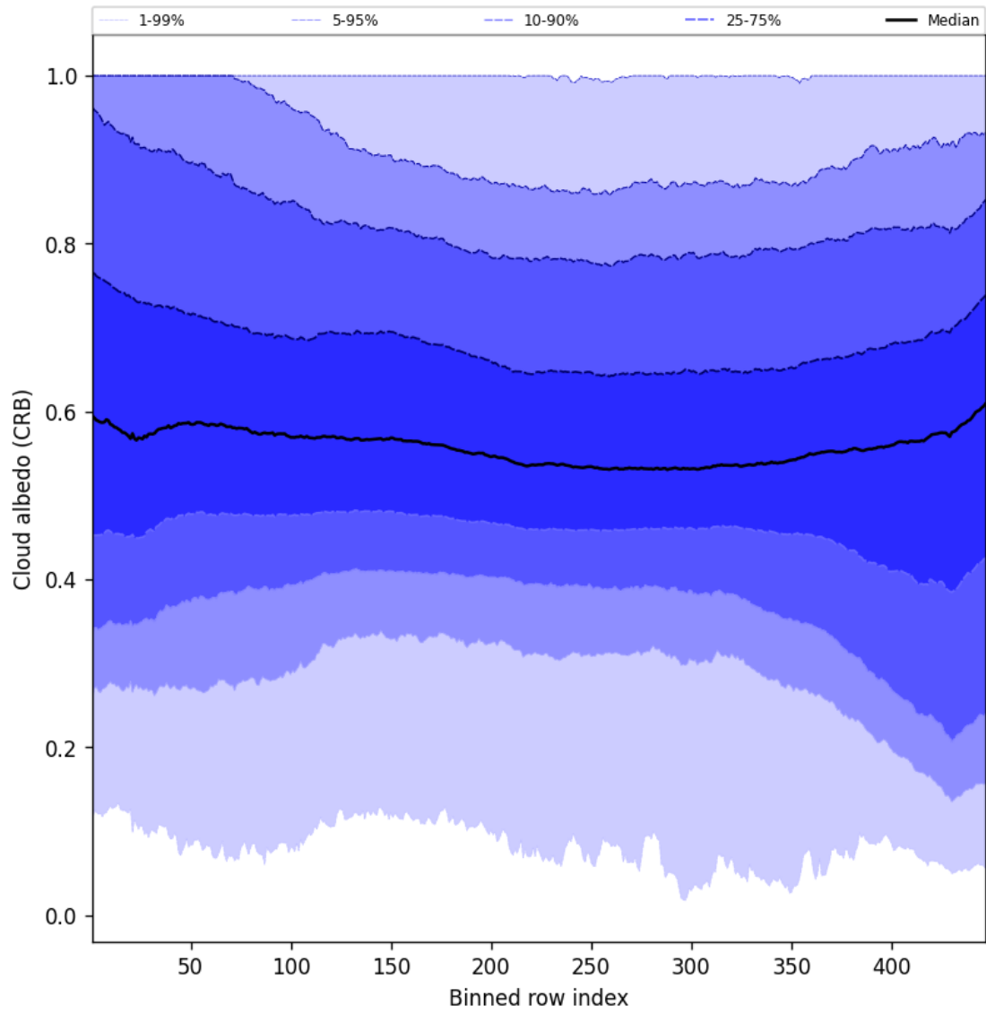
Figure 60: Along track statistics of “Cloud albedo (CRB)” for 2025-08-20 to 2025-08-22
