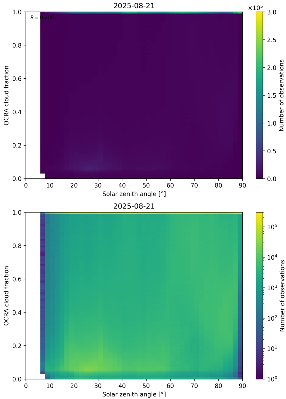
Figure 100: Scatter density plot of “Solar zenith angle” against “OCRA cloud fraction” for 2025-08-20 to 2025-08-22.
