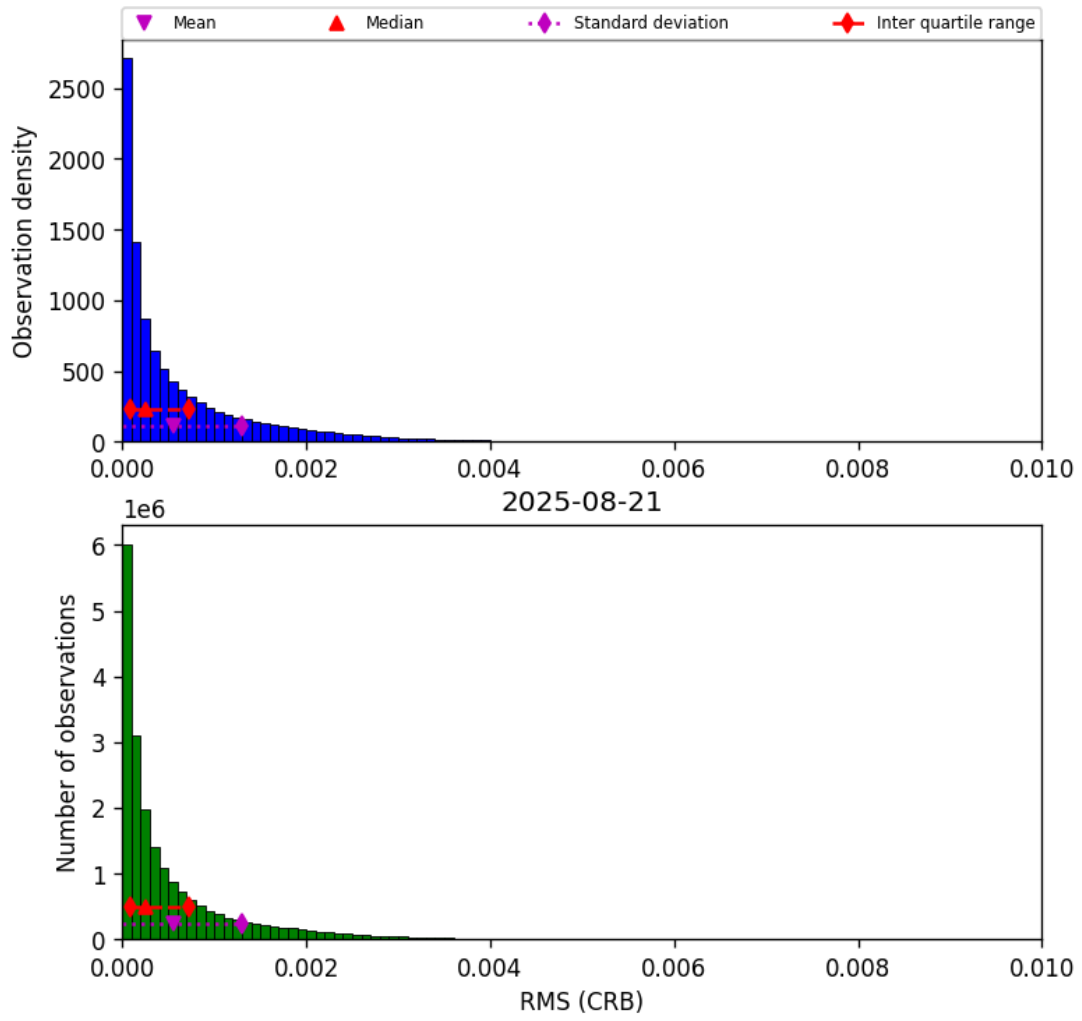
Figure 48: Histogram of “RMS (CRB)” for 2025-08-20 to 2025-08-22
