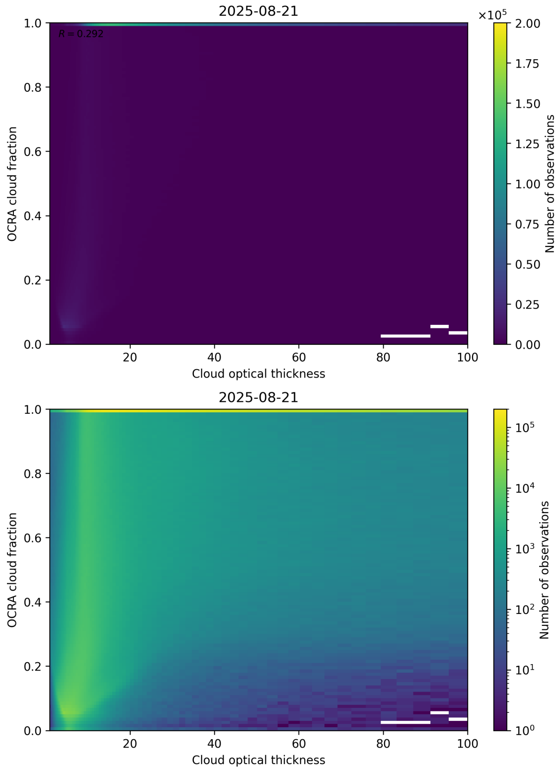
Figure 83: Scatter density plot of “Cloud optical thickness” against “OCRA cloud fraction” for 2025-08-20 to 2025-08-22.
