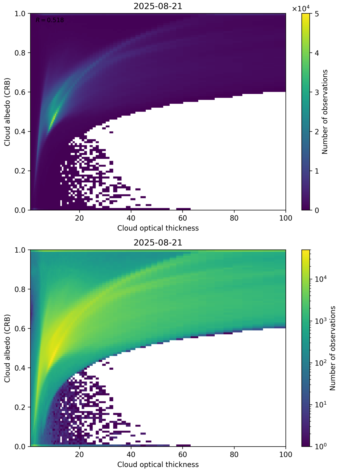
Figure 82: Scatter density plot of “Cloud optical thickness” against “Cloud albedo (CRB)” for 2025-08-20 to 2025-08-22.
