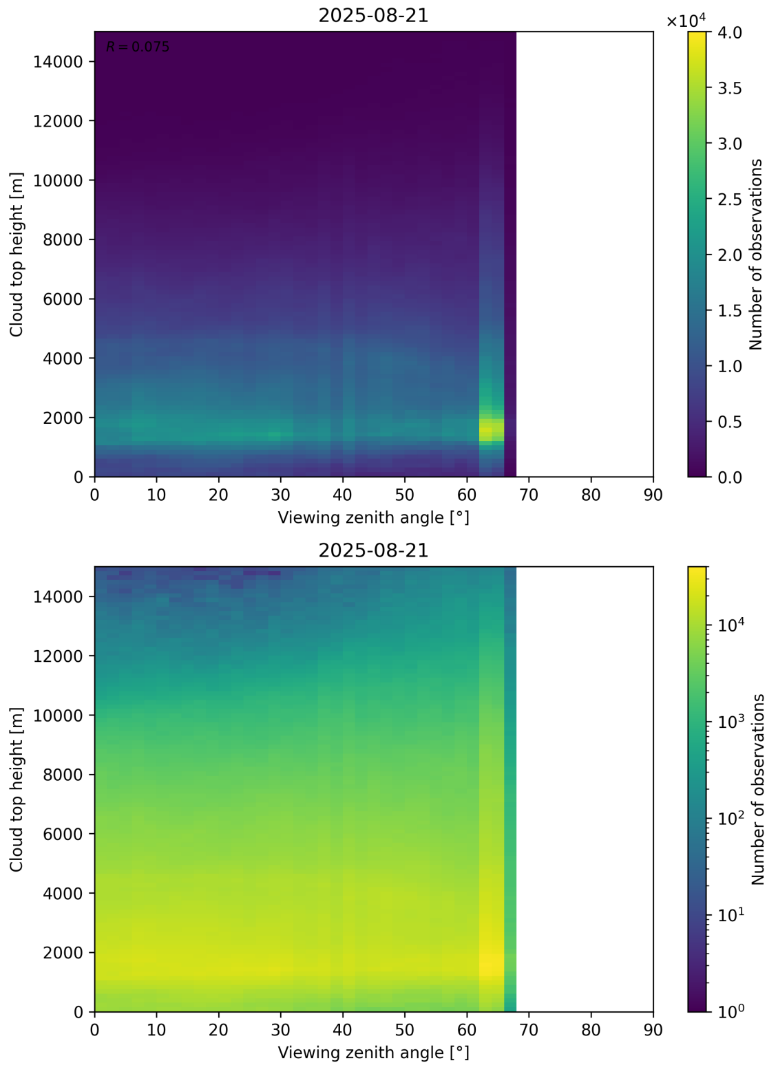
Figure 112: Scatter density plot of “Viewing zenith angle” against “Cloud top height” for 2025-08-20 to 2025-08-22.
