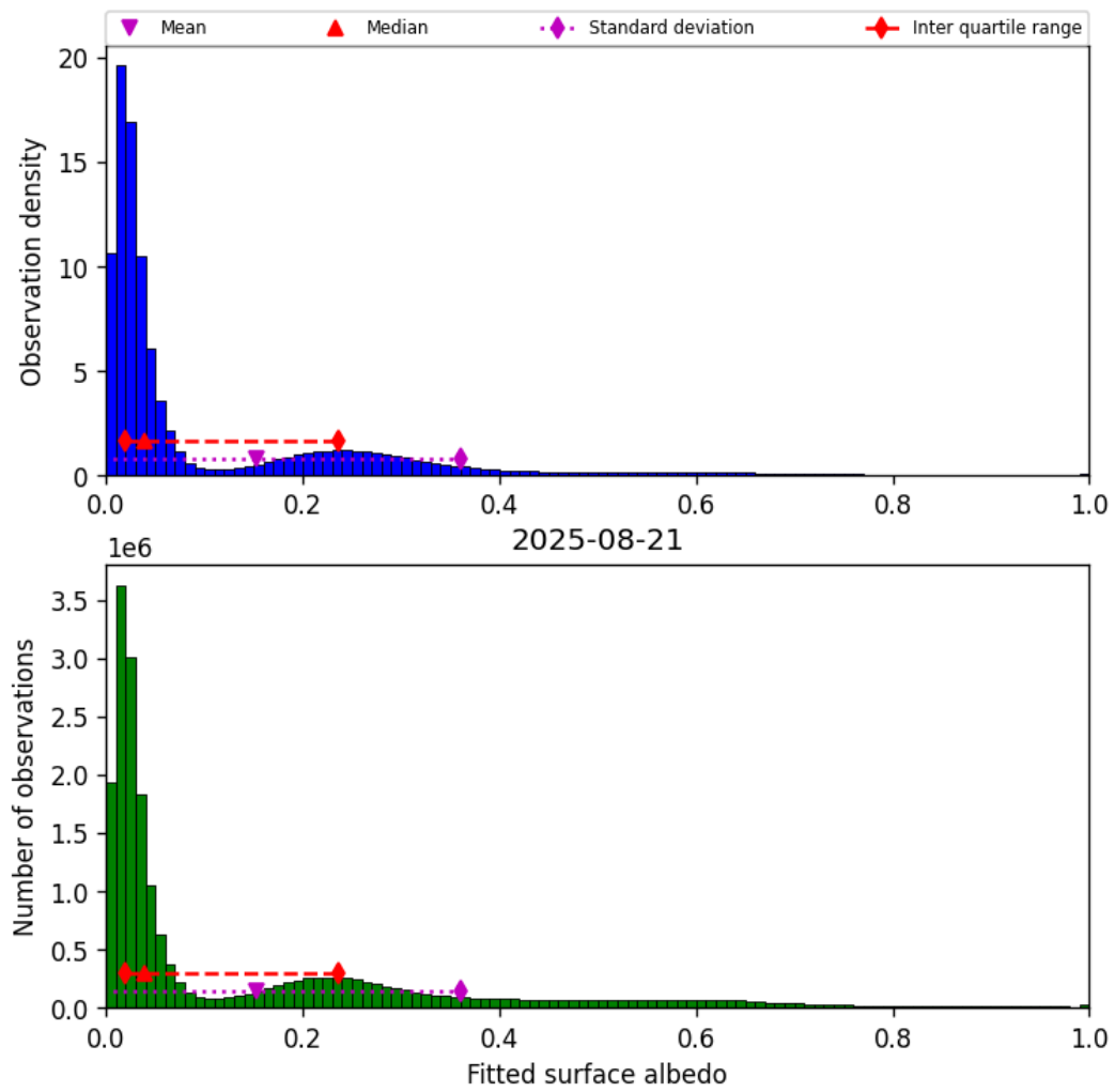
Figure 45: Histogram of “Fitted surface albedo” for 2025-08-20 to 2025-08-22
