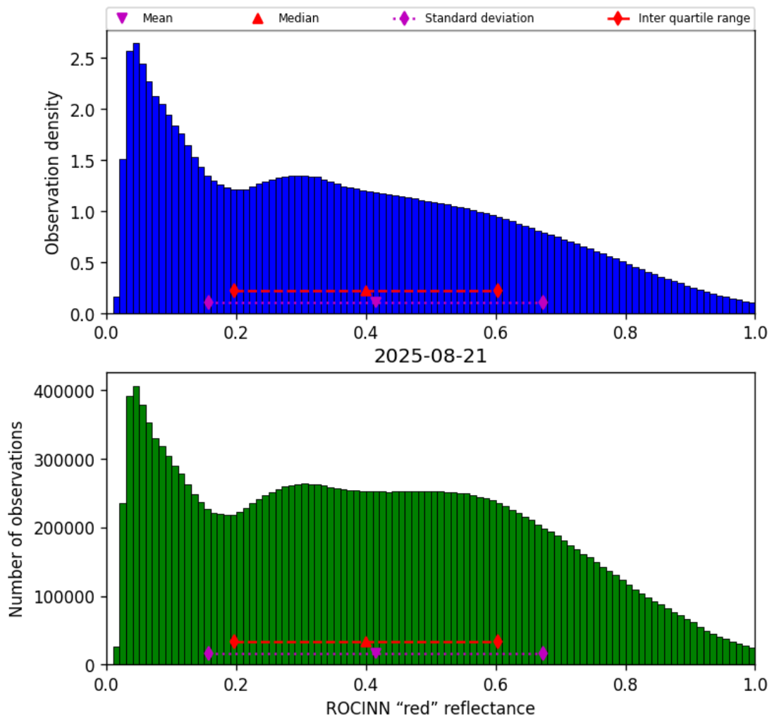
Figure 53: Histogram of “ROCINN “red” reflectance” for 2025-08-20 to 2025-08-22
