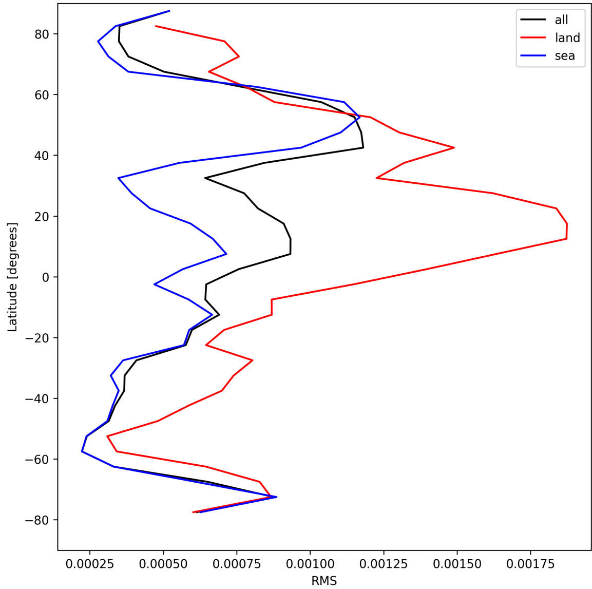
Figure 31: Zonal average of “RMS” for 2025-08-20 to 2025-08-22.
