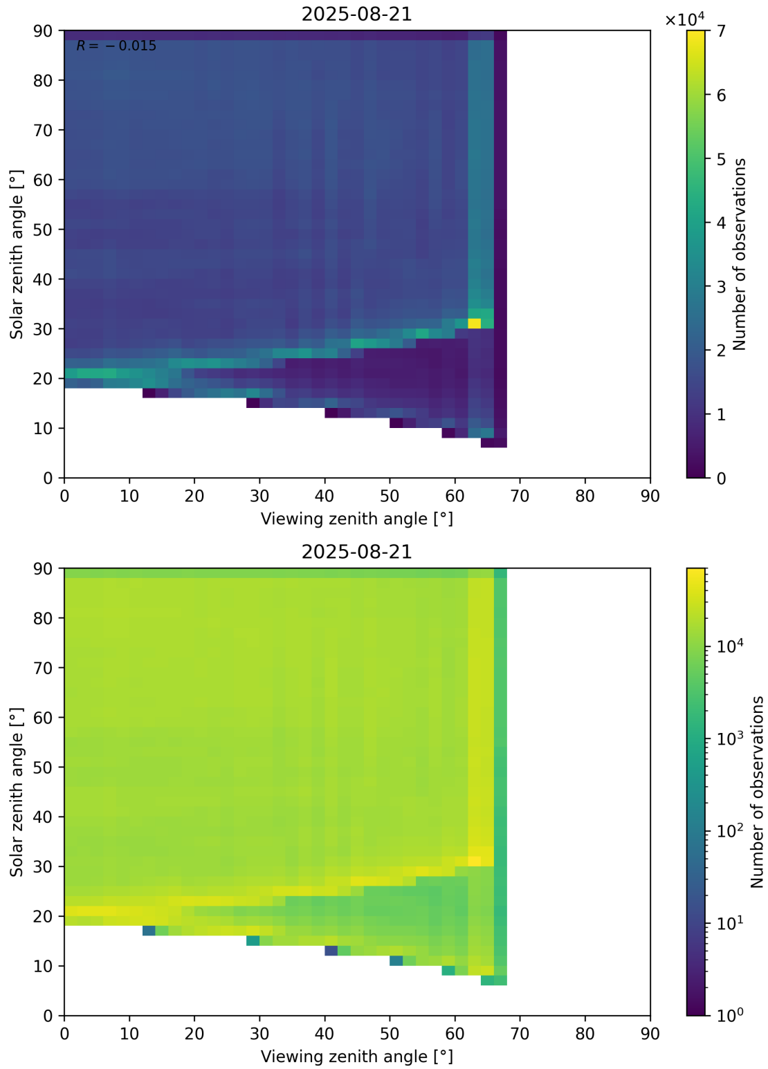
Figure 114: Scatter density plot of “Viewing zenith angle” against “Solar zenith angle” for 2025-08-20 to 2025-08-22.
