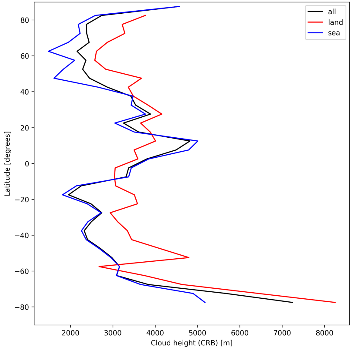
Figure 27: Zonal average of “Cloud height (CRB)” for 2025-08-20 to 2025-08-22.
