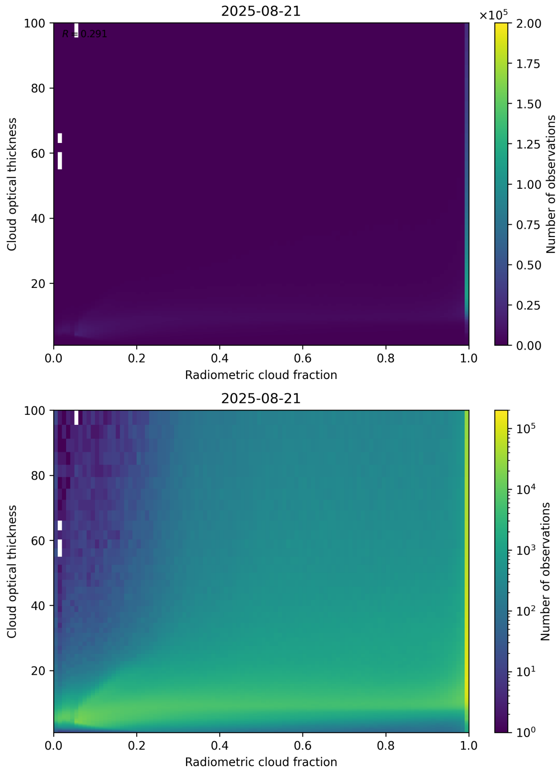
Figure 75: Scatter density plot of “Radiometric cloud fraction” against “Cloud optical thickness” for 2025-08-20 to 2025-08-22.
