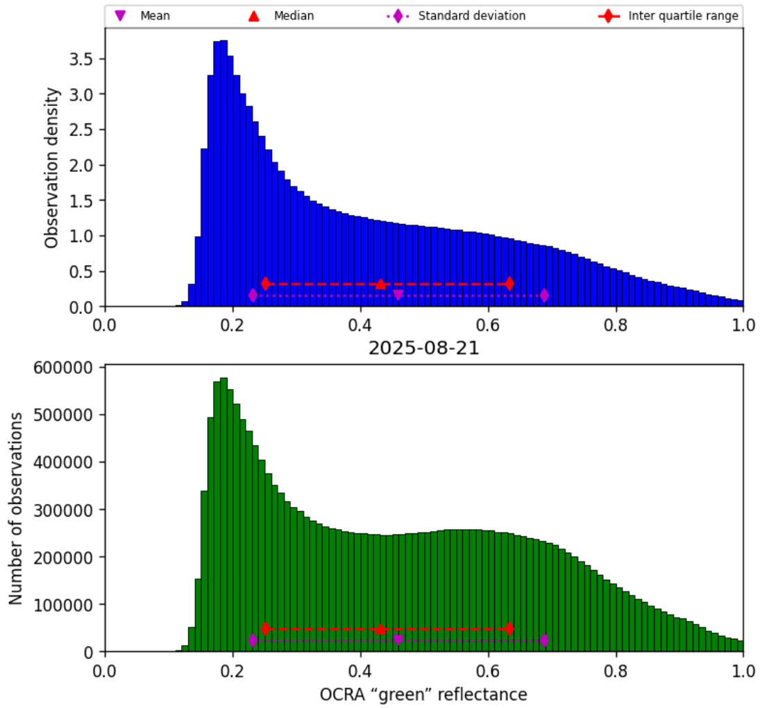
Figure 52: Histogram of “OCRA “green” reflectance” for 2025-08-20 to 2025-08-22
