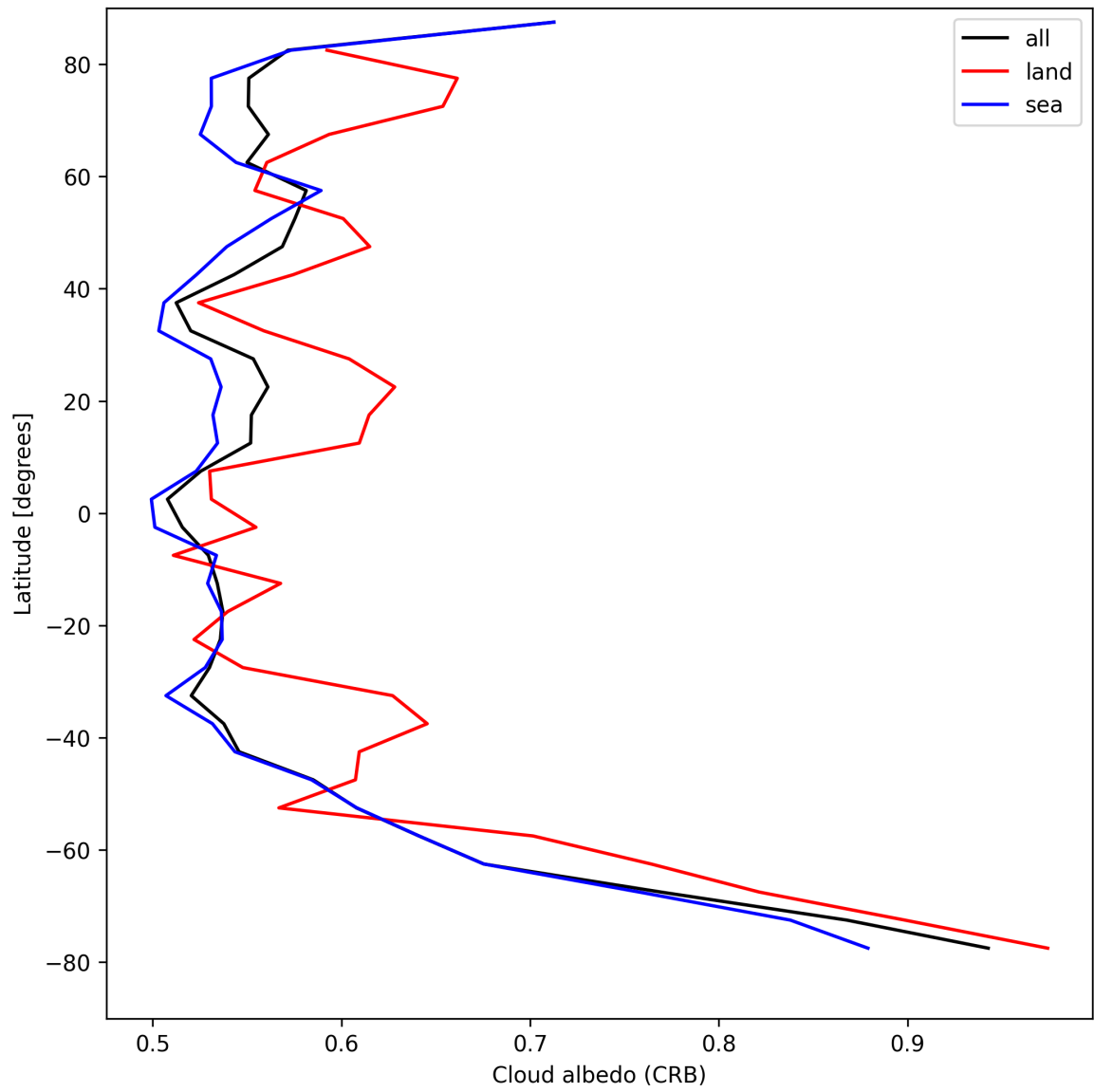
Figure 28: Zonal average of “Cloud albedo (CRB)” for 2025-08-20 to 2025-08-22.
