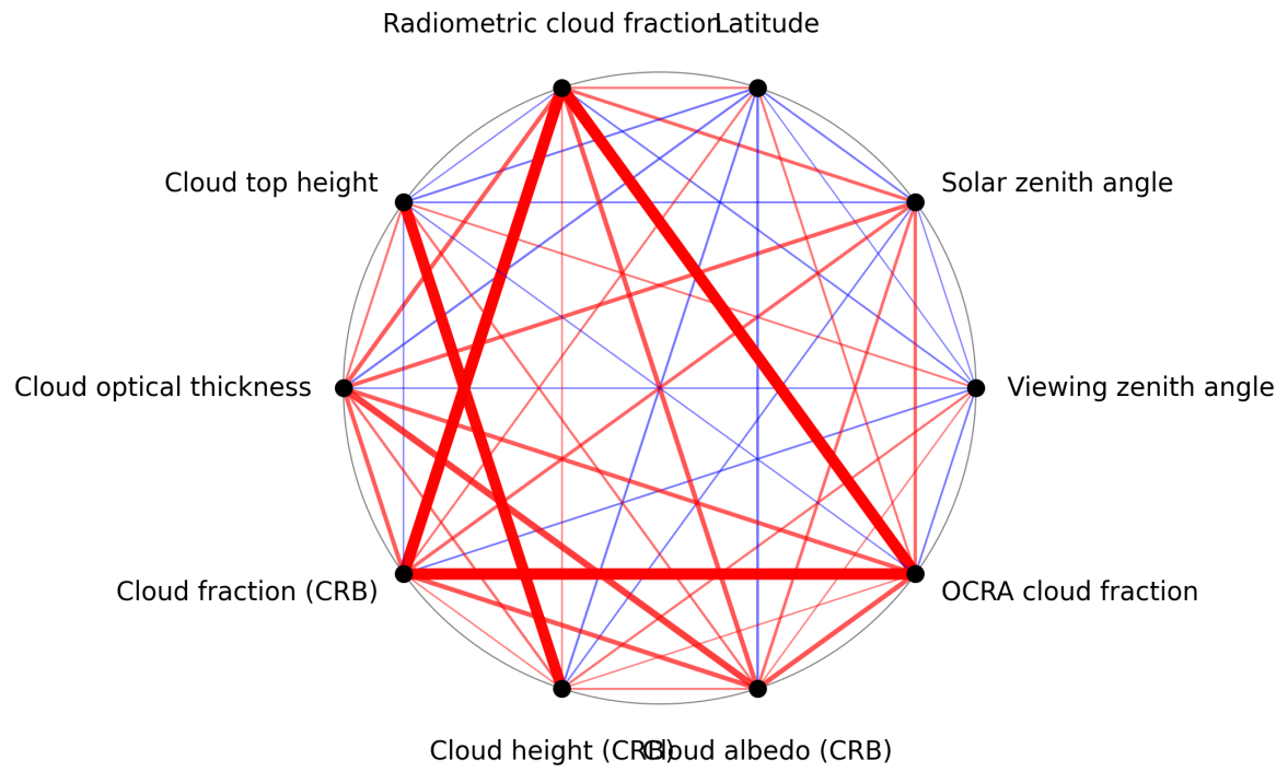
Figure 1: Map of correlation graph for 2025-08-20 to 2025-08-22.
