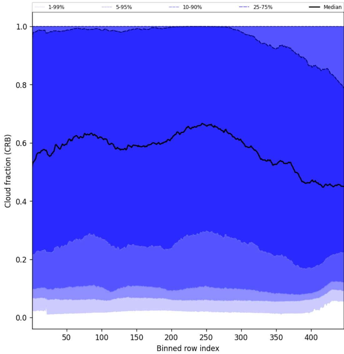
Figure 58: Along track statistics of “Cloud fraction (CRB)” for 2025-08-20 to 2025-08-22
