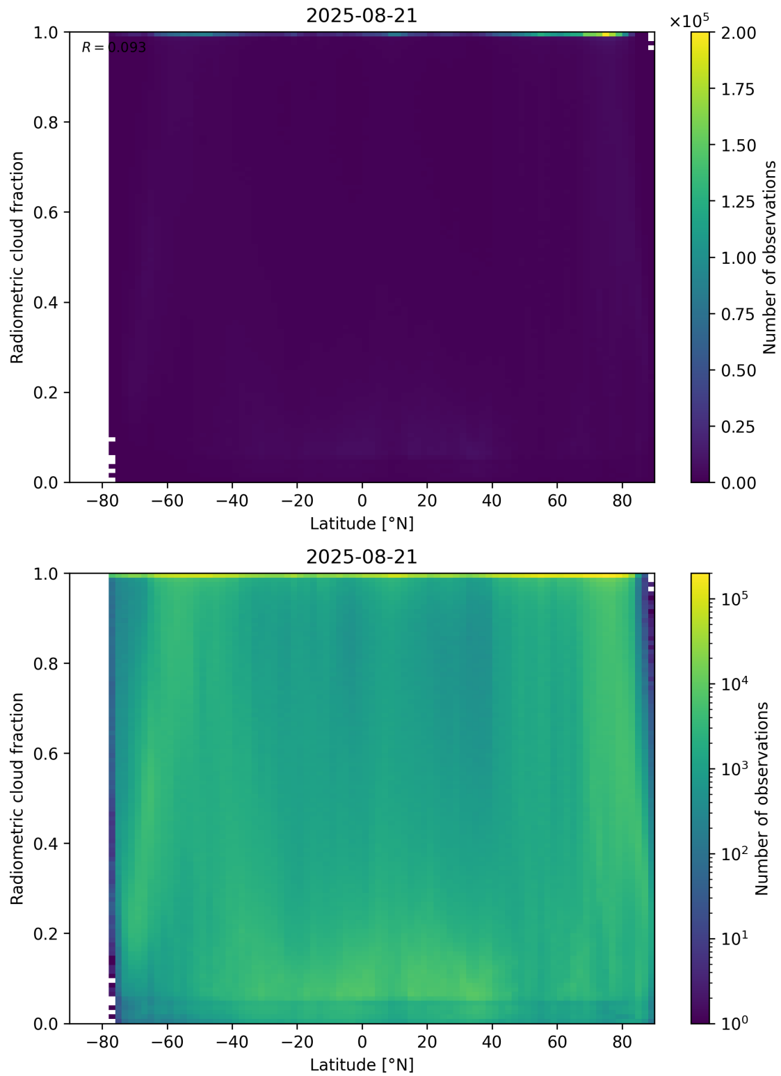
Figure 92: Scatter density plot of “Latitude” against “Radiometric cloud fraction” for 2025-08-20 to 2025-08-22.
