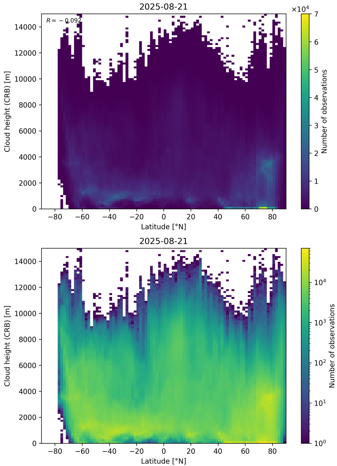
Figure 95: Scatter density plot of “Latitude” against “Cloud height (CRB)” for 2025-08-20 to 2025-08-22.
