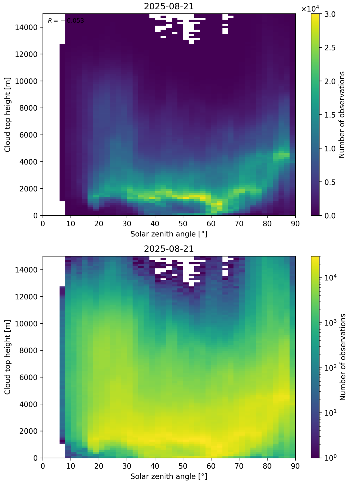
Figure 104: Scatter density plot of “Solar zenith angle” against “Cloud top height” for 2025-08-20 to 2025-08-22.
