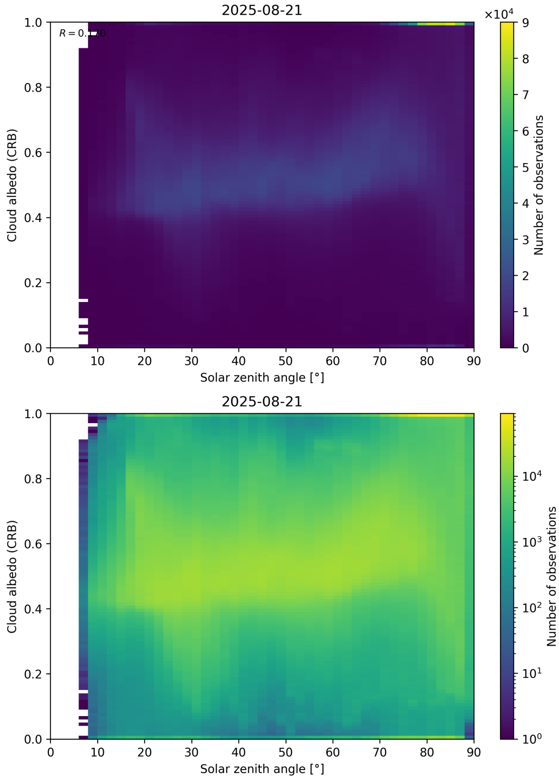
Figure 98: Scatter density plot of “Solar zenith angle” against “Cloud albedo (CRB)” for 2025-08-20 to 2025-08-22.
