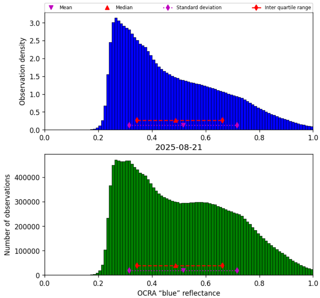
Figure 51: Histogram of “OCRA “blue” reflectance” for 2025-08-20 to 2025-08-22
