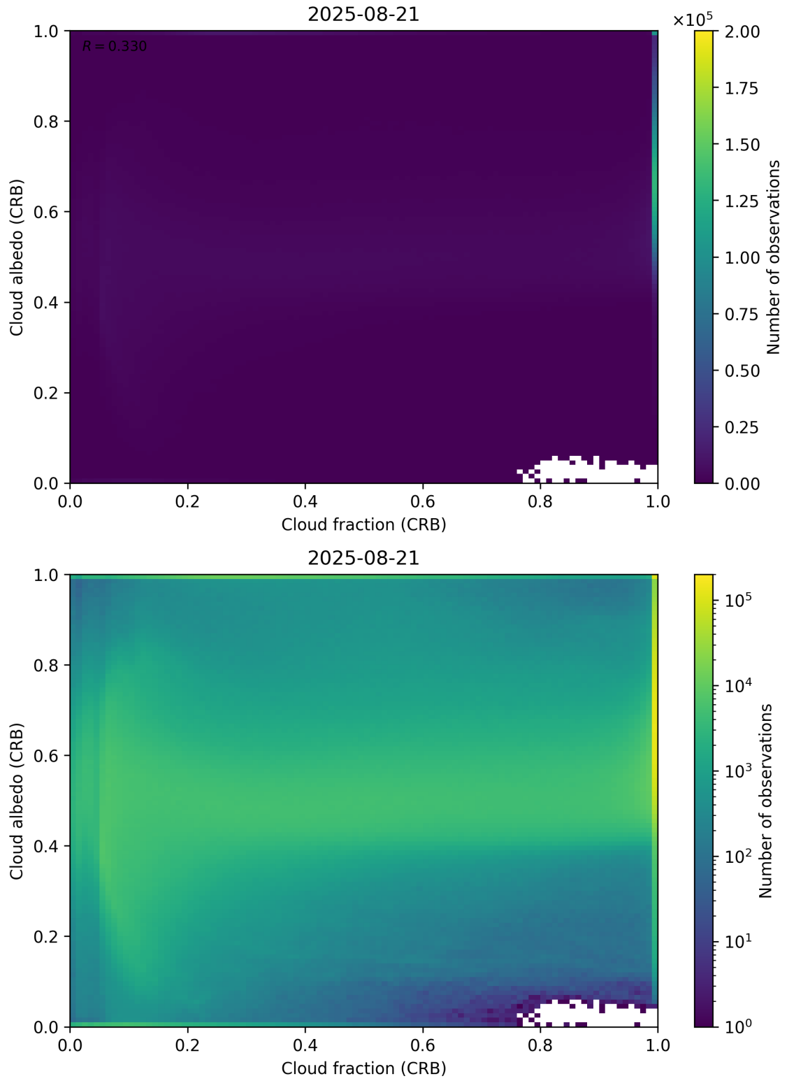
Figure 77: Scatter density plot of “Cloud fraction (CRB)” against “Cloud albedo (CRB)” for 2025-08-20 to 2025-08-22.
