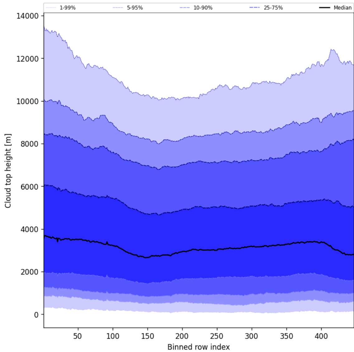
Figure 56: Along track statistics of “Cloud top height” for 2025-08-20 to 2025-08-22
