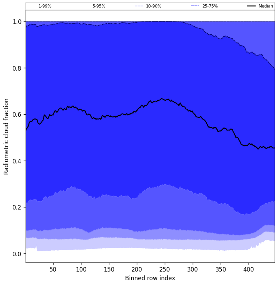
Figure 55: Along track statistics of “Radiometric cloud fraction” for 2025-08-20 to 2025-08-22
