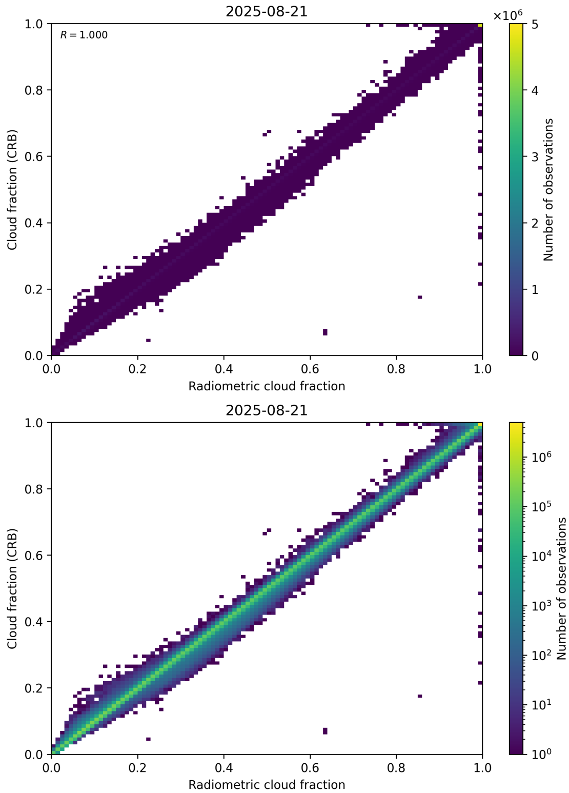
Figure 73: Scatter density plot of “Radiometric cloud fraction” against “Cloud fraction (CRB)” for 2025-08-20 to 2025-08-22.
