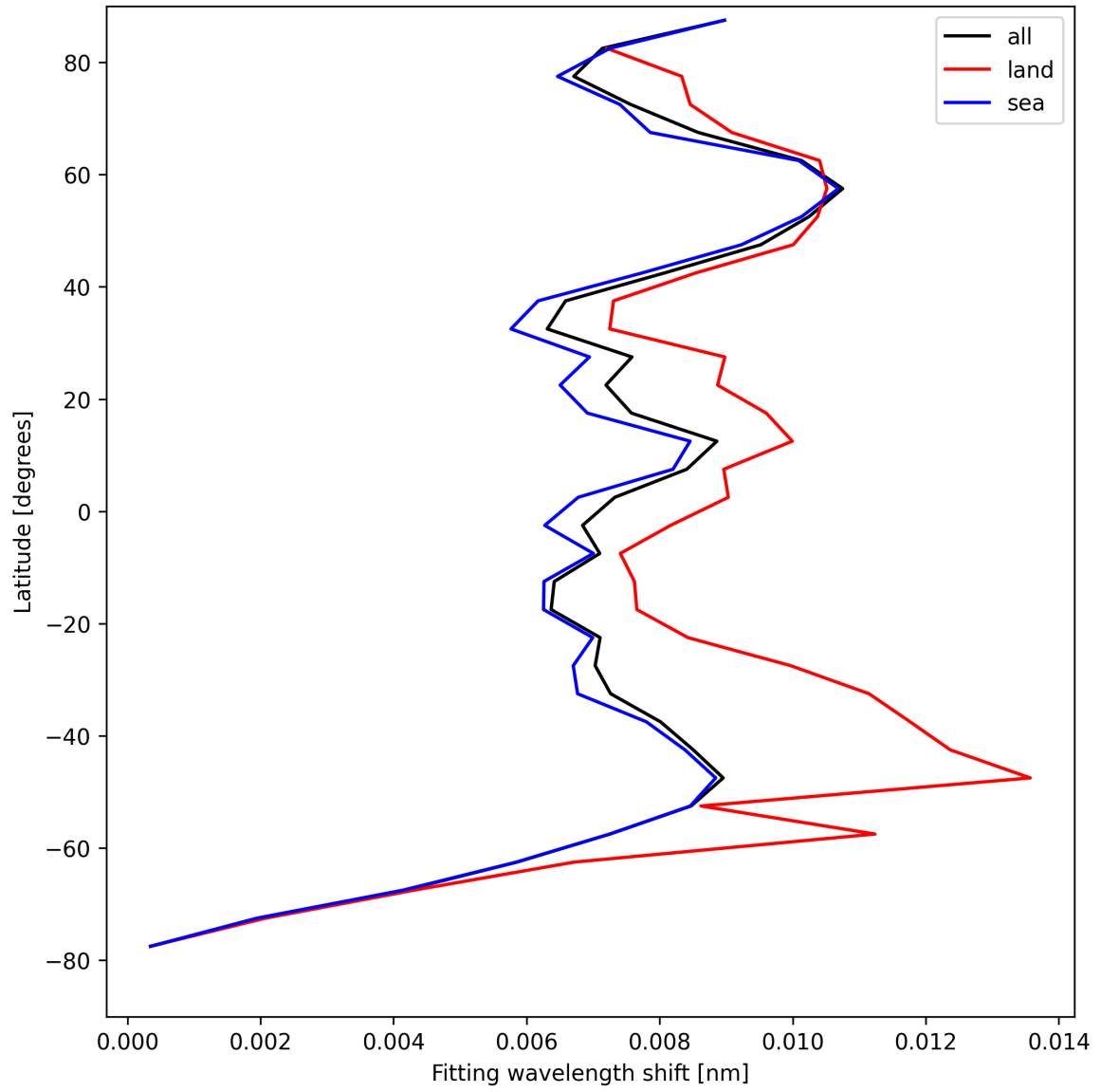
Figure 33: Zonal average of “Fitting wavelength shift” for 2025-08-20 to 2025-08-22.
