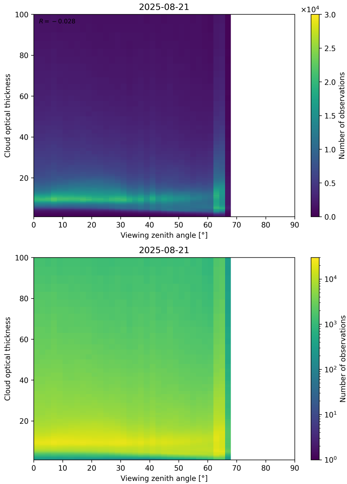
Figure 111: Scatter density plot of “Viewing zenith angle” against “Cloud optical thickness” for 2025-08-20 to 2025-08-22.
