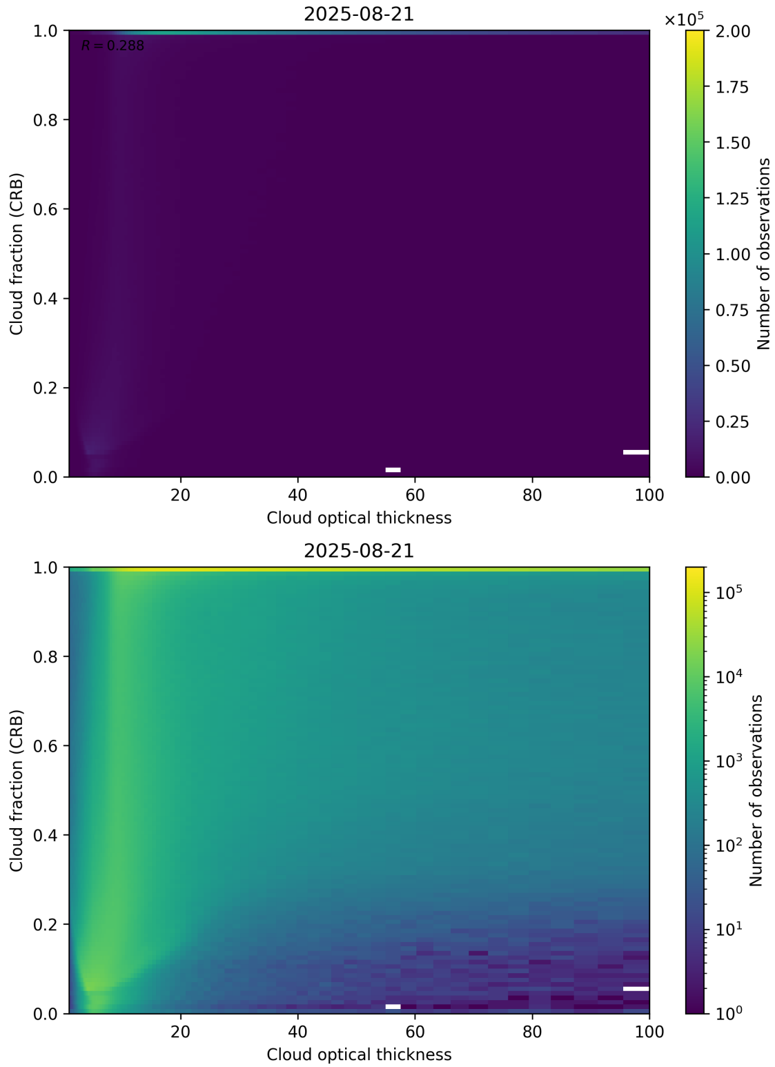
Figure 84: Scatter density plot of “Cloud optical thickness” against “Cloud fraction (CRB)” for 2025-08-20 to 2025-08-22.
