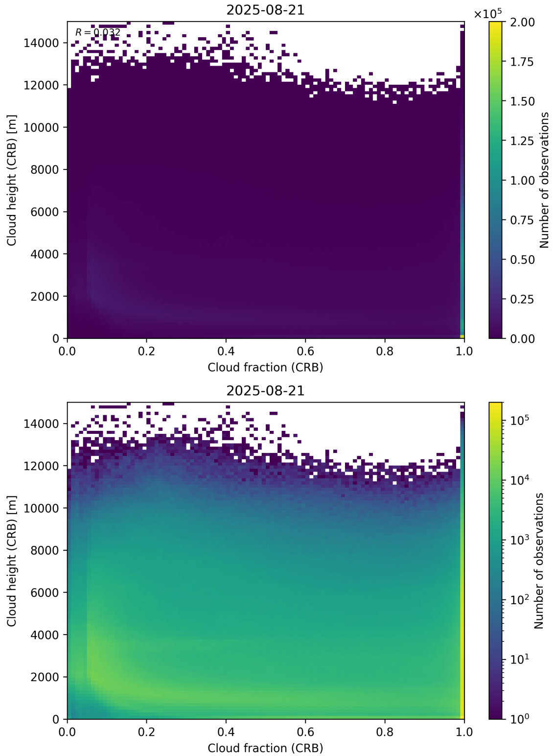
Figure 79: Scatter density plot of “Cloud fraction (CRB)” against “Cloud height (CRB)” for 2025-08-20 to 2025-08-22.
