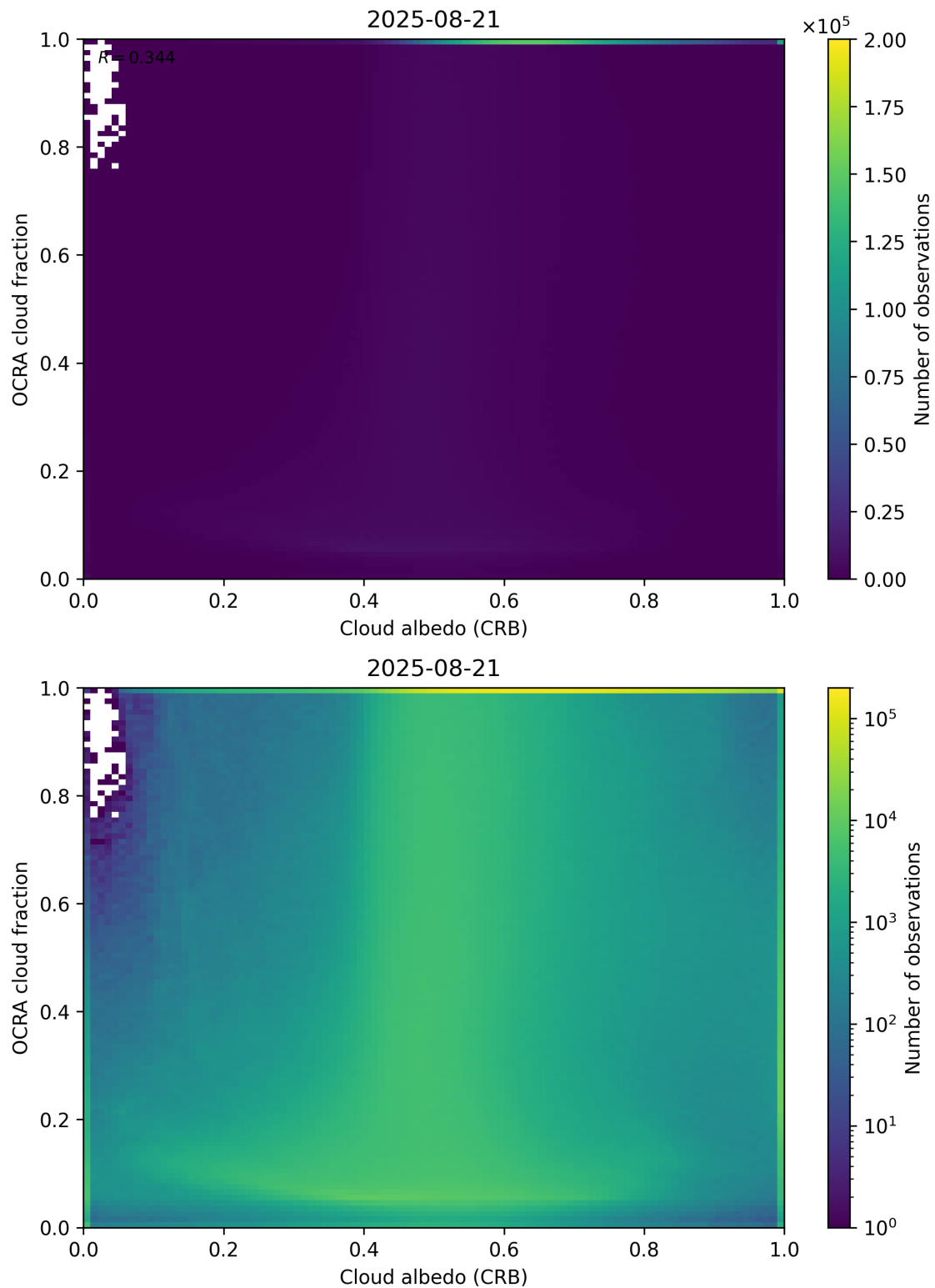
Figure 70: Scatter density plot of “Cloud albedo (CRB)” against “OCRA cloud fraction” for 2025-08-20 to 2025-08-22.
