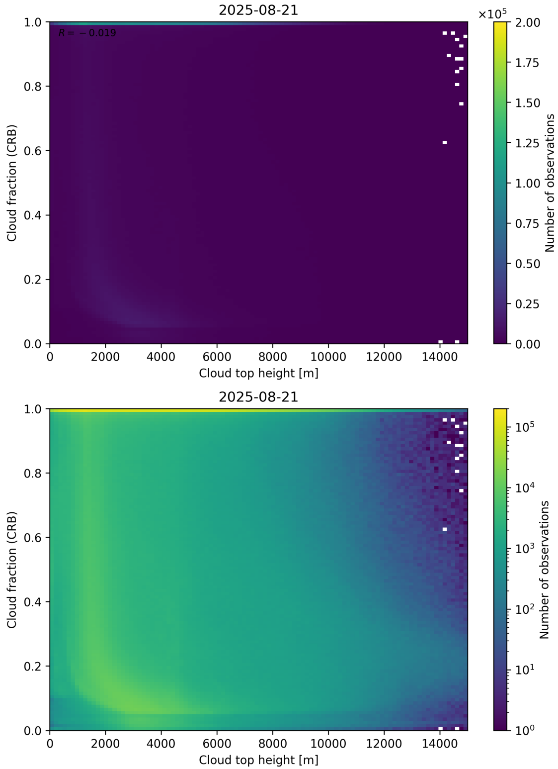
Figure 88: Scatter density plot of “Cloud top height” against “Cloud fraction (CRB)” for 2025-08-20 to 2025-08-22.
