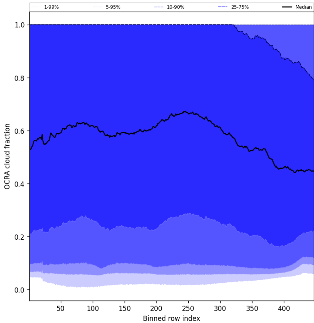
Figure 66: Along track statistics of “OCRA cloud fraction” for 2025-08-20 to 2025-08-22
