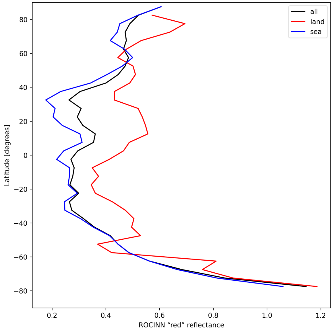
Figure 37: Zonal average of "ROCINN "red" reflectance" for 2025-08-20 to 2025-08-22.
