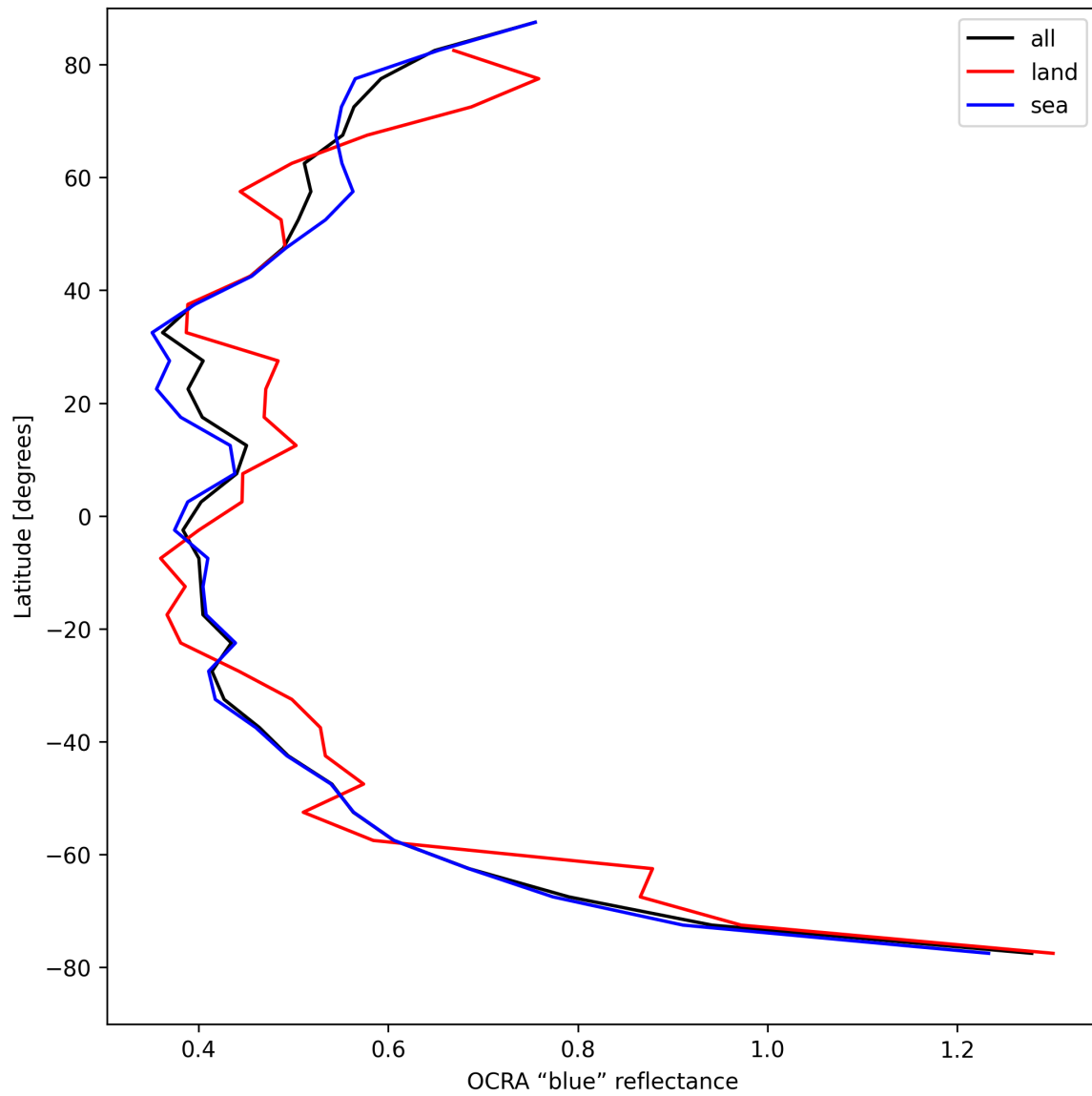
Figure 35: Zonal average of "OCRA "blue" reflectance" for 2025-08-20 to 2025-08-22.
