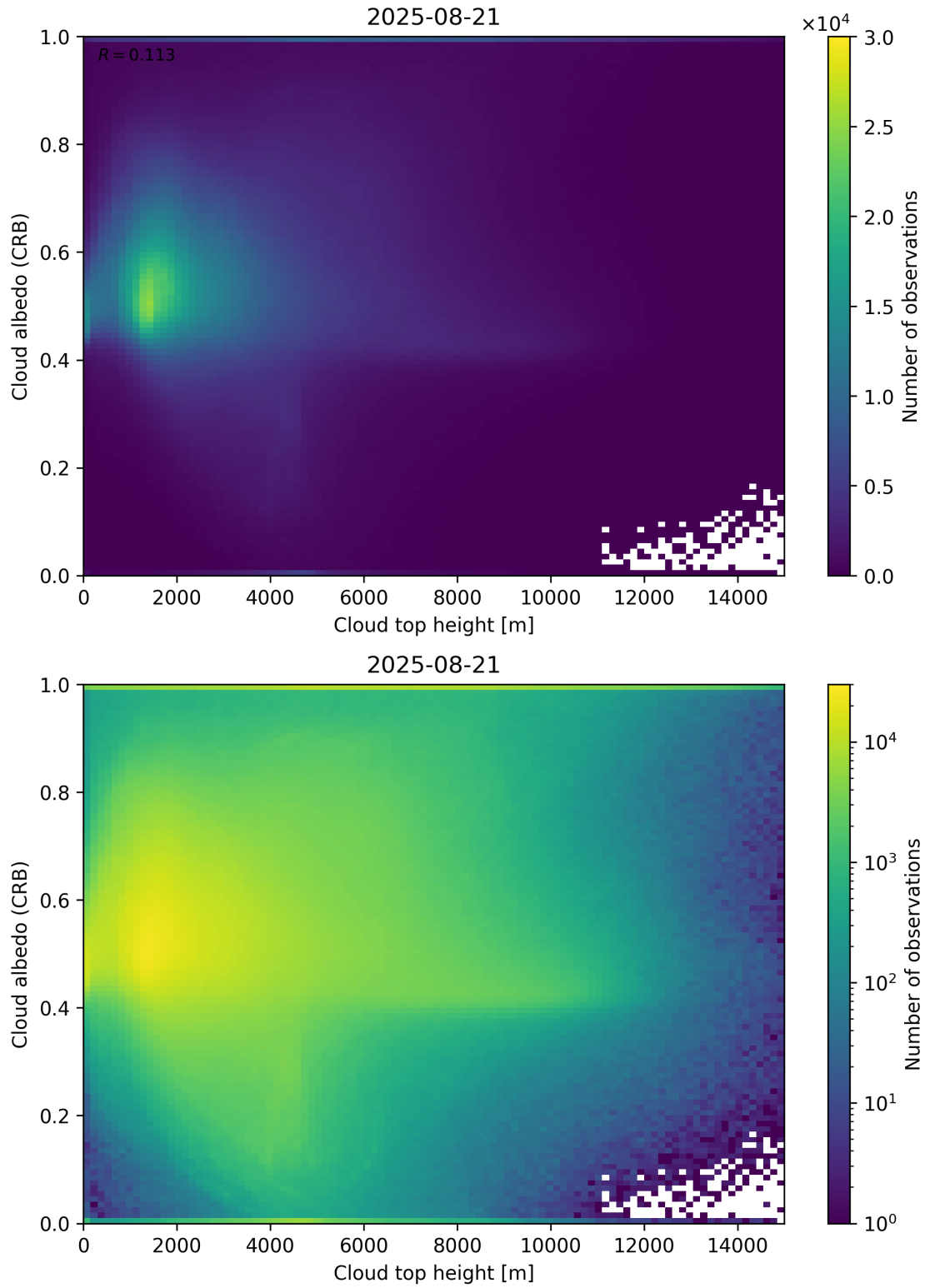
Figure 86: Scatter density plot of “Cloud top height” against “Cloud albedo (CRB)” for 2025-08-20 to 2025-08-22.
