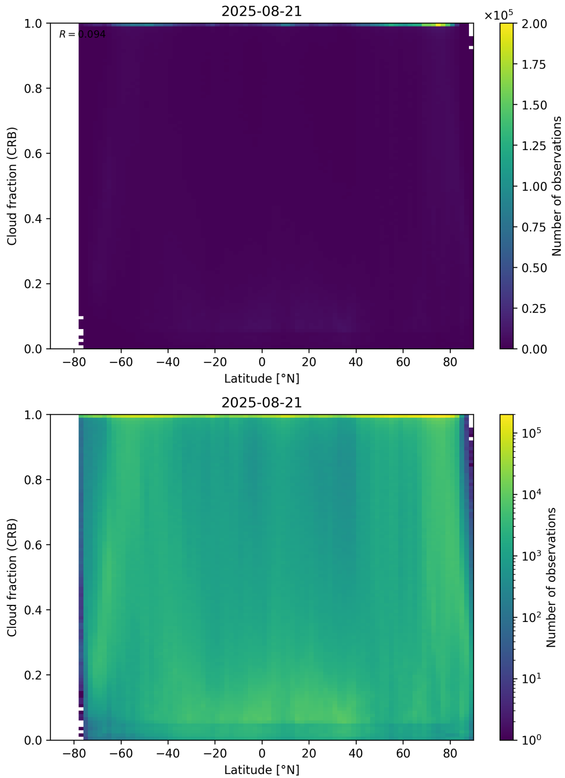
Figure 94: Scatter density plot of “Latitude” against “Cloud fraction (CRB)” for 2025-08-20 to 2025-08-22.
