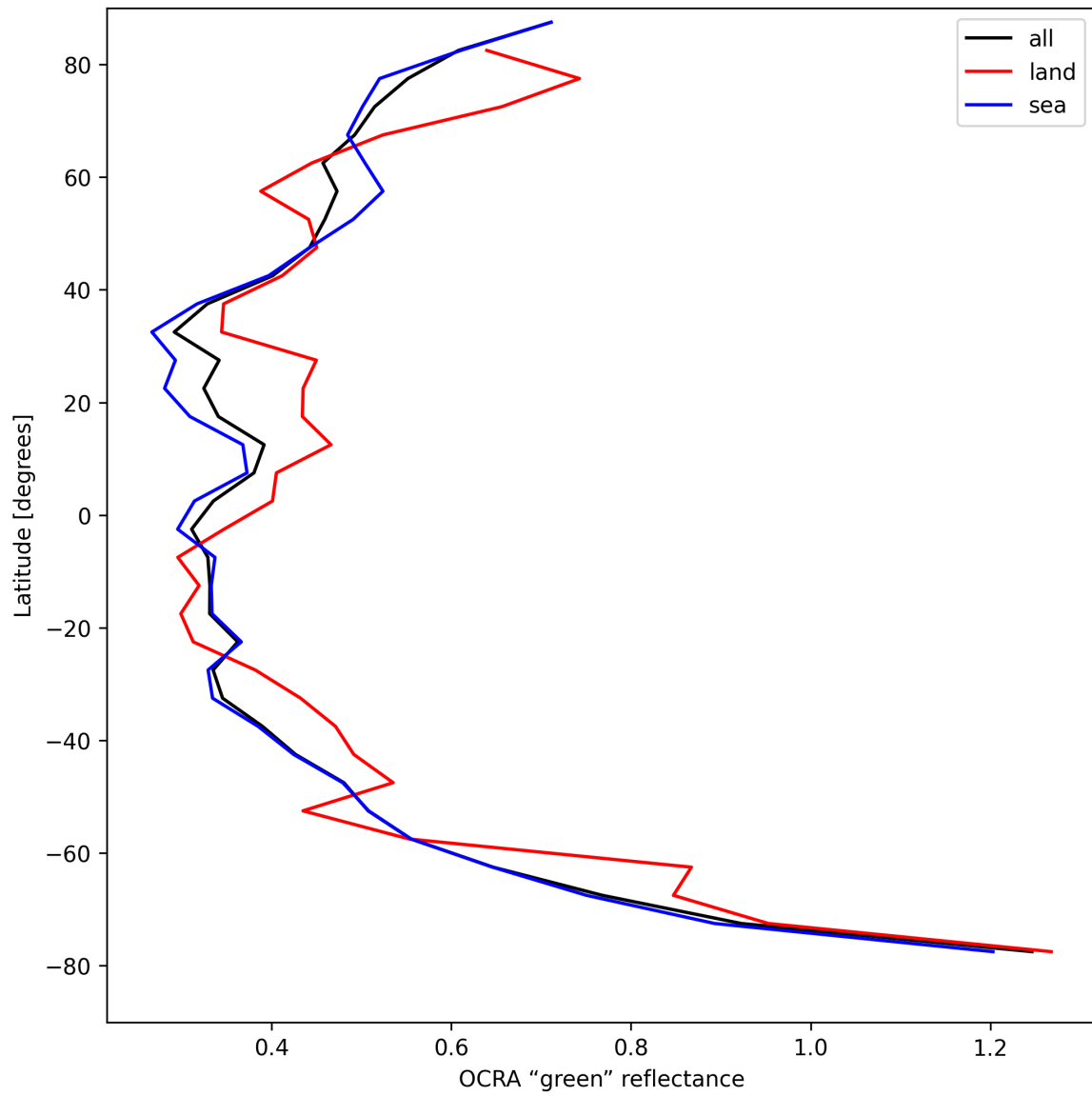
Figure 36: Zonal average of “OCRA “green” reflectance” for 2025-08-20 to 2025-08-22.
