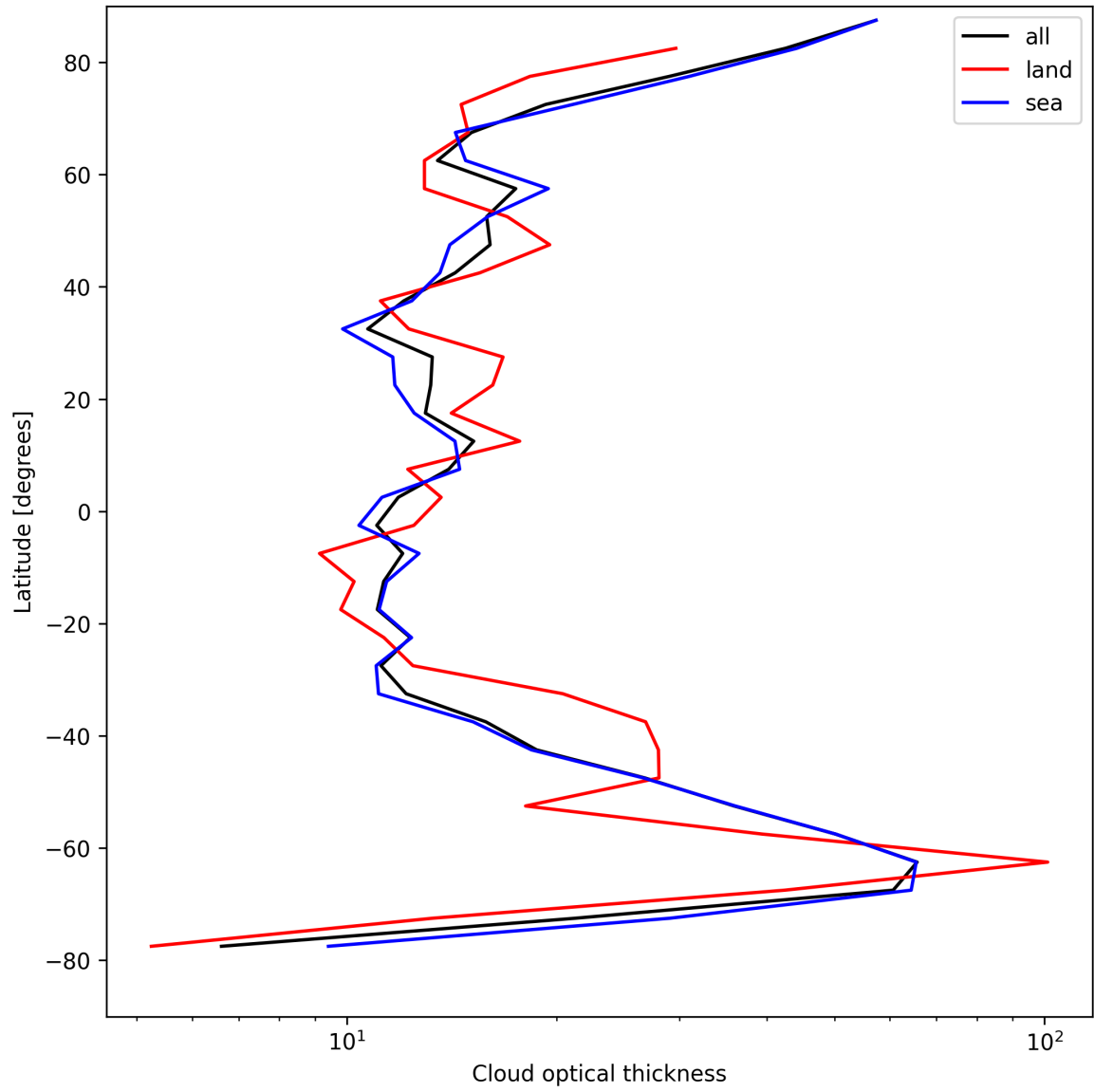
Figure 25: Zonal average of “Cloud optical thickness” for 2025-08-20 to 2025-08-22.
