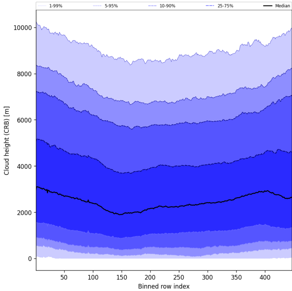
Figure 59: Along track statistics of “Cloud height (CRB)” for 2025-08-20 to 2025-08-22
