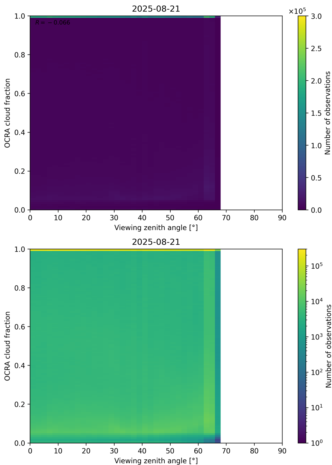
Figure 108: Scatter density plot of “Viewing zenith angle” against “OCRA cloud fraction” for 2025-08-20 to 2025-08-22.
