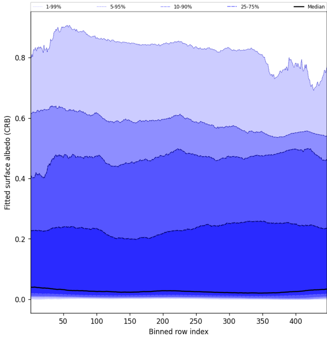
Figure 62: Along track statistics of “Fitted surface albedo (CRB)” for 2025-08-20 to 2025-08-22
