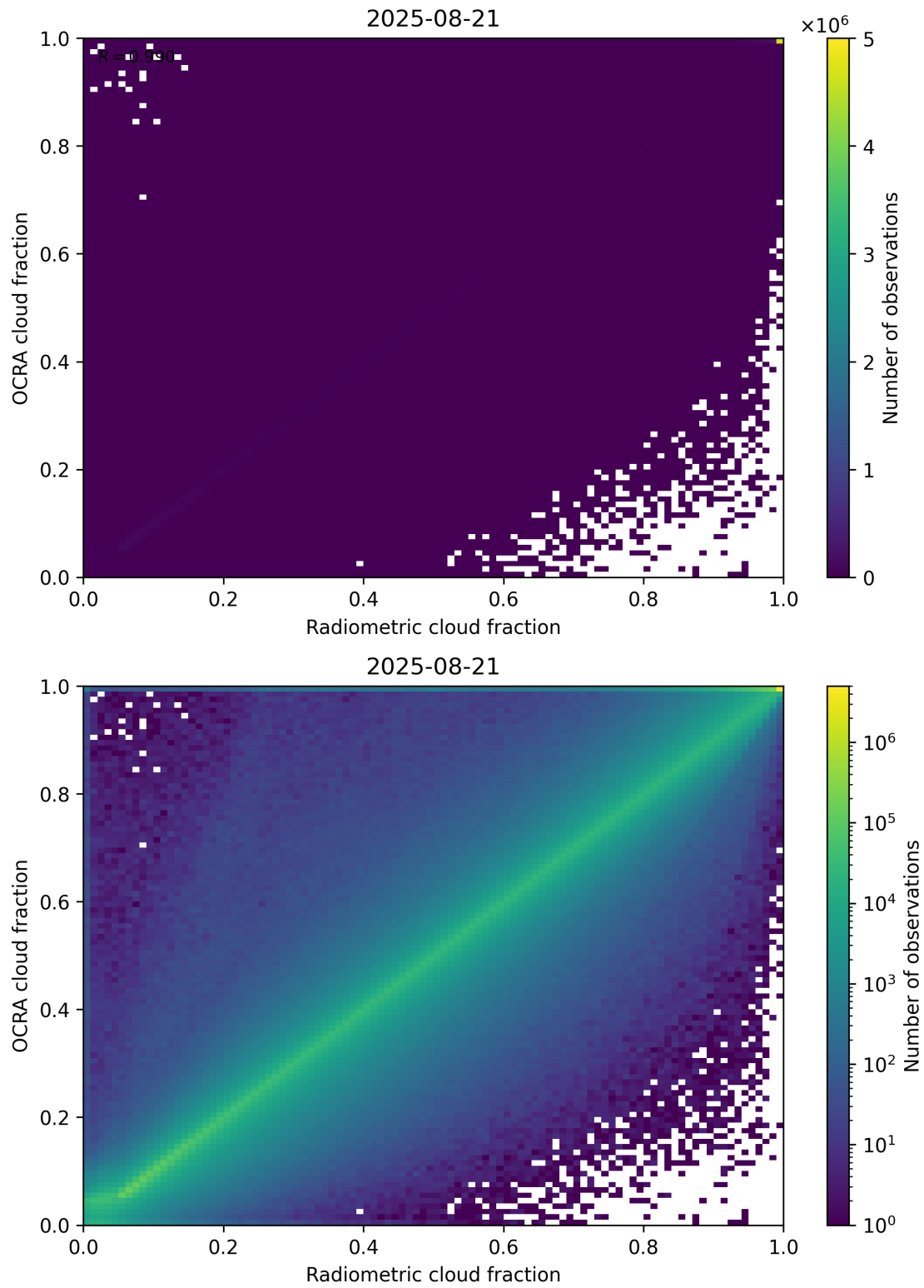
Figure 72: Scatter density plot of “Radiometric cloud fraction” against “OCRA cloud fraction” for 2025-08-20 to 2025-08-22.
