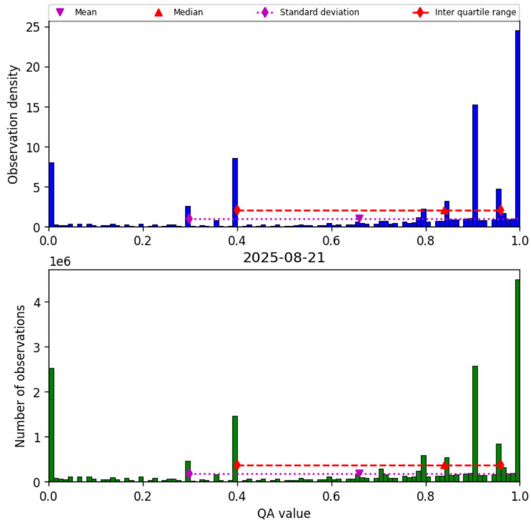
Figure 38: Histogram of “QA value” for 2025-08-20 to 2025-08-22
