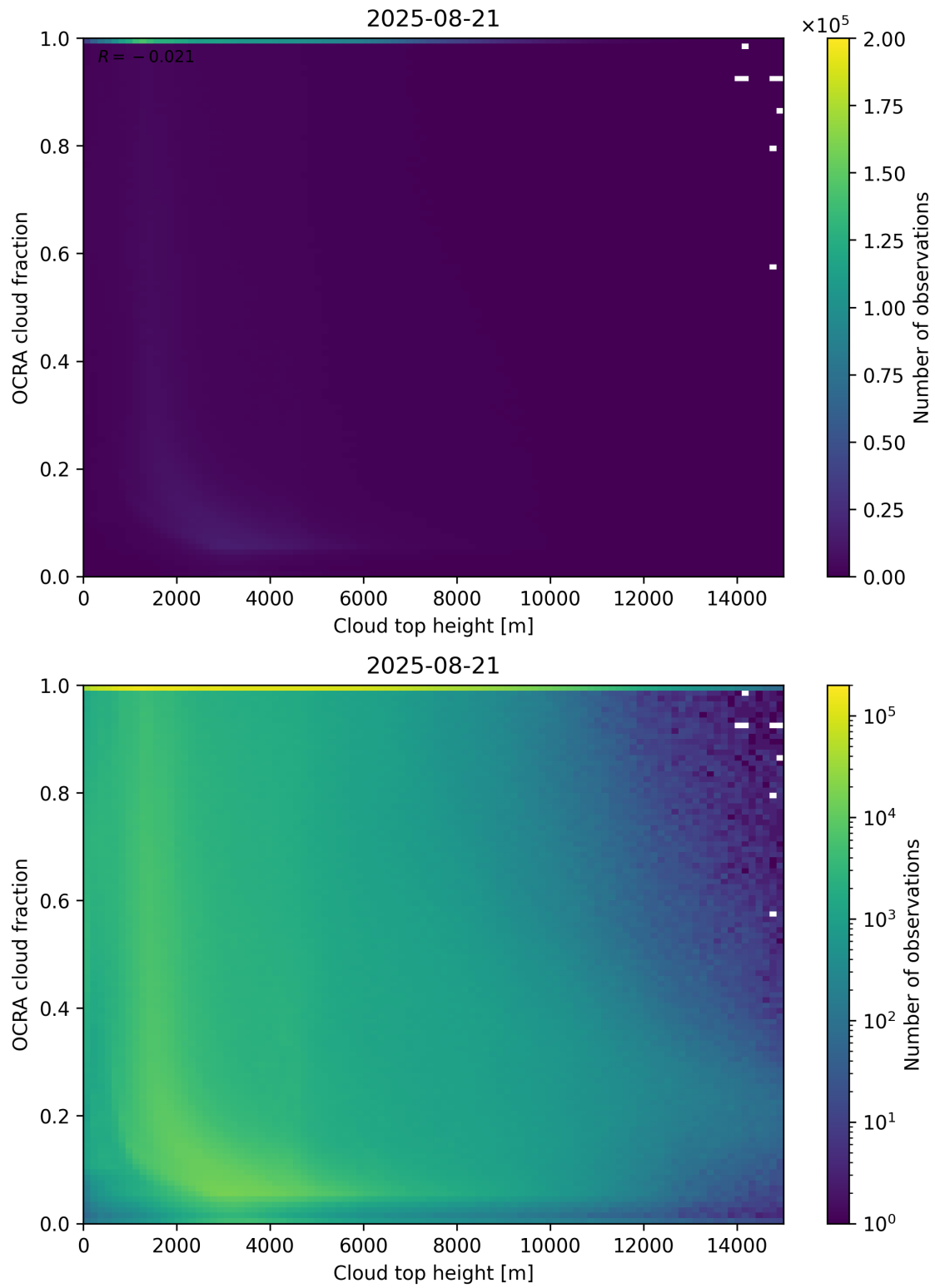
Figure 87: Scatter density plot of “Cloud top height” against “OCRA cloud fraction” for 2025-08-20 to 2025-08-22.
