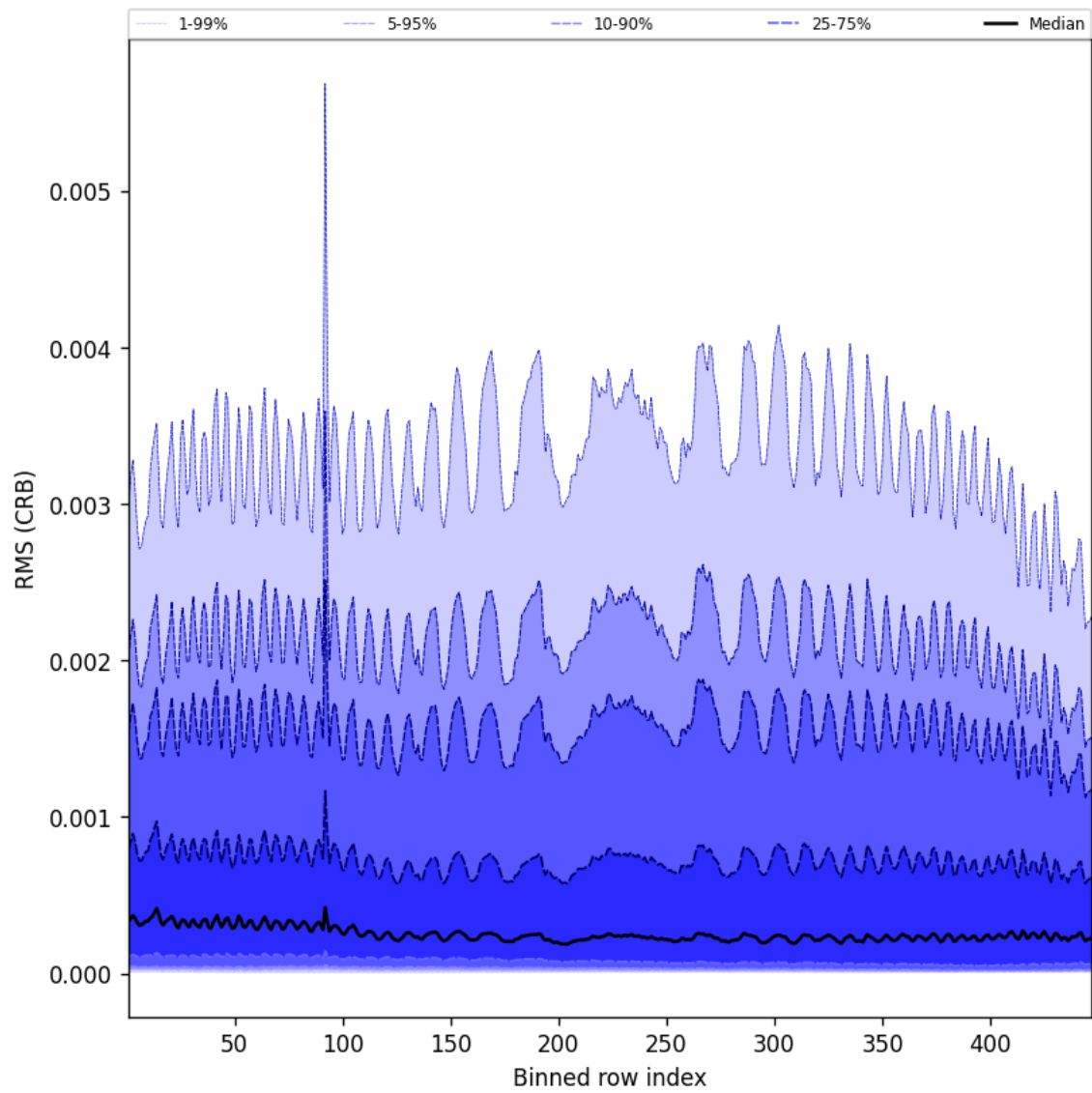
Figure 64: Along track statistics of “RMS (CRB)” for 2025-08-20 to 2025-08-22
