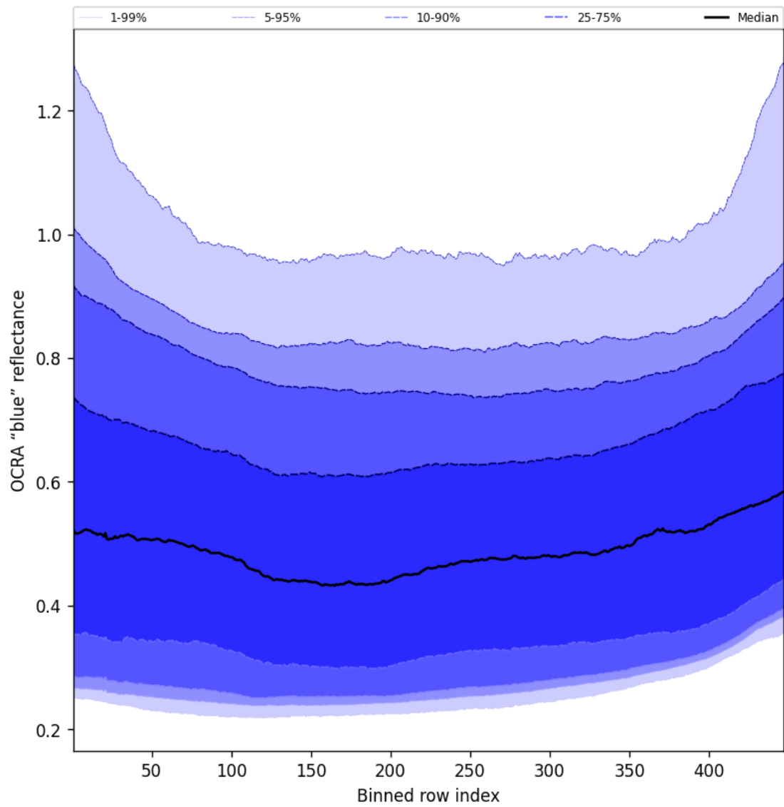
Figure 67: Along track statistics of “OCRA “blue” reflectance” for 2025-08-20 to 2025-08-22
