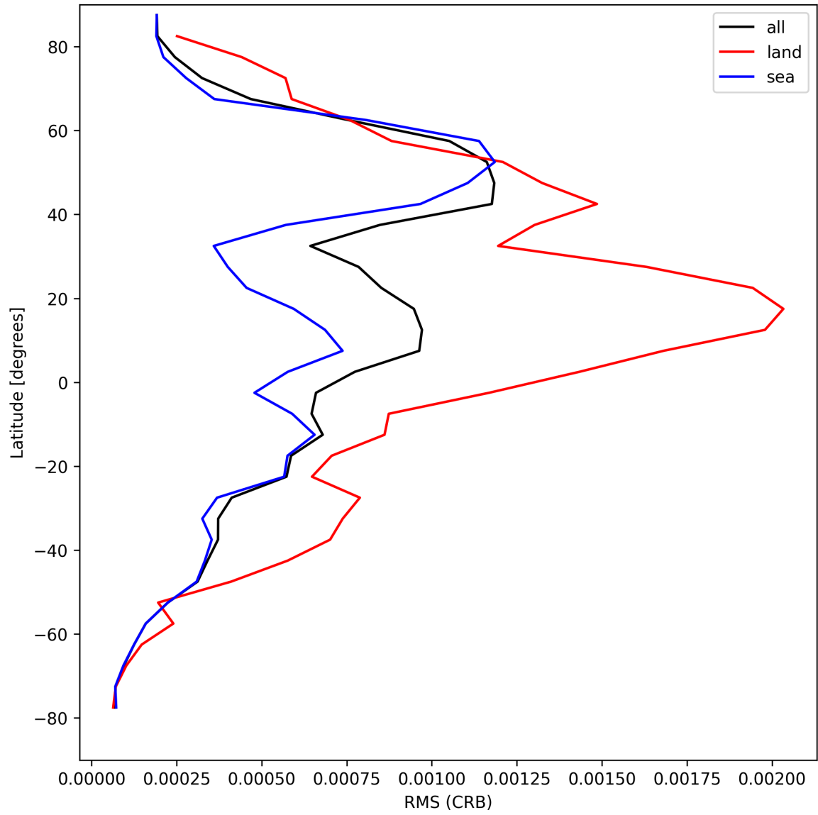
Figure 32: Zonal average of “RMS (CRB)” for 2025-08-20 to 2025-08-22.
