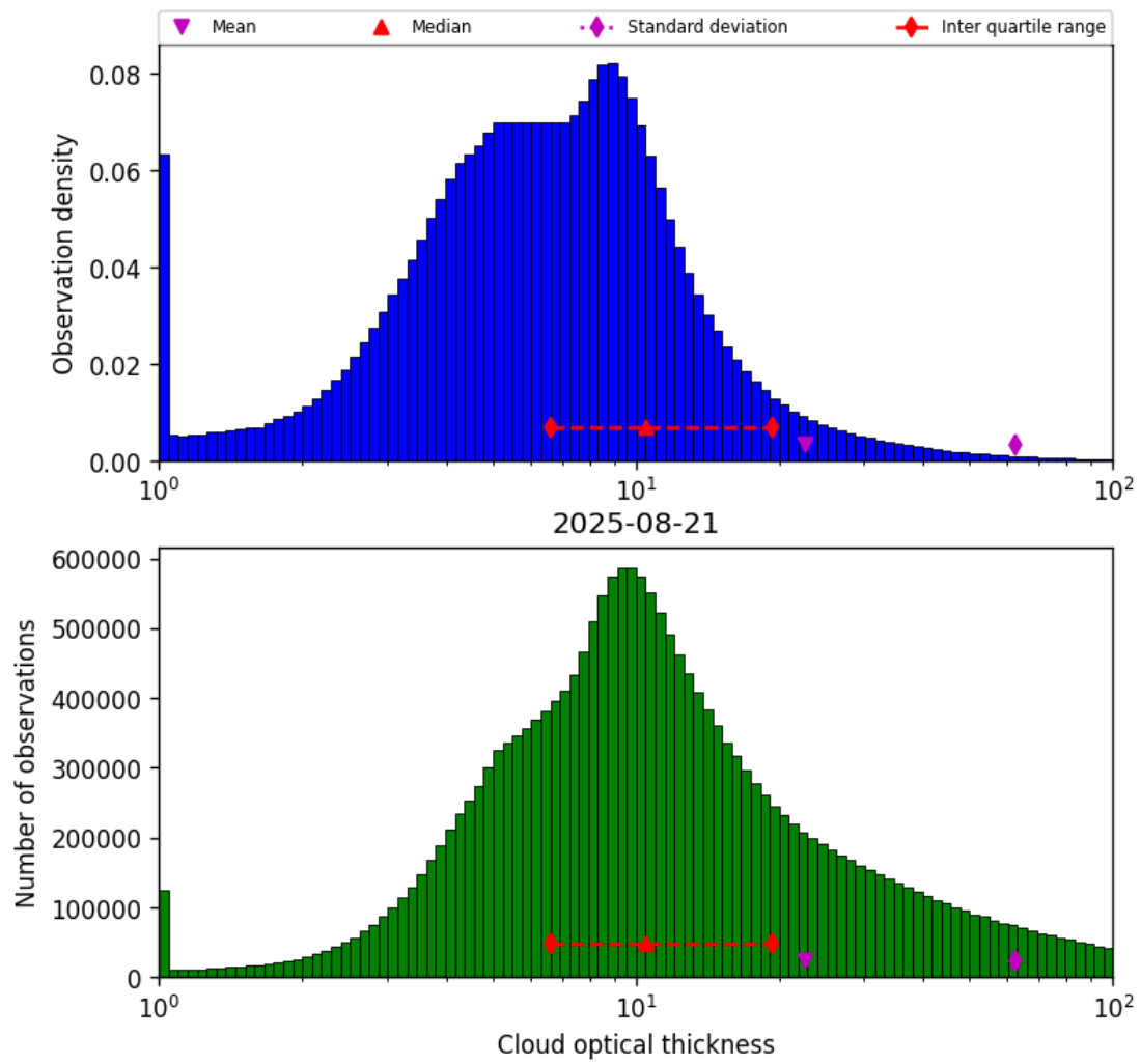
Figure 41: Histogram of “Cloud optical thickness” for 2025-08-20 to 2025-08-22
