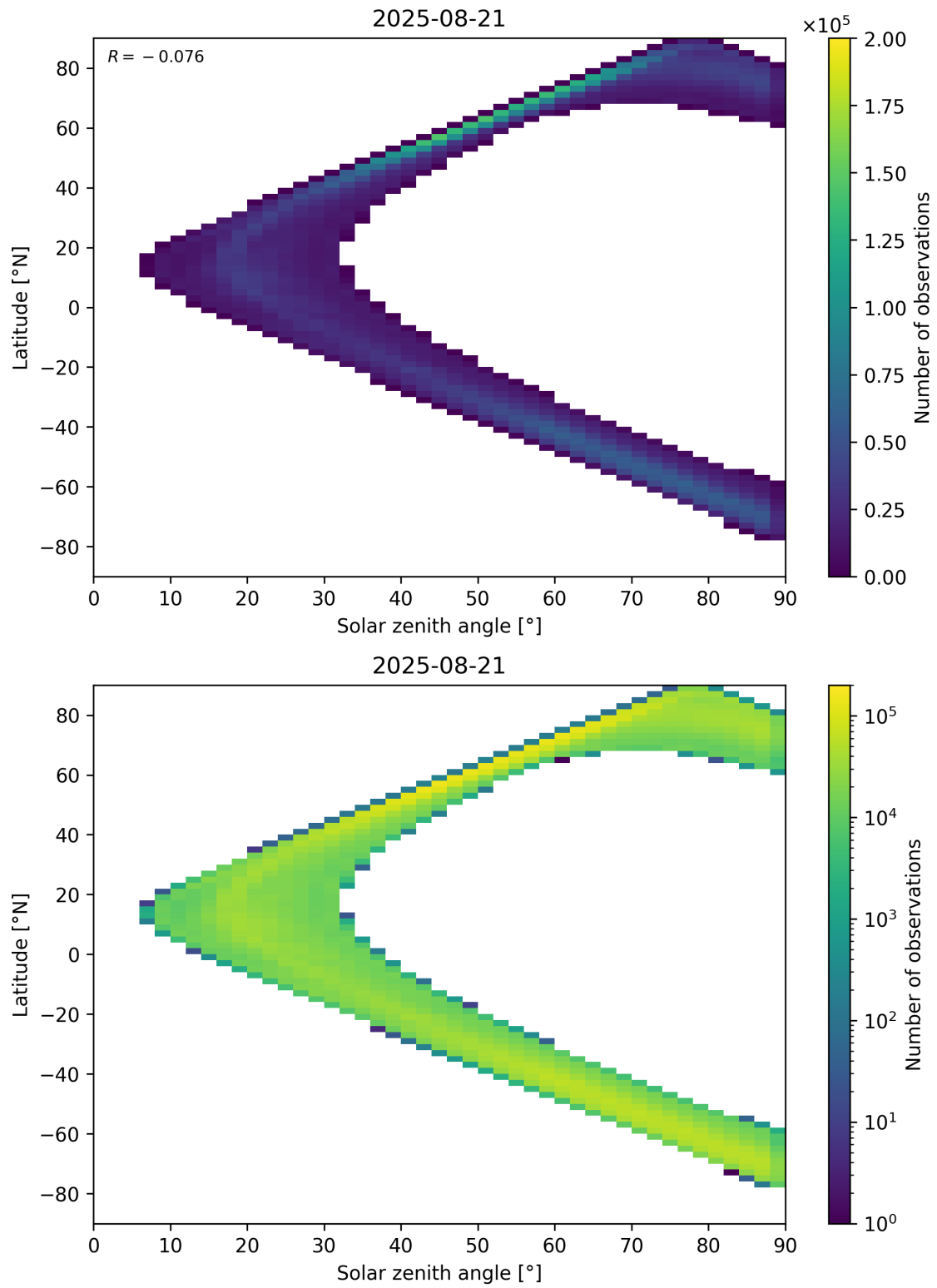
Figure 105: Scatter density plot of “Solar zenith angle” against “Latitude” for 2025-08-20 to 2025-08-22.
