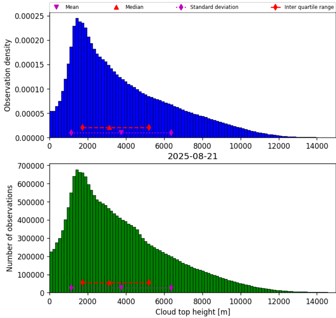
Figure 40: Histogram of “Cloud top height” for 2025-08-20 to 2025-08-22
