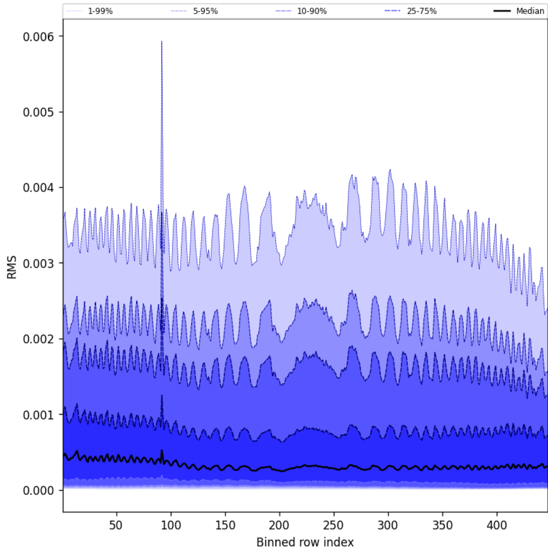
Figure 63: Along track statistics of “RMS” for 2025-08-20 to 2025-08-22
