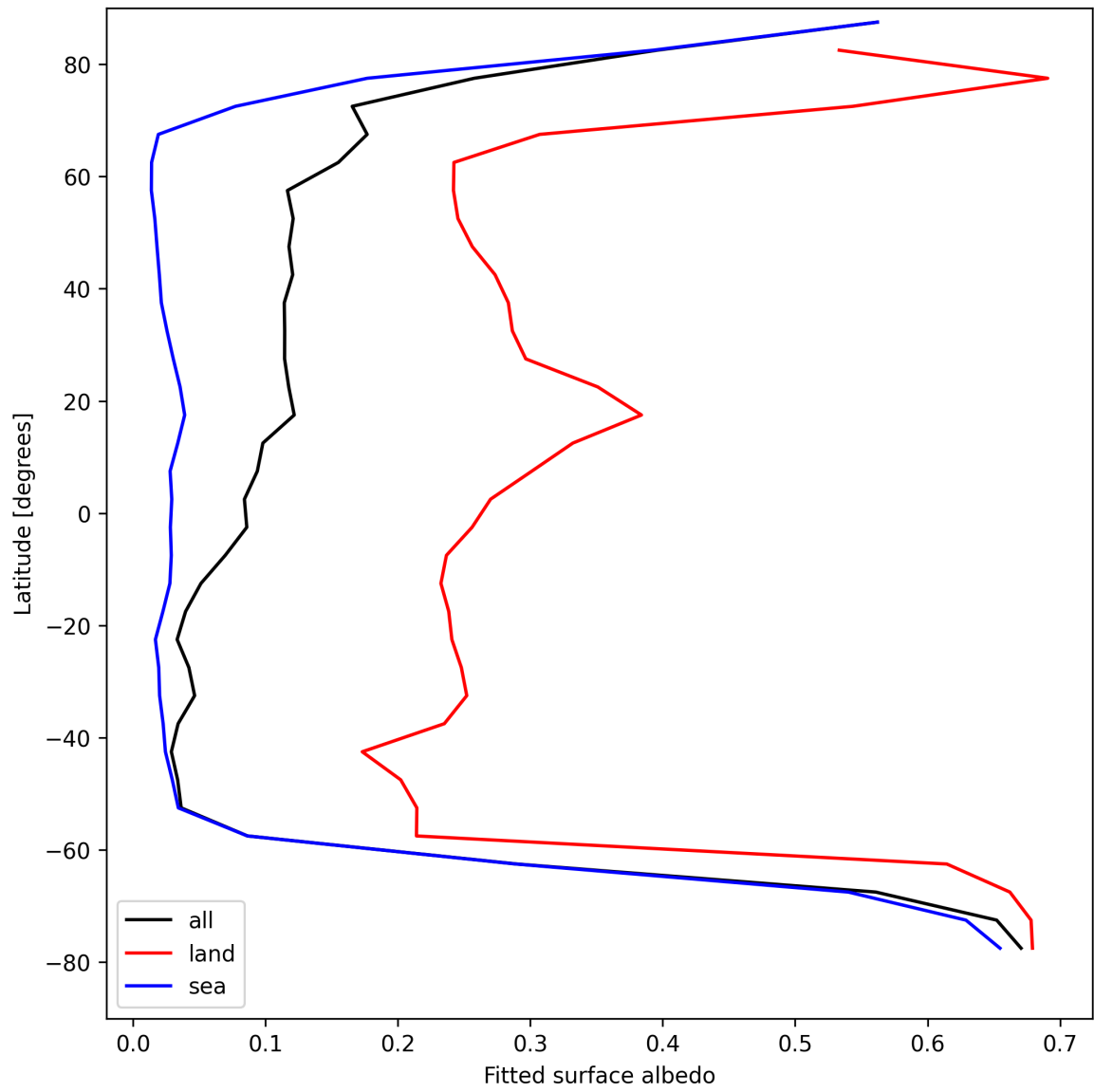
Figure 29: Zonal average of “Fitted surface albedo” for 2025-08-20 to 2025-08-22.
