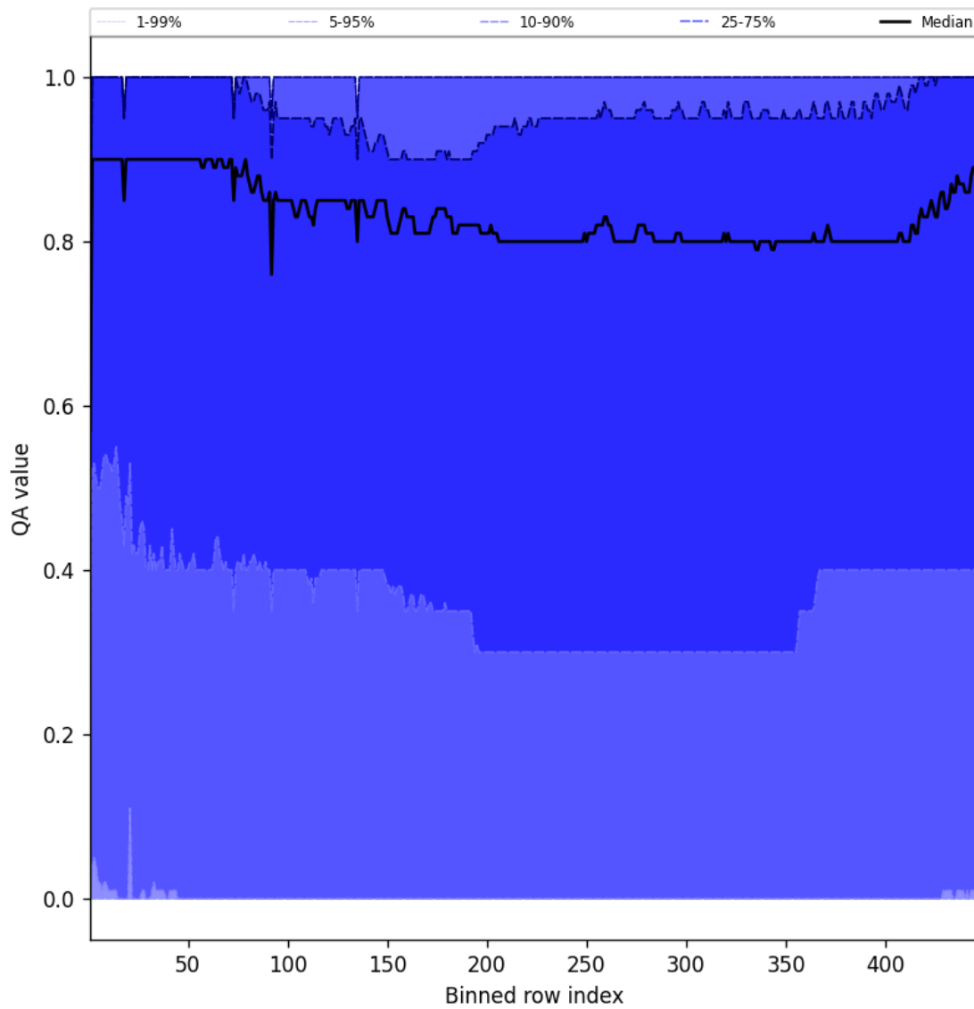
Figure 54: Along track statistics of “QA value” for 2025-08-20 to 2025-08-22
