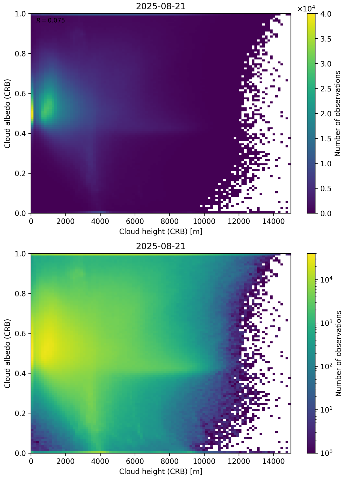
Figure 80: Scatter density plot of “Cloud height (CRB)” against “Cloud albedo (CRB)” for 2025-08-20 to 2025-08-22.
