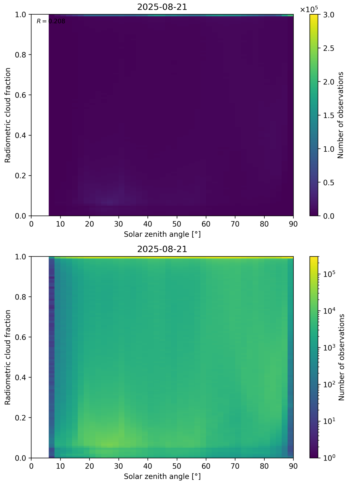
Figure 99: Scatter density plot of “Solar zenith angle” against “Radiometric cloud fraction” for 2025-08-20 to 2025-08-22.
