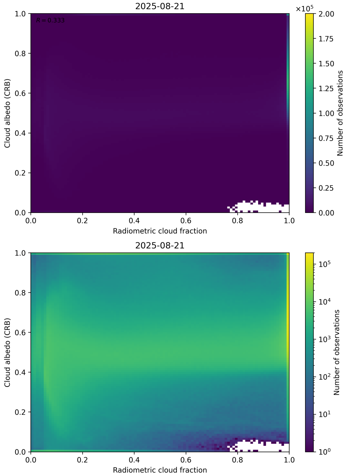
Figure 71: Scatter density plot of “Radiometric cloud fraction” against “Cloud albedo (CRB)” for 2025-08-20 to 2025-08-22.
