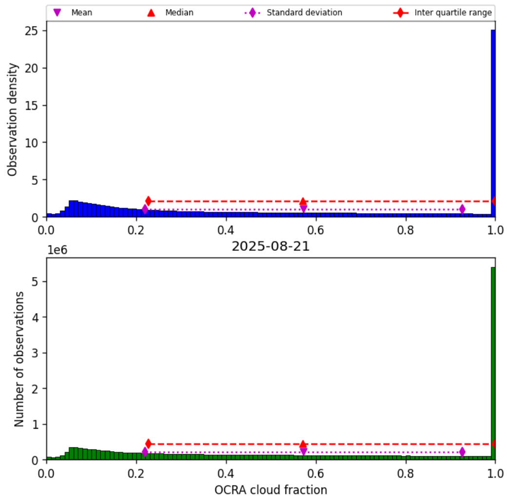
Figure 50: Histogram of “OCRA cloud fraction” for 2025-08-20 to 2025-08-22
