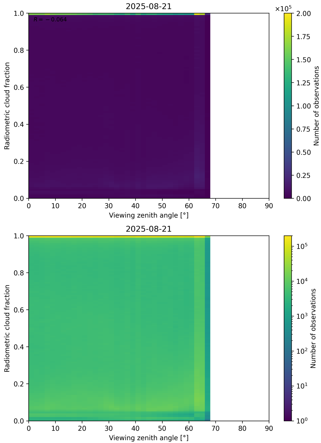
Figure 107: Scatter density plot of “Viewing zenith angle” against “Radiometric cloud fraction” for 2025-08-20 to 2025-08-22.
