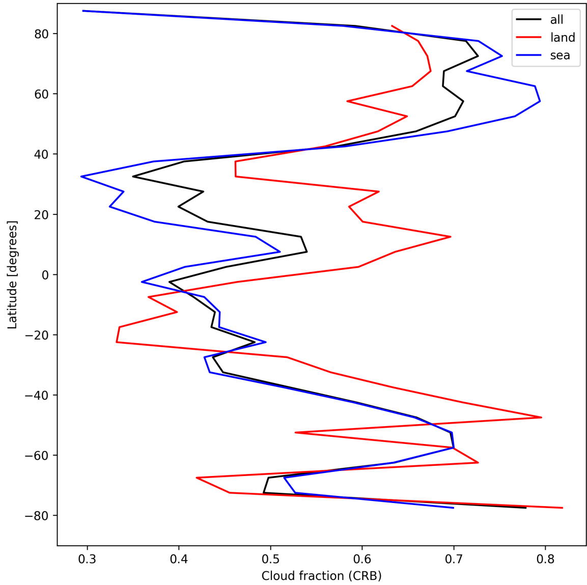
Figure 26: Zonal average of “Cloud fraction (CRB)” for 2025-08-20 to 2025-08-22.
