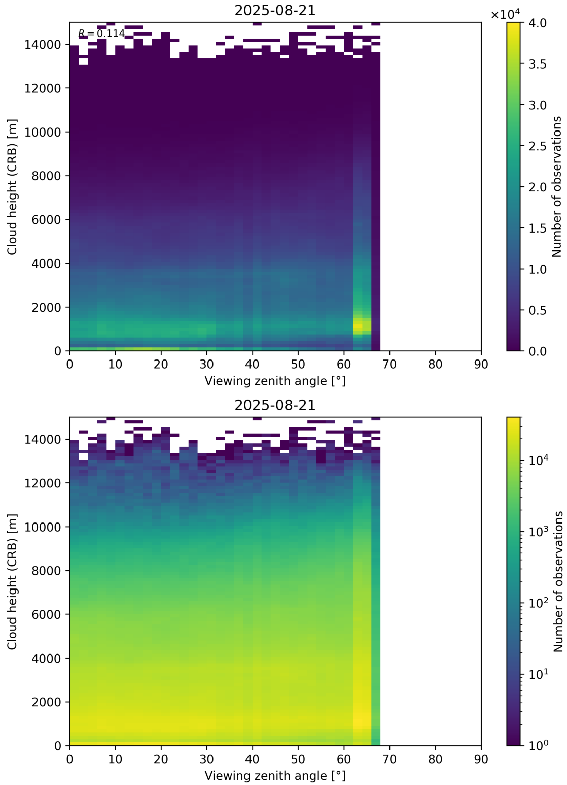
Figure 110: Scatter density plot of “Viewing zenith angle” against “Cloud height (CRB)” for 2025-08-20 to 2025-08-22.
