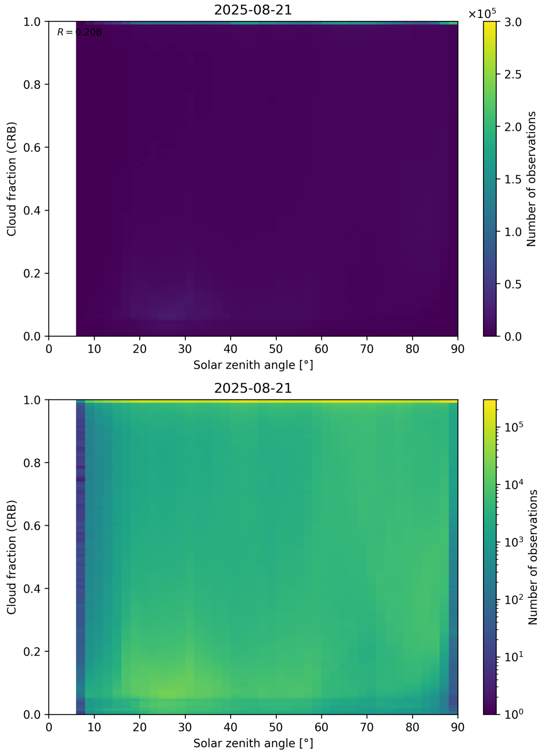
Figure 101: Scatter density plot of “Solar zenith angle” against “Cloud fraction (CRB)” for 2025-08-20 to 2025-08-22.
