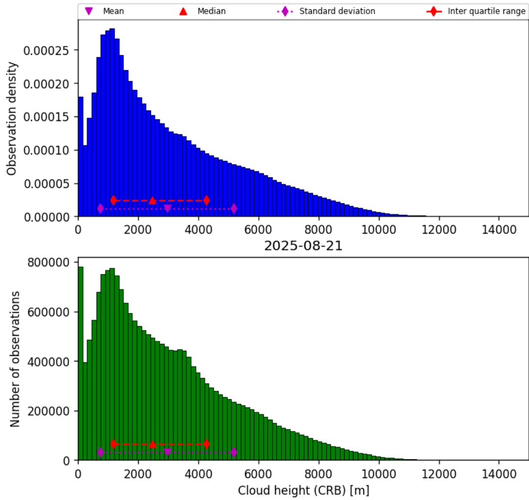
Figure 43: Histogram of “Cloud height (CRB)” for 2025-08-20 to 2025-08-22
