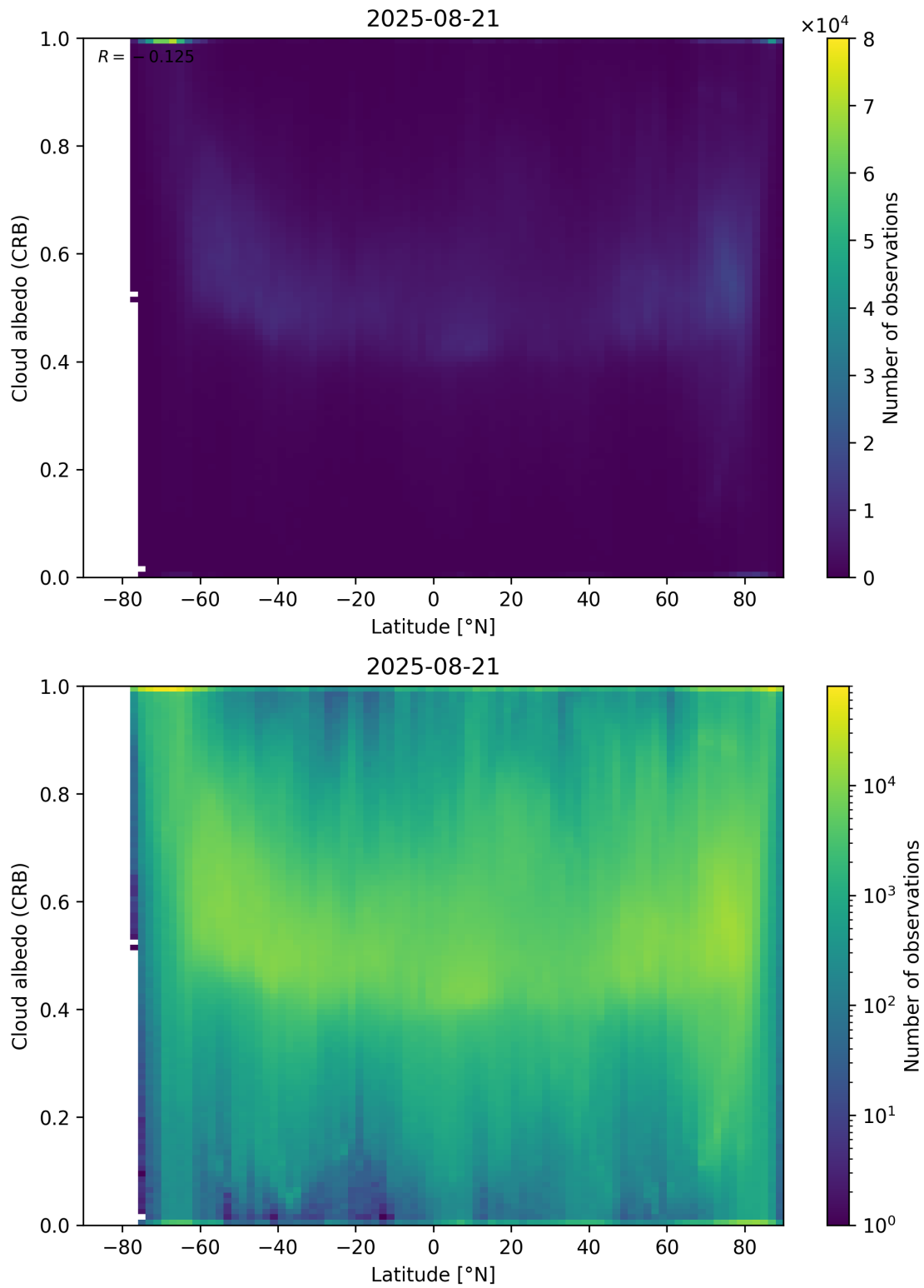
Figure 91: Scatter density plot of “Latitude” against “Cloud albedo (CRB)” for 2025-08-20 to 2025-08-22.
