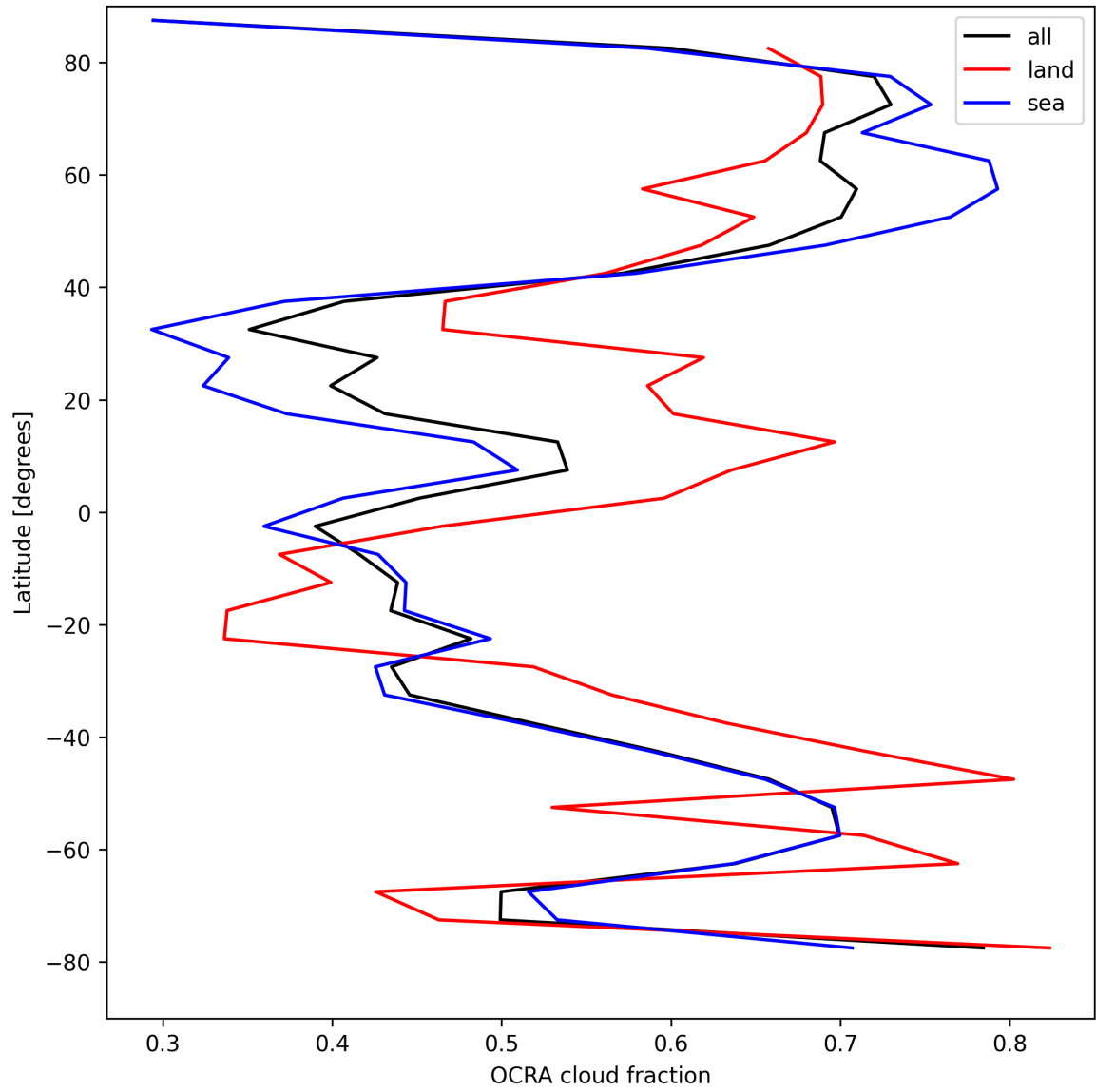
Figure 34: Zonal average of “OCRA cloud fraction” for 2025-08-20 to 2025-08-22.
