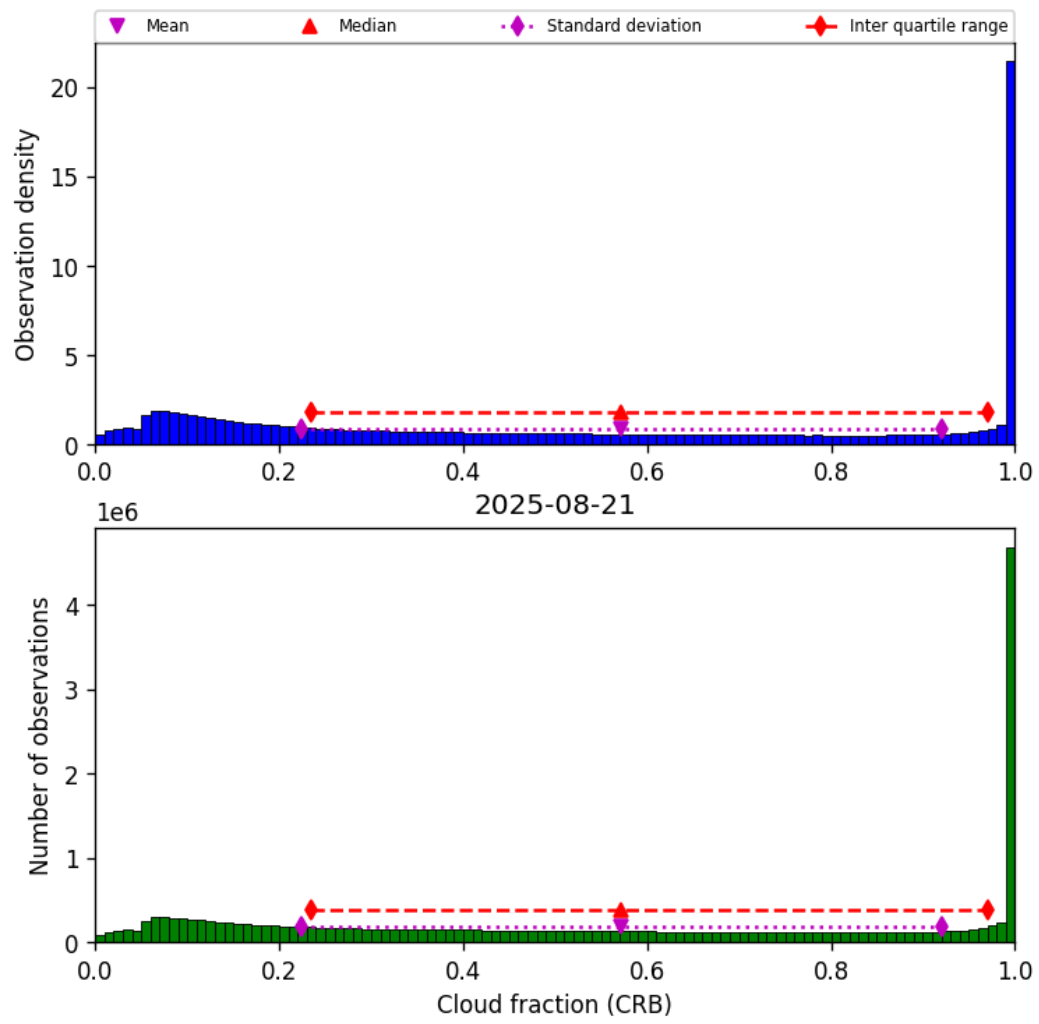
Figure 42: Histogram of “Cloud fraction (CRB)” for 2025-08-20 to 2025-08-22
