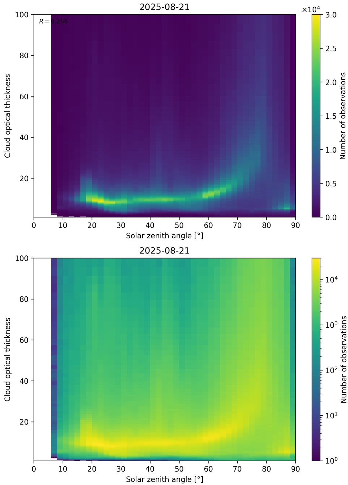
Figure 103: Scatter density plot of “Solar zenith angle” against “Cloud optical thickness” for 2025-08-20 to 2025-08-22.
