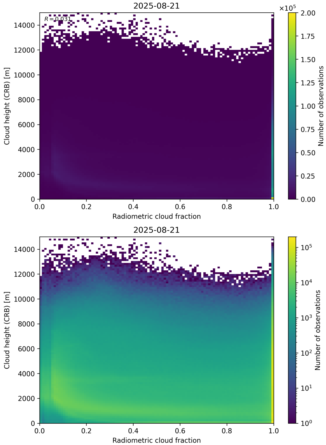
Figure 74: Scatter density plot of “Radiometric cloud fraction” against “Cloud height (CRB)” for 2025-08-20 to 2025-08-22.
