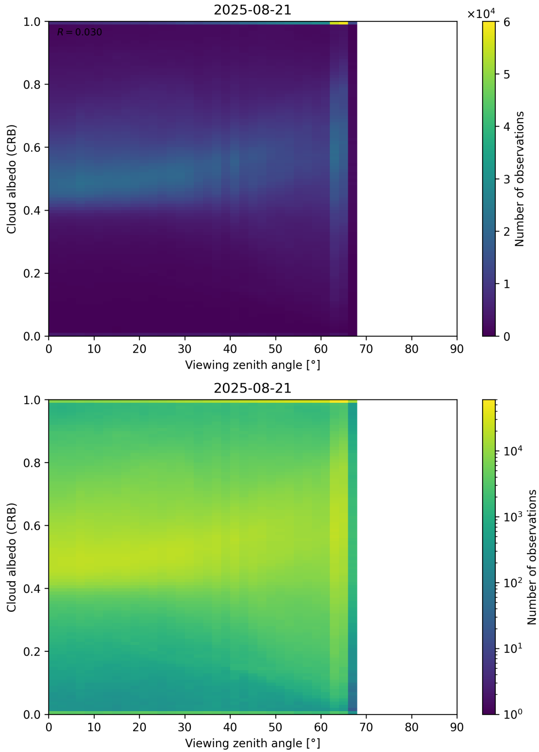
Figure 106: Scatter density plot of “Viewing zenith angle” against “Cloud albedo (CRB)” for 2025-08-20 to 2025-08-22.
