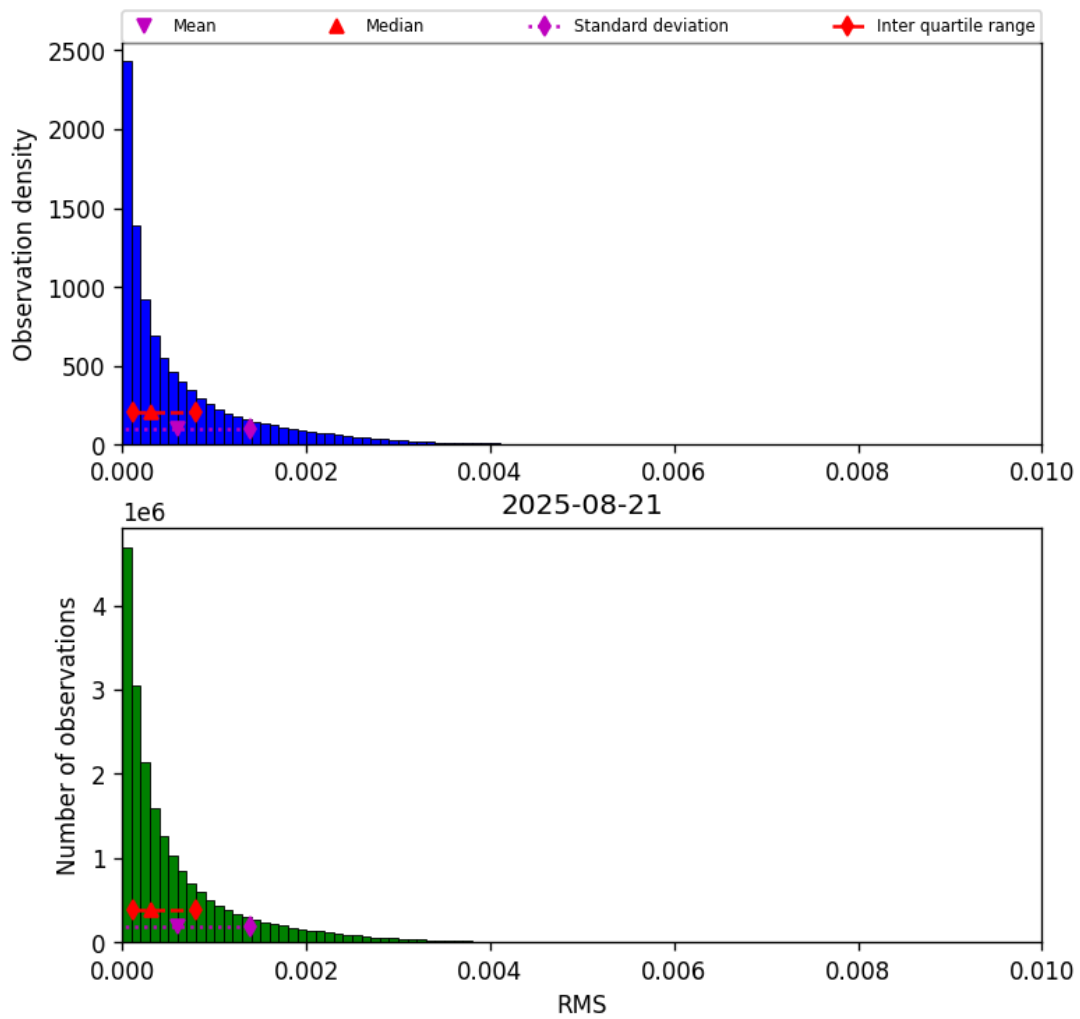
Figure 47: Histogram of “RMS” for 2025-08-20 to 2025-08-22
