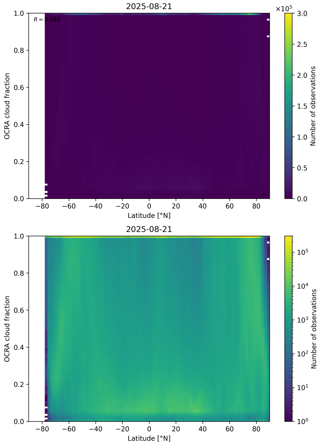
Figure 93: Scatter density plot of “Latitude” against “OCRA cloud fraction” for 2025-08-20 to 2025-08-22.
