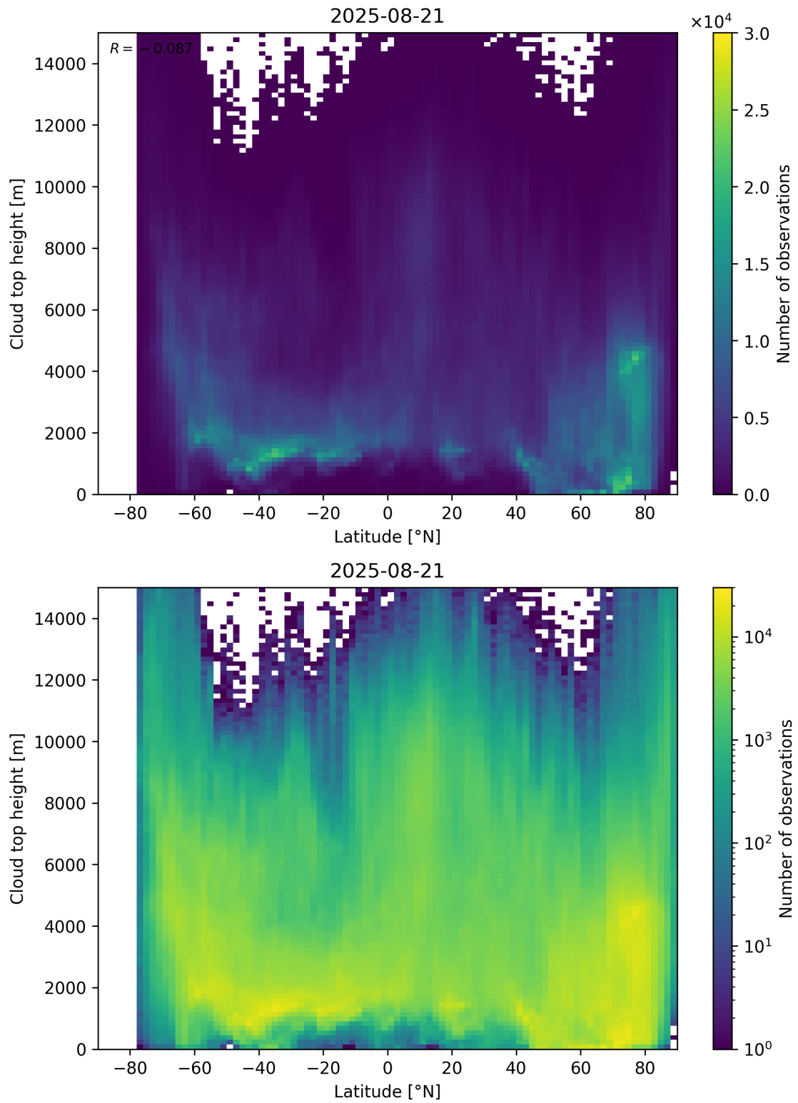
Figure 97: Scatter density plot of “Latitude” against “Cloud top height” for 2025-08-20 to 2025-08-22.
