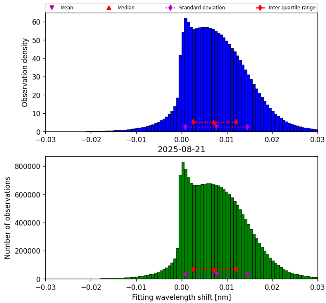
Figure 49: Histogram of “Fitting wavelength shift” for 2025-08-20 to 2025-08-22
