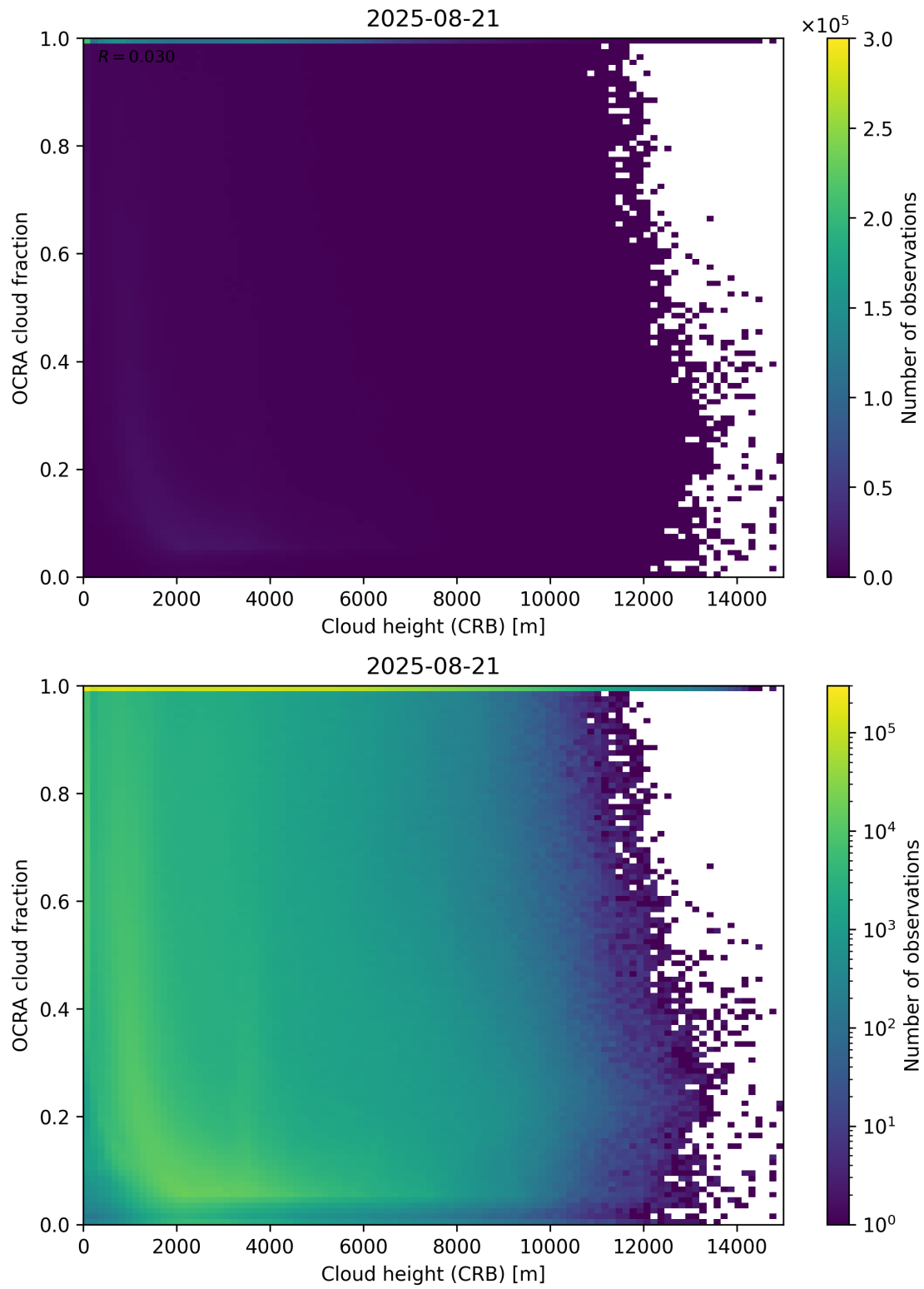
Figure 81: Scatter density plot of “Cloud height (CRB)” against “OCRA cloud fraction” for 2025-08-20 to 2025-08-22.
