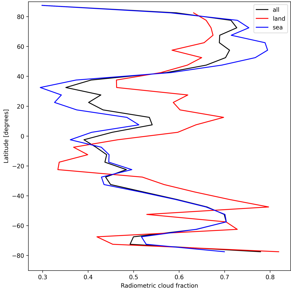
Figure 23: Zonal average of “Radiometric cloud fraction” for 2025-08-20 to 2025-08-22.
