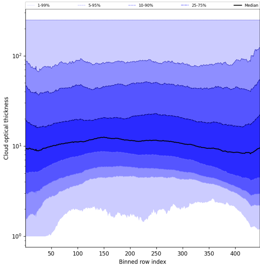
Figure 57: Along track statistics of “Cloud optical thickness” for 2025-08-20 to 2025-08-22
