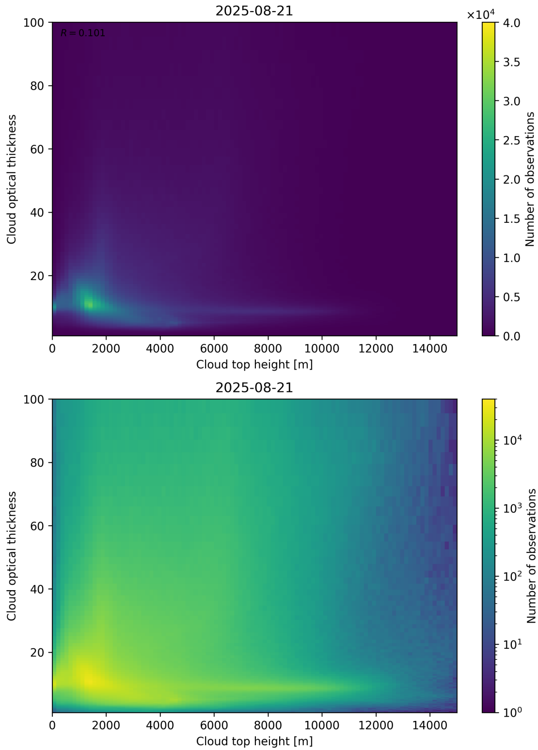
Figure 90: Scatter density plot of “Cloud top height” against “Cloud optical thickness” for 2025-08-20 to 2025-08-22.
