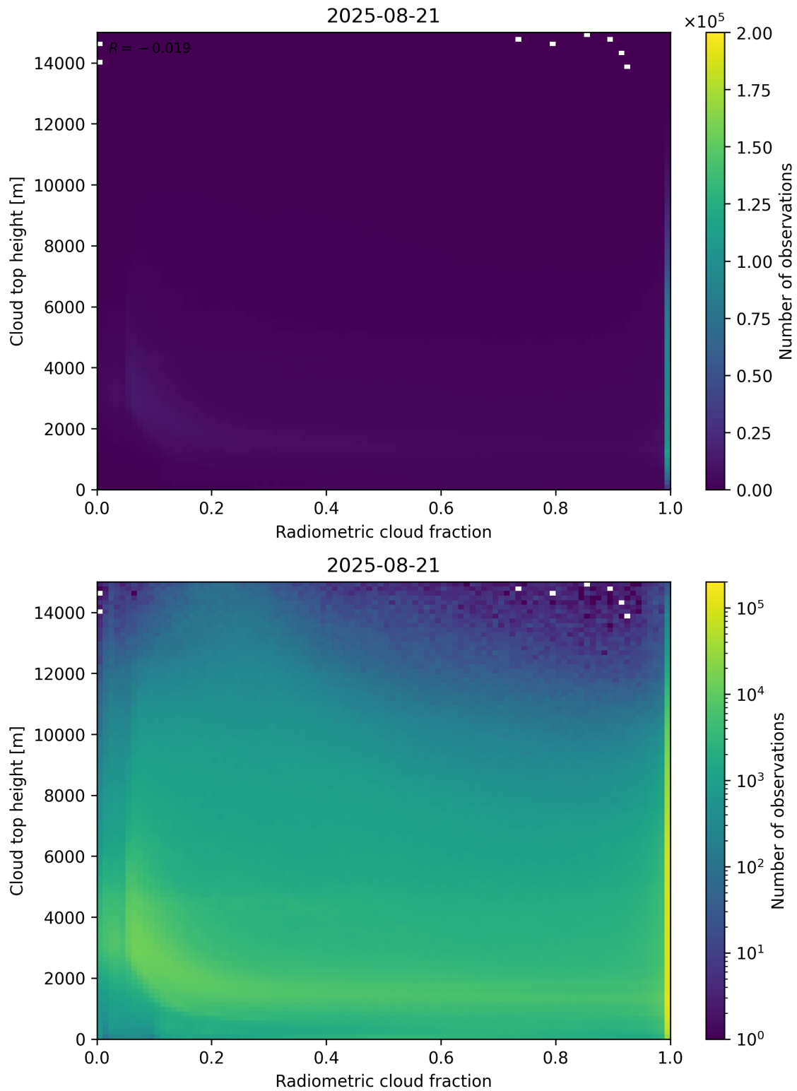
Figure 76: Scatter density plot of “Radiometric cloud fraction” against “Cloud top height” for 2025-08-20 to 2025-08-22.
