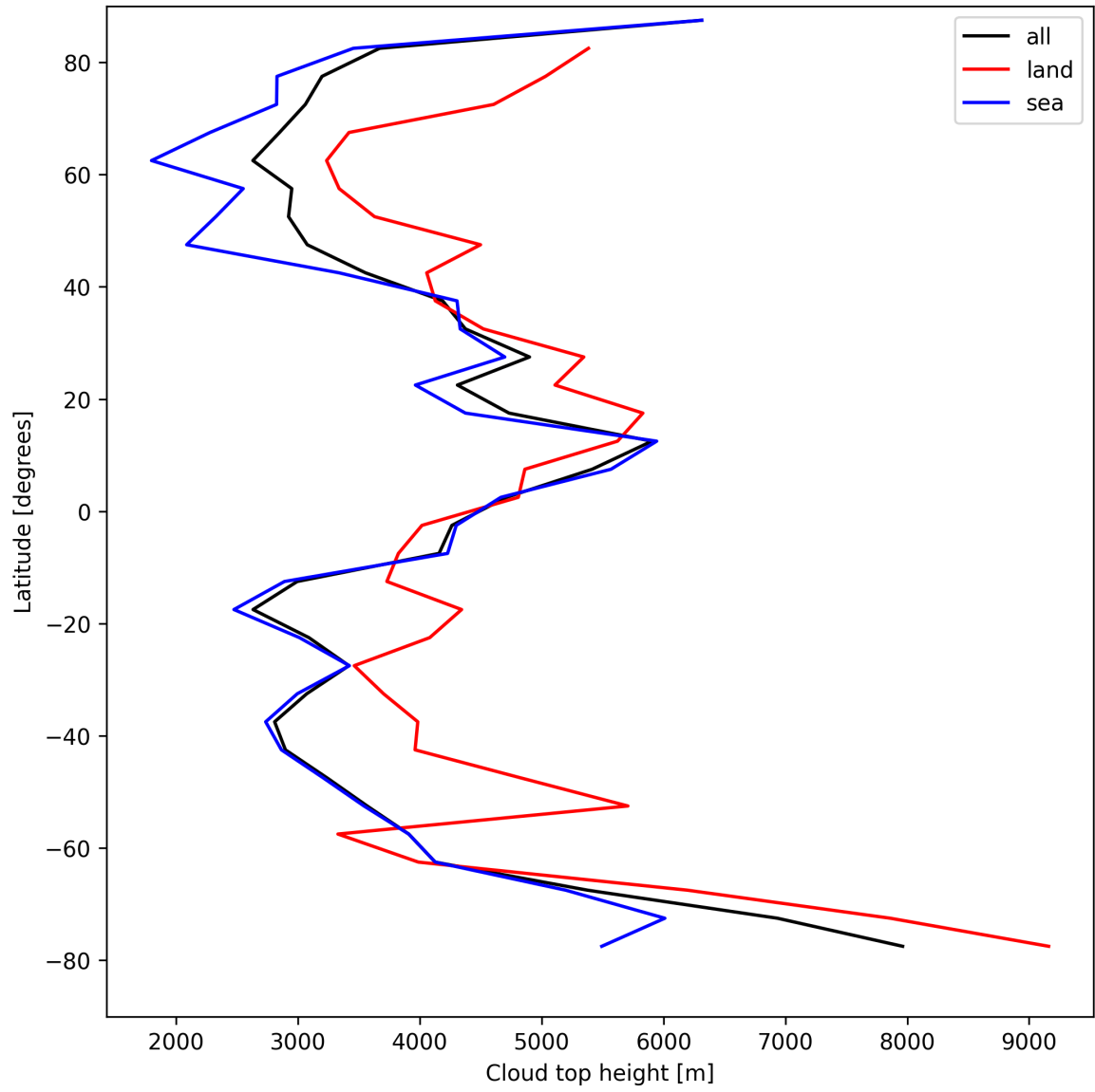
Figure 24: Zonal average of “Cloud top height” for 2025-08-20 to 2025-08-22.
