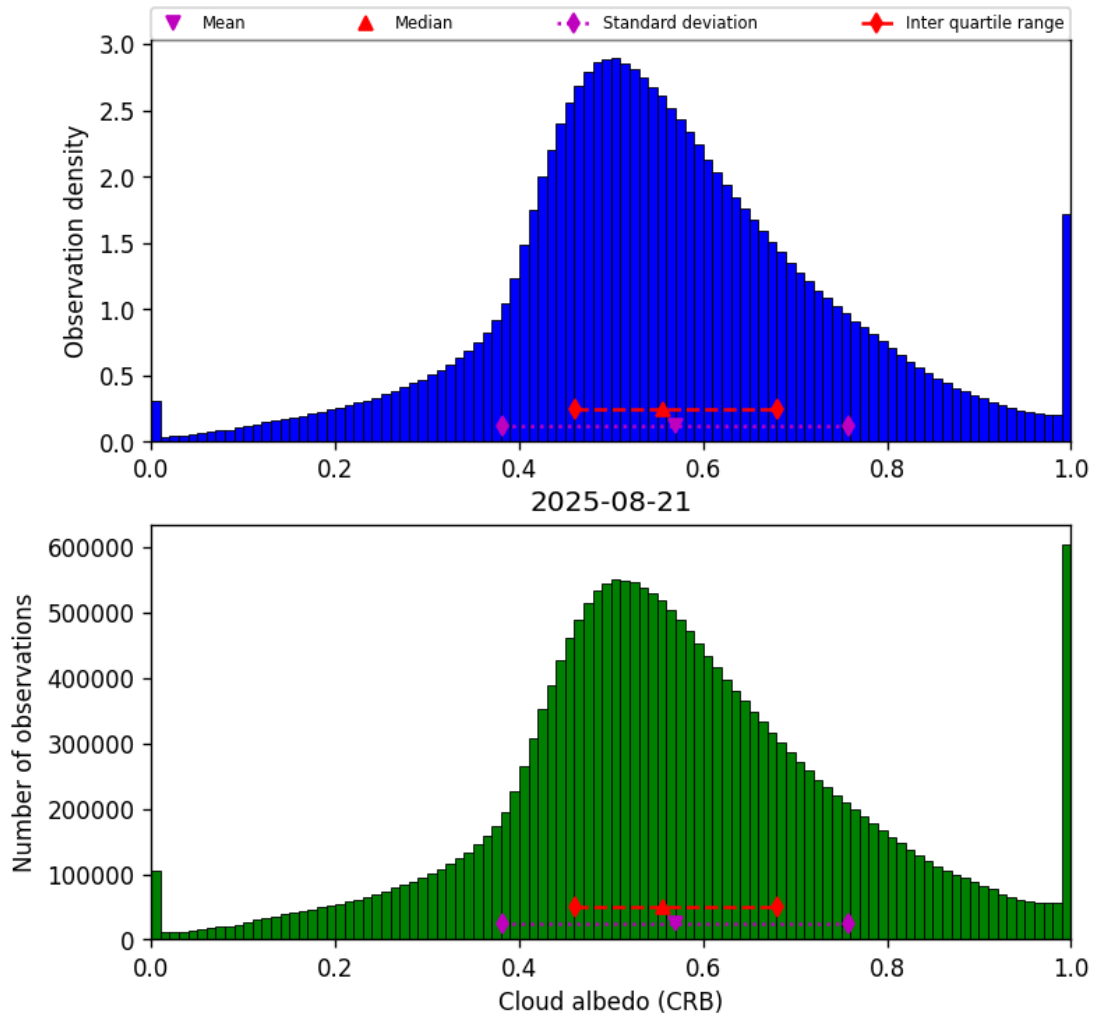
Figure 44: Histogram of “Cloud albedo (CRB)” for 2025-08-20 to 2025-08-22
