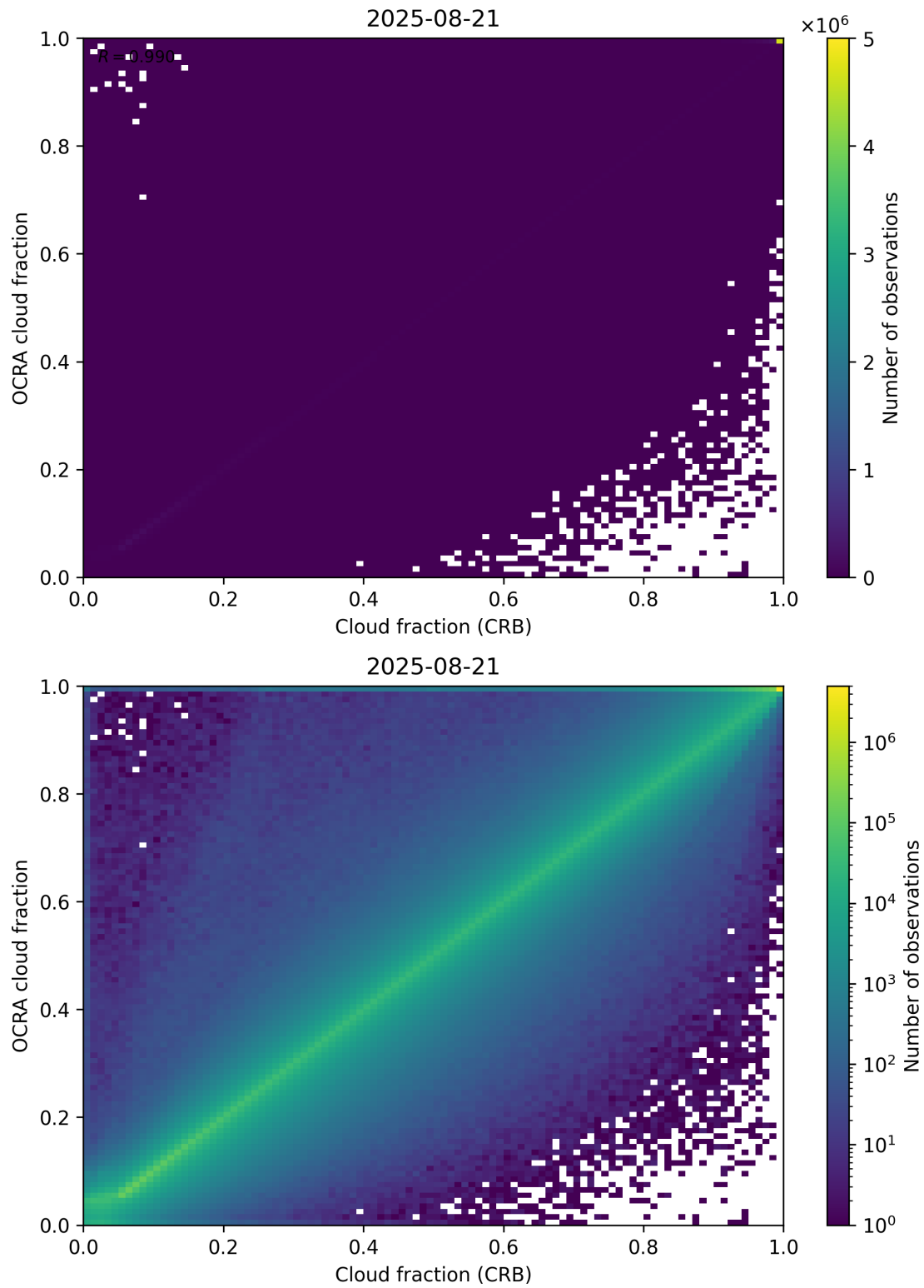
Figure 78: Scatter density plot of “Cloud fraction (CRB)” against “OCRA cloud fraction” for 2025-08-20 to 2025-08-22.
