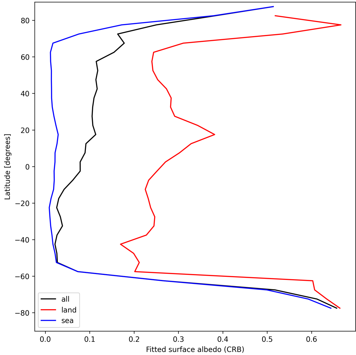
Figure 30: Zonal average of “Fitted surface albedo (CRB)” for 2025-08-20 to 2025-08-22.
