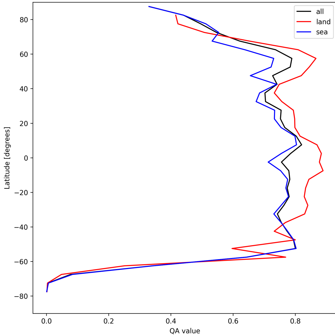
Figure 22: Zonal average of “QA value” for 2025-08-20 to 2025-08-22.
