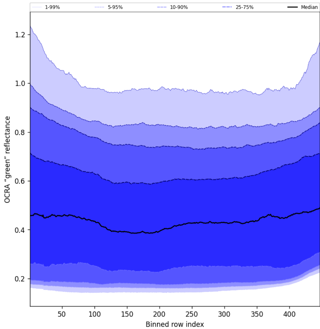
Figure 68: Along track statistics of “OCRA “green” reflectance” for 2025-08-20 to 2025-08-22
