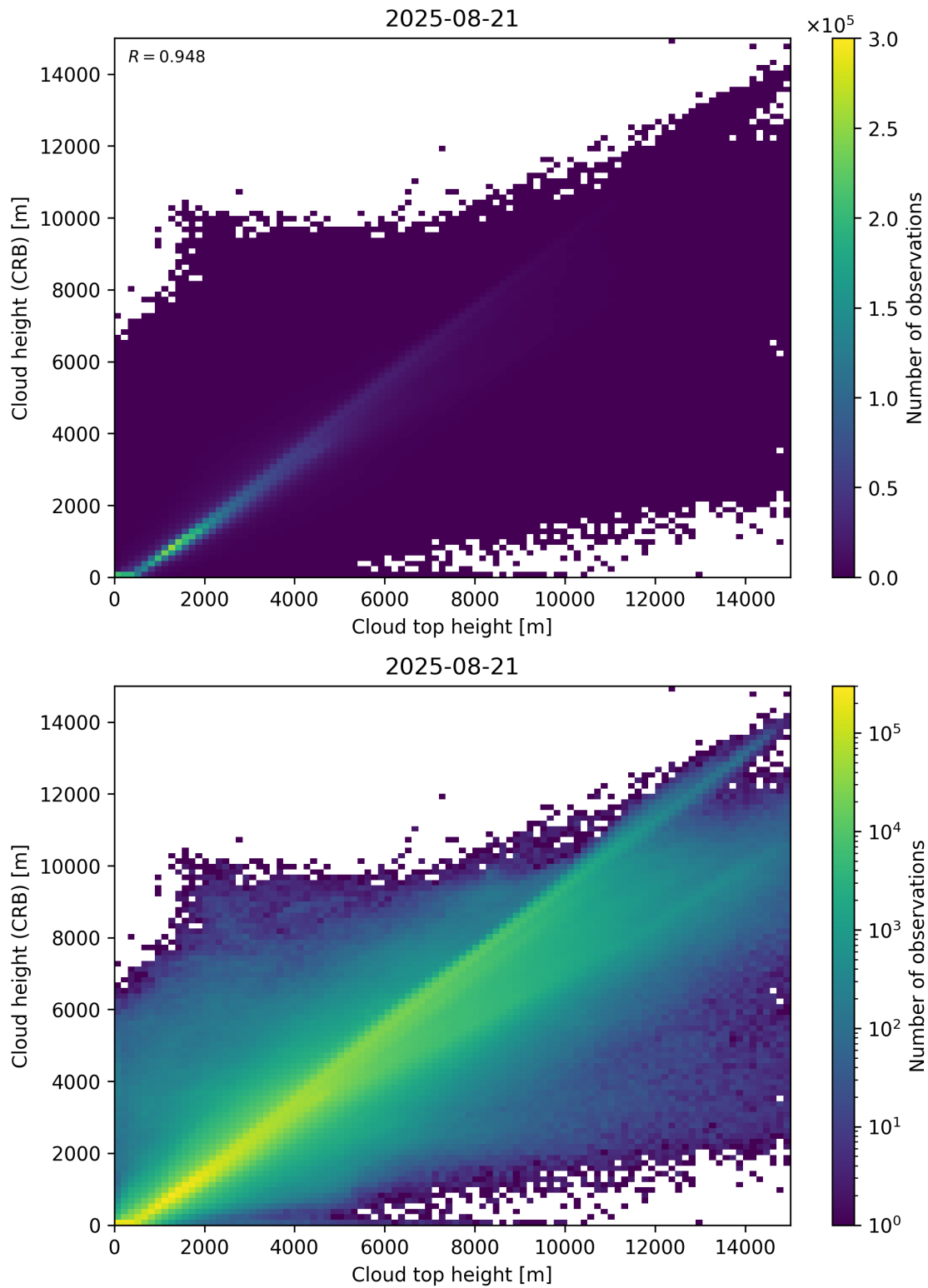
Figure 89: Scatter density plot of “Cloud top height” against “Cloud height (CRB)” for 2025-08-20 to 2025-08-22.
