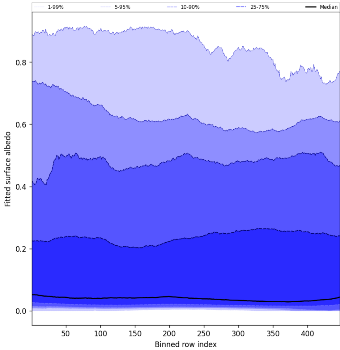
Figure 61: Along track statistics of “Fitted surface albedo” for 2025-08-20 to 2025-08-22
