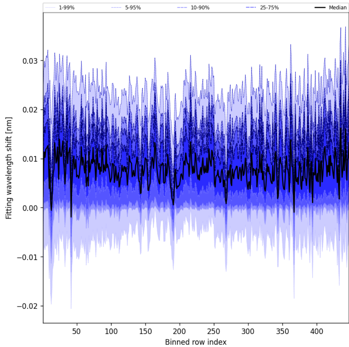
Figure 65: Along track statistics of “Fitting wavelength shift” for 2025-08-20 to 2025-08-22
