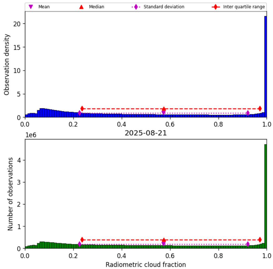
Figure 39: Histogram of “Radiometric cloud fraction” for 2025-08-20 to 2025-08-22
