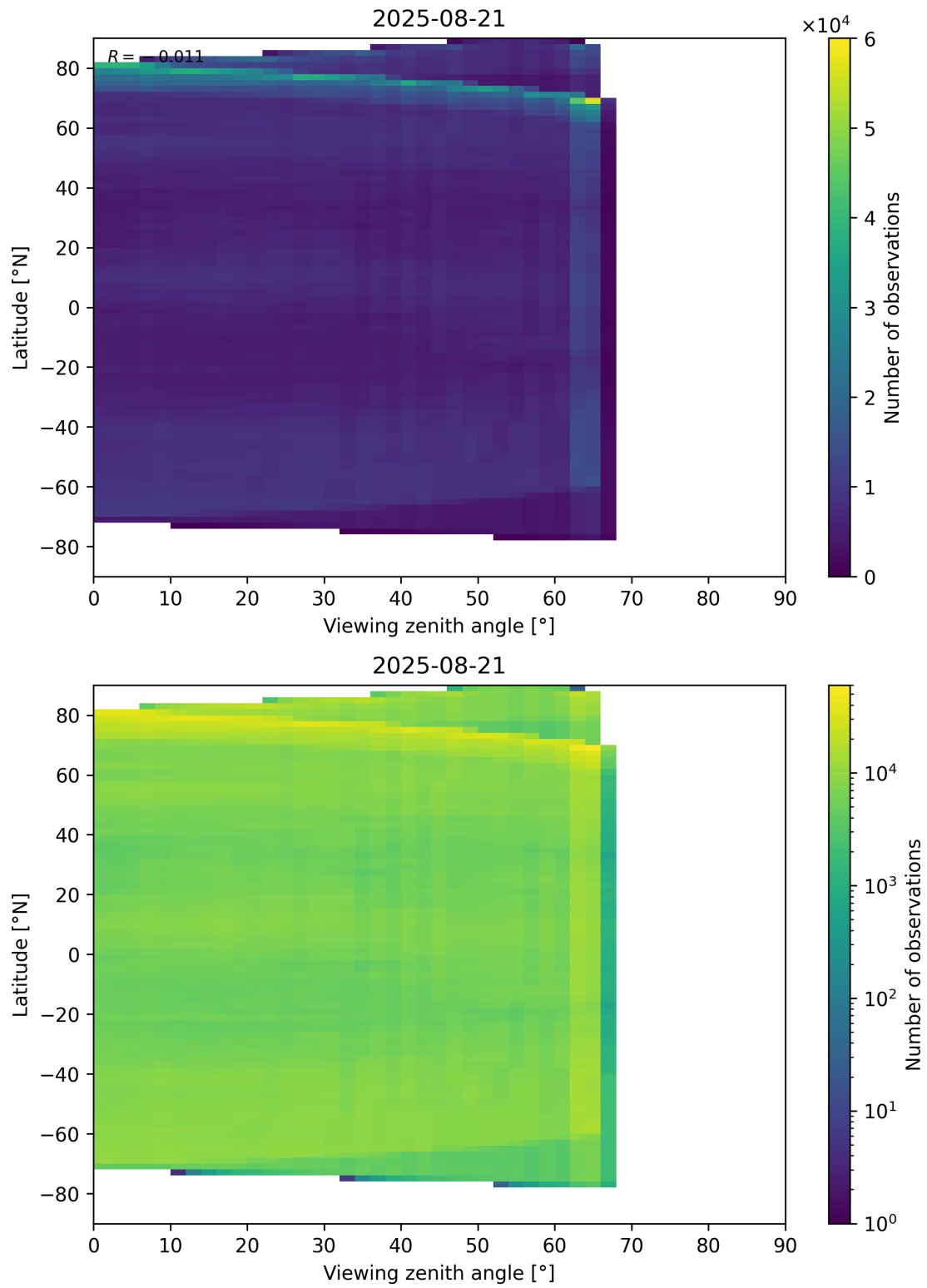
Figure 113: Scatter density plot of “Viewing zenith angle” against “Latitude” for 2025-08-20 to 2025-08-22.
