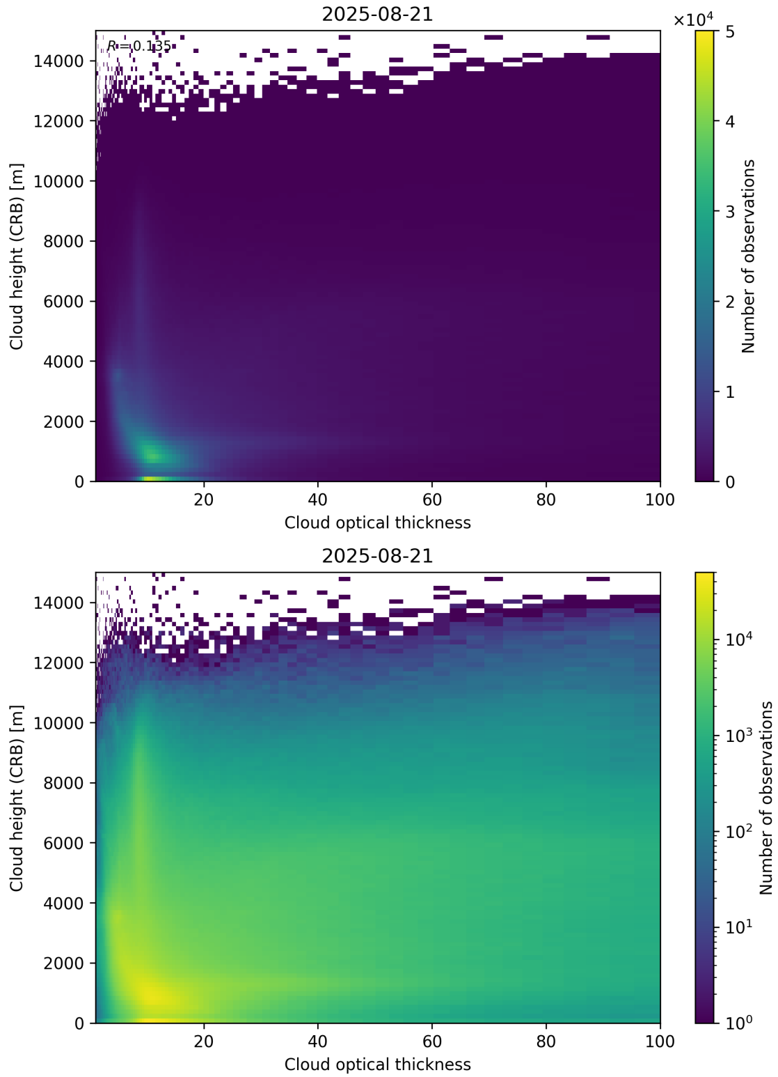
Figure 85: Scatter density plot of “Cloud optical thickness” against “Cloud height (CRB)” for 2025-08-20 to 2025-08-22.
