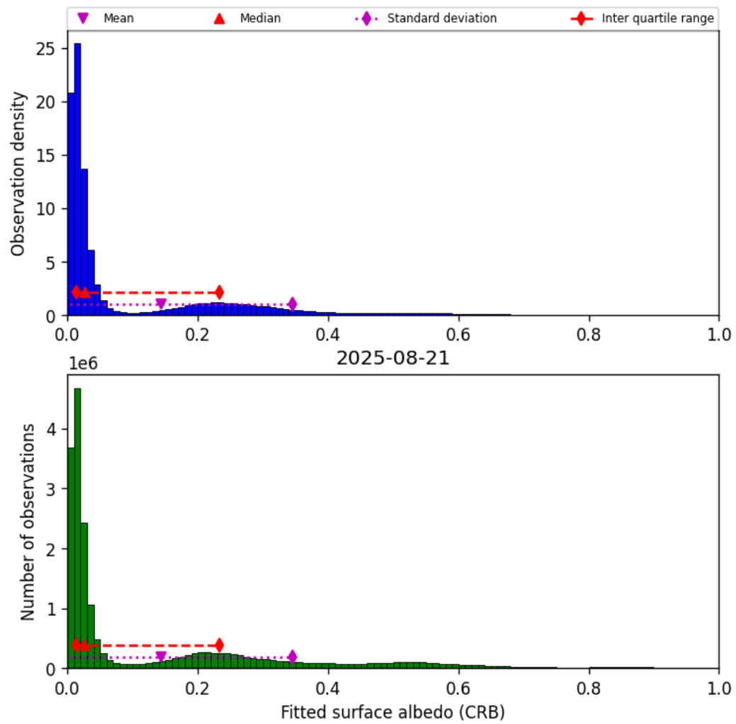
Figure 46: Histogram of “Fitted surface albedo (CRB)” for 2025-08-20 to 2025-08-22
