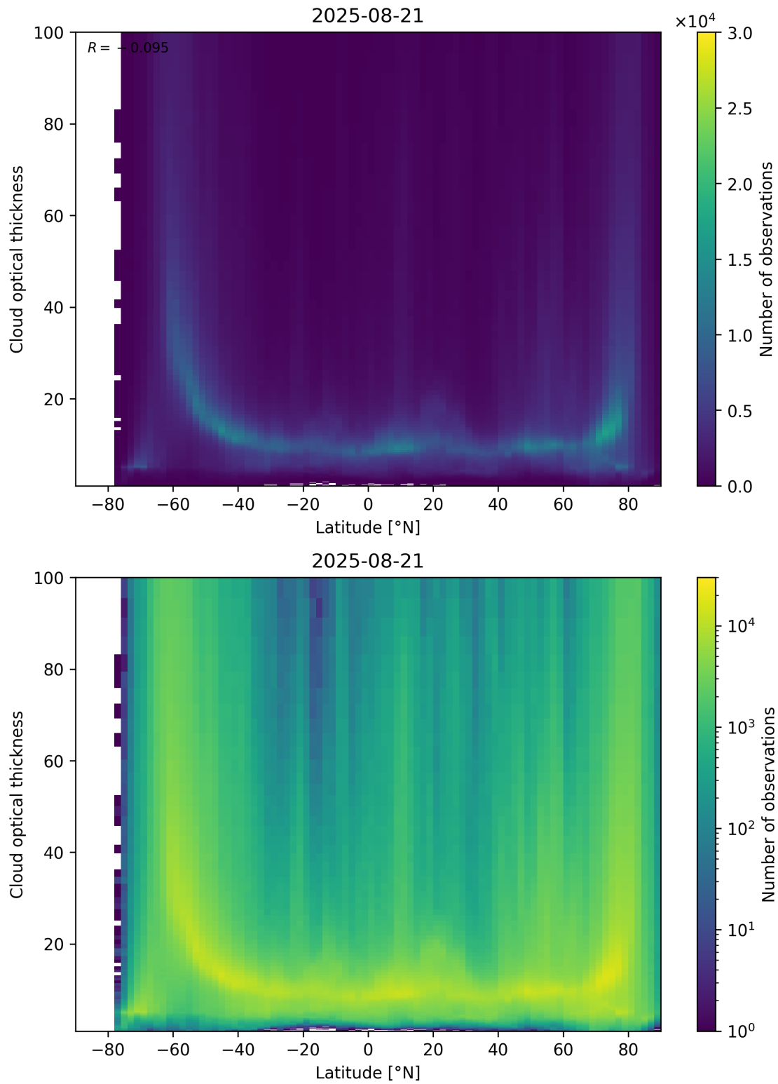
Figure 96: Scatter density plot of “Latitude” against “Cloud optical thickness” for 2025-08-20 to 2025-08-22.
