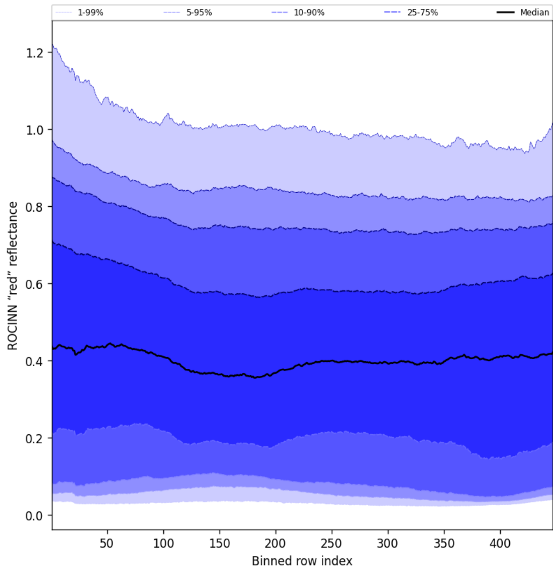
Figure 69: Along track statistics of “ROCINN “red” reflectance” for 2025-08-20 to 2025-08-22
