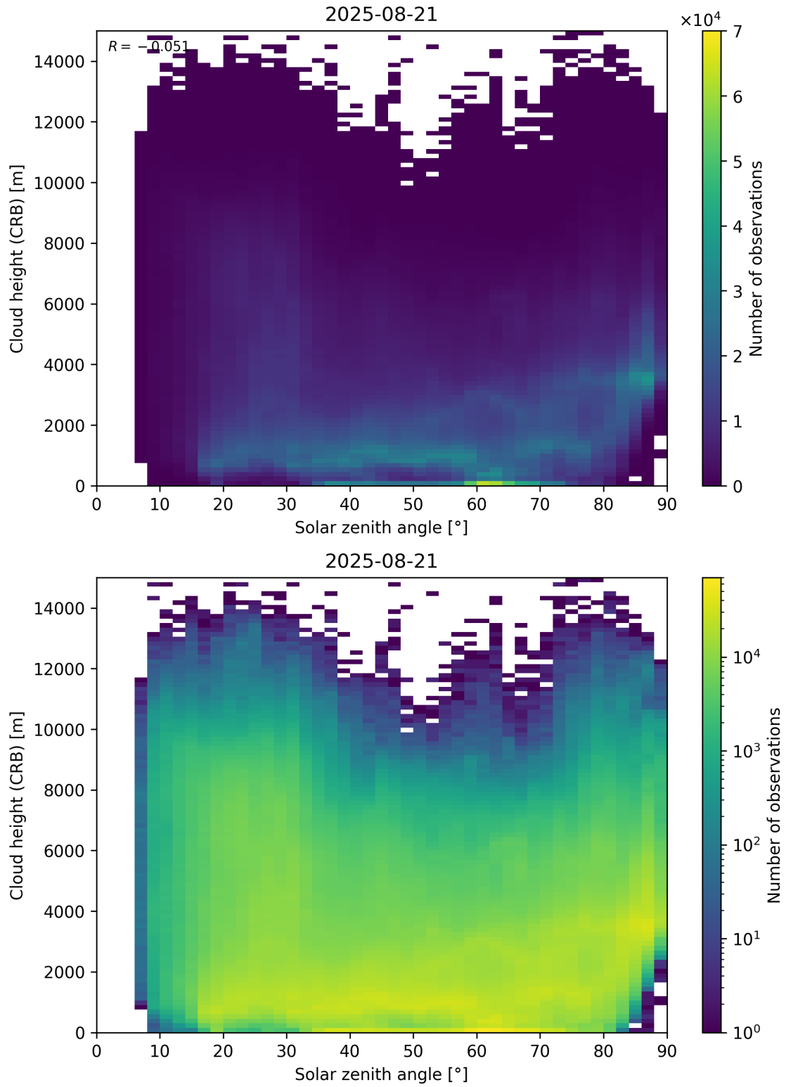
Figure 102: Scatter density plot of “Solar zenith angle” against “Cloud height (CRB)” for 2025-08-20 to 2025-08-22.
