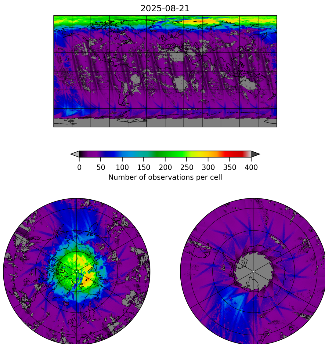
Figure 21: Map of the number of observations for 2025-08-20 to 2025-08-22
