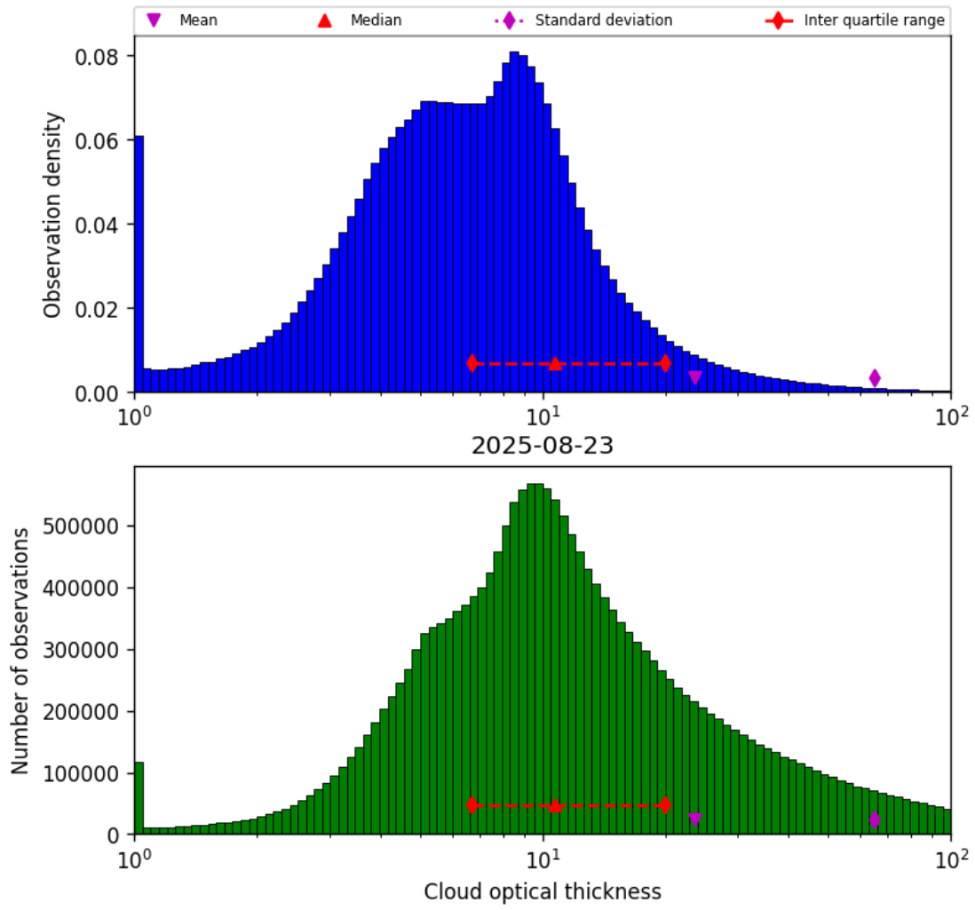
Figure 41: Histogram of “Cloud optical thickness” for 2025-08-22 to 2025-08-24
