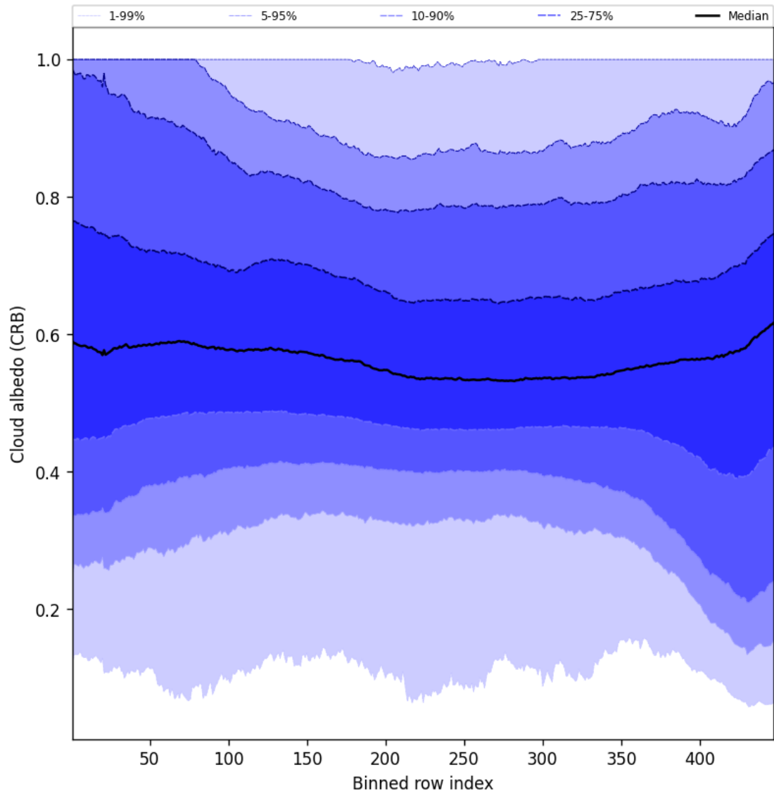
Figure 60: Along track statistics of “Cloud albedo (CRB)” for 2025-08-22 to 2025-08-24
