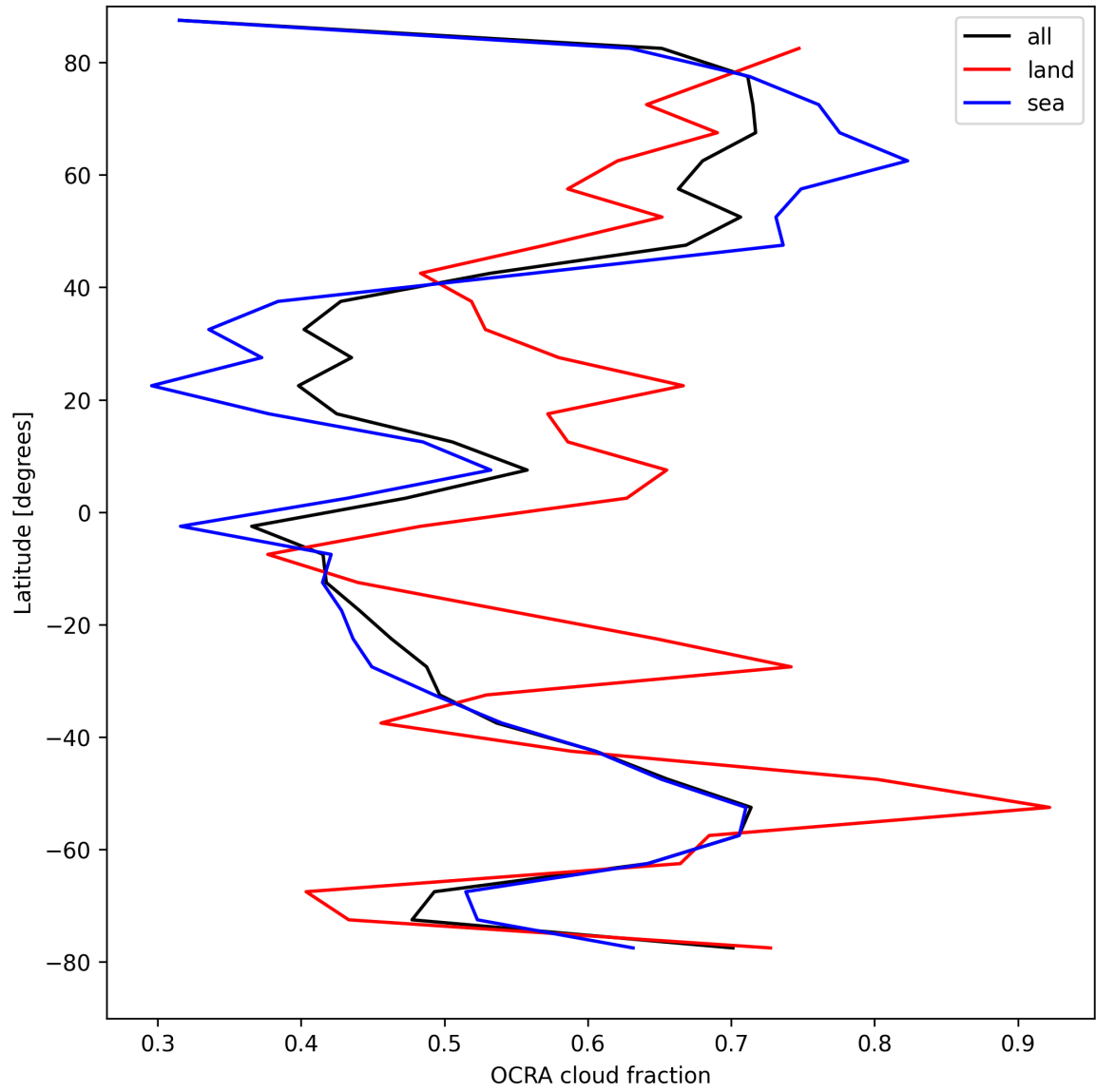
Figure 34: Zonal average of “OCRA cloud fraction” for 2025-08-22 to 2025-08-24.
