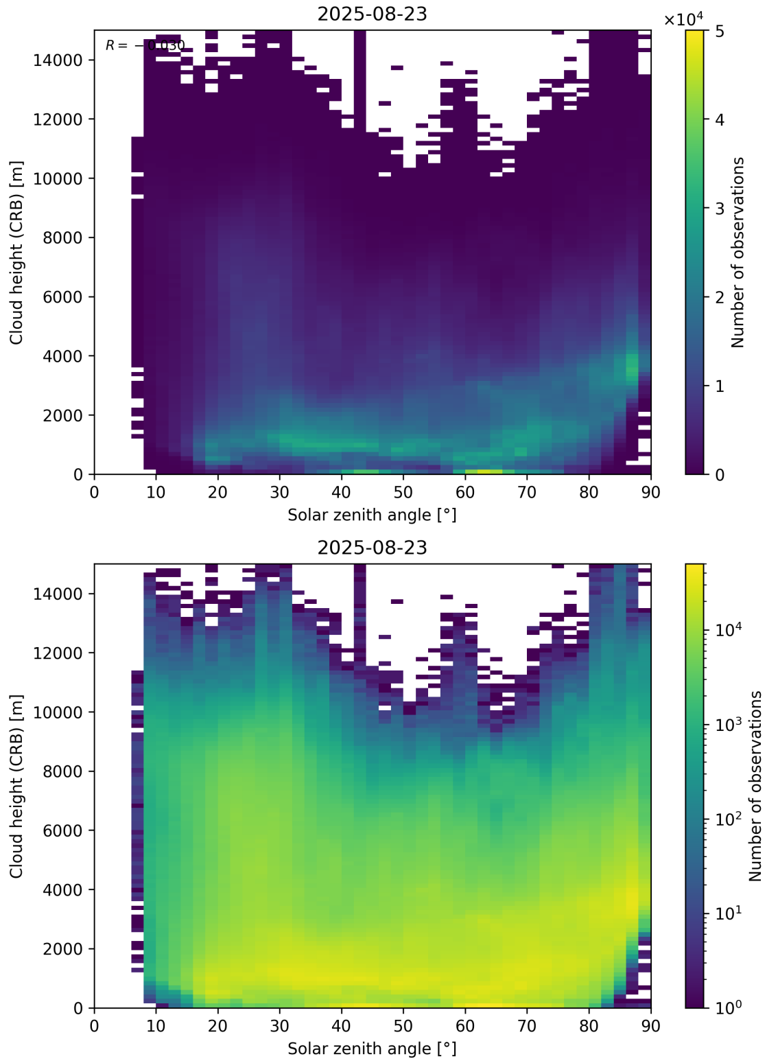
Figure 102: Scatter density plot of “Solar zenith angle” against “Cloud height (CRB)” for 2025-08-22 to 2025-08-24.
