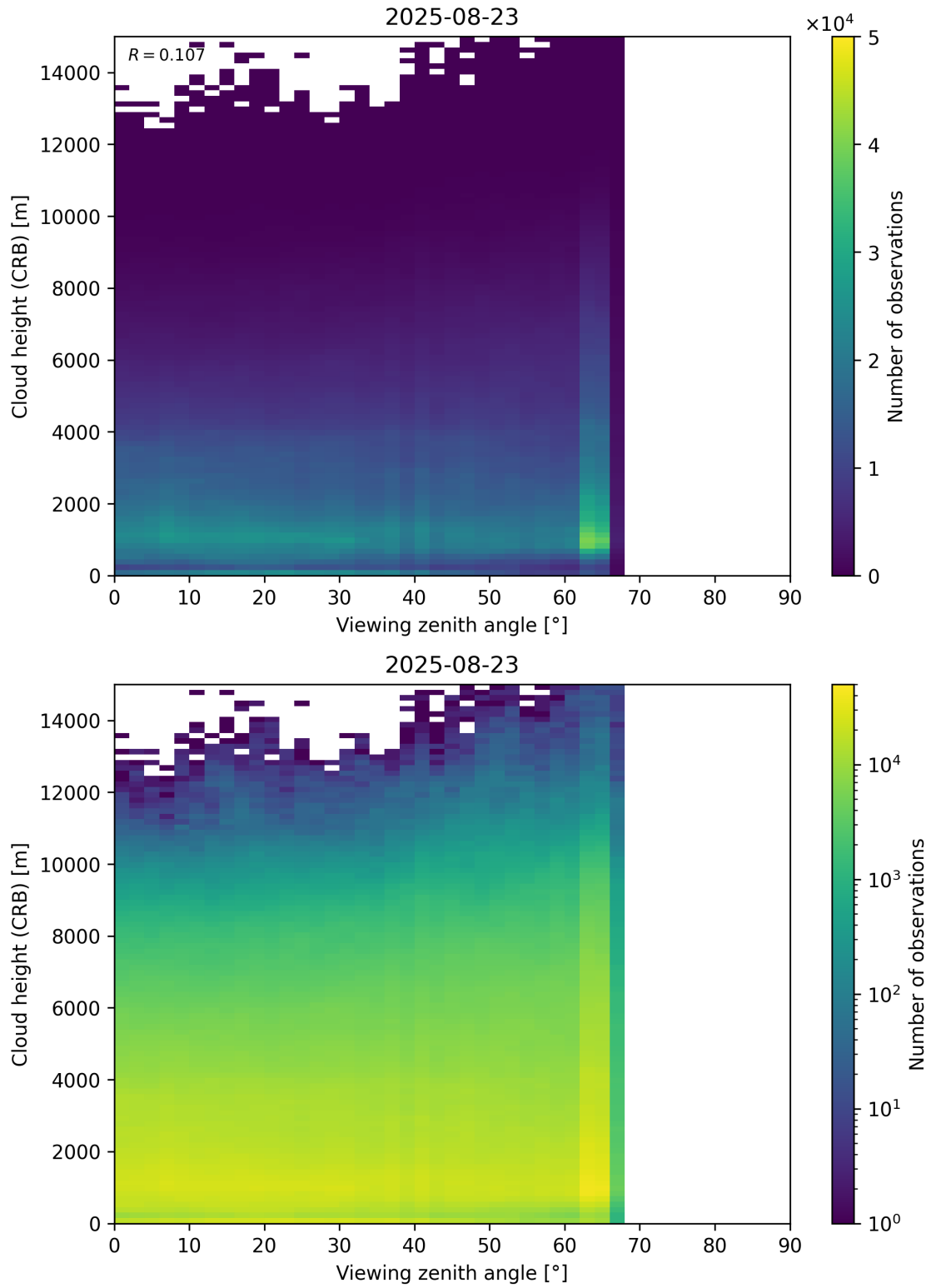
Figure 110: Scatter density plot of “Viewing zenith angle” against “Cloud height (CRB)” for 2025-08-22 to 2025-08-24.
