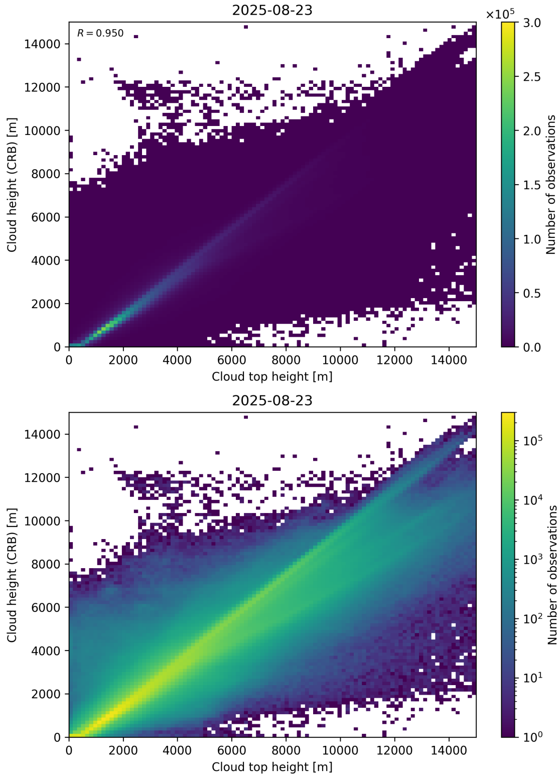
Figure 89: Scatter density plot of “Cloud top height” against “Cloud height (CRB)” for 2025-08-22 to 2025-08-24.
