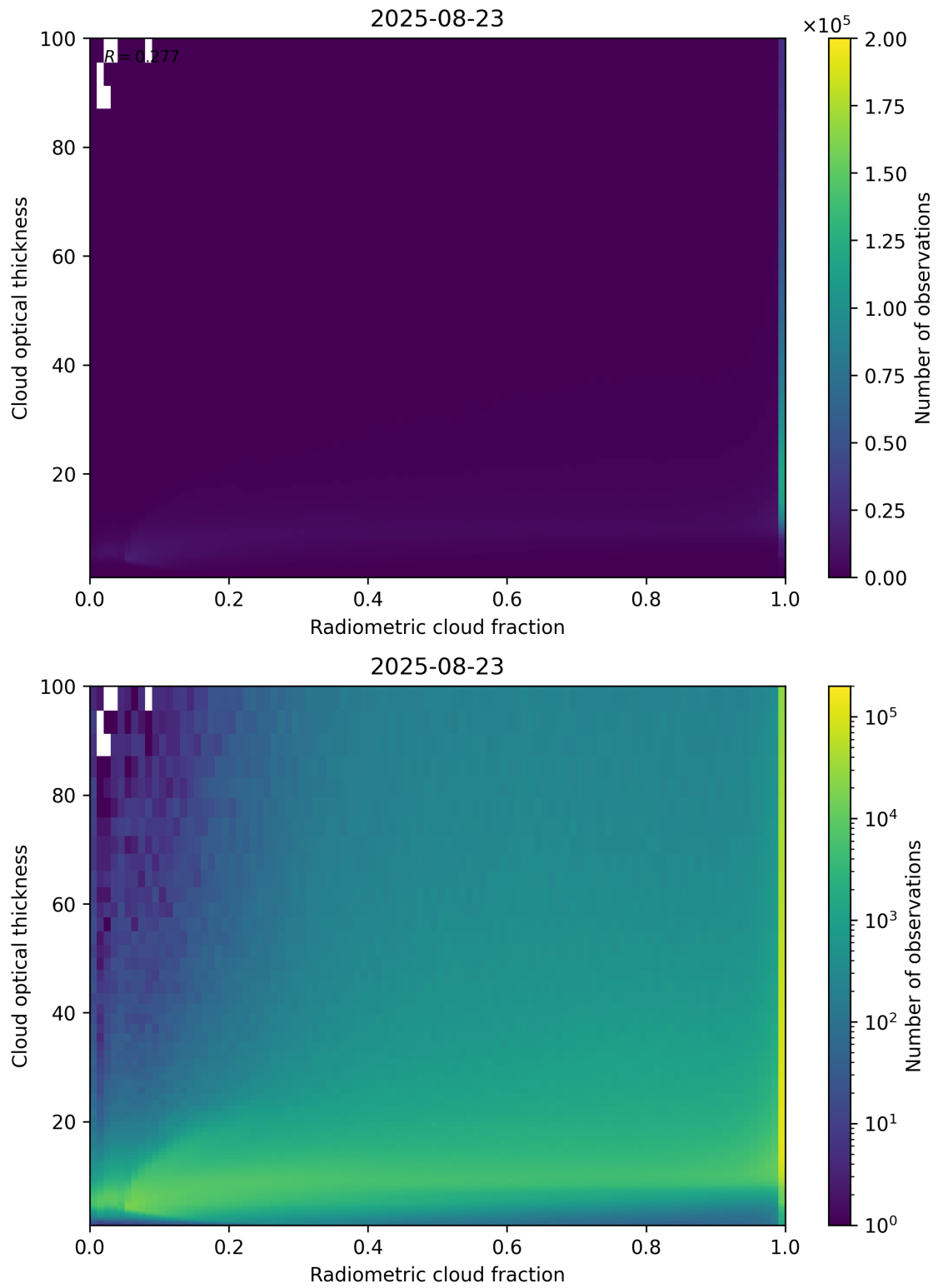
Figure 75: Scatter density plot of “Radiometric cloud fraction” against “Cloud optical thickness” for 2025-08-22 to 2025-08-24.
