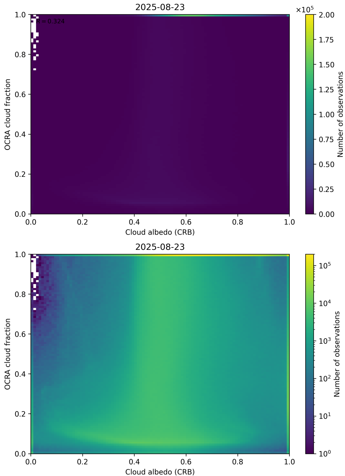
Figure 70: Scatter density plot of “Cloud albedo (CRB)” against “OCRA cloud fraction” for 2025-08-22 to 2025-08-24.
