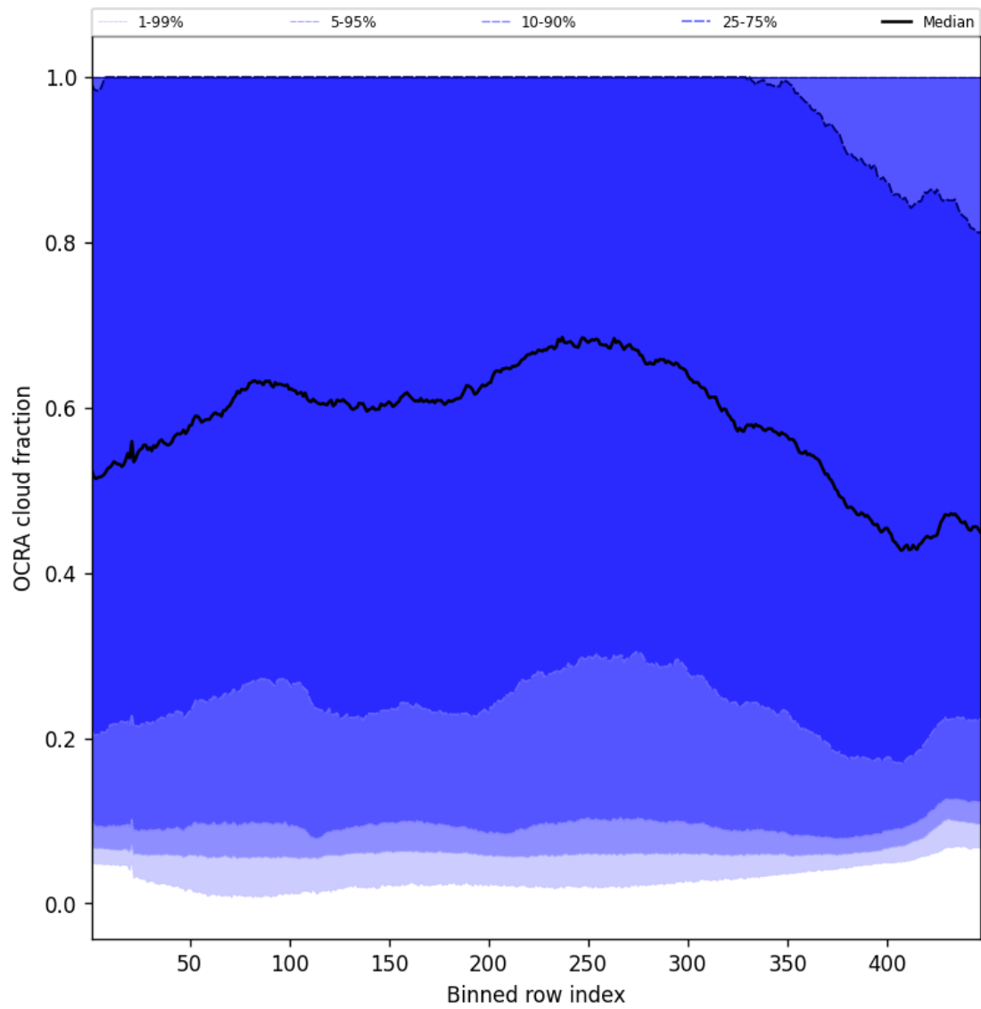
Figure 66: Along track statistics of “OCRA cloud fraction” for 2025-08-22 to 2025-08-24
