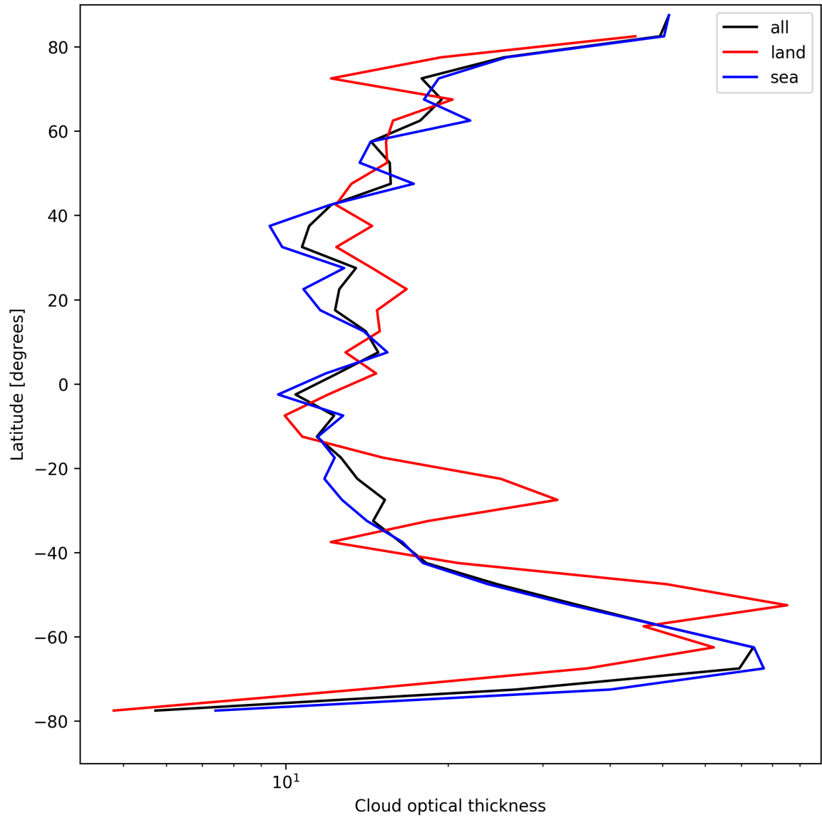
Figure 25: Zonal average of “Cloud optical thickness” for 2025-08-22 to 2025-08-24.
