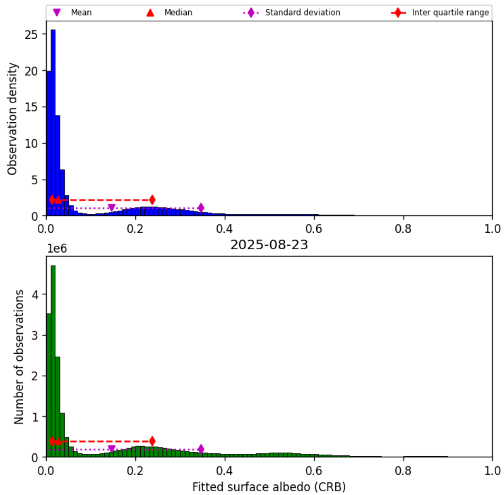
Figure 46: Histogram of “Fitted surface albedo (CRB)” for 2025-08-22 to 2025-08-24
