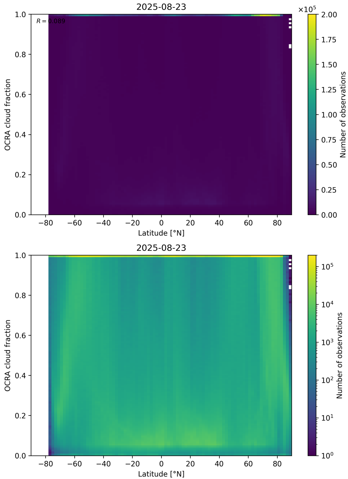
Figure 93: Scatter density plot of “Latitude” against “OCRA cloud fraction” for 2025-08-22 to 2025-08-24.
