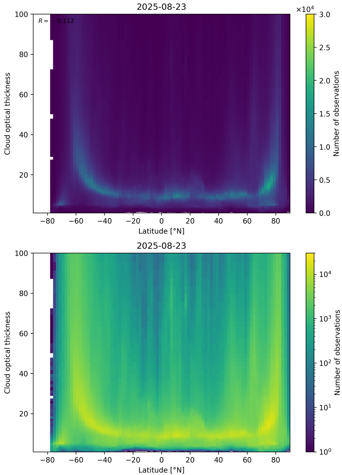
Figure 96: Scatter density plot of “Latitude” against “Cloud optical thickness” for 2025-08-22 to 2025-08-24.
