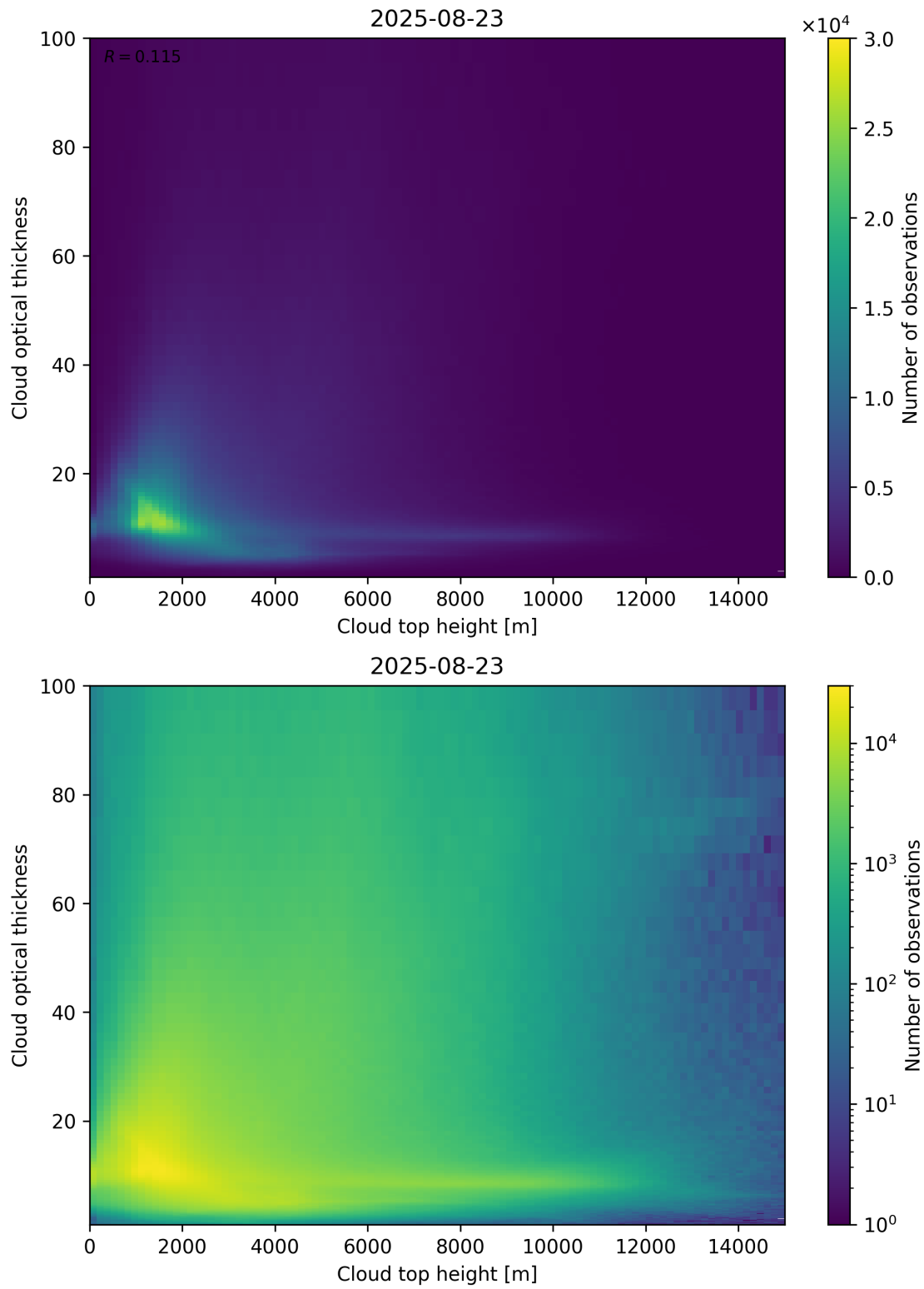
Figure 90: Scatter density plot of “Cloud top height” against “Cloud optical thickness” for 2025-08-22 to 2025-08-24.
