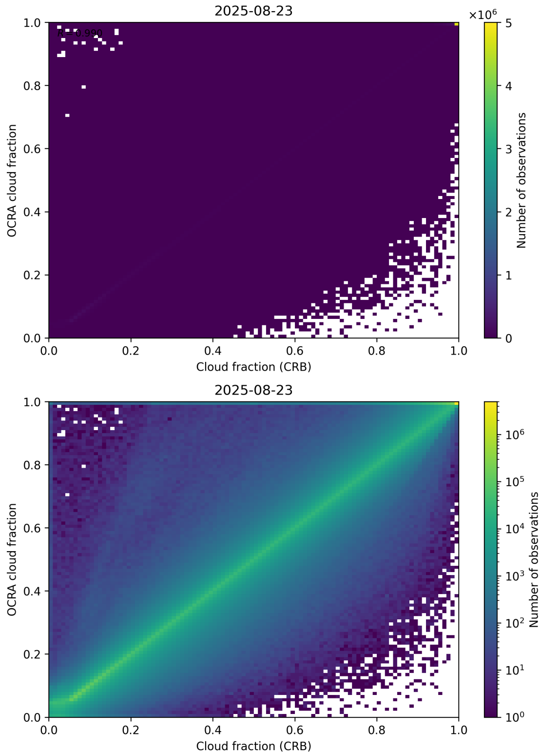
Figure 78: Scatter density plot of “Cloud fraction (CRB)” against “OCRA cloud fraction” for 2025-08-22 to 2025-08-24.
