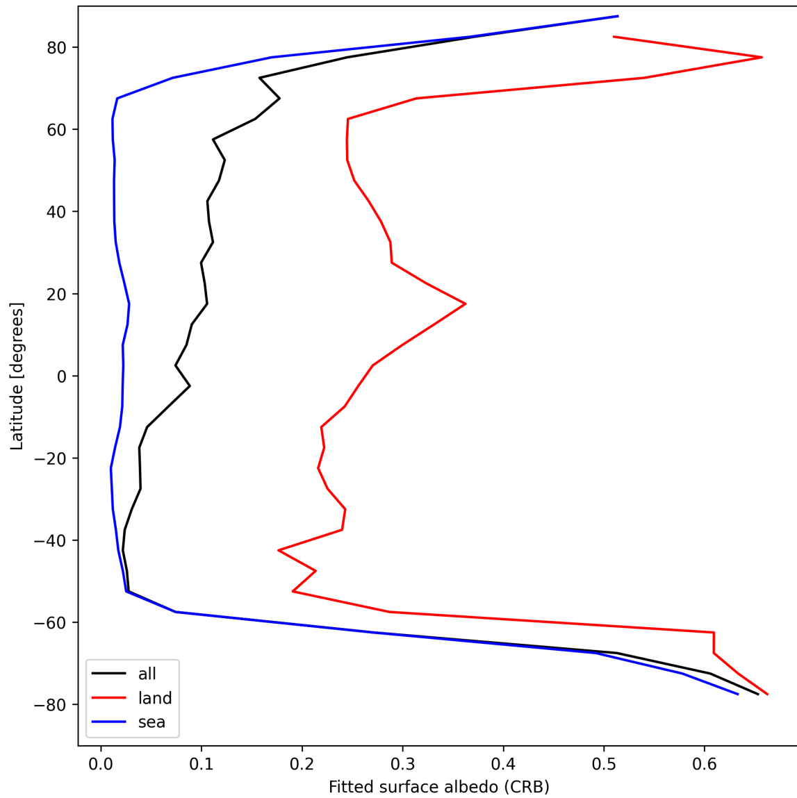
Figure 30: Zonal average of “Fitted surface albedo (CRB)” for 2025-08-22 to 2025-08-24.
