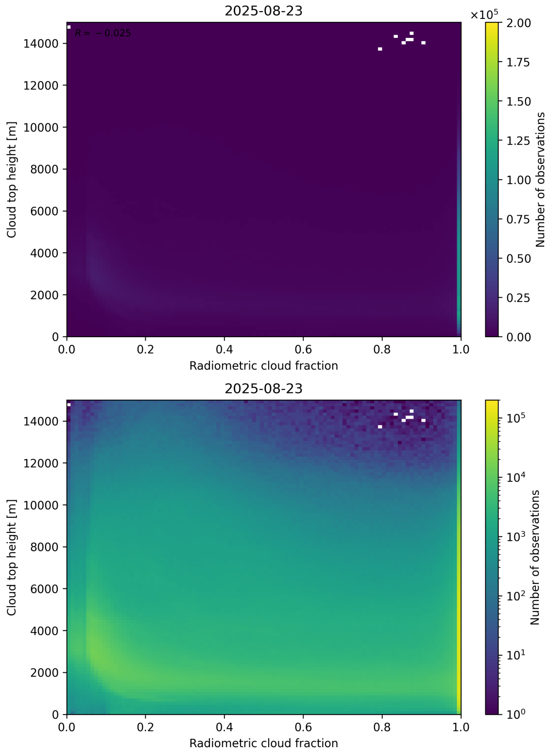
Figure 76: Scatter density plot of “Radiometric cloud fraction” against “Cloud top height” for 2025-08-22 to 2025-08-24.
