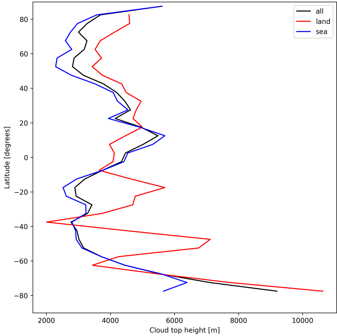
Figure 24: Zonal average of “Cloud top height” for 2025-08-22 to 2025-08-24.
