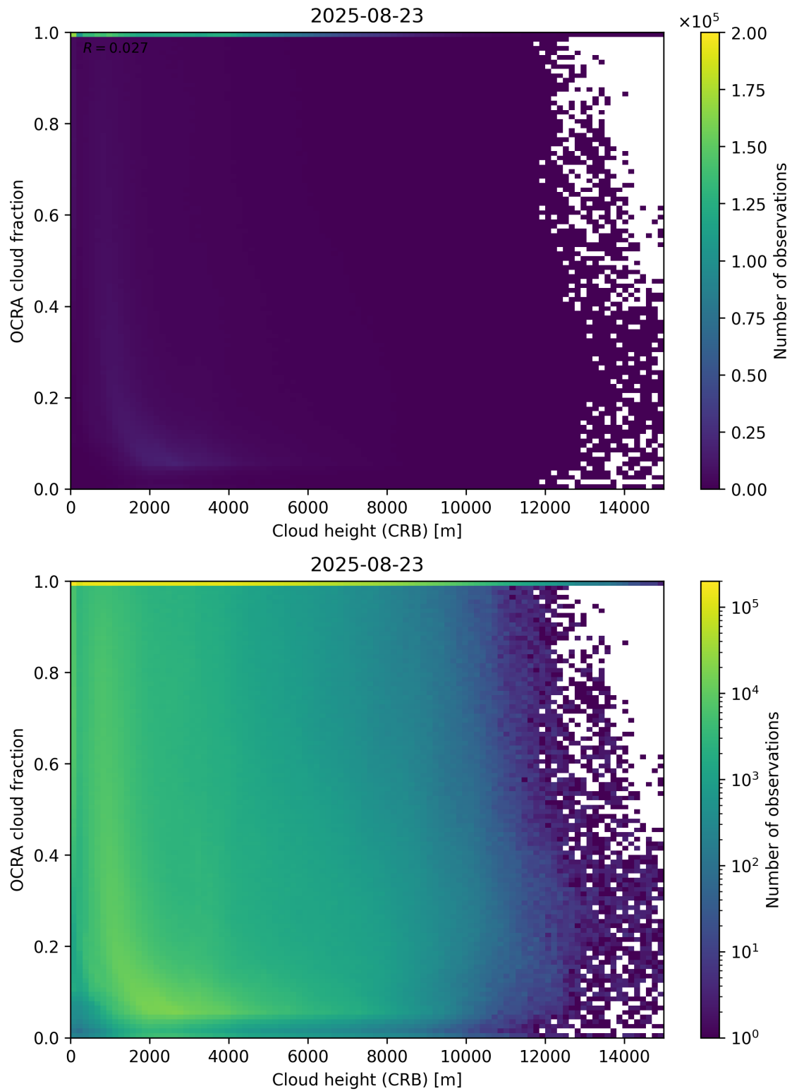
Figure 81: Scatter density plot of “Cloud height (CRB)” against “OCRA cloud fraction” for 2025-08-22 to 2025-08-24.
