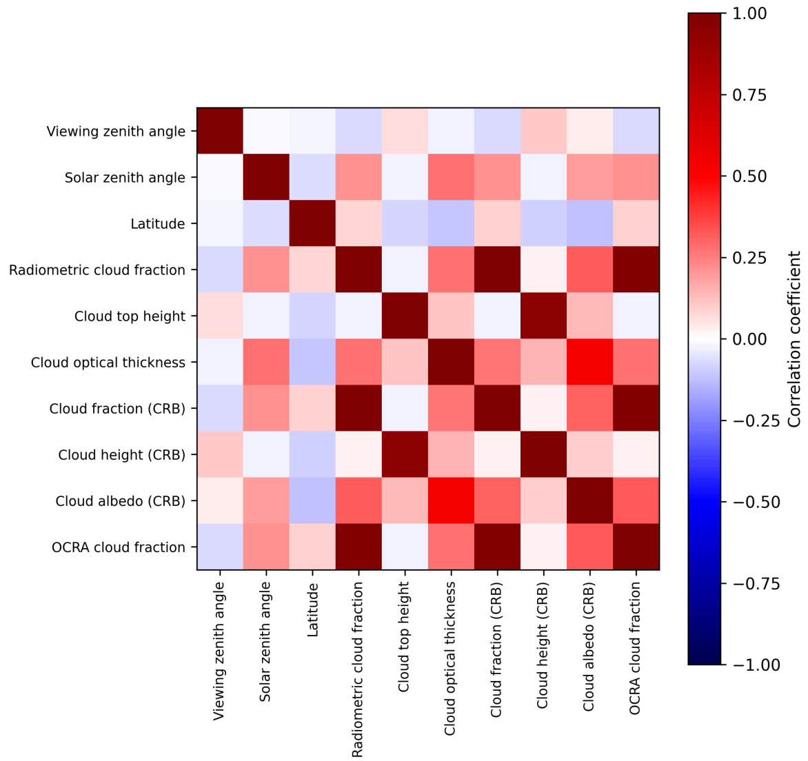
Figure 2: Map of correlation matrix for 2025-08-22 to 2025-08-24.
