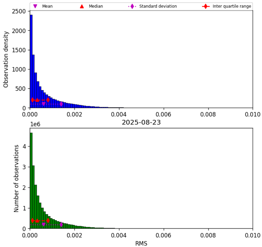
Figure 47: Histogram of “RMS” for 2025-08-22 to 2025-08-24
