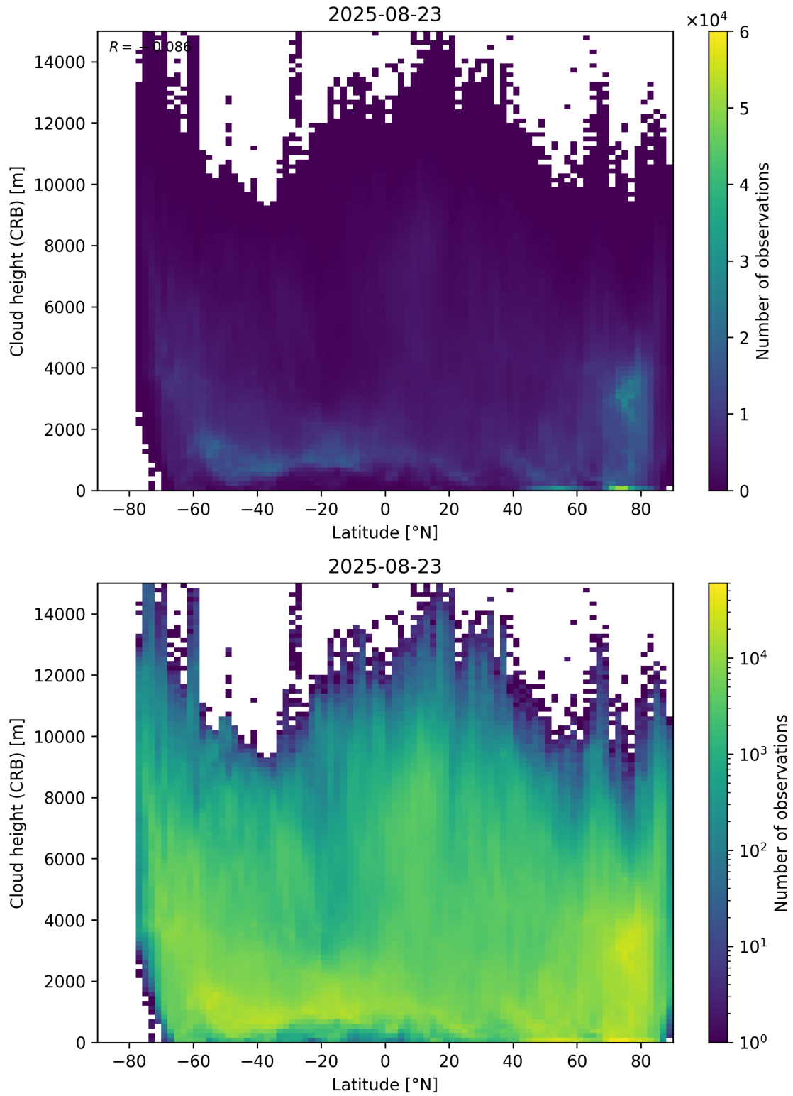
Figure 95: Scatter density plot of “Latitude” against “Cloud height (CRB)” for 2025-08-22 to 2025-08-24.
