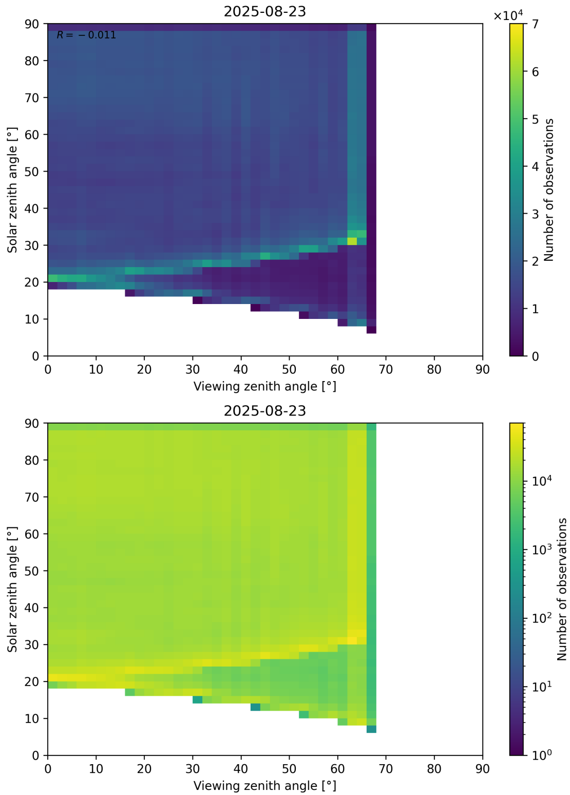
Figure 114: Scatter density plot of “Viewing zenith angle” against “Solar zenith angle” for 2025-08-22 to 2025-08-24.
