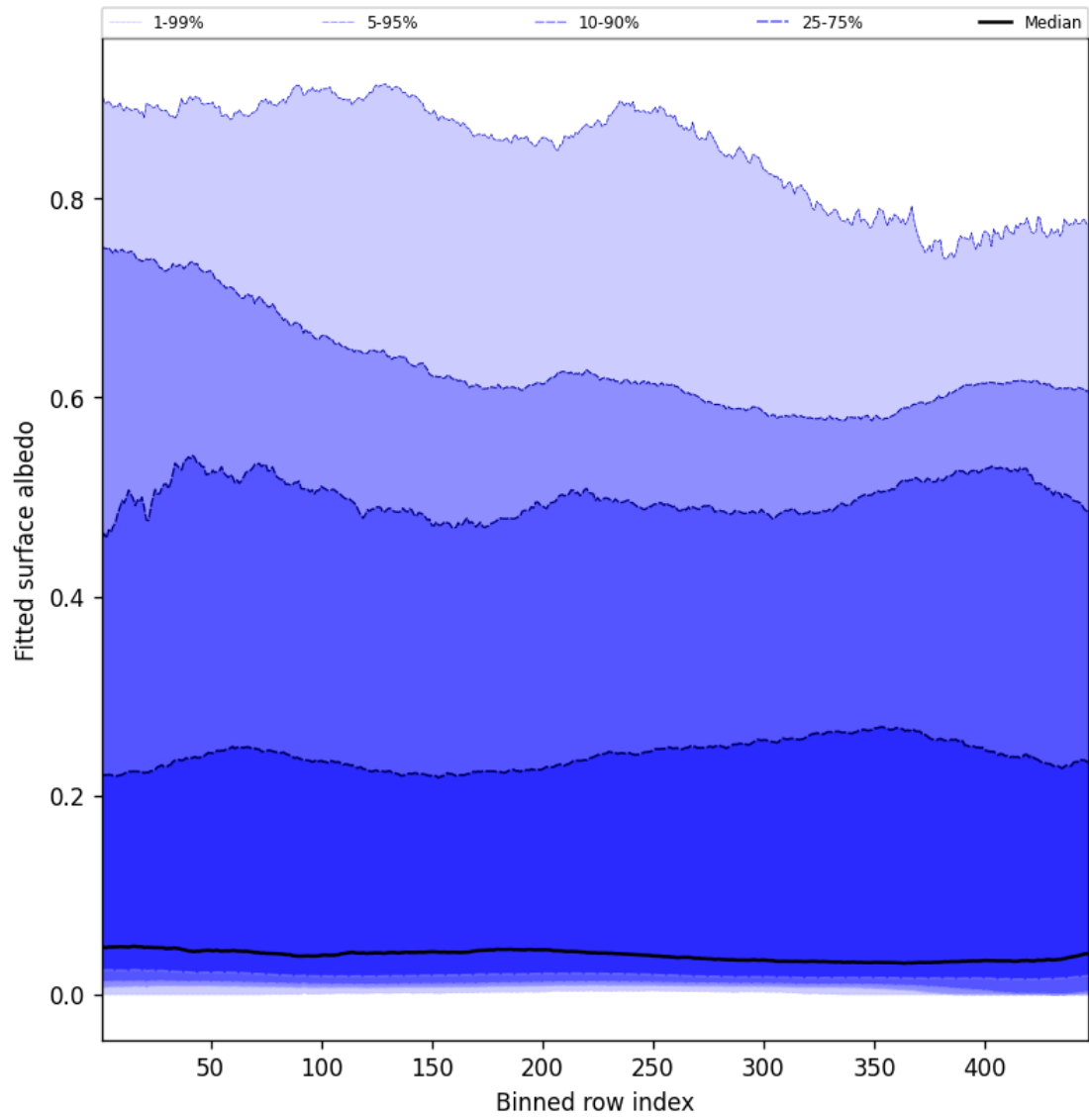
Figure 61: Along track statistics of “Fitted surface albedo” for 2025-08-22 to 2025-08-24
