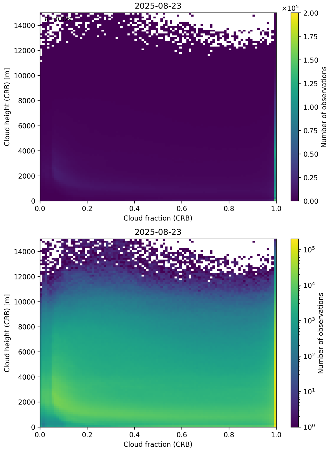
Figure 79: Scatter density plot of “Cloud fraction (CRB)” against “Cloud height (CRB)” for 2025-08-22 to 2025-08-24.
