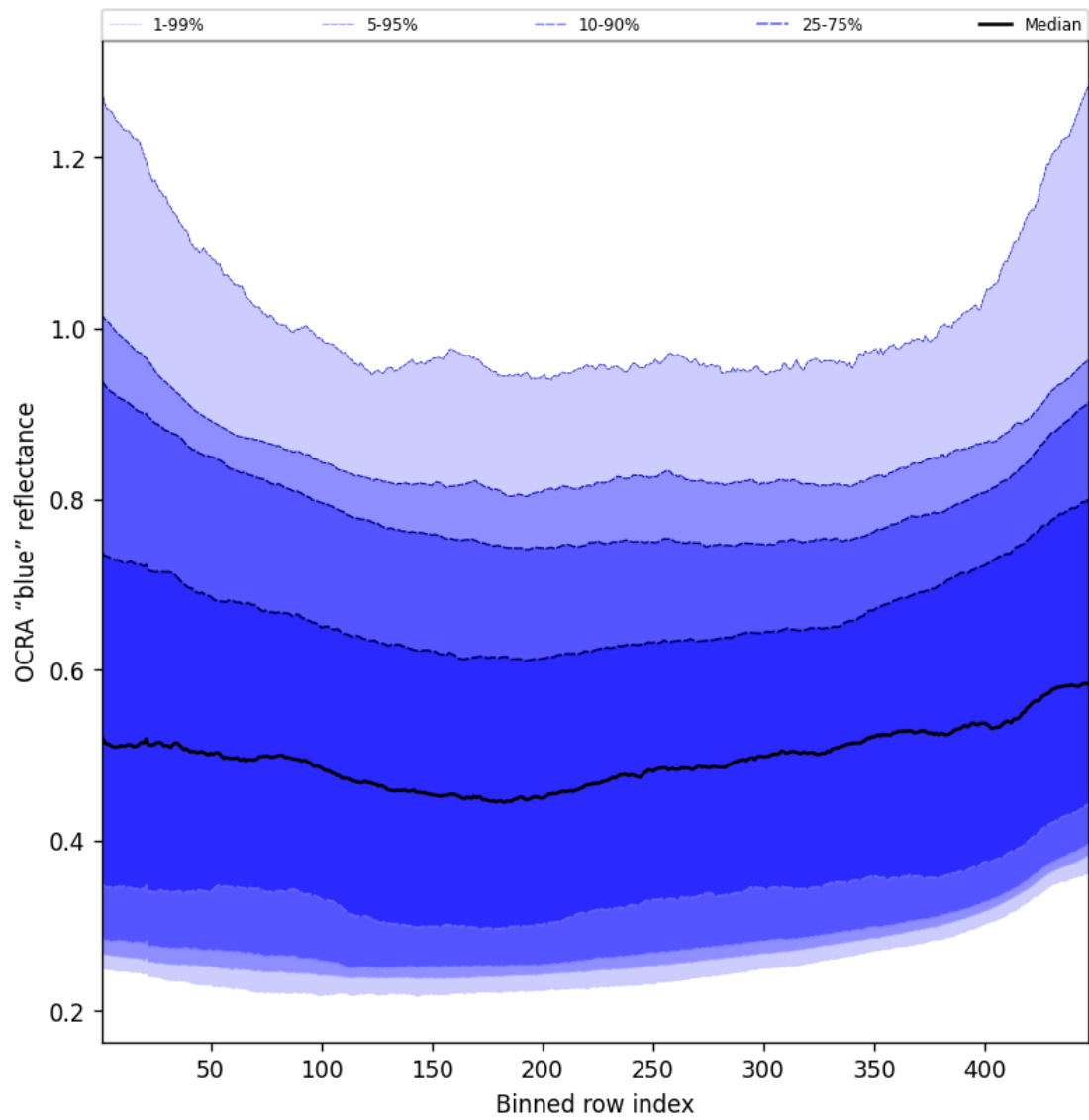
Figure 67: Along track statistics of “OCRA “blue” reflectance” for 2025-08-22 to 2025-08-24
