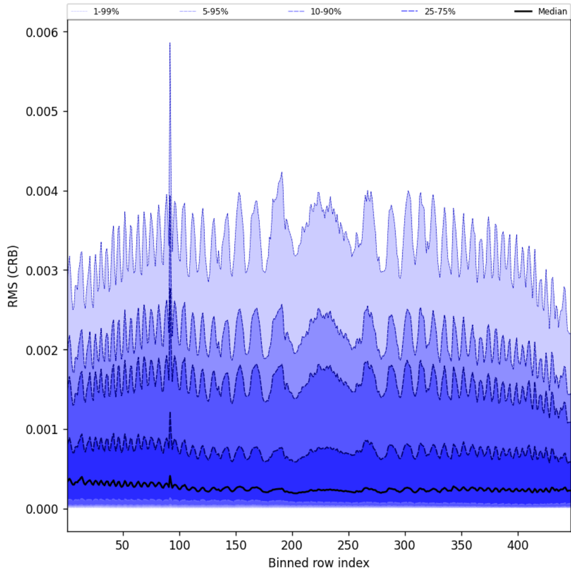
Figure 64: Along track statistics of “RMS (CRB)” for 2025-08-22 to 2025-08-24
