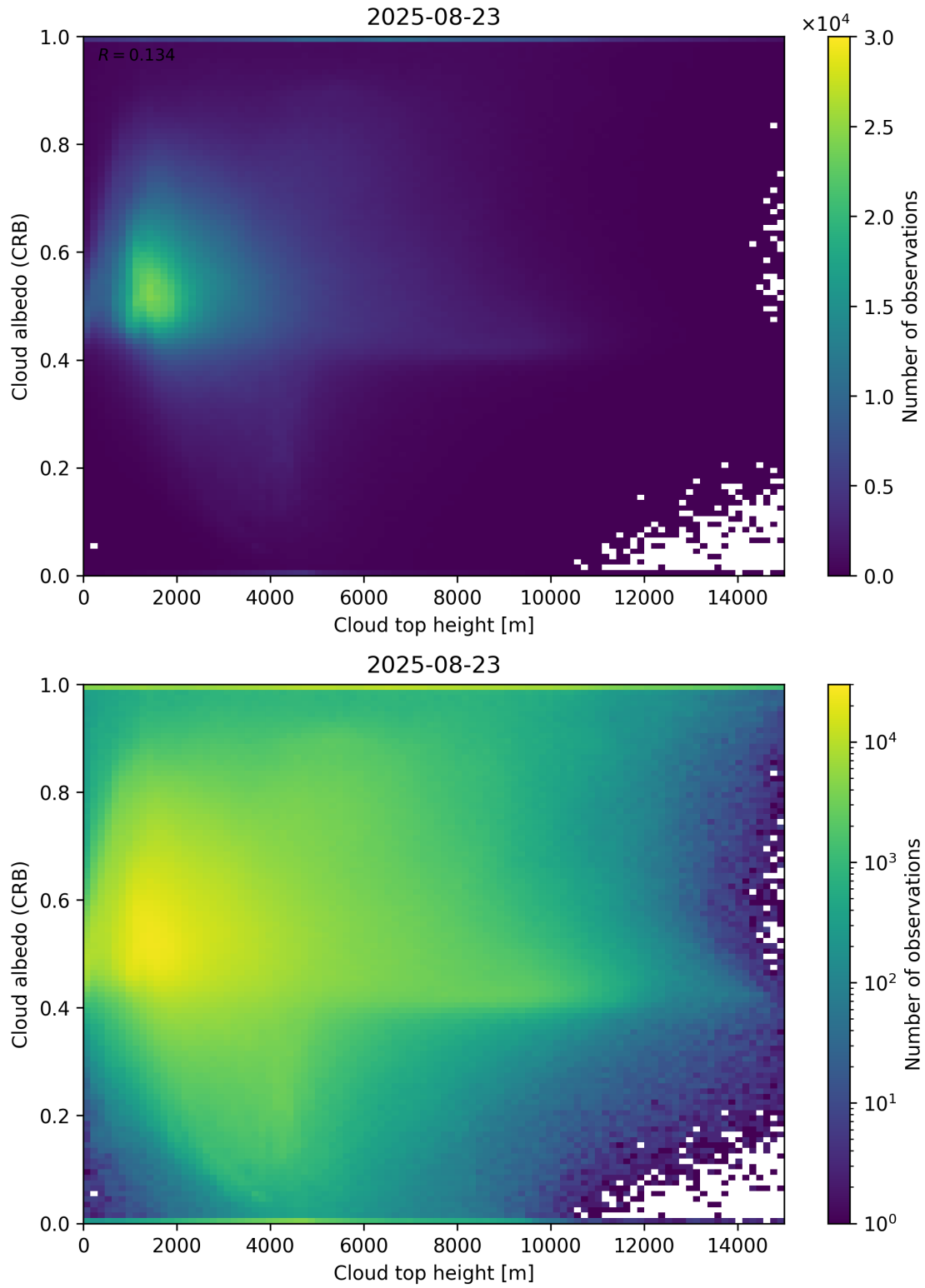
Figure 86: Scatter density plot of “Cloud top height” against “Cloud albedo (CRB)” for 2025-08-22 to 2025-08-24.
