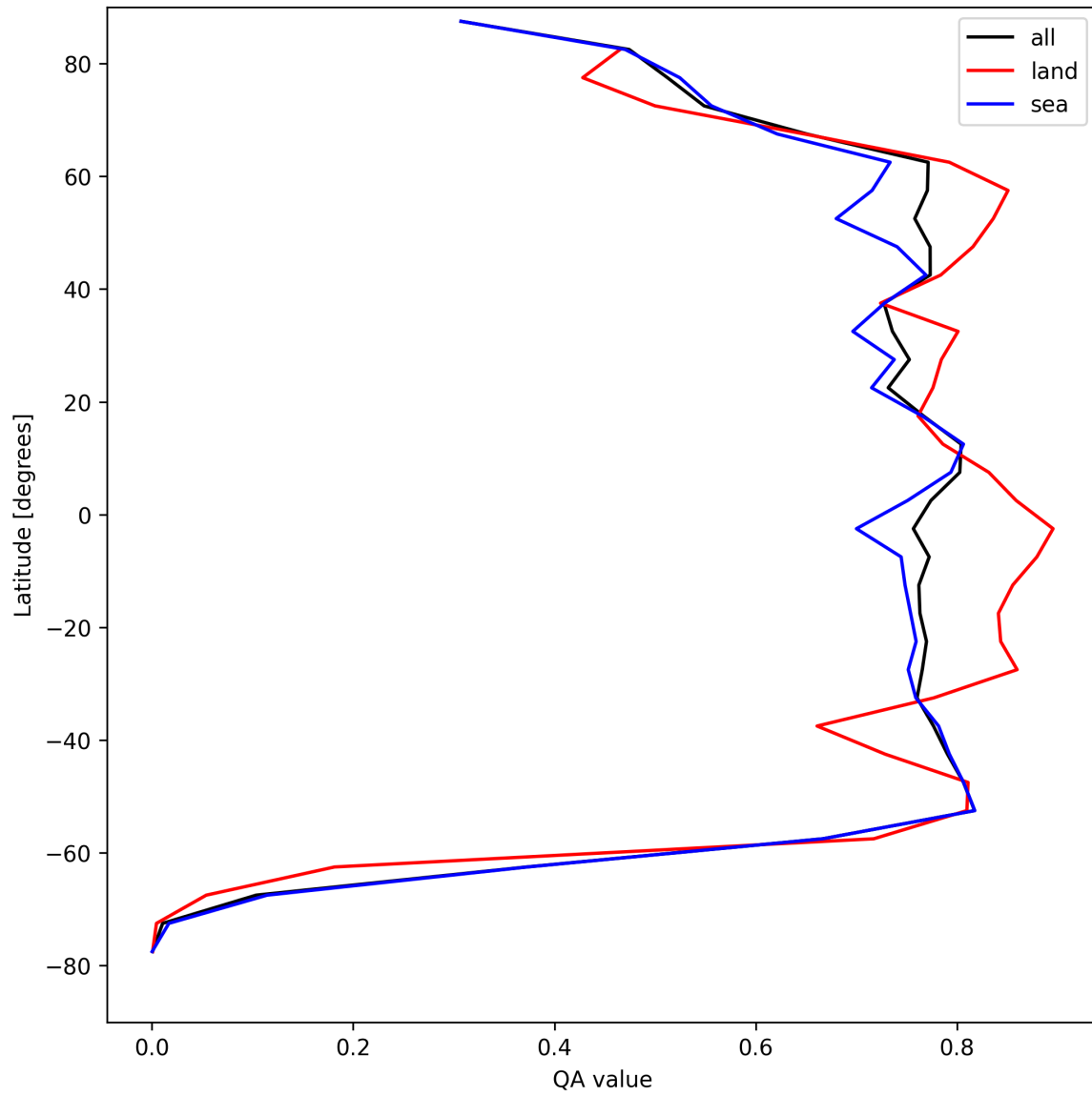
Figure 22: Zonal average of “QA value” for 2025-08-22 to 2025-08-24.
