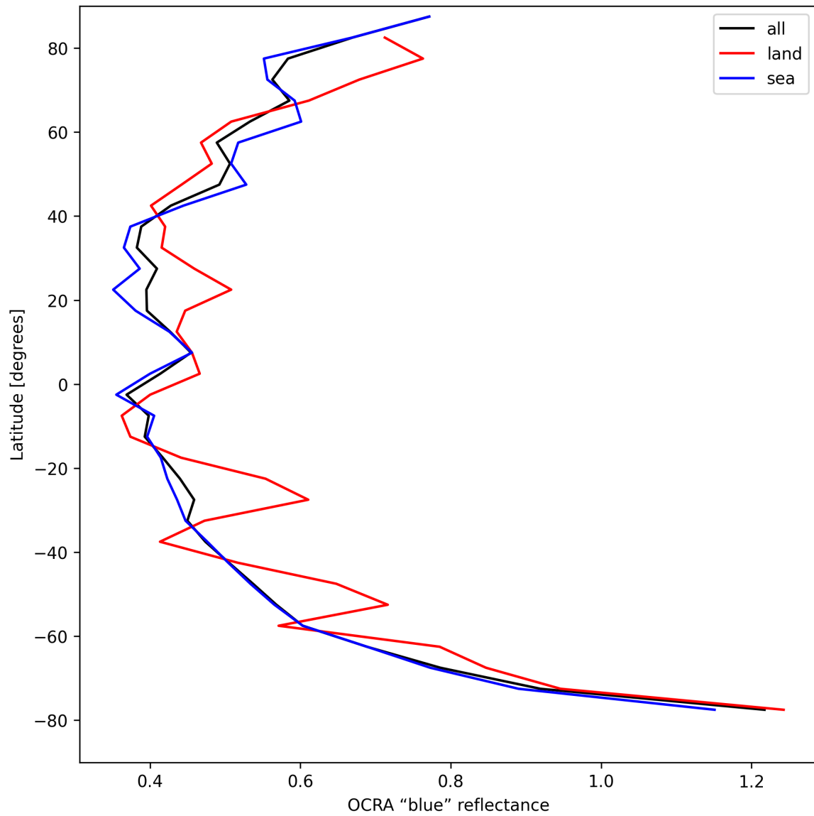
Figure 35: Zonal average of “OCRA “blue” reflectance” for 2025-08-22 to 2025-08-24.
