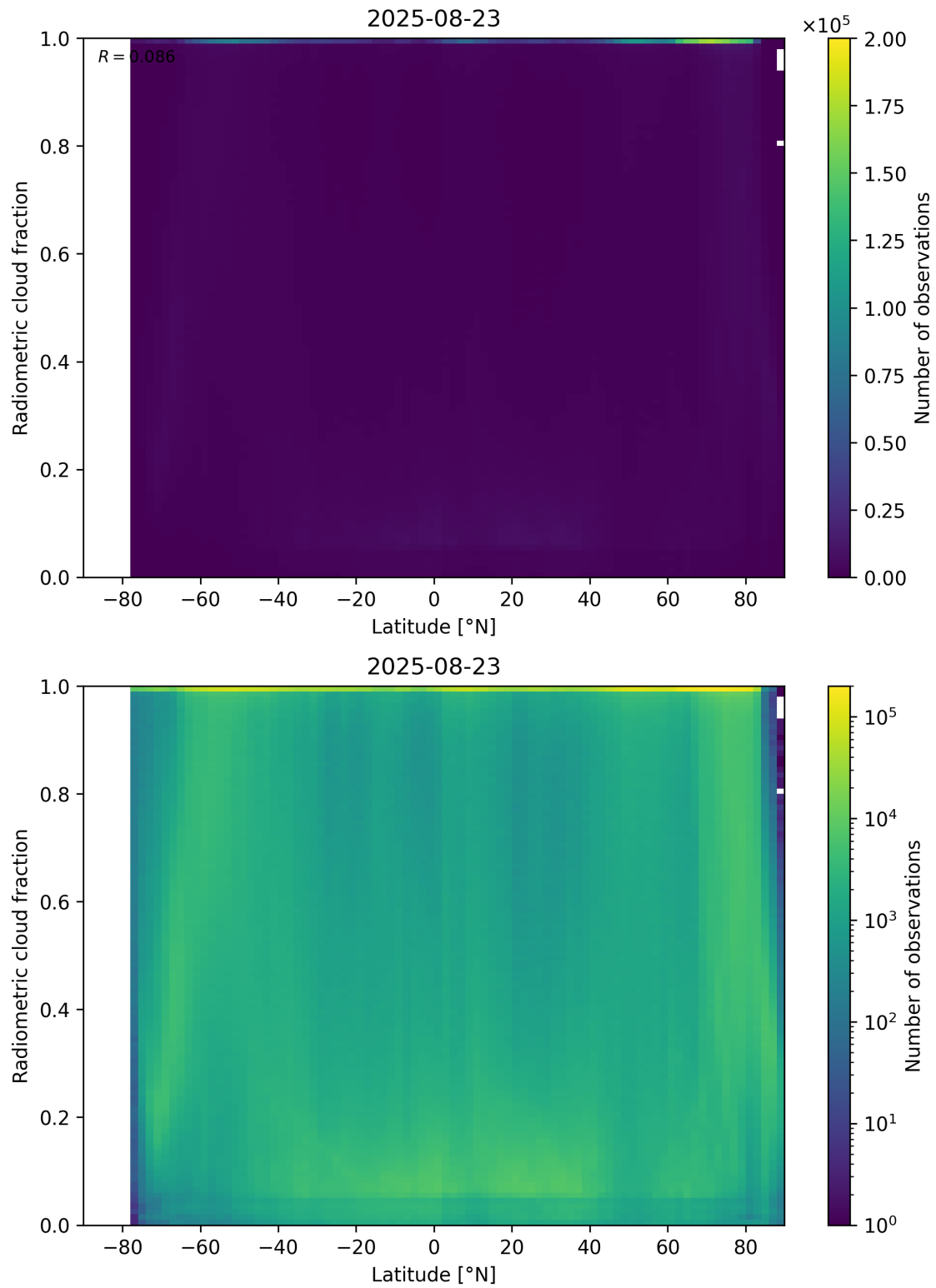
Figure 92: Scatter density plot of “Latitude” against “Radiometric cloud fraction” for 2025-08-22 to 2025-08-24.
