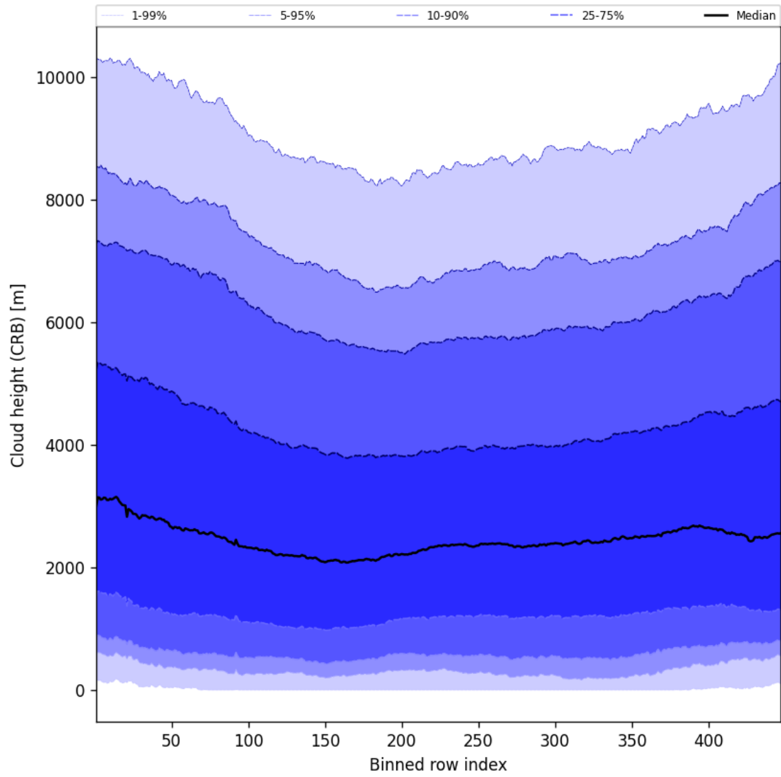
Figure 59: Along track statistics of “Cloud height (CRB)” for 2025-08-22 to 2025-08-24
