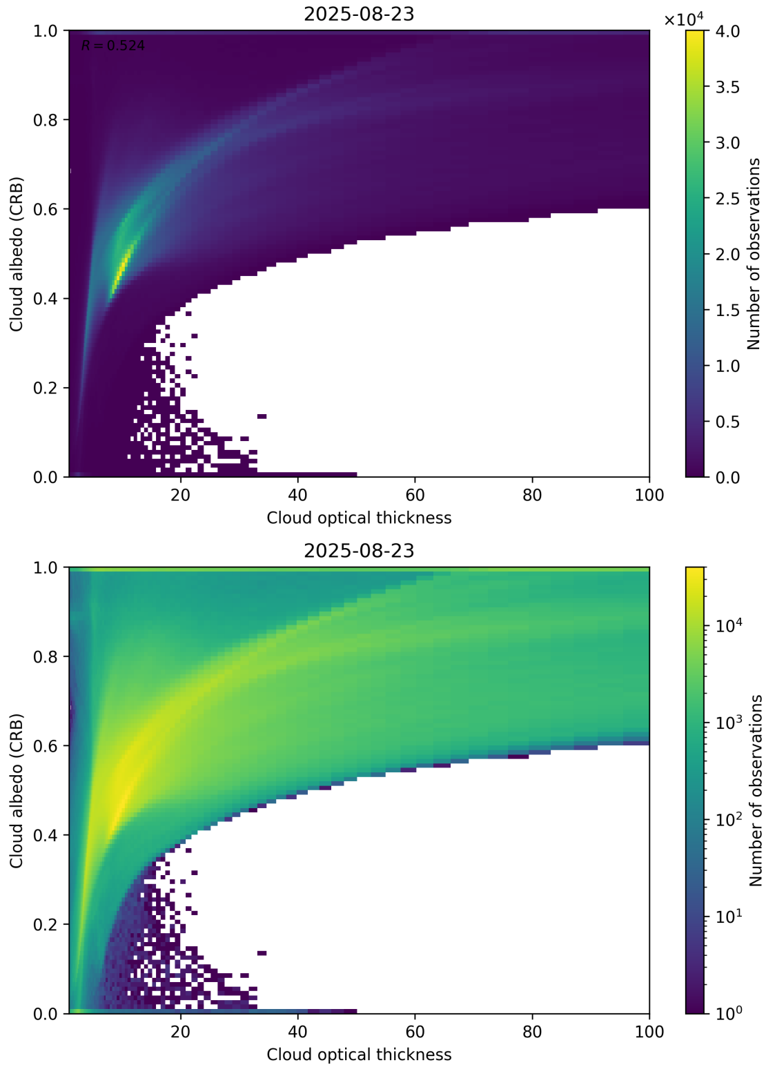
Figure 82: Scatter density plot of “Cloud optical thickness” against “Cloud albedo (CRB)” for 2025-08-22 to 2025-08-24.
