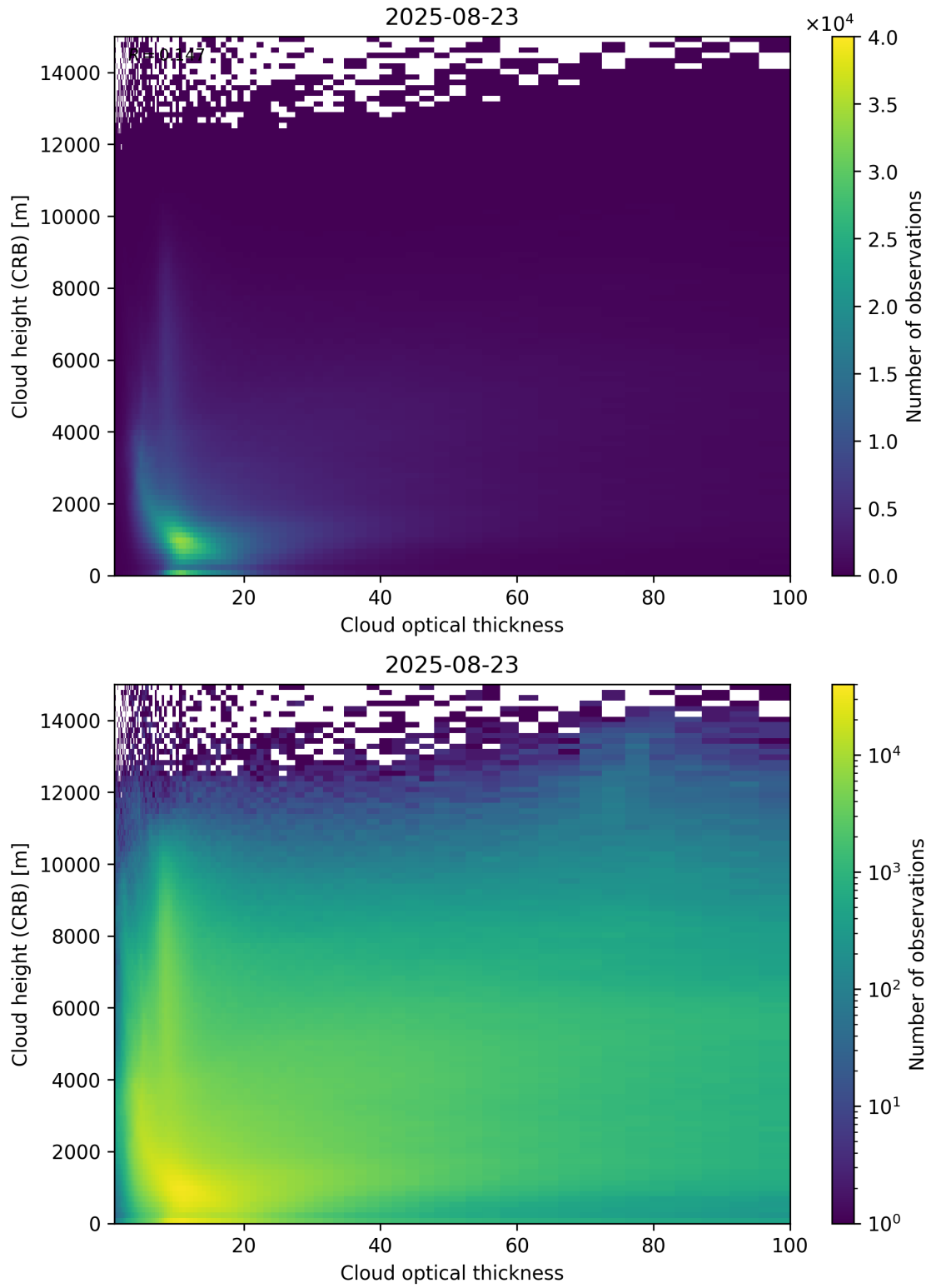
Figure 85: Scatter density plot of “Cloud optical thickness” against “Cloud height (CRB)” for 2025-08-22 to 2025-08-24.
