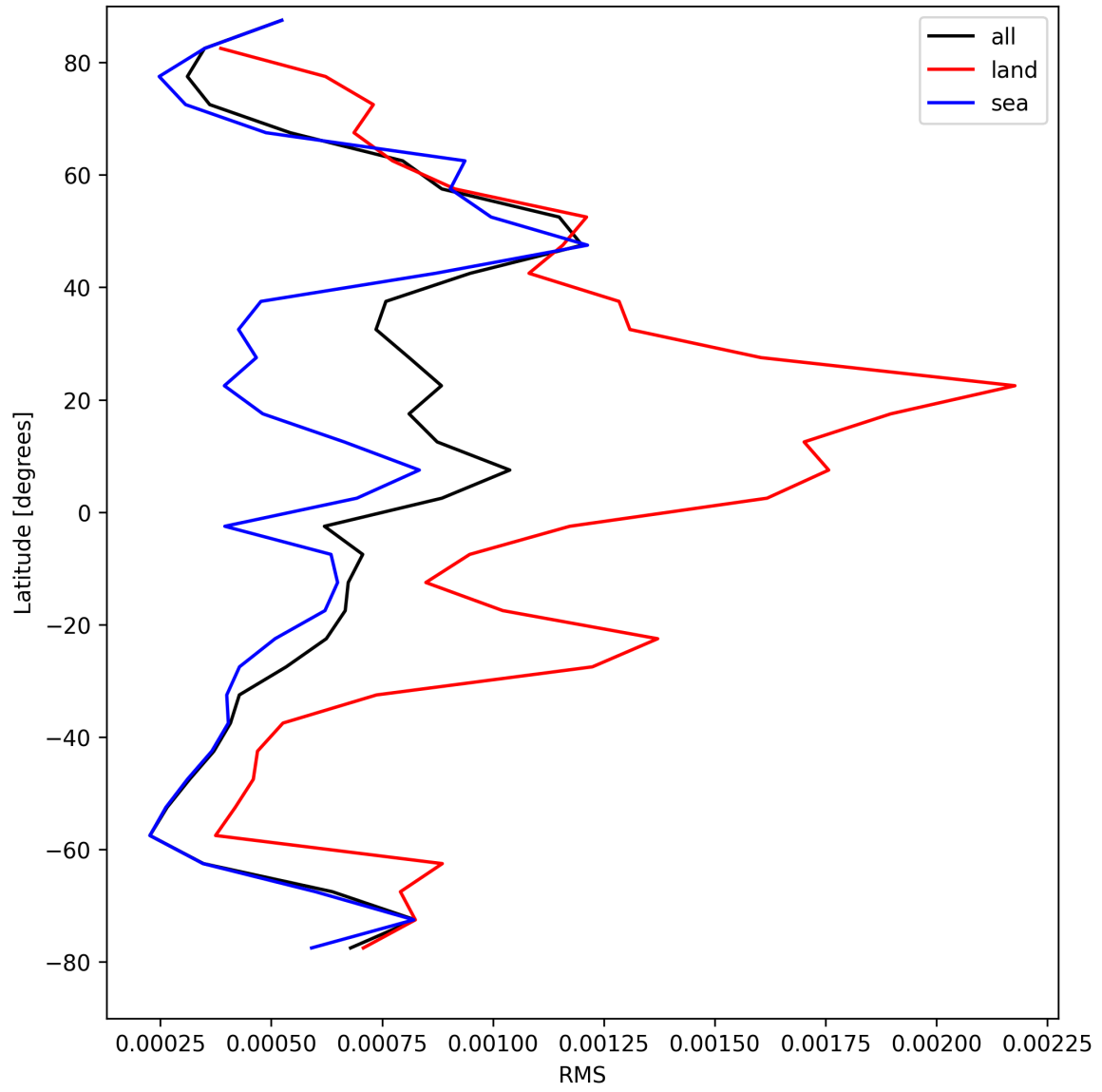
Figure 31: Zonal average of “RMS” for 2025-08-22 to 2025-08-24.
