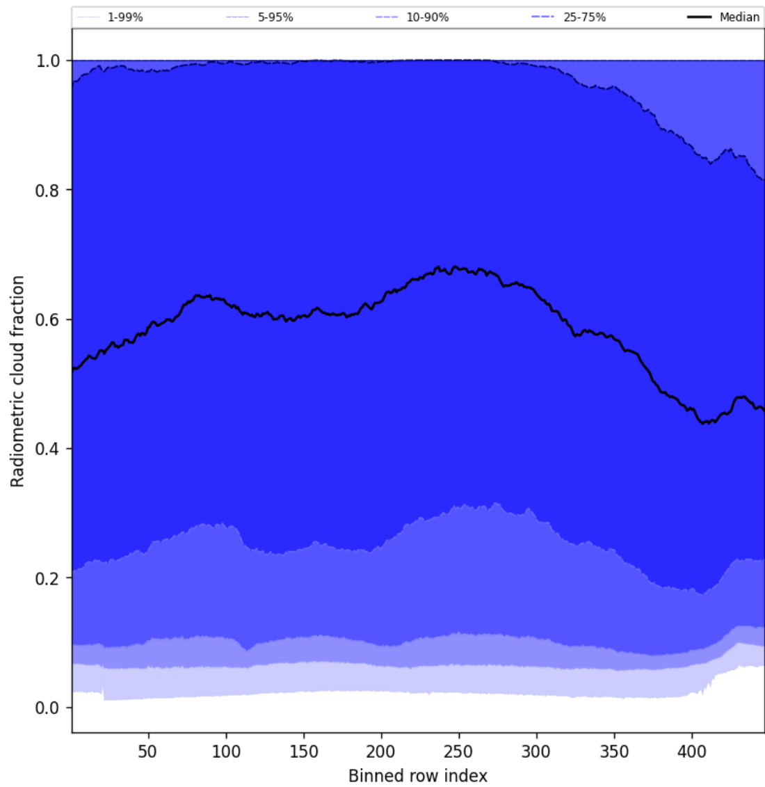
Figure 55: Along track statistics of “Radiometric cloud fraction” for 2025-08-22 to 2025-08-24
