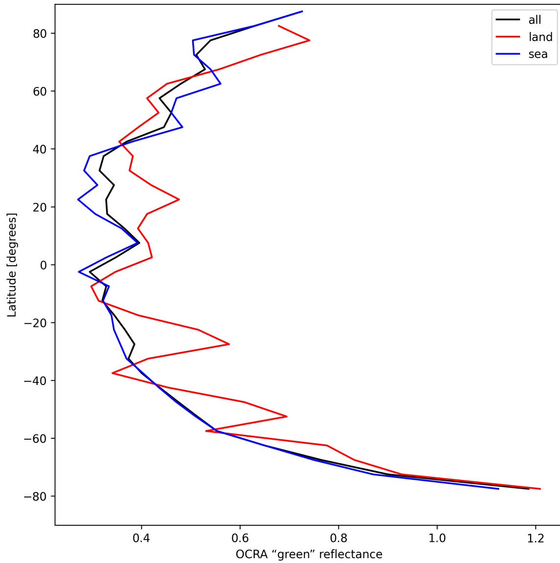
Figure 36: Zonal average of “OCRA “green” reflectance” for 2025-08-22 to 2025-08-24.
