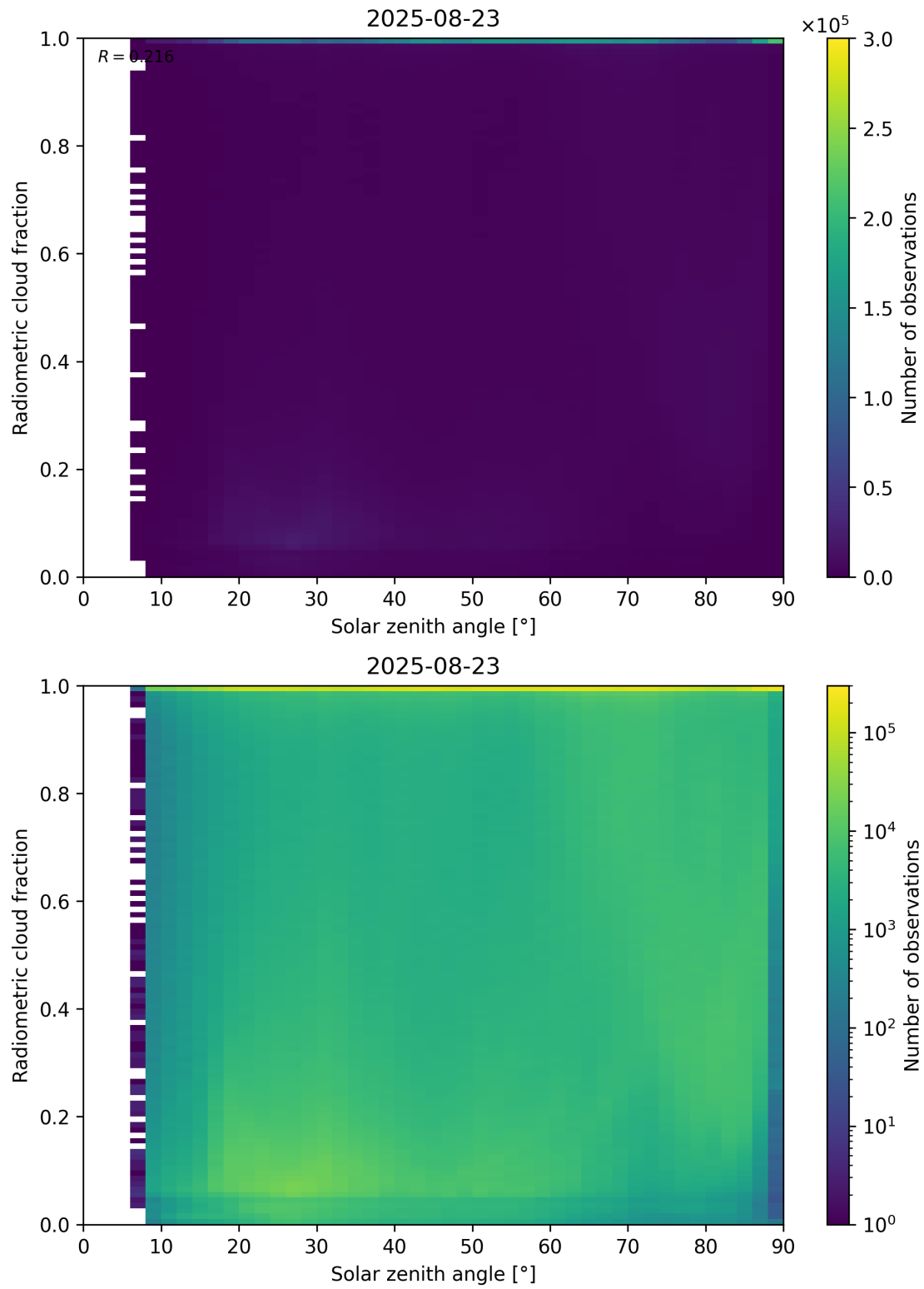
Figure 99: Scatter density plot of “Solar zenith angle” against “Radiometric cloud fraction” for 2025-08-22 to 2025-08-24.
