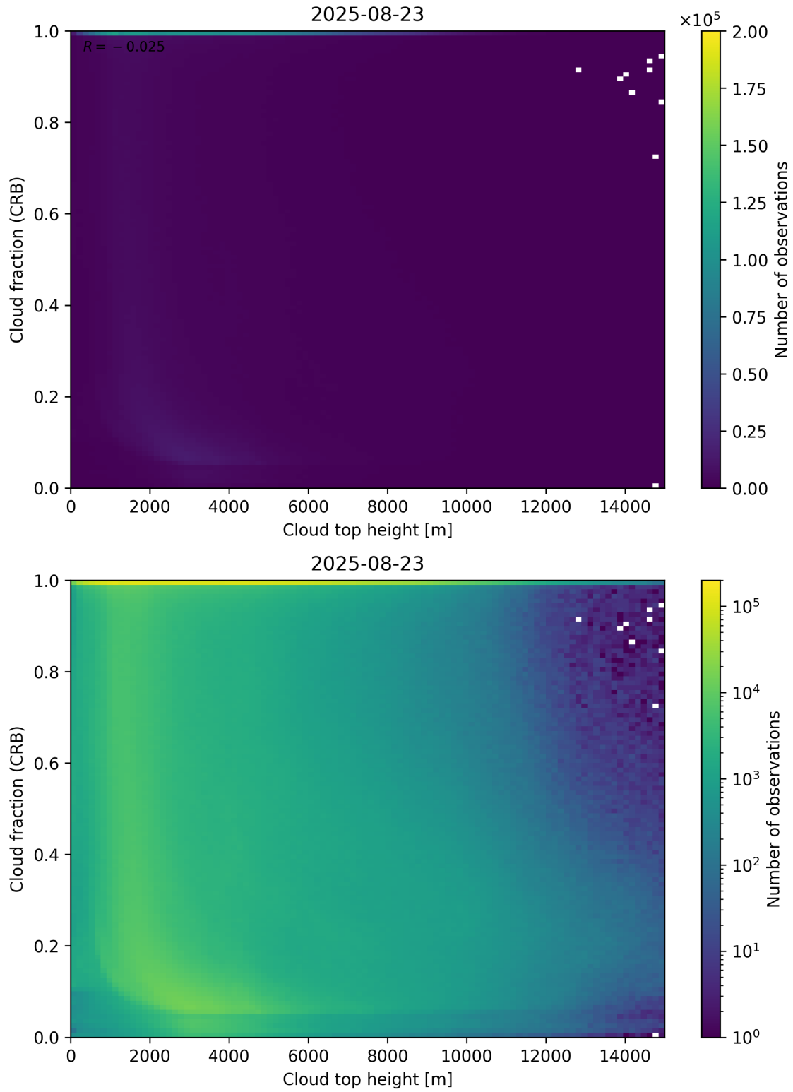
Figure 88: Scatter density plot of “Cloud top height” against “Cloud fraction (CRB)” for 2025-08-22 to 2025-08-24.
