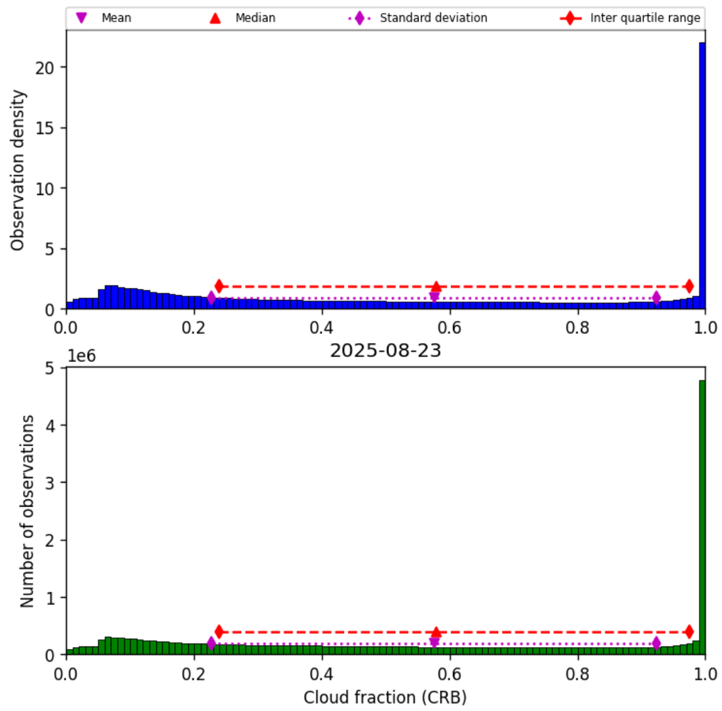
Figure 42: Histogram of “Cloud fraction (CRB)” for 2025-08-22 to 2025-08-24
