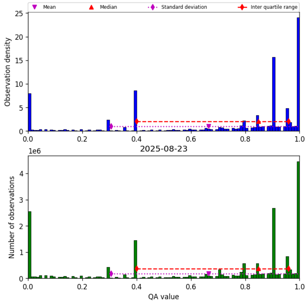
Figure 38: Histogram of “QA value” for 2025-08-22 to 2025-08-24
