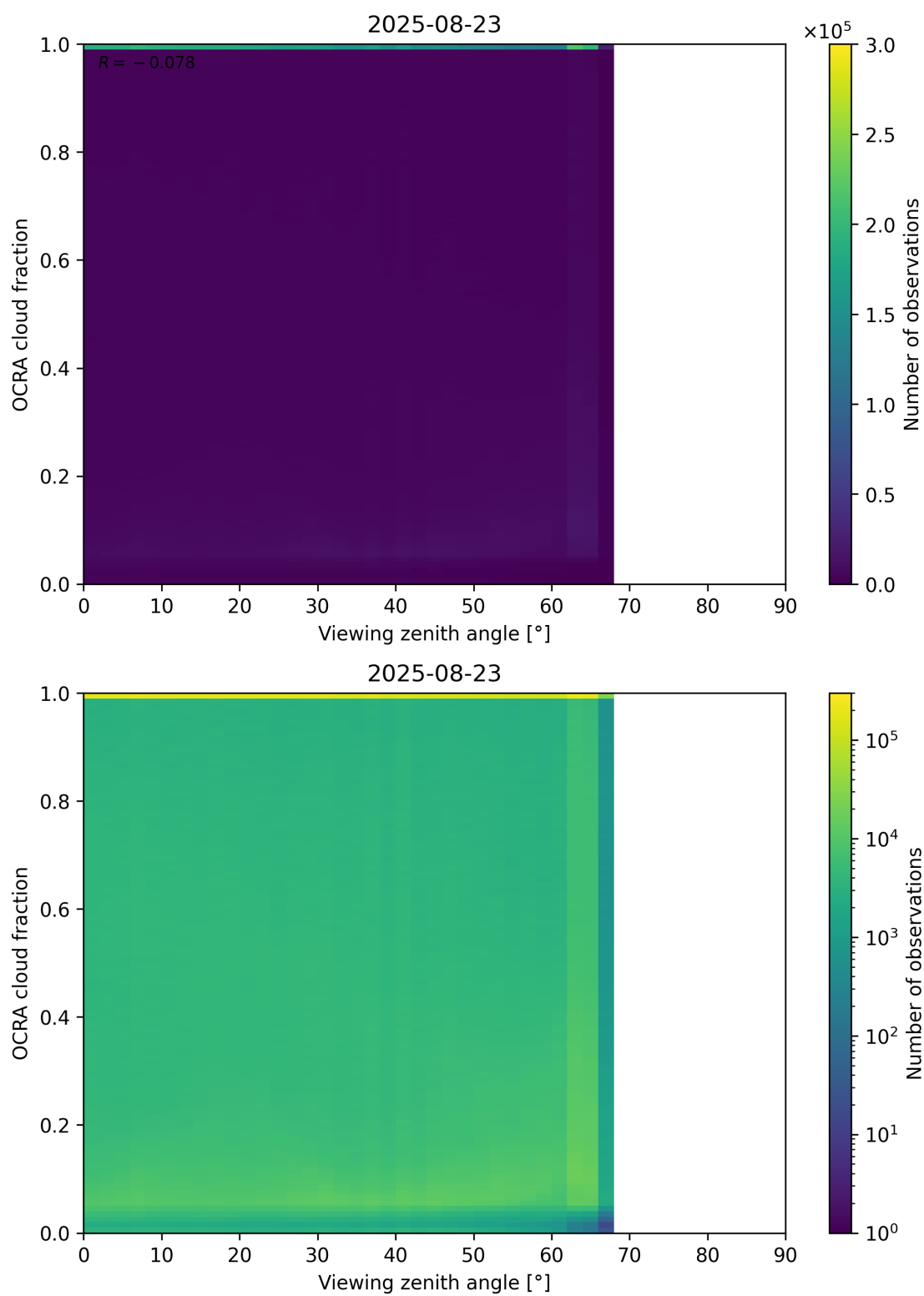
Figure 108: Scatter density plot of “Viewing zenith angle” against “OCRA cloud fraction” for 2025-08-22 to 2025-08-24.
