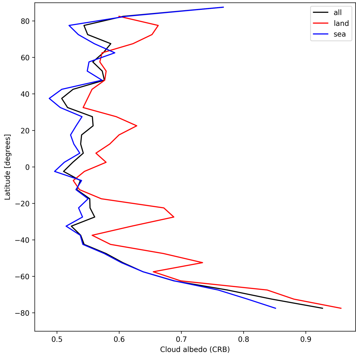
Figure 28: Zonal average of “Cloud albedo (CRB)” for 2025-08-22 to 2025-08-24.
