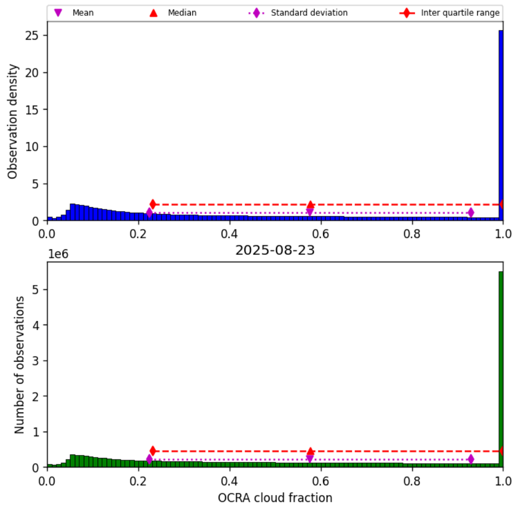
Figure 50: Histogram of “OCRA cloud fraction” for 2025-08-22 to 2025-08-24
