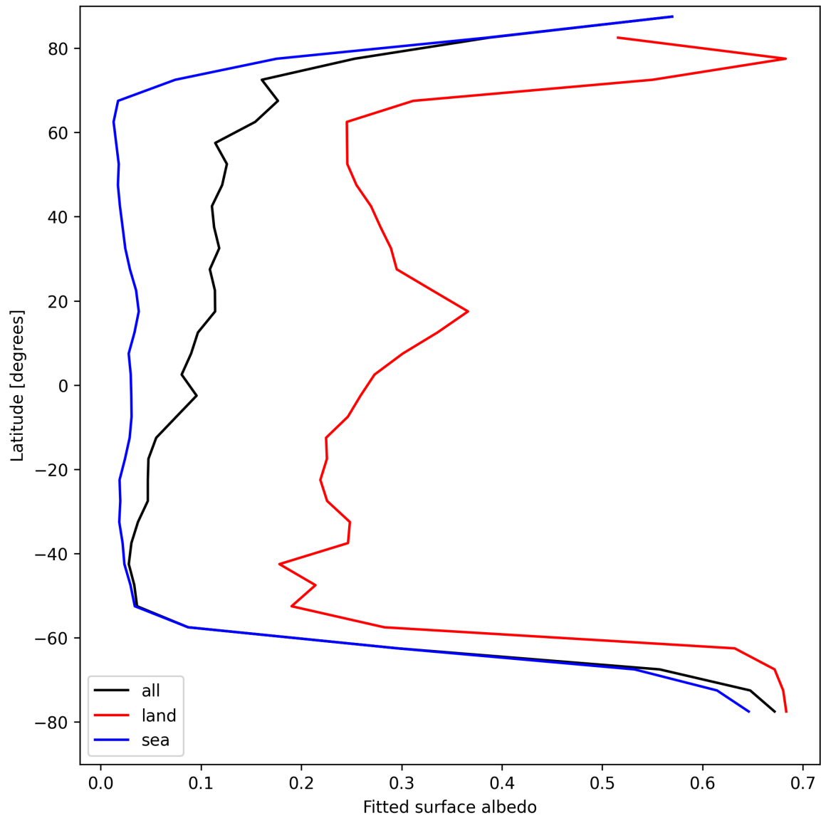
Figure 29: Zonal average of “Fitted surface albedo” for 2025-08-22 to 2025-08-24.
