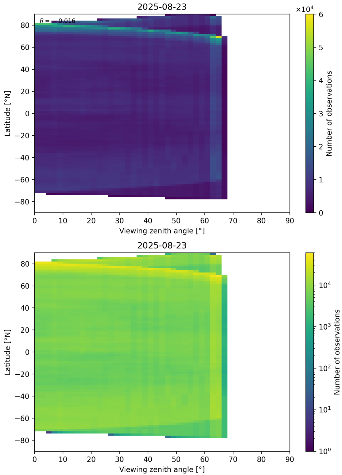
Figure 113: Scatter density plot of “Viewing zenith angle” against “Latitude” for 2025-08-22 to 2025-08-24.
