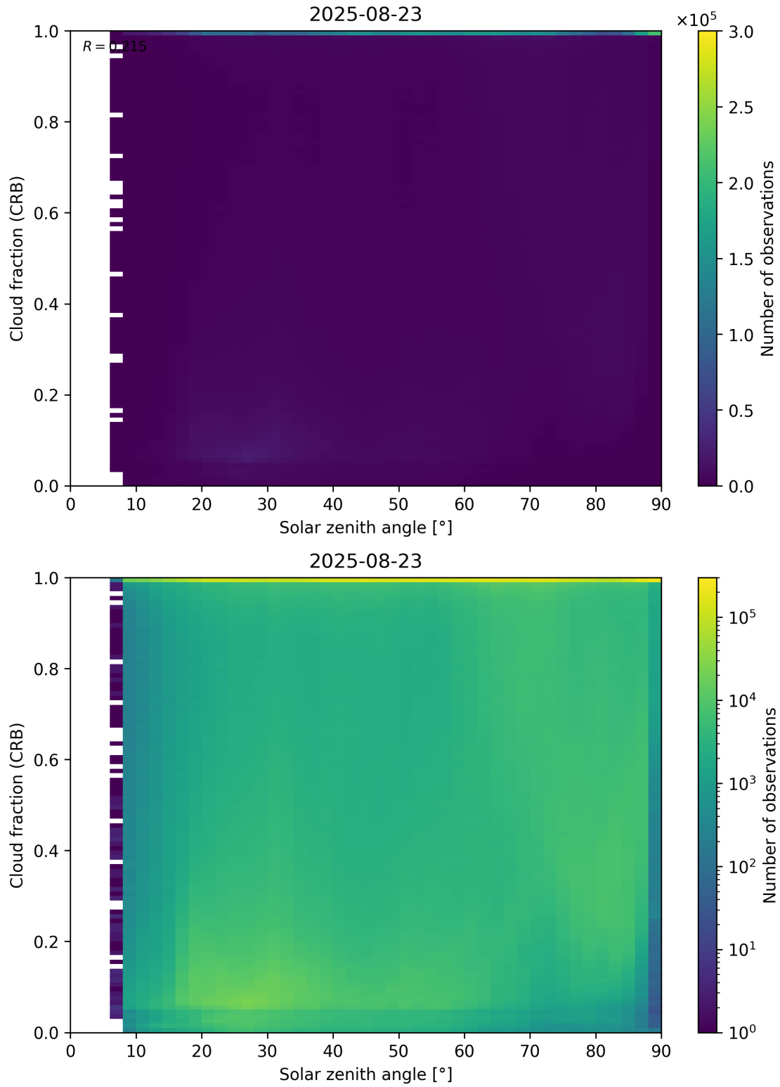
Figure 101: Scatter density plot of “Solar zenith angle” against “Cloud fraction (CRB)” for 2025-08-22 to 2025-08-24.
