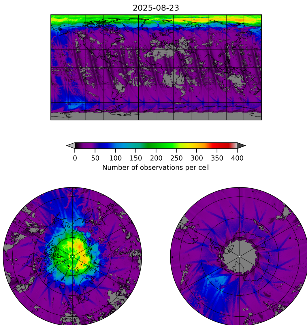
Figure 21: Map of the number of observations for 2025-08-22 to 2025-08-24
