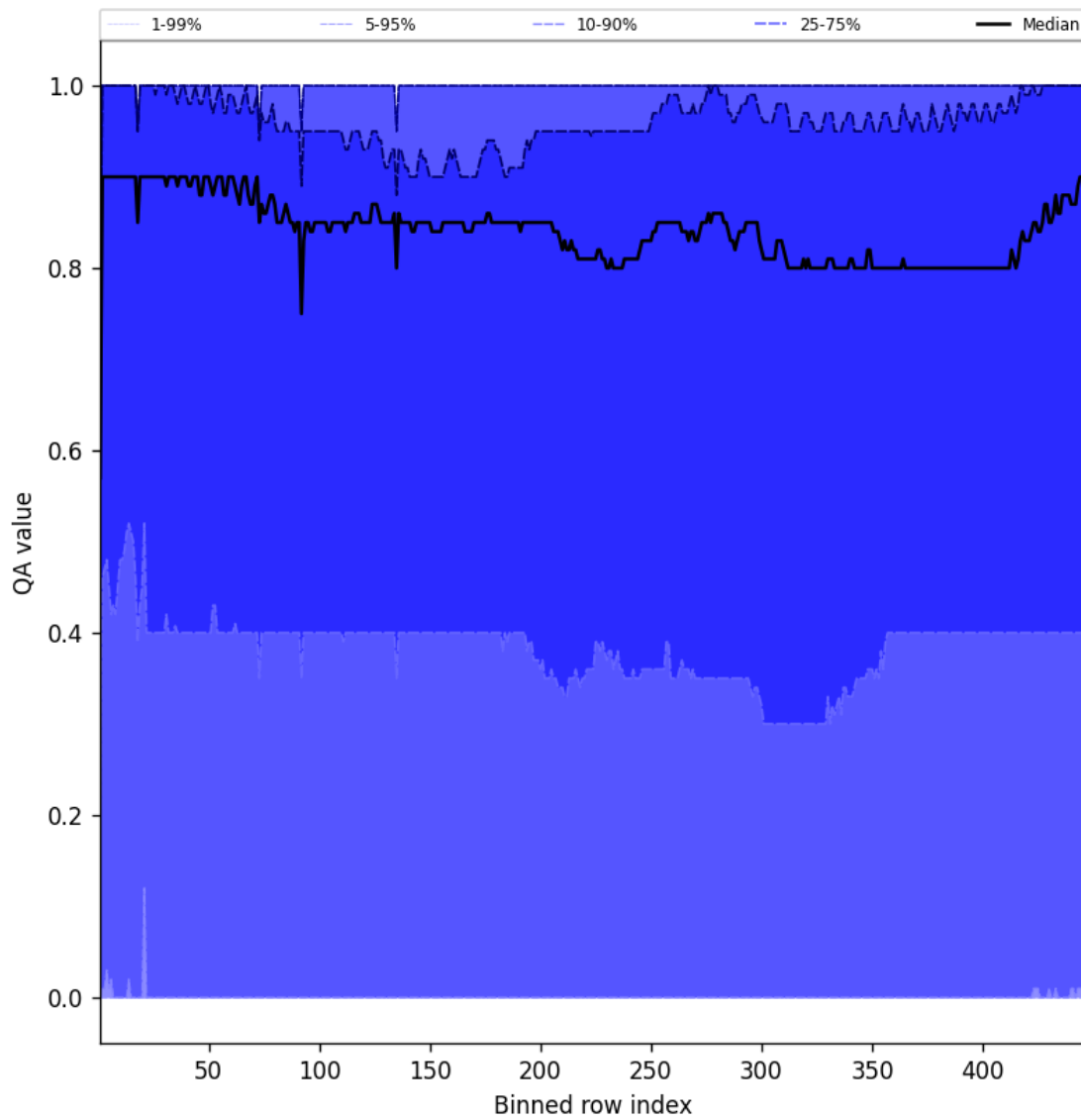
Figure 54: Along track statistics of “QA value” for 2025-08-22 to 2025-08-24
