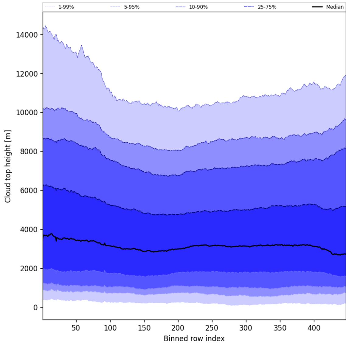
Figure 56: Along track statistics of “Cloud top height” for 2025-08-22 to 2025-08-24
