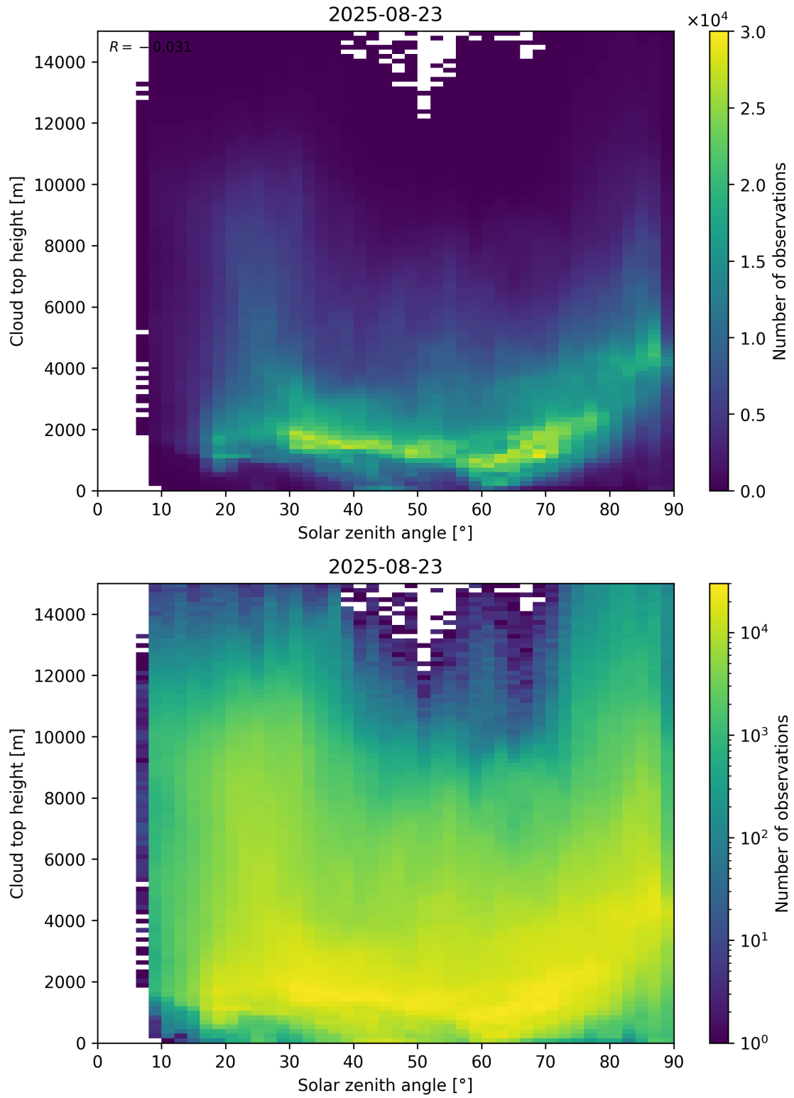
Figure 104: Scatter density plot of “Solar zenith angle” against “Cloud top height” for 2025-08-22 to 2025-08-24.
