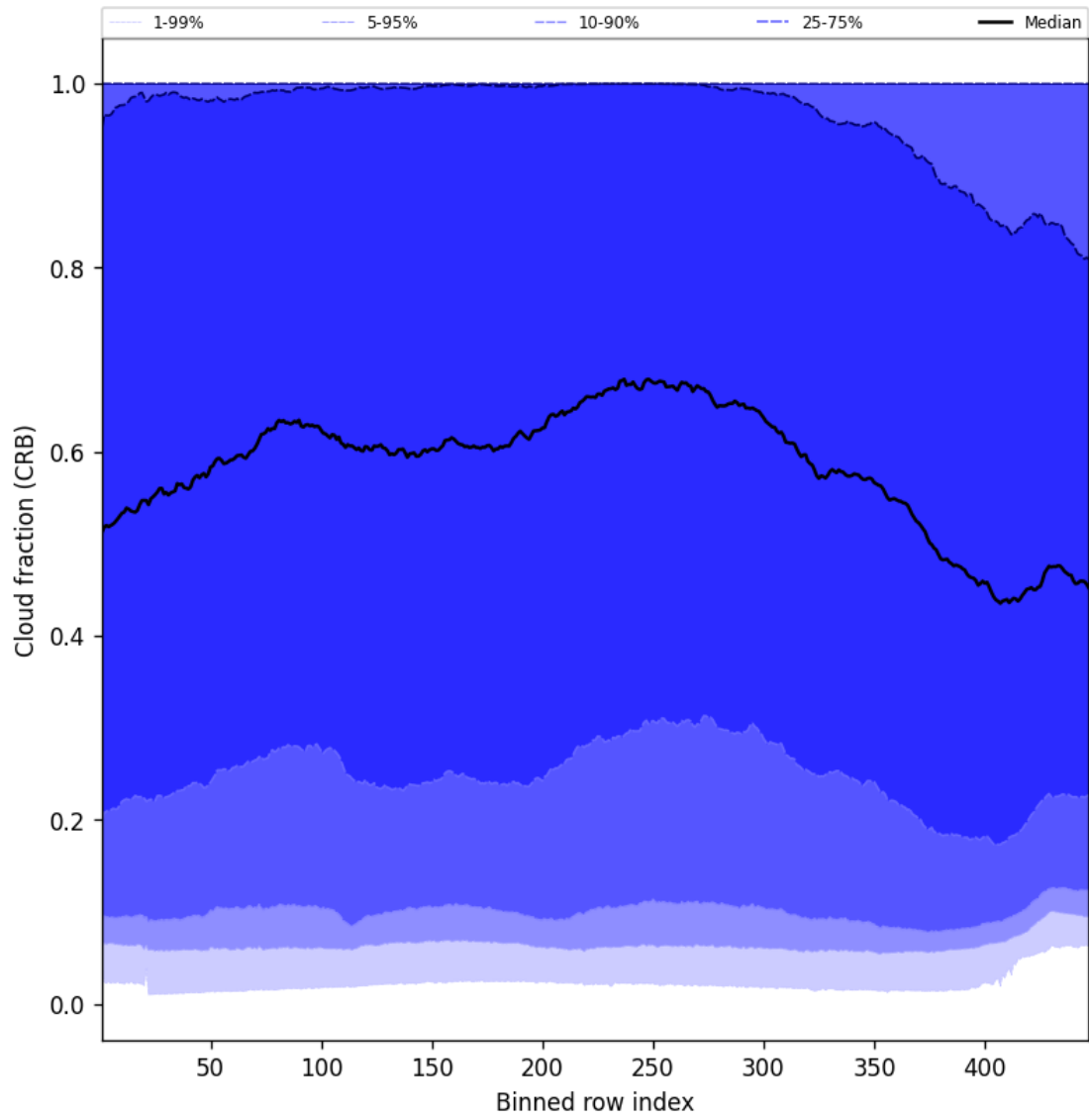
Figure 58: Along track statistics of “Cloud fraction (CRB)” for 2025-08-22 to 2025-08-24
