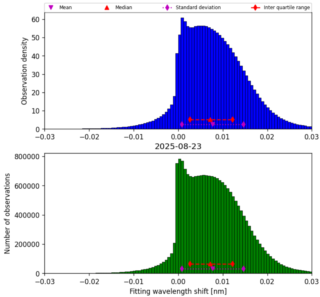
Figure 49: Histogram of “Fitting wavelength shift” for 2025-08-22 to 2025-08-24
