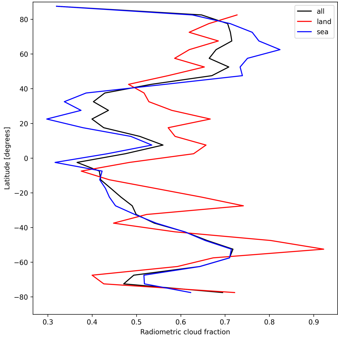
Figure 23: Zonal average of “Radiometric cloud fraction” for 2025-08-22 to 2025-08-24.
