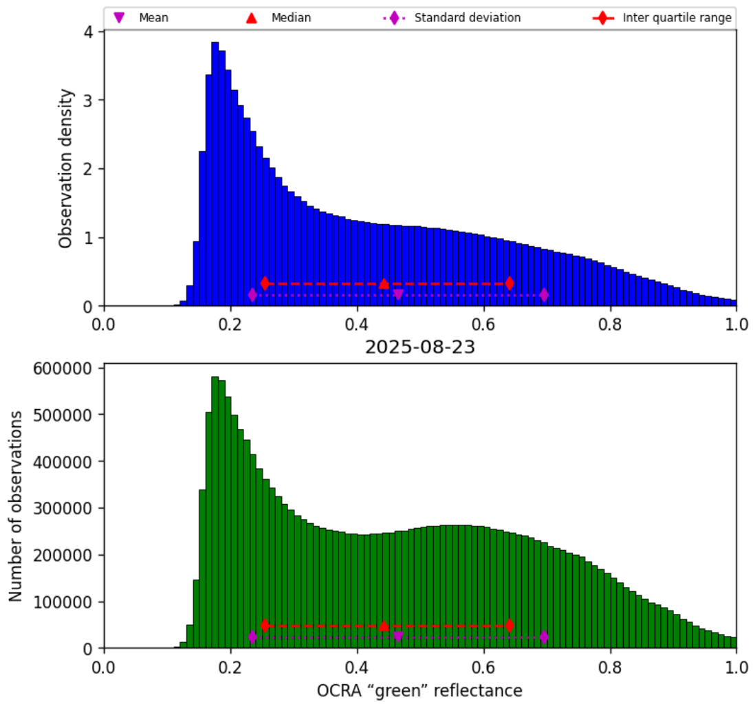
Figure 52: Histogram of “OCRA “green” reflectance” for 2025-08-22 to 2025-08-24
