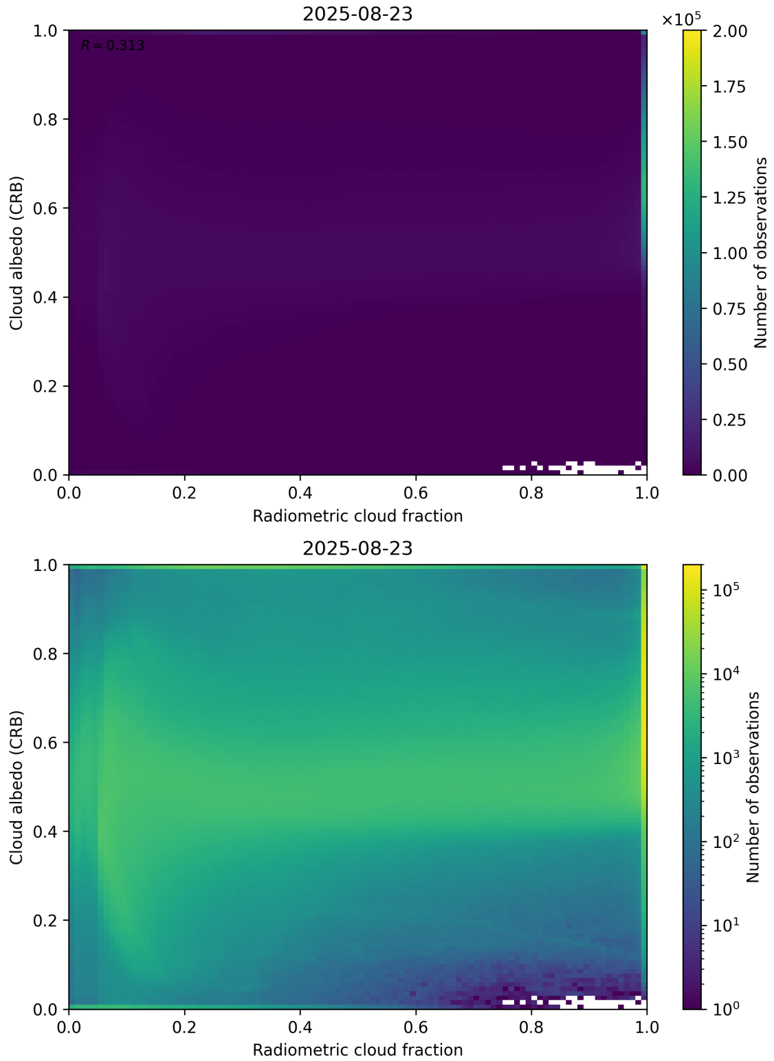
Figure 71: Scatter density plot of “Radiometric cloud fraction” against “Cloud albedo (CRB)” for 2025-08-22 to 2025-08-24.
