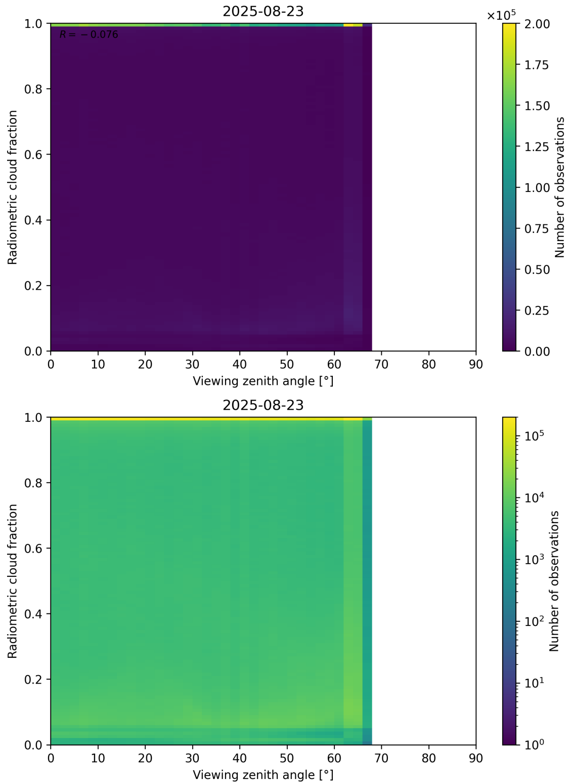
Figure 107: Scatter density plot of “Viewing zenith angle” against “Radiometric cloud fraction” for 2025-08-22 to 2025-08-24.
