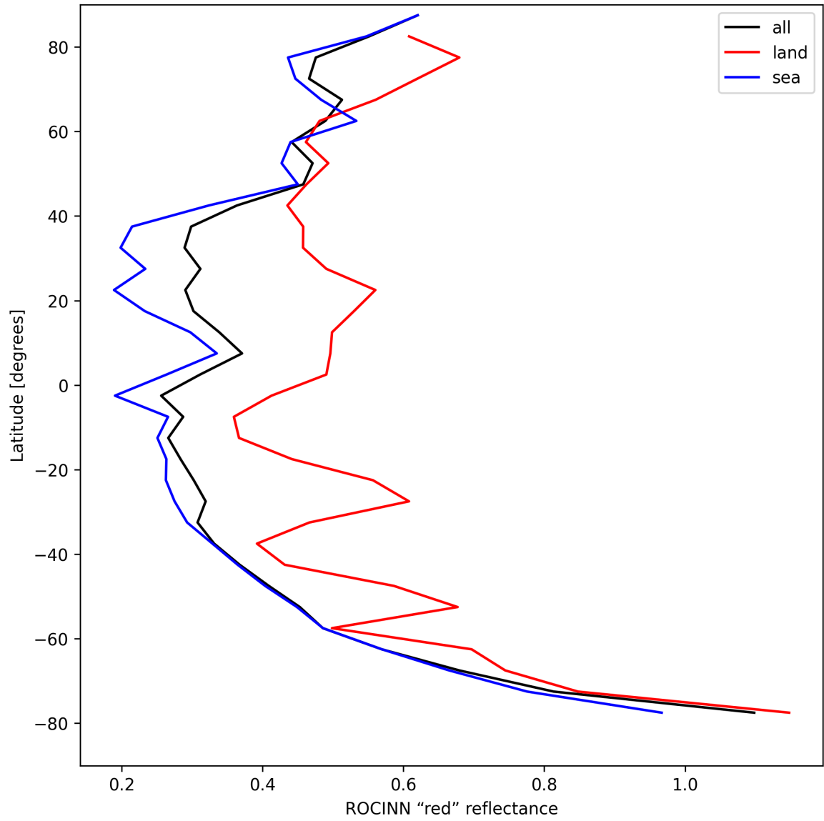
Figure 37: Zonal average of “ROCINN “red” reflectance” for 2025-08-22 to 2025-08-24.
