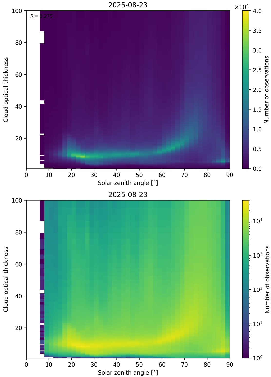
Figure 103: Scatter density plot of “Solar zenith angle” against “Cloud optical thickness” for 2025-08-22 to 2025-08-24.
