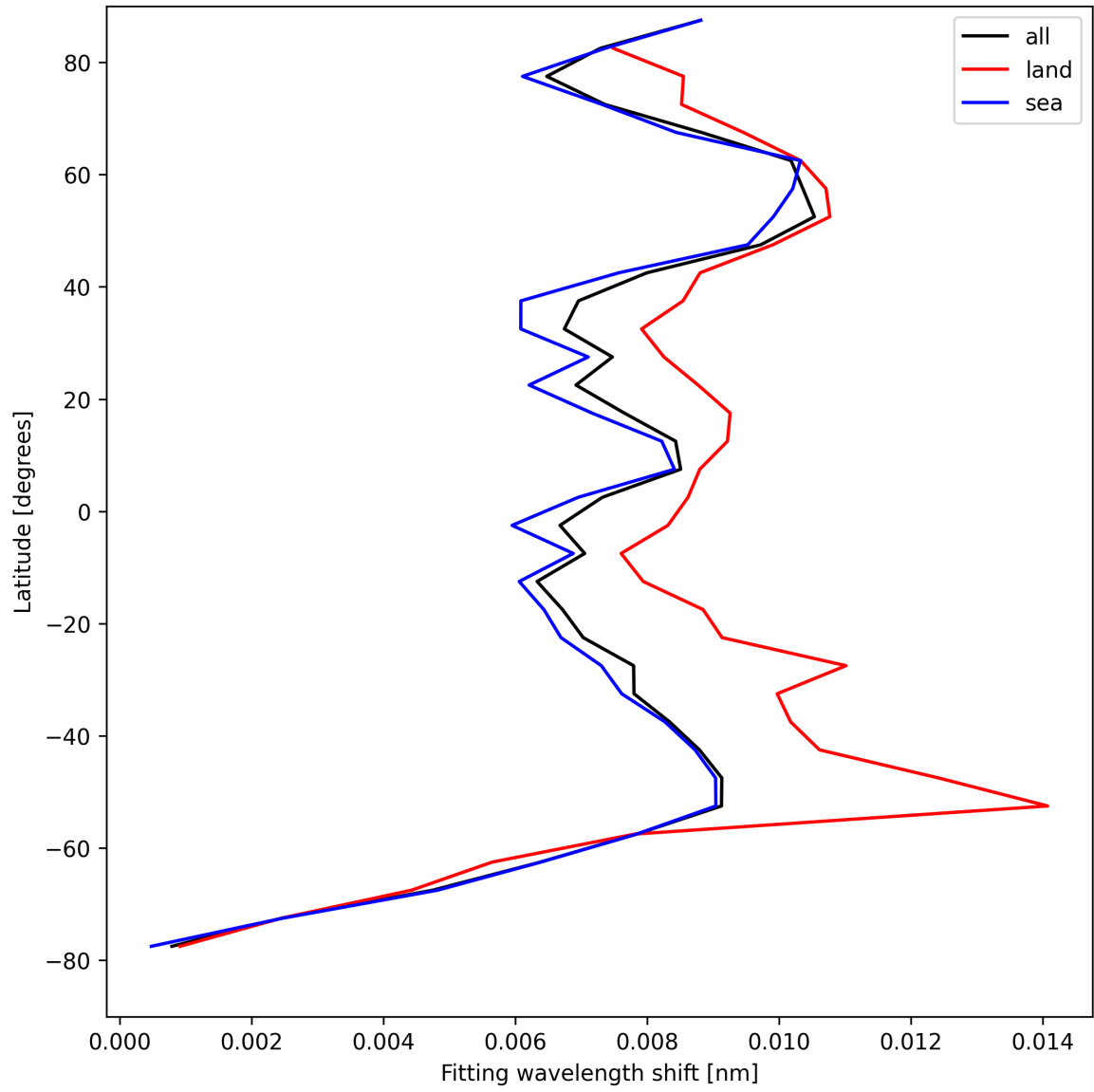
Figure 33: Zonal average of “Fitting wavelength shift” for 2025-08-22 to 2025-08-24.
