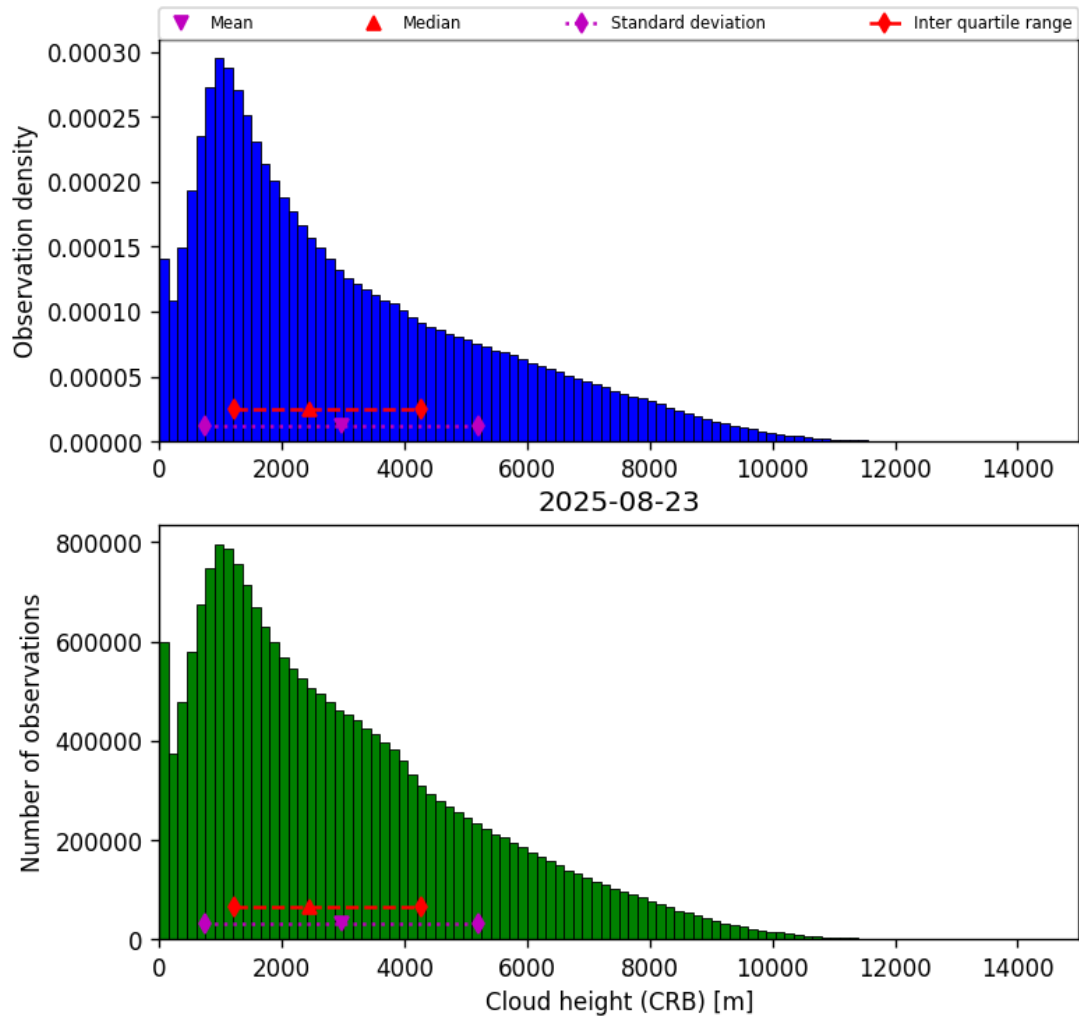
Figure 43: Histogram of “Cloud height (CRB)” for 2025-08-22 to 2025-08-24
