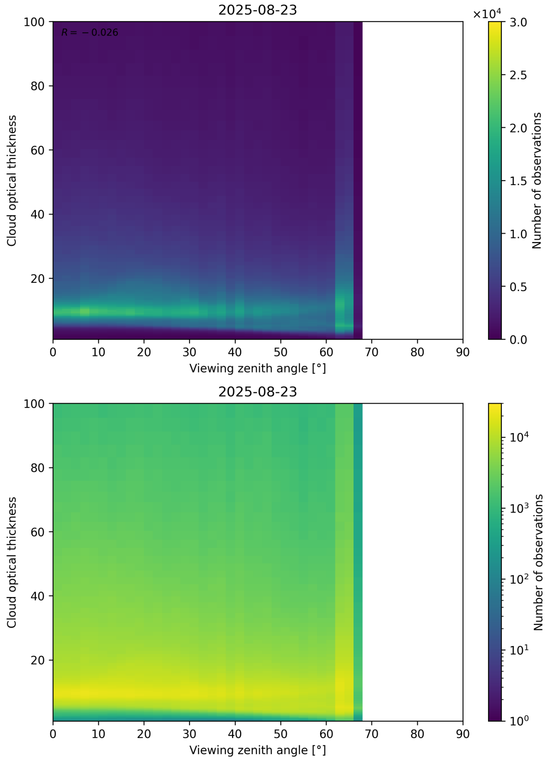
Figure 111: Scatter density plot of “Viewing zenith angle” against “Cloud optical thickness” for 2025-08-22 to 2025-08-24.
