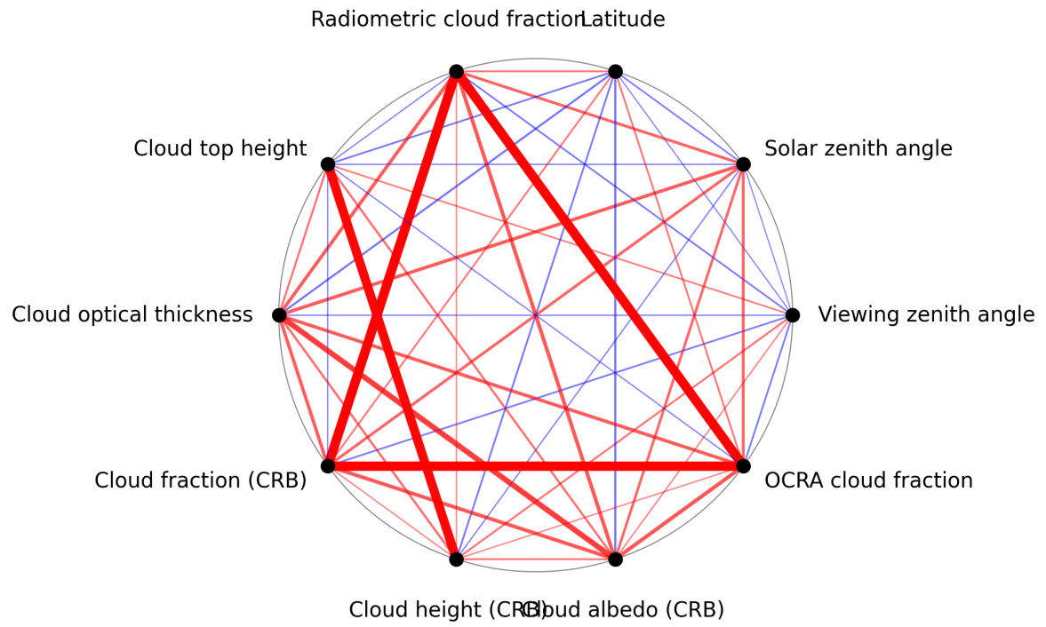
Figure 1: Map of correlation graph for 2025-08-22 to 2025-08-24.
