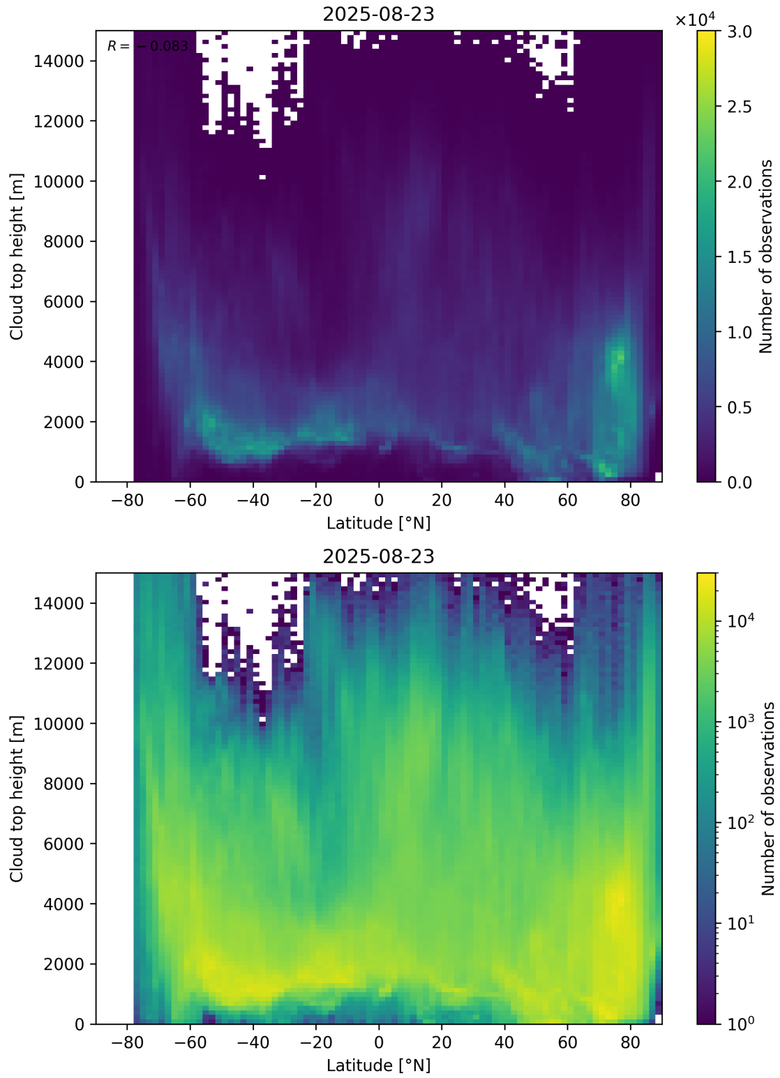
Figure 97: Scatter density plot of “Latitude” against “Cloud top height” for 2025-08-22 to 2025-08-24.
