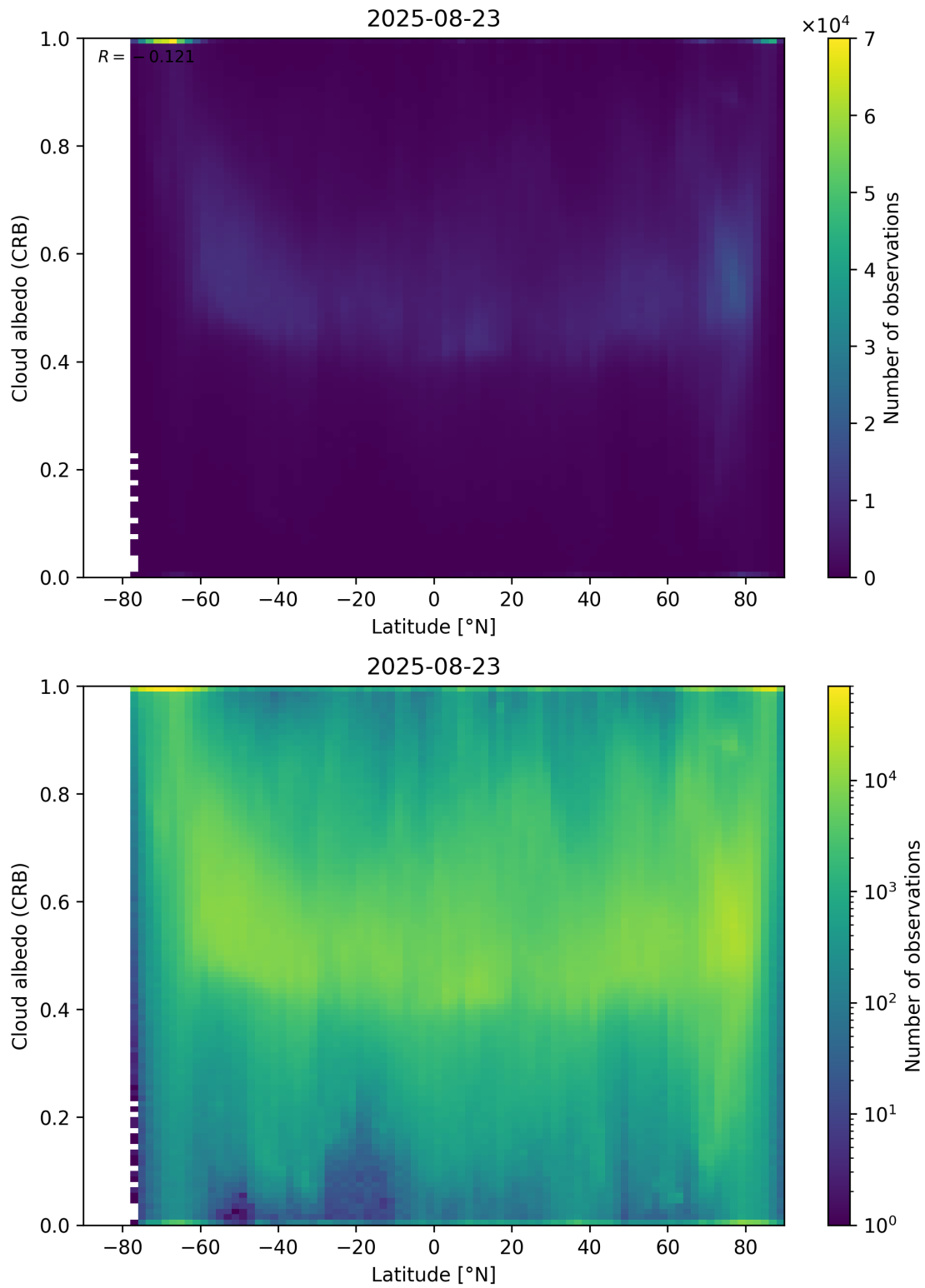
Figure 91: Scatter density plot of “Latitude” against “Cloud albedo (CRB)” for 2025-08-22 to 2025-08-24.
