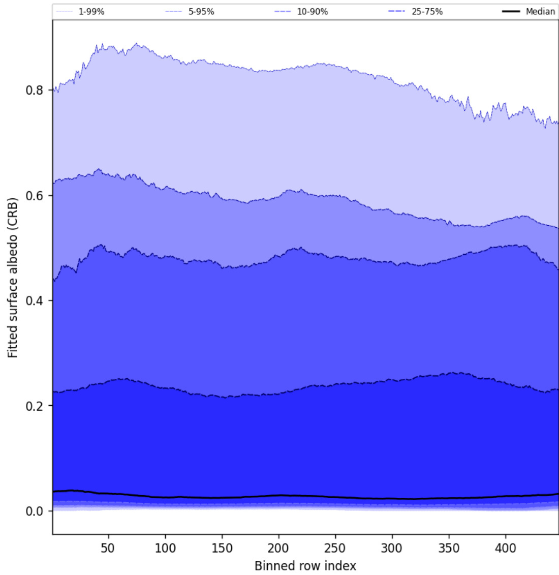
Figure 62: Along track statistics of “Fitted surface albedo (CRB)” for 2025-08-22 to 2025-08-24
