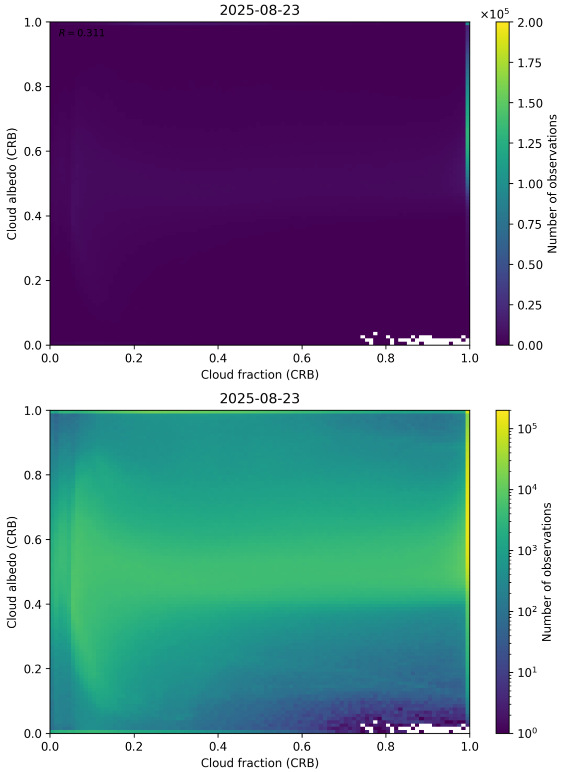
Figure 77: Scatter density plot of “Cloud fraction (CRB)” against “Cloud albedo (CRB)” for 2025-08-22 to 2025-08-24.
