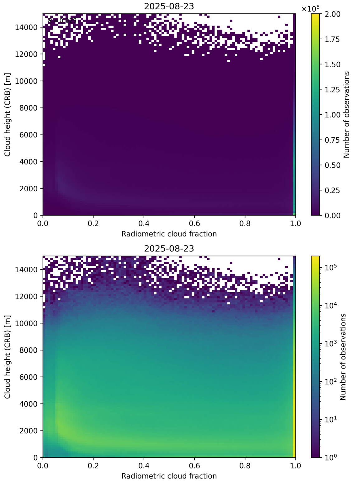
Figure 74: Scatter density plot of “Radiometric cloud fraction” against “Cloud height (CRB)” for 2025-08-22 to 2025-08-24.
