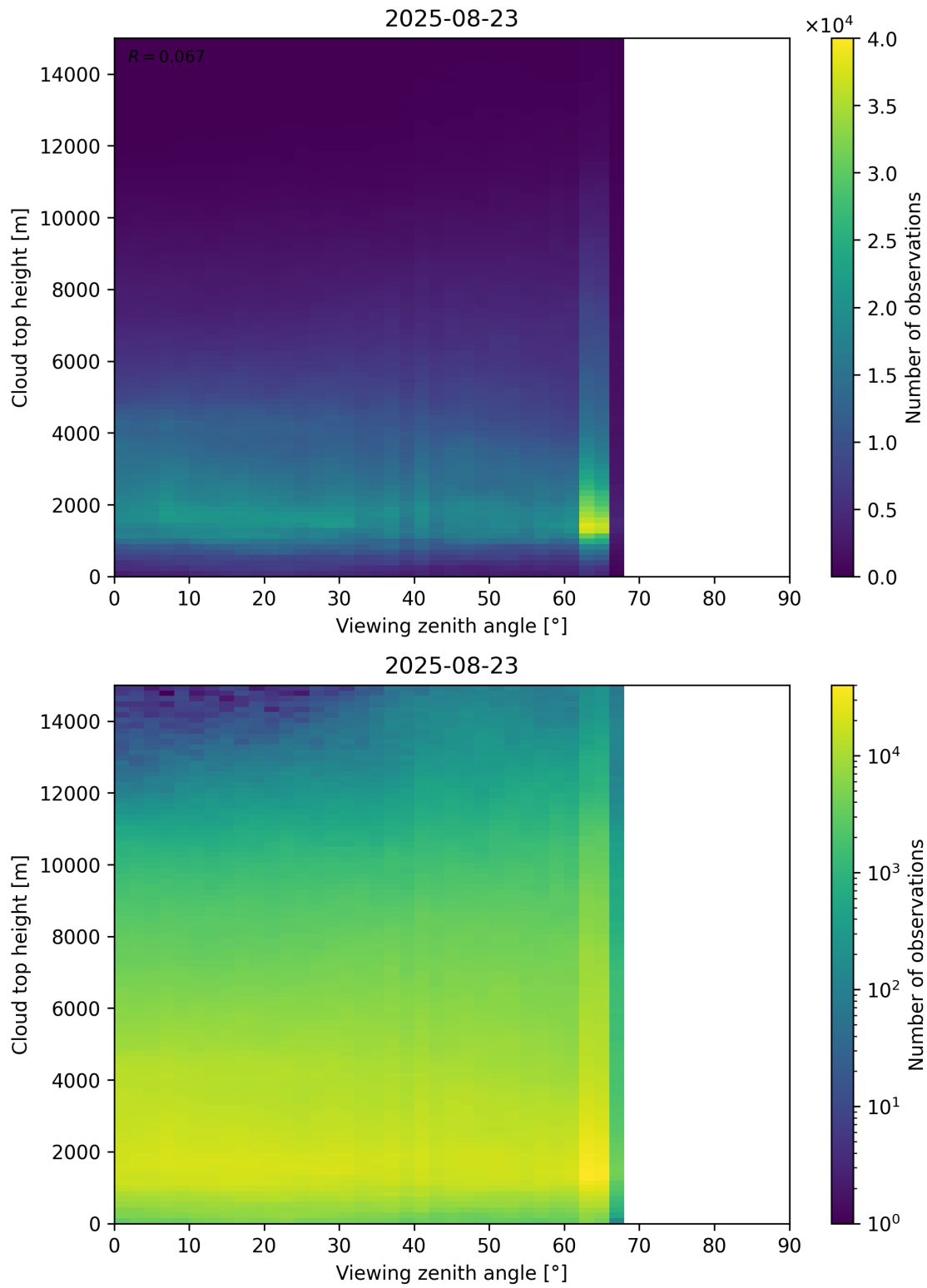
Figure 112: Scatter density plot of “Viewing zenith angle” against “Cloud top height” for 2025-08-22 to 2025-08-24.
