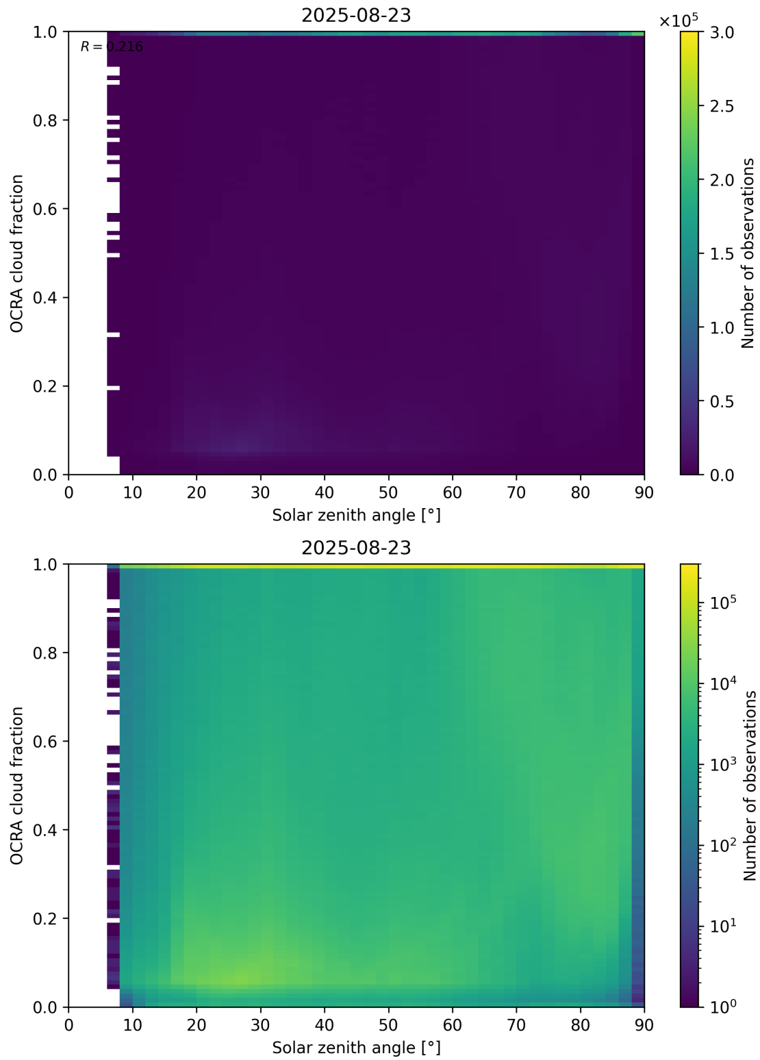
Figure 100: Scatter density plot of “Solar zenith angle” against “OCRA cloud fraction” for 2025-08-22 to 2025-08-24.
