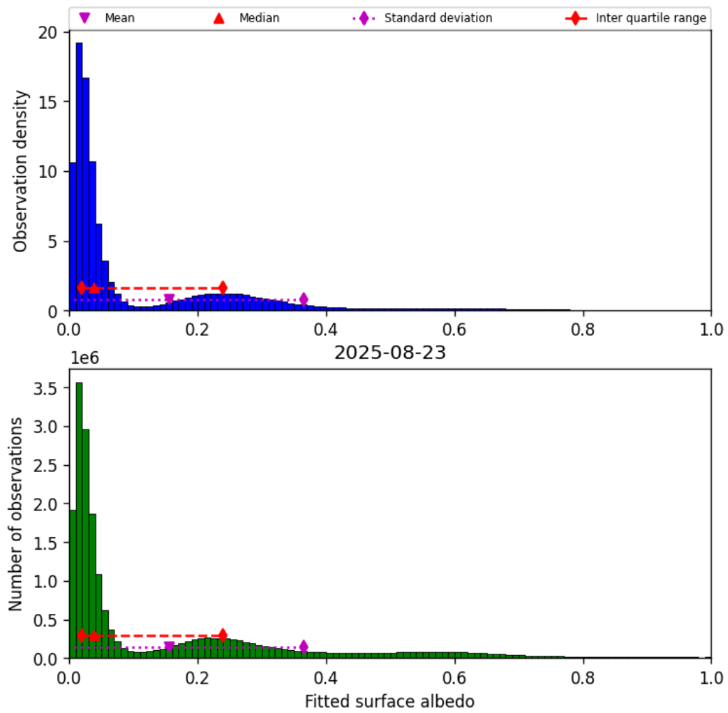
Figure 45: Histogram of “Fitted surface albedo” for 2025-08-22 to 2025-08-24
