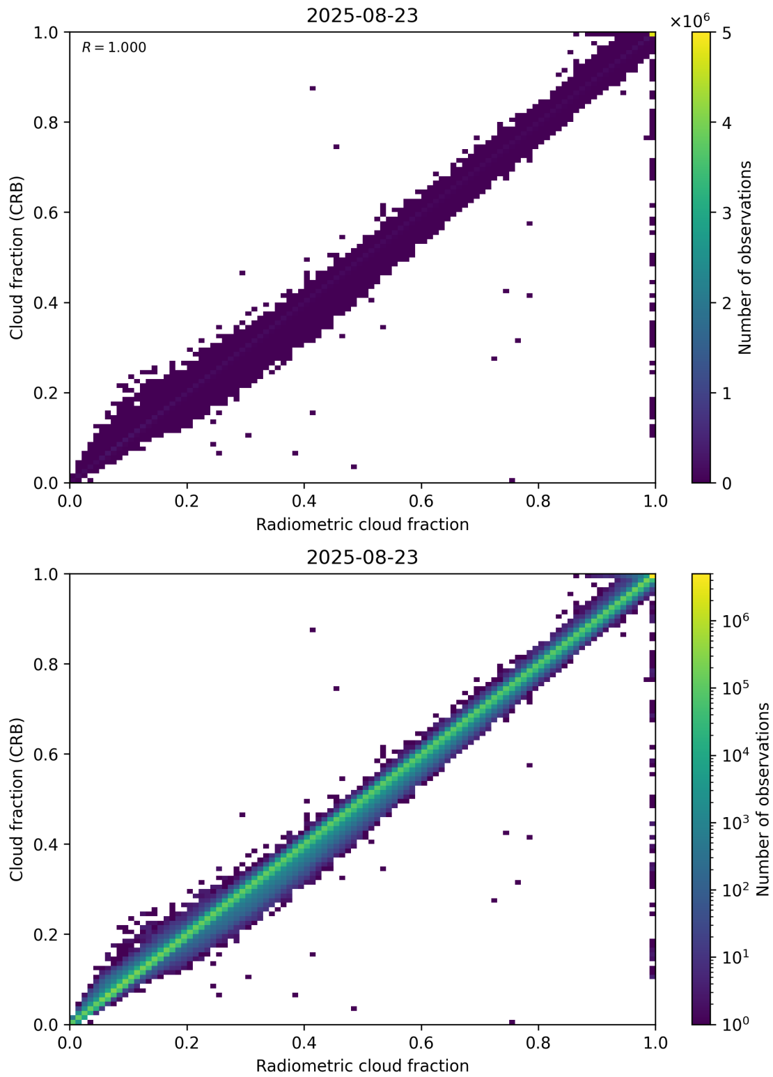
Figure 73: Scatter density plot of “Radiometric cloud fraction” against “Cloud fraction (CRB)” for 2025-08-22 to 2025-08-24.
