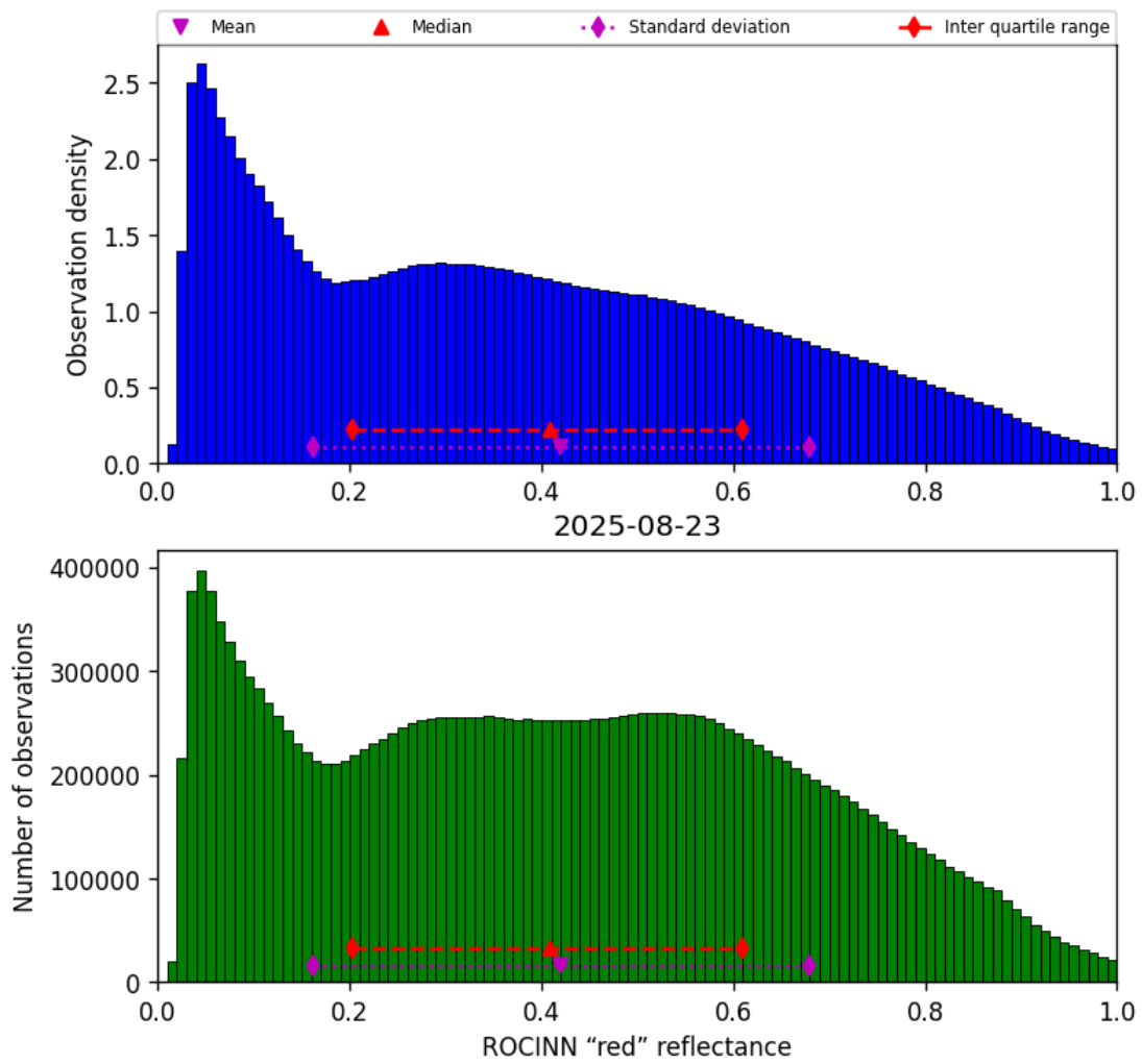
Figure 53: Histogram of “ROCINN “red” reflectance” for 2025-08-22 to 2025-08-24
