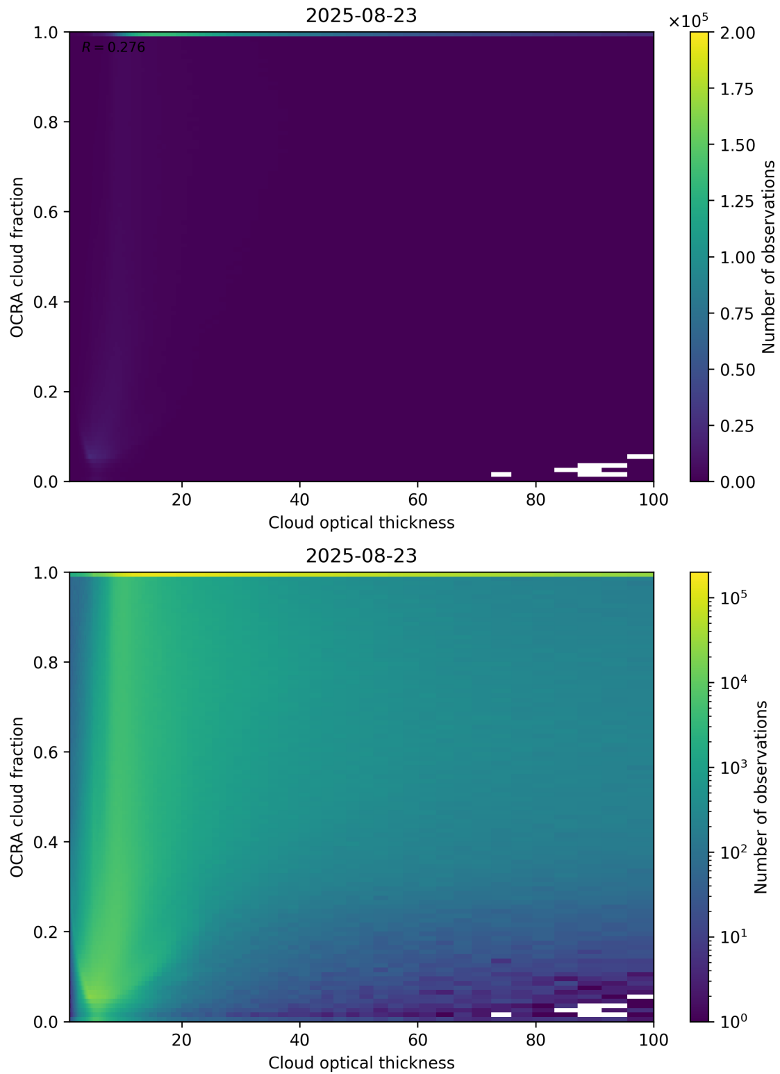
Figure 83: Scatter density plot of “Cloud optical thickness” against “OCRA cloud fraction” for 2025-08-22 to 2025-08-24.
