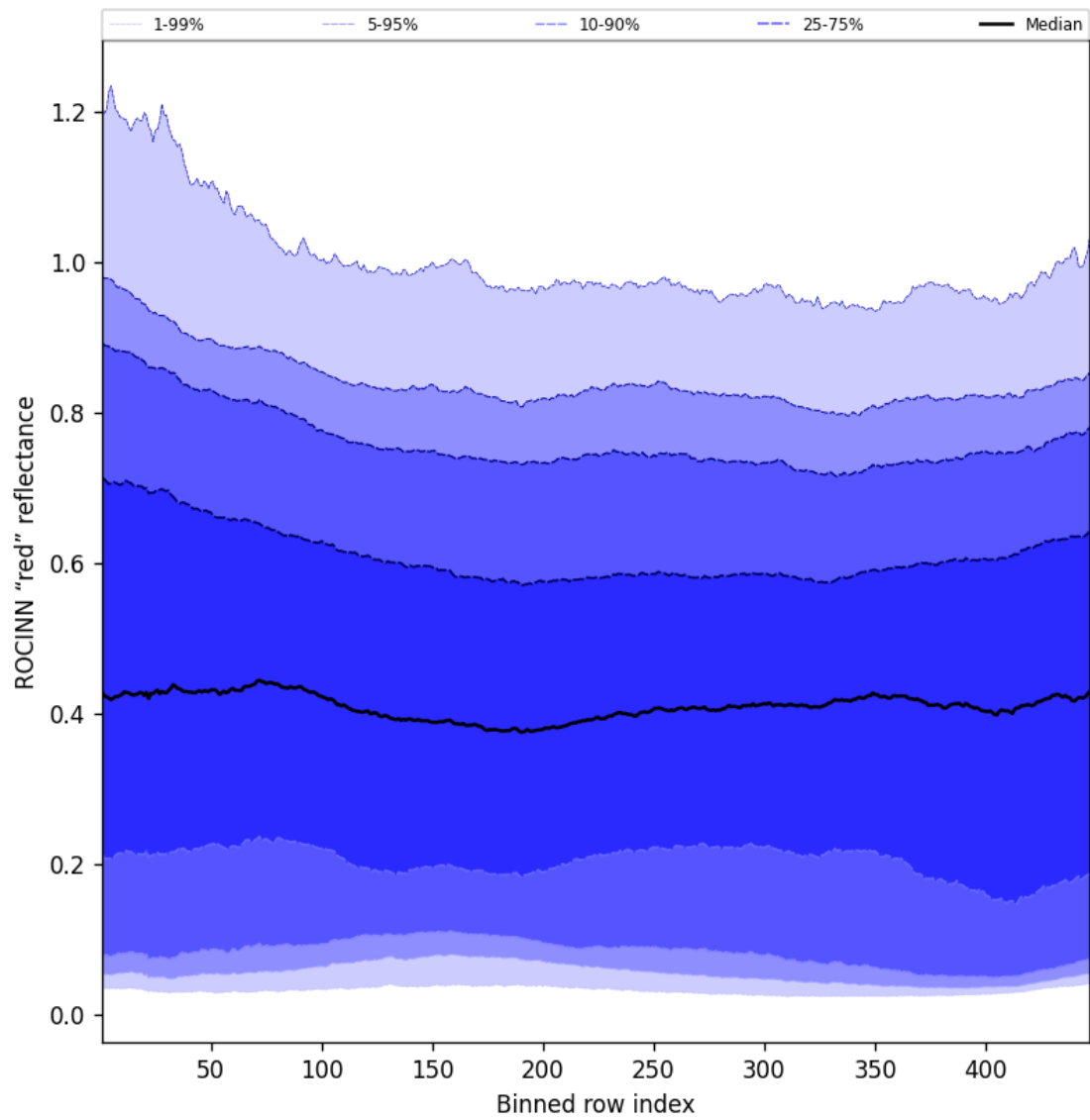
Figure 69: Along track statistics of "ROCINN "red" reflectance" for 2025-08-22 to 2025-08-24
