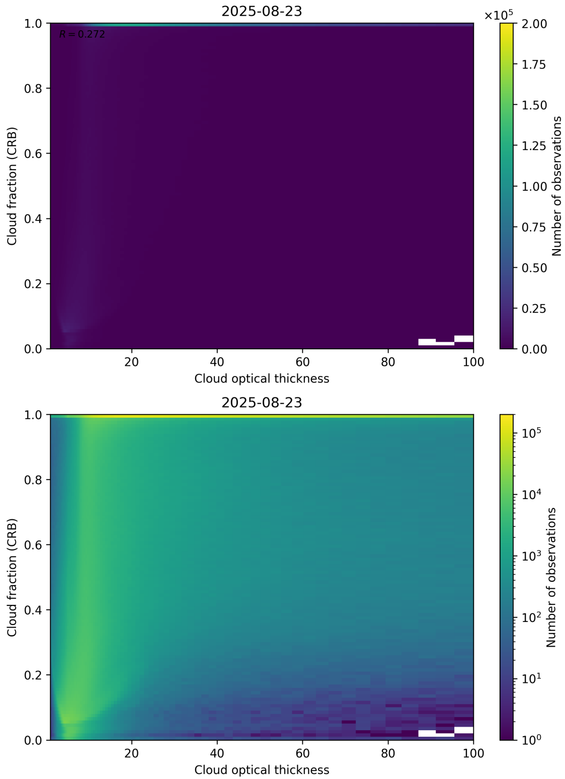
Figure 84: Scatter density plot of “Cloud optical thickness” against “Cloud fraction (CRB)” for 2025-08-22 to 2025-08-24.
