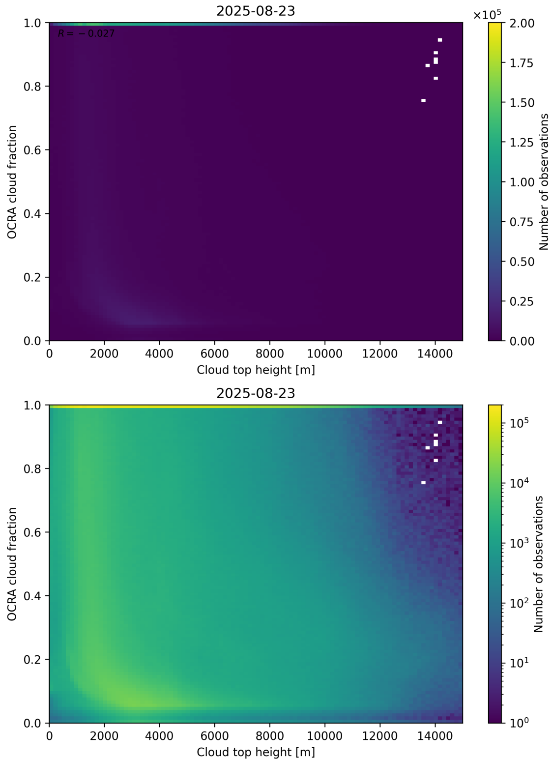
Figure 87: Scatter density plot of “Cloud top height” against “OCRA cloud fraction” for 2025-08-22 to 2025-08-24.
