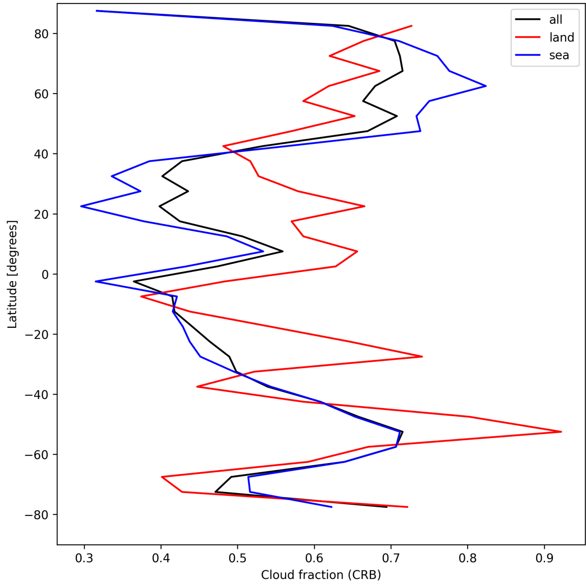
Figure 26: Zonal average of “Cloud fraction (CRB)” for 2025-08-22 to 2025-08-24.
