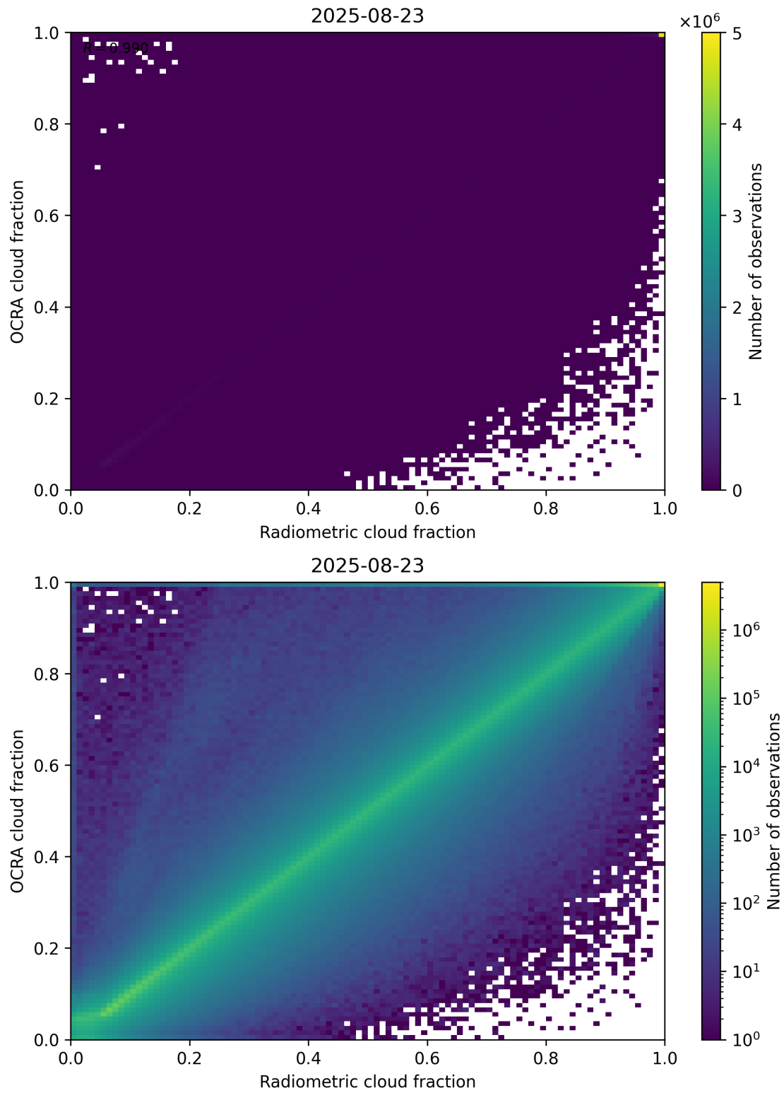
Figure 72: Scatter density plot of “Radiometric cloud fraction” against “OCRA cloud fraction” for 2025-08-22 to 2025-08-24.
