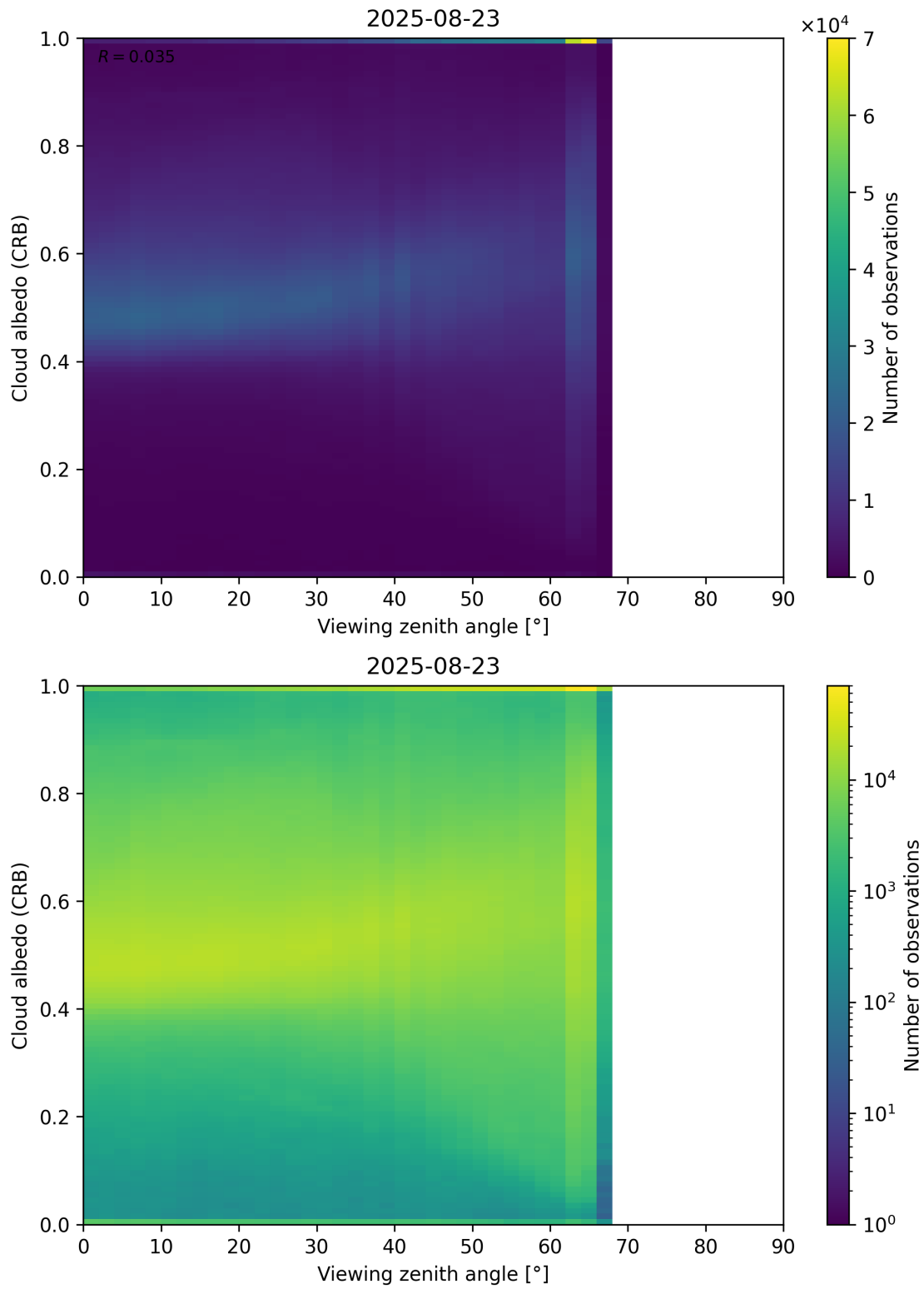
Figure 106: Scatter density plot of “Viewing zenith angle” against “Cloud albedo (CRB)” for 2025-08-22 to 2025-08-24.
