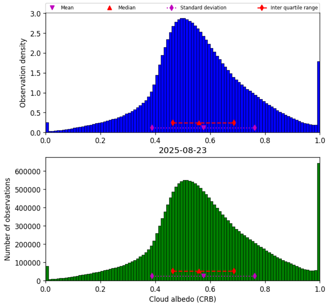
Figure 44: Histogram of “Cloud albedo (CRB)” for 2025-08-22 to 2025-08-24
