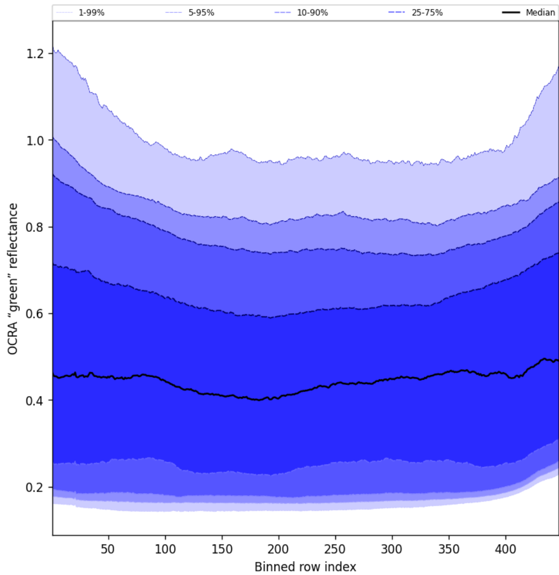
Figure 68: Along track statistics of "OCRA "green" reflectance" for 2025-08-22 to 2025-08-24
