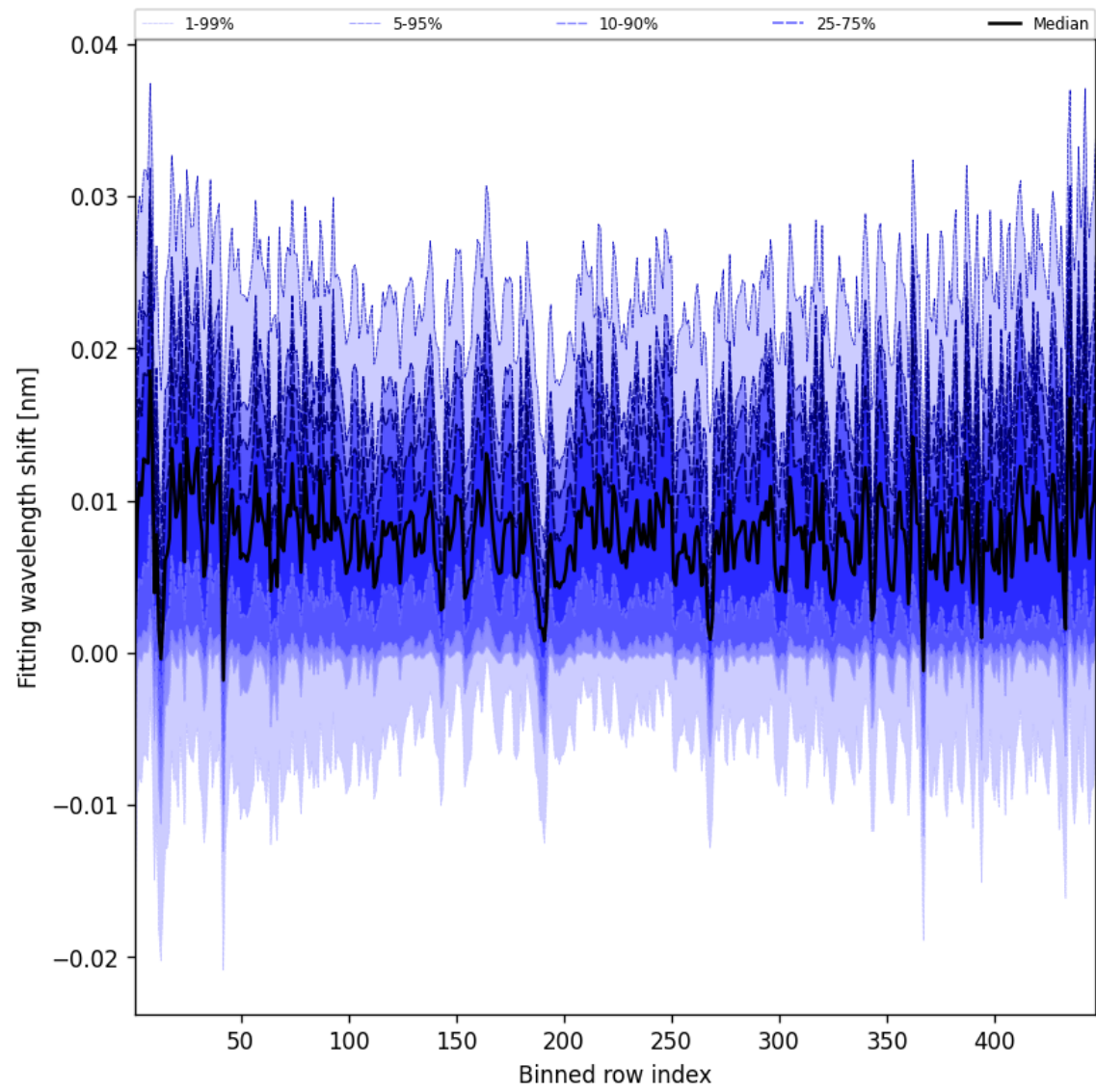
Figure 65: Along track statistics of “Fitting wavelength shift” for 2025-08-22 to 2025-08-24
