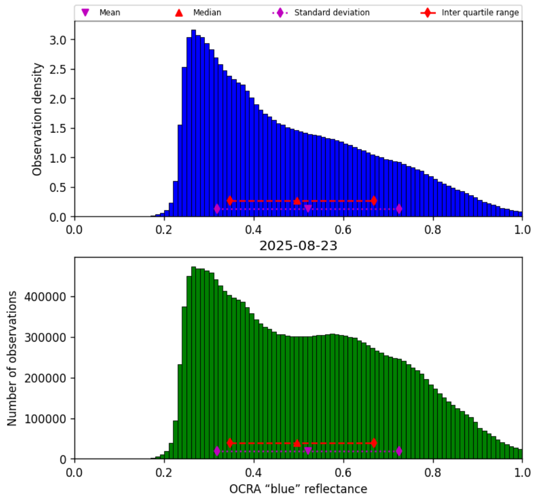
Figure 51: Histogram of “OCRA “blue” reflectance” for 2025-08-22 to 2025-08-24
