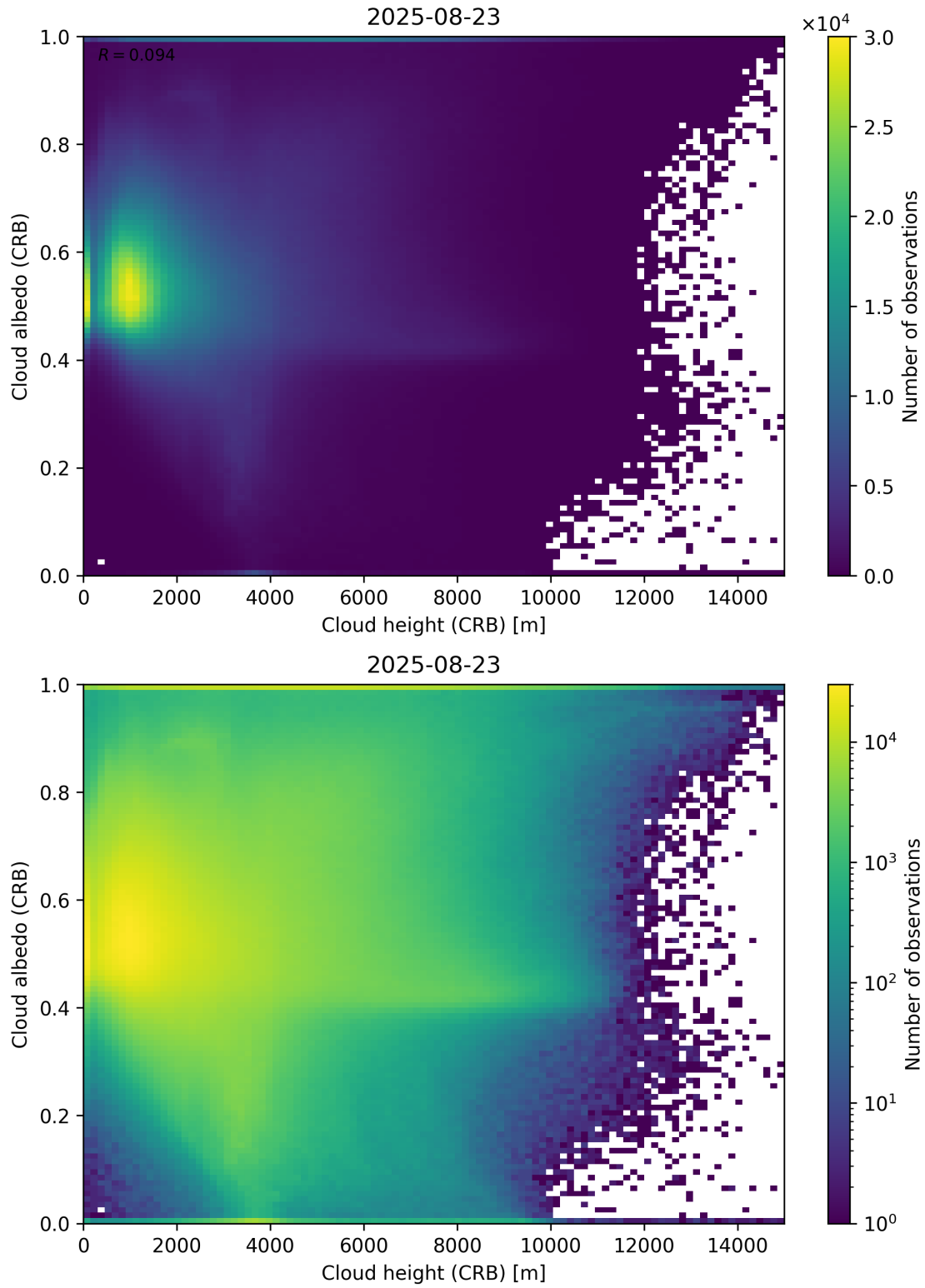
Figure 80: Scatter density plot of “Cloud height (CRB)” against “Cloud albedo (CRB)” for 2025-08-22 to 2025-08-24.
