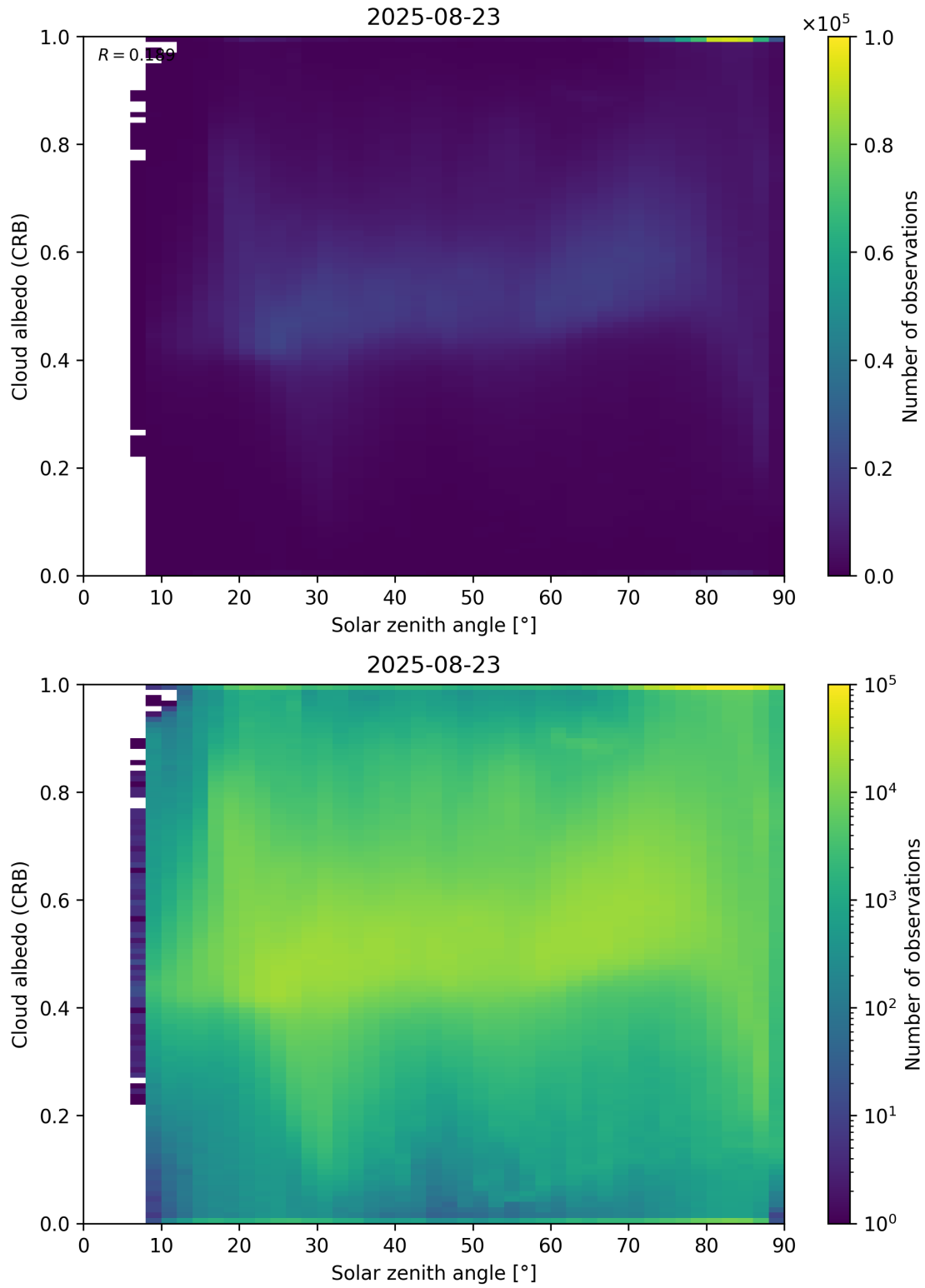
Figure 98: Scatter density plot of “Solar zenith angle” against “Cloud albedo (CRB)” for 2025-08-22 to 2025-08-24.
