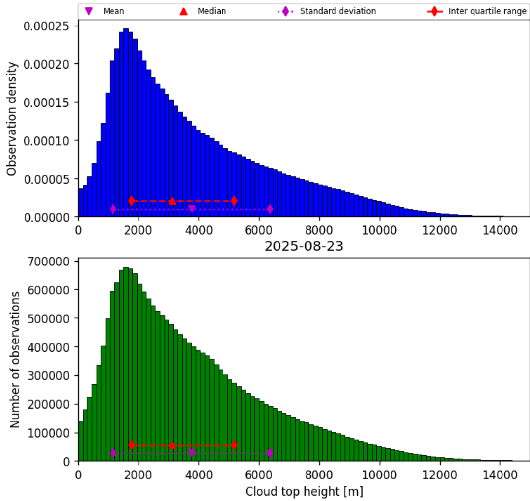
Figure 40: Histogram of “Cloud top height” for 2025-08-22 to 2025-08-24
