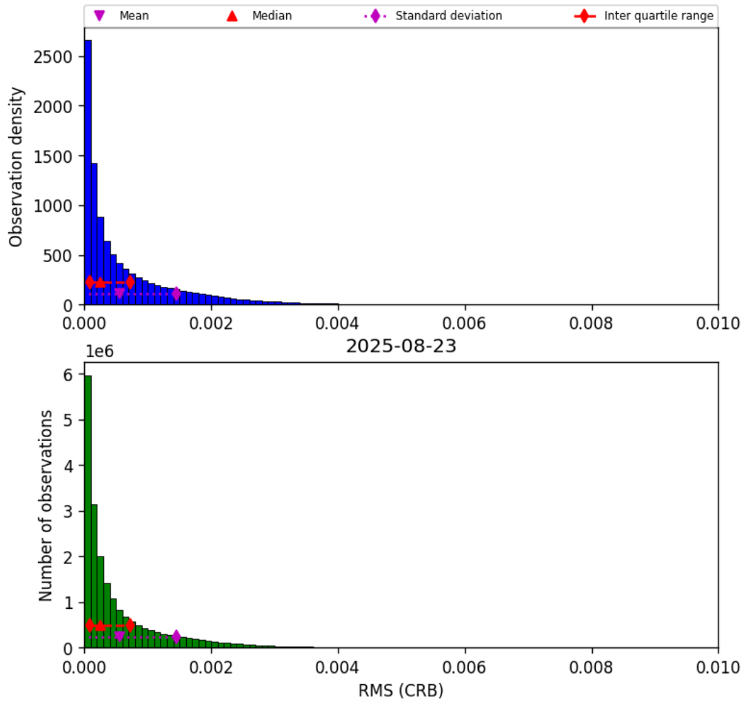
Figure 48: Histogram of “RMS (CRB)” for 2025-08-22 to 2025-08-24
