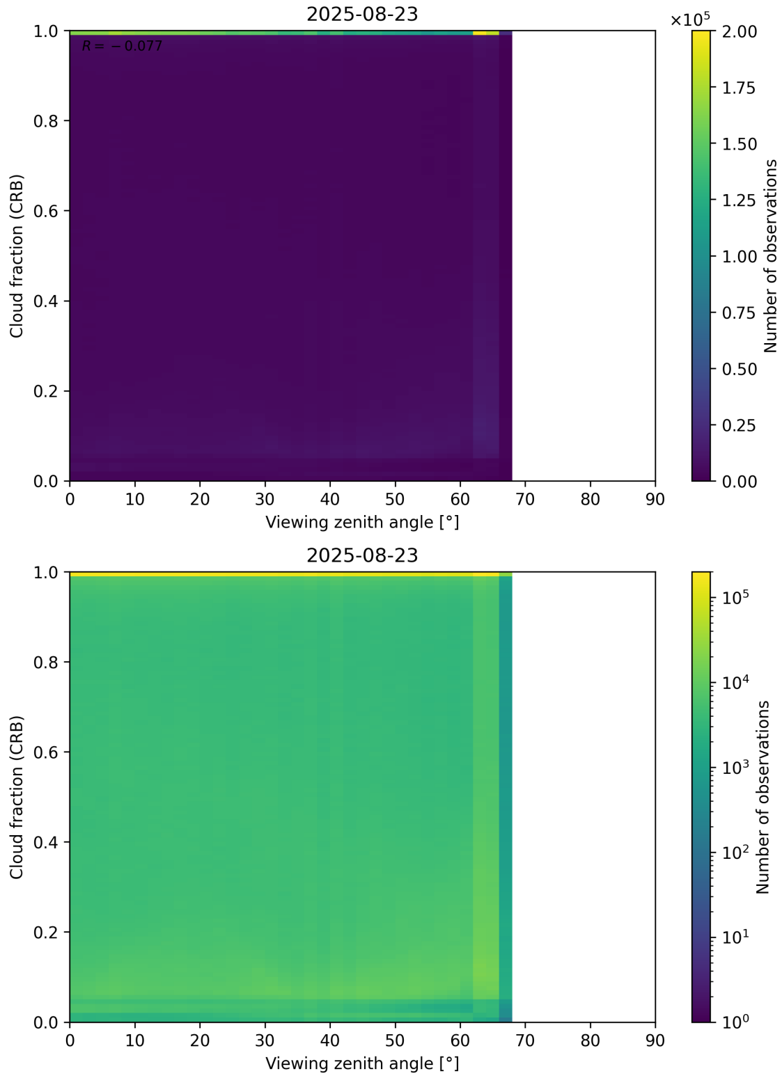
Figure 109: Scatter density plot of “Viewing zenith angle” against “Cloud fraction (CRB)” for 2025-08-22 to 2025-08-24.
