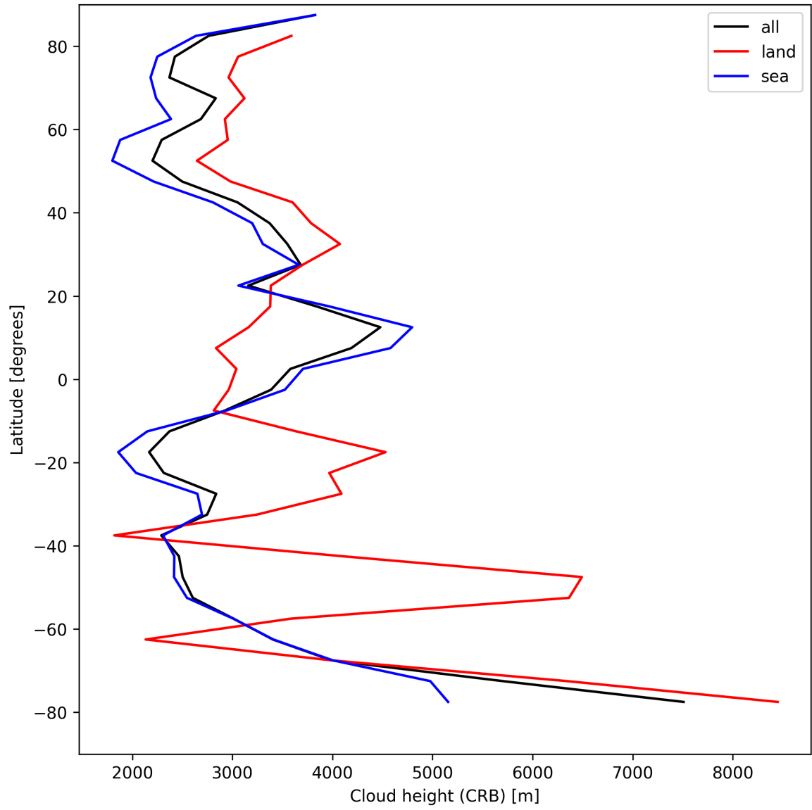
Figure 27: Zonal average of “Cloud height (CRB)” for 2025-08-22 to 2025-08-24.
