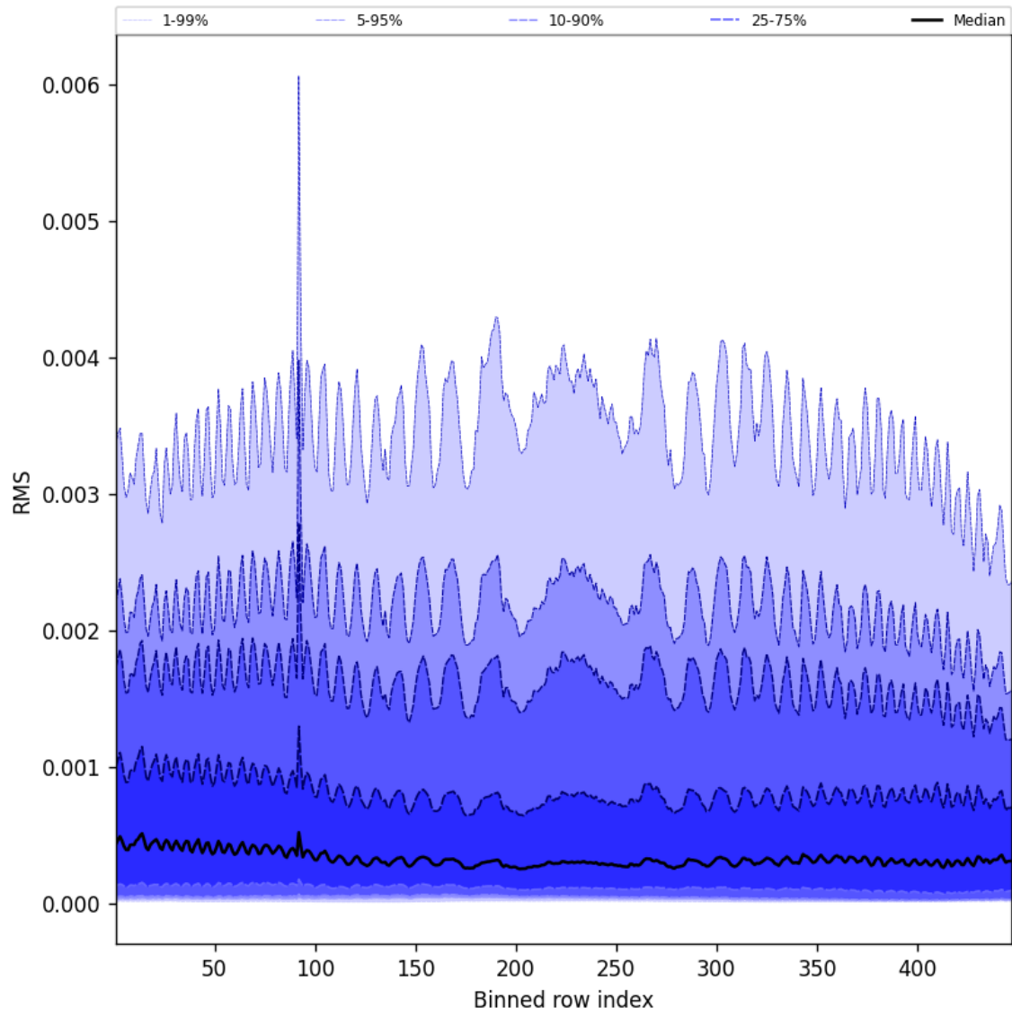
Figure 63: Along track statistics of “RMS” for 2025-08-22 to 2025-08-24
