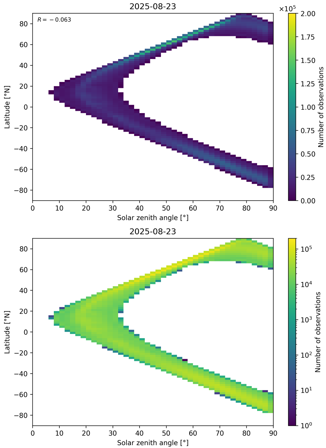
Figure 105: Scatter density plot of “Solar zenith angle” against “Latitude” for 2025-08-22 to 2025-08-24.
