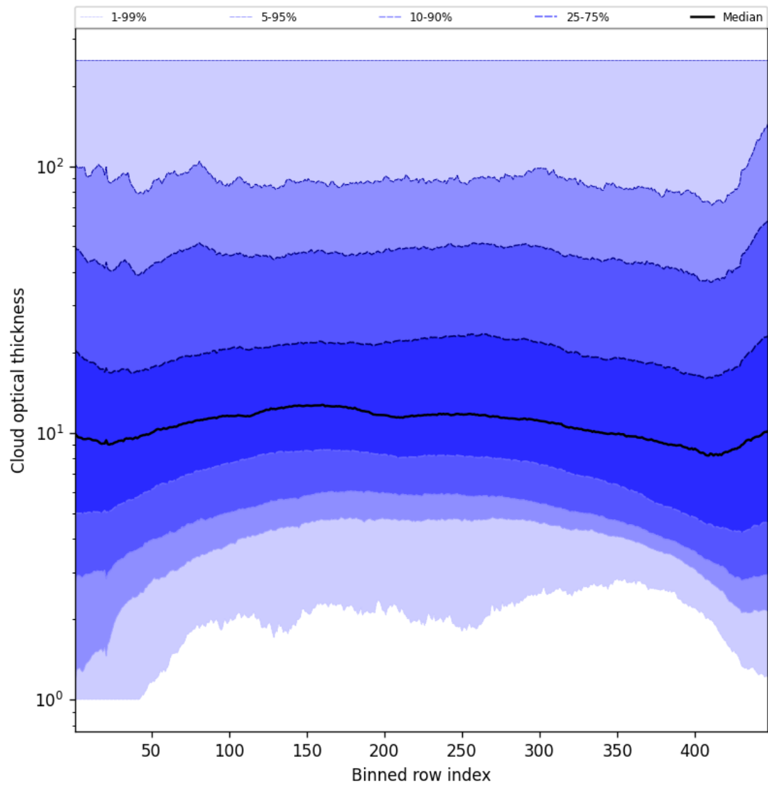
Figure 57: Along track statistics of “Cloud optical thickness” for 2025-08-22 to 2025-08-24
