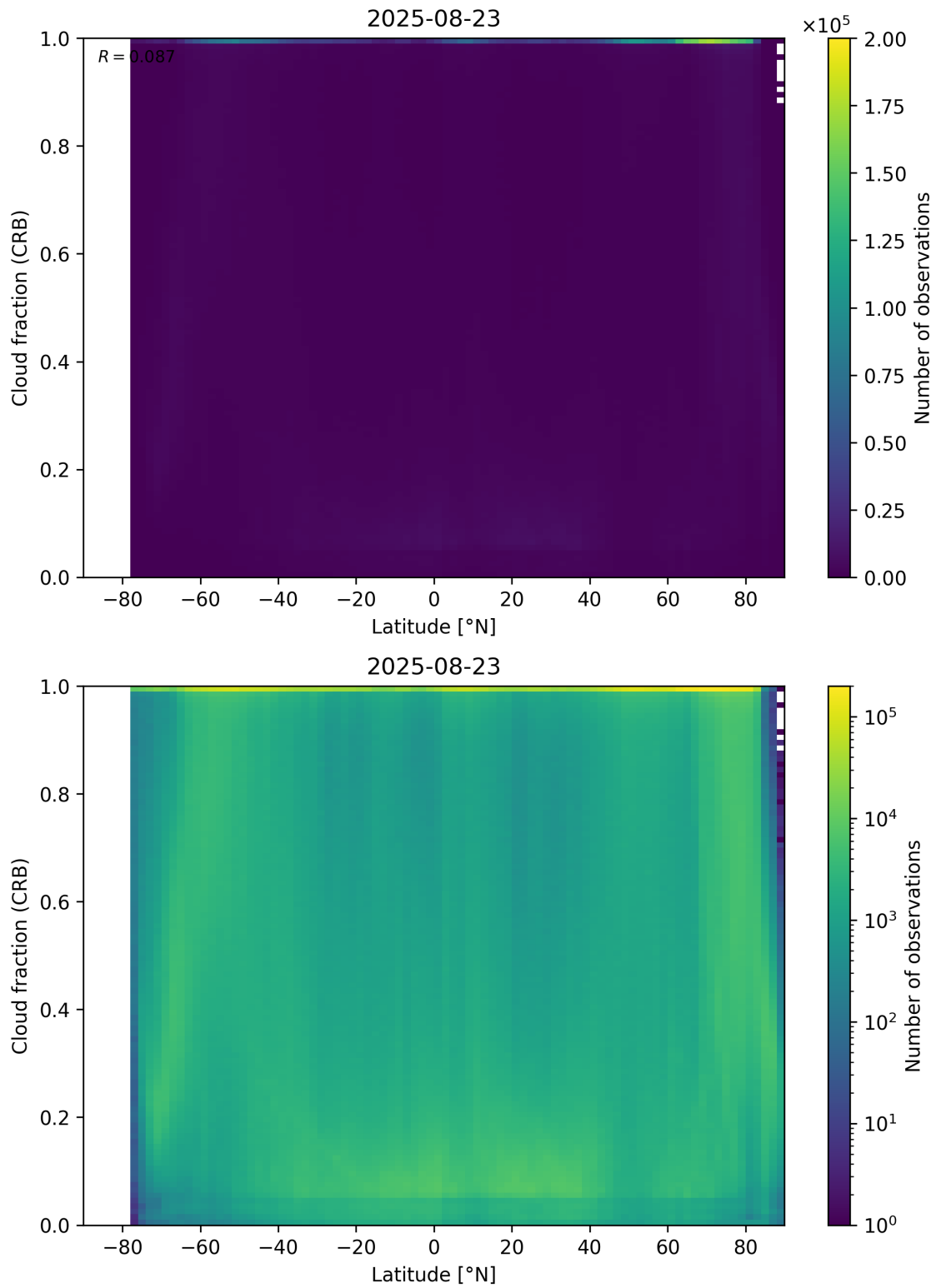
Figure 94: Scatter density plot of “Latitude” against “Cloud fraction (CRB)” for 2025-08-22 to 2025-08-24.
