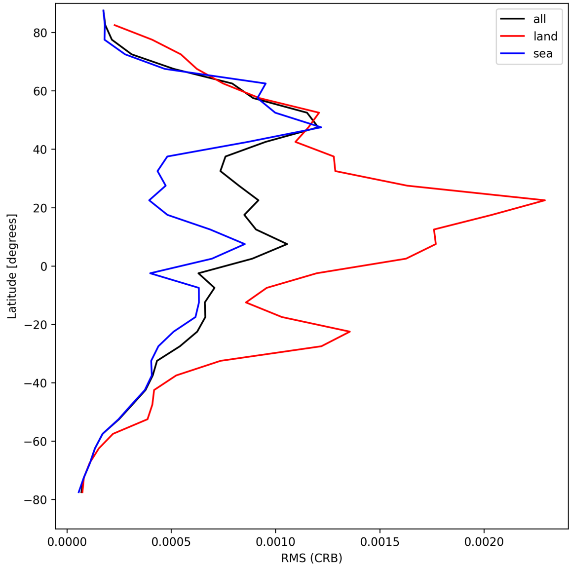
Figure 32: Zonal average of “RMS (CRB)” for 2025-08-22 to 2025-08-24.
