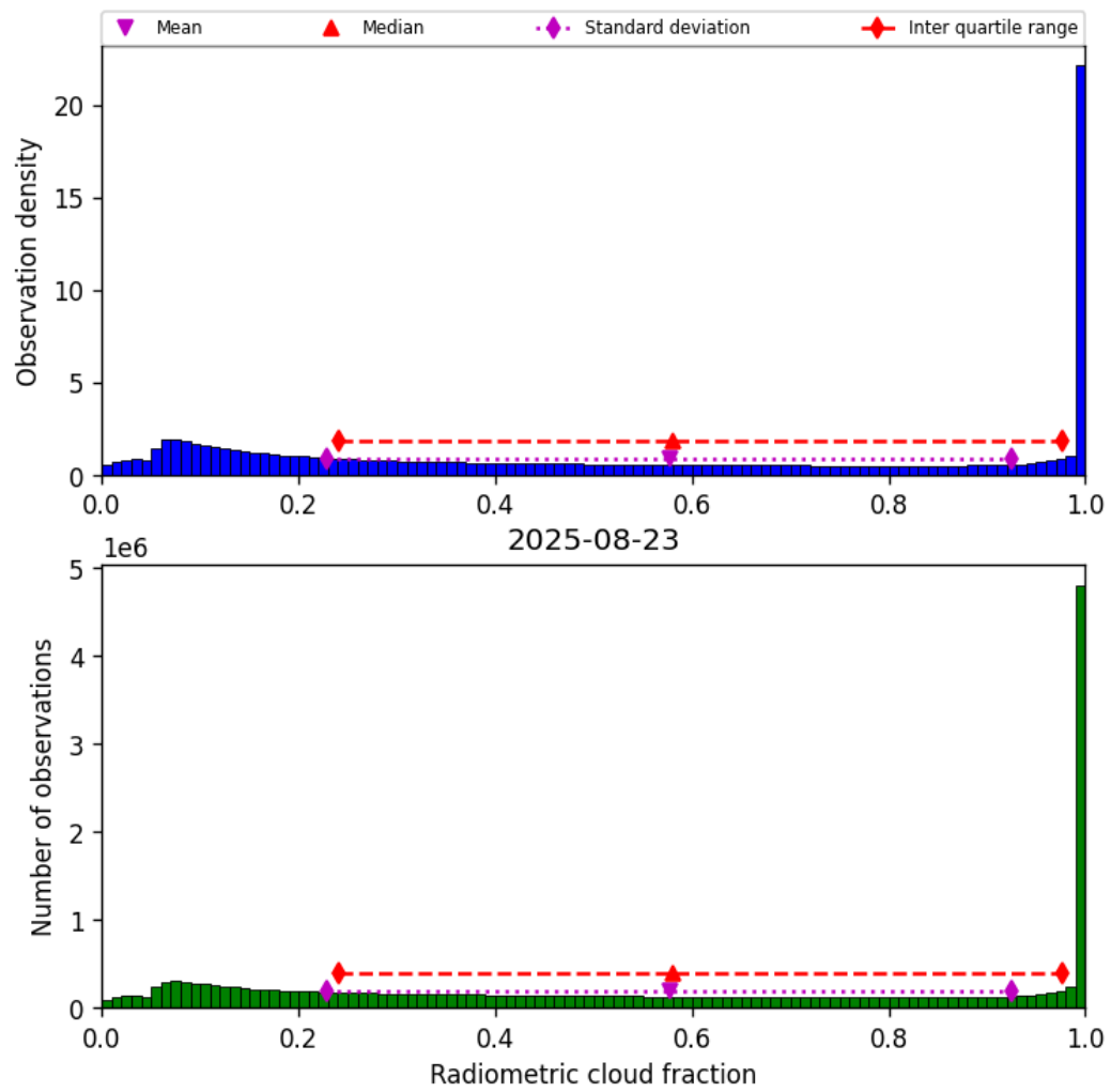
Figure 39: Histogram of “Radiometric cloud fraction” for 2025-08-22 to 2025-08-24
