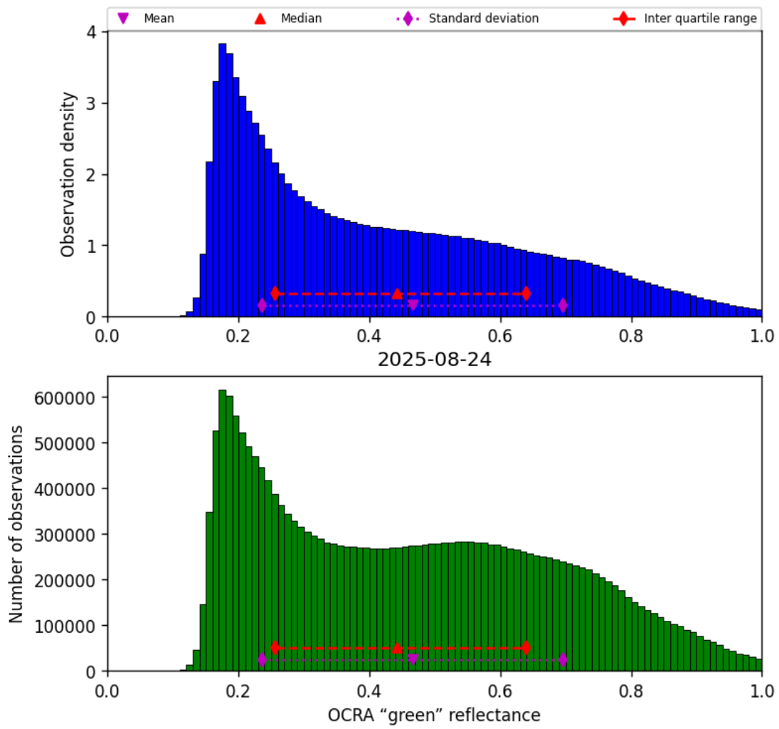
Figure 52: Histogram of “OCRA “green” reflectance” for 2025-08-23 to 2025-08-25
