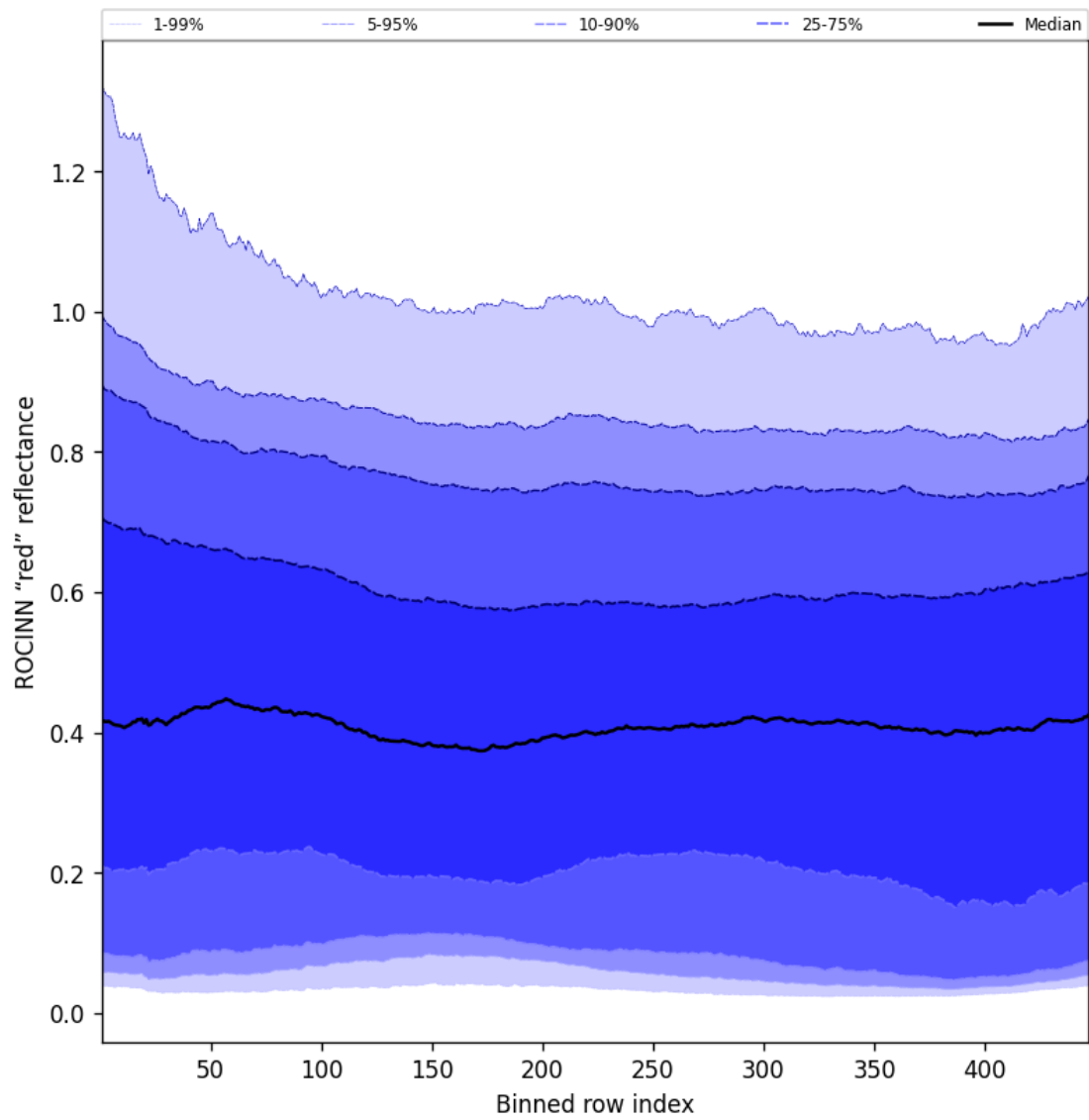
Figure 69: Along track statistics of “ROCINN “red” reflectance” for 2025-08-23 to 2025-08-25
