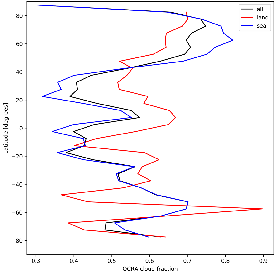
Figure 34: Zonal average of “OCRA cloud fraction” for 2025-08-23 to 2025-08-25.
