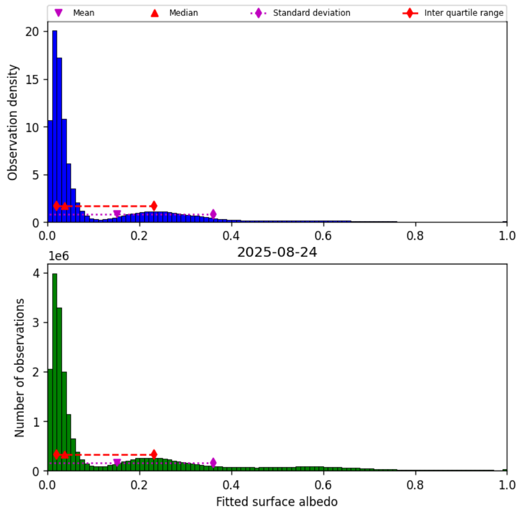
Figure 45: Histogram of “Fitted surface albedo” for 2025-08-23 to 2025-08-25
