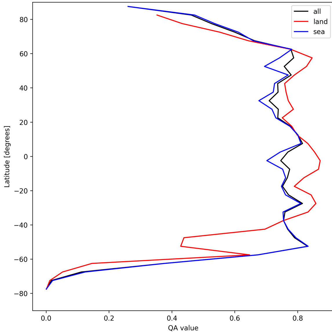
Figure 22: Zonal average of “QA value” for 2025-08-23 to 2025-08-25.
