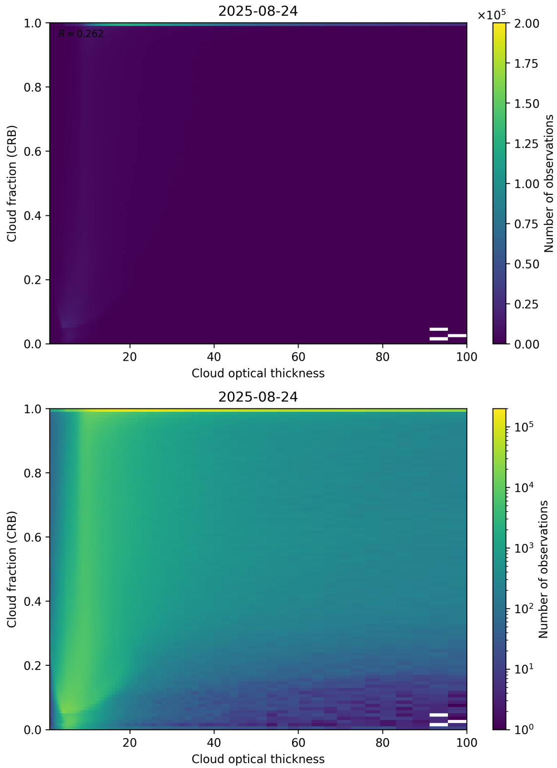
Figure 84: Scatter density plot of “Cloud optical thickness” against “Cloud fraction (CRB)” for 2025-08-23 to 2025-08-25.
