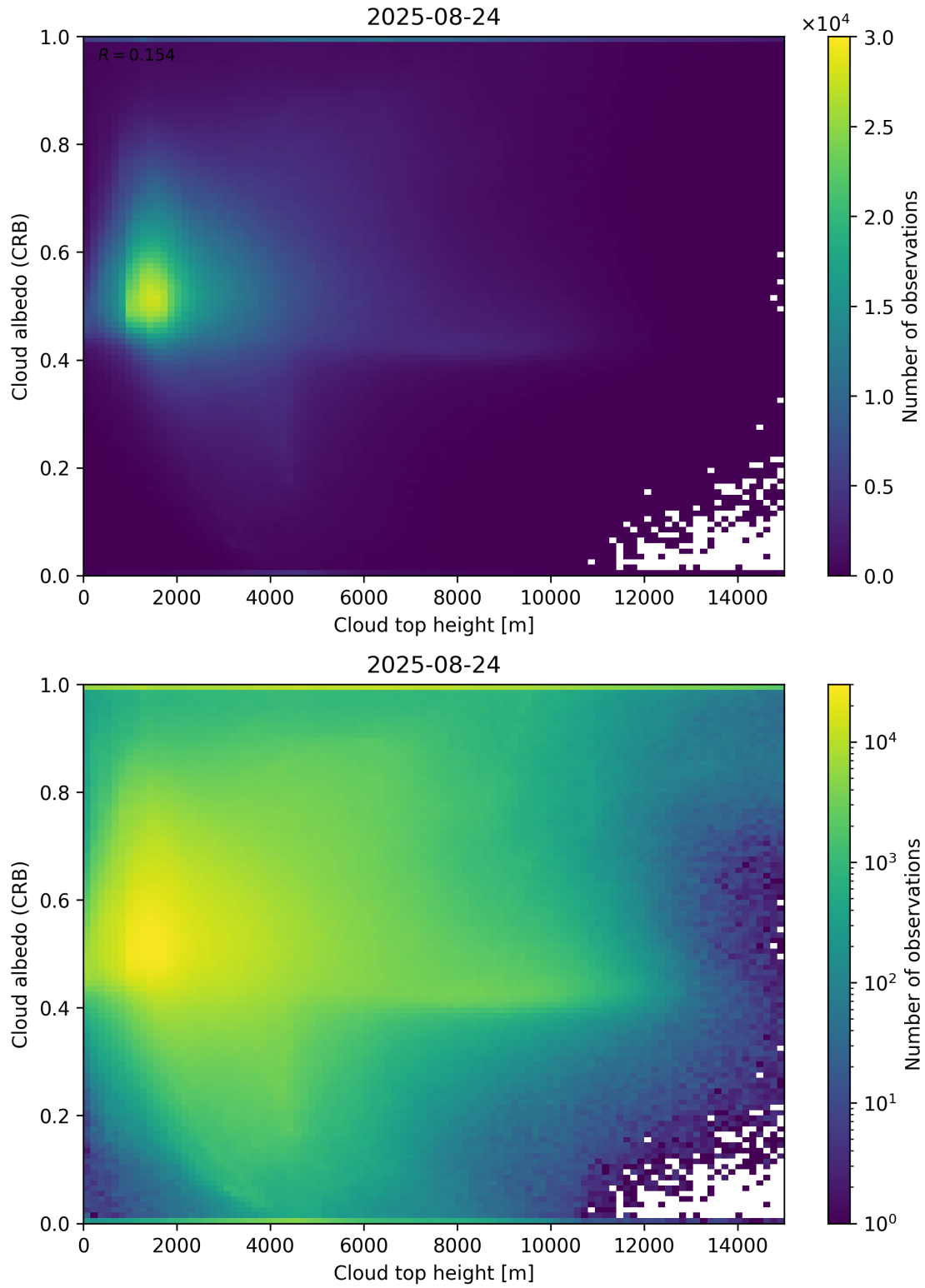
Figure 86: Scatter density plot of “Cloud top height” against “Cloud albedo (CRB)” for 2025-08-23 to 2025-08-25.
