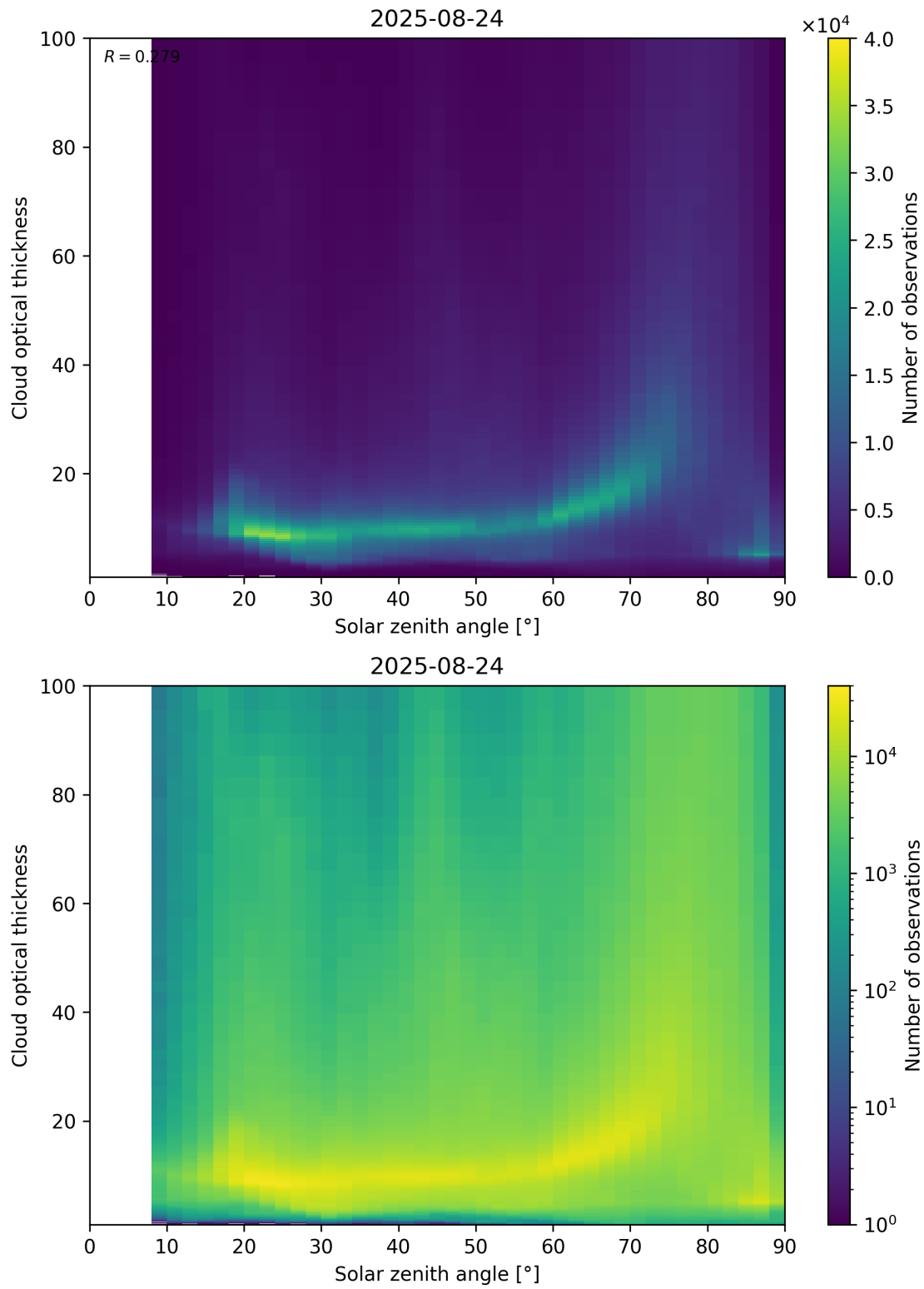
Figure 103: Scatter density plot of “Solar zenith angle” against “Cloud optical thickness” for 2025-08-23 to 2025-08-25.
