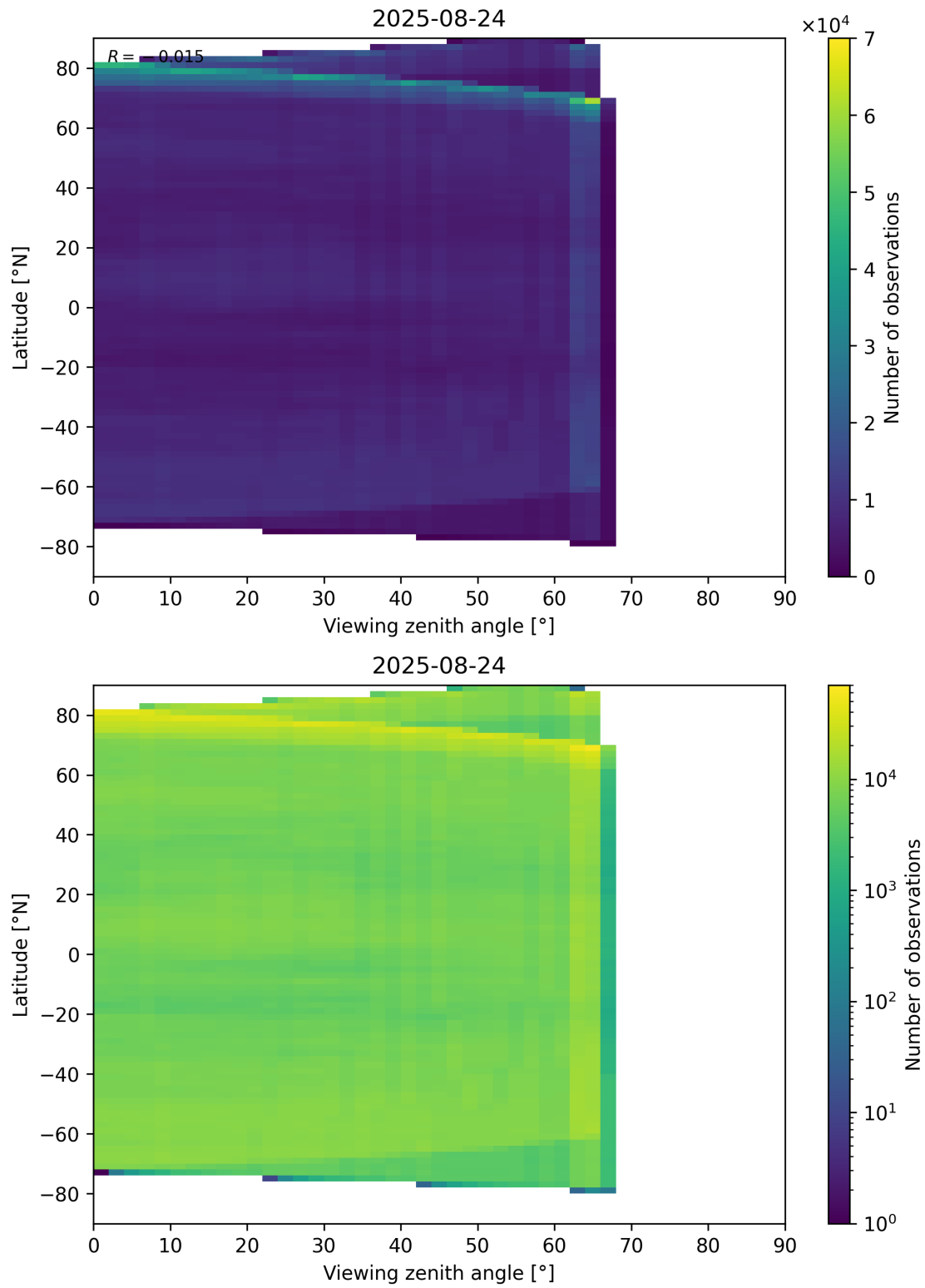
Figure 113: Scatter density plot of “Viewing zenith angle” against “Latitude” for 2025-08-23 to 2025-08-25.
