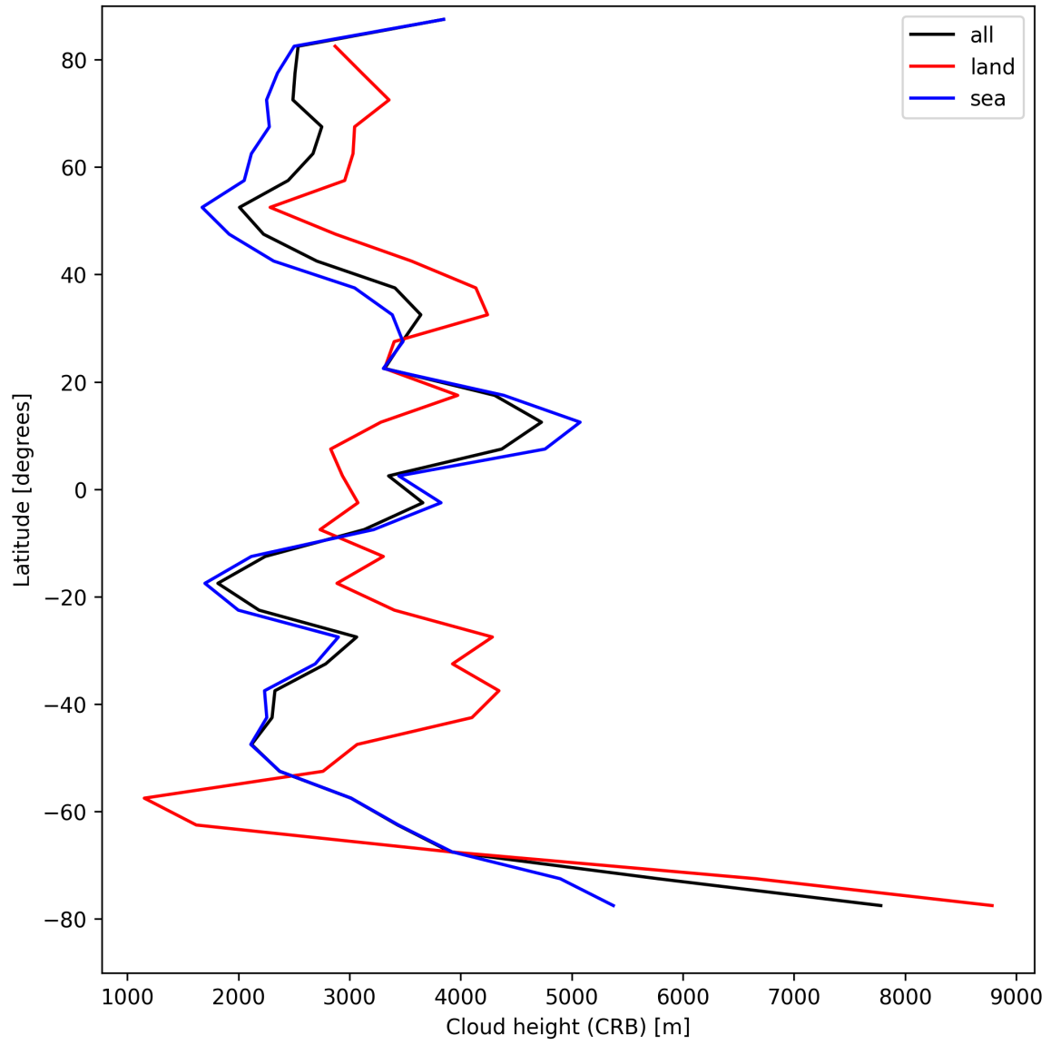
Figure 27: Zonal average of “Cloud height (CRB)” for 2025-08-23 to 2025-08-25.
