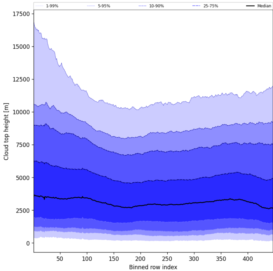
Figure 56: Along track statistics of “Cloud top height” for 2025-08-23 to 2025-08-25
