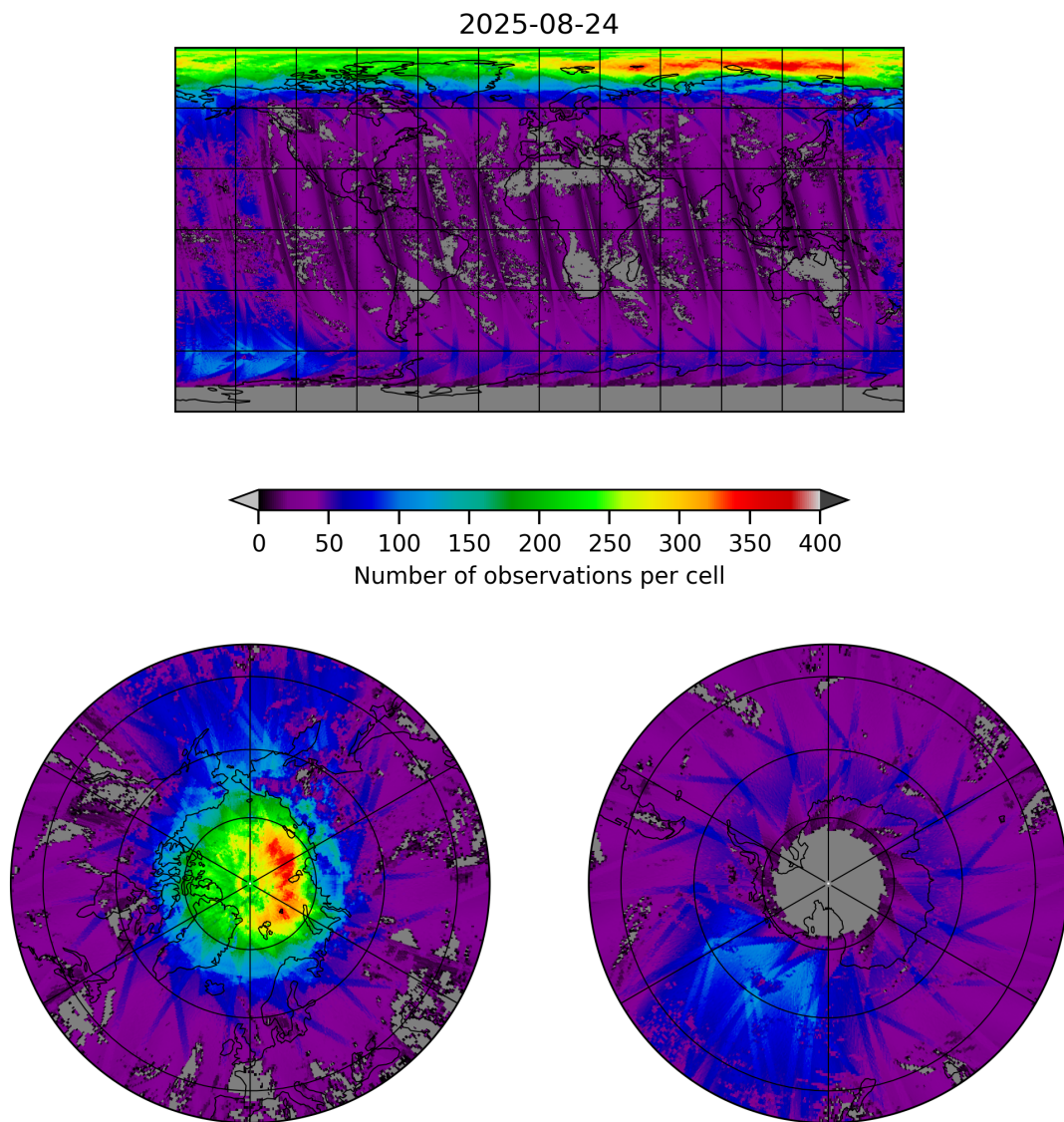
Figure 21: Map of the number of observations for 2025-08-23 to 2025-08-25
