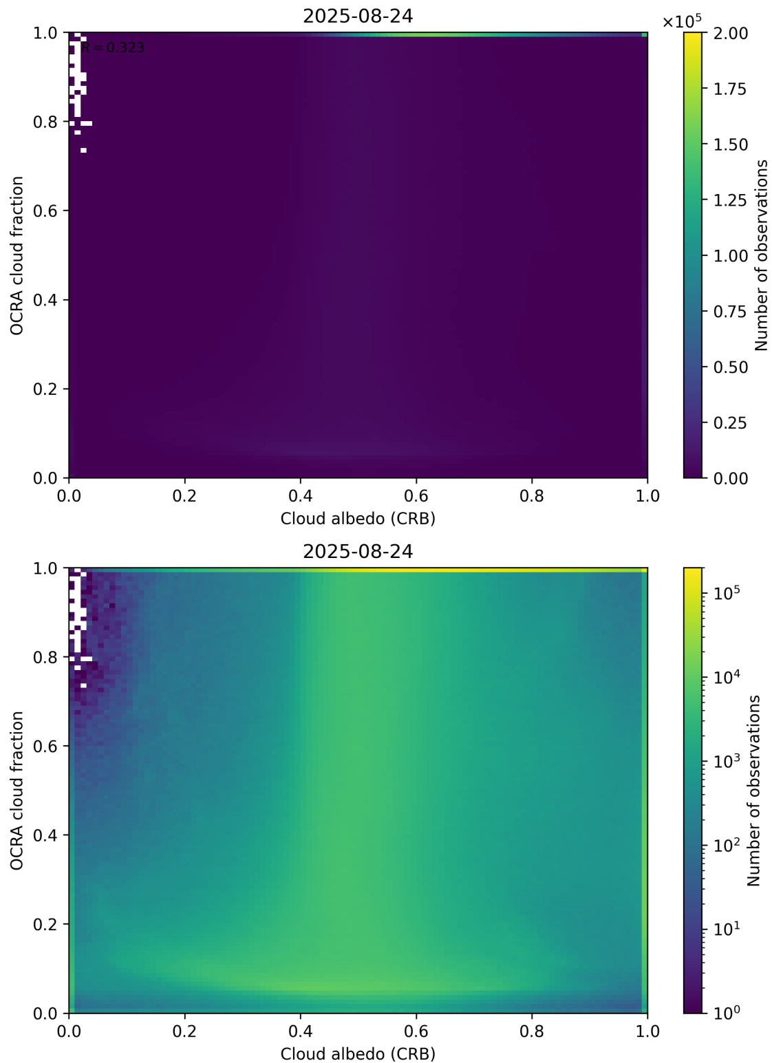
Figure 70: Scatter density plot of “Cloud albedo (CRB)” against “OCRA cloud fraction” for 2025-08-23 to 2025-08-25.
