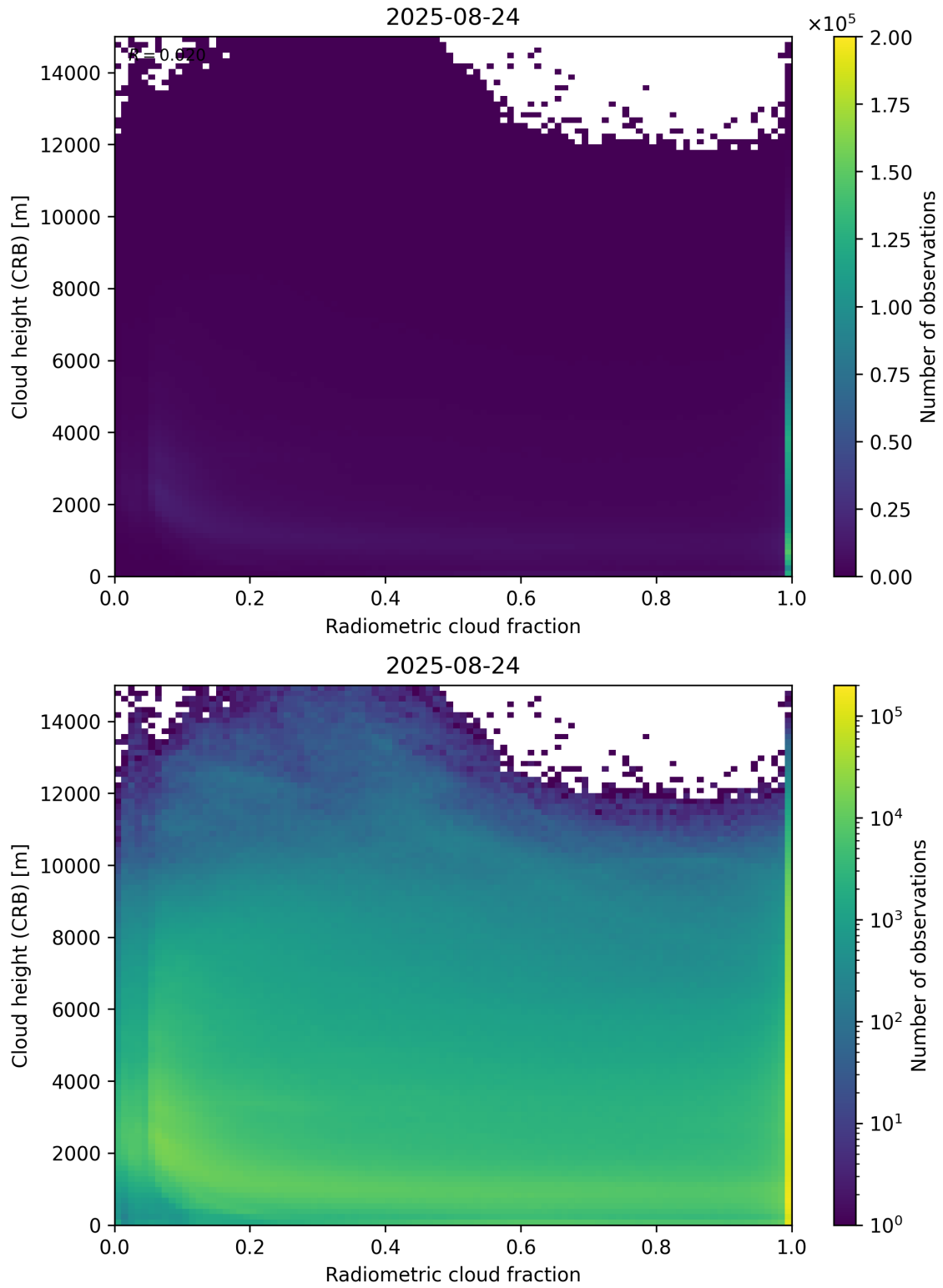
Figure 74: Scatter density plot of “Radiometric cloud fraction” against “Cloud height (CRB)” for 2025-08-23 to 2025-08-25.
