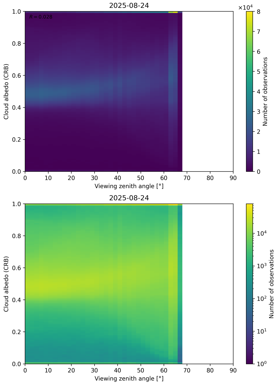
Figure 106: Scatter density plot of “Viewing zenith angle” against “Cloud albedo (CRB)” for 2025-08-23 to 2025-08-25.
