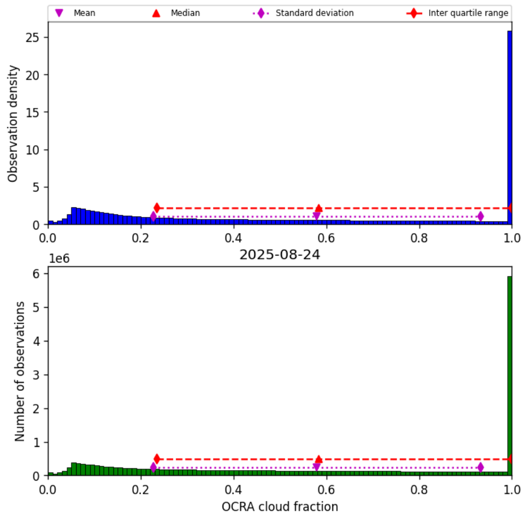
Figure 50: Histogram of “OCRA cloud fraction” for 2025-08-23 to 2025-08-25
