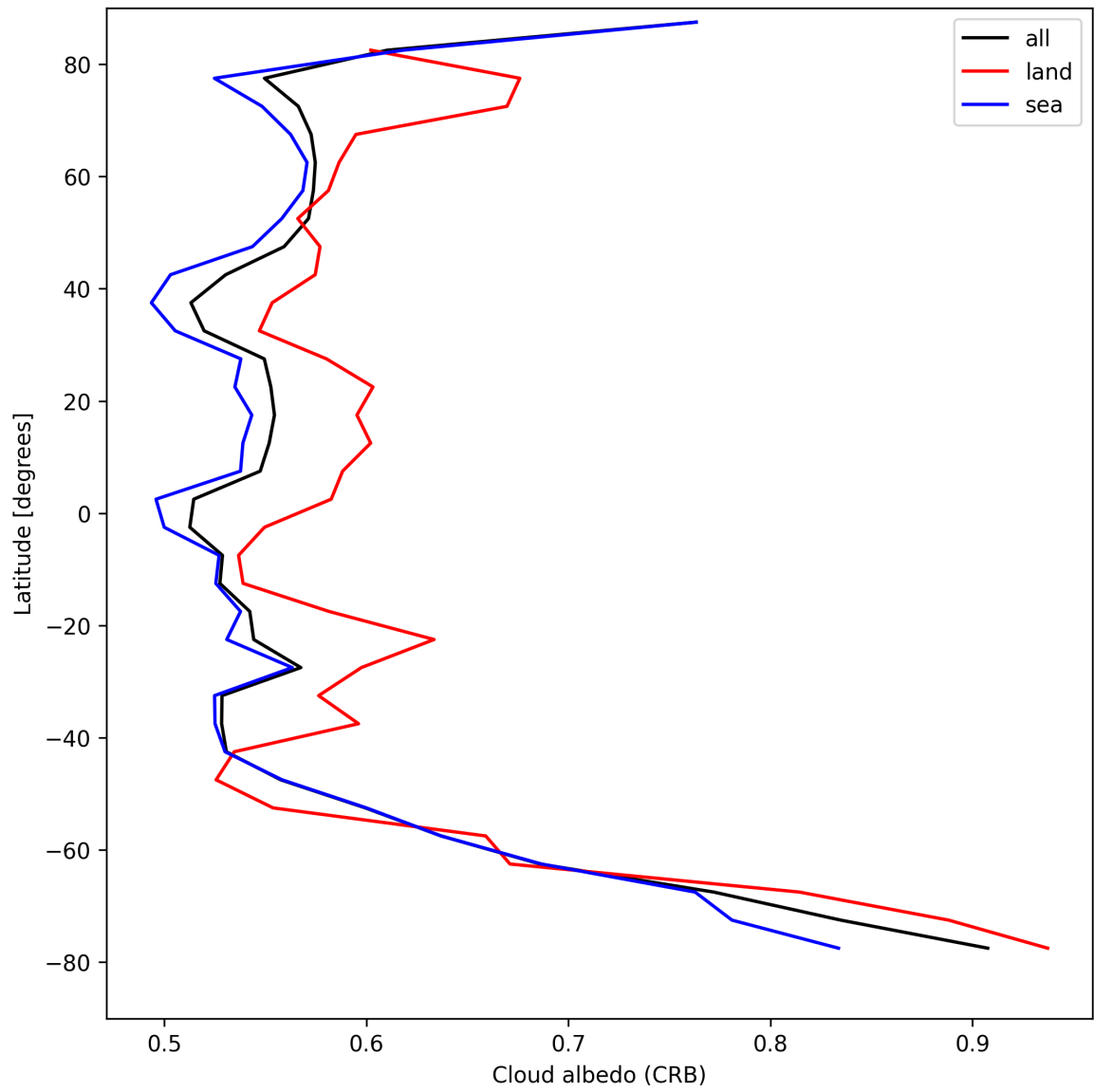
Figure 28: Zonal average of “Cloud albedo (CRB)” for 2025-08-23 to 2025-08-25.
