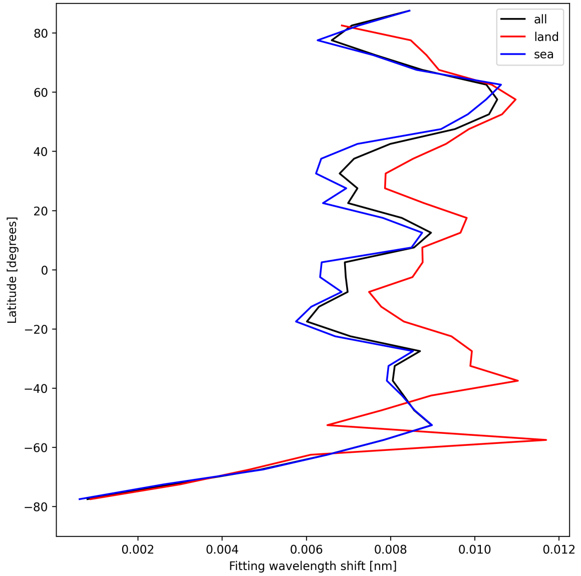
Figure 33: Zonal average of “Fitting wavelength shift” for 2025-08-23 to 2025-08-25.
