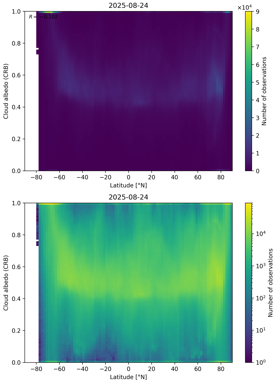
Figure 91: Scatter density plot of “Latitude” against “Cloud albedo (CRB)” for 2025-08-23 to 2025-08-25.
