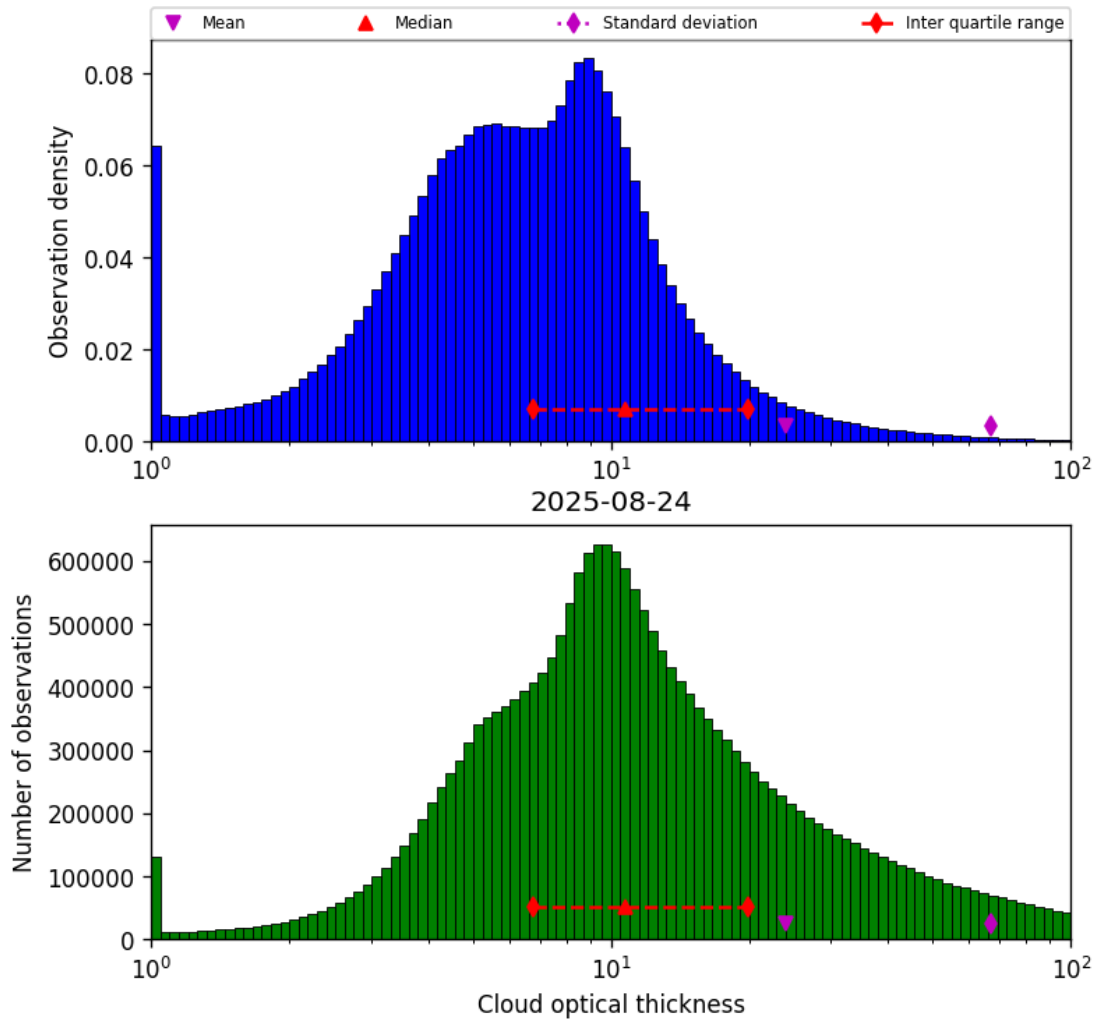
Figure 41: Histogram of “Cloud optical thickness” for 2025-08-23 to 2025-08-25
