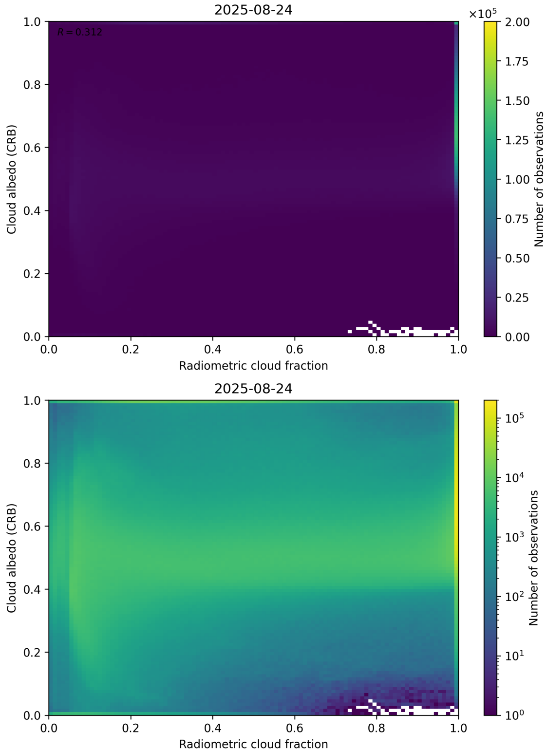
Figure 71: Scatter density plot of “Radiometric cloud fraction” against “Cloud albedo (CRB)” for 2025-08-23 to 2025-08-25.
