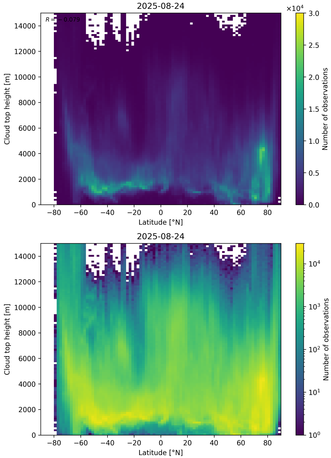
Figure 97: Scatter density plot of “Latitude” against “Cloud top height” for 2025-08-23 to 2025-08-25.
