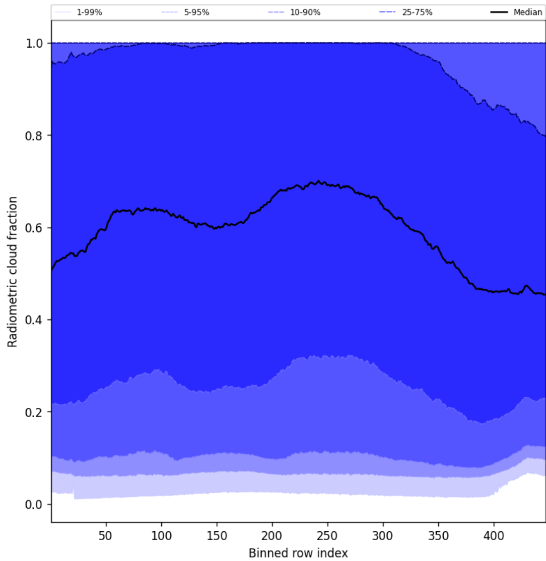
Figure 55: Along track statistics of “Radiometric cloud fraction” for 2025-08-23 to 2025-08-25
