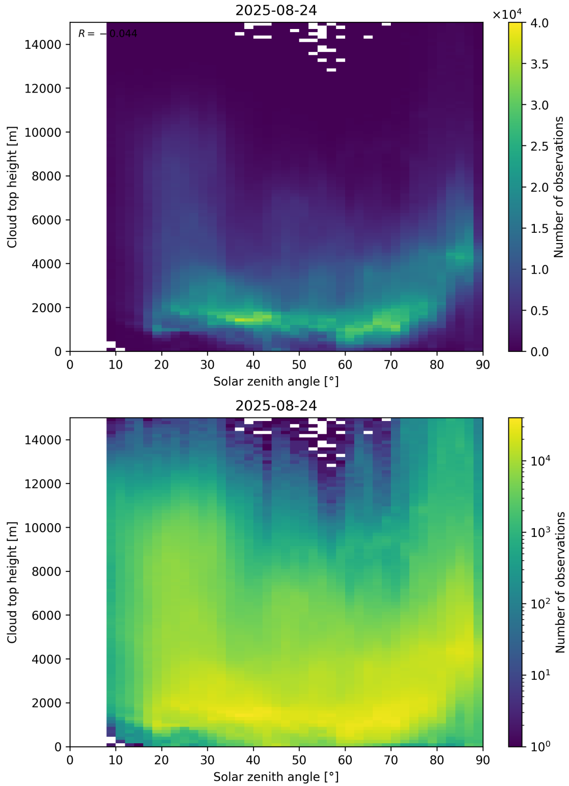
Figure 104: Scatter density plot of “Solar zenith angle” against “Cloud top height” for 2025-08-23 to 2025-08-25.
