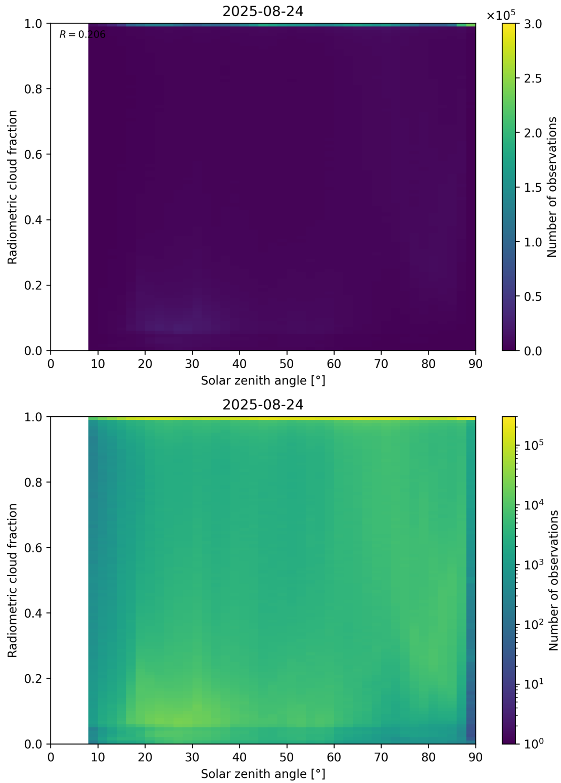
Figure 99: Scatter density plot of “Solar zenith angle” against “Radiometric cloud fraction” for 2025-08-23 to 2025-08-25.
