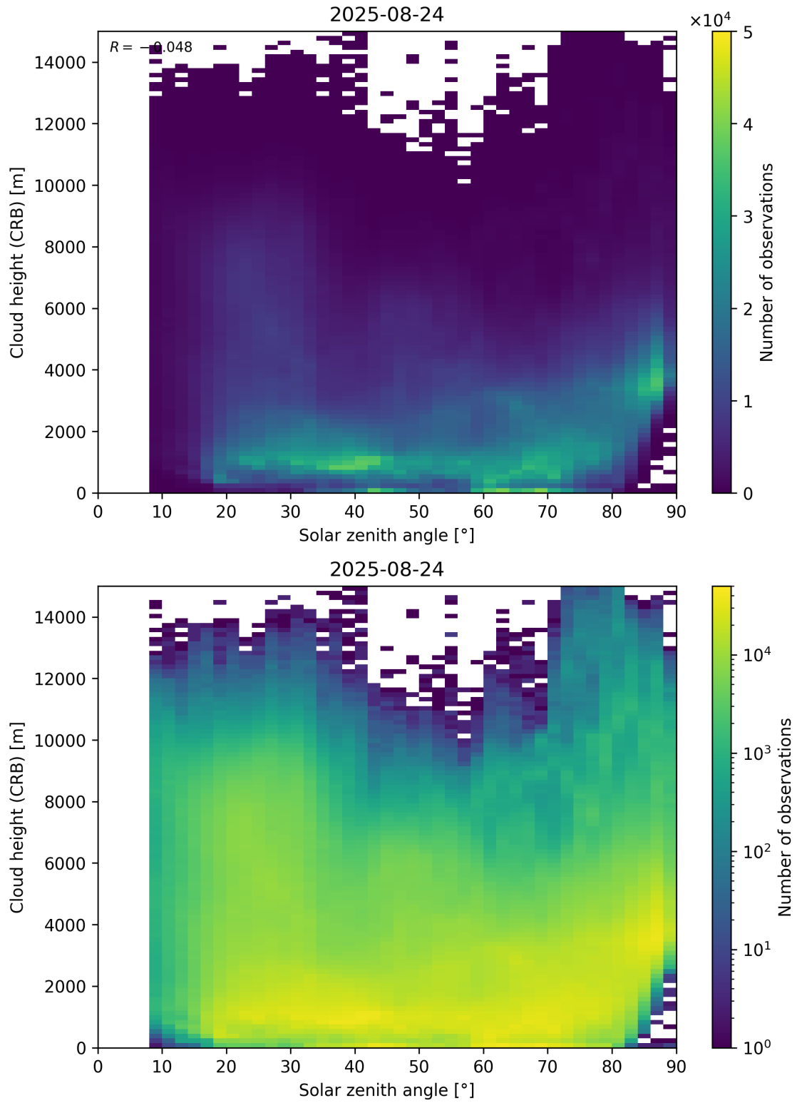
Figure 102: Scatter density plot of “Solar zenith angle” against “Cloud height (CRB)” for 2025-08-23 to 2025-08-25.
