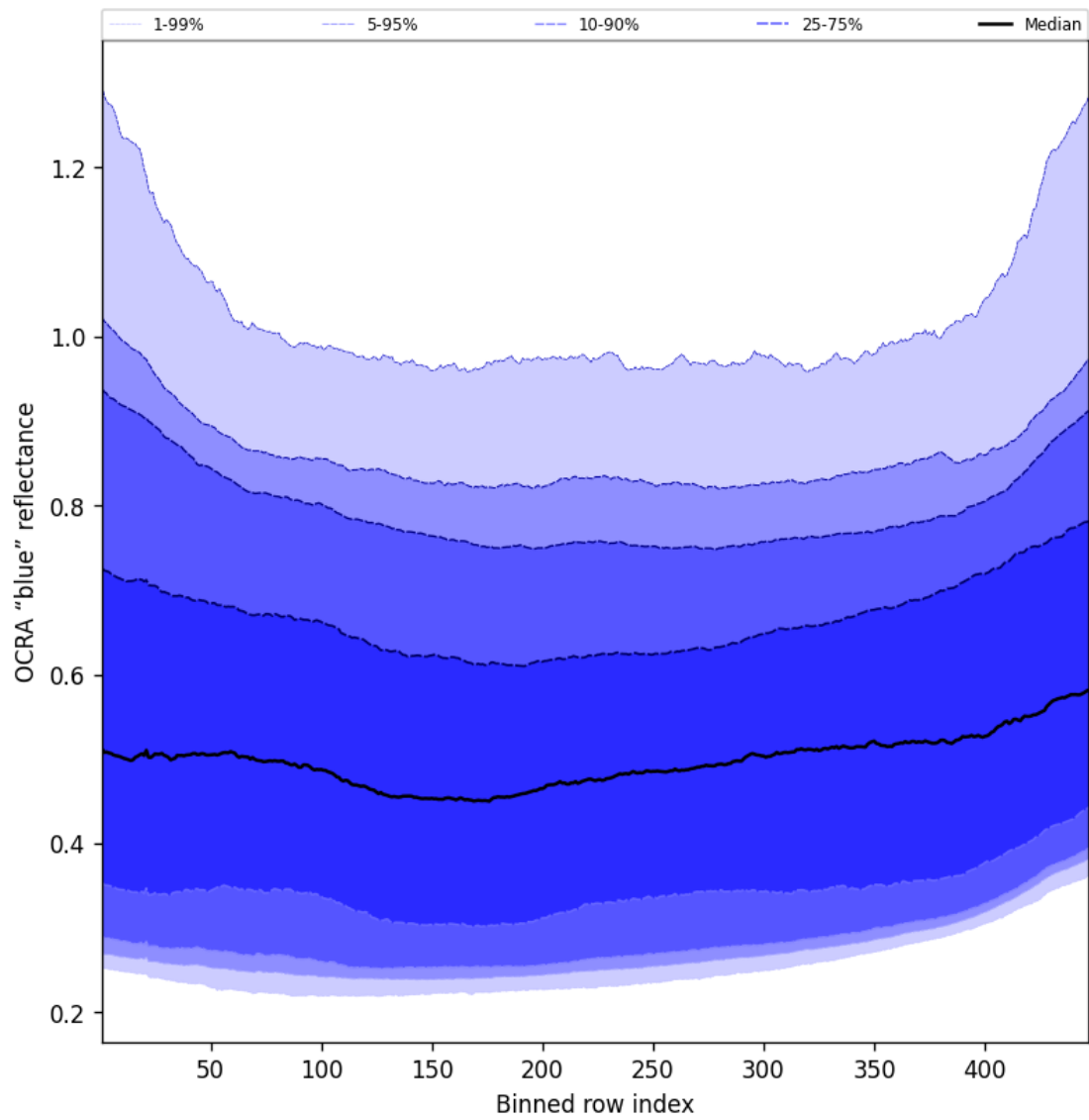
Figure 67: Along track statistics of “OCRA “blue” reflectance” for 2025-08-23 to 2025-08-25
