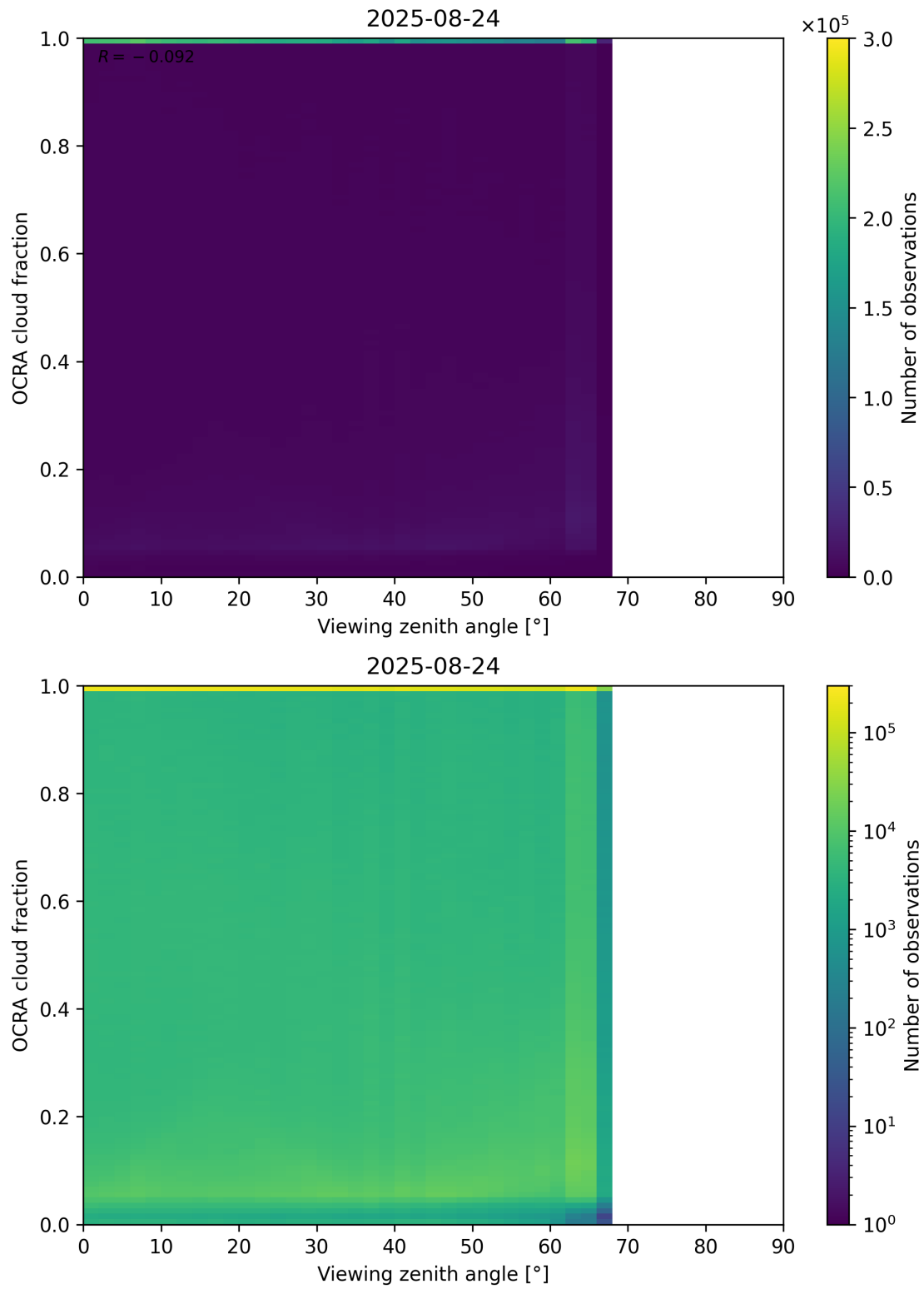
Figure 108: Scatter density plot of “Viewing zenith angle” against “OCRA cloud fraction” for 2025-08-23 to 2025-08-25.
