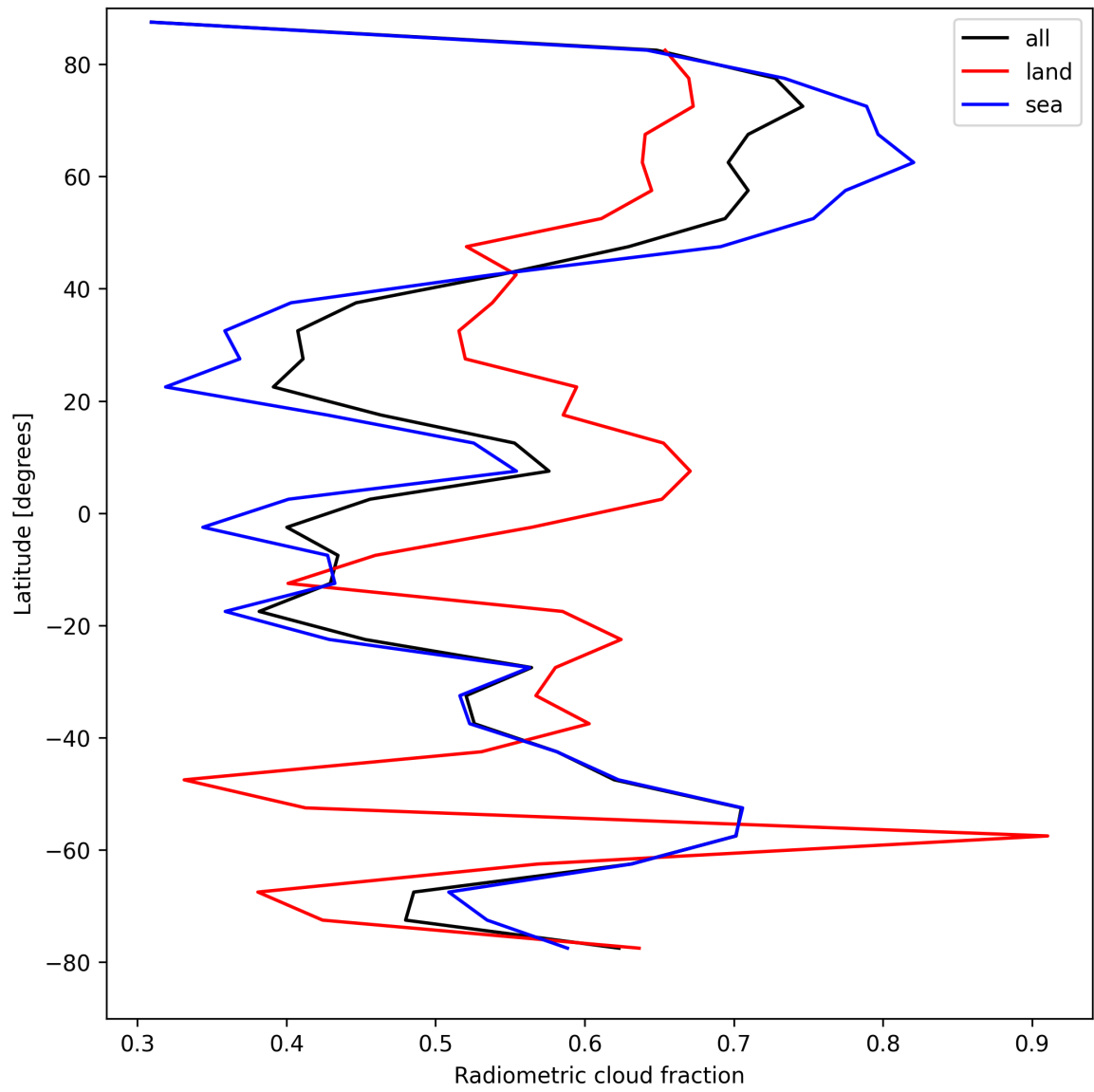
Figure 23: Zonal average of “Radiometric cloud fraction” for 2025-08-23 to 2025-08-25.
