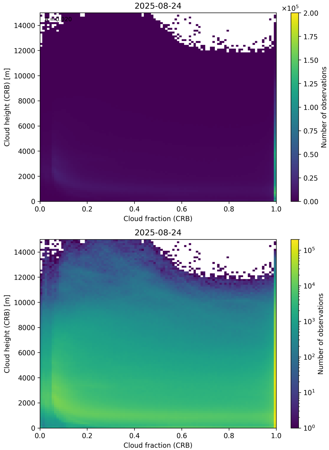
Figure 79: Scatter density plot of “Cloud fraction (CRB)” against “Cloud height (CRB)” for 2025-08-23 to 2025-08-25.
