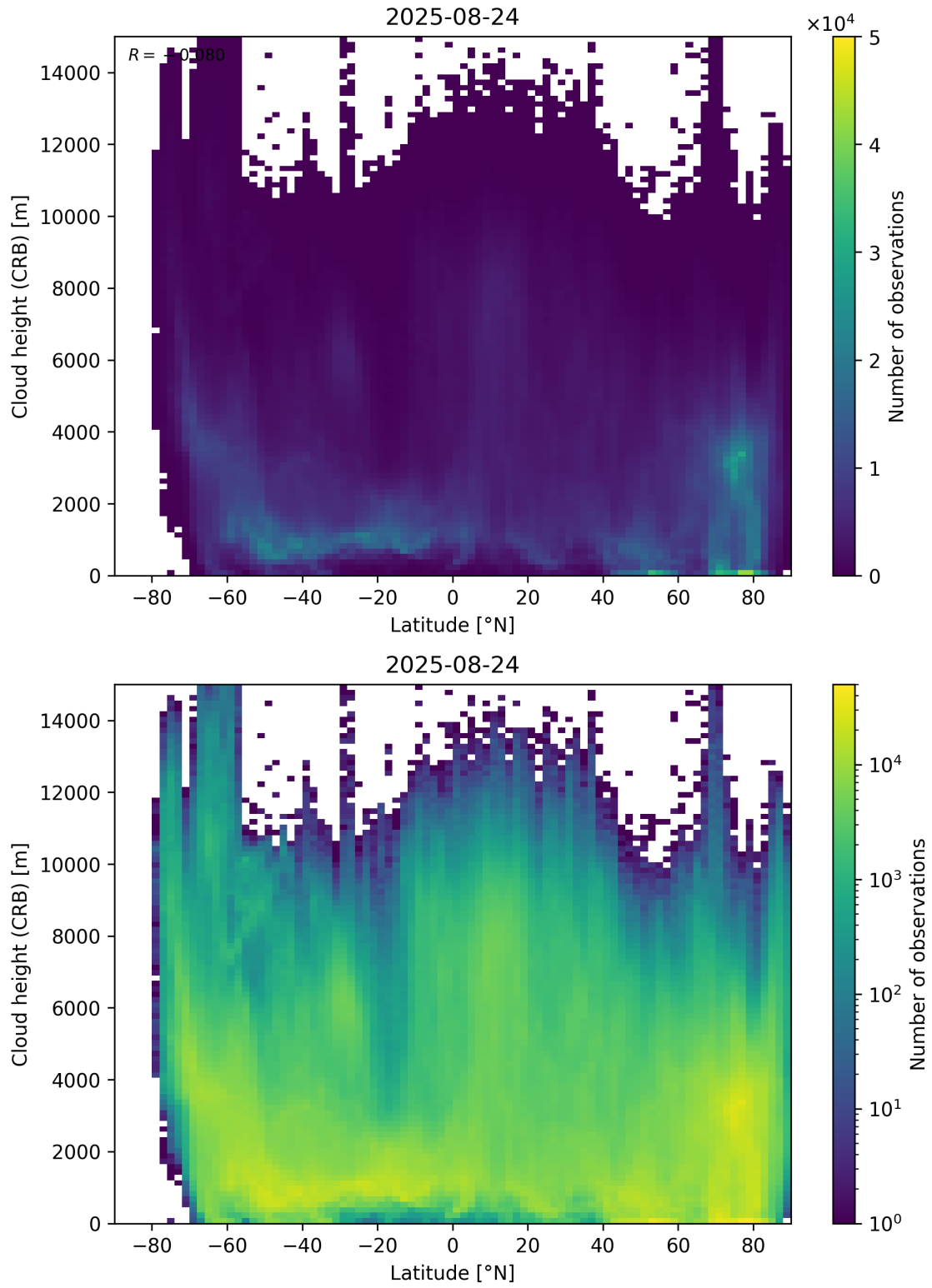
Figure 95: Scatter density plot of “Latitude” against “Cloud height (CRB)” for 2025-08-23 to 2025-08-25.
