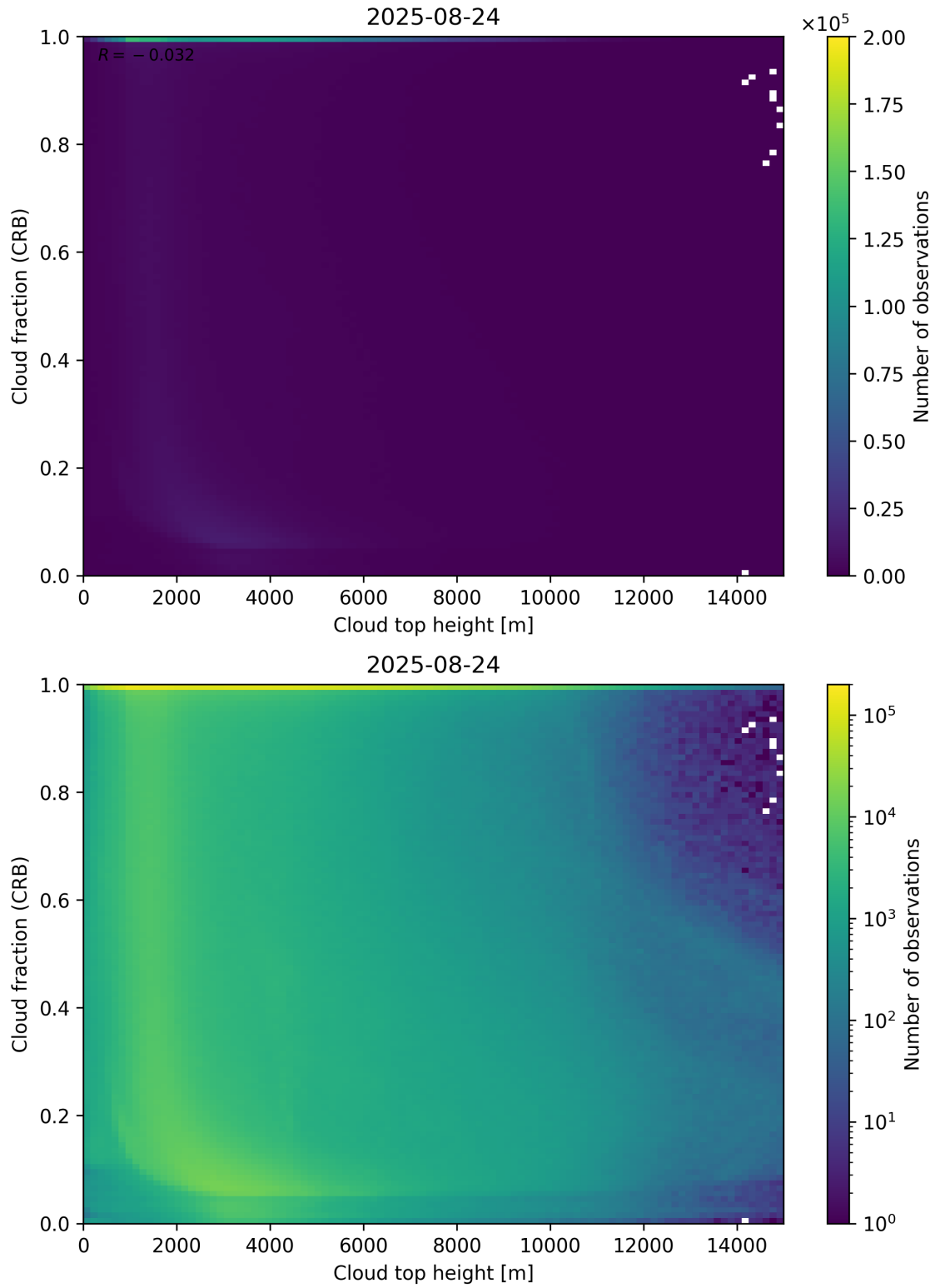
Figure 88: Scatter density plot of “Cloud top height” against “Cloud fraction (CRB)” for 2025-08-23 to 2025-08-25.
