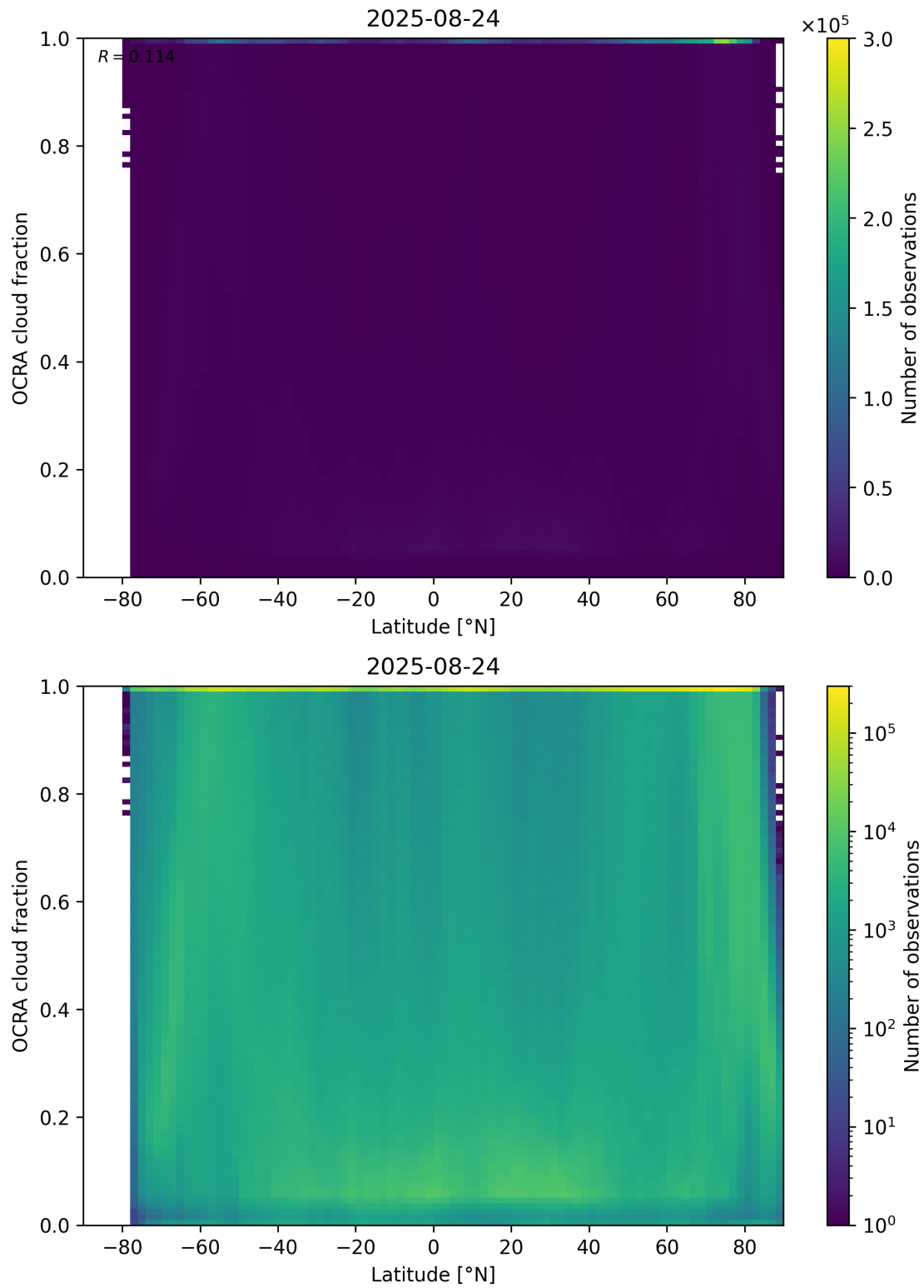
Figure 93: Scatter density plot of “Latitude” against “OCRA cloud fraction” for 2025-08-23 to 2025-08-25.
