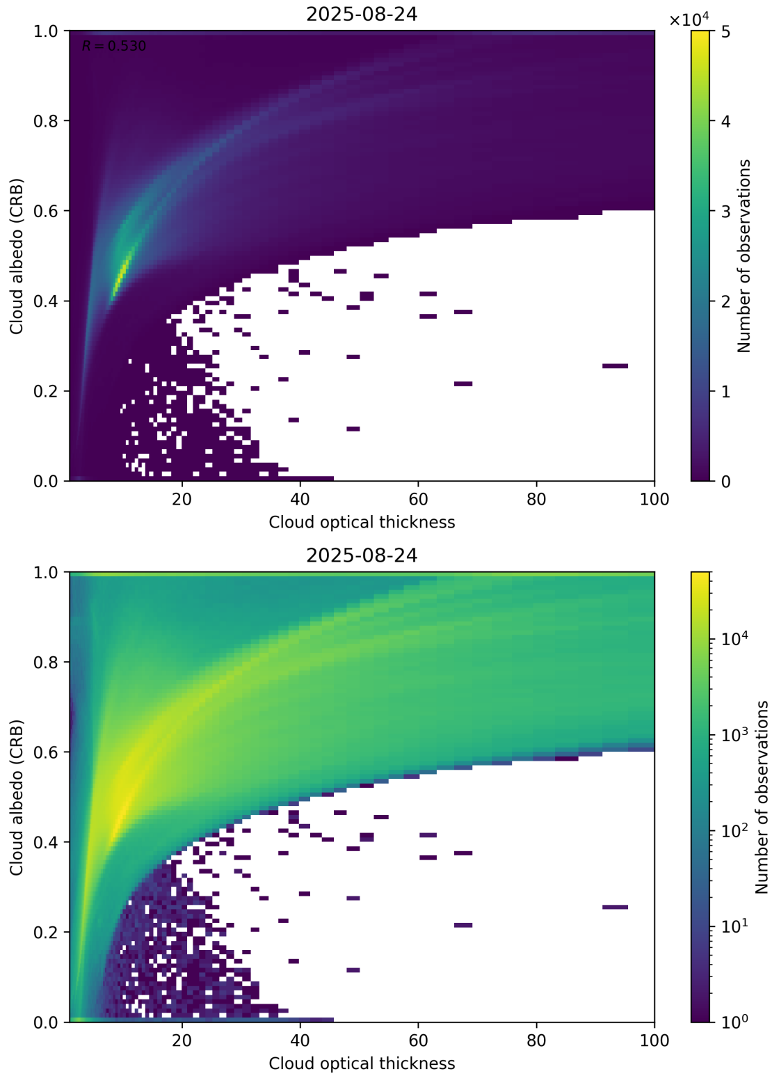
Figure 82: Scatter density plot of “Cloud optical thickness” against “Cloud albedo (CRB)” for 2025-08-23 to 2025-08-25.
