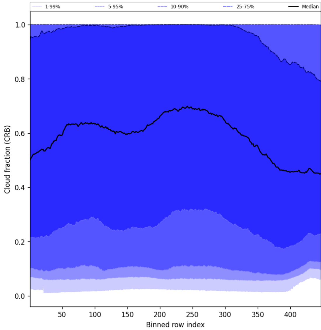
Figure 58: Along track statistics of “Cloud fraction (CRB)” for 2025-08-23 to 2025-08-25
