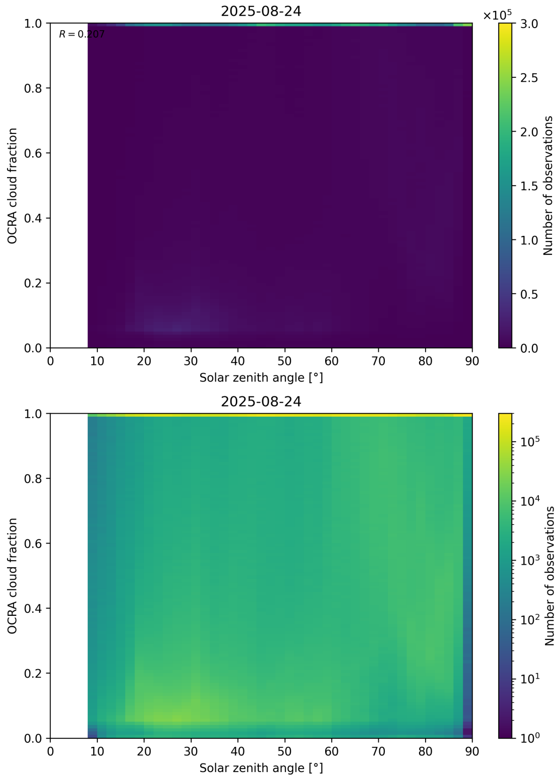
Figure 100: Scatter density plot of “Solar zenith angle” against “OCRA cloud fraction” for 2025-08-23 to 2025-08-25.
