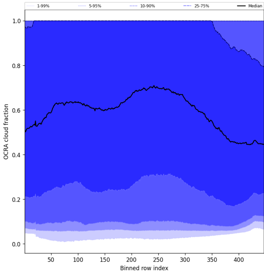
Figure 66: Along track statistics of “OCRA cloud fraction” for 2025-08-23 to 2025-08-25
