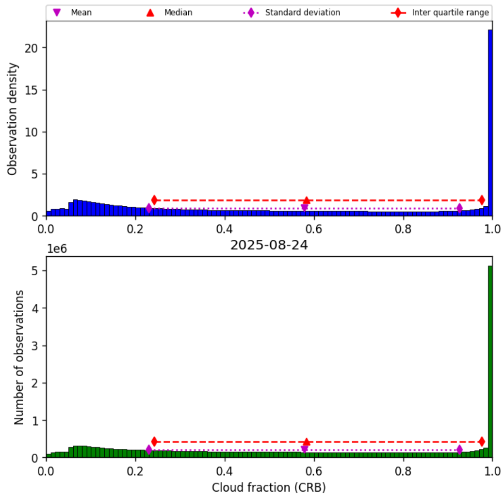
Figure 42: Histogram of “Cloud fraction (CRB)” for 2025-08-23 to 2025-08-25
