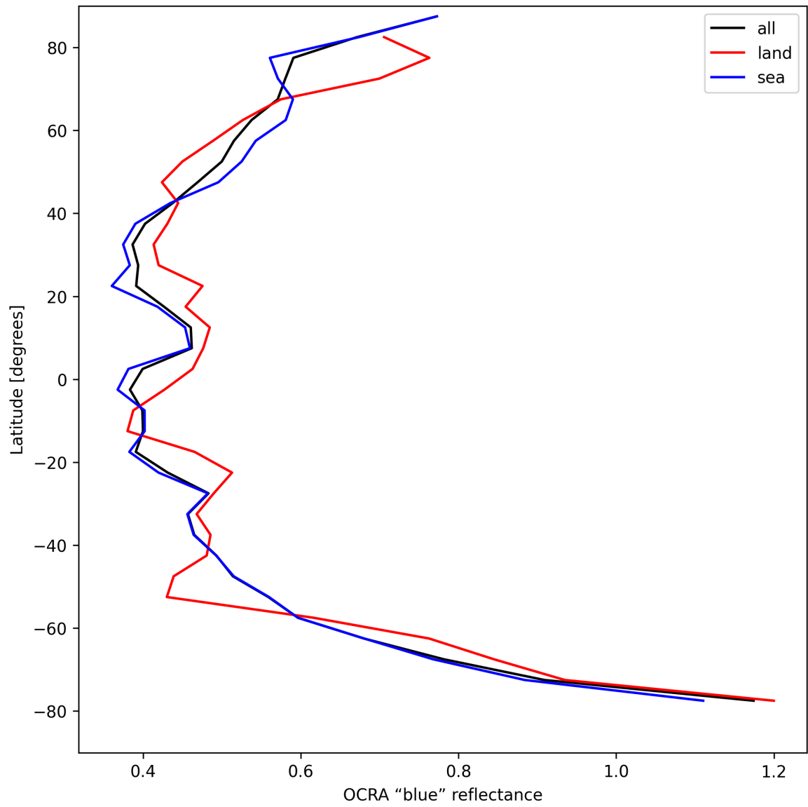
Figure 35: Zonal average of "OCRA "blue" reflectance" for 2025-08-23 to 2025-08-25.
