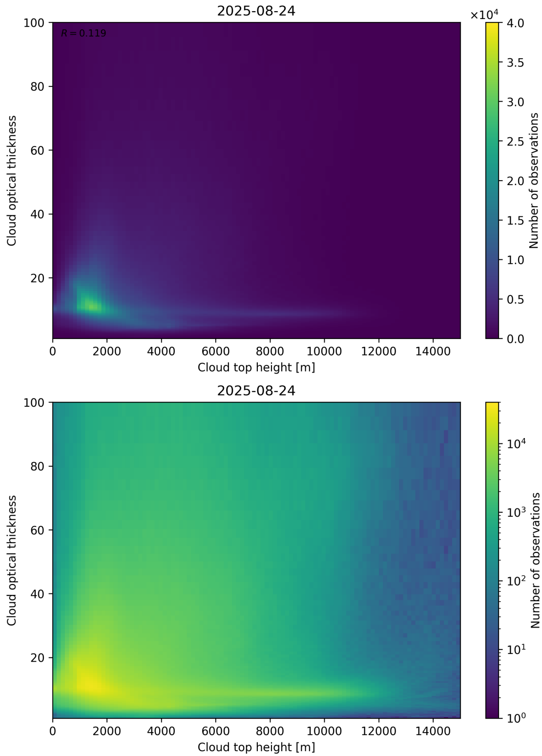
Figure 90: Scatter density plot of “Cloud top height” against “Cloud optical thickness” for 2025-08-23 to 2025-08-25.
