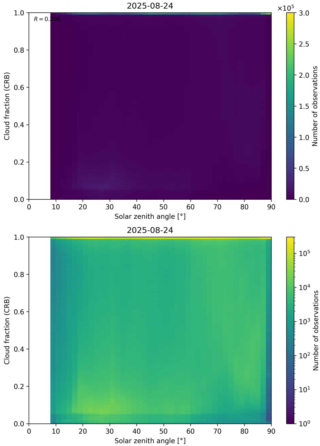
Figure 101: Scatter density plot of “Solar zenith angle” against “Cloud fraction (CRB)” for 2025-08-23 to 2025-08-25.
