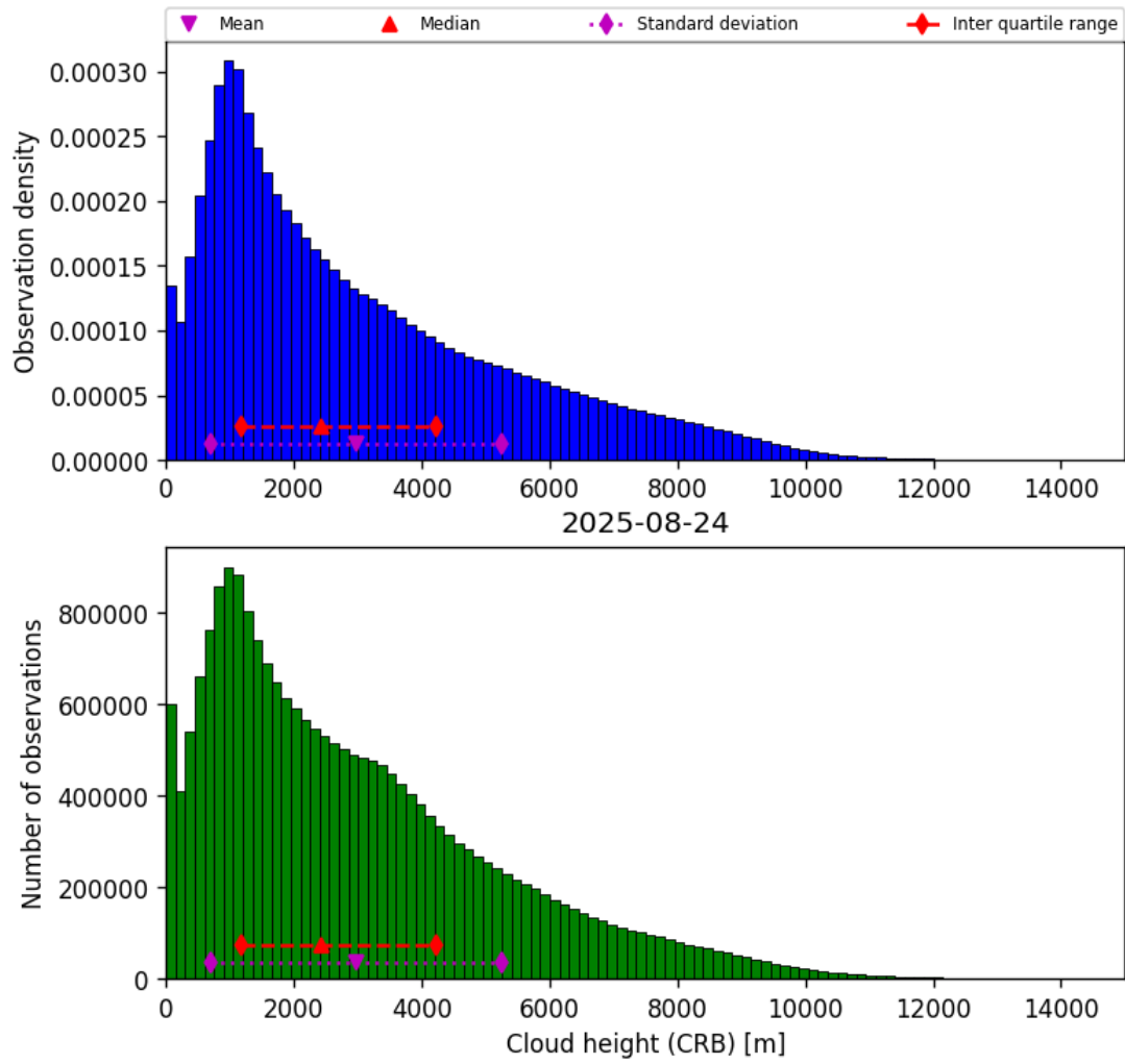
Figure 43: Histogram of “Cloud height (CRB)” for 2025-08-23 to 2025-08-25
