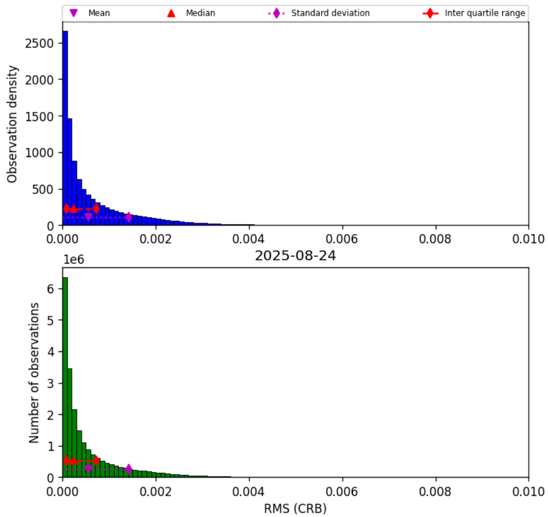
Figure 48: Histogram of “RMS (CRB)” for 2025-08-23 to 2025-08-25
