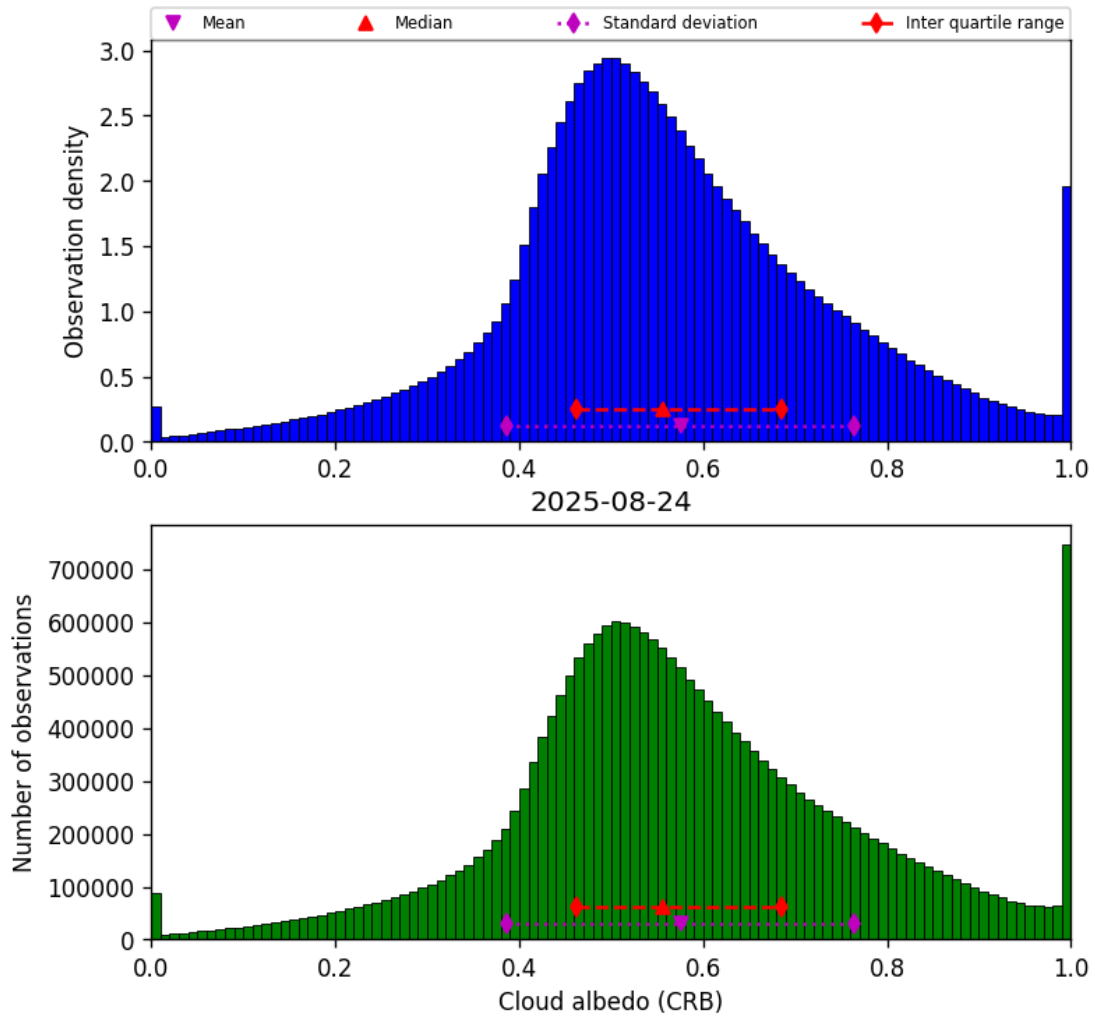
Figure 44: Histogram of “Cloud albedo (CRB)” for 2025-08-23 to 2025-08-25
