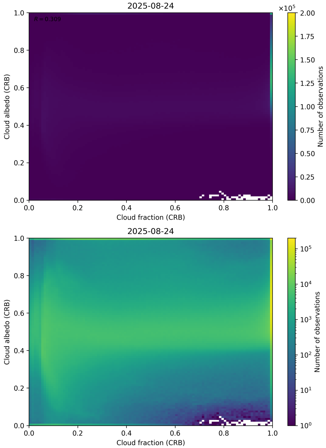
Figure 77: Scatter density plot of “Cloud fraction (CRB)” against “Cloud albedo (CRB)” for 2025-08-23 to 2025-08-25.
