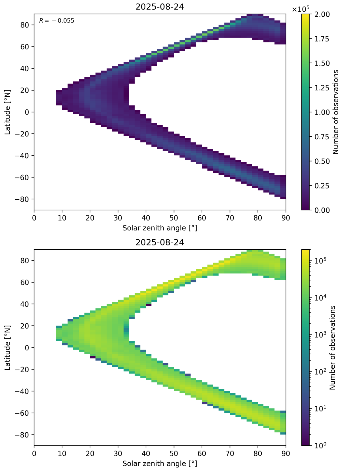
Figure 105: Scatter density plot of “Solar zenith angle” against “Latitude” for 2025-08-23 to 2025-08-25.
