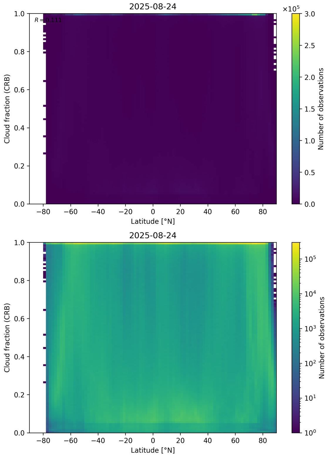
Figure 94: Scatter density plot of “Latitude” against “Cloud fraction (CRB)” for 2025-08-23 to 2025-08-25.
