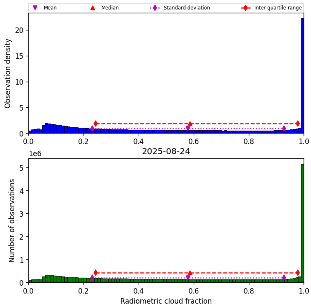
Figure 39: Histogram of “Radiometric cloud fraction” for 2025-08-23 to 2025-08-25
