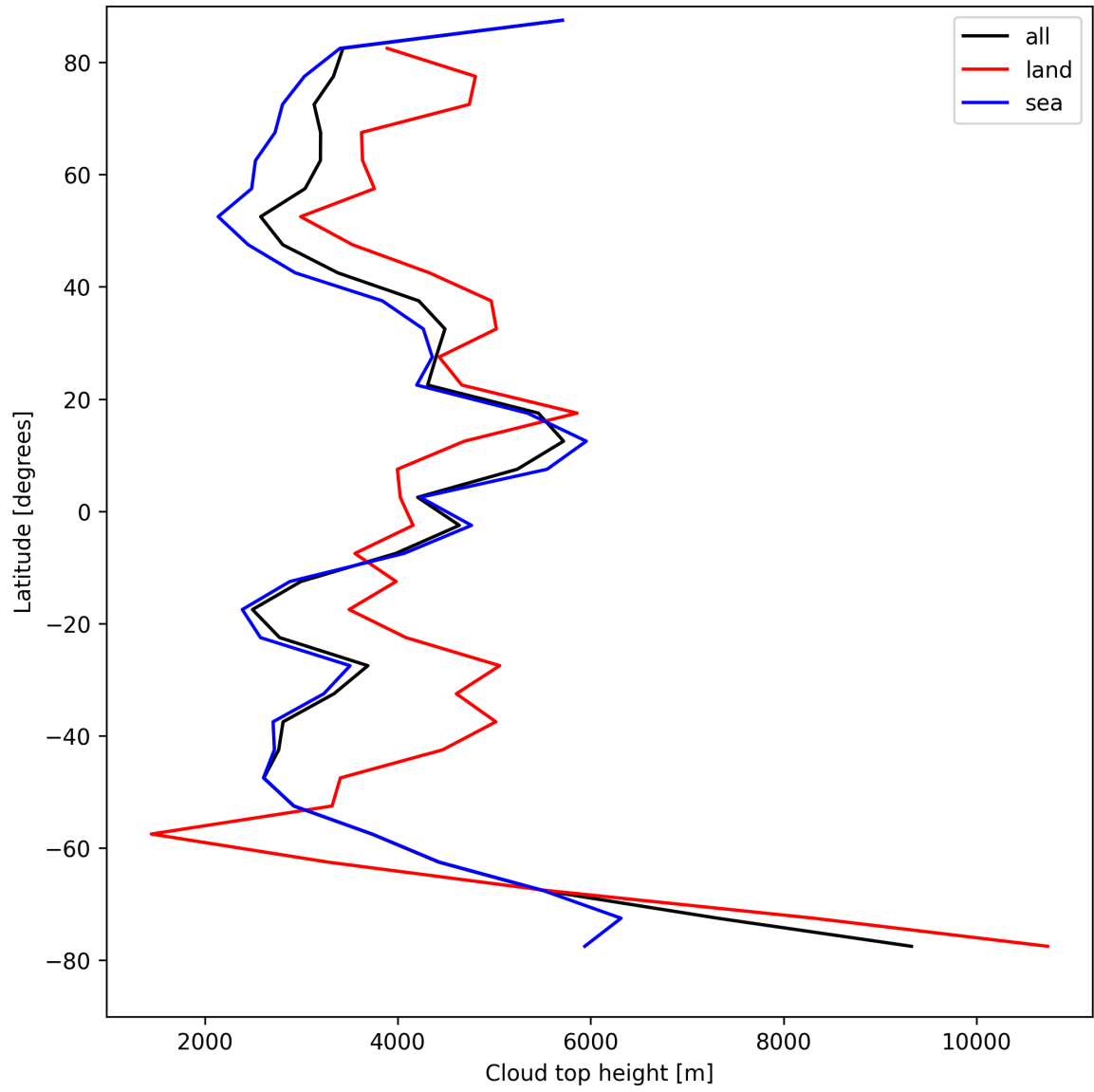
Figure 24: Zonal average of “Cloud top height” for 2025-08-23 to 2025-08-25.
