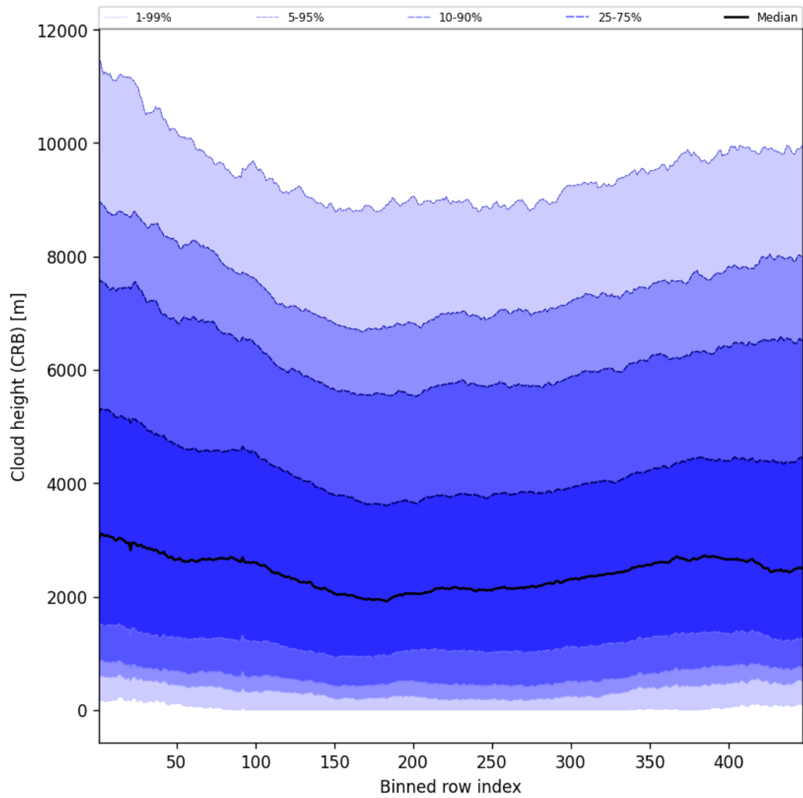
Figure 59: Along track statistics of “Cloud height (CRB)” for 2025-08-23 to 2025-08-25
