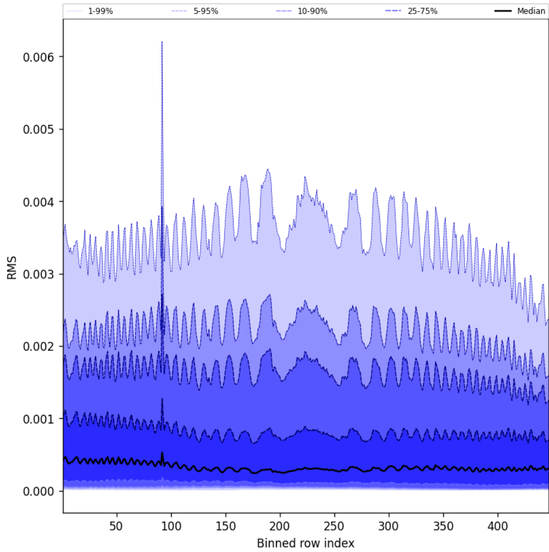
Figure 63: Along track statistics of “RMS” for 2025-08-23 to 2025-08-25
