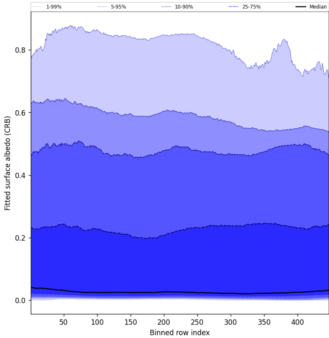
Figure 62: Along track statistics of “Fitted surface albedo (CRB)” for 2025-08-23 to 2025-08-25
