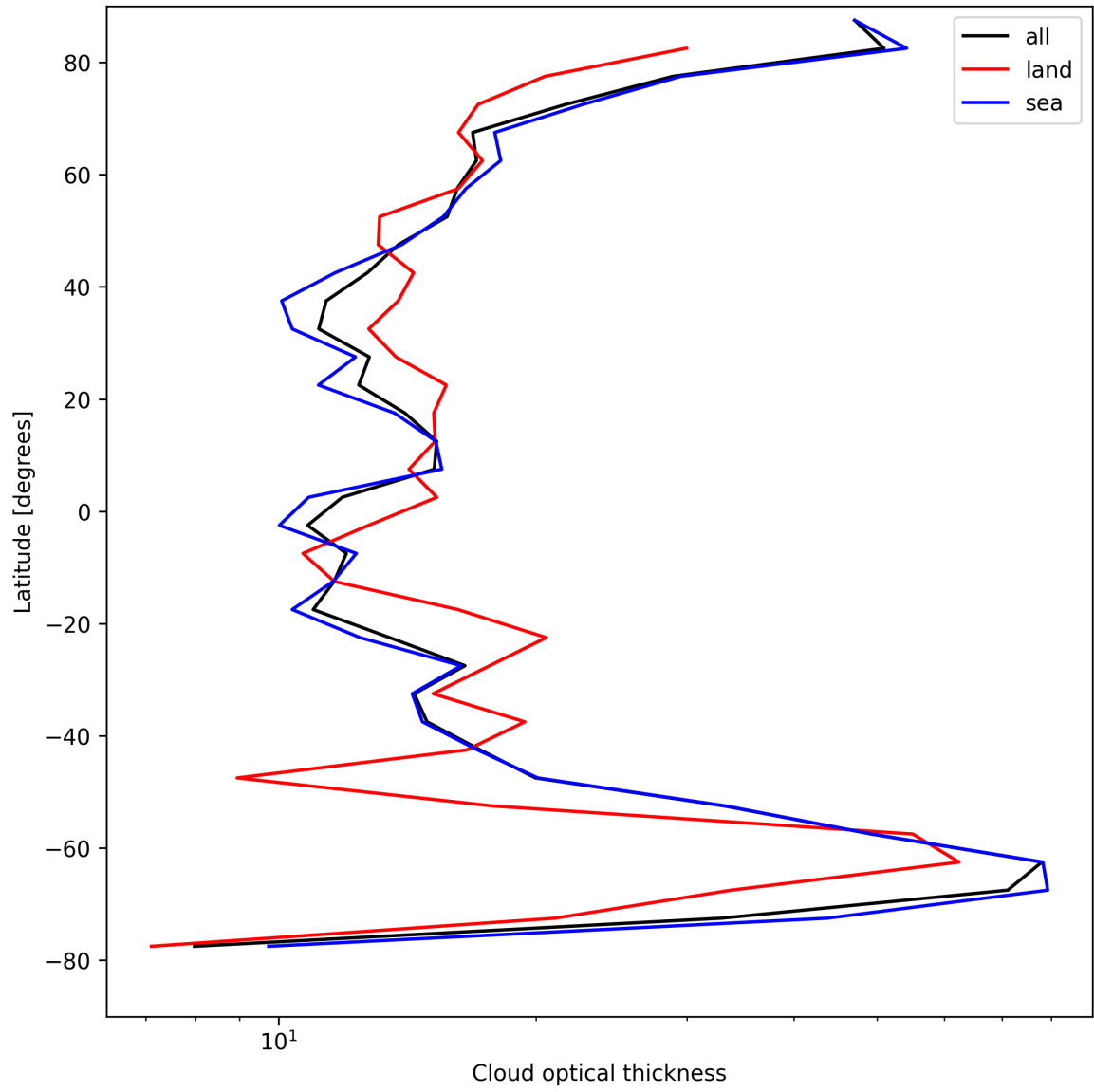
Figure 25: Zonal average of “Cloud optical thickness” for 2025-08-23 to 2025-08-25.
