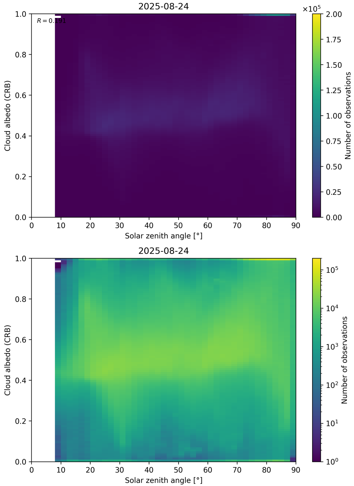
Figure 98: Scatter density plot of “Solar zenith angle” against “Cloud albedo (CRB)” for 2025-08-23 to 2025-08-25.
