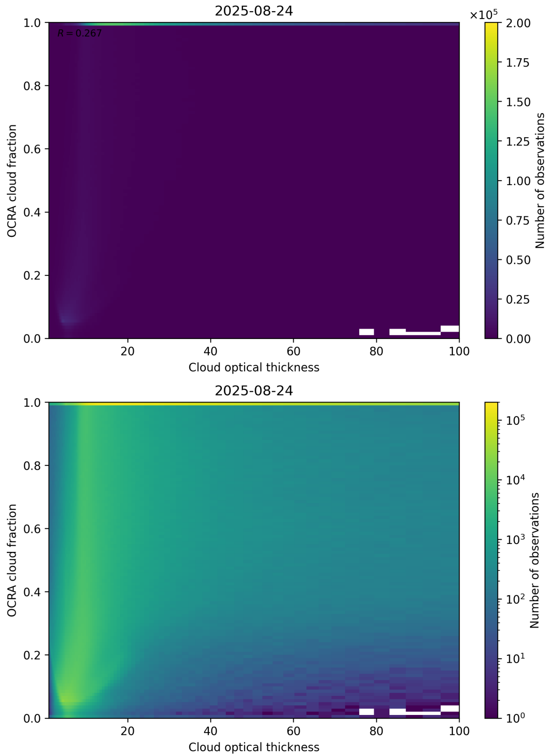
Figure 83: Scatter density plot of “Cloud optical thickness” against “OCRA cloud fraction” for 2025-08-23 to 2025-08-25.
