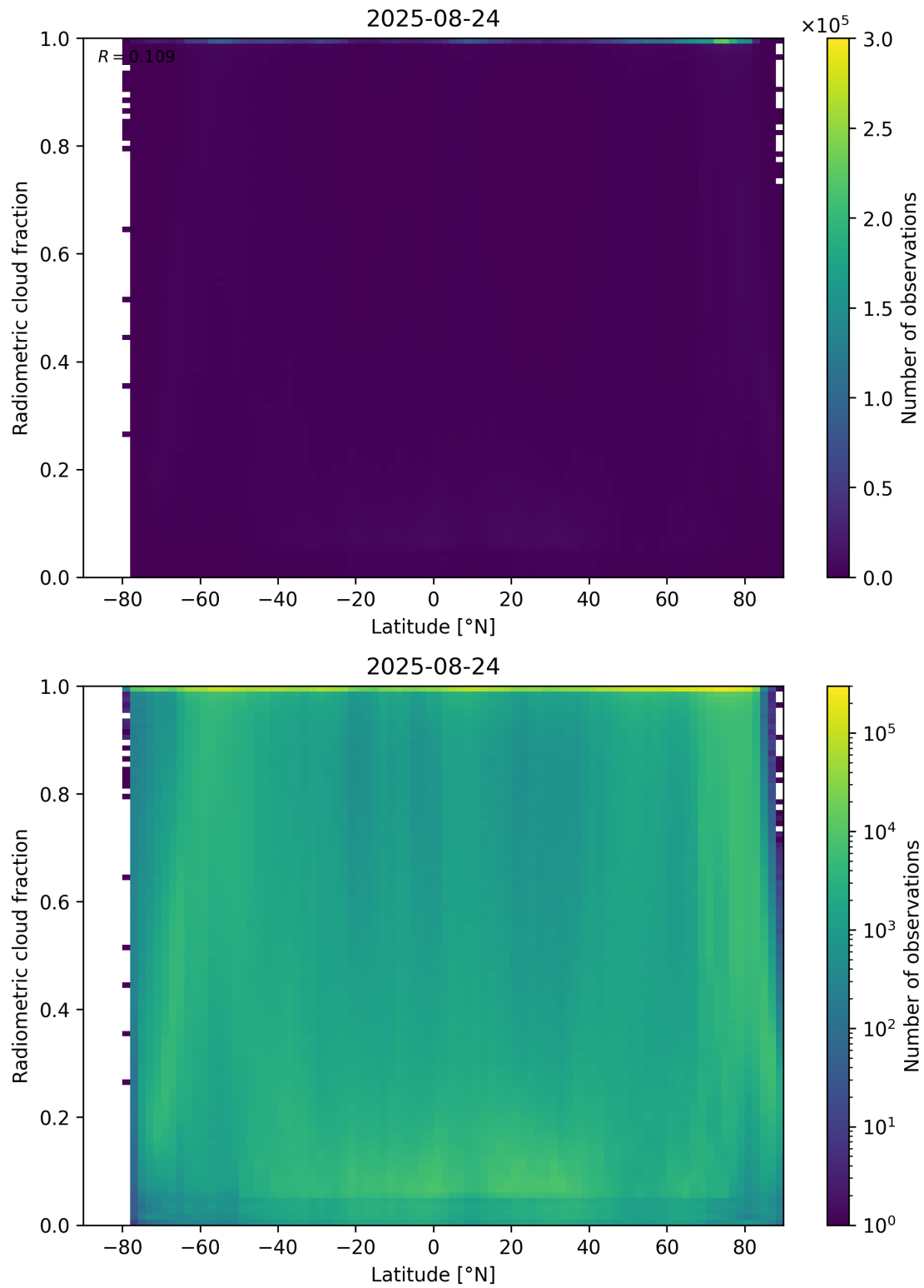
Figure 92: Scatter density plot of “Latitude” against “Radiometric cloud fraction” for 2025-08-23 to 2025-08-25.
