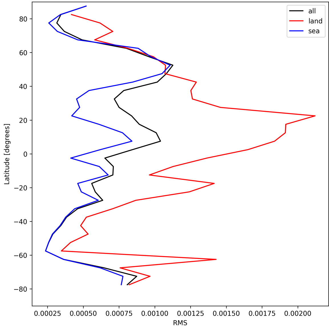
Figure 31: Zonal average of “RMS” for 2025-08-23 to 2025-08-25.
