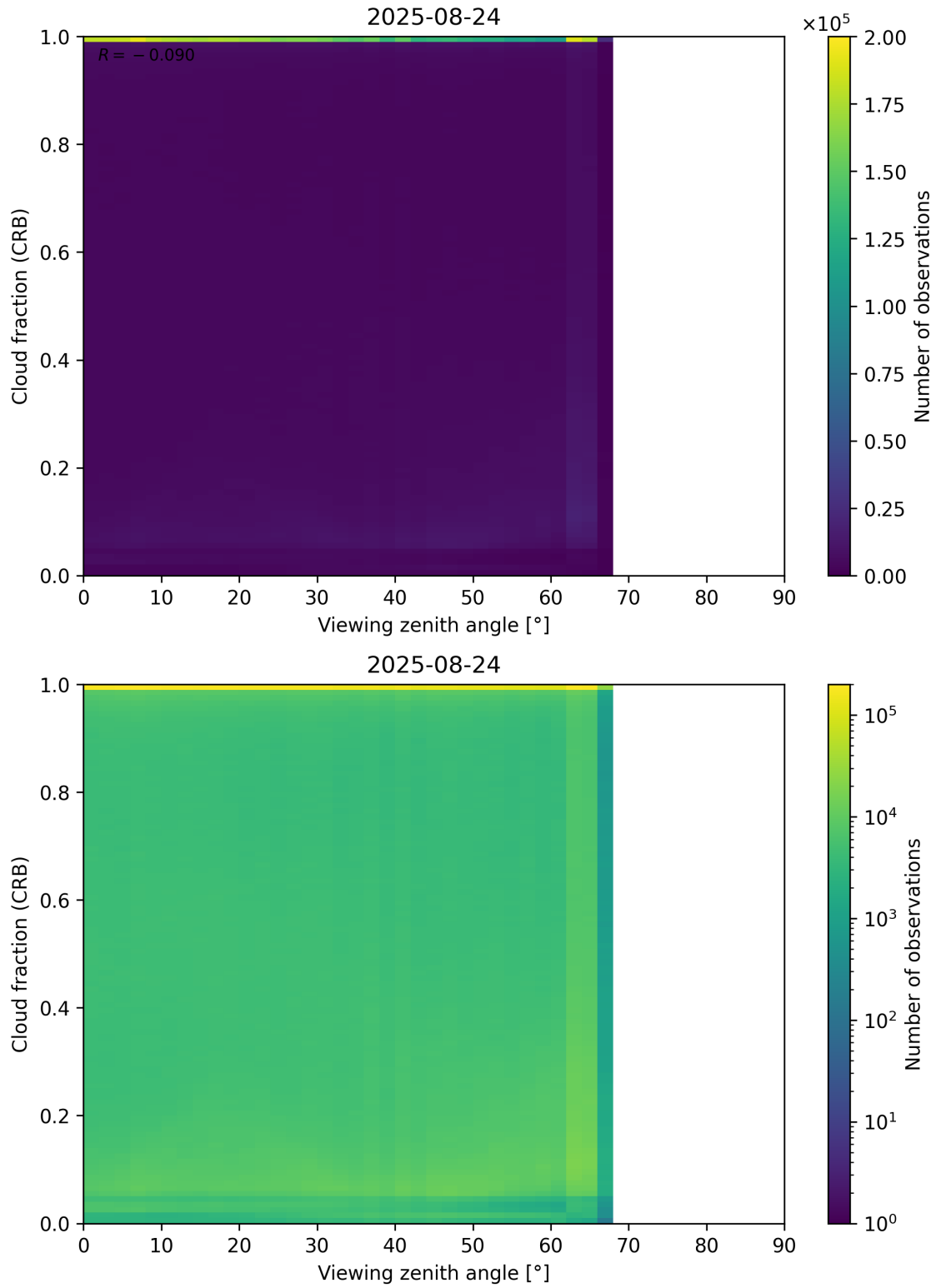
Figure 109: Scatter density plot of “Viewing zenith angle” against “Cloud fraction (CRB)” for 2025-08-23 to 2025-08-25.
