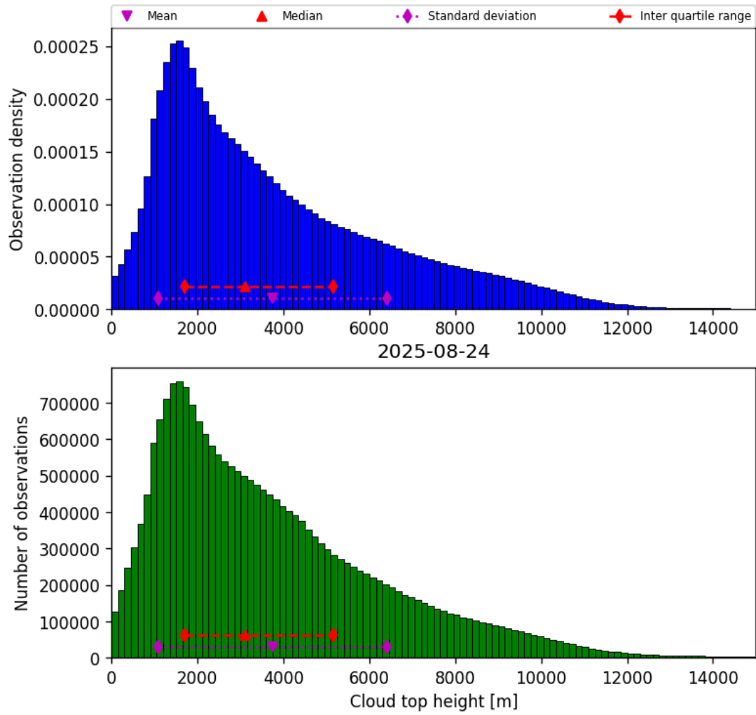
Figure 40: Histogram of “Cloud top height” for 2025-08-23 to 2025-08-25
