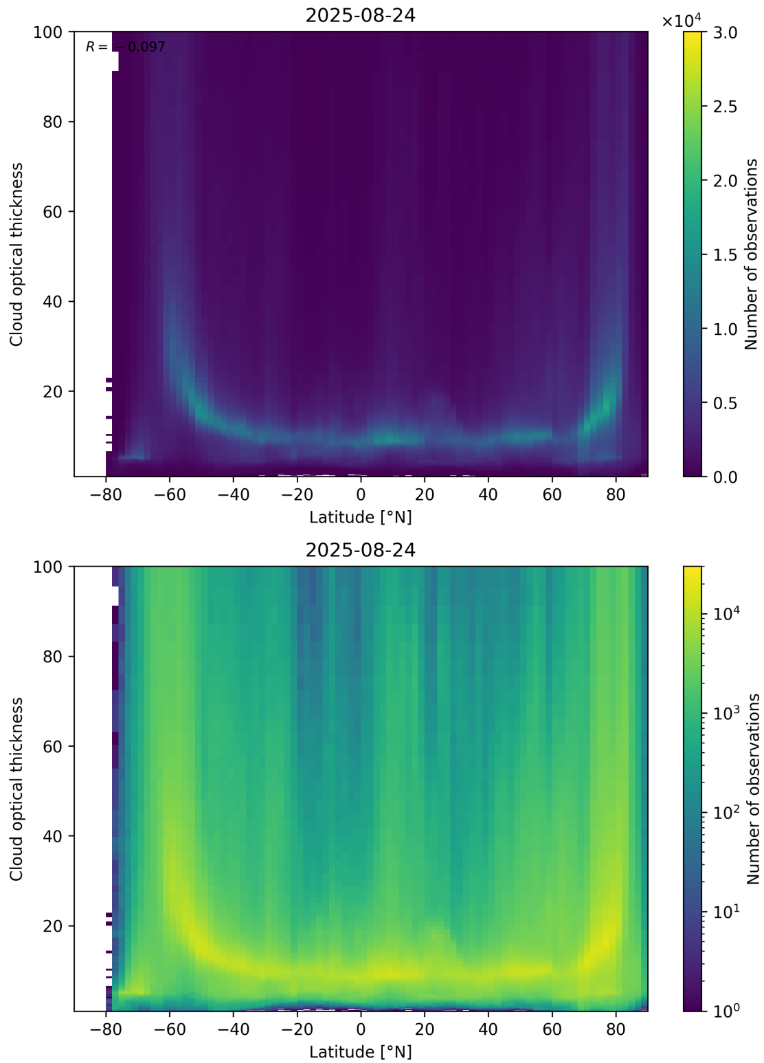
Figure 96: Scatter density plot of “Latitude” against “Cloud optical thickness” for 2025-08-23 to 2025-08-25.
