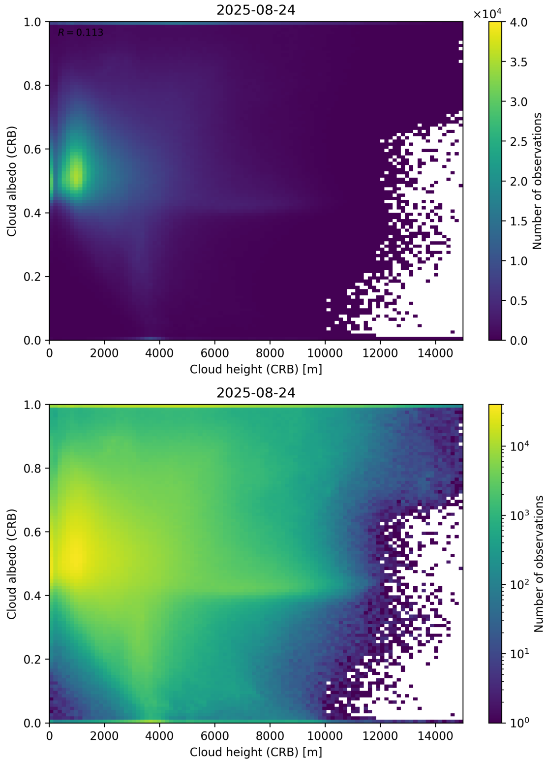
Figure 80: Scatter density plot of “Cloud height (CRB)” against “Cloud albedo (CRB)” for 2025-08-23 to 2025-08-25.
