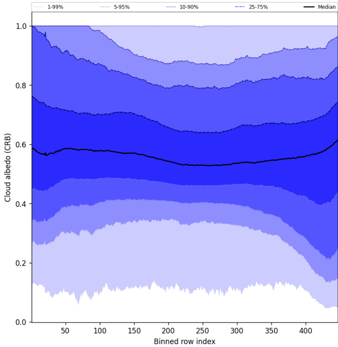
Figure 60: Along track statistics of “Cloud albedo (CRB)” for 2025-08-23 to 2025-08-25
