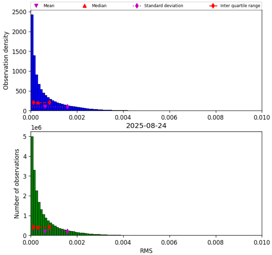
Figure 47: Histogram of “RMS” for 2025-08-23 to 2025-08-25
