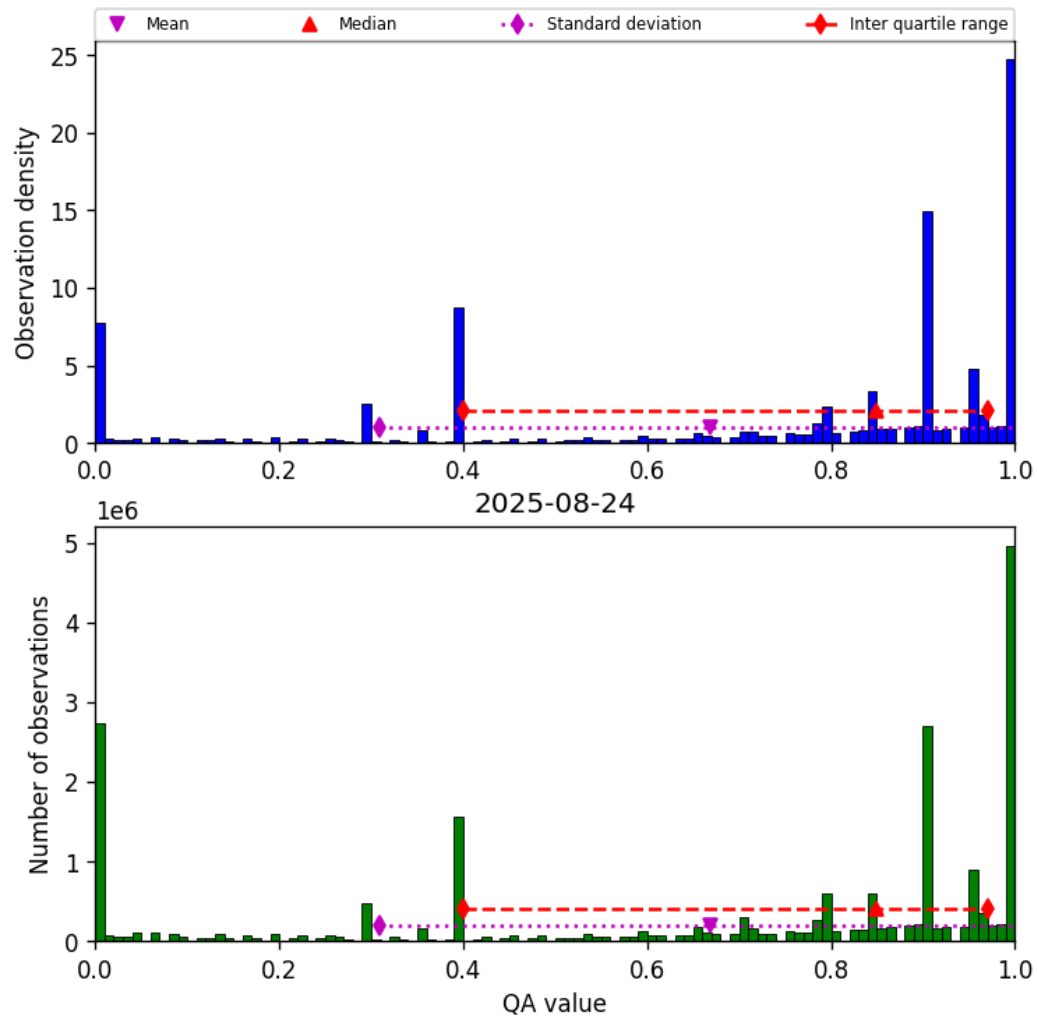
Figure 38: Histogram of “QA value” for 2025-08-23 to 2025-08-25
