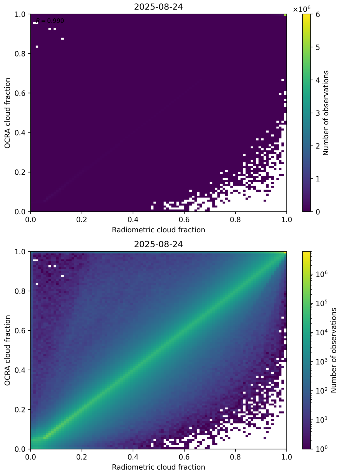
Figure 72: Scatter density plot of “Radiometric cloud fraction” against “OCRA cloud fraction” for 2025-08-23 to 2025-08-25.
