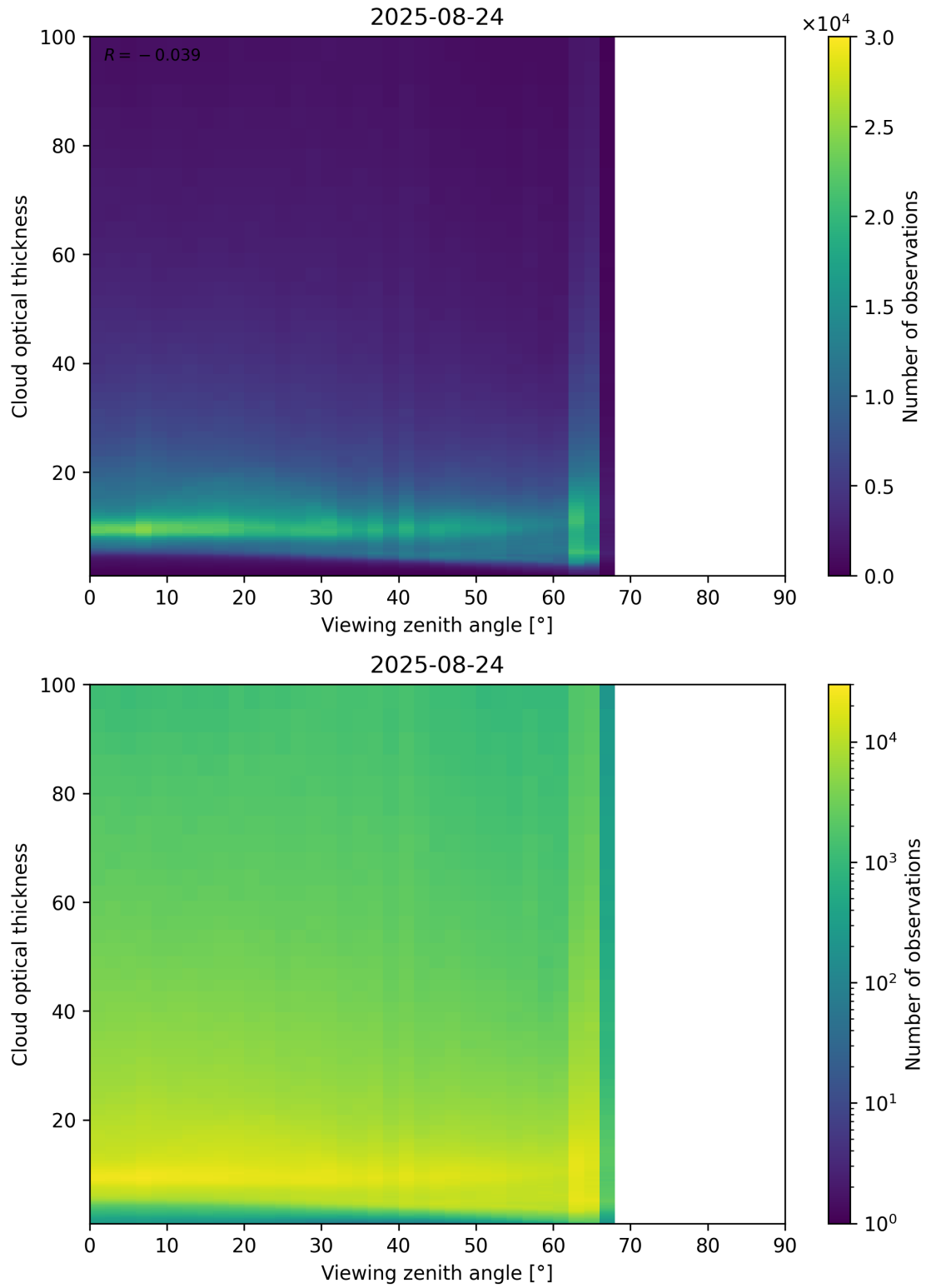
Figure 111: Scatter density plot of “Viewing zenith angle” against “Cloud optical thickness” for 2025-08-23 to 2025-08-25.
