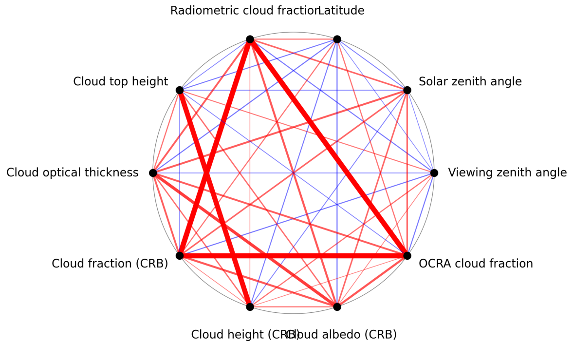
Figure 1: Map of correlation graph for 2025-08-23 to 2025-08-25.
