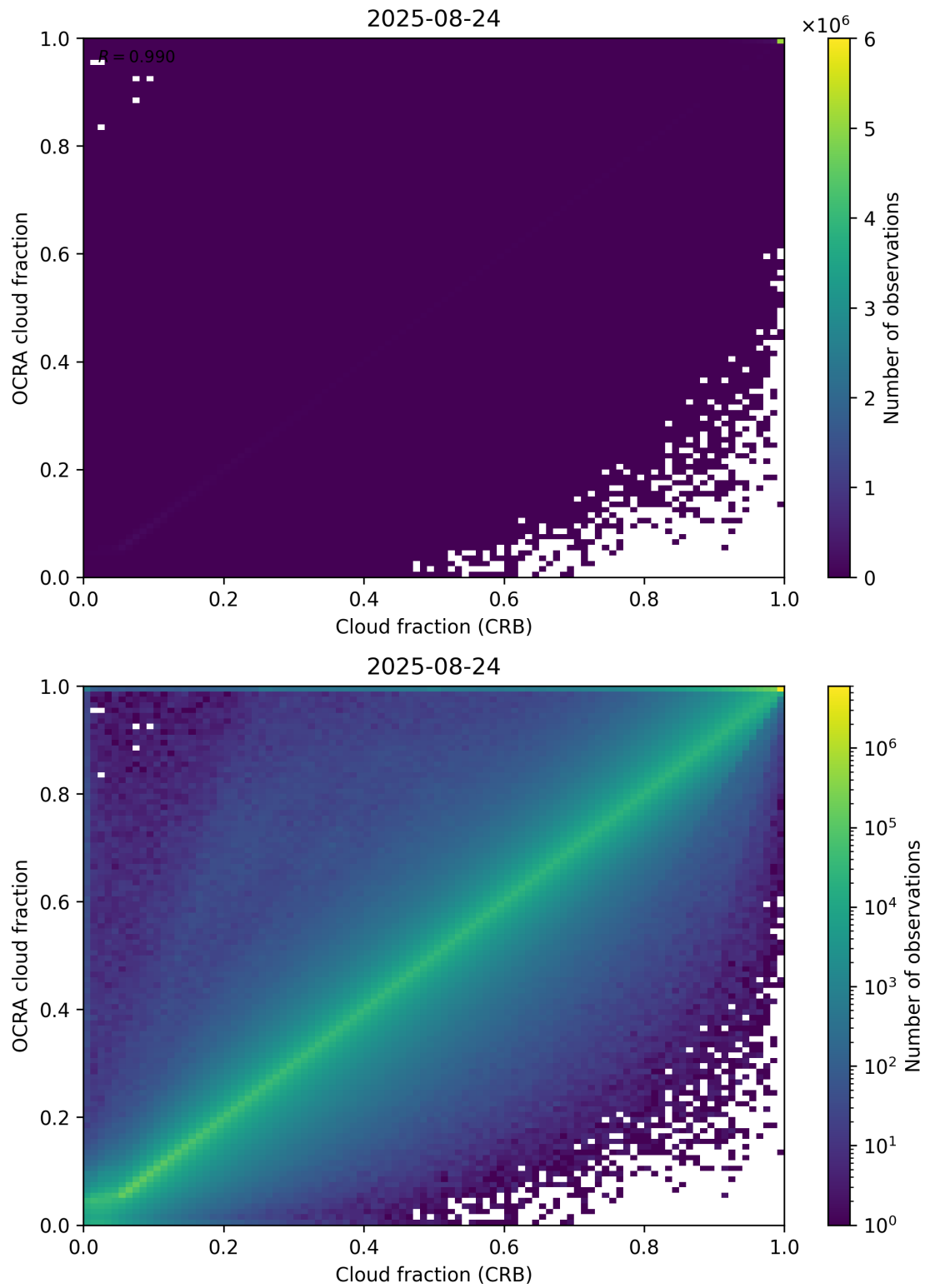
Figure 78: Scatter density plot of “Cloud fraction (CRB)” against “OCRA cloud fraction” for 2025-08-23 to 2025-08-25.
