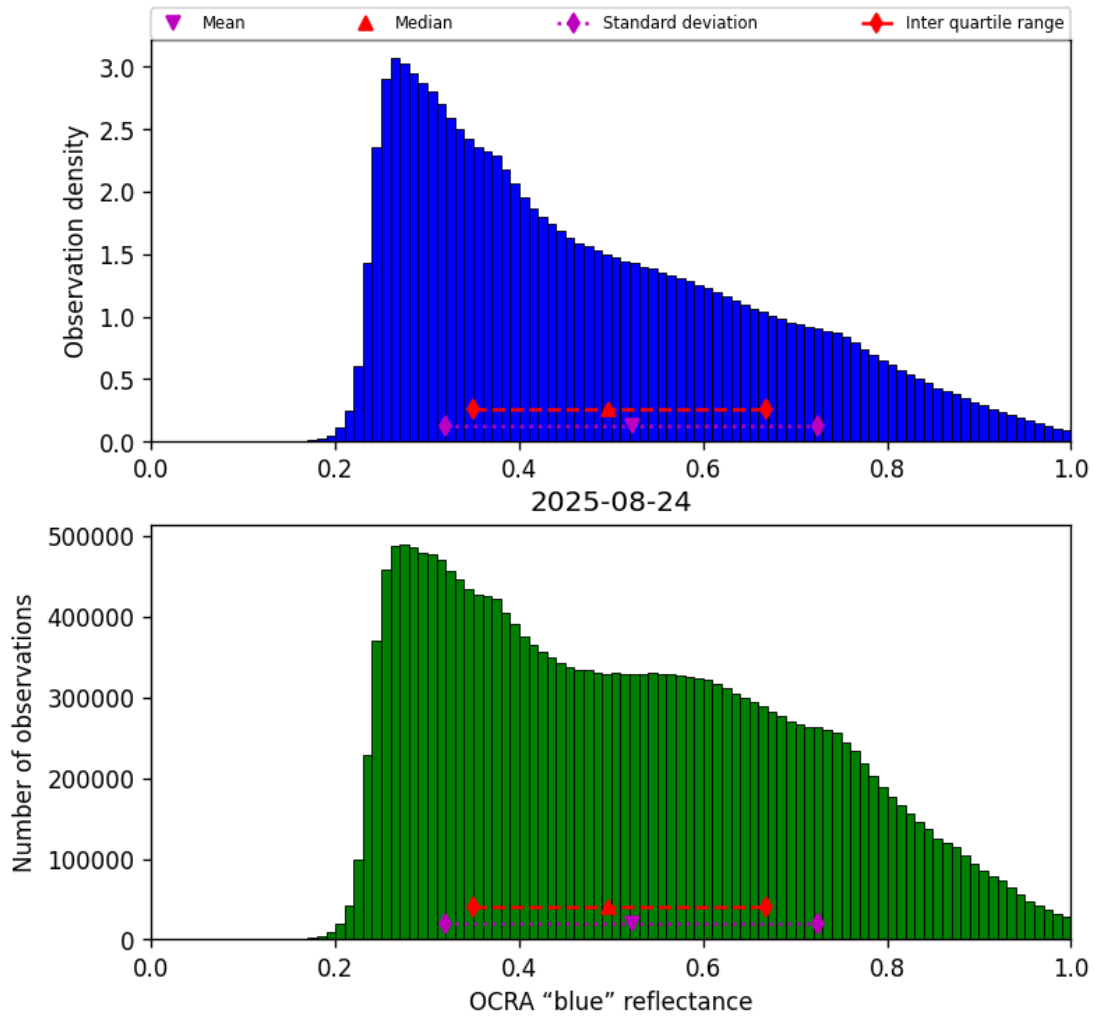
Figure 51: Histogram of “OCRA “blue” reflectance” for 2025-08-23 to 2025-08-25
