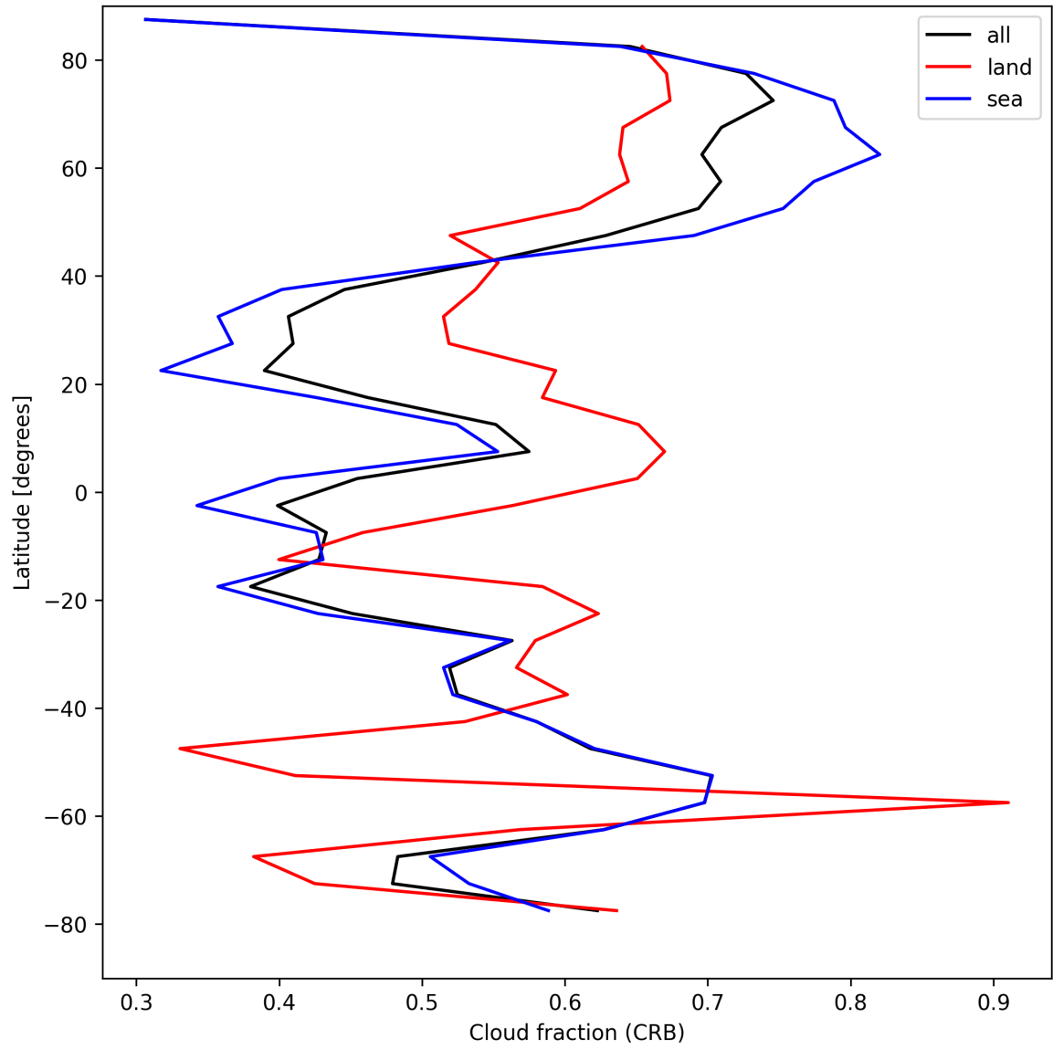
Figure 26: Zonal average of “Cloud fraction (CRB)” for 2025-08-23 to 2025-08-25.
