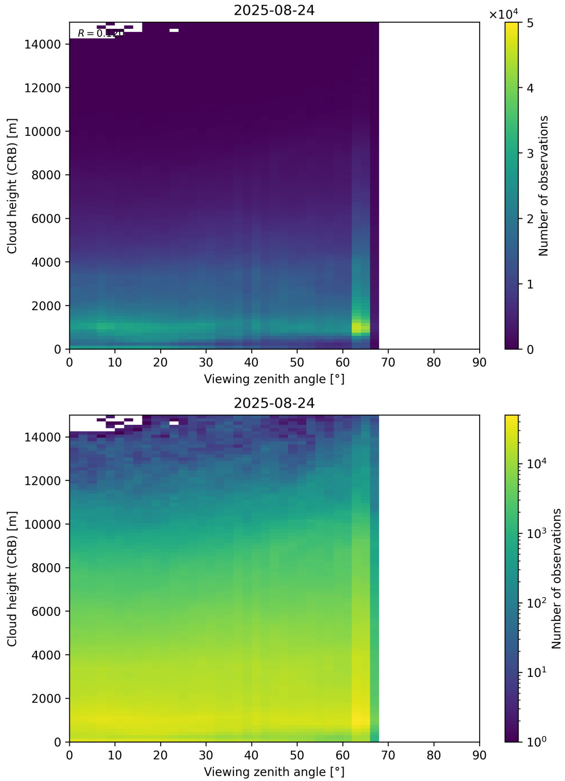
Figure 110: Scatter density plot of “Viewing zenith angle” against “Cloud height (CRB)” for 2025-08-23 to 2025-08-25.
