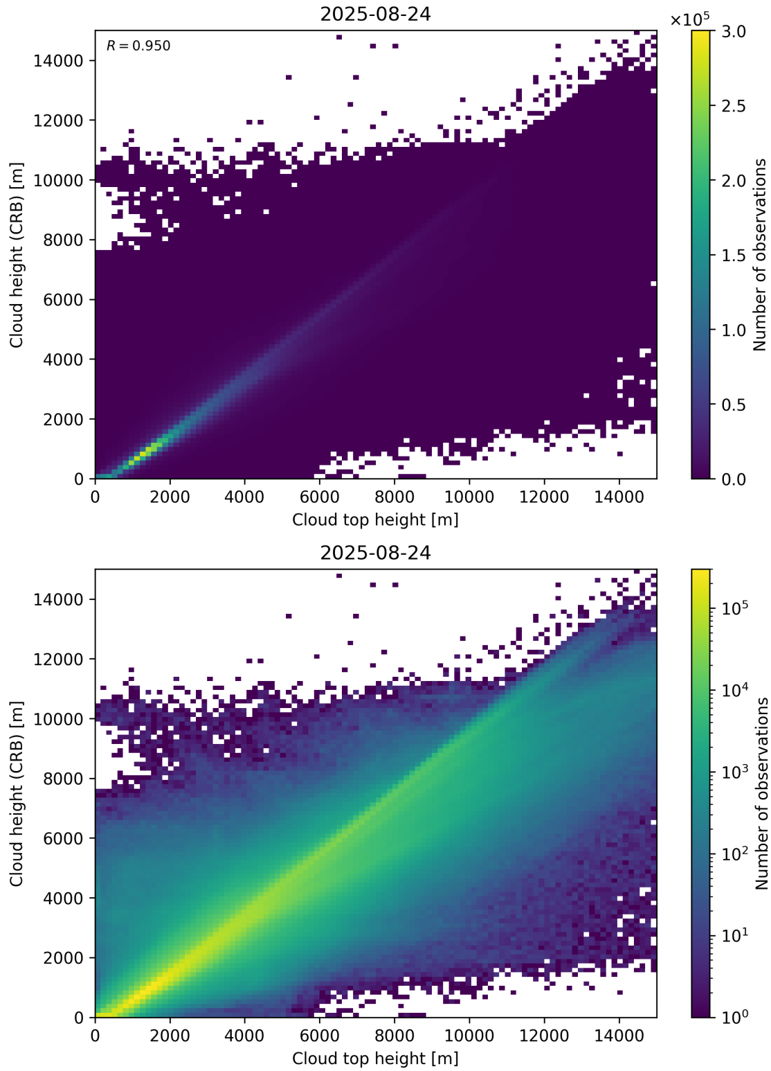
Figure 89: Scatter density plot of “Cloud top height” against “Cloud height (CRB)” for 2025-08-23 to 2025-08-25.
