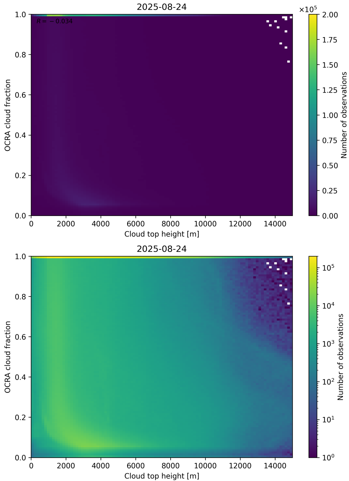
Figure 87: Scatter density plot of “Cloud top height” against “OCRA cloud fraction” for 2025-08-23 to 2025-08-25.
