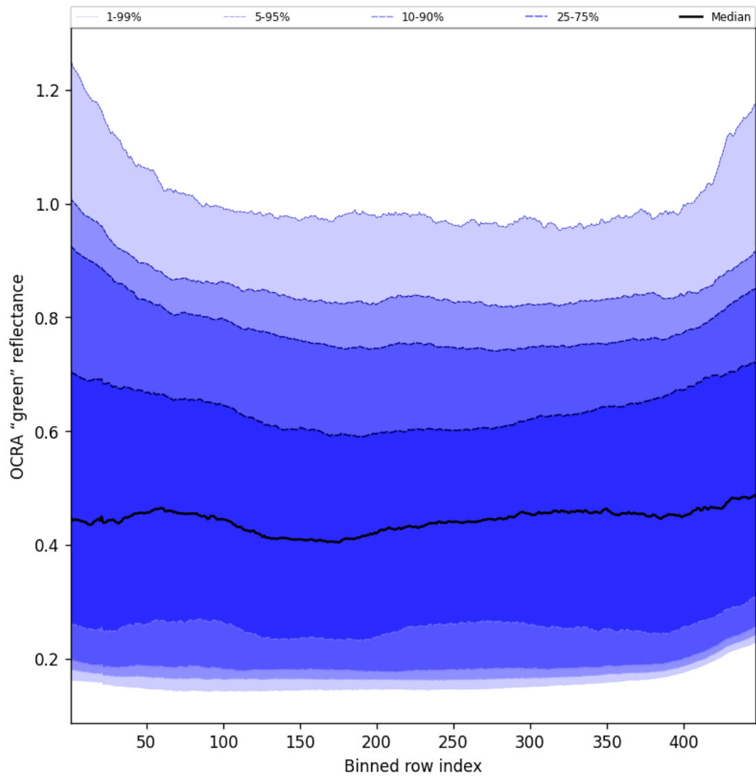
Figure 68: Along track statistics of "OCRA "green" reflectance" for 2025-08-23 to 2025-08-25
