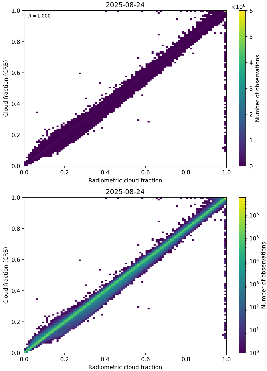
Figure 73: Scatter density plot of “Radiometric cloud fraction” against “Cloud fraction (CRB)” for 2025-08-23 to 2025-08-25.
