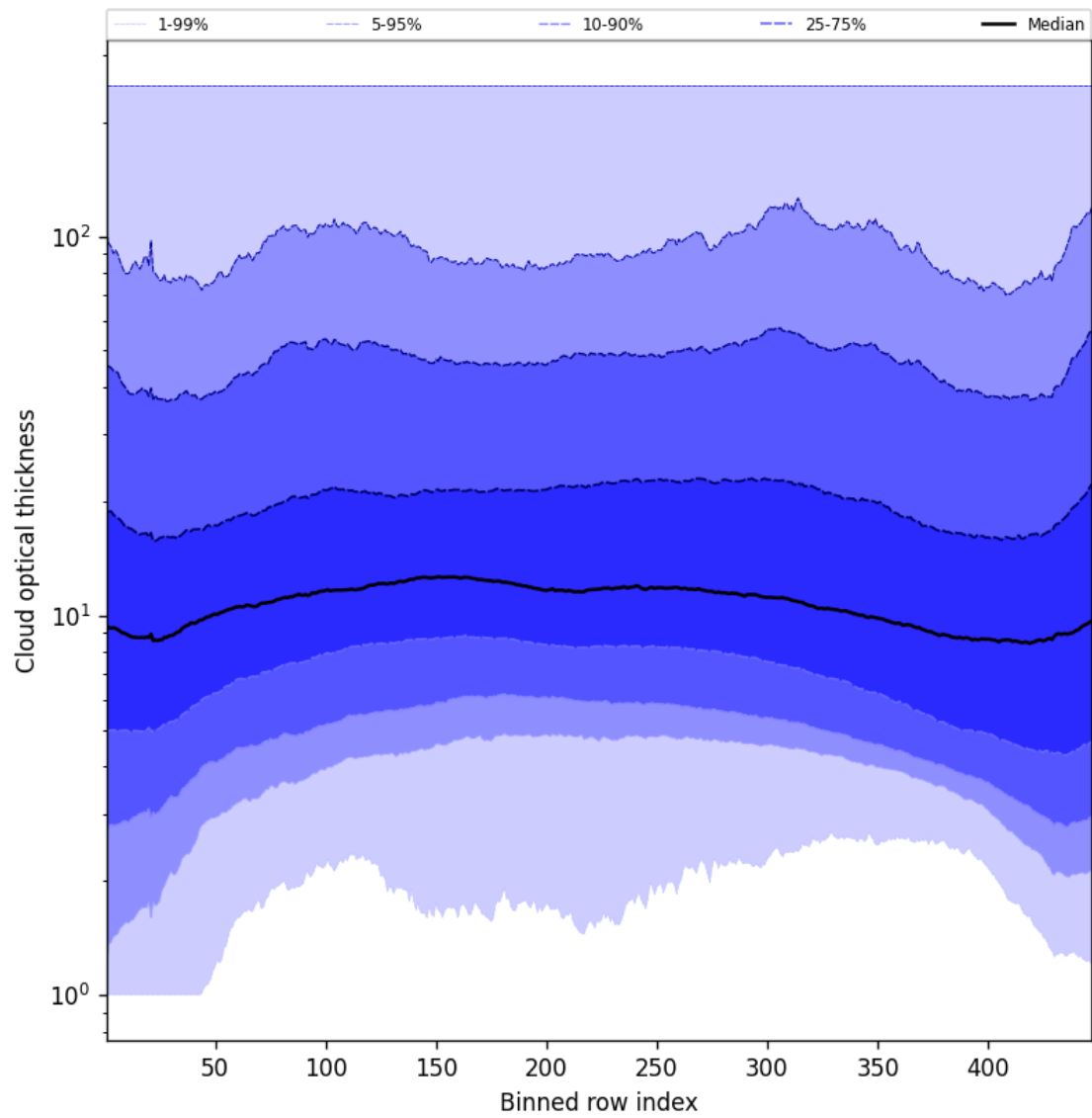
Figure 57: Along track statistics of “Cloud optical thickness” for 2025-08-23 to 2025-08-25
