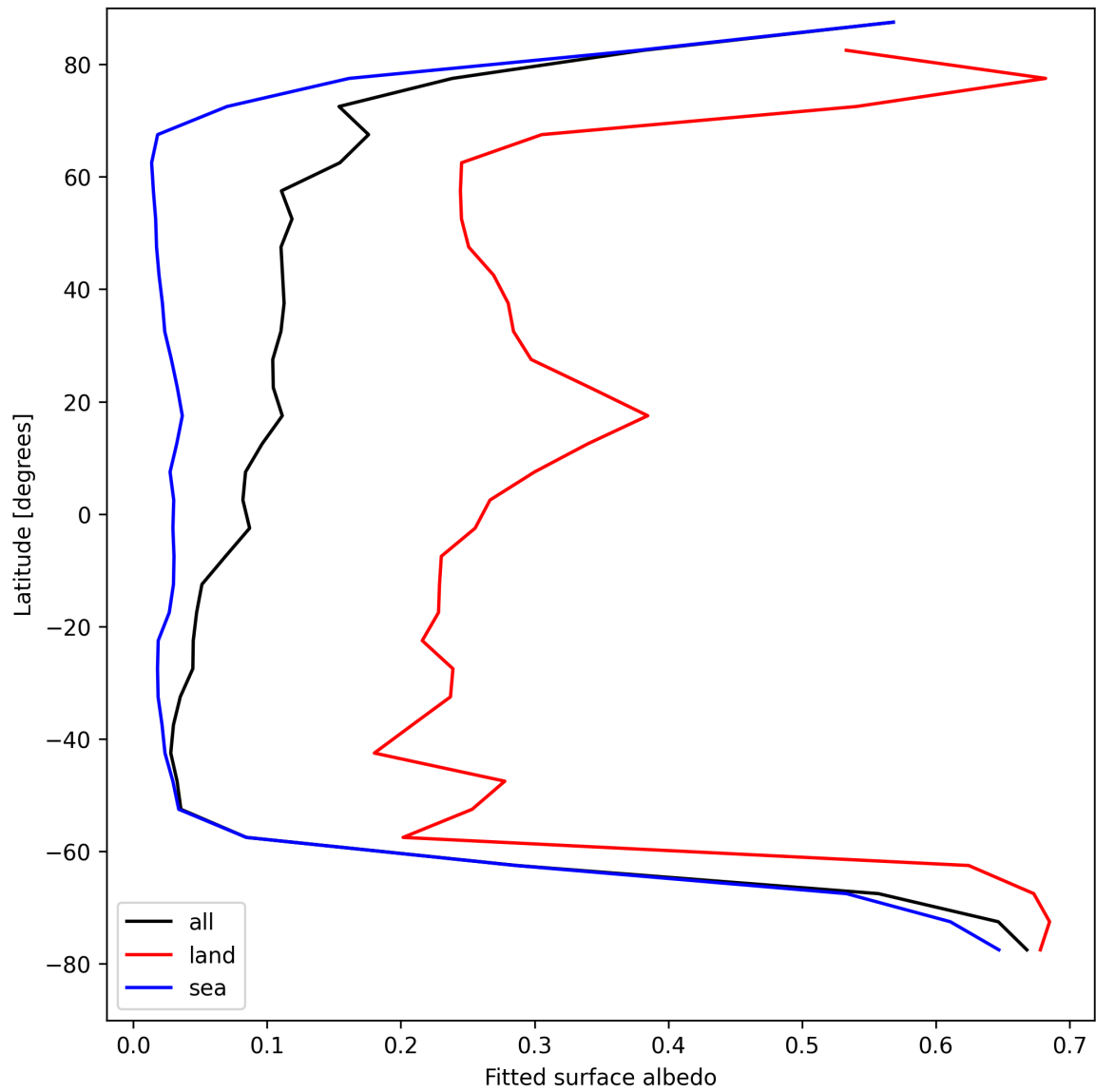
Figure 29: Zonal average of “Fitted surface albedo” for 2025-08-23 to 2025-08-25.
