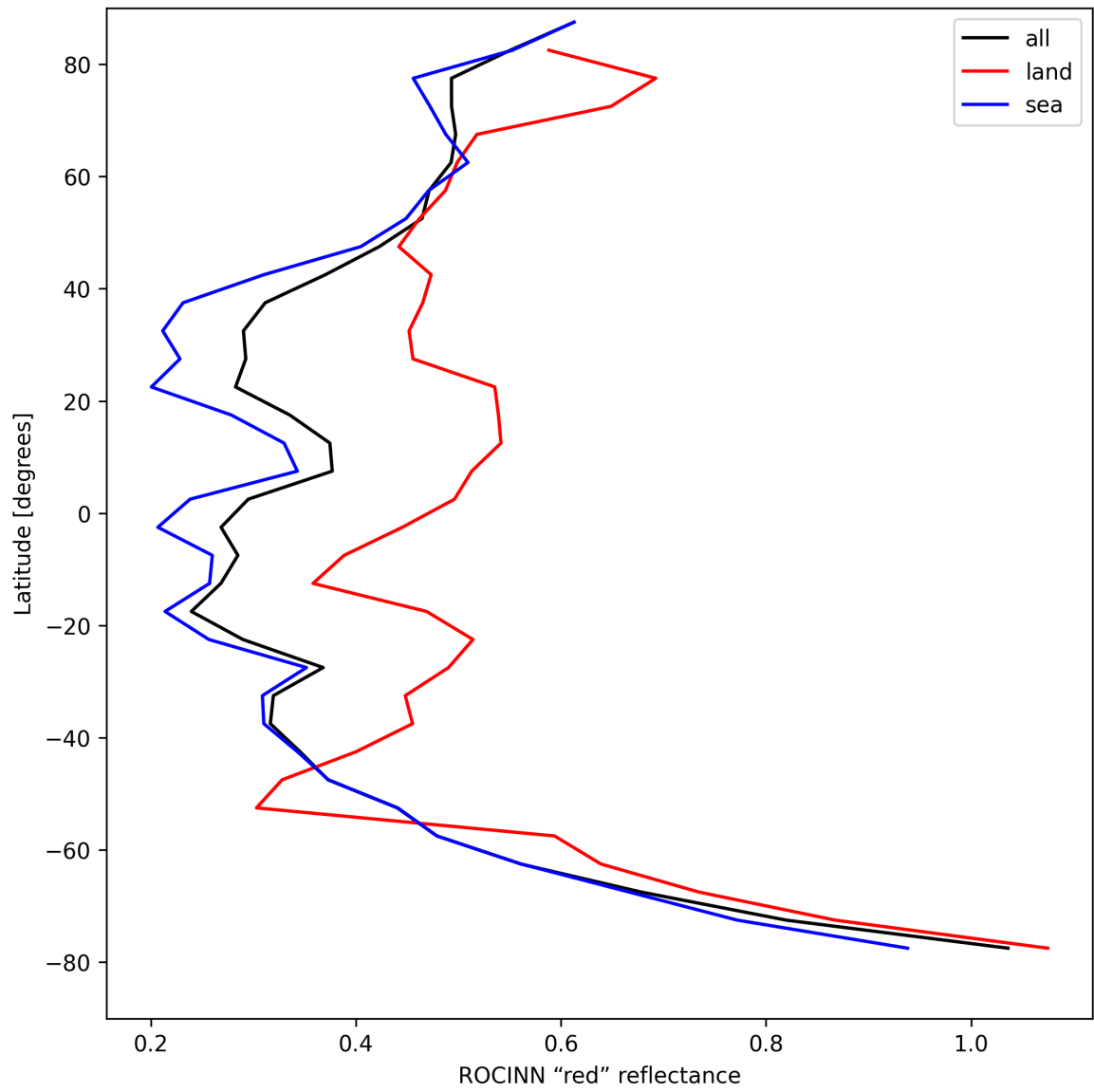
Figure 37: Zonal average of “ROCINN “red” reflectance” for 2025-08-23 to 2025-08-25.
