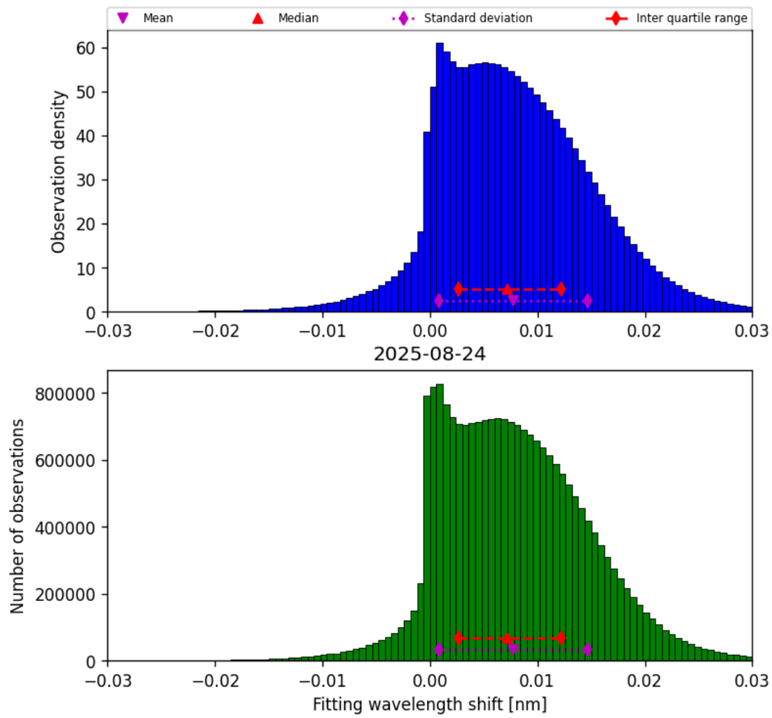
Figure 49: Histogram of “Fitting wavelength shift” for 2025-08-23 to 2025-08-25
