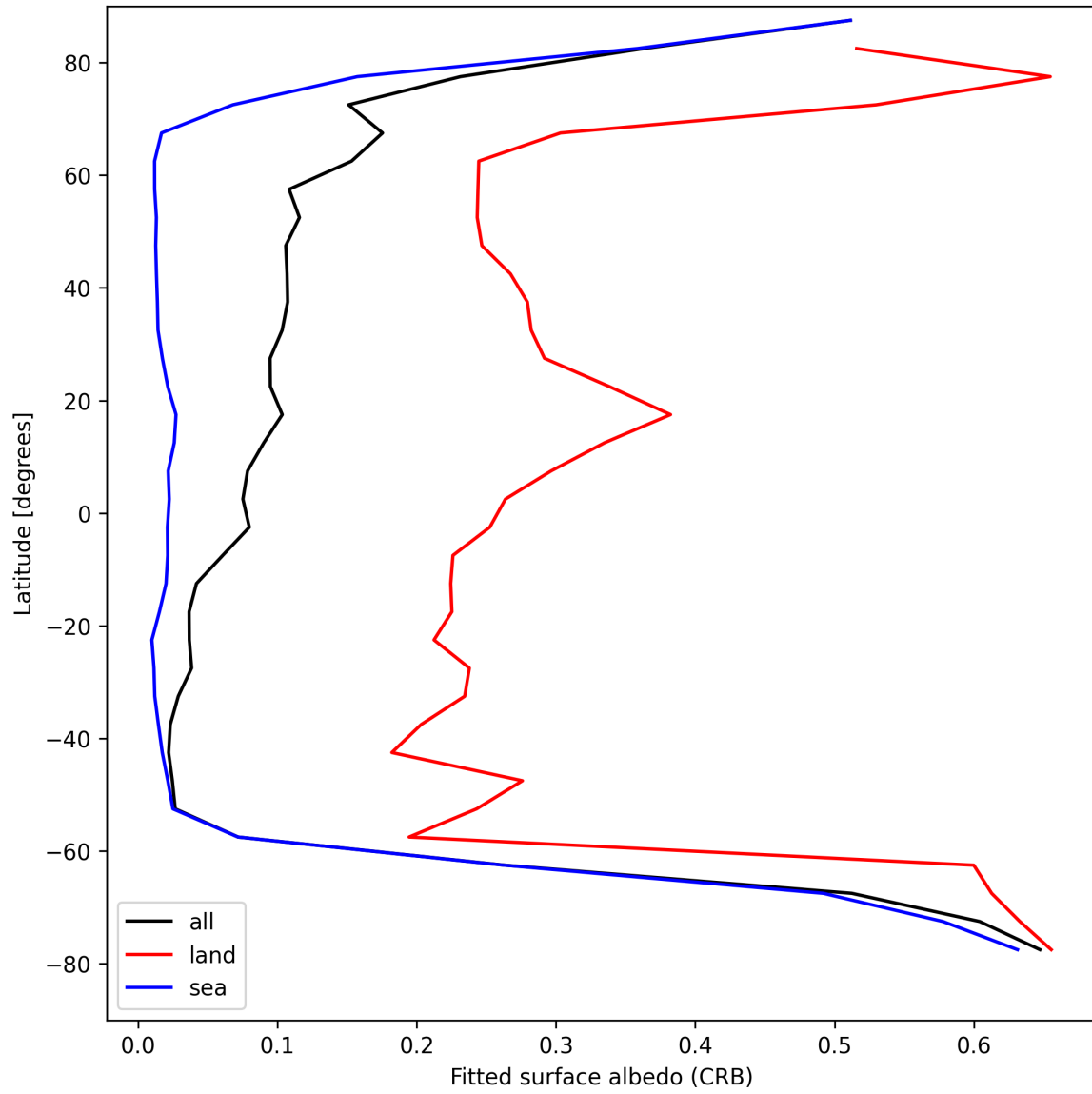
Figure 30: Zonal average of “Fitted surface albedo (CRB)” for 2025-08-23 to 2025-08-25.
