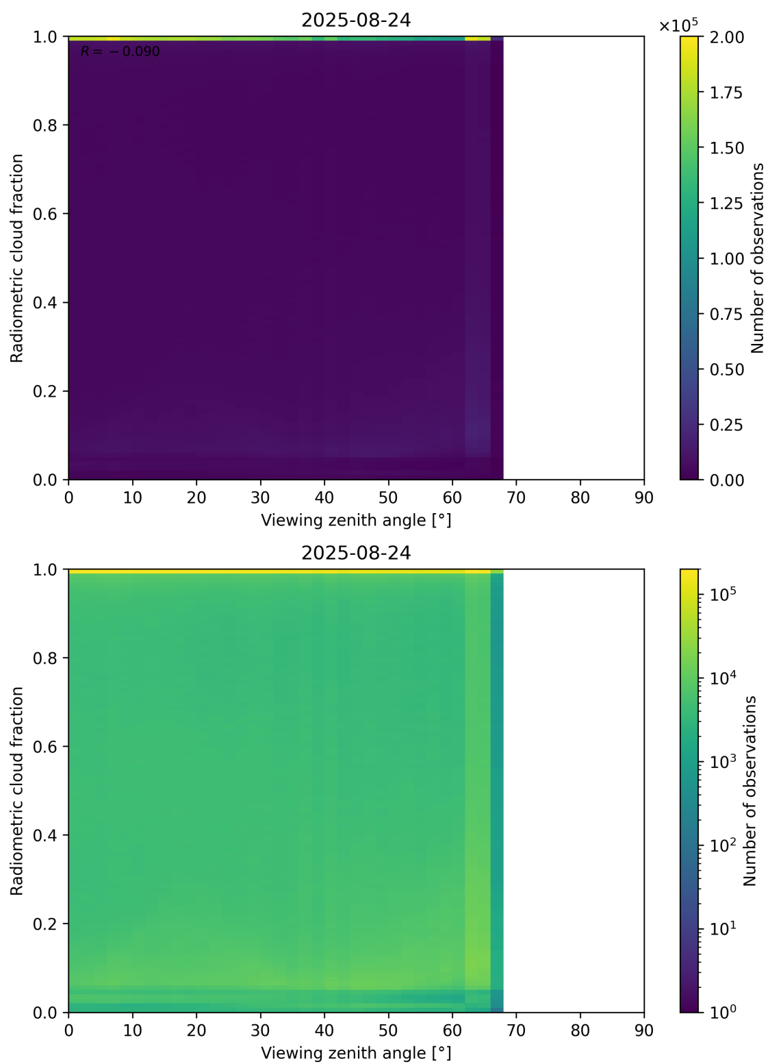
Figure 107: Scatter density plot of “Viewing zenith angle” against “Radiometric cloud fraction” for 2025-08-23 to 2025-08-25.
