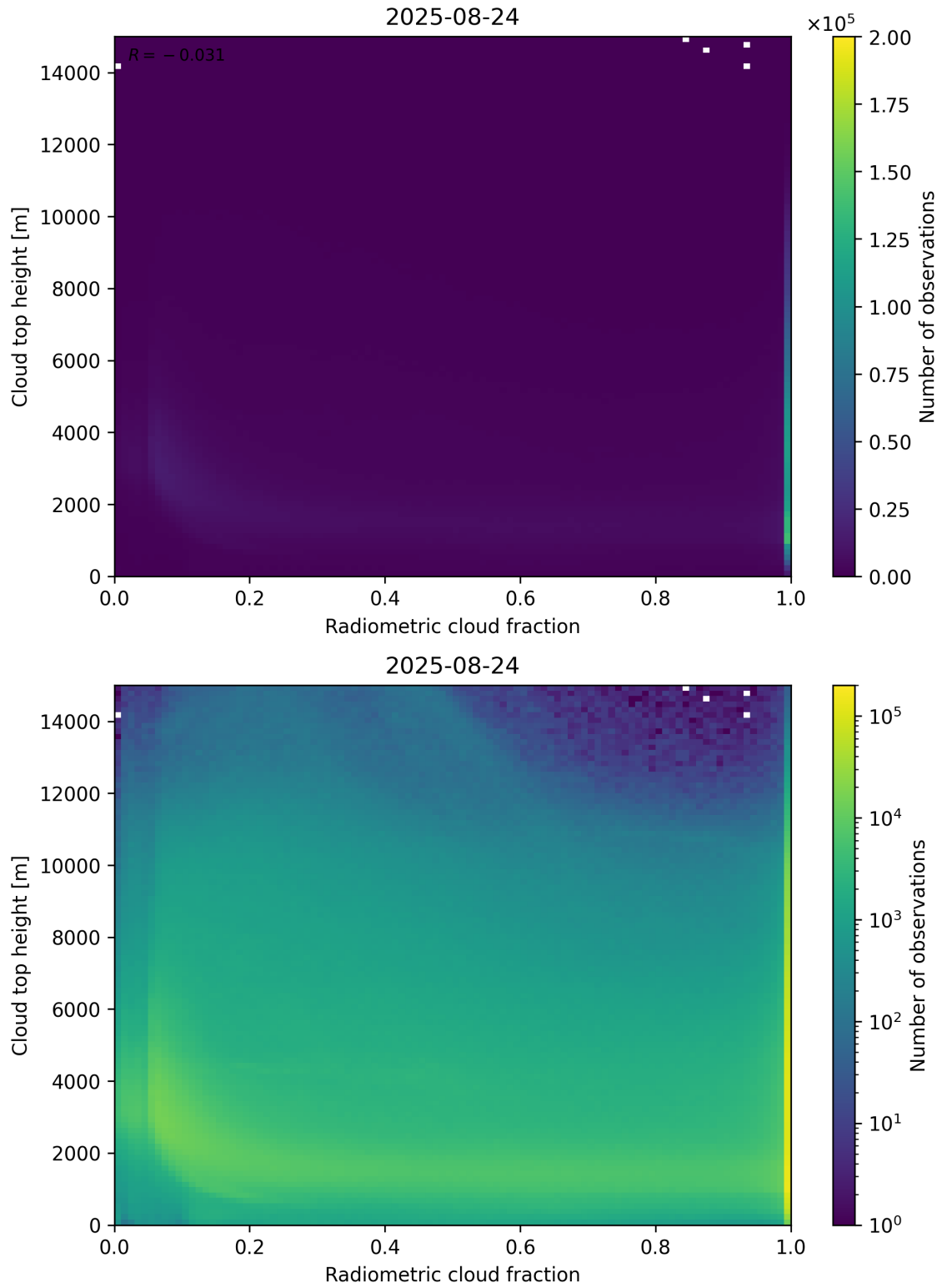
Figure 76: Scatter density plot of “Radiometric cloud fraction” against “Cloud top height” for 2025-08-23 to 2025-08-25.
