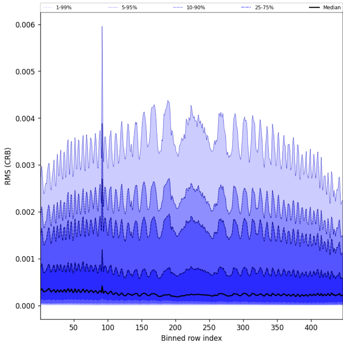
Figure 64: Along track statistics of “RMS (CRB)” for 2025-08-23 to 2025-08-25
