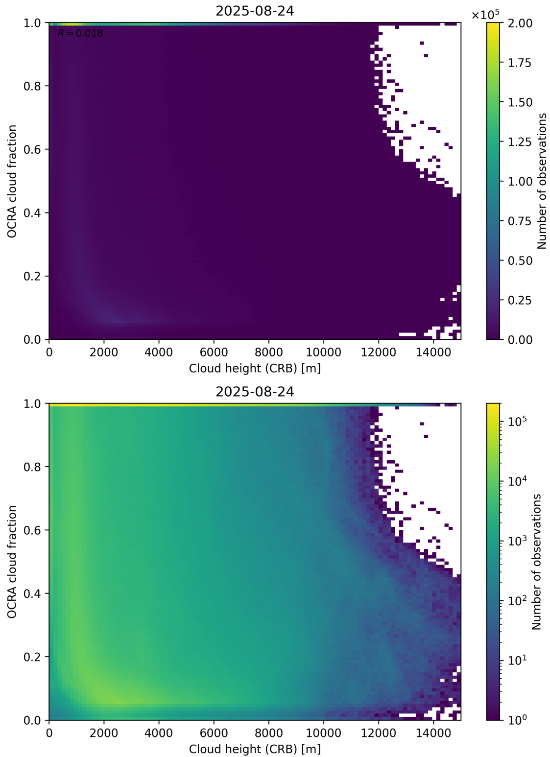
Figure 81: Scatter density plot of “Cloud height (CRB)” against “OCRA cloud fraction” for 2025-08-23 to 2025-08-25.
