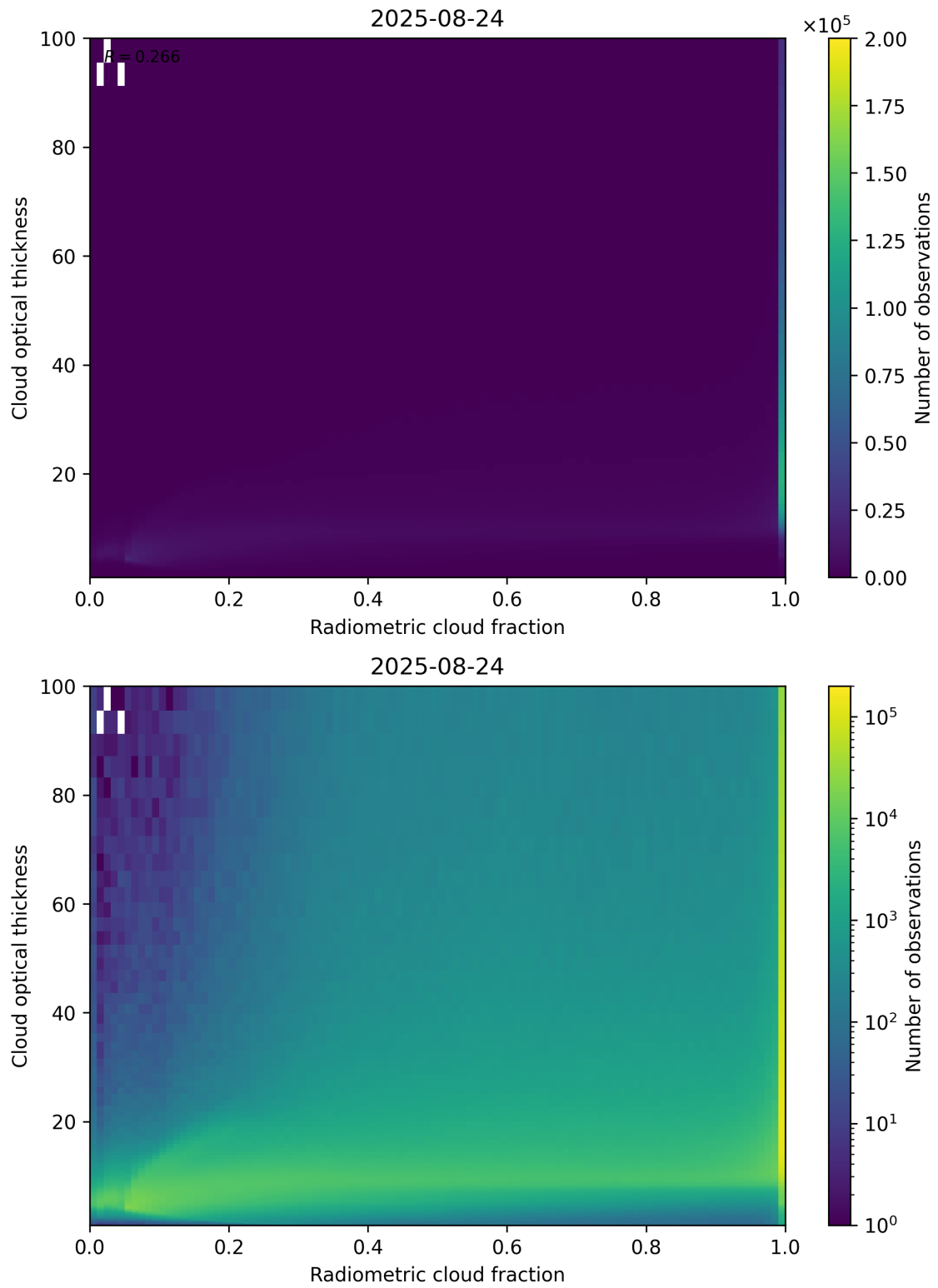
Figure 75: Scatter density plot of “Radiometric cloud fraction” against “Cloud optical thickness” for 2025-08-23 to 2025-08-25.
