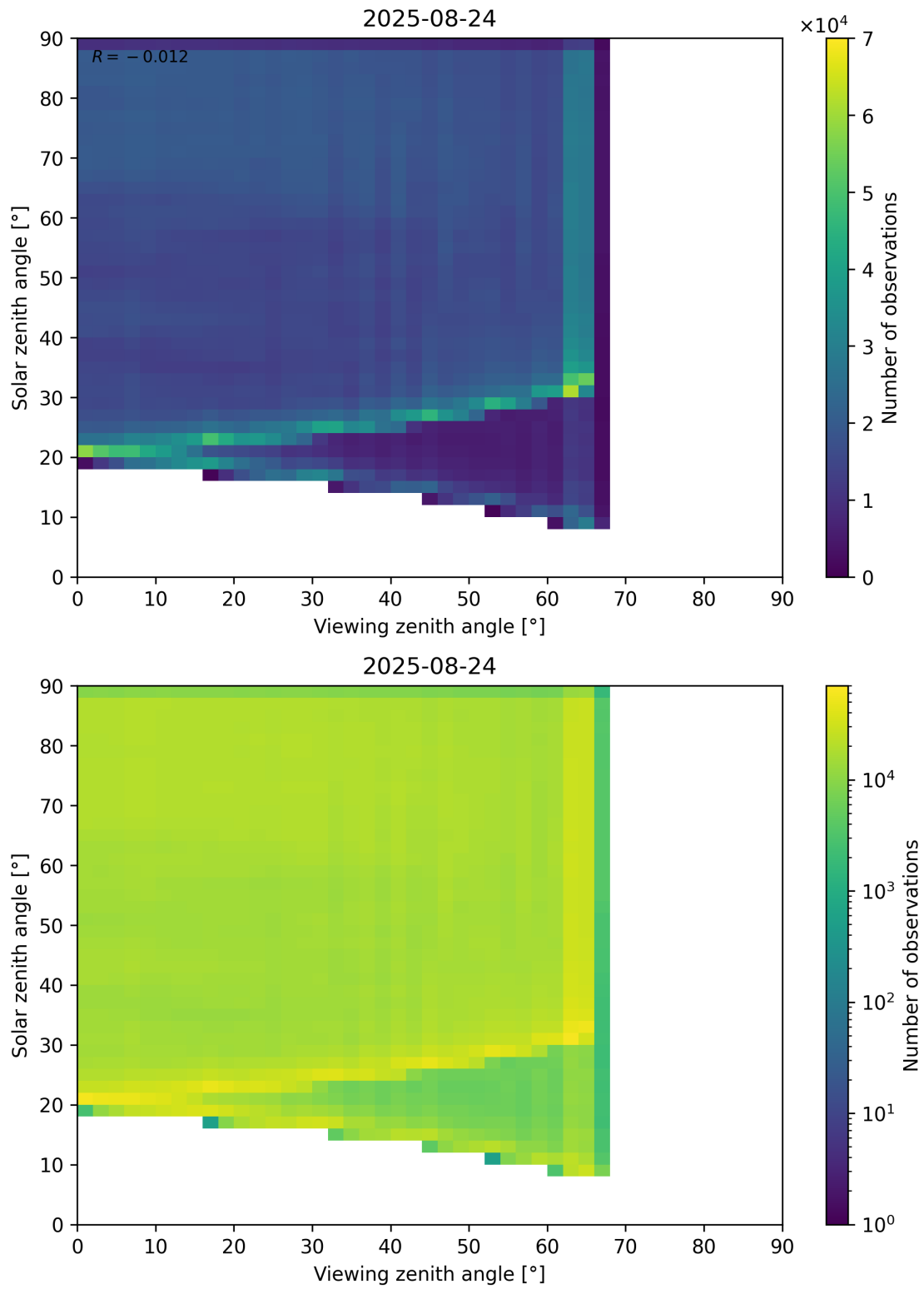
Figure 114: Scatter density plot of “Viewing zenith angle” against “Solar zenith angle” for 2025-08-23 to 2025-08-25.
