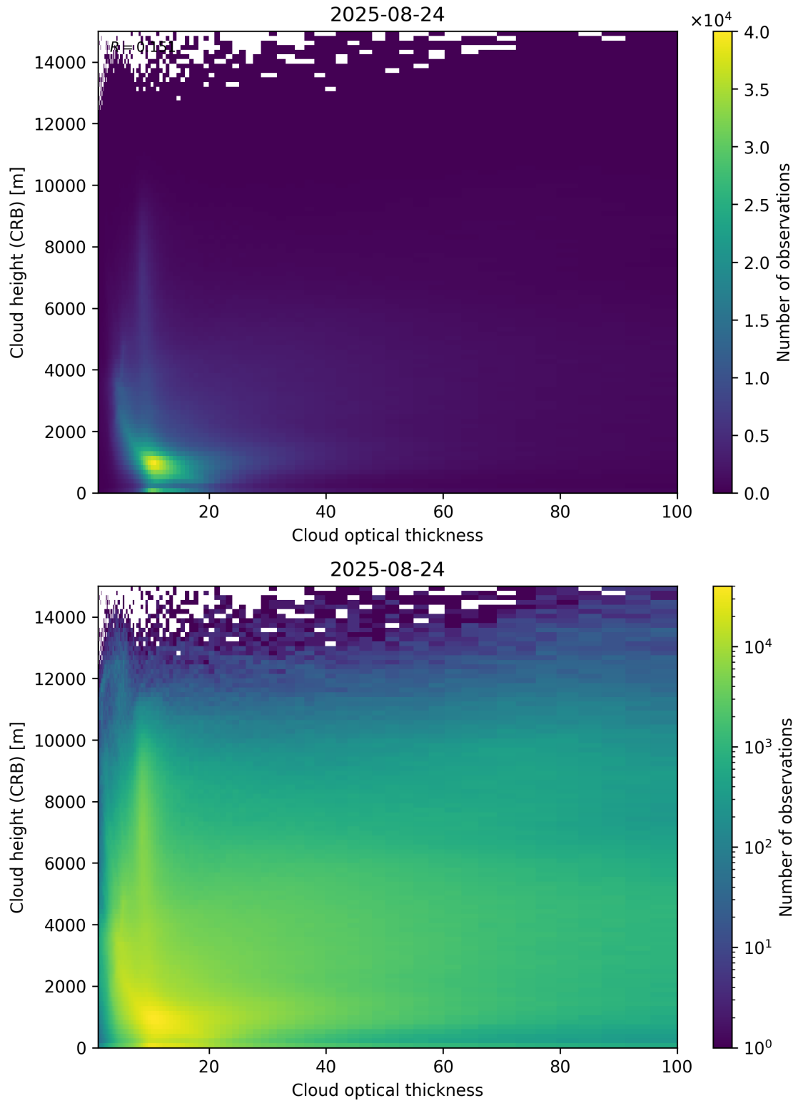
Figure 85: Scatter density plot of “Cloud optical thickness” against “Cloud height (CRB)” for 2025-08-23 to 2025-08-25.
