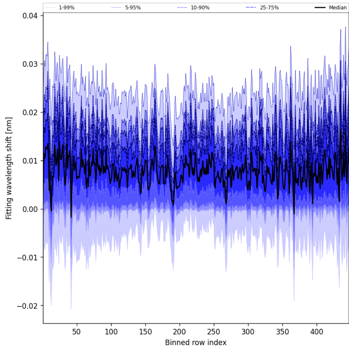
Figure 65: Along track statistics of “Fitting wavelength shift” for 2025-08-23 to 2025-08-25
