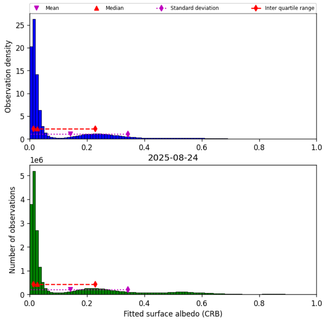
Figure 46: Histogram of “Fitted surface albedo (CRB)” for 2025-08-23 to 2025-08-25
