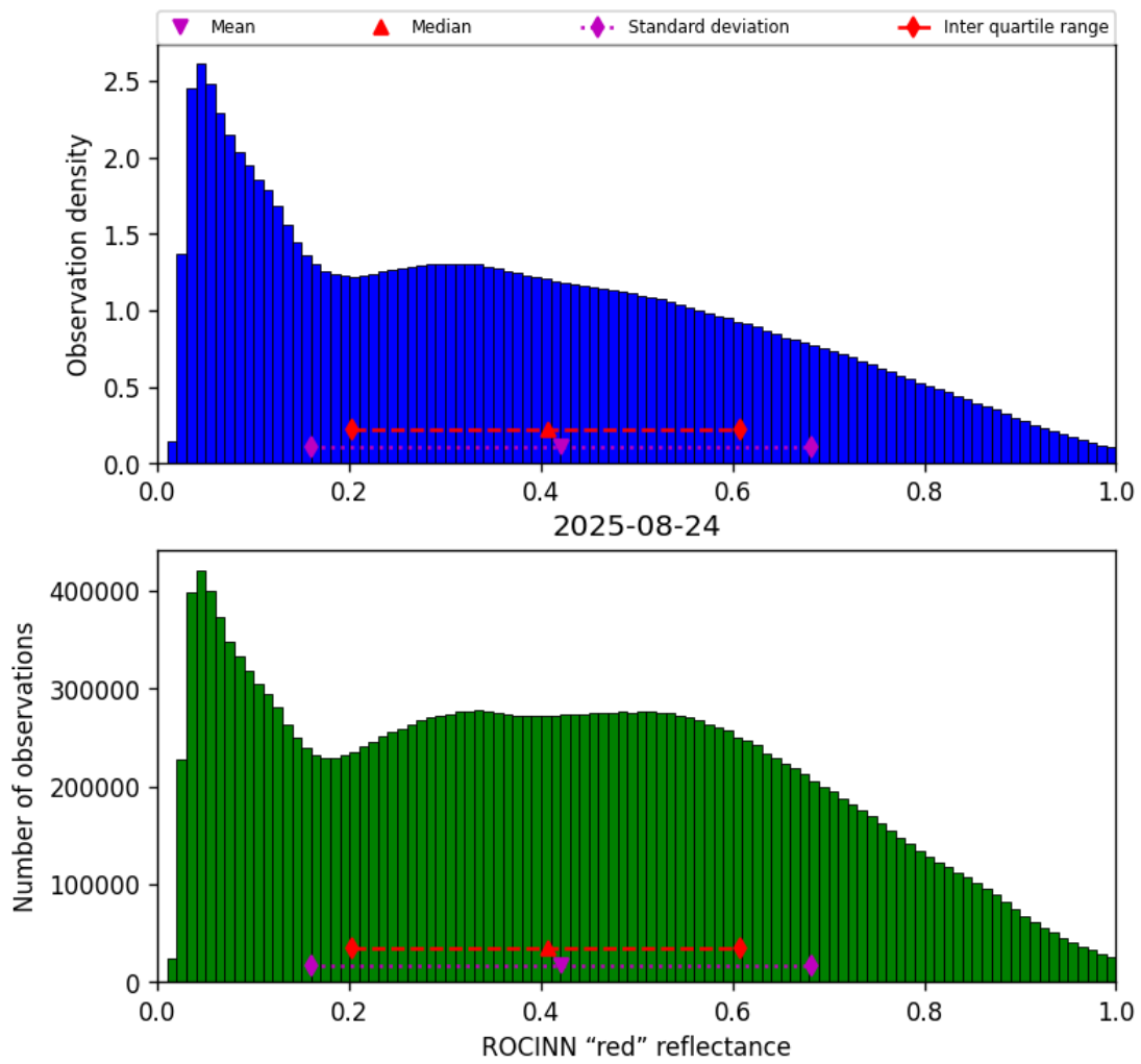
Figure 53: Histogram of “ROCINN “red” reflectance” for 2025-08-23 to 2025-08-25
