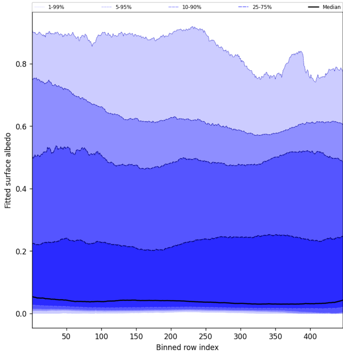
Figure 61: Along track statistics of “Fitted surface albedo” for 2025-08-23 to 2025-08-25
