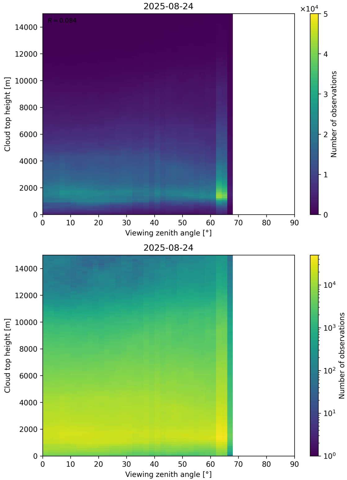
Figure 112: Scatter density plot of “Viewing zenith angle” against “Cloud top height” for 2025-08-23 to 2025-08-25.
