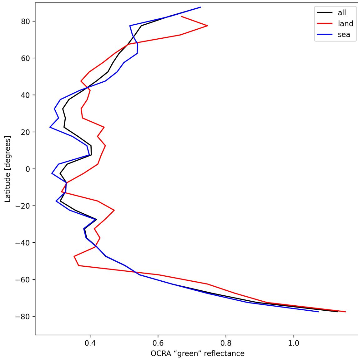
Figure 36: Zonal average of “OCRA “green” reflectance” for 2025-08-23 to 2025-08-25.
