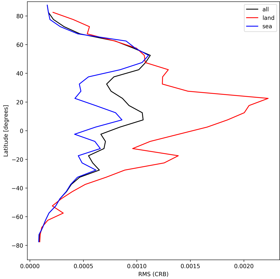
Figure 32: Zonal average of “RMS (CRB)” for 2025-08-23 to 2025-08-25.
