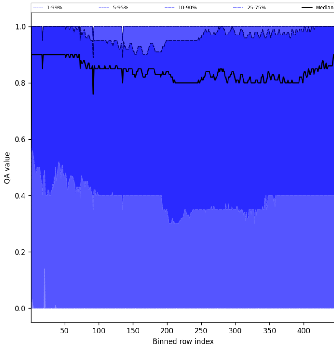
Figure 54: Along track statistics of “QA value” for 2025-08-23 to 2025-08-25
