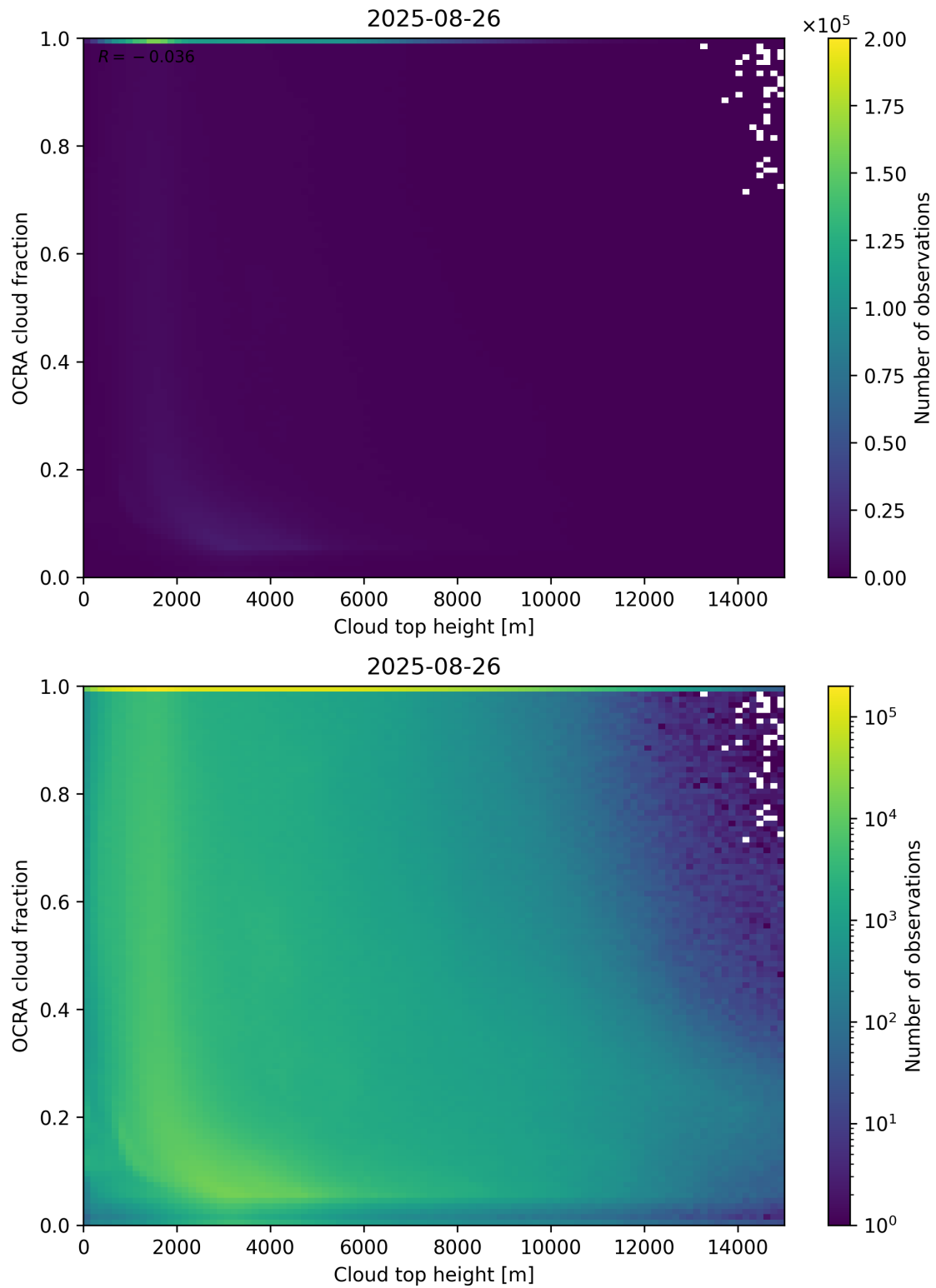
Figure 87: Scatter density plot of “Cloud top height” against “OCRA cloud fraction” for 2025-08-25 to 2025-08-27.
