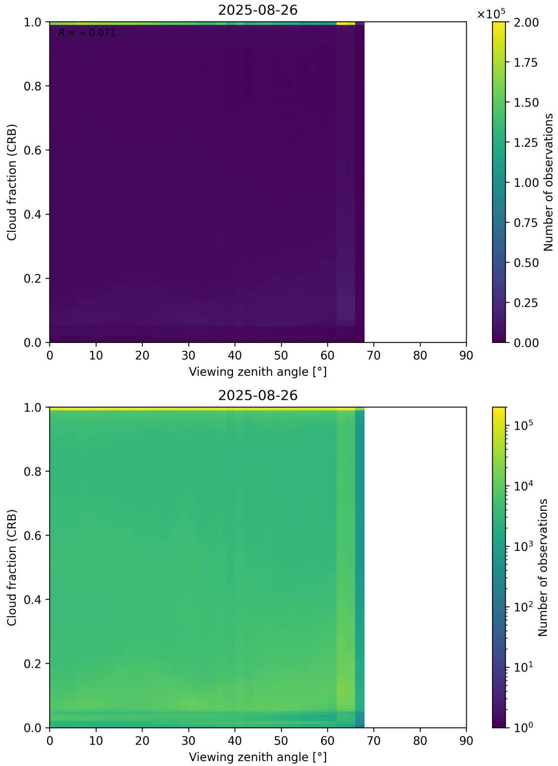
Figure 109: Scatter density plot of “Viewing zenith angle” against “Cloud fraction (CRB)” for 2025-08-25 to 2025-08-27.
