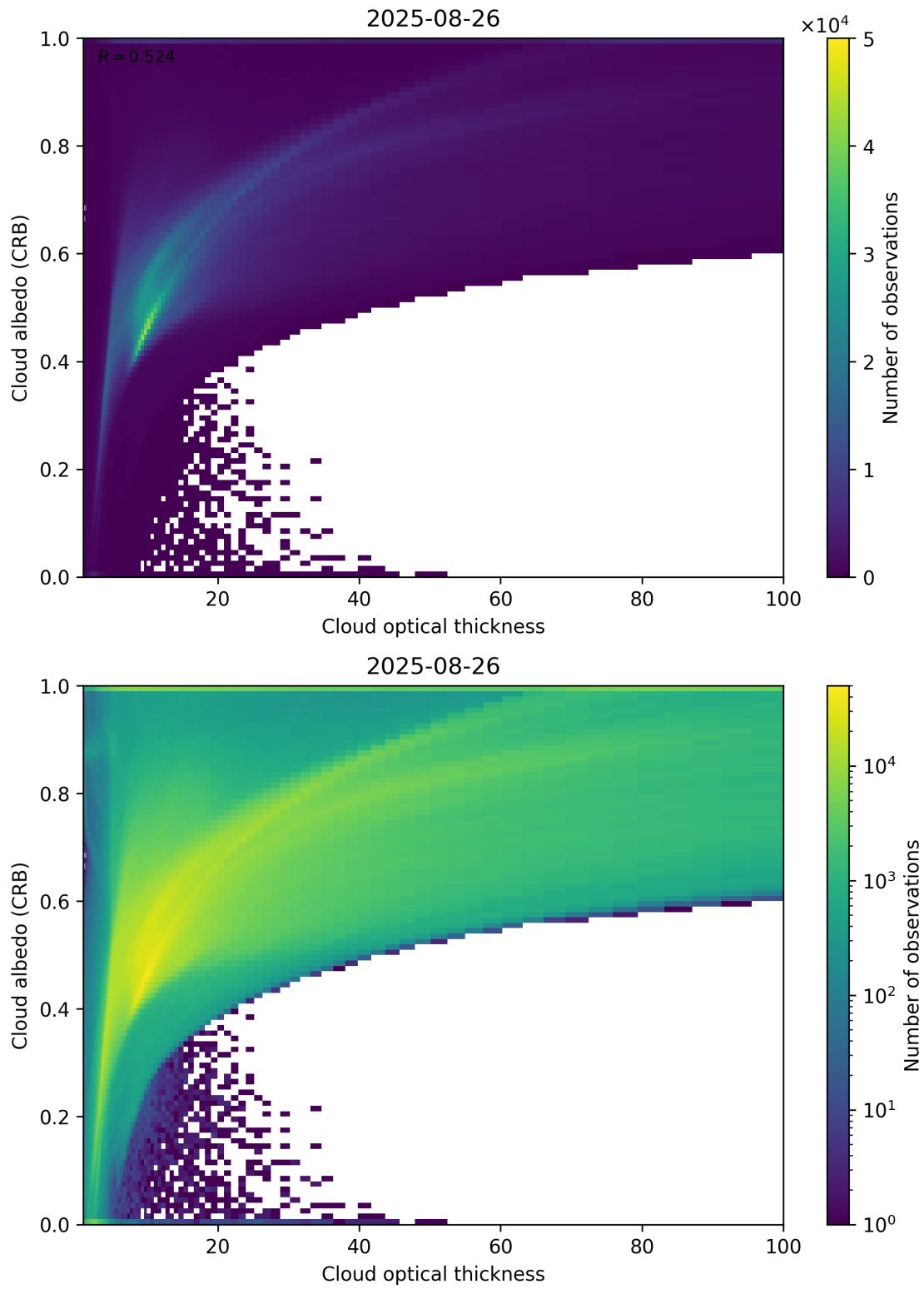
Figure 82: Scatter density plot of “Cloud optical thickness” against “Cloud albedo (CRB)” for 2025-08-25 to 2025-08-27.
