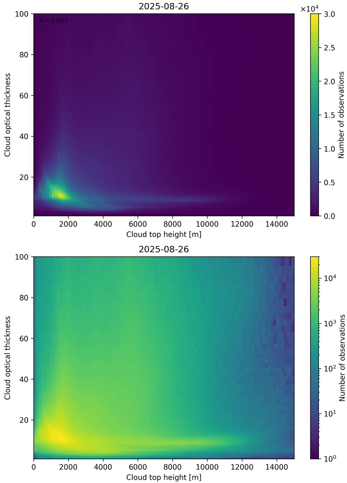
Figure 90: Scatter density plot of “Cloud top height” against “Cloud optical thickness” for 2025-08-25 to 2025-08-27.
