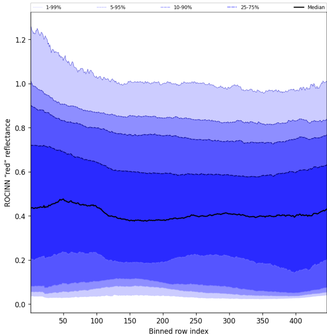
Figure 69: Along track statistics of “ROCINN “red” reflectance” for 2025-08-25 to 2025-08-27
