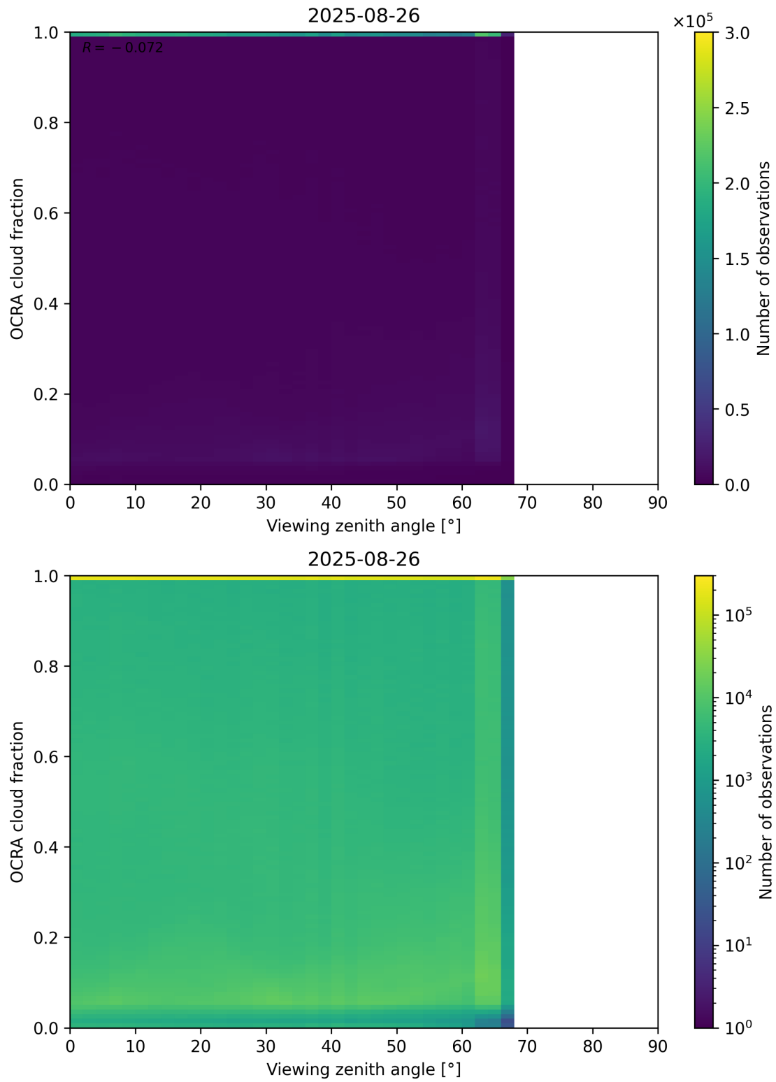
Figure 108: Scatter density plot of “Viewing zenith angle” against “OCRA cloud fraction” for 2025-08-25 to 2025-08-27.
