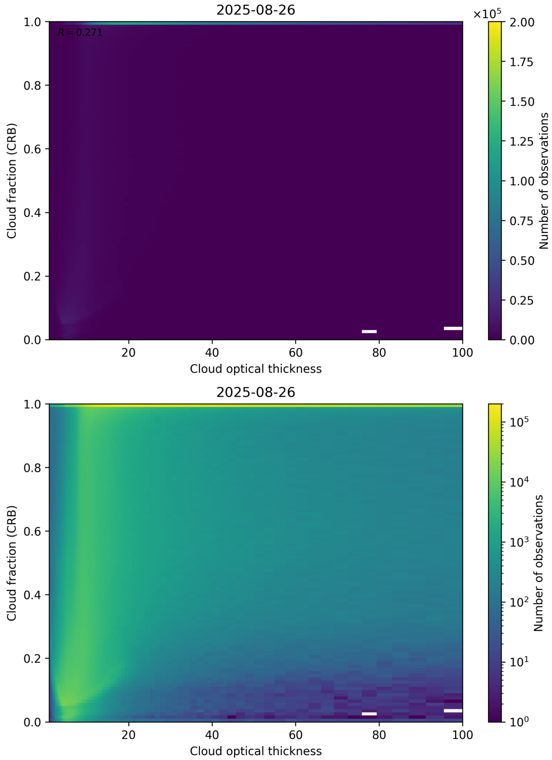
Figure 84: Scatter density plot of “Cloud optical thickness” against “Cloud fraction (CRB)” for 2025-08-25 to 2025-08-27.
