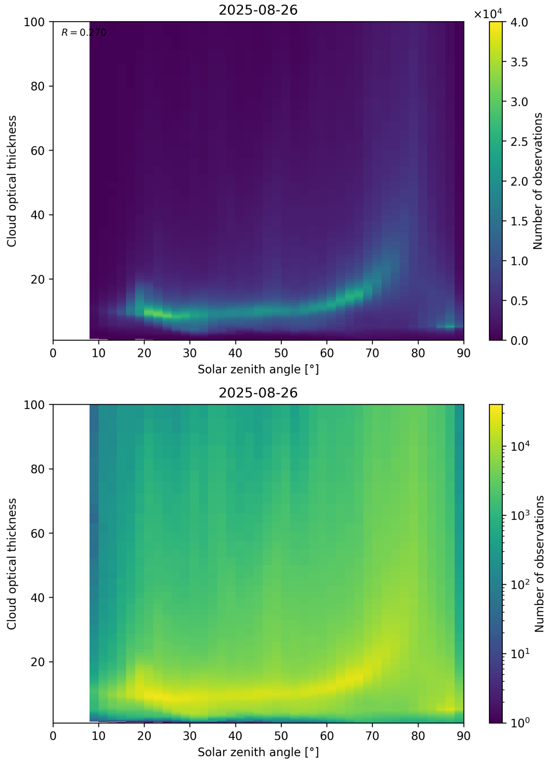
Figure 103: Scatter density plot of “Solar zenith angle” against “Cloud optical thickness” for 2025-08-25 to 2025-08-27.
