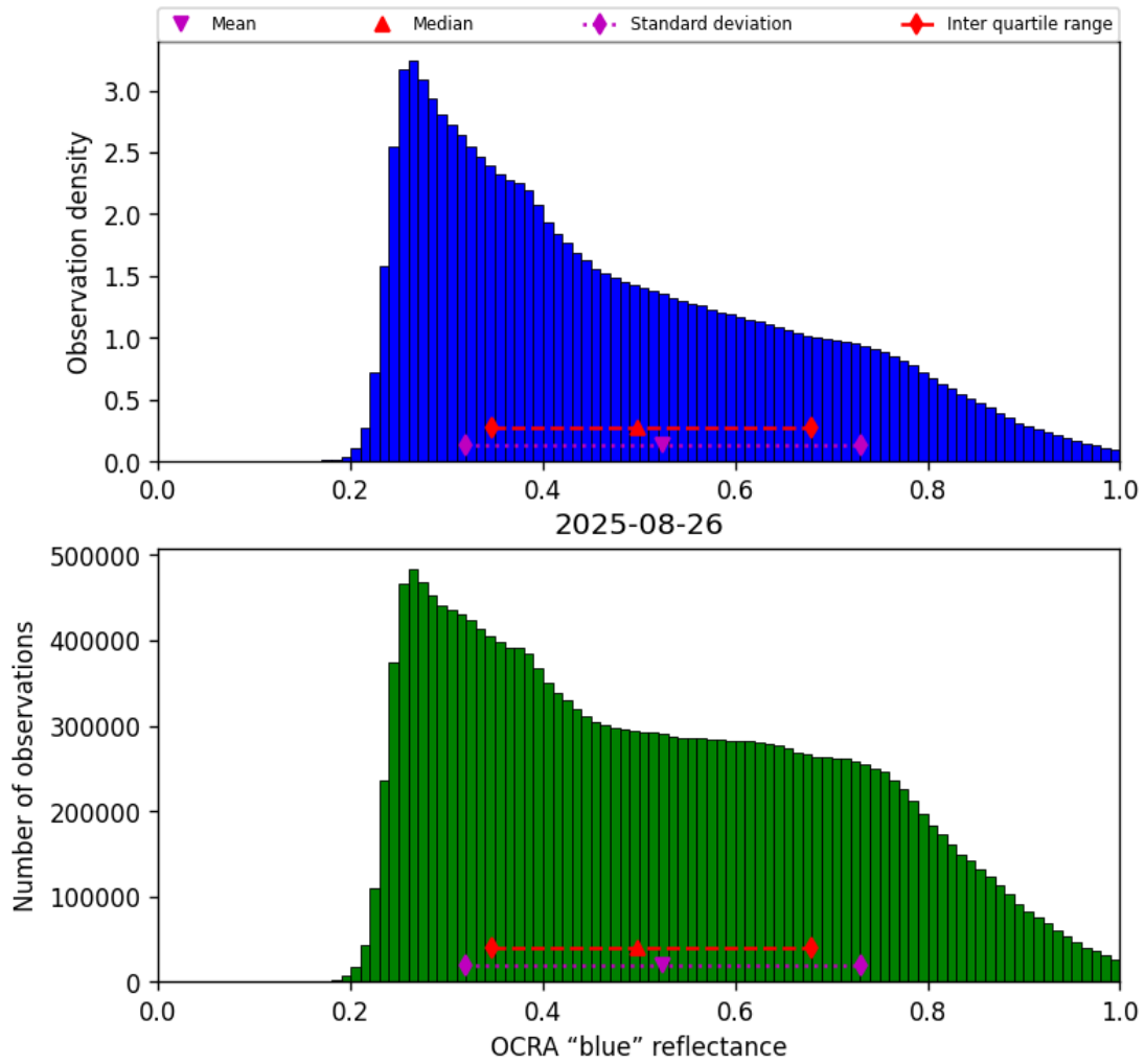
Figure 51: Histogram of “OCRA “blue” reflectance” for 2025-08-25 to 2025-08-27
