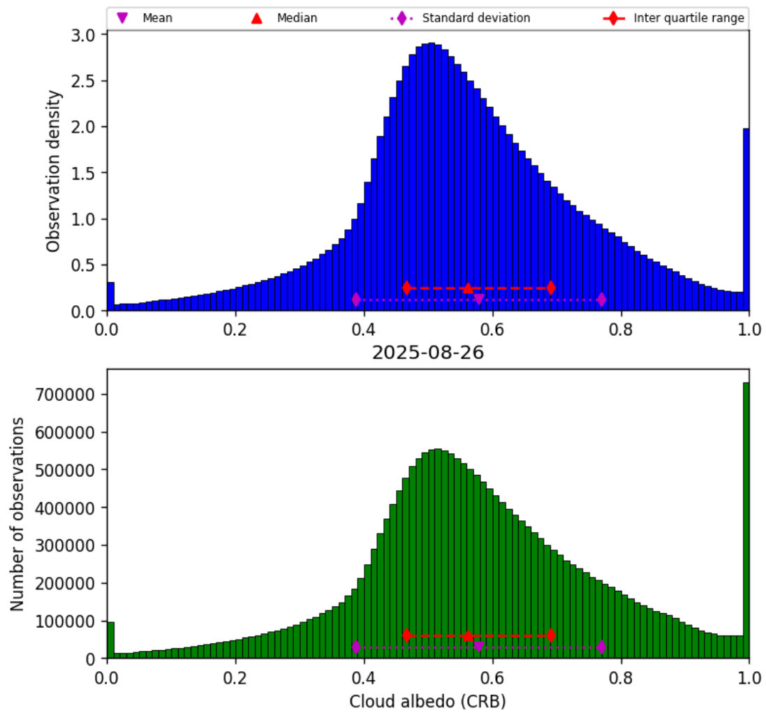
Figure 44: Histogram of “Cloud albedo (CRB)” for 2025-08-25 to 2025-08-27
