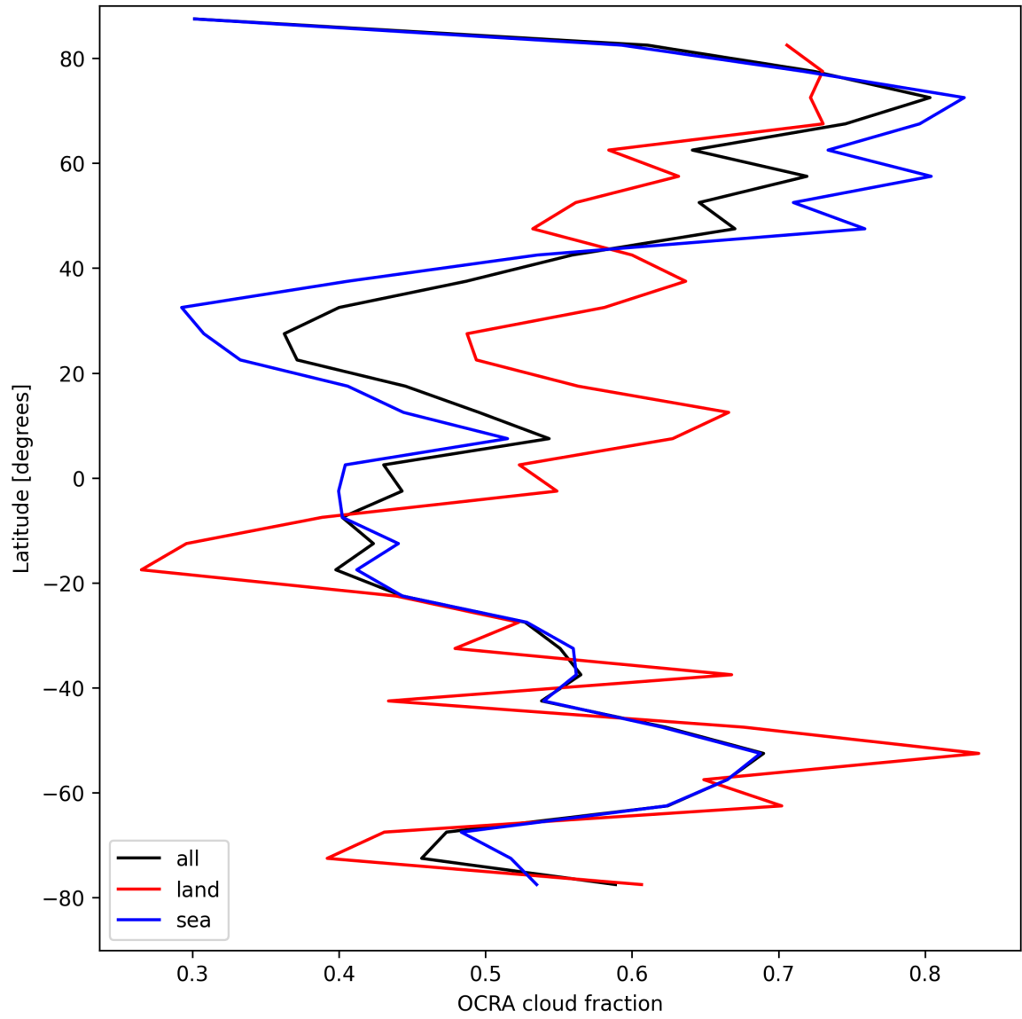
Figure 34: Zonal average of “OCRA cloud fraction” for 2025-08-25 to 2025-08-27.
