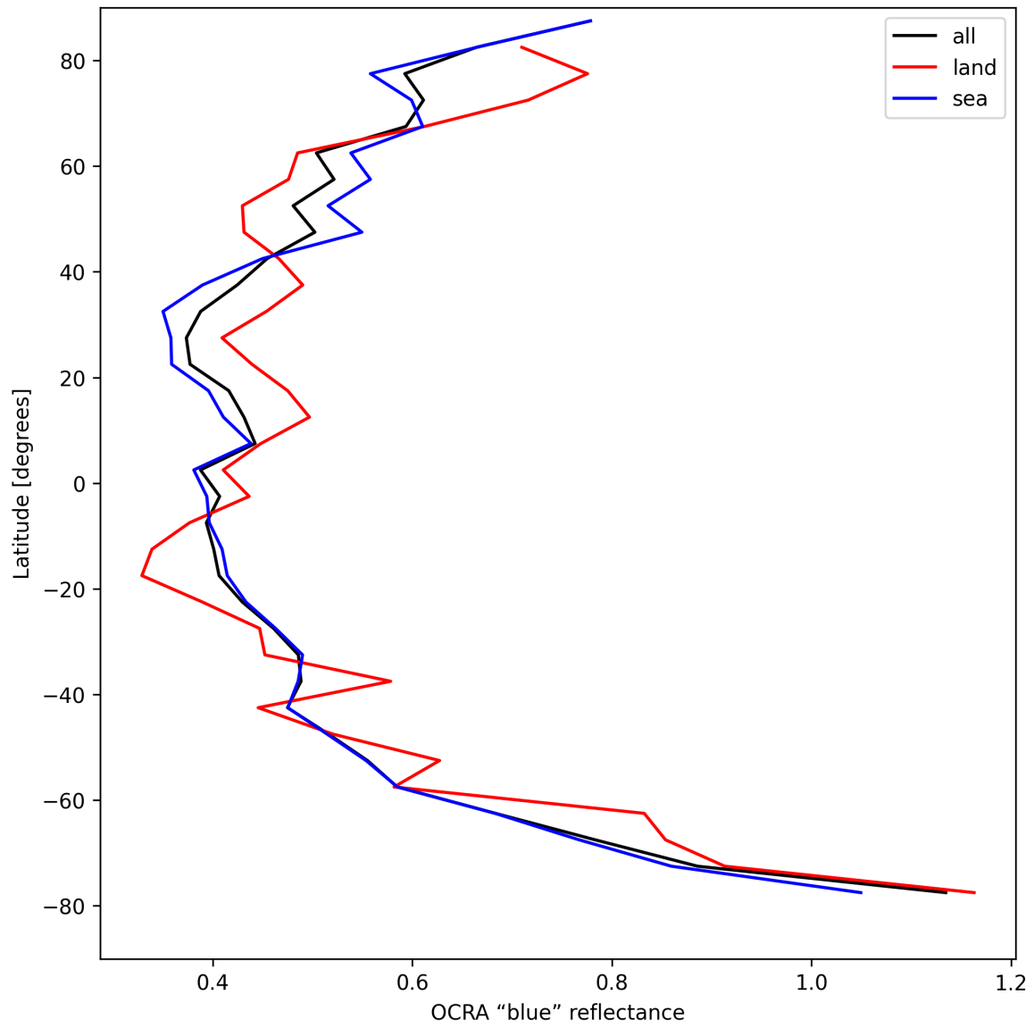
Figure 35: Zonal average of “OCRA “blue” reflectance” for 2025-08-25 to 2025-08-27.
