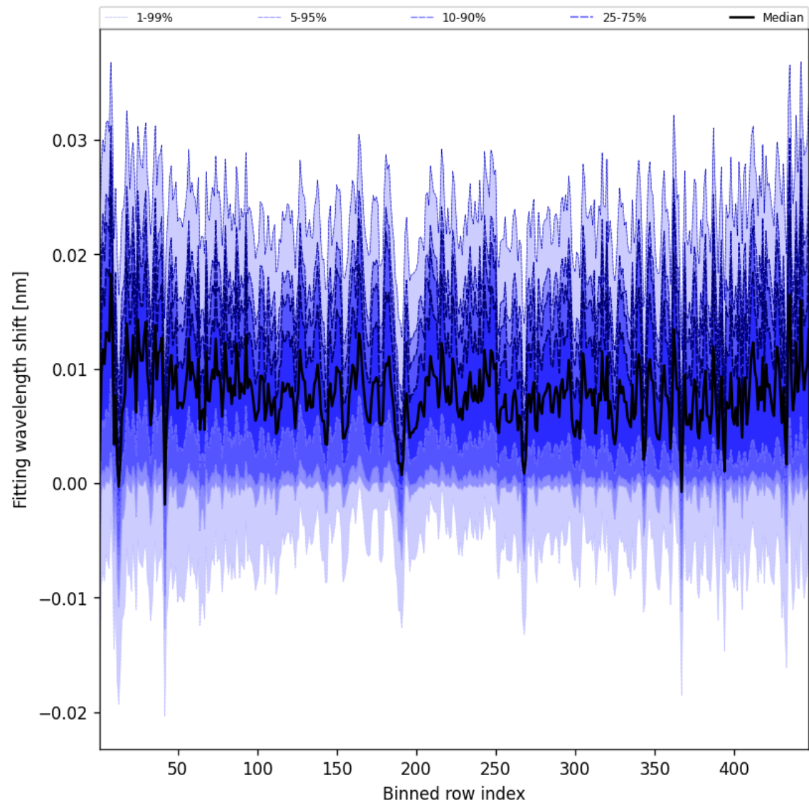
Figure 65: Along track statistics of “Fitting wavelength shift” for 2025-08-25 to 2025-08-27
