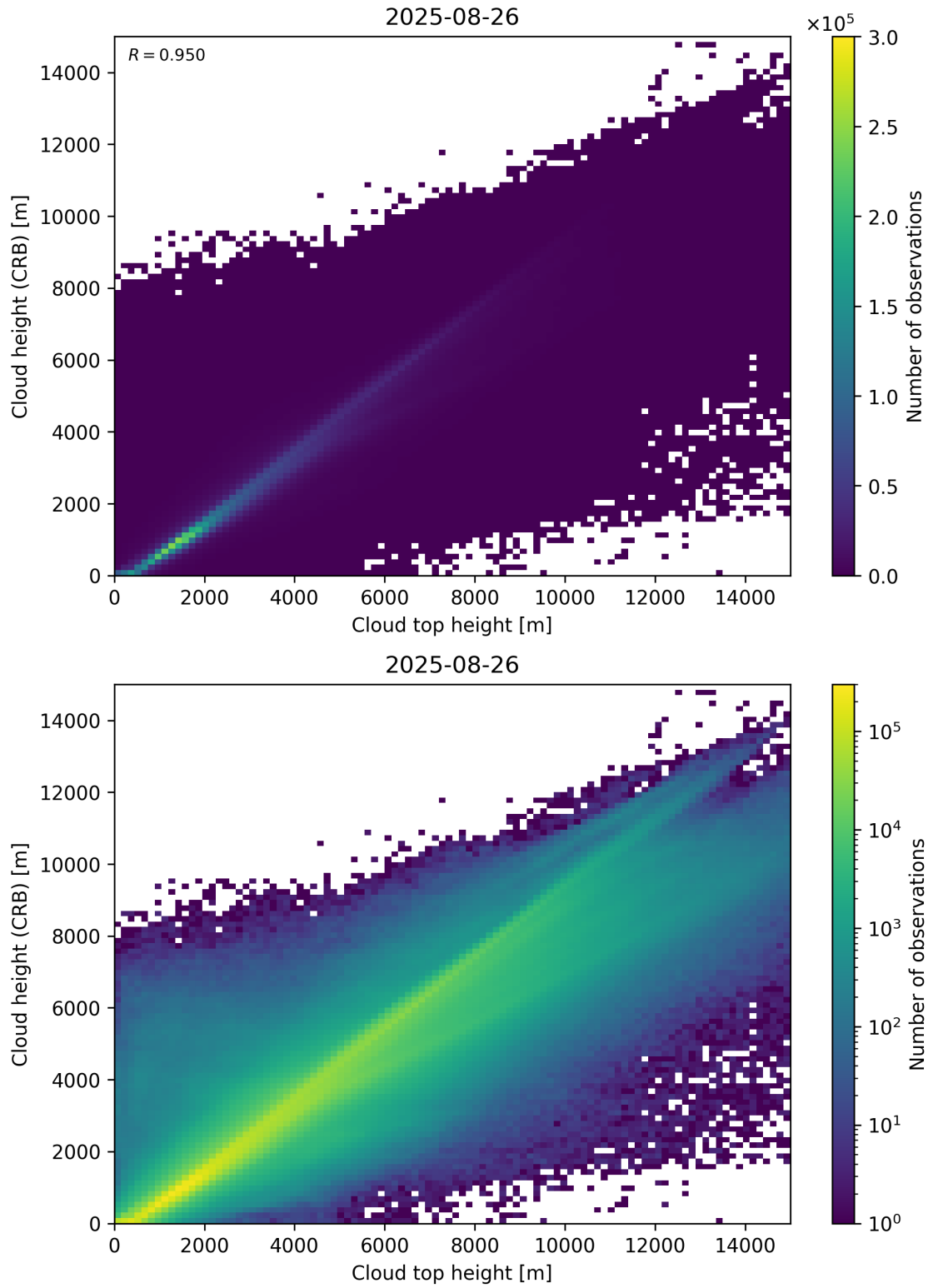
Figure 89: Scatter density plot of “Cloud top height” against “Cloud height (CRB)” for 2025-08-25 to 2025-08-27.
