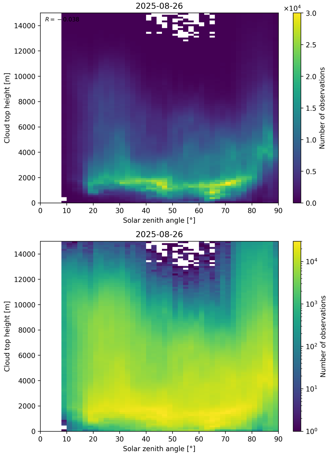
Figure 104: Scatter density plot of “Solar zenith angle” against “Cloud top height” for 2025-08-25 to 2025-08-27.
