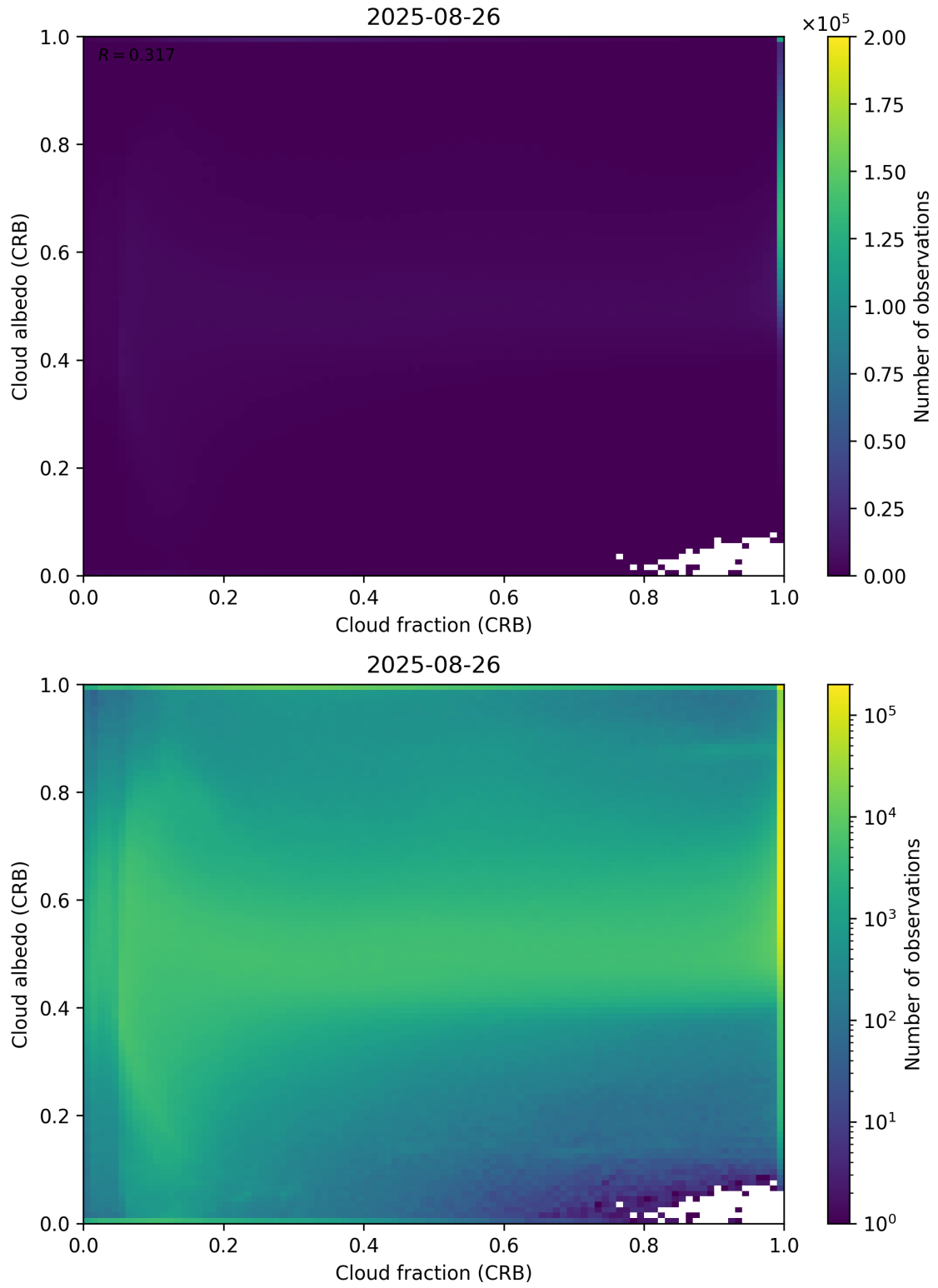
Figure 77: Scatter density plot of “Cloud fraction (CRB)” against “Cloud albedo (CRB)” for 2025-08-25 to 2025-08-27.
