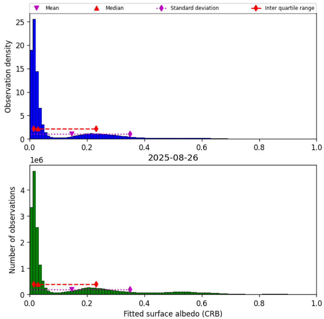
Figure 46: Histogram of “Fitted surface albedo (CRB)” for 2025-08-25 to 2025-08-27
