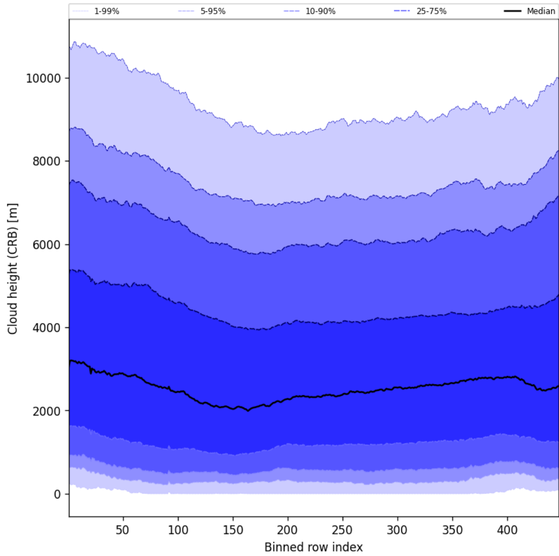
Figure 59: Along track statistics of “Cloud height (CRB)” for 2025-08-25 to 2025-08-27
