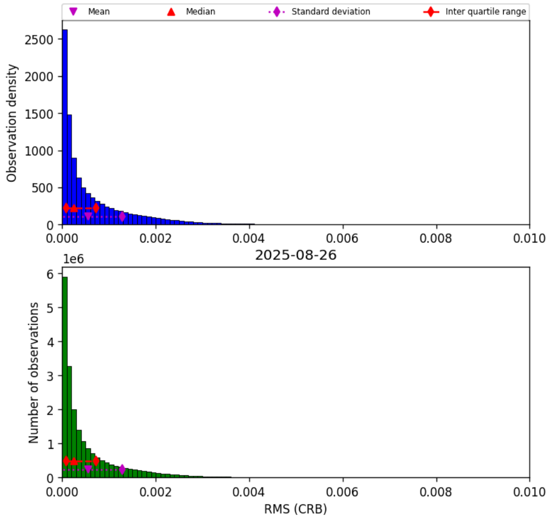
Figure 48: Histogram of “RMS (CRB)” for 2025-08-25 to 2025-08-27
