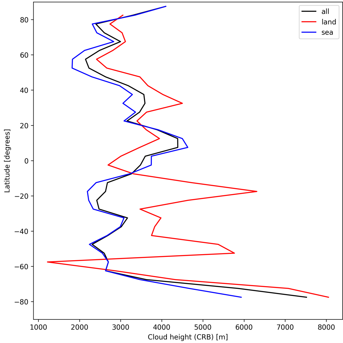
Figure 27: Zonal average of “Cloud height (CRB)” for 2025-08-25 to 2025-08-27.
