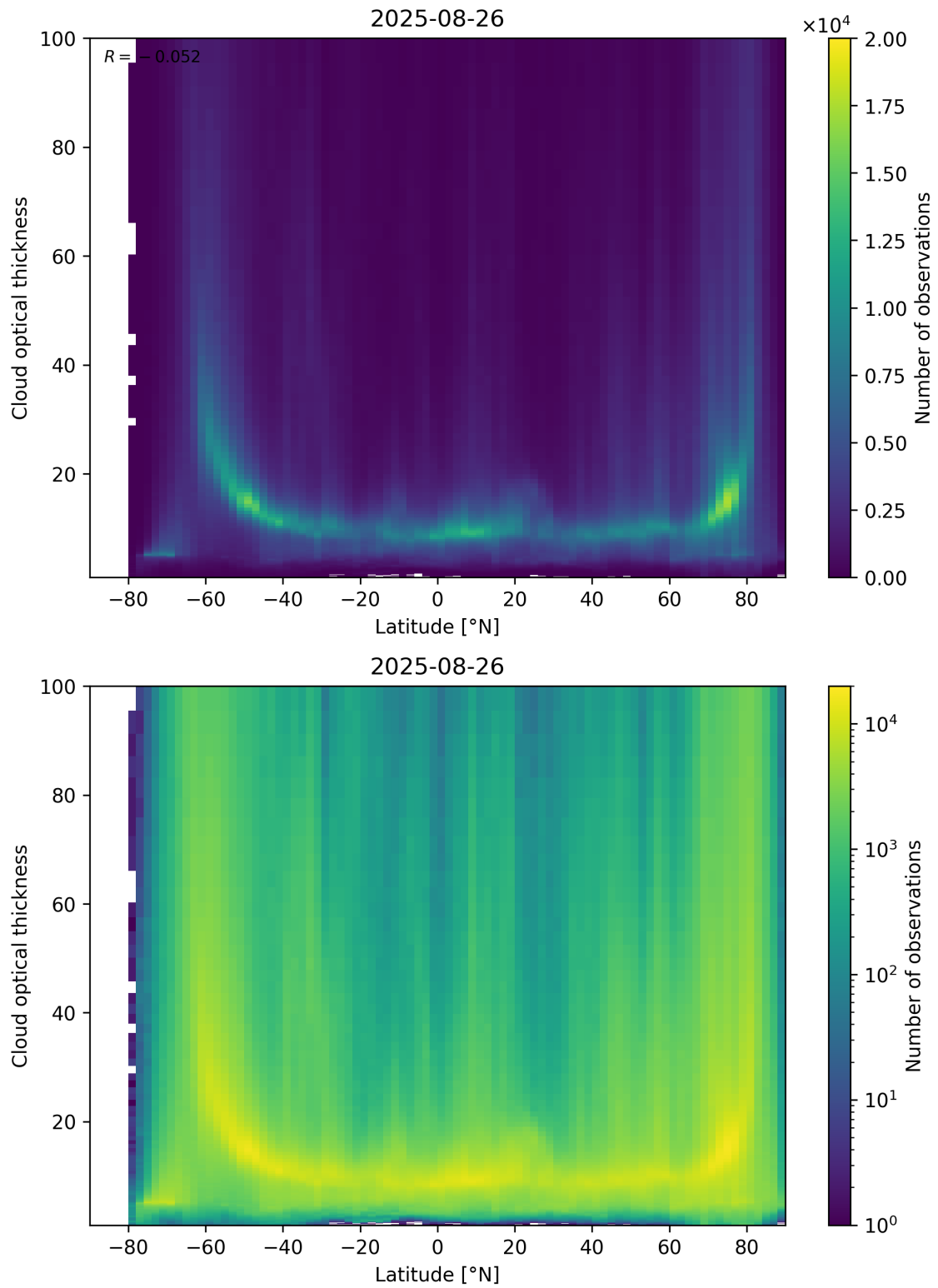
Figure 96: Scatter density plot of “Latitude” against “Cloud optical thickness” for 2025-08-25 to 2025-08-27.
