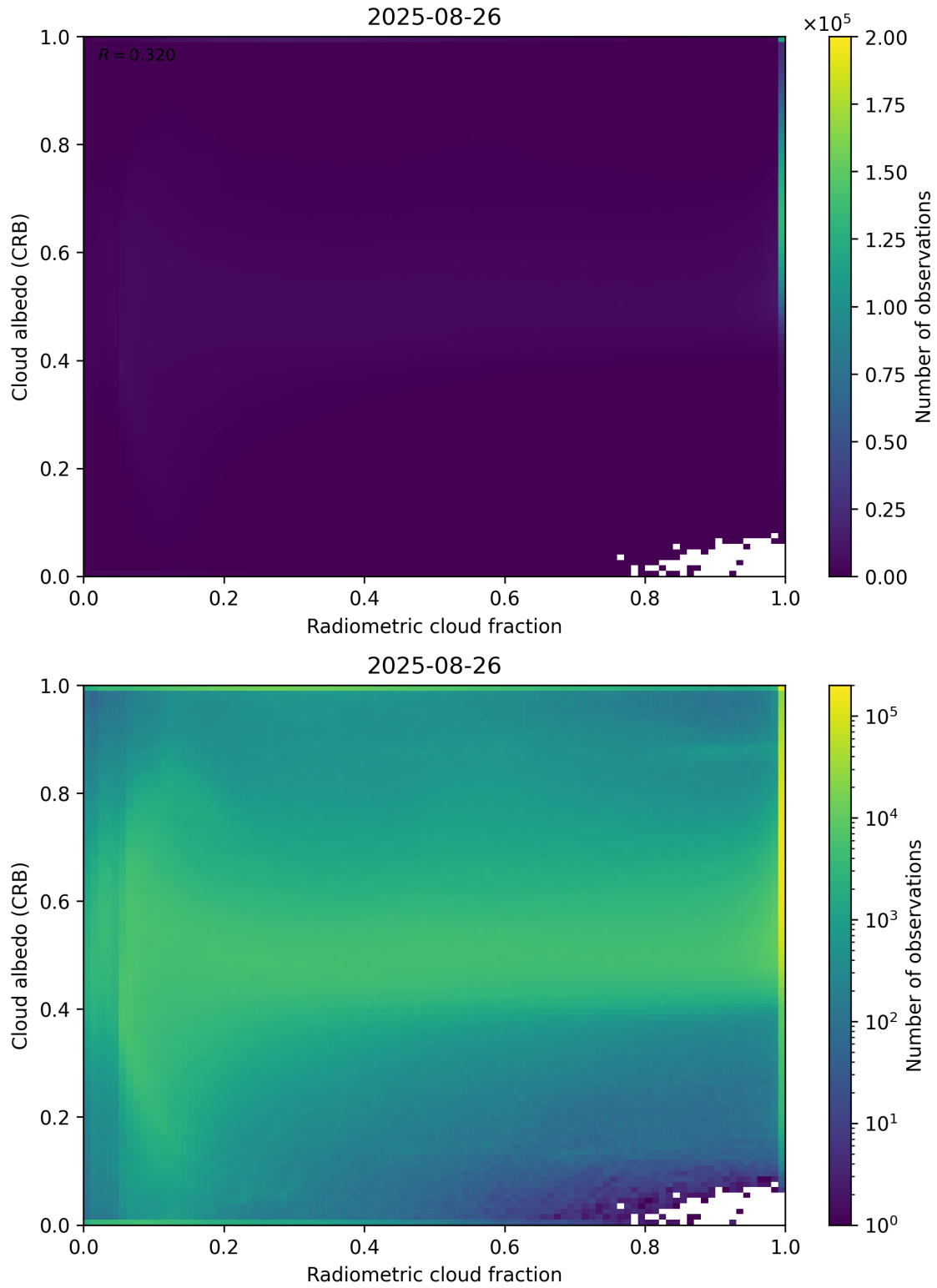
Figure 71: Scatter density plot of “Radiometric cloud fraction” against “Cloud albedo (CRB)” for 2025-08-25 to 2025-08-27.
