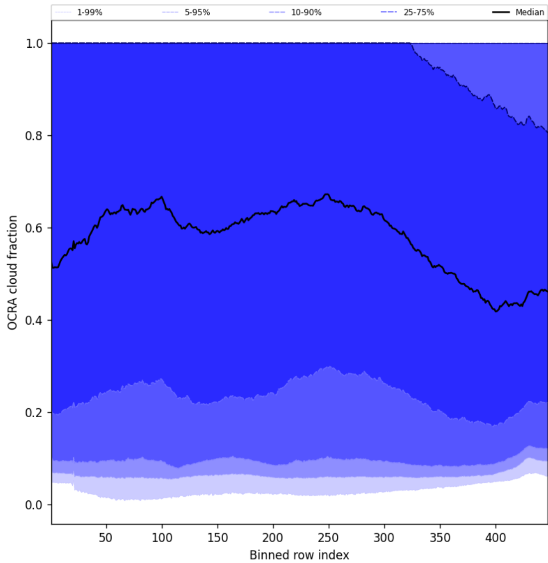
Figure 66: Along track statistics of “OCRA cloud fraction” for 2025-08-25 to 2025-08-27
