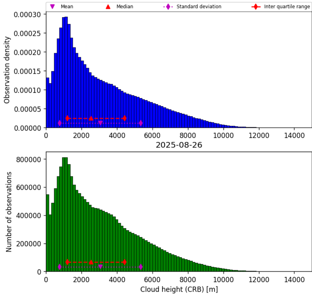
Figure 43: Histogram of “Cloud height (CRB)” for 2025-08-25 to 2025-08-27
