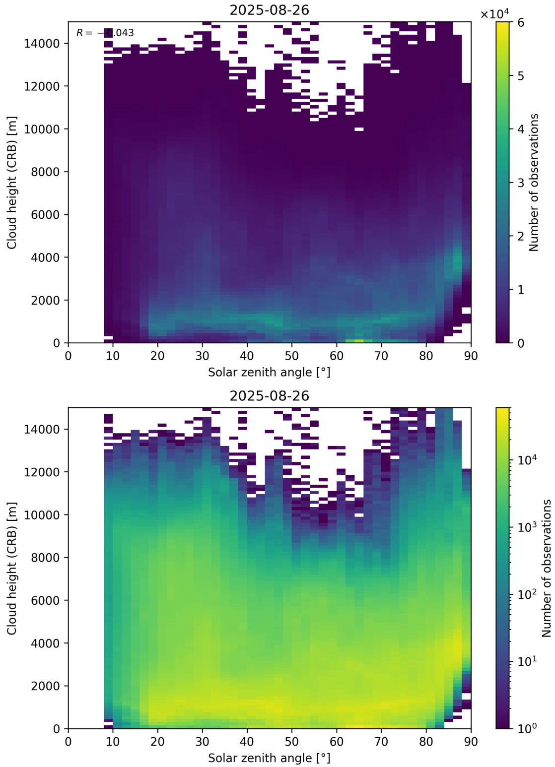
Figure 102: Scatter density plot of “Solar zenith angle” against “Cloud height (CRB)” for 2025-08-25 to 2025-08-27.
