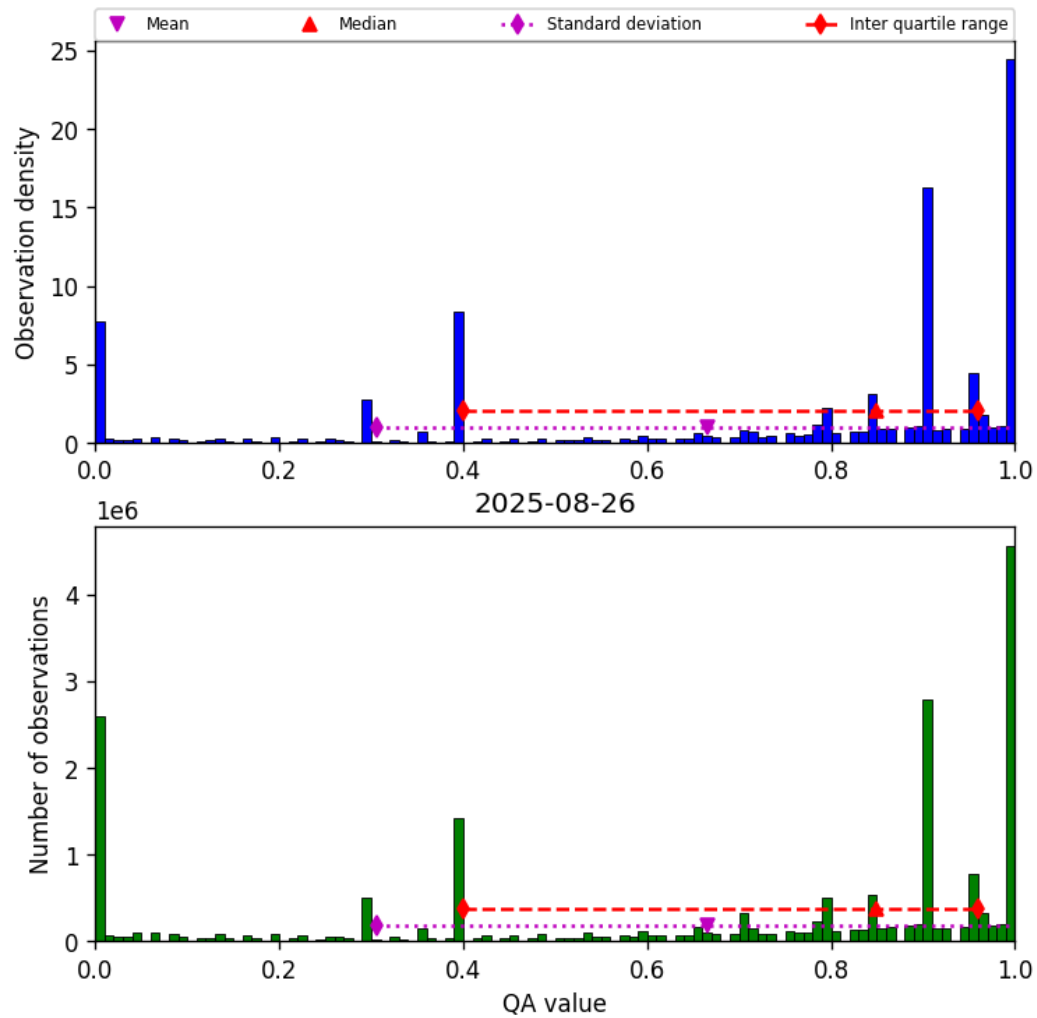
Figure 38: Histogram of “QA value” for 2025-08-25 to 2025-08-27
