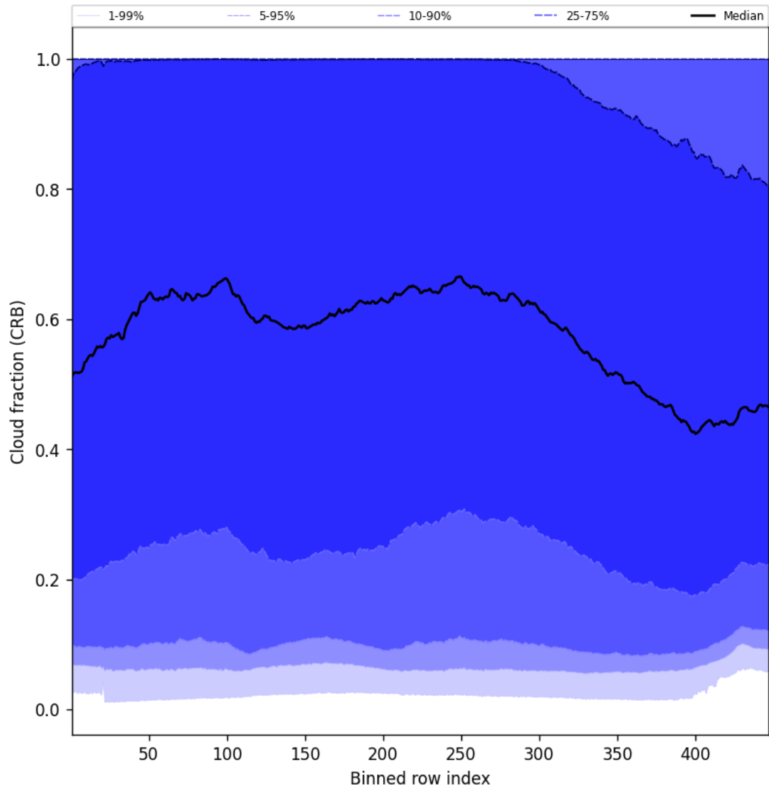
Figure 58: Along track statistics of “Cloud fraction (CRB)” for 2025-08-25 to 2025-08-27
