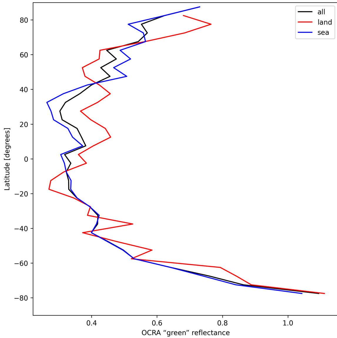
Figure 36: Zonal average of “OCRA “green” reflectance” for 2025-08-25 to 2025-08-27.
