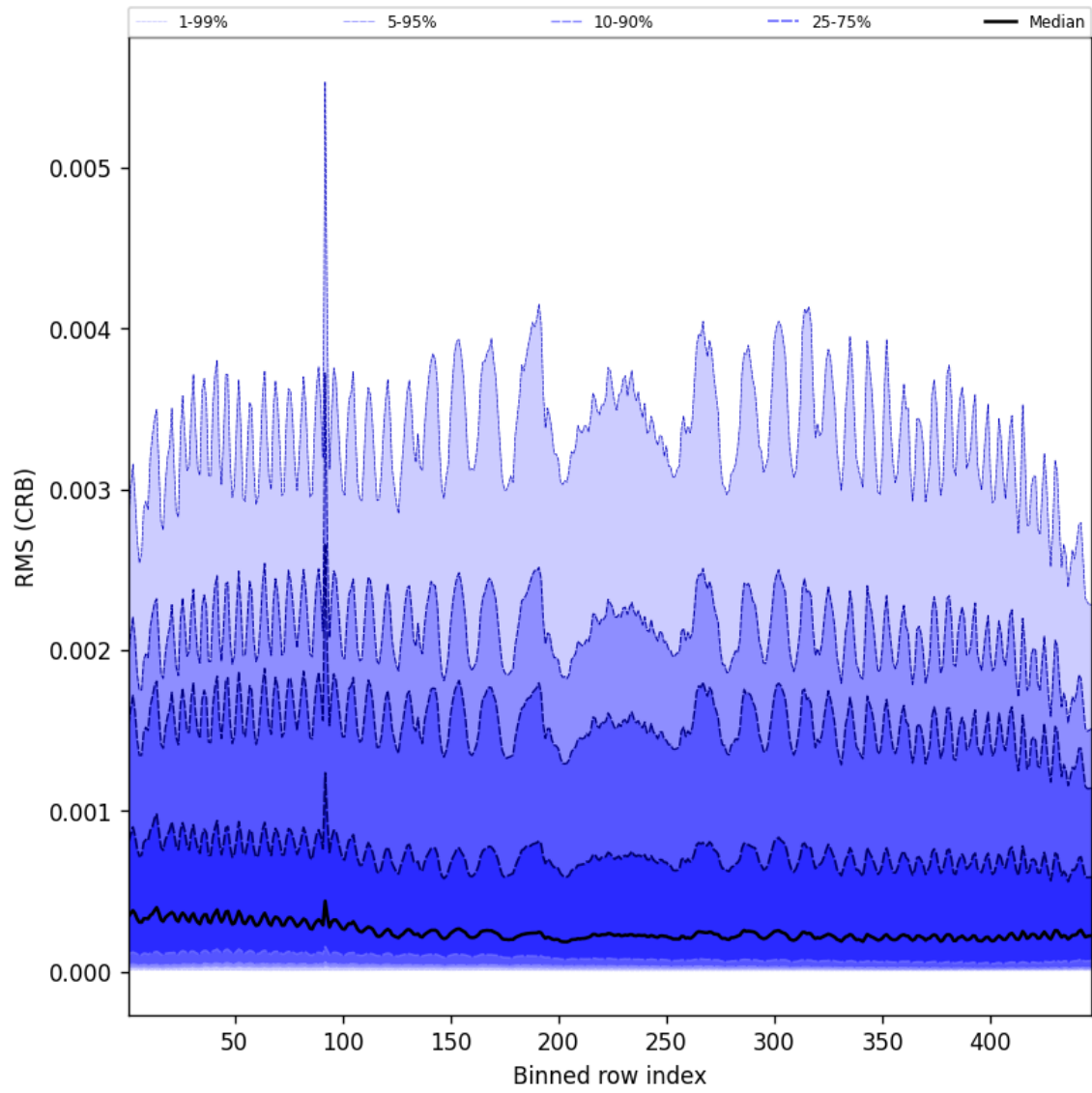
Figure 64: Along track statistics of “RMS (CRB)” for 2025-08-25 to 2025-08-27
