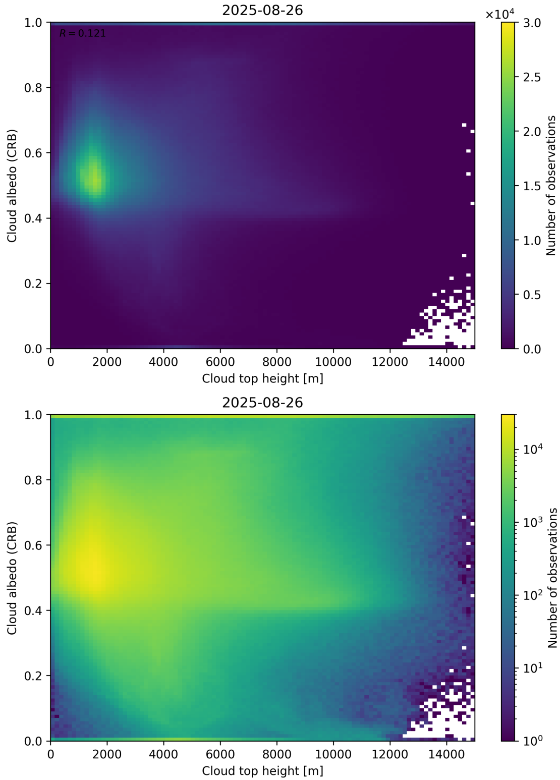
Figure 86: Scatter density plot of “Cloud top height” against “Cloud albedo (CRB)” for 2025-08-25 to 2025-08-27.
