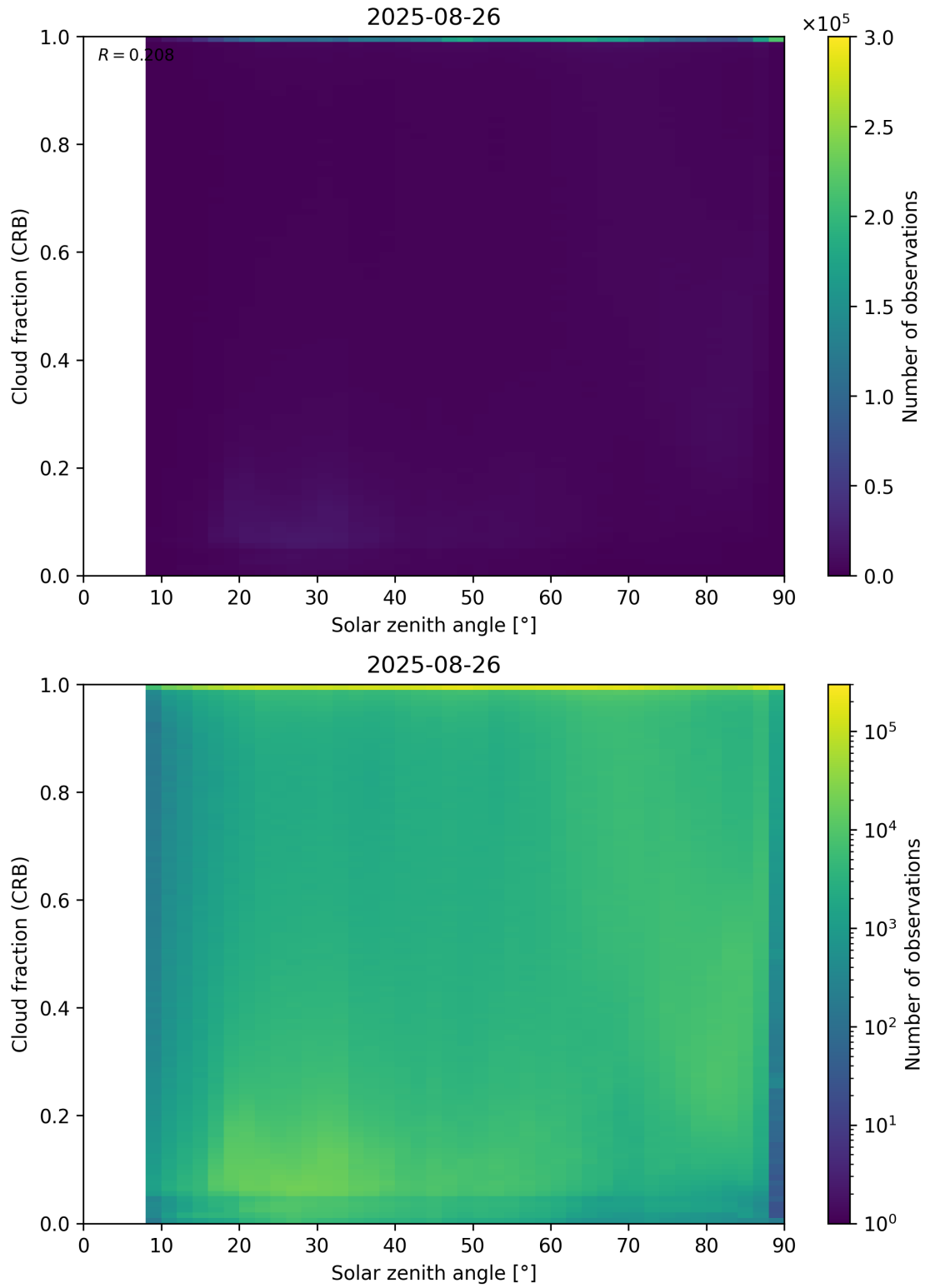
Figure 101: Scatter density plot of “Solar zenith angle” against “Cloud fraction (CRB)” for 2025-08-25 to 2025-08-27.
