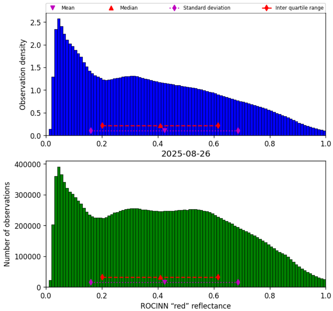
Figure 53: Histogram of “ROCINN “red” reflectance” for 2025-08-25 to 2025-08-27
