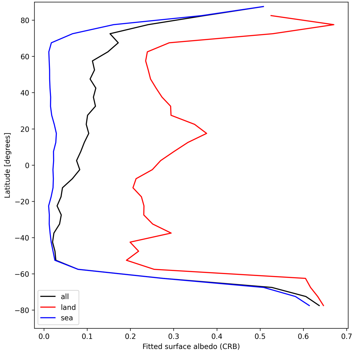
Figure 30: Zonal average of “Fitted surface albedo (CRB)” for 2025-08-25 to 2025-08-27.
