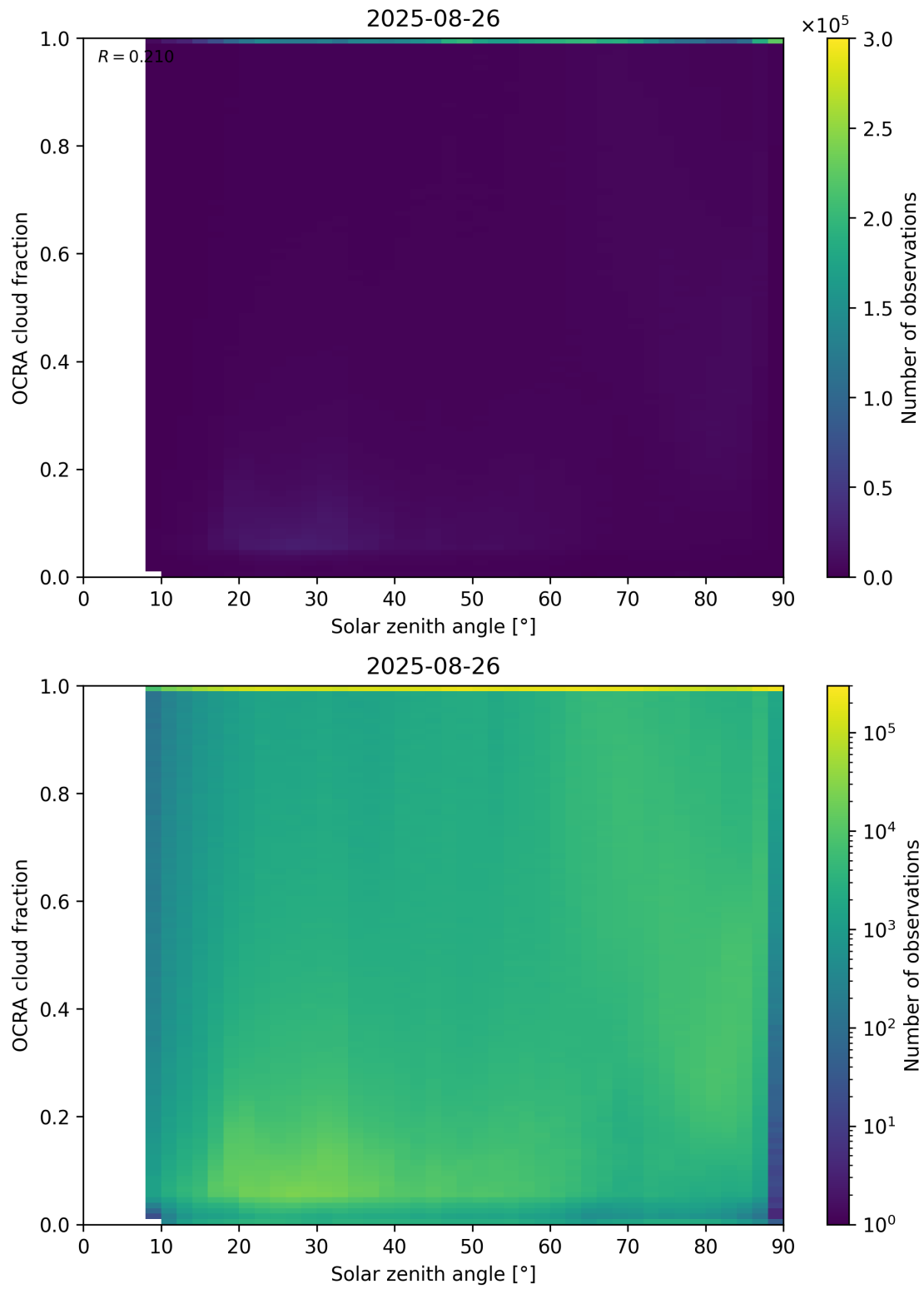
Figure 100: Scatter density plot of “Solar zenith angle” against “OCRA cloud fraction” for 2025-08-25 to 2025-08-27.
