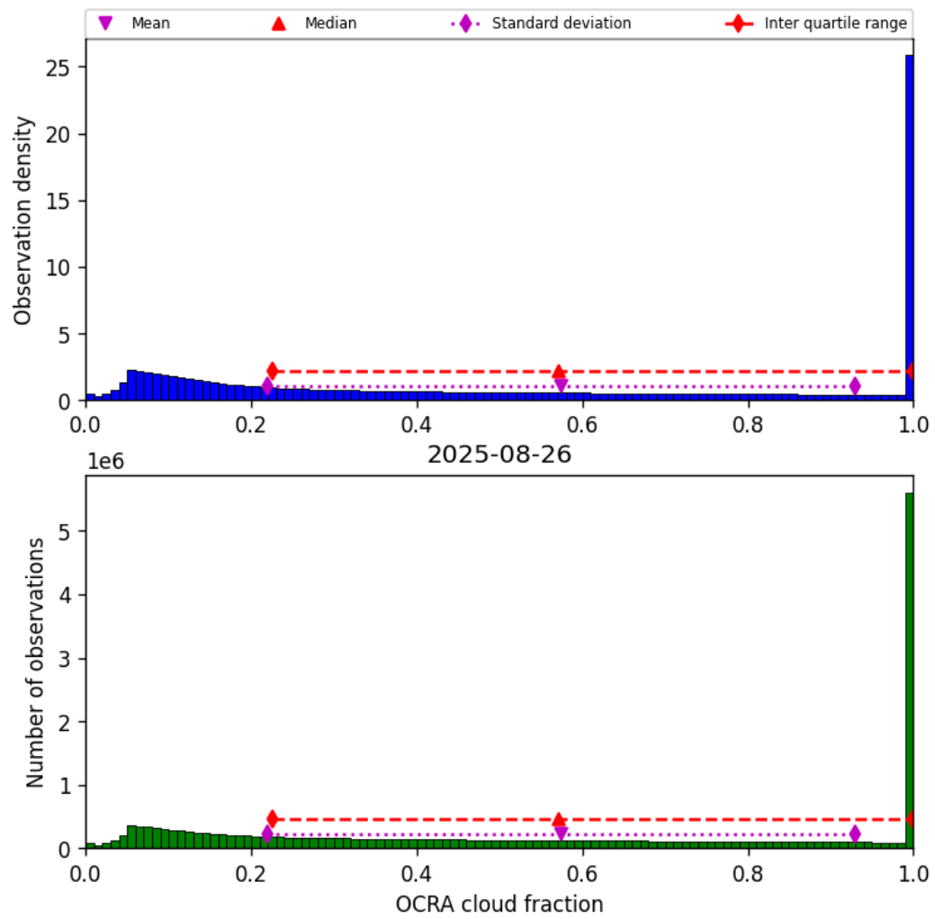
Figure 50: Histogram of “OCRA cloud fraction” for 2025-08-25 to 2025-08-27
