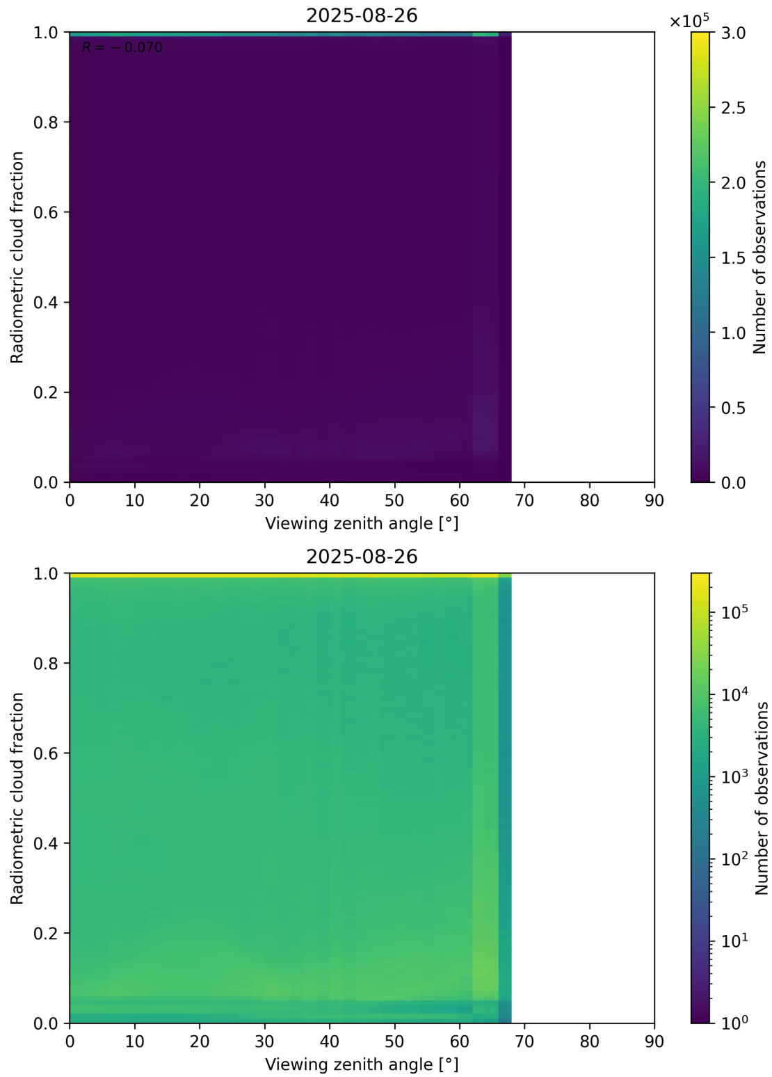
Figure 107: Scatter density plot of “Viewing zenith angle” against “Radiometric cloud fraction” for 2025-08-25 to 2025-08-27.
