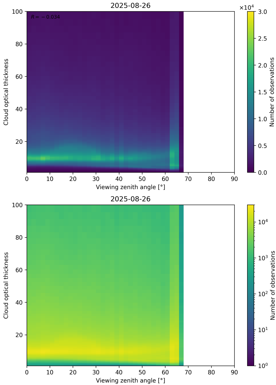
Figure 111: Scatter density plot of “Viewing zenith angle” against “Cloud optical thickness” for 2025-08-25 to 2025-08-27.
