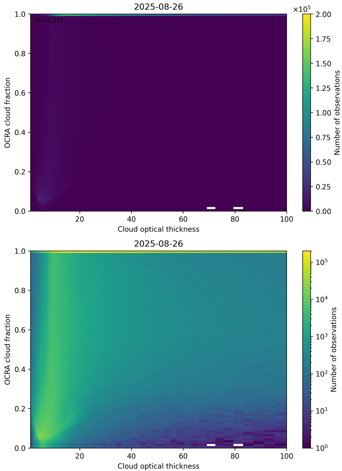
Figure 83: Scatter density plot of “Cloud optical thickness” against “OCRA cloud fraction” for 2025-08-25 to 2025-08-27.
