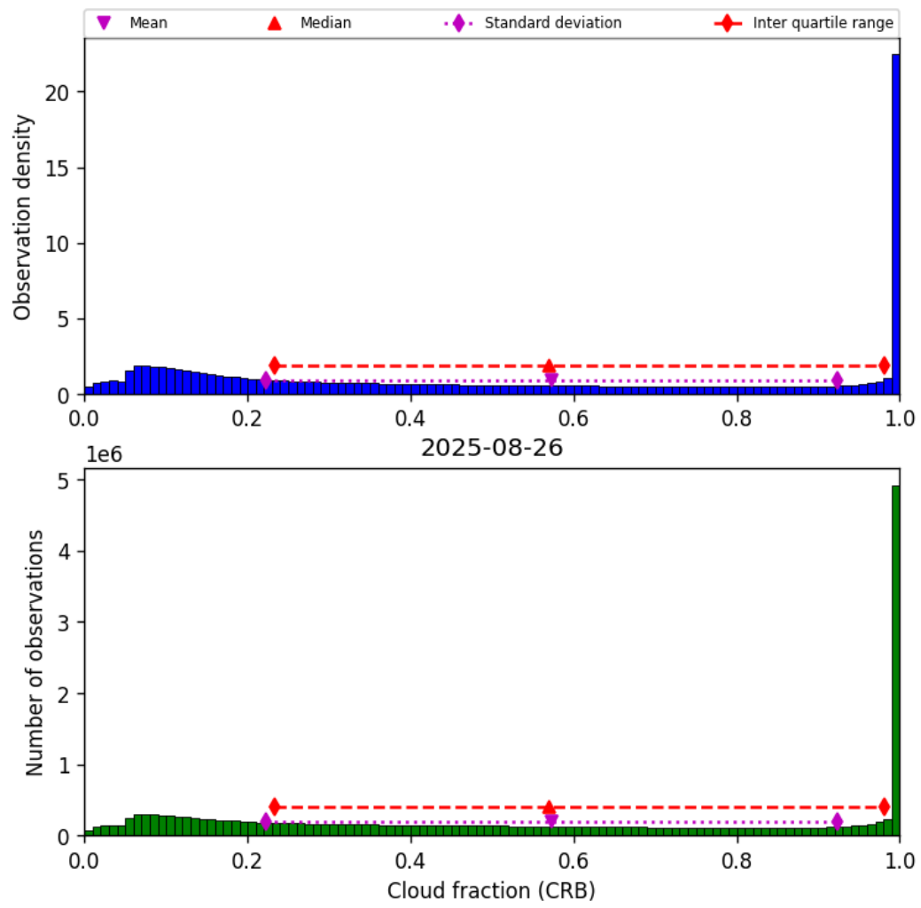
Figure 42: Histogram of “Cloud fraction (CRB)” for 2025-08-25 to 2025-08-27
