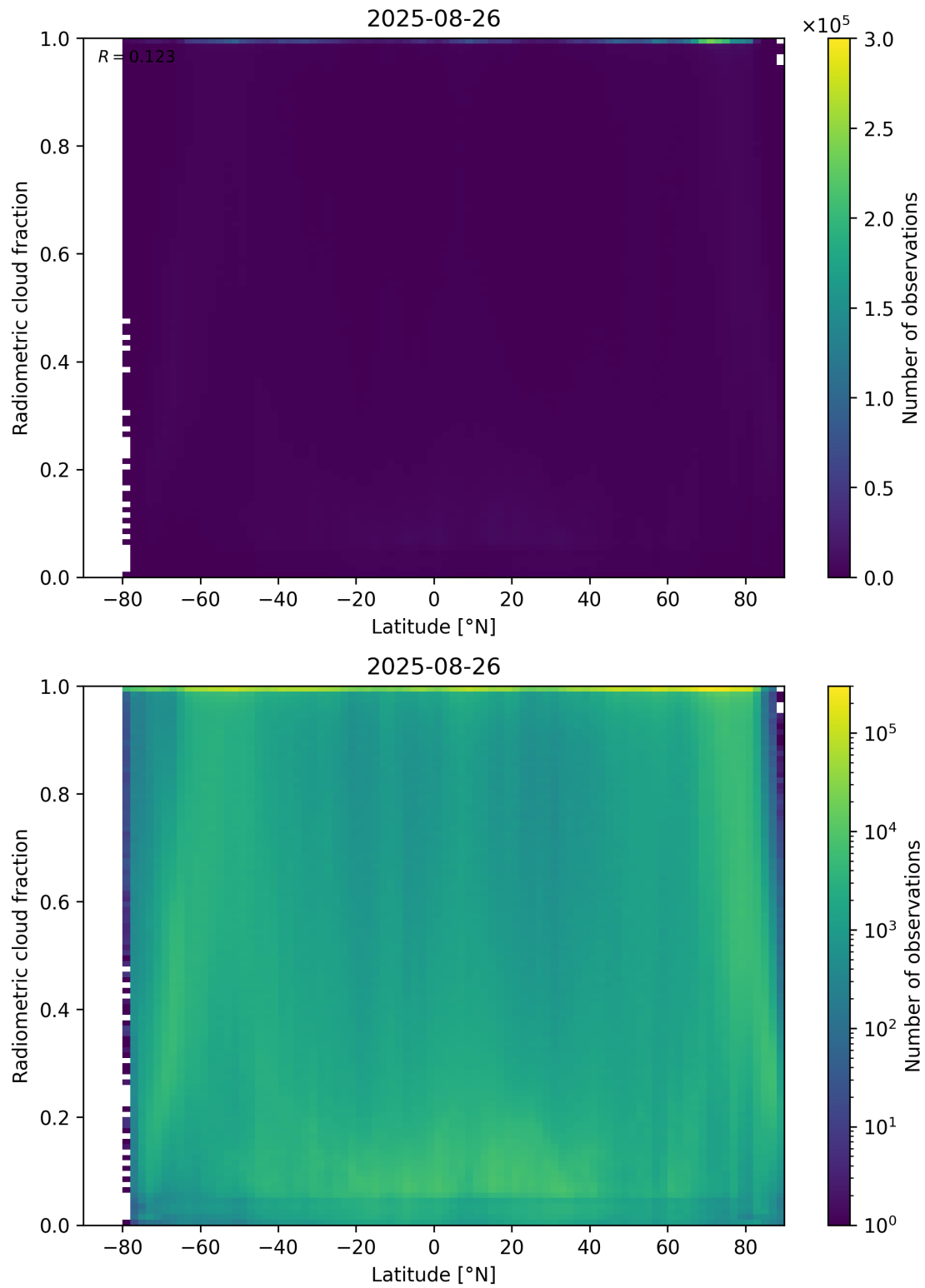
Figure 92: Scatter density plot of “Latitude” against “Radiometric cloud fraction” for 2025-08-25 to 2025-08-27.
