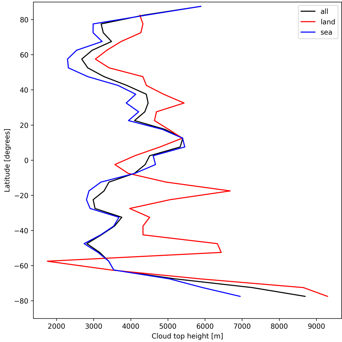
Figure 24: Zonal average of “Cloud top height” for 2025-08-25 to 2025-08-27.
