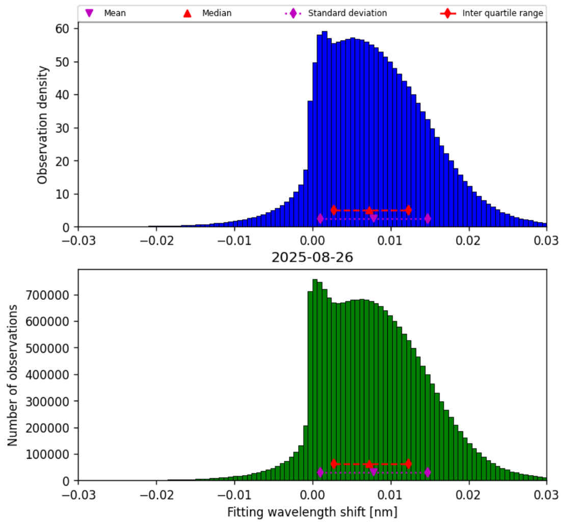
Figure 49: Histogram of “Fitting wavelength shift” for 2025-08-25 to 2025-08-27
