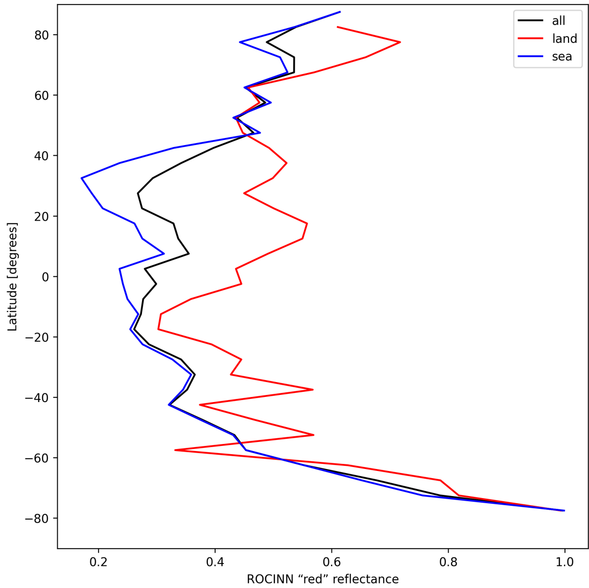
Figure 37: Zonal average of “ROCINN “red” reflectance” for 2025-08-25 to 2025-08-27.
