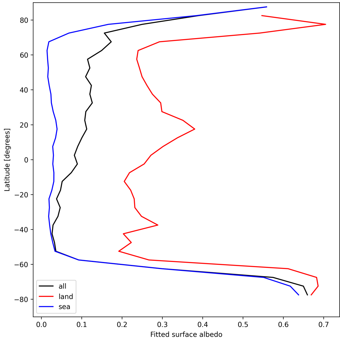
Figure 29: Zonal average of “Fitted surface albedo” for 2025-08-25 to 2025-08-27.
