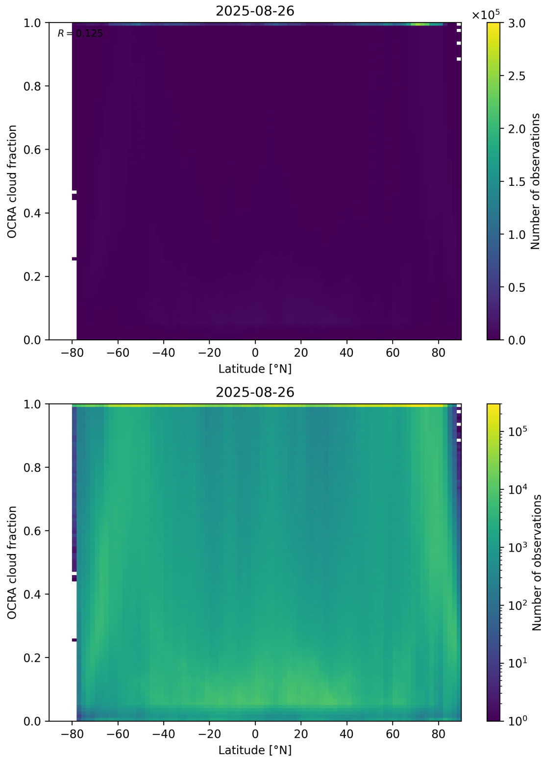
Figure 93: Scatter density plot of “Latitude” against “OCRA cloud fraction” for 2025-08-25 to 2025-08-27.
