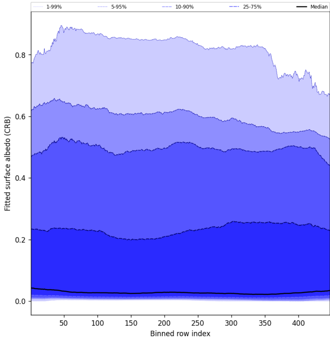
Figure 62: Along track statistics of “Fitted surface albedo (CRB)” for 2025-08-25 to 2025-08-27
