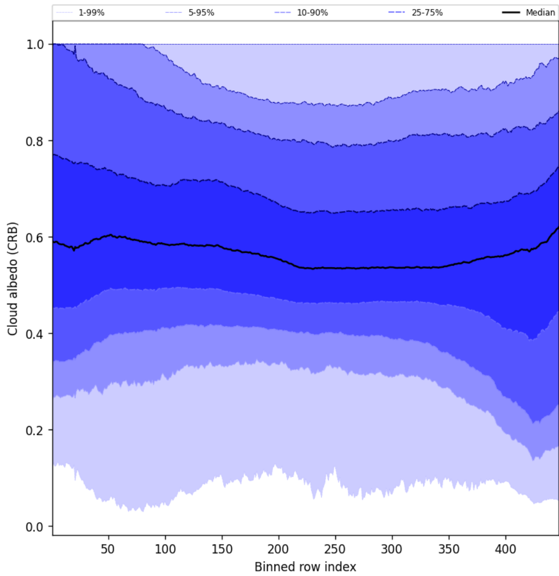
Figure 60: Along track statistics of “Cloud albedo (CRB)” for 2025-08-25 to 2025-08-27
