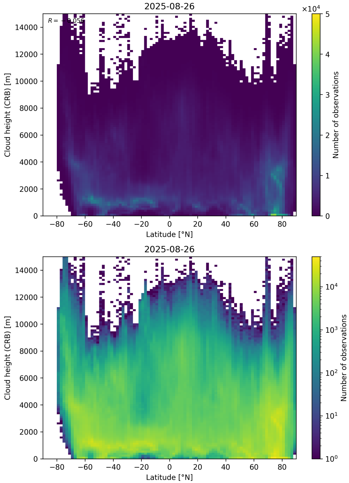
Figure 95: Scatter density plot of “Latitude” against “Cloud height (CRB)” for 2025-08-25 to 2025-08-27.
