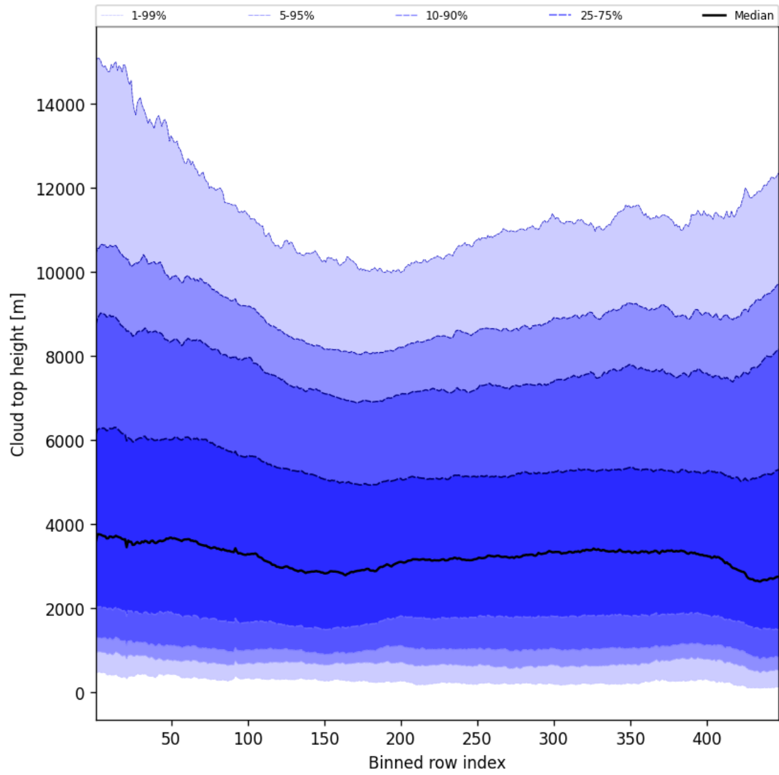
Figure 56: Along track statistics of "Cloud top height" for 2025-08-25 to 2025-08-27
