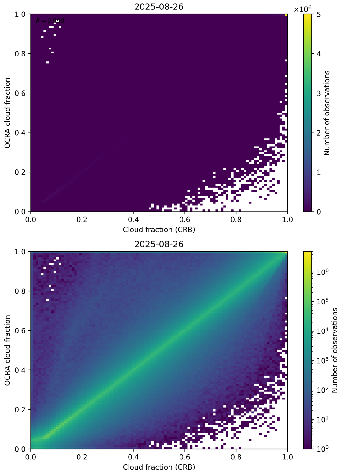
Figure 78: Scatter density plot of “Cloud fraction (CRB)” against “OCRA cloud fraction” for 2025-08-25 to 2025-08-27.
