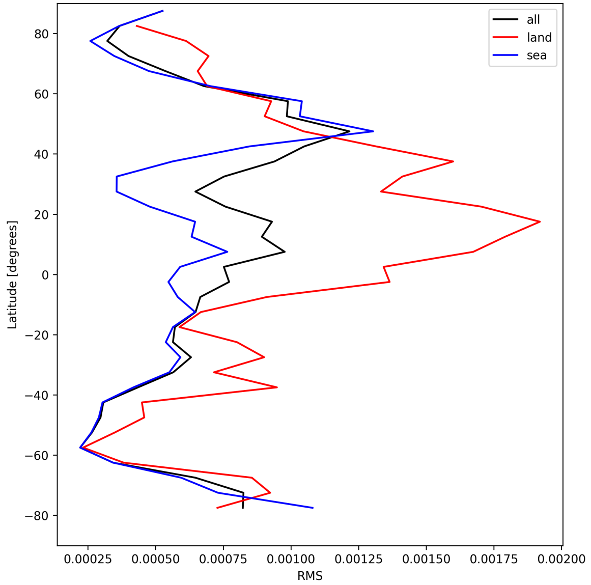
Figure 31: Zonal average of “RMS” for 2025-08-25 to 2025-08-27.
