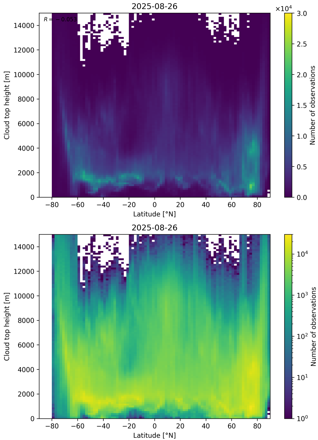
Figure 97: Scatter density plot of “Latitude” against “Cloud top height” for 2025-08-25 to 2025-08-27.
