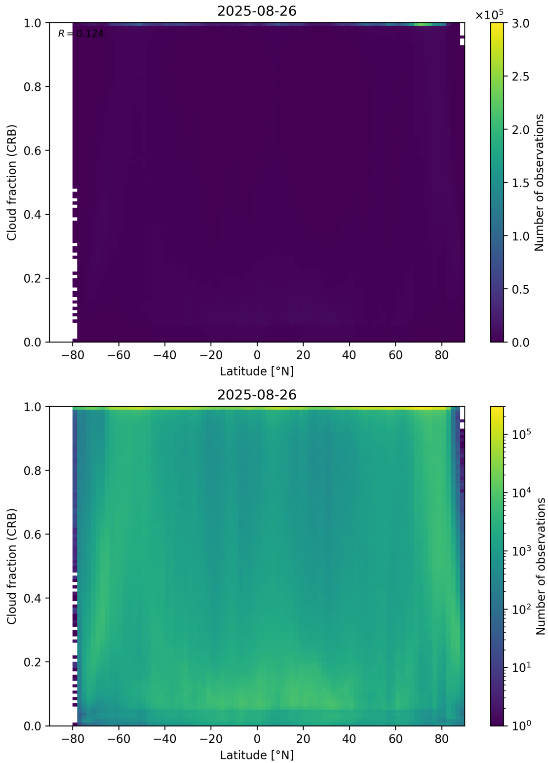
Figure 94: Scatter density plot of “Latitude” against “Cloud fraction (CRB)” for 2025-08-25 to 2025-08-27.
