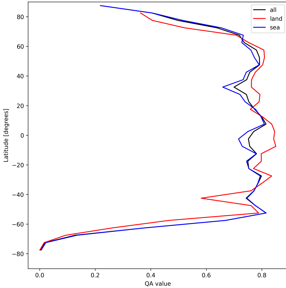
Figure 22: Zonal average of “QA value” for 2025-08-25 to 2025-08-27.
