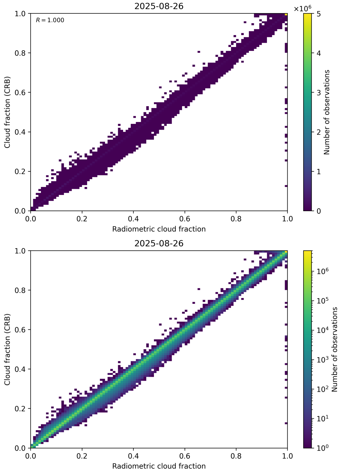
Figure 73: Scatter density plot of “Radiometric cloud fraction” against “Cloud fraction (CRB)” for 2025-08-25 to 2025-08-27.
