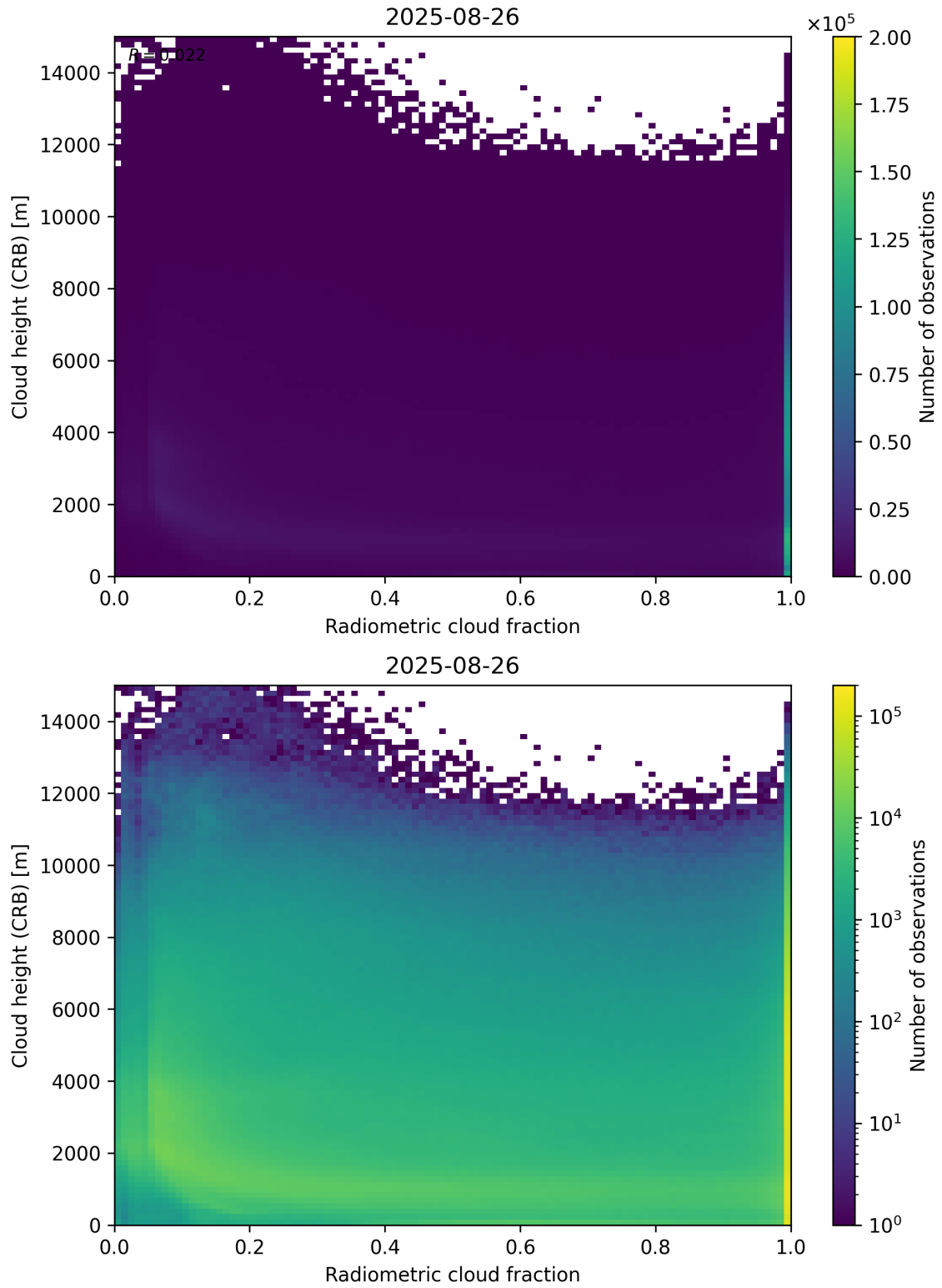
Figure 74: Scatter density plot of “Radiometric cloud fraction” against “Cloud height (CRB)” for 2025-08-25 to 2025-08-27.
