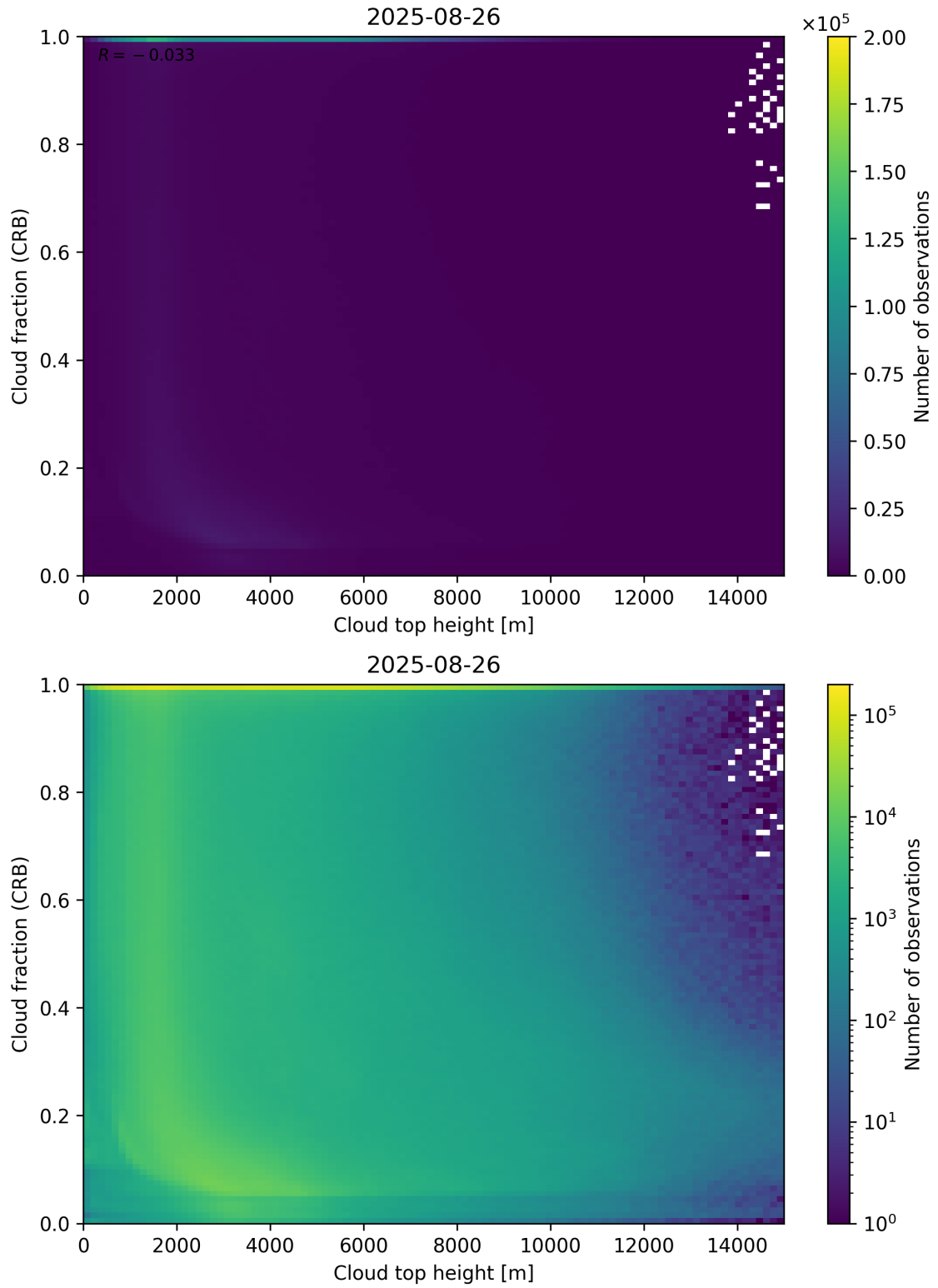
Figure 88: Scatter density plot of “Cloud top height” against “Cloud fraction (CRB)” for 2025-08-25 to 2025-08-27.
