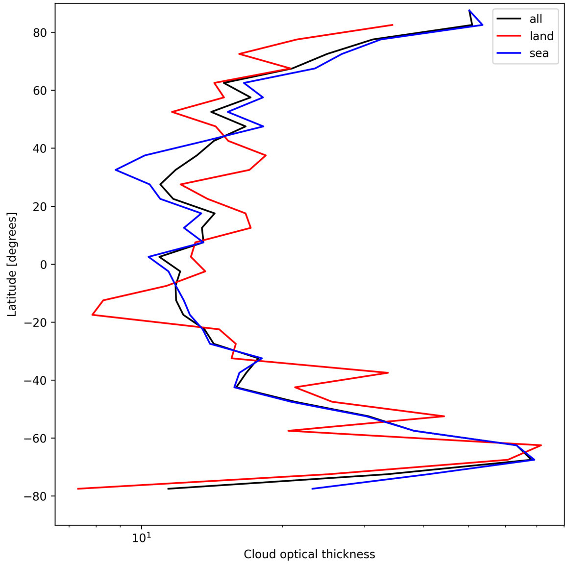
Figure 25: Zonal average of “Cloud optical thickness” for 2025-08-25 to 2025-08-27.
