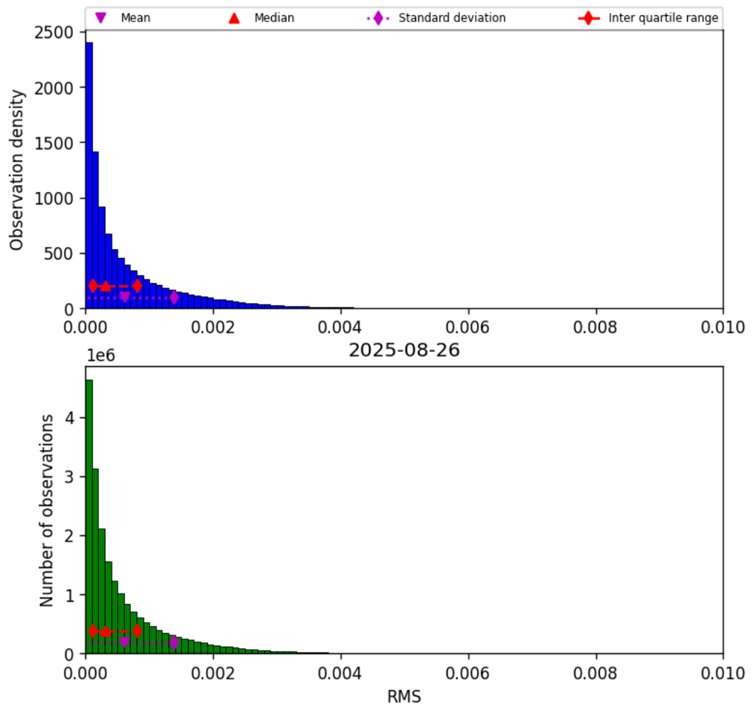
Figure 47: Histogram of “RMS” for 2025-08-25 to 2025-08-27
