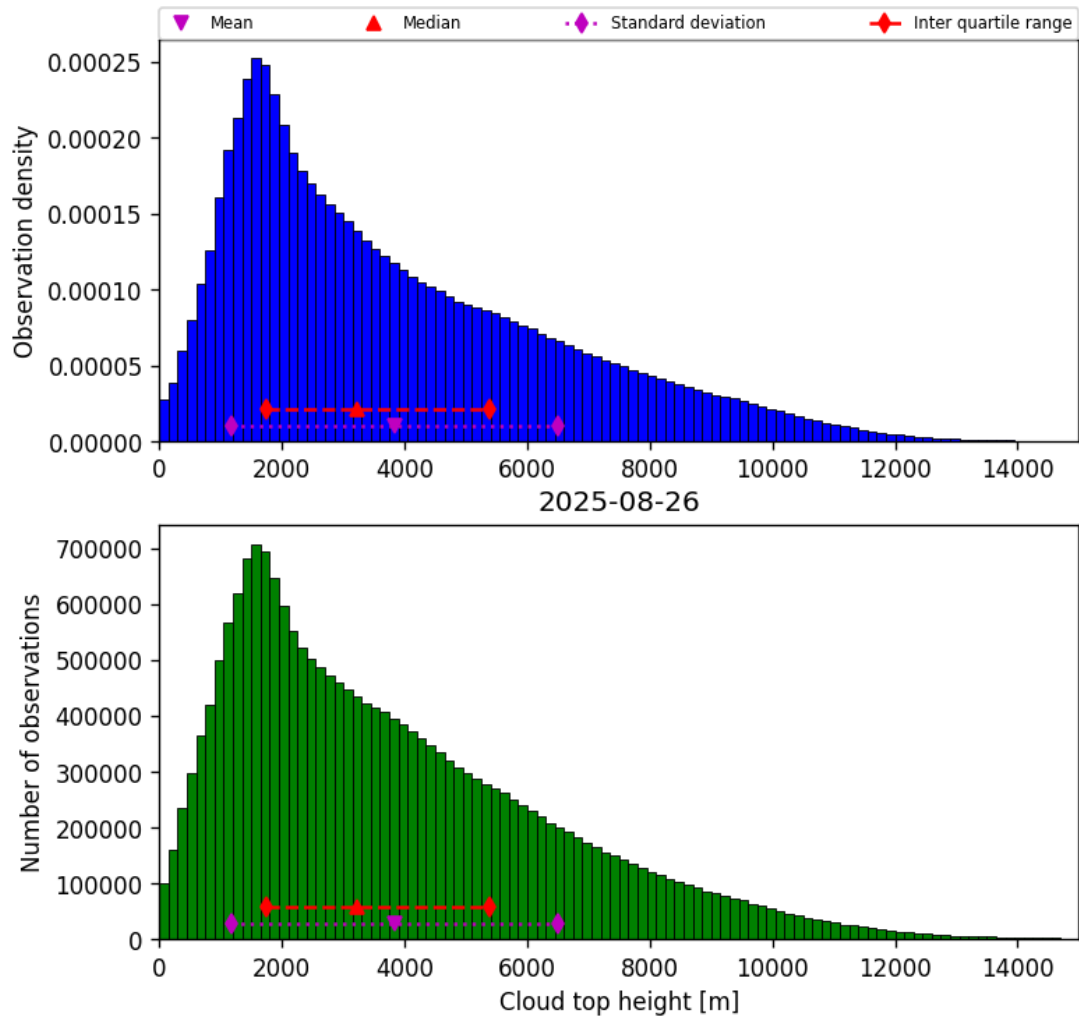
Figure 40: Histogram of “Cloud top height” for 2025-08-25 to 2025-08-27
