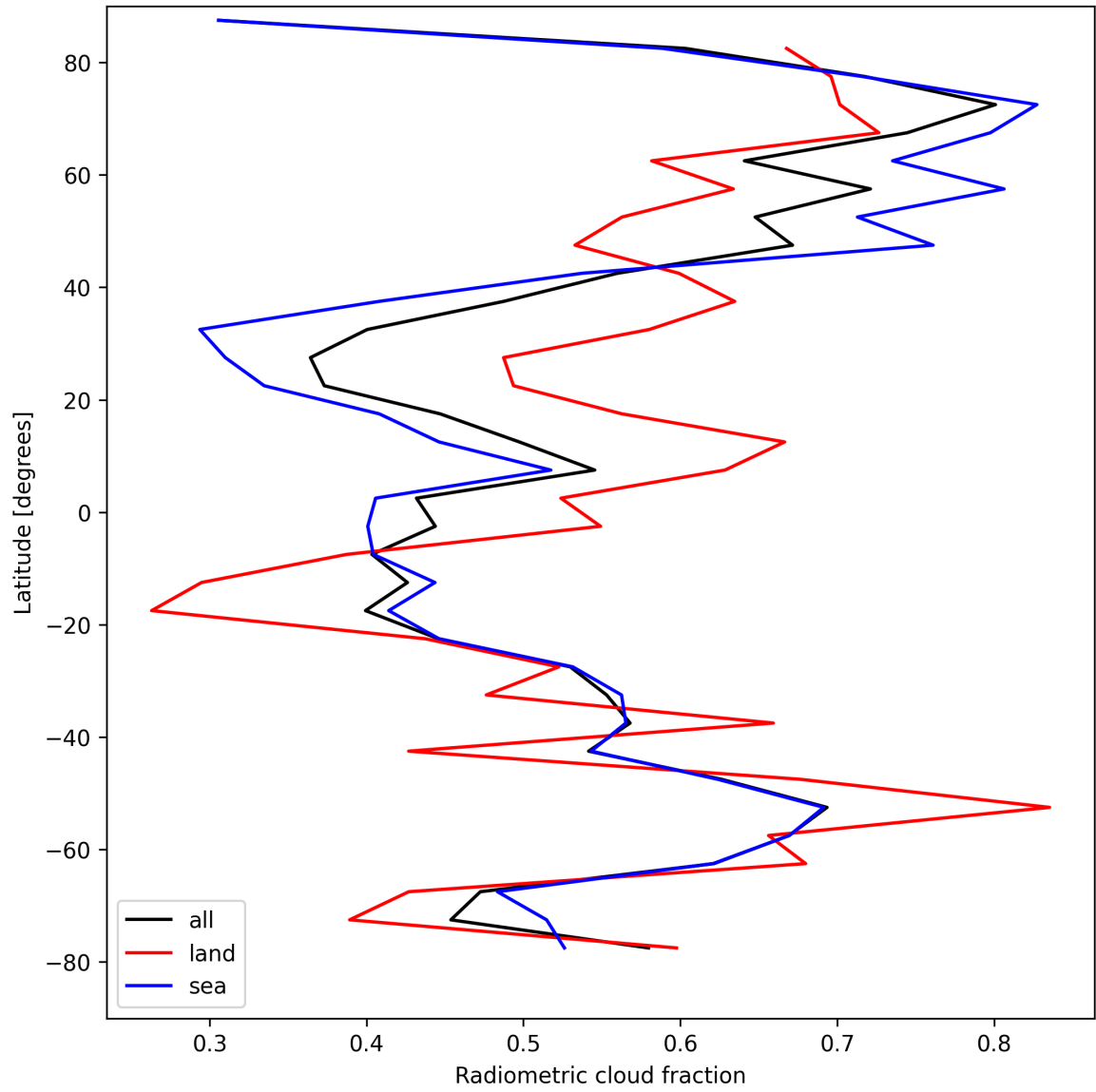
Figure 23: Zonal average of “Radiometric cloud fraction” for 2025-08-25 to 2025-08-27.
