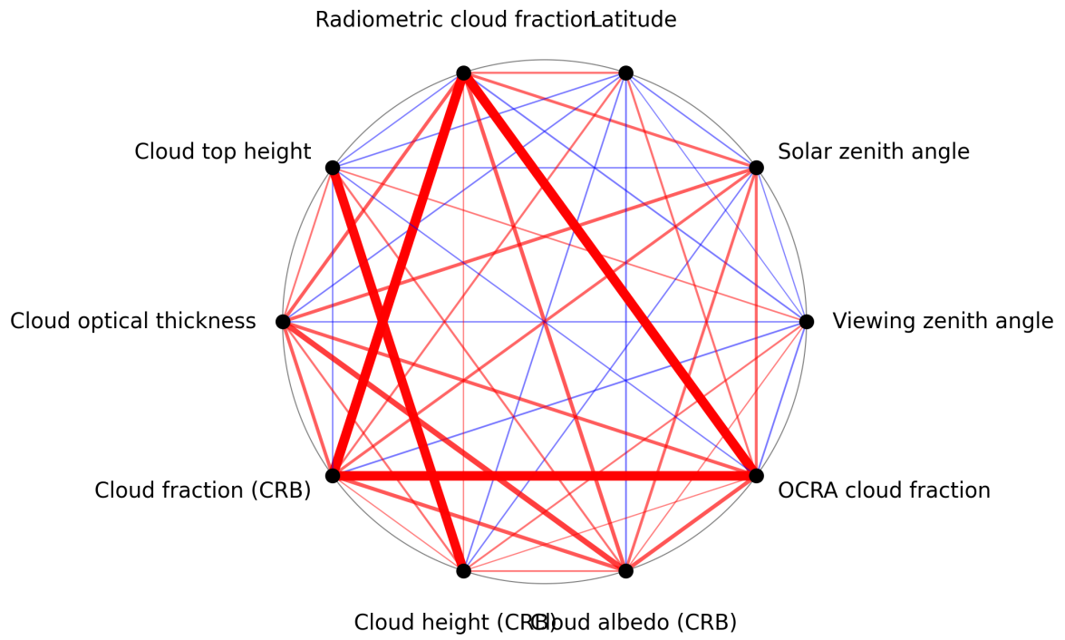
Figure 1: Map of correlation graph for 2025-08-25 to 2025-08-27.
