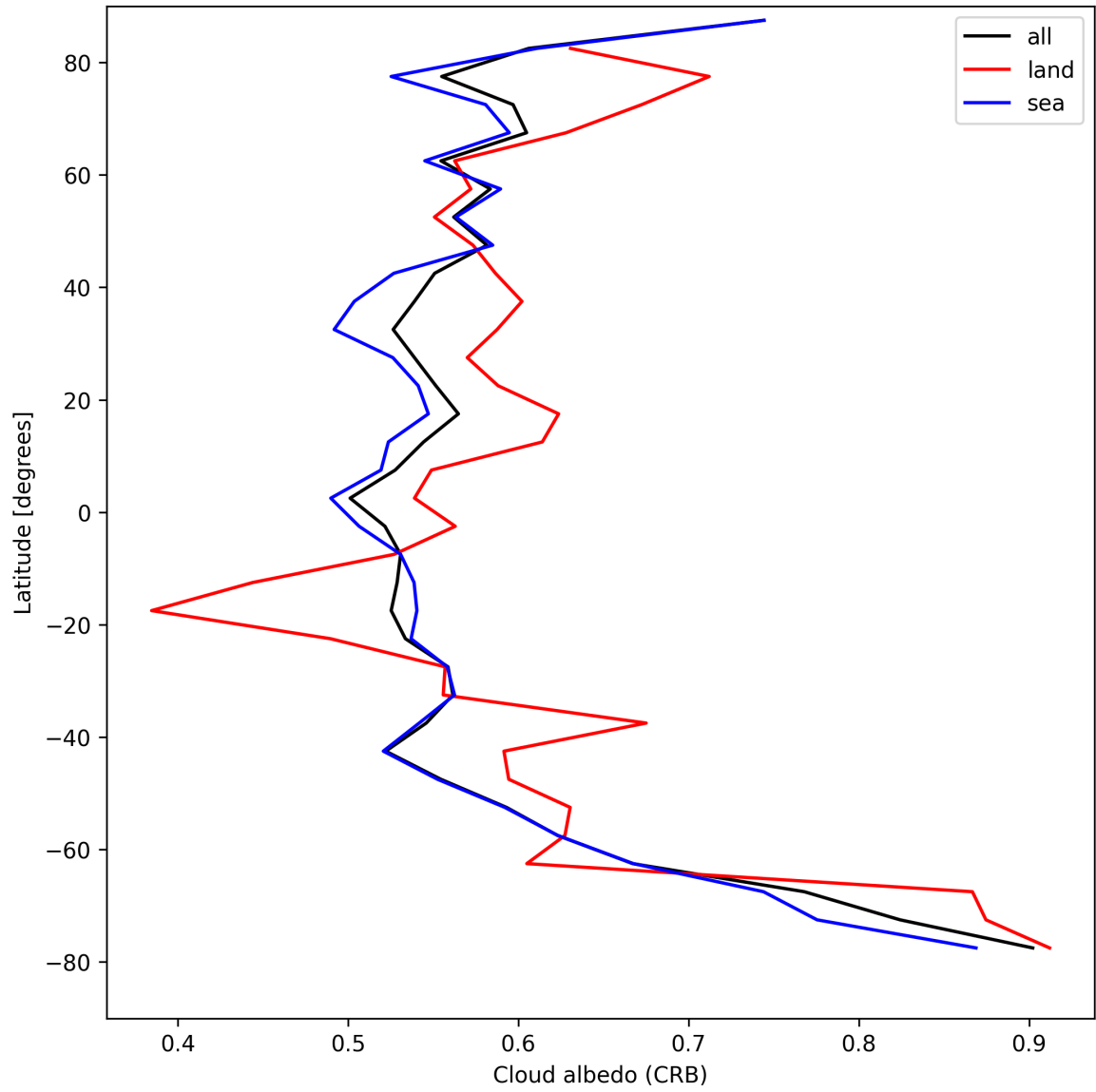
Figure 28: Zonal average of “Cloud albedo (CRB)” for 2025-08-25 to 2025-08-27.
