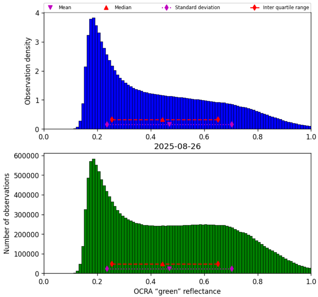
Figure 52: Histogram of “OCRA “green” reflectance” for 2025-08-25 to 2025-08-27
