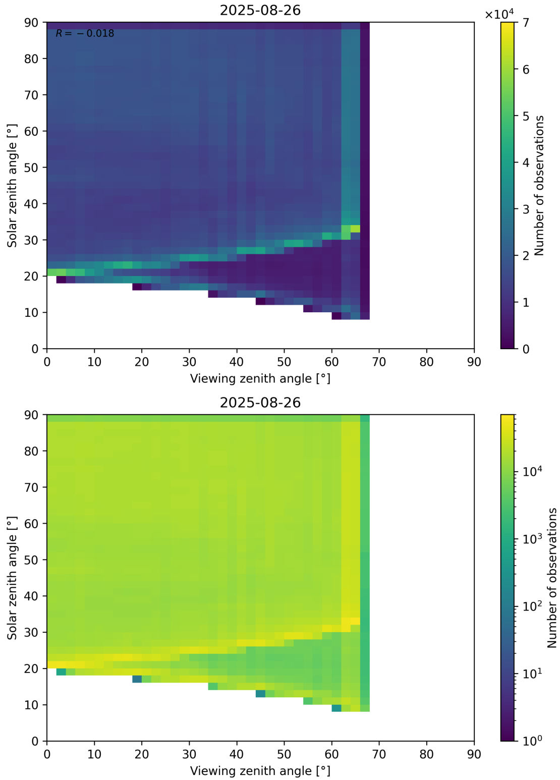
Figure 114: Scatter density plot of “Viewing zenith angle” against “Solar zenith angle” for 2025-08-25 to 2025-08-27.
