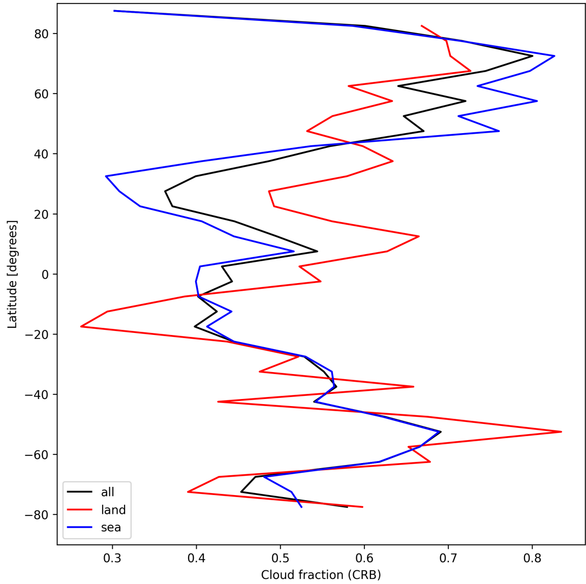
Figure 26: Zonal average of “Cloud fraction (CRB)” for 2025-08-25 to 2025-08-27.
