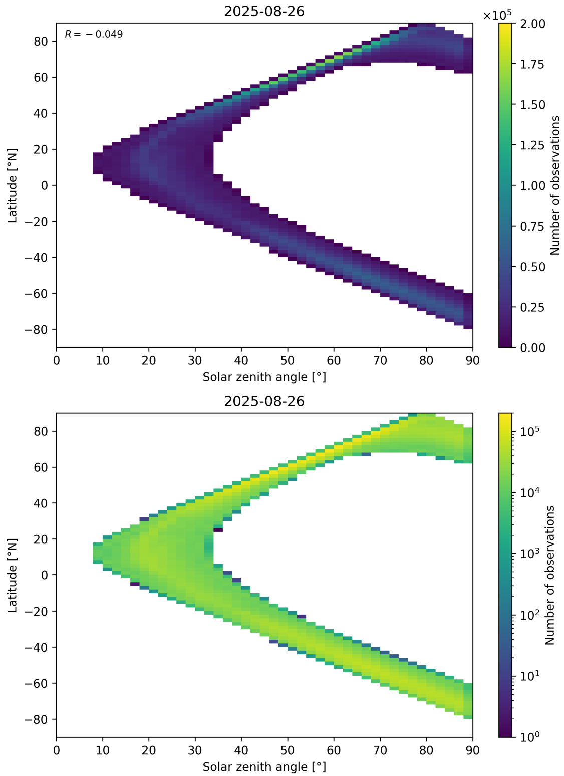
Figure 105: Scatter density plot of “Solar zenith angle” against “Latitude” for 2025-08-25 to 2025-08-27.
