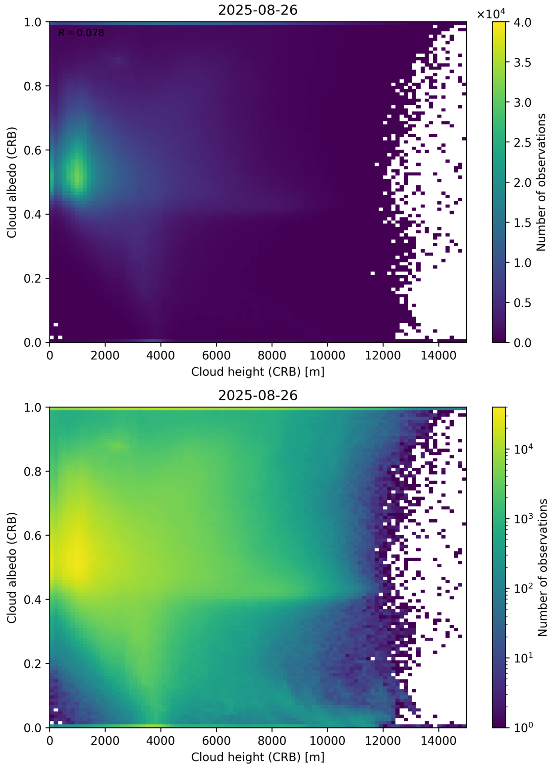
Figure 80: Scatter density plot of “Cloud height (CRB)” against “Cloud albedo (CRB)” for 2025-08-25 to 2025-08-27.
