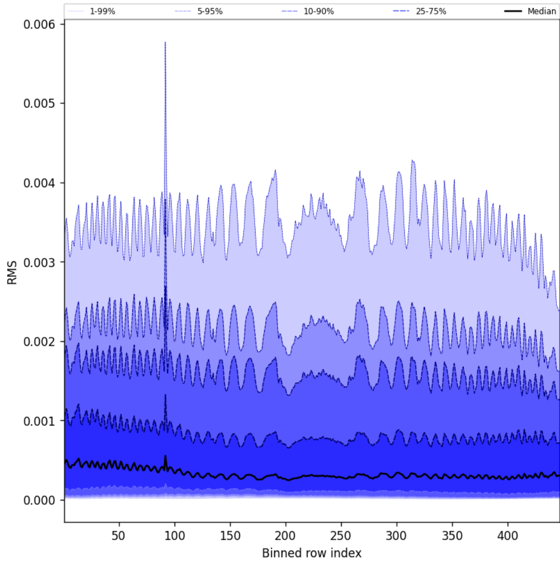
Figure 63: Along track statistics of “RMS” for 2025-08-25 to 2025-08-27
