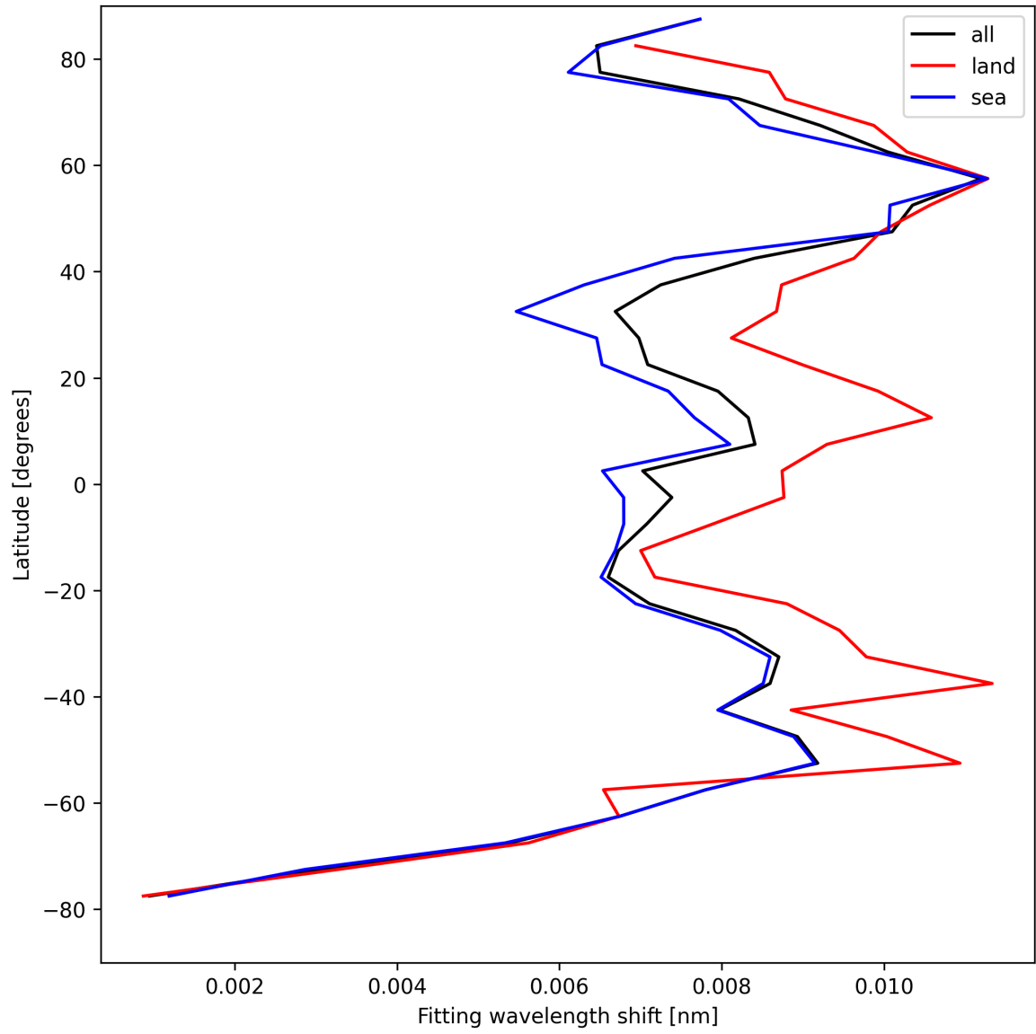
Figure 33: Zonal average of “Fitting wavelength shift” for 2025-08-25 to 2025-08-27.
