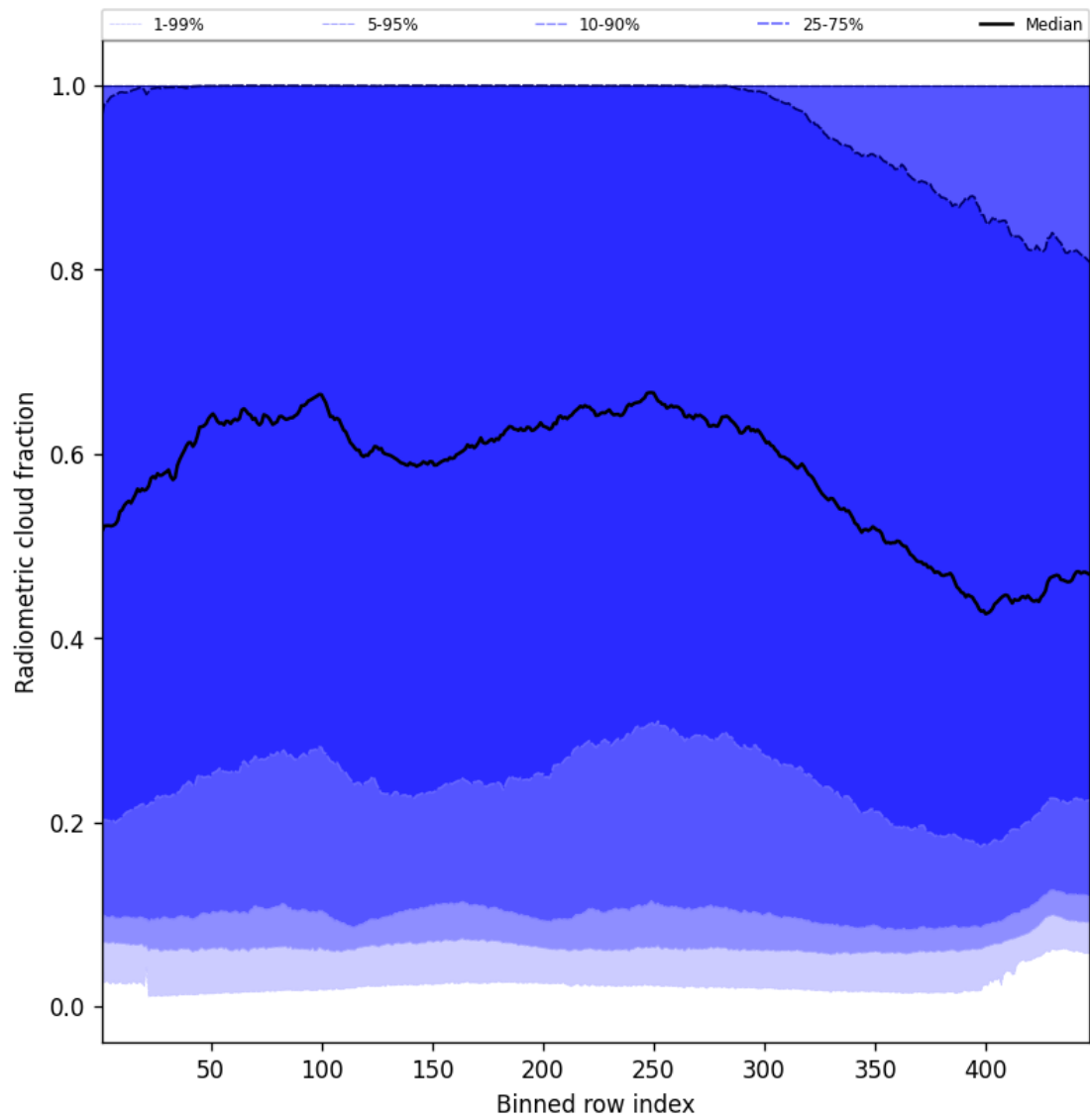
Figure 55: Along track statistics of “Radiometric cloud fraction” for 2025-08-25 to 2025-08-27
