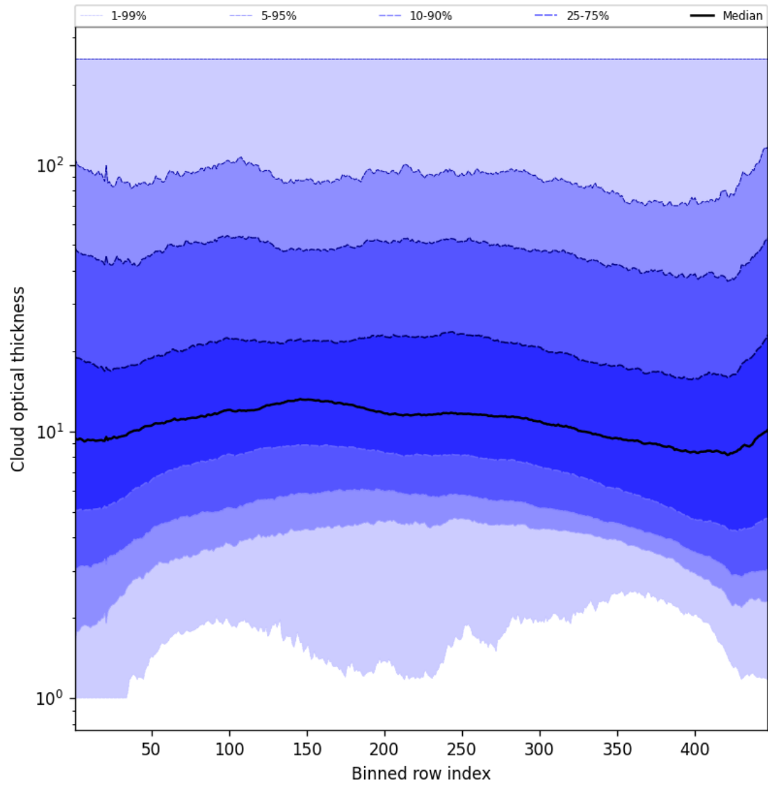
Figure 57: Along track statistics of “Cloud optical thickness” for 2025-08-25 to 2025-08-27
