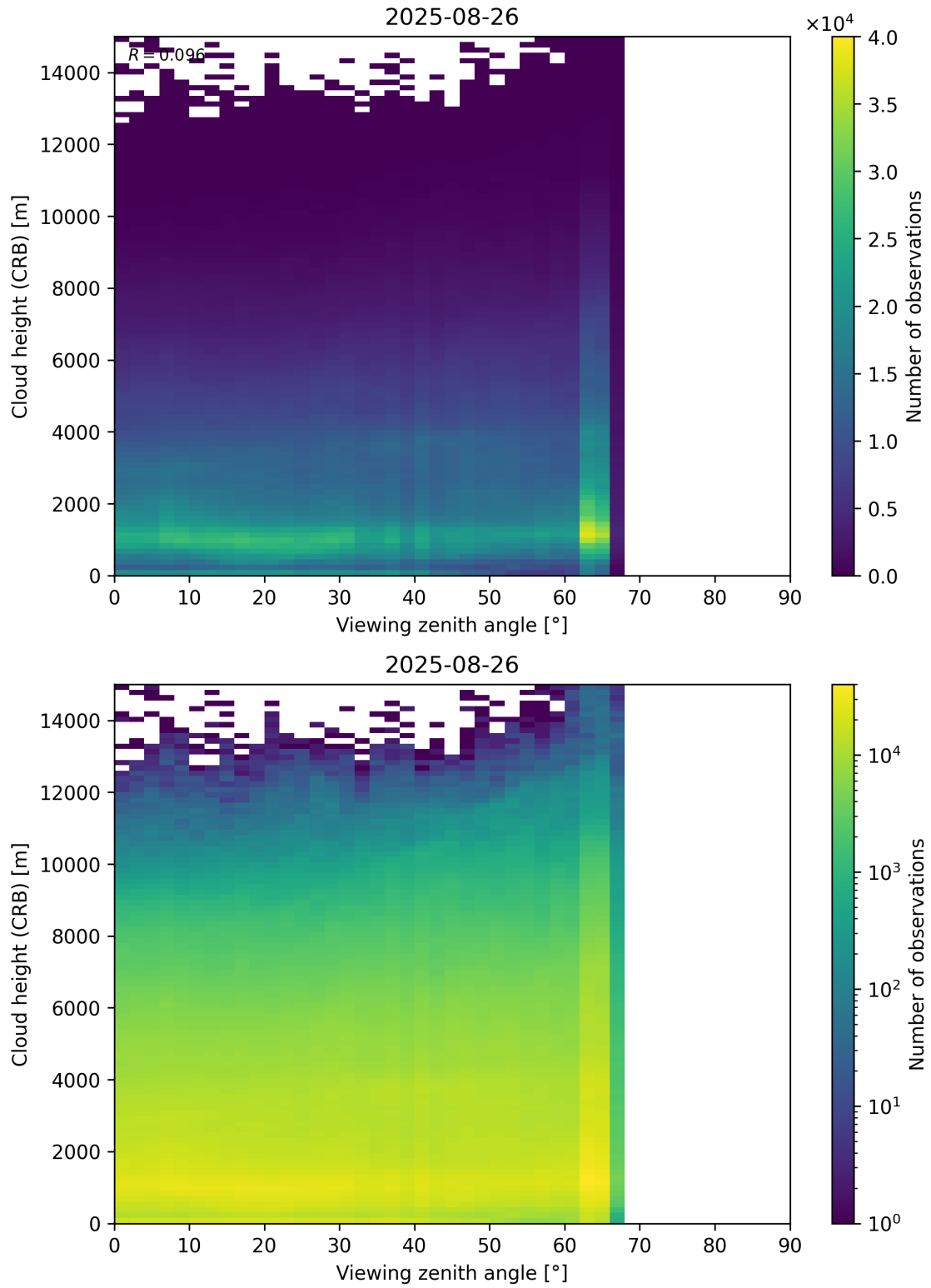
Figure 110: Scatter density plot of “Viewing zenith angle” against “Cloud height (CRB)” for 2025-08-25 to 2025-08-27.
