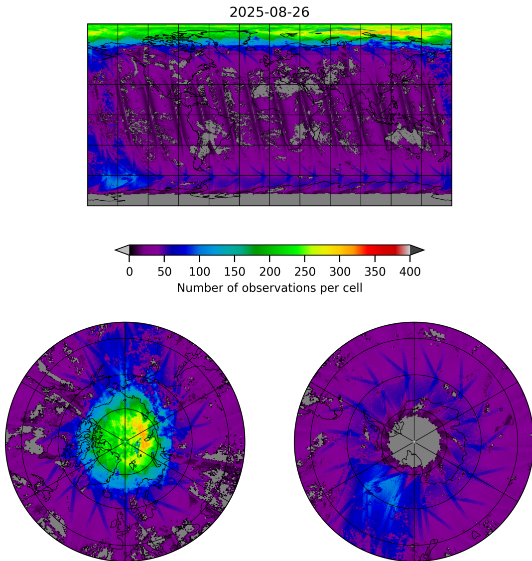
Figure 21: Map of the number of observations for 2025-08-25 to 2025-08-27
