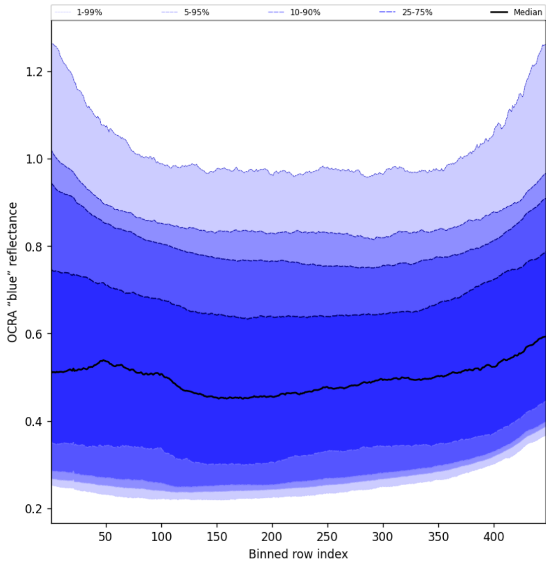
Figure 67: Along track statistics of “OCRA “blue” reflectance” for 2025-08-25 to 2025-08-27
