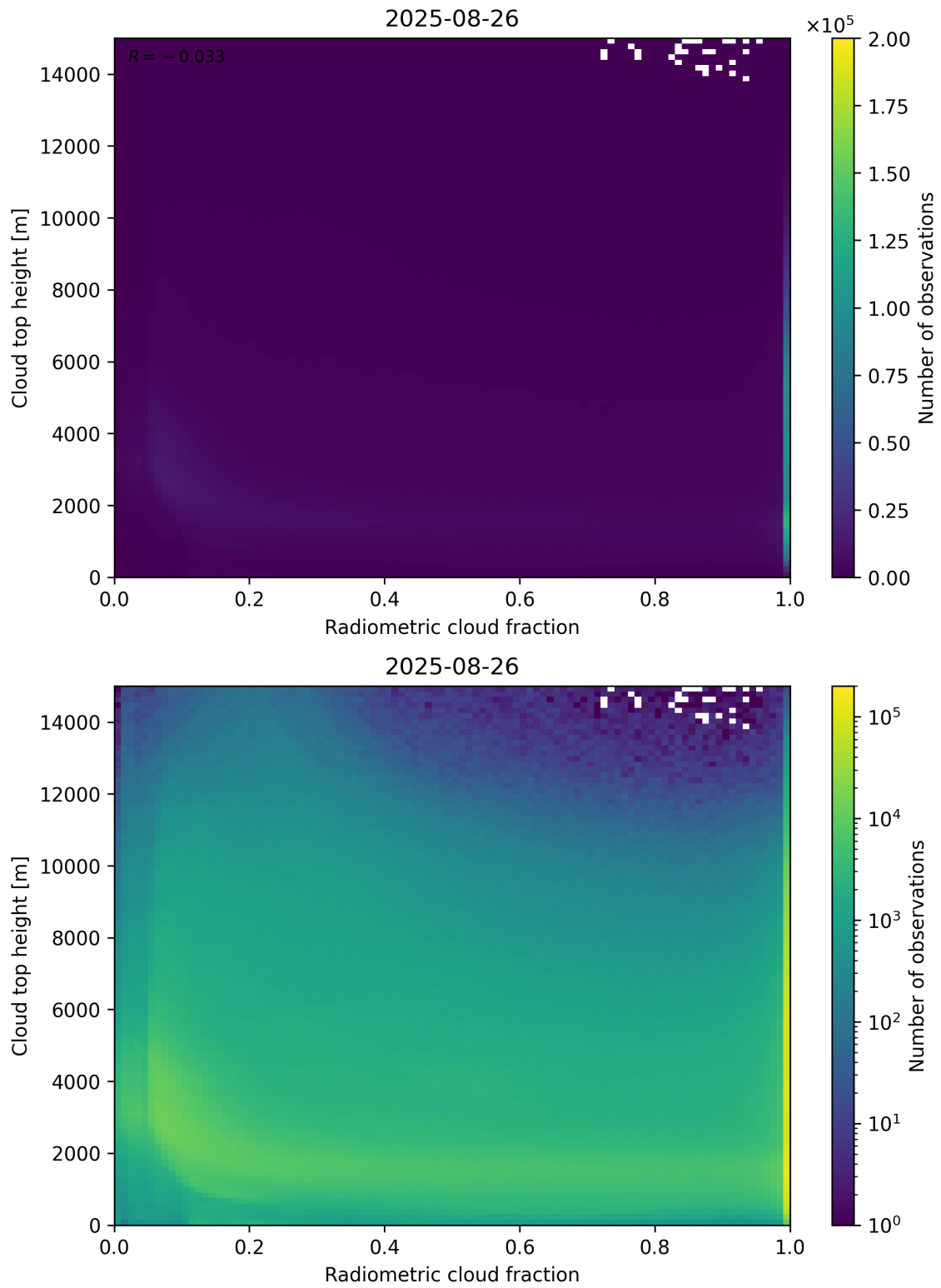
Figure 76: Scatter density plot of “Radiometric cloud fraction” against “Cloud top height” for 2025-08-25 to 2025-08-27.
