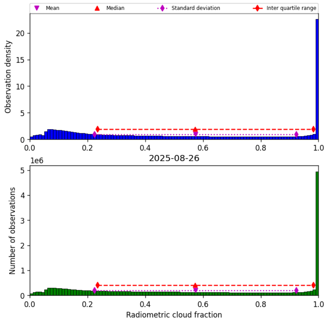
Figure 39: Histogram of “Radiometric cloud fraction” for 2025-08-25 to 2025-08-27
