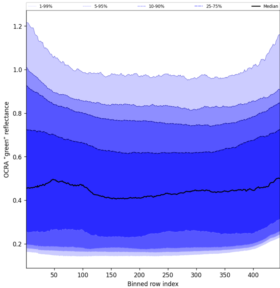
Figure 68: Along track statistics of “OCRA “green” reflectance” for 2025-08-25 to 2025-08-27
