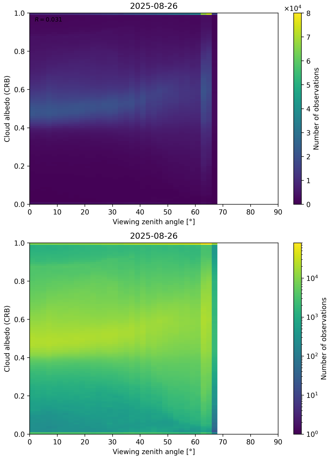
Figure 106: Scatter density plot of “Viewing zenith angle” against “Cloud albedo (CRB)” for 2025-08-25 to 2025-08-27.
