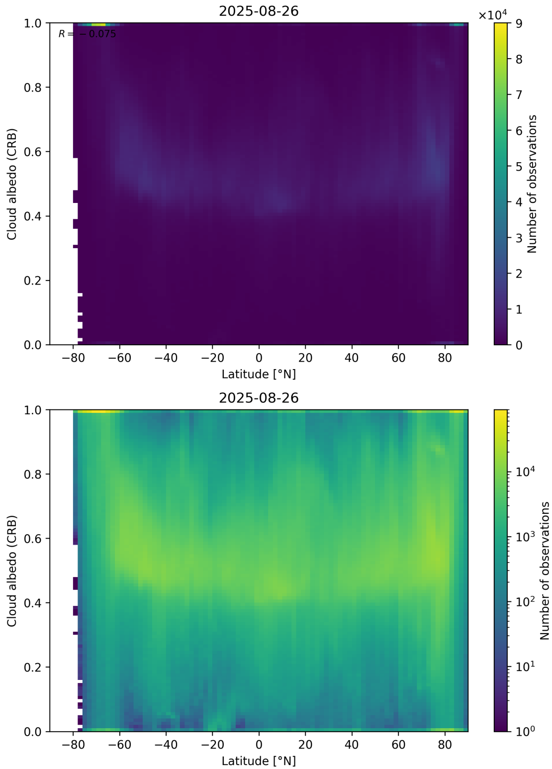
Figure 91: Scatter density plot of “Latitude” against “Cloud albedo (CRB)” for 2025-08-25 to 2025-08-27.
