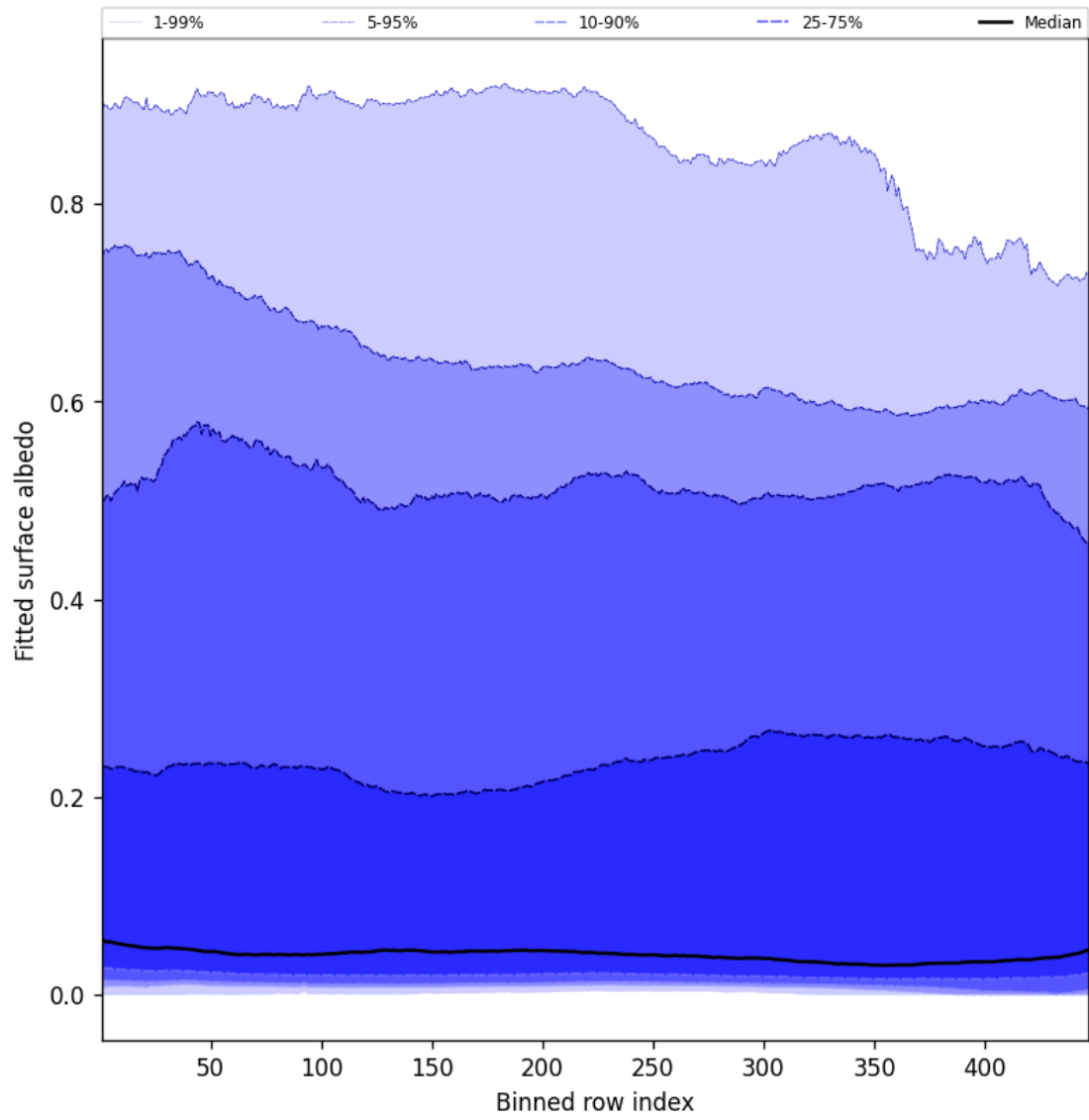
Figure 61: Along track statistics of “Fitted surface albedo” for 2025-08-25 to 2025-08-27
