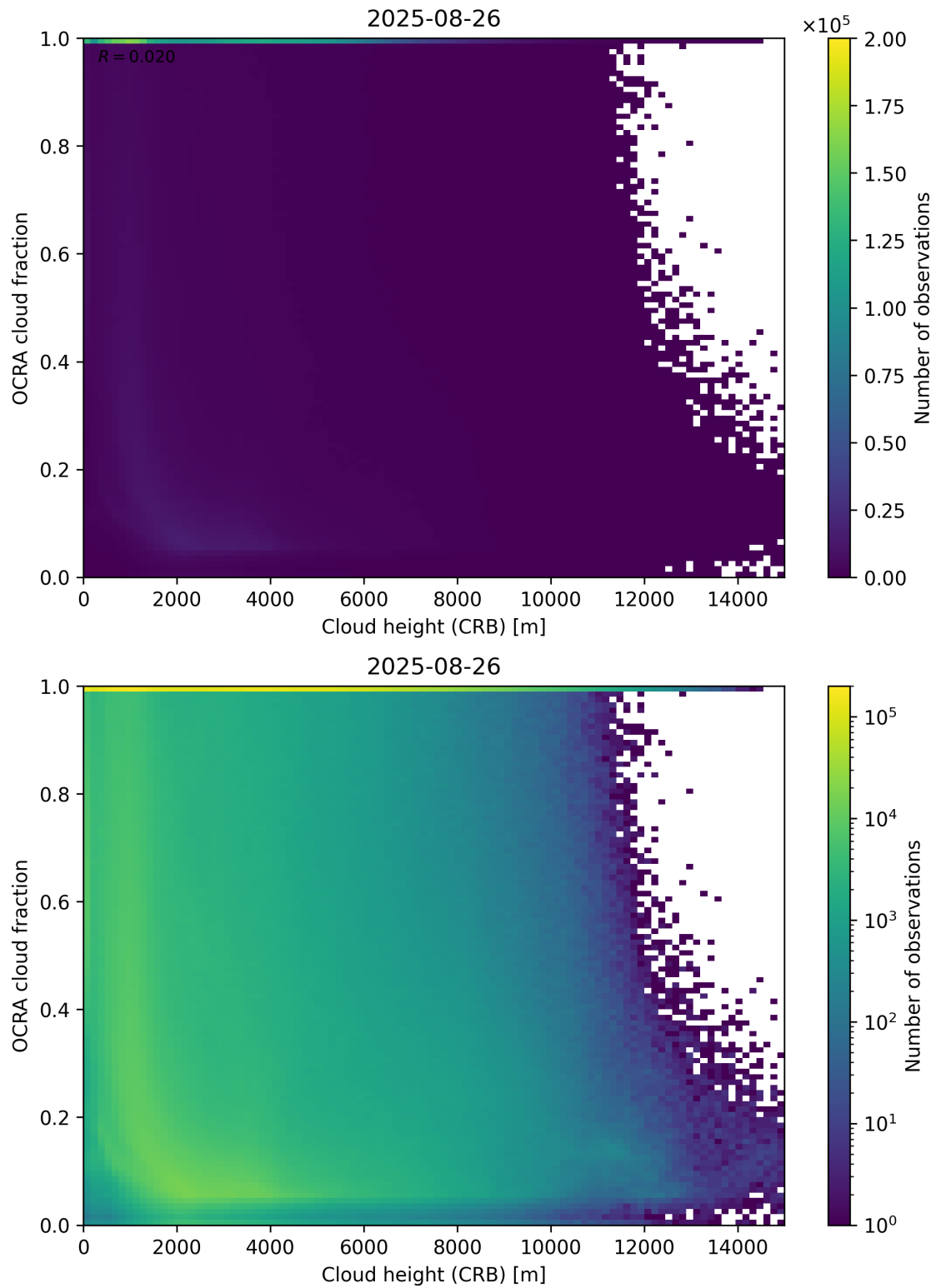
Figure 81: Scatter density plot of “Cloud height (CRB)” against “OCRA cloud fraction” for 2025-08-25 to 2025-08-27.
