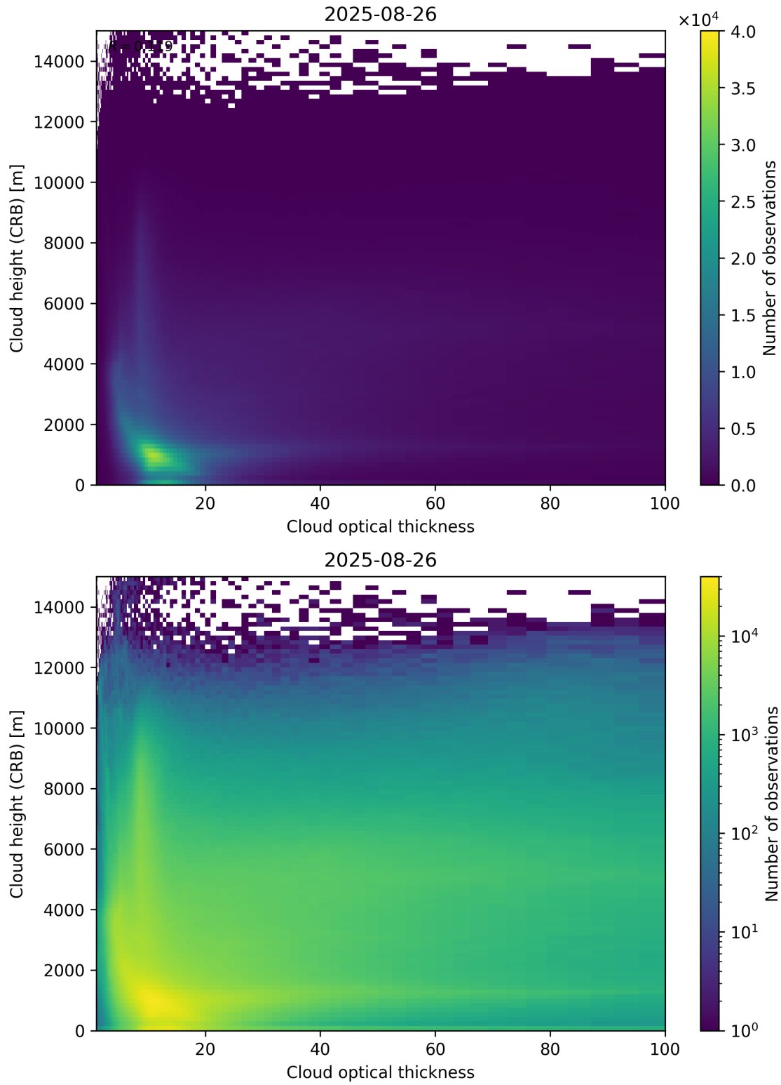
Figure 85: Scatter density plot of “Cloud optical thickness” against “Cloud height (CRB)” for 2025-08-25 to 2025-08-27.
