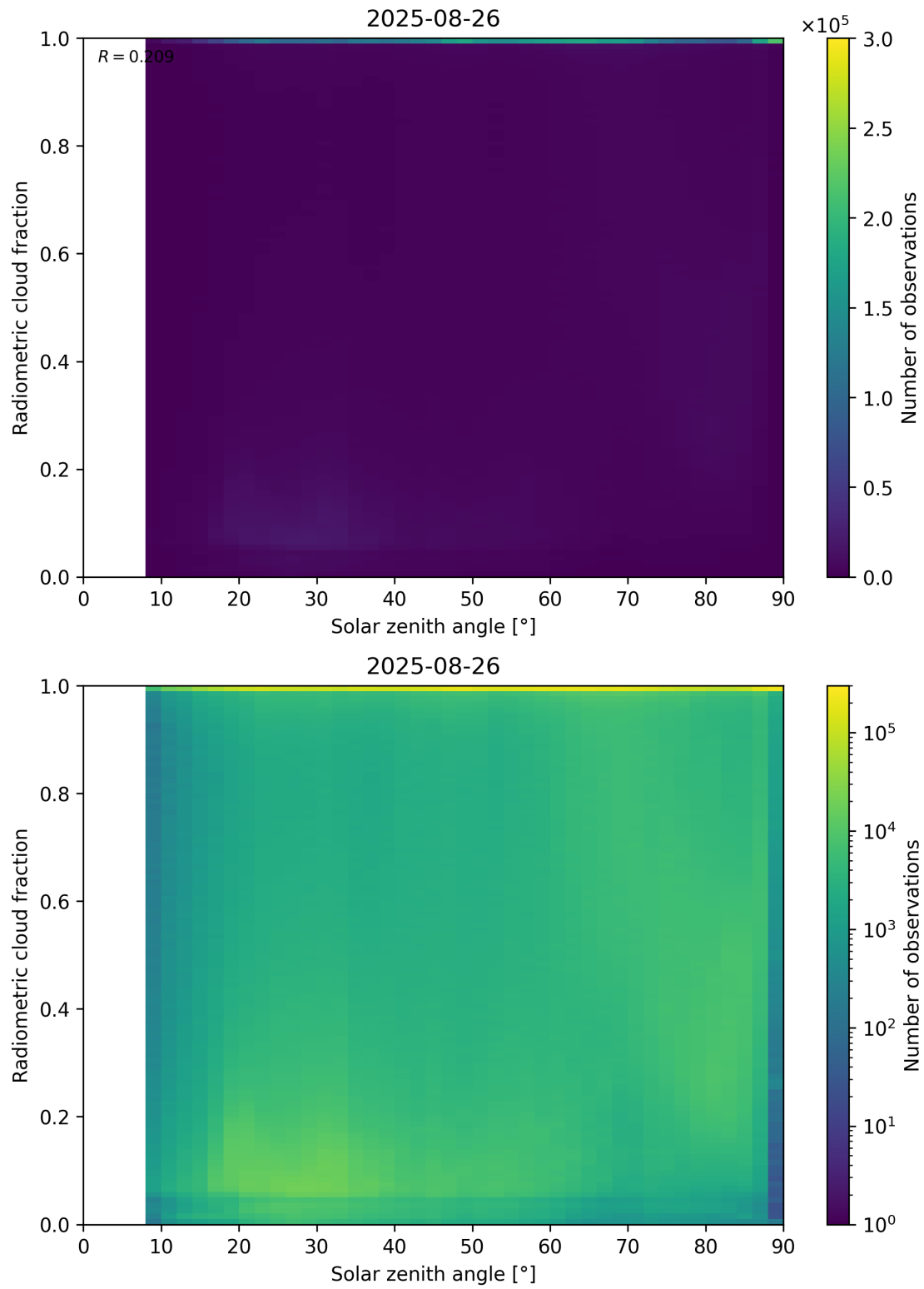
Figure 99: Scatter density plot of “Solar zenith angle” against “Radiometric cloud fraction” for 2025-08-25 to 2025-08-27.
