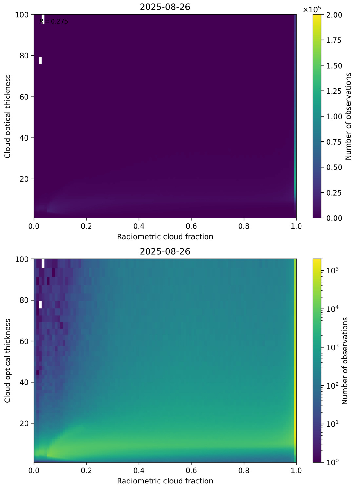
Figure 75: Scatter density plot of “Radiometric cloud fraction” against “Cloud optical thickness” for 2025-08-25 to 2025-08-27.
