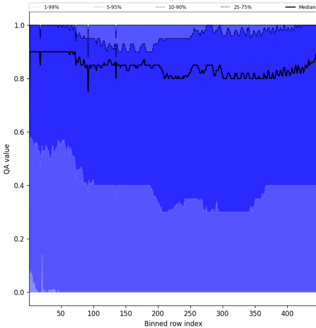
Figure 54: Along track statistics of “QA value” for 2025-08-25 to 2025-08-27
