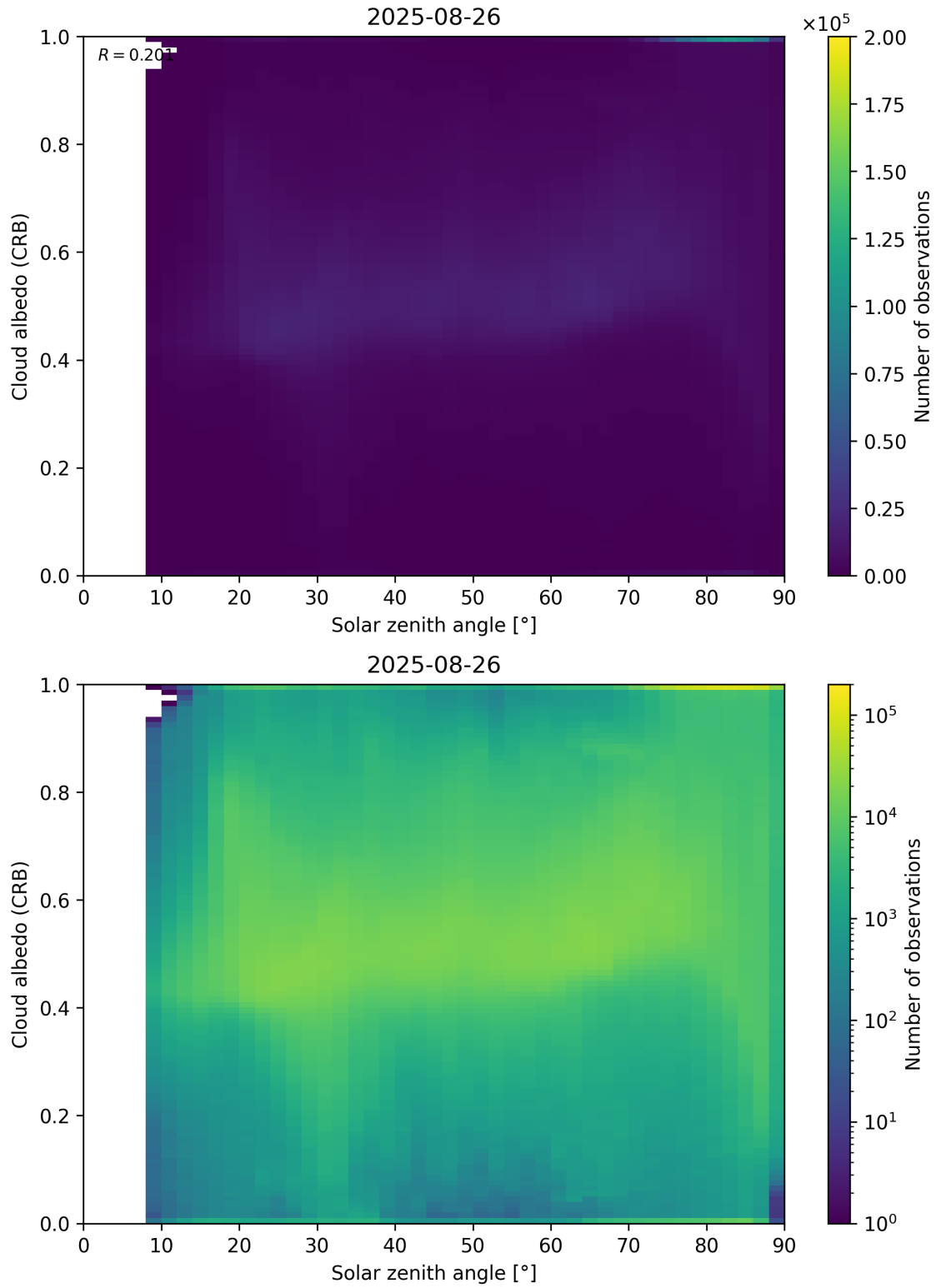
Figure 98: Scatter density plot of “Solar zenith angle” against “Cloud albedo (CRB)” for 2025-08-25 to 2025-08-27.
