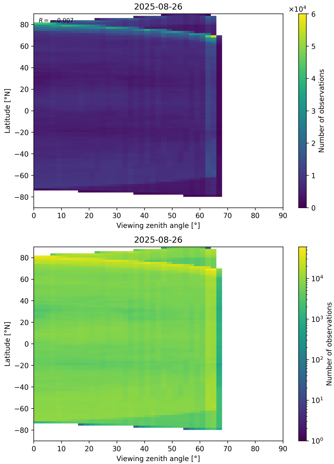
Figure 113: Scatter density plot of “Viewing zenith angle” against “Latitude” for 2025-08-25 to 2025-08-27.
