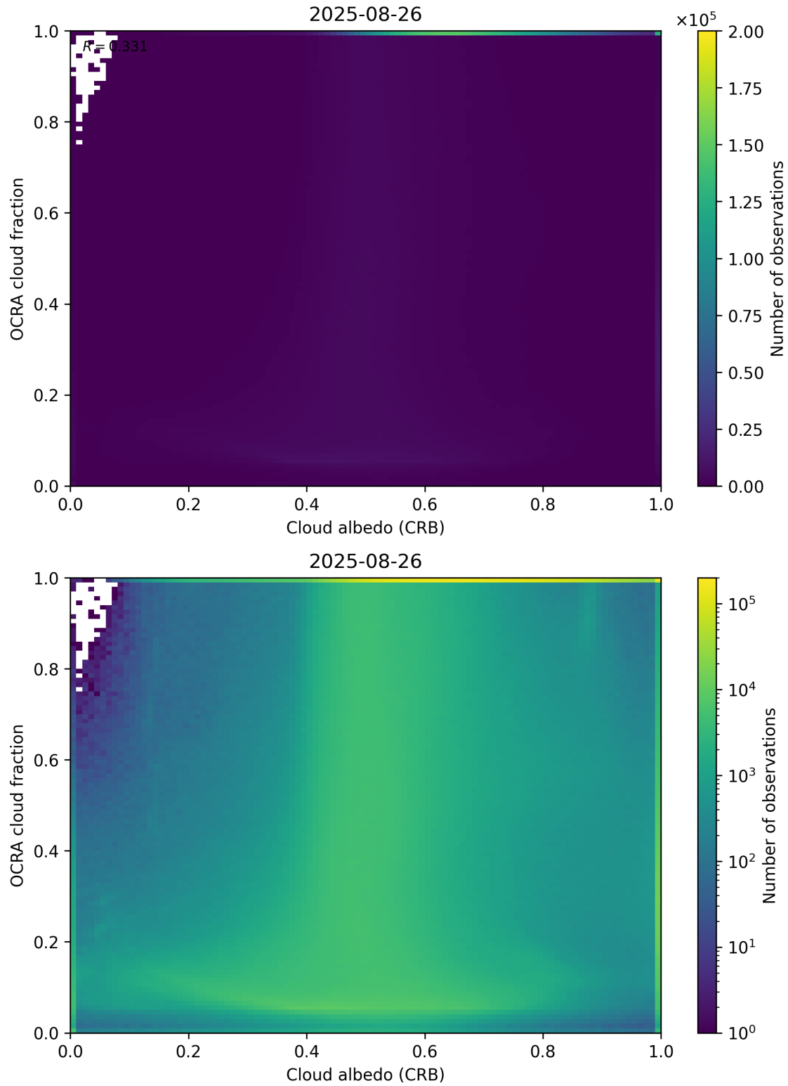
Figure 70: Scatter density plot of “Cloud albedo (CRB)” against “OCRA cloud fraction” for 2025-08-25 to 2025-08-27.
