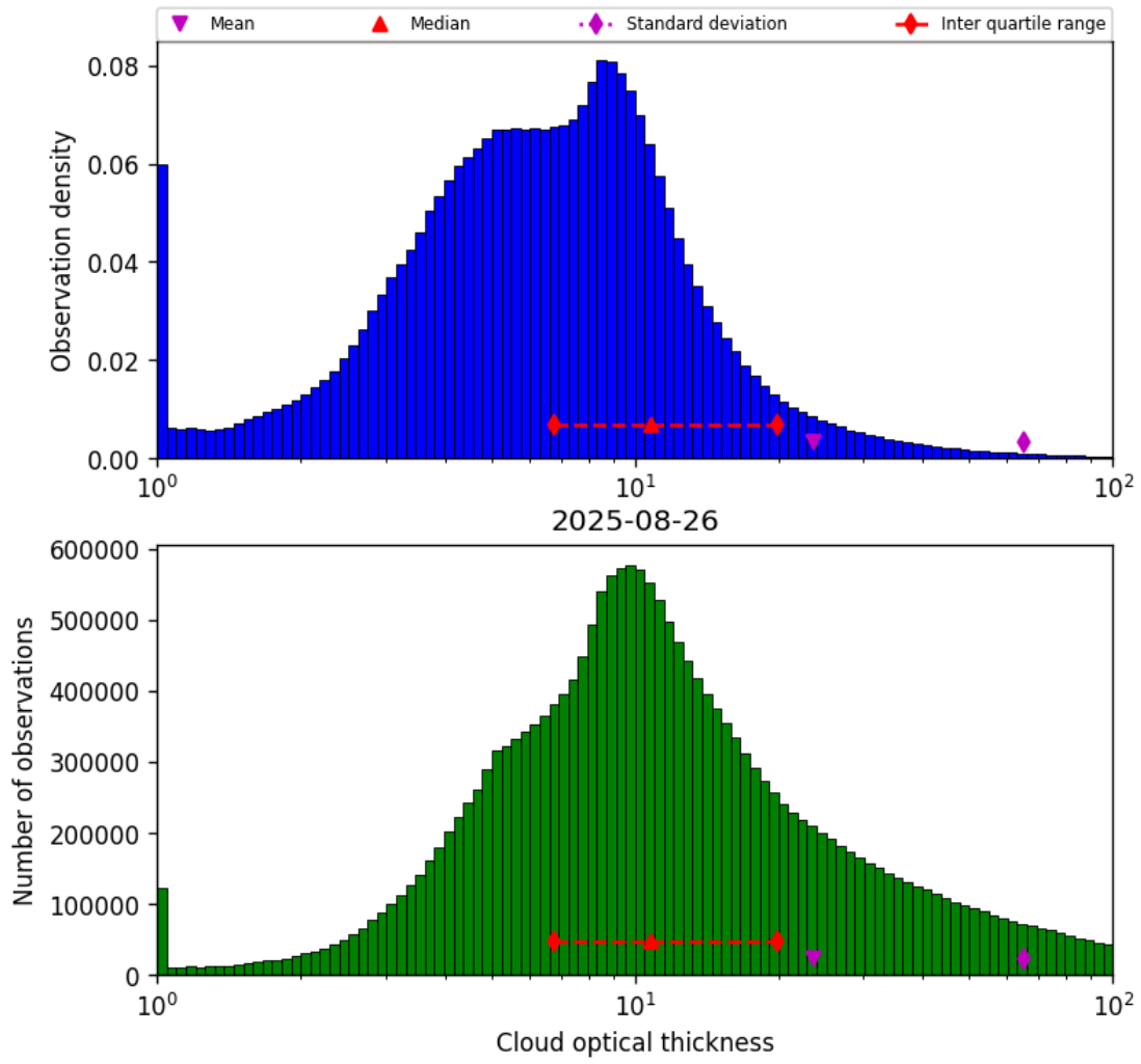
Figure 41: Histogram of “Cloud optical thickness” for 2025-08-25 to 2025-08-27
