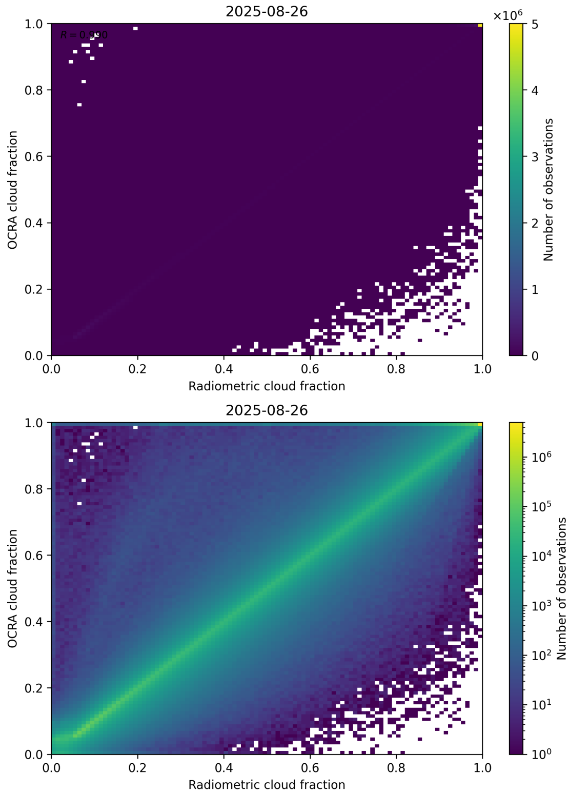
Figure 72: Scatter density plot of “Radiometric cloud fraction” against “OCRA cloud fraction” for 2025-08-25 to 2025-08-27.
