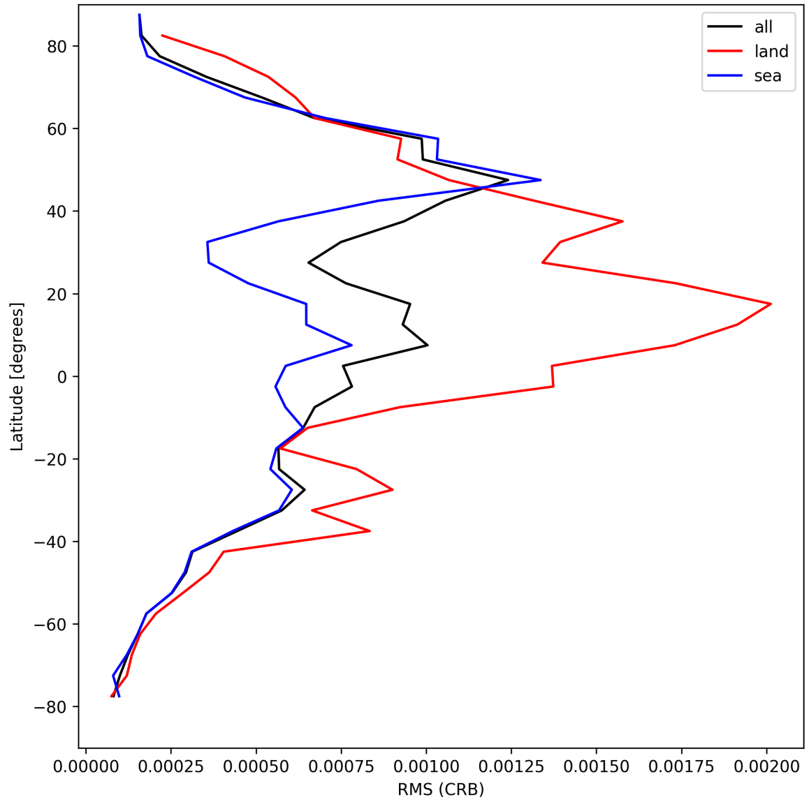
Figure 32: Zonal average of “RMS (CRB)” for 2025-08-25 to 2025-08-27.
