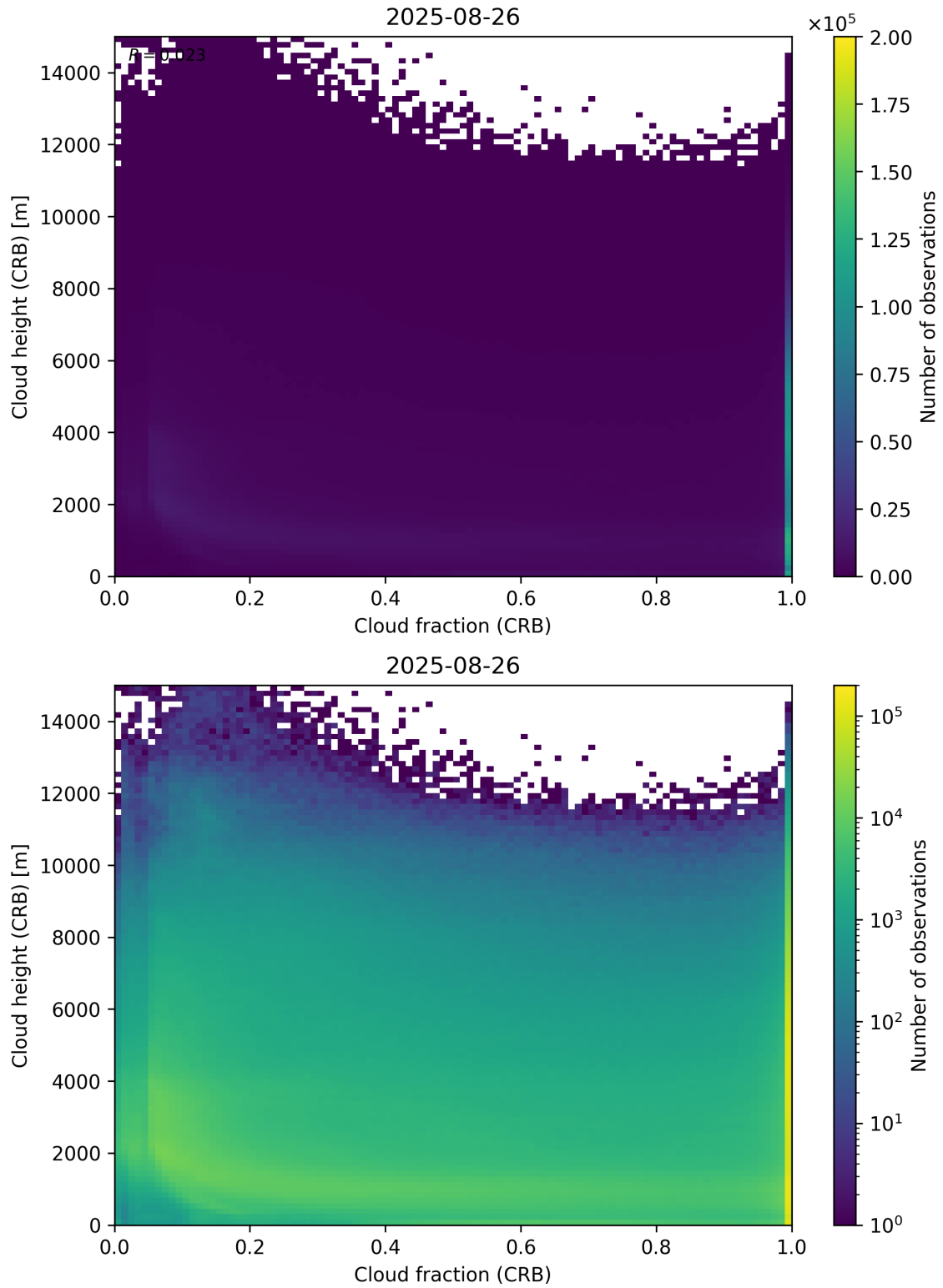
Figure 79: Scatter density plot of “Cloud fraction (CRB)” against “Cloud height (CRB)” for 2025-08-25 to 2025-08-27.
