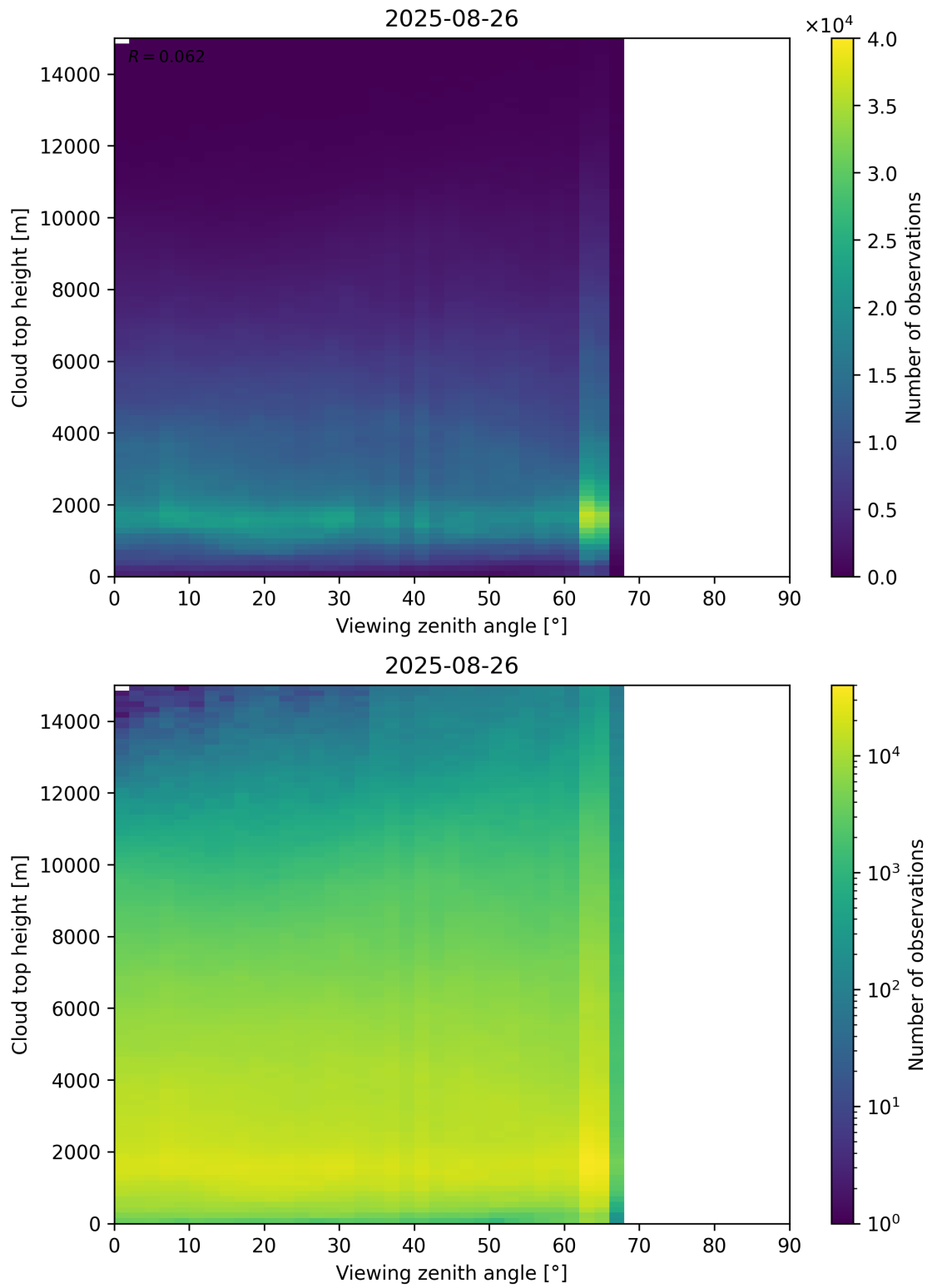
Figure 112: Scatter density plot of “Viewing zenith angle” against “Cloud top height” for 2025-08-25 to 2025-08-27.
