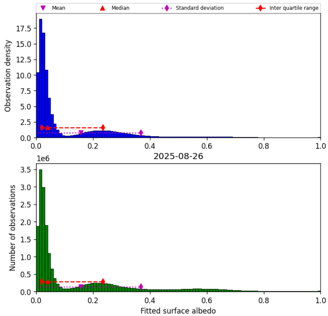
Figure 45: Histogram of “Fitted surface albedo” for 2025-08-25 to 2025-08-27
