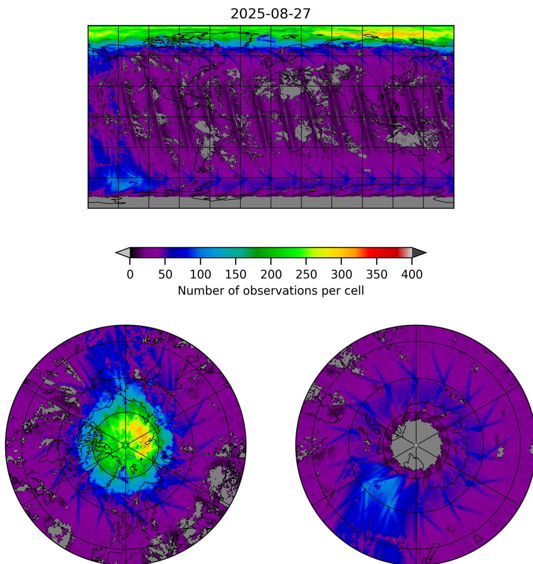
Figure 21: Map of the number of observations for 2025-08-26 to 2025-08-28
