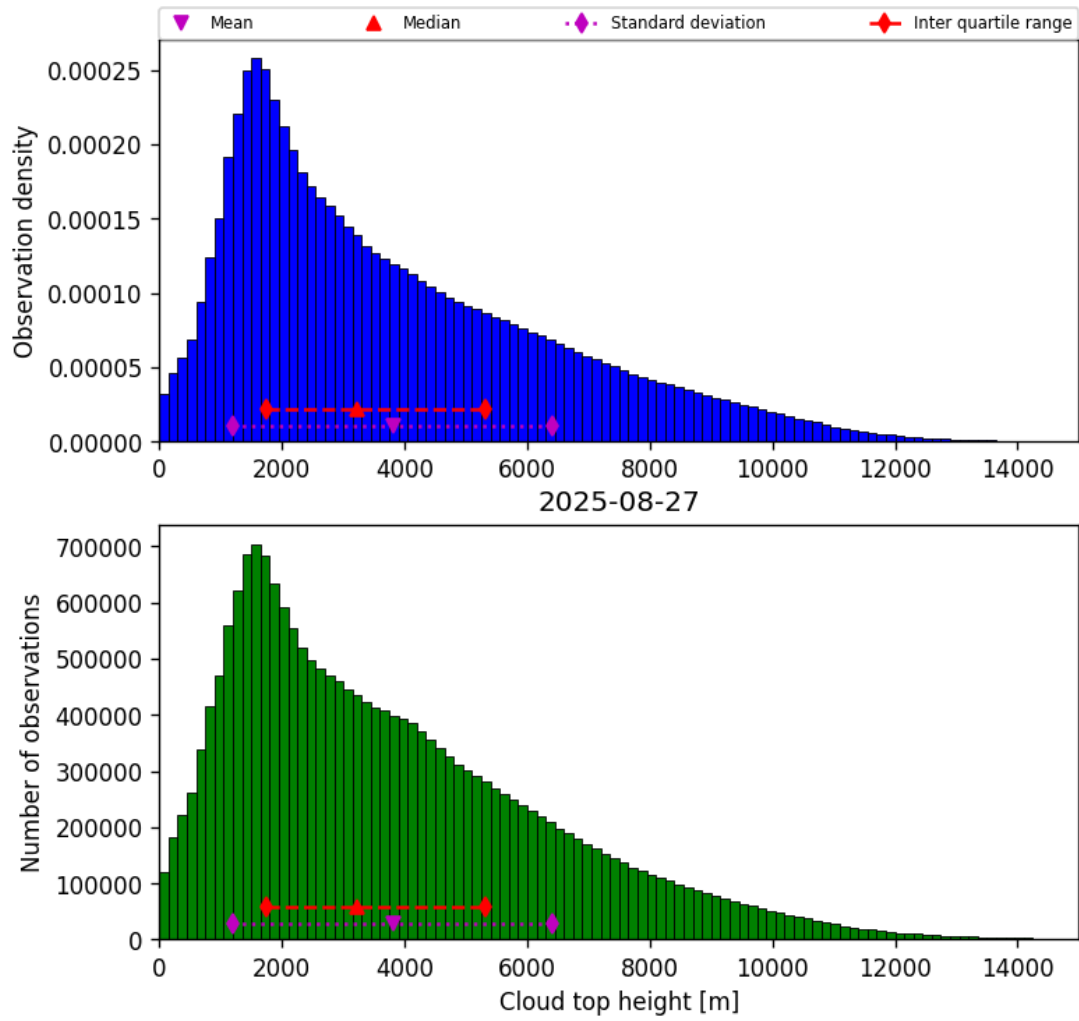
Figure 40: Histogram of “Cloud top height” for 2025-08-26 to 2025-08-28
