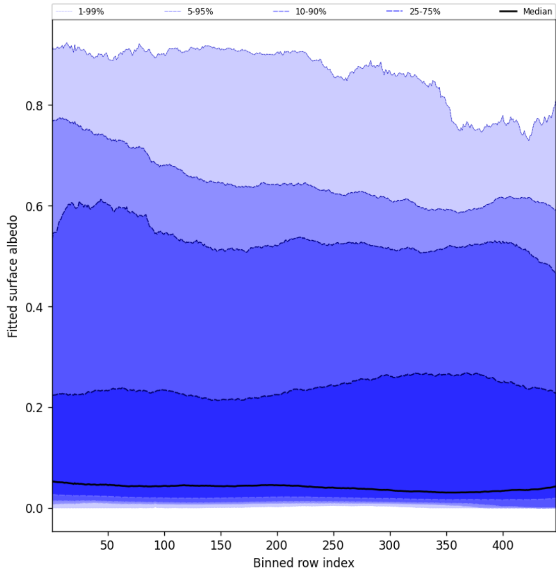
Figure 61: Along track statistics of “Fitted surface albedo” for 2025-08-26 to 2025-08-28
