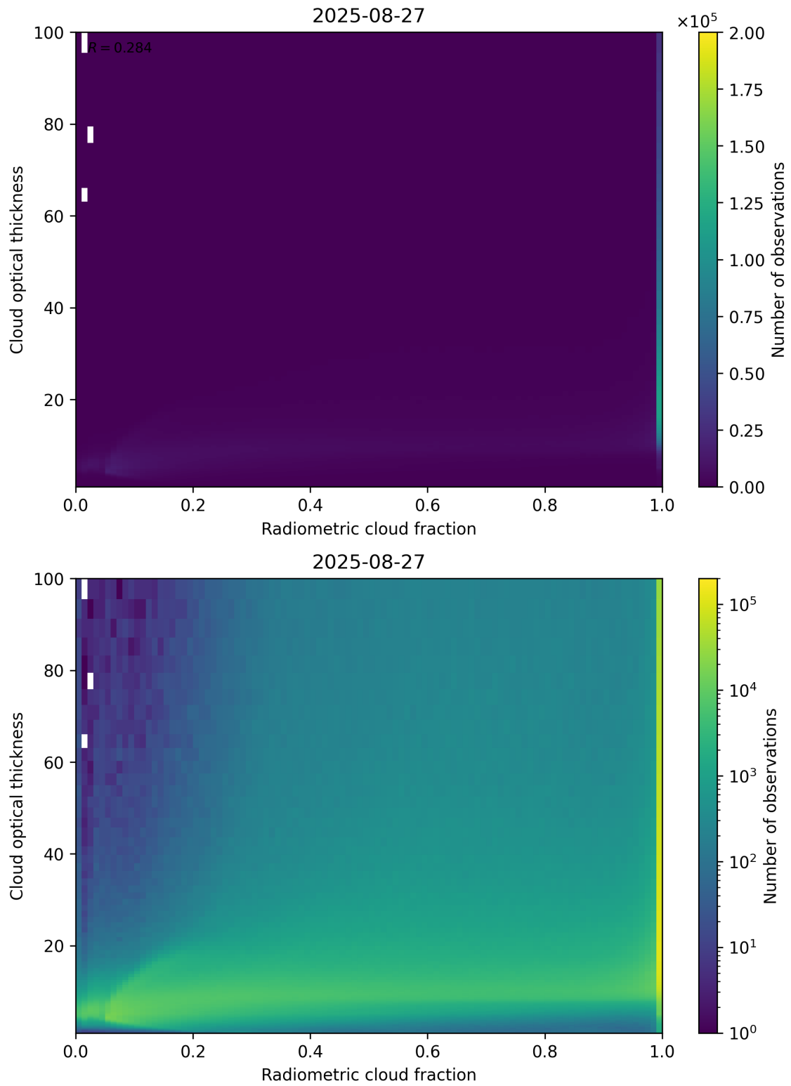
Figure 75: Scatter density plot of “Radiometric cloud fraction” against “Cloud optical thickness” for 2025-08-26 to 2025-08-28.
