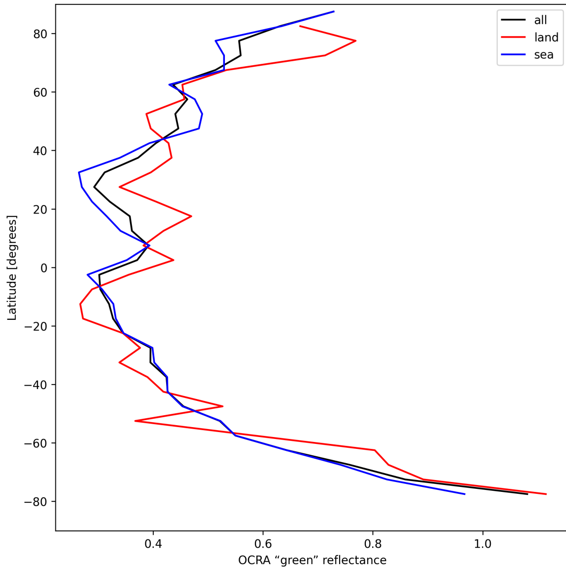
Figure 36: Zonal average of “OCRA “green” reflectance” for 2025-08-26 to 2025-08-28.
