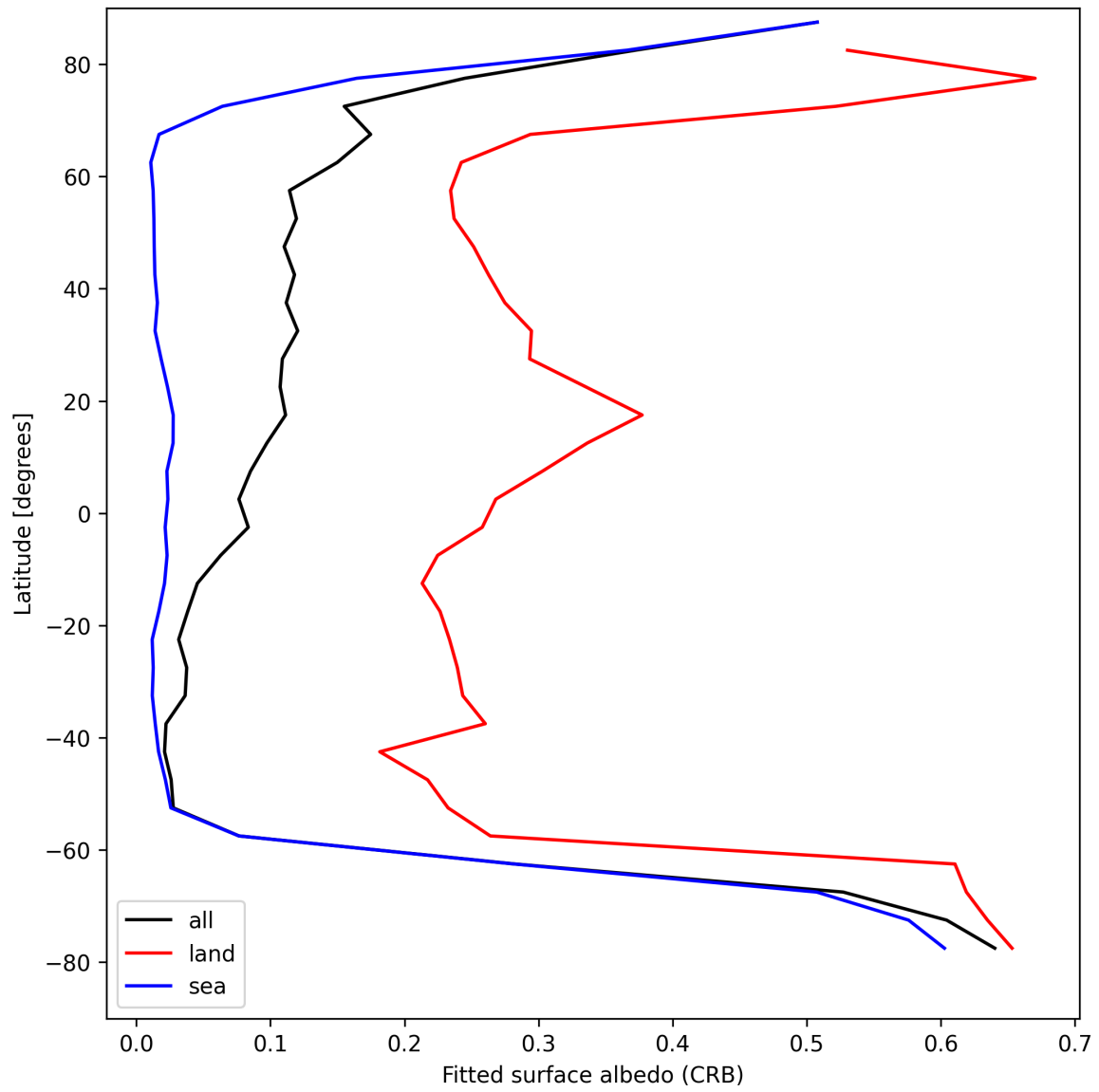
Figure 30: Zonal average of “Fitted surface albedo (CRB)” for 2025-08-26 to 2025-08-28.
