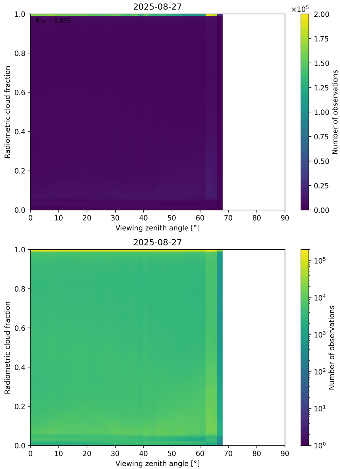
Figure 107: Scatter density plot of “Viewing zenith angle” against “Radiometric cloud fraction” for 2025-08-26 to 2025-08-28.
