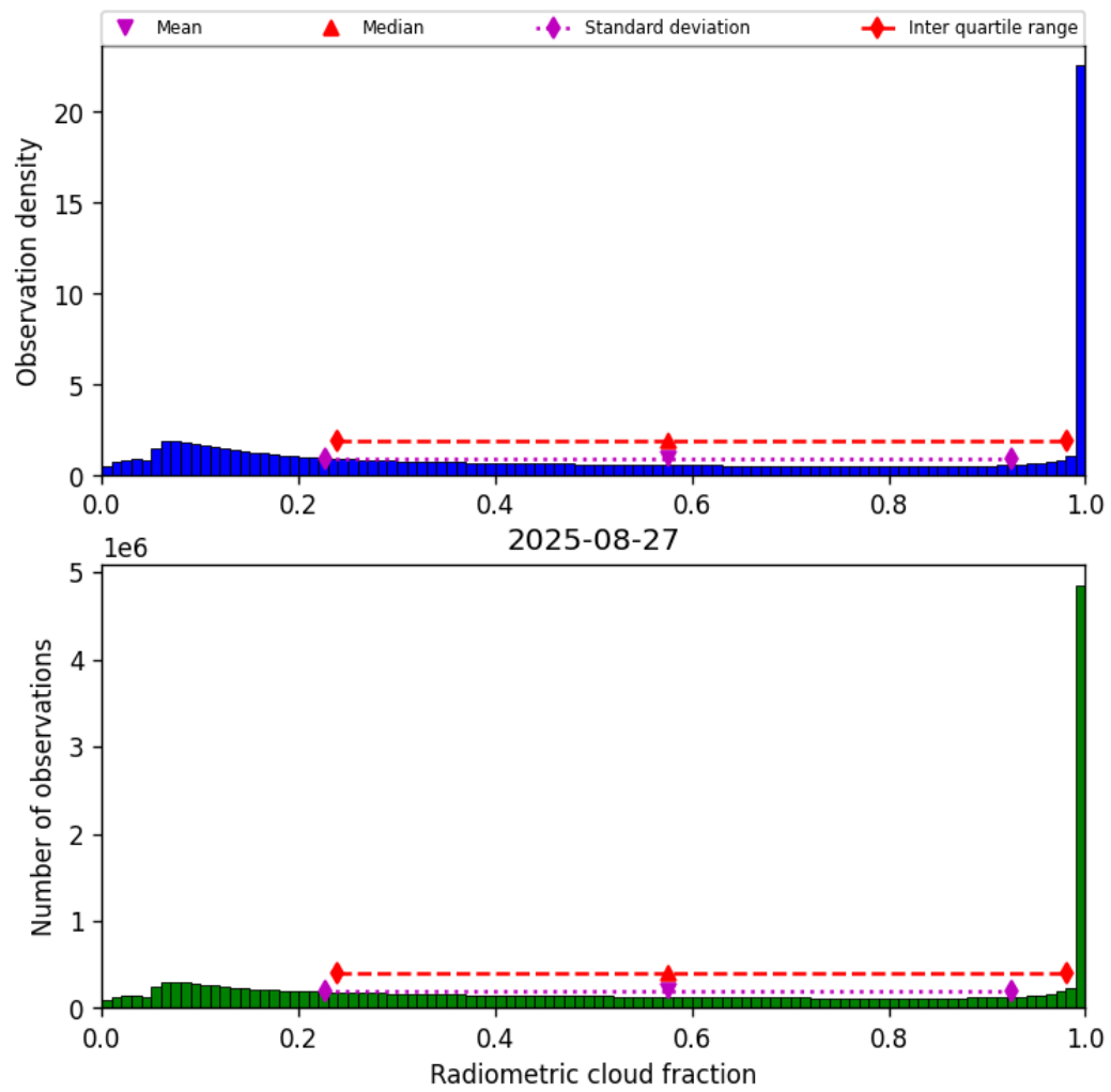
Figure 39: Histogram of “Radiometric cloud fraction” for 2025-08-26 to 2025-08-28
