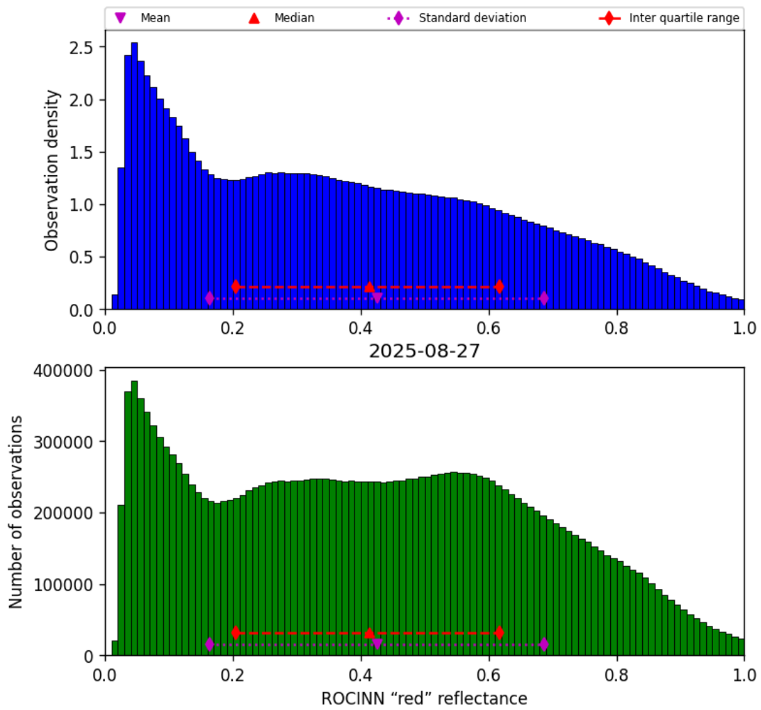
Figure 53: Histogram of "ROCINN "red" reflectance" for 2025-08-26 to 2025-08-28
