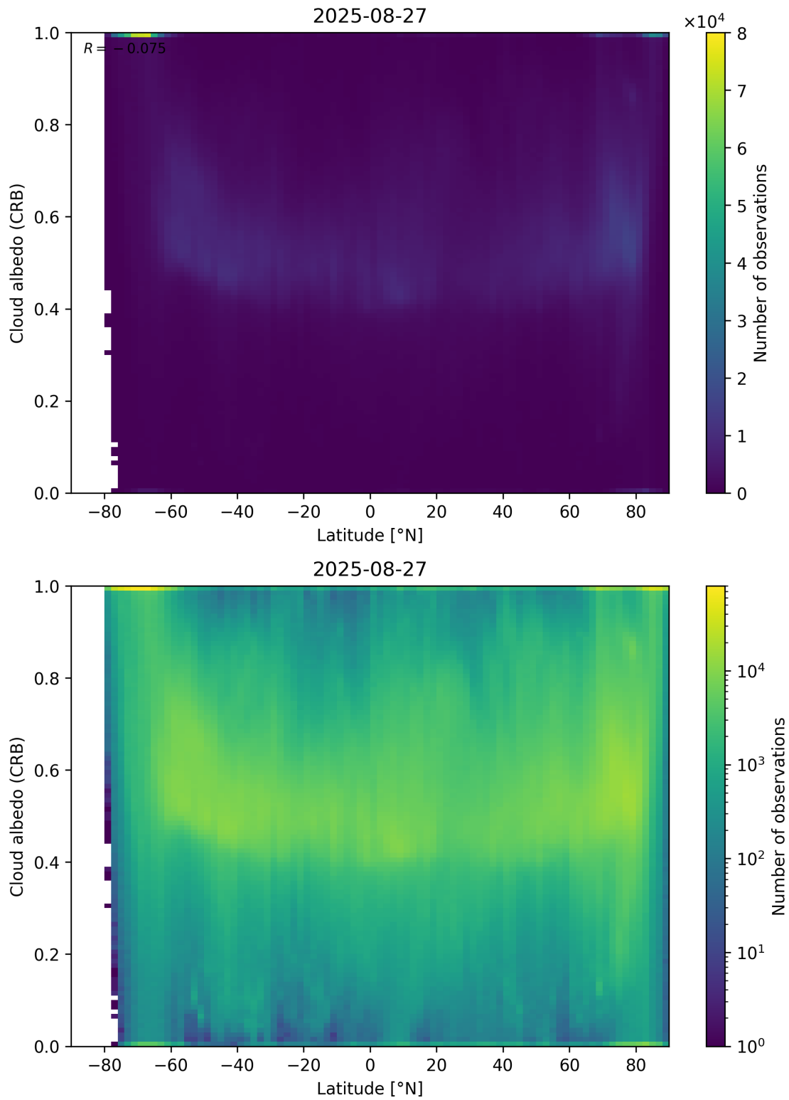
Figure 91: Scatter density plot of “Latitude” against “Cloud albedo (CRB)” for 2025-08-26 to 2025-08-28.
