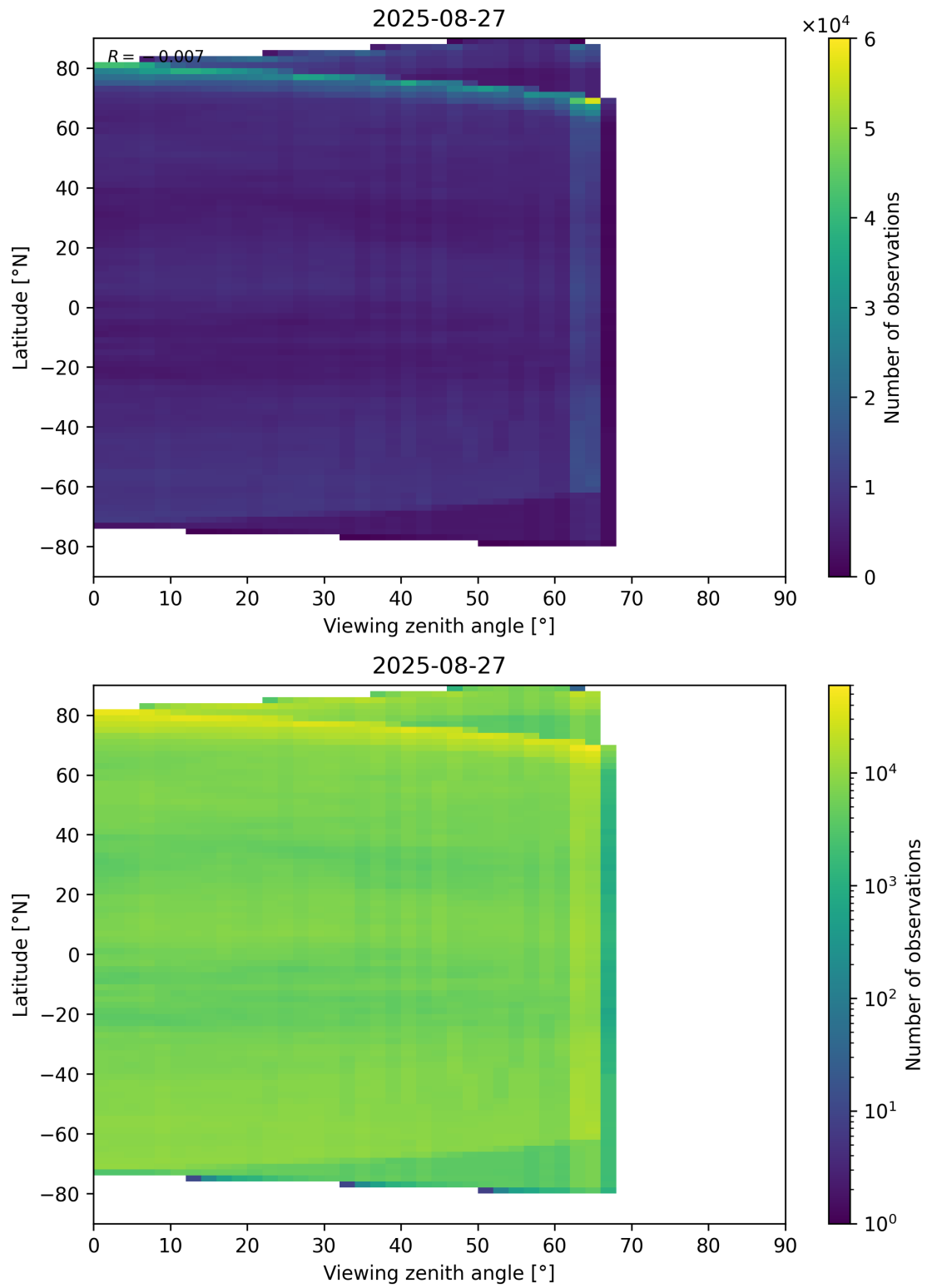
Figure 113: Scatter density plot of “Viewing zenith angle” against “Latitude” for 2025-08-26 to 2025-08-28.
