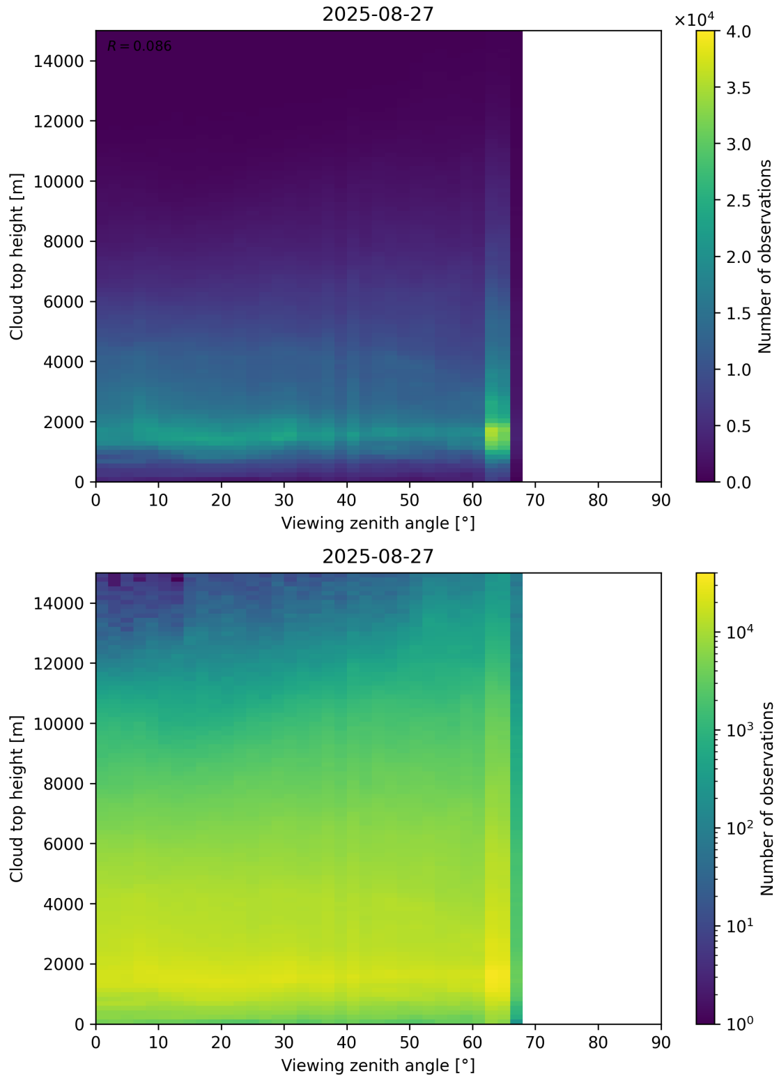
Figure 112: Scatter density plot of “Viewing zenith angle” against “Cloud top height” for 2025-08-26 to 2025-08-28.
