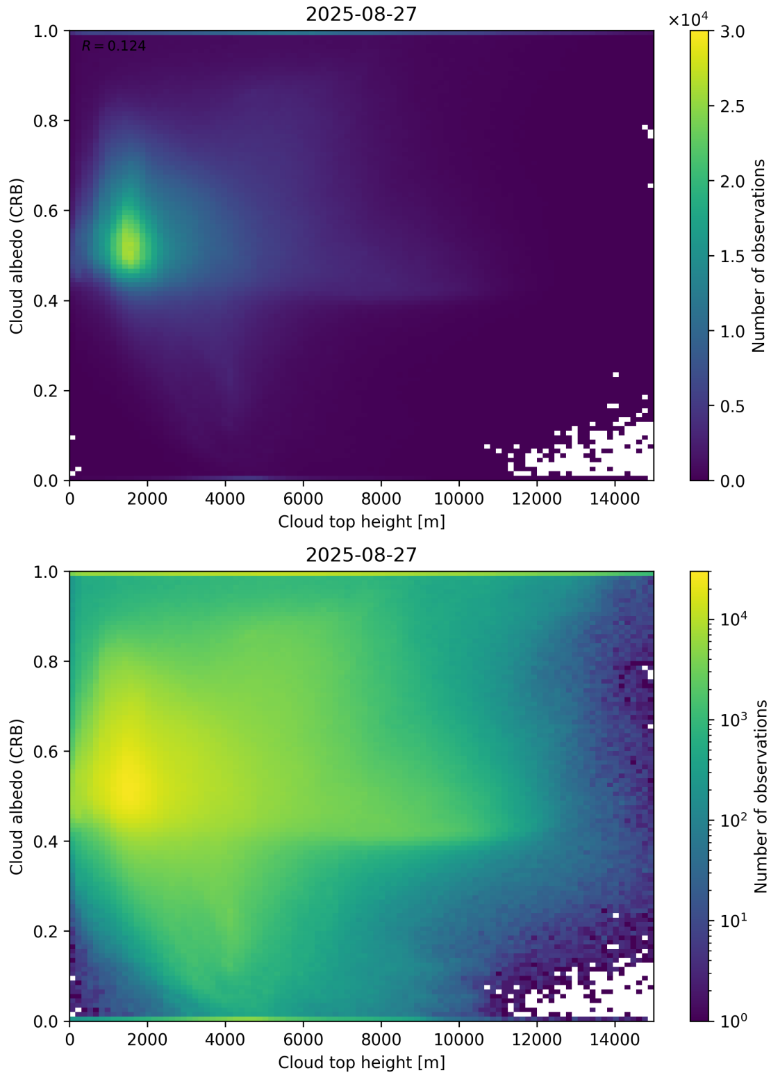
Figure 86: Scatter density plot of “Cloud top height” against “Cloud albedo (CRB)” for 2025-08-26 to 2025-08-28.
