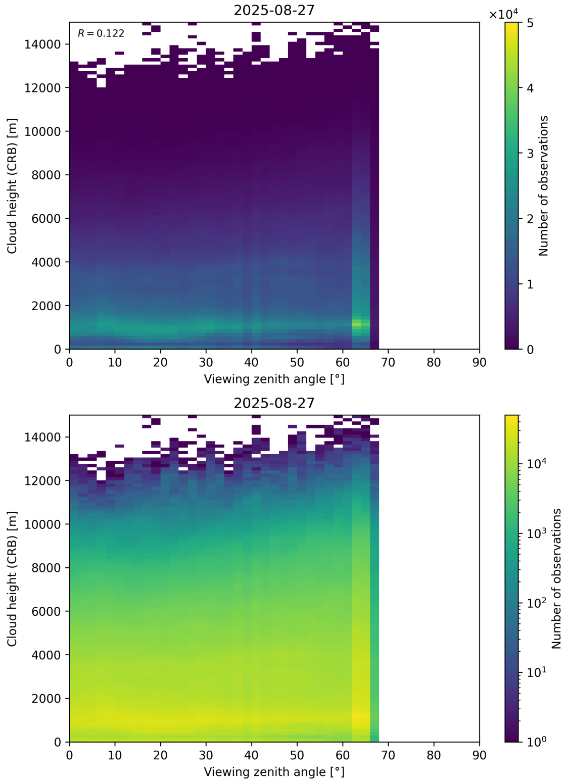
Figure 110: Scatter density plot of “Viewing zenith angle” against “Cloud height (CRB)” for 2025-08-26 to 2025-08-28.
