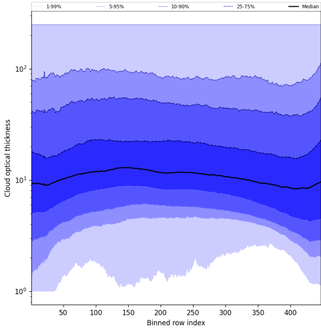
Figure 57: Along track statistics of “Cloud optical thickness” for 2025-08-26 to 2025-08-28
