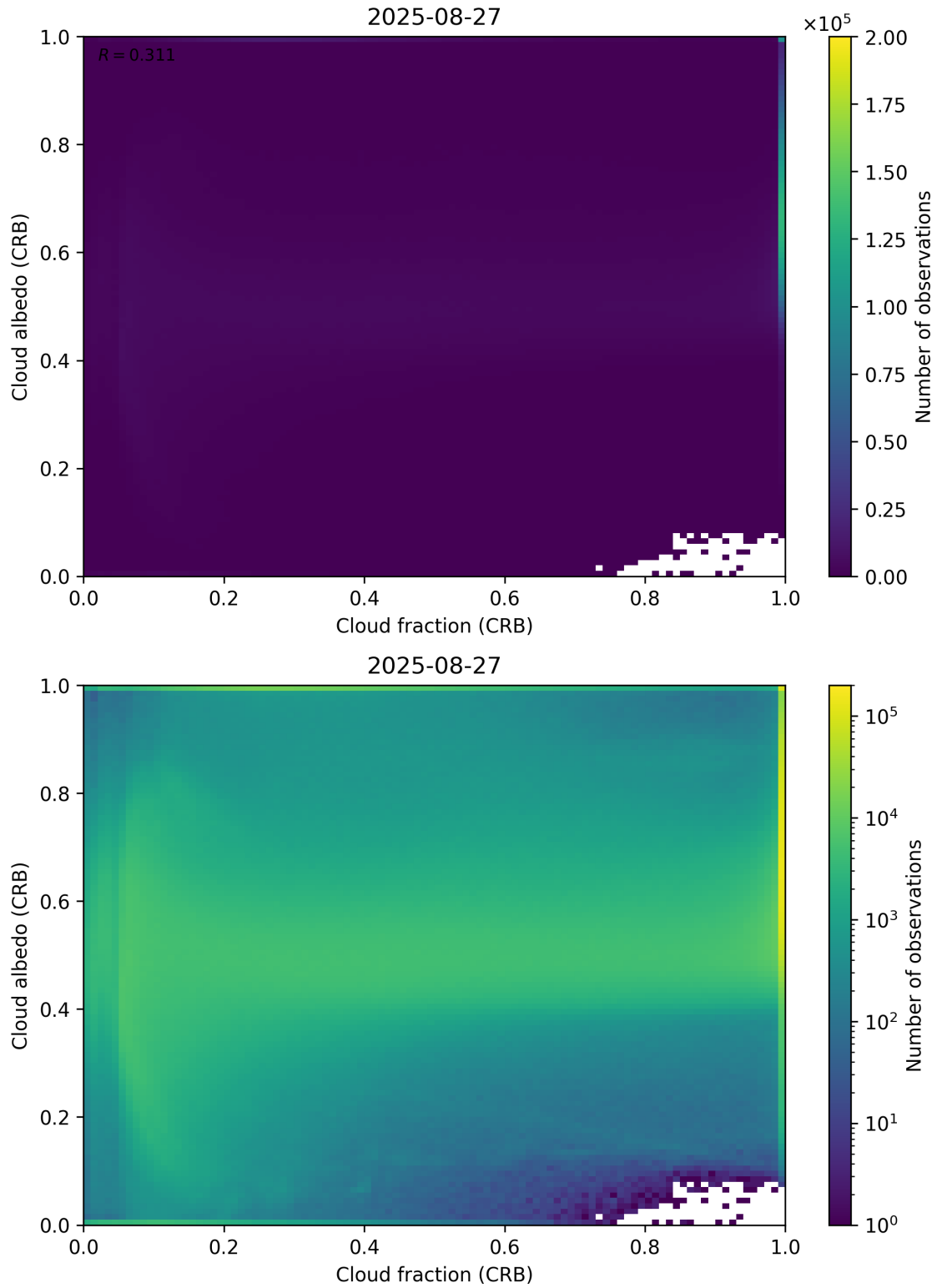
Figure 77: Scatter density plot of “Cloud fraction (CRB)” against “Cloud albedo (CRB)” for 2025-08-26 to 2025-08-28.
