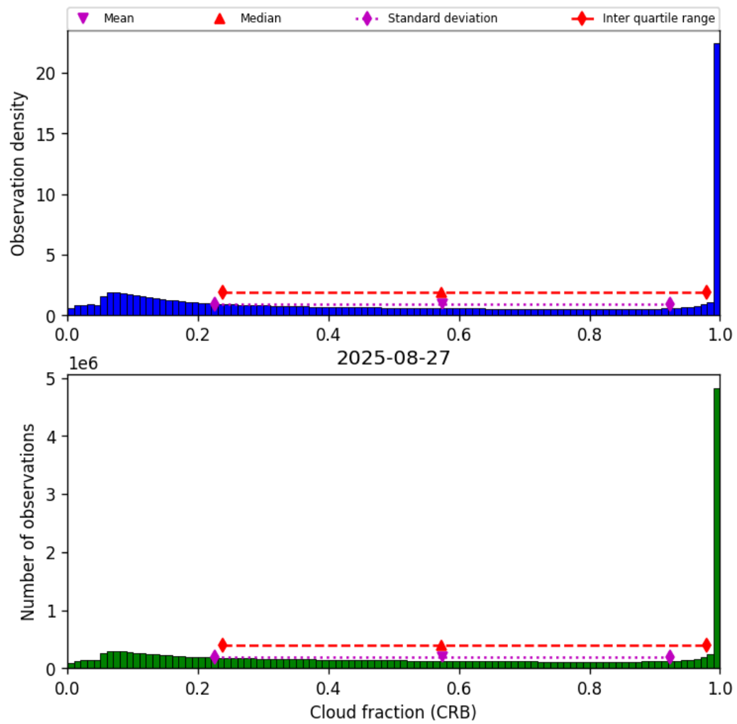
Figure 42: Histogram of “Cloud fraction (CRB)” for 2025-08-26 to 2025-08-28
