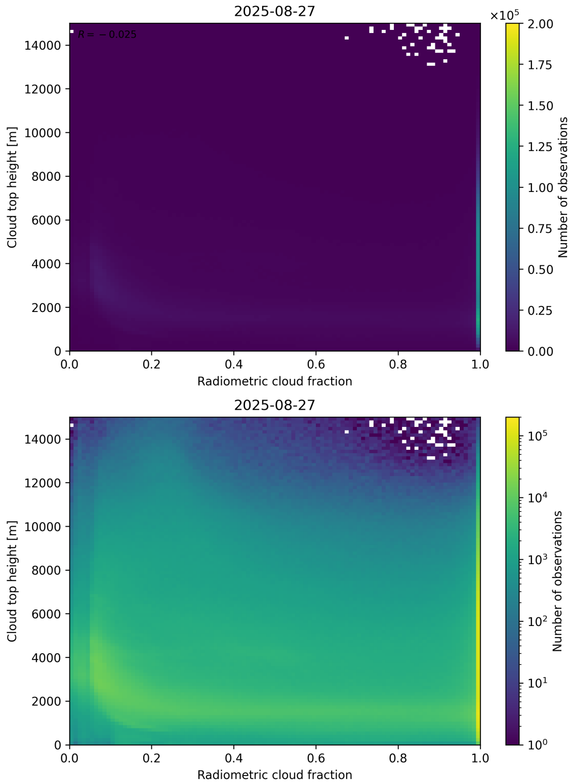
Figure 76: Scatter density plot of “Radiometric cloud fraction” against “Cloud top height” for 2025-08-26 to 2025-08-28.
