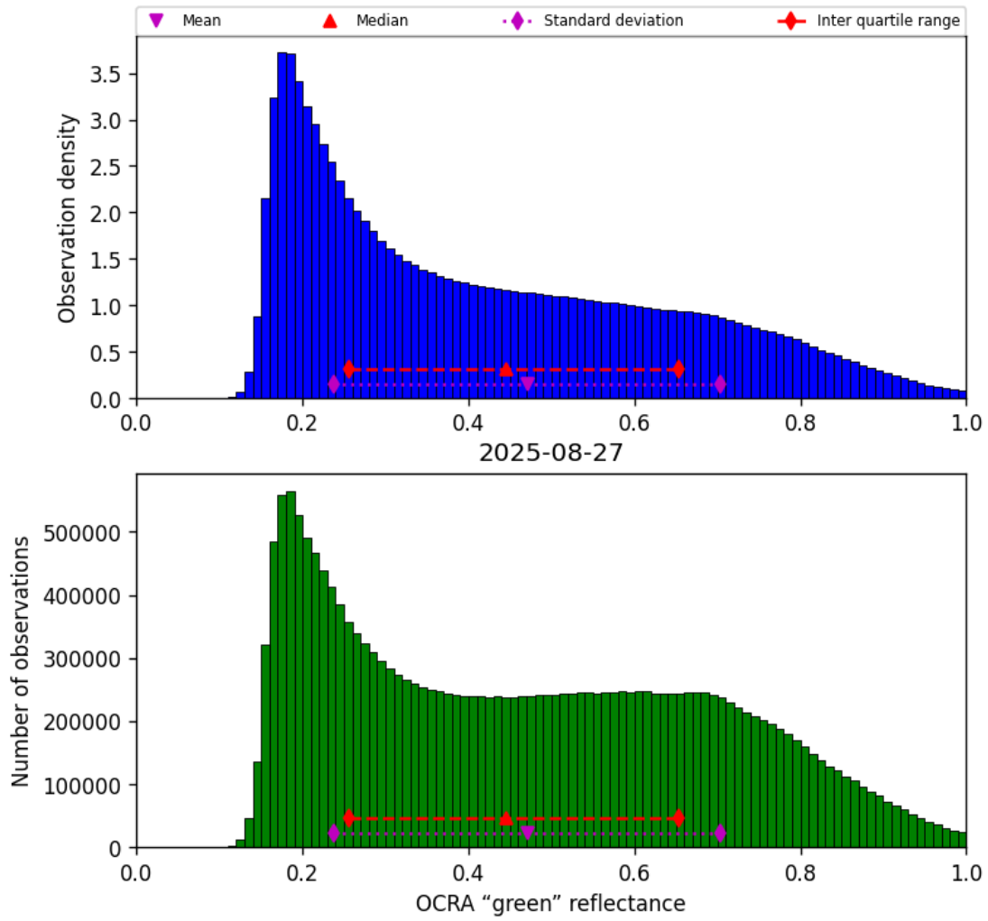
Figure 52: Histogram of “OCRA “green” reflectance” for 2025-08-26 to 2025-08-28
