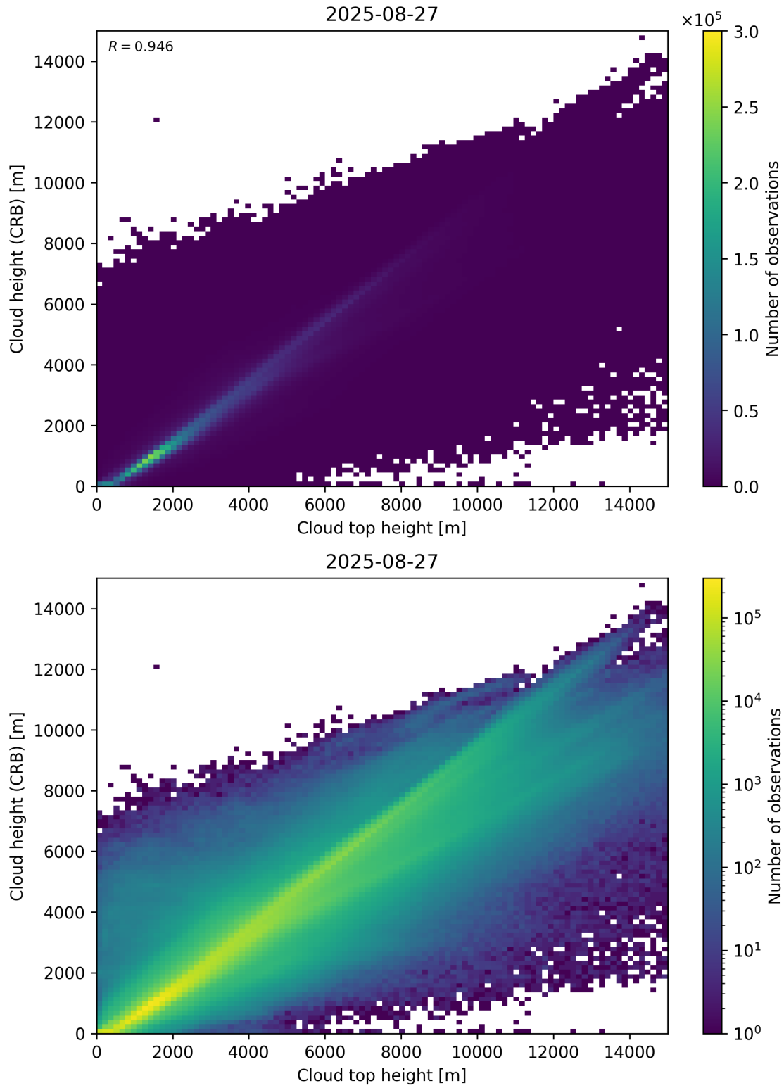
Figure 89: Scatter density plot of “Cloud top height” against “Cloud height (CRB)” for 2025-08-26 to 2025-08-28.
