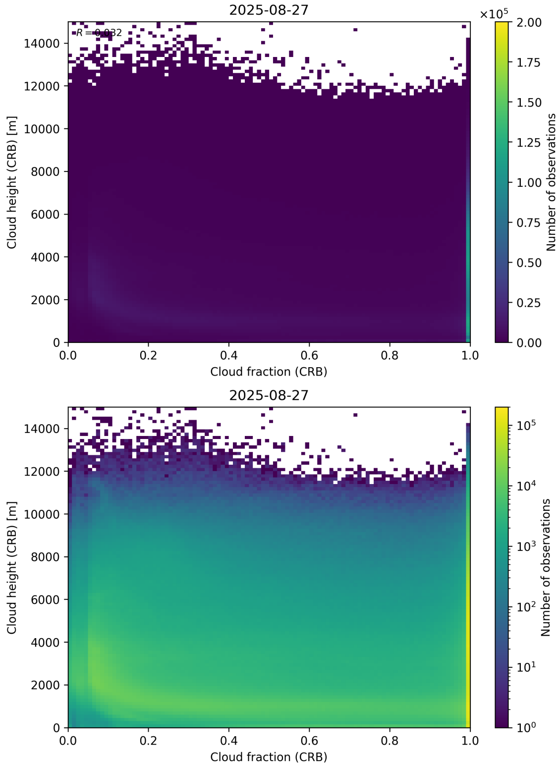
Figure 79: Scatter density plot of “Cloud fraction (CRB)” against “Cloud height (CRB)” for 2025-08-26 to 2025-08-28.
