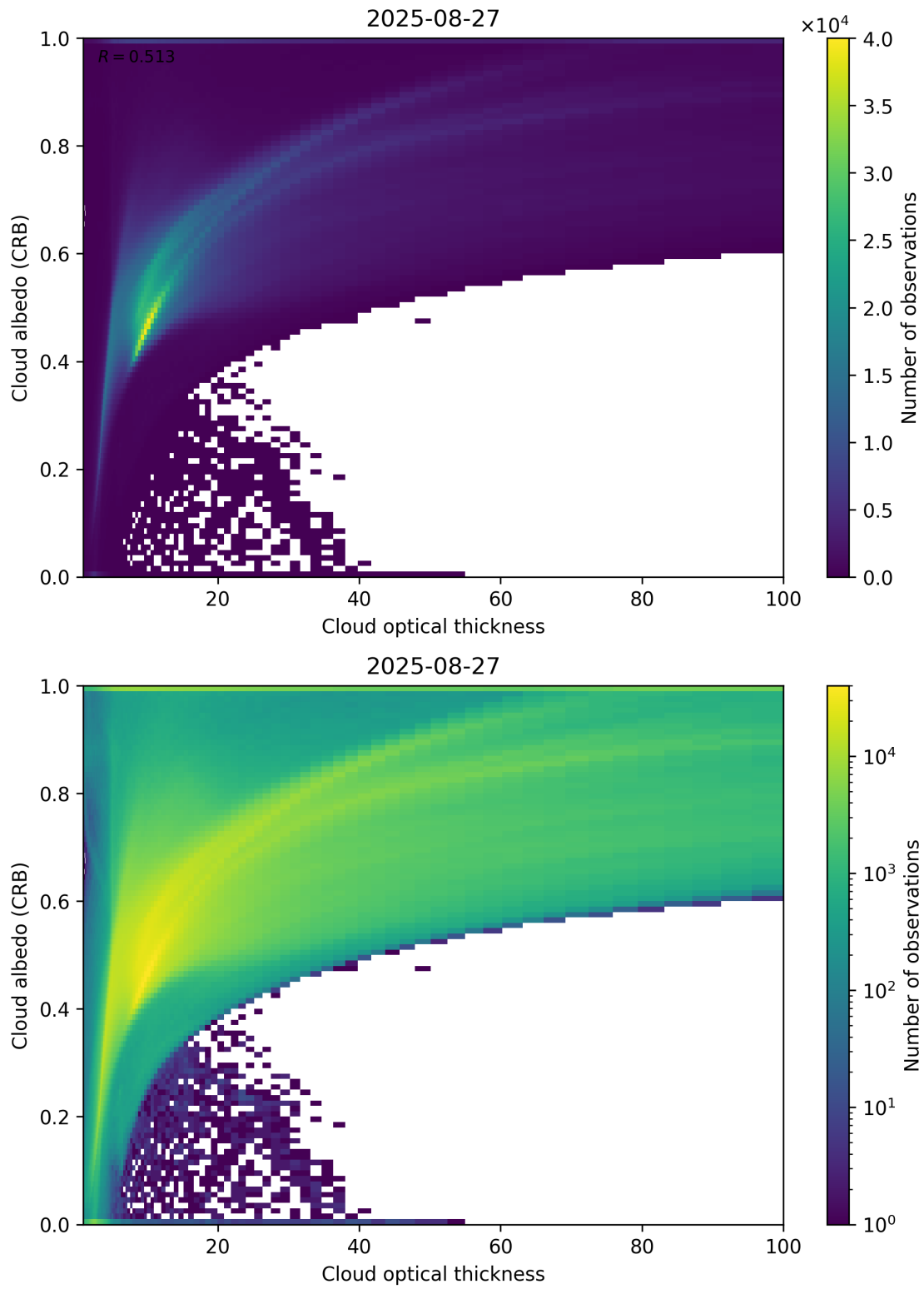
Figure 82: Scatter density plot of “Cloud optical thickness” against “Cloud albedo (CRB)” for 2025-08-26 to 2025-08-28.
