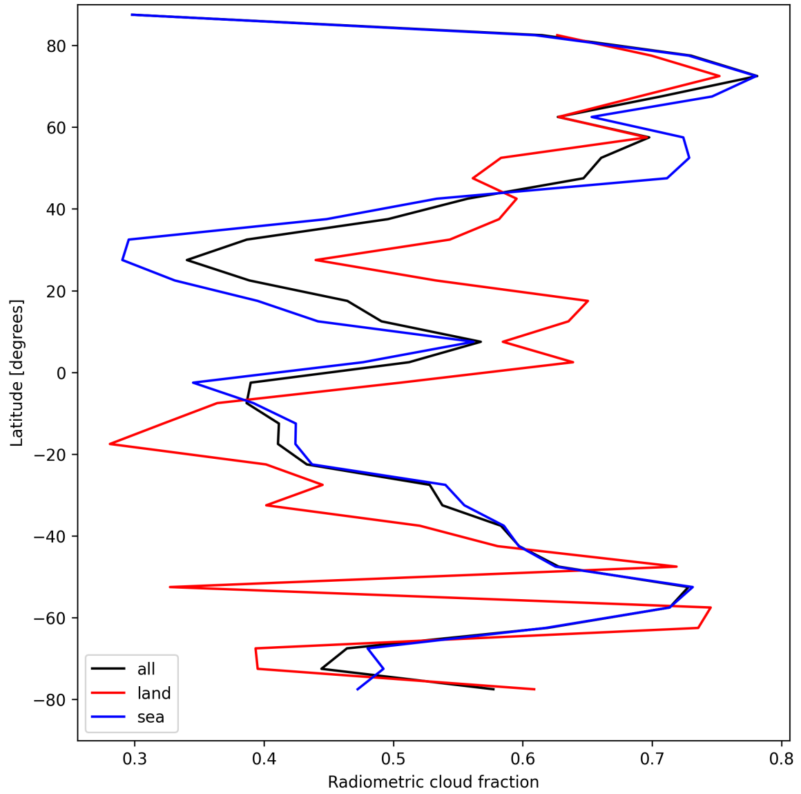
Figure 23: Zonal average of “Radiometric cloud fraction” for 2025-08-26 to 2025-08-28.
