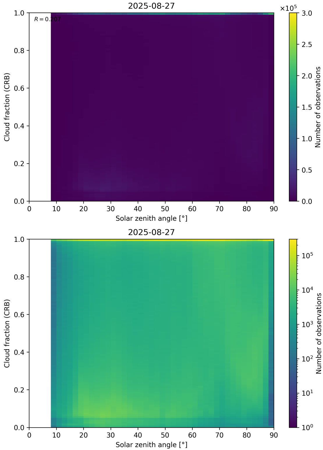
Figure 101: Scatter density plot of “Solar zenith angle” against “Cloud fraction (CRB)” for 2025-08-26 to 2025-08-28.
