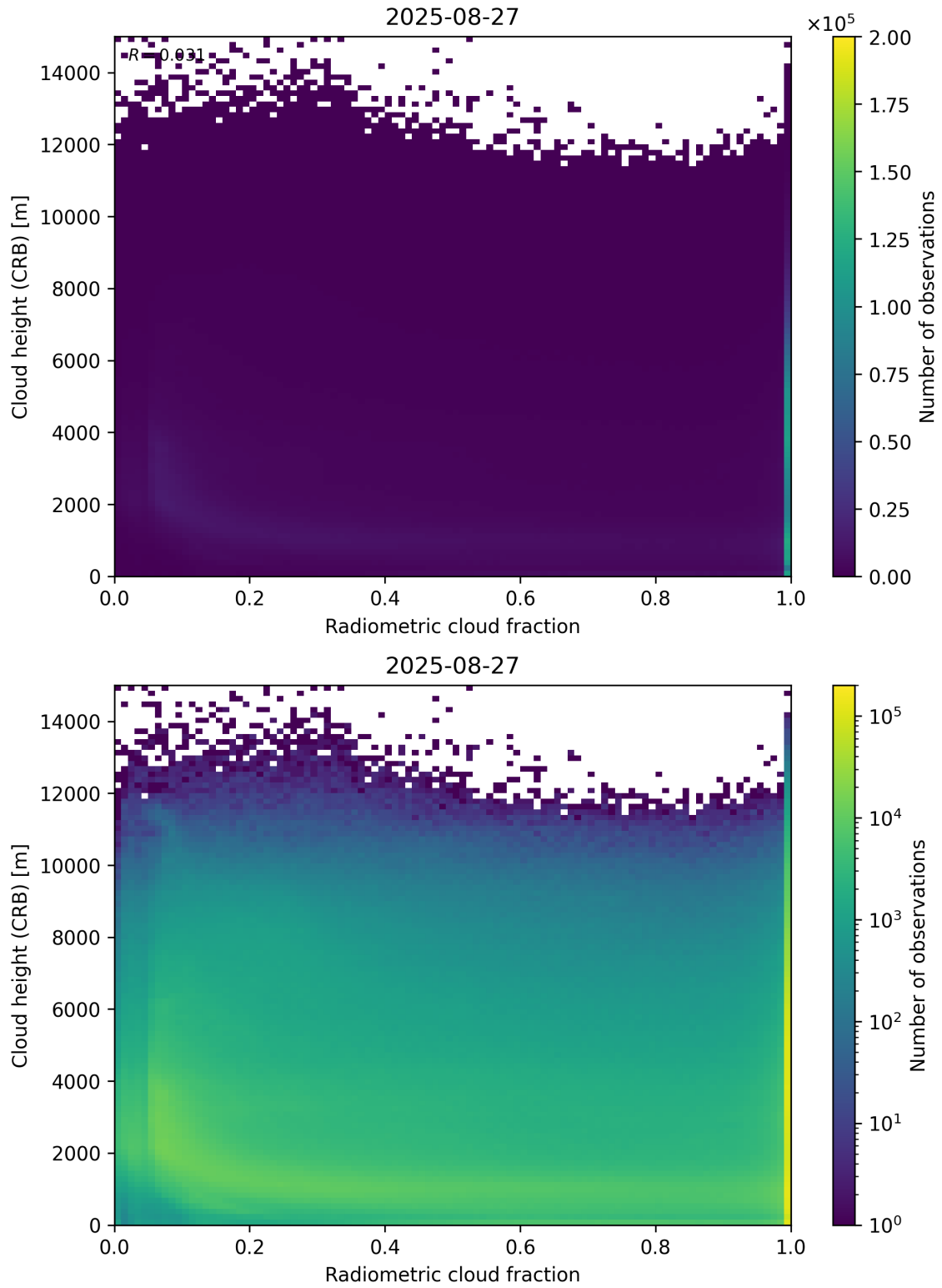
Figure 74: Scatter density plot of “Radiometric cloud fraction” against “Cloud height (CRB)” for 2025-08-26 to 2025-08-28.
