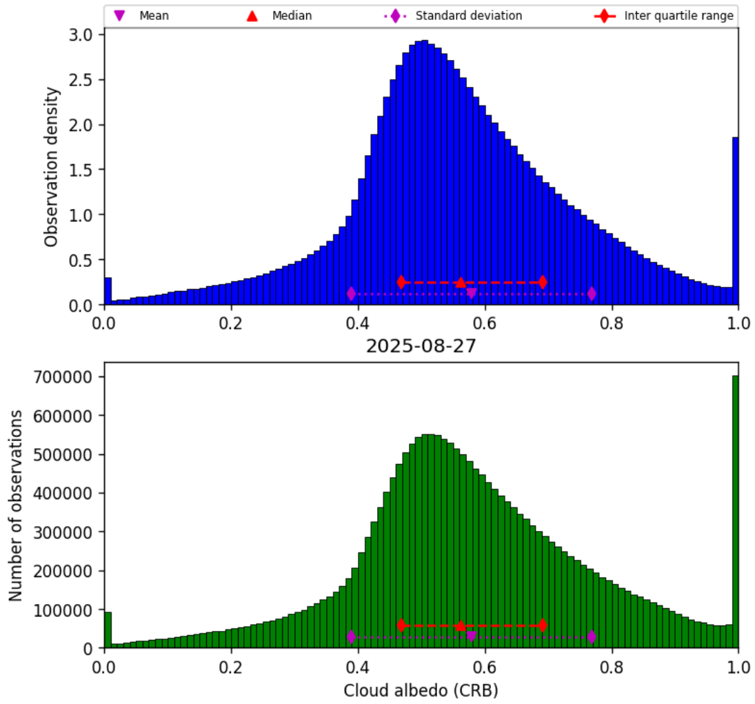
Figure 44: Histogram of “Cloud albedo (CRB)” for 2025-08-26 to 2025-08-28
