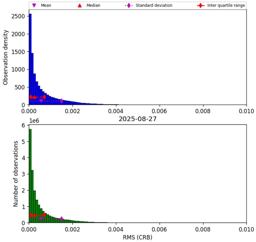
Figure 48: Histogram of “RMS (CRB)” for 2025-08-26 to 2025-08-28
