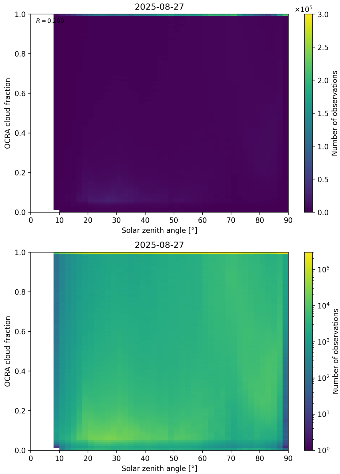
Figure 100: Scatter density plot of “Solar zenith angle” against “OCRA cloud fraction” for 2025-08-26 to 2025-08-28.
