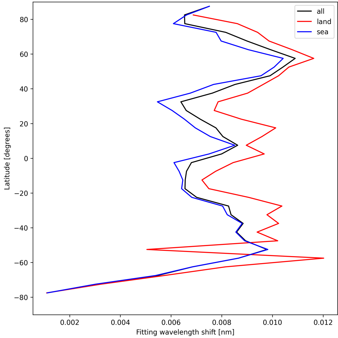
Figure 33: Zonal average of “Fitting wavelength shift” for 2025-08-26 to 2025-08-28.
