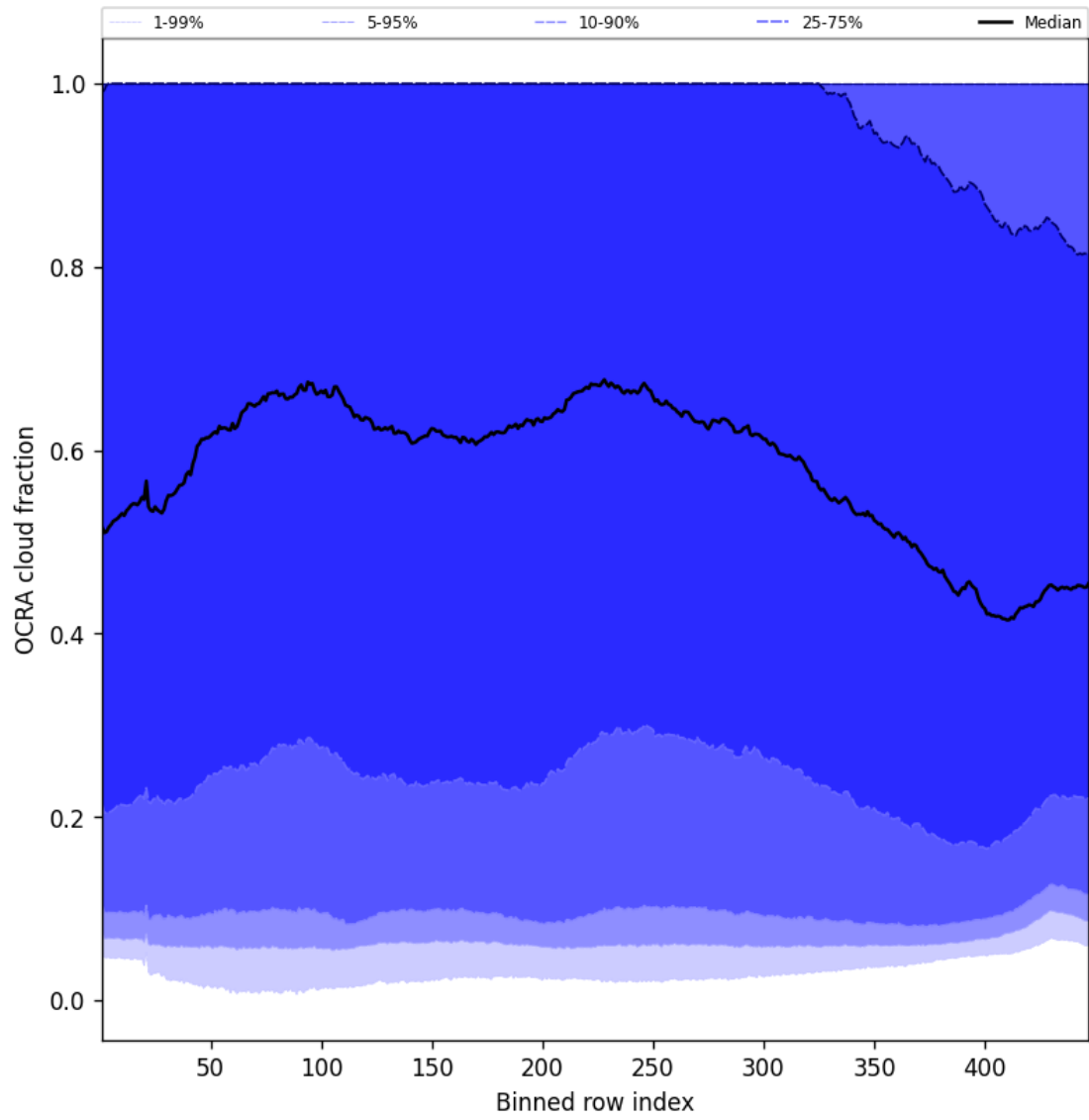
Figure 66: Along track statistics of “OCRA cloud fraction” for 2025-08-26 to 2025-08-28
