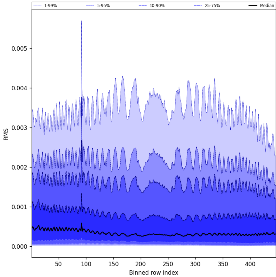
Figure 63: Along track statistics of “RMS” for 2025-08-26 to 2025-08-28
