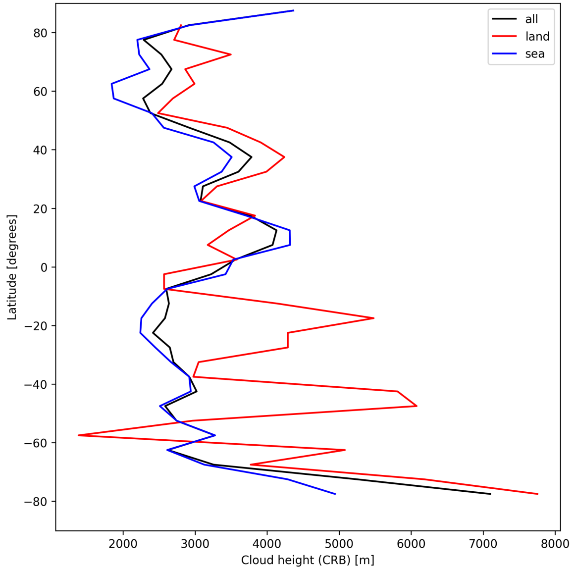
Figure 27: Zonal average of “Cloud height (CRB)” for 2025-08-26 to 2025-08-28.
