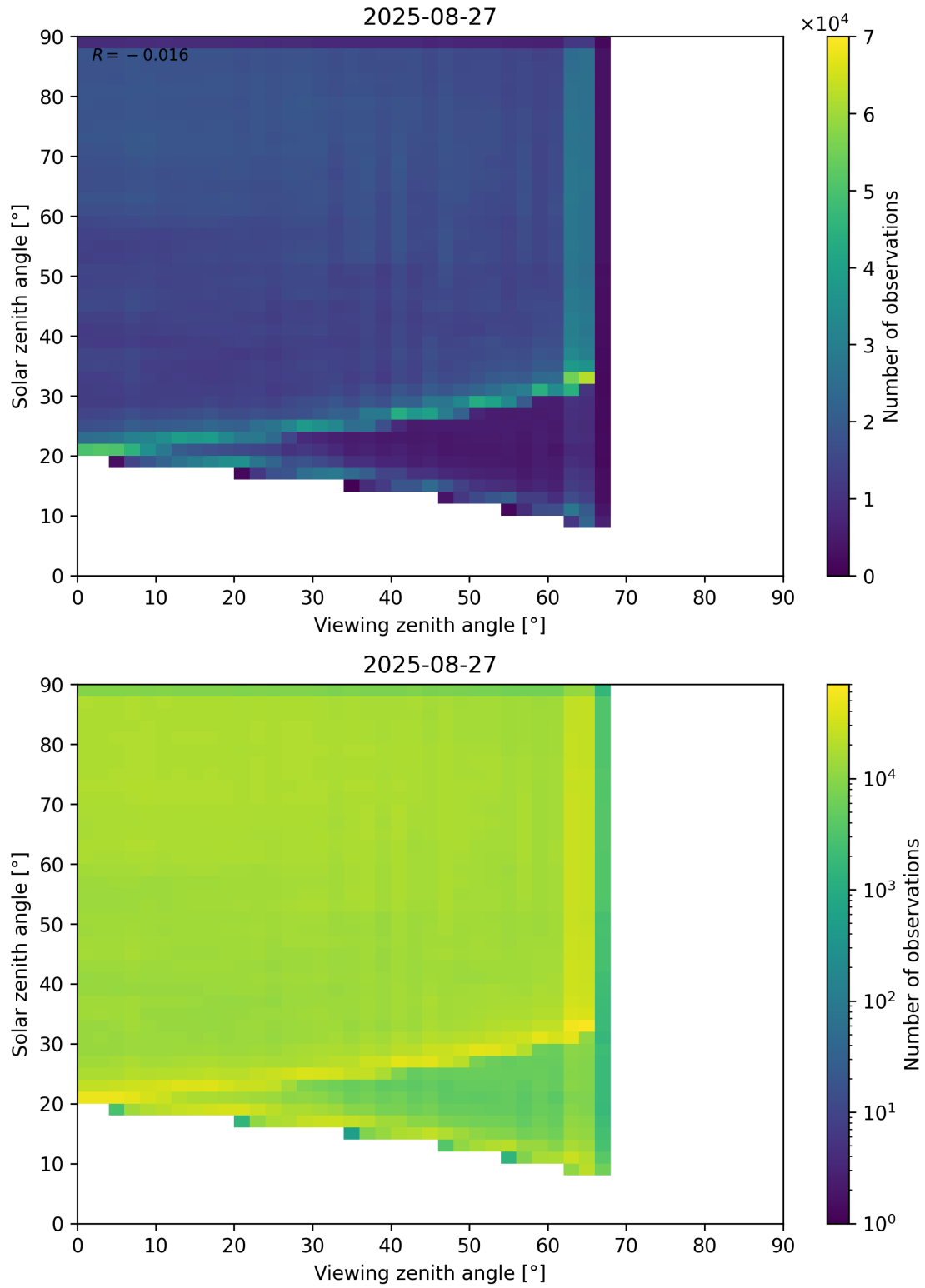
Figure 114: Scatter density plot of “Viewing zenith angle” against “Solar zenith angle” for 2025-08-26 to 2025-08-28.
