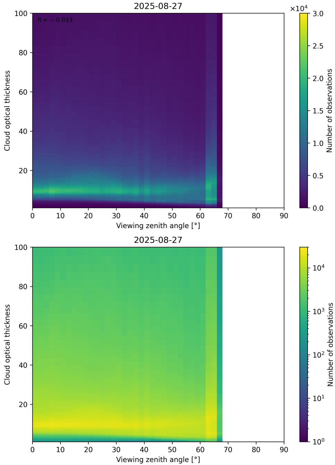
Figure 111: Scatter density plot of “Viewing zenith angle” against “Cloud optical thickness” for 2025-08-26 to 2025-08-28.
