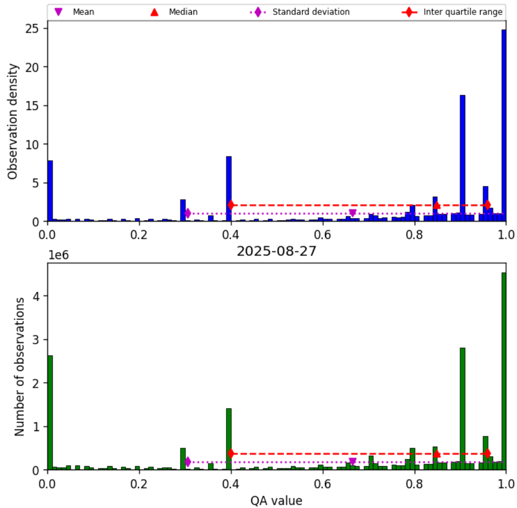
Figure 38: Histogram of “QA value” for 2025-08-26 to 2025-08-28
