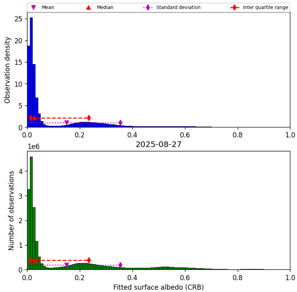
Figure 46: Histogram of “Fitted surface albedo (CRB)” for 2025-08-26 to 2025-08-28
