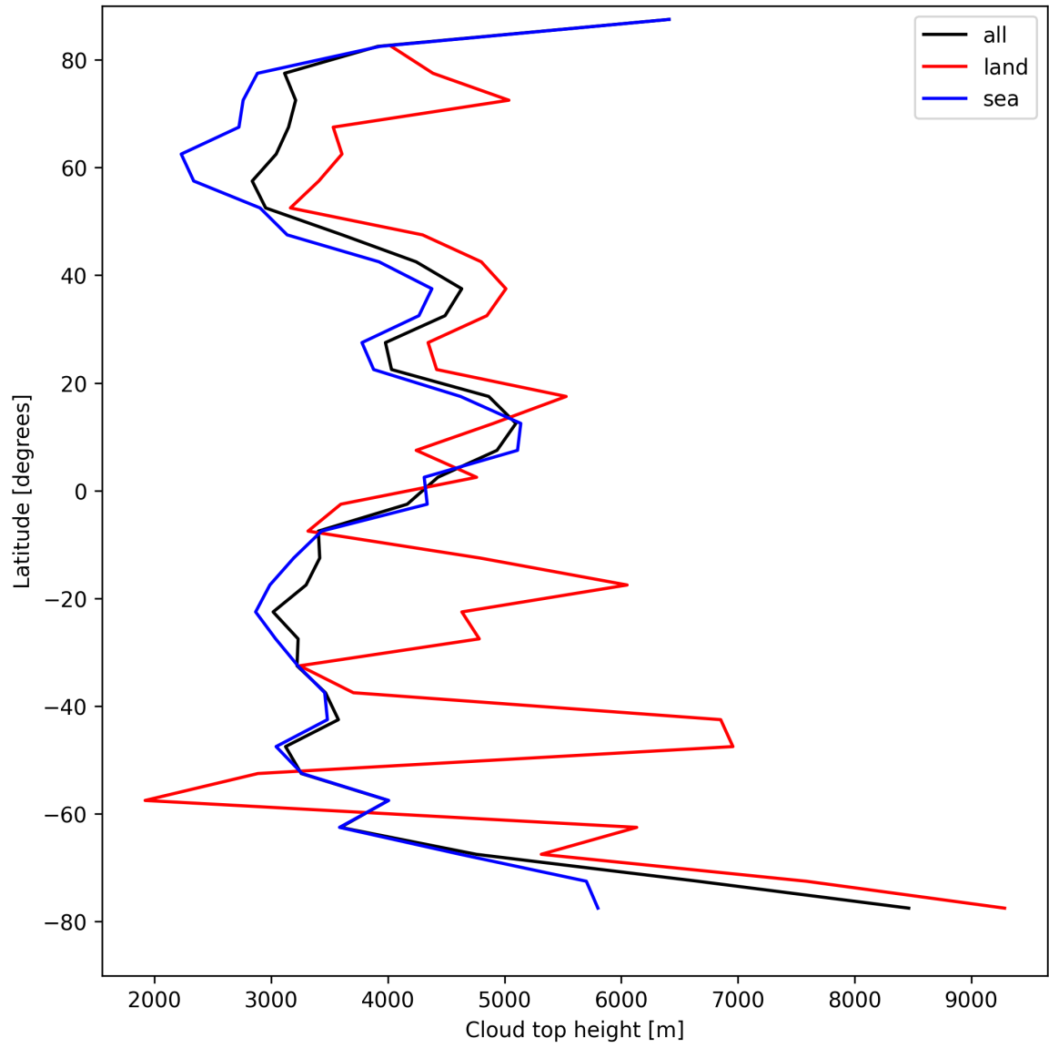
Figure 24: Zonal average of “Cloud top height” for 2025-08-26 to 2025-08-28.
