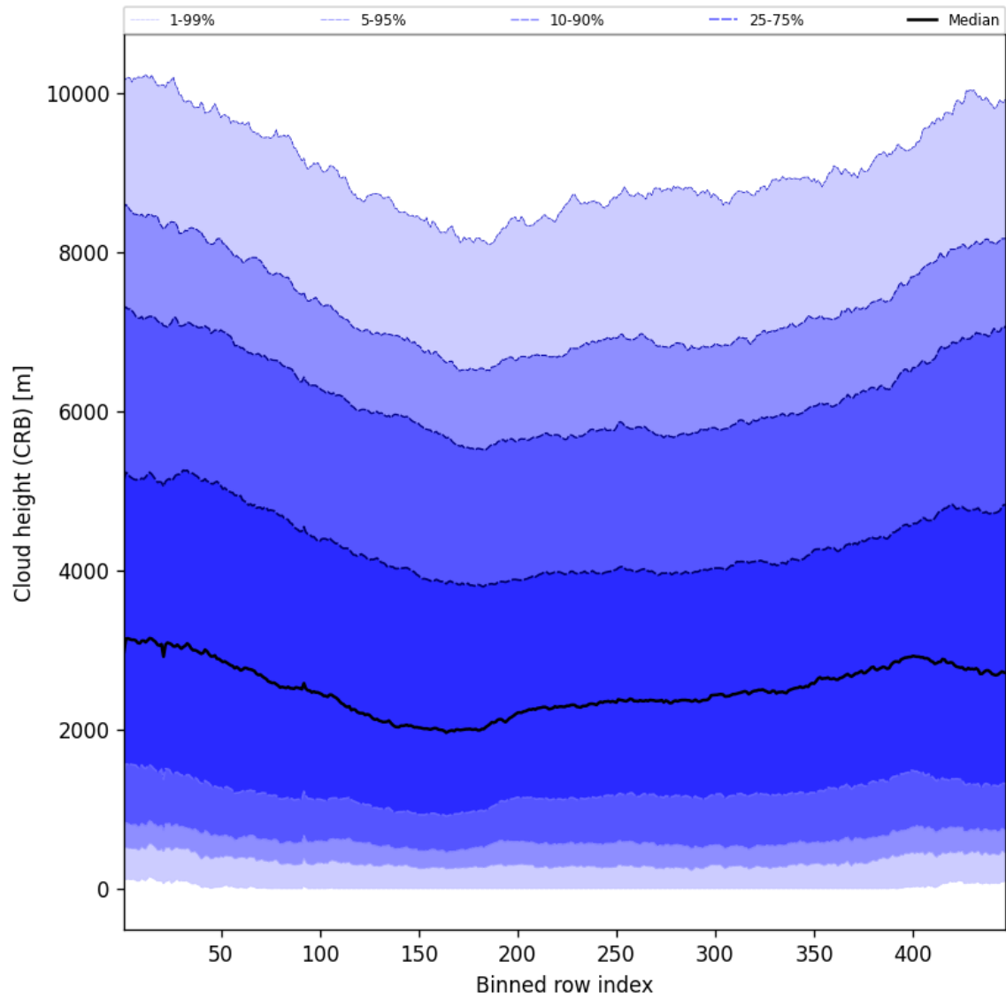
Figure 59: Along track statistics of “Cloud height (CRB)” for 2025-08-26 to 2025-08-28
