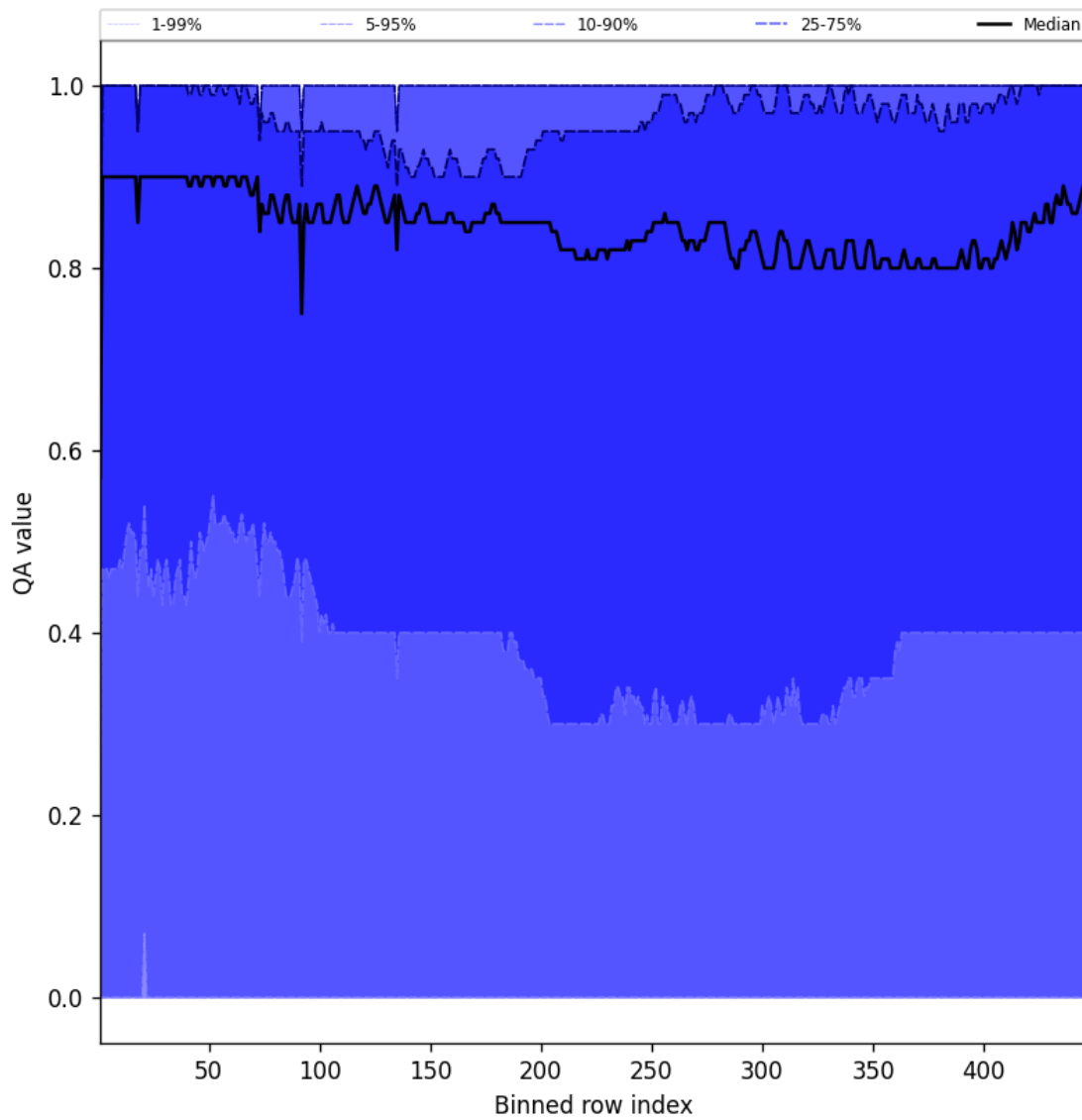
Figure 54: Along track statistics of “QA value” for 2025-08-26 to 2025-08-28
