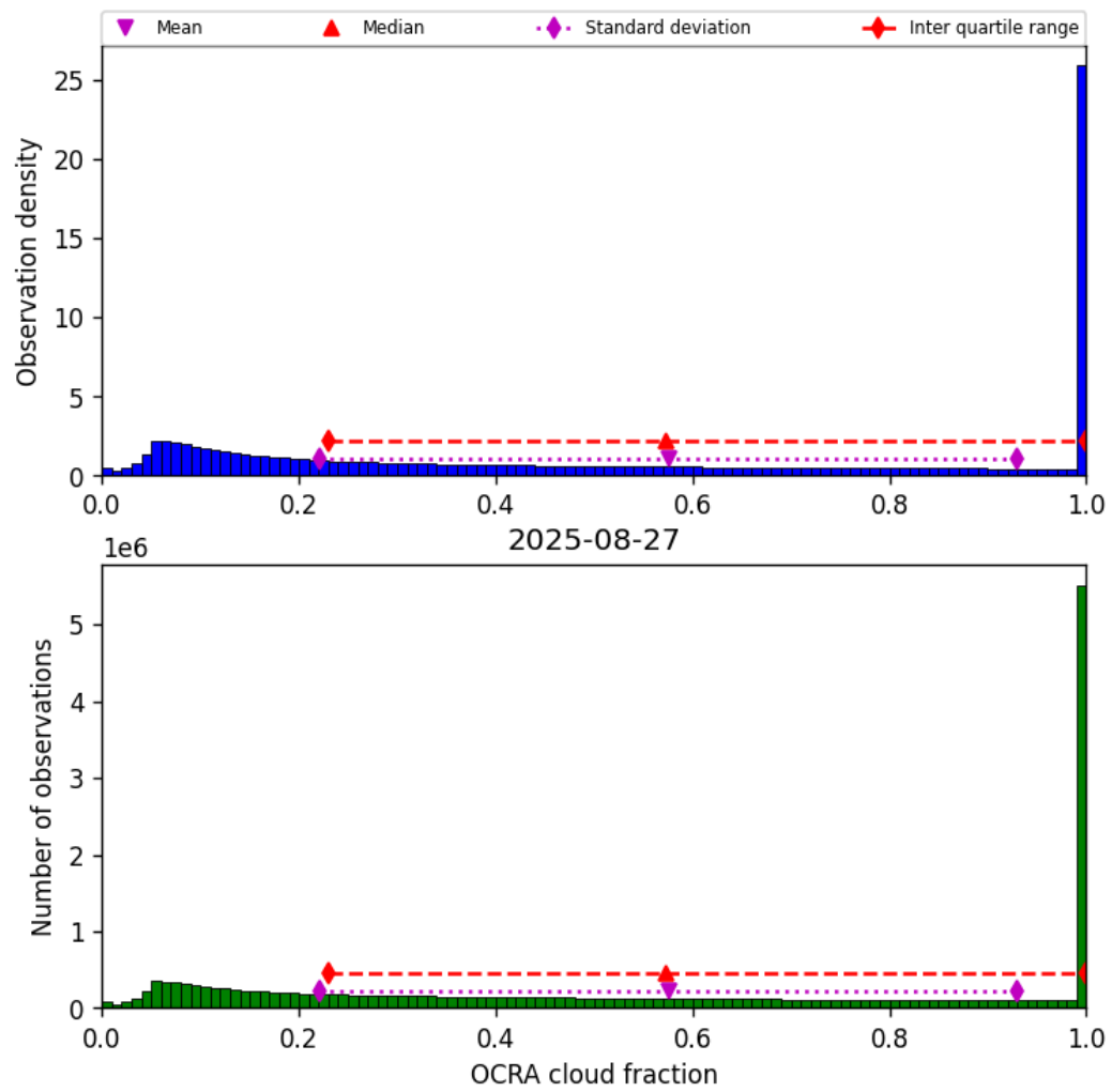
Figure 50: Histogram of “OCRA cloud fraction” for 2025-08-26 to 2025-08-28
