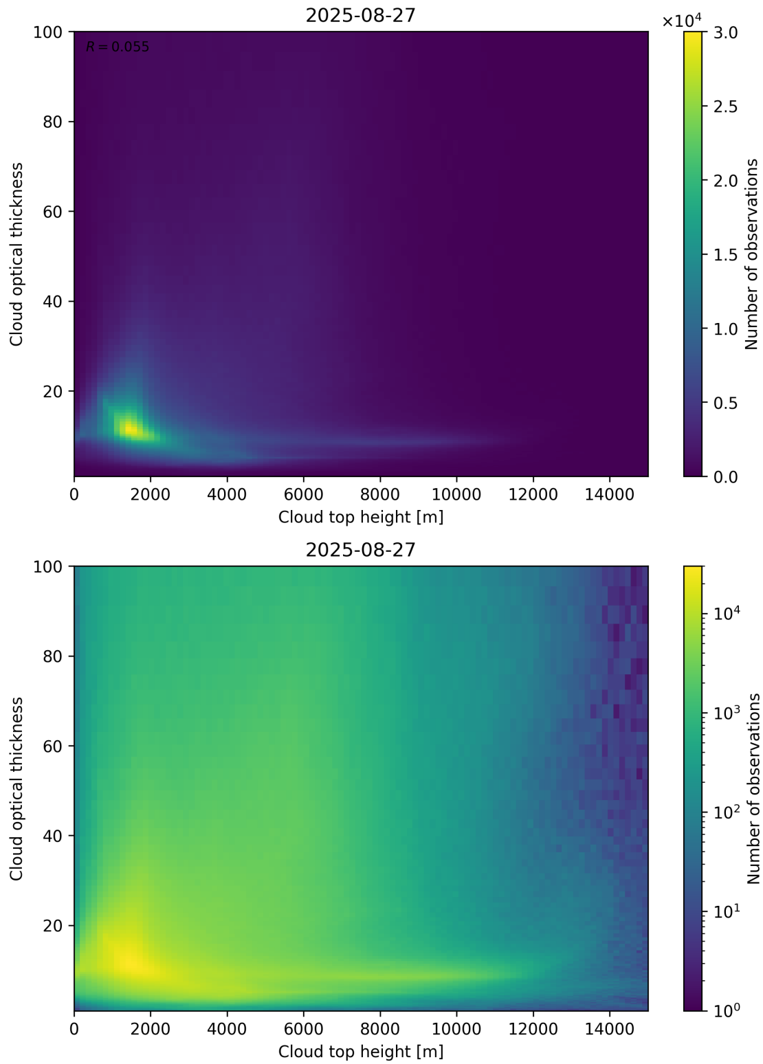
Figure 90: Scatter density plot of “Cloud top height” against “Cloud optical thickness” for 2025-08-26 to 2025-08-28.
