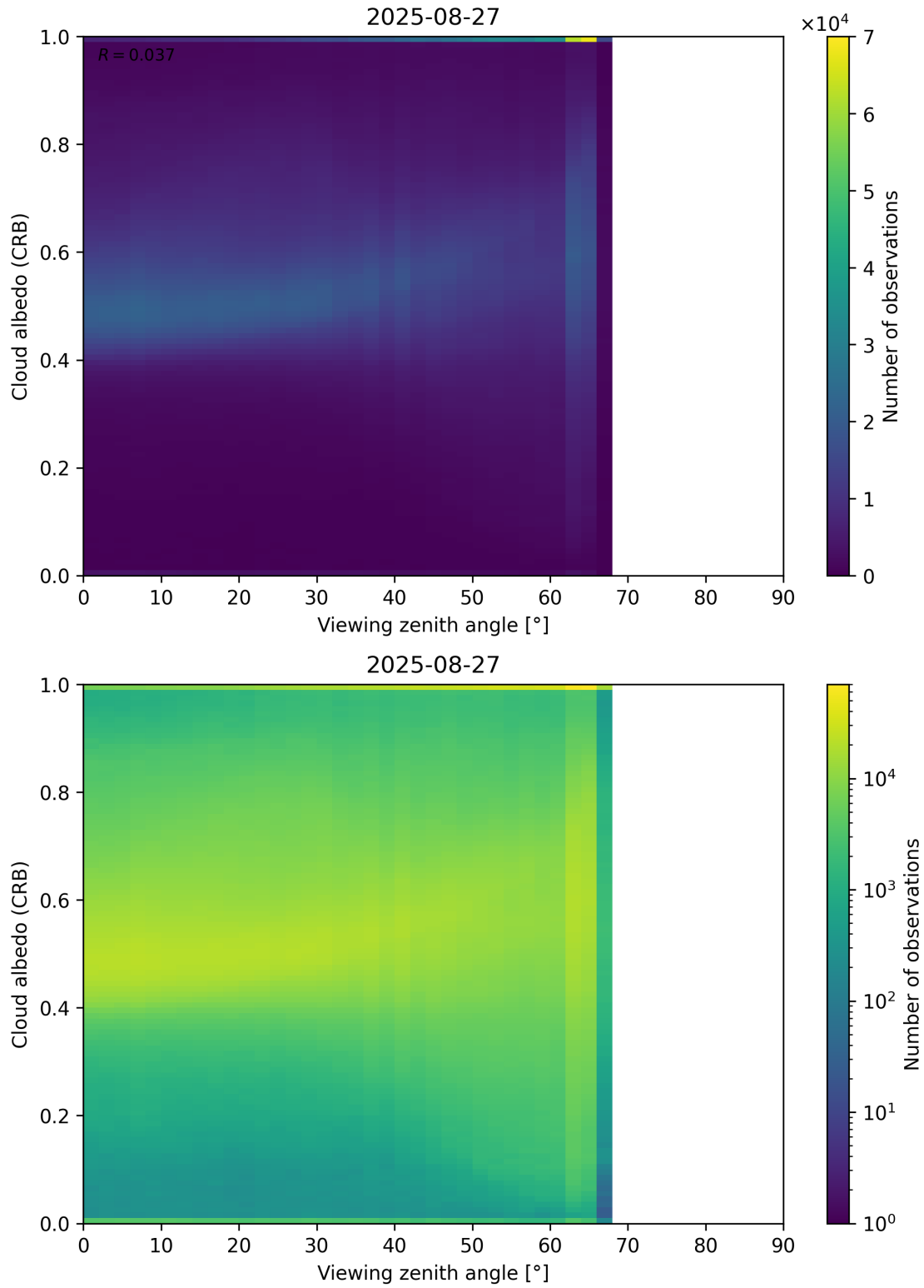
Figure 106: Scatter density plot of “Viewing zenith angle” against “Cloud albedo (CRB)” for 2025-08-26 to 2025-08-28.
