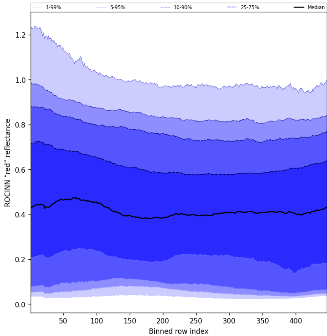
Figure 69: Along track statistics of "ROCINN "red" reflectance" for 2025-08-26 to 2025-08-28
