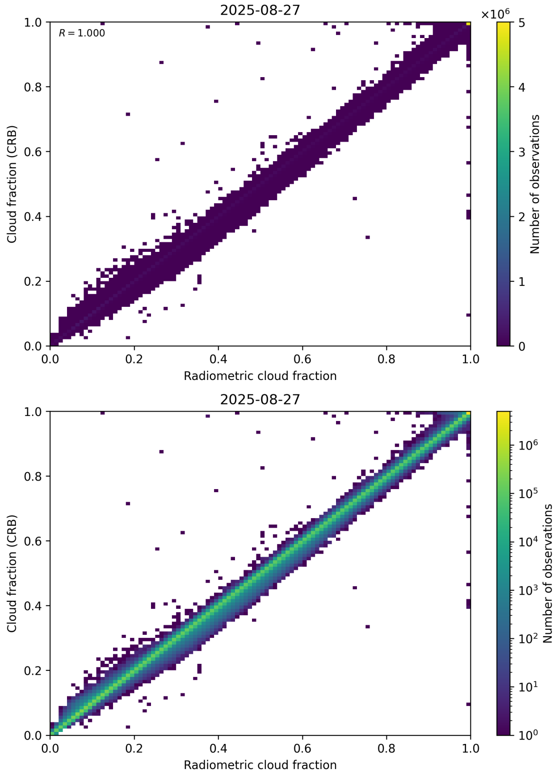
Figure 73: Scatter density plot of “Radiometric cloud fraction” against “Cloud fraction (CRB)” for 2025-08-26 to 2025-08-28.
