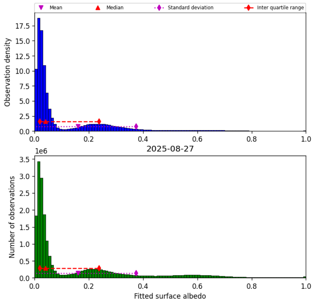
Figure 45: Histogram of “Fitted surface albedo” for 2025-08-26 to 2025-08-28
