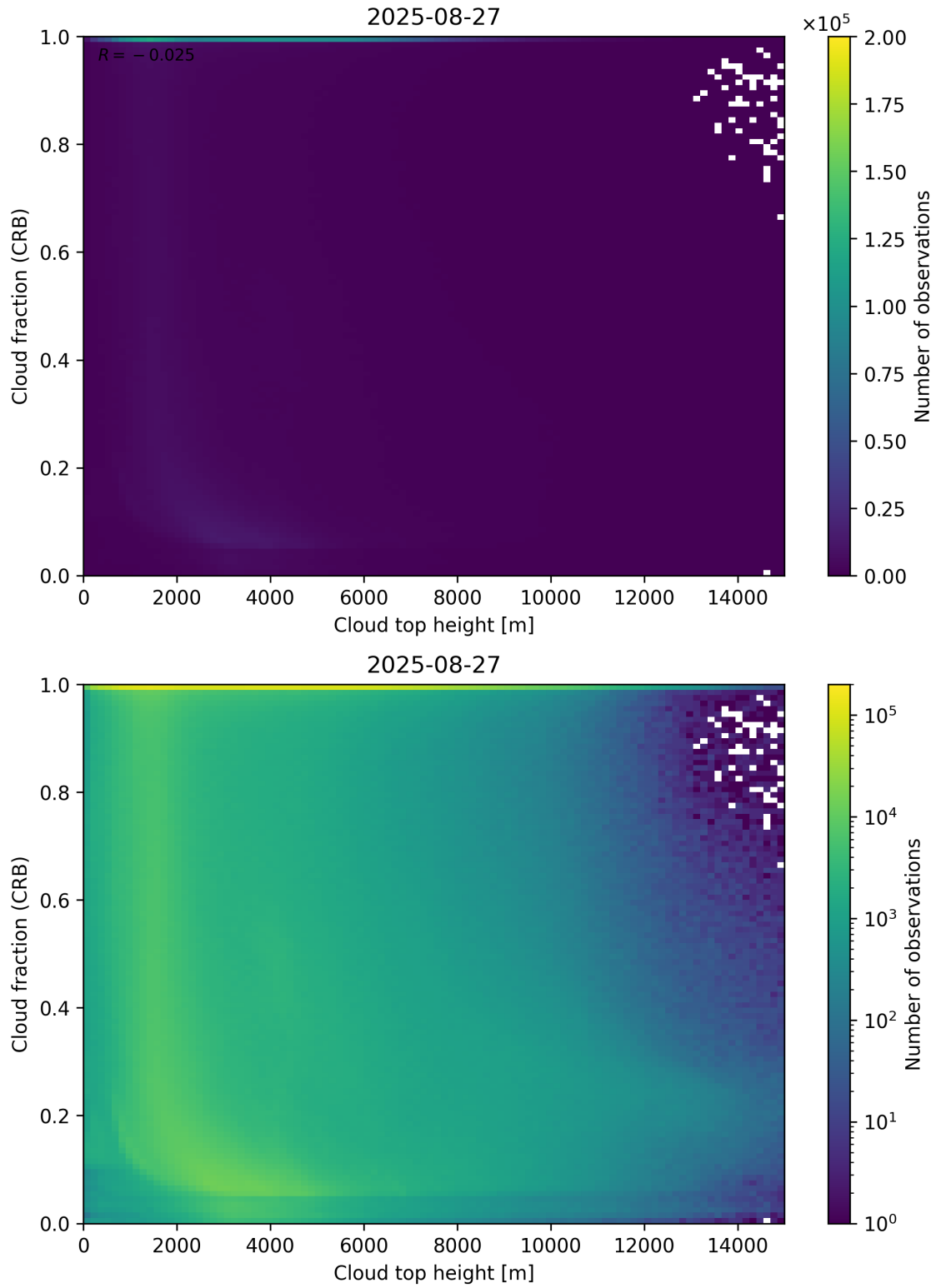
Figure 88: Scatter density plot of “Cloud top height” against “Cloud fraction (CRB)” for 2025-08-26 to 2025-08-28.
