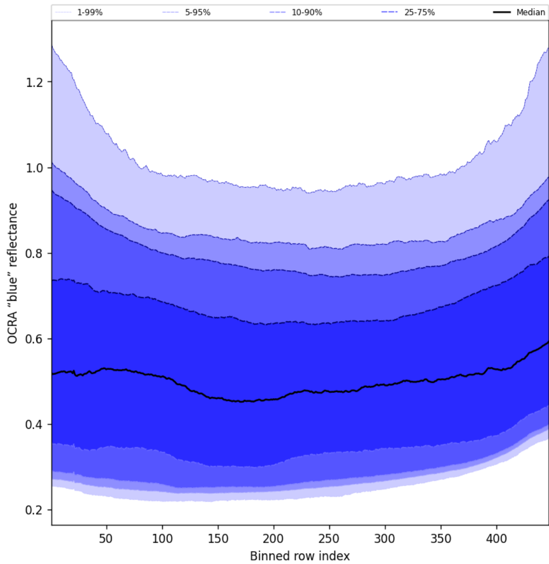
Figure 67: Along track statistics of "OCRA "blue" reflectance" for 2025-08-26 to 2025-08-28
