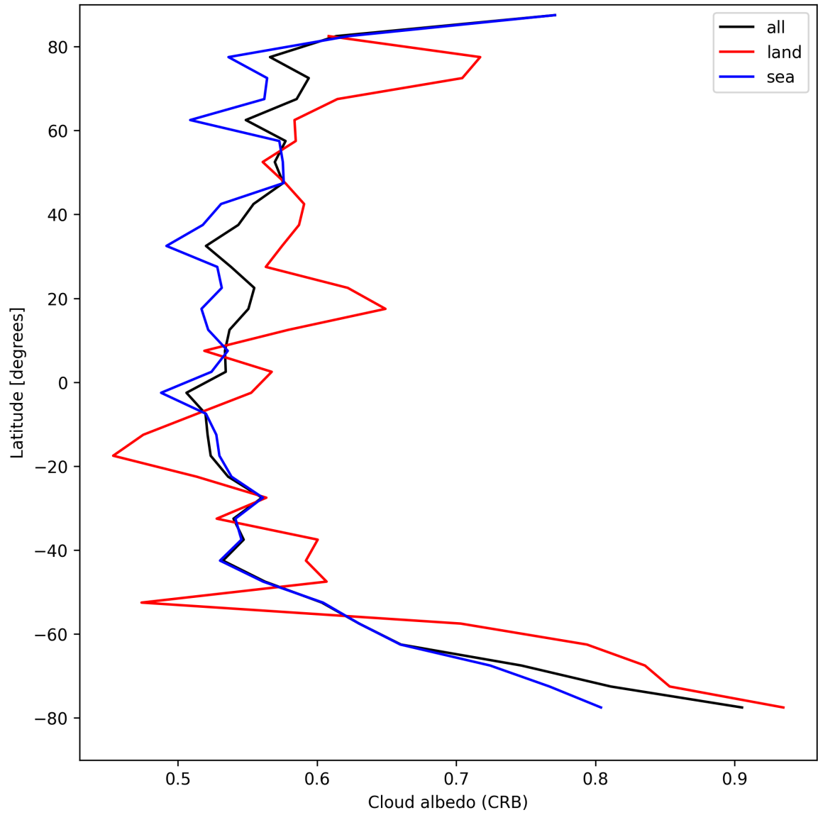
Figure 28: Zonal average of “Cloud albedo (CRB)” for 2025-08-26 to 2025-08-28.
