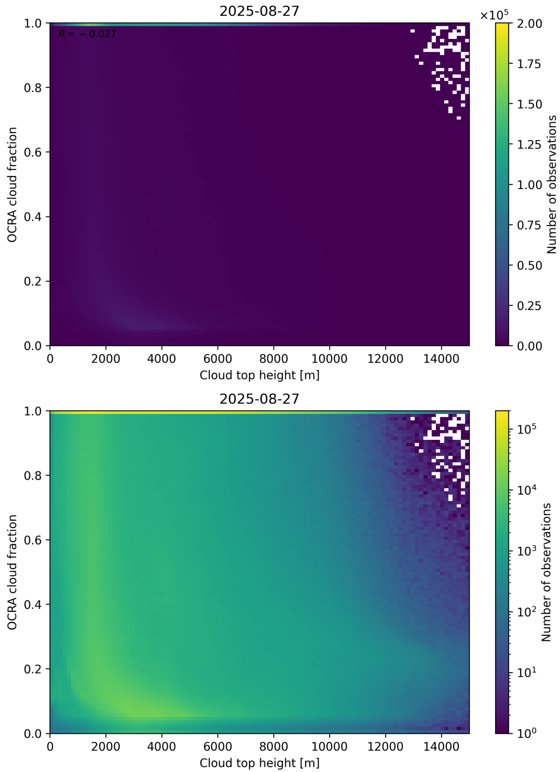
Figure 87: Scatter density plot of “Cloud top height” against “OCRA cloud fraction” for 2025-08-26 to 2025-08-28.
