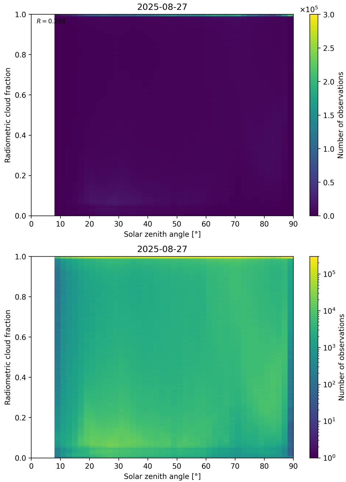
Figure 99: Scatter density plot of “Solar zenith angle” against “Radiometric cloud fraction” for 2025-08-26 to 2025-08-28.
