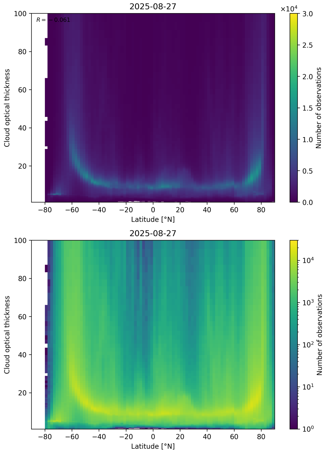
Figure 96: Scatter density plot of “Latitude” against “Cloud optical thickness” for 2025-08-26 to 2025-08-28.
