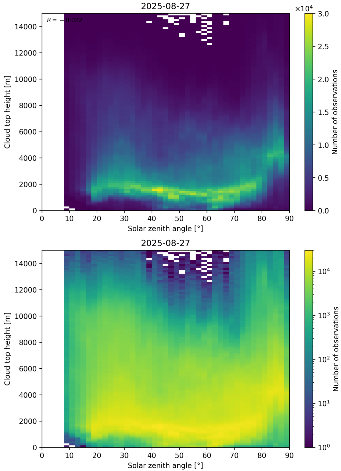
Figure 104: Scatter density plot of “Solar zenith angle” against “Cloud top height” for 2025-08-26 to 2025-08-28.
