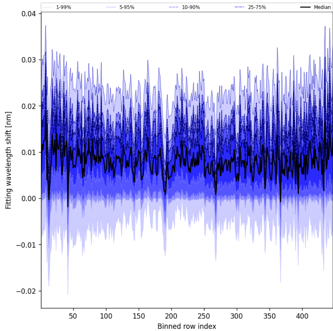
Figure 65: Along track statistics of “Fitting wavelength shift” for 2025-08-26 to 2025-08-28
