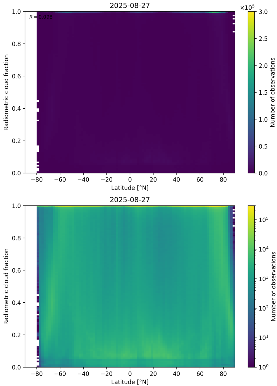
Figure 92: Scatter density plot of “Latitude” against “Radiometric cloud fraction” for 2025-08-26 to 2025-08-28.
