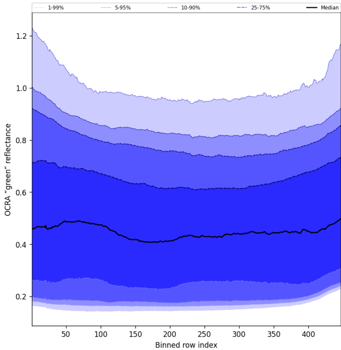
Figure 68: Along track statistics of “OCRA “green” reflectance” for 2025-08-26 to 2025-08-28
