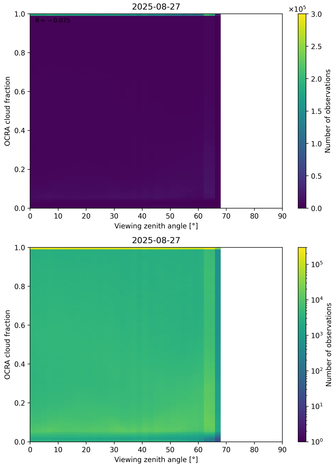
Figure 108: Scatter density plot of “Viewing zenith angle” against “OCRA cloud fraction” for 2025-08-26 to 2025-08-28.
