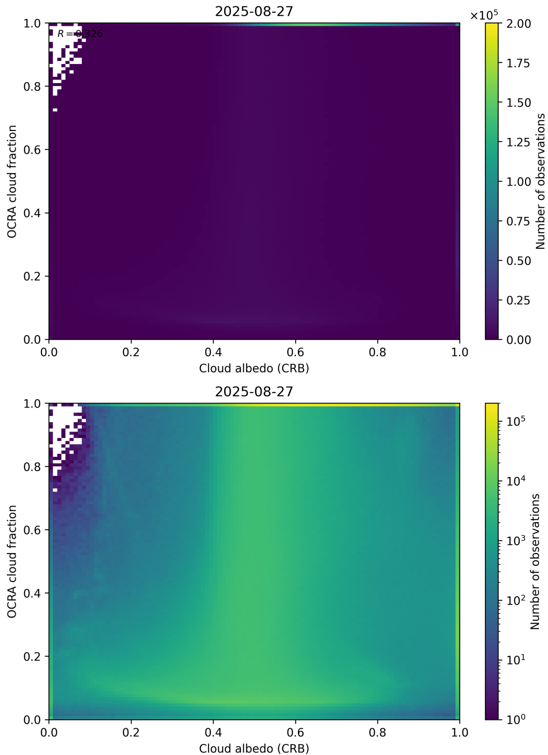
Figure 70: Scatter density plot of “Cloud albedo (CRB)” against “OCRA cloud fraction” for 2025-08-26 to 2025-08-28.
