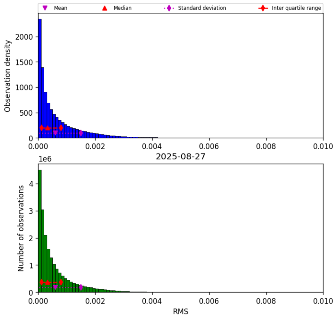
Figure 47: Histogram of “RMS” for 2025-08-26 to 2025-08-28
