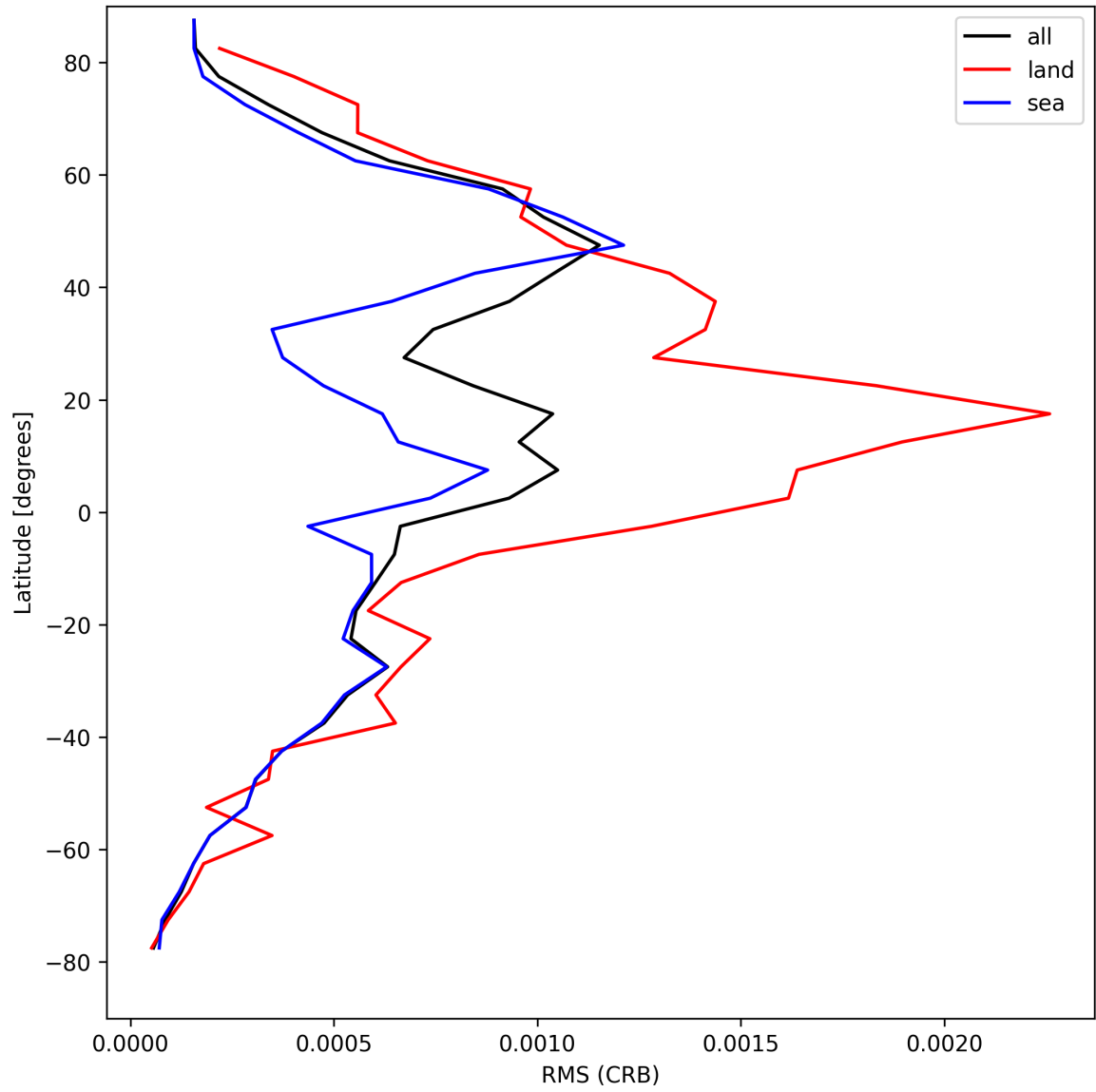
Figure 32: Zonal average of “RMS (CRB)” for 2025-08-26 to 2025-08-28.
