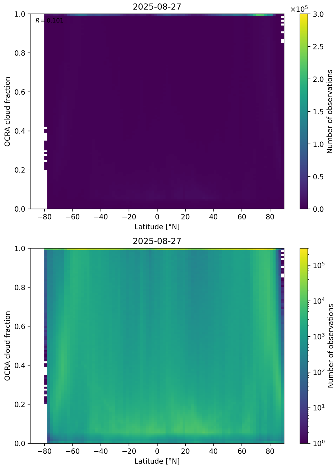
Figure 93: Scatter density plot of “Latitude” against “OCRA cloud fraction” for 2025-08-26 to 2025-08-28.
