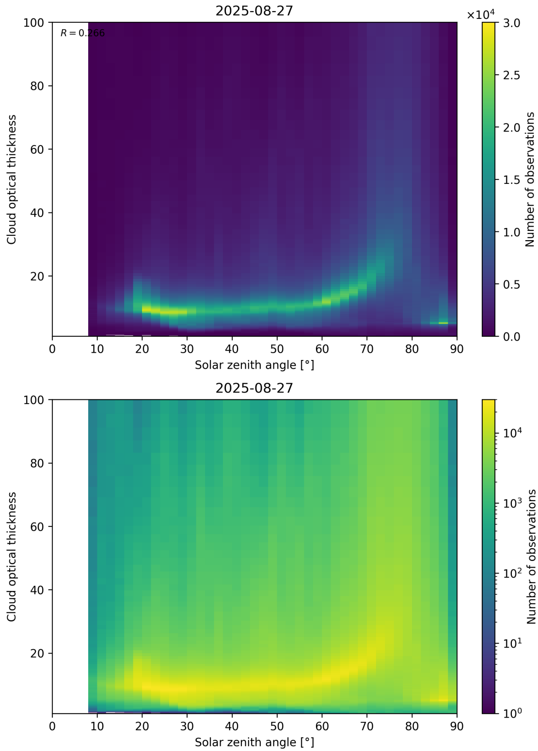
Figure 103: Scatter density plot of “Solar zenith angle” against “Cloud optical thickness” for 2025-08-26 to 2025-08-28.
