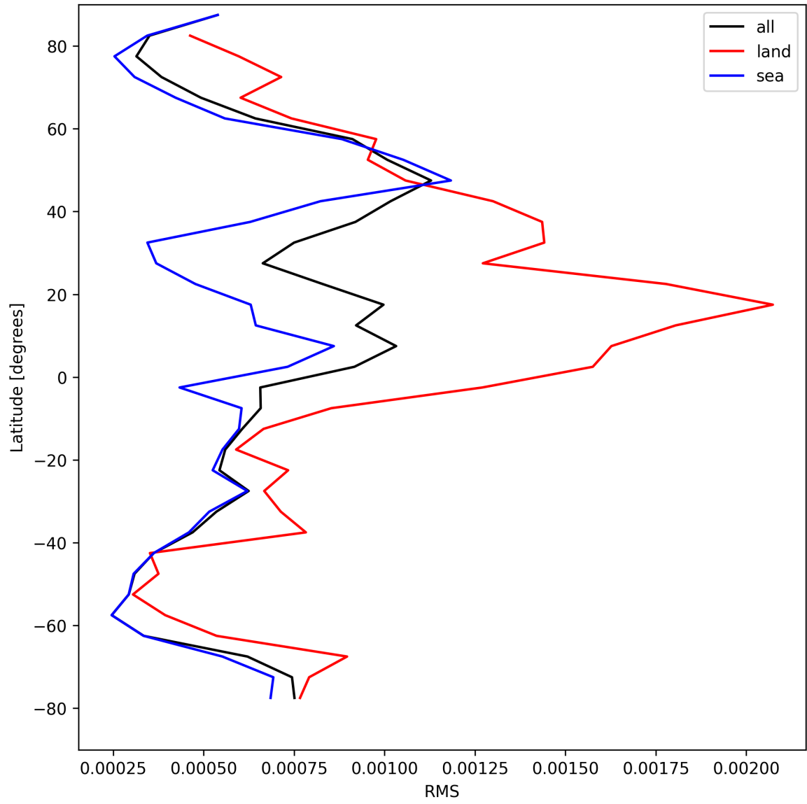
Figure 31: Zonal average of “RMS” for 2025-08-26 to 2025-08-28.
