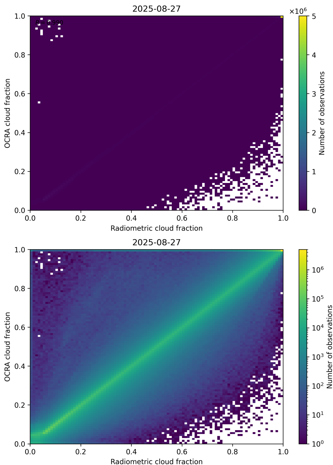
Figure 72: Scatter density plot of “Radiometric cloud fraction” against “OCRA cloud fraction” for 2025-08-26 to 2025-08-28.
