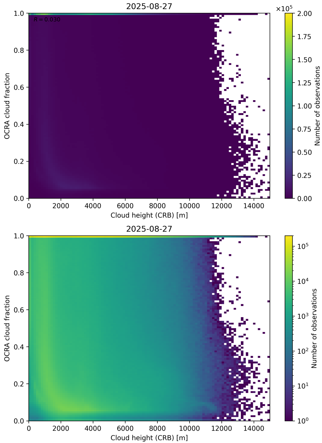
Figure 81: Scatter density plot of “Cloud height (CRB)” against “OCRA cloud fraction” for 2025-08-26 to 2025-08-28.
