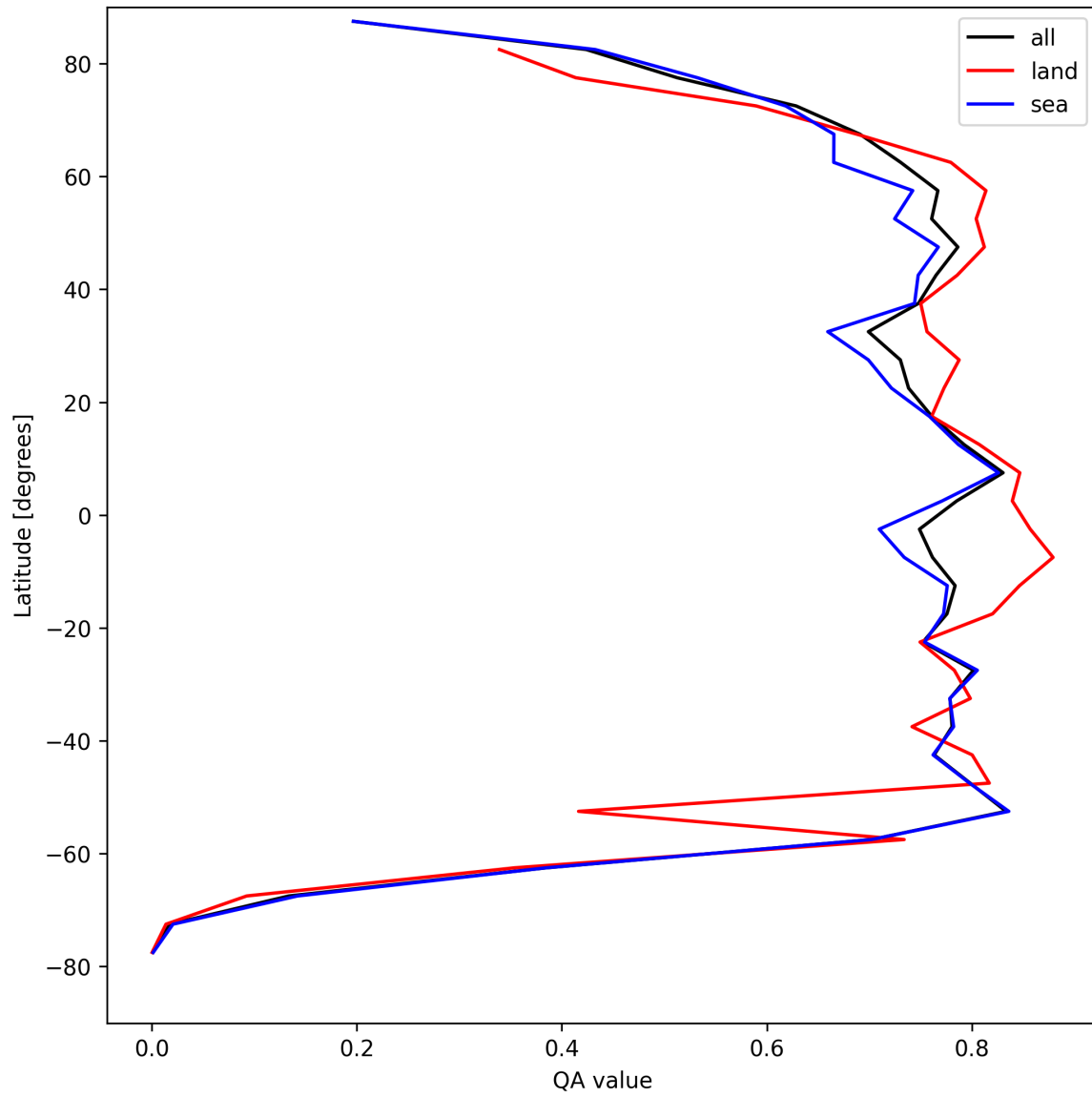
Figure 22: Zonal average of “QA value” for 2025-08-26 to 2025-08-28.
