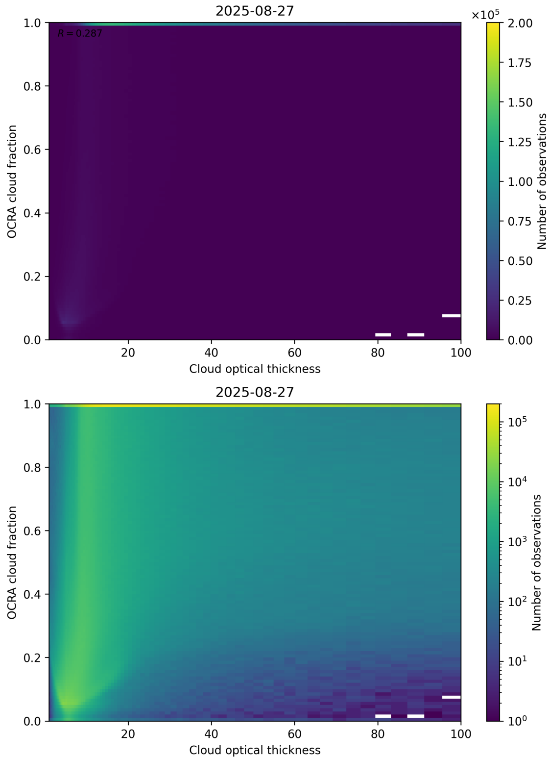
Figure 83: Scatter density plot of “Cloud optical thickness” against “OCRA cloud fraction” for 2025-08-26 to 2025-08-28.
