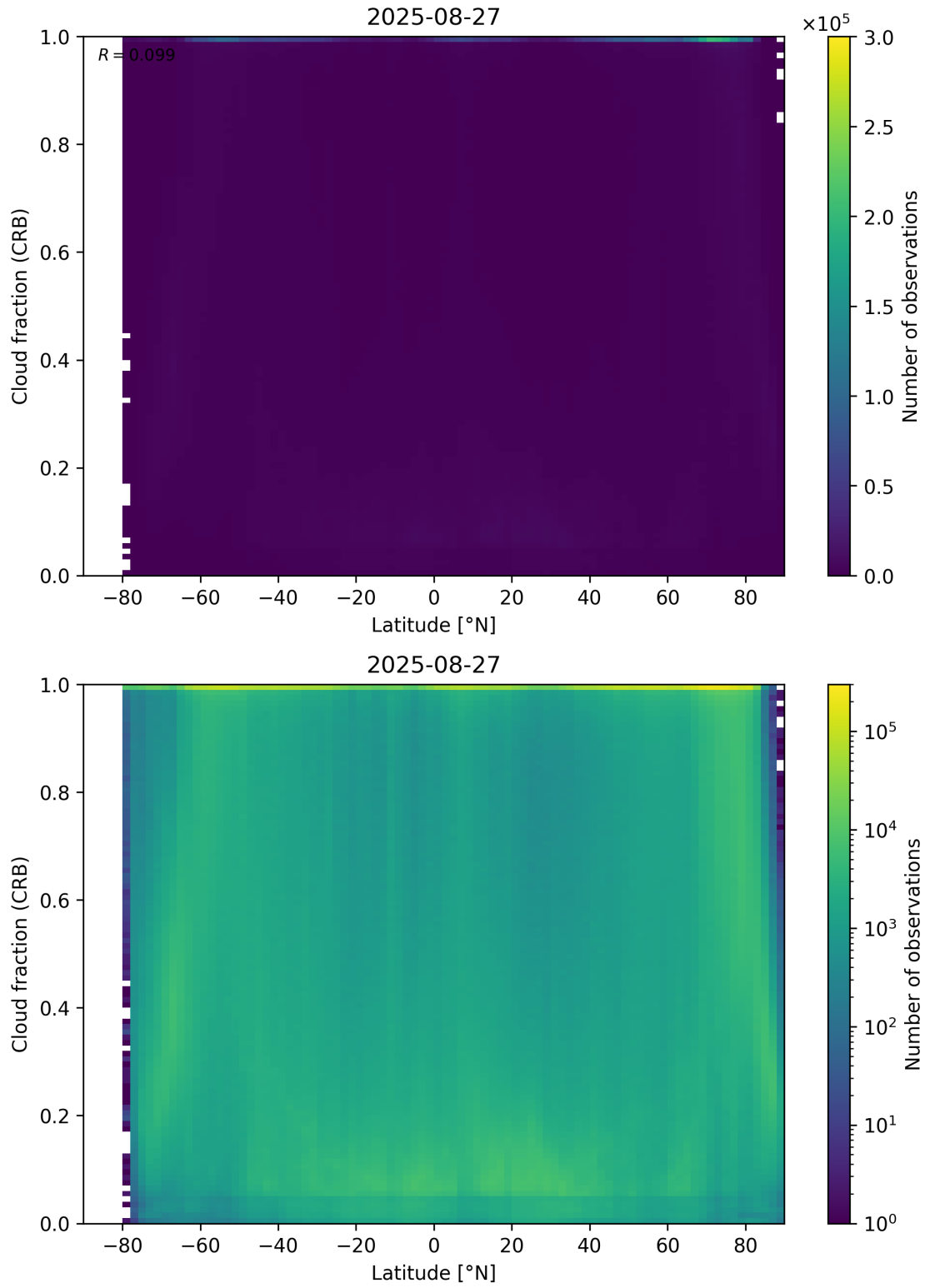
Figure 94: Scatter density plot of “Latitude” against “Cloud fraction (CRB)” for 2025-08-26 to 2025-08-28.
