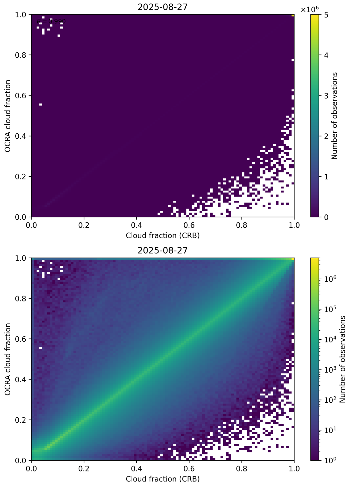
Figure 78: Scatter density plot of “Cloud fraction (CRB)” against “OCRA cloud fraction” for 2025-08-26 to 2025-08-28.
