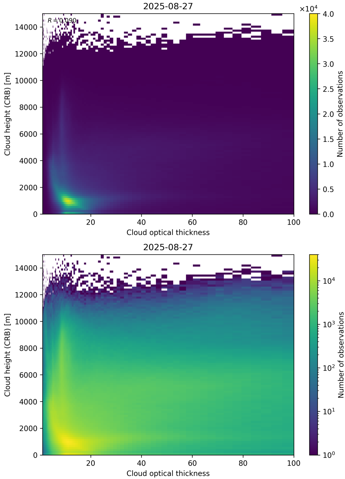
Figure 85: Scatter density plot of “Cloud optical thickness” against “Cloud height (CRB)” for 2025-08-26 to 2025-08-28.
