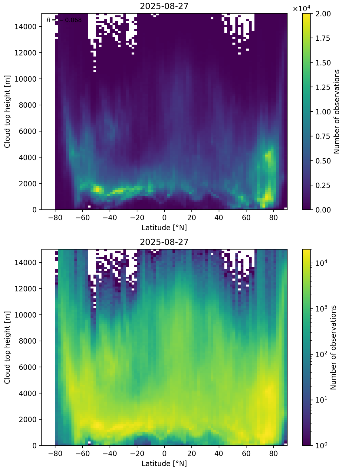
Figure 97: Scatter density plot of “Latitude” against “Cloud top height” for 2025-08-26 to 2025-08-28.
