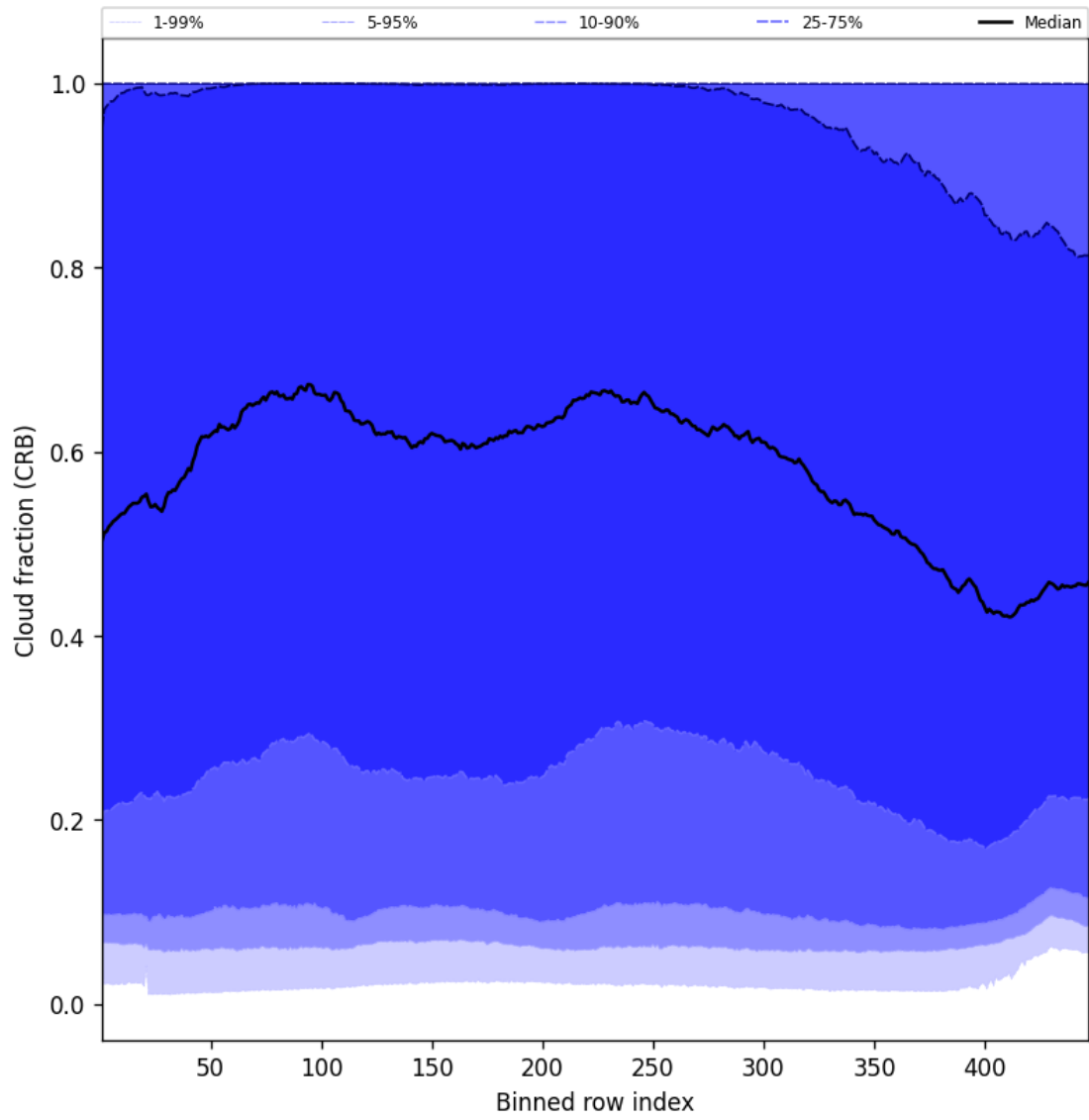
Figure 58: Along track statistics of “Cloud fraction (CRB)” for 2025-08-26 to 2025-08-28
