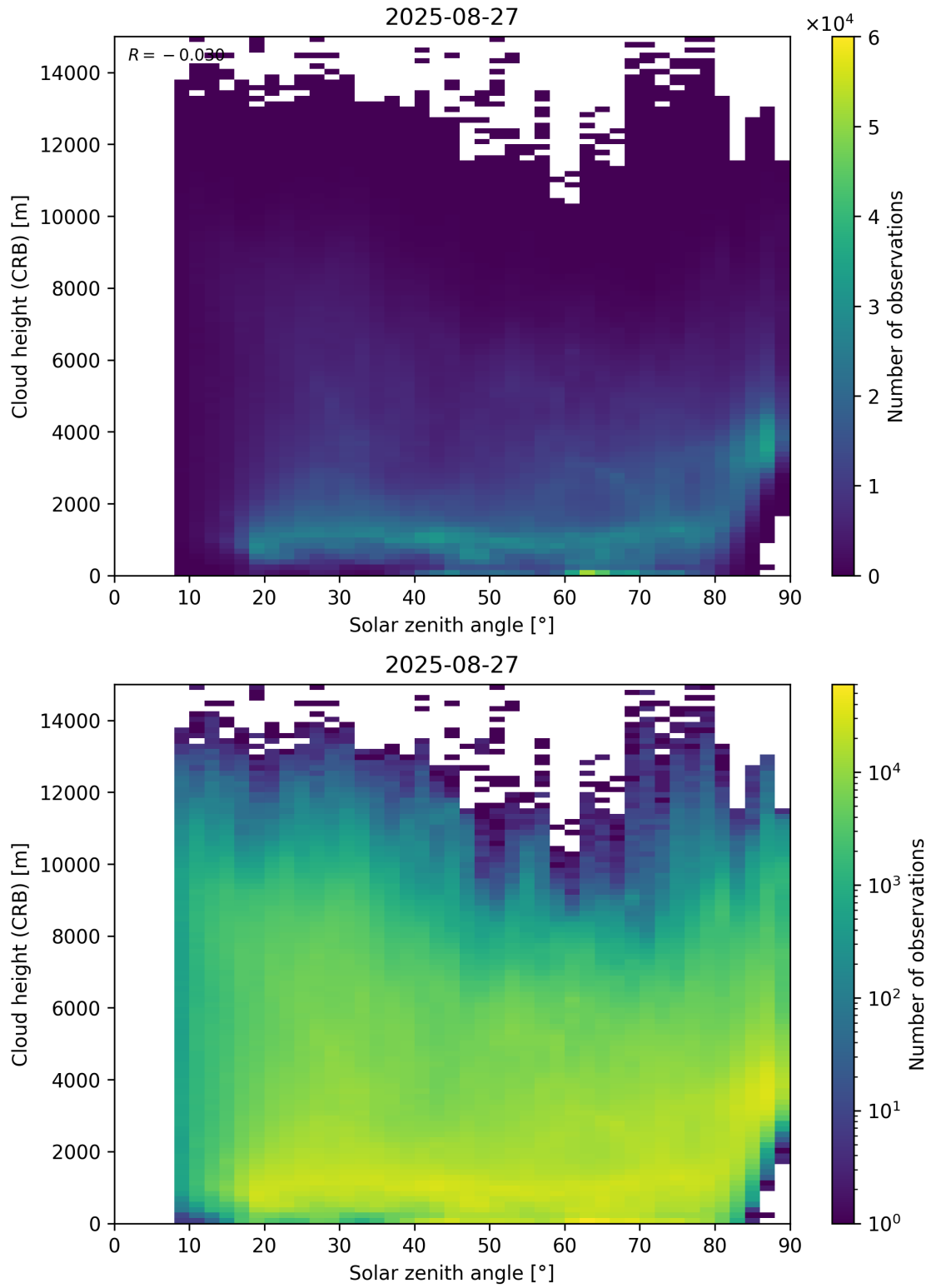
Figure 102: Scatter density plot of “Solar zenith angle” against “Cloud height (CRB)” for 2025-08-26 to 2025-08-28.
