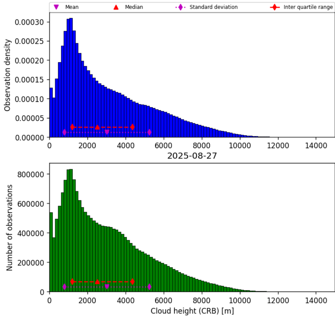
Figure 43: Histogram of “Cloud height (CRB)” for 2025-08-26 to 2025-08-28
