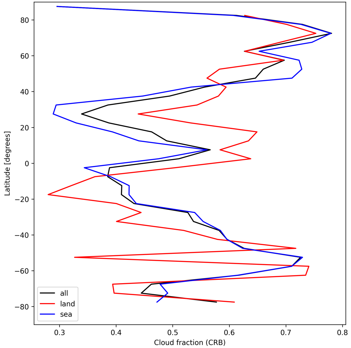
Figure 26: Zonal average of “Cloud fraction (CRB)” for 2025-08-26 to 2025-08-28.
