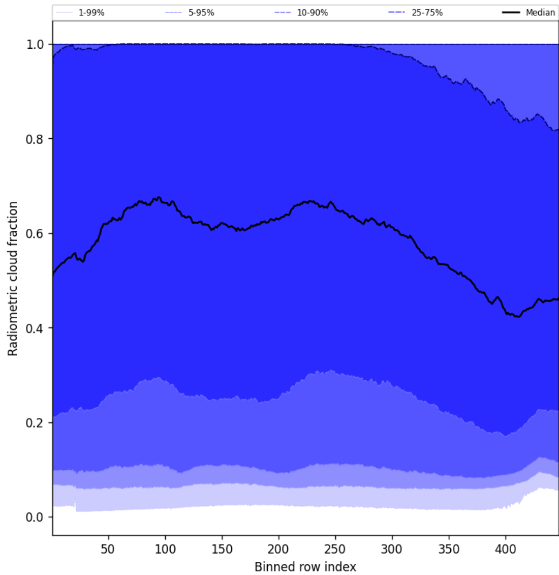
Figure 55: Along track statistics of “Radiometric cloud fraction” for 2025-08-26 to 2025-08-28
