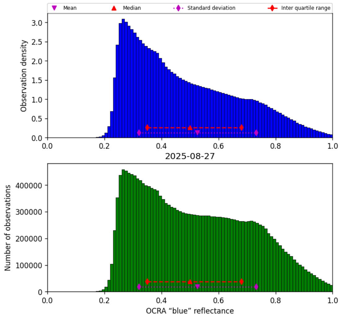
Figure 51: Histogram of “OCRA “blue” reflectance” for 2025-08-26 to 2025-08-28
