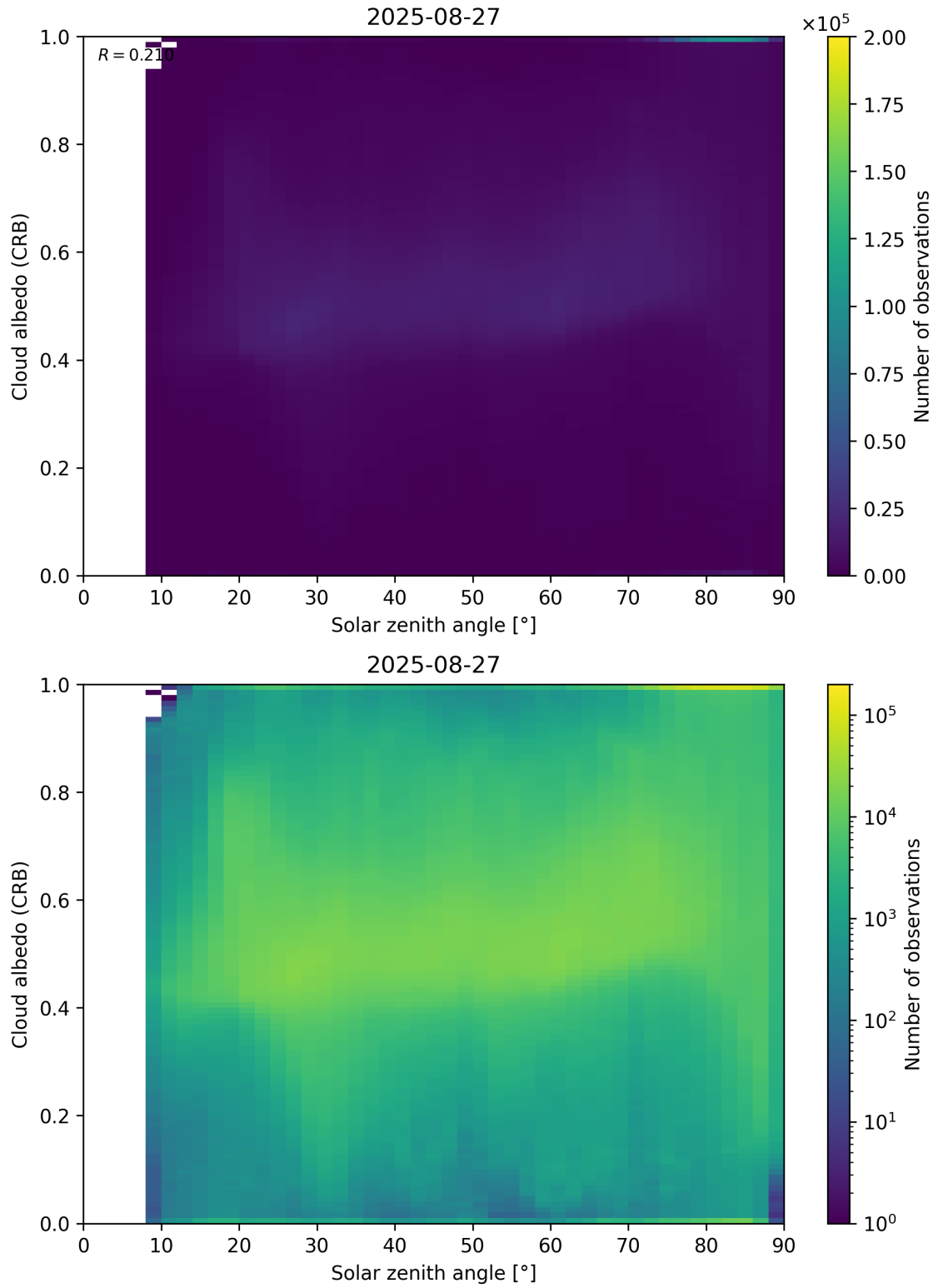
Figure 98: Scatter density plot of “Solar zenith angle” against “Cloud albedo (CRB)” for 2025-08-26 to 2025-08-28.
