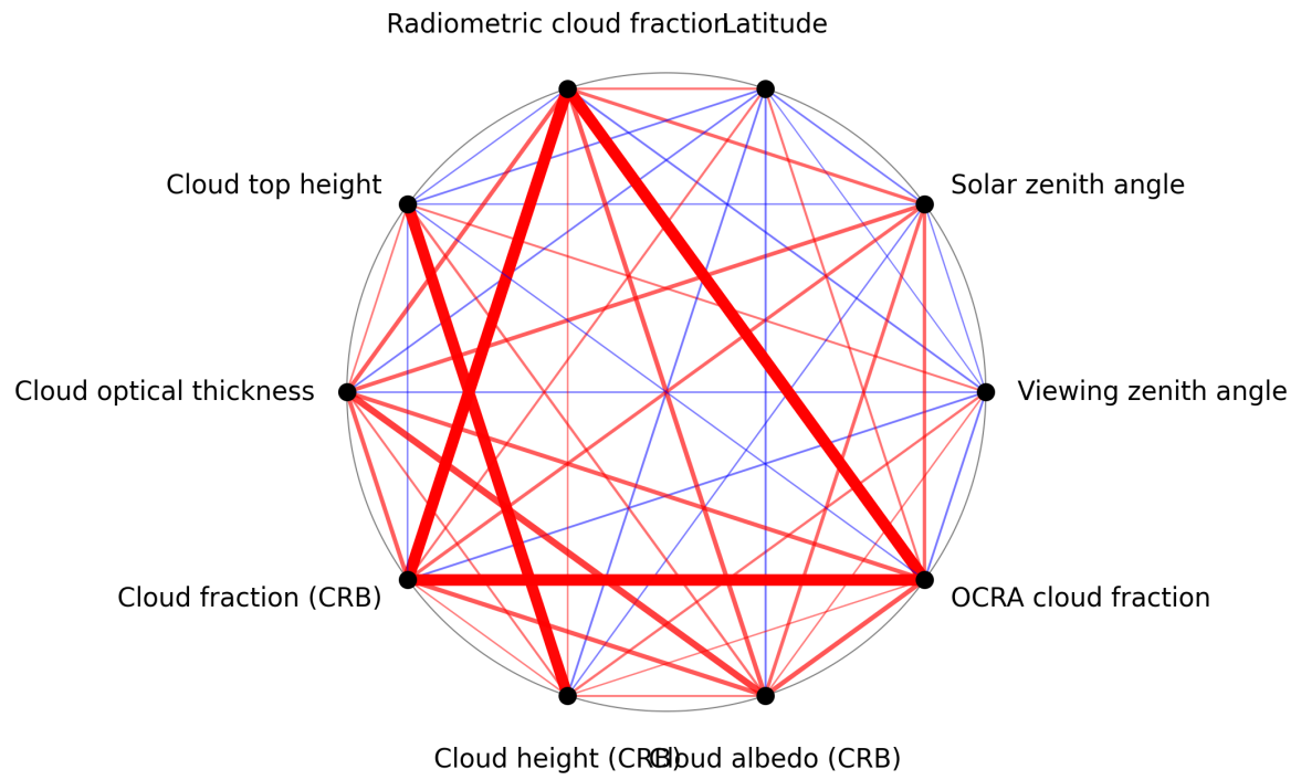
Figure 1: Map of correlation graph for 2025-08-26 to 2025-08-28.
