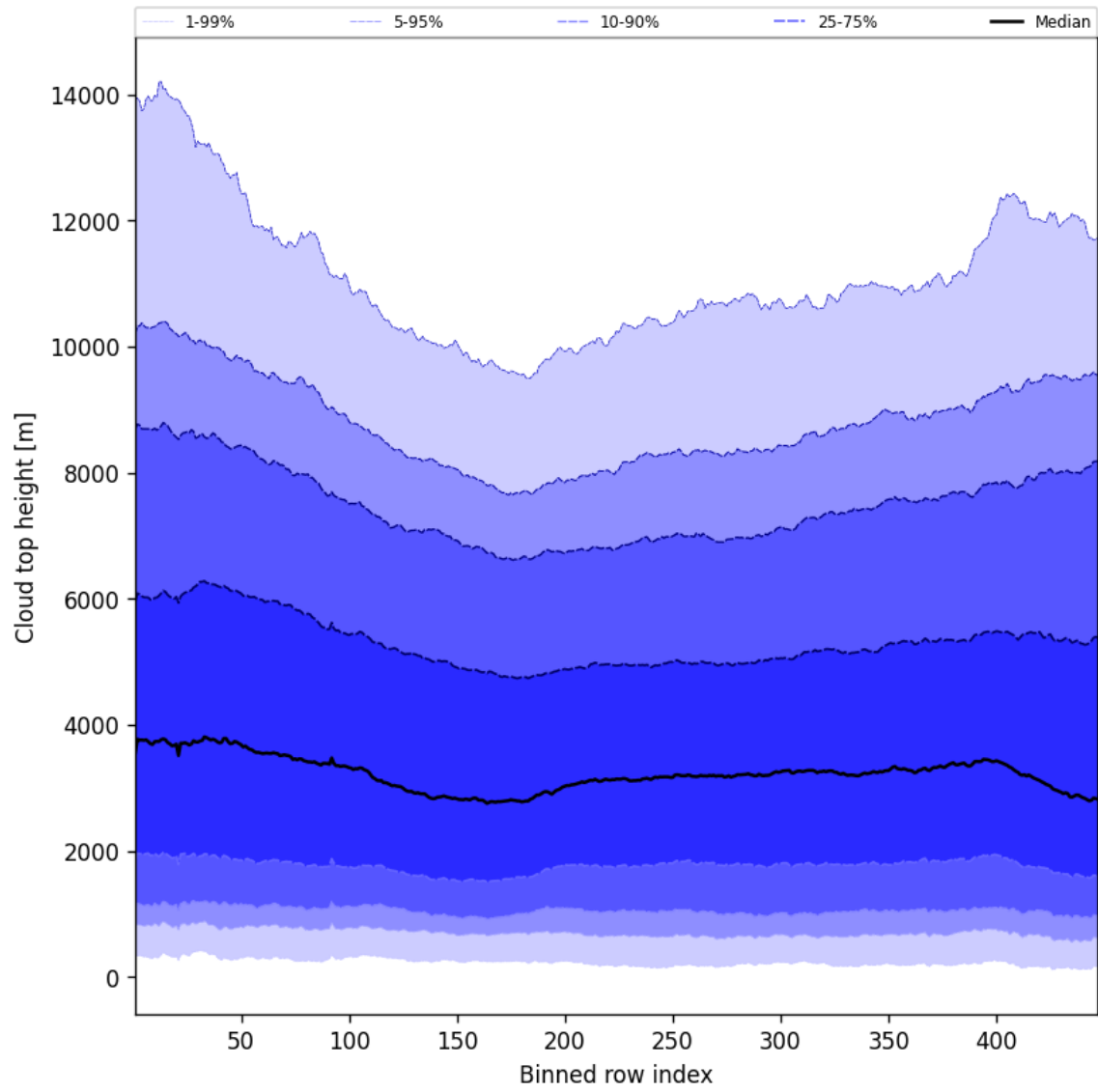
Figure 56: Along track statistics of “Cloud top height” for 2025-08-26 to 2025-08-28
