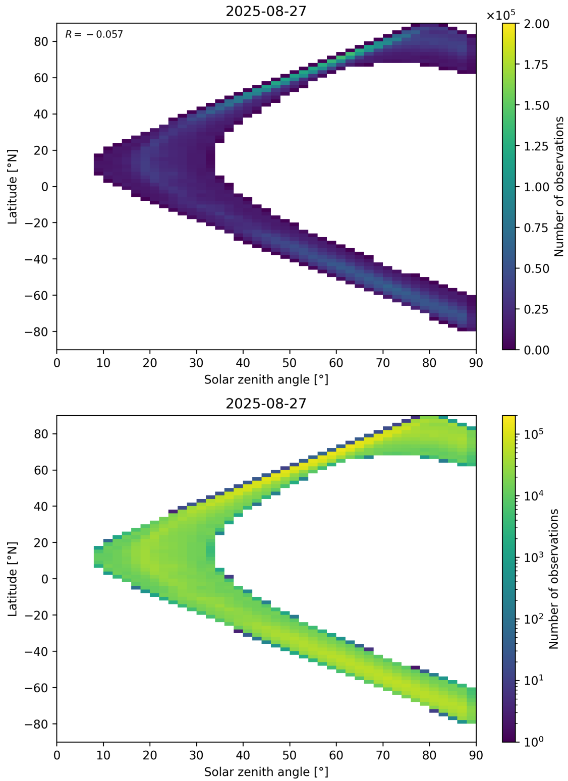
Figure 105: Scatter density plot of “Solar zenith angle” against “Latitude” for 2025-08-26 to 2025-08-28.
