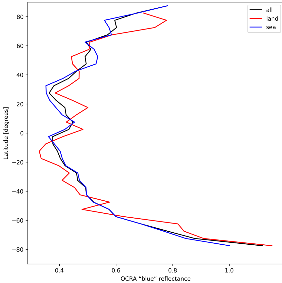
Figure 35: Zonal average of “OCRA “blue” reflectance” for 2025-08-26 to 2025-08-28.
