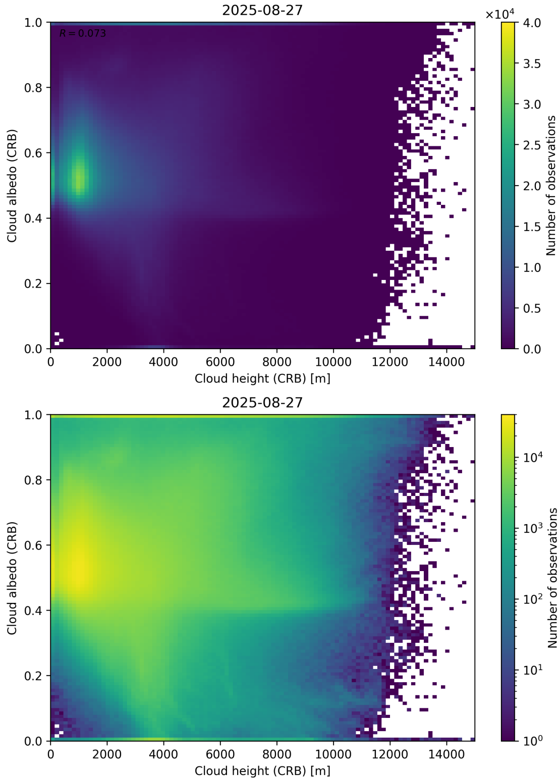
Figure 80: Scatter density plot of “Cloud height (CRB)” against “Cloud albedo (CRB)” for 2025-08-26 to 2025-08-28.
