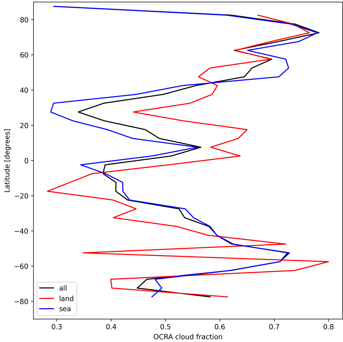
Figure 34: Zonal average of “OCRA cloud fraction” for 2025-08-26 to 2025-08-28.
