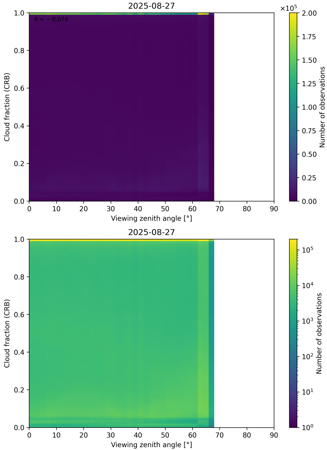
Figure 109: Scatter density plot of “Viewing zenith angle” against “Cloud fraction (CRB)” for 2025-08-26 to 2025-08-28.
