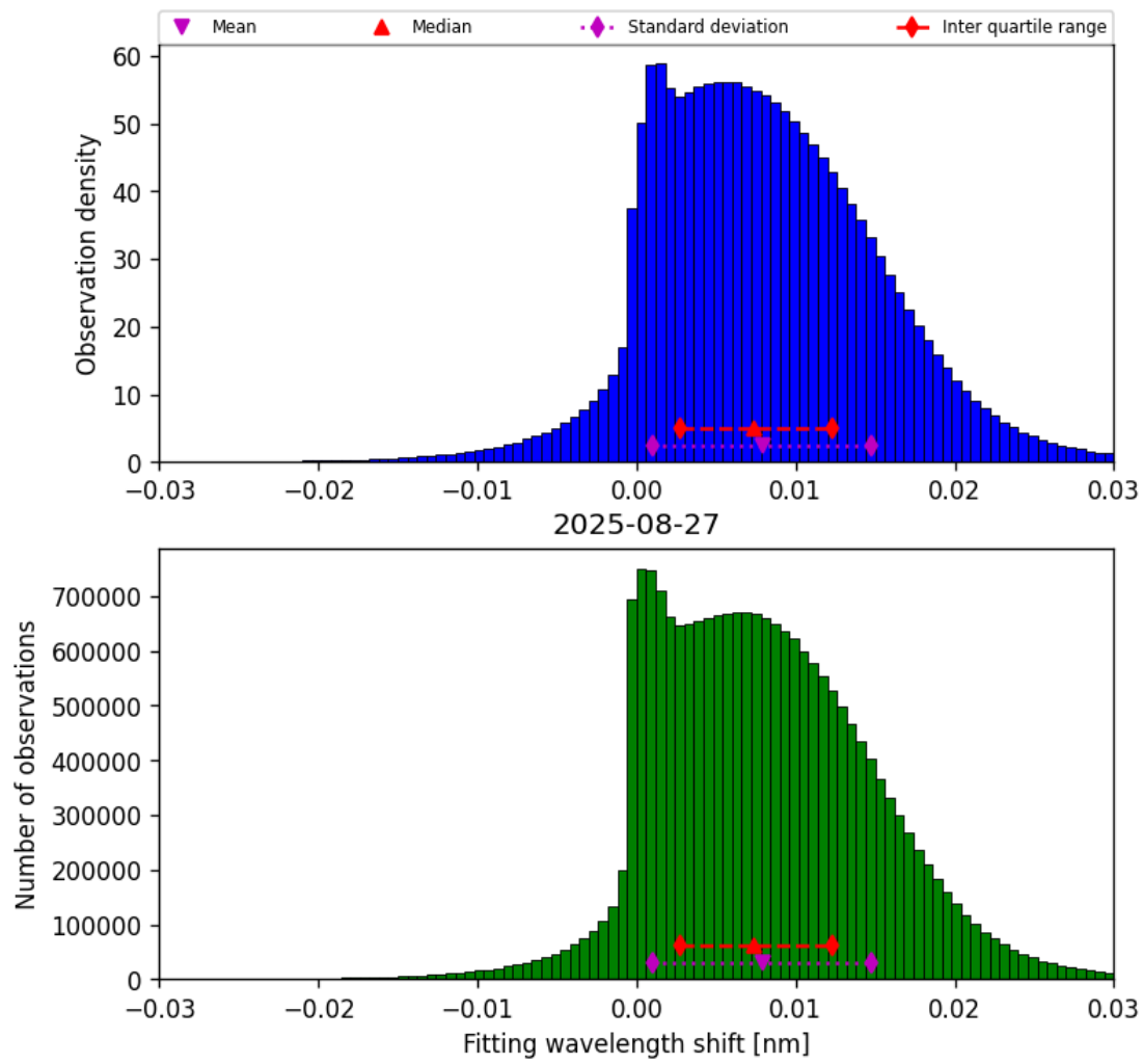
Figure 49: Histogram of “Fitting wavelength shift” for 2025-08-26 to 2025-08-28
