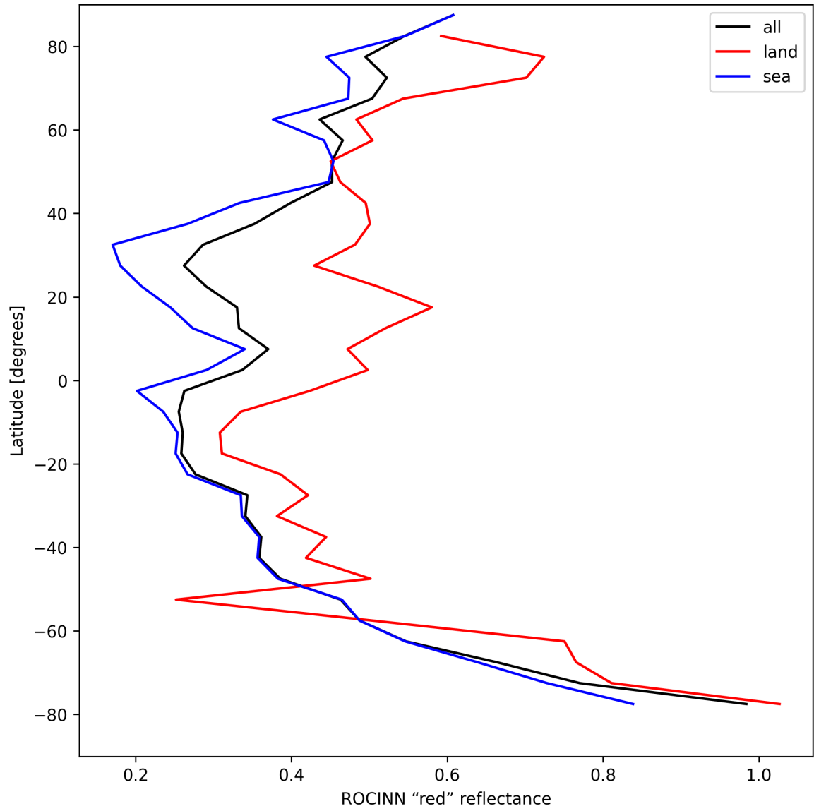
Figure 37: Zonal average of “ROCINN “red” reflectance” for 2025-08-26 to 2025-08-28.
