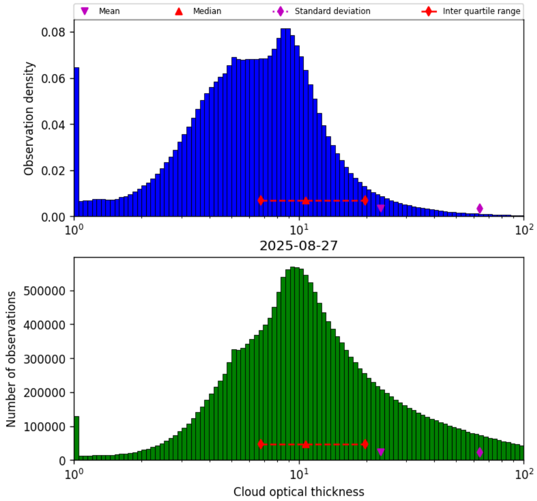
Figure 41: Histogram of “Cloud optical thickness” for 2025-08-26 to 2025-08-28
