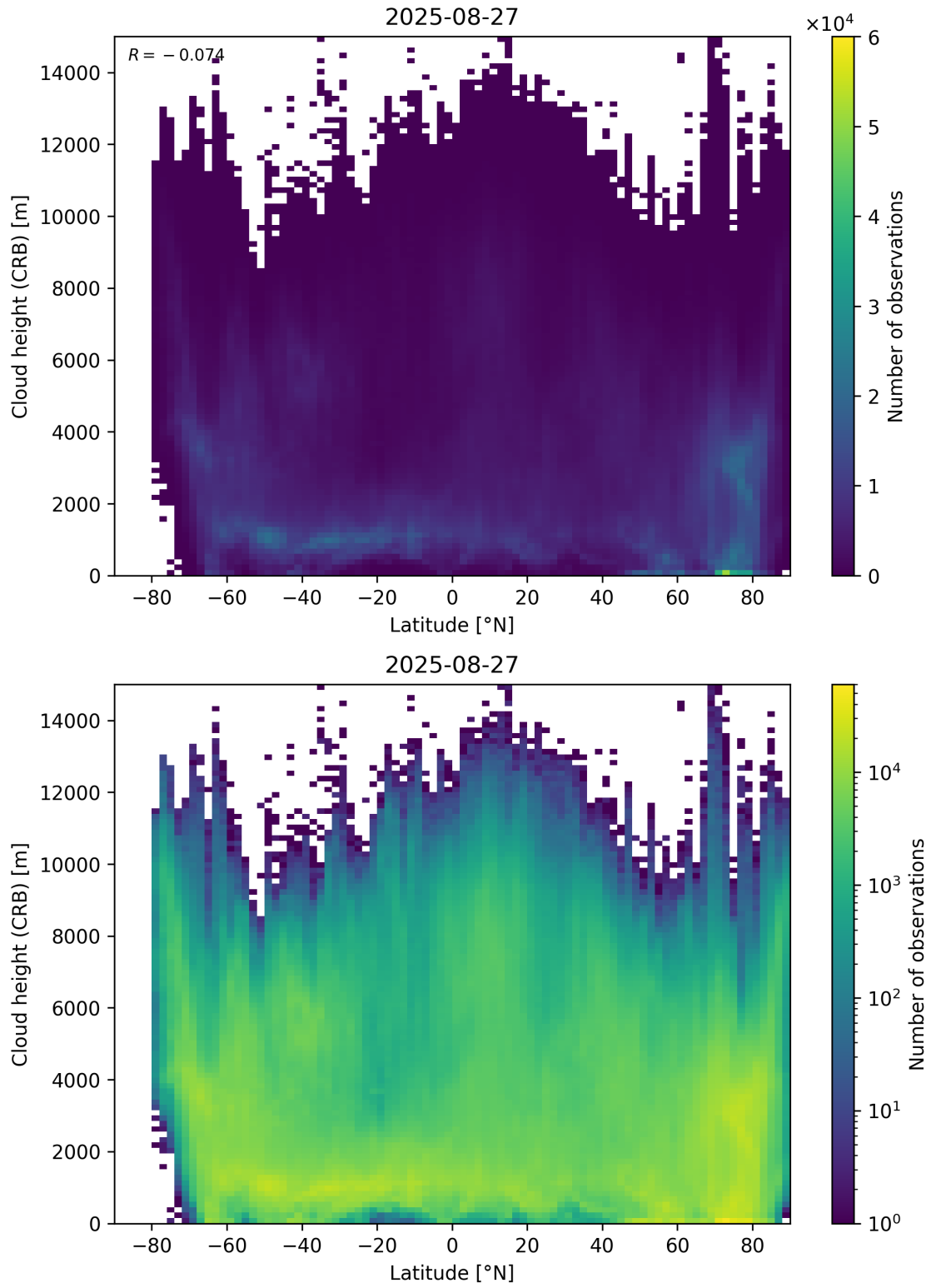
Figure 95: Scatter density plot of “Latitude” against “Cloud height (CRB)” for 2025-08-26 to 2025-08-28.
