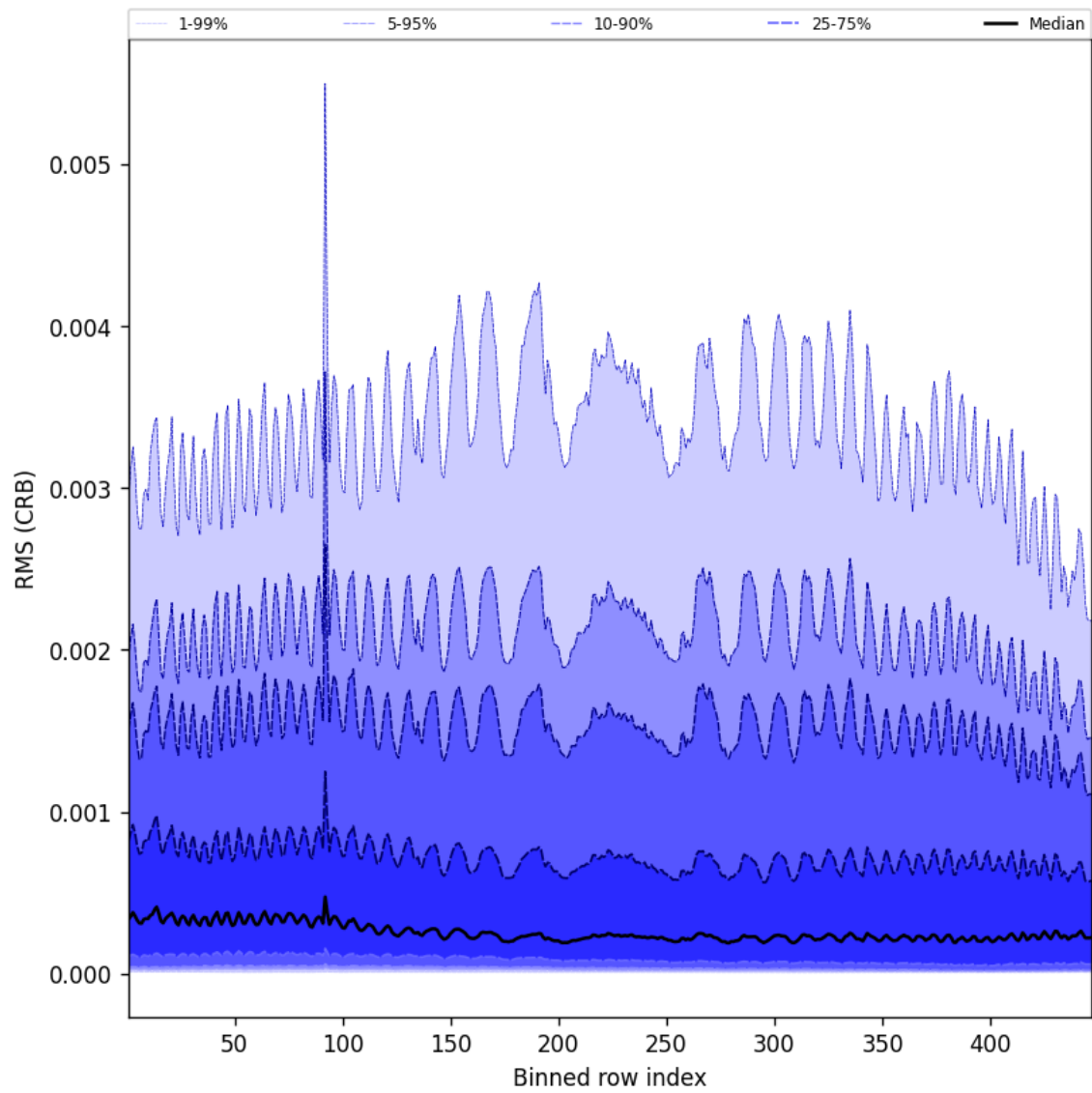
Figure 64: Along track statistics of “RMS (CRB)” for 2025-08-26 to 2025-08-28
