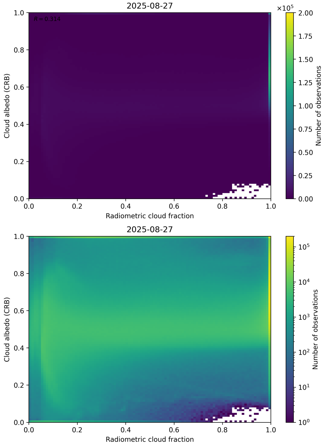
Figure 71: Scatter density plot of “Radiometric cloud fraction” against “Cloud albedo (CRB)” for 2025-08-26 to 2025-08-28.
