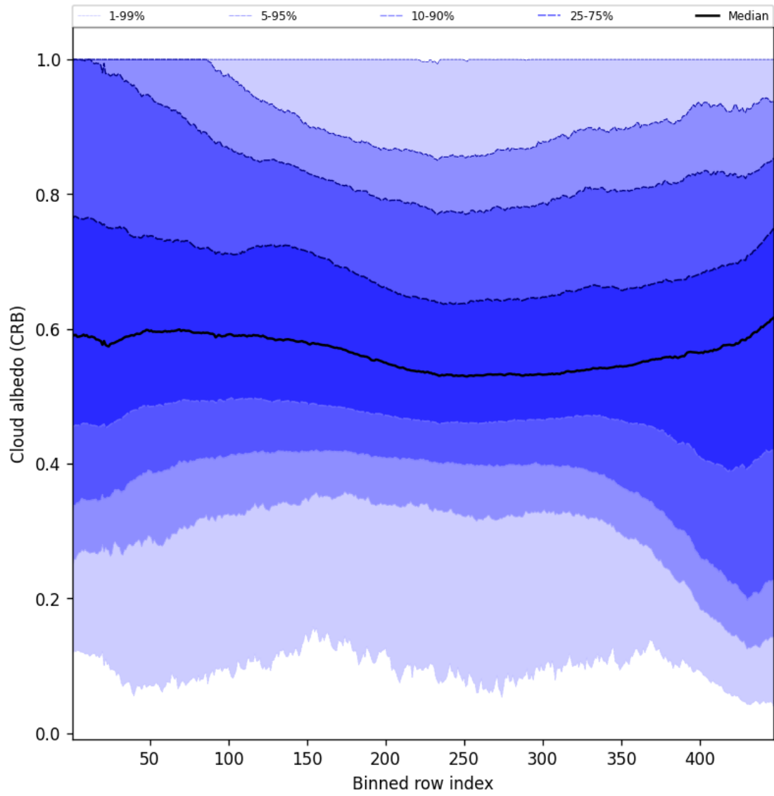
Figure 60: Along track statistics of “Cloud albedo (CRB)” for 2025-08-26 to 2025-08-28
