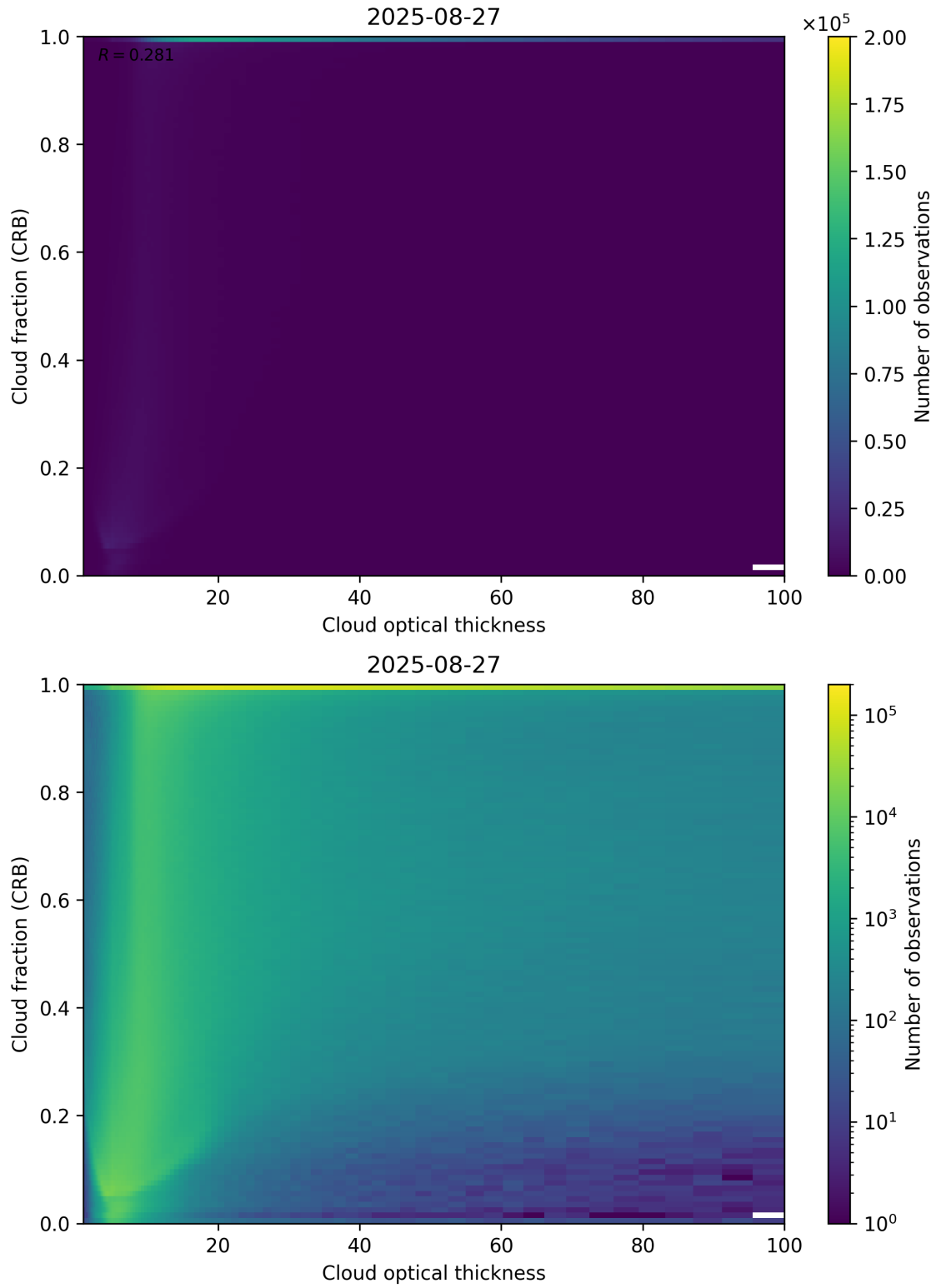
Figure 84: Scatter density plot of “Cloud optical thickness” against “Cloud fraction (CRB)” for 2025-08-26 to 2025-08-28.
