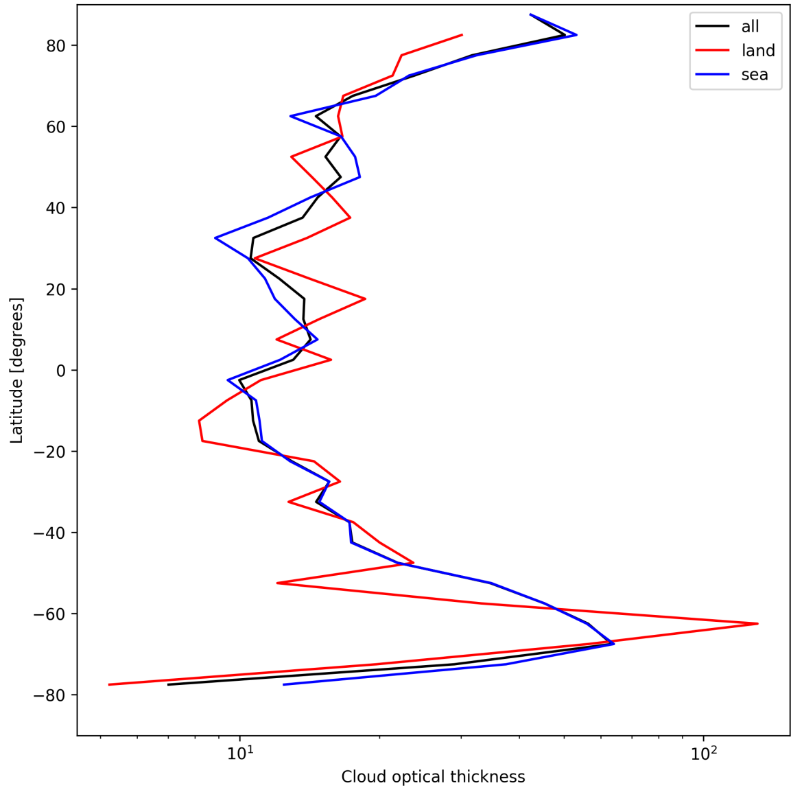
Figure 25: Zonal average of “Cloud optical thickness” for 2025-08-26 to 2025-08-28.
