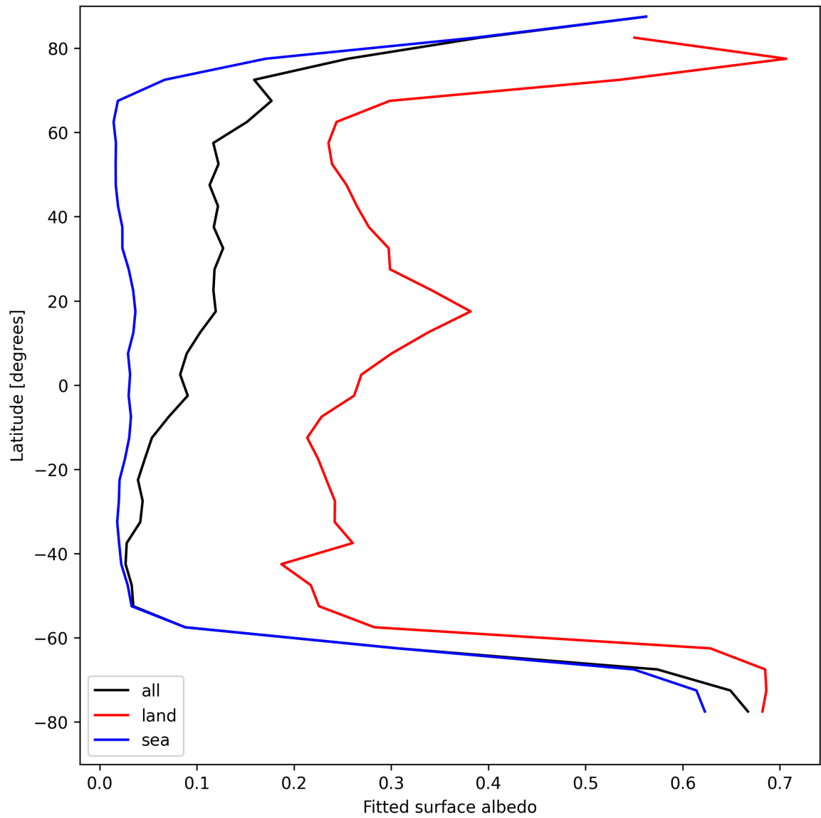
Figure 29: Zonal average of “Fitted surface albedo” for 2025-08-26 to 2025-08-28.
