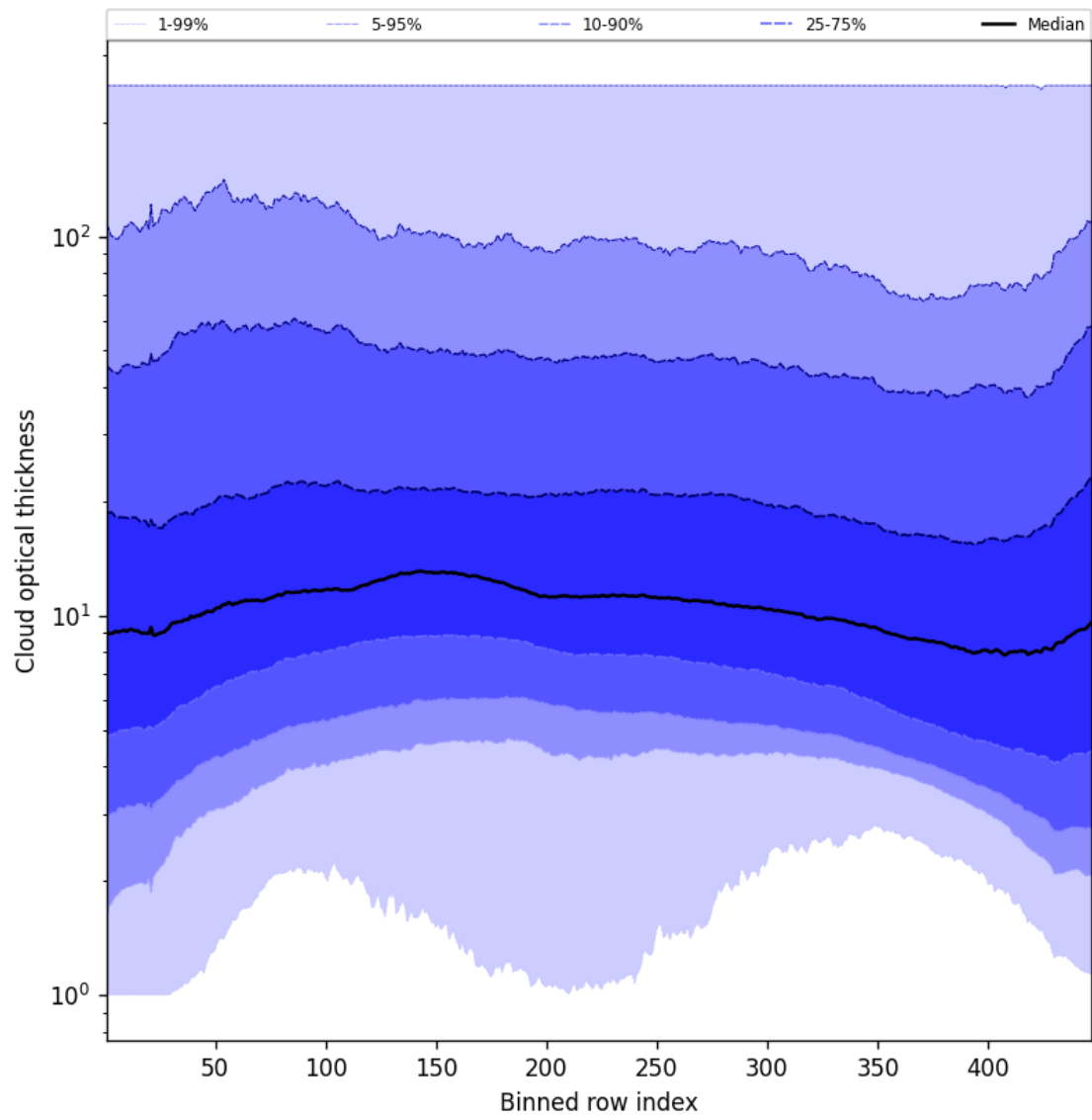
Figure 57: Along track statistics of “Cloud optical thickness” for 2025-08-30 to 2025-08-31
