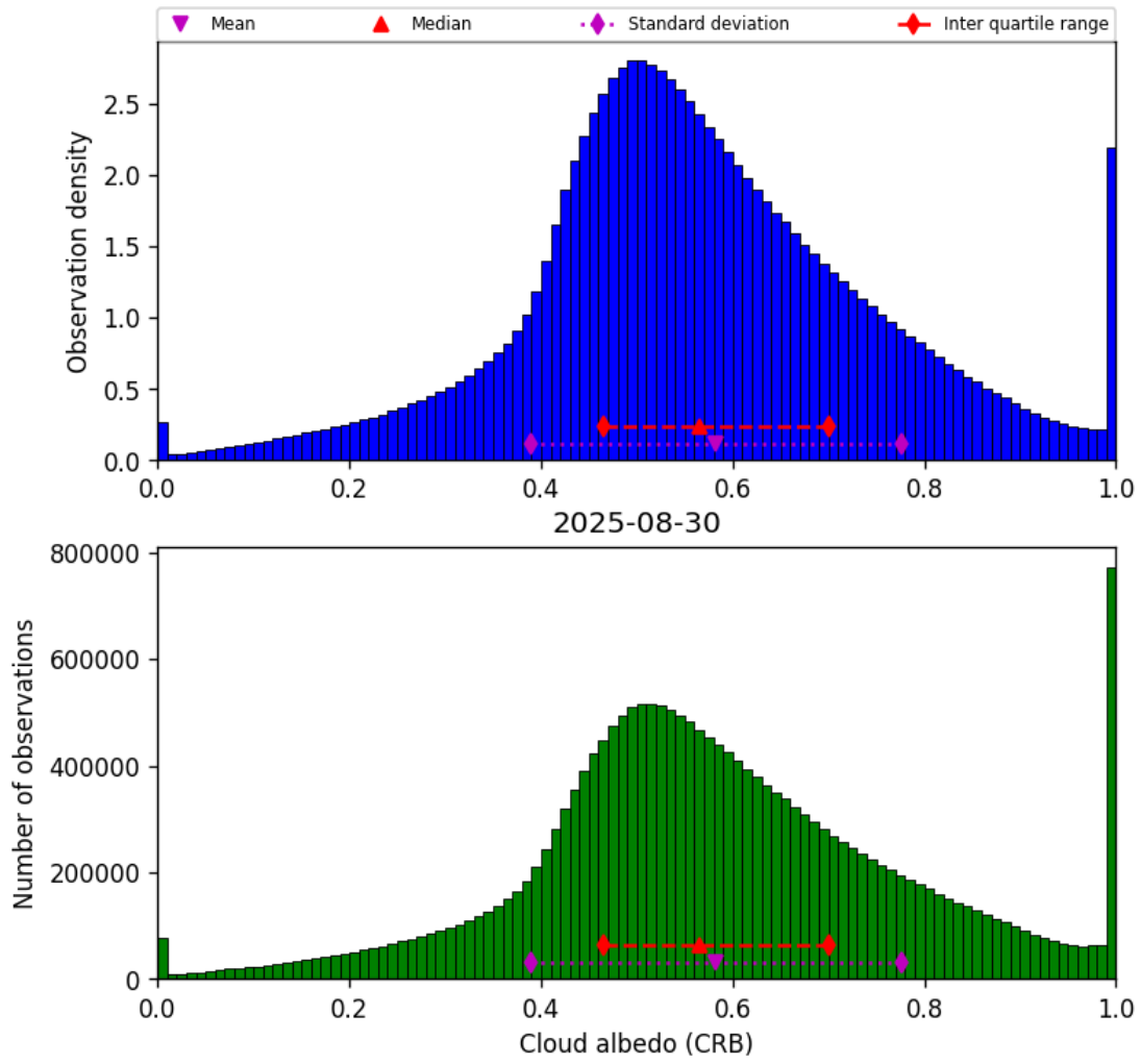
Figure 44: Histogram of “Cloud albedo (CRB)” for 2025-08-30 to 2025-08-31
