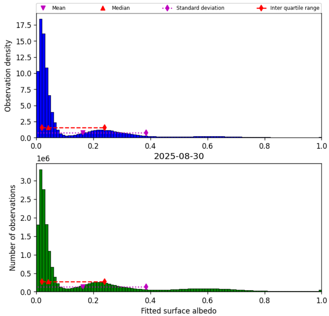
Figure 45: Histogram of “Fitted surface albedo” for 2025-08-30 to 2025-08-31
