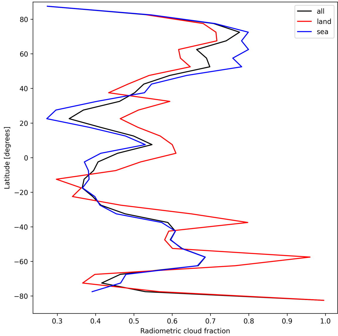
Figure 23: Zonal average of “Radiometric cloud fraction” for 2025-08-30 to 2025-08-31.
