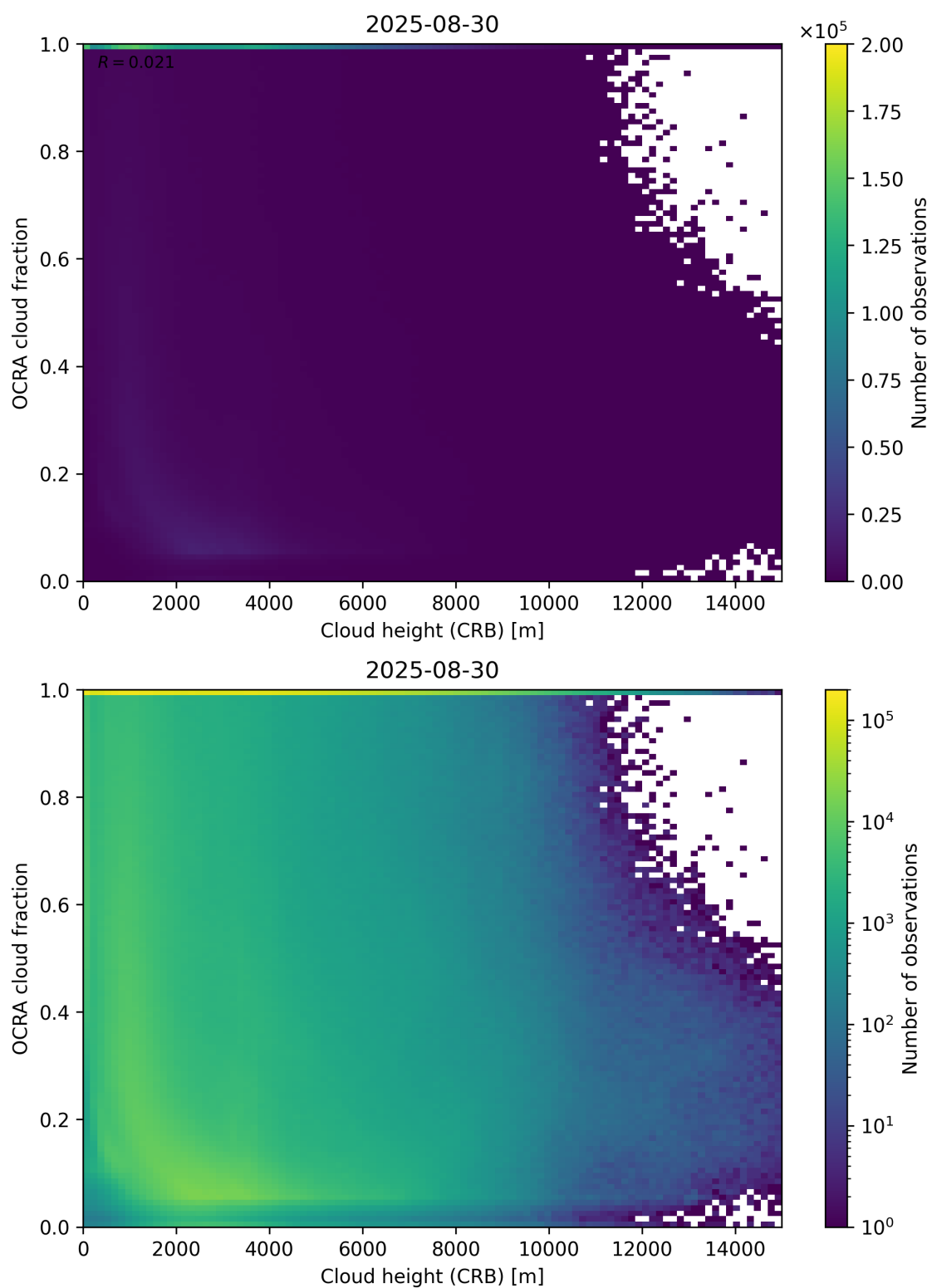
Figure 81: Scatter density plot of “Cloud height (CRB)” against “OCRA cloud fraction” for 2025-08-30 to 2025-08-31.
