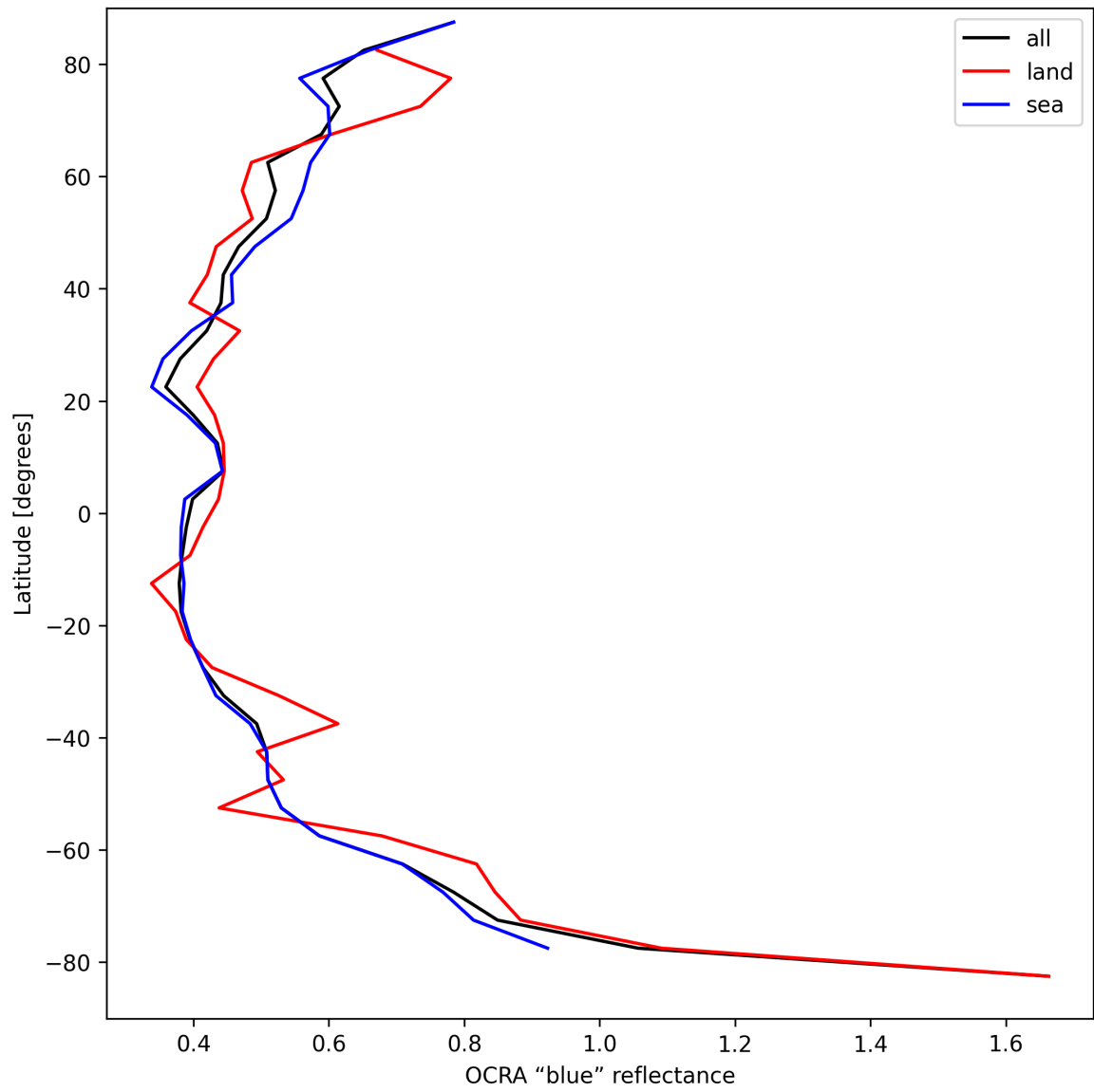
Figure 35: Zonal average of “OCRA “blue” reflectance” for 2025-08-30 to 2025-08-31.
