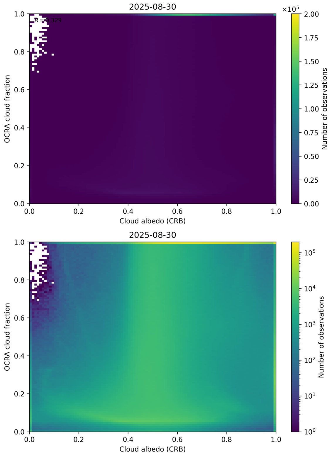
Figure 70: Scatter density plot of “Cloud albedo (CRB)” against “OCRA cloud fraction” for 2025-08-30 to 2025-08-31.
