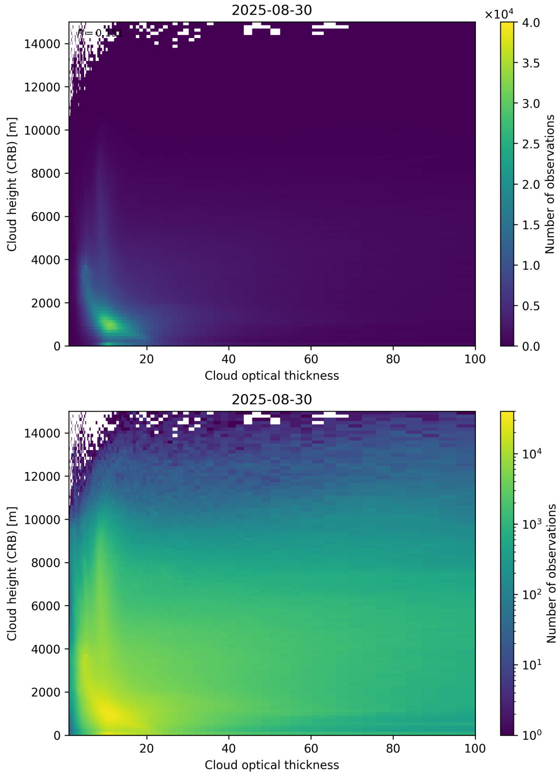
Figure 85: Scatter density plot of “Cloud optical thickness” against “Cloud height (CRB)” for 2025-08-30 to 2025-08-31.
