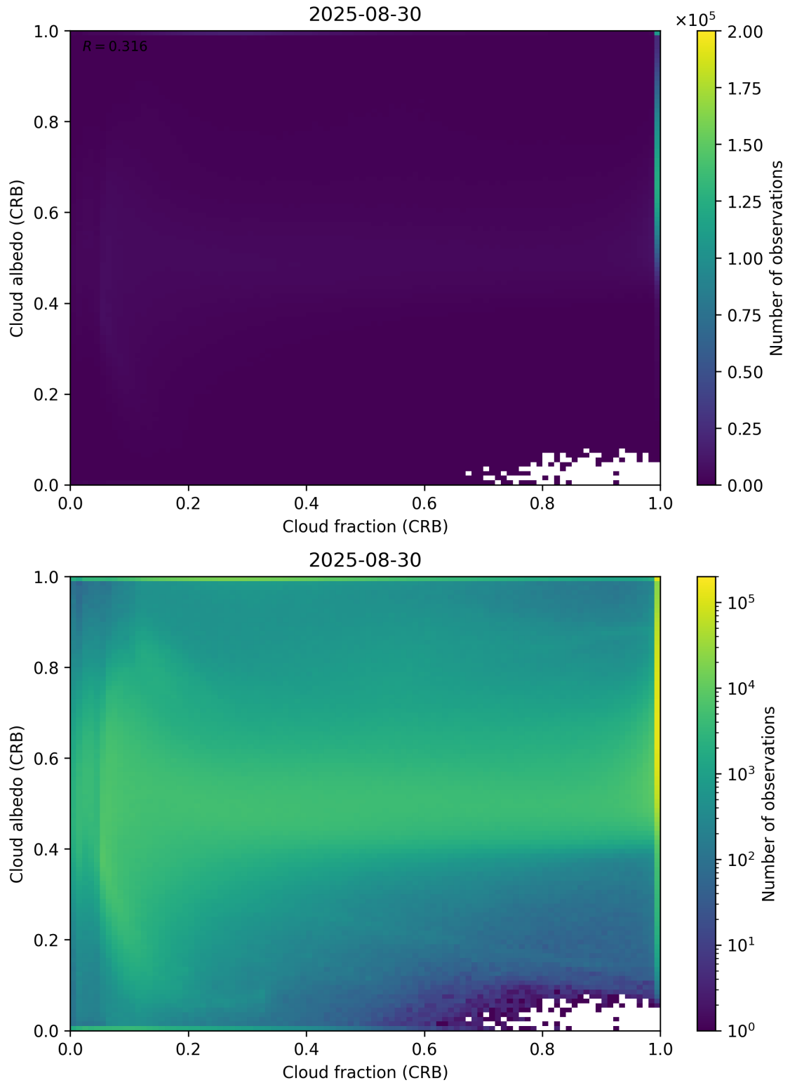
Figure 77: Scatter density plot of “Cloud fraction (CRB)” against “Cloud albedo (CRB)” for 2025-08-30 to 2025-08-31.
