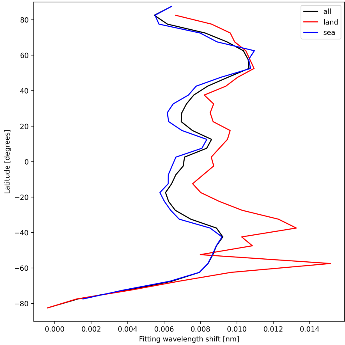
Figure 33: Zonal average of “Fitting wavelength shift” for 2025-08-30 to 2025-08-31.
