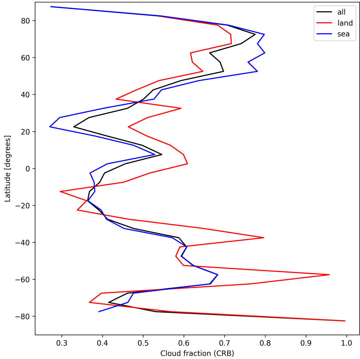
Figure 26: Zonal average of “Cloud fraction (CRB)” for 2025-08-30 to 2025-08-31.
