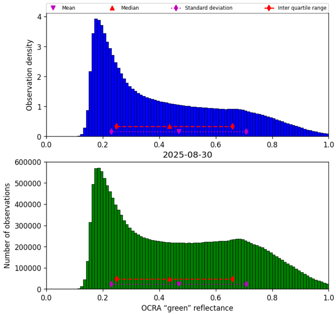
Figure 52: Histogram of “OCRA “green” reflectance” for 2025-08-30 to 2025-08-31
