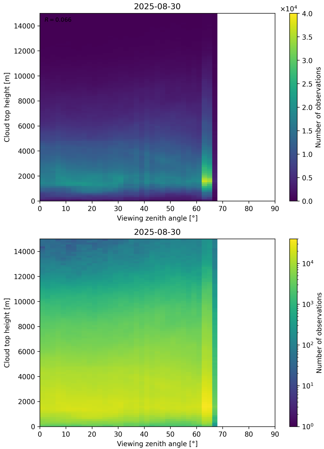
Figure 112: Scatter density plot of “Viewing zenith angle” against “Cloud top height” for 2025-08-30 to 2025-08-31.
