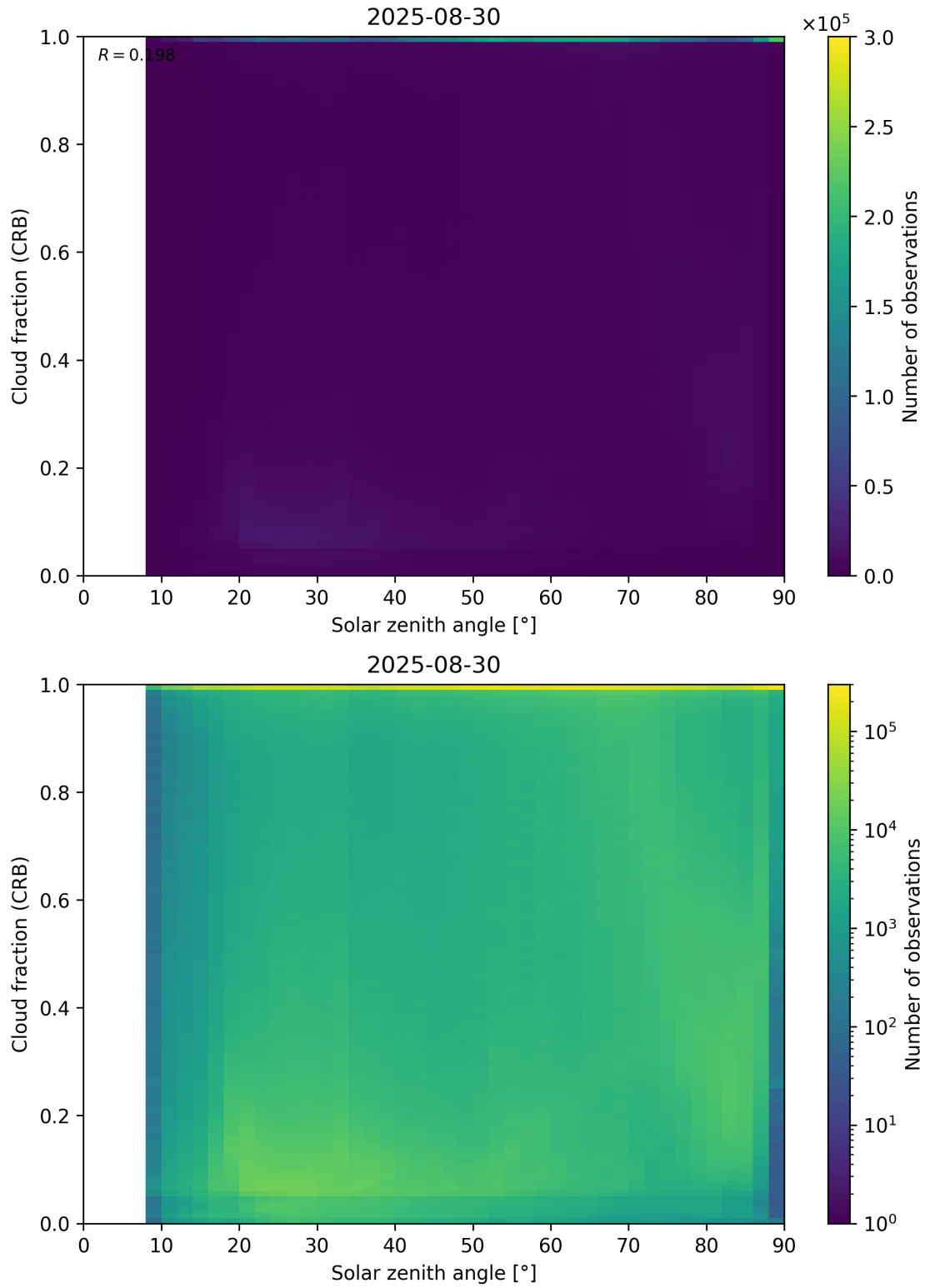
Figure 101: Scatter density plot of “Solar zenith angle” against “Cloud fraction (CRB)” for 2025-08-30 to 2025-08-31.
