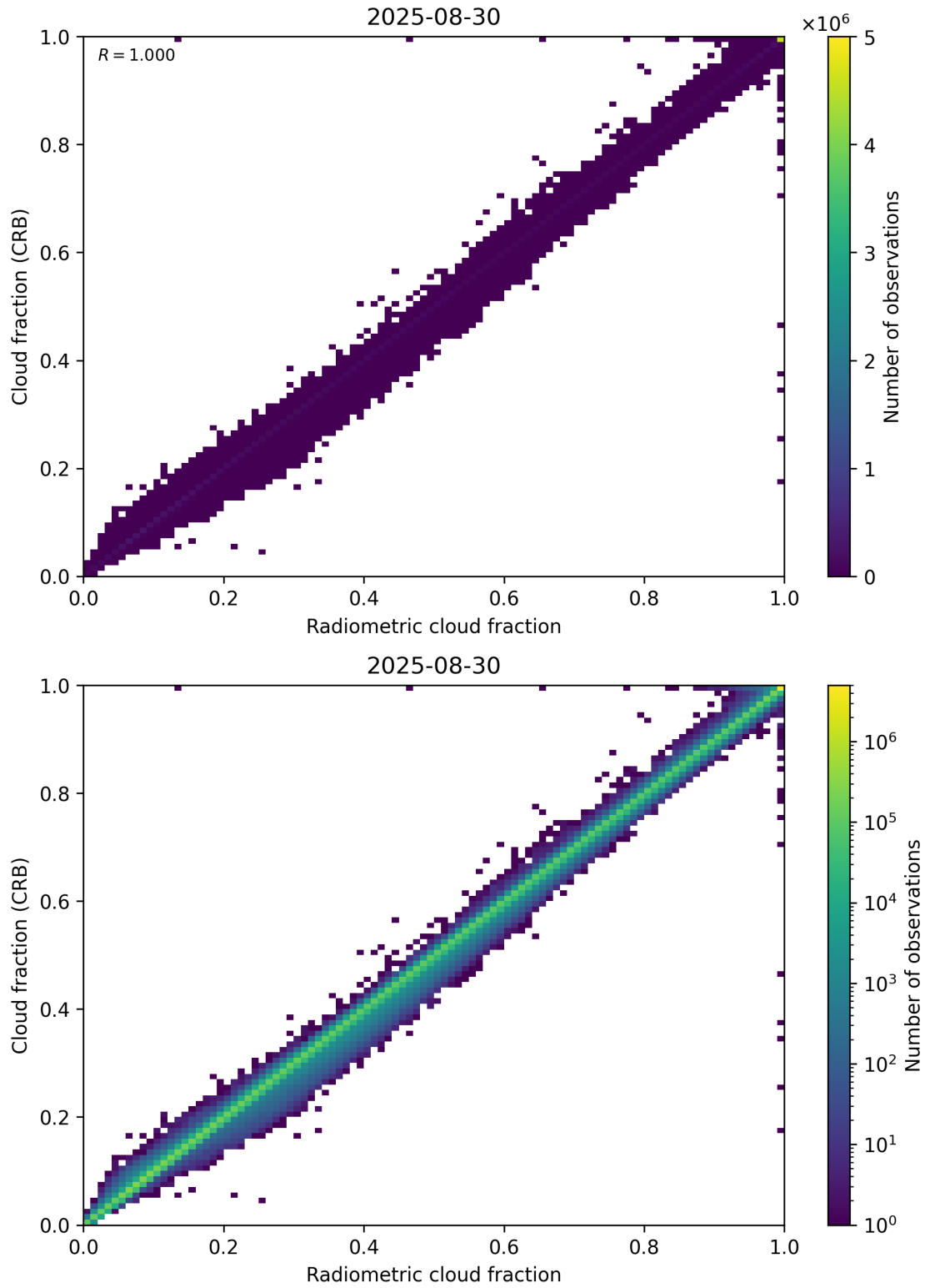
Figure 73: Scatter density plot of “Radiometric cloud fraction” against “Cloud fraction (CRB)” for 2025-08-30 to 2025-08-31.
