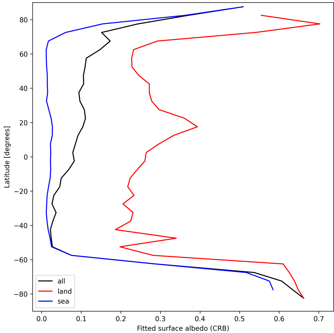
Figure 30: Zonal average of “Fitted surface albedo (CRB)” for 2025-08-30 to 2025-08-31.
