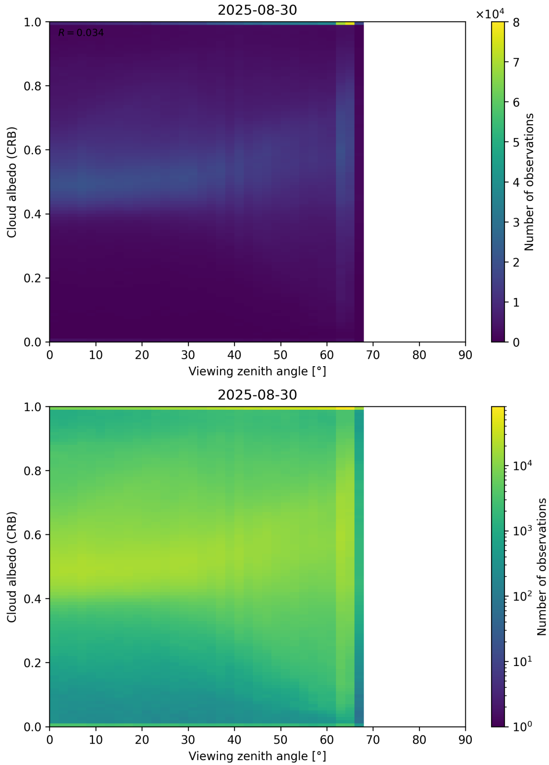
Figure 106: Scatter density plot of “Viewing zenith angle” against “Cloud albedo (CRB)” for 2025-08-30 to 2025-08-31.
