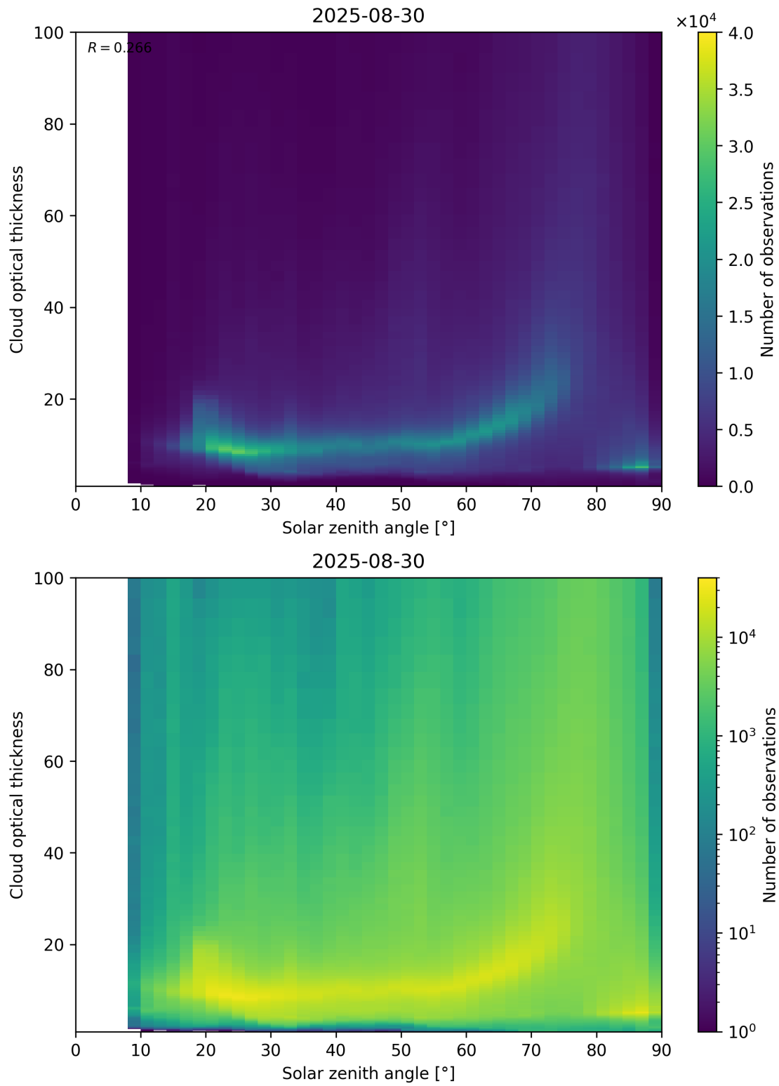
Figure 103: Scatter density plot of “Solar zenith angle” against “Cloud optical thickness” for 2025-08-30 to 2025-08-31.
