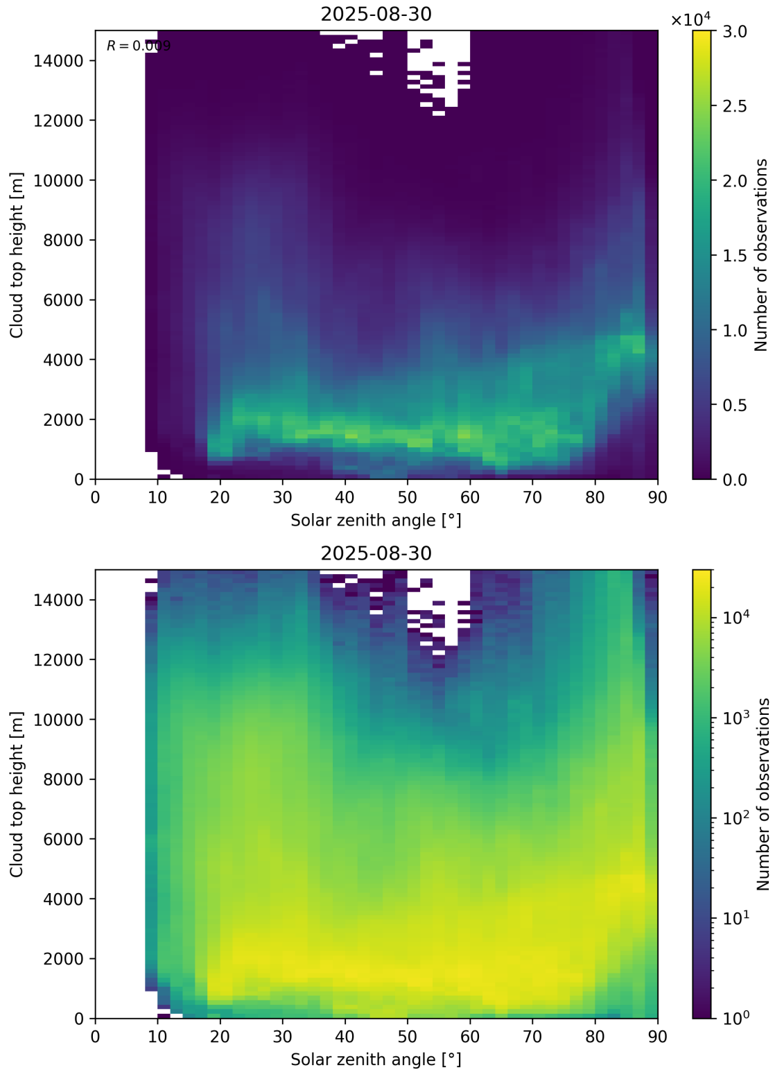
Figure 104: Scatter density plot of “Solar zenith angle” against “Cloud top height” for 2025-08-30 to 2025-08-31.
