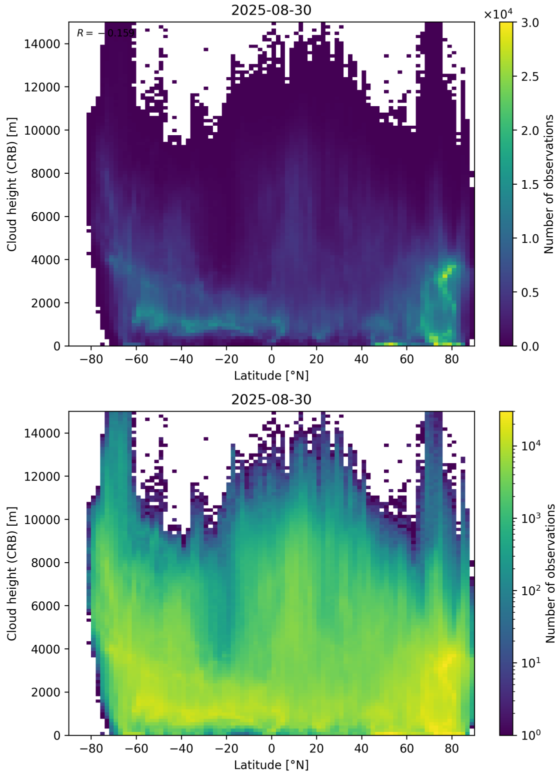
Figure 95: Scatter density plot of “Latitude” against “Cloud height (CRB)” for 2025-08-30 to 2025-08-31.
