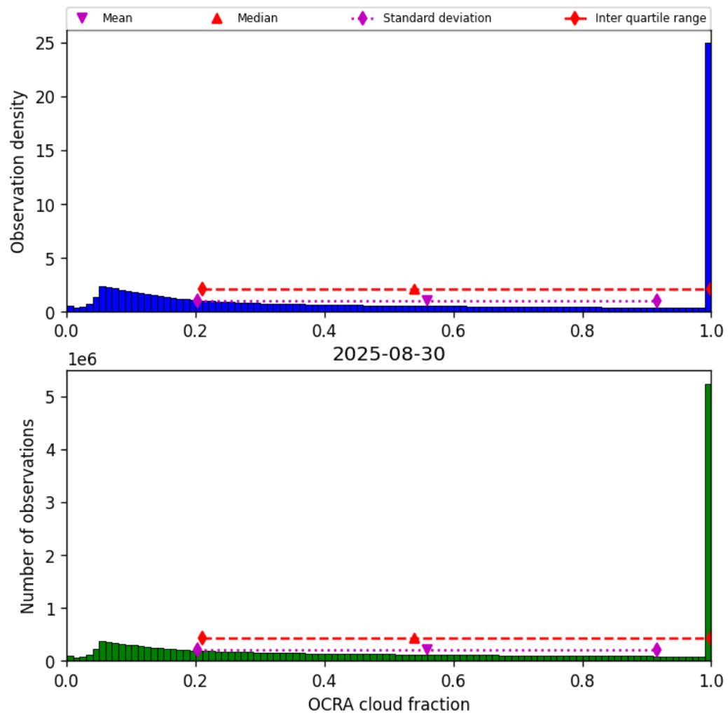
Figure 50: Histogram of “OCRA cloud fraction” for 2025-08-30 to 2025-08-31
