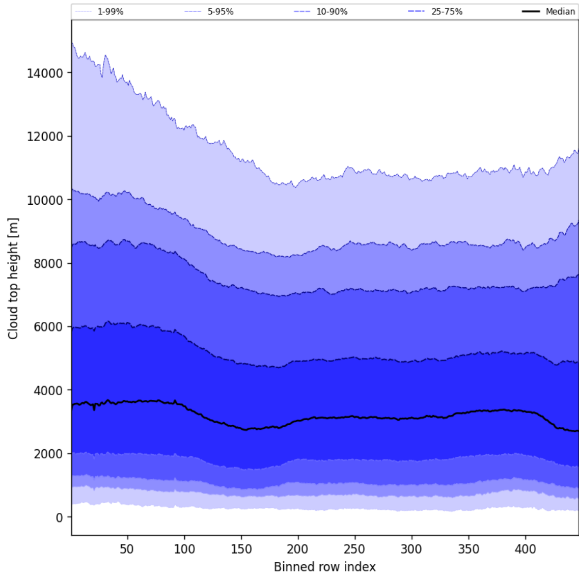
Figure 56: Along track statistics of “Cloud top height” for 2025-08-30 to 2025-08-31
