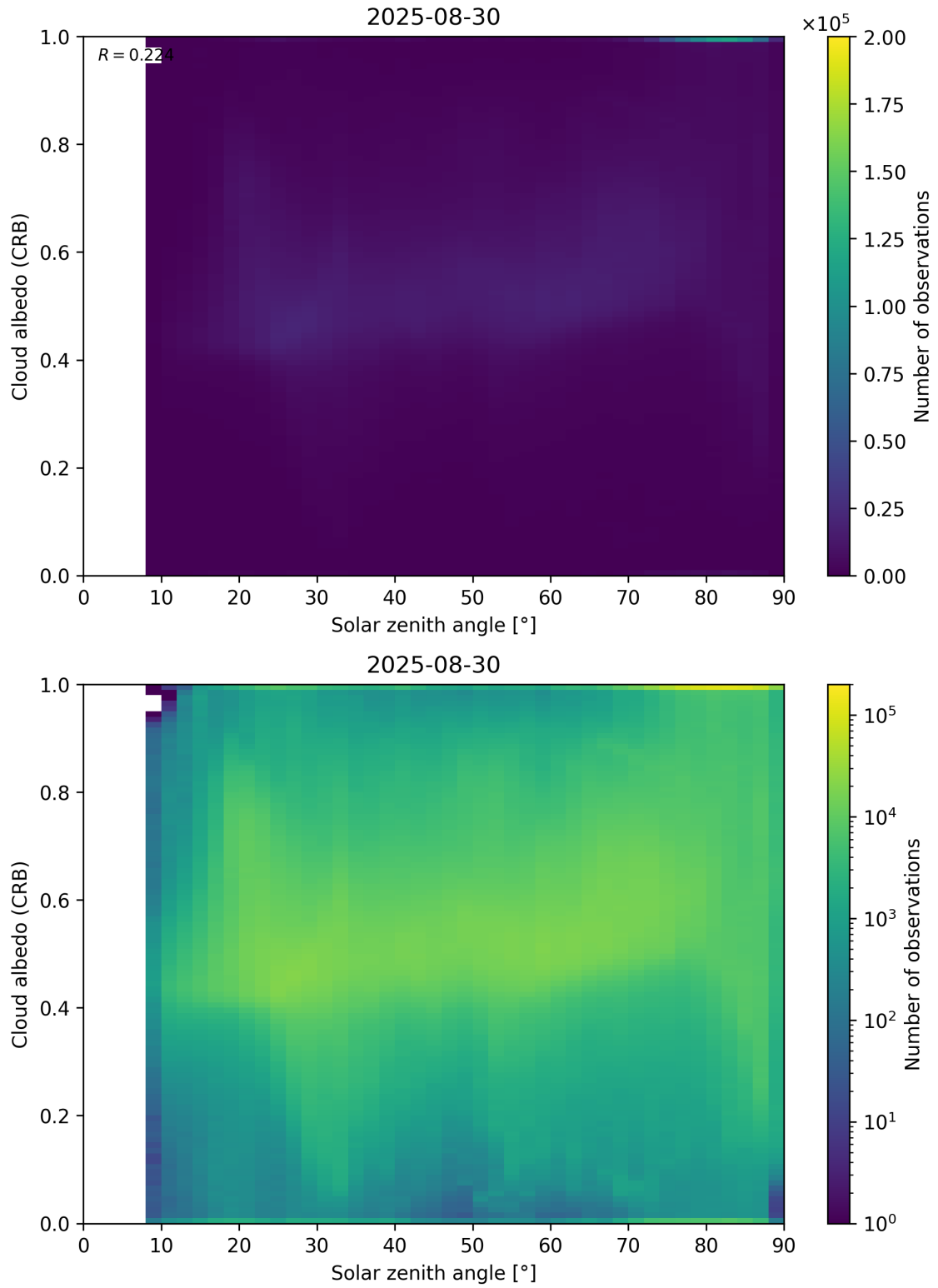
Figure 98: Scatter density plot of “Solar zenith angle” against “Cloud albedo (CRB)” for 2025-08-30 to 2025-08-31.
