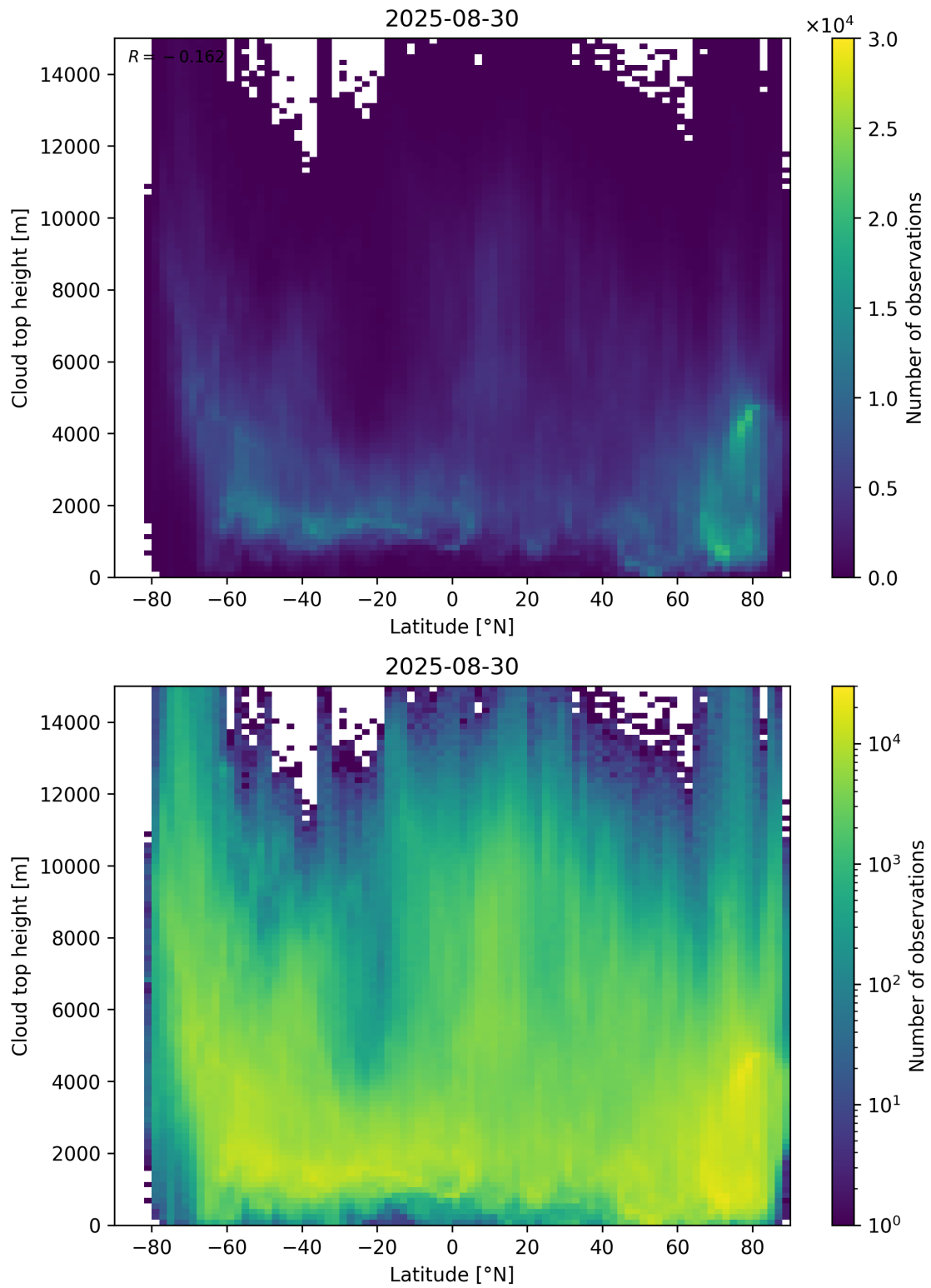
Figure 97: Scatter density plot of “Latitude” against “Cloud top height” for 2025-08-30 to 2025-08-31.
