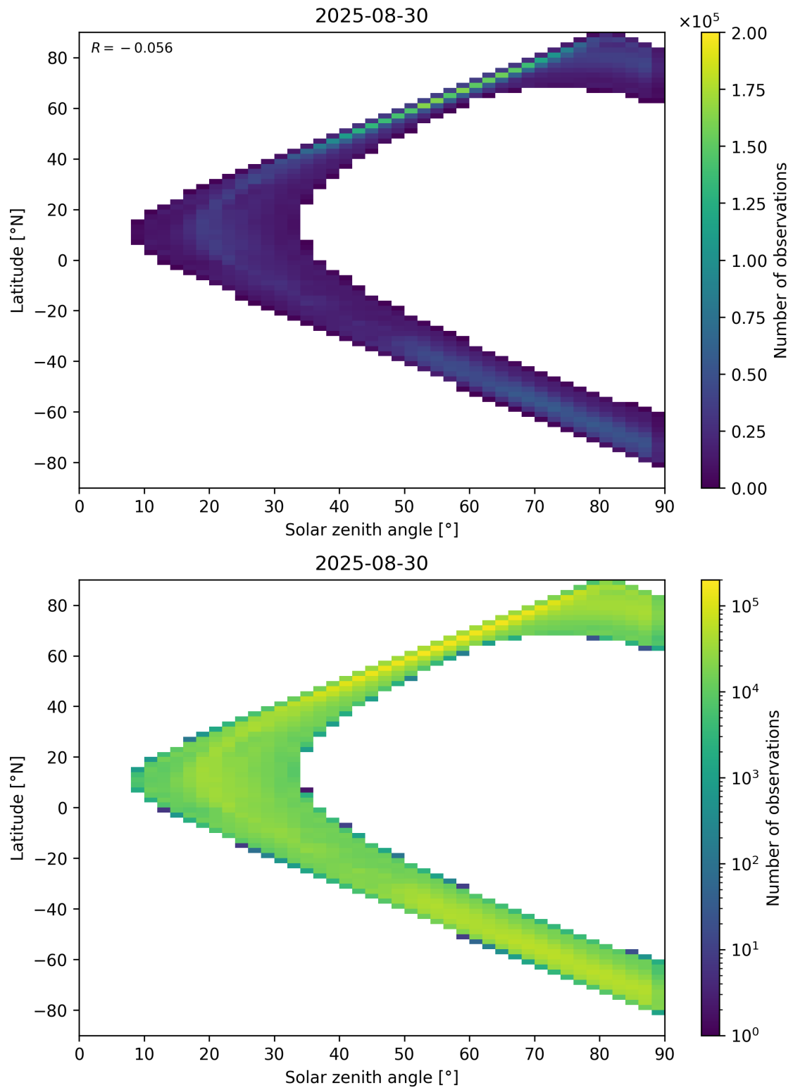
Figure 105: Scatter density plot of “Solar zenith angle” against “Latitude” for 2025-08-30 to 2025-08-31.
