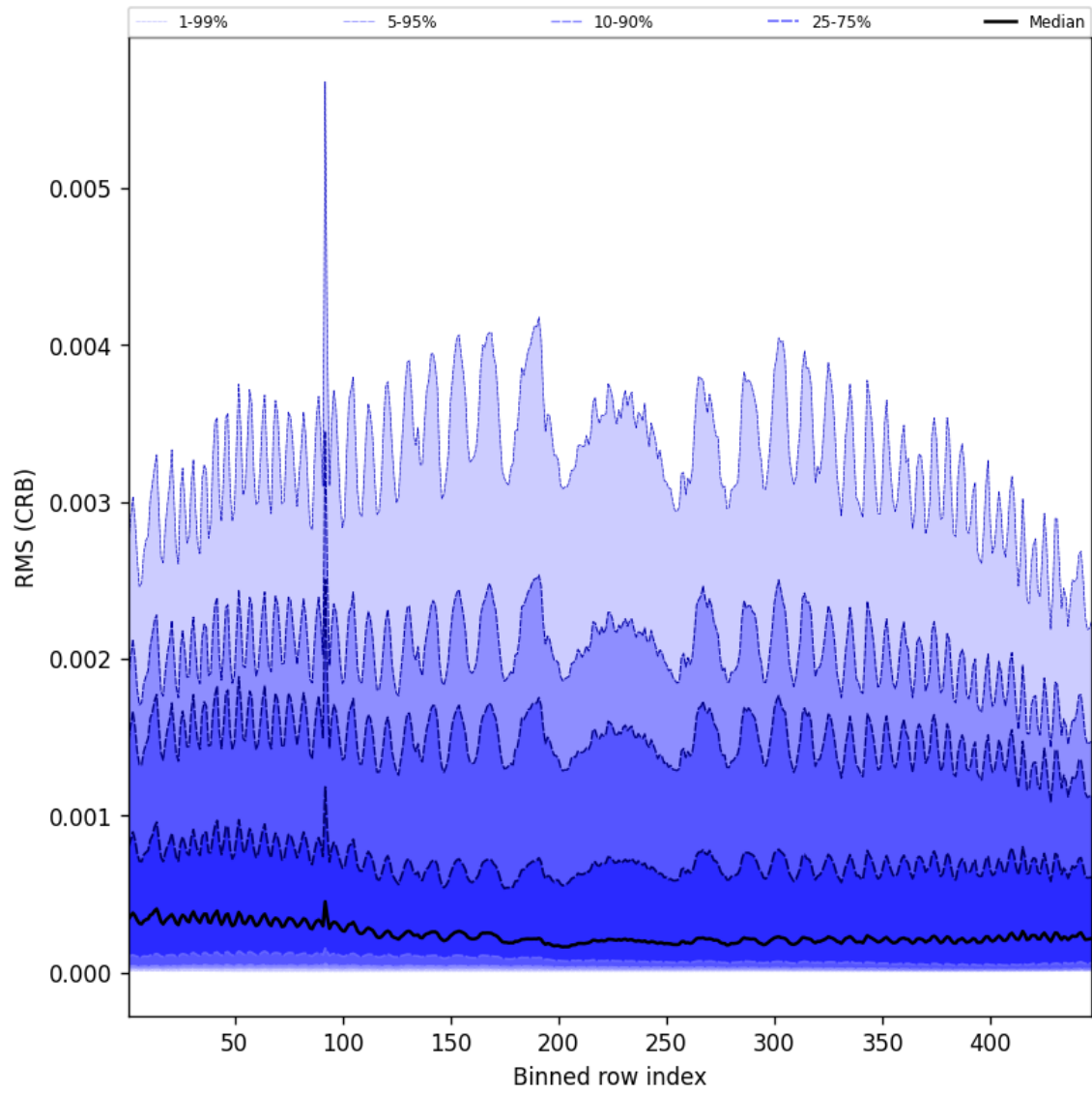
Figure 64: Along track statistics of “RMS (CRB)” for 2025-08-30 to 2025-08-31
