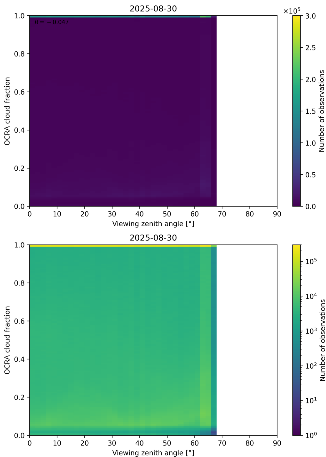
Figure 108: Scatter density plot of “Viewing zenith angle” against “OCRA cloud fraction” for 2025-08-30 to 2025-08-31.
