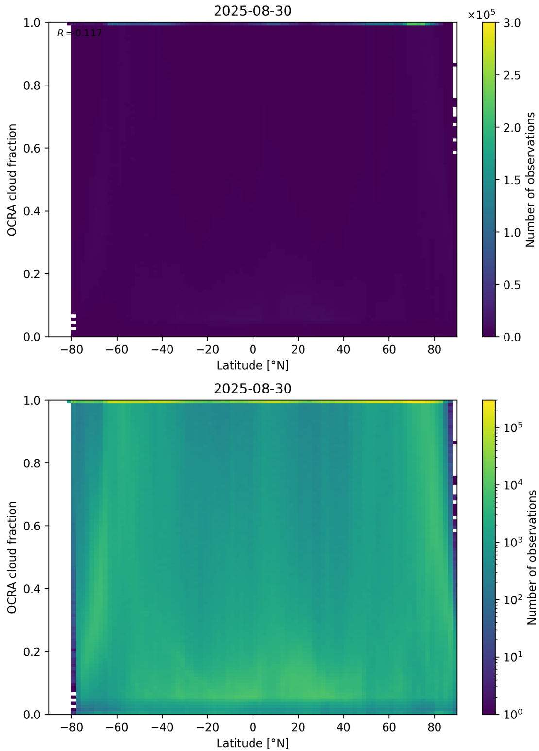
Figure 93: Scatter density plot of “Latitude” against “OCRA cloud fraction” for 2025-08-30 to 2025-08-31.
