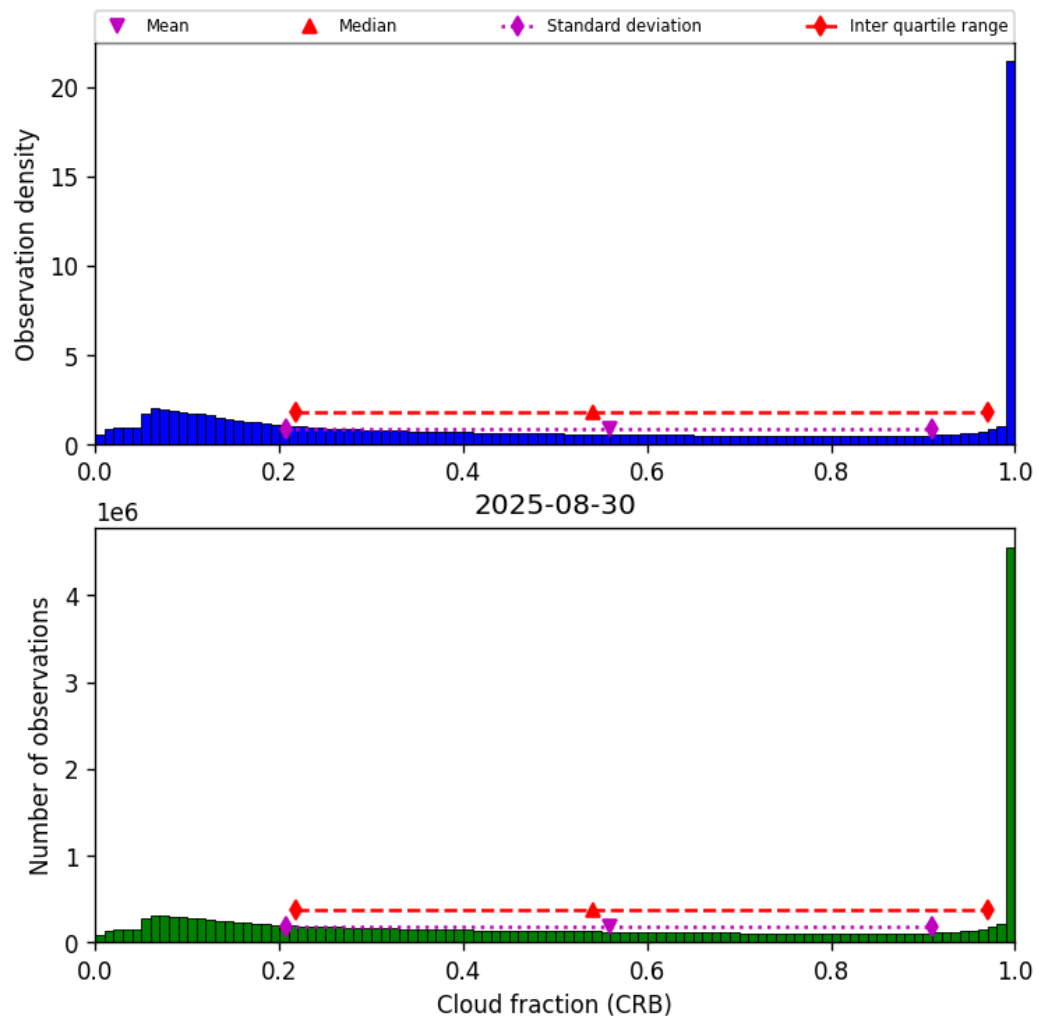
Figure 42: Histogram of “Cloud fraction (CRB)” for 2025-08-30 to 2025-08-31
