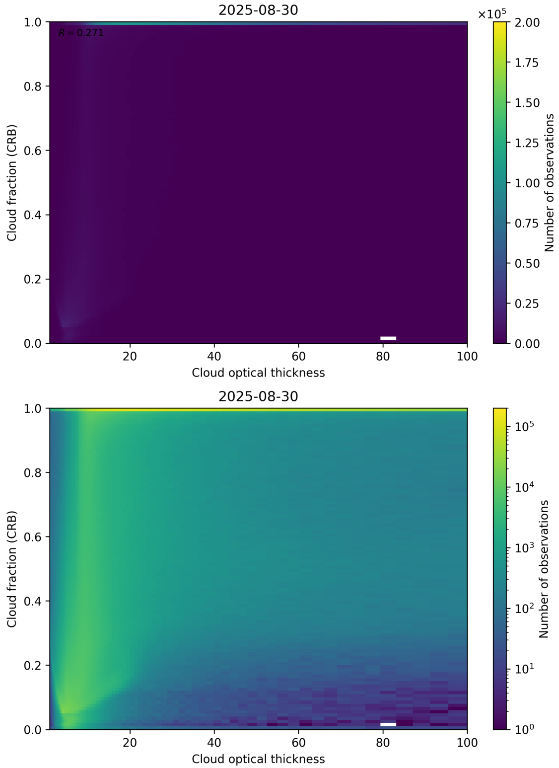
Figure 84: Scatter density plot of “Cloud optical thickness” against “Cloud fraction (CRB)” for 2025-08-30 to 2025-08-31.
