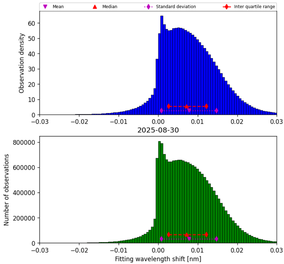
Figure 49: Histogram of “Fitting wavelength shift” for 2025-08-30 to 2025-08-31
