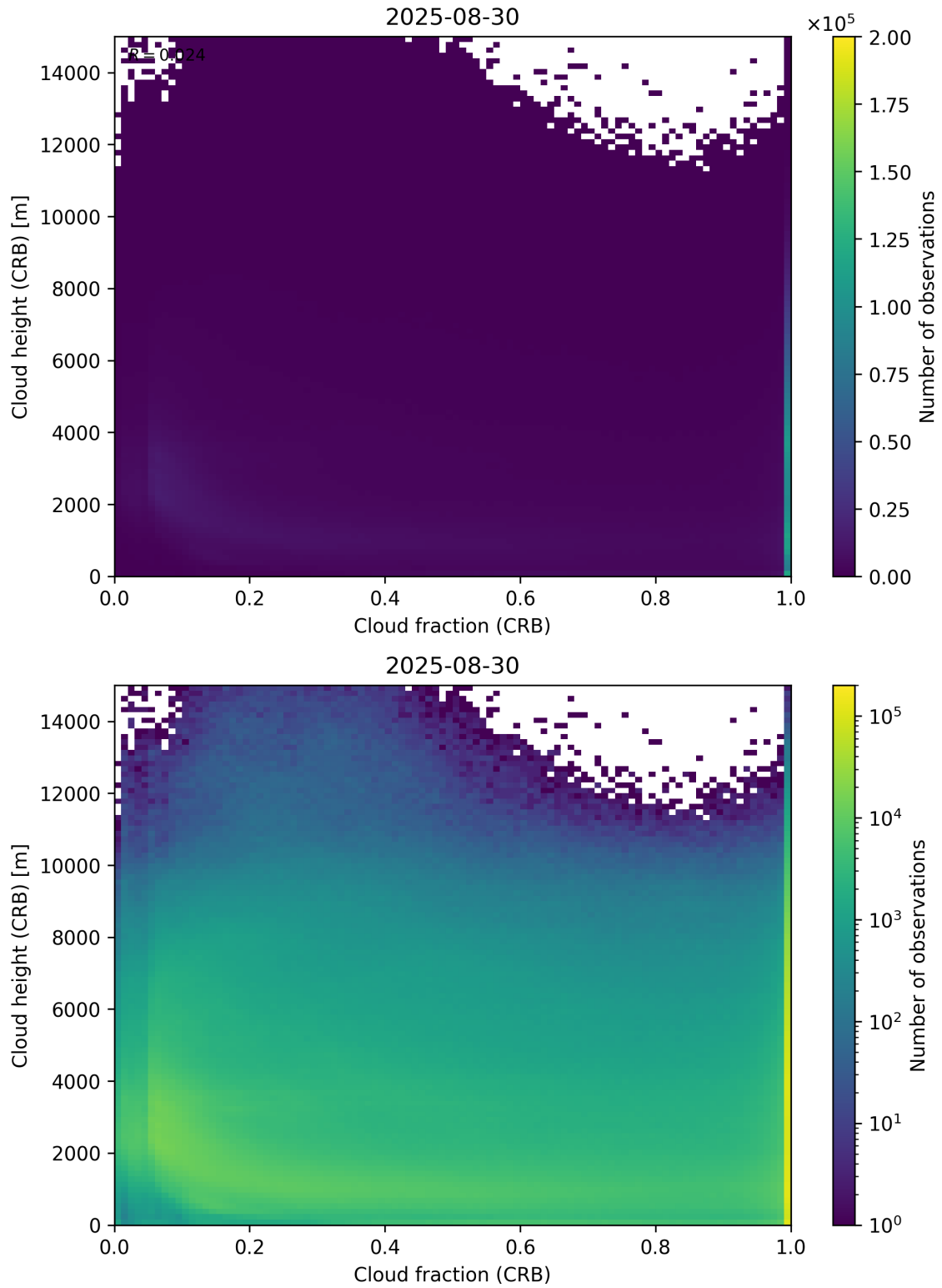
Figure 79: Scatter density plot of “Cloud fraction (CRB)” against “Cloud height (CRB)” for 2025-08-30 to 2025-08-31.
