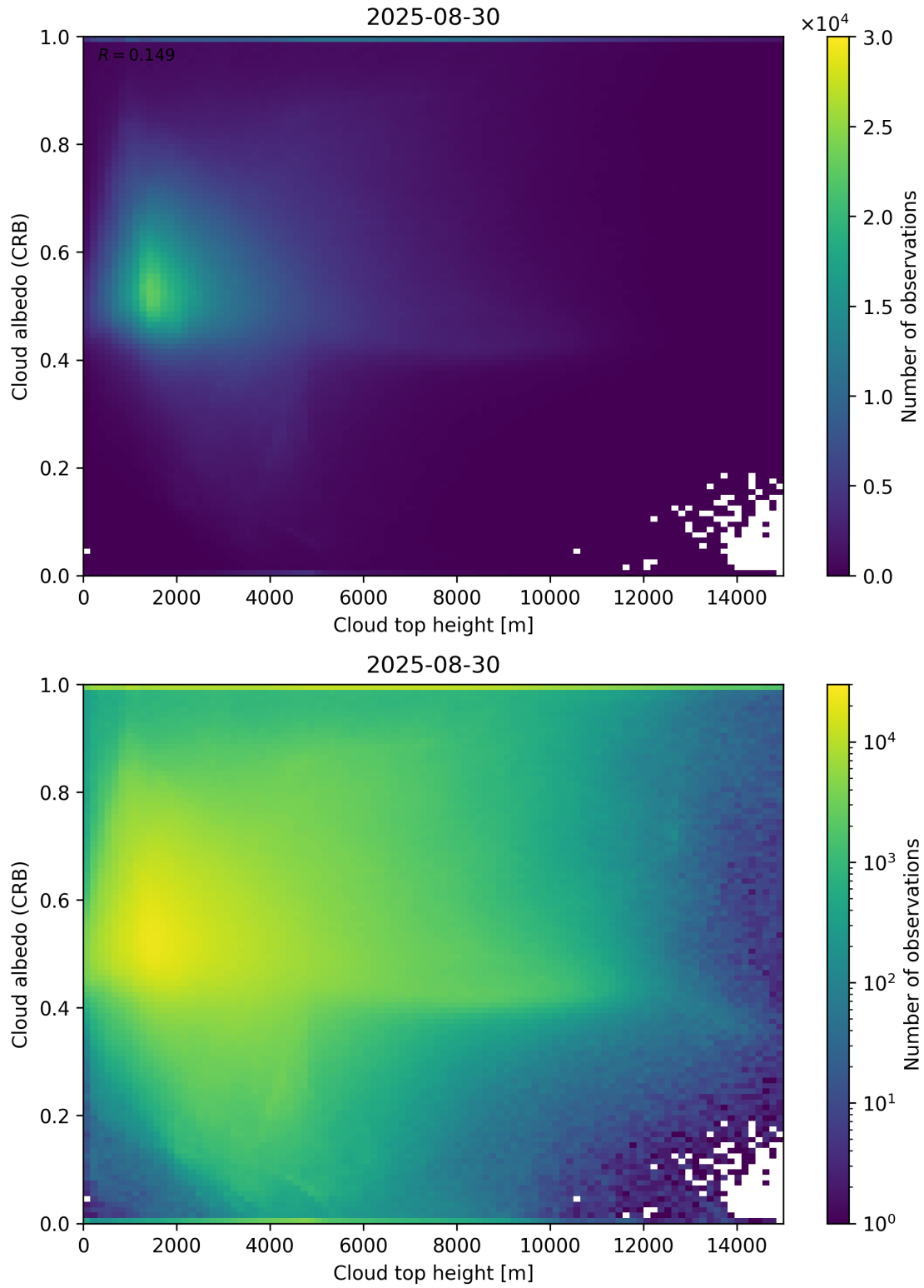
Figure 86: Scatter density plot of “Cloud top height” against “Cloud albedo (CRB)” for 2025-08-30 to 2025-08-31.
