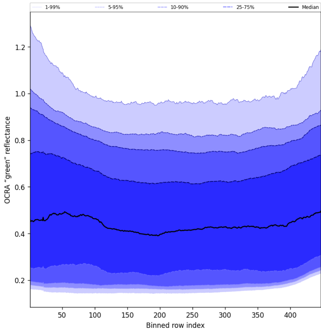
Figure 68: Along track statistics of “OCRA “green” reflectance” for 2025-08-30 to 2025-08-31
