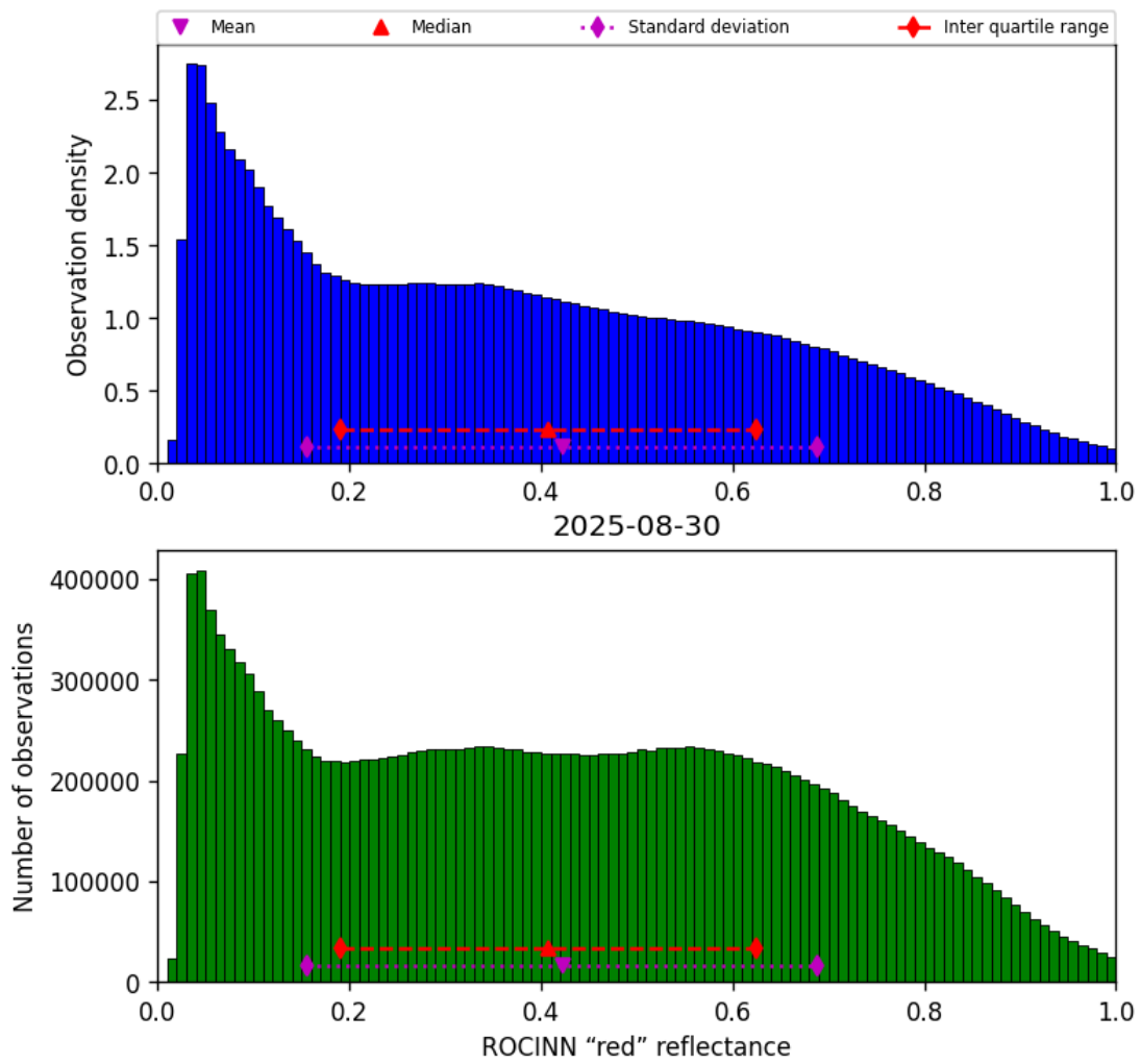
Figure 53: Histogram of “ROCINN “red” reflectance” for 2025-08-30 to 2025-08-31
