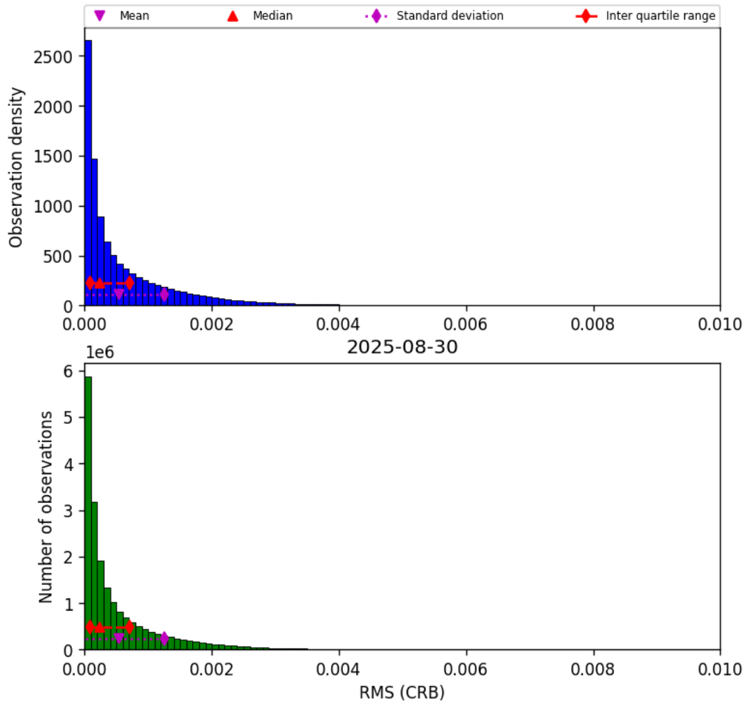
Figure 48: Histogram of “RMS (CRB)” for 2025-08-30 to 2025-08-31
