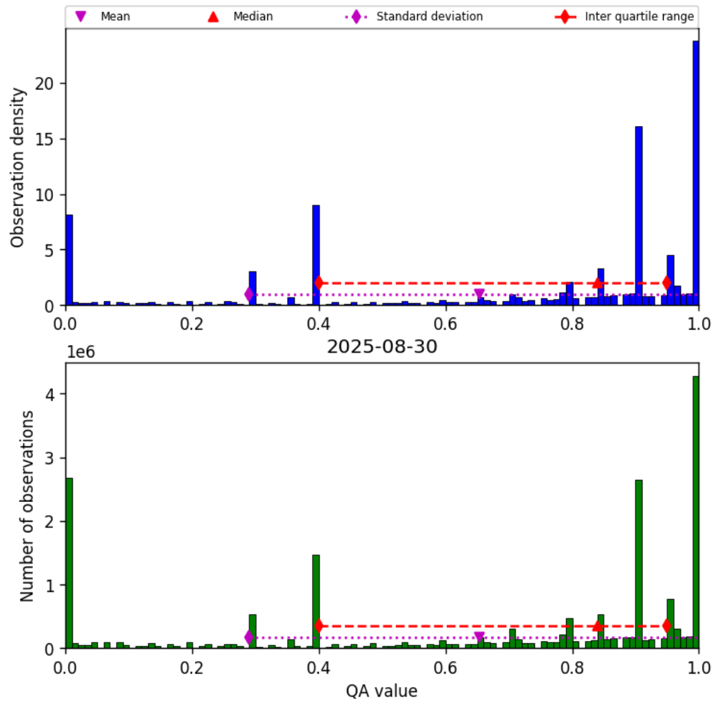
Figure 38: Histogram of “QA value” for 2025-08-30 to 2025-08-31
