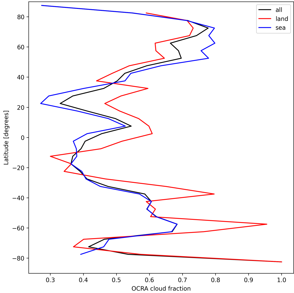
Figure 34: Zonal average of “OCRA cloud fraction” for 2025-08-30 to 2025-08-31.
