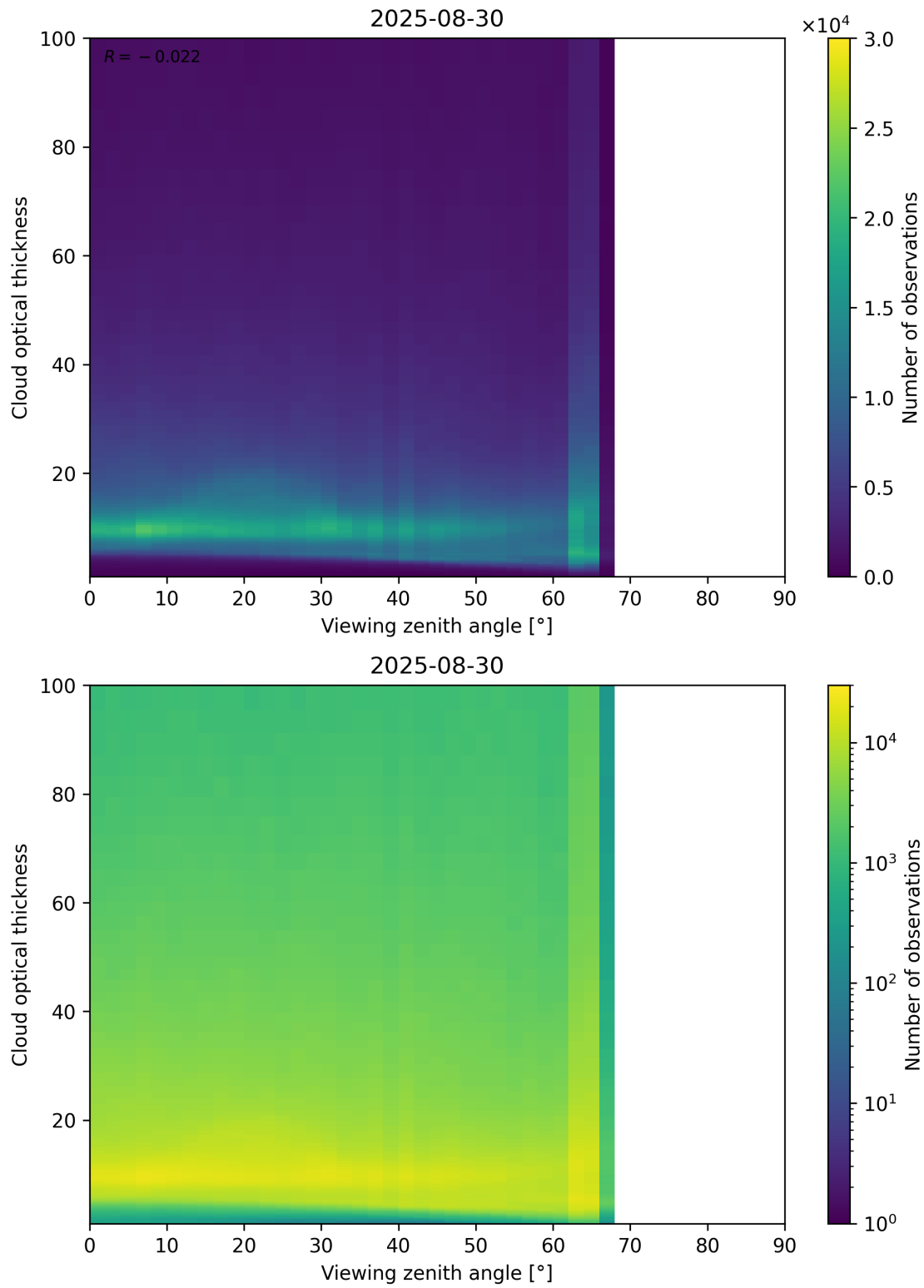
Figure 111: Scatter density plot of “Viewing zenith angle” against “Cloud optical thickness” for 2025-08-30 to 2025-08-31.
