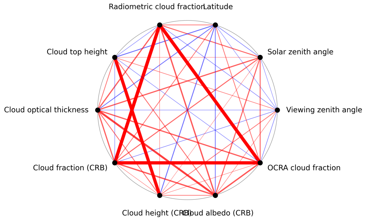
Figure 1: Map of correlation graph for 2025-08-30 to 2025-08-31.
