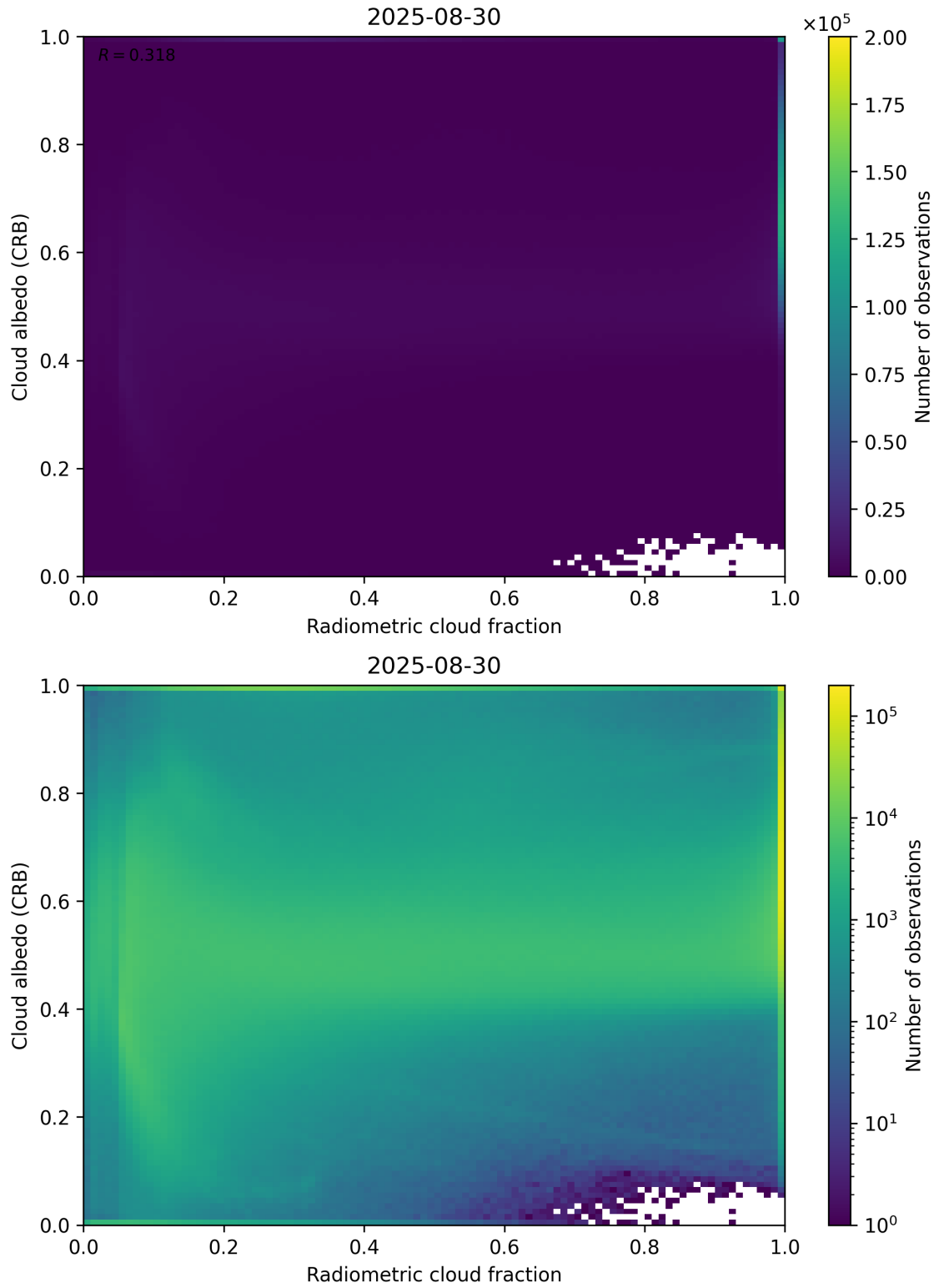
Figure 71: Scatter density plot of “Radiometric cloud fraction” against “Cloud albedo (CRB)” for 2025-08-30 to 2025-08-31.
