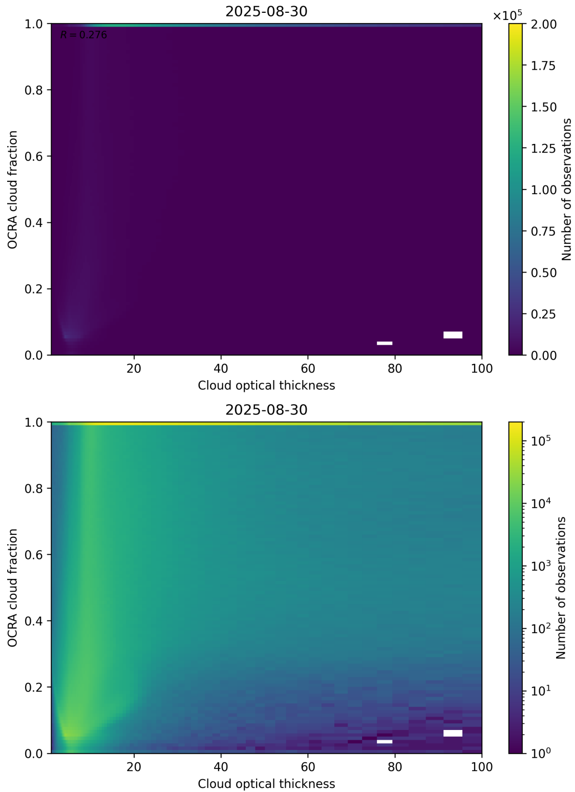
Figure 83: Scatter density plot of “Cloud optical thickness” against “OCRA cloud fraction” for 2025-08-30 to 2025-08-31.
