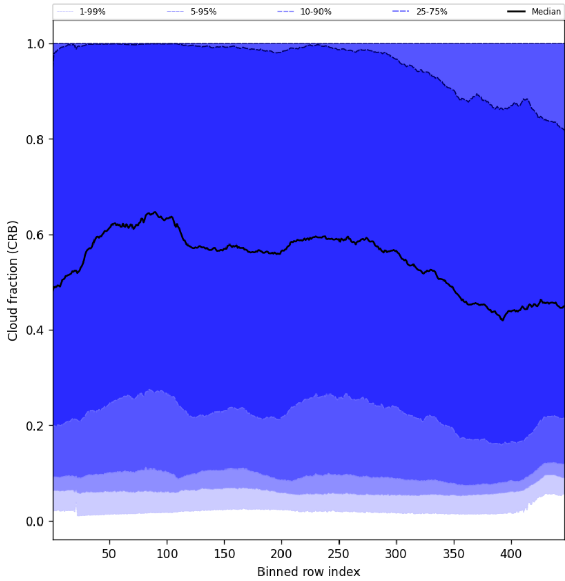
Figure 58: Along track statistics of “Cloud fraction (CRB)” for 2025-08-30 to 2025-08-31
