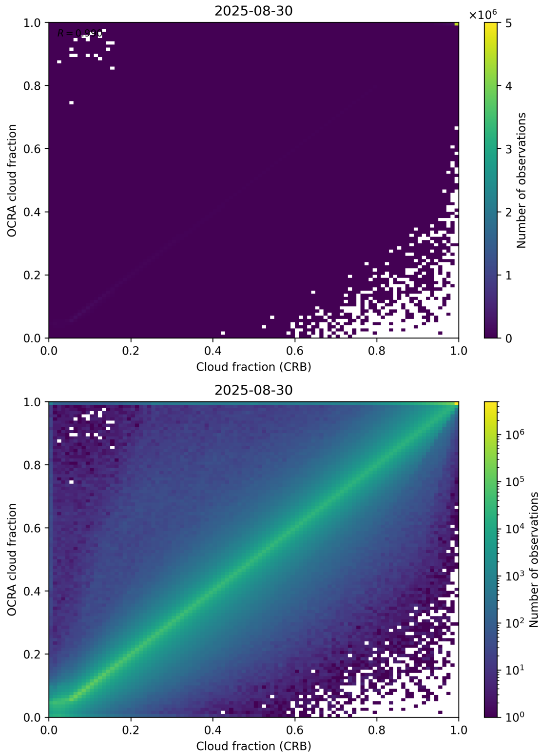
Figure 78: Scatter density plot of “Cloud fraction (CRB)” against “OCRA cloud fraction” for 2025-08-30 to 2025-08-31.
