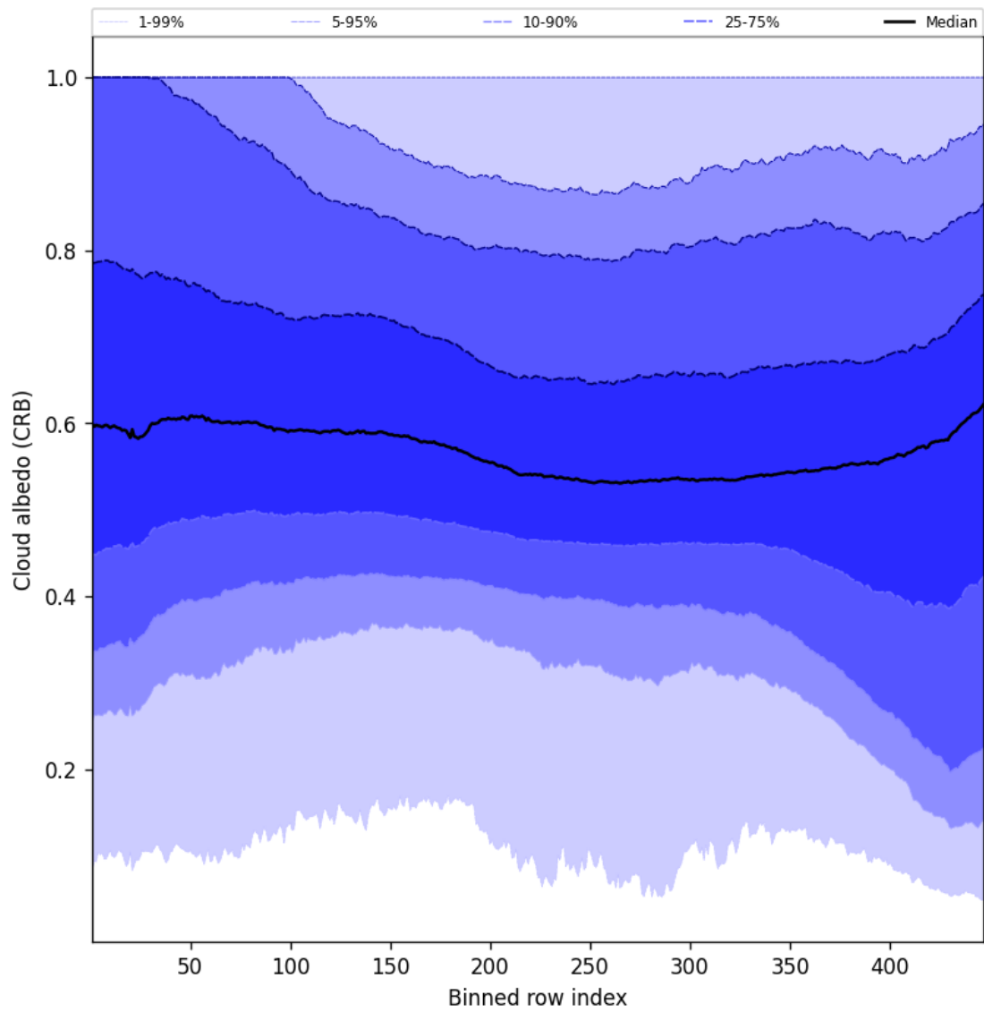
Figure 60: Along track statistics of “Cloud albedo (CRB)” for 2025-08-30 to 2025-08-31
