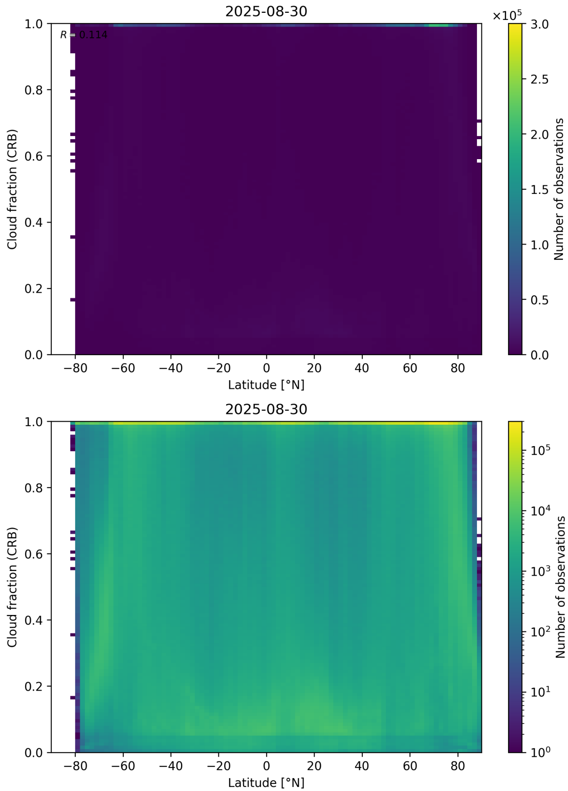
Figure 94: Scatter density plot of “Latitude” against “Cloud fraction (CRB)” for 2025-08-30 to 2025-08-31.
