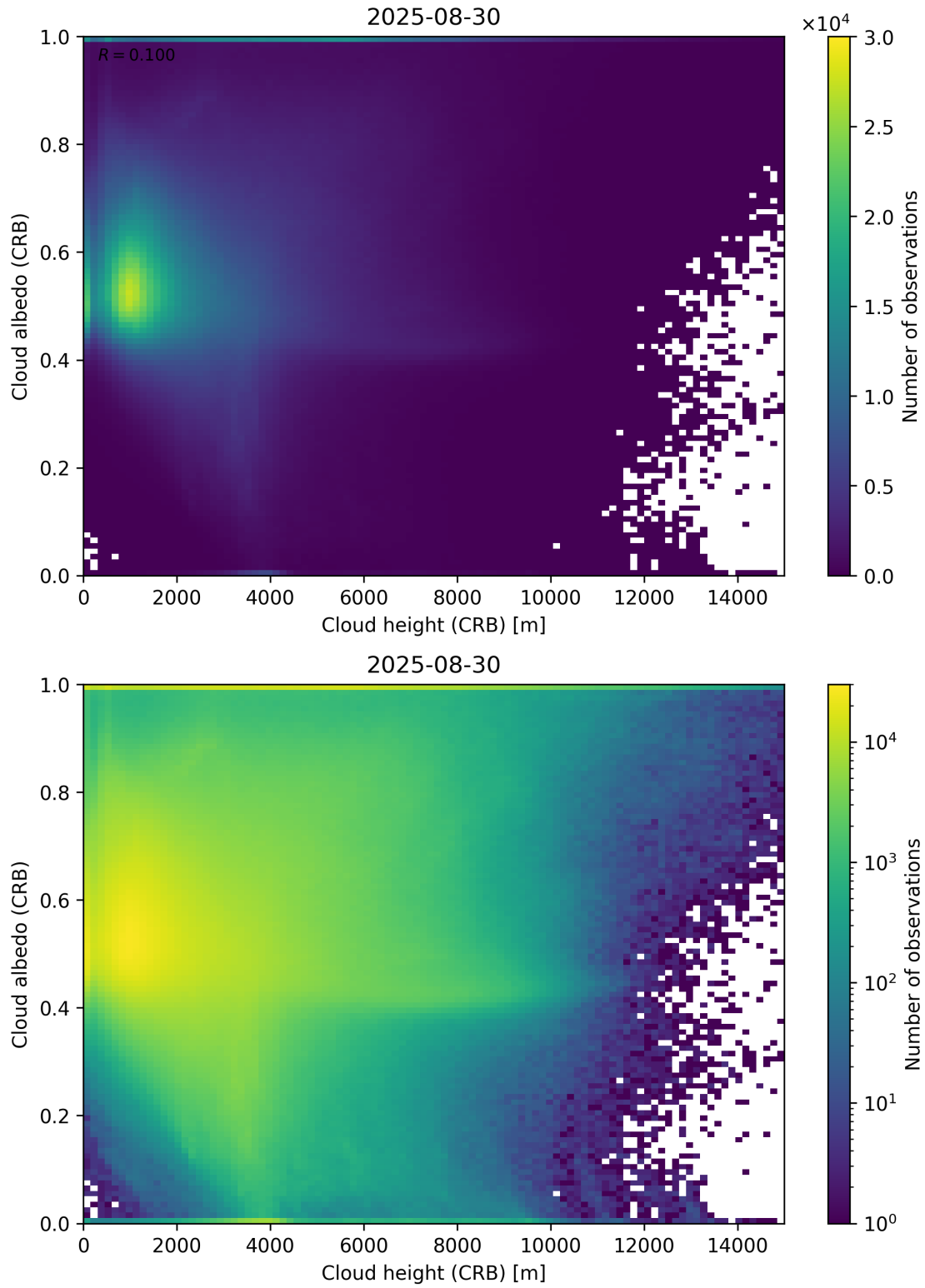
Figure 80: Scatter density plot of “Cloud height (CRB)” against “Cloud albedo (CRB)” for 2025-08-30 to 2025-08-31.
