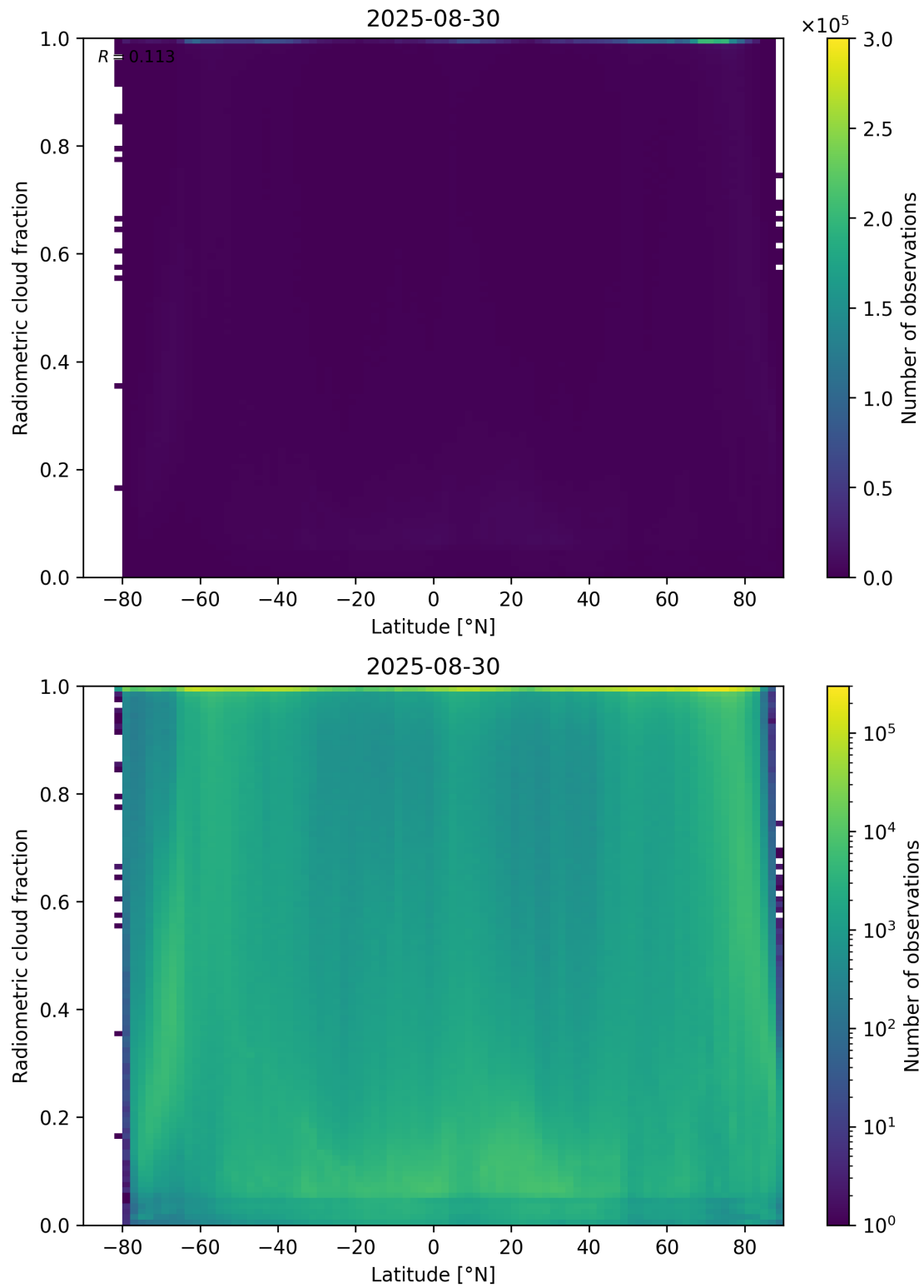
Figure 92: Scatter density plot of “Latitude” against “Radiometric cloud fraction” for 2025-08-30 to 2025-08-31.
