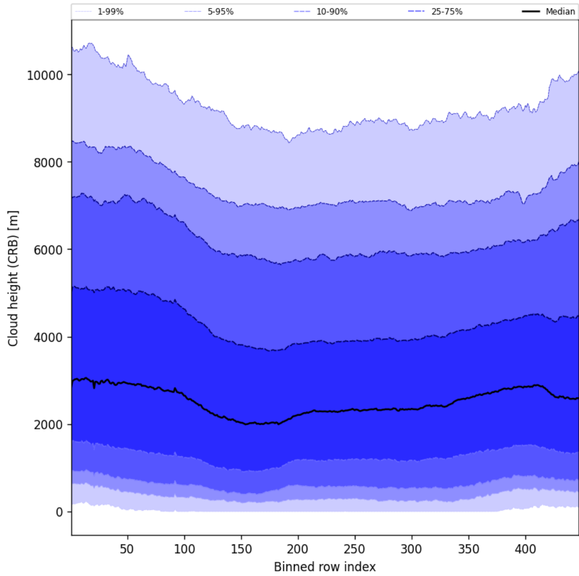
Figure 59: Along track statistics of “Cloud height (CRB)” for 2025-08-30 to 2025-08-31
