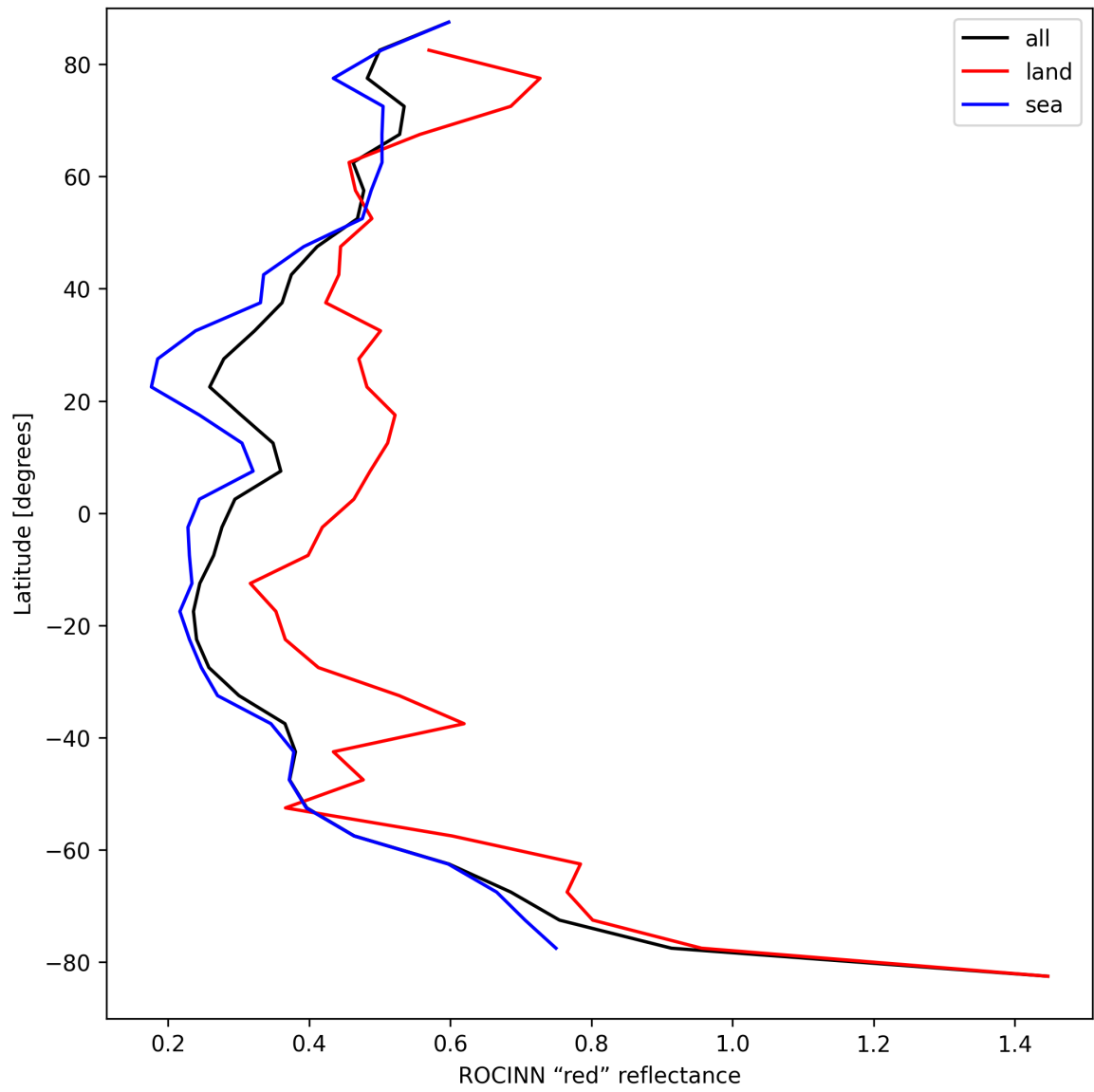
Figure 37: Zonal average of “ROCINN “red” reflectance” for 2025-08-30 to 2025-08-31.
