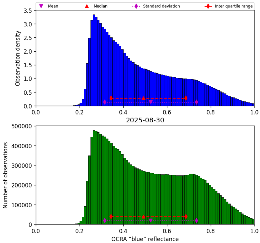
Figure 51: Histogram of “OCRA “blue” reflectance” for 2025-08-30 to 2025-08-31
