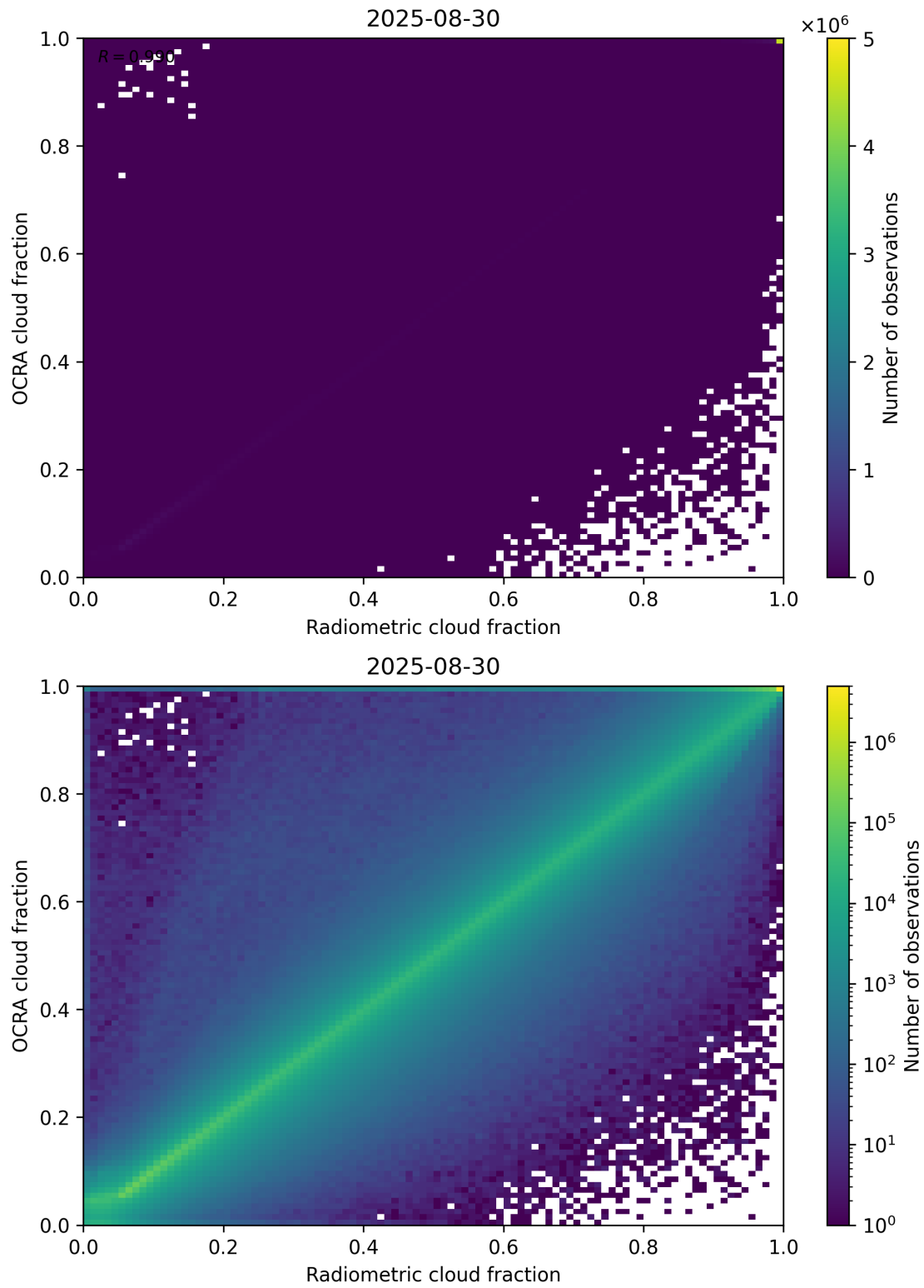
Figure 72: Scatter density plot of “Radiometric cloud fraction” against “OCRA cloud fraction” for 2025-08-30 to 2025-08-31.
