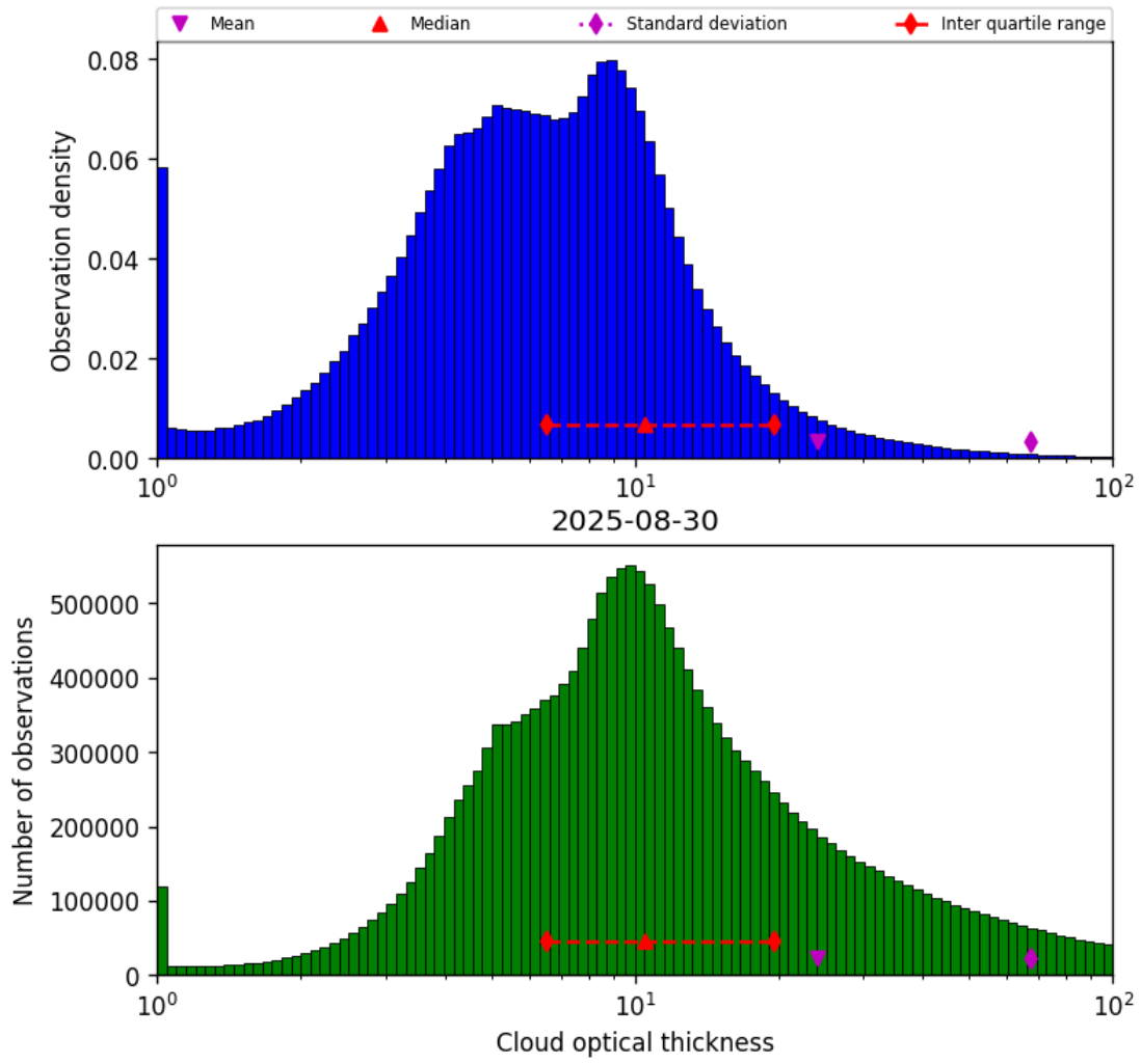
Figure 41: Histogram of “Cloud optical thickness” for 2025-08-30 to 2025-08-31
