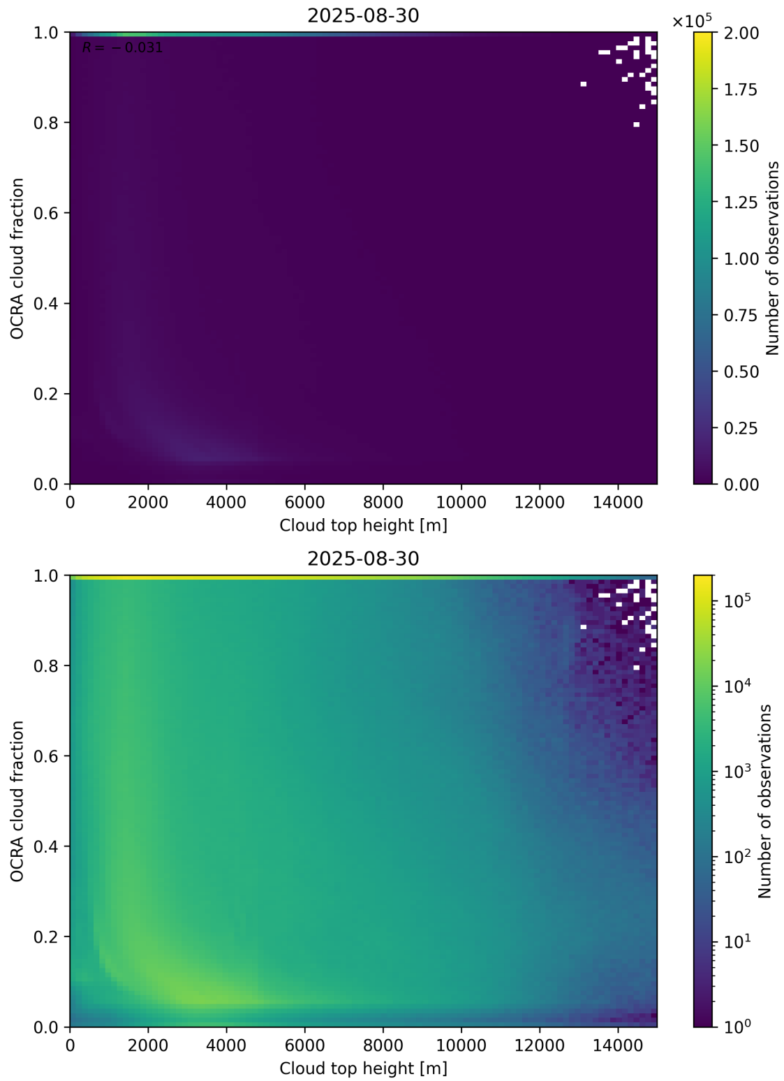
Figure 87: Scatter density plot of “Cloud top height” against “OCRA cloud fraction” for 2025-08-30 to 2025-08-31.
