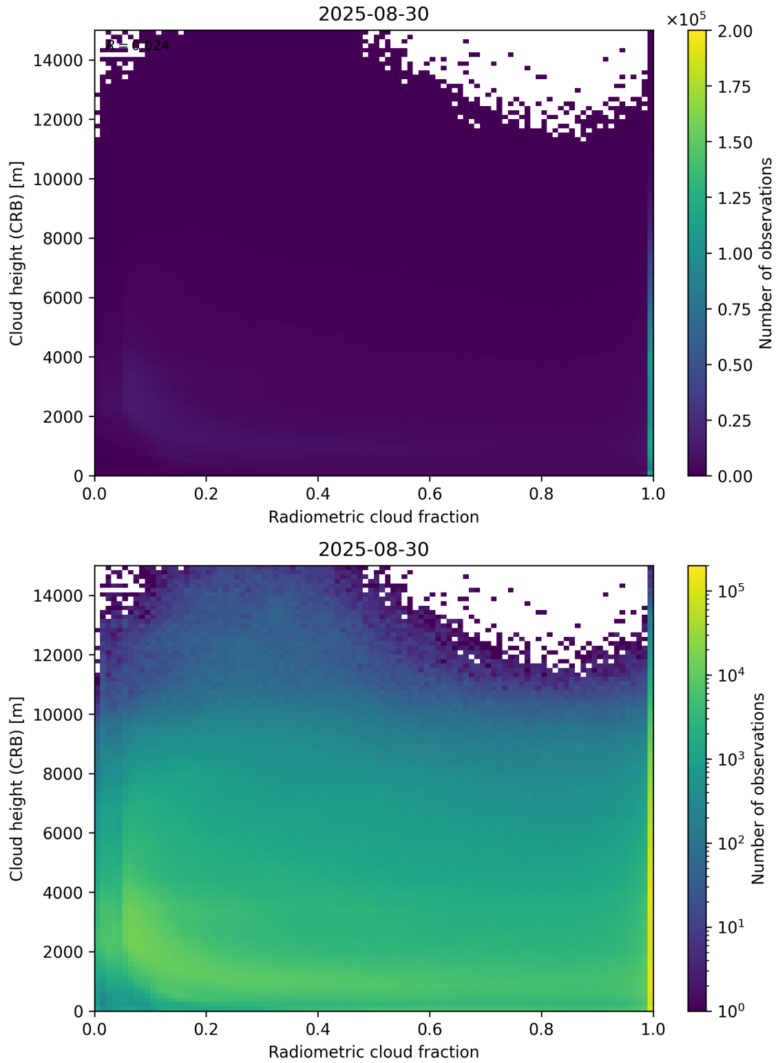
Figure 74: Scatter density plot of “Radiometric cloud fraction” against “Cloud height (CRB)” for 2025-08-30 to 2025-08-31.
