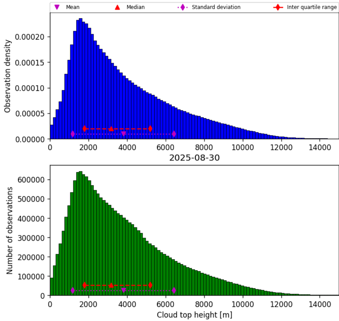
Figure 40: Histogram of “Cloud top height” for 2025-08-30 to 2025-08-31
