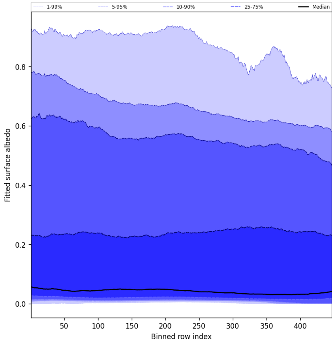
Figure 61: Along track statistics of “Fitted surface albedo” for 2025-08-30 to 2025-08-31
