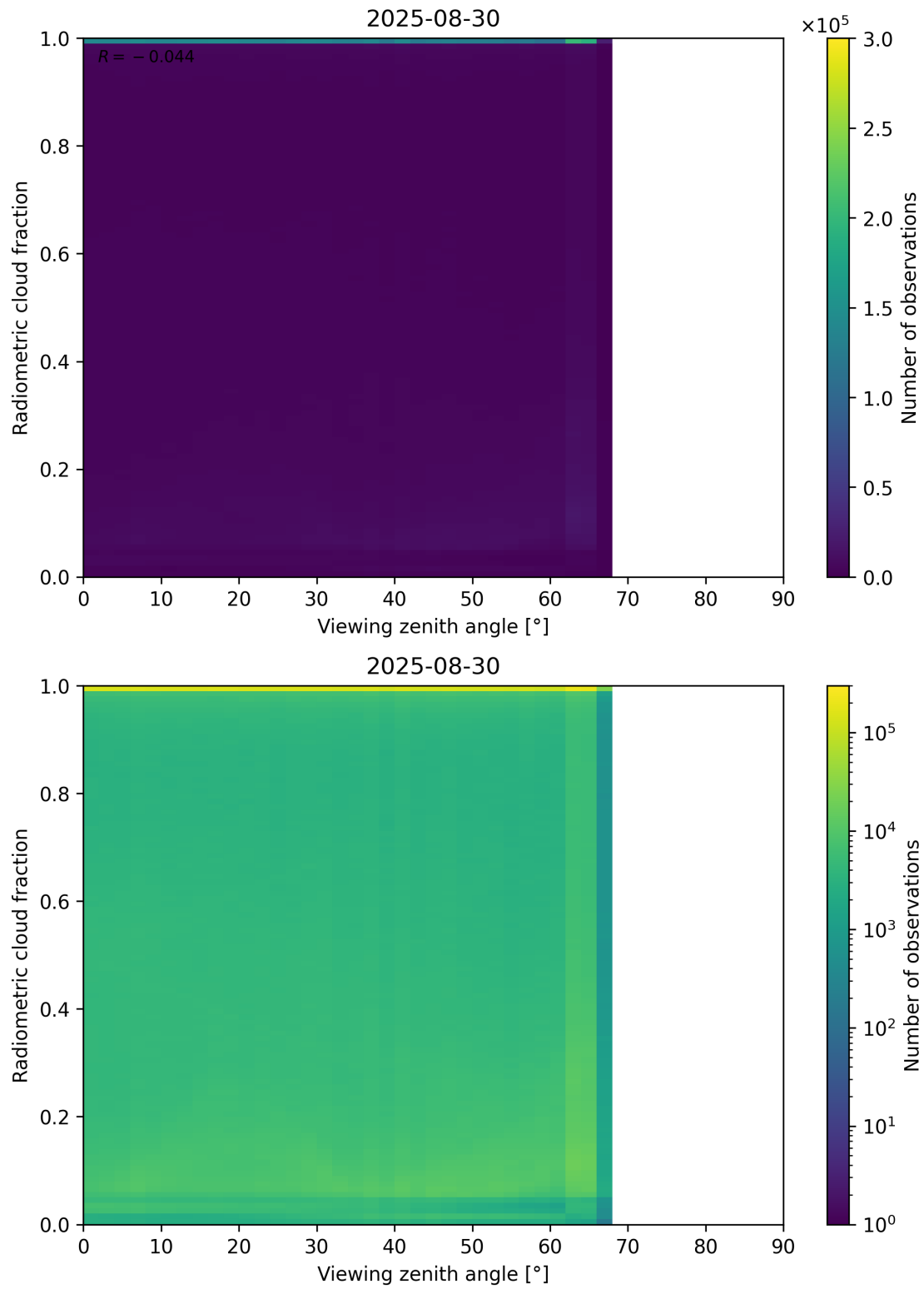
Figure 107: Scatter density plot of “Viewing zenith angle” against “Radiometric cloud fraction” for 2025-08-30 to 2025-08-31.
