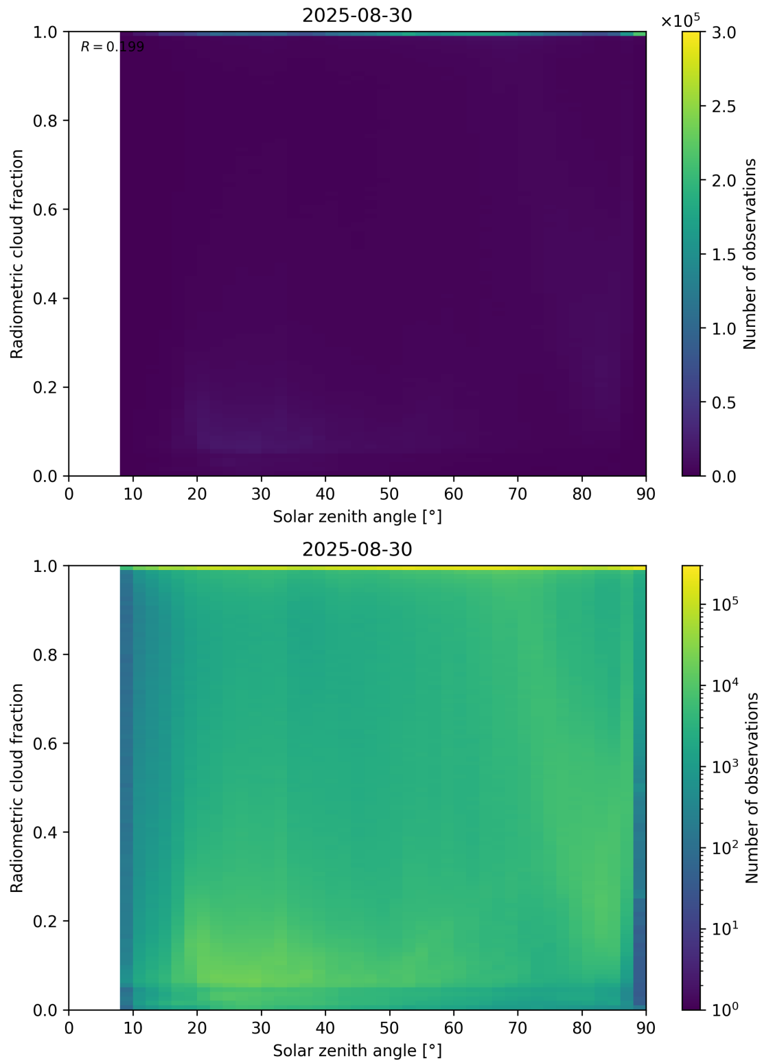
Figure 99: Scatter density plot of “Solar zenith angle” against “Radiometric cloud fraction” for 2025-08-30 to 2025-08-31.
