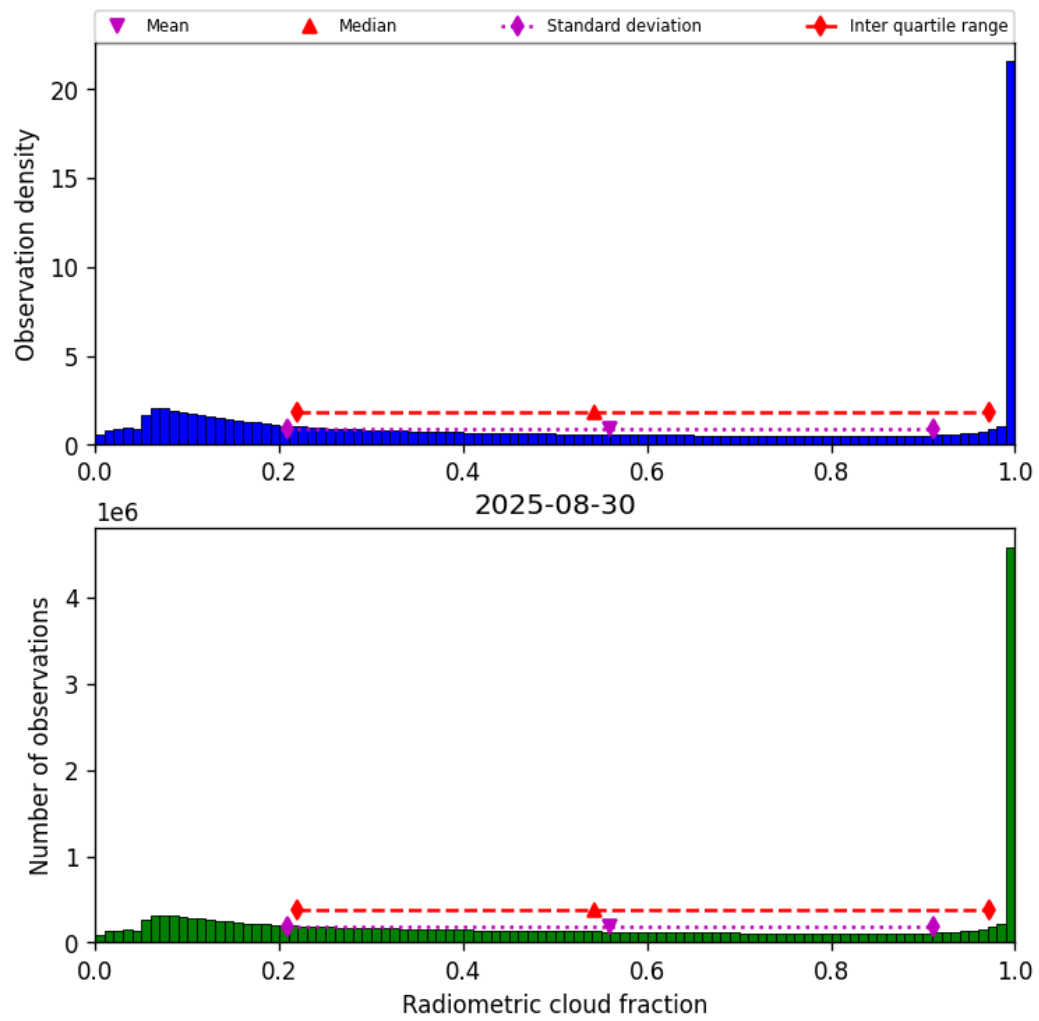
Figure 39: Histogram of “Radiometric cloud fraction” for 2025-08-30 to 2025-08-31
