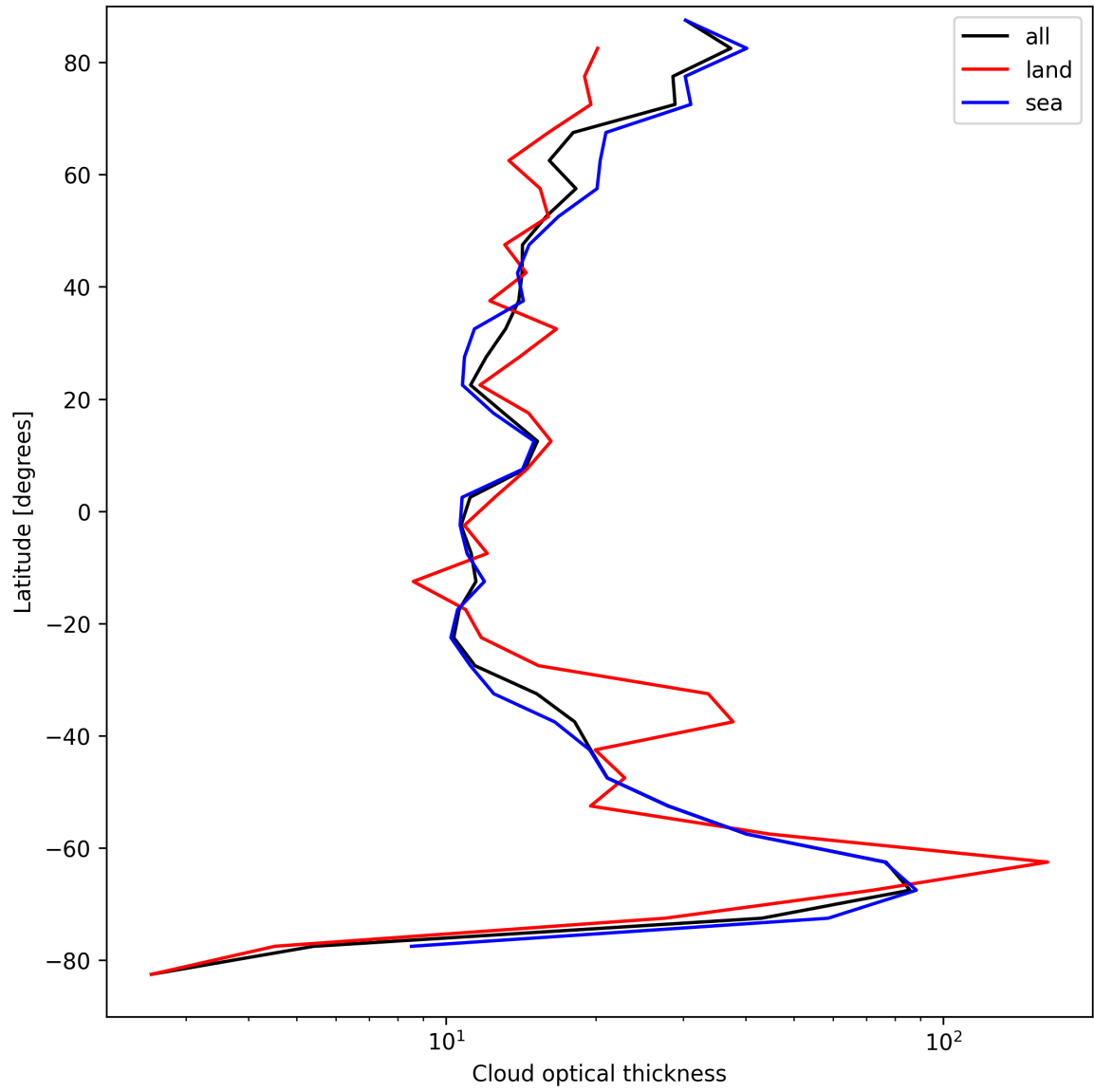
Figure 25: Zonal average of “Cloud optical thickness” for 2025-08-30 to 2025-08-31.
