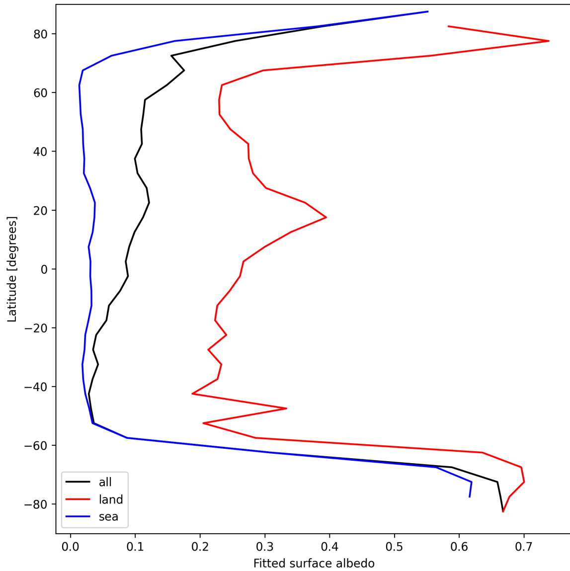
Figure 29: Zonal average of “Fitted surface albedo” for 2025-08-30 to 2025-08-31.
