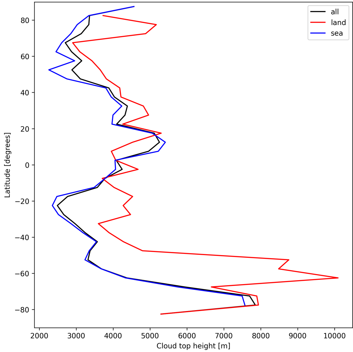
Figure 24: Zonal average of “Cloud top height” for 2025-08-30 to 2025-08-31.
