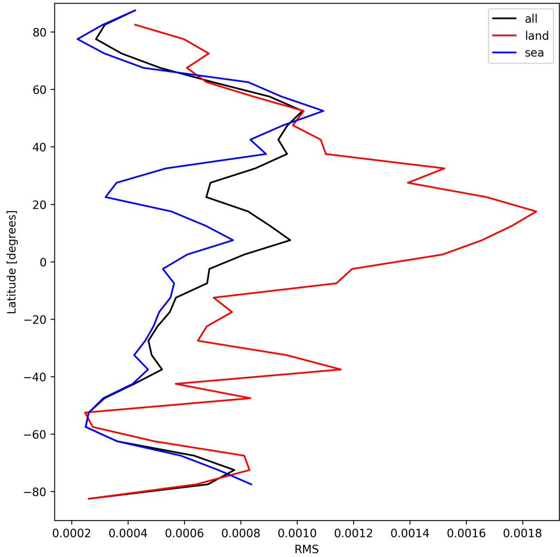
Figure 31: Zonal average of “RMS” for 2025-08-30 to 2025-08-31.
