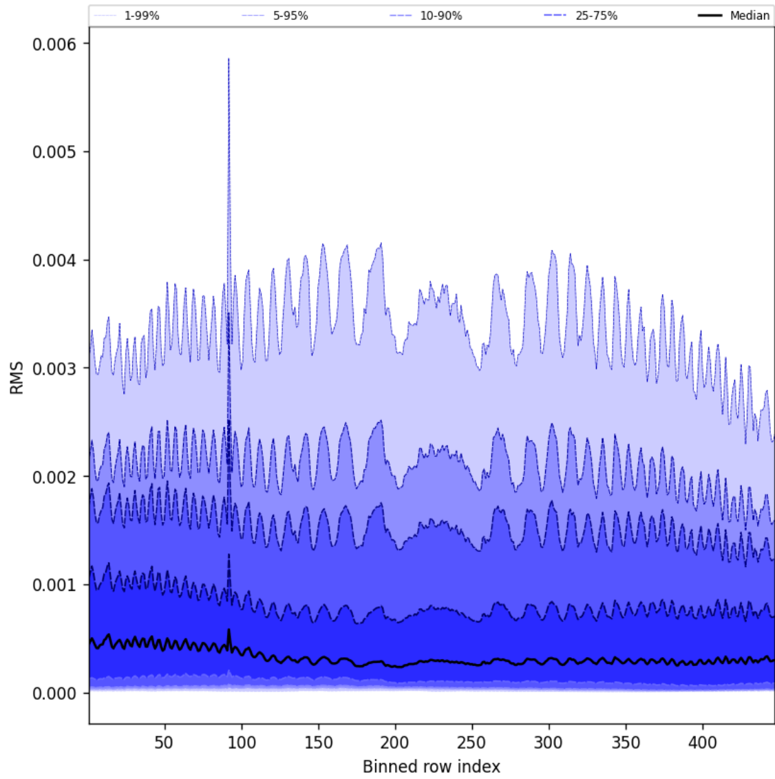
Figure 63: Along track statistics of “RMS” for 2025-08-30 to 2025-08-31
