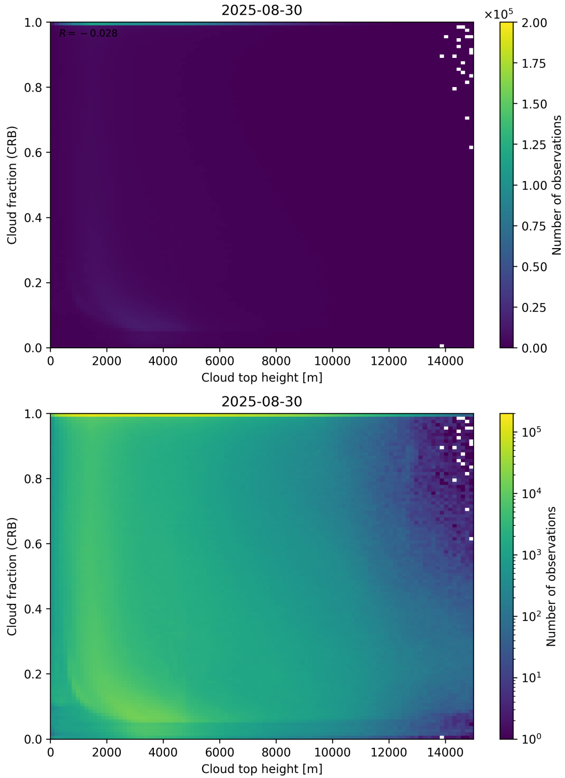
Figure 88: Scatter density plot of “Cloud top height” against “Cloud fraction (CRB)” for 2025-08-30 to 2025-08-31.
