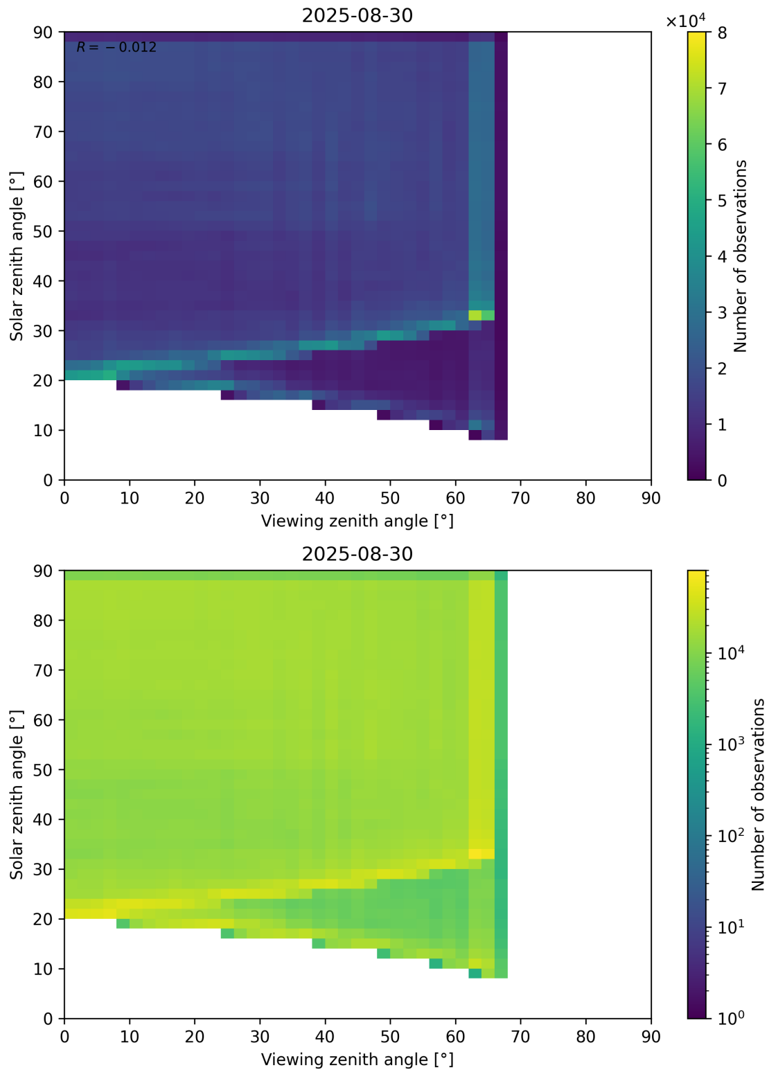
Figure 114: Scatter density plot of “Viewing zenith angle” against “Solar zenith angle” for 2025-08-30 to 2025-08-31.
