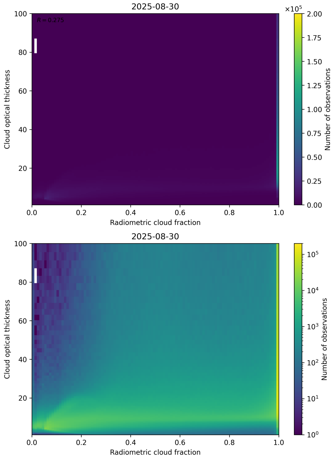
Figure 75: Scatter density plot of “Radiometric cloud fraction” against “Cloud optical thickness” for 2025-08-30 to 2025-08-31.
