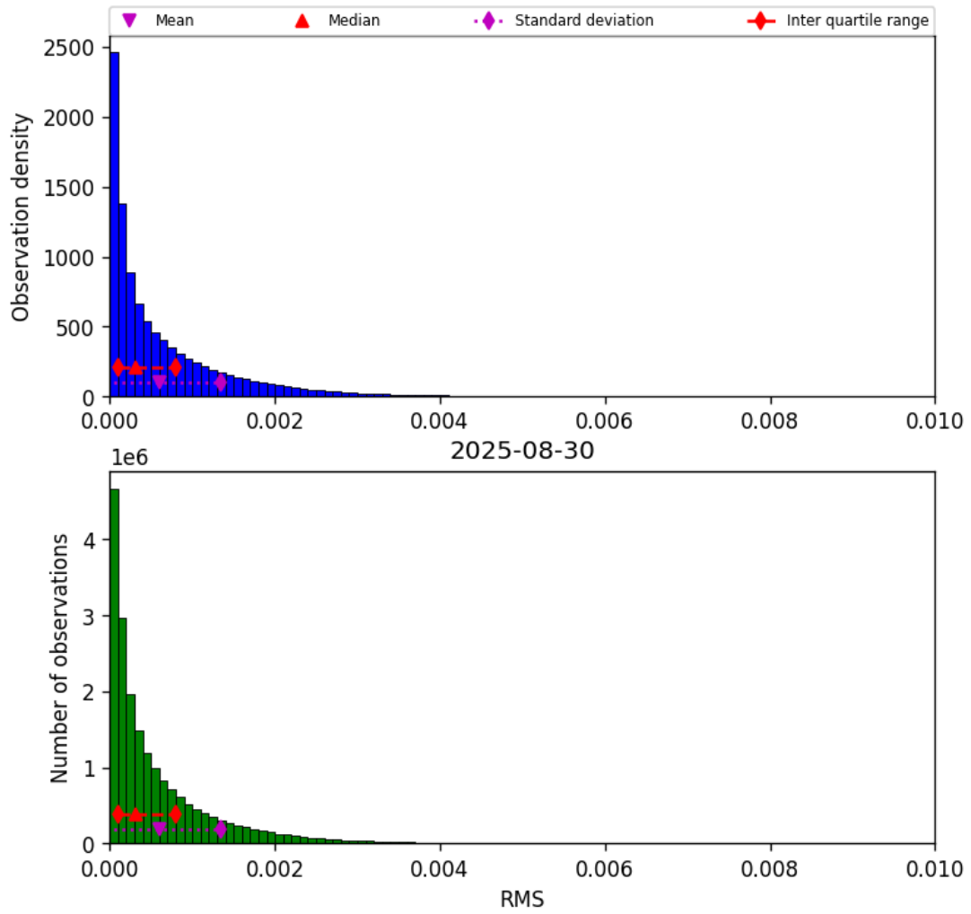
Figure 47: Histogram of “RMS” for 2025-08-30 to 2025-08-31
