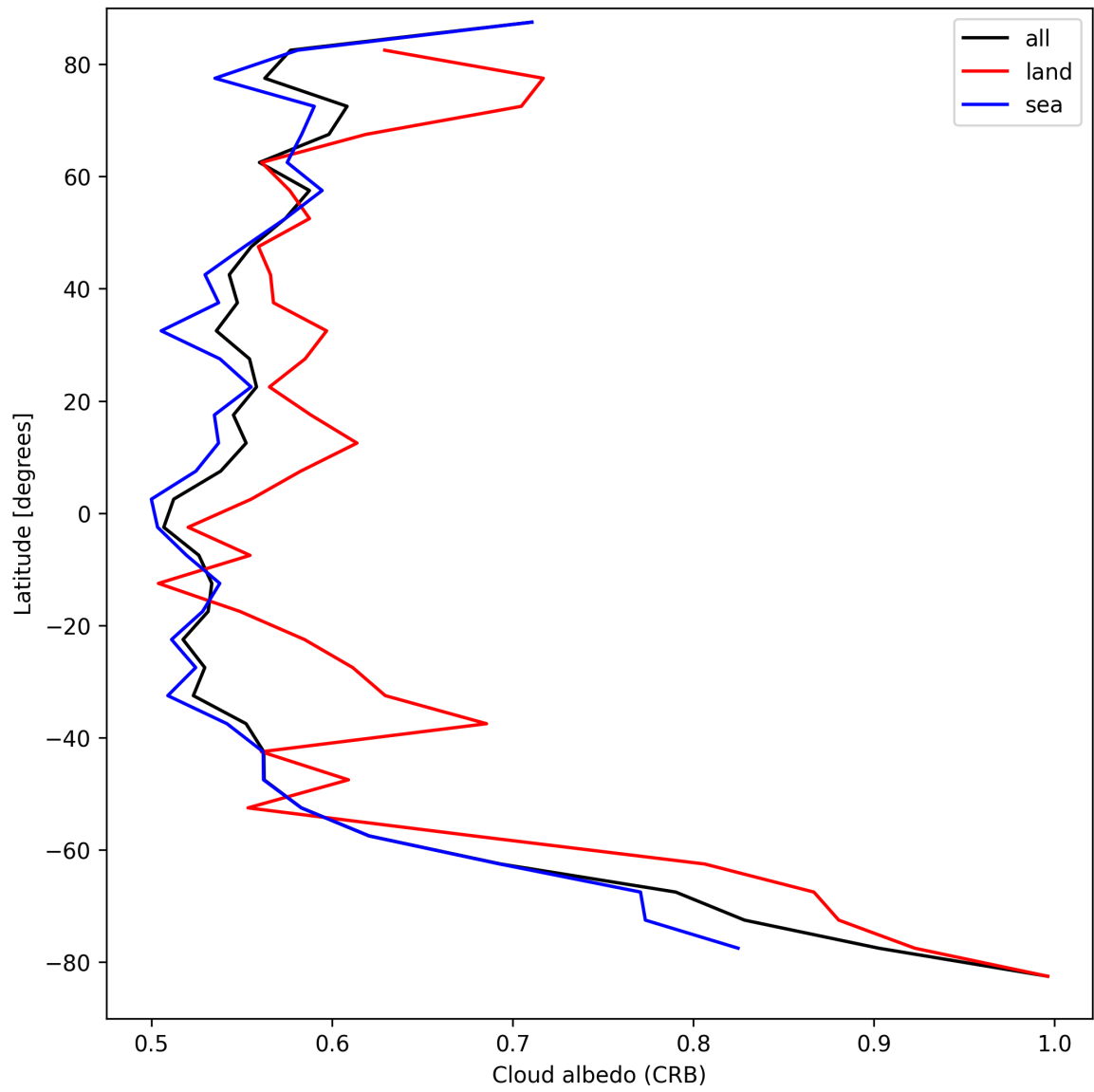
Figure 28: Zonal average of “Cloud albedo (CRB)” for 2025-08-30 to 2025-08-31.
