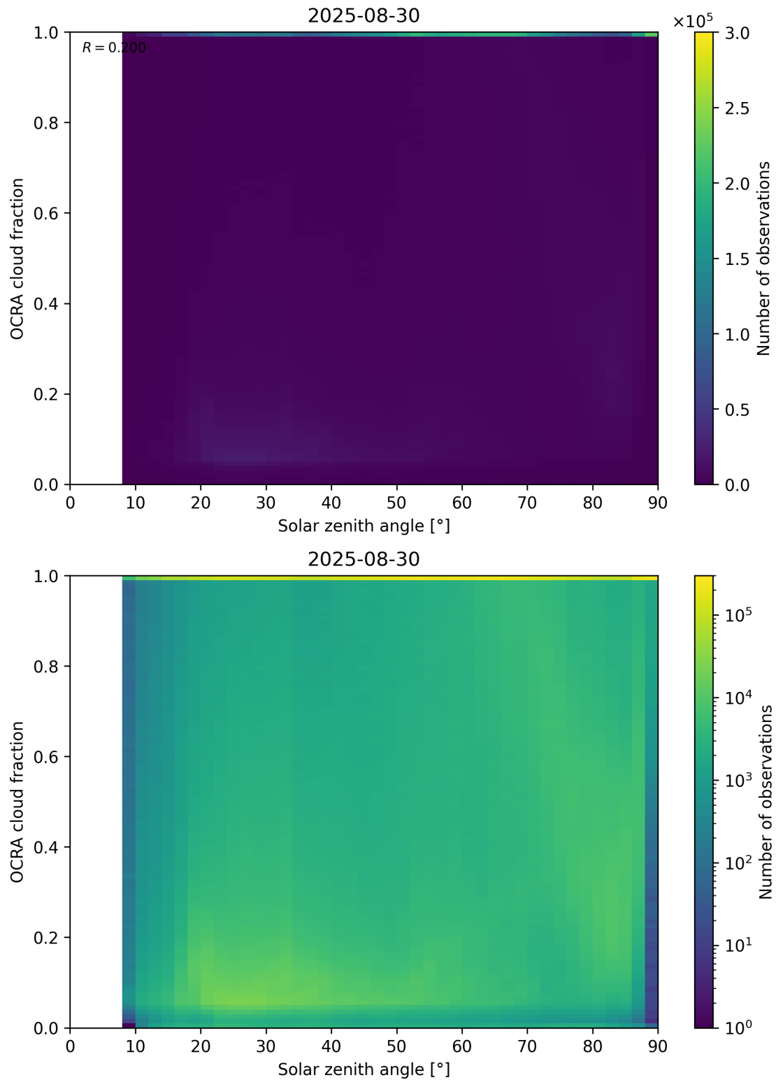
Figure 100: Scatter density plot of “Solar zenith angle” against “OCRA cloud fraction” for 2025-08-30 to 2025-08-31.
