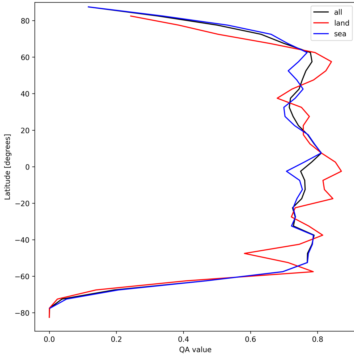
Figure 22: Zonal average of “QA value” for 2025-08-30 to 2025-08-31.
