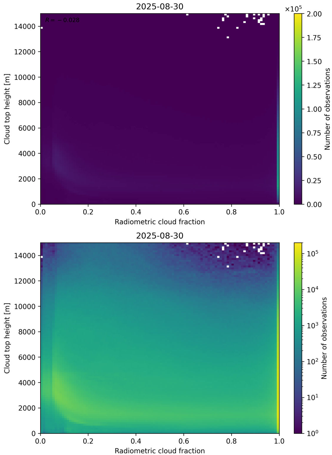
Figure 76: Scatter density plot of “Radiometric cloud fraction” against “Cloud top height” for 2025-08-30 to 2025-08-31.
