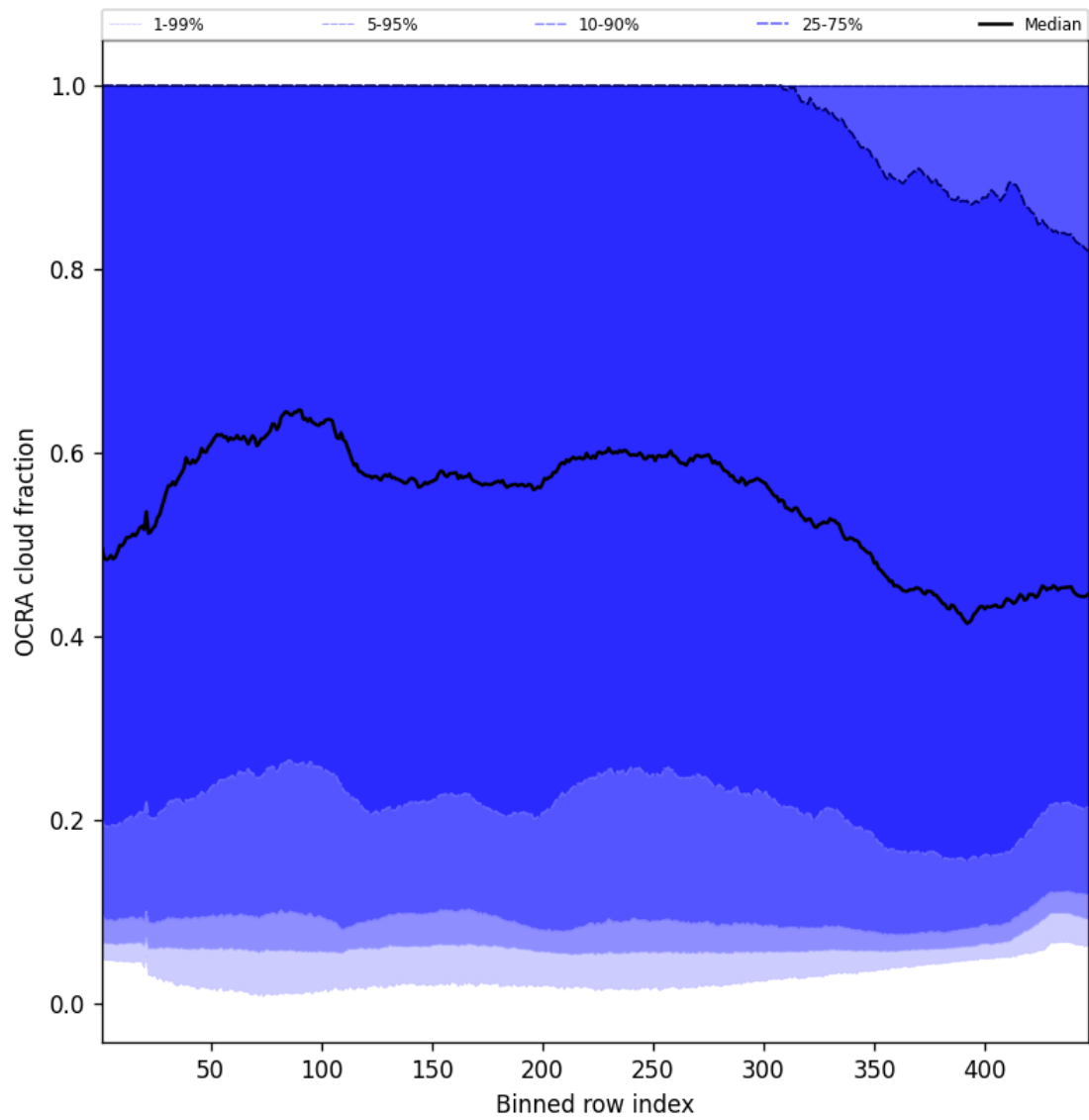
Figure 66: Along track statistics of “OCRA cloud fraction” for 2025-08-30 to 2025-08-31
