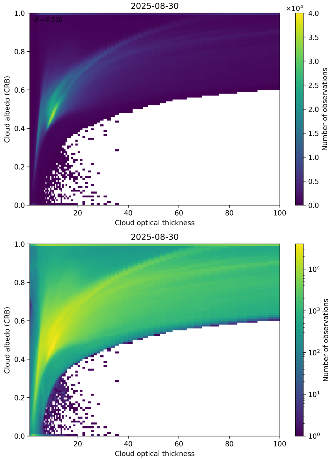
Figure 82: Scatter density plot of “Cloud optical thickness” against “Cloud albedo (CRB)” for 2025-08-30 to 2025-08-31.
