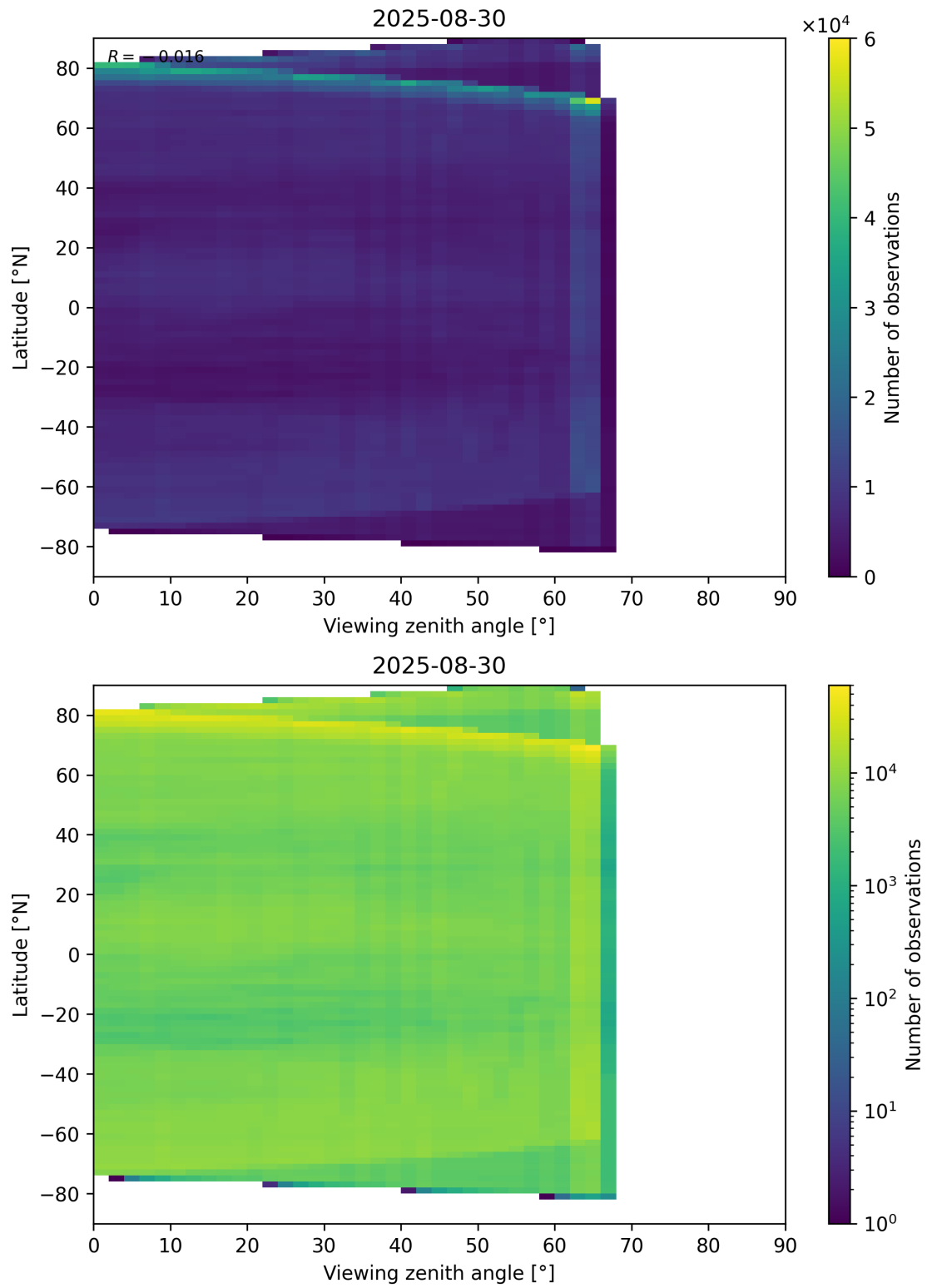
Figure 113: Scatter density plot of “Viewing zenith angle” against “Latitude” for 2025-08-30 to 2025-08-31.
