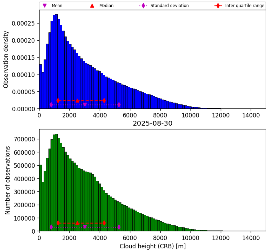
Figure 43: Histogram of “Cloud height (CRB)” for 2025-08-30 to 2025-08-31
