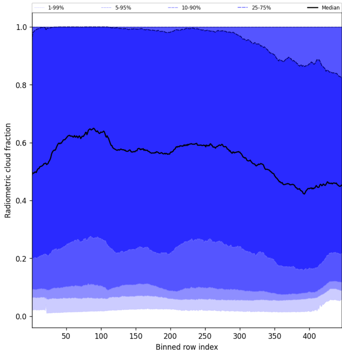
Figure 55: Along track statistics of “Radiometric cloud fraction” for 2025-08-30 to 2025-08-31
