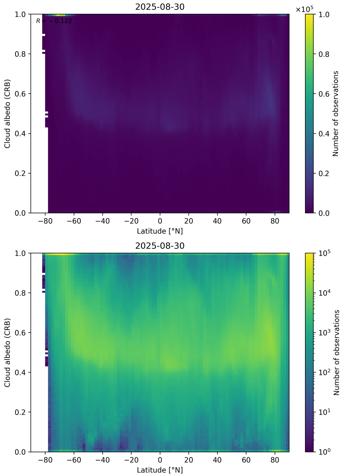
Figure 91: Scatter density plot of “Latitude” against “Cloud albedo (CRB)” for 2025-08-30 to 2025-08-31.
