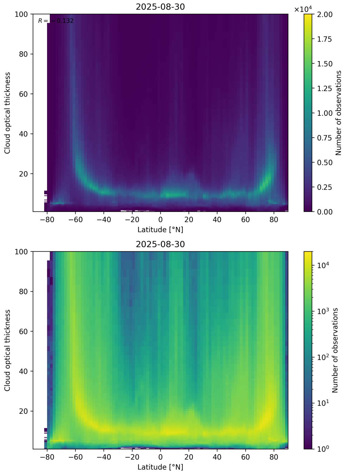
Figure 96: Scatter density plot of “Latitude” against “Cloud optical thickness” for 2025-08-30 to 2025-08-31.
