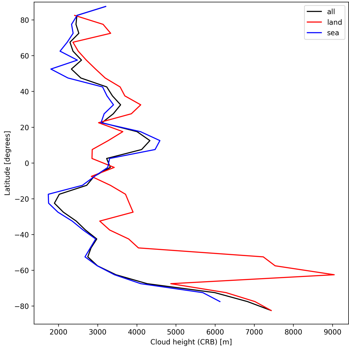
Figure 27: Zonal average of “Cloud height (CRB)” for 2025-08-30 to 2025-08-31.
