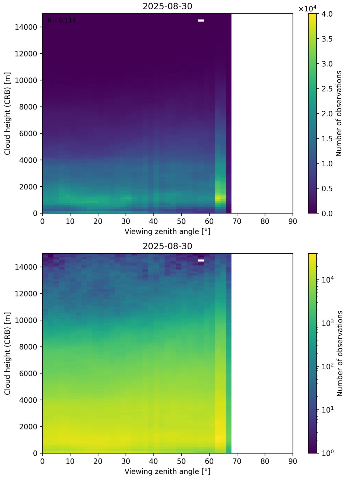
Figure 110: Scatter density plot of “Viewing zenith angle” against “Cloud height (CRB)” for 2025-08-30 to 2025-08-31.
