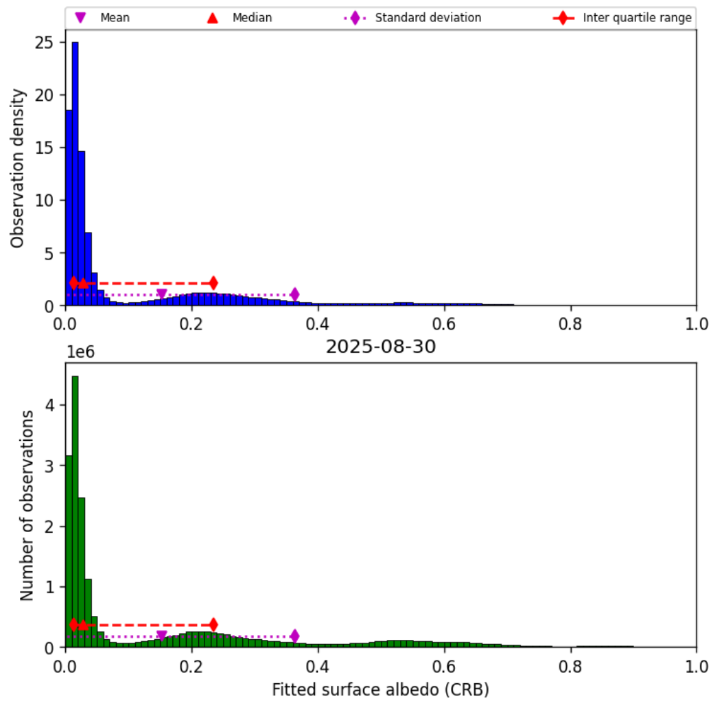
Figure 46: Histogram of “Fitted surface albedo (CRB)” for 2025-08-30 to 2025-08-31
