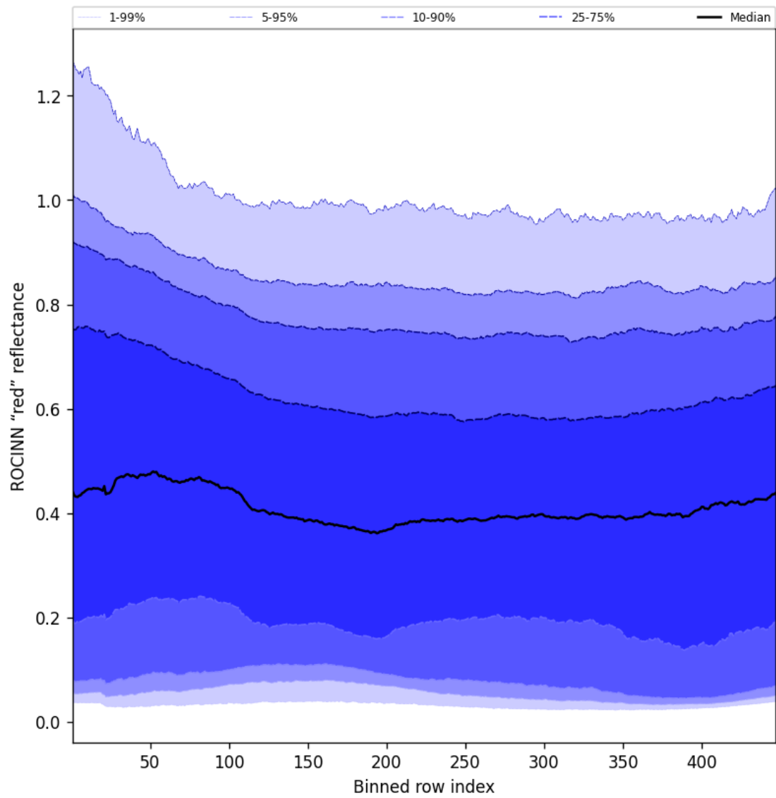
Figure 69: Along track statistics of "ROCINN "red" reflectance" for 2025-08-30 to 2025-08-31
