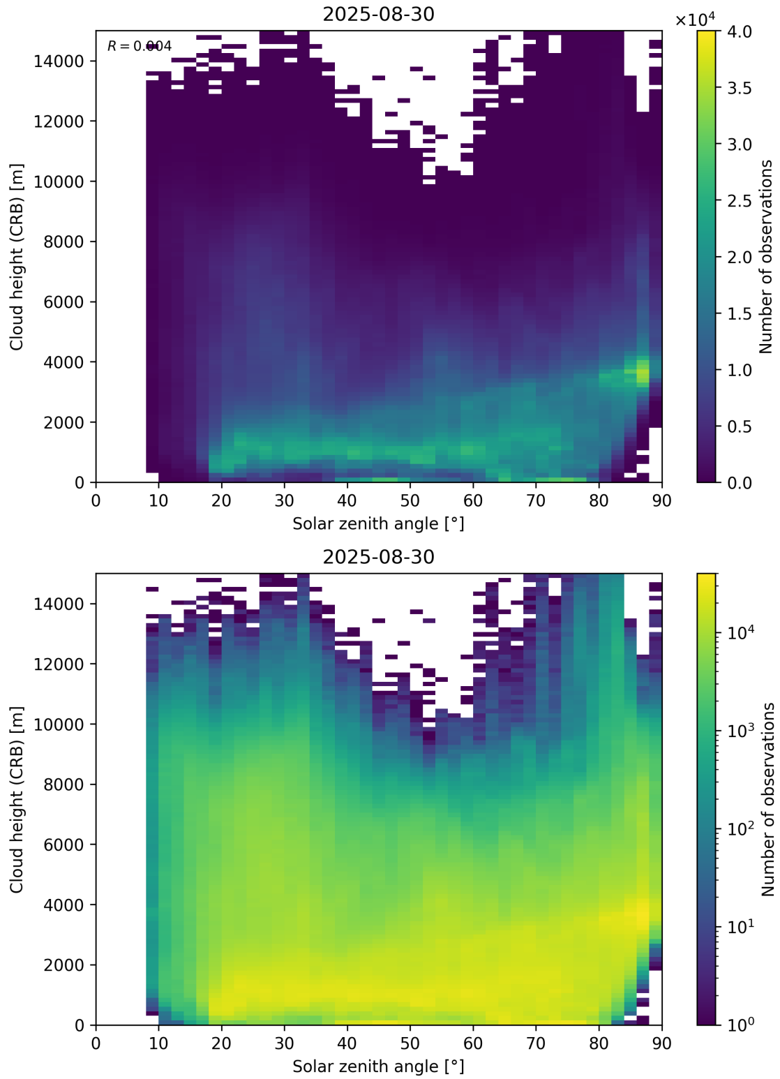
Figure 102: Scatter density plot of “Solar zenith angle” against “Cloud height (CRB)” for 2025-08-30 to 2025-08-31.
