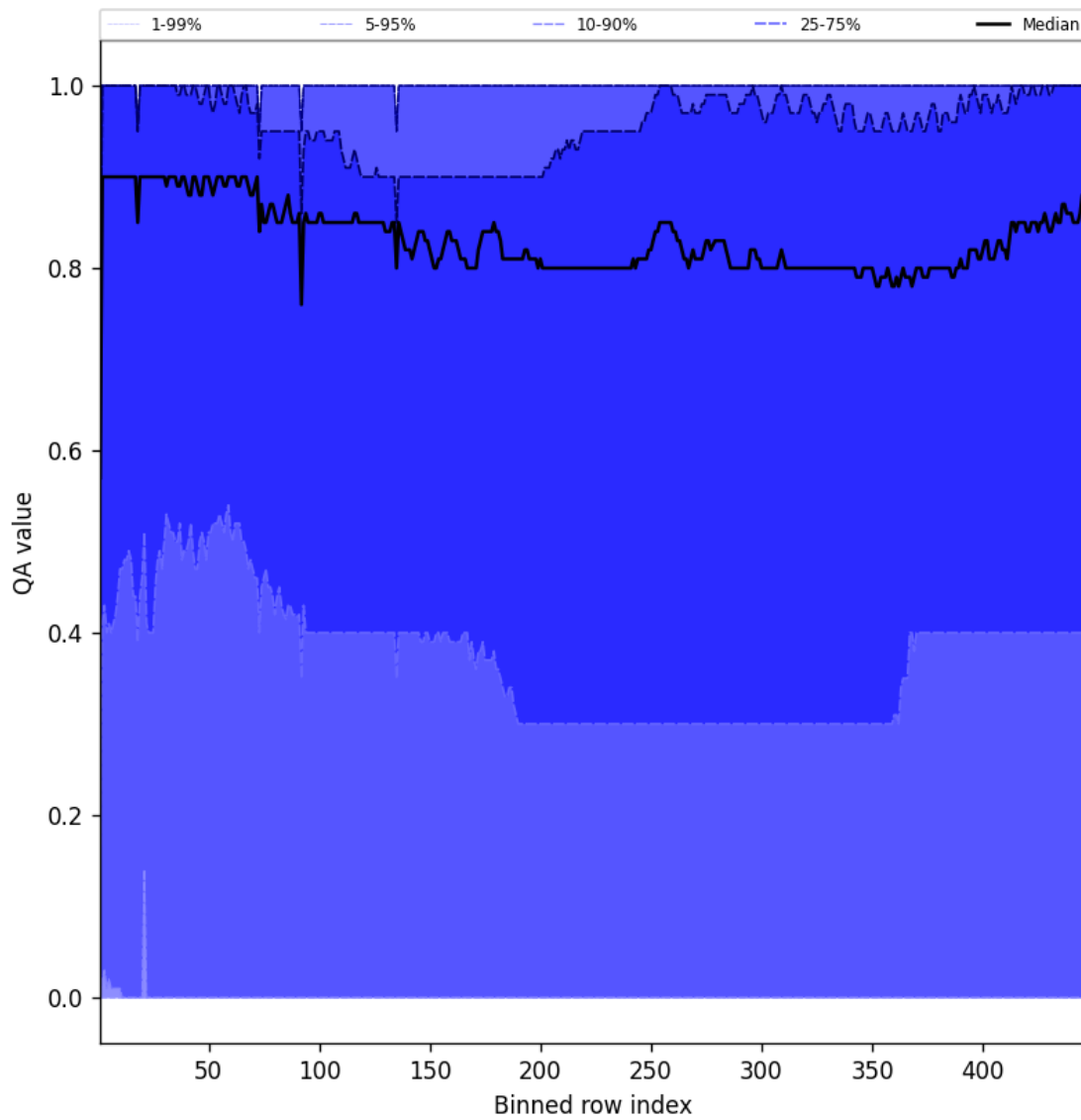
Figure 54: Along track statistics of “QA value” for 2025-08-30 to 2025-08-31
