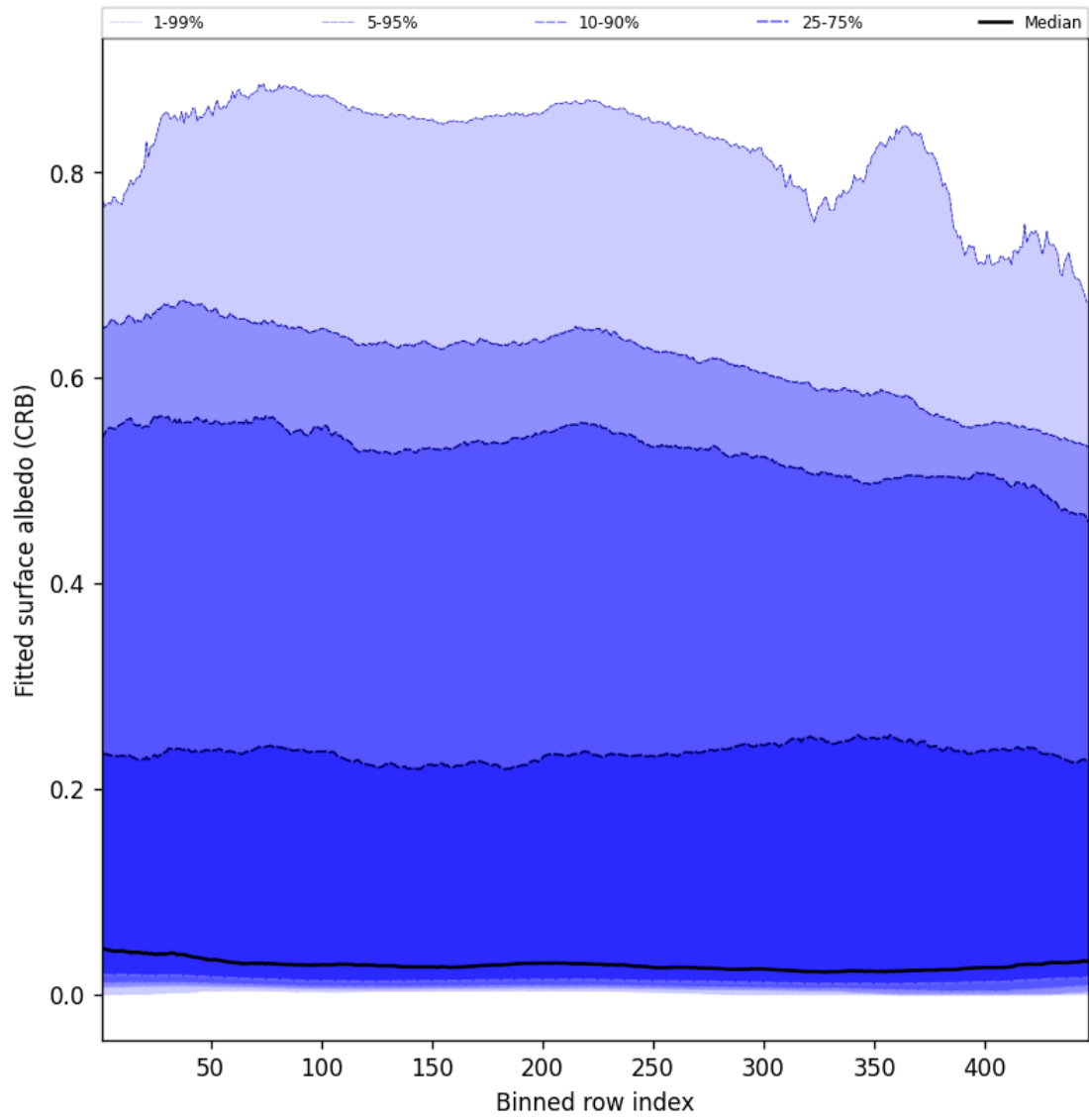
Figure 62: Along track statistics of “Fitted surface albedo (CRB)” for 2025-08-30 to 2025-08-31
