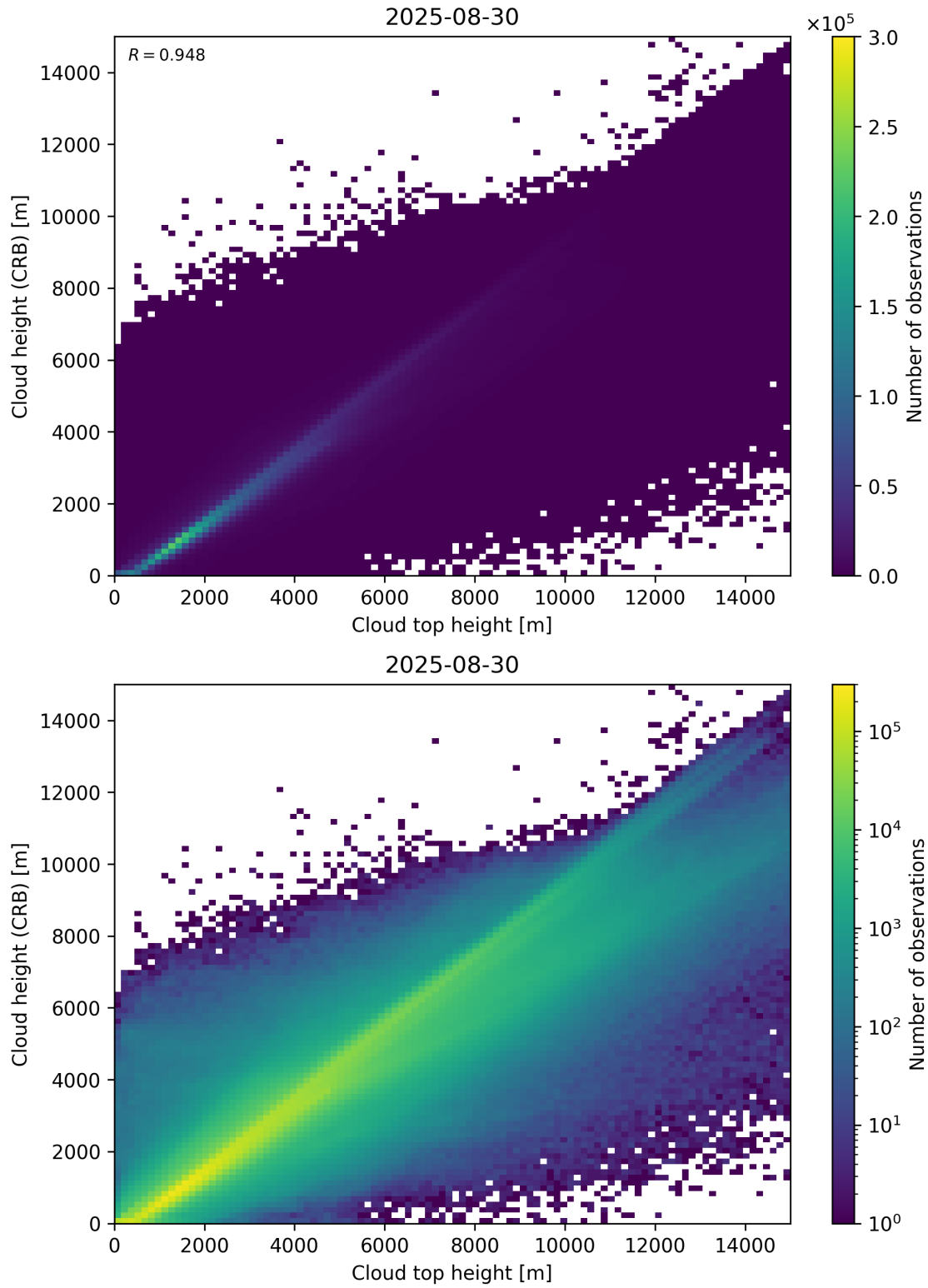
Figure 89: Scatter density plot of “Cloud top height” against “Cloud height (CRB)” for 2025-08-30 to 2025-08-31.
