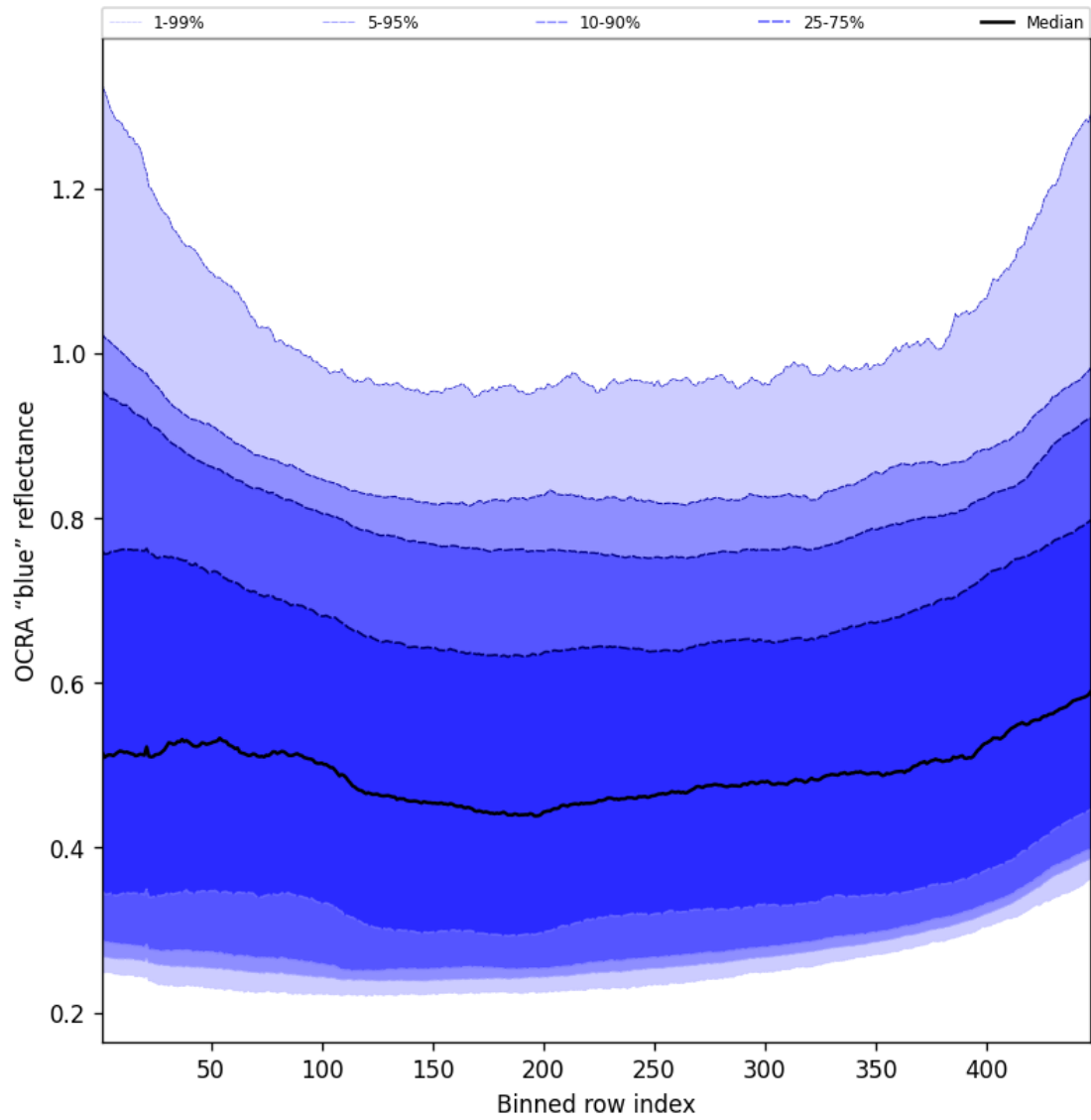
Figure 67: Along track statistics of “OCRA “blue” reflectance” for 2025-08-30 to 2025-08-31
