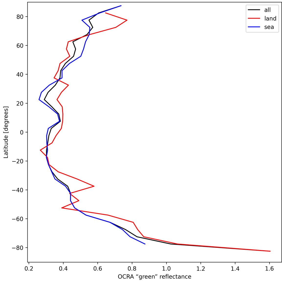
Figure 36: Zonal average of “OCRA “green” reflectance” for 2025-08-30 to 2025-08-31.
