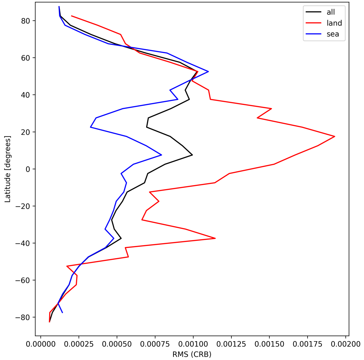
Figure 32: Zonal average of “RMS (CRB)” for 2025-08-30 to 2025-08-31.
