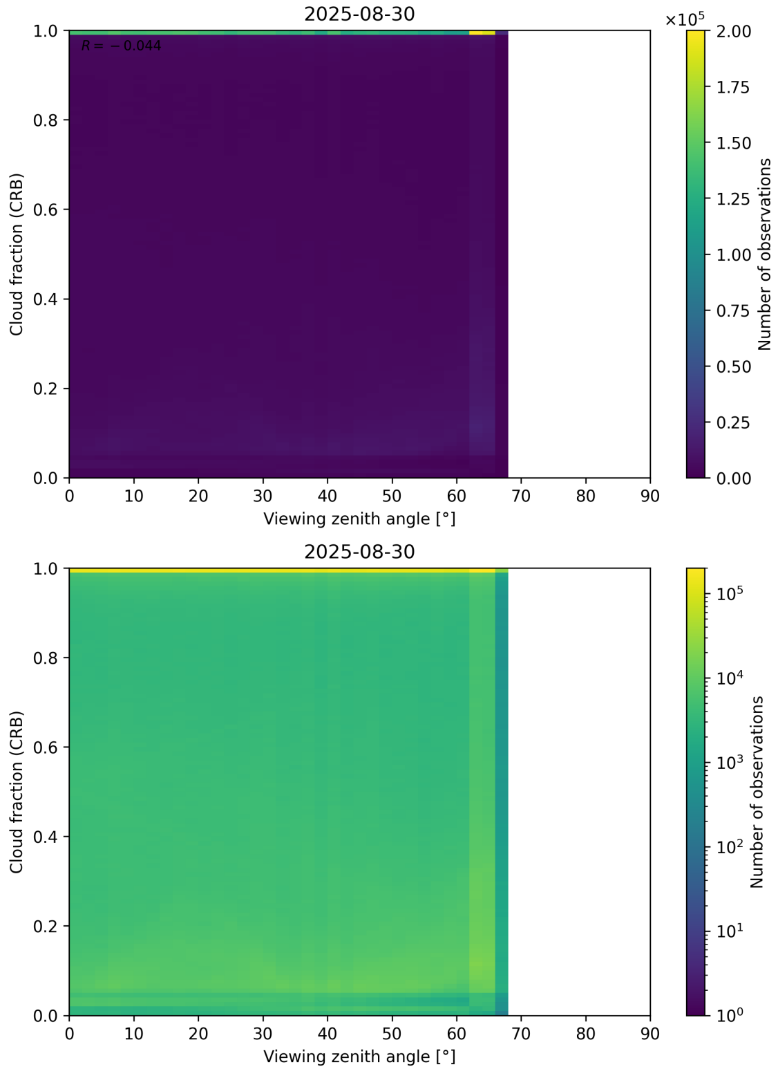
Figure 109: Scatter density plot of “Viewing zenith angle” against “Cloud fraction (CRB)” for 2025-08-30 to 2025-08-31.
