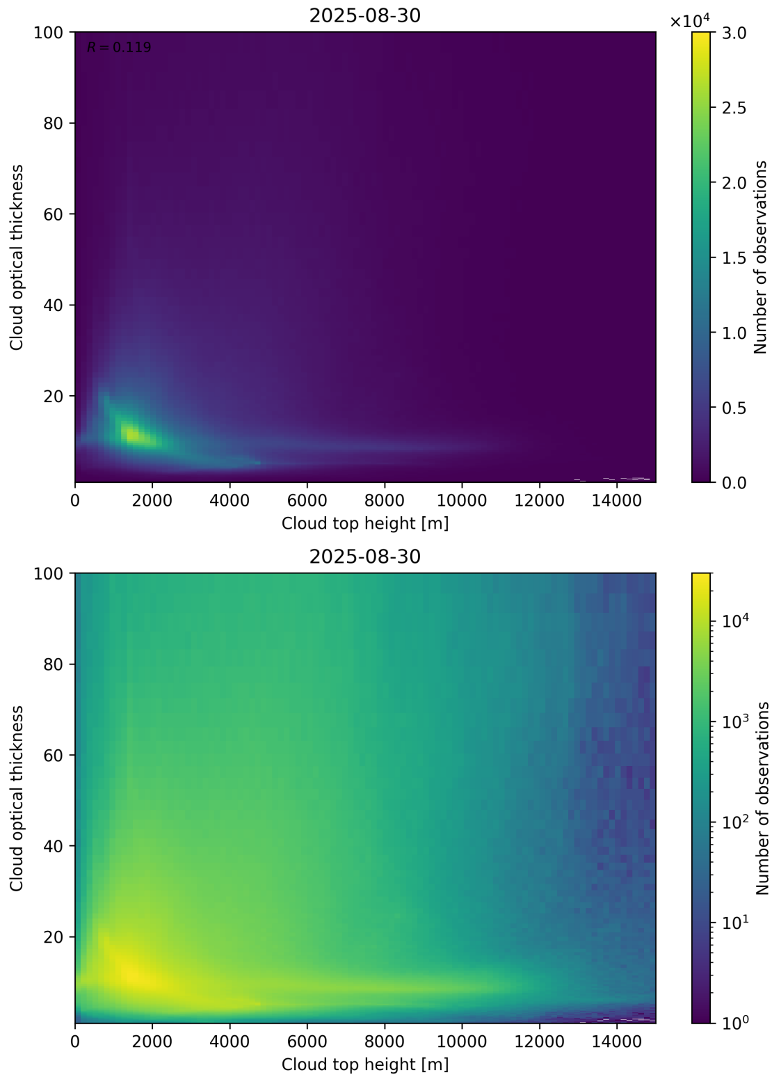
Figure 90: Scatter density plot of “Cloud top height” against “Cloud optical thickness” for 2025-08-30 to 2025-08-31.
