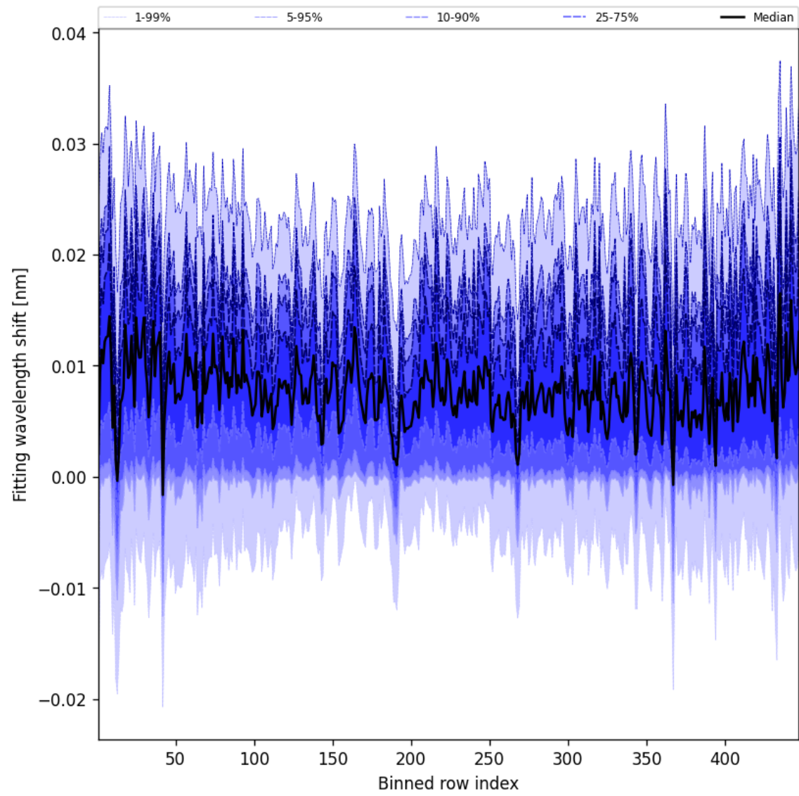
Figure 65: Along track statistics of “Fitting wavelength shift” for 2025-08-30 to 2025-08-31
