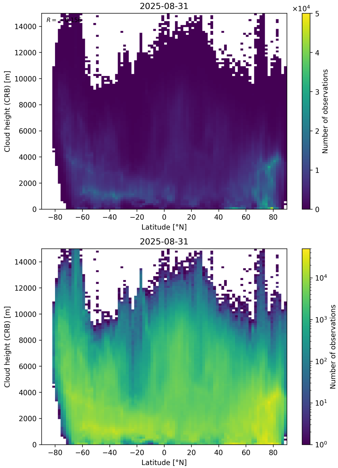
Figure 95: Scatter density plot of “Latitude” against “Cloud height (CRB)” for 2025-08-30 to 2025-09-01.
