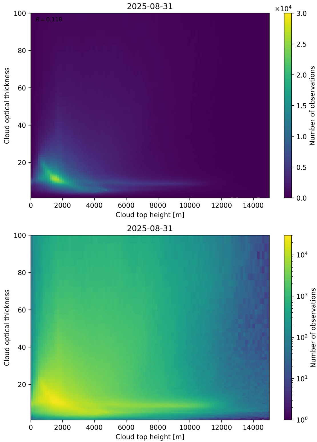
Figure 90: Scatter density plot of “Cloud top height” against “Cloud optical thickness” for 2025-08-30 to 2025-09-01.
