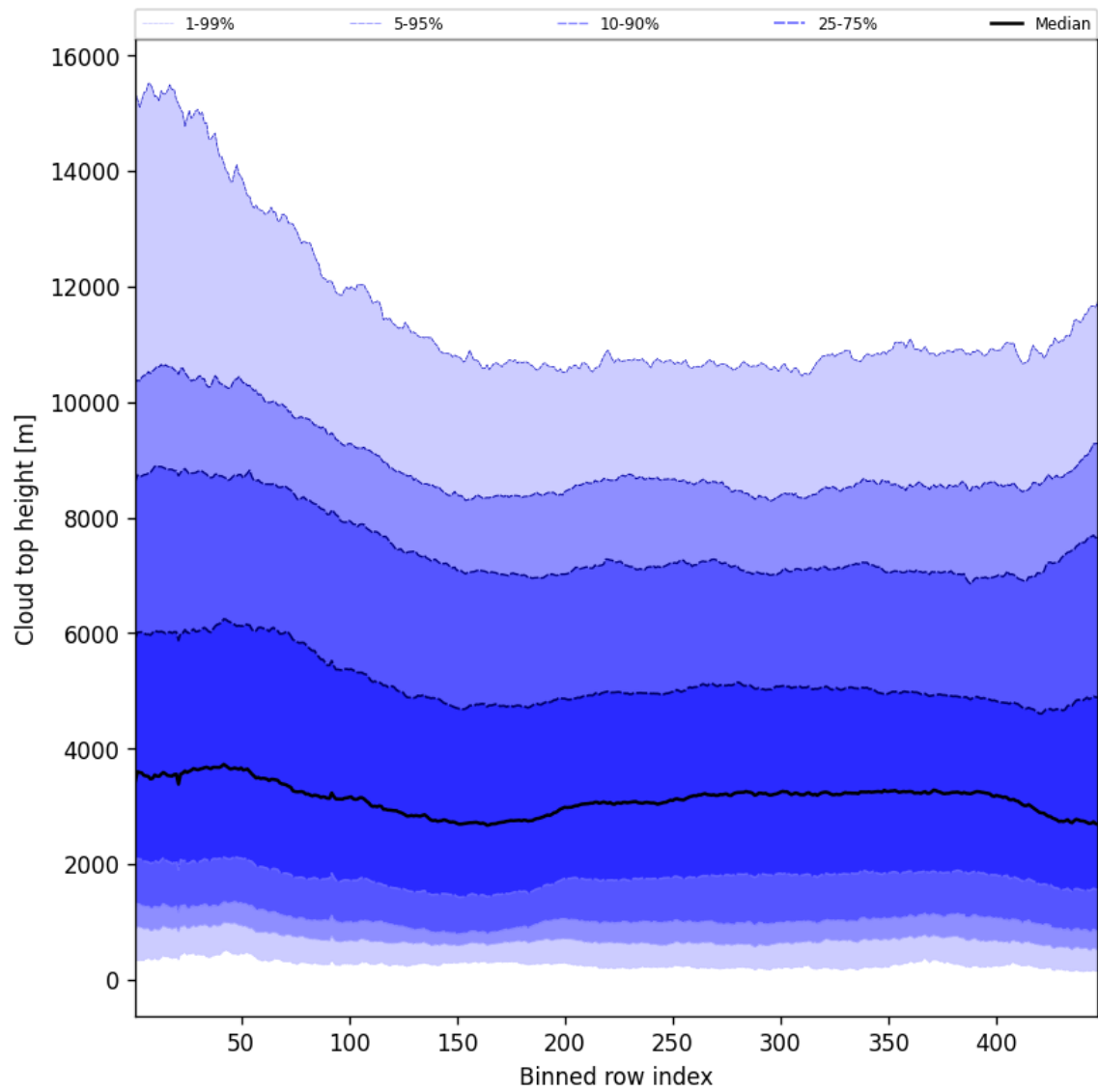
Figure 56: Along track statistics of “Cloud top height” for 2025-08-30 to 2025-09-01
