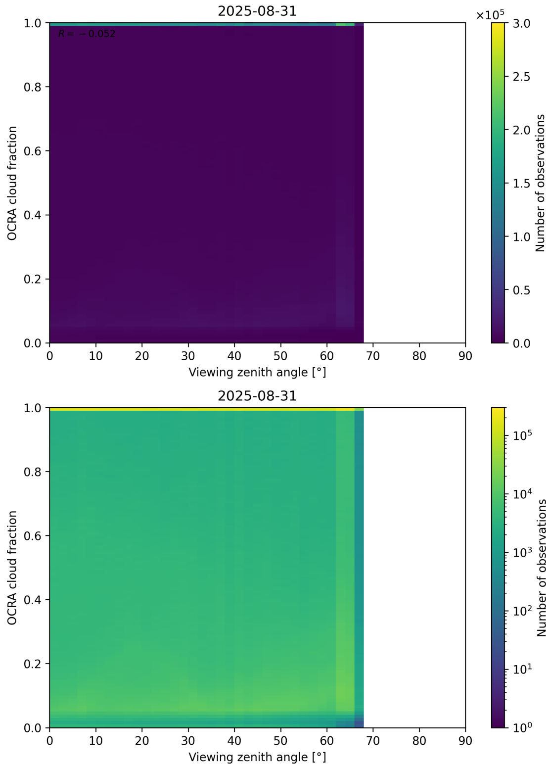
Figure 108: Scatter density plot of “Viewing zenith angle” against “OCRA cloud fraction” for 2025-08-30 to 2025-09-01.
