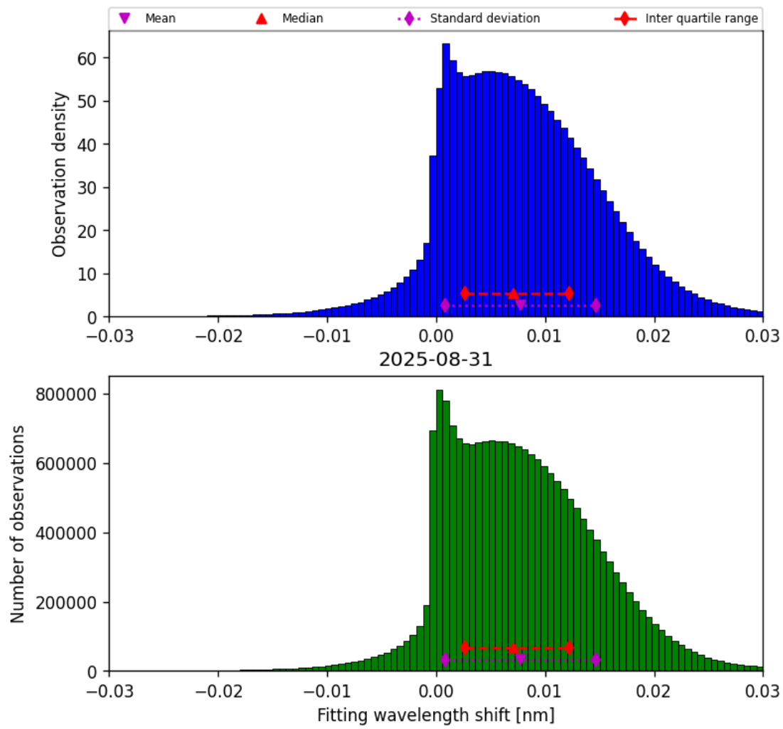
Figure 49: Histogram of “Fitting wavelength shift” for 2025-08-30 to 2025-09-01
