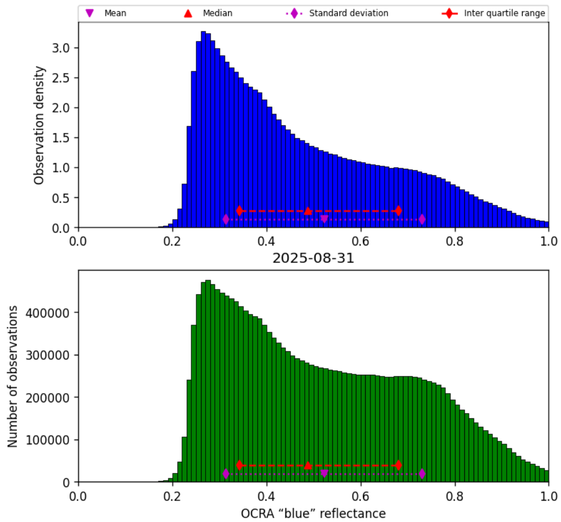
Figure 51: Histogram of “OCRA “blue” reflectance” for 2025-08-30 to 2025-09-01
