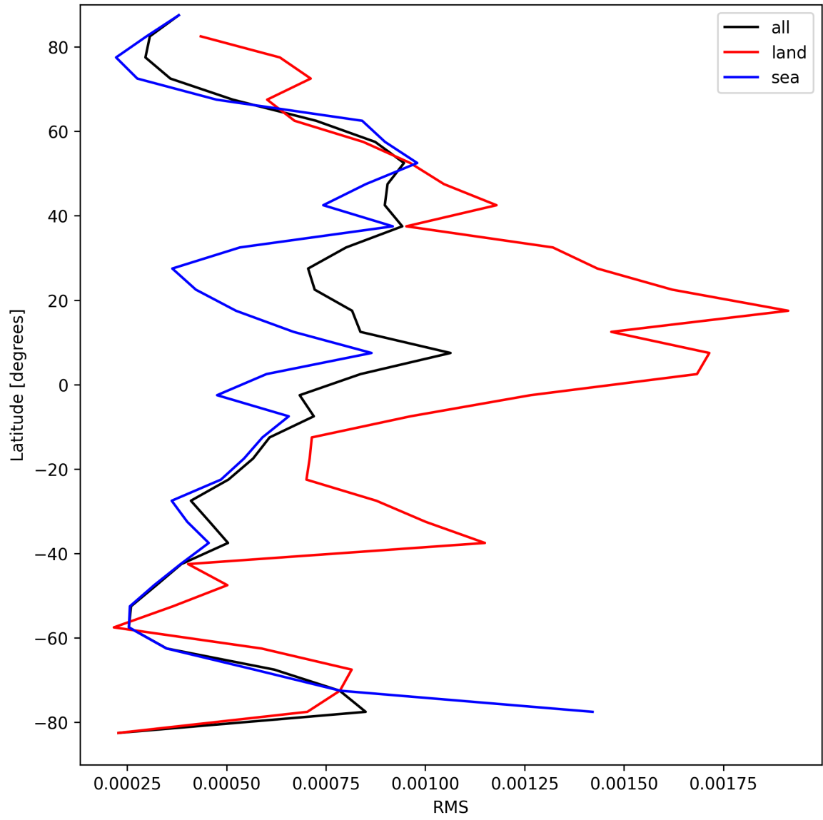
Figure 31: Zonal average of “RMS” for 2025-08-30 to 2025-09-01.
