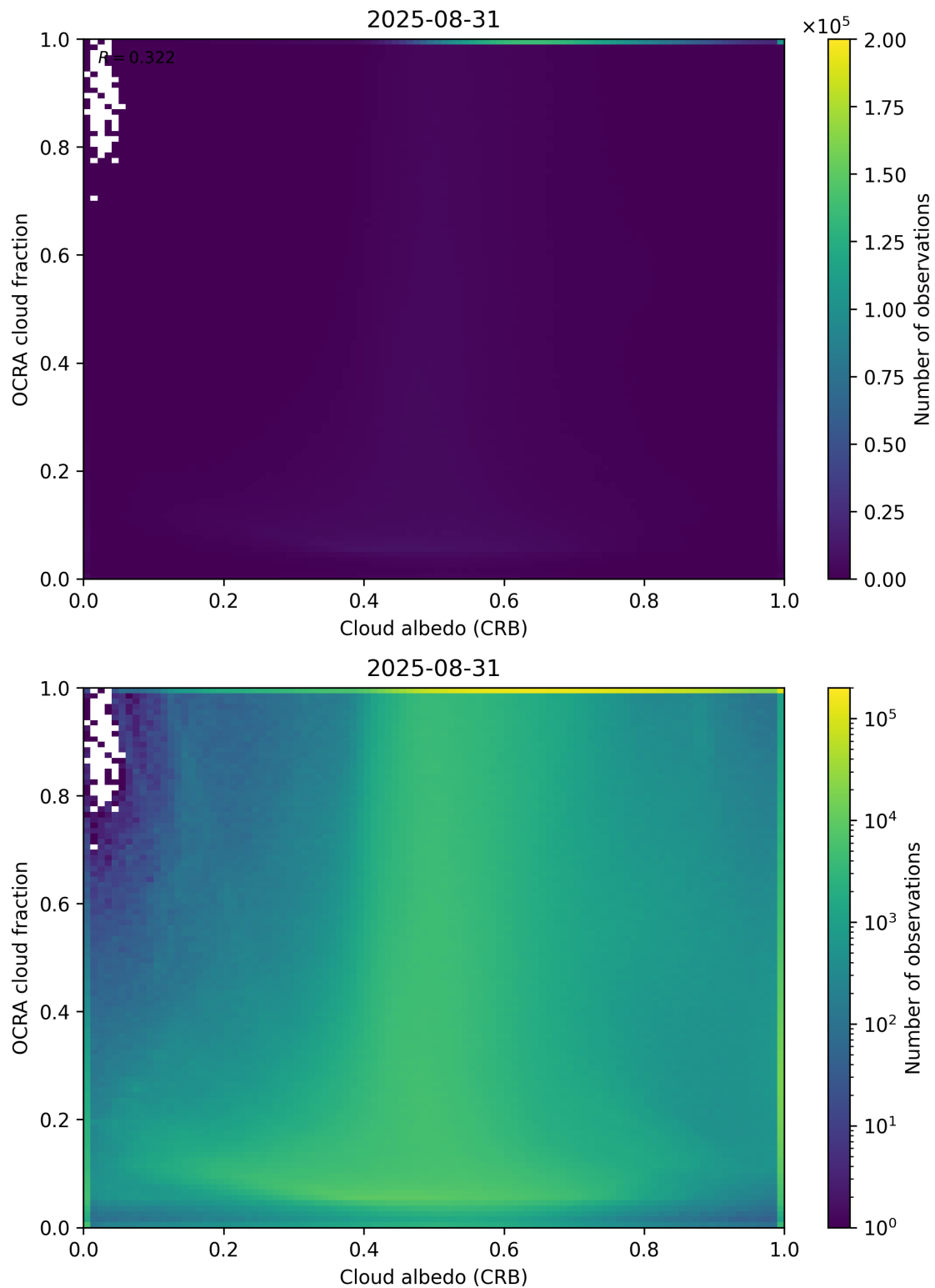
Figure 70: Scatter density plot of “Cloud albedo (CRB)” against “OCRA cloud fraction” for 2025-08-30 to 2025-09-01.
