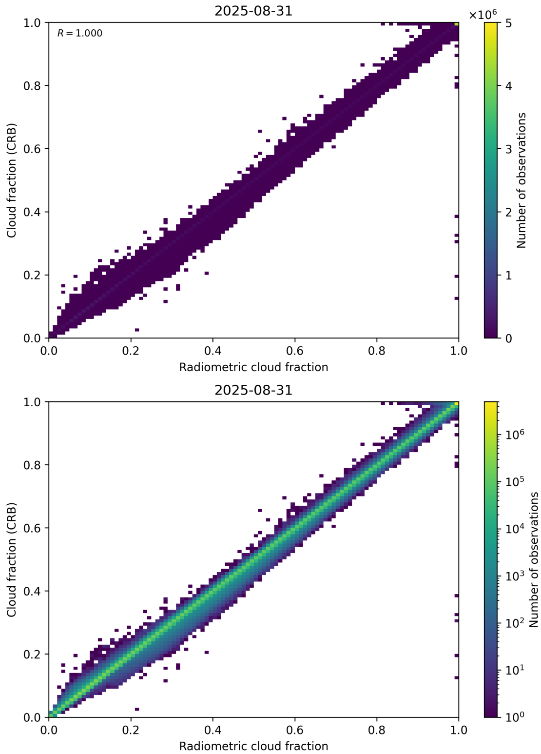
Figure 73: Scatter density plot of “Radiometric cloud fraction” against “Cloud fraction (CRB)” for 2025-08-30 to 2025-09-01.
