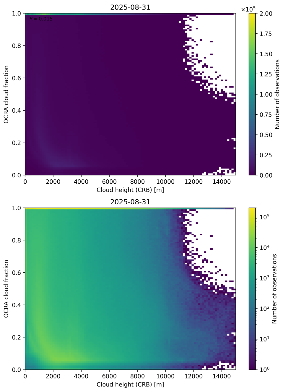
Figure 81: Scatter density plot of “Cloud height (CRB)” against “OCRA cloud fraction” for 2025-08-30 to 2025-09-01.
