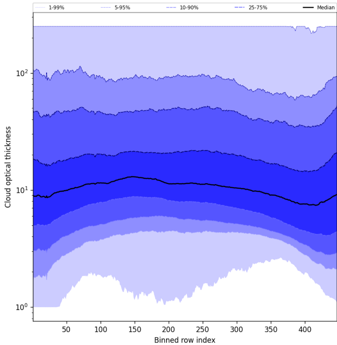
Figure 57: Along track statistics of “Cloud optical thickness” for 2025-08-30 to 2025-09-01
