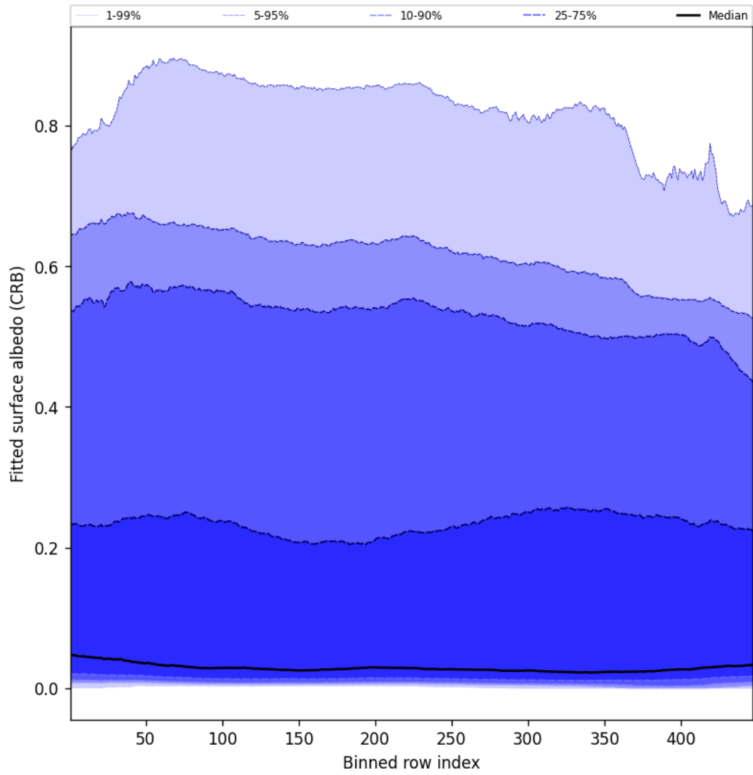
Figure 62: Along track statistics of “Fitted surface albedo (CRB)” for 2025-08-30 to 2025-09-01
