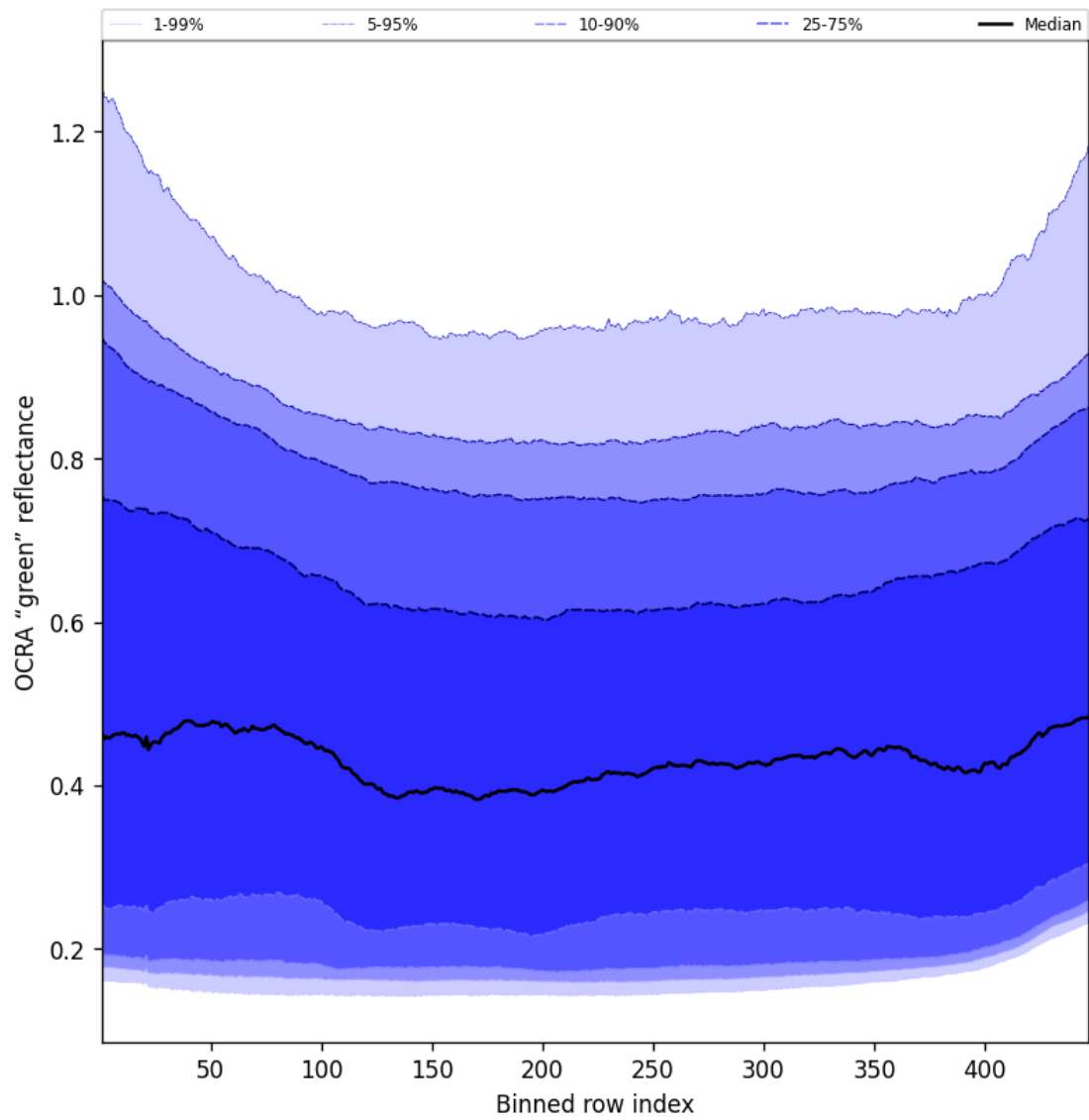
Figure 68: Along track statistics of “OCRA “green” reflectance” for 2025-08-30 to 2025-09-01
