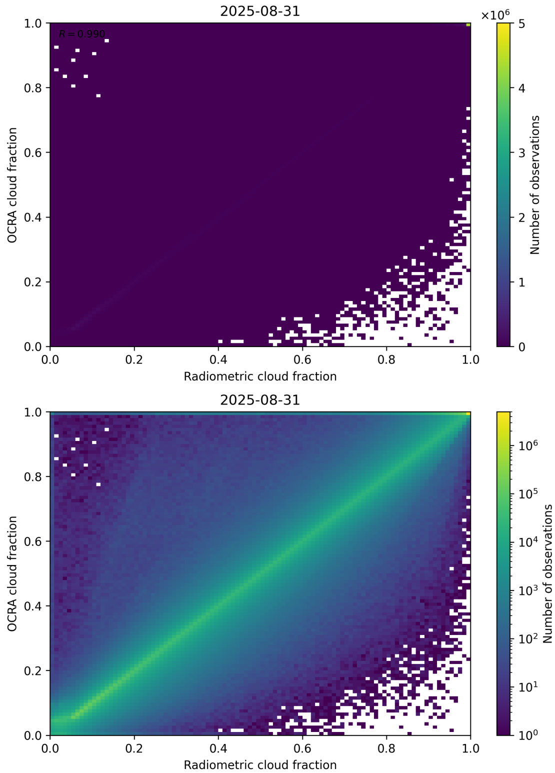
Figure 72: Scatter density plot of “Radiometric cloud fraction” against “OCRA cloud fraction” for 2025-08-30 to 2025-09-01.
