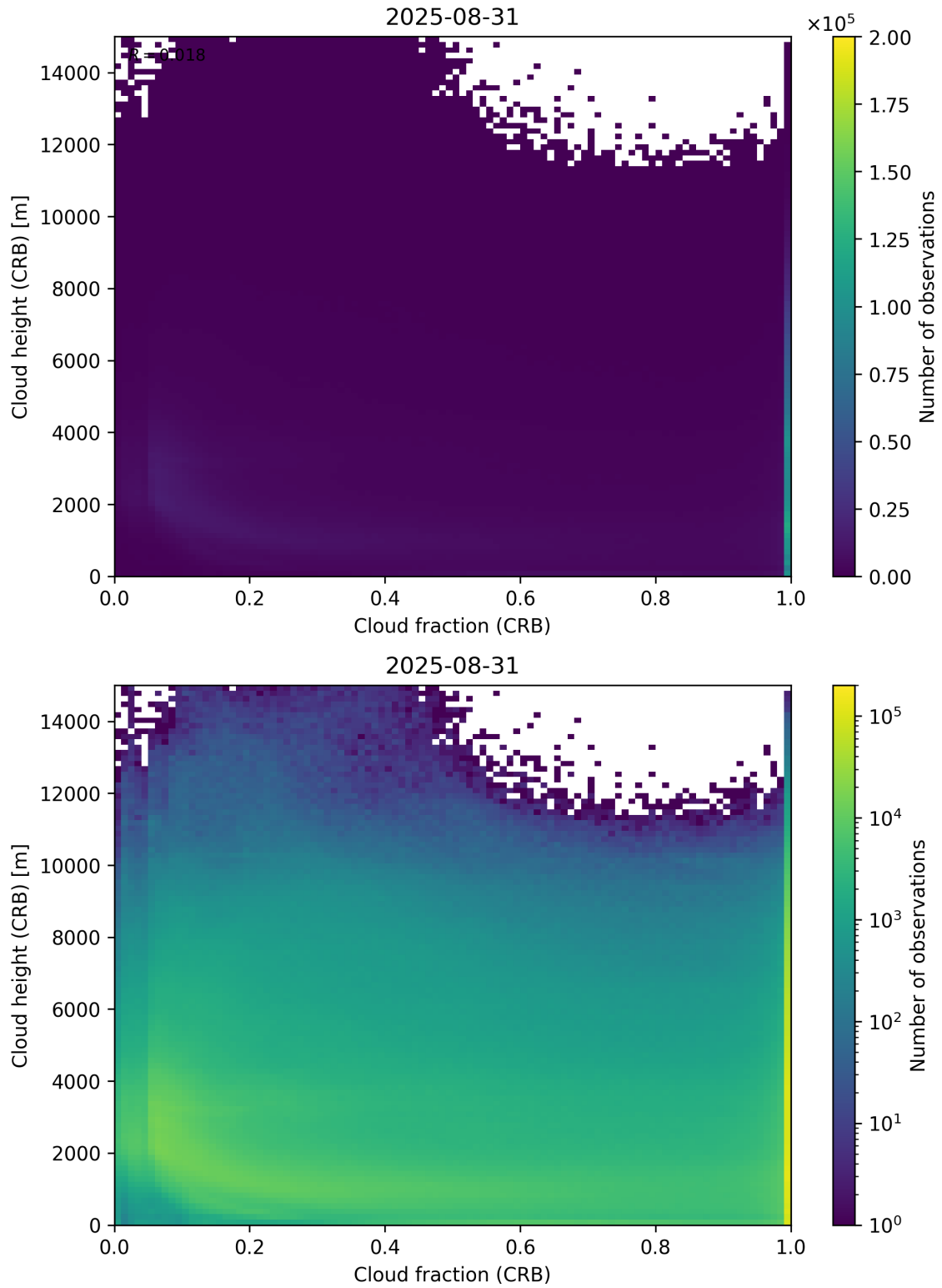
Figure 79: Scatter density plot of “Cloud fraction (CRB)” against “Cloud height (CRB)” for 2025-08-30 to 2025-09-01.
