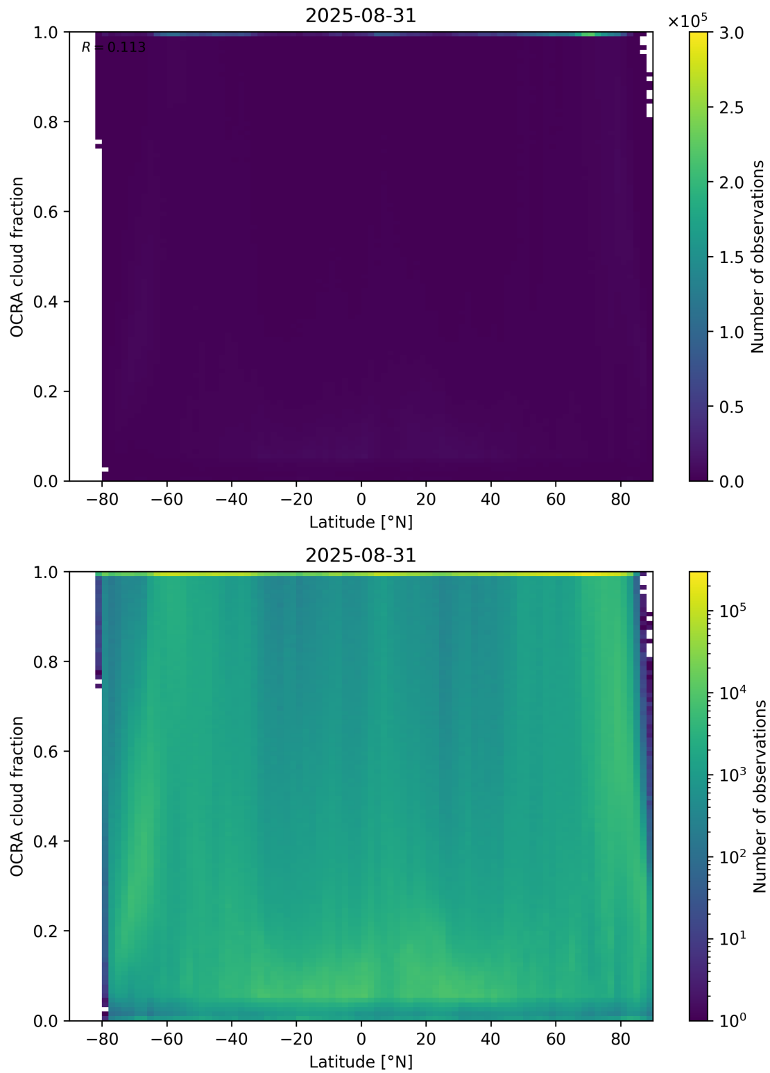
Figure 93: Scatter density plot of “Latitude” against “OCRA cloud fraction” for 2025-08-30 to 2025-09-01.
