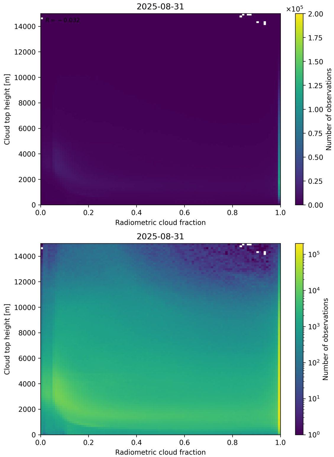
Figure 76: Scatter density plot of “Radiometric cloud fraction” against “Cloud top height” for 2025-08-30 to 2025-09-01.
