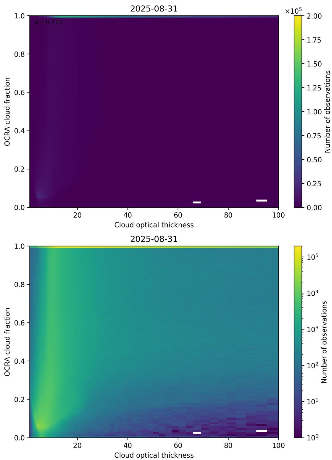
Figure 83: Scatter density plot of “Cloud optical thickness” against “OCRA cloud fraction” for 2025-08-30 to 2025-09-01.
