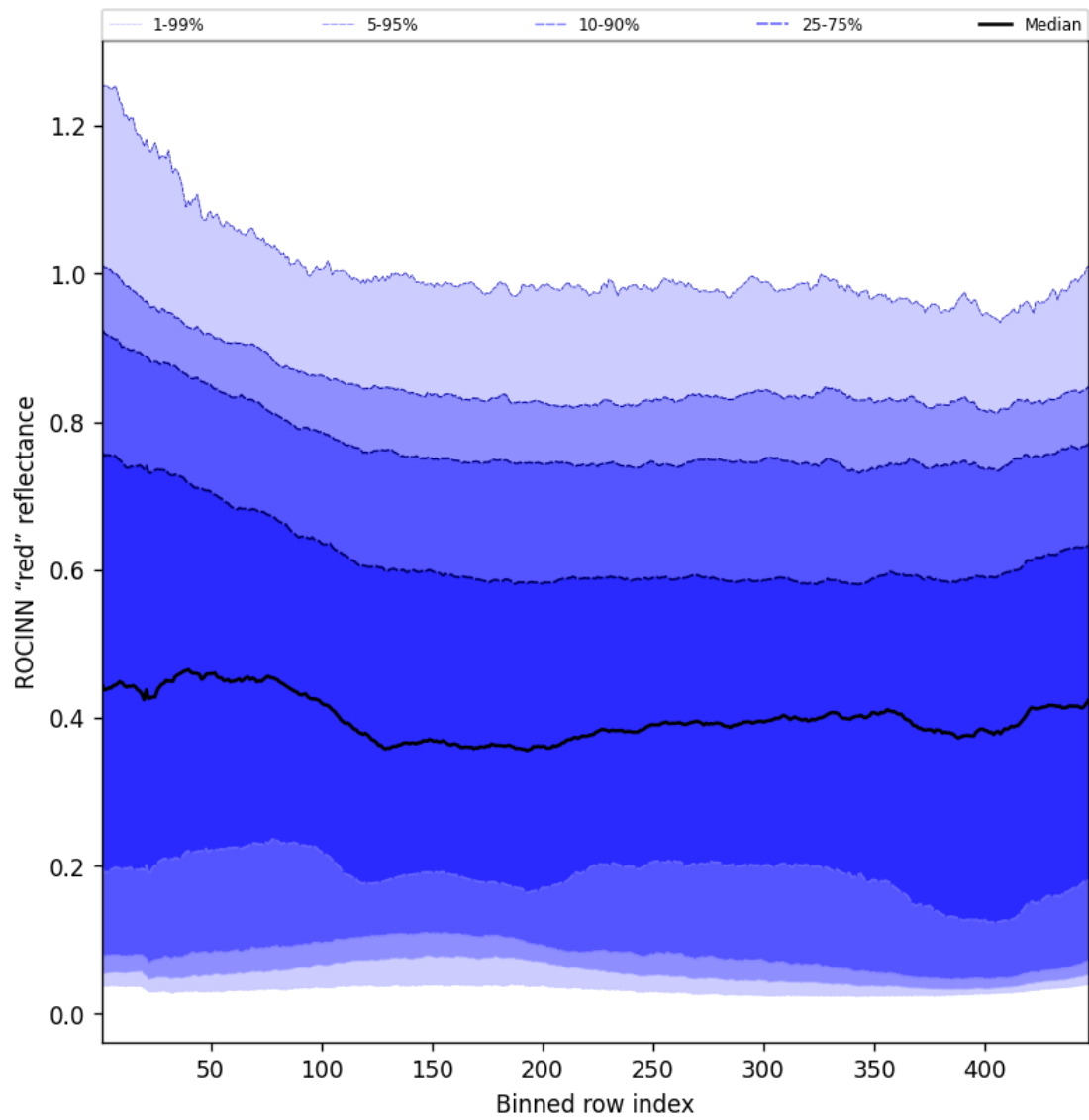
Figure 69: Along track statistics of “ROCINN “red” reflectance” for 2025-08-30 to 2025-09-01
