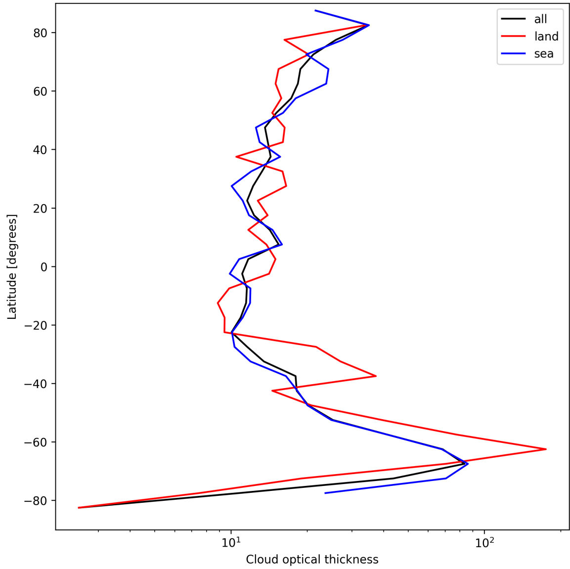
Figure 25: Zonal average of “Cloud optical thickness” for 2025-08-30 to 2025-09-01.
