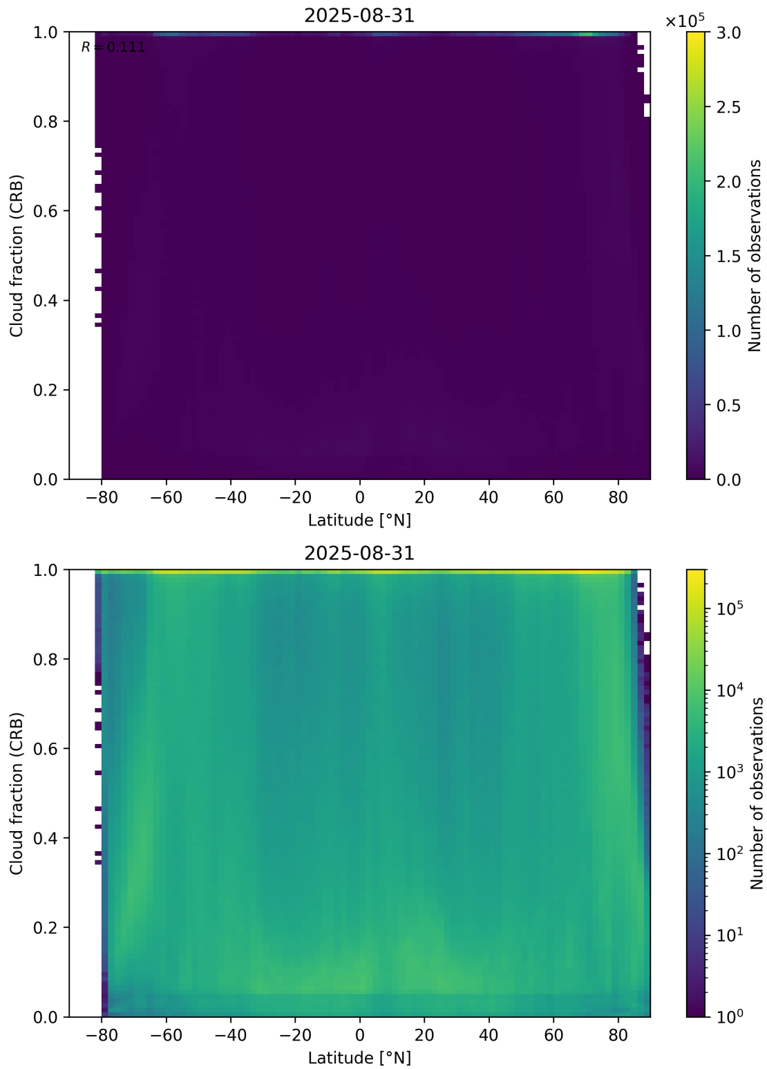
Figure 94: Scatter density plot of “Latitude” against “Cloud fraction (CRB)” for 2025-08-30 to 2025-09-01.
