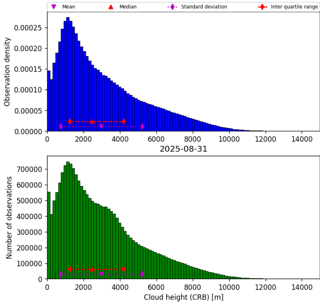
Figure 43: Histogram of “Cloud height (CRB)” for 2025-08-30 to 2025-09-01
