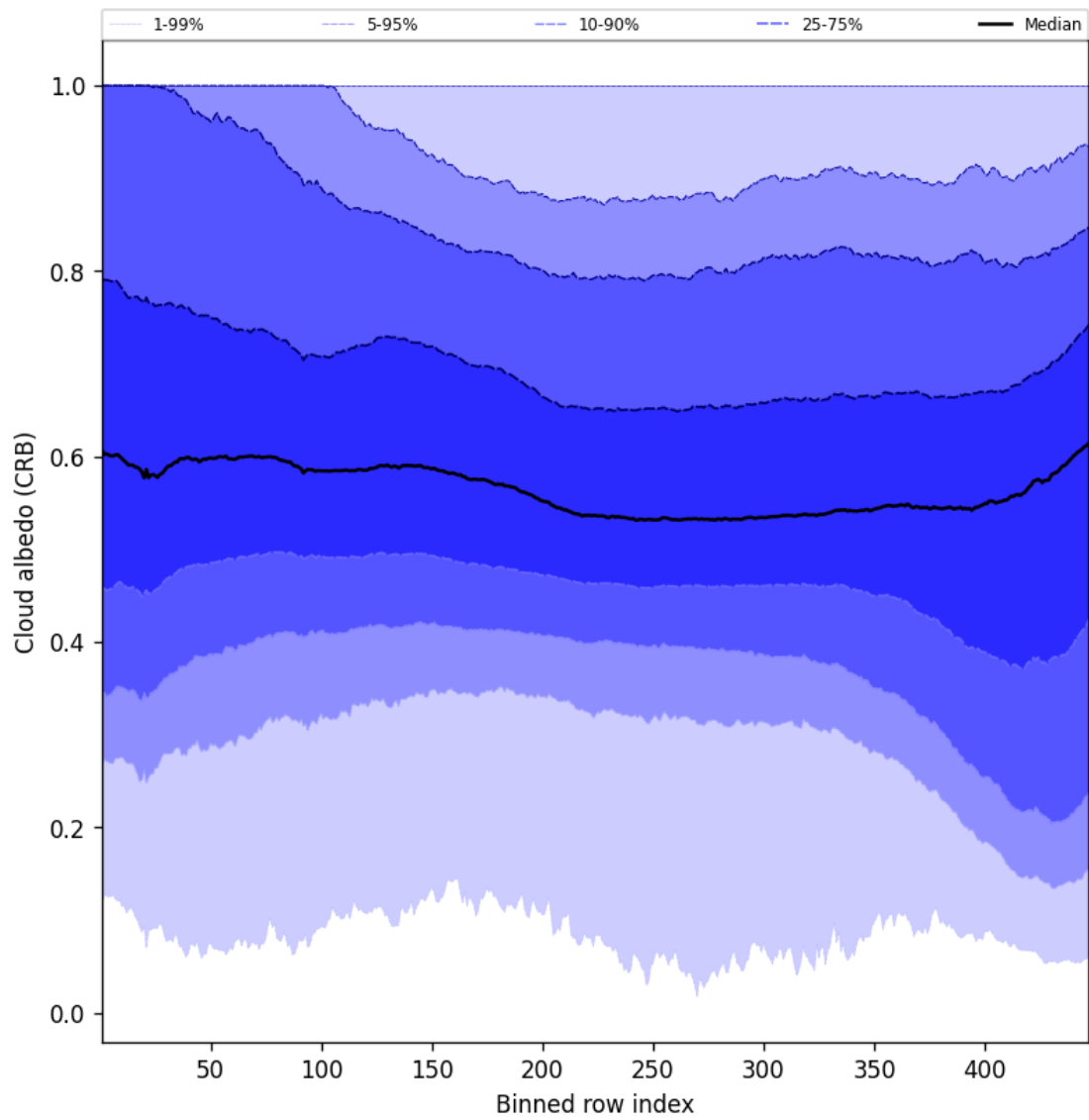
Figure 60: Along track statistics of “Cloud albedo (CRB)” for 2025-08-30 to 2025-09-01
