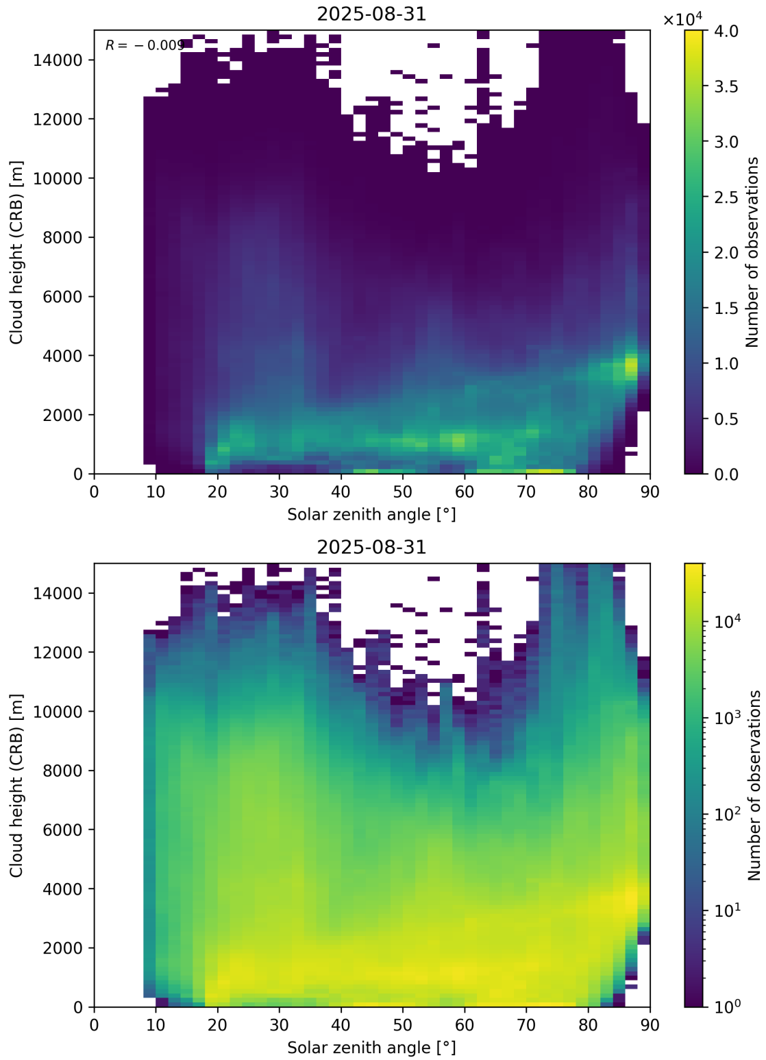
Figure 102: Scatter density plot of “Solar zenith angle” against “Cloud height (CRB)” for 2025-08-30 to 2025-09-01.
