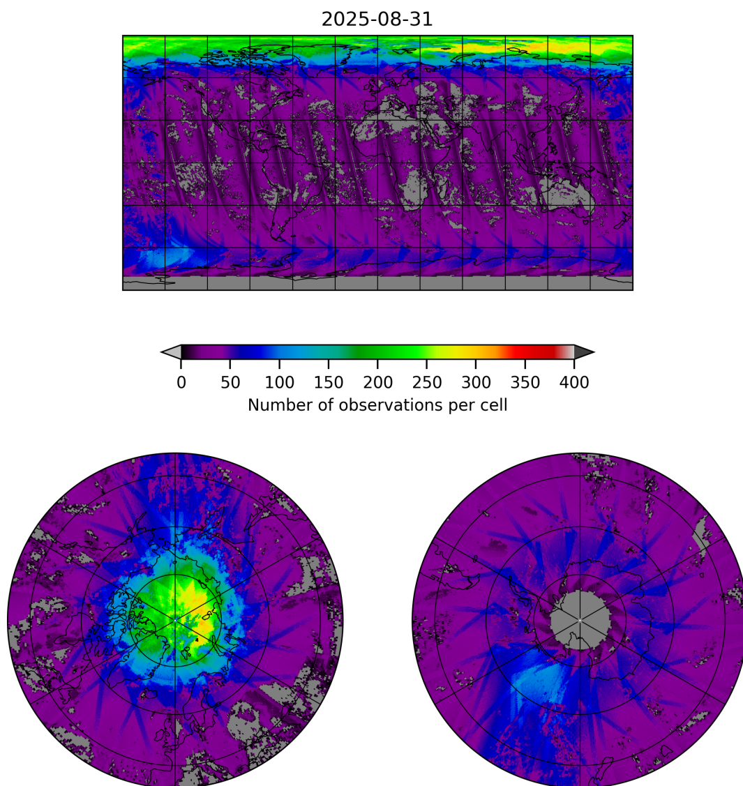
Figure 21: Map of the number of observations for 2025-08-30 to 2025-09-01
