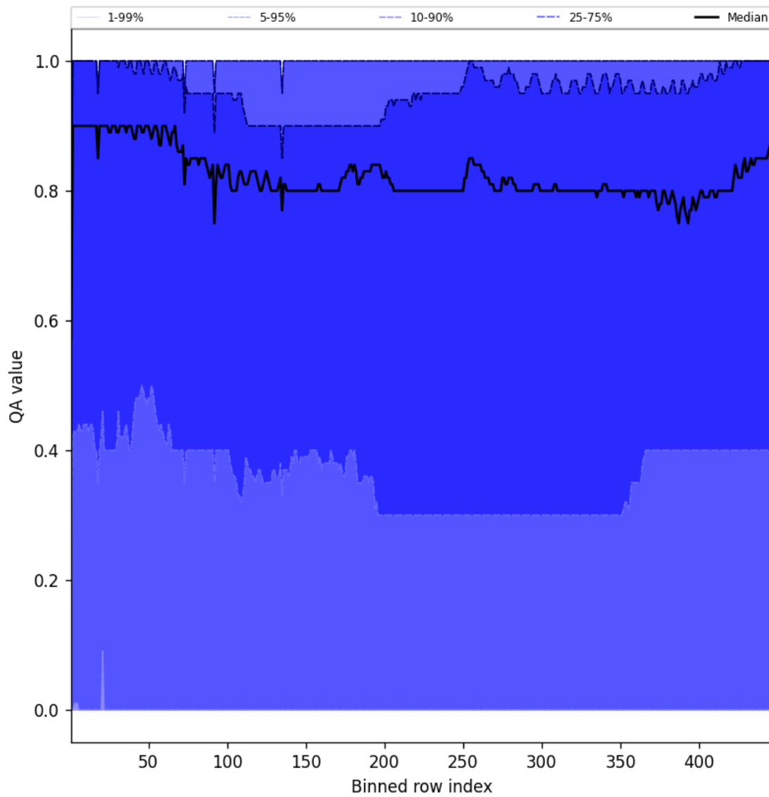
Figure 54: Along track statistics of “QA value” for 2025-08-30 to 2025-09-01
