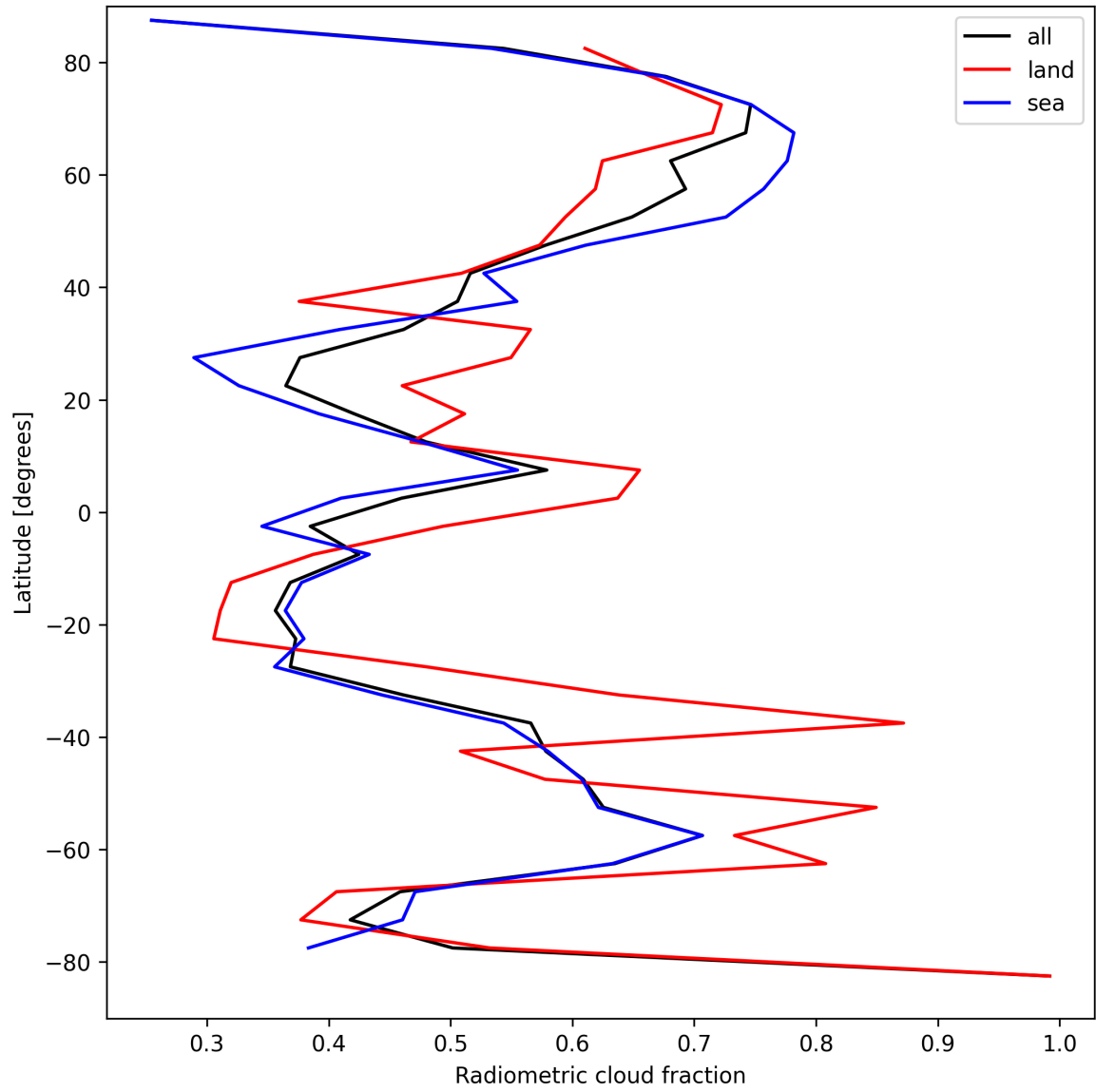
Figure 23: Zonal average of “Radiometric cloud fraction” for 2025-08-30 to 2025-09-01.
