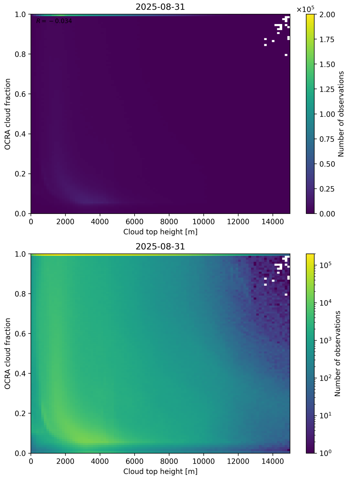
Figure 87: Scatter density plot of “Cloud top height” against “OCRA cloud fraction” for 2025-08-30 to 2025-09-01.
