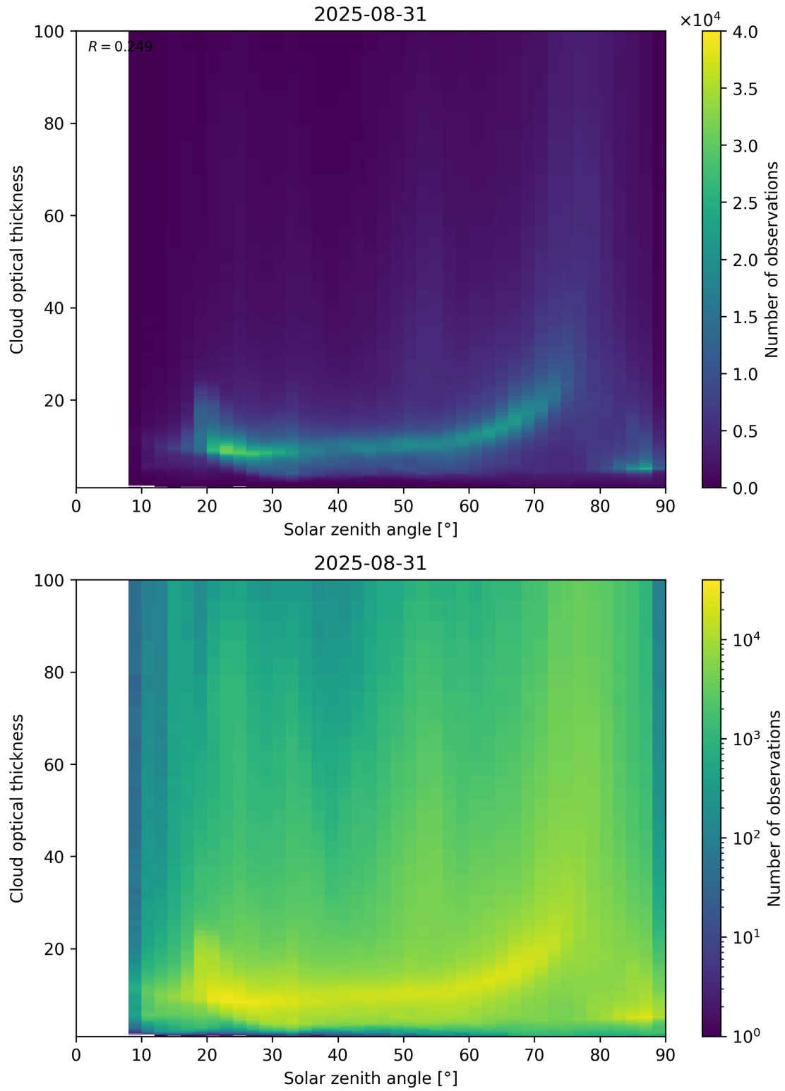
Figure 103: Scatter density plot of “Solar zenith angle” against “Cloud optical thickness” for 2025-08-30 to 2025-09-01.
