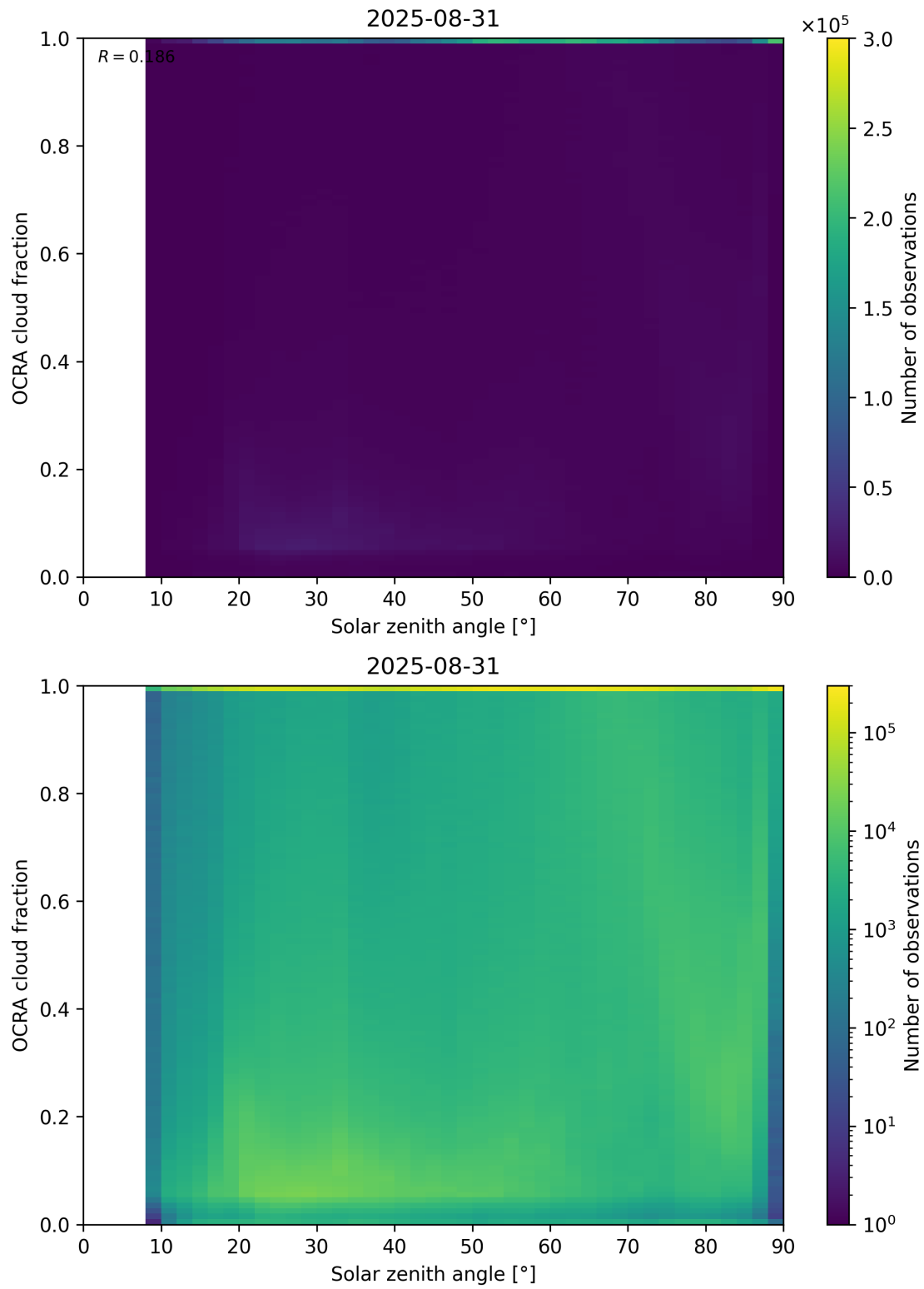
Figure 100: Scatter density plot of “Solar zenith angle” against “OCRA cloud fraction” for 2025-08-30 to 2025-09-01.
