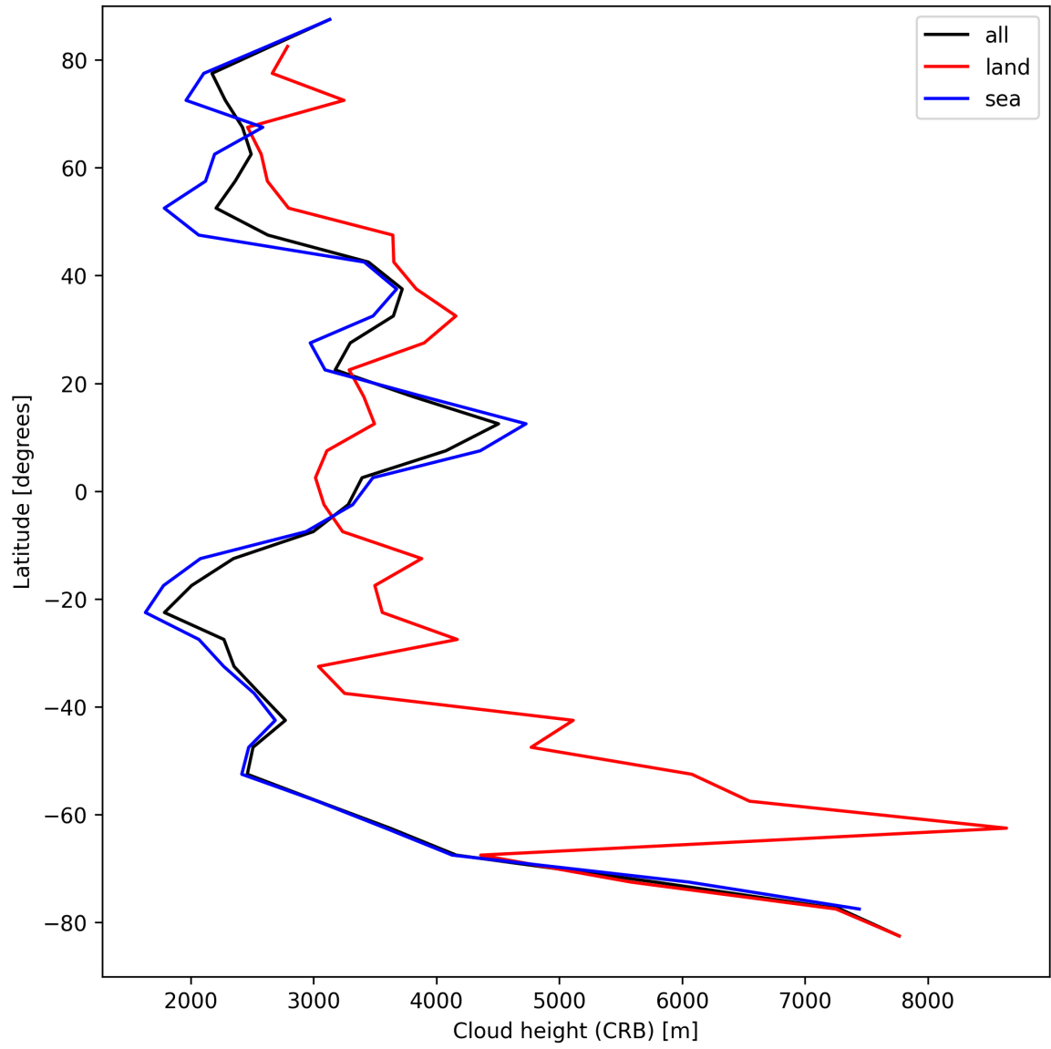
Figure 27: Zonal average of “Cloud height (CRB)” for 2025-08-30 to 2025-09-01.
