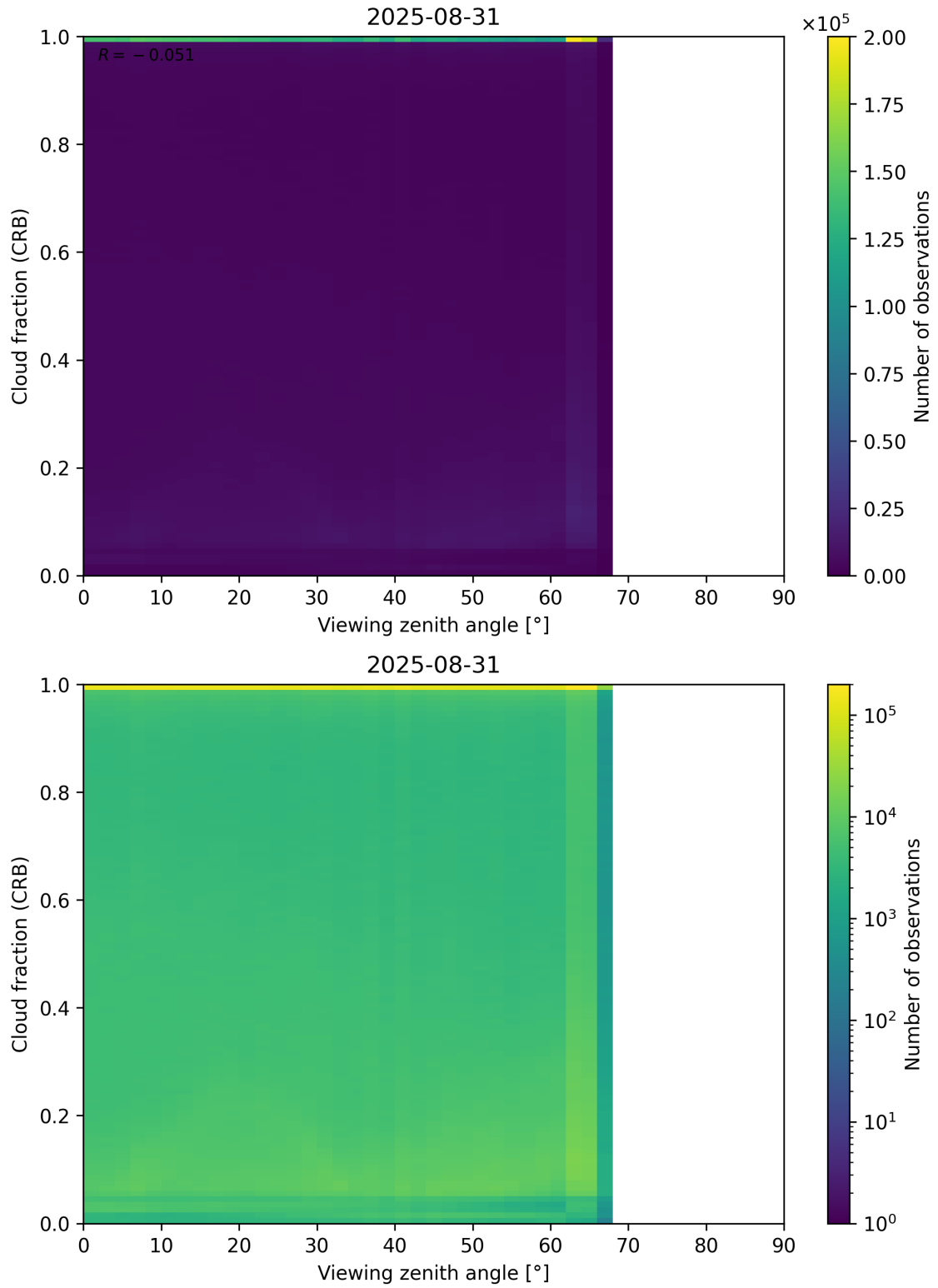
Figure 109: Scatter density plot of “Viewing zenith angle” against “Cloud fraction (CRB)” for 2025-08-30 to 2025-09-01.
