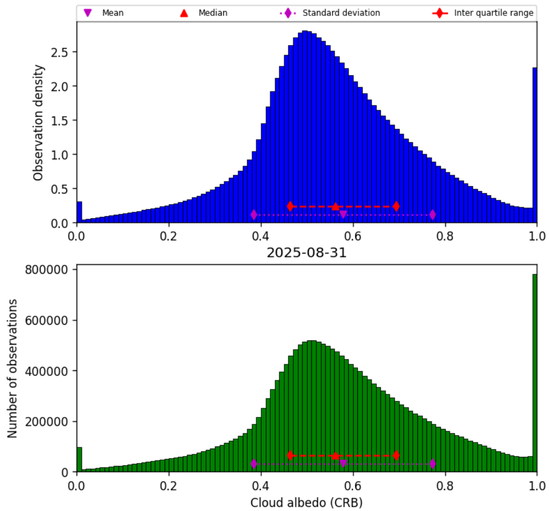
Figure 44: Histogram of “Cloud albedo (CRB)” for 2025-08-30 to 2025-09-01
