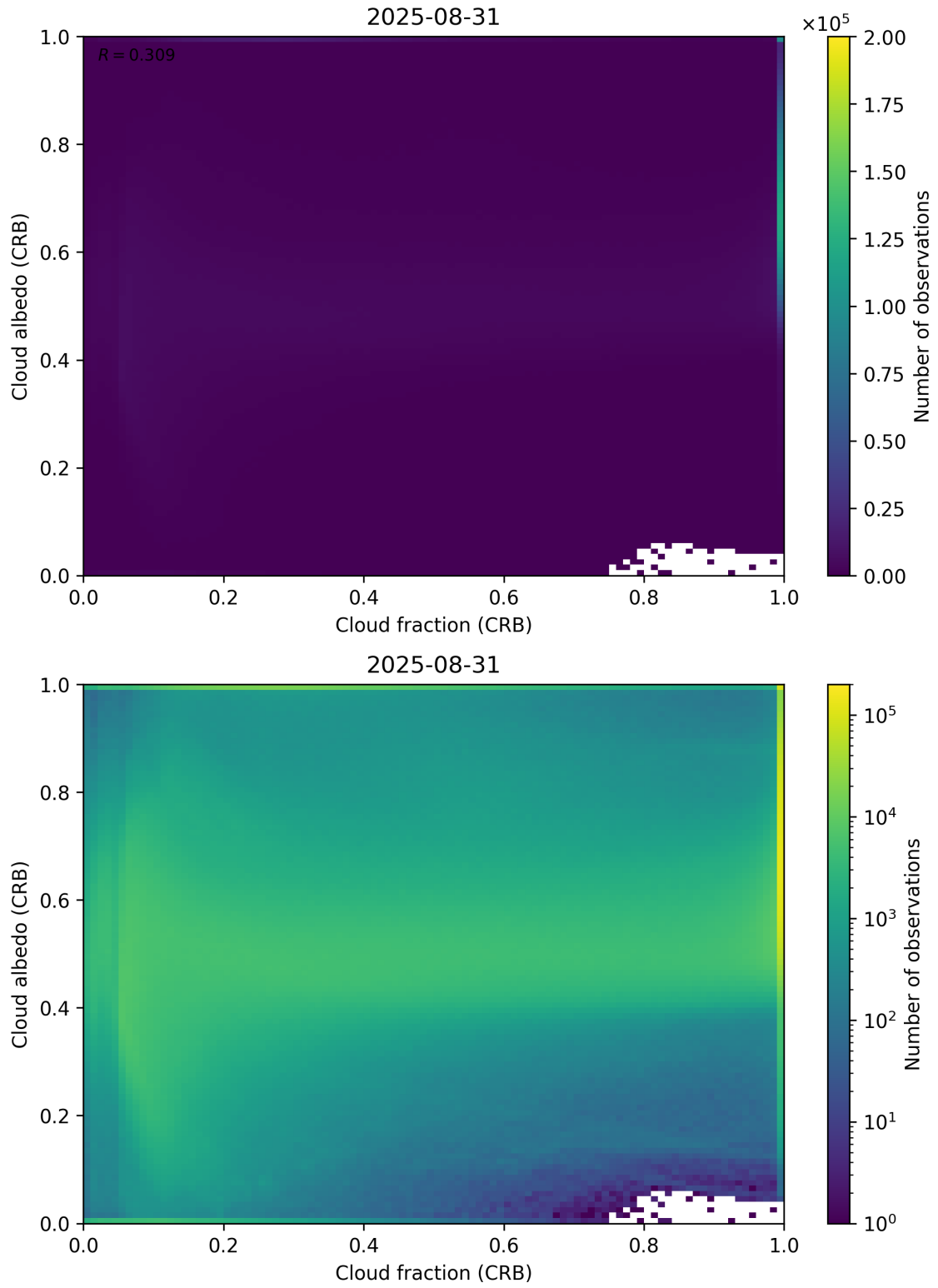
Figure 77: Scatter density plot of “Cloud fraction (CRB)” against “Cloud albedo (CRB)” for 2025-08-30 to 2025-09-01.
