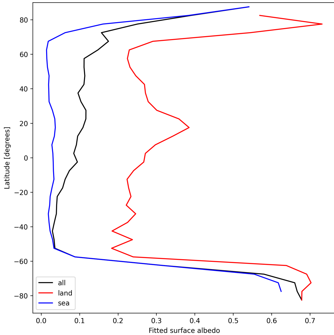
Figure 29: Zonal average of “Fitted surface albedo” for 2025-08-30 to 2025-09-01.
