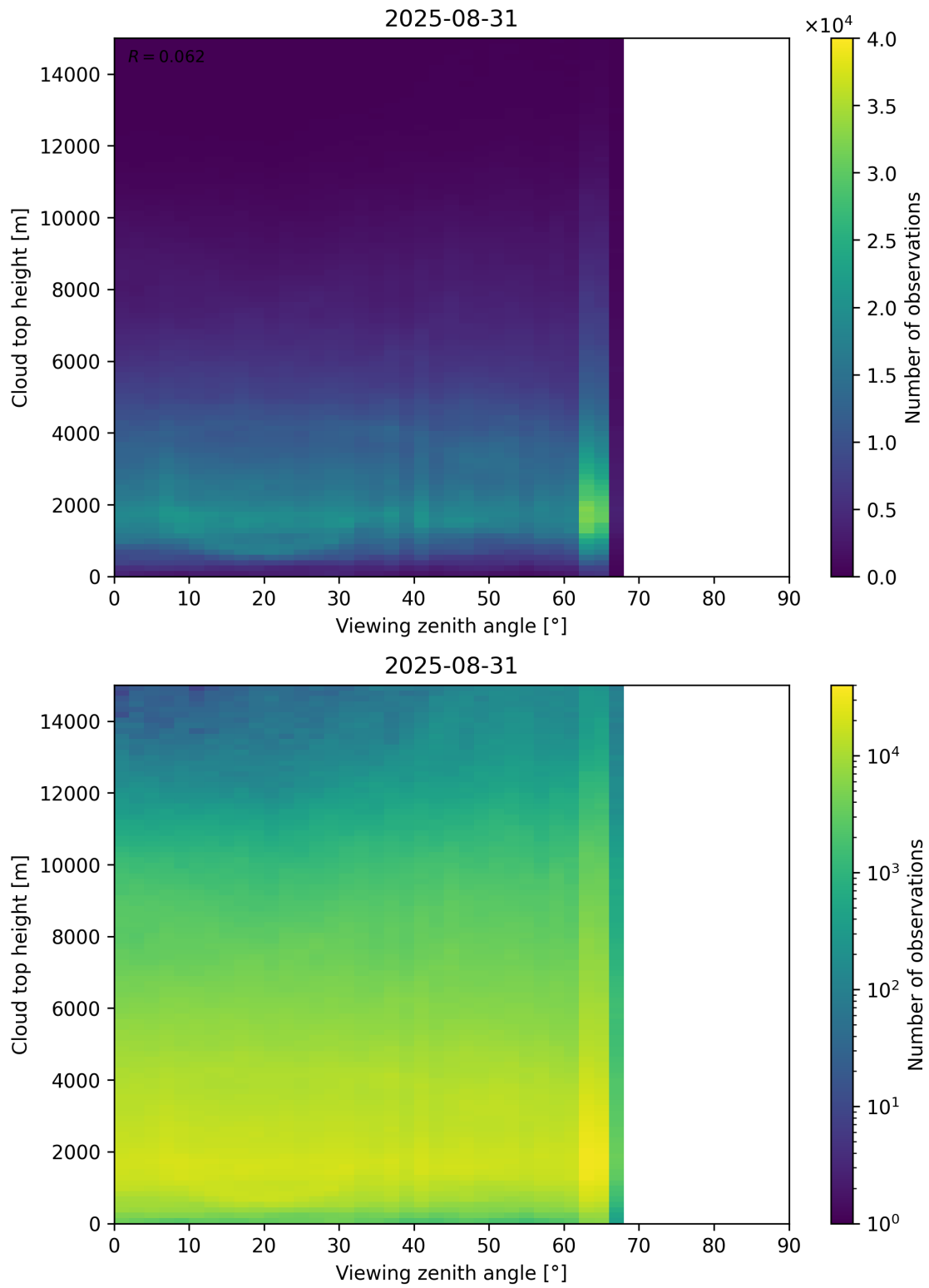
Figure 112: Scatter density plot of “Viewing zenith angle” against “Cloud top height” for 2025-08-30 to 2025-09-01.
