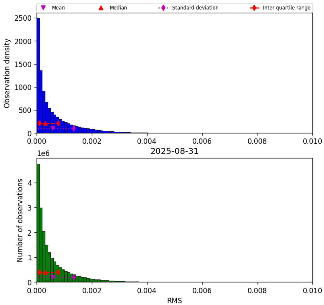
Figure 47: Histogram of “RMS” for 2025-08-30 to 2025-09-01
