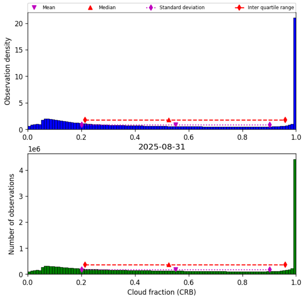
Figure 42: Histogram of “Cloud fraction (CRB)” for 2025-08-30 to 2025-09-01
