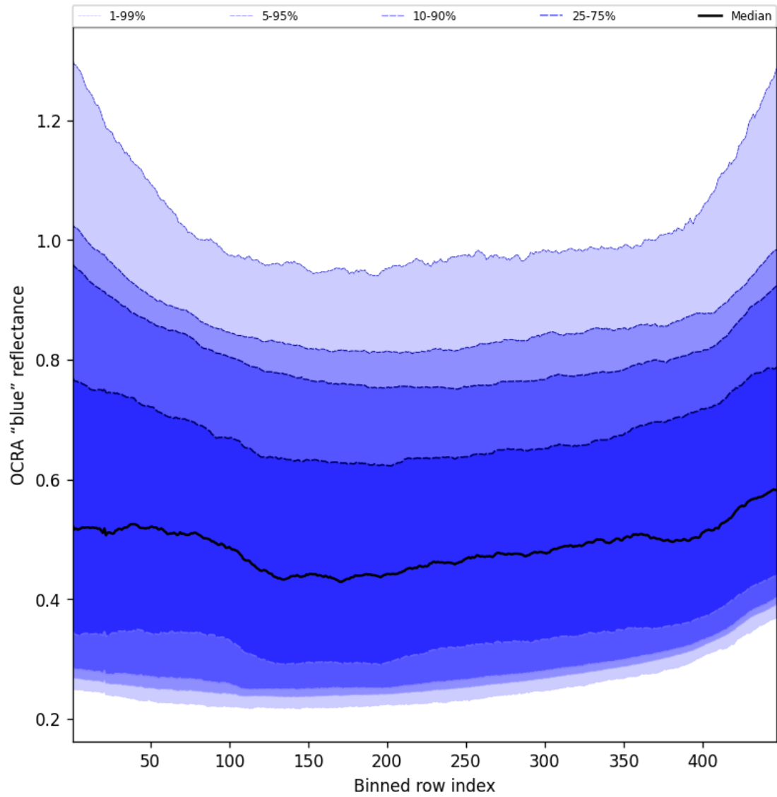
Figure 67: Along track statistics of “OCRA “blue” reflectance” for 2025-08-30 to 2025-09-01
