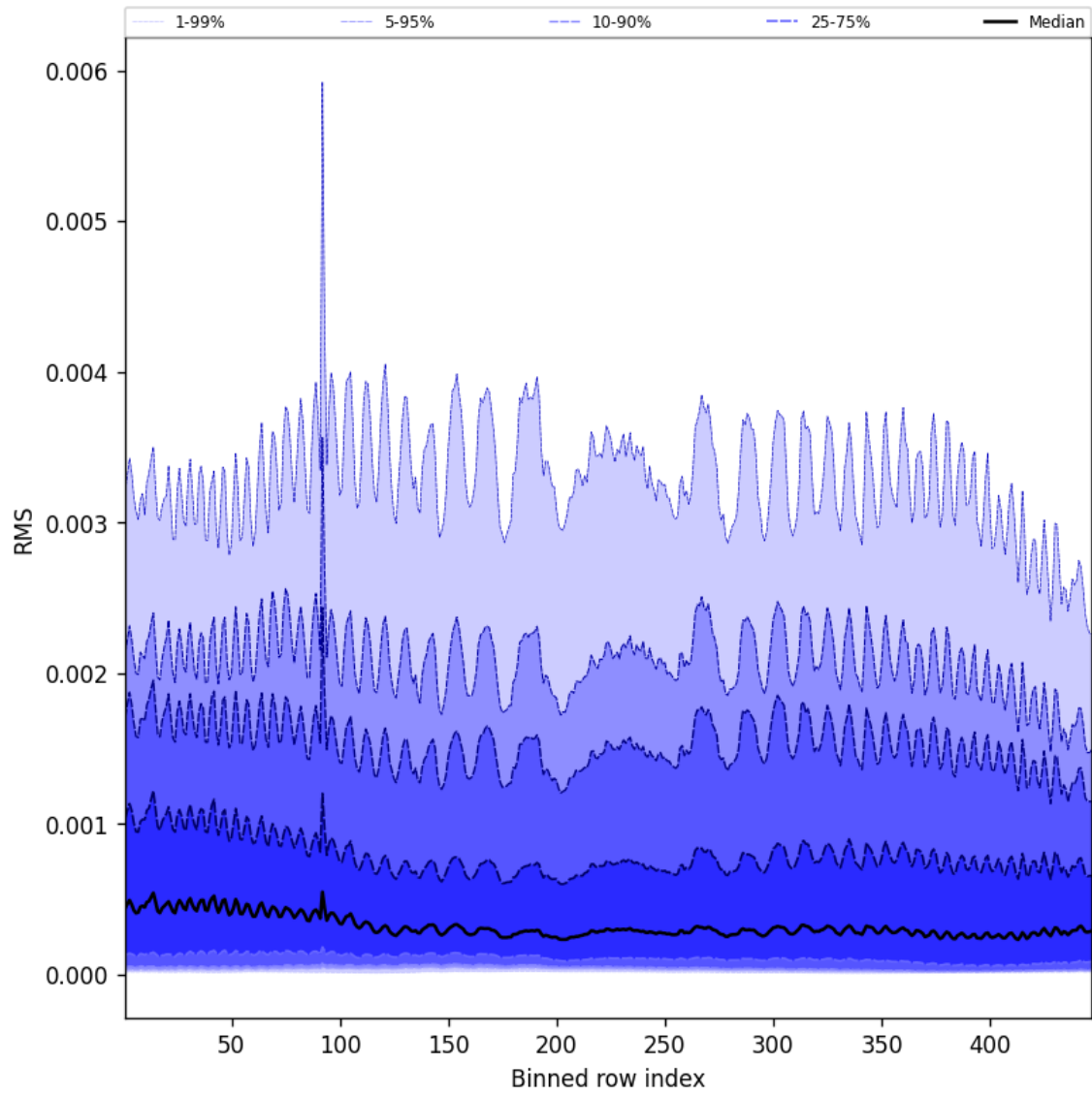
Figure 63: Along track statistics of “RMS” for 2025-08-30 to 2025-09-01
