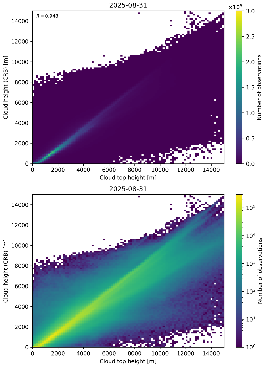
Figure 89: Scatter density plot of “Cloud top height” against “Cloud height (CRB)” for 2025-08-30 to 2025-09-01.
