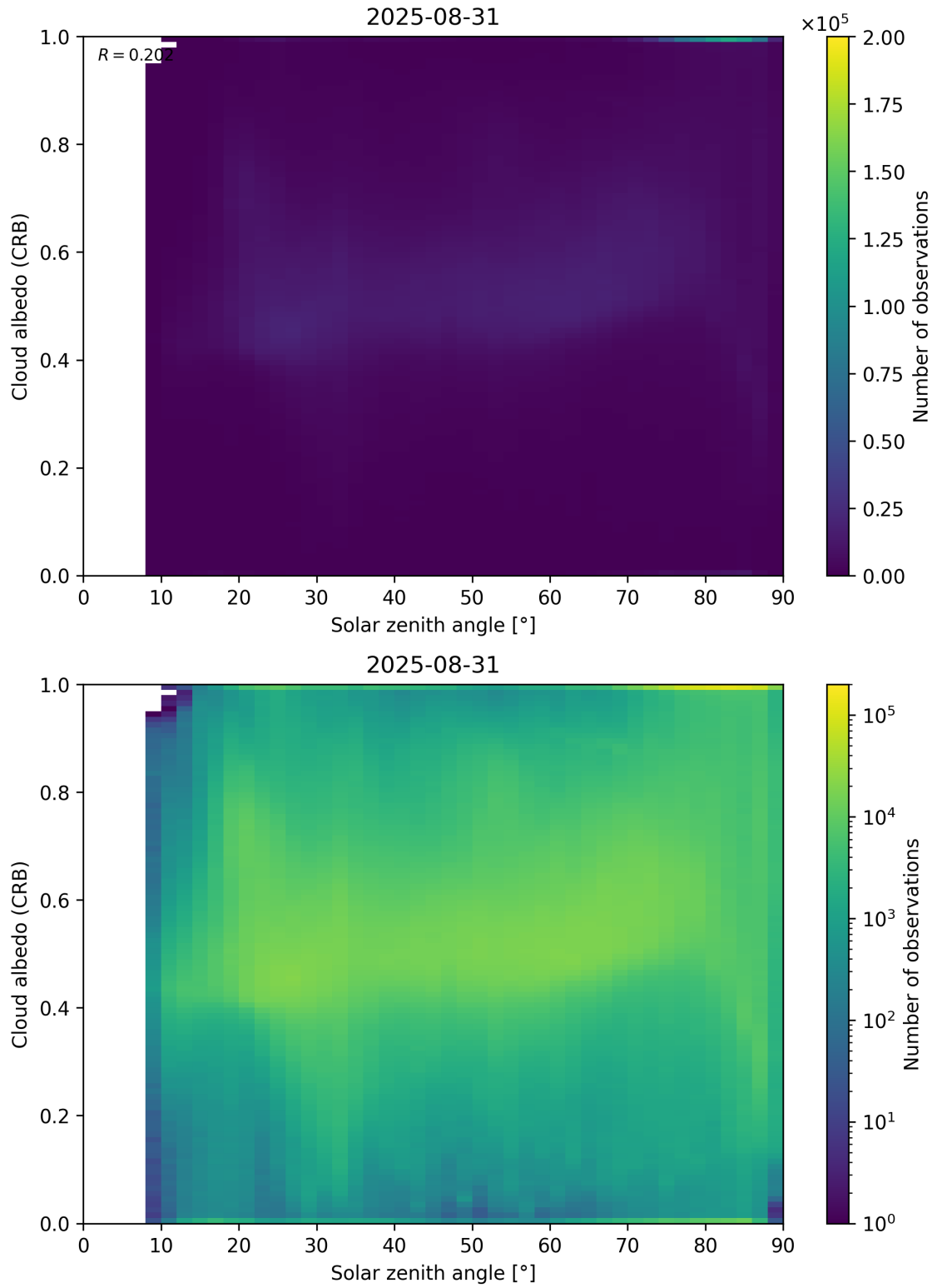
Figure 98: Scatter density plot of “Solar zenith angle” against “Cloud albedo (CRB)” for 2025-08-30 to 2025-09-01.
