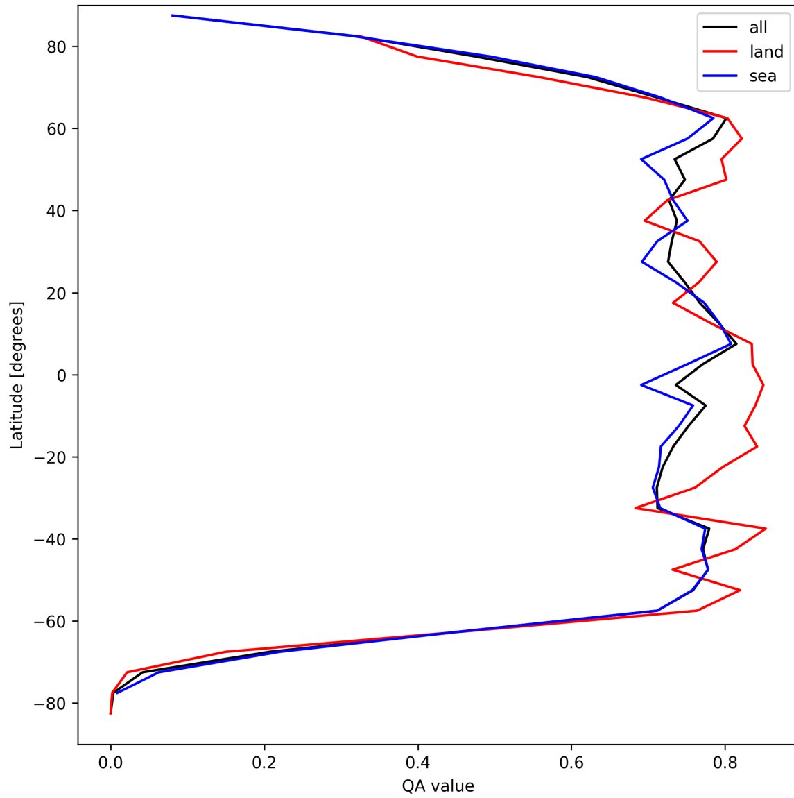
Figure 22: Zonal average of “QA value” for 2025-08-30 to 2025-09-01.
