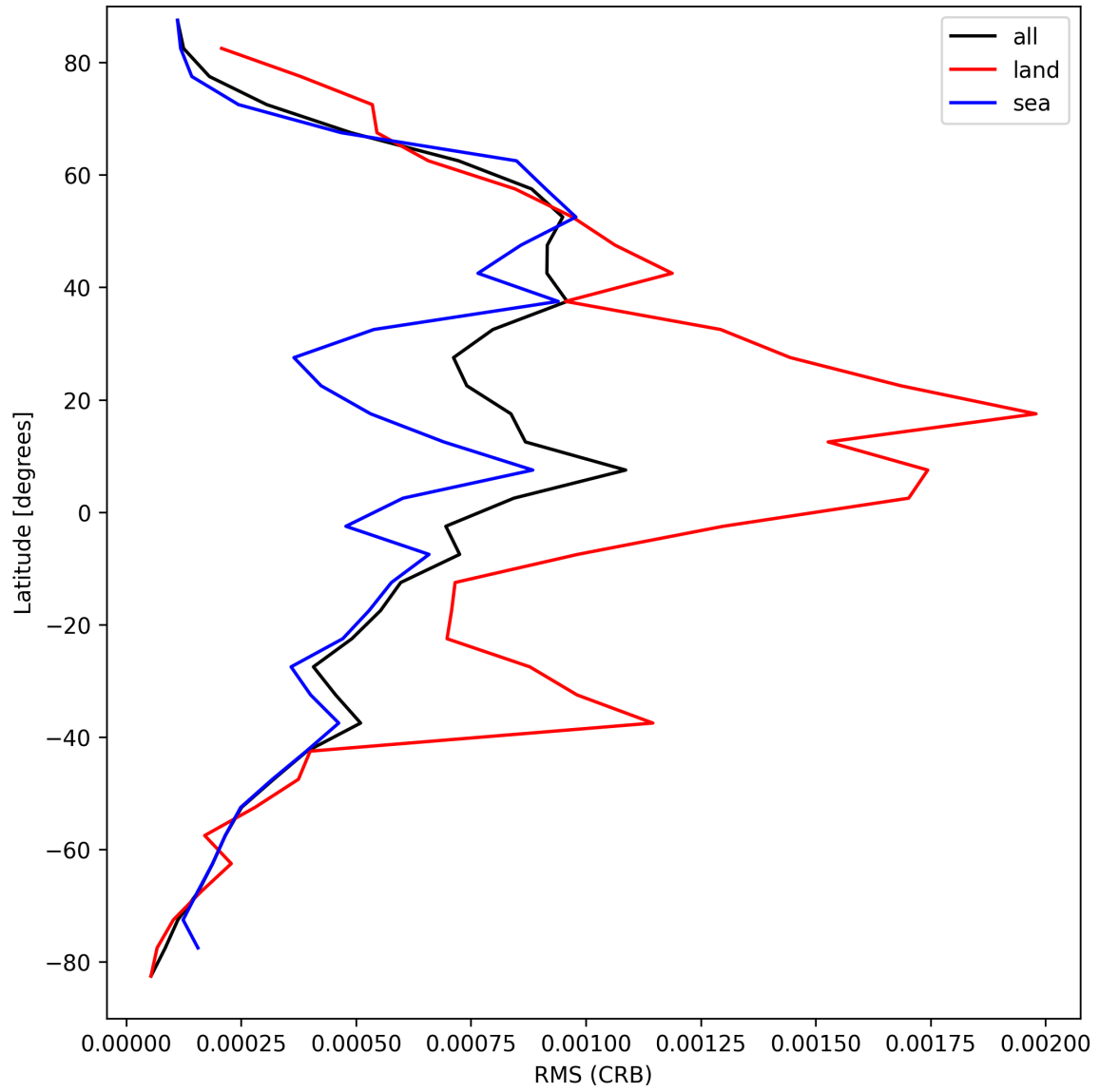
Figure 32: Zonal average of “RMS (CRB)” for 2025-08-30 to 2025-09-01.
