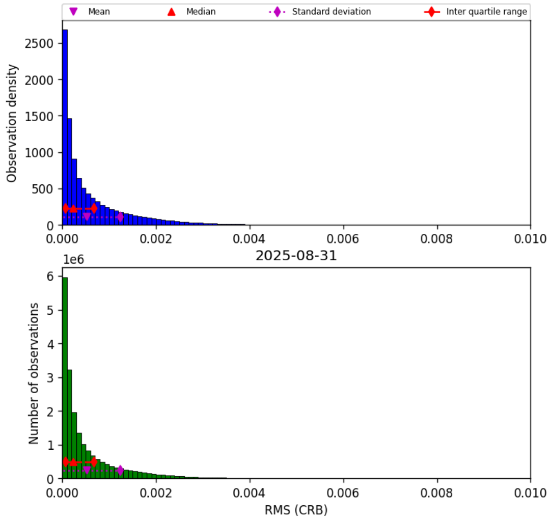
Figure 48: Histogram of “RMS (CRB)” for 2025-08-30 to 2025-09-01
