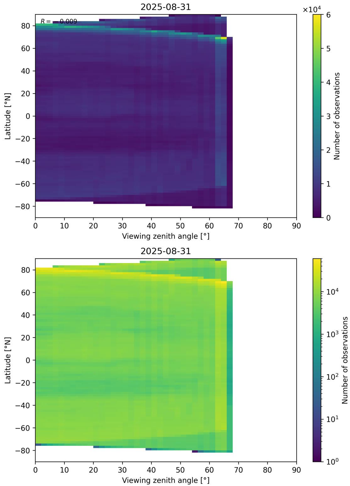
Figure 113: Scatter density plot of “Viewing zenith angle” against “Latitude” for 2025-08-30 to 2025-09-01.
