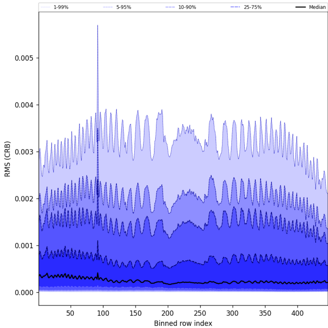
Figure 64: Along track statistics of “RMS (CRB)” for 2025-08-30 to 2025-09-01
