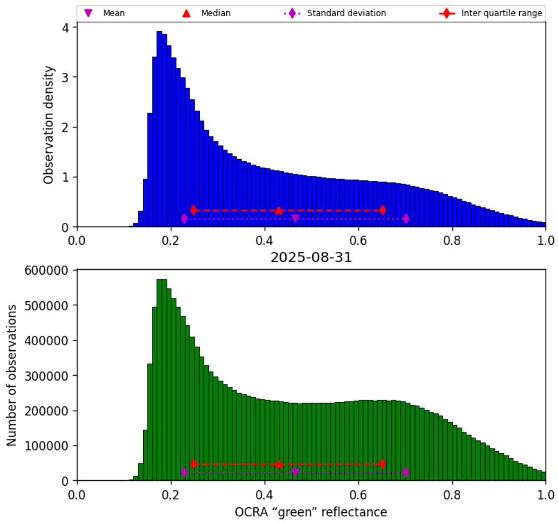
Figure 52: Histogram of “OCRA “green” reflectance” for 2025-08-30 to 2025-09-01
