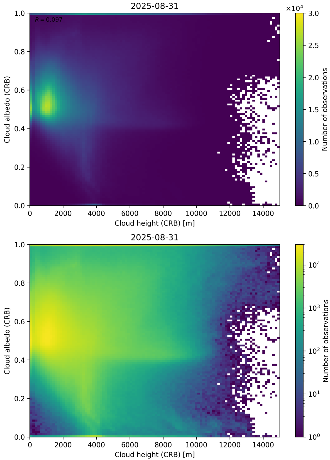
Figure 80: Scatter density plot of “Cloud height (CRB)” against “Cloud albedo (CRB)” for 2025-08-30 to 2025-09-01.
