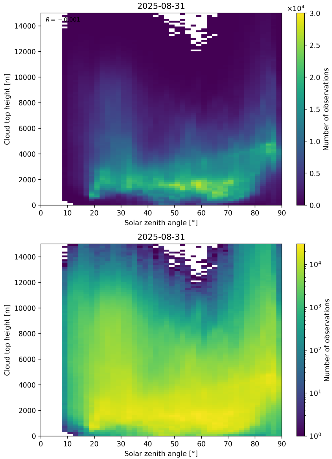
Figure 104: Scatter density plot of “Solar zenith angle” against “Cloud top height” for 2025-08-30 to 2025-09-01.
