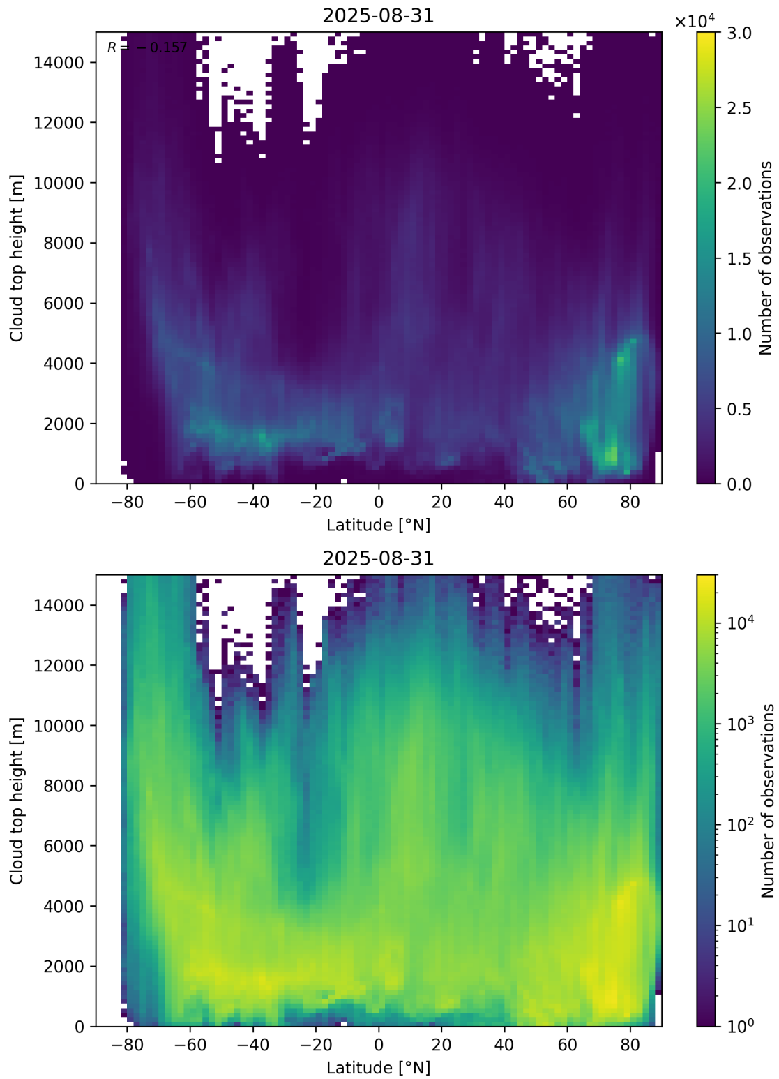
Figure 97: Scatter density plot of “Latitude” against “Cloud top height” for 2025-08-30 to 2025-09-01.
