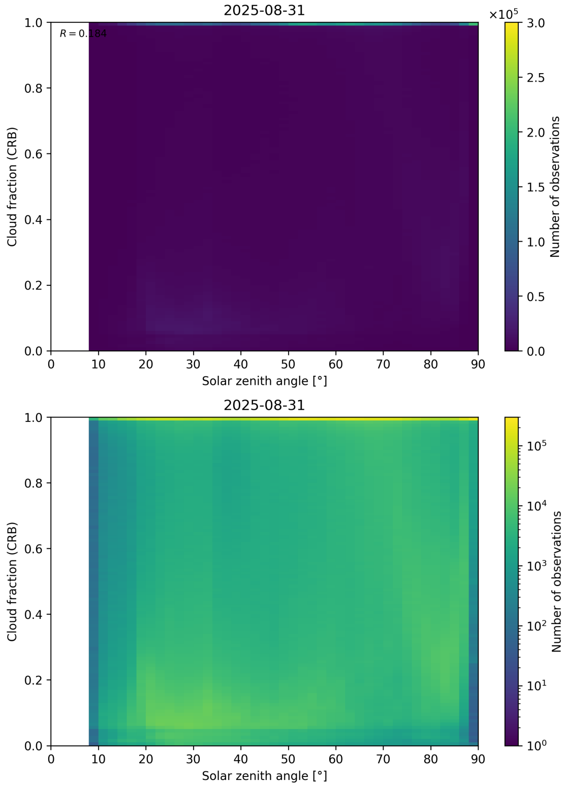
Figure 101: Scatter density plot of “Solar zenith angle” against “Cloud fraction (CRB)” for 2025-08-30 to 2025-09-01.
