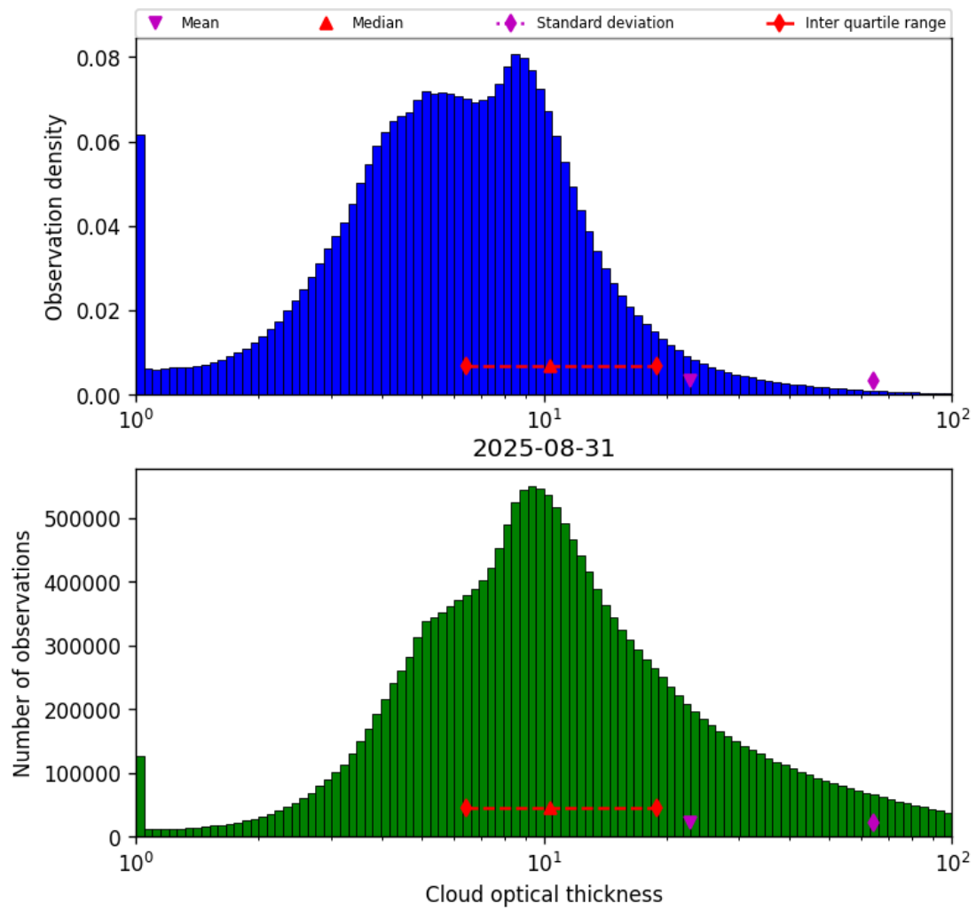
Figure 41: Histogram of “Cloud optical thickness” for 2025-08-30 to 2025-09-01
