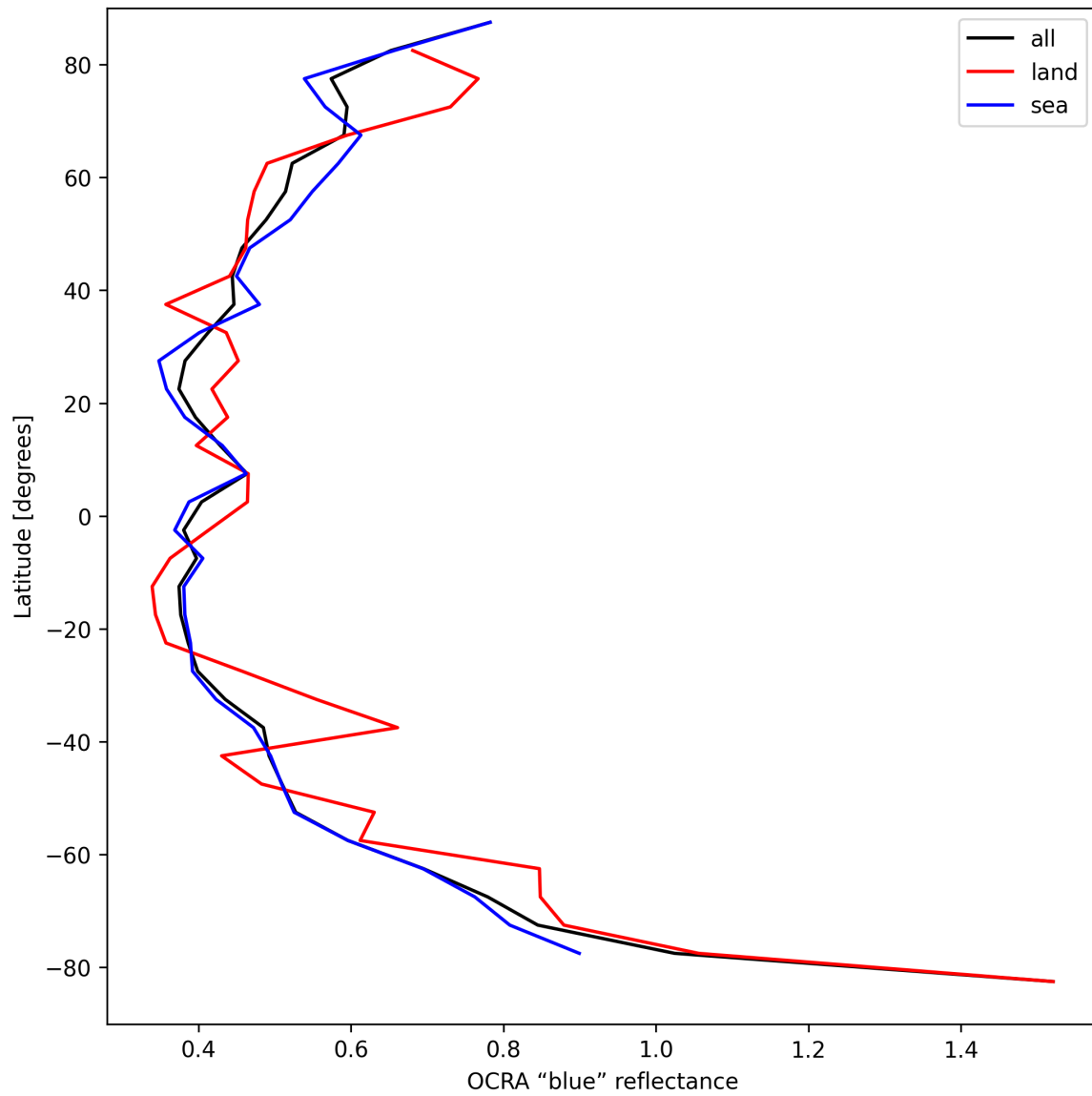
Figure 35: Zonal average of “OCRA “blue” reflectance” for 2025-08-30 to 2025-09-01.
