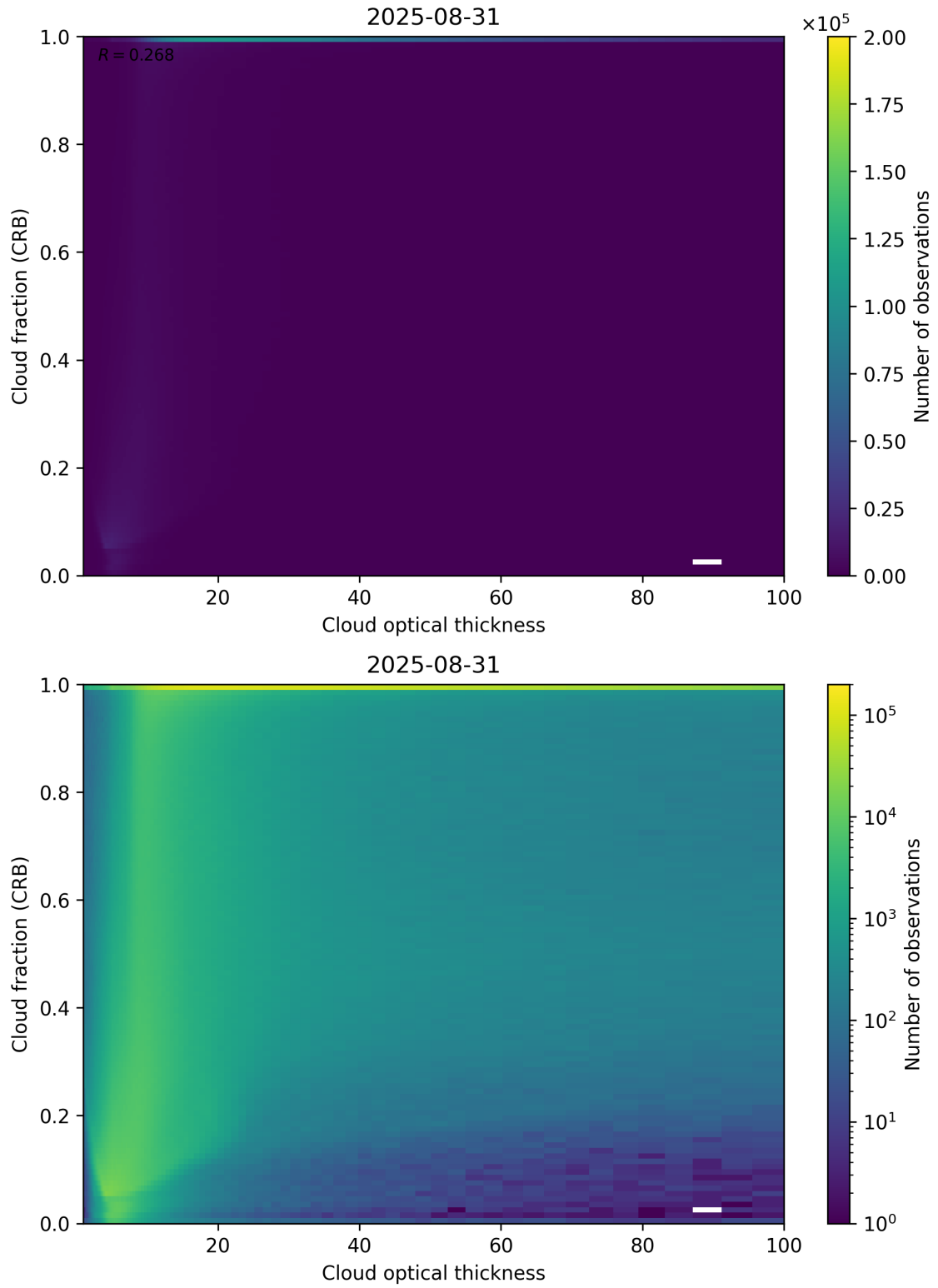
Figure 84: Scatter density plot of “Cloud optical thickness” against “Cloud fraction (CRB)” for 2025-08-30 to 2025-09-01.
