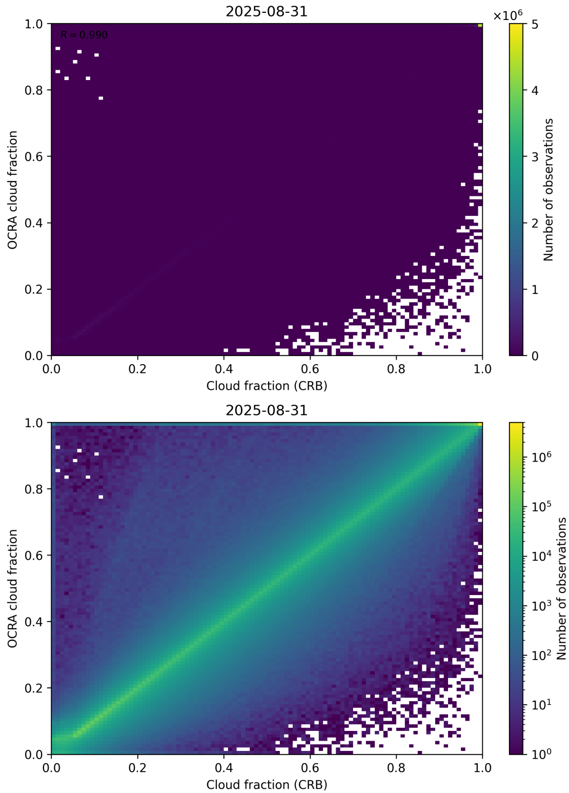
Figure 78: Scatter density plot of “Cloud fraction (CRB)” against “OCRA cloud fraction” for 2025-08-30 to 2025-09-01.
