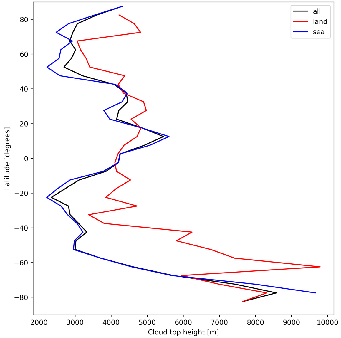
Figure 24: Zonal average of “Cloud top height” for 2025-08-30 to 2025-09-01.
