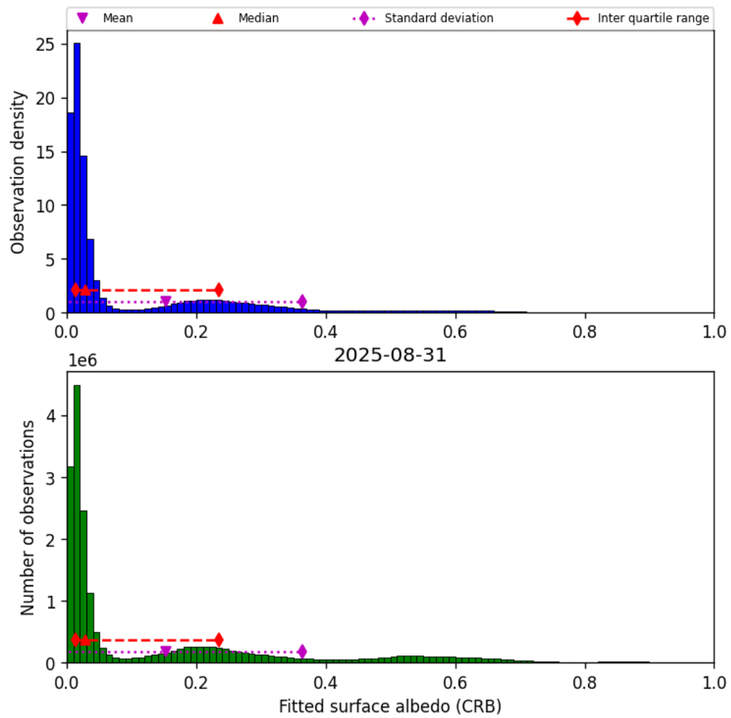
Figure 46: Histogram of “Fitted surface albedo (CRB)” for 2025-08-30 to 2025-09-01
