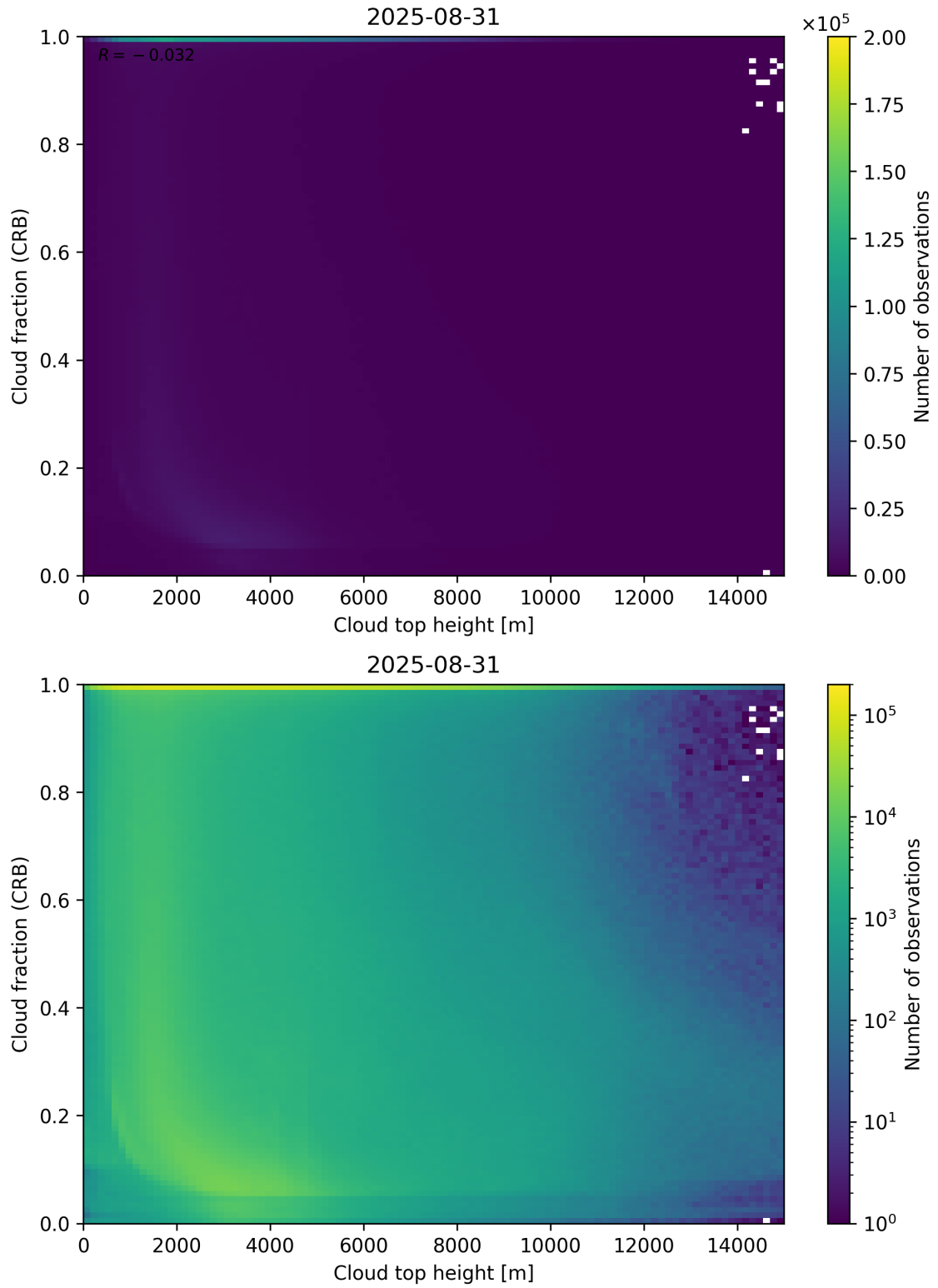
Figure 88: Scatter density plot of “Cloud top height” against “Cloud fraction (CRB)” for 2025-08-30 to 2025-09-01.
