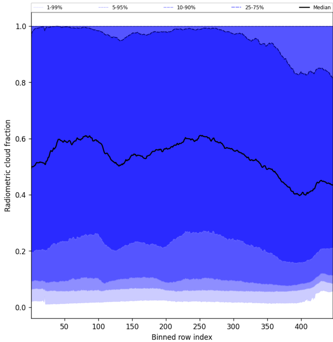
Figure 55: Along track statistics of “Radiometric cloud fraction” for 2025-08-30 to 2025-09-01
