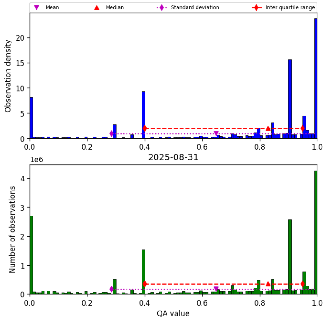
Figure 38: Histogram of “QA value” for 2025-08-30 to 2025-09-01
