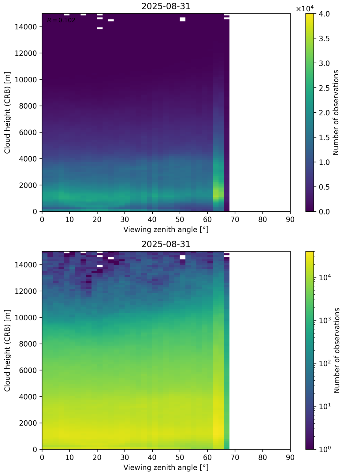
Figure 110: Scatter density plot of “Viewing zenith angle” against “Cloud height (CRB)” for 2025-08-30 to 2025-09-01.
