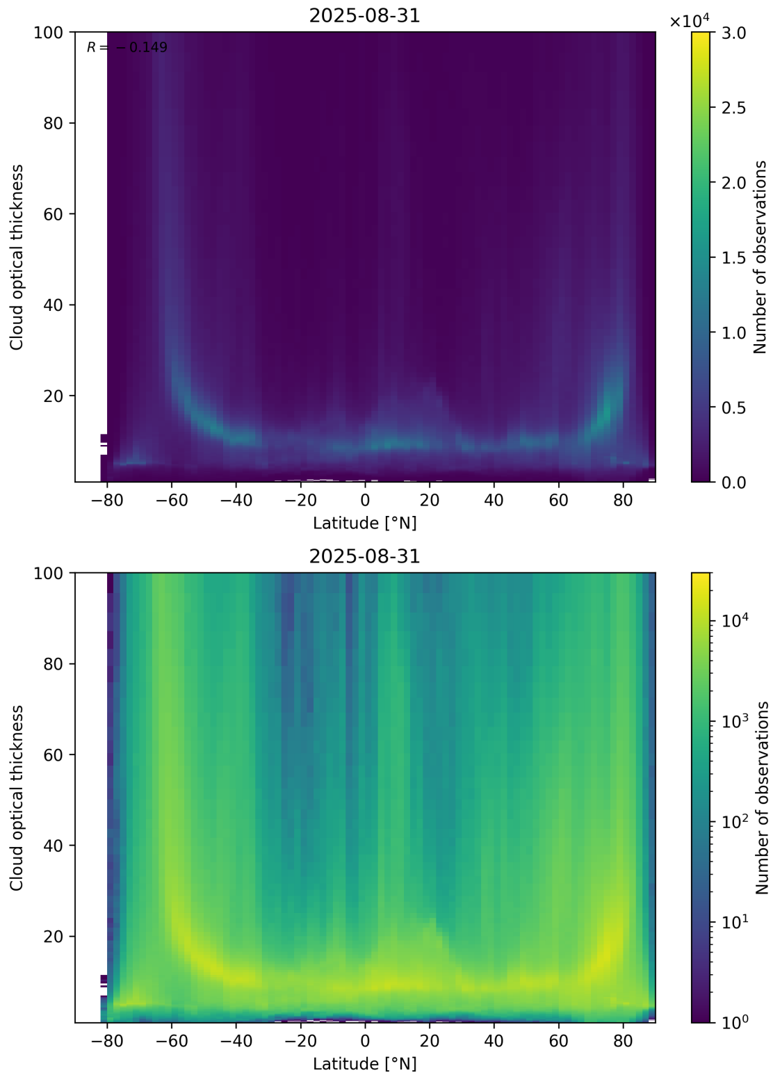
Figure 96: Scatter density plot of “Latitude” against “Cloud optical thickness” for 2025-08-30 to 2025-09-01.
