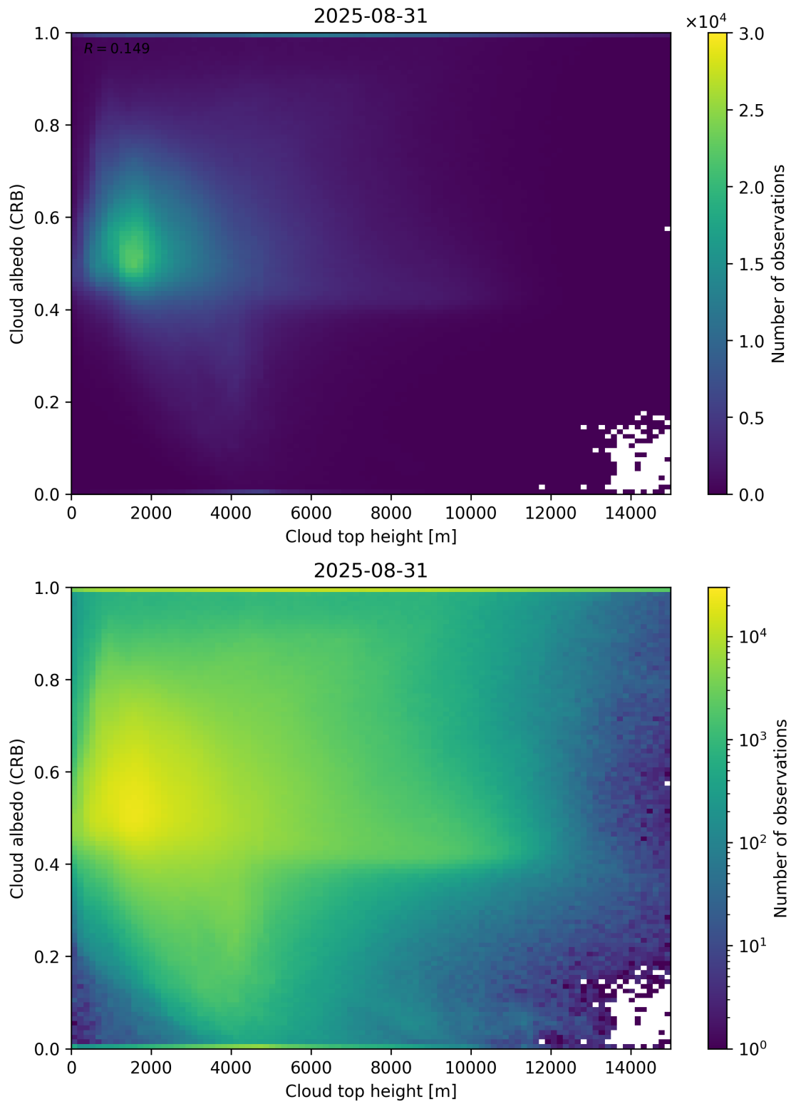
Figure 86: Scatter density plot of “Cloud top height” against “Cloud albedo (CRB)” for 2025-08-30 to 2025-09-01.
