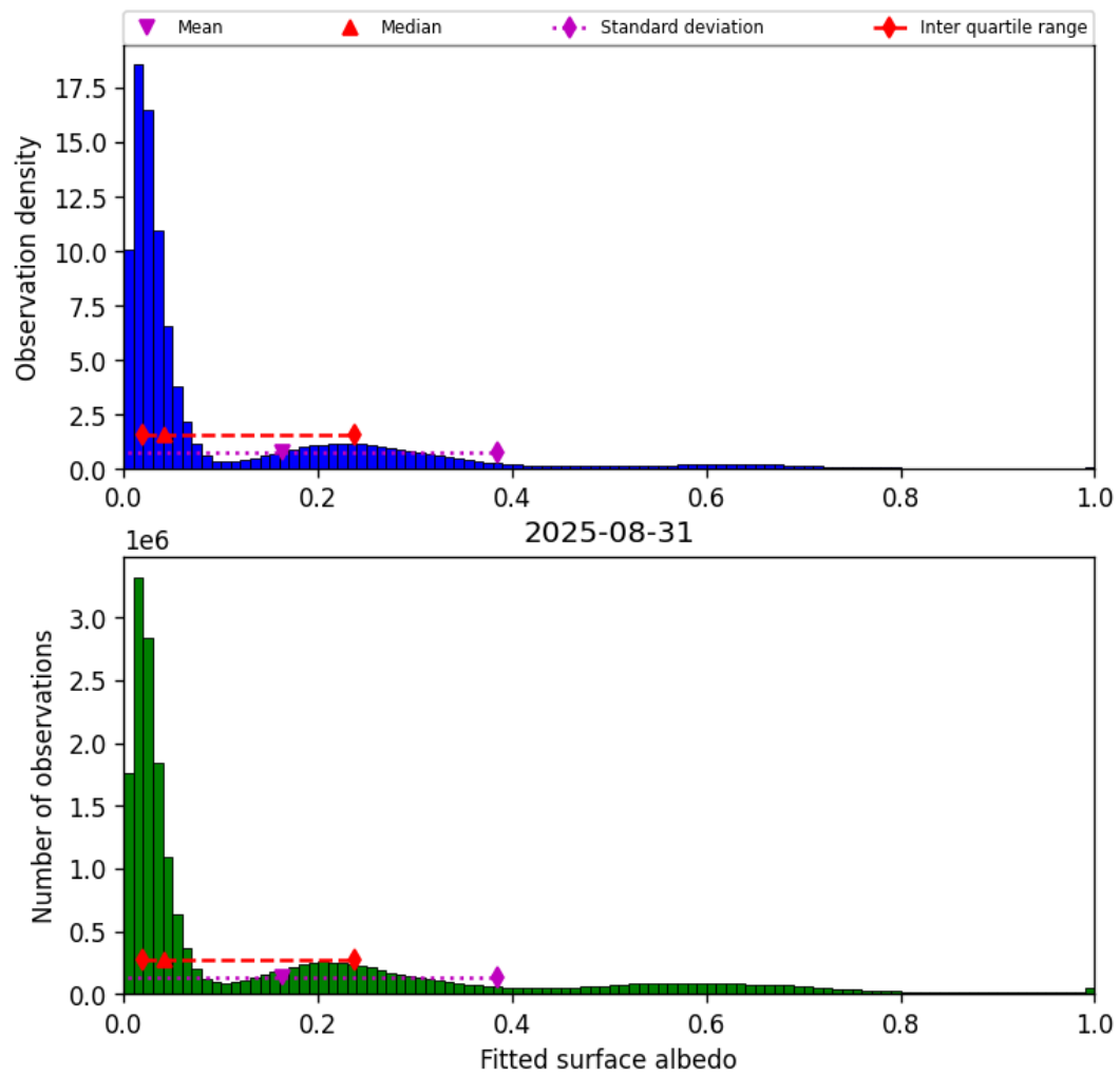
Figure 45: Histogram of “Fitted surface albedo” for 2025-08-30 to 2025-09-01
