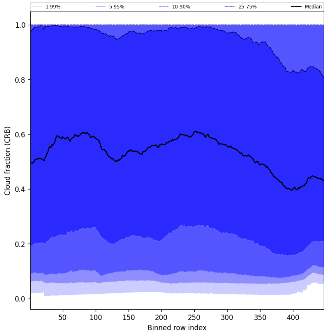
Figure 58: Along track statistics of “Cloud fraction (CRB)” for 2025-08-30 to 2025-09-01
