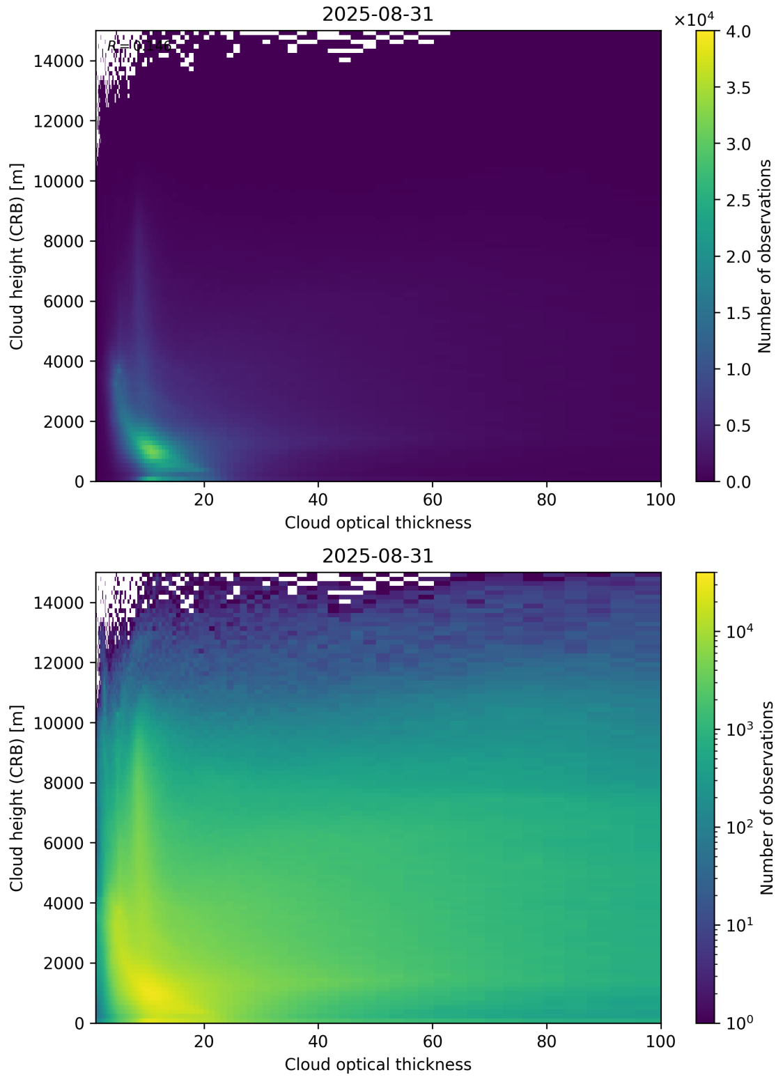
Figure 85: Scatter density plot of “Cloud optical thickness” against “Cloud height (CRB)” for 2025-08-30 to 2025-09-01.
