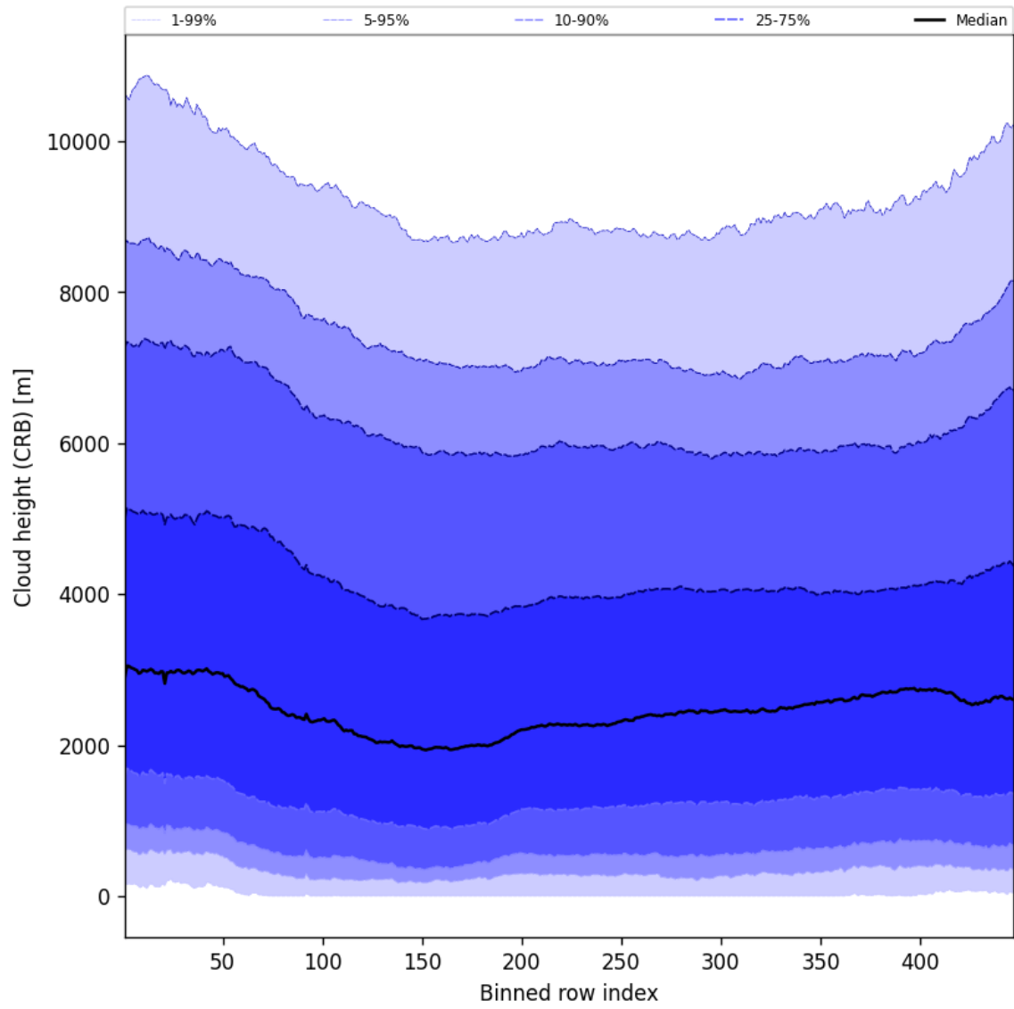
Figure 59: Along track statistics of “Cloud height (CRB)” for 2025-08-30 to 2025-09-01
