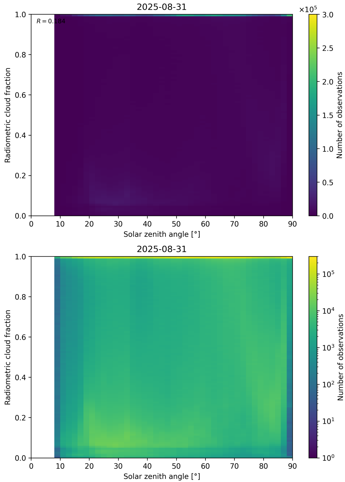
Figure 99: Scatter density plot of “Solar zenith angle” against “Radiometric cloud fraction” for 2025-08-30 to 2025-09-01.
