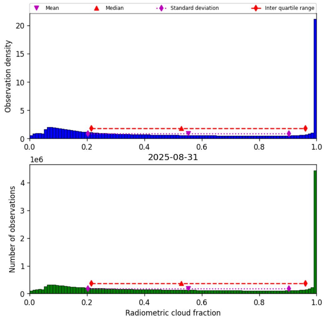
Figure 39: Histogram of “Radiometric cloud fraction” for 2025-08-30 to 2025-09-01
