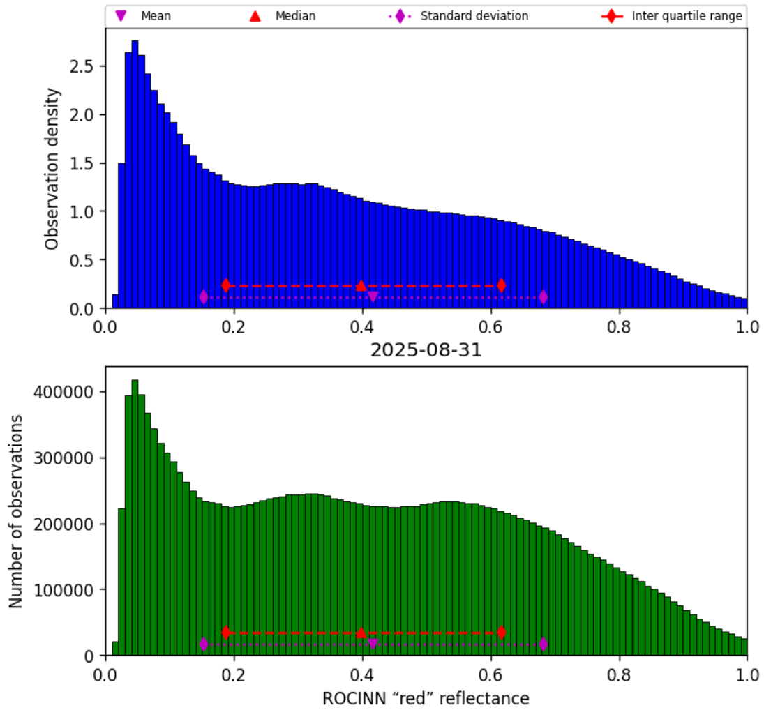
Figure 53: Histogram of “ROCINN “red” reflectance” for 2025-08-30 to 2025-09-01
