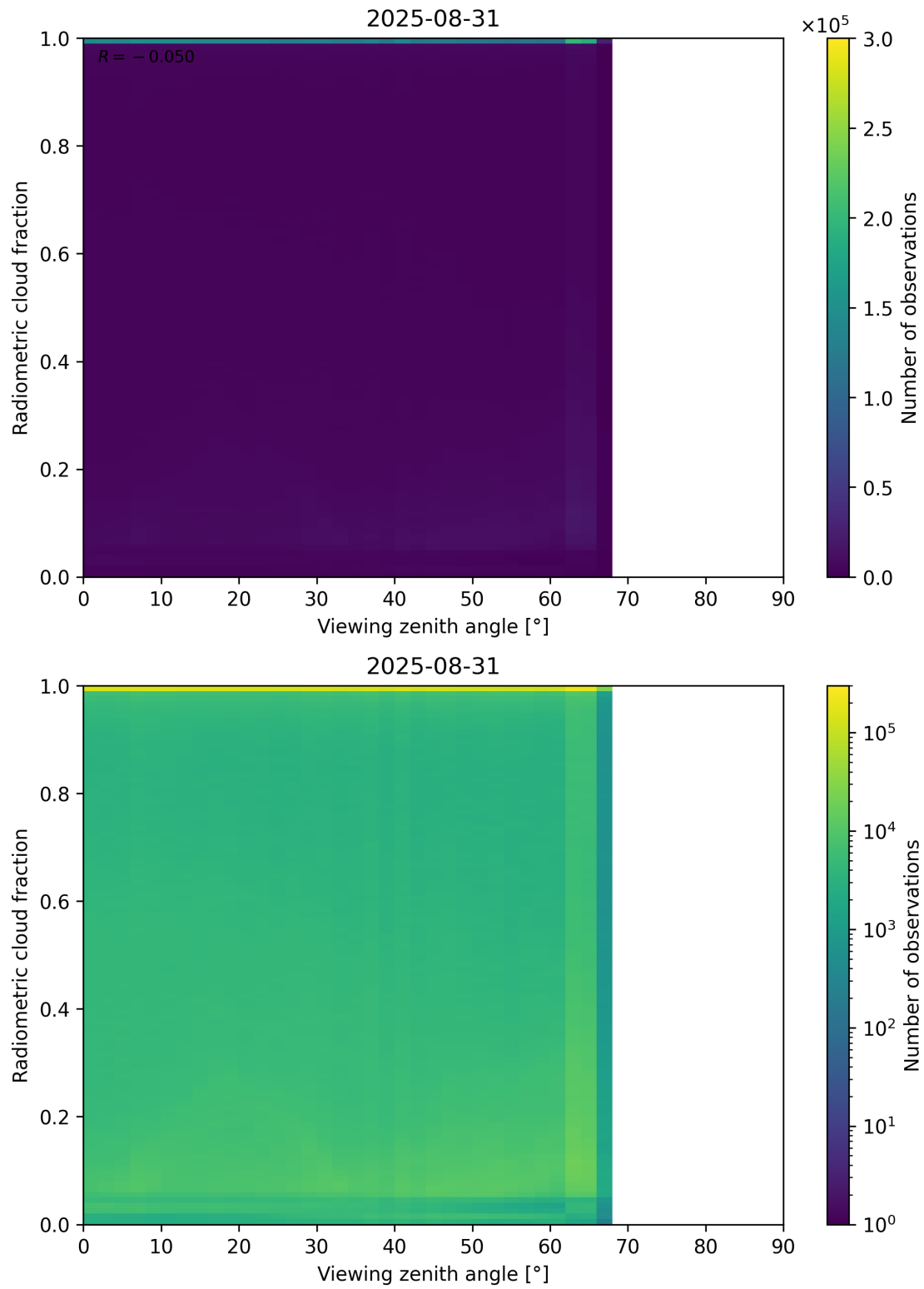
Figure 107: Scatter density plot of “Viewing zenith angle” against “Radiometric cloud fraction” for 2025-08-30 to 2025-09-01.
