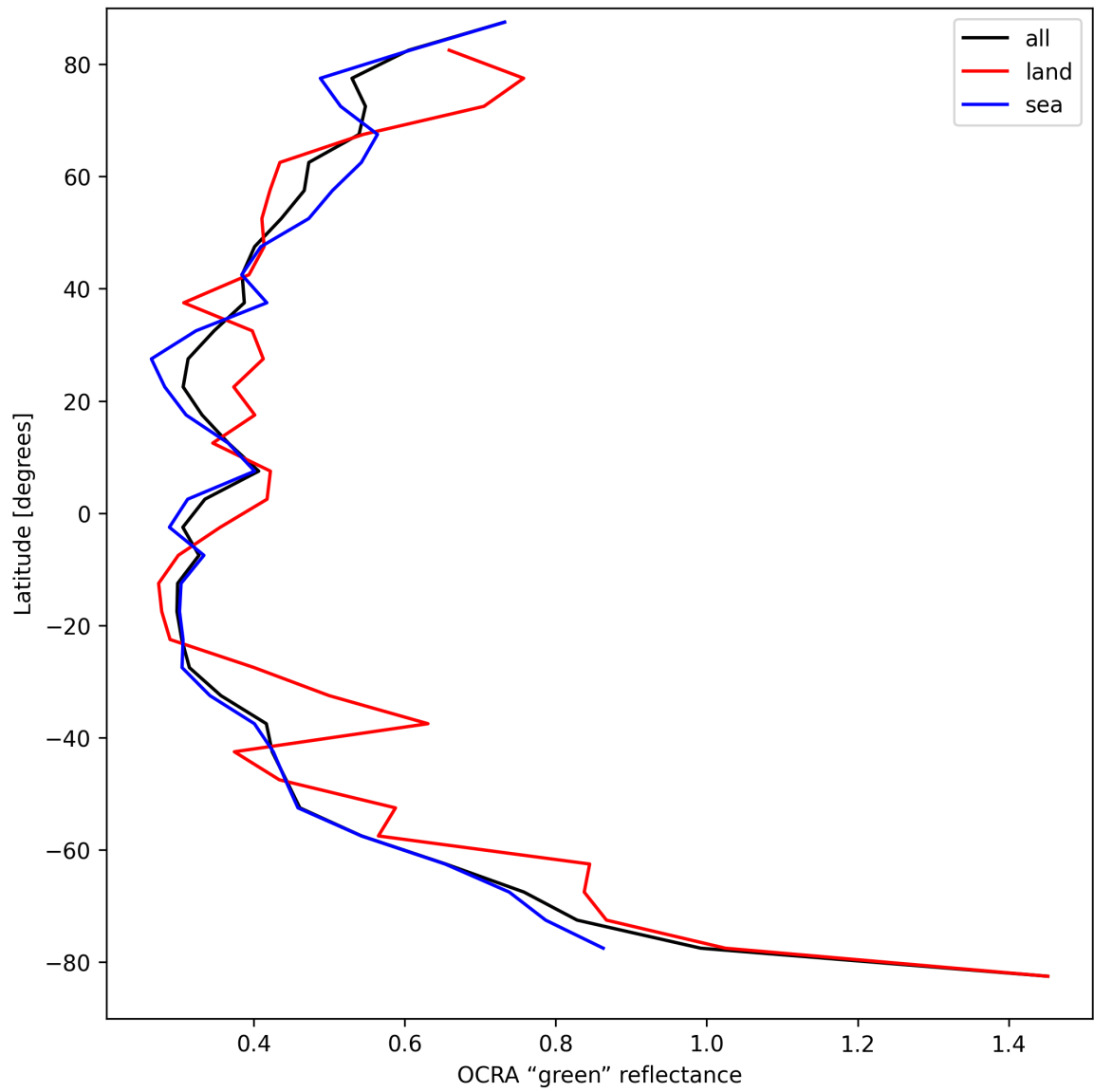
Figure 36: Zonal average of “OCRA “green” reflectance” for 2025-08-30 to 2025-09-01.
