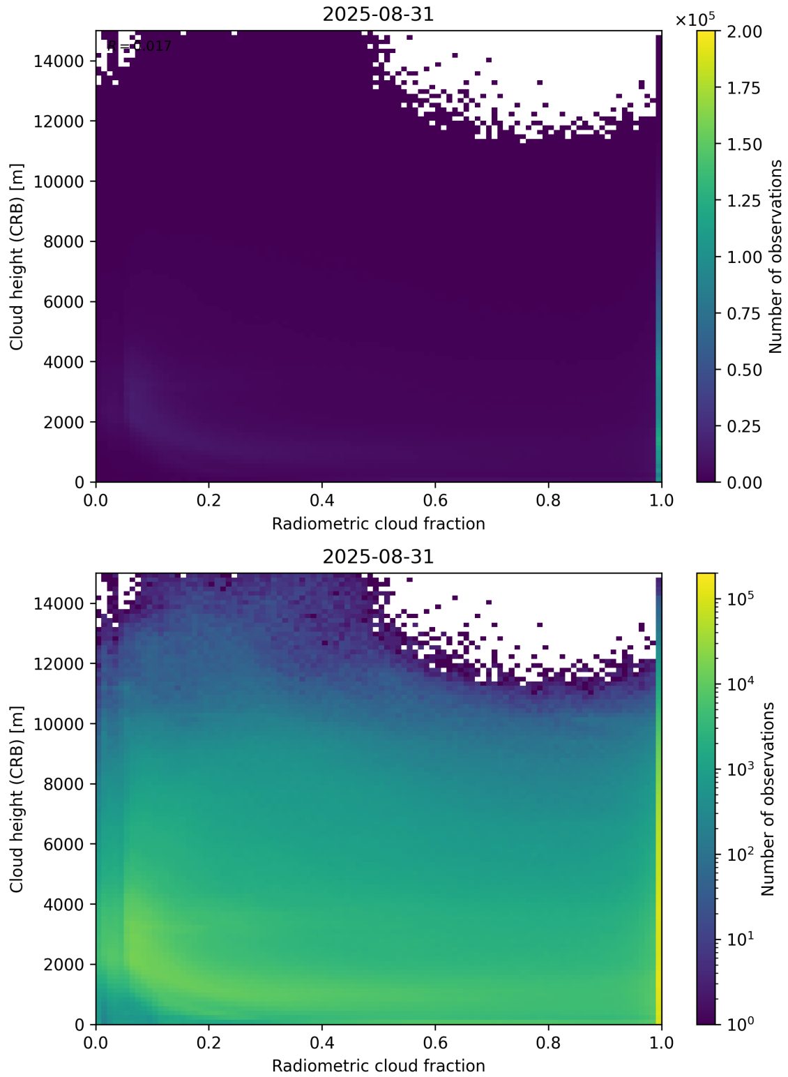
Figure 74: Scatter density plot of “Radiometric cloud fraction” against “Cloud height (CRB)” for 2025-08-30 to 2025-09-01.
