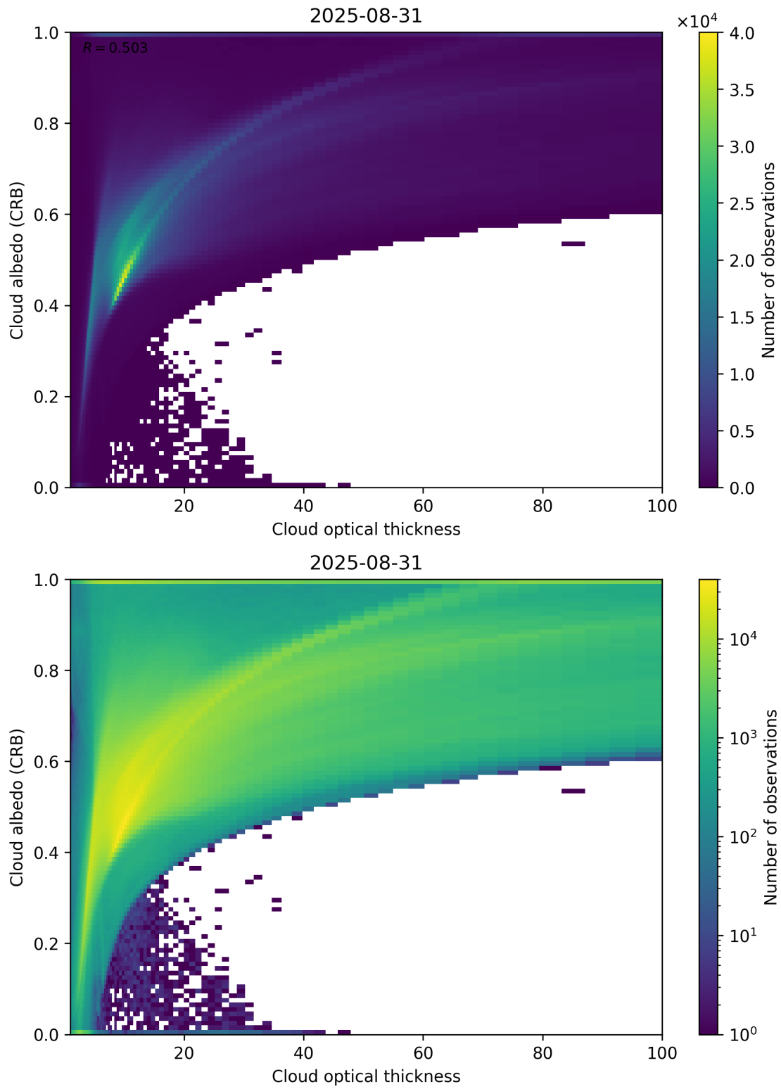
Figure 82: Scatter density plot of “Cloud optical thickness” against “Cloud albedo (CRB)” for 2025-08-30 to 2025-09-01.
