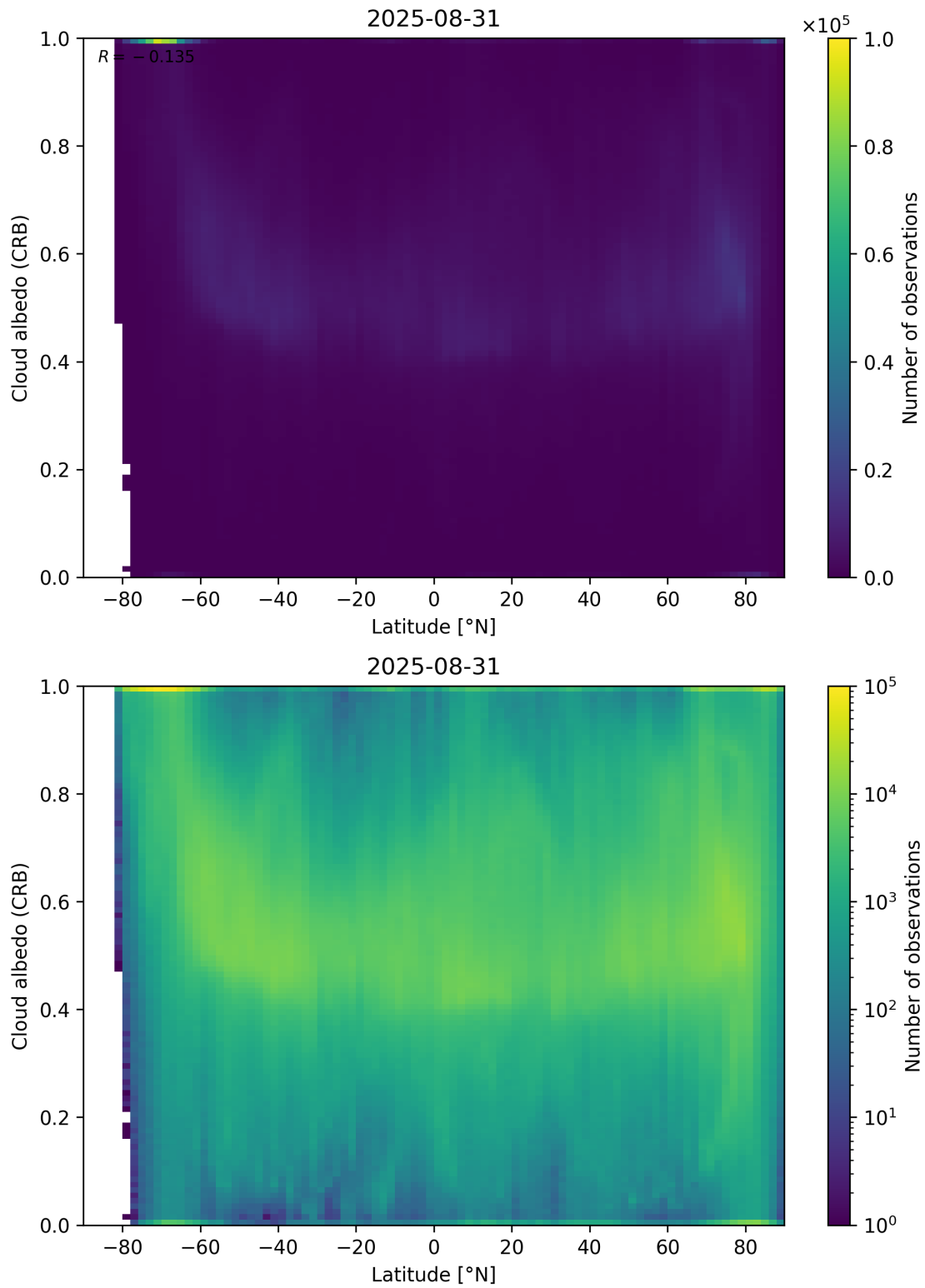
Figure 91: Scatter density plot of “Latitude” against “Cloud albedo (CRB)” for 2025-08-30 to 2025-09-01.
