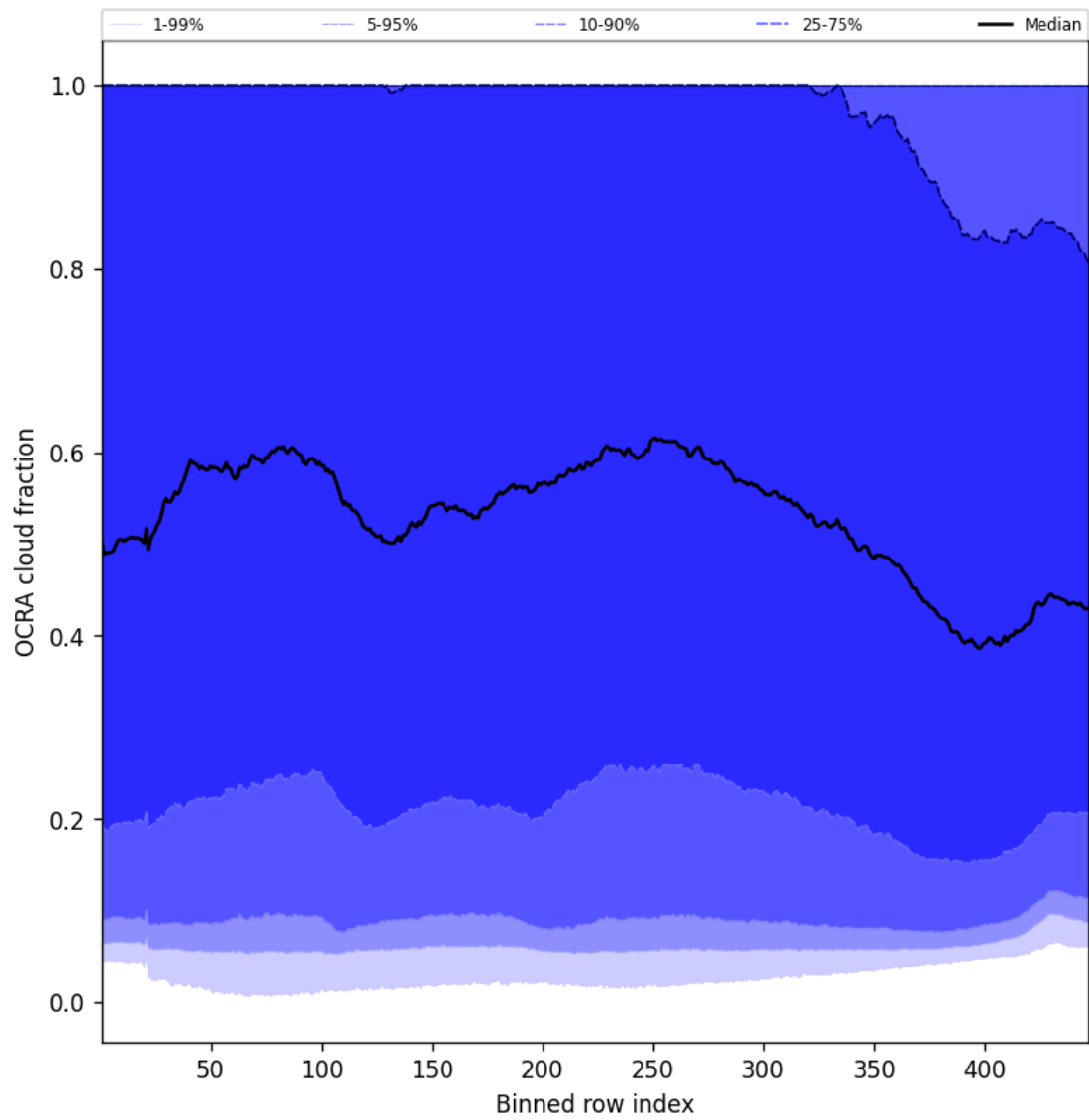
Figure 66: Along track statistics of “OCRA cloud fraction” for 2025-08-30 to 2025-09-01
