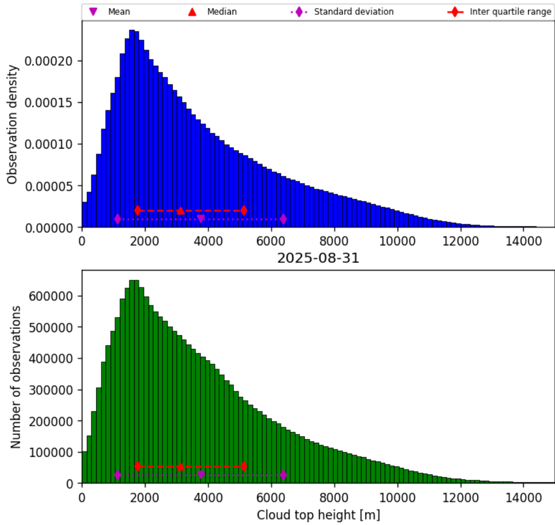
Figure 40: Histogram of “Cloud top height” for 2025-08-30 to 2025-09-01
