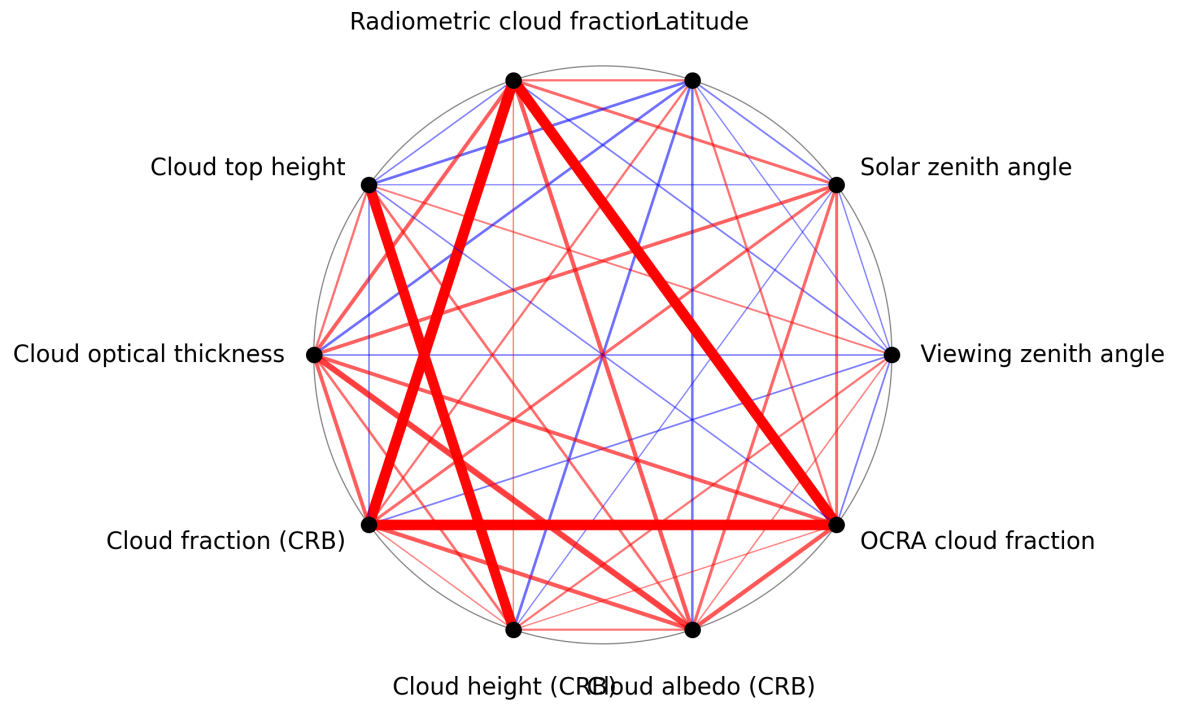
Figure 1: Map of correlation graph for 2025-08-30 to 2025-09-01.
