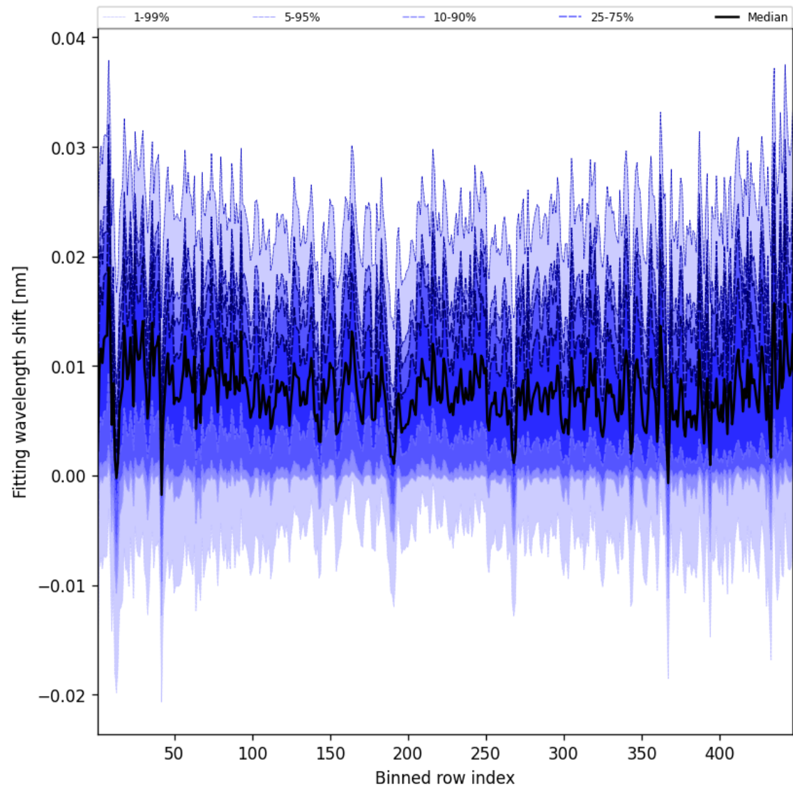
Figure 65: Along track statistics of “Fitting wavelength shift” for 2025-08-30 to 2025-09-01
