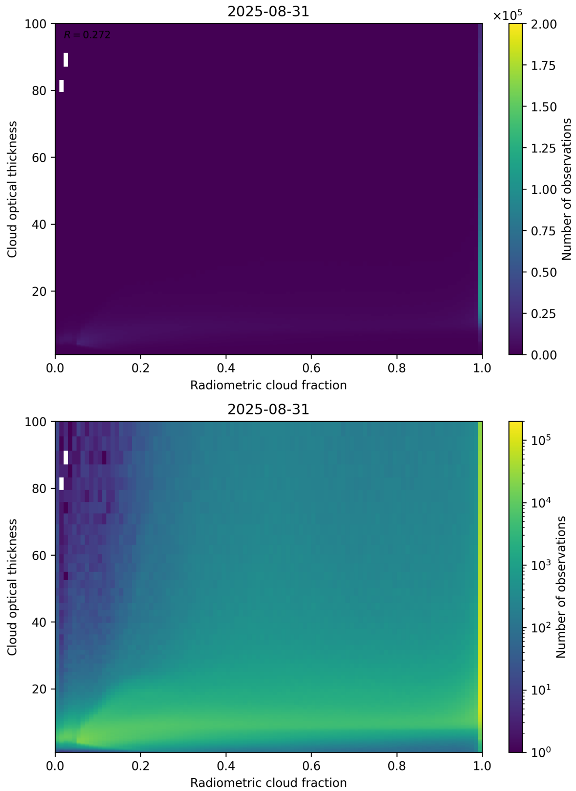
Figure 75: Scatter density plot of “Radiometric cloud fraction” against “Cloud optical thickness” for 2025-08-30 to 2025-09-01.
