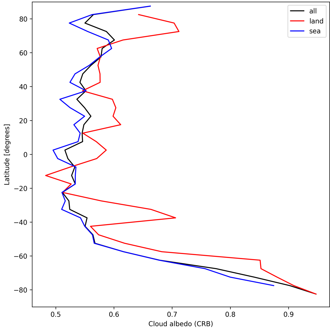
Figure 28: Zonal average of “Cloud albedo (CRB)” for 2025-08-30 to 2025-09-01.
