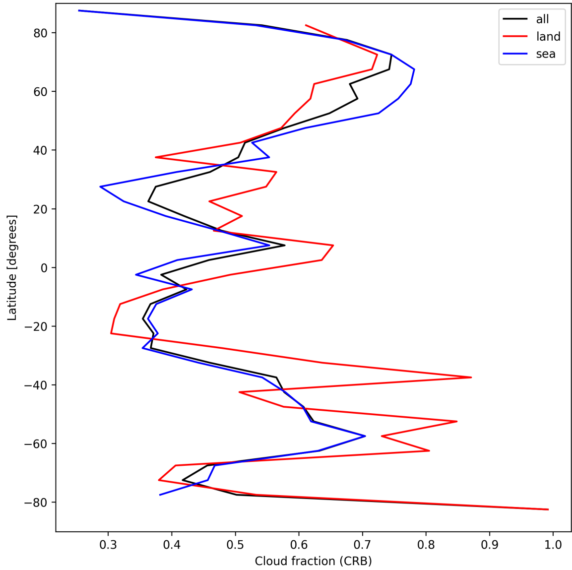
Figure 26: Zonal average of “Cloud fraction (CRB)” for 2025-08-30 to 2025-09-01.
