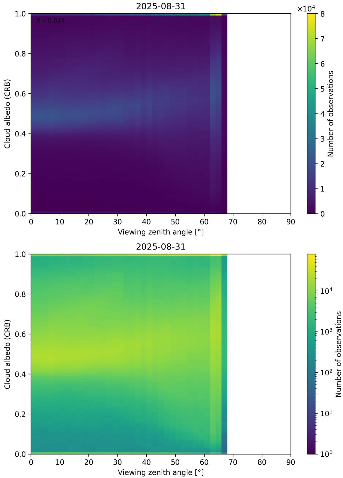
Figure 106: Scatter density plot of “Viewing zenith angle” against “Cloud albedo (CRB)” for 2025-08-30 to 2025-09-01.
