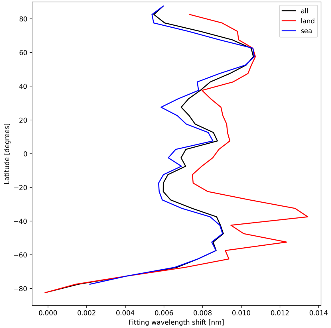
Figure 33: Zonal average of “Fitting wavelength shift” for 2025-08-30 to 2025-09-01.
