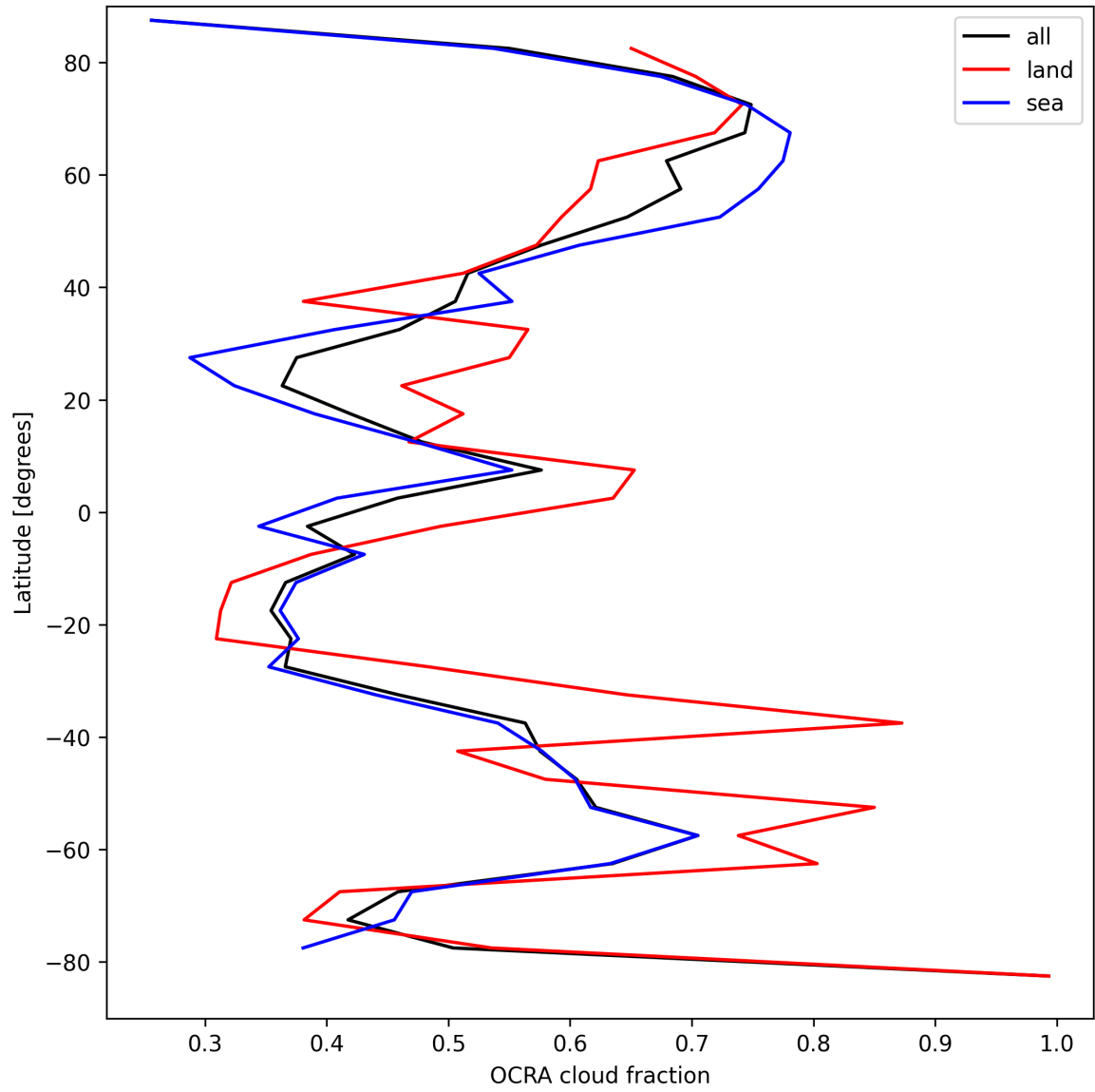
Figure 34: Zonal average of “OCRA cloud fraction” for 2025-08-30 to 2025-09-01.
