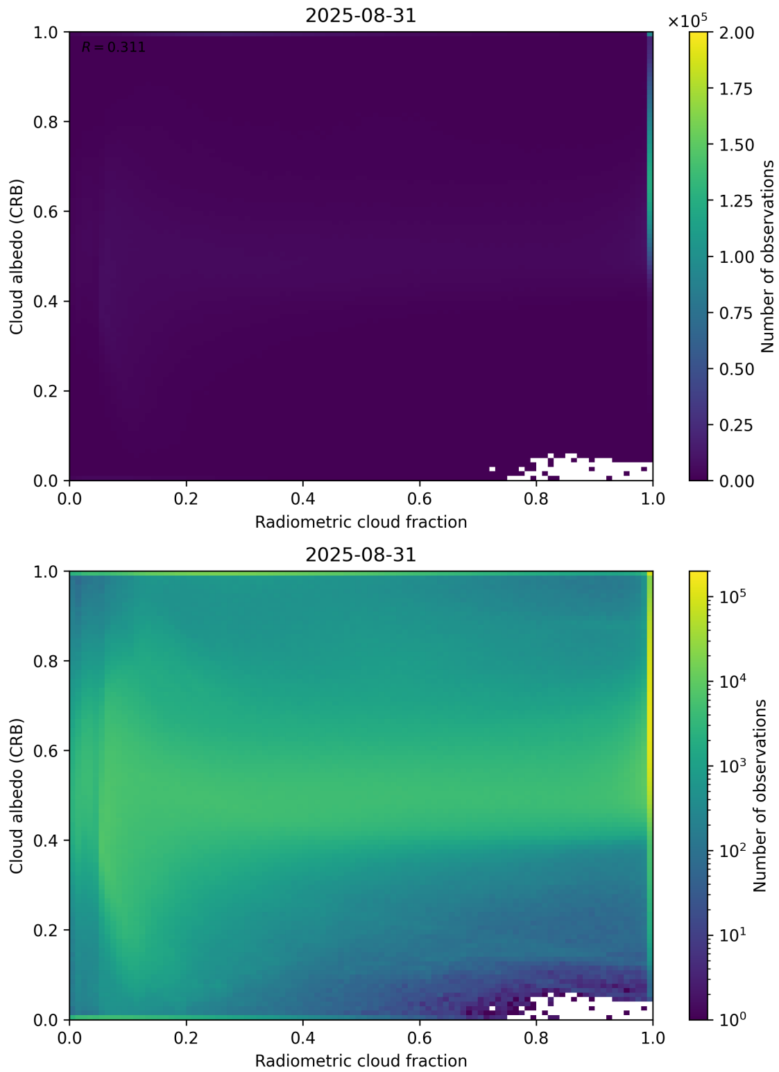
Figure 71: Scatter density plot of “Radiometric cloud fraction” against “Cloud albedo (CRB)” for 2025-08-30 to 2025-09-01.
