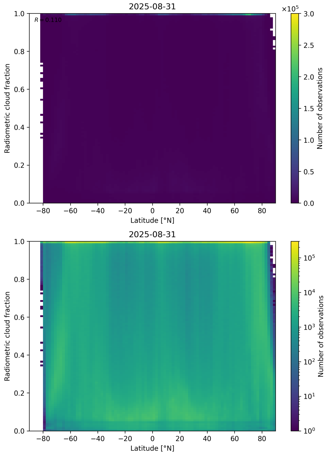
Figure 92: Scatter density plot of “Latitude” against “Radiometric cloud fraction” for 2025-08-30 to 2025-09-01.
