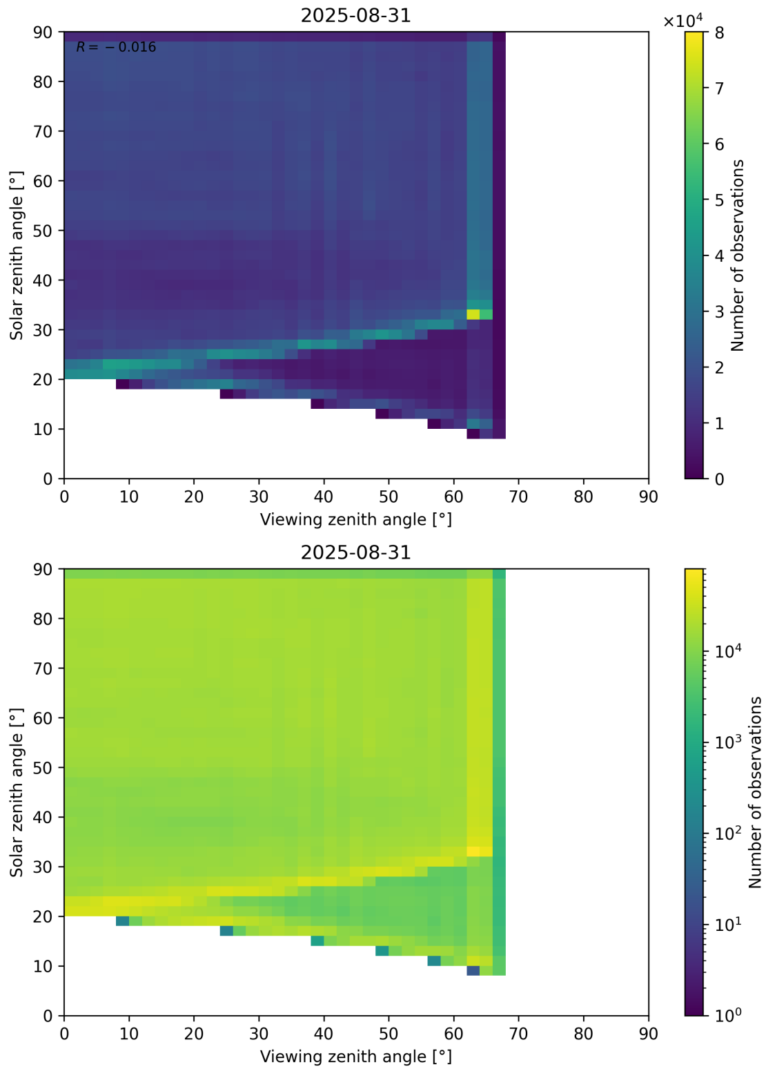
Figure 114: Scatter density plot of “Viewing zenith angle” against “Solar zenith angle” for 2025-08-30 to 2025-09-01.
