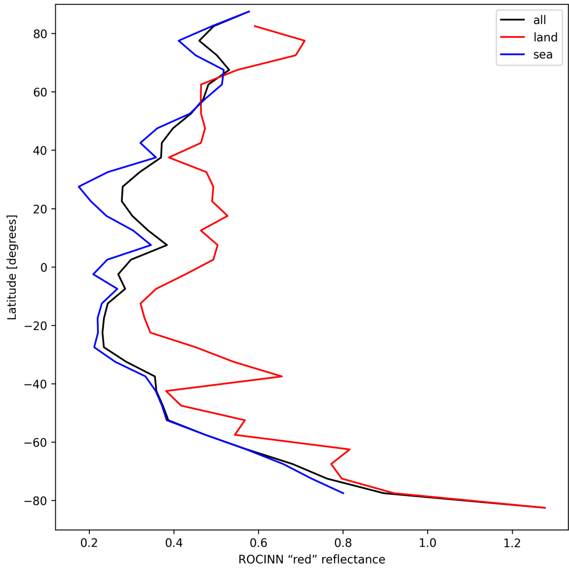
Figure 37: Zonal average of “ROCINN “red” reflectance” for 2025-08-30 to 2025-09-01.
