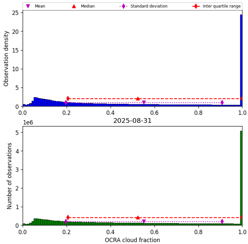
Figure 50: Histogram of “OCRA cloud fraction” for 2025-08-30 to 2025-09-01
