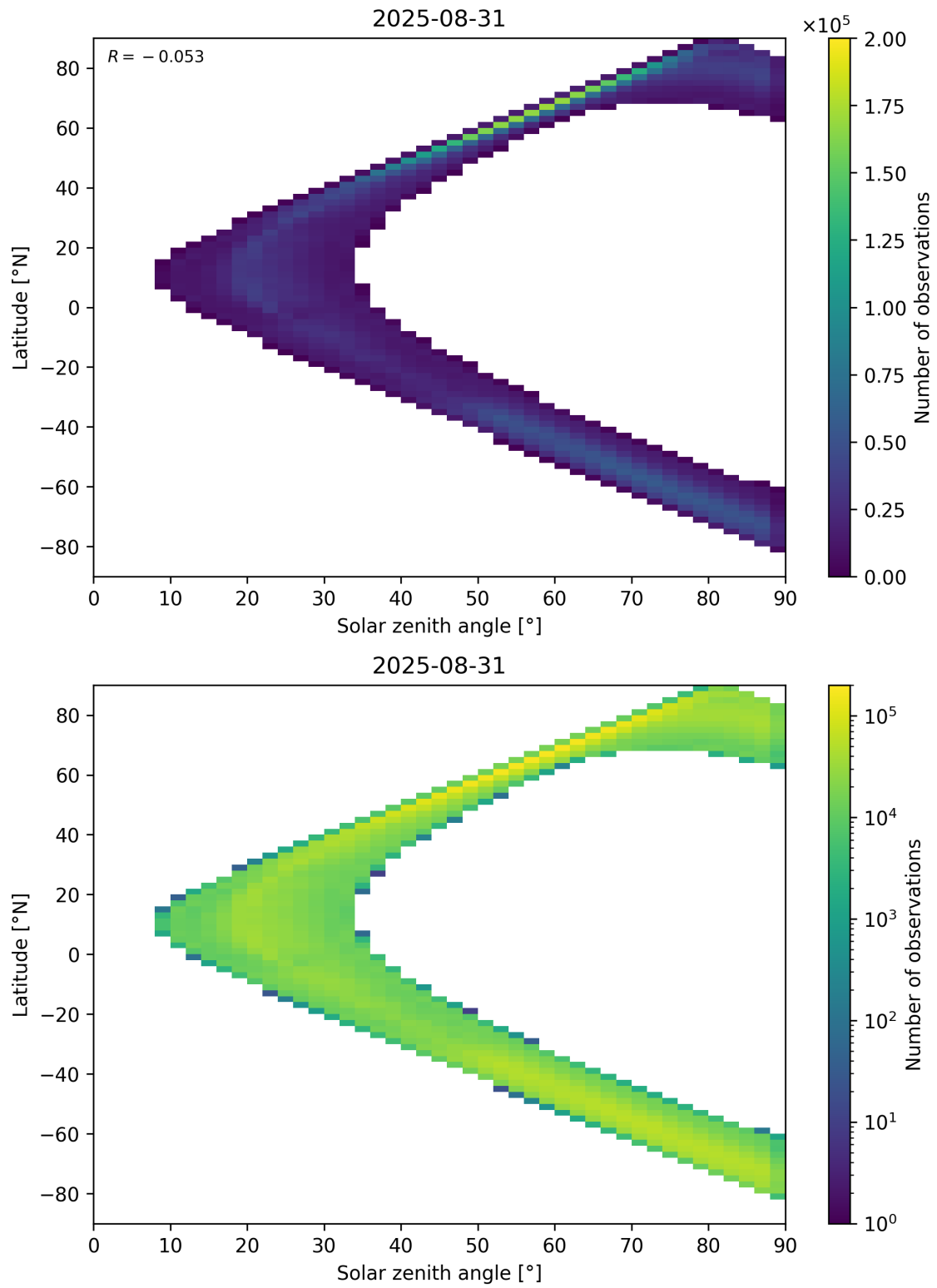
Figure 105: Scatter density plot of “Solar zenith angle” against “Latitude” for 2025-08-30 to 2025-09-01.
