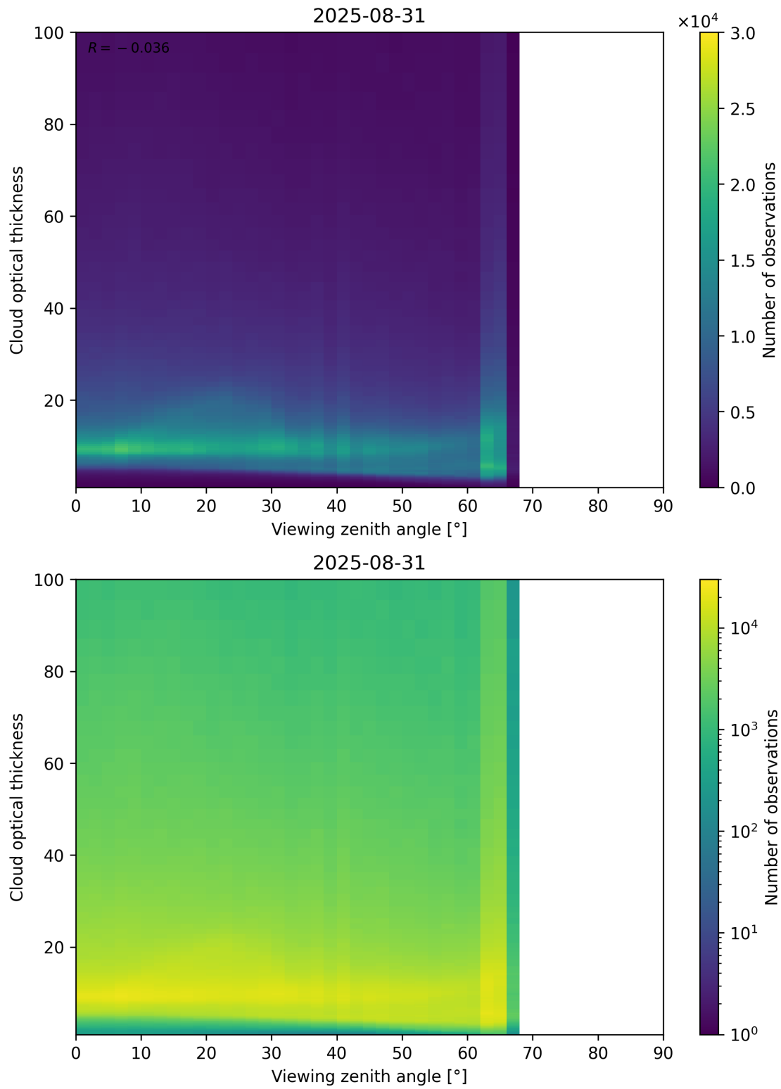
Figure 111: Scatter density plot of “Viewing zenith angle” against “Cloud optical thickness” for 2025-08-30 to 2025-09-01.
