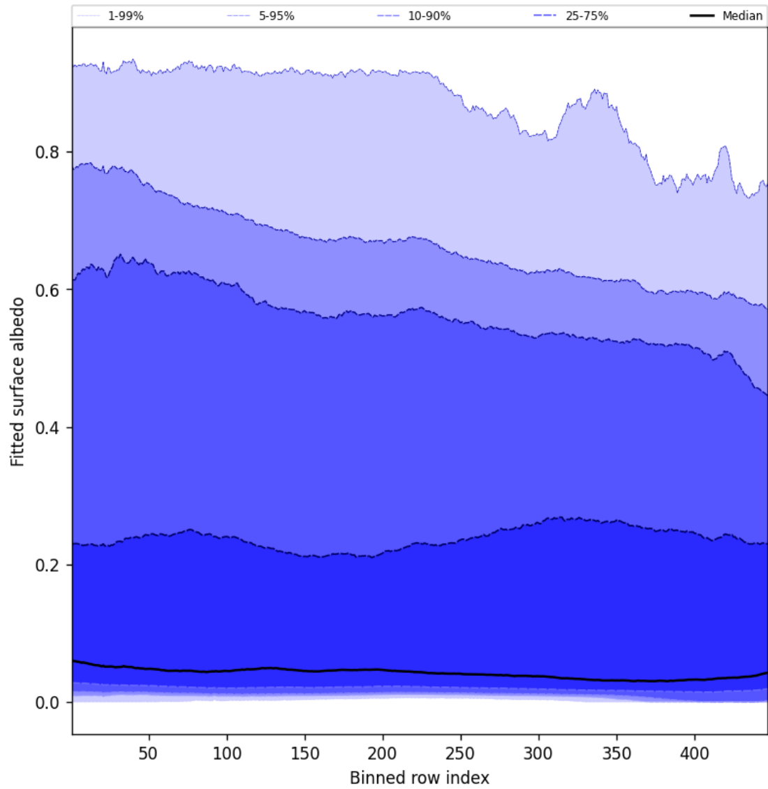
Figure 61: Along track statistics of “Fitted surface albedo” for 2025-08-30 to 2025-09-01
