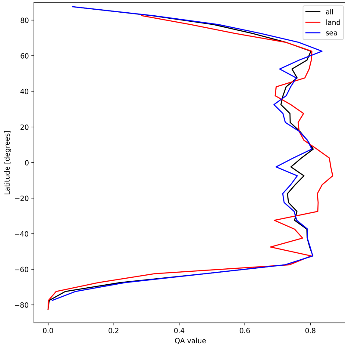
Figure 22: Zonal average of “QA value” for 2025-08-31 to 2025-09-02.
