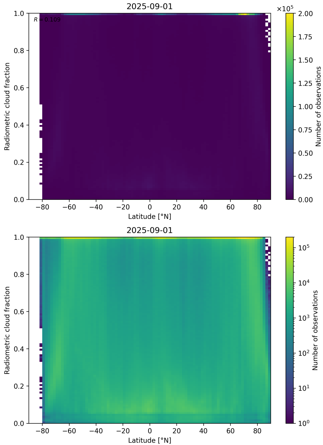
Figure 92: Scatter density plot of “Latitude” against “Radiometric cloud fraction” for 2025-08-31 to 2025-09-02.
