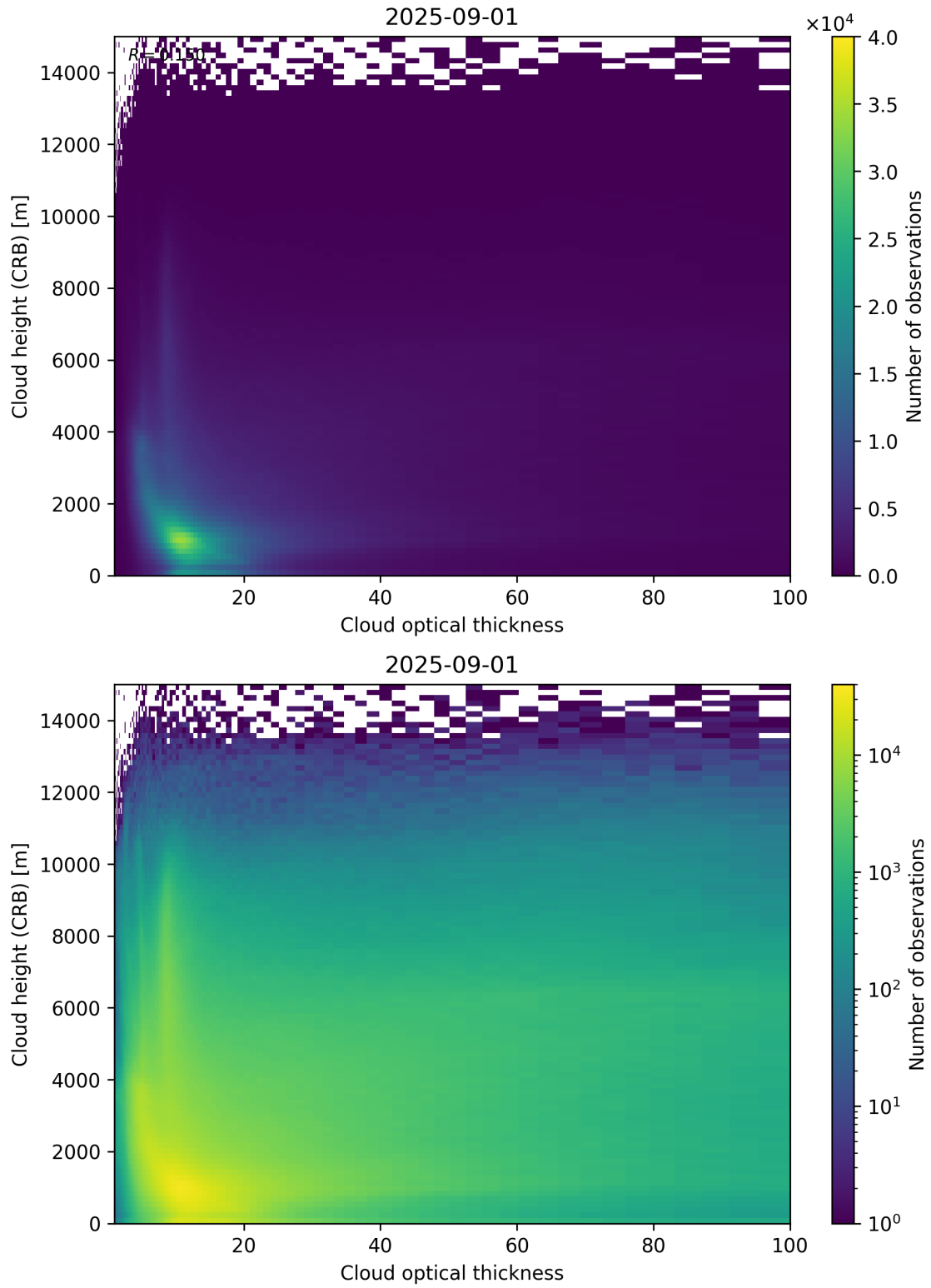
Figure 85: Scatter density plot of “Cloud optical thickness” against “Cloud height (CRB)” for 2025-08-31 to 2025-09-02.
