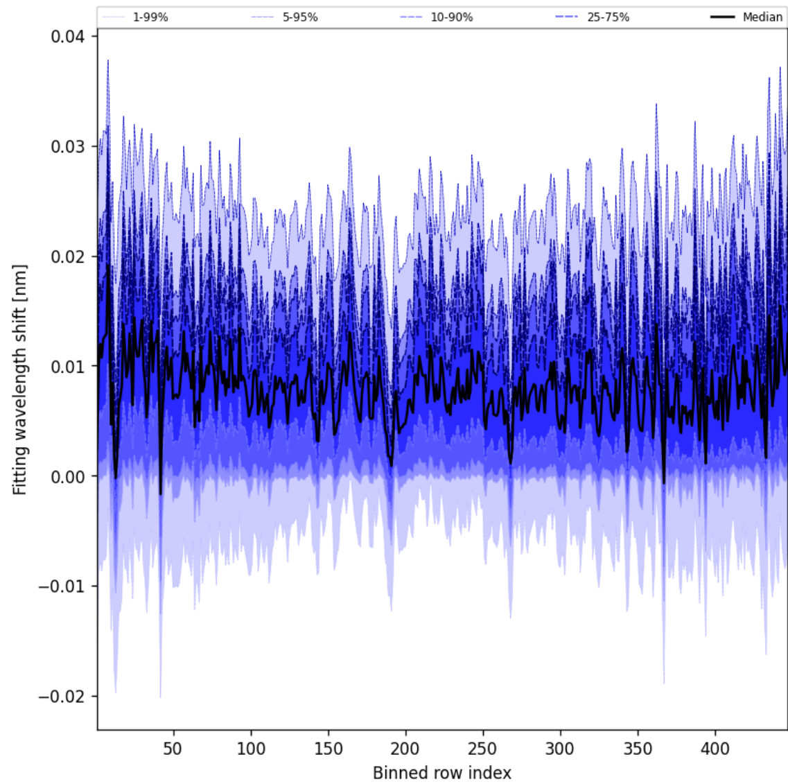
Figure 65: Along track statistics of “Fitting wavelength shift” for 2025-08-31 to 2025-09-02
