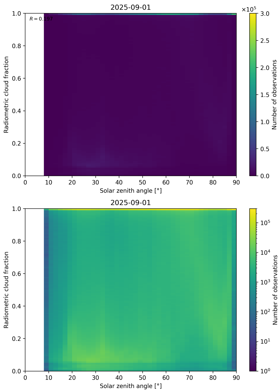
Figure 99: Scatter density plot of “Solar zenith angle” against “Radiometric cloud fraction” for 2025-08-31 to 2025-09-02.
