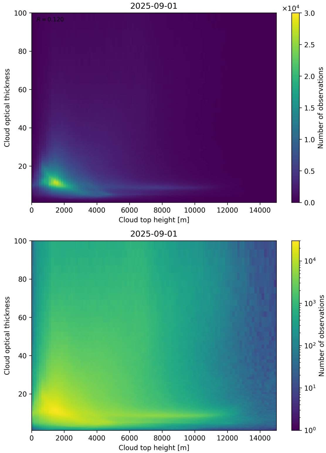
Figure 90: Scatter density plot of “Cloud top height” against “Cloud optical thickness” for 2025-08-31 to 2025-09-02.
