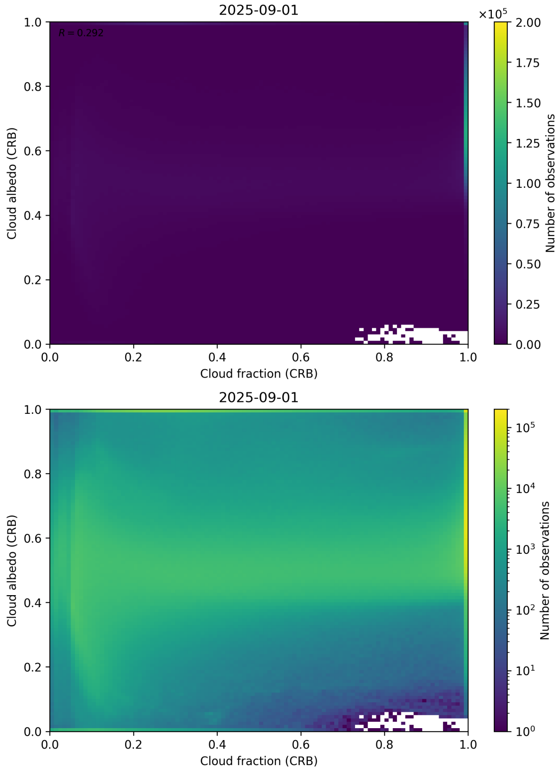
Figure 77: Scatter density plot of “Cloud fraction (CRB)” against “Cloud albedo (CRB)” for 2025-08-31 to 2025-09-02.
