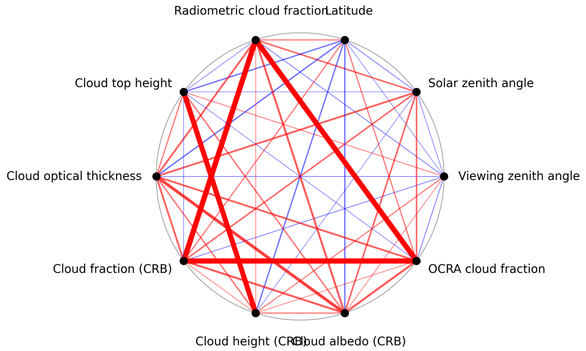
Figure 1: Map of correlation graph for 2025-08-31 to 2025-09-02.
