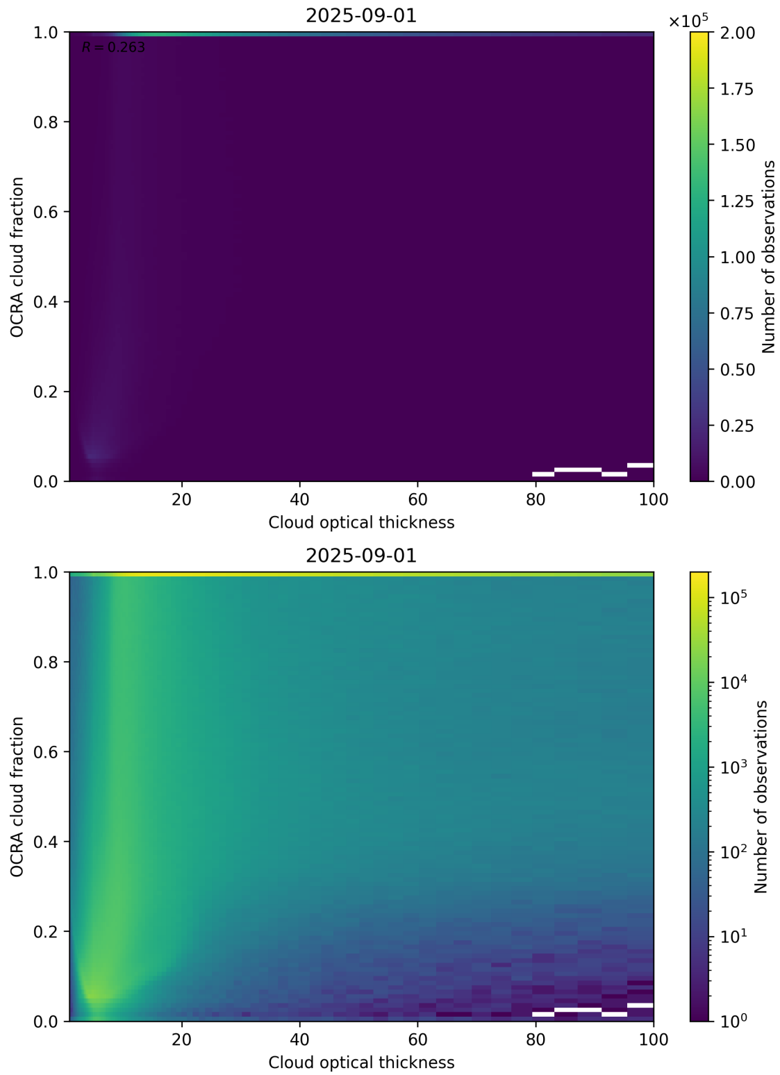
Figure 83: Scatter density plot of “Cloud optical thickness” against “OCRA cloud fraction” for 2025-08-31 to 2025-09-02.
