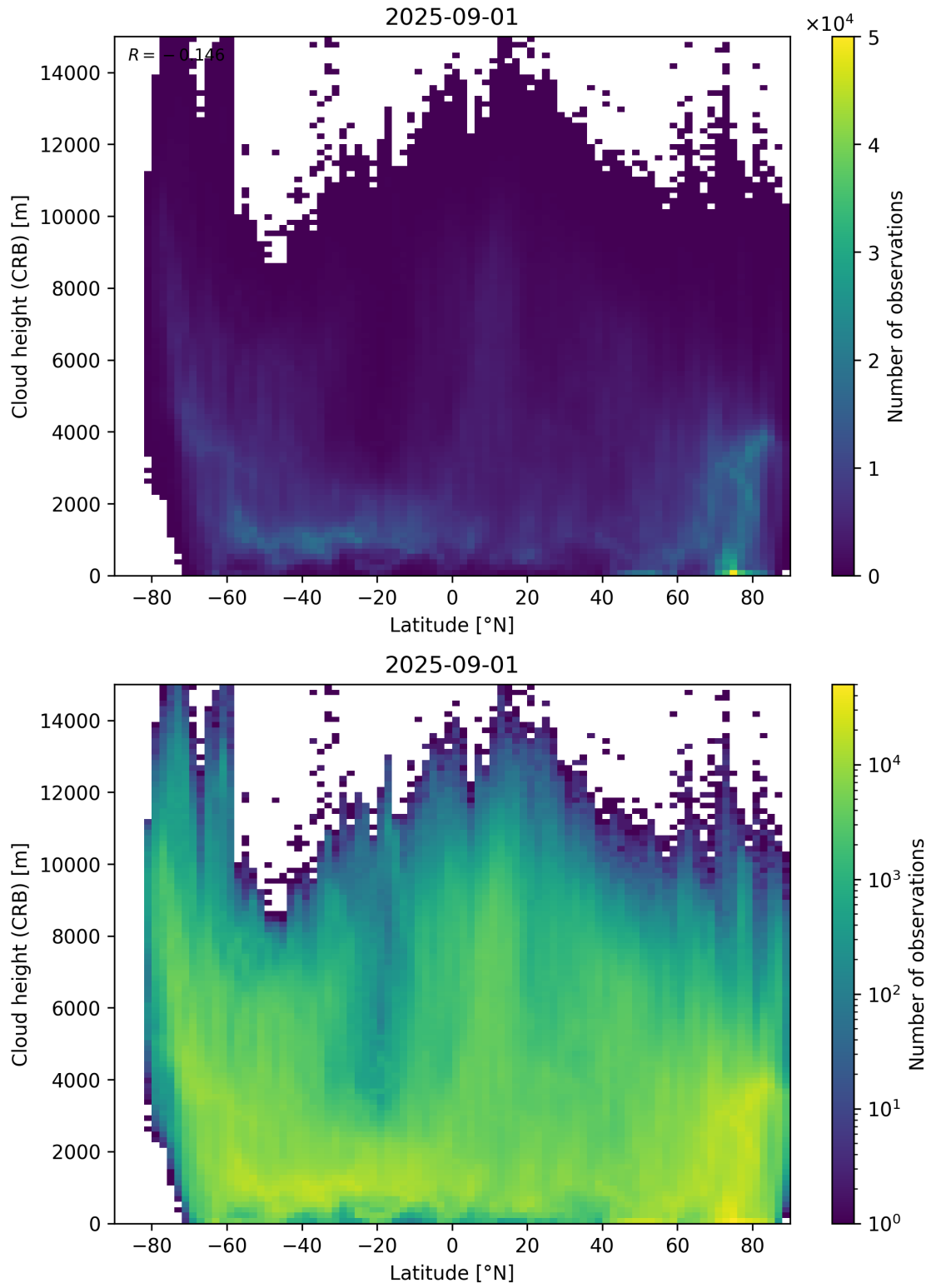
Figure 95: Scatter density plot of “Latitude” against “Cloud height (CRB)” for 2025-08-31 to 2025-09-02.
