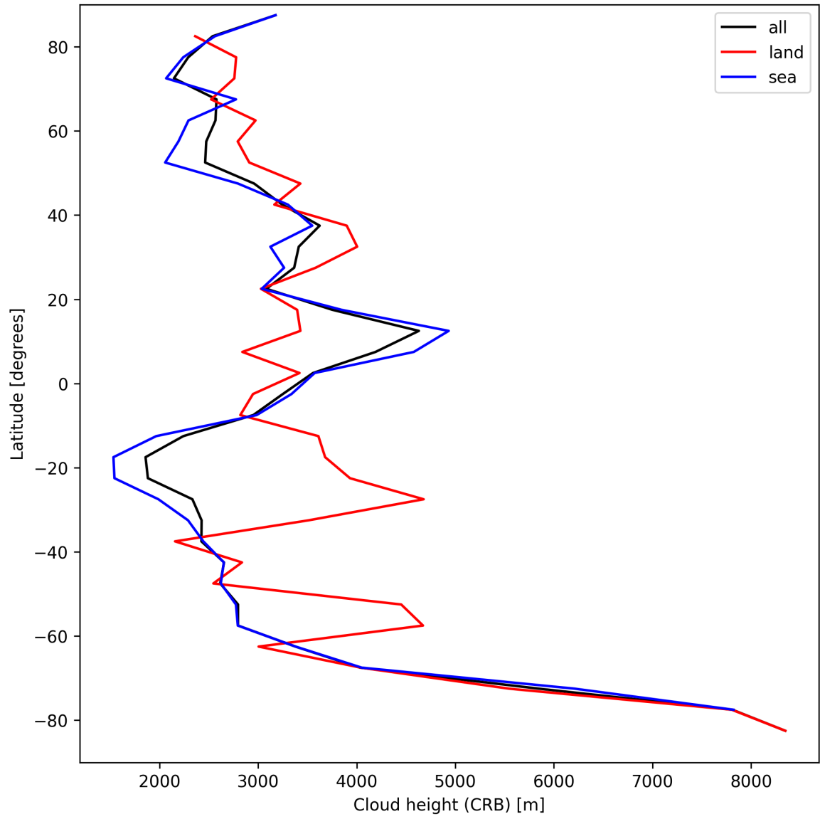
Figure 27: Zonal average of “Cloud height (CRB)” for 2025-08-31 to 2025-09-02.
