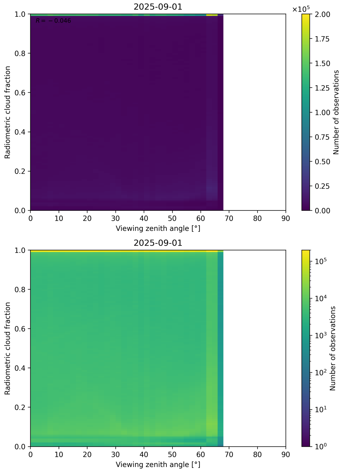
Figure 107: Scatter density plot of “Viewing zenith angle” against “Radiometric cloud fraction” for 2025-08-31 to 2025-09-02.
