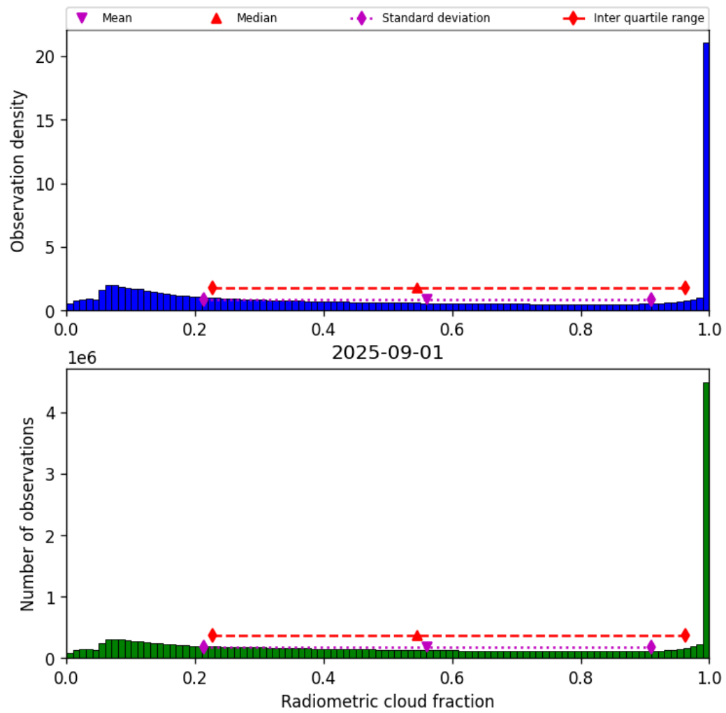
Figure 39: Histogram of “Radiometric cloud fraction” for 2025-08-31 to 2025-09-02
