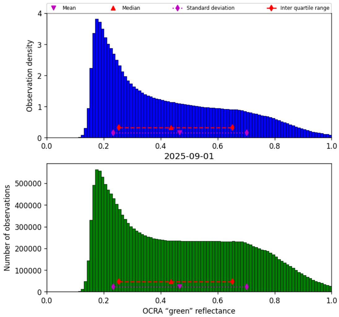
Figure 52: Histogram of “OCRA “green” reflectance” for 2025-08-31 to 2025-09-02
