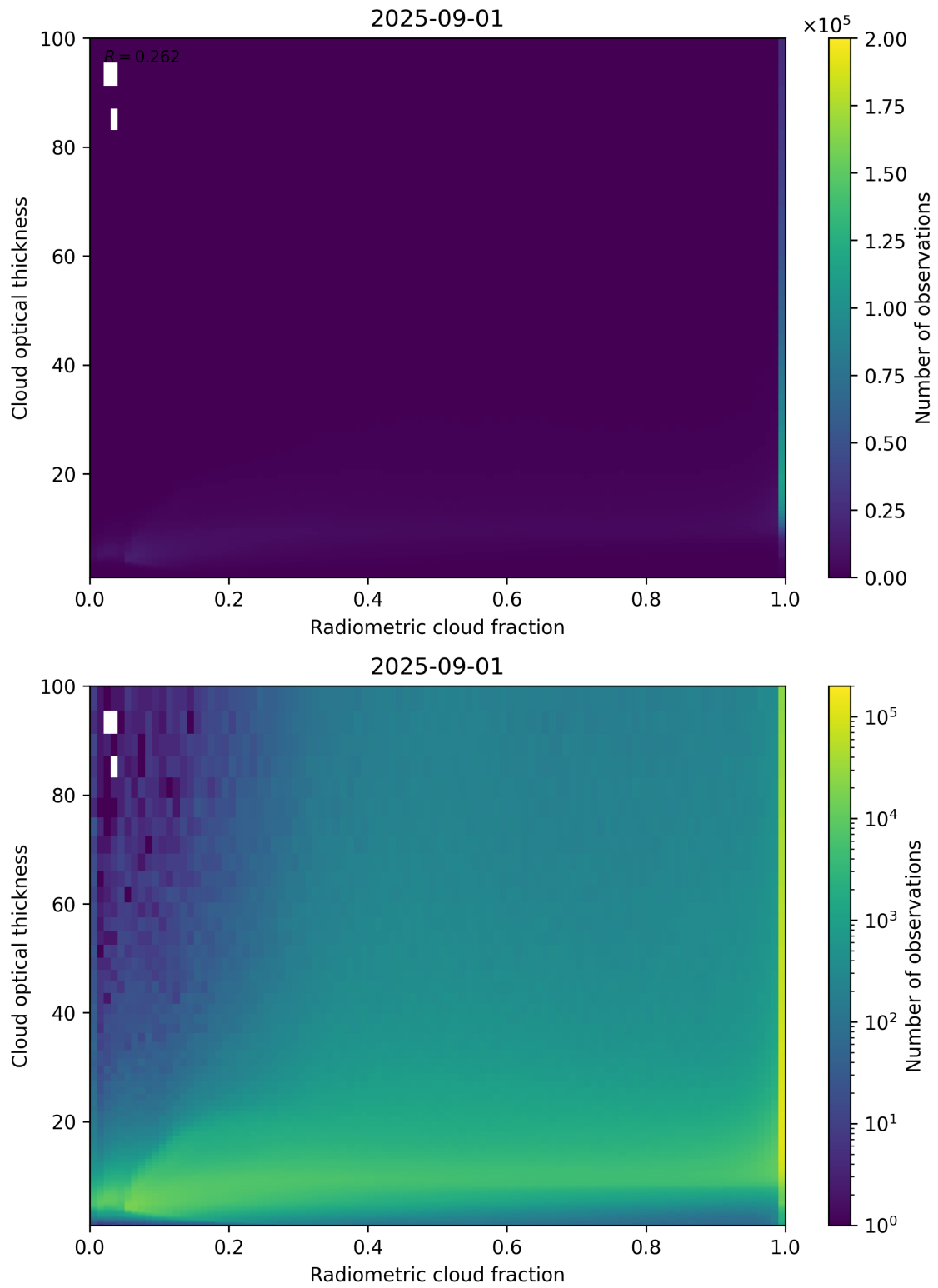
Figure 75: Scatter density plot of “Radiometric cloud fraction” against “Cloud optical thickness” for 2025-08-31 to 2025-09-02.
