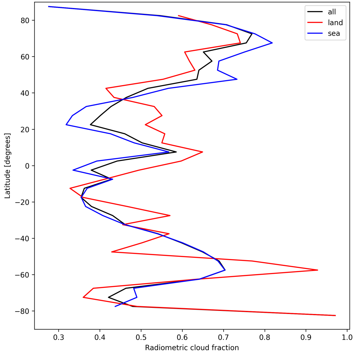
Figure 23: Zonal average of “Radiometric cloud fraction” for 2025-08-31 to 2025-09-02.
