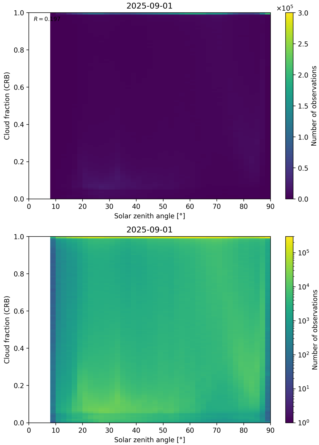
Figure 101: Scatter density plot of “Solar zenith angle” against “Cloud fraction (CRB)” for 2025-08-31 to 2025-09-02.
