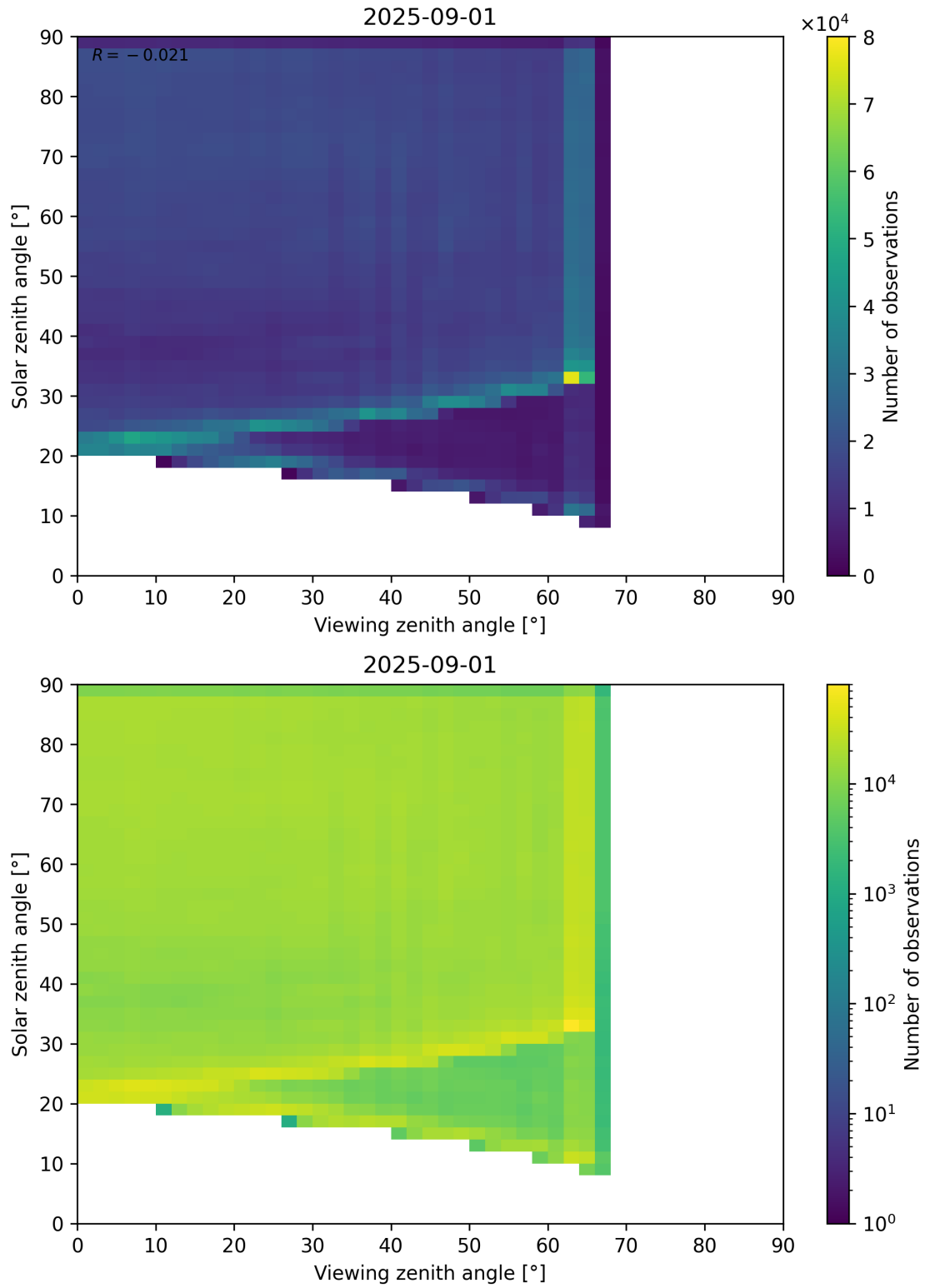
Figure 114: Scatter density plot of “Viewing zenith angle” against “Solar zenith angle” for 2025-08-31 to 2025-09-02.
