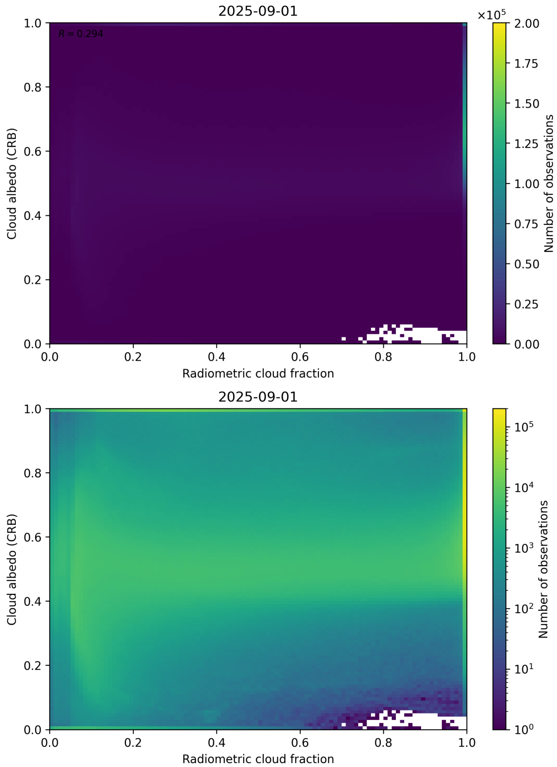
Figure 71: Scatter density plot of “Radiometric cloud fraction” against “Cloud albedo (CRB)” for 2025-08-31 to 2025-09-02.
