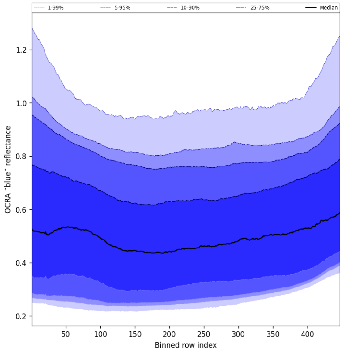
Figure 67: Along track statistics of “OCRA “blue” reflectance” for 2025-08-31 to 2025-09-02
