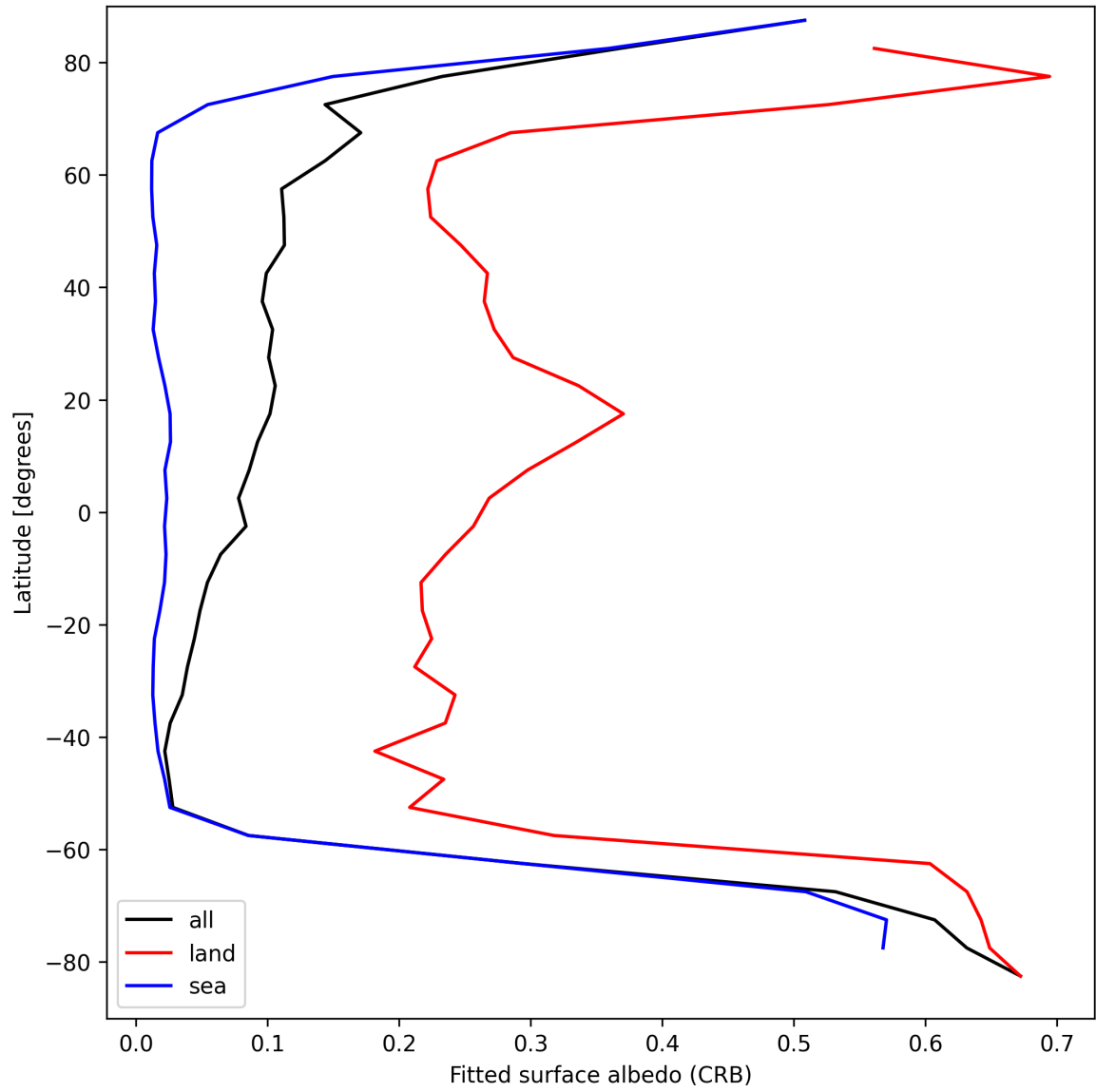
Figure 30: Zonal average of "Fitted surface albedo (CRB)" for 2025-08-31 to 2025-09-02.
