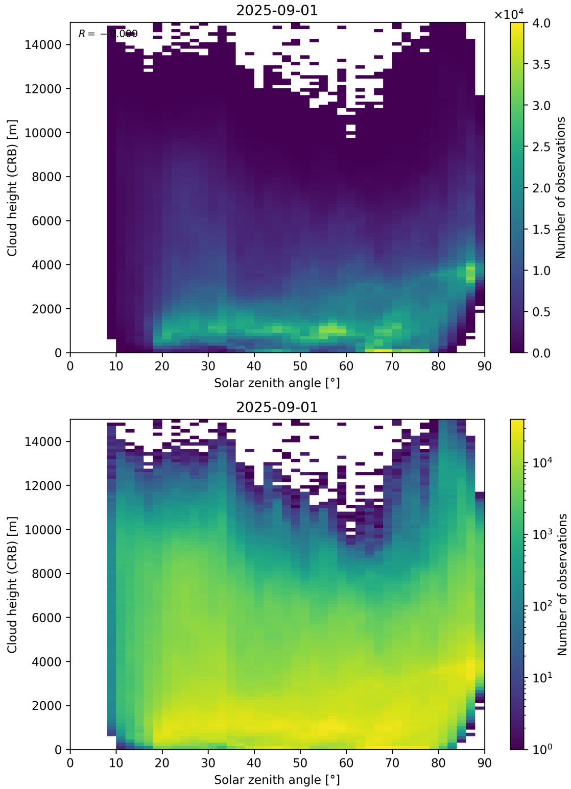
Figure 102: Scatter density plot of “Solar zenith angle” against “Cloud height (CRB)” for 2025-08-31 to 2025-09-02.
