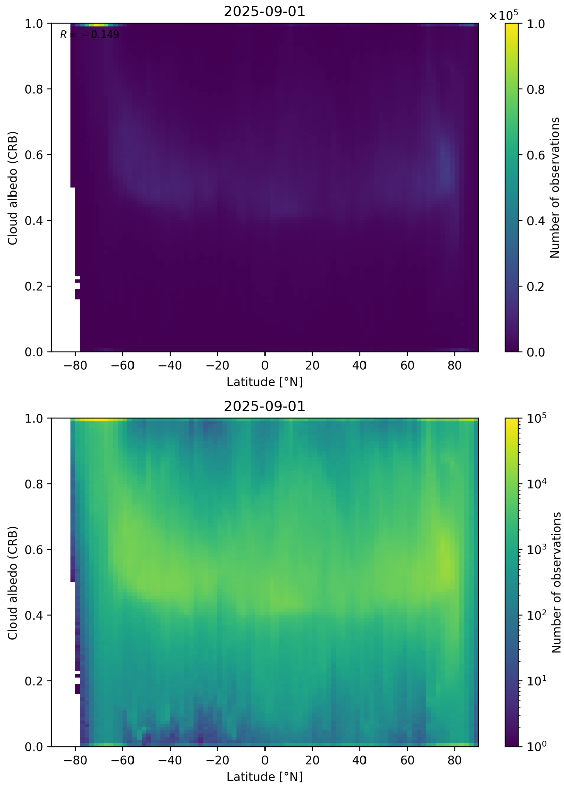
Figure 91: Scatter density plot of “Latitude” against “Cloud albedo (CRB)” for 2025-08-31 to 2025-09-02.
