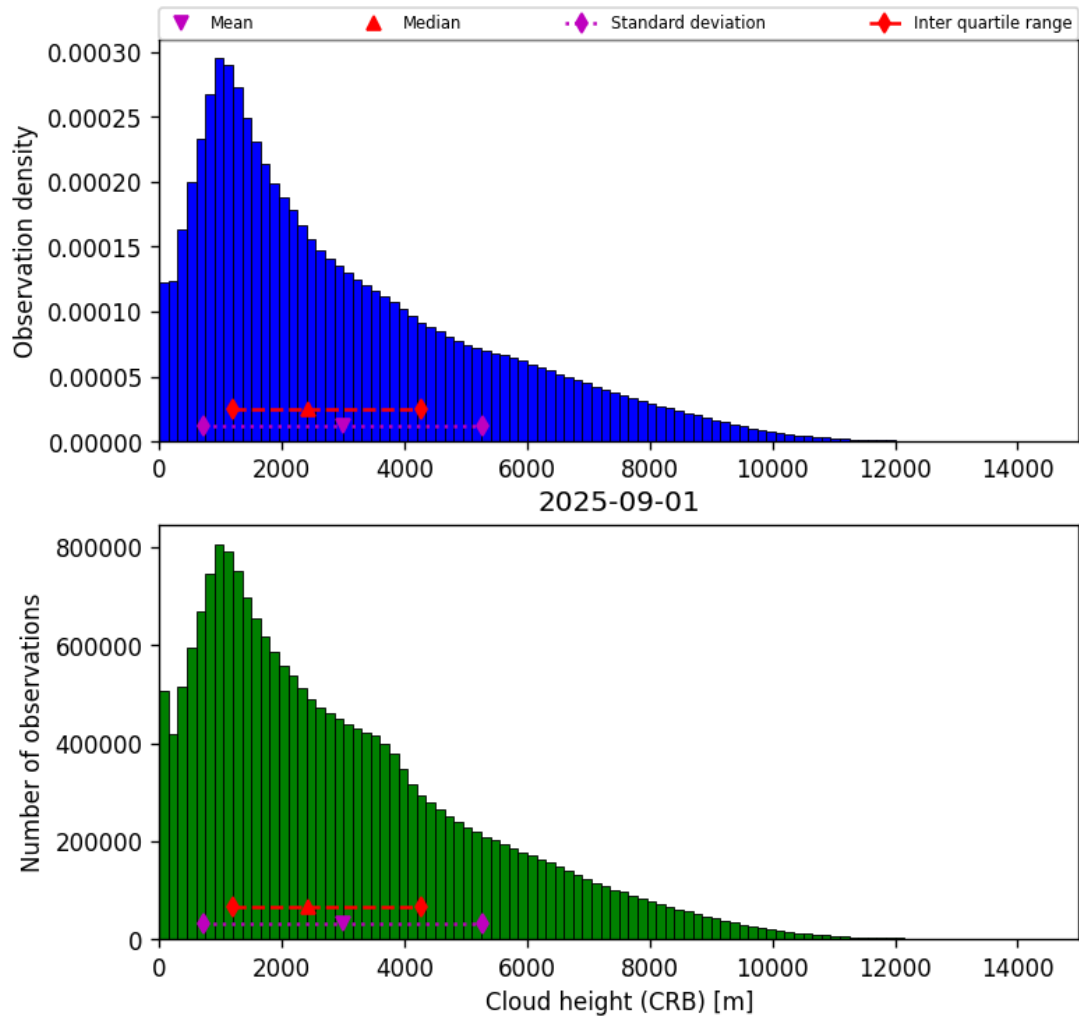
Figure 43: Histogram of “Cloud height (CRB)” for 2025-08-31 to 2025-09-02
