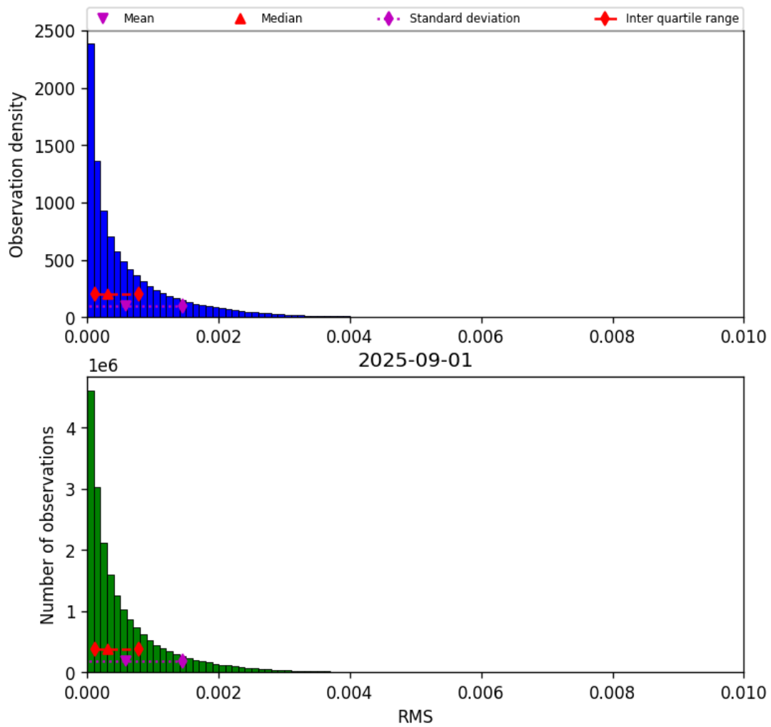
Figure 47: Histogram of “RMS” for 2025-08-31 to 2025-09-02
