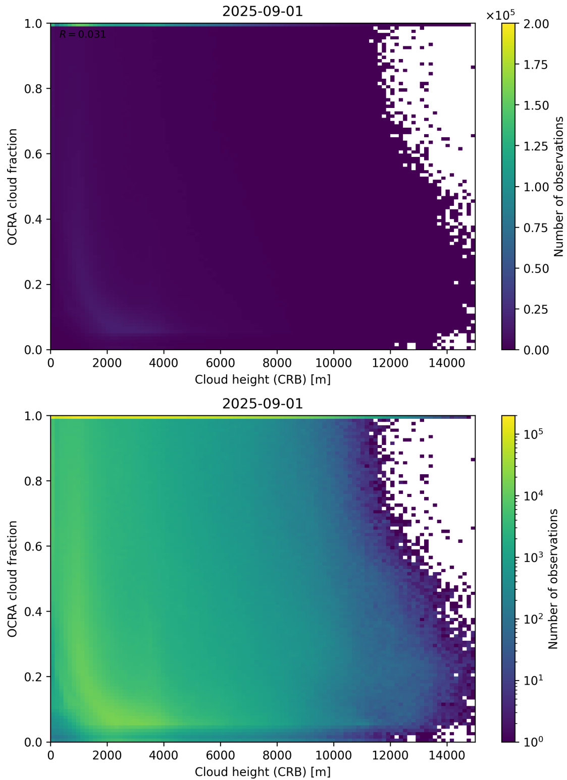
Figure 81: Scatter density plot of “Cloud height (CRB)” against “OCRA cloud fraction” for 2025-08-31 to 2025-09-02.
