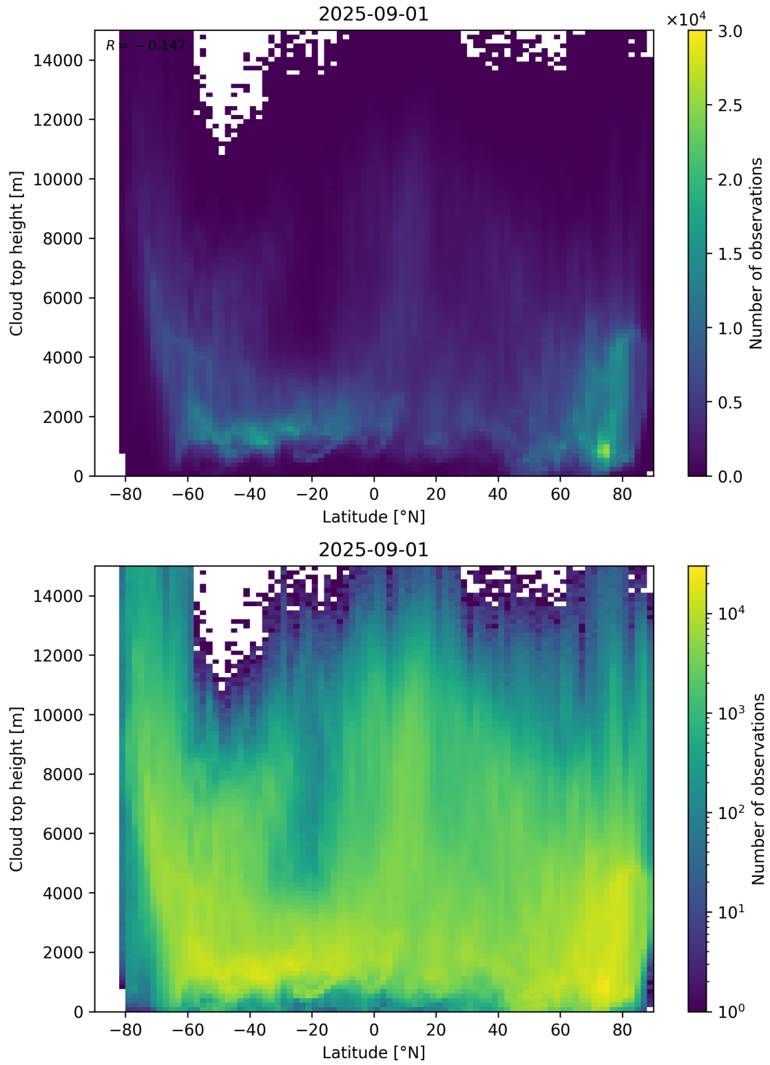
Figure 97: Scatter density plot of “Latitude” against “Cloud top height” for 2025-08-31 to 2025-09-02.
