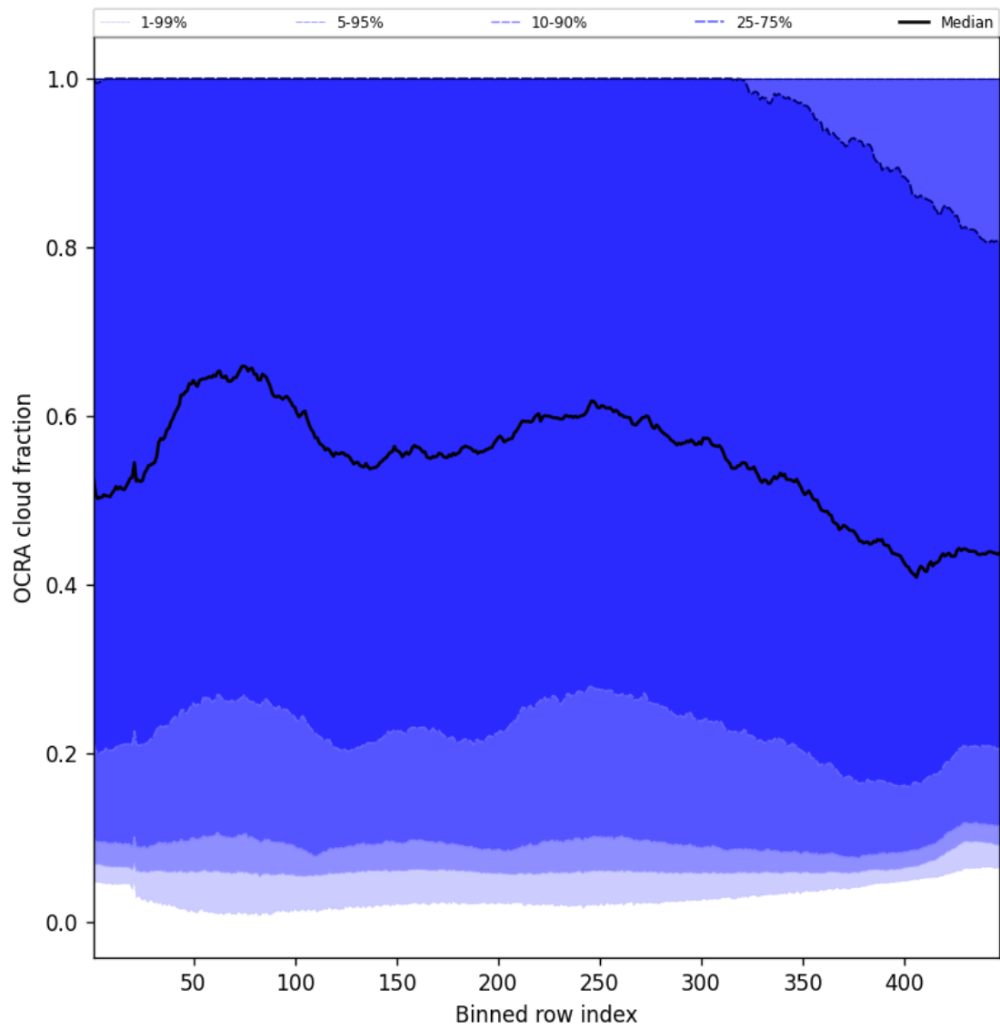
Figure 66: Along track statistics of “OCRA cloud fraction” for 2025-08-31 to 2025-09-02
