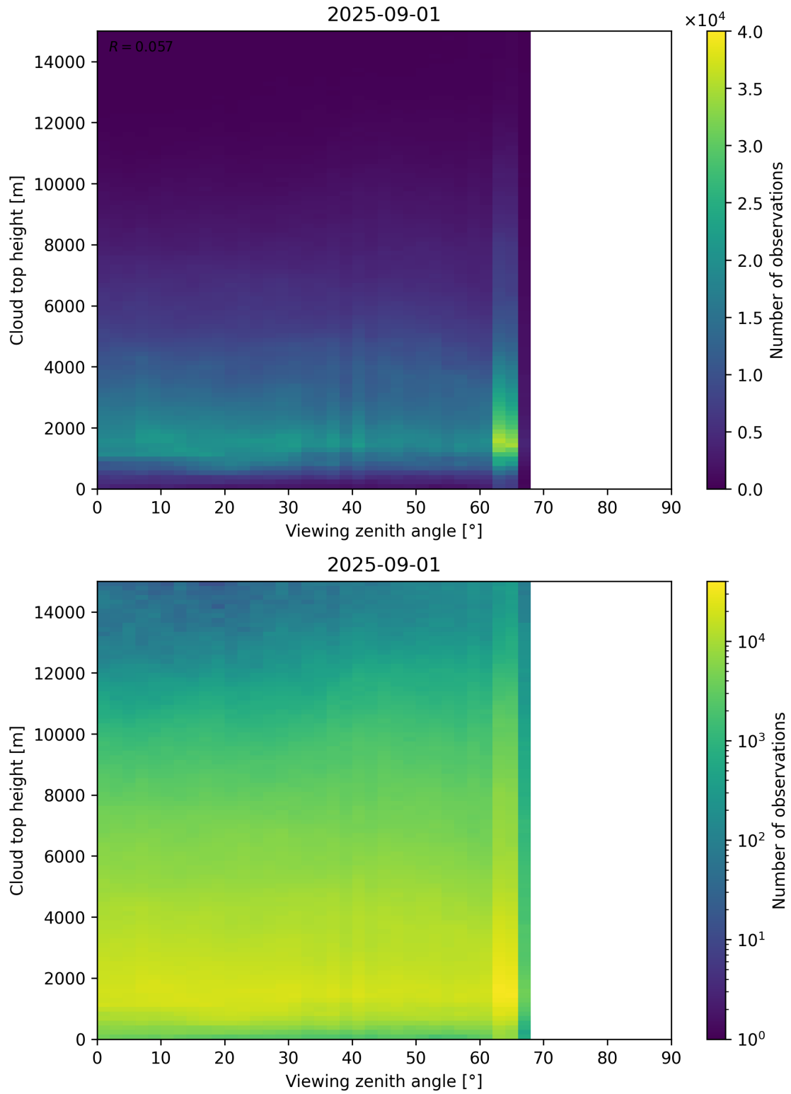
Figure 112: Scatter density plot of “Viewing zenith angle” against “Cloud top height” for 2025-08-31 to 2025-09-02.
