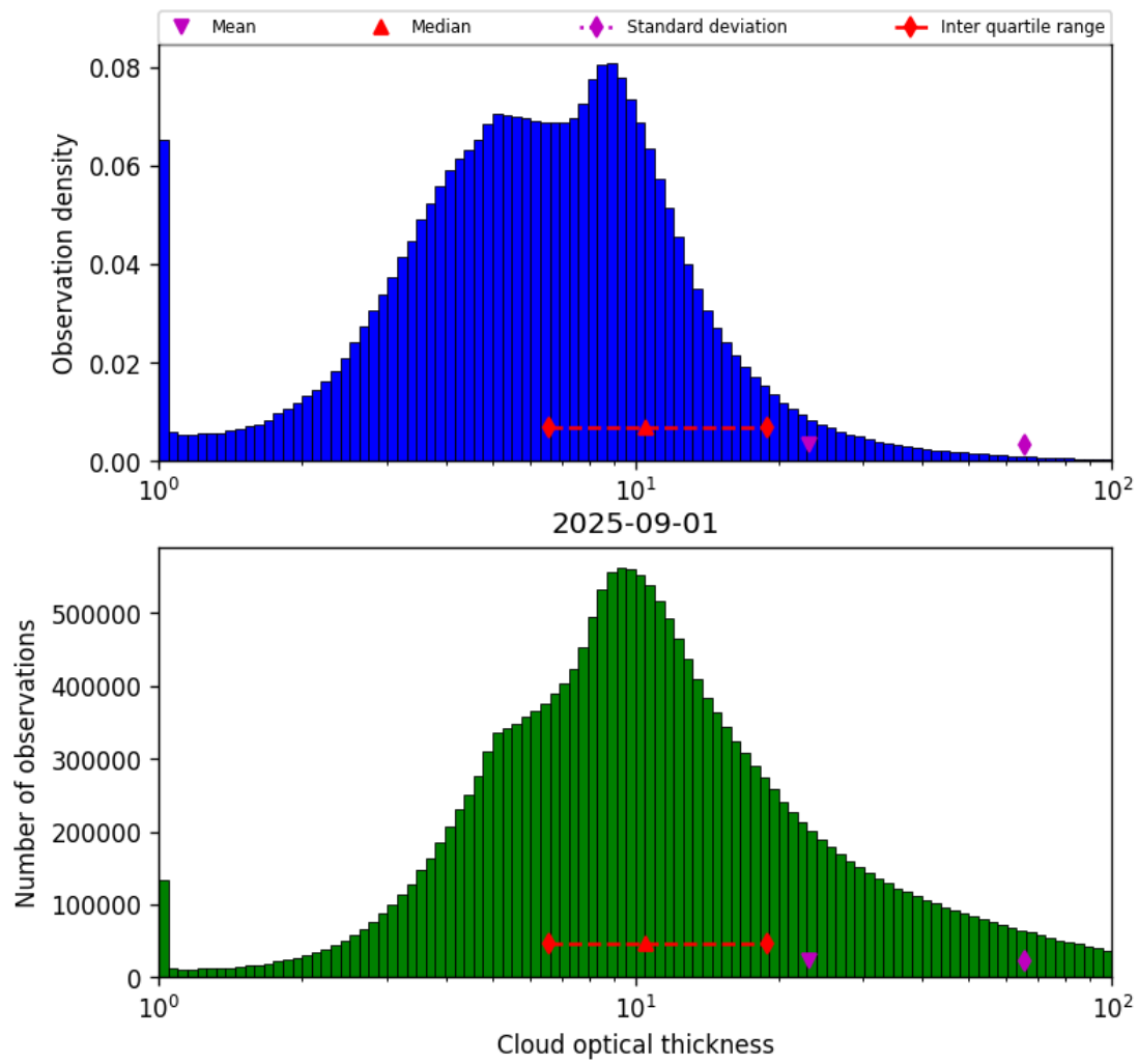
Figure 41: Histogram of “Cloud optical thickness” for 2025-08-31 to 2025-09-02
