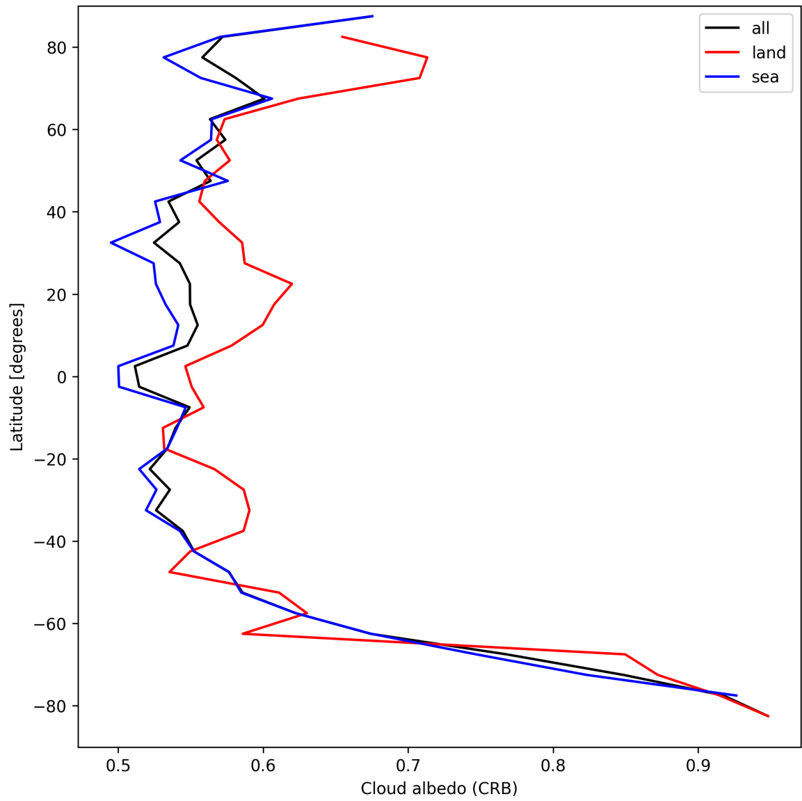
Figure 28: Zonal average of “Cloud albedo (CRB)” for 2025-08-31 to 2025-09-02.
