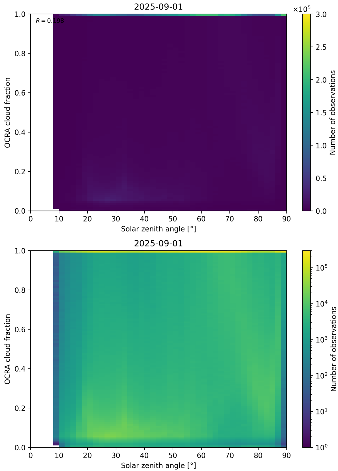
Figure 100: Scatter density plot of “Solar zenith angle” against “OCRA cloud fraction” for 2025-08-31 to 2025-09-02.
