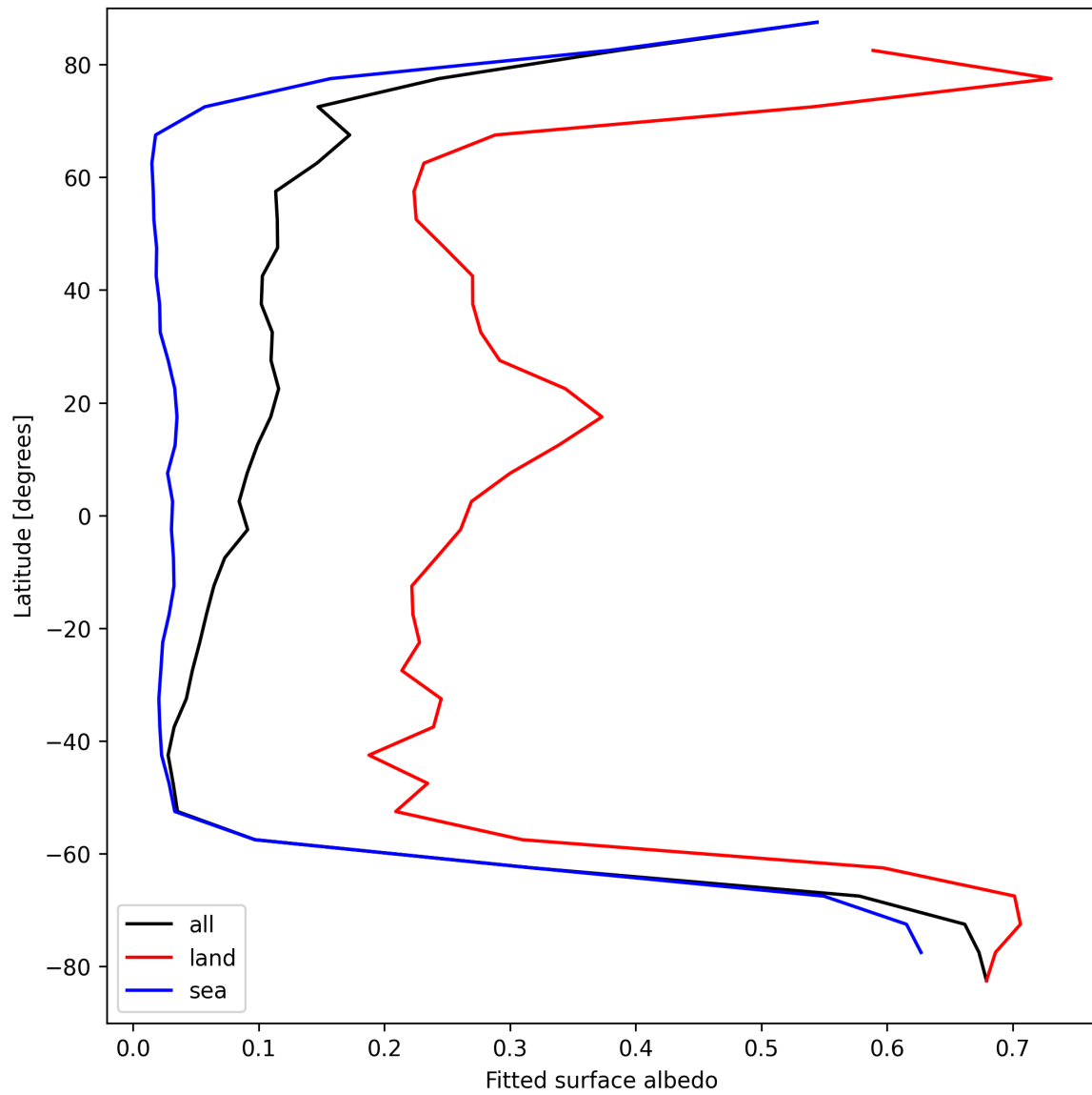
Figure 29: Zonal average of “Fitted surface albedo” for 2025-08-31 to 2025-09-02.
