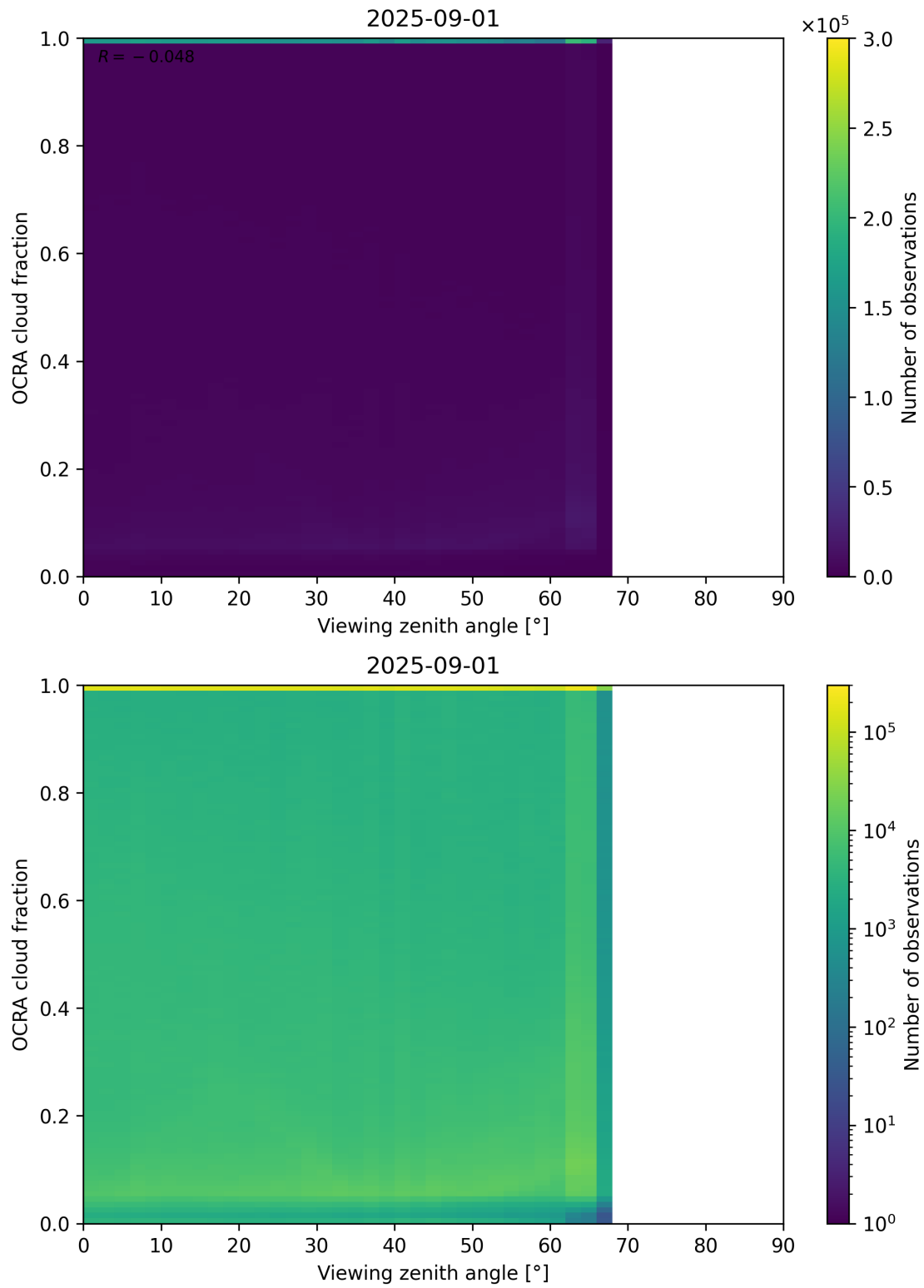
Figure 108: Scatter density plot of “Viewing zenith angle” against “OCRA cloud fraction” for 2025-08-31 to 2025-09-02.
