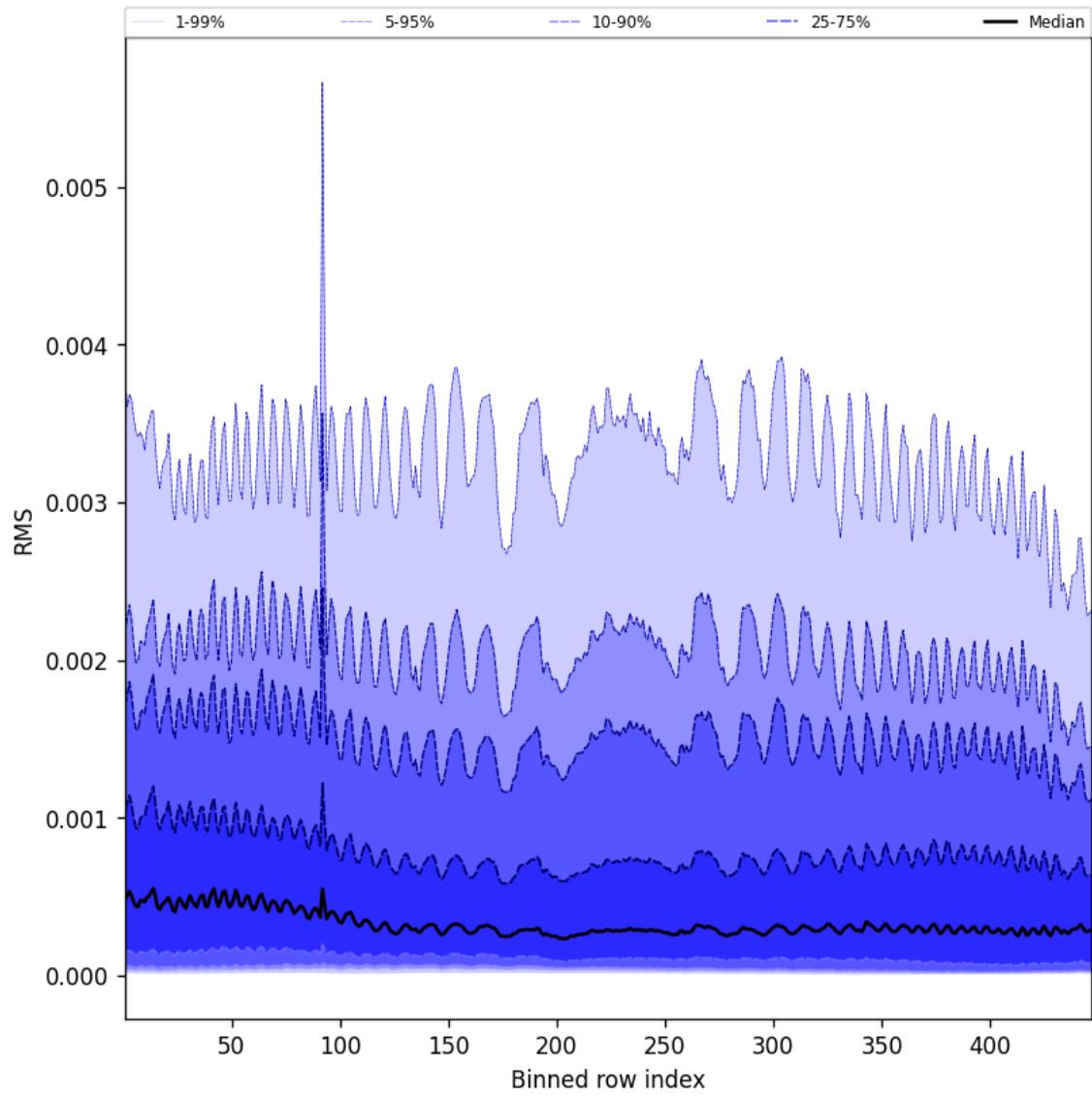
Figure 63: Along track statistics of “RMS” for 2025-08-31 to 2025-09-02
