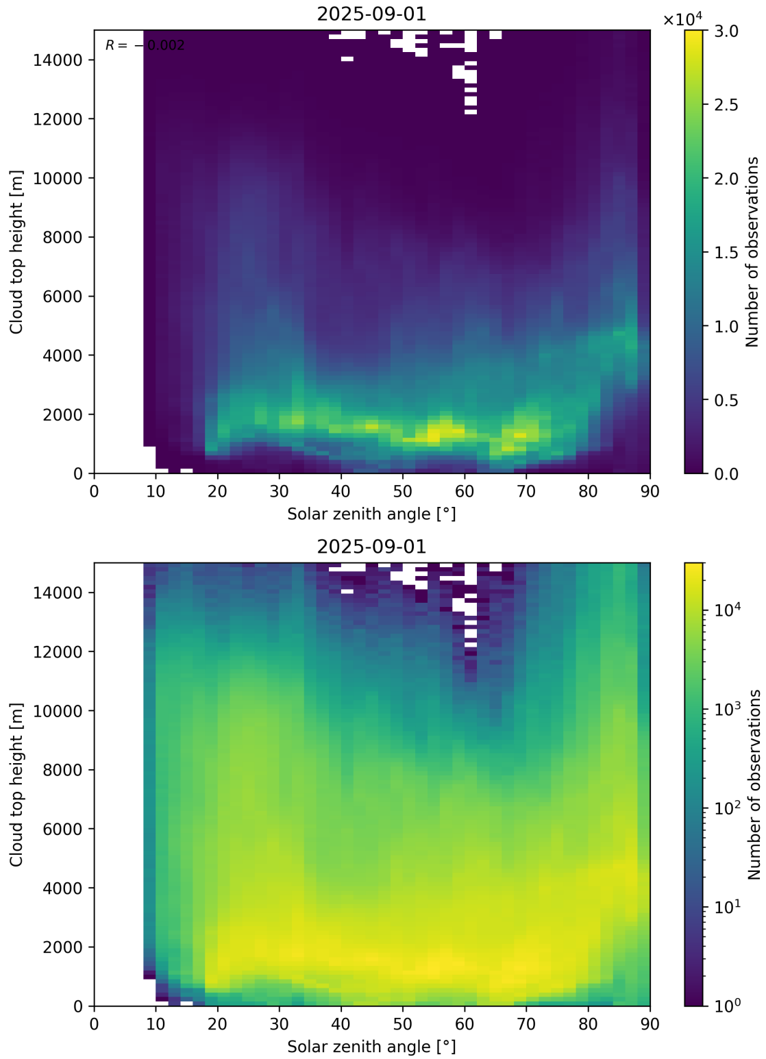
Figure 104: Scatter density plot of “Solar zenith angle” against “Cloud top height” for 2025-08-31 to 2025-09-02.
