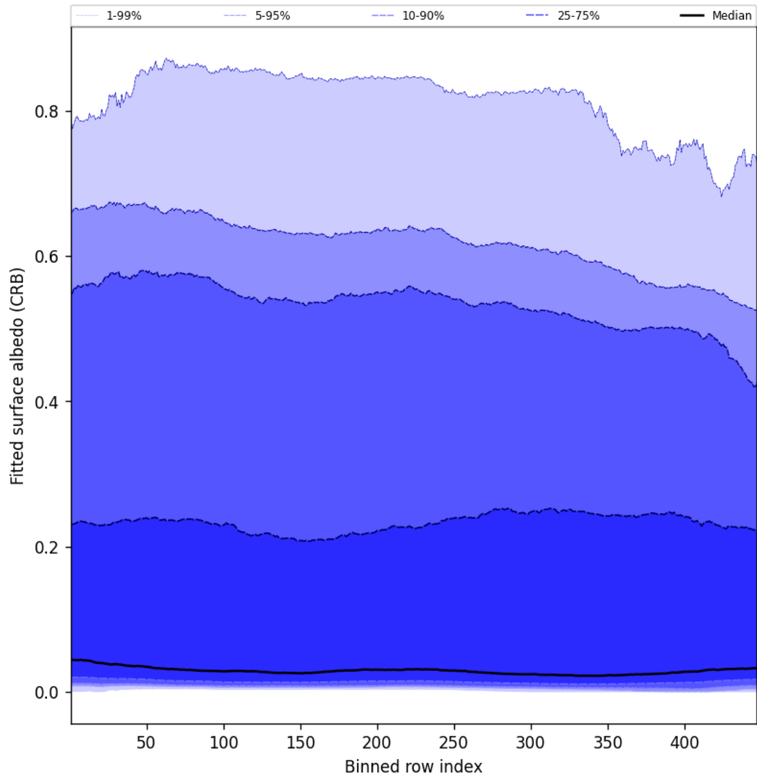
Figure 62: Along track statistics of “Fitted surface albedo (CRB)” for 2025-08-31 to 2025-09-02
