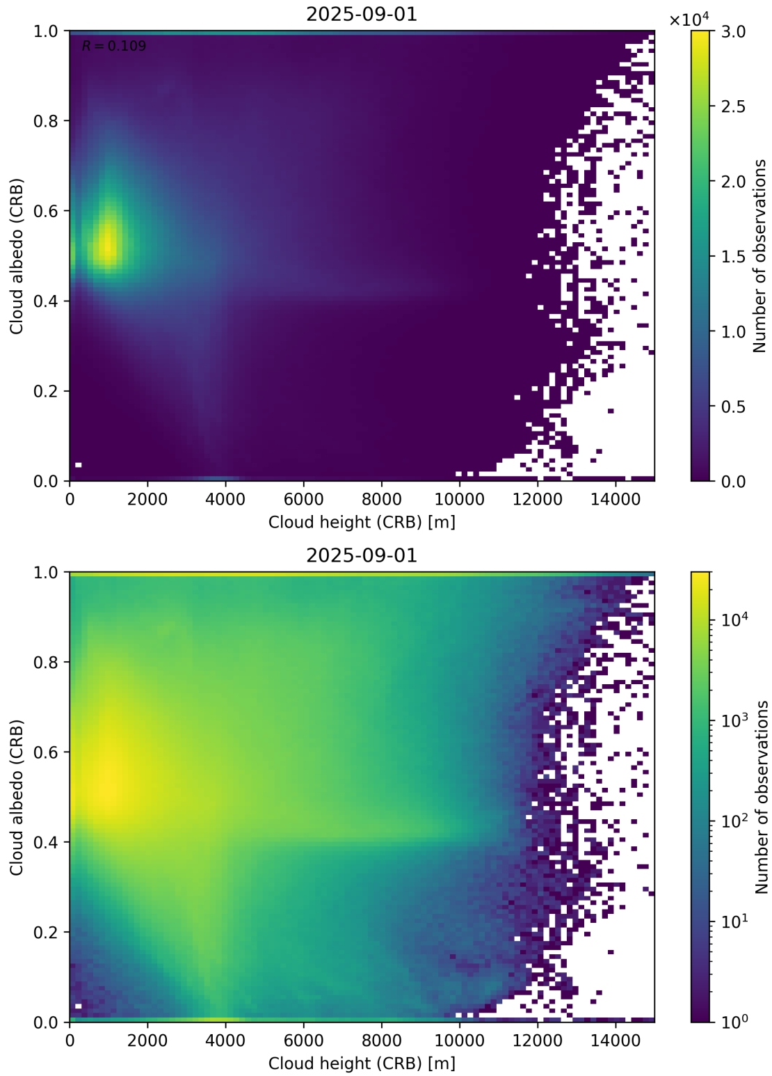
Figure 80: Scatter density plot of “Cloud height (CRB)” against “Cloud albedo (CRB)” for 2025-08-31 to 2025-09-02.
