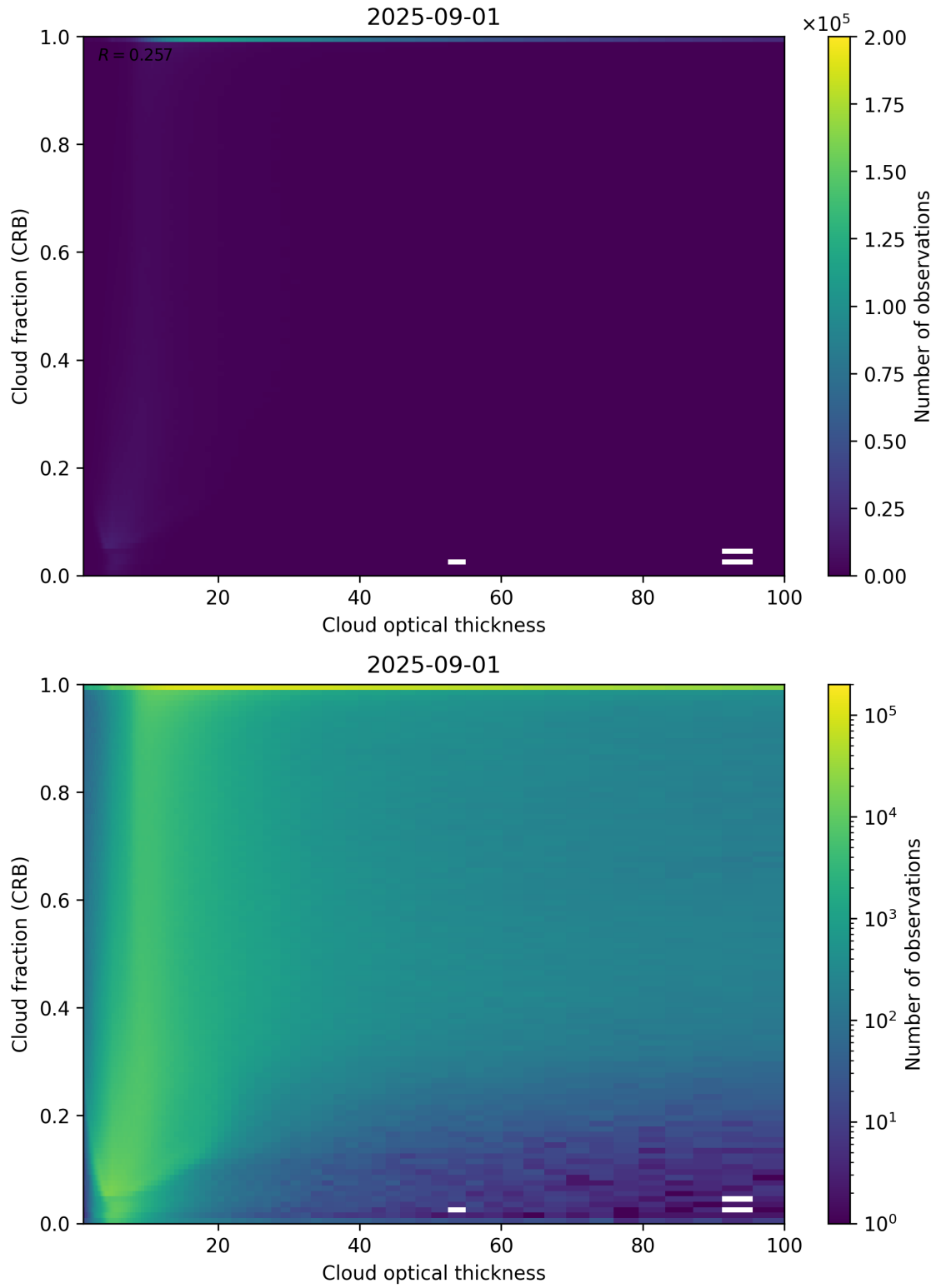
Figure 84: Scatter density plot of “Cloud optical thickness” against “Cloud fraction (CRB)” for 2025-08-31 to 2025-09-02.
