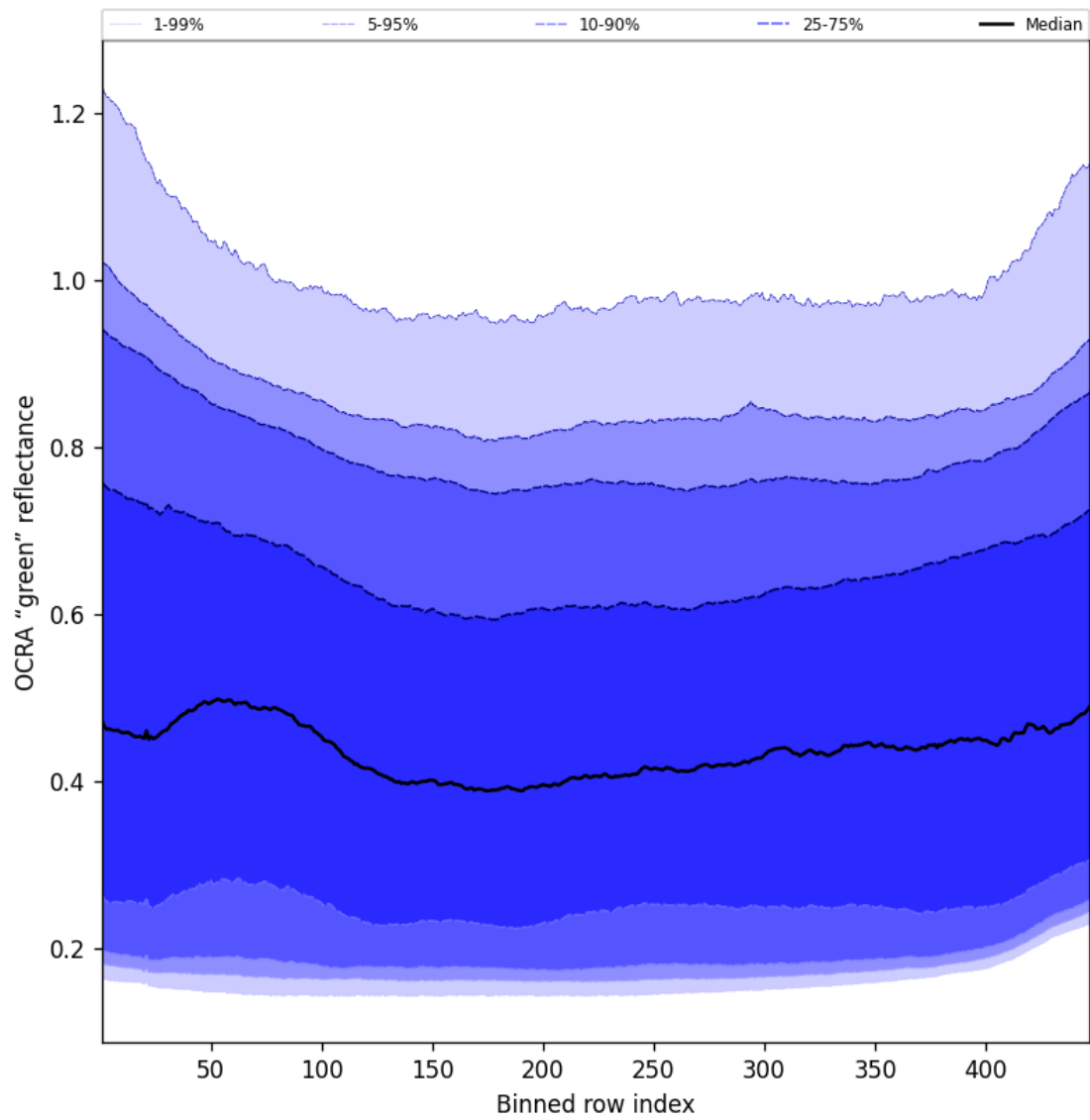
Figure 68: Along track statistics of “OCRA “green” reflectance” for 2025-08-31 to 2025-09-02
