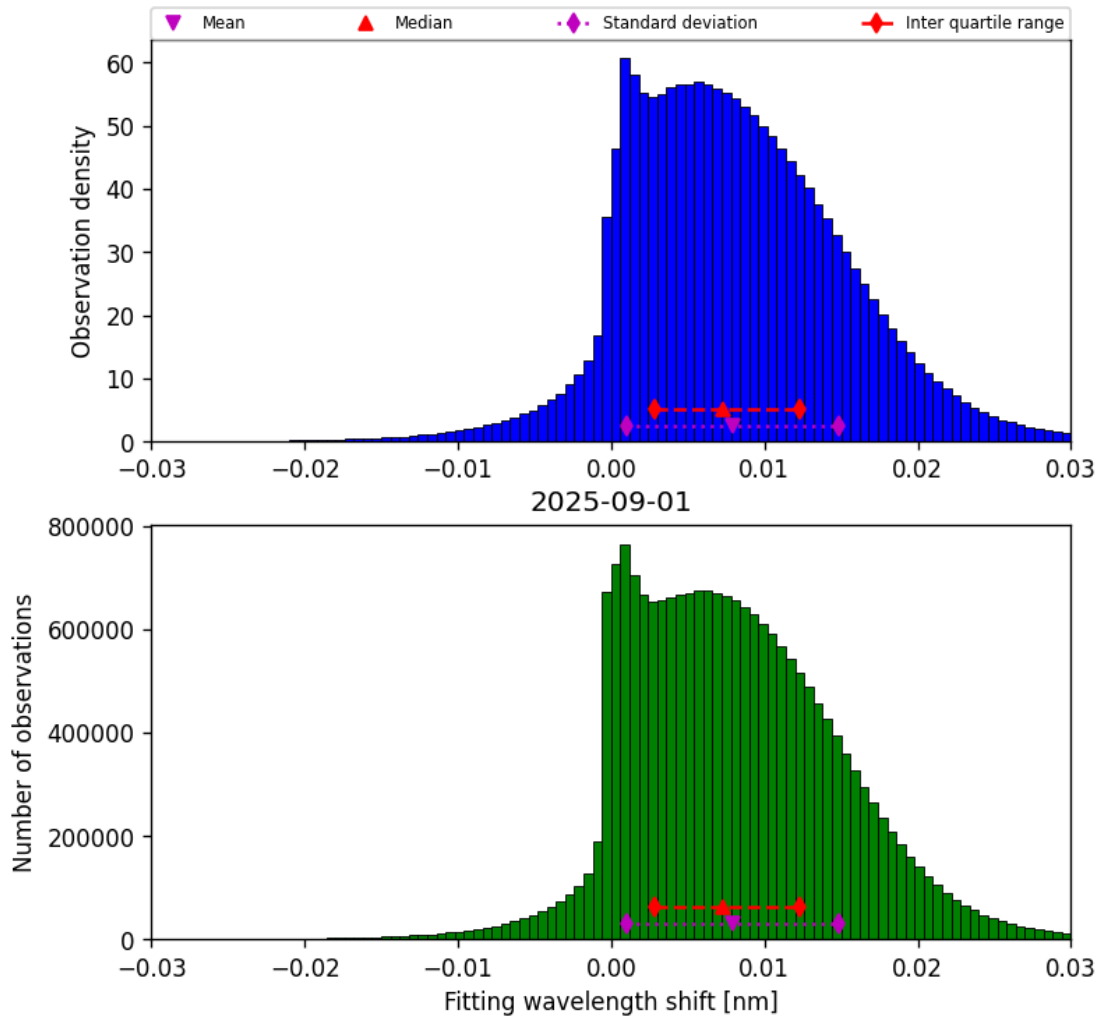
Figure 49: Histogram of “Fitting wavelength shift” for 2025-08-31 to 2025-09-02
