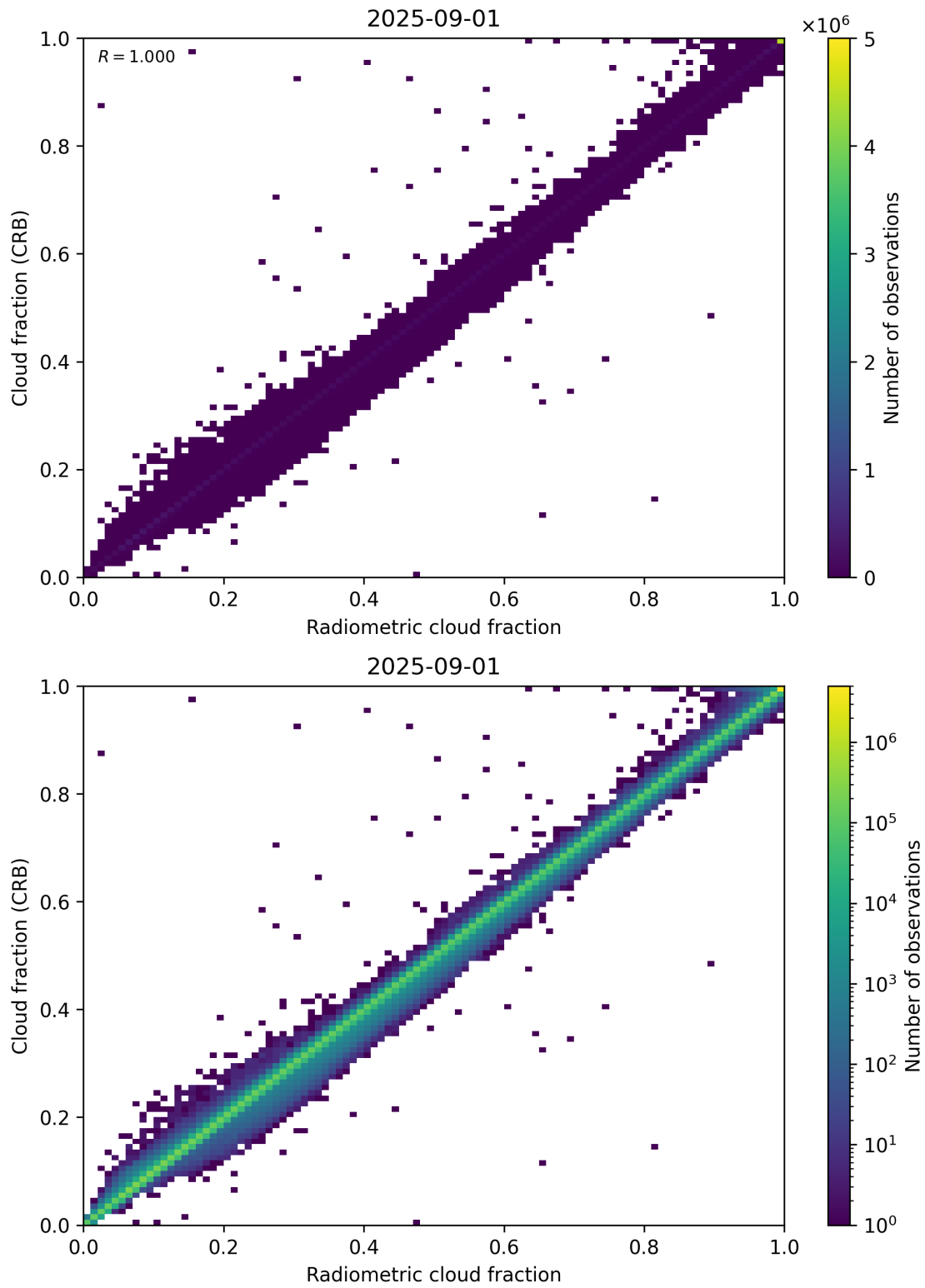
Figure 73: Scatter density plot of “Radiometric cloud fraction” against “Cloud fraction (CRB)” for 2025-08-31 to 2025-09-02.
