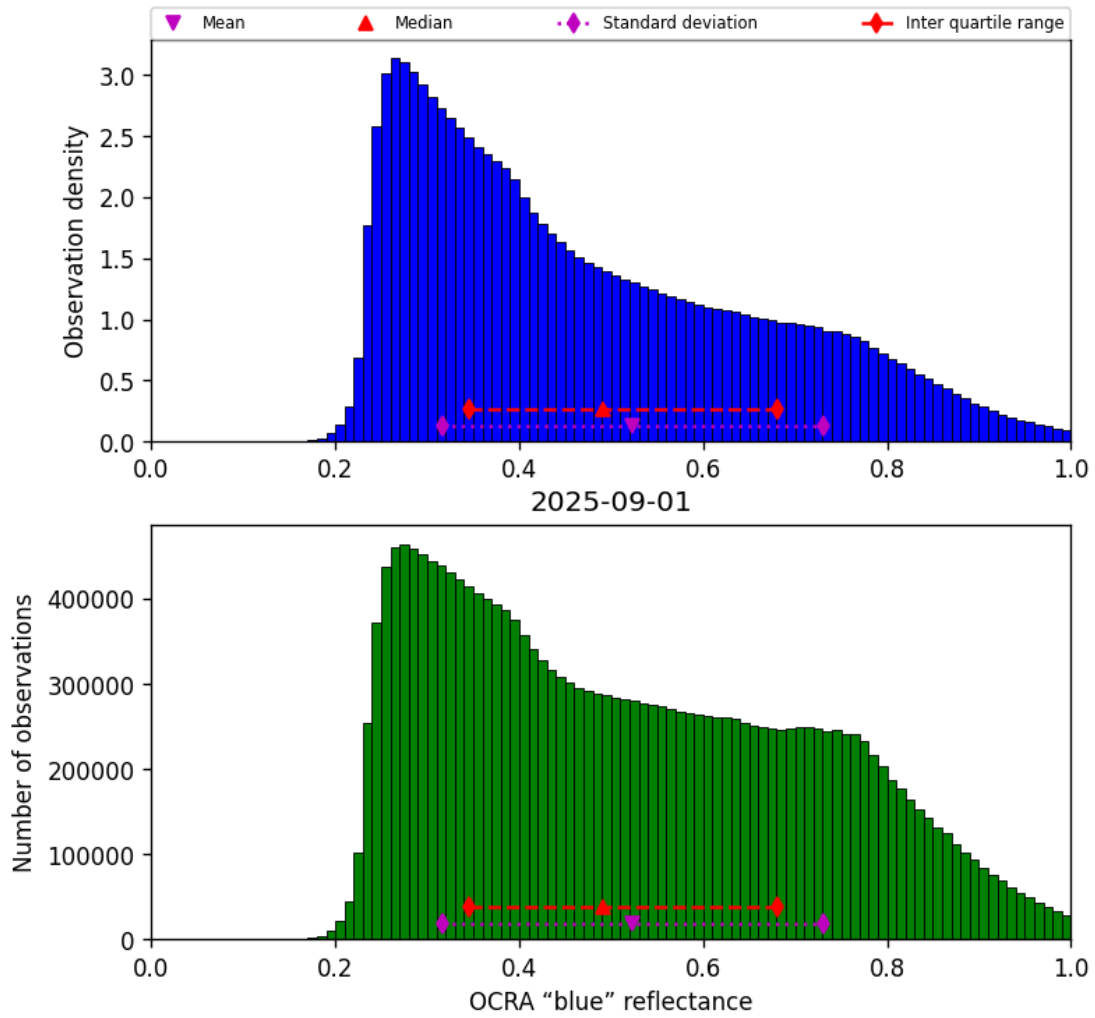
Figure 51: Histogram of “OCRA “blue” reflectance” for 2025-08-31 to 2025-09-02
