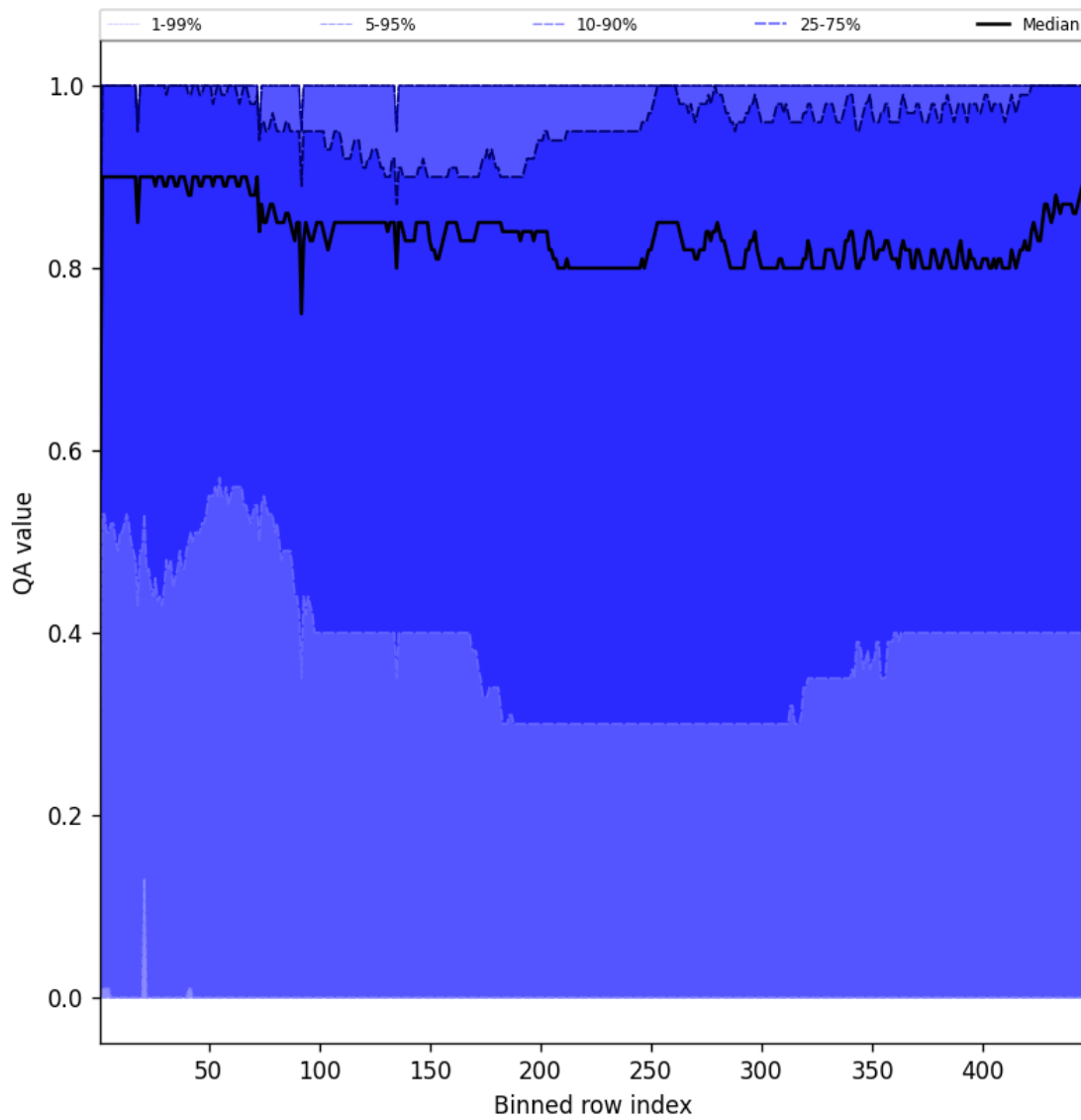
Figure 54: Along track statistics of “QA value” for 2025-08-31 to 2025-09-02
