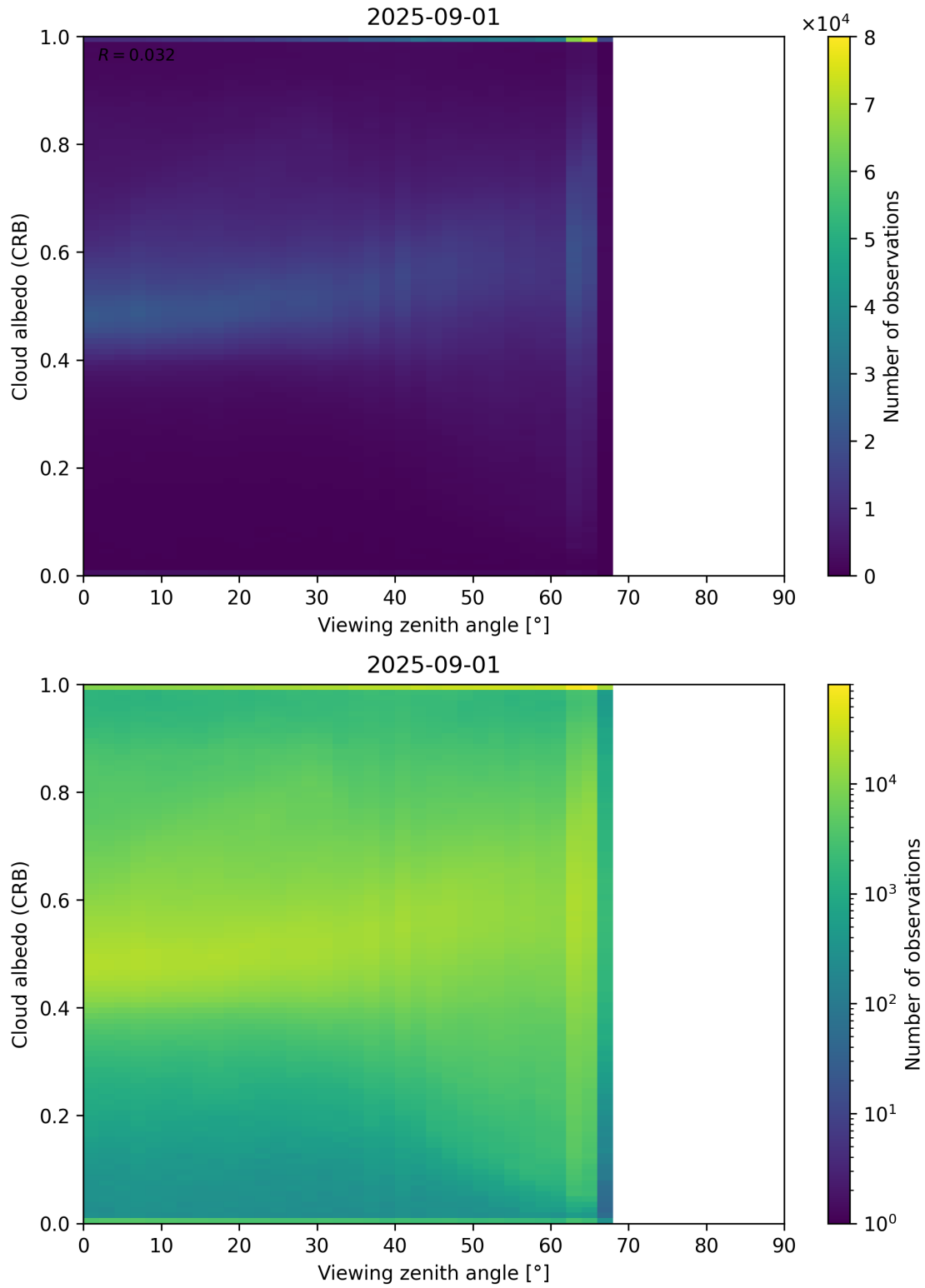
Figure 106: Scatter density plot of “Viewing zenith angle” against “Cloud albedo (CRB)” for 2025-08-31 to 2025-09-02.
