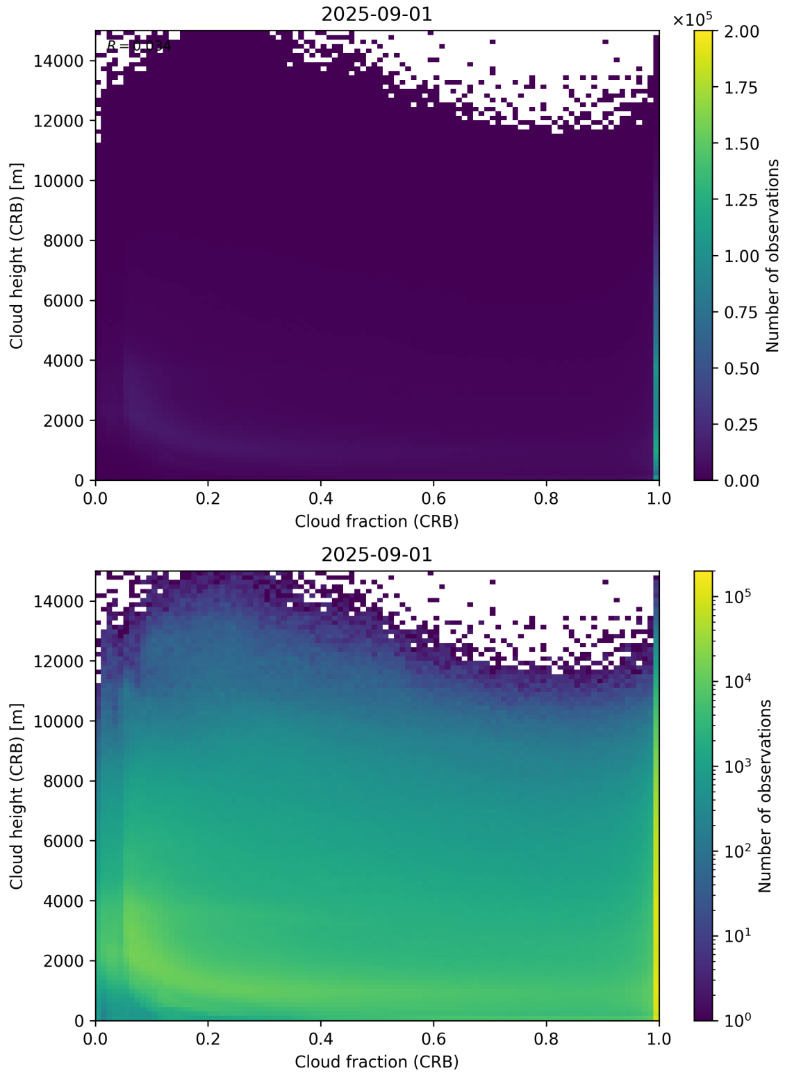
Figure 79: Scatter density plot of “Cloud fraction (CRB)” against “Cloud height (CRB)” for 2025-08-31 to 2025-09-02.
