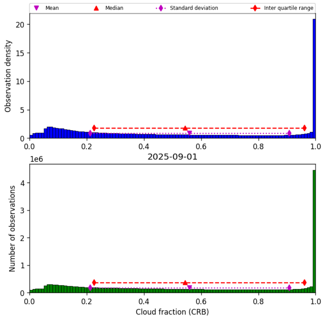
Figure 42: Histogram of “Cloud fraction (CRB)” for 2025-08-31 to 2025-09-02
