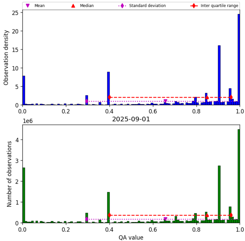
Figure 38: Histogram of “QA value” for 2025-08-31 to 2025-09-02
