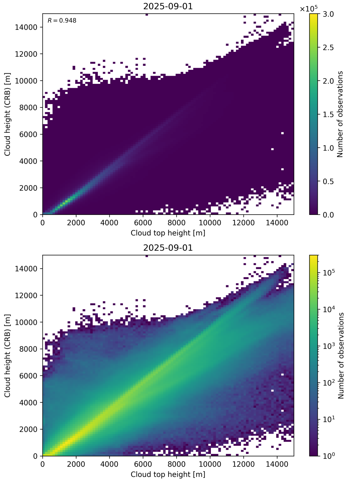
Figure 89: Scatter density plot of “Cloud top height” against “Cloud height (CRB)” for 2025-08-31 to 2025-09-02.
