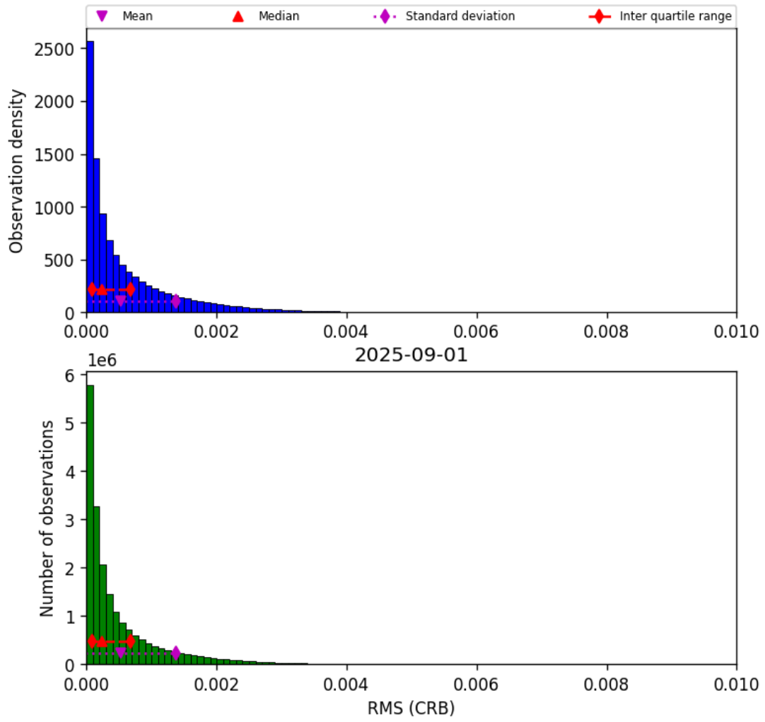
Figure 48: Histogram of “RMS (CRB)” for 2025-08-31 to 2025-09-02
