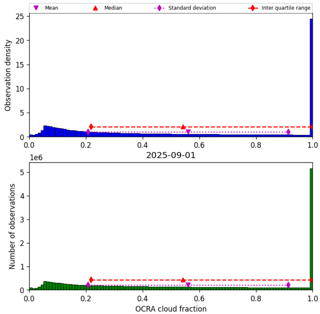
Figure 50: Histogram of “OCRA cloud fraction” for 2025-08-31 to 2025-09-02
