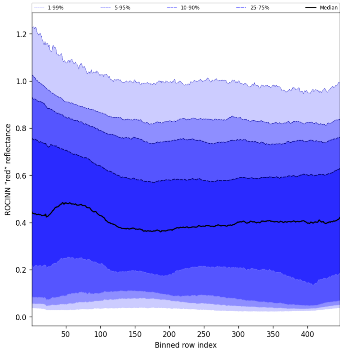
Figure 69: Along track statistics of "ROCINN "red" reflectance" for 2025-08-31 to 2025-09-02
