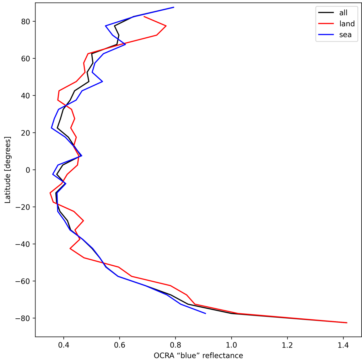
Figure 35: Zonal average of “OCRA “blue” reflectance” for 2025-08-31 to 2025-09-02.
