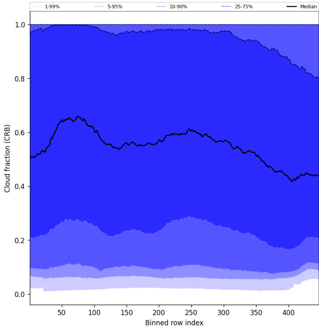
Figure 58: Along track statistics of “Cloud fraction (CRB)” for 2025-08-31 to 2025-09-02
