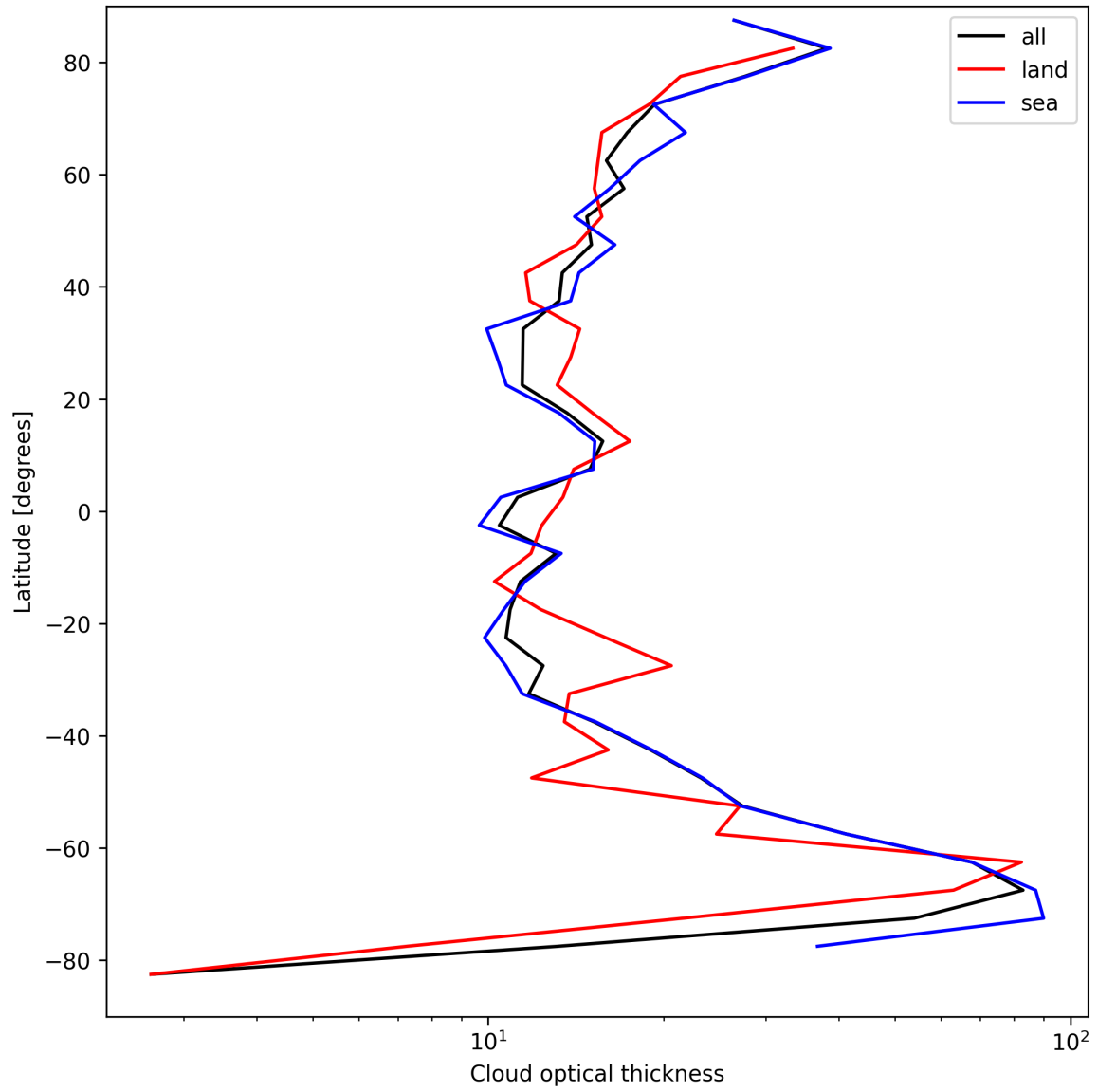
Figure 25: Zonal average of “Cloud optical thickness” for 2025-08-31 to 2025-09-02.
