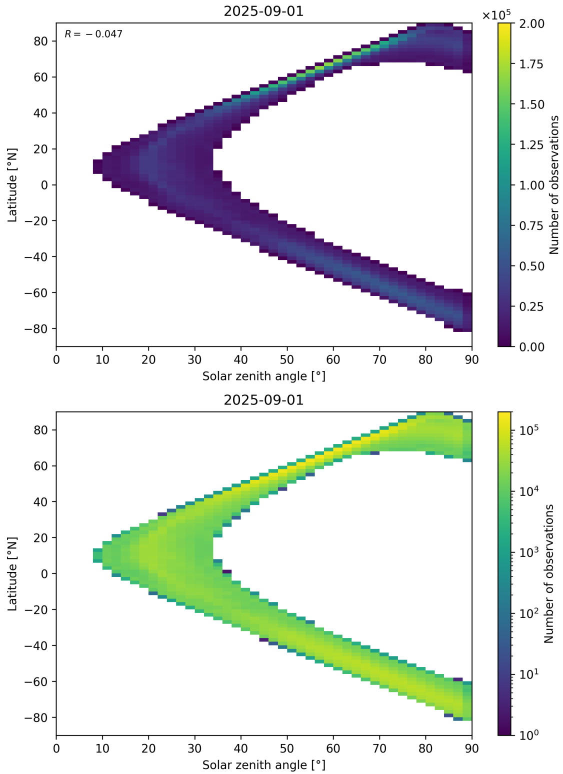
Figure 105: Scatter density plot of “Solar zenith angle” against “Latitude” for 2025-08-31 to 2025-09-02.
