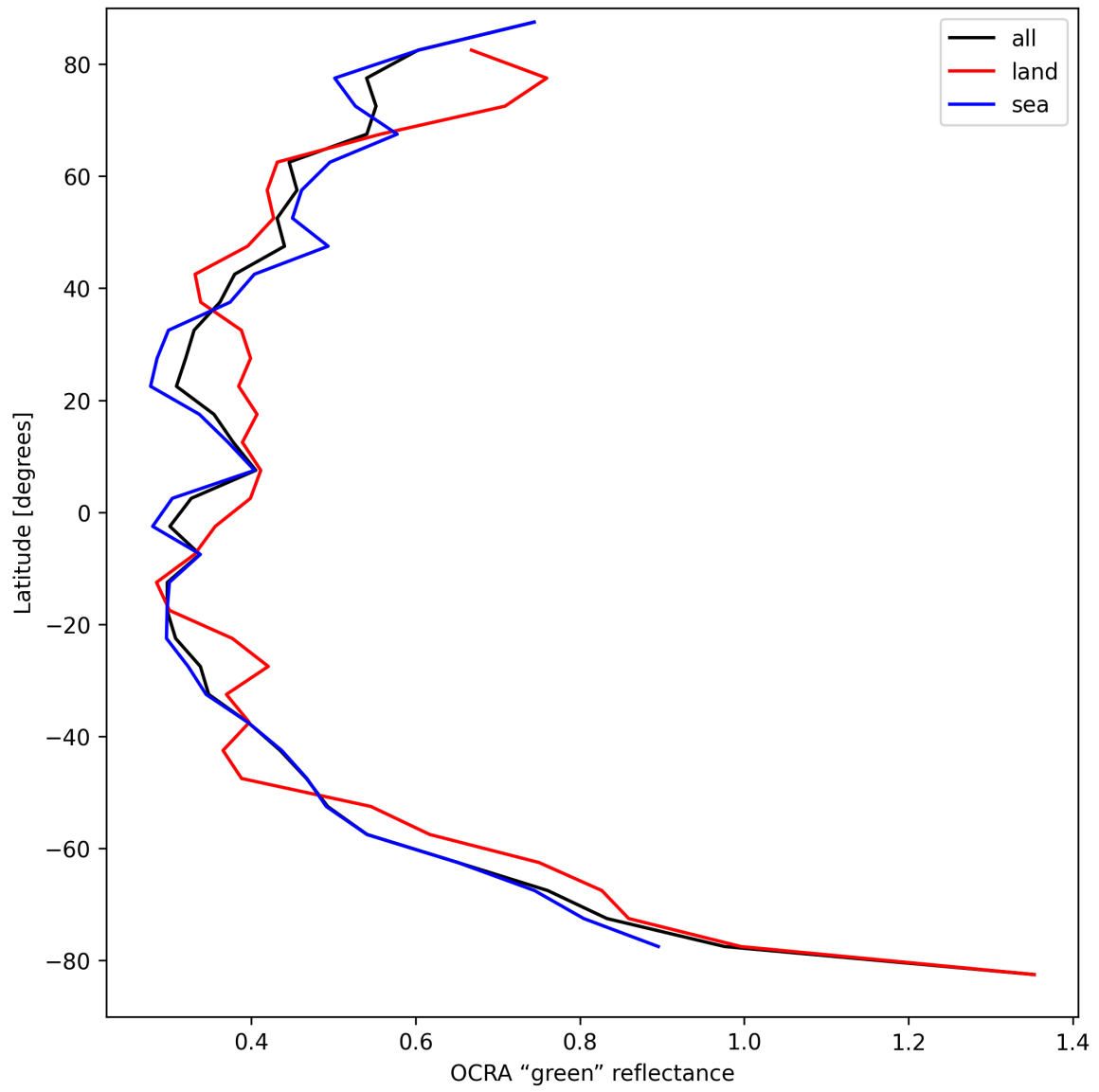
Figure 36: Zonal average of "OCRA "green" reflectance" for 2025-08-31 to 2025-09-02.
