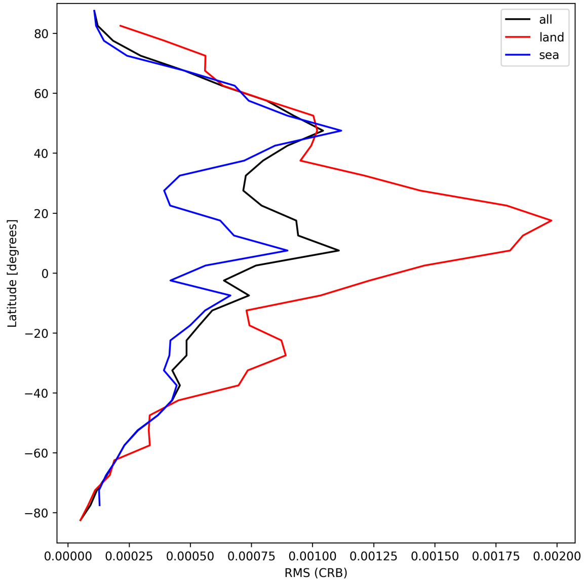
Figure 32: Zonal average of “RMS (CRB)” for 2025-08-31 to 2025-09-02.
