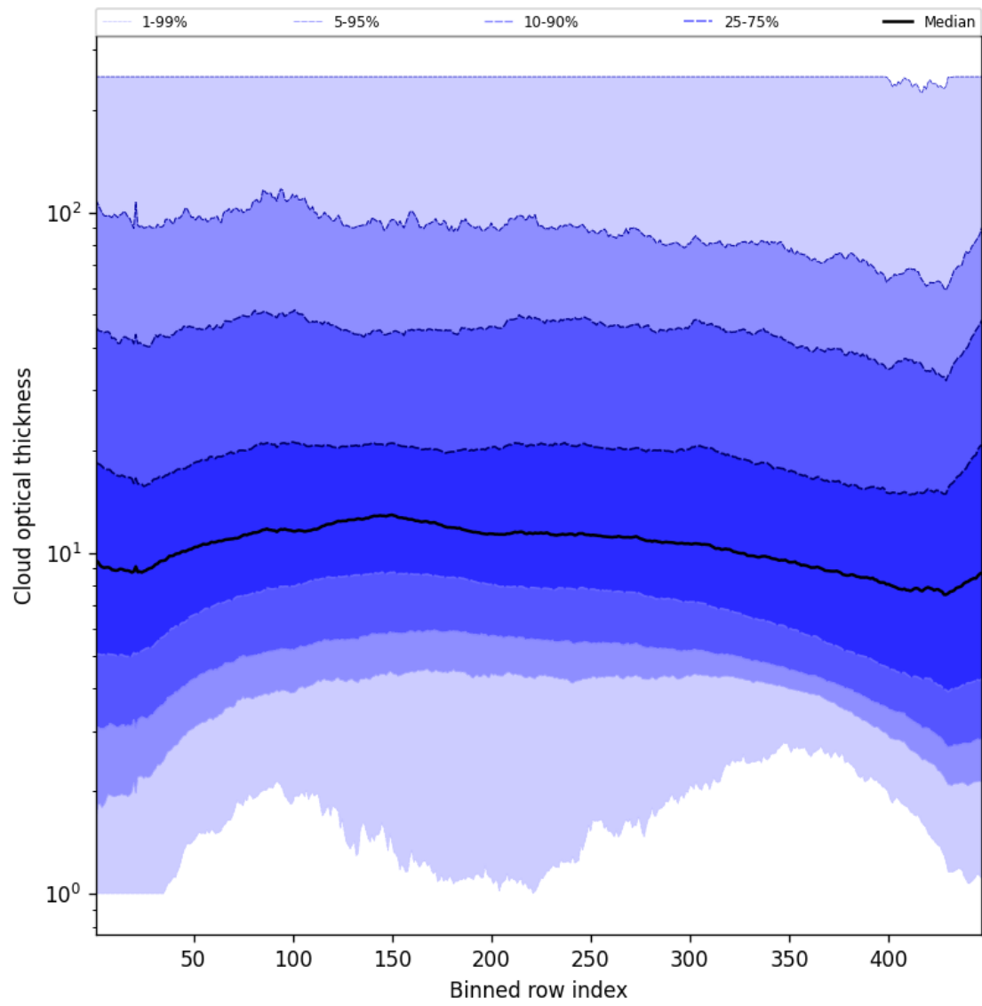
Figure 57: Along track statistics of “Cloud optical thickness” for 2025-08-31 to 2025-09-02
