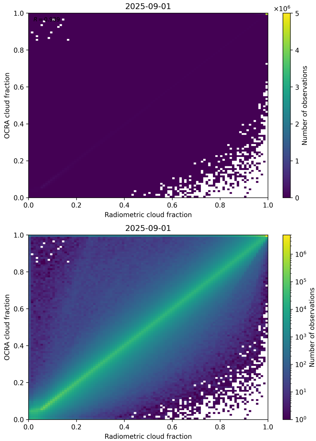
Figure 72: Scatter density plot of “Radiometric cloud fraction” against “OCRA cloud fraction” for 2025-08-31 to 2025-09-02.
