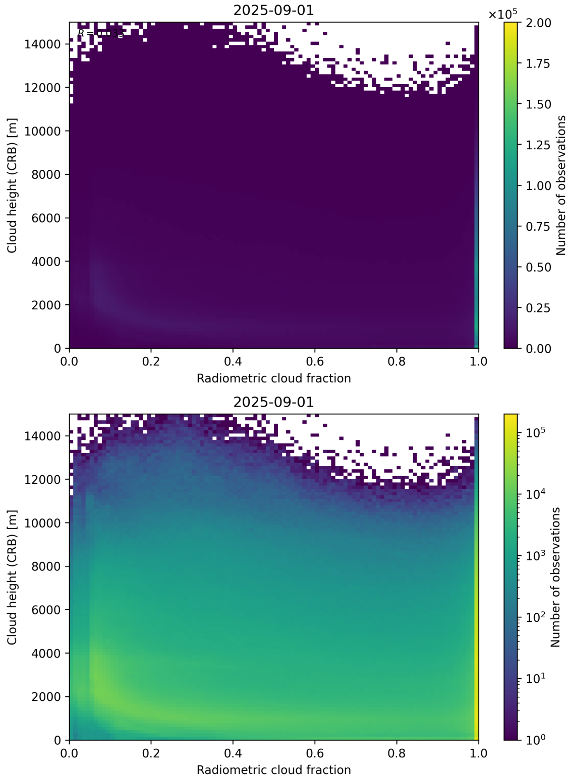
Figure 74: Scatter density plot of “Radiometric cloud fraction” against “Cloud height (CRB)” for 2025-08-31 to 2025-09-02.
