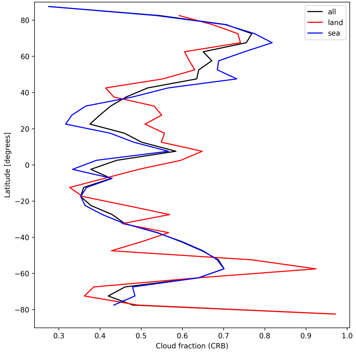
Figure 26: Zonal average of “Cloud fraction (CRB)” for 2025-08-31 to 2025-09-02.
