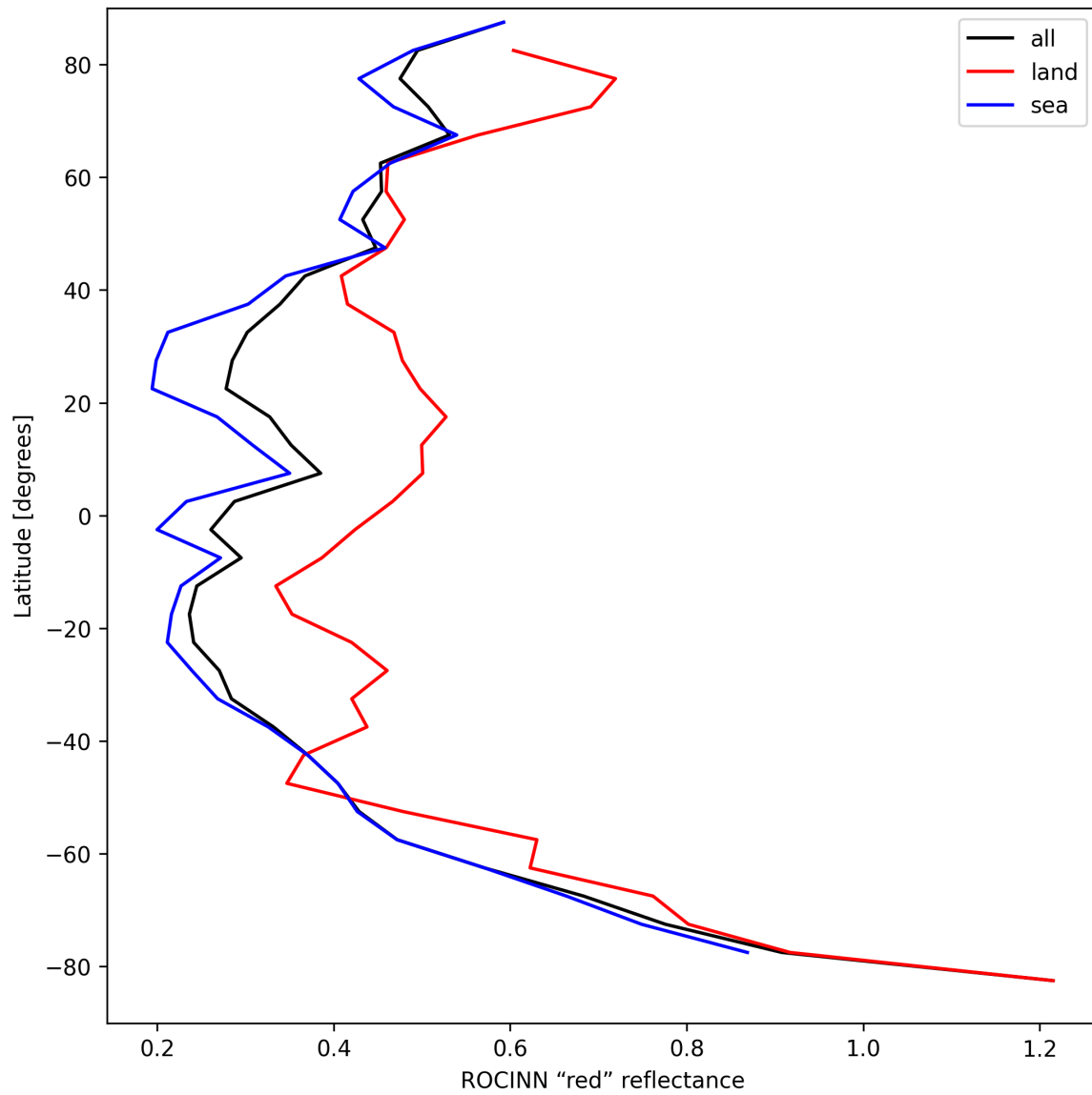
Figure 37: Zonal average of “ROCINN “red” reflectance” for 2025-08-31 to 2025-09-02.
