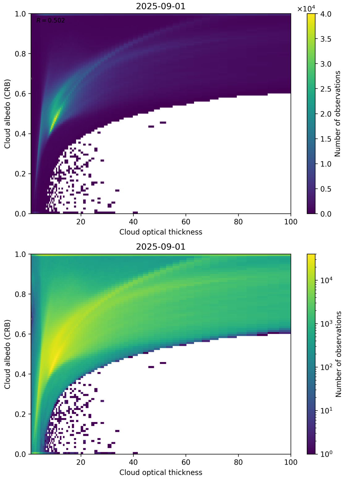
Figure 82: Scatter density plot of “Cloud optical thickness” against “Cloud albedo (CRB)” for 2025-08-31 to 2025-09-02.
