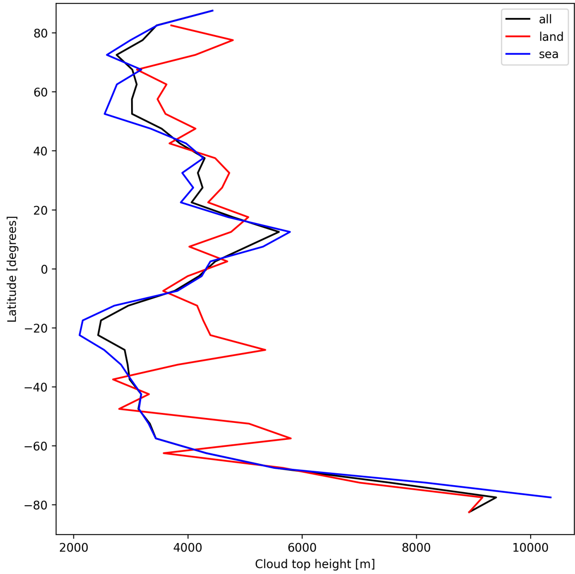
Figure 24: Zonal average of “Cloud top height” for 2025-08-31 to 2025-09-02.
