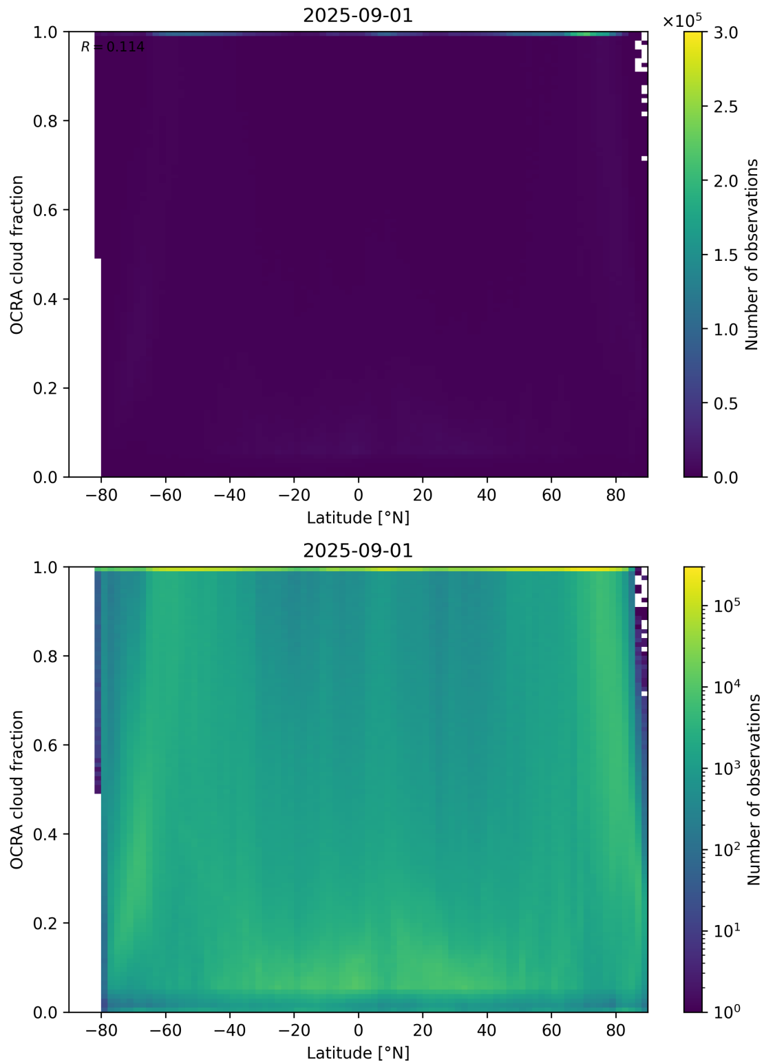
Figure 93: Scatter density plot of “Latitude” against “OCRA cloud fraction” for 2025-08-31 to 2025-09-02.
