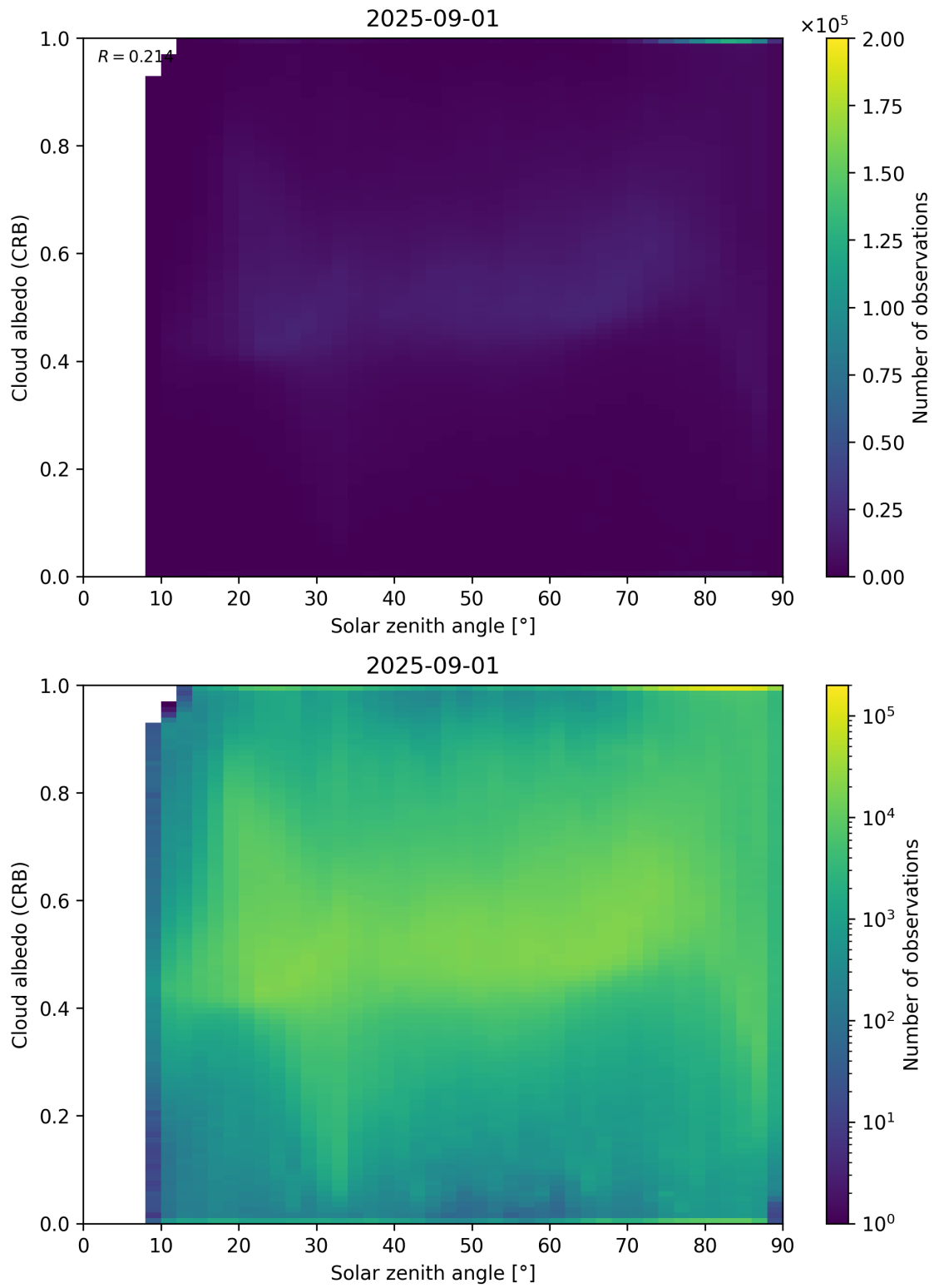
Figure 98: Scatter density plot of “Solar zenith angle” against “Cloud albedo (CRB)” for 2025-08-31 to 2025-09-02.
