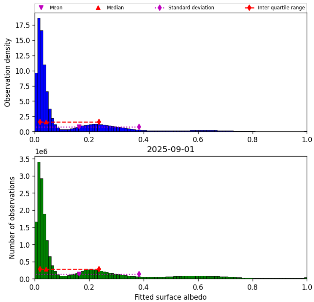
Figure 45: Histogram of “Fitted surface albedo” for 2025-08-31 to 2025-09-02
