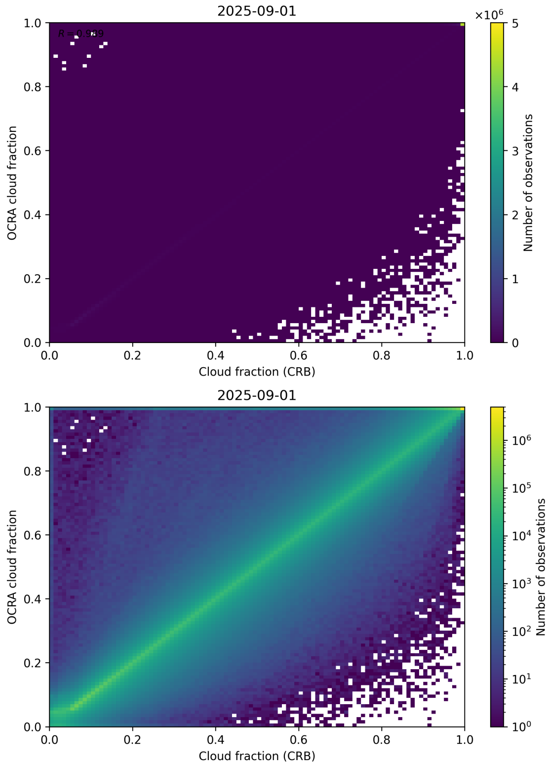
Figure 78: Scatter density plot of “Cloud fraction (CRB)” against “OCRA cloud fraction” for 2025-08-31 to 2025-09-02.
