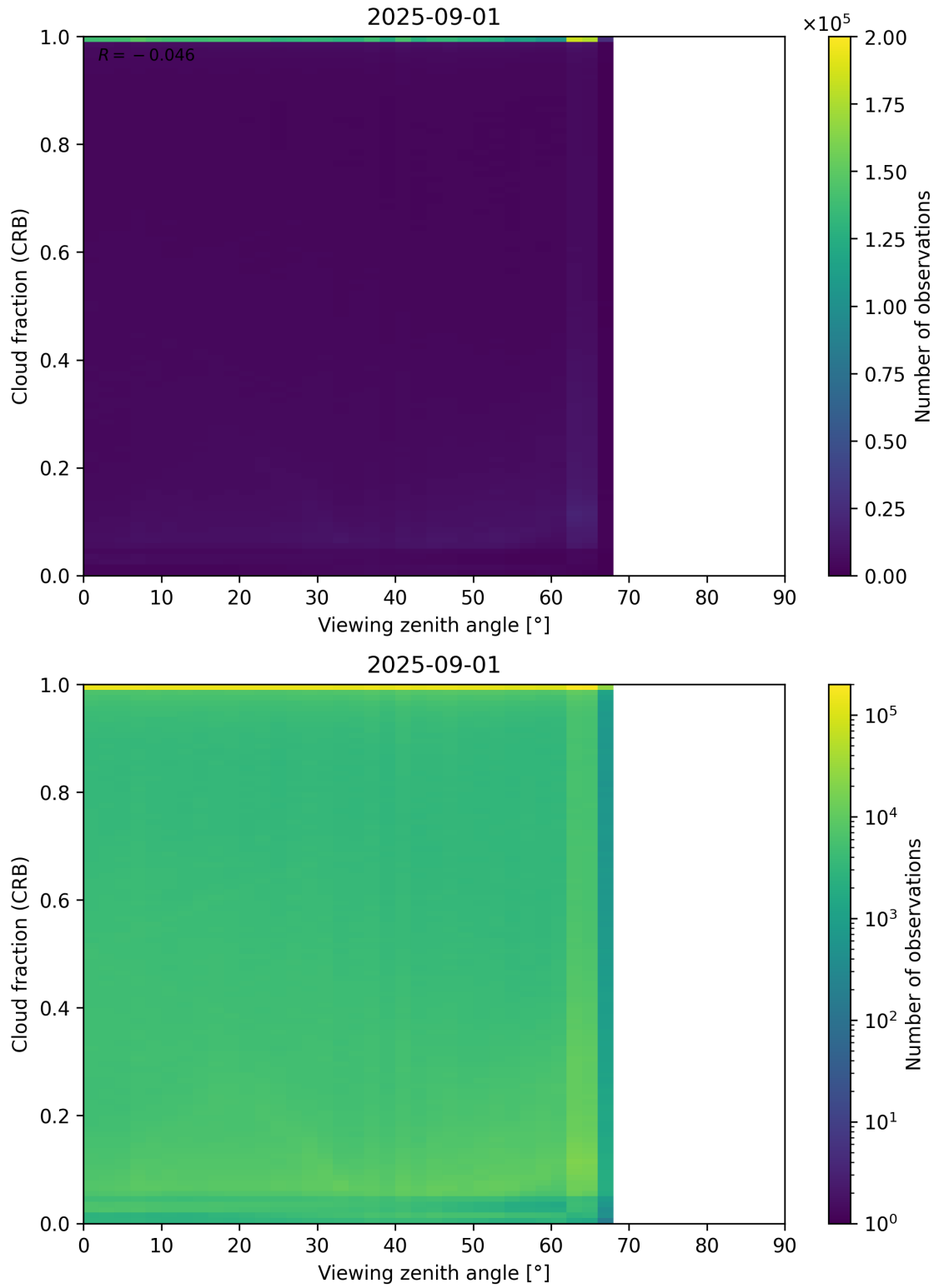
Figure 109: Scatter density plot of “Viewing zenith angle” against “Cloud fraction (CRB)” for 2025-08-31 to 2025-09-02.
