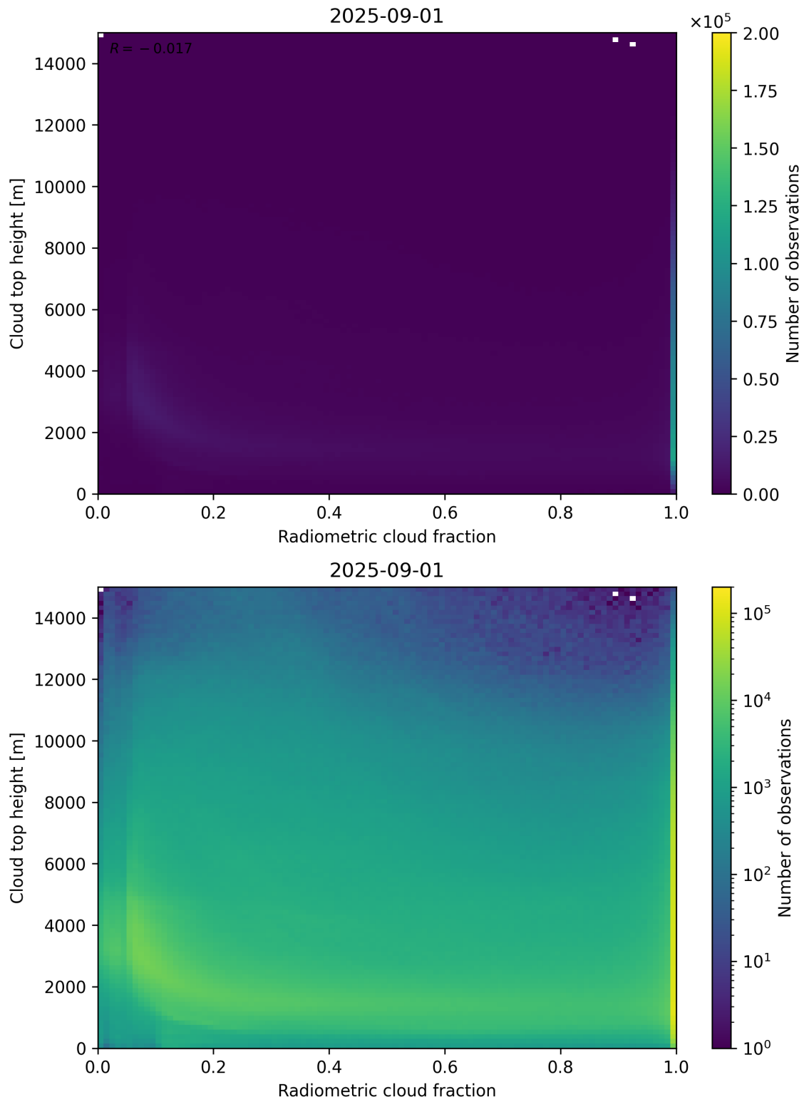
Figure 76: Scatter density plot of “Radiometric cloud fraction” against “Cloud top height” for 2025-08-31 to 2025-09-02.
