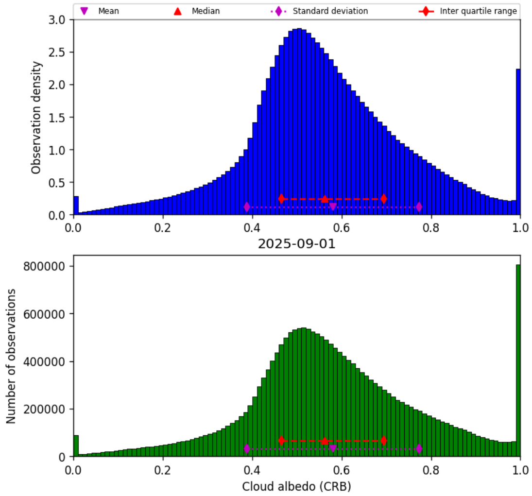
Figure 44: Histogram of “Cloud albedo (CRB)” for 2025-08-31 to 2025-09-02
