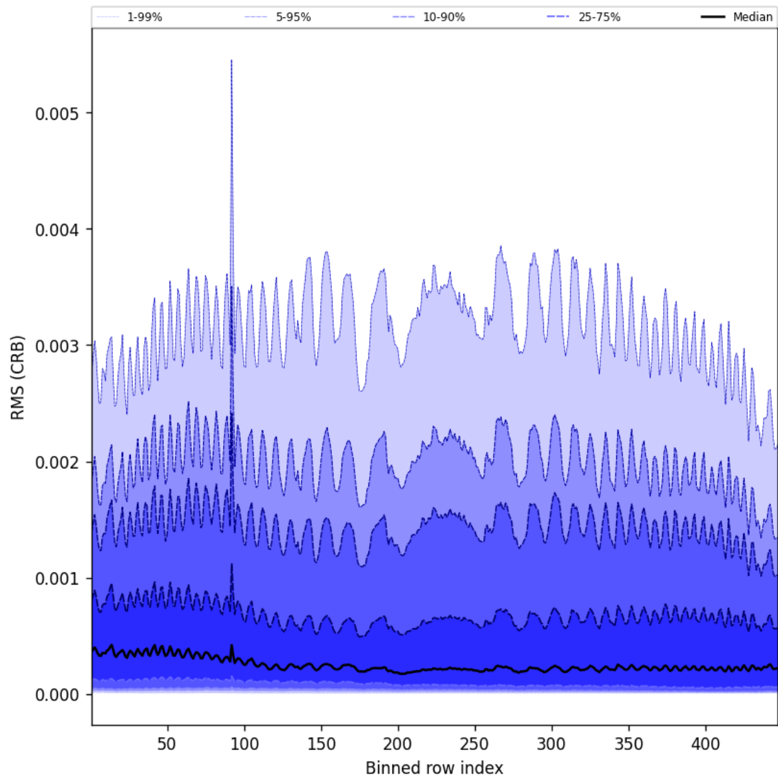
Figure 64: Along track statistics of “RMS (CRB)” for 2025-08-31 to 2025-09-02
