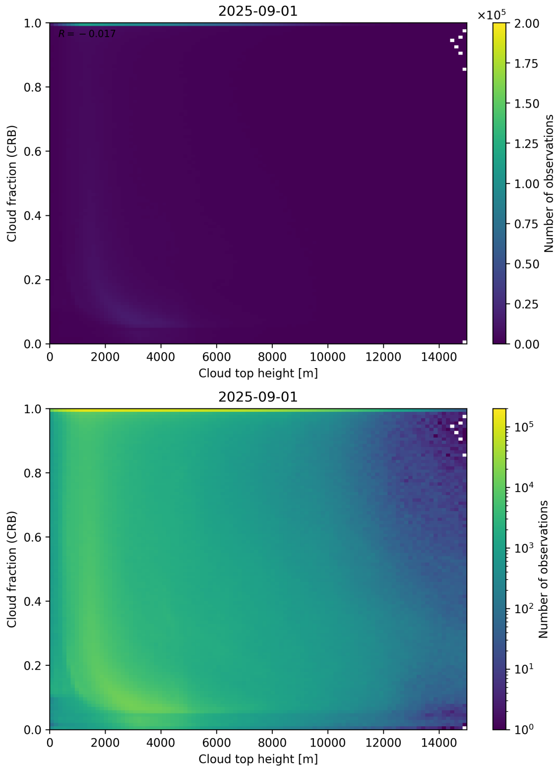
Figure 88: Scatter density plot of “Cloud top height” against “Cloud fraction (CRB)” for 2025-08-31 to 2025-09-02.
