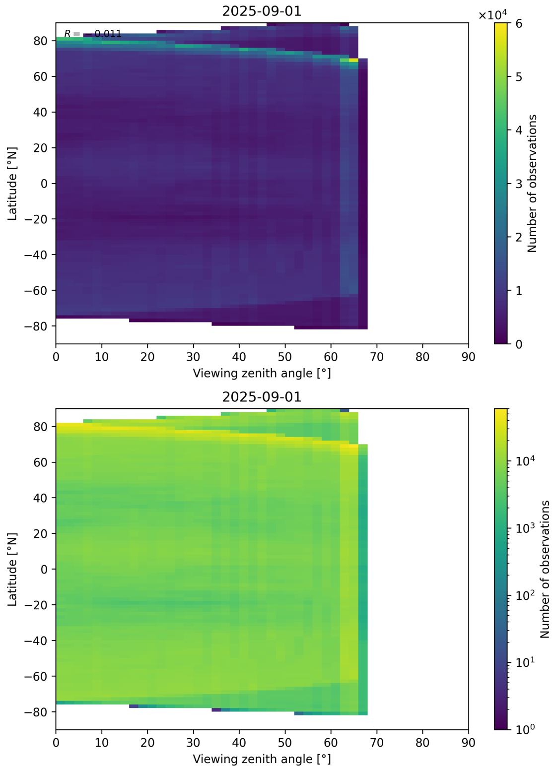
Figure 113: Scatter density plot of “Viewing zenith angle” against “Latitude” for 2025-08-31 to 2025-09-02.
