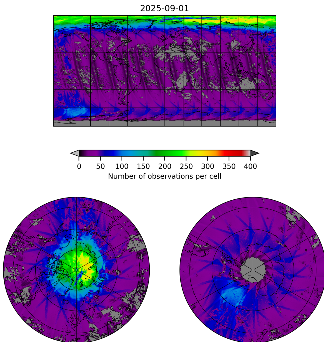
Figure 21: Map of the number of observations for 2025-08-31 to 2025-09-02
