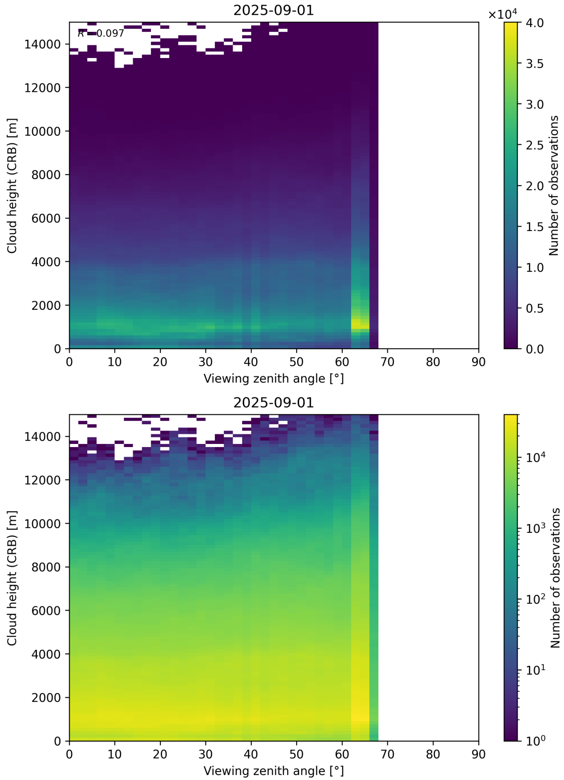
Figure 110: Scatter density plot of “Viewing zenith angle” against “Cloud height (CRB)” for 2025-08-31 to 2025-09-02.
