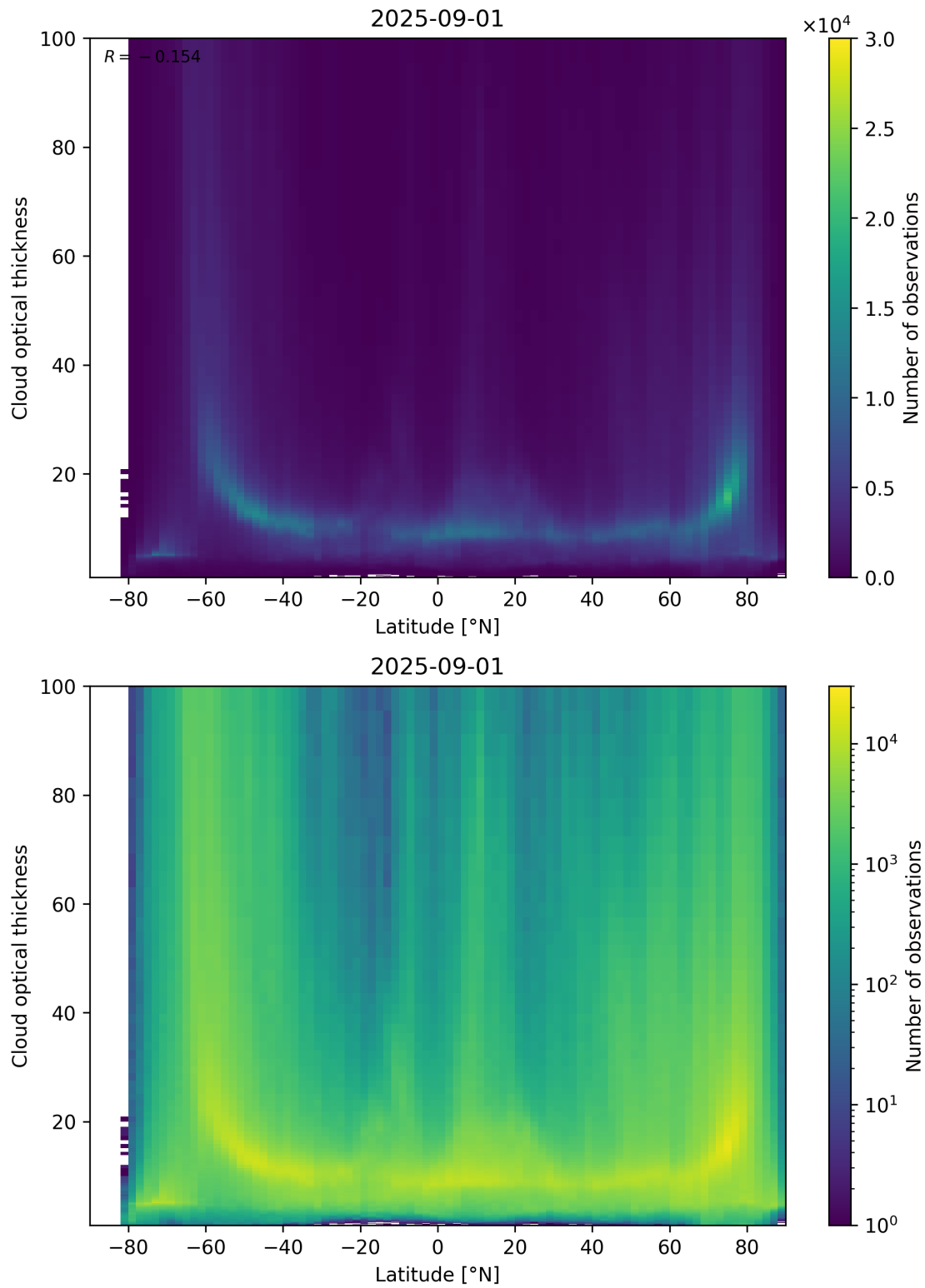
Figure 96: Scatter density plot of “Latitude” against “Cloud optical thickness” for 2025-08-31 to 2025-09-02.
