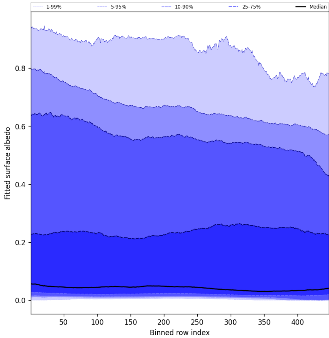
Figure 61: Along track statistics of “Fitted surface albedo” for 2025-08-31 to 2025-09-02
