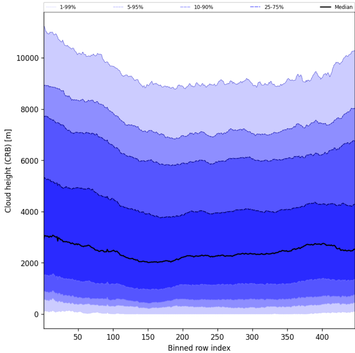
Figure 59: Along track statistics of “Cloud height (CRB)” for 2025-08-31 to 2025-09-02
