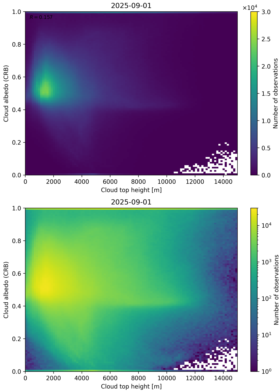
Figure 86: Scatter density plot of “Cloud top height” against “Cloud albedo (CRB)” for 2025-08-31 to 2025-09-02.
