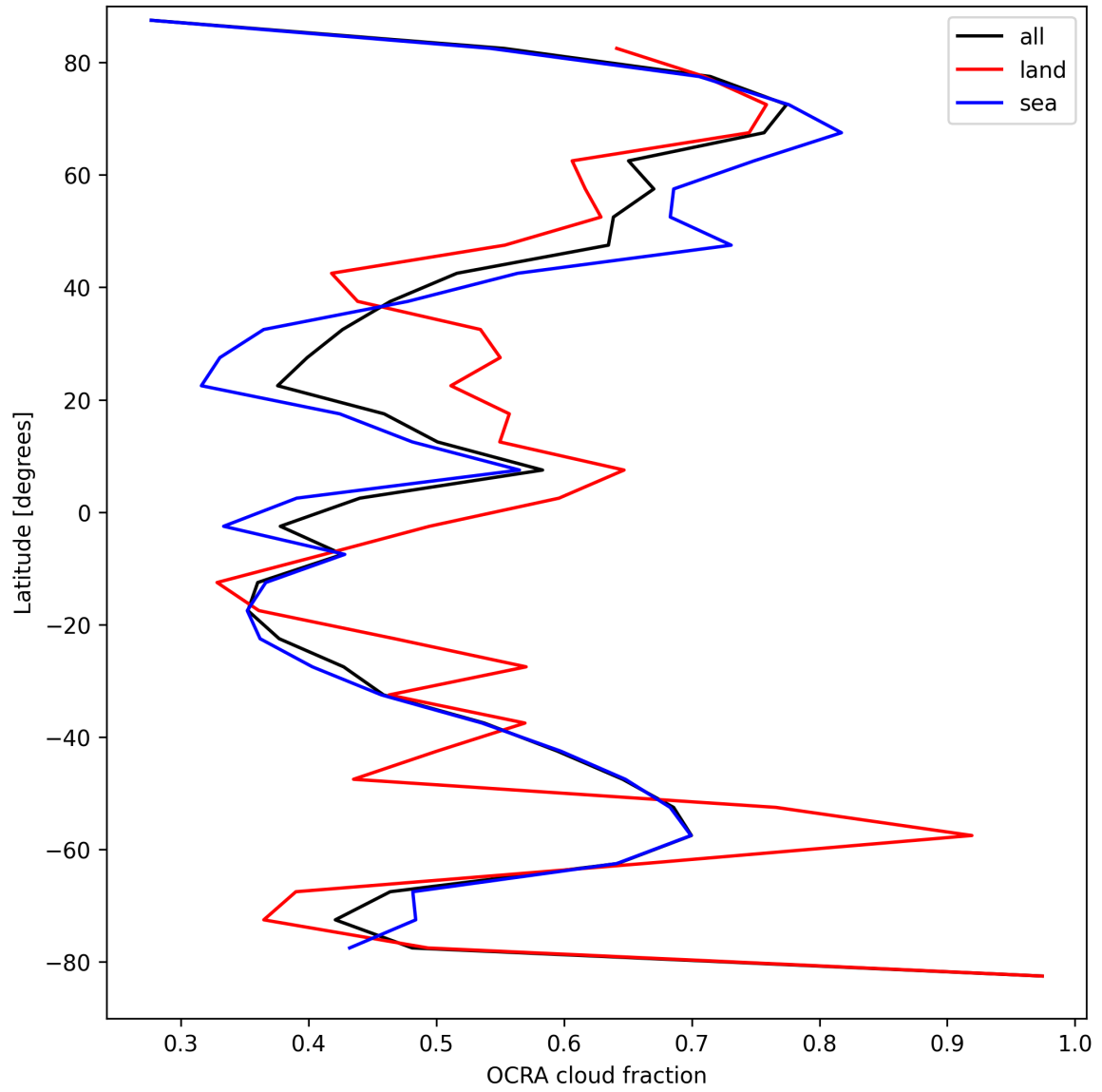
Figure 34: Zonal average of “OCRA cloud fraction” for 2025-08-31 to 2025-09-02.
