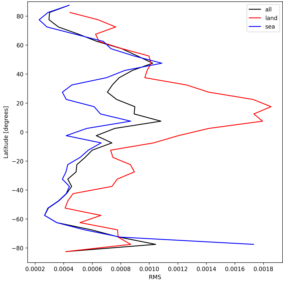
Figure 31: Zonal average of “RMS” for 2025-08-31 to 2025-09-02.
