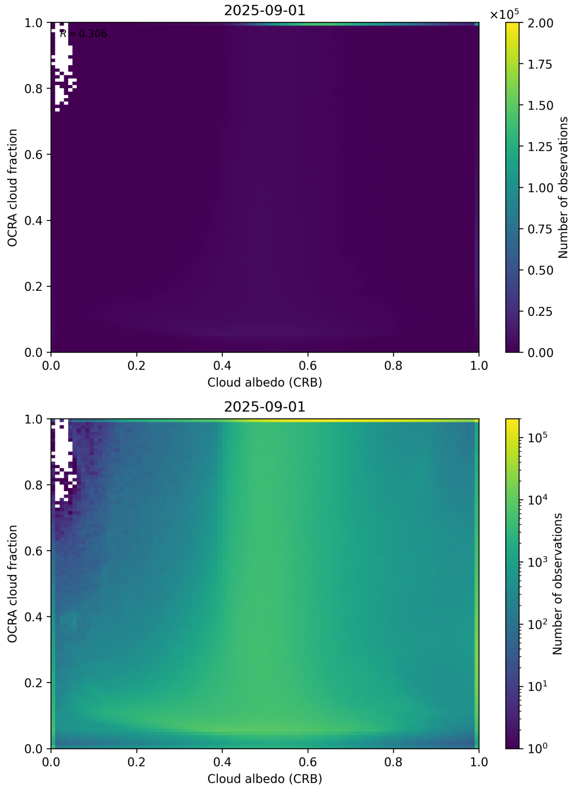
Figure 70: Scatter density plot of “Cloud albedo (CRB)” against “OCRA cloud fraction” for 2025-08-31 to 2025-09-02.
