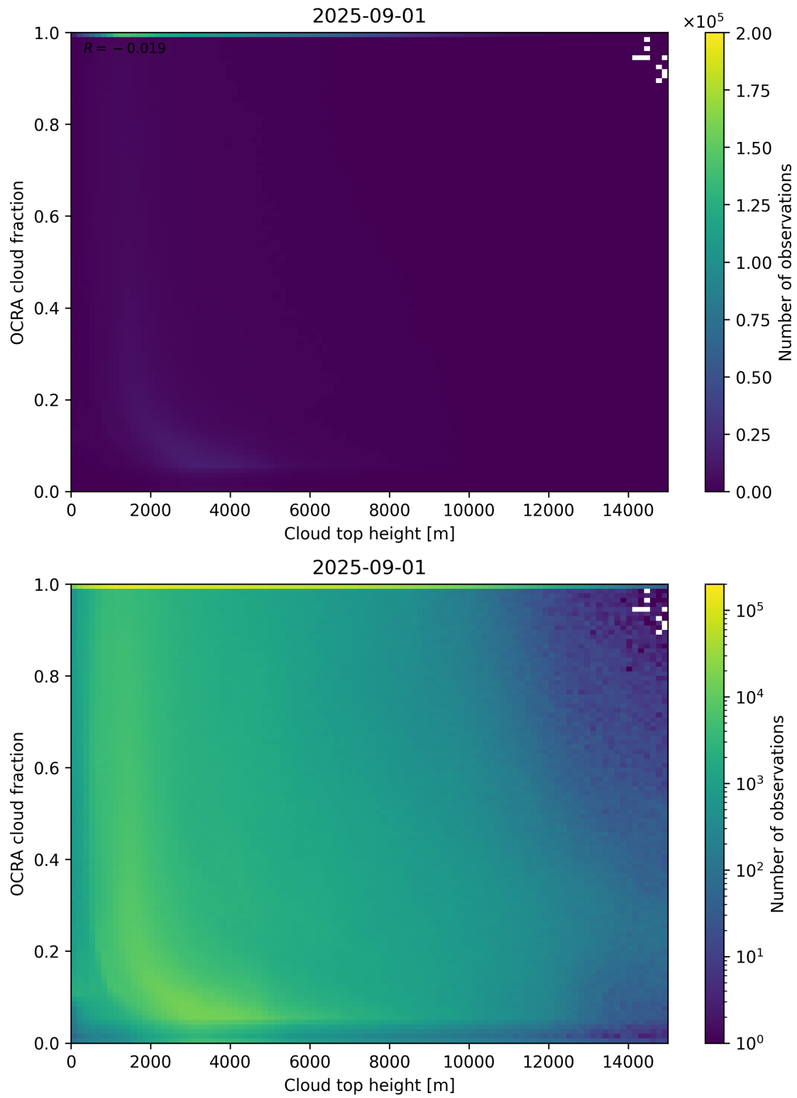
Figure 87: Scatter density plot of “Cloud top height” against “OCRA cloud fraction” for 2025-08-31 to 2025-09-02.
