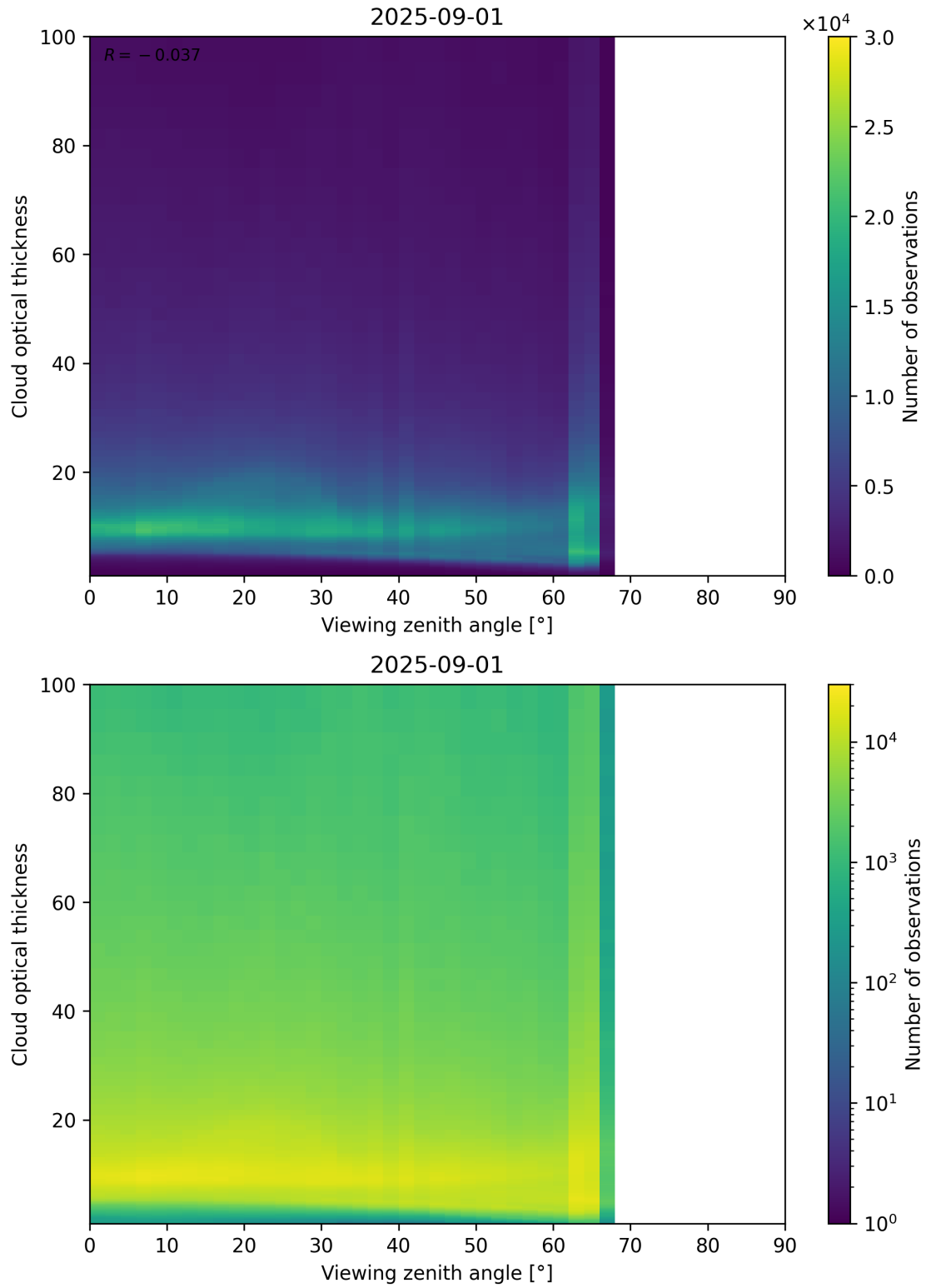
Figure 111: Scatter density plot of “Viewing zenith angle” against “Cloud optical thickness” for 2025-08-31 to 2025-09-02.
