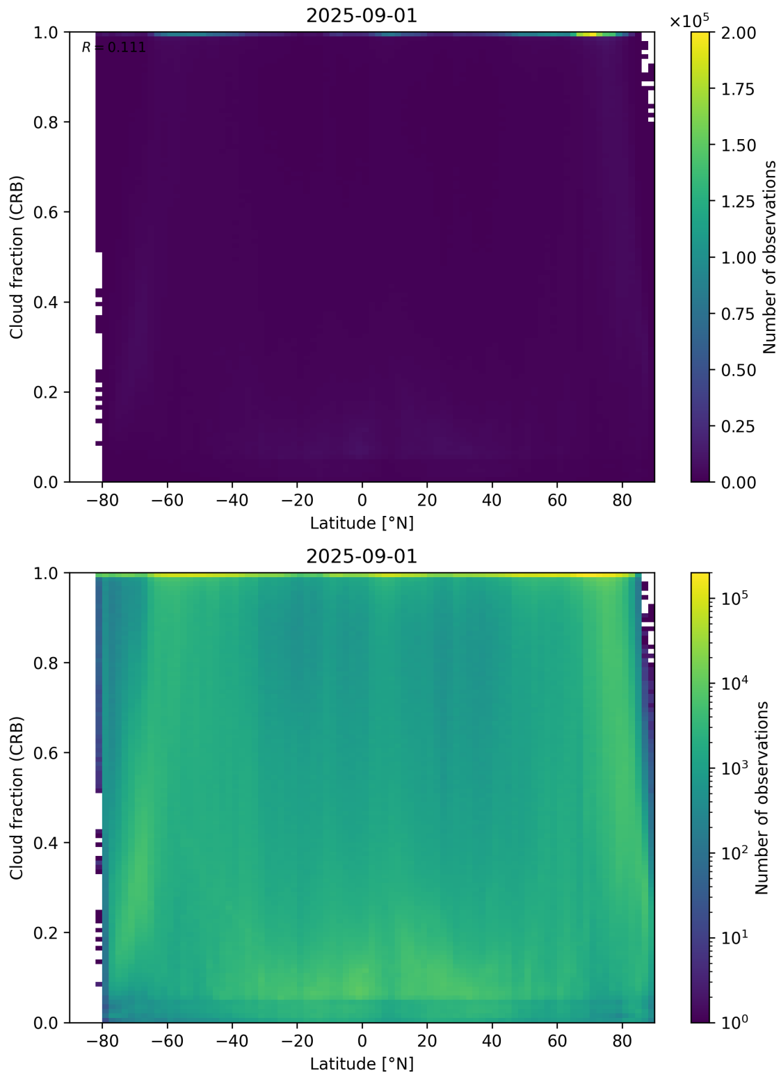
Figure 94: Scatter density plot of “Latitude” against “Cloud fraction (CRB)” for 2025-08-31 to 2025-09-02.
