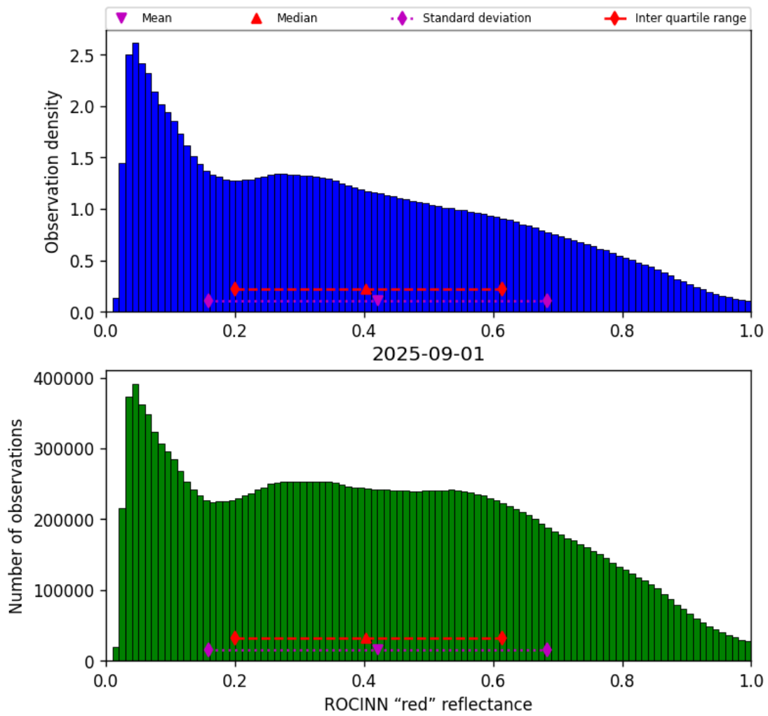
Figure 53: Histogram of “ROCINN “red” reflectance” for 2025-08-31 to 2025-09-02
