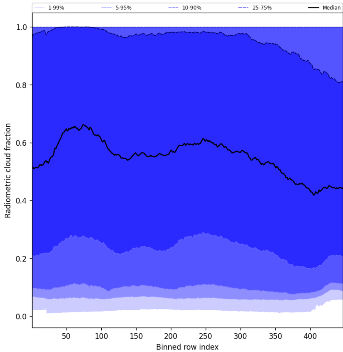
Figure 55: Along track statistics of “Radiometric cloud fraction” for 2025-08-31 to 2025-09-02
