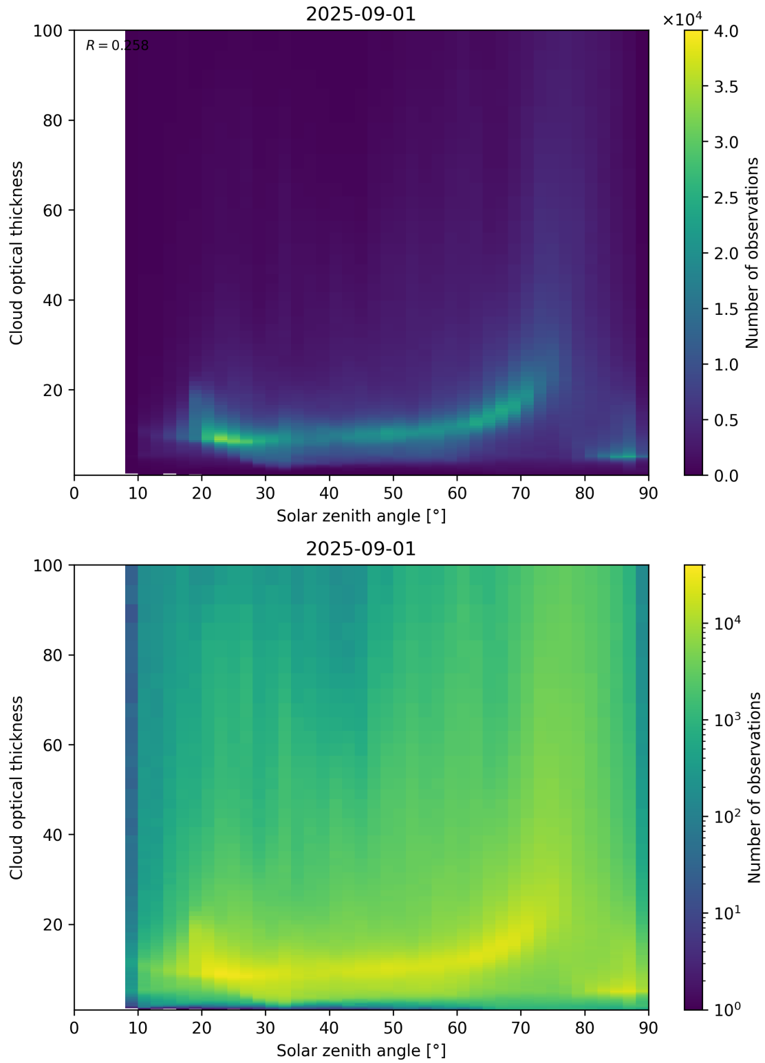
Figure 103: Scatter density plot of “Solar zenith angle” against “Cloud optical thickness” for 2025-08-31 to 2025-09-02.
