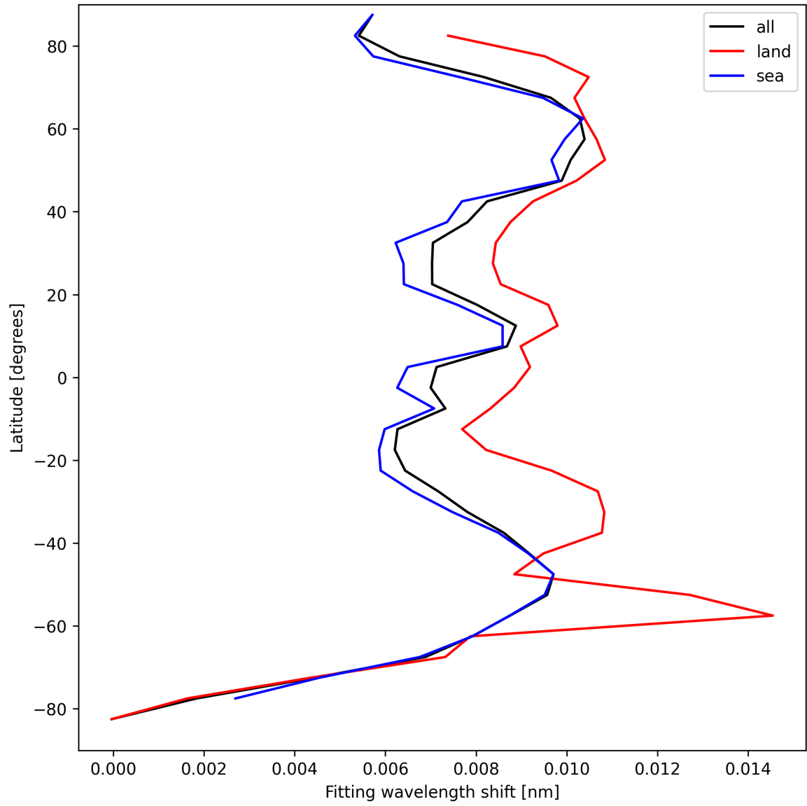
Figure 33: Zonal average of “Fitting wavelength shift” for 2025-08-31 to 2025-09-02.
