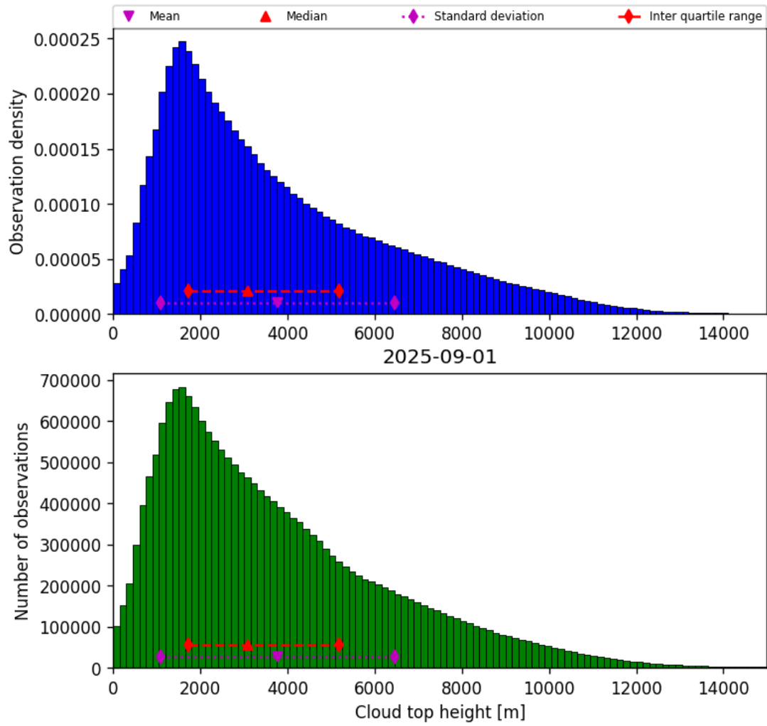
Figure 40: Histogram of “Cloud top height” for 2025-08-31 to 2025-09-02
