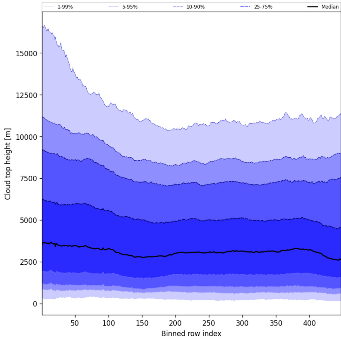
Figure 56: Along track statistics of “Cloud top height” for 2025-08-31 to 2025-09-02
