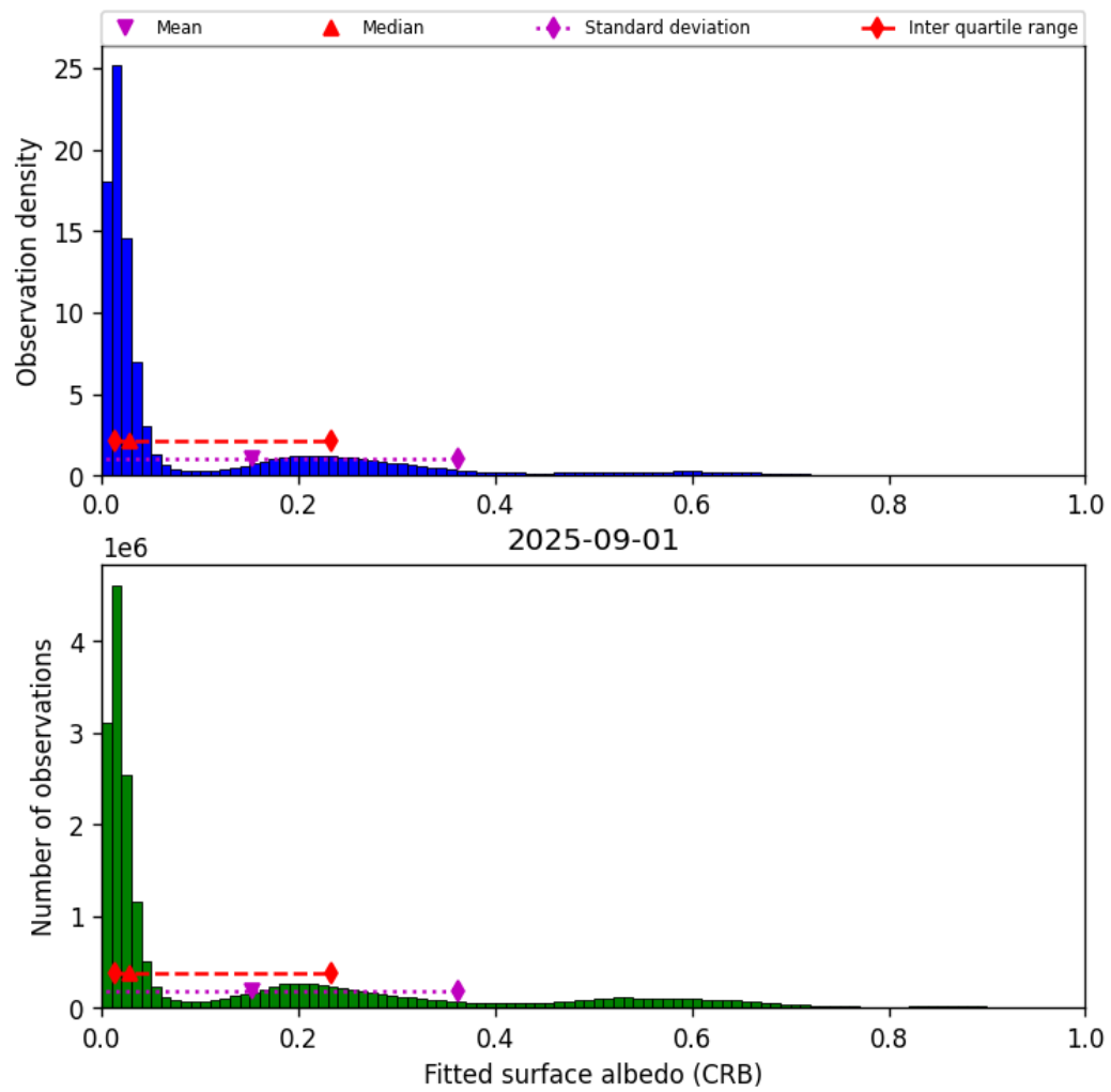
Figure 46: Histogram of “Fitted surface albedo (CRB)” for 2025-08-31 to 2025-09-02
