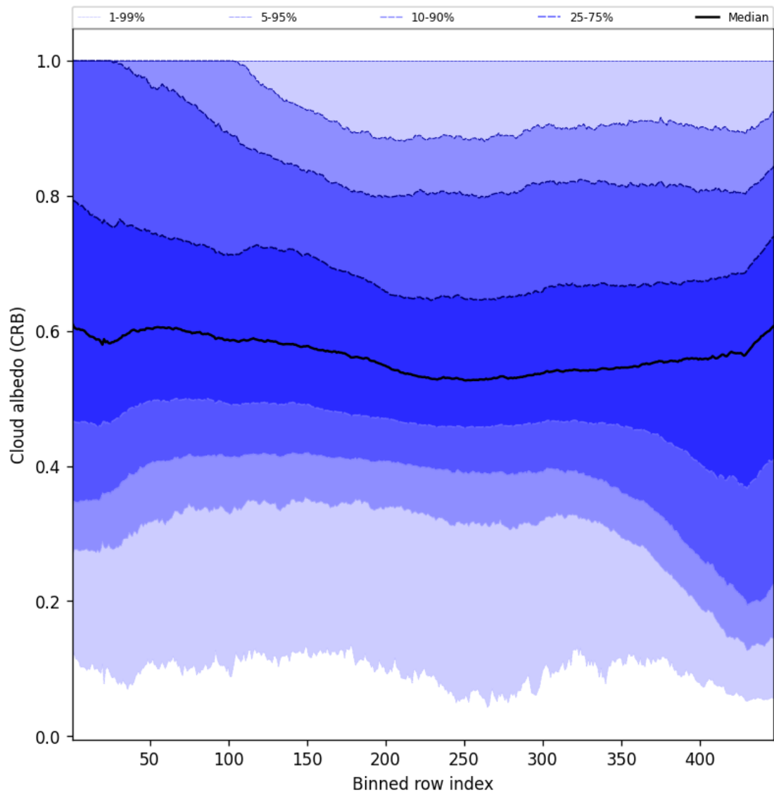
Figure 60: Along track statistics of “Cloud albedo (CRB)” for 2025-08-31 to 2025-09-02
