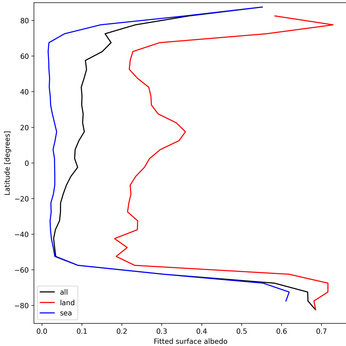
Figure 29: Zonal average of “Fitted surface albedo” for 2025-09-02 to 2025-09-04.
