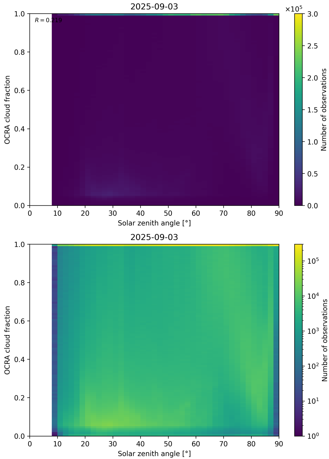
Figure 100: Scatter density plot of “Solar zenith angle” against “OCRA cloud fraction” for 2025-09-02 to 2025-09-04.
