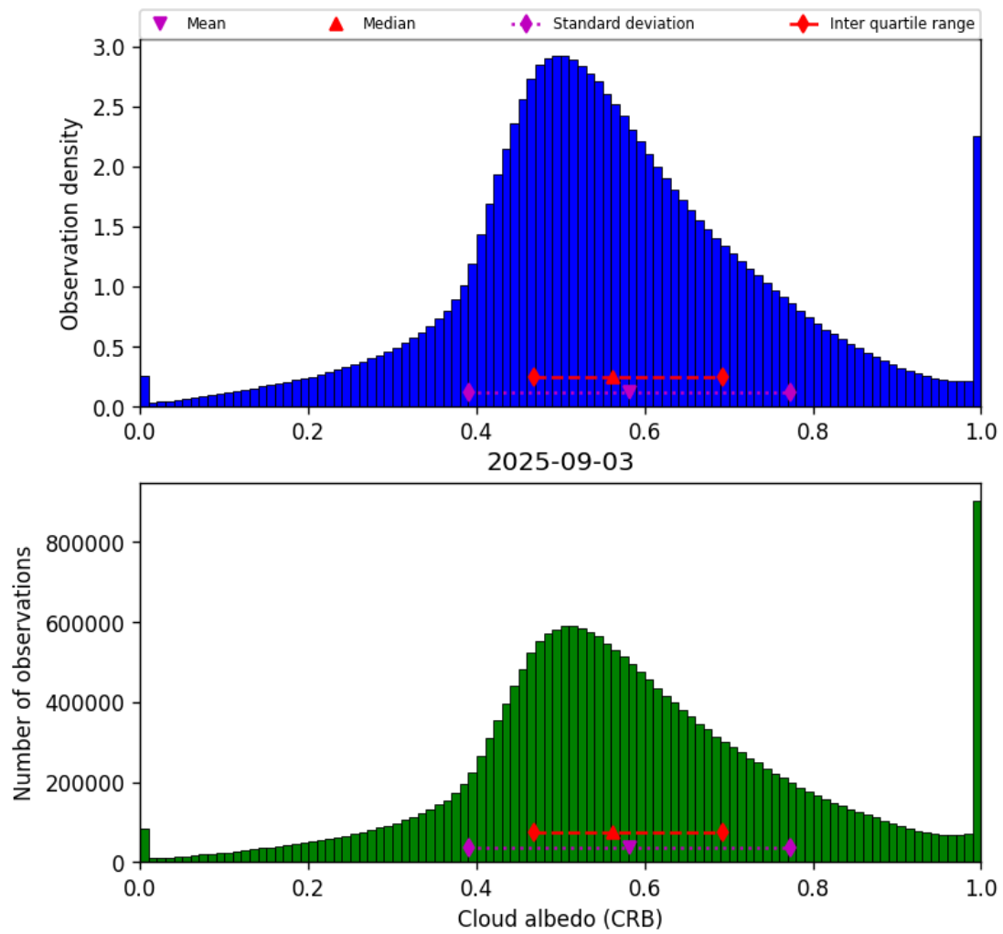
Figure 44: Histogram of “Cloud albedo (CRB)” for 2025-09-02 to 2025-09-04
