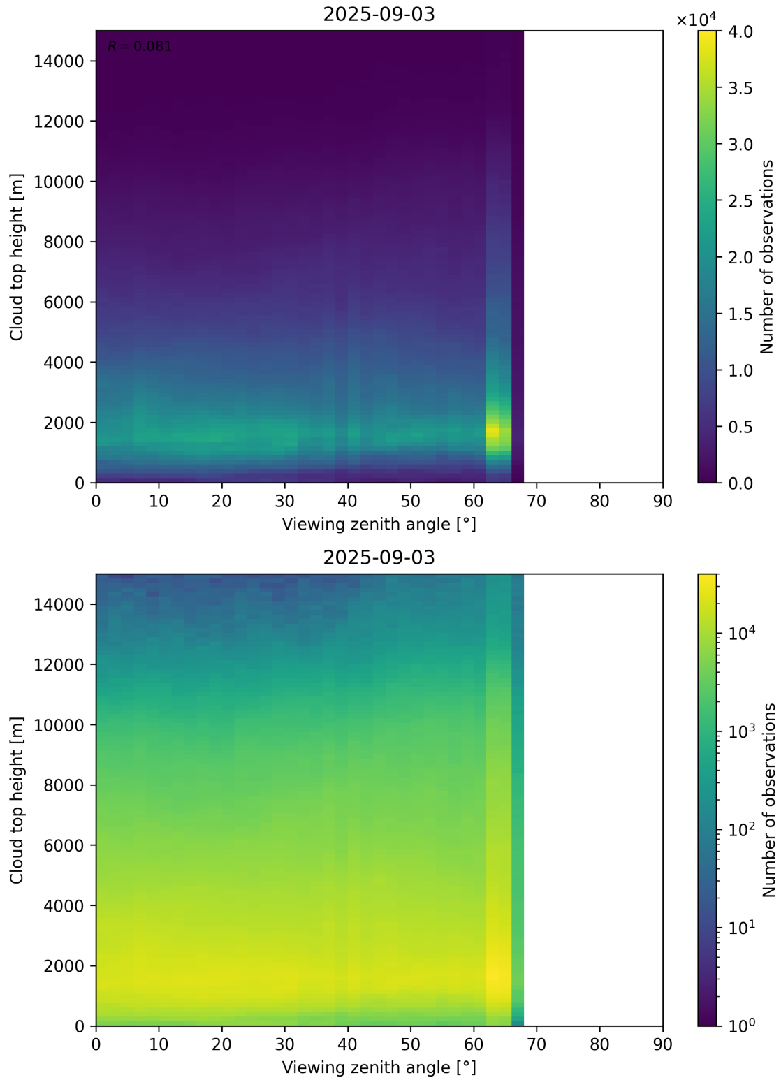
Figure 112: Scatter density plot of “Viewing zenith angle” against “Cloud top height” for 2025-09-02 to 2025-09-04.
