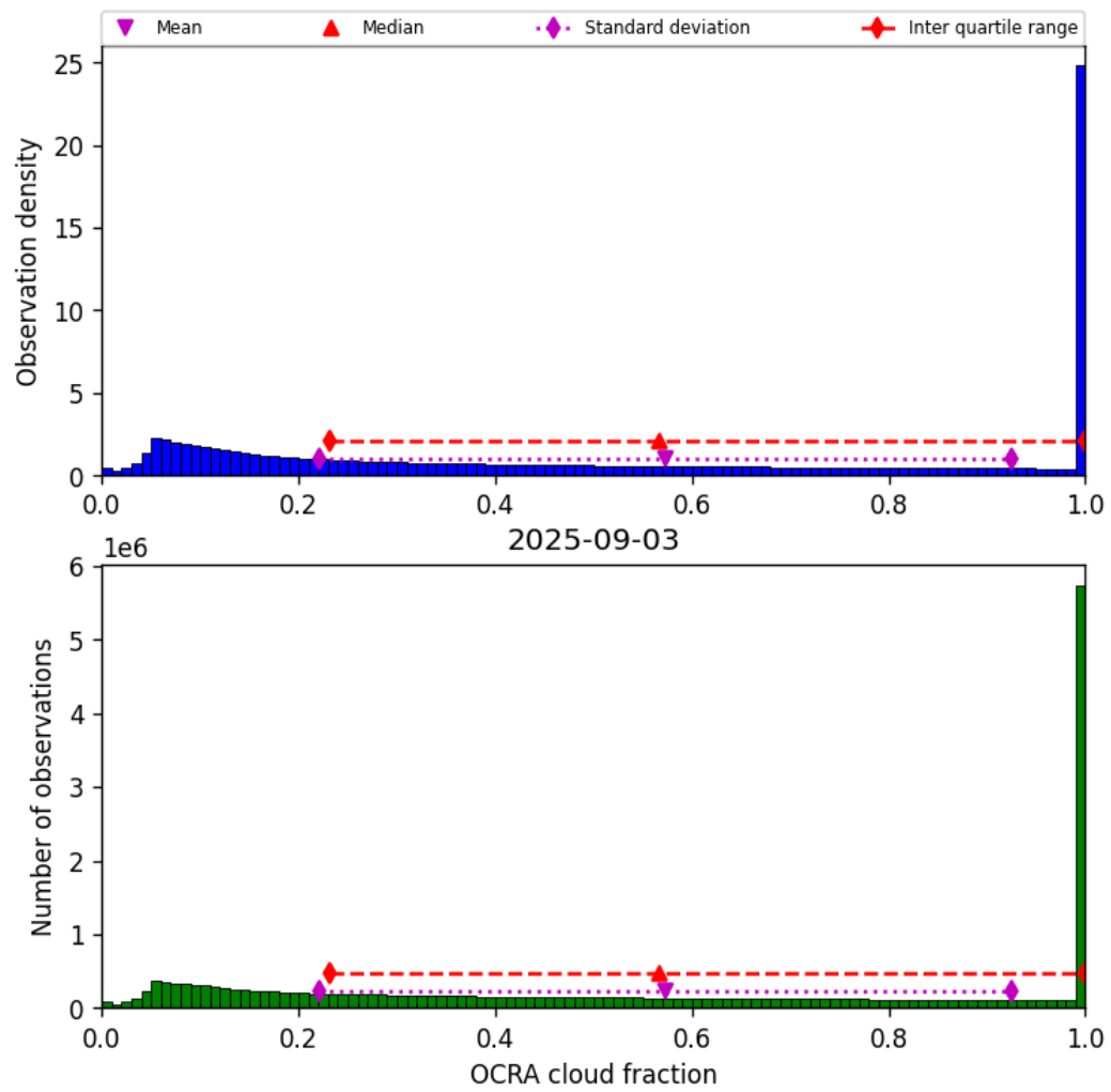
Figure 50: Histogram of “OCRA cloud fraction” for 2025-09-02 to 2025-09-04
