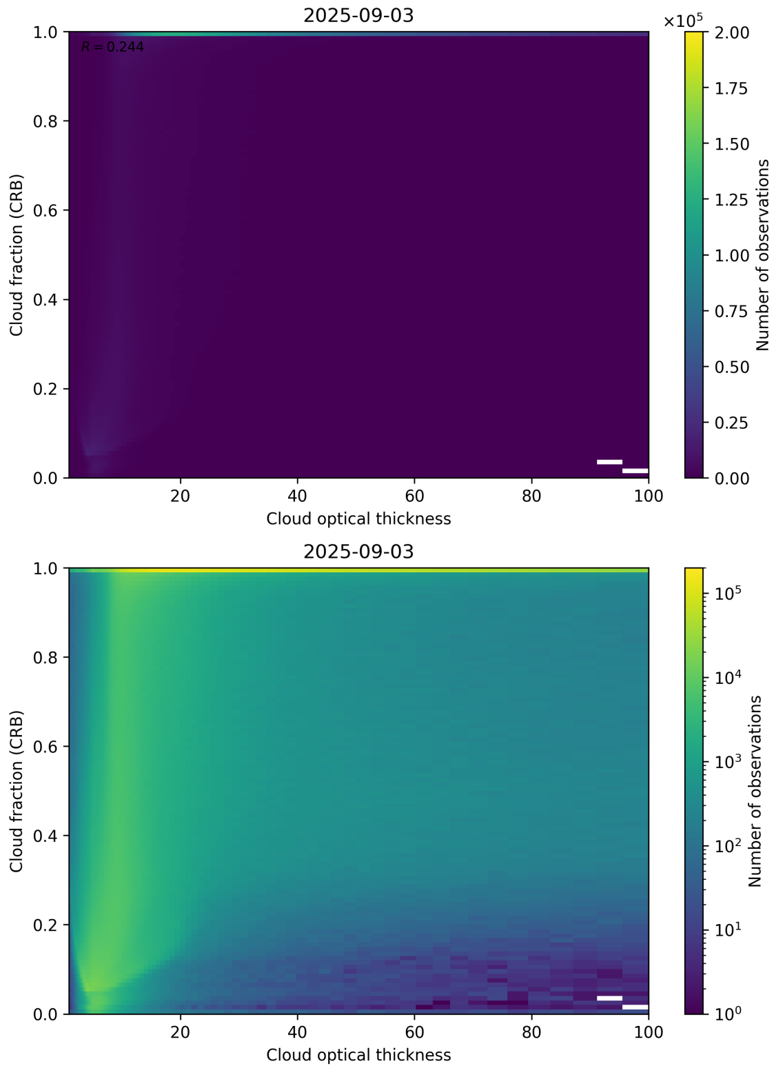
Figure 84: Scatter density plot of “Cloud optical thickness” against “Cloud fraction (CRB)” for 2025-09-02 to 2025-09-04.
