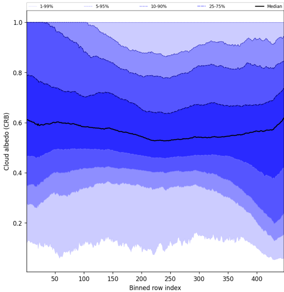
Figure 60: Along track statistics of “Cloud albedo (CRB)” for 2025-09-02 to 2025-09-04
