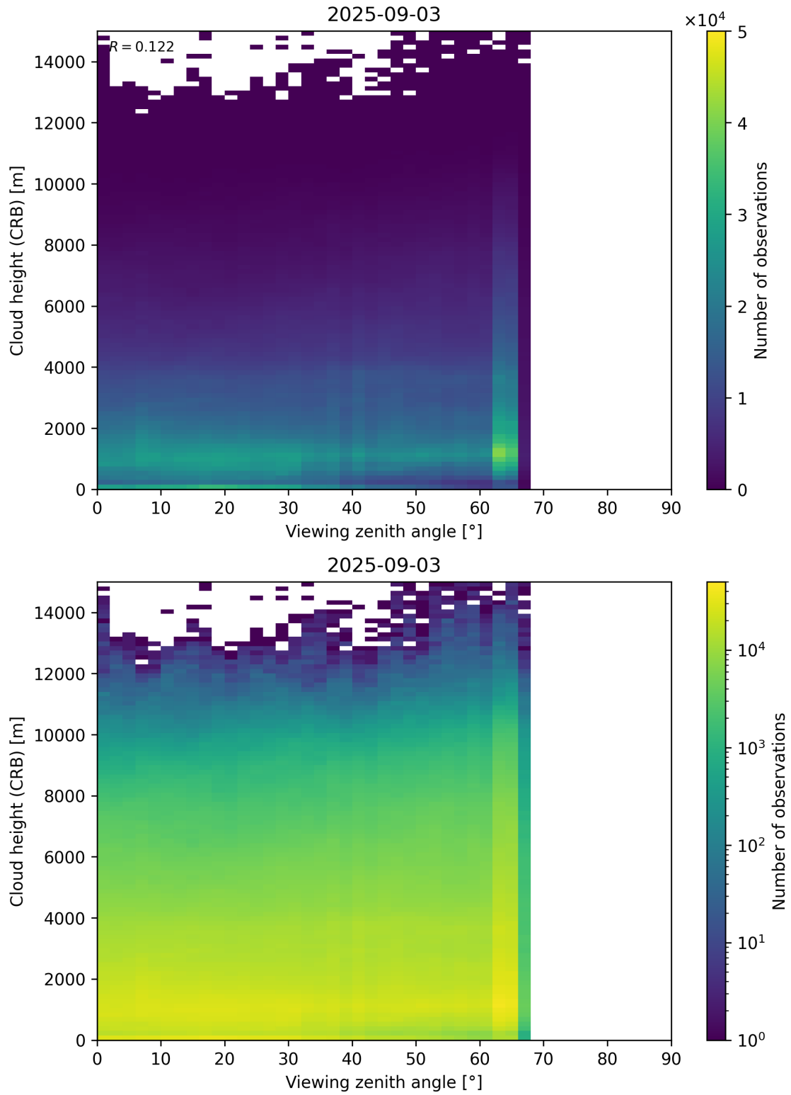
Figure 110: Scatter density plot of “Viewing zenith angle” against “Cloud height (CRB)” for 2025-09-02 to 2025-09-04.
