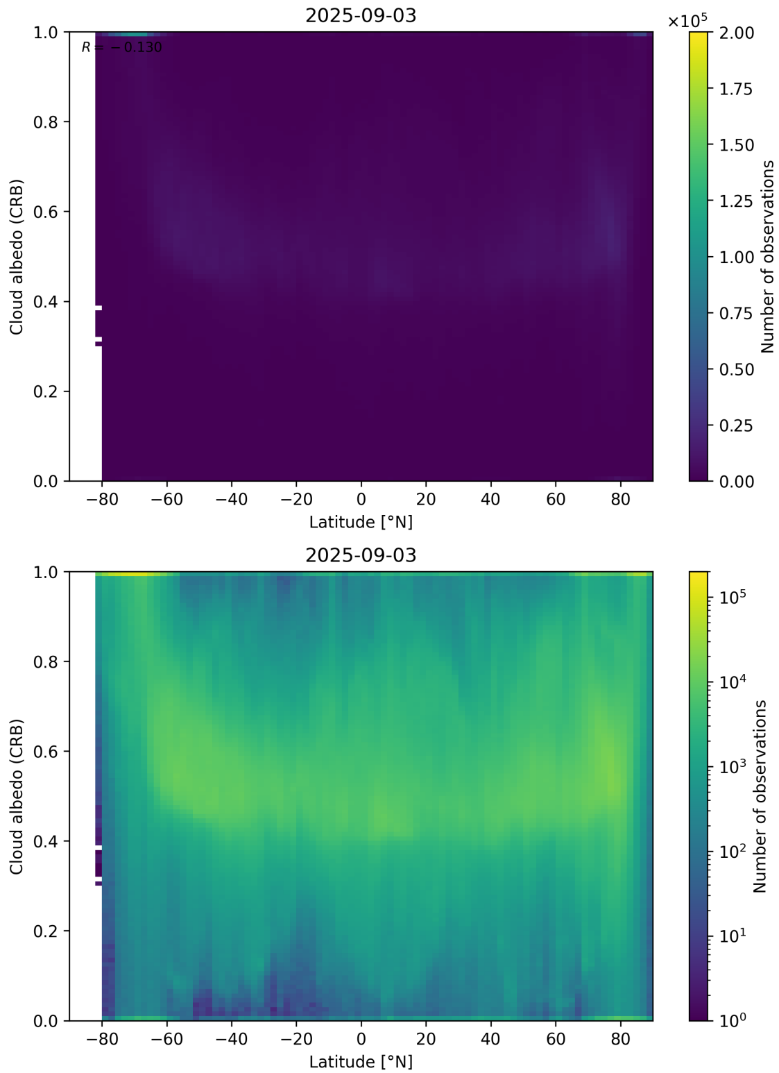
Figure 91: Scatter density plot of “Latitude” against “Cloud albedo (CRB)” for 2025-09-02 to 2025-09-04.
