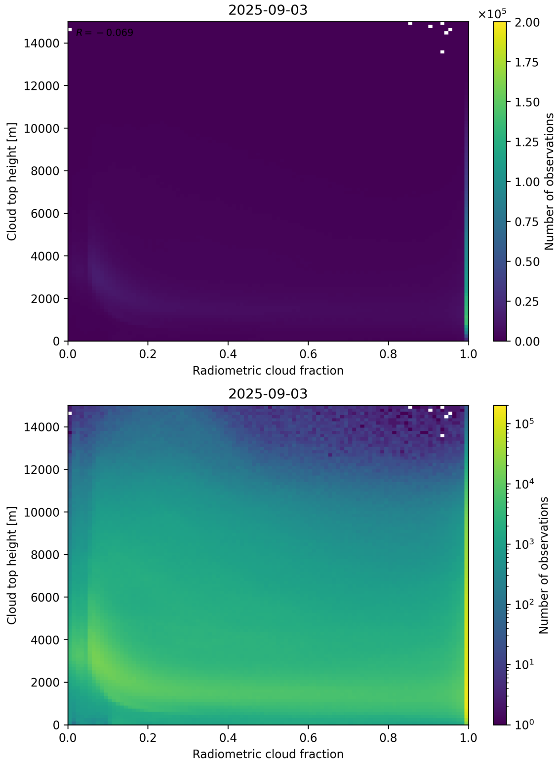
Figure 76: Scatter density plot of “Radiometric cloud fraction” against “Cloud top height” for 2025-09-02 to 2025-09-04.
