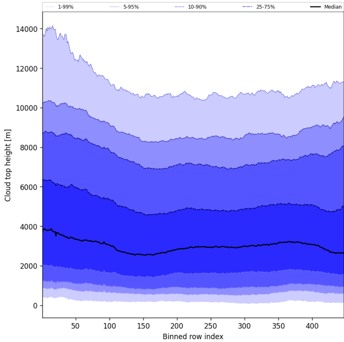
Figure 56: Along track statistics of “Cloud top height” for 2025-09-02 to 2025-09-04
