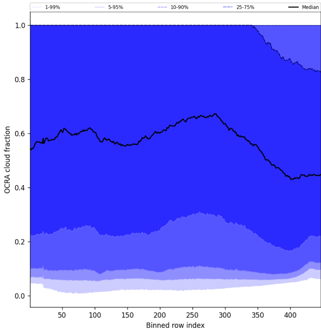
Figure 66: Along track statistics of “OCRA cloud fraction” for 2025-09-02 to 2025-09-04
