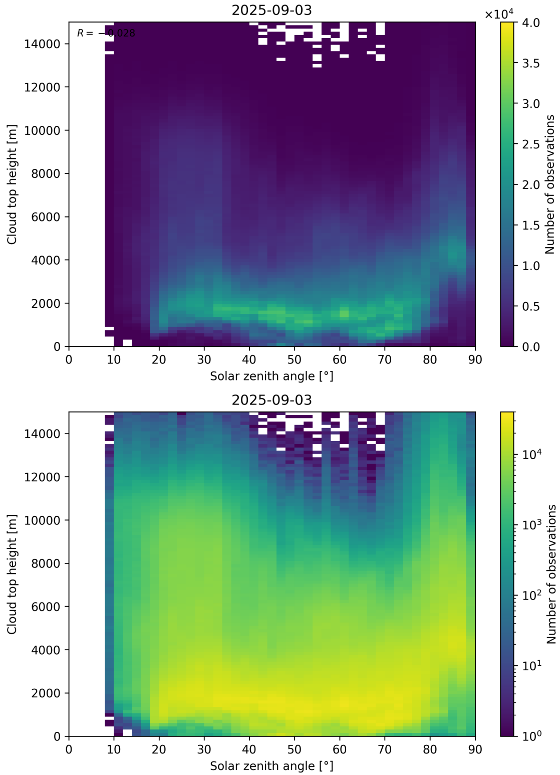
Figure 104: Scatter density plot of “Solar zenith angle” against “Cloud top height” for 2025-09-02 to 2025-09-04.
