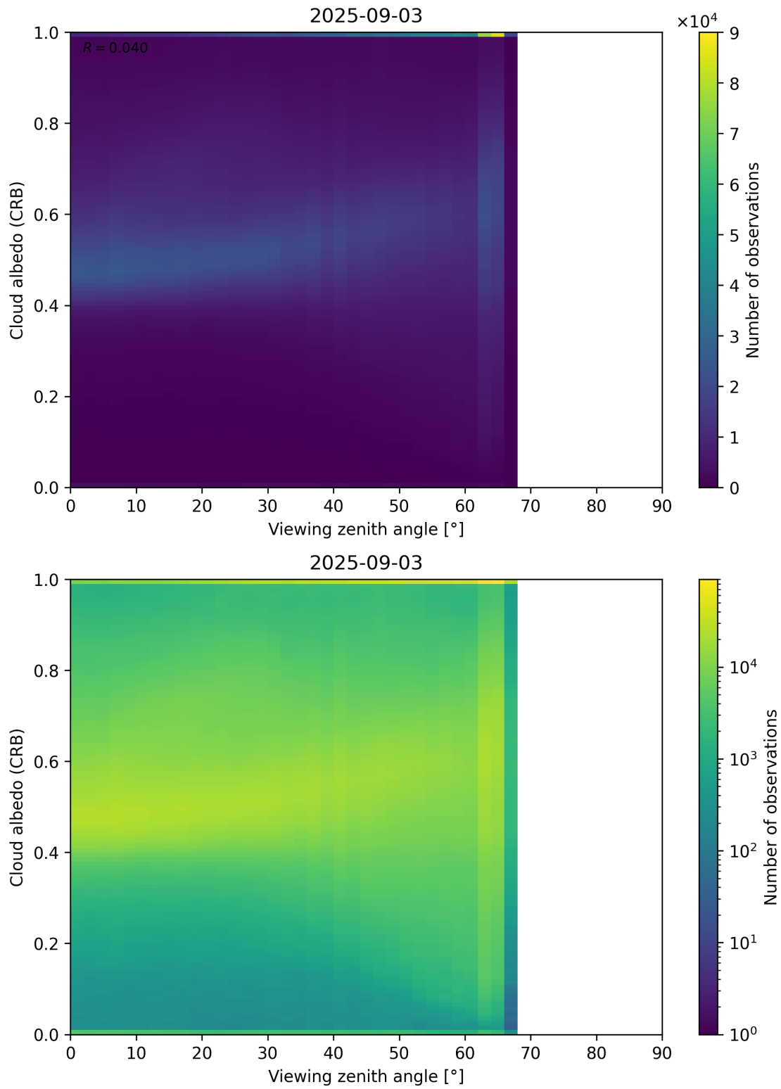
Figure 106: Scatter density plot of “Viewing zenith angle” against “Cloud albedo (CRB)” for 2025-09-02 to 2025-09-04.
