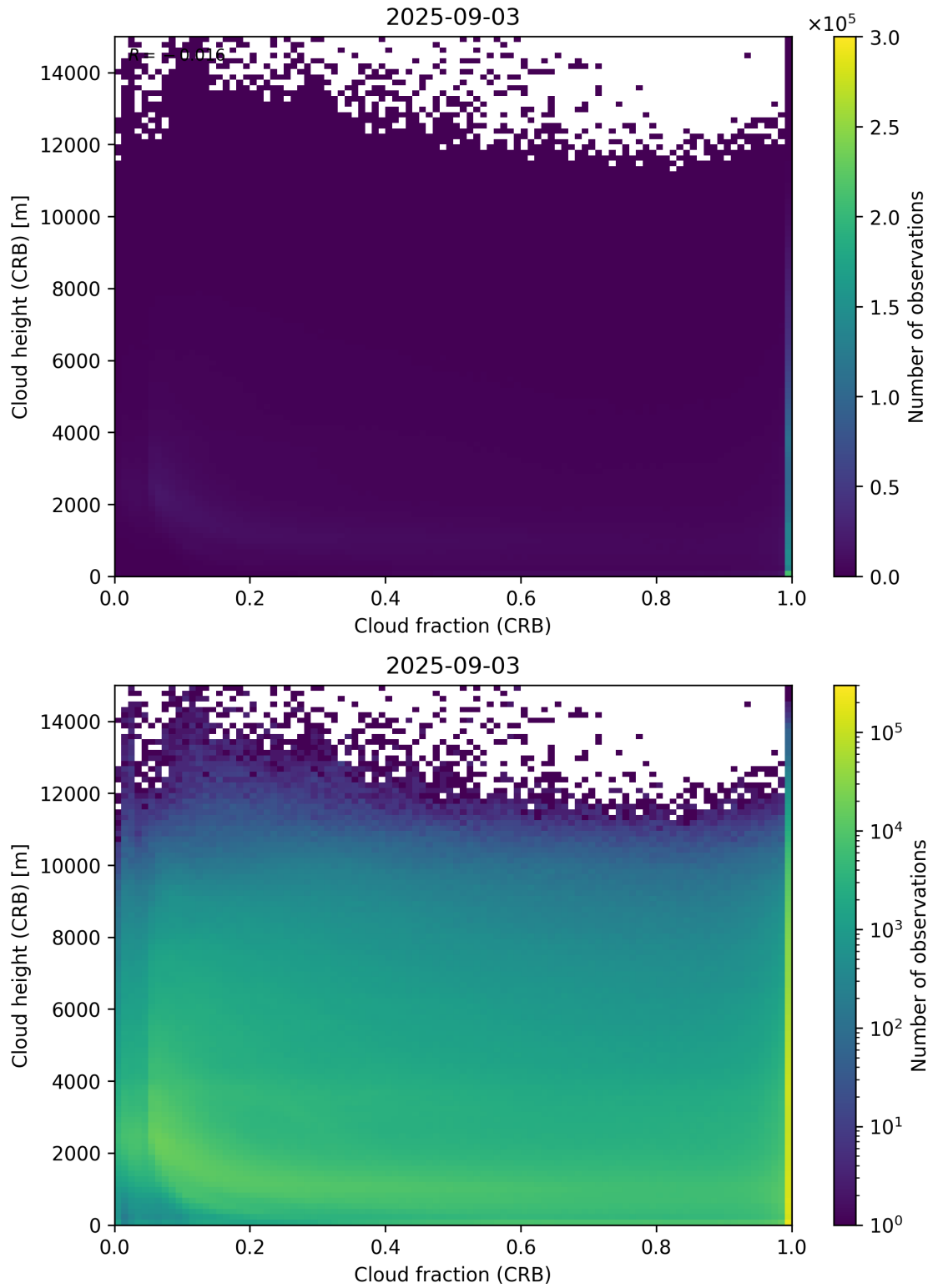
Figure 79: Scatter density plot of “Cloud fraction (CRB)” against “Cloud height (CRB)” for 2025-09-02 to 2025-09-04.
