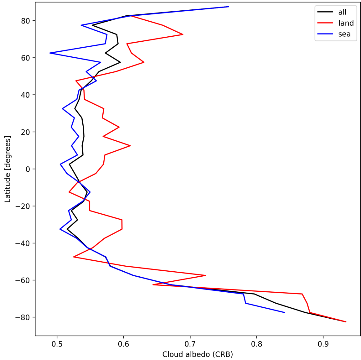
Figure 28: Zonal average of “Cloud albedo (CRB)” for 2025-09-02 to 2025-09-04.
