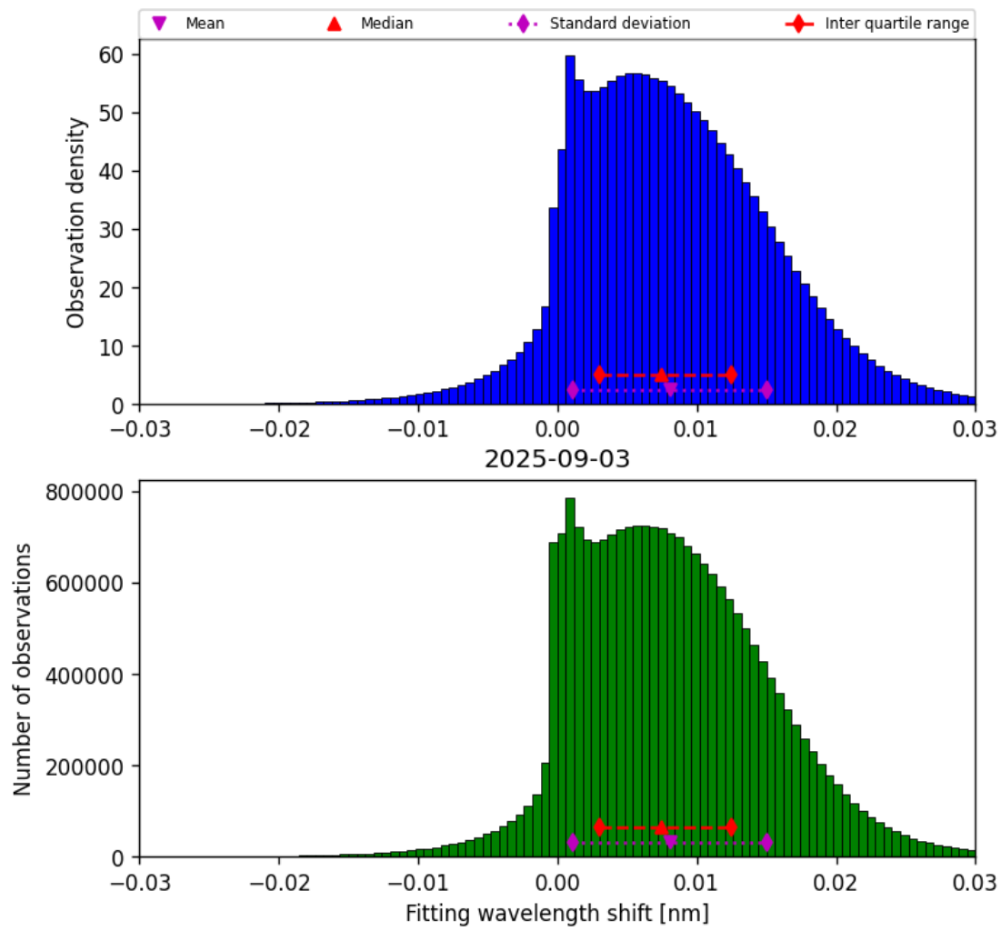
Figure 49: Histogram of “Fitting wavelength shift” for 2025-09-02 to 2025-09-04
