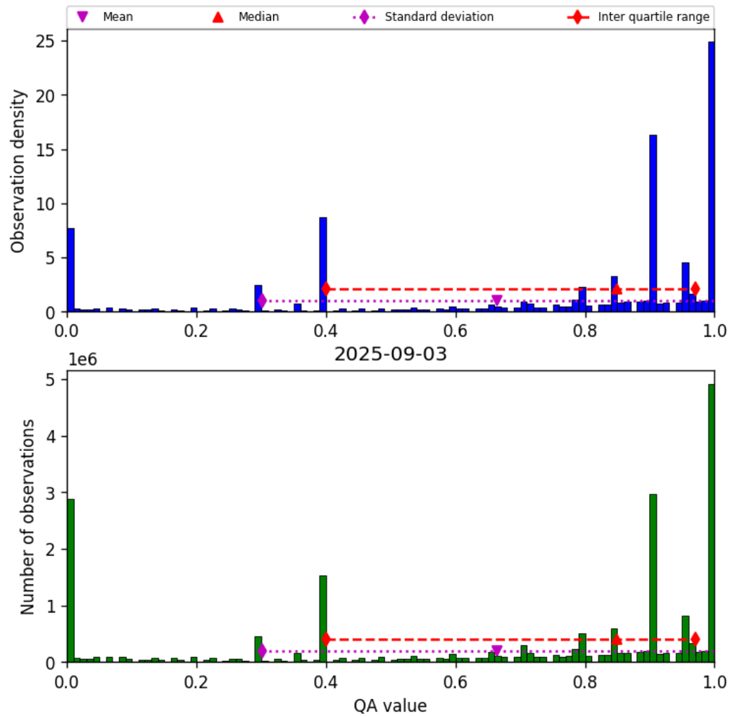
Figure 38: Histogram of “QA value” for 2025-09-02 to 2025-09-04
