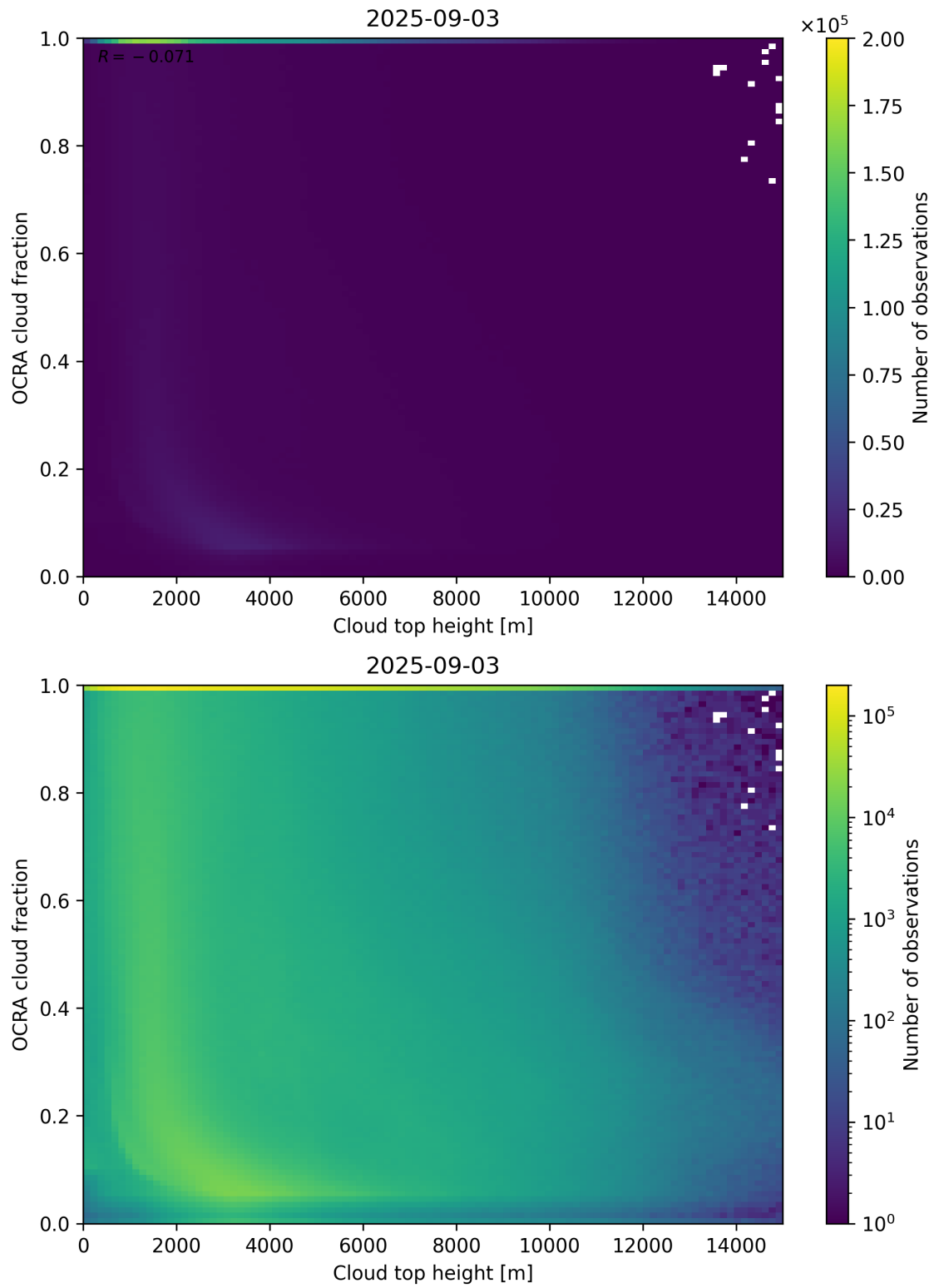
Figure 87: Scatter density plot of “Cloud top height” against “OCRA cloud fraction” for 2025-09-02 to 2025-09-04.
