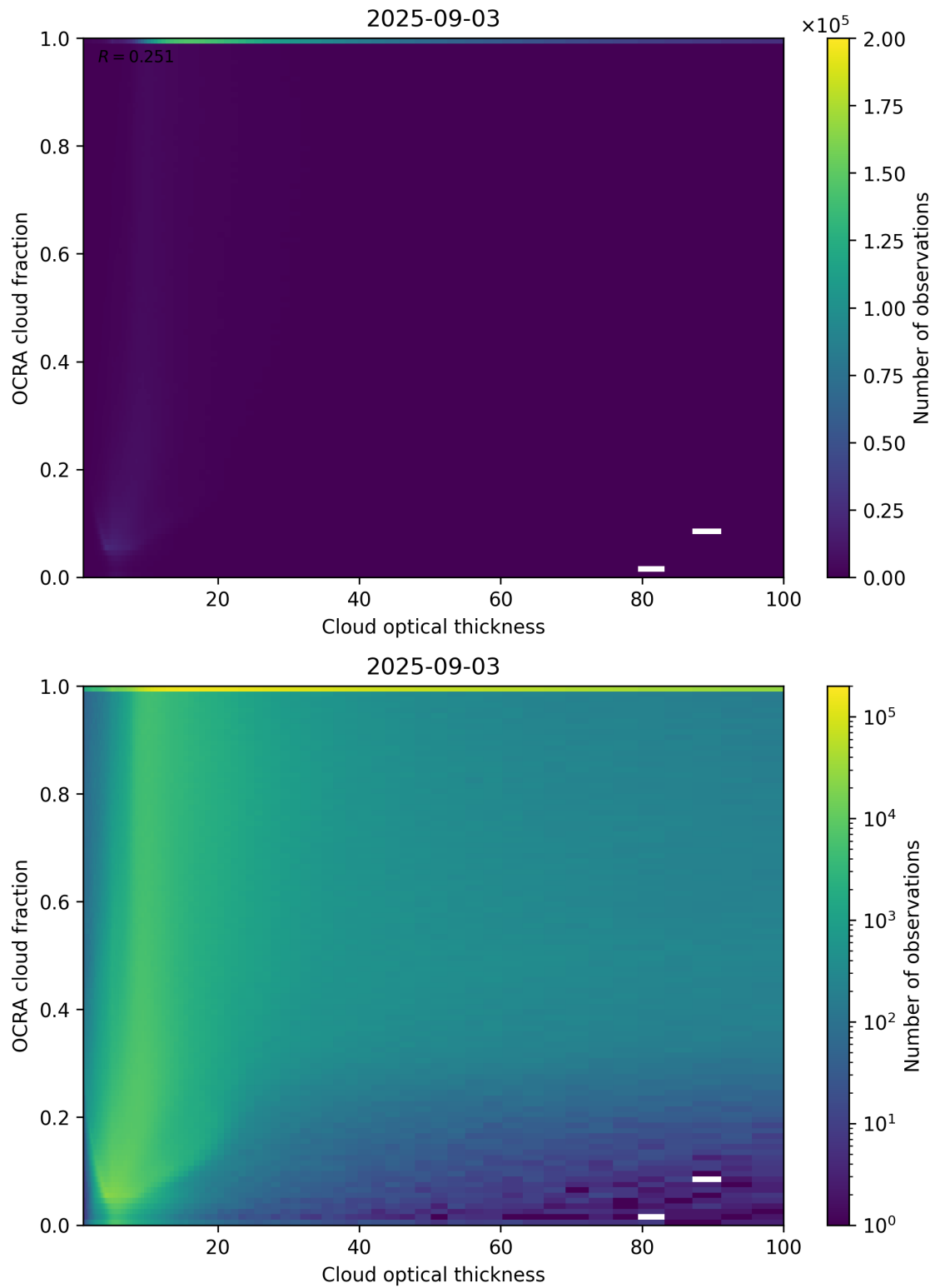
Figure 83: Scatter density plot of “Cloud optical thickness” against “OCRA cloud fraction” for 2025-09-02 to 2025-09-04.
