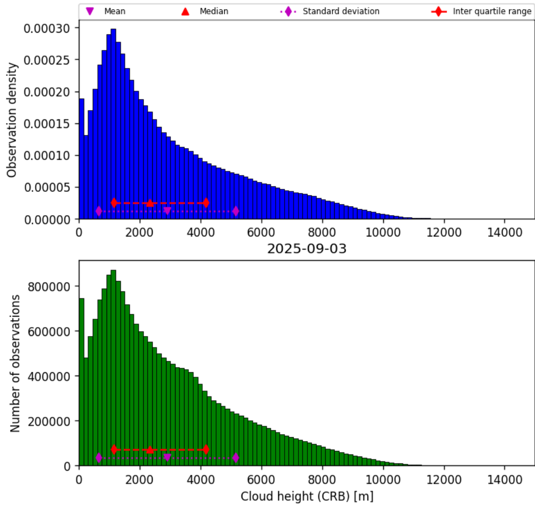
Figure 43: Histogram of “Cloud height (CRB)” for 2025-09-02 to 2025-09-04
