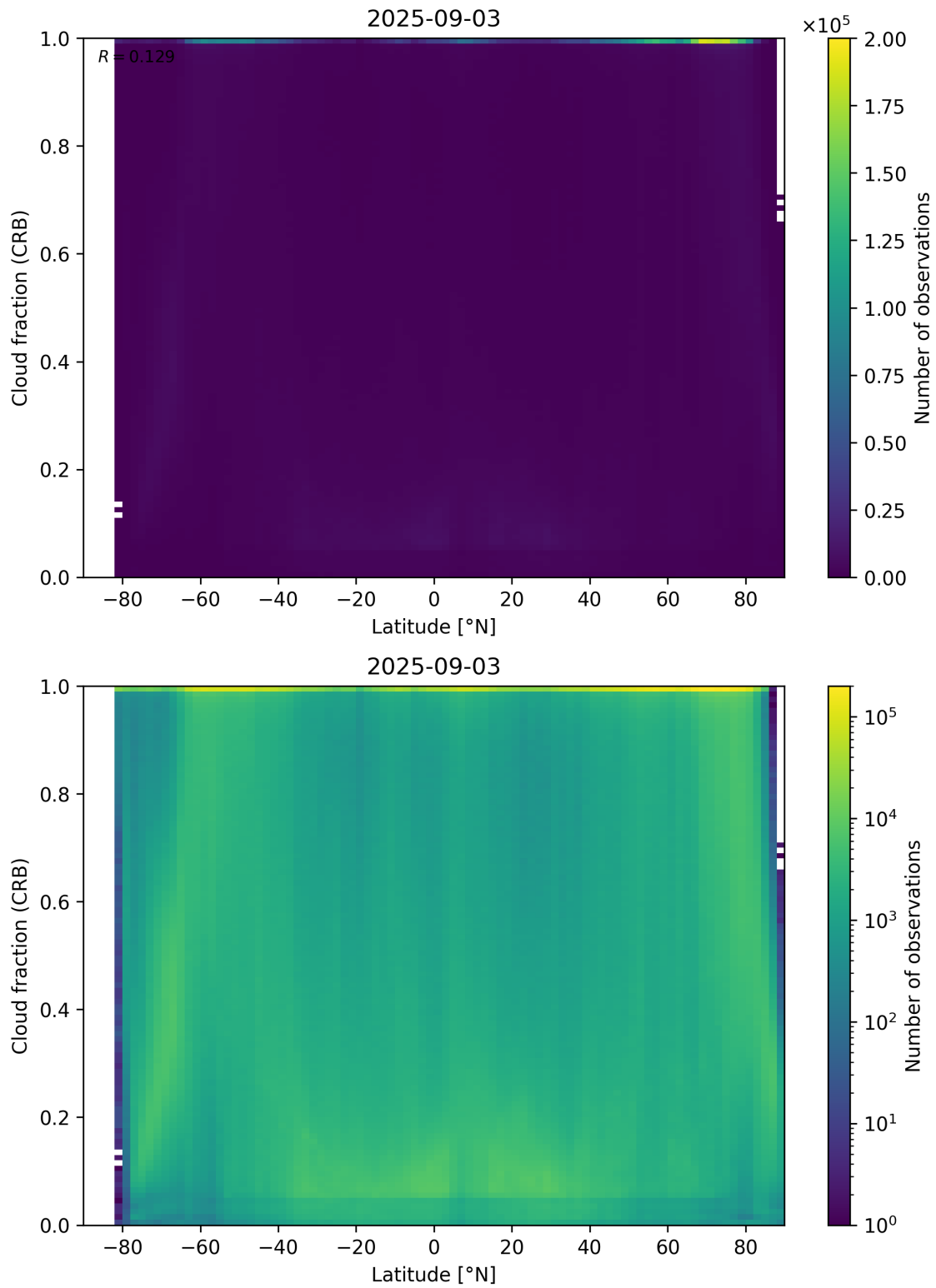
Figure 94: Scatter density plot of “Latitude” against “Cloud fraction (CRB)” for 2025-09-02 to 2025-09-04.
