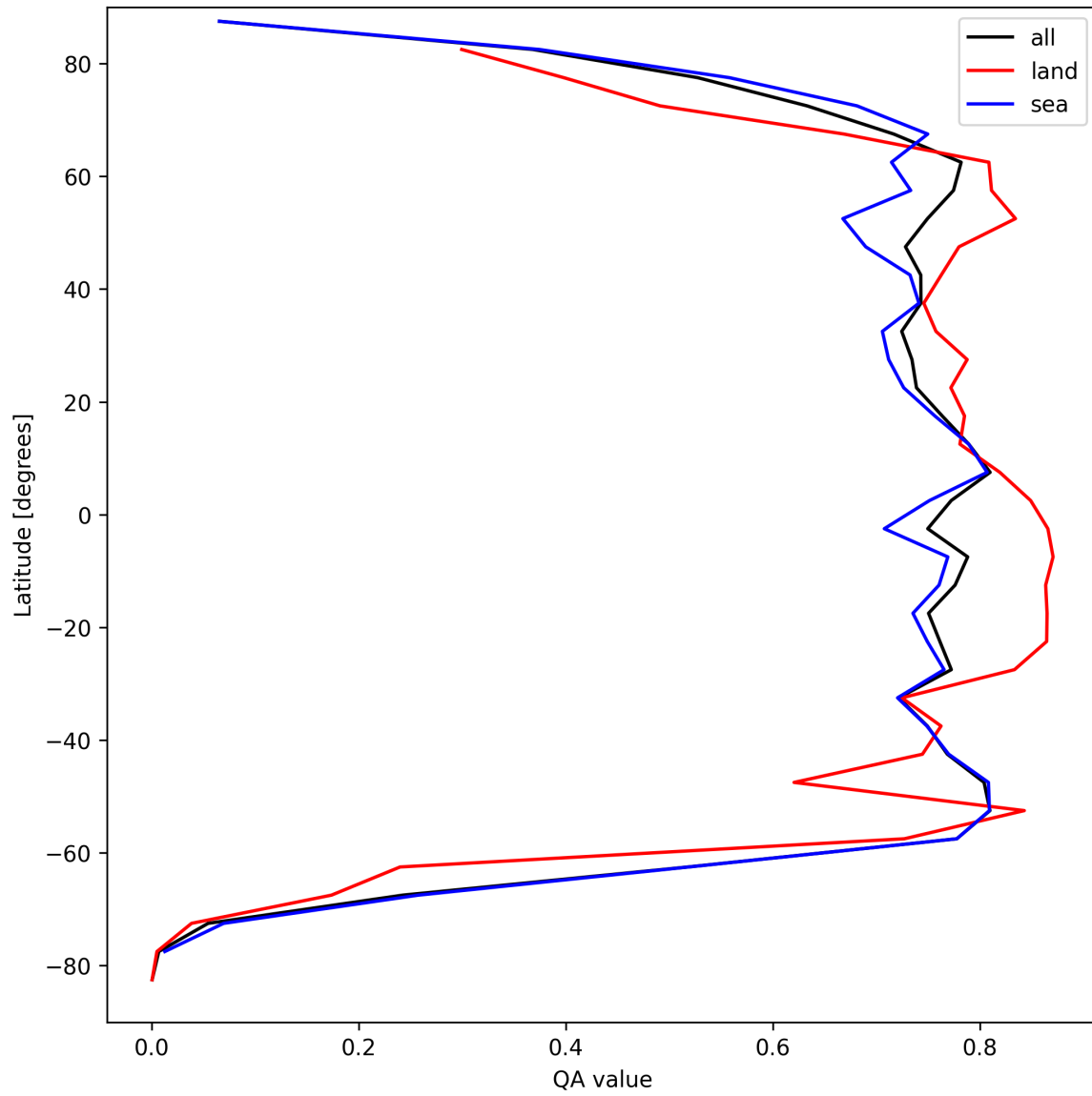
Figure 22: Zonal average of “QA value” for 2025-09-02 to 2025-09-04.
