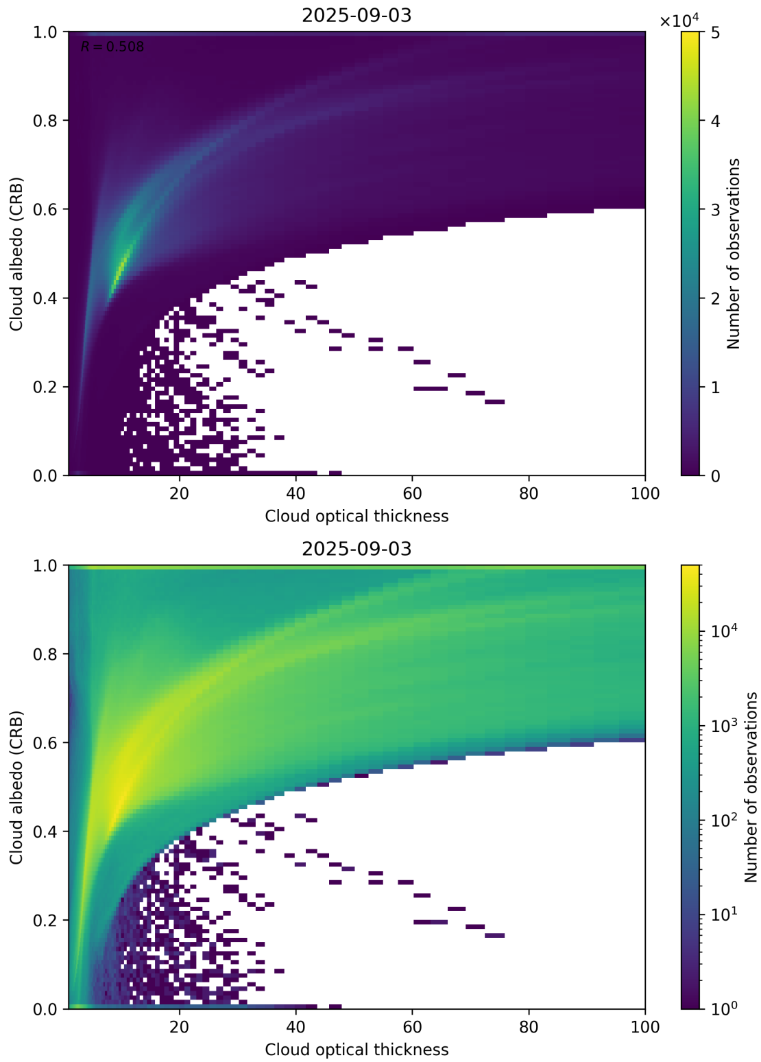
Figure 82: Scatter density plot of “Cloud optical thickness” against “Cloud albedo (CRB)” for 2025-09-02 to 2025-09-04.
