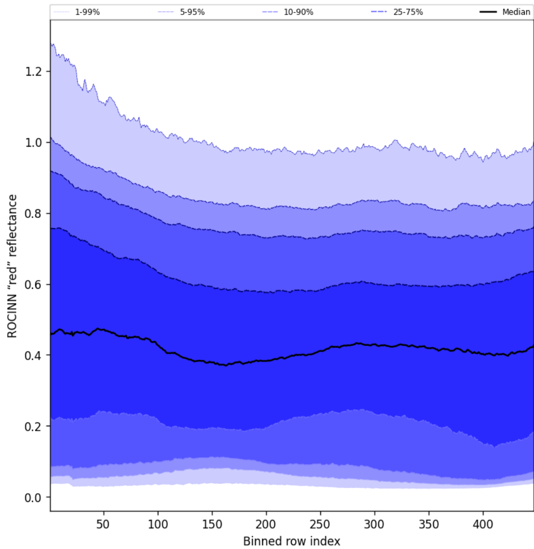
Figure 69: Along track statistics of “ROCINN “red” reflectance” for 2025-09-02 to 2025-09-04
