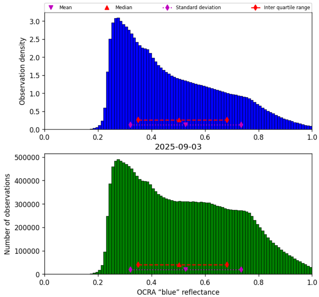
Figure 51: Histogram of “OCRA “blue” reflectance” for 2025-09-02 to 2025-09-04
