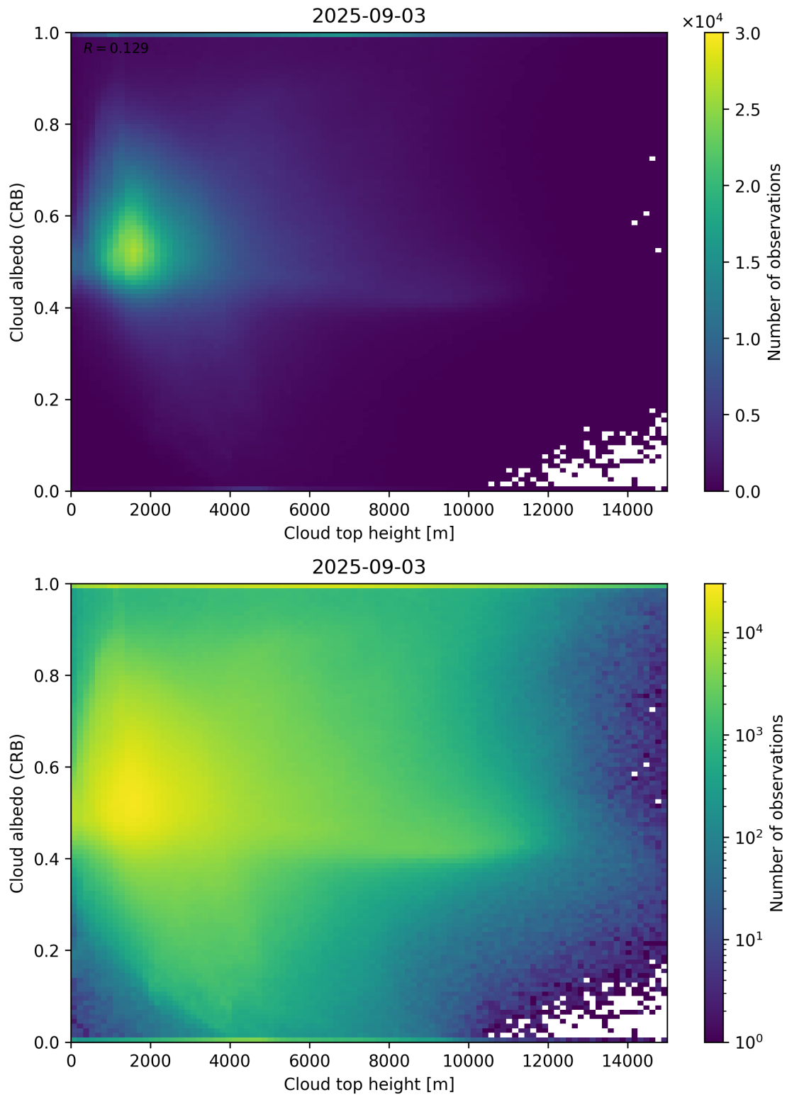
Figure 86: Scatter density plot of “Cloud top height” against “Cloud albedo (CRB)” for 2025-09-02 to 2025-09-04.
