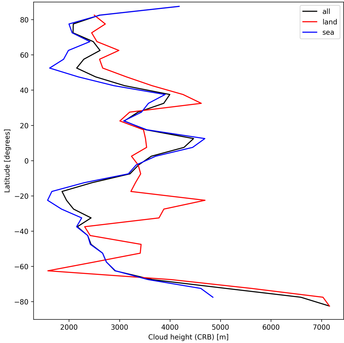
Figure 27: Zonal average of “Cloud height (CRB)” for 2025-09-02 to 2025-09-04.
