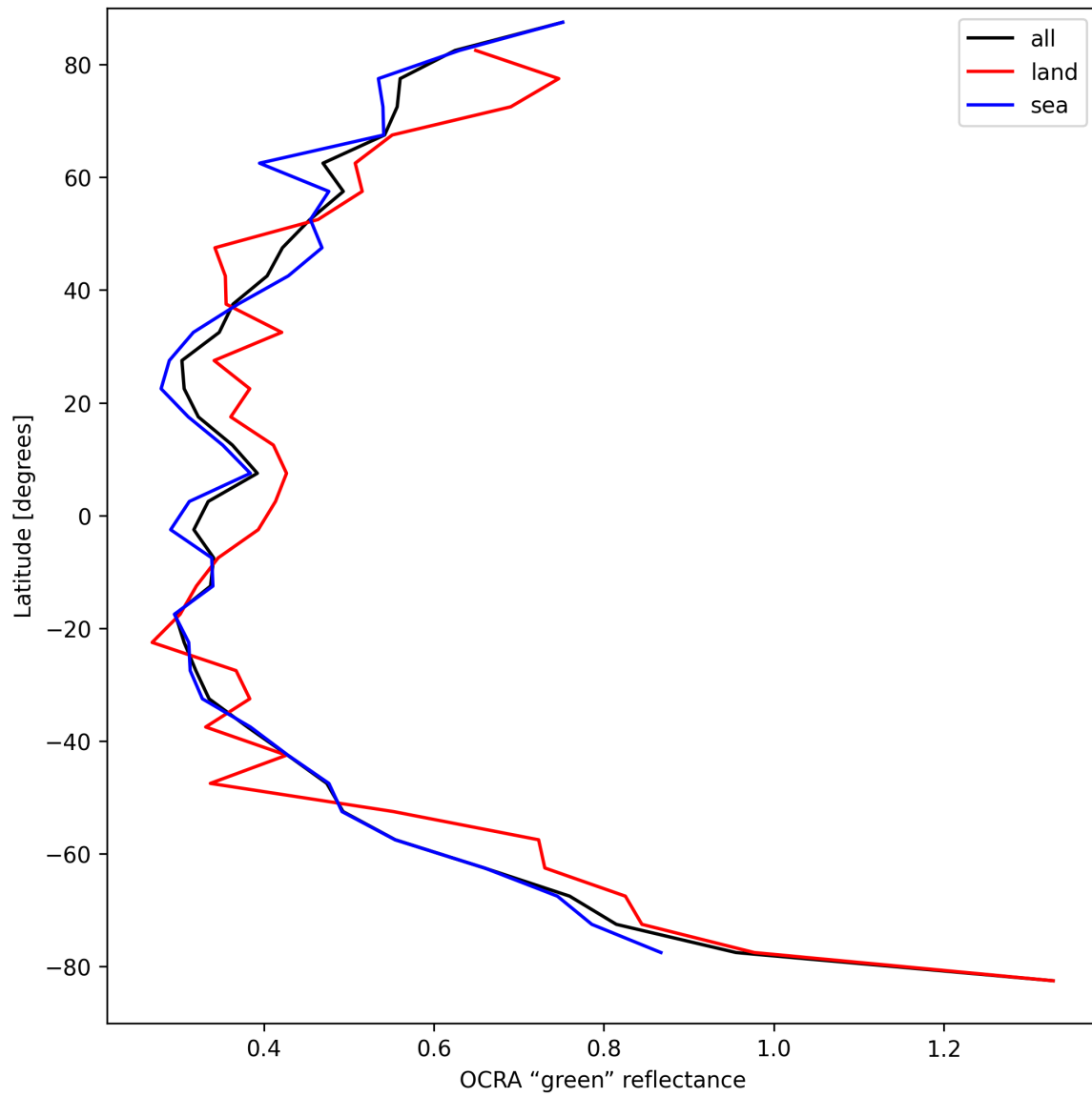
Figure 36: Zonal average of “OCRA “green” reflectance” for 2025-09-02 to 2025-09-04.
