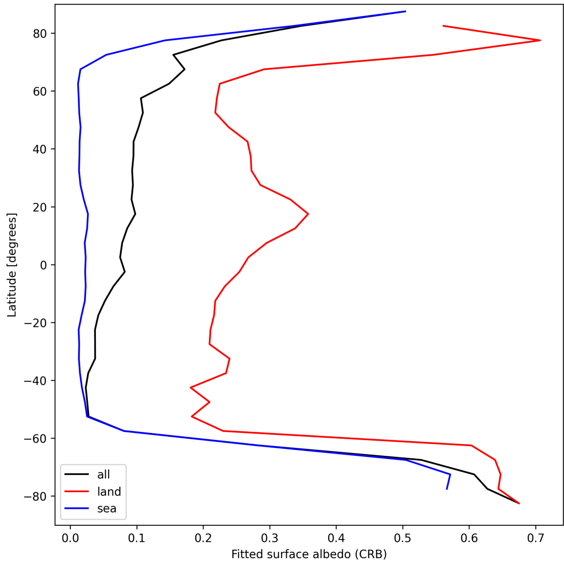
Figure 30: Zonal average of “Fitted surface albedo (CRB)” for 2025-09-02 to 2025-09-04.
