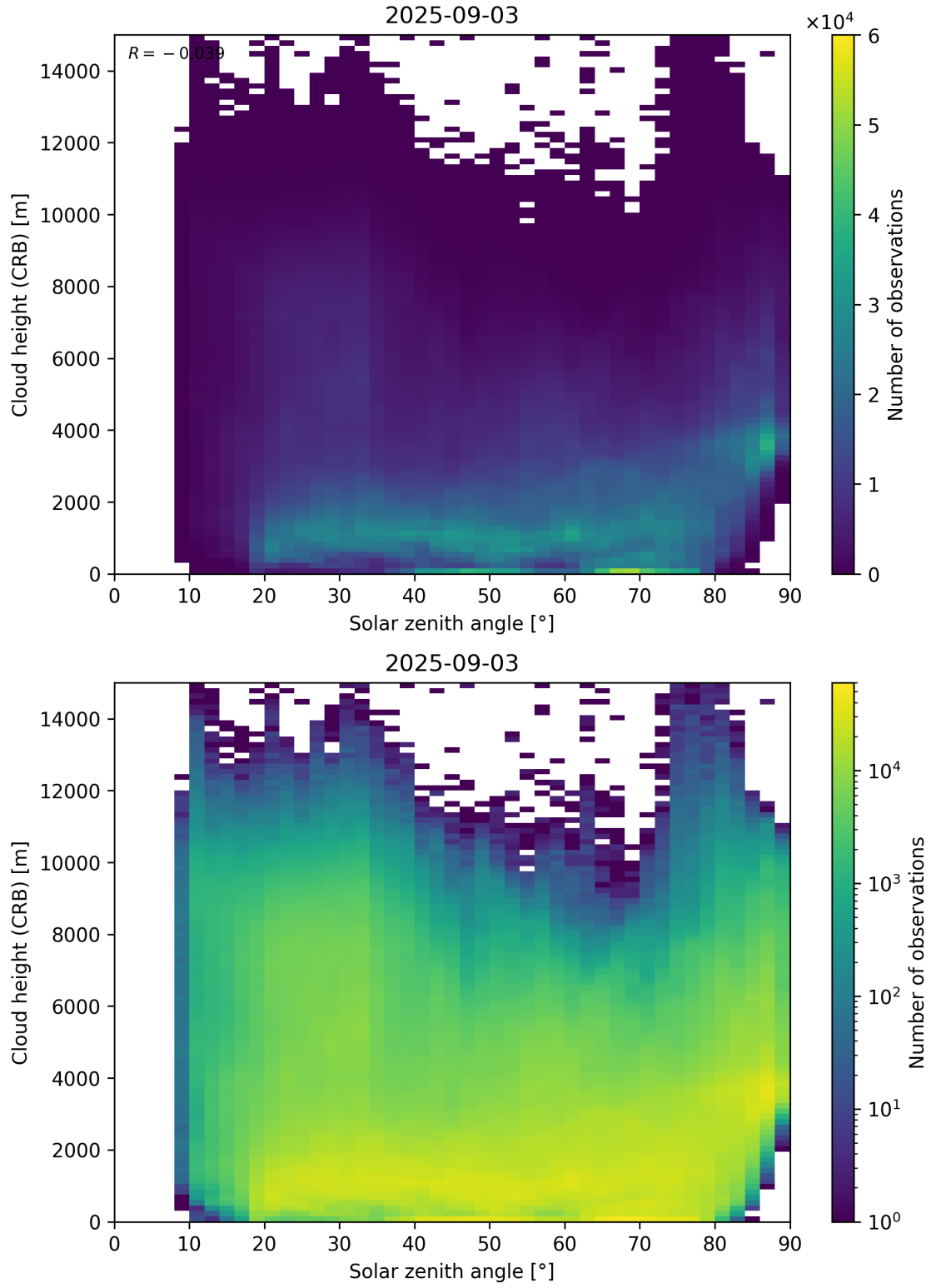
Figure 102: Scatter density plot of “Solar zenith angle” against “Cloud height (CRB)” for 2025-09-02 to 2025-09-04.
