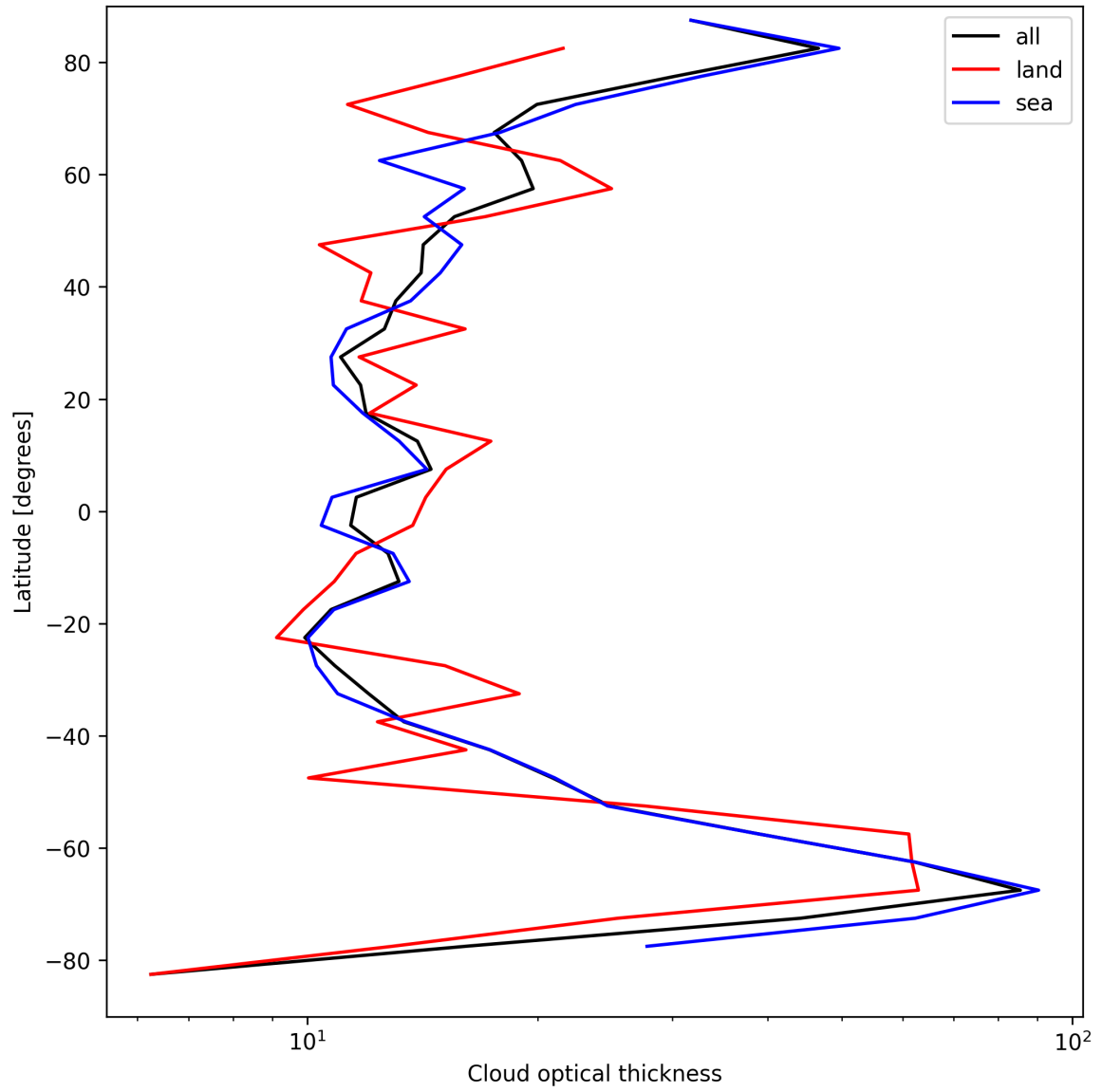
Figure 25: Zonal average of “Cloud optical thickness” for 2025-09-02 to 2025-09-04.
