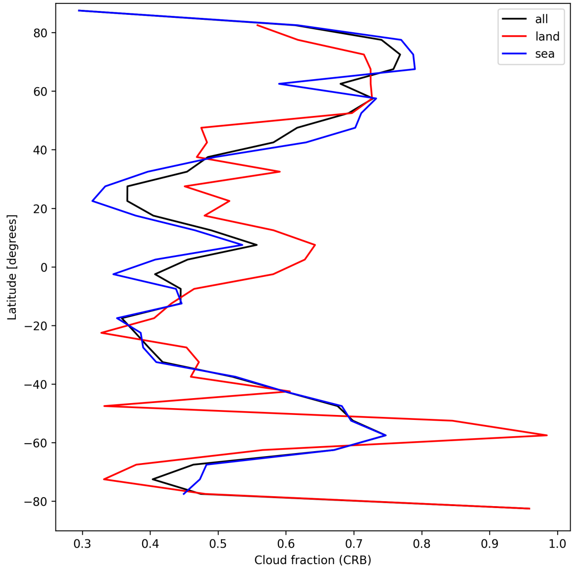
Figure 26: Zonal average of “Cloud fraction (CRB)” for 2025-09-02 to 2025-09-04.
