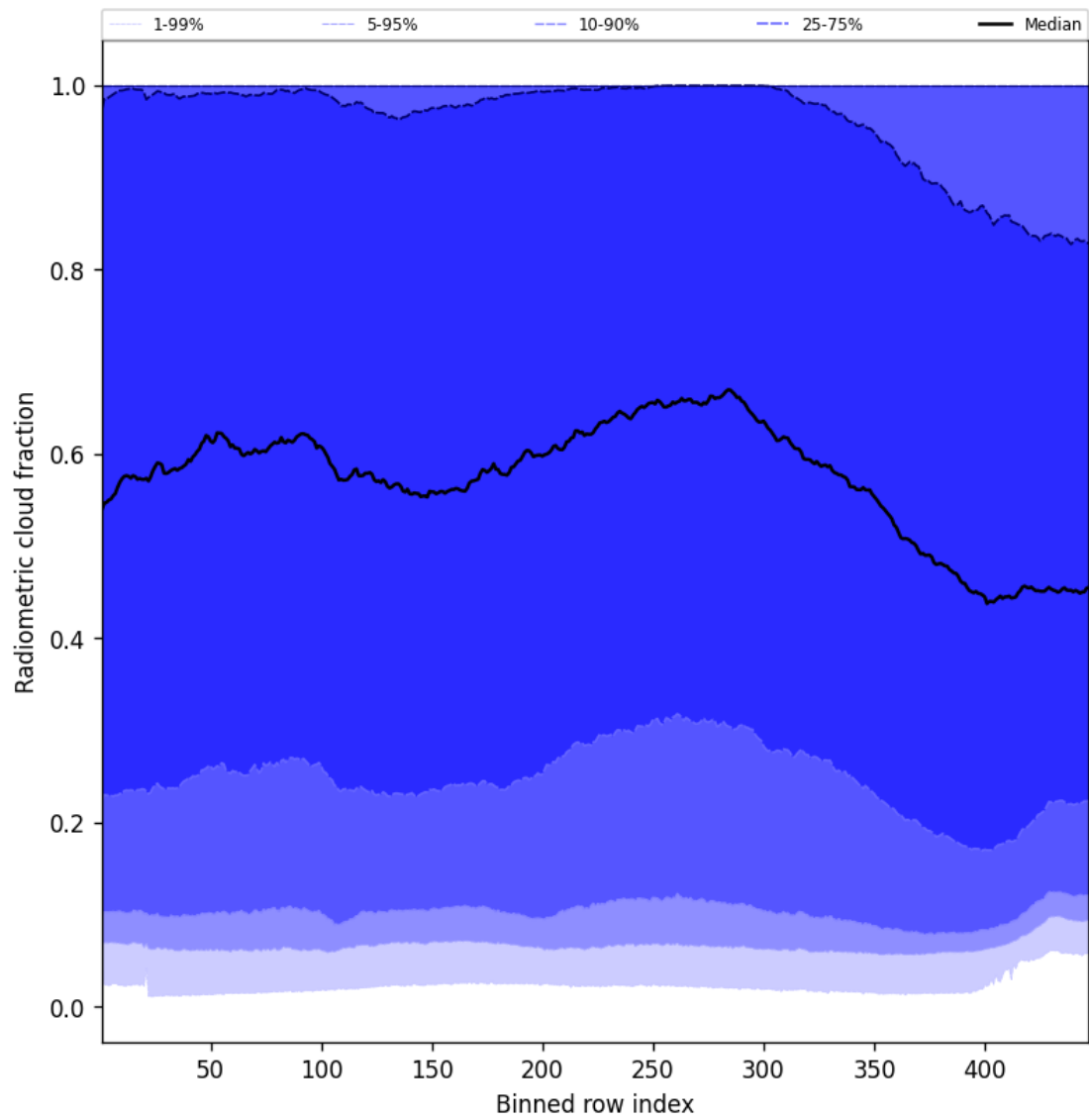
Figure 55: Along track statistics of “Radiometric cloud fraction” for 2025-09-02 to 2025-09-04
