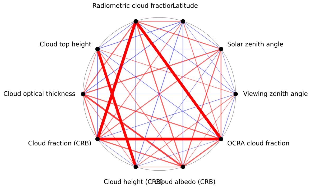
Figure 1: Map of correlation graph for 2025-09-02 to 2025-09-04.
