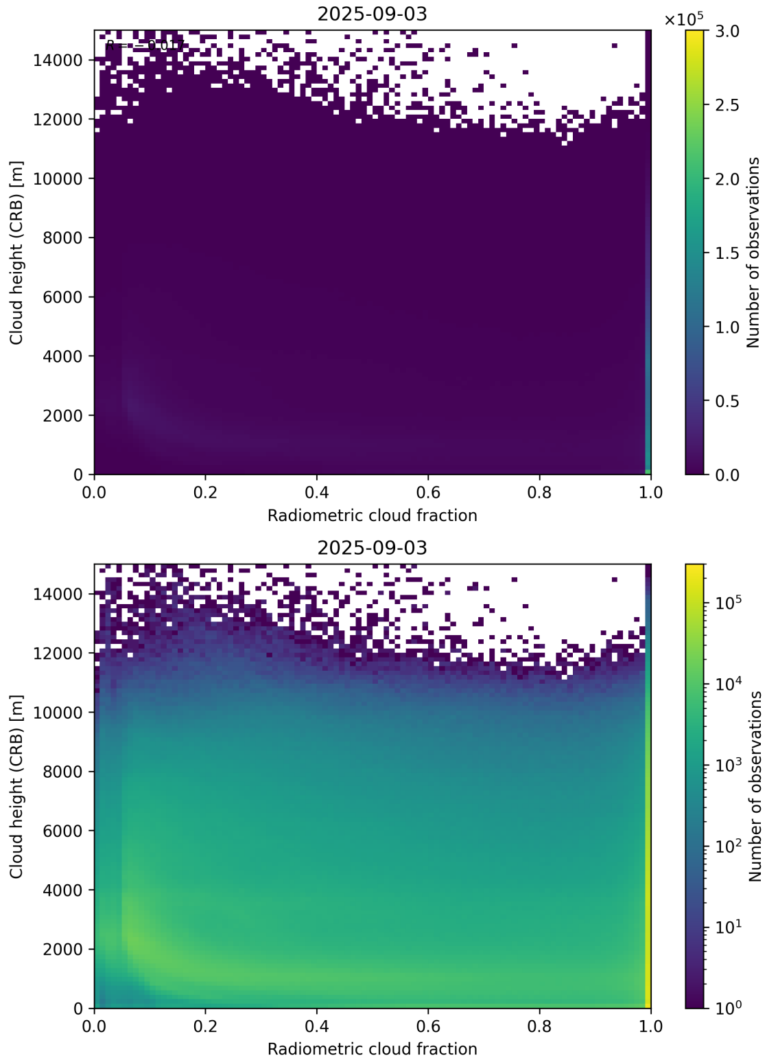
Figure 74: Scatter density plot of “Radiometric cloud fraction” against “Cloud height (CRB)” for 2025-09-02 to 2025-09-04.
