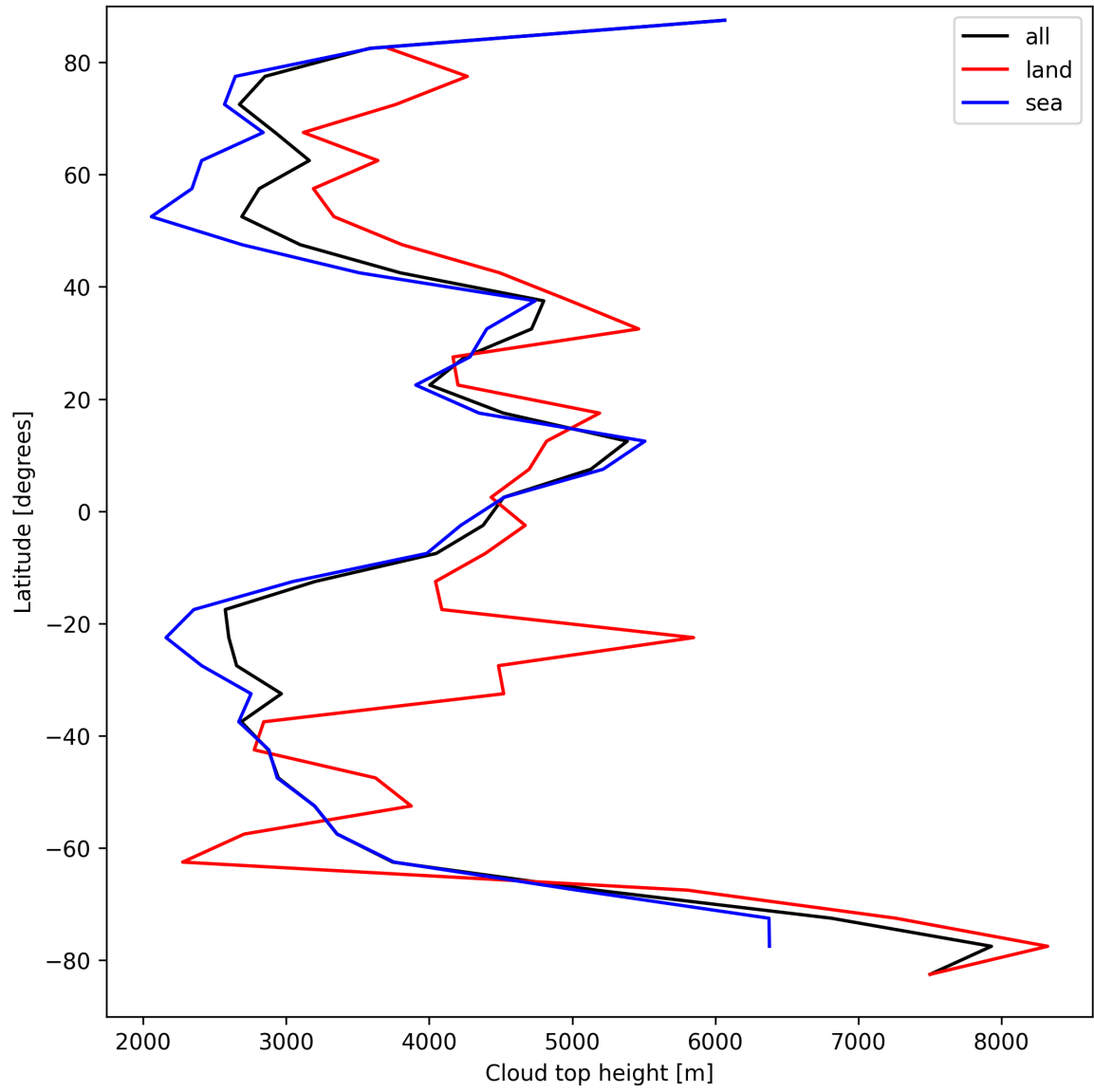
Figure 24: Zonal average of “Cloud top height” for 2025-09-02 to 2025-09-04.
