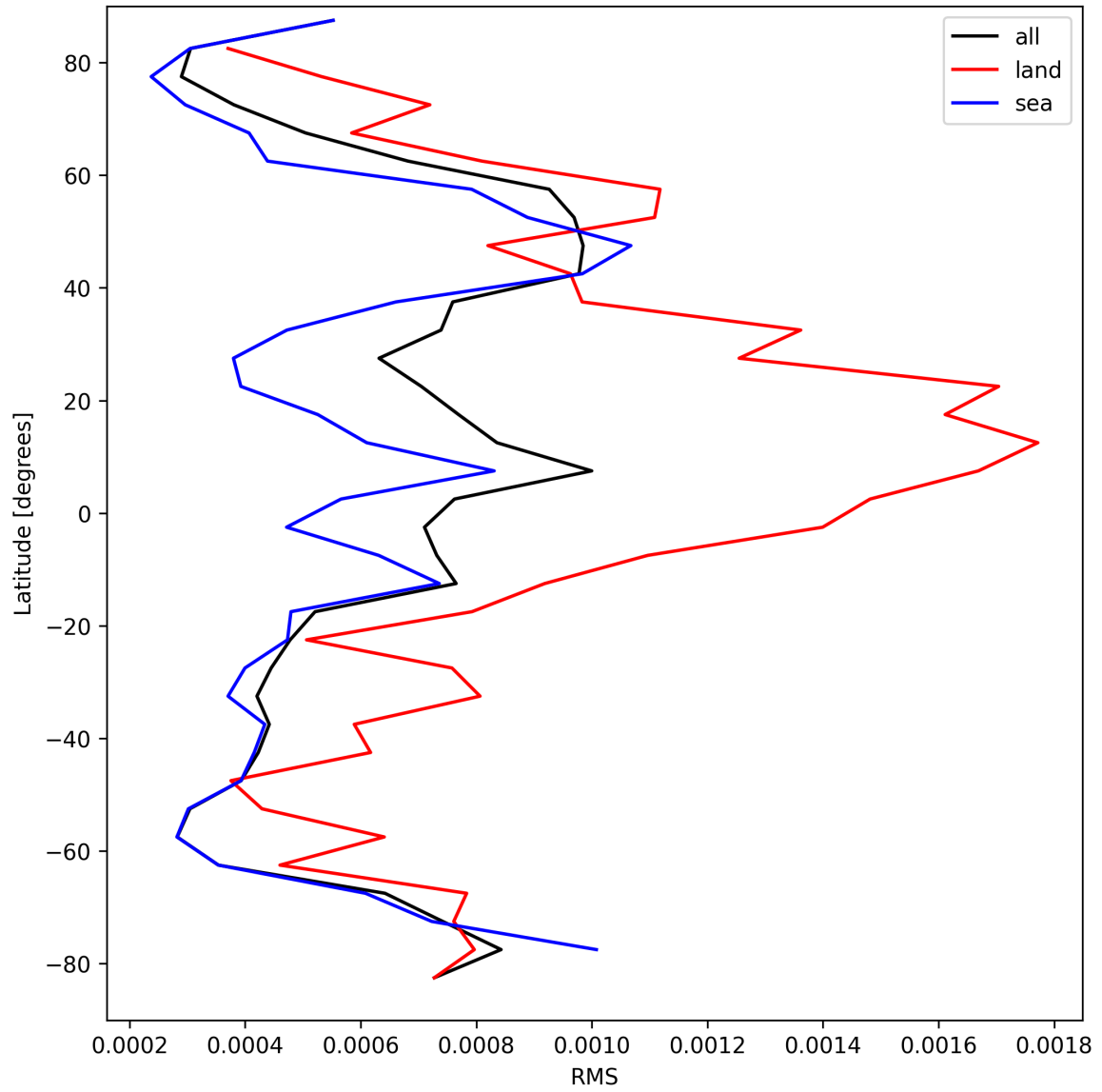
Figure 31: Zonal average of “RMS” for 2025-09-02 to 2025-09-04.
