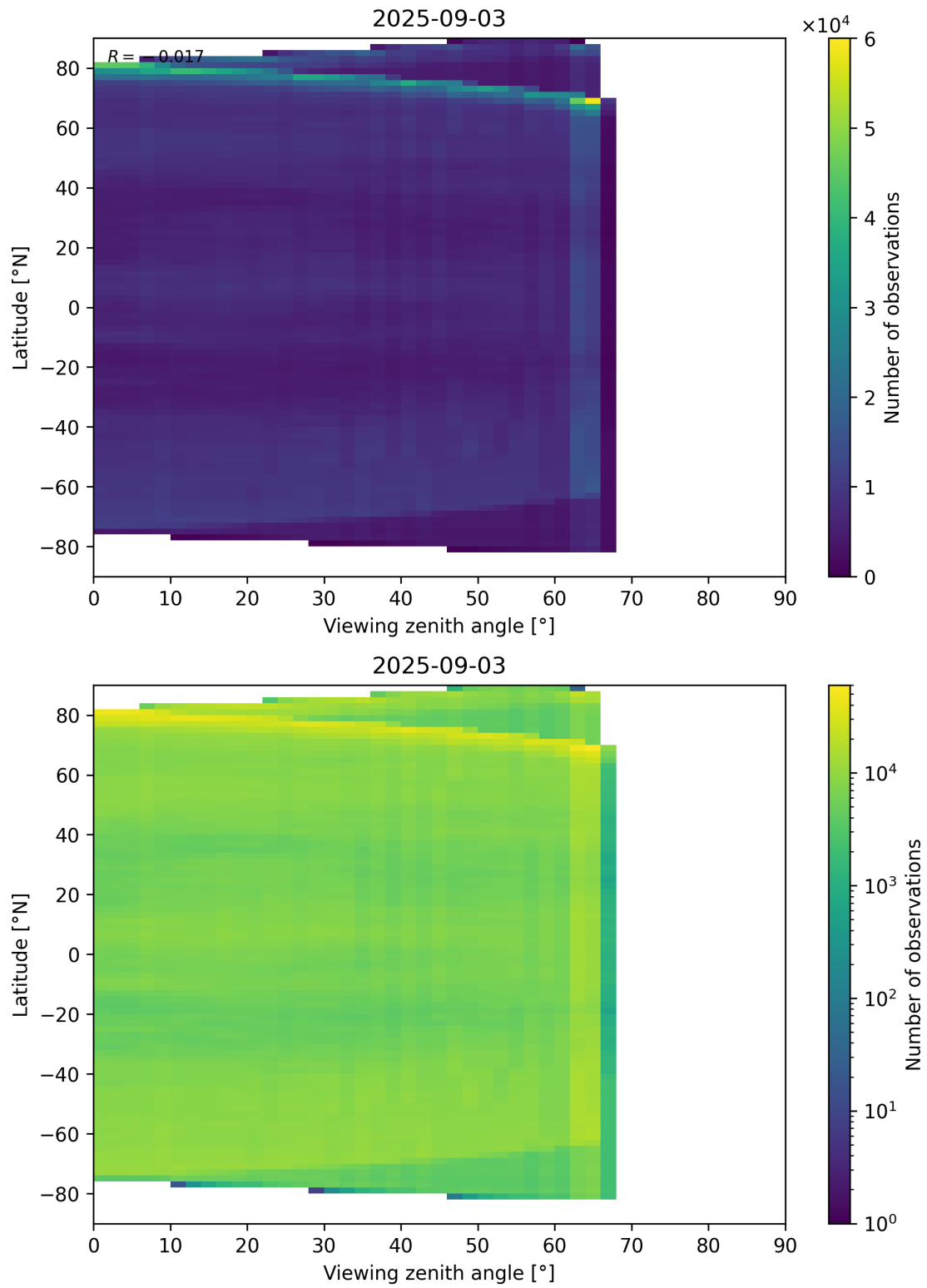
Figure 113: Scatter density plot of “Viewing zenith angle” against “Latitude” for 2025-09-02 to 2025-09-04.
