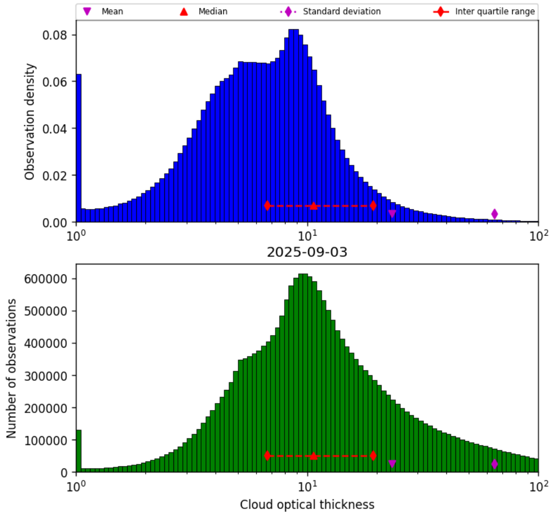
Figure 41: Histogram of “Cloud optical thickness” for 2025-09-02 to 2025-09-04
