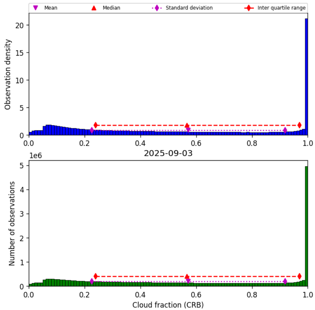
Figure 42: Histogram of “Cloud fraction (CRB)” for 2025-09-02 to 2025-09-04
