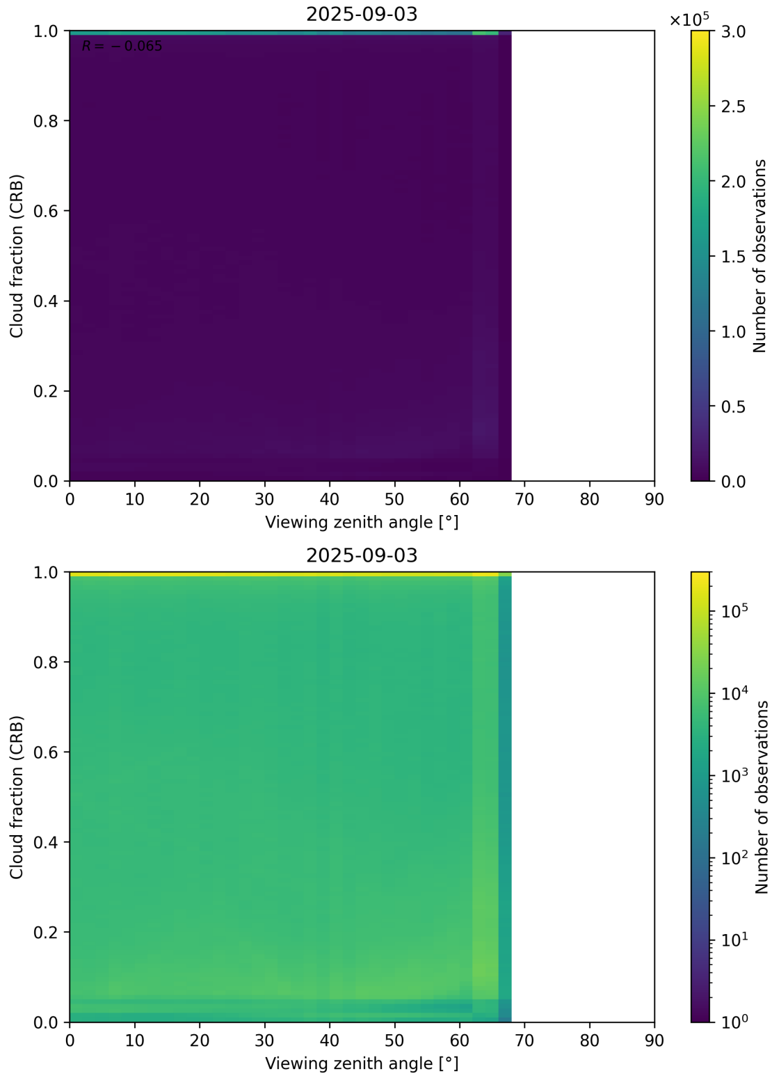
Figure 109: Scatter density plot of “Viewing zenith angle” against “Cloud fraction (CRB)” for 2025-09-02 to 2025-09-04.
