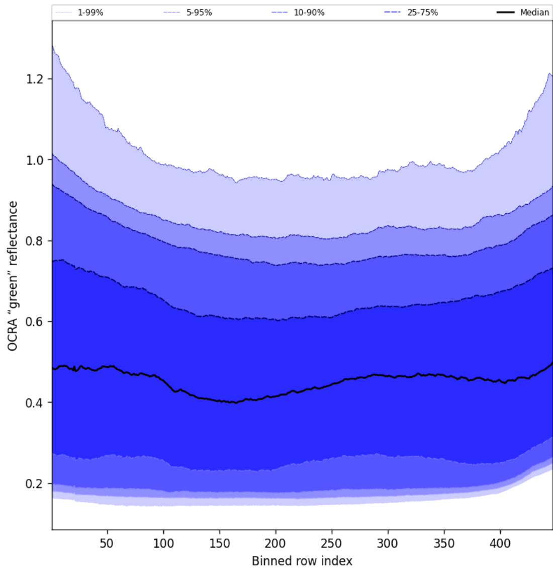
Figure 68: Along track statistics of “OCRA “green” reflectance” for 2025-09-02 to 2025-09-04
