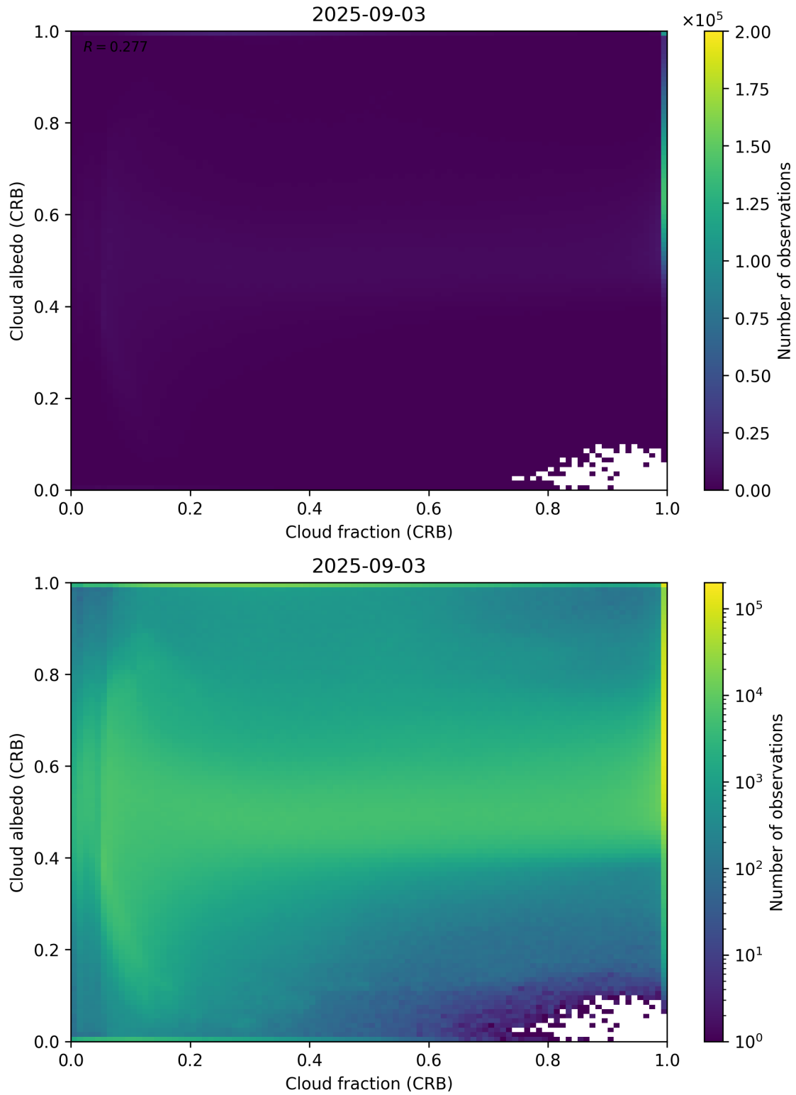
Figure 77: Scatter density plot of “Cloud fraction (CRB)” against “Cloud albedo (CRB)” for 2025-09-02 to 2025-09-04.
