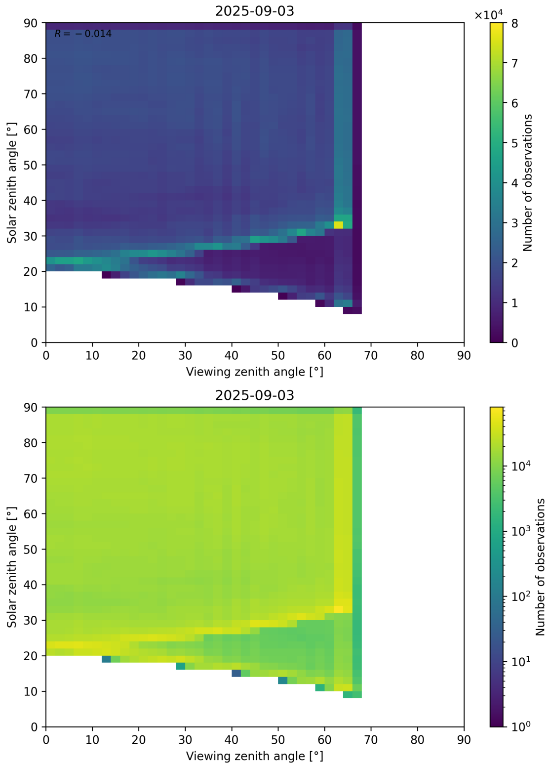
Figure 114: Scatter density plot of “Viewing zenith angle” against “Solar zenith angle” for 2025-09-02 to 2025-09-04.
