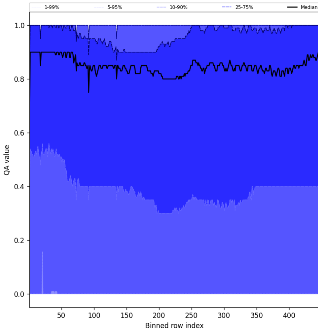
Figure 54: Along track statistics of “QA value” for 2025-09-02 to 2025-09-04
