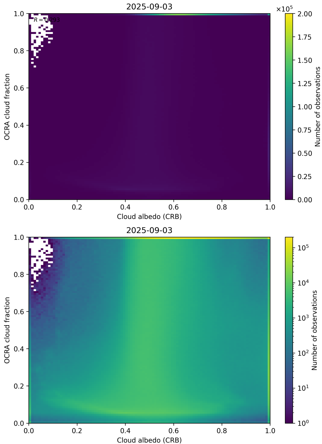
Figure 70: Scatter density plot of “Cloud albedo (CRB)” against “OCRA cloud fraction” for 2025-09-02 to 2025-09-04.
