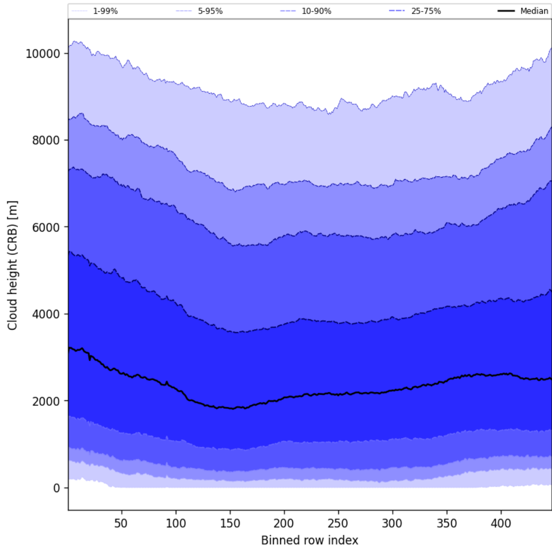
Figure 59: Along track statistics of “Cloud height (CRB)” for 2025-09-02 to 2025-09-04
