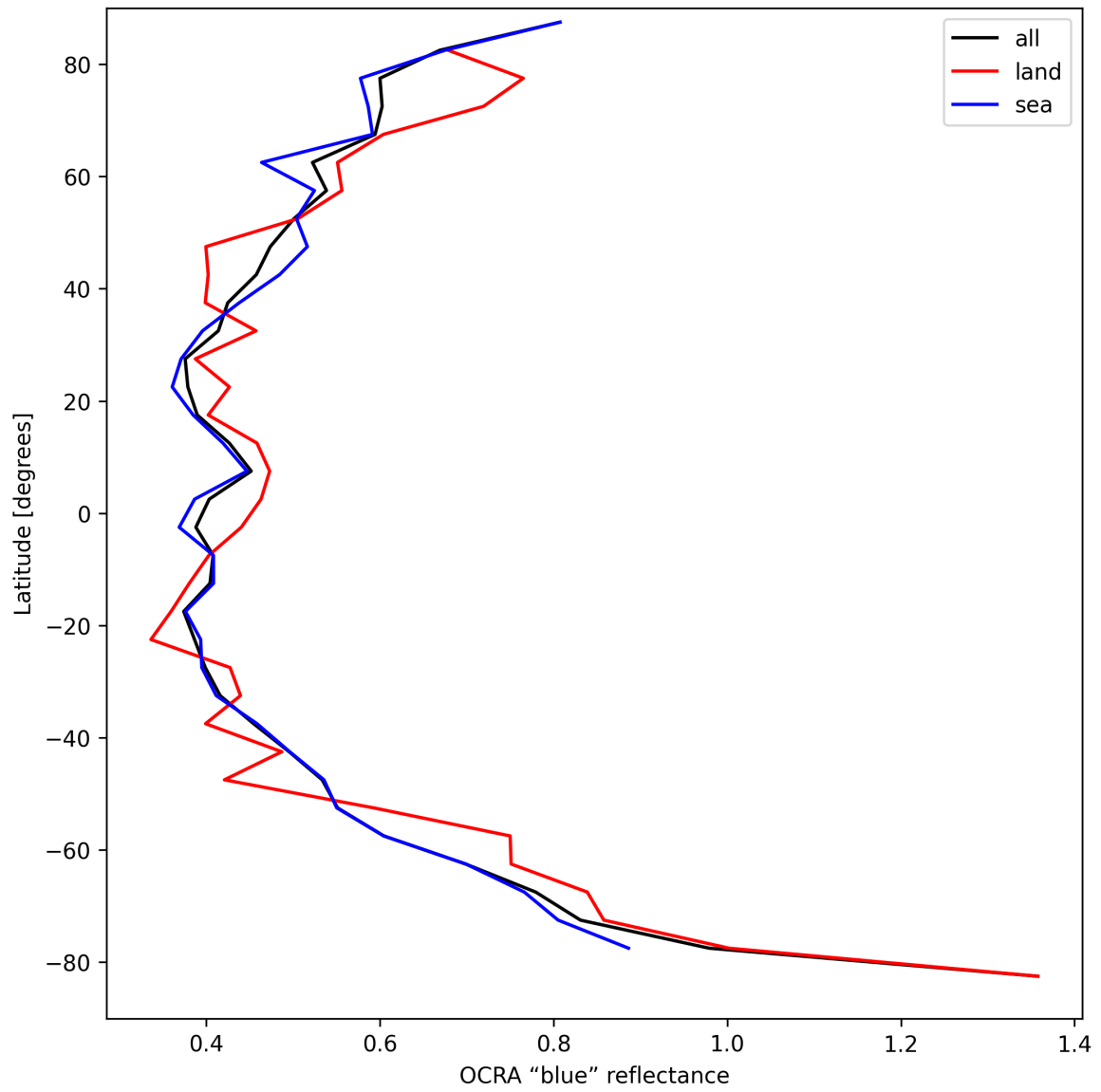
Figure 35: Zonal average of “OCRA “blue” reflectance” for 2025-09-02 to 2025-09-04.
