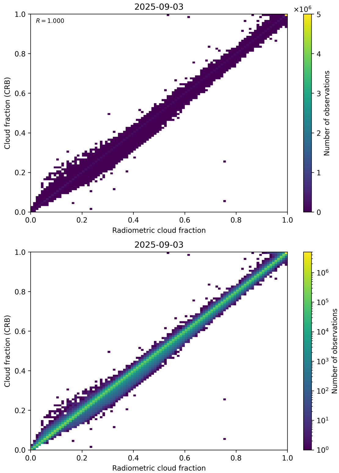
Figure 73: Scatter density plot of “Radiometric cloud fraction” against “Cloud fraction (CRB)” for 2025-09-02 to 2025-09-04.
