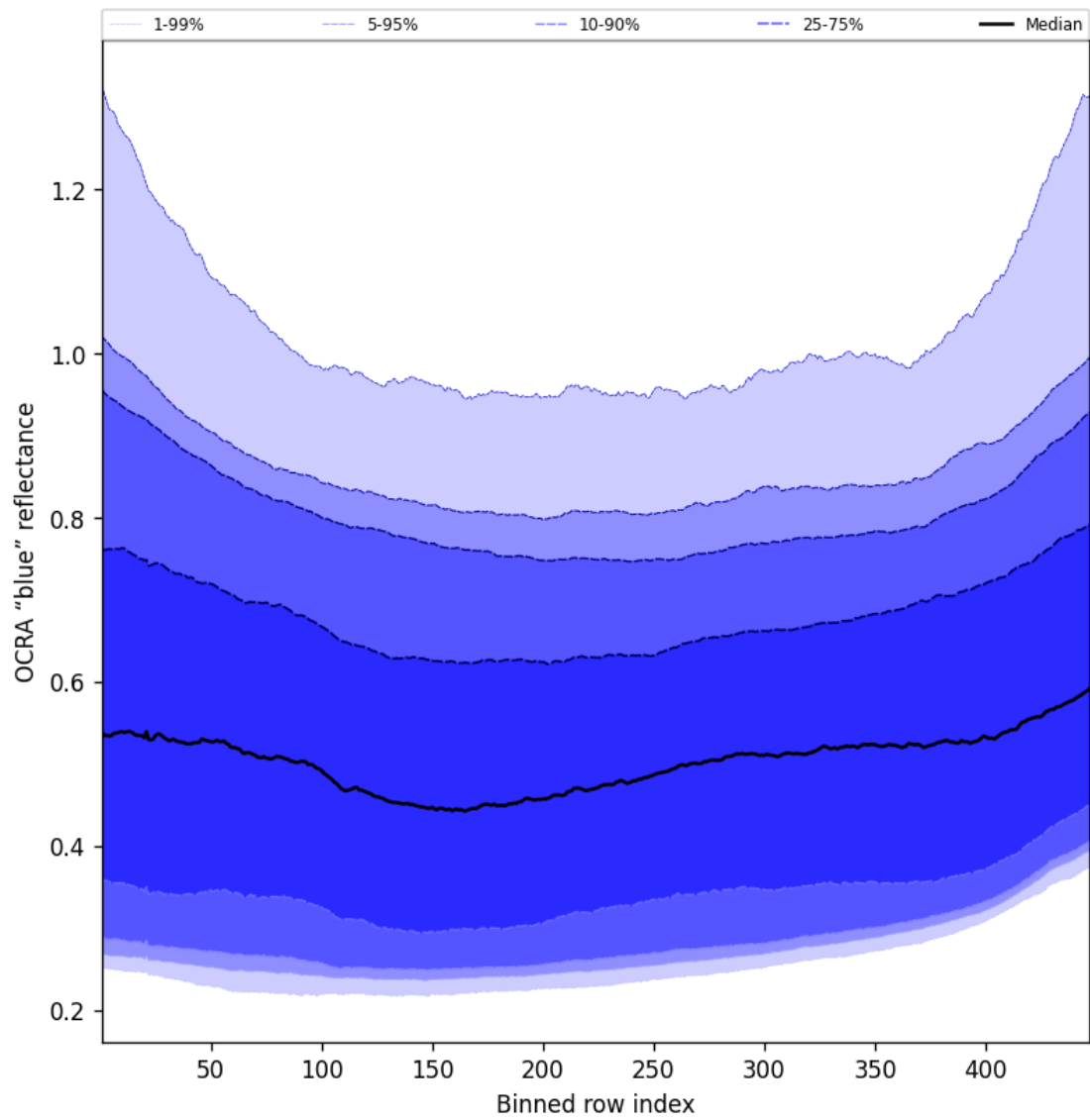
Figure 67: Along track statistics of “OCRA “blue” reflectance” for 2025-09-02 to 2025-09-04
