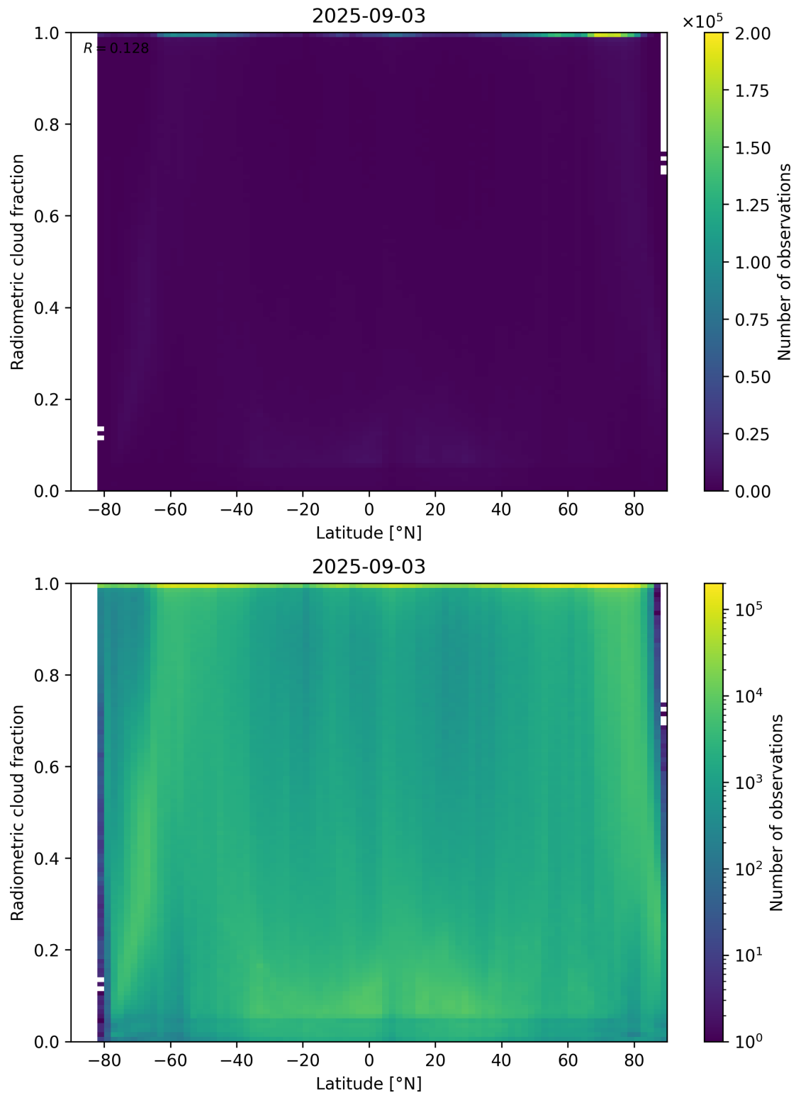
Figure 92: Scatter density plot of “Latitude” against “Radiometric cloud fraction” for 2025-09-02 to 2025-09-04.
