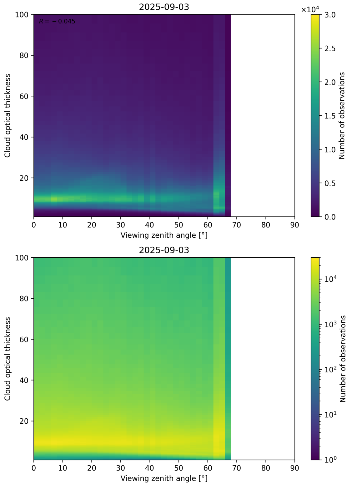
Figure 111: Scatter density plot of “Viewing zenith angle” against “Cloud optical thickness” for 2025-09-02 to 2025-09-04.
