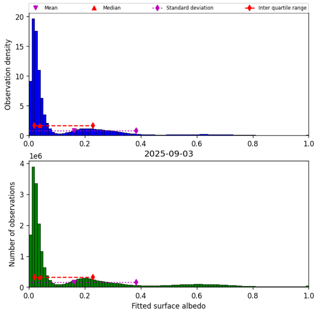
Figure 45: Histogram of “Fitted surface albedo” for 2025-09-02 to 2025-09-04
