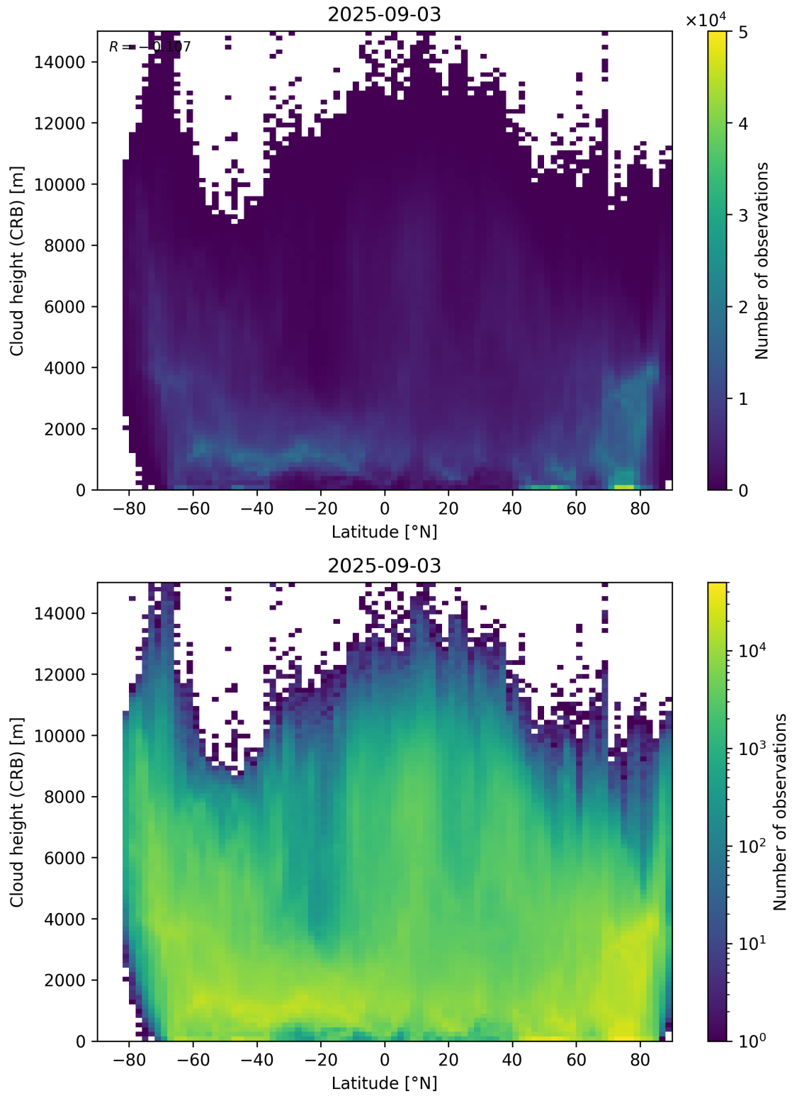
Figure 95: Scatter density plot of “Latitude” against “Cloud height (CRB)” for 2025-09-02 to 2025-09-04.
