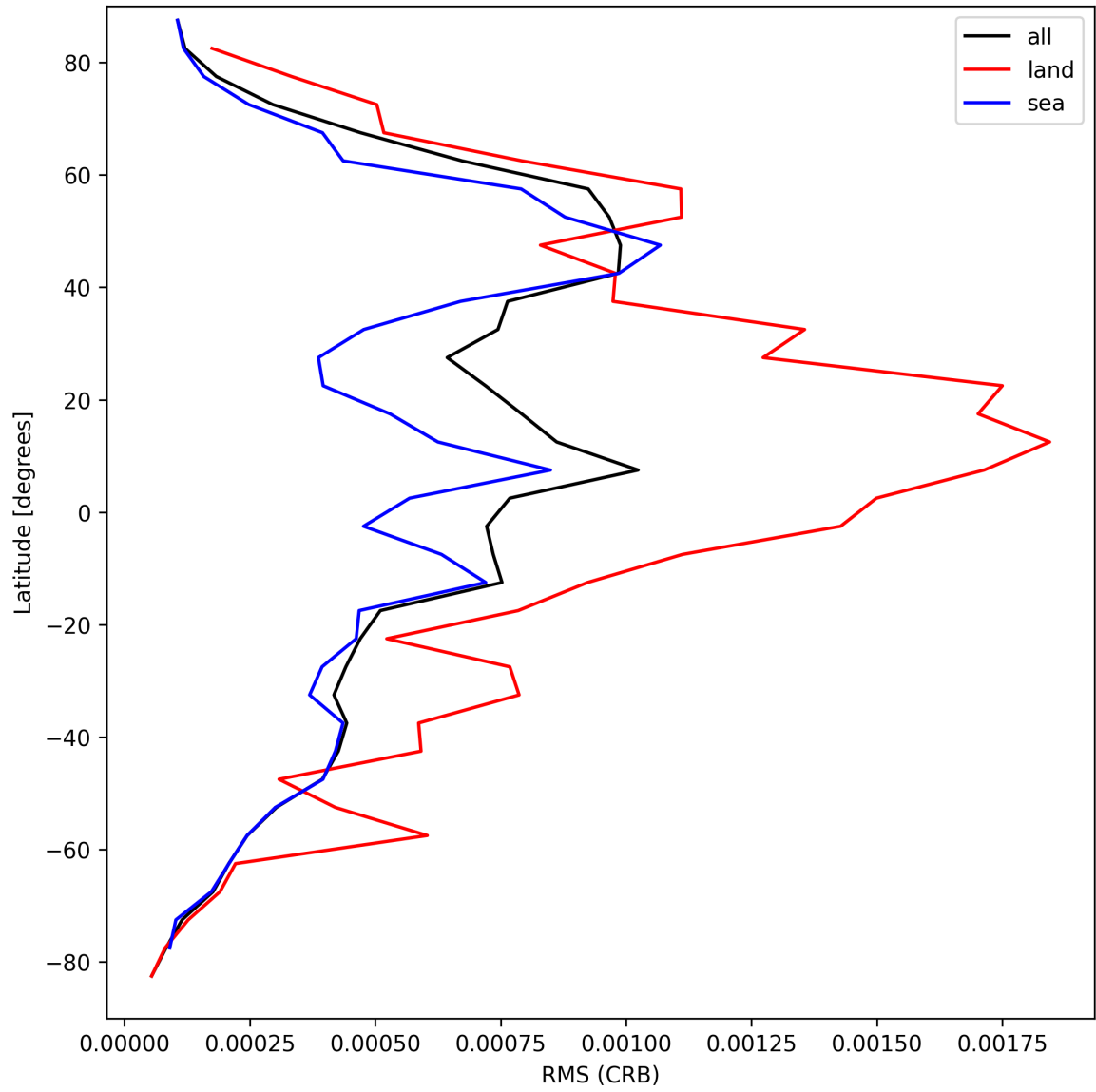
Figure 32: Zonal average of “RMS (CRB)” for 2025-09-02 to 2025-09-04.
