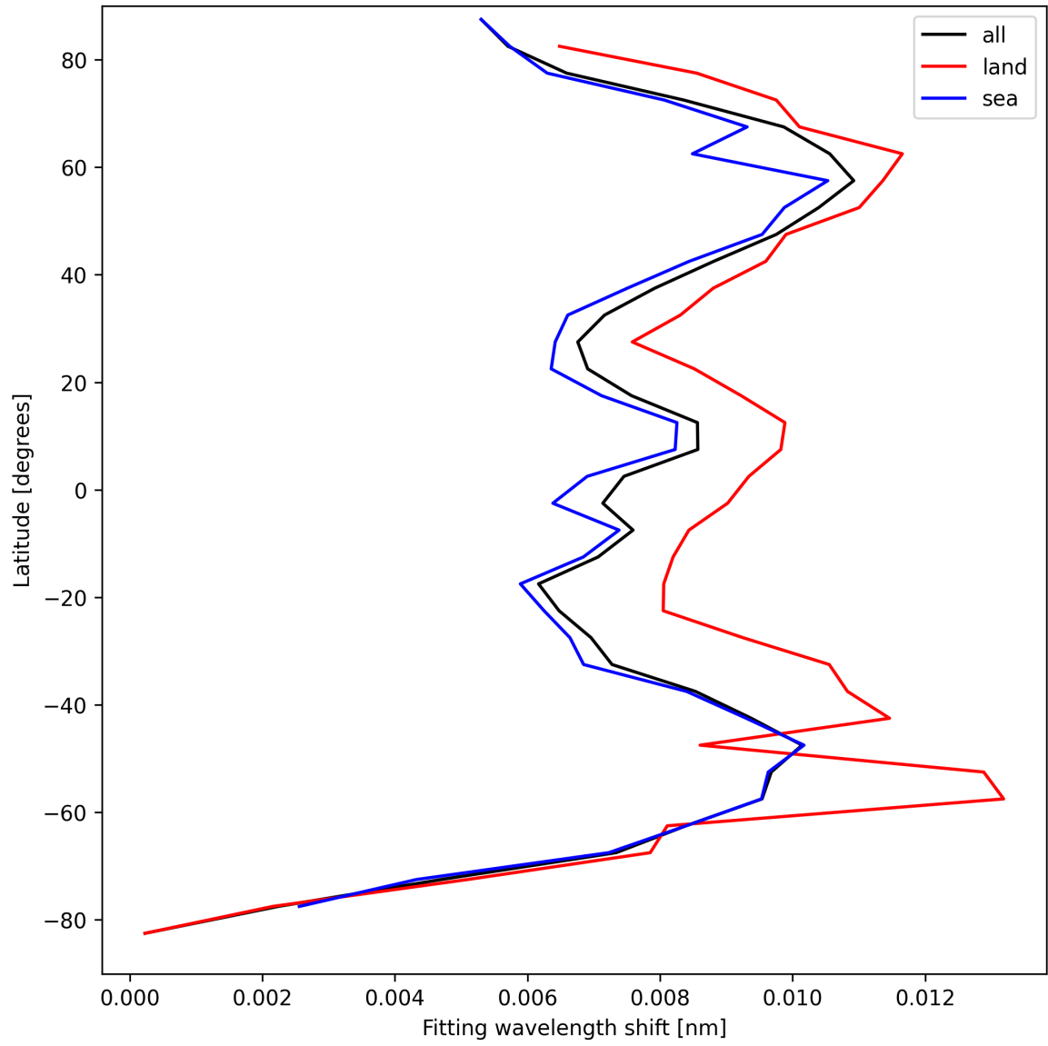
Figure 33: Zonal average of “Fitting wavelength shift” for 2025-09-02 to 2025-09-04.
