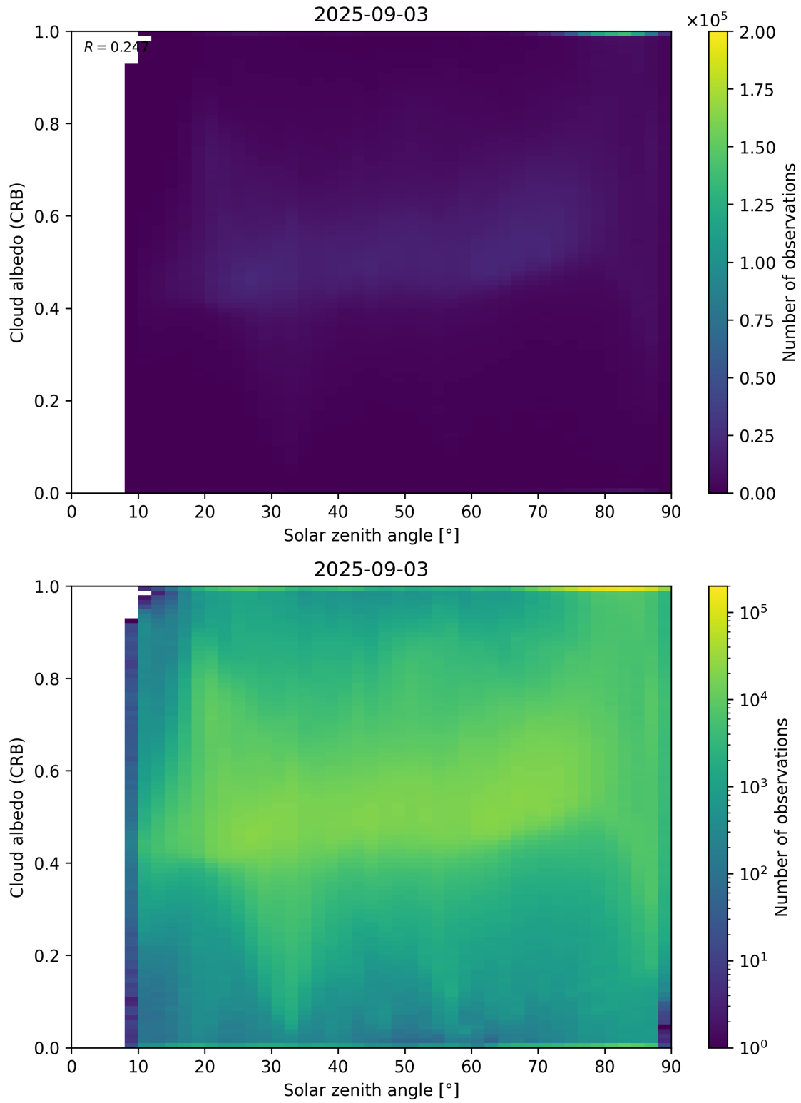
Figure 98: Scatter density plot of “Solar zenith angle” against “Cloud albedo (CRB)” for 2025-09-02 to 2025-09-04.
