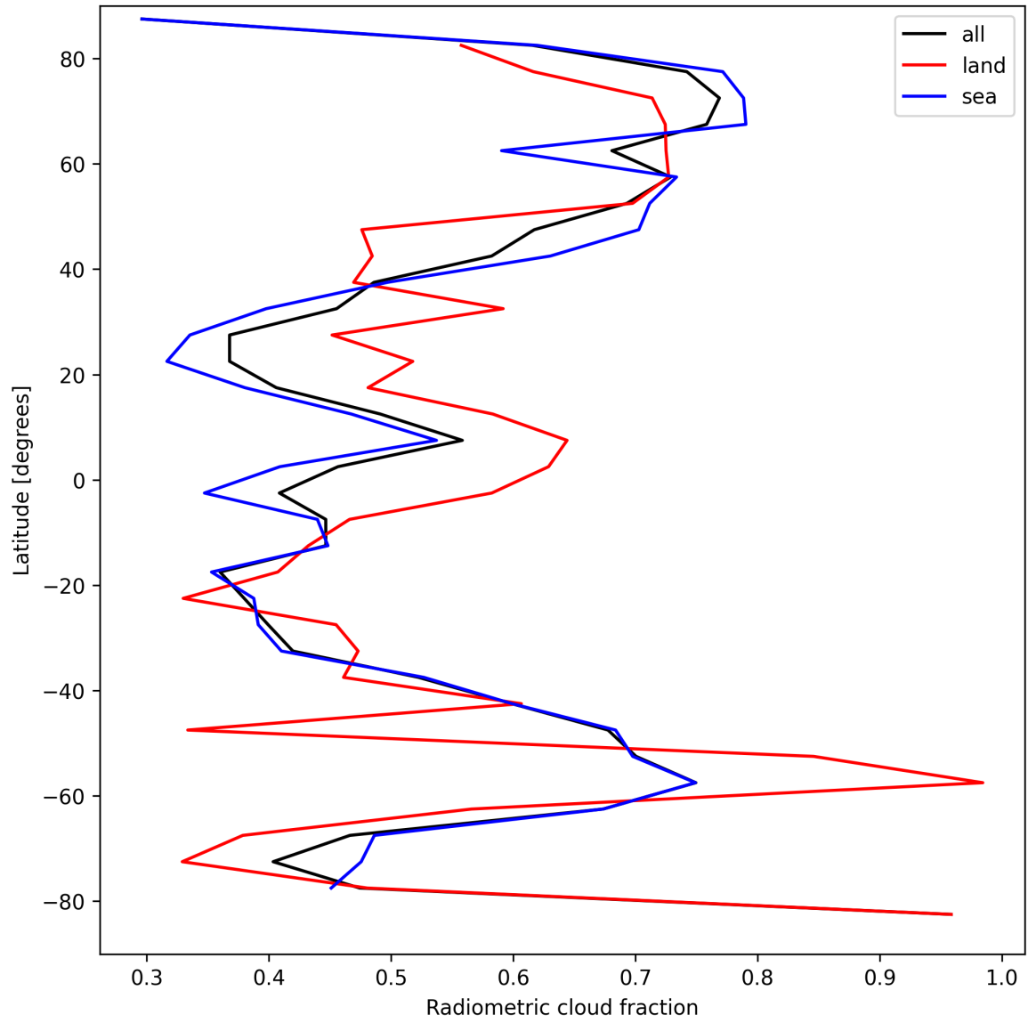
Figure 23: Zonal average of “Radiometric cloud fraction” for 2025-09-02 to 2025-09-04.
