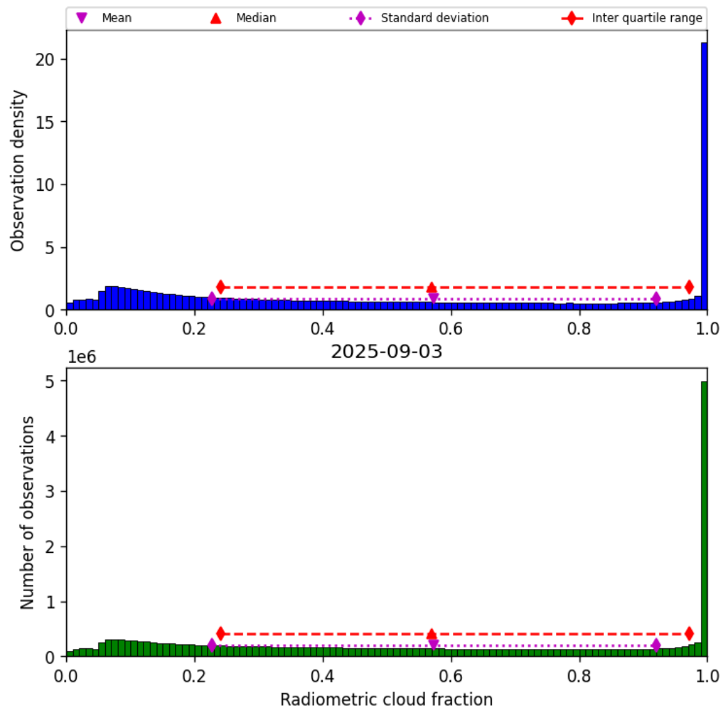
Figure 39: Histogram of “Radiometric cloud fraction” for 2025-09-02 to 2025-09-04
