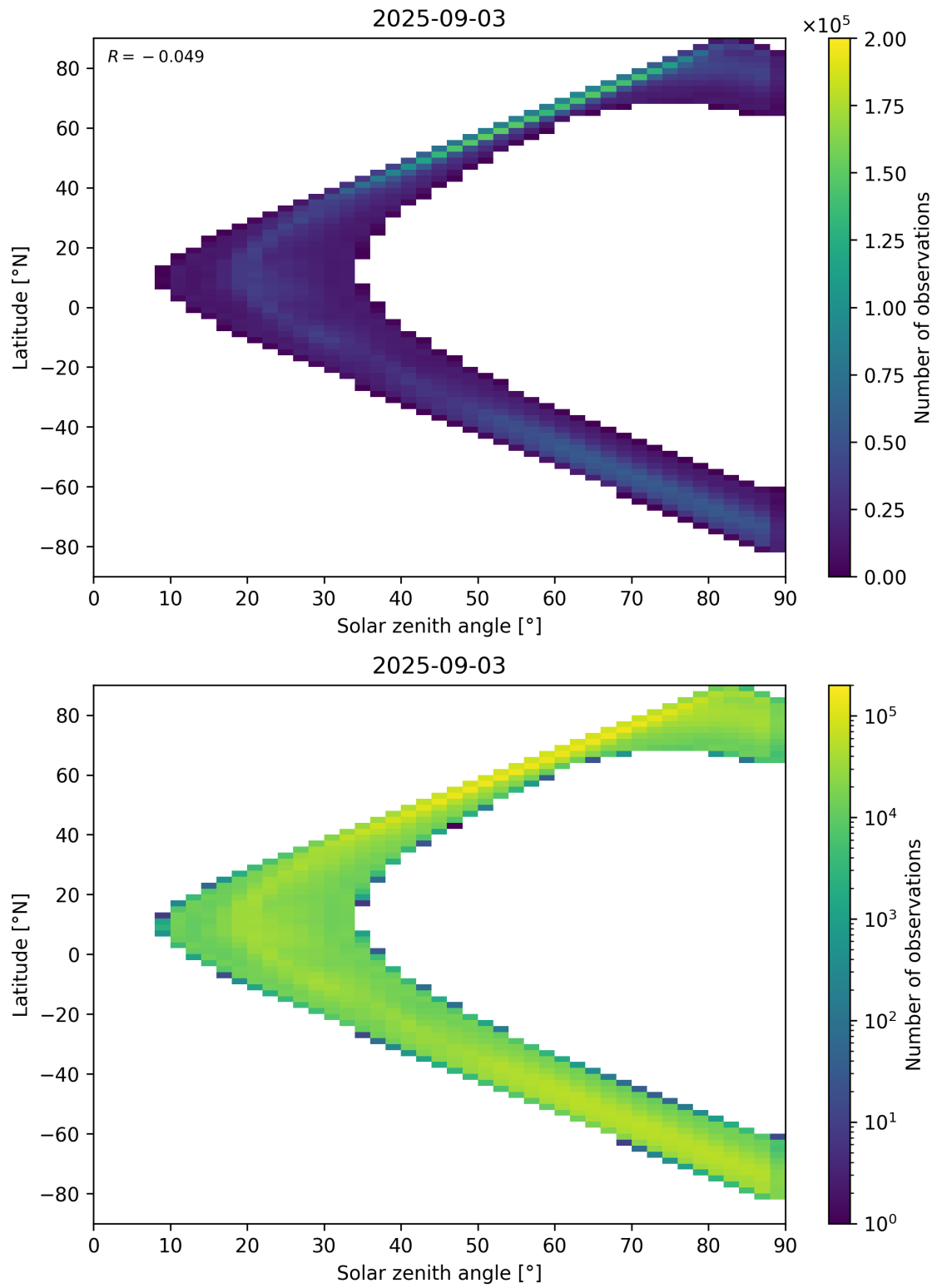
Figure 105: Scatter density plot of “Solar zenith angle” against “Latitude” for 2025-09-02 to 2025-09-04.
