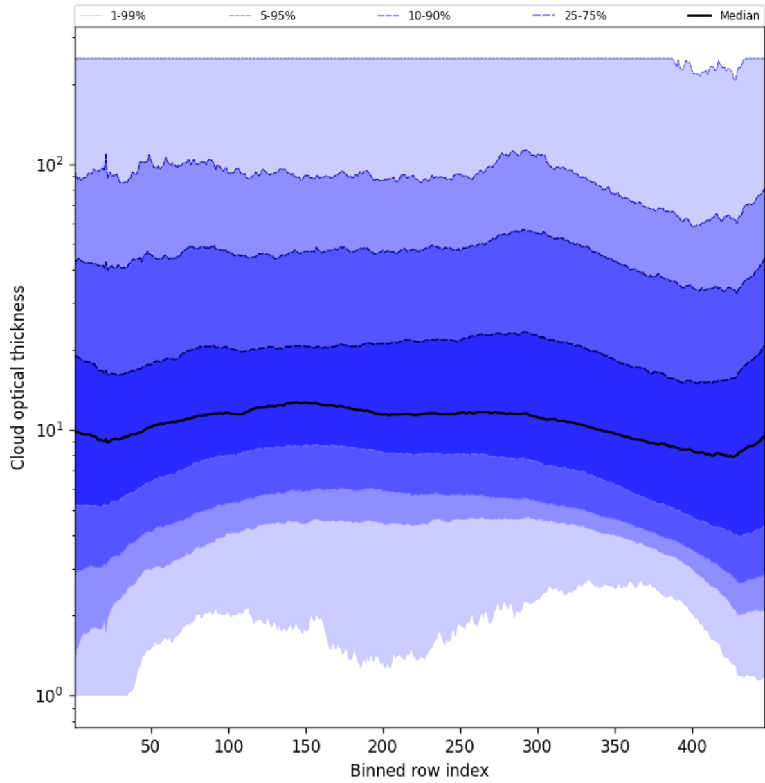
Figure 57: Along track statistics of “Cloud optical thickness” for 2025-09-02 to 2025-09-04
