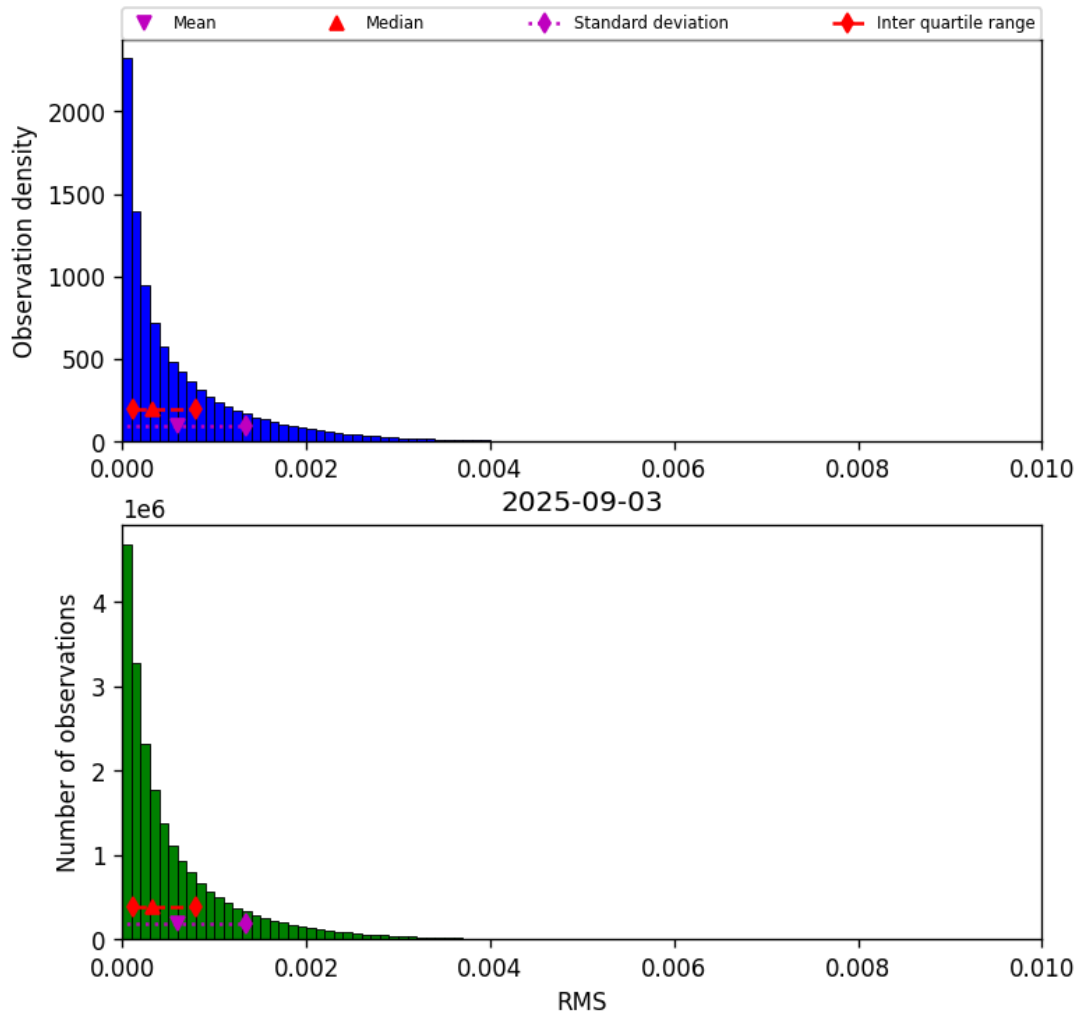
Figure 47: Histogram of “RMS” for 2025-09-02 to 2025-09-04
