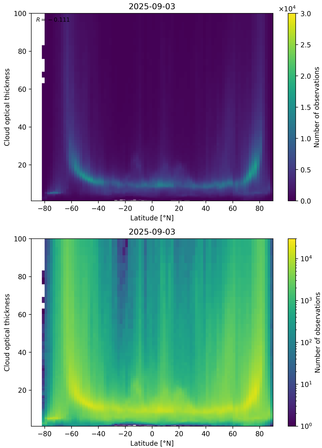
Figure 96: Scatter density plot of “Latitude” against “Cloud optical thickness” for 2025-09-02 to 2025-09-04.
