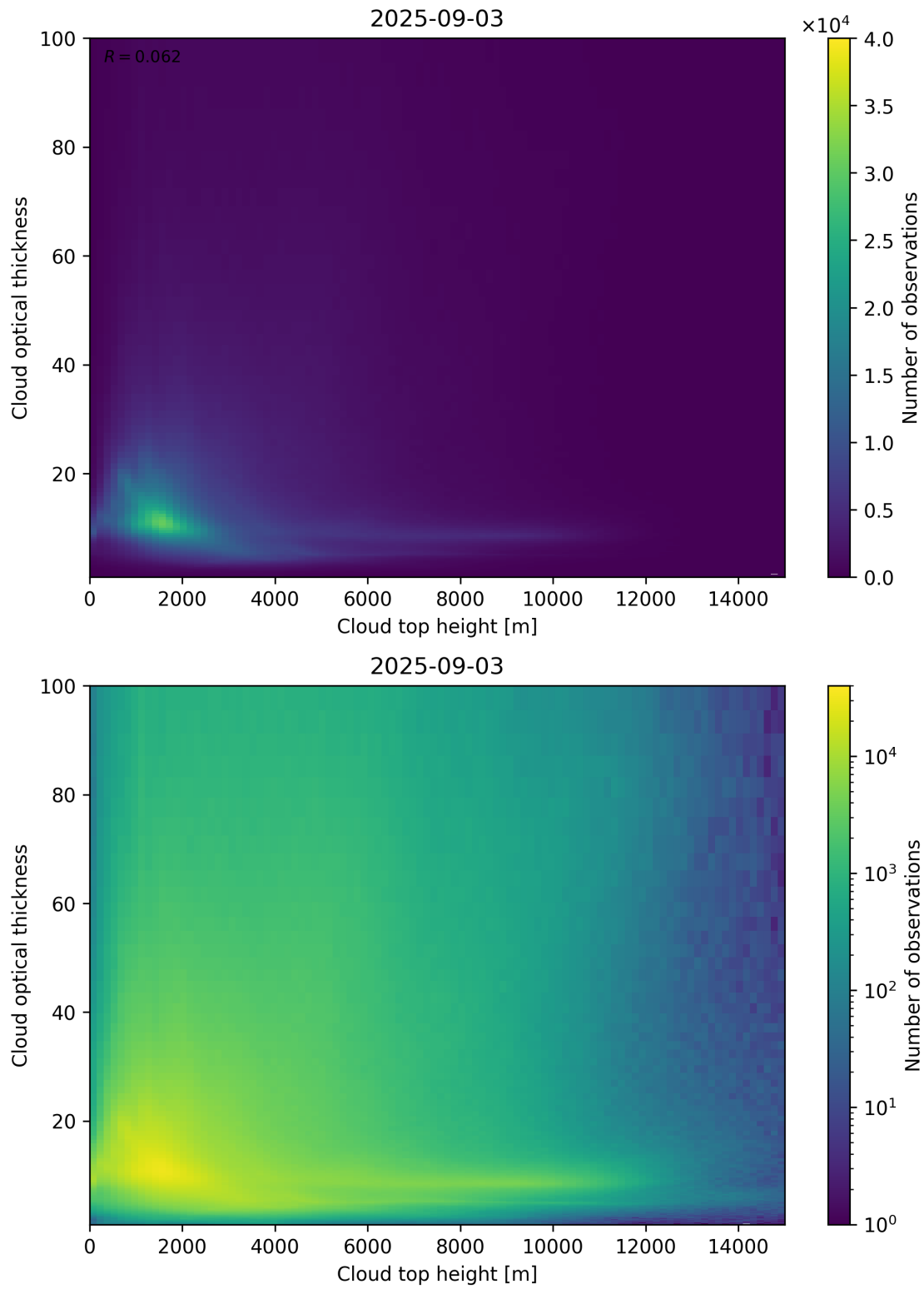
Figure 90: Scatter density plot of “Cloud top height” against “Cloud optical thickness” for 2025-09-02 to 2025-09-04.
