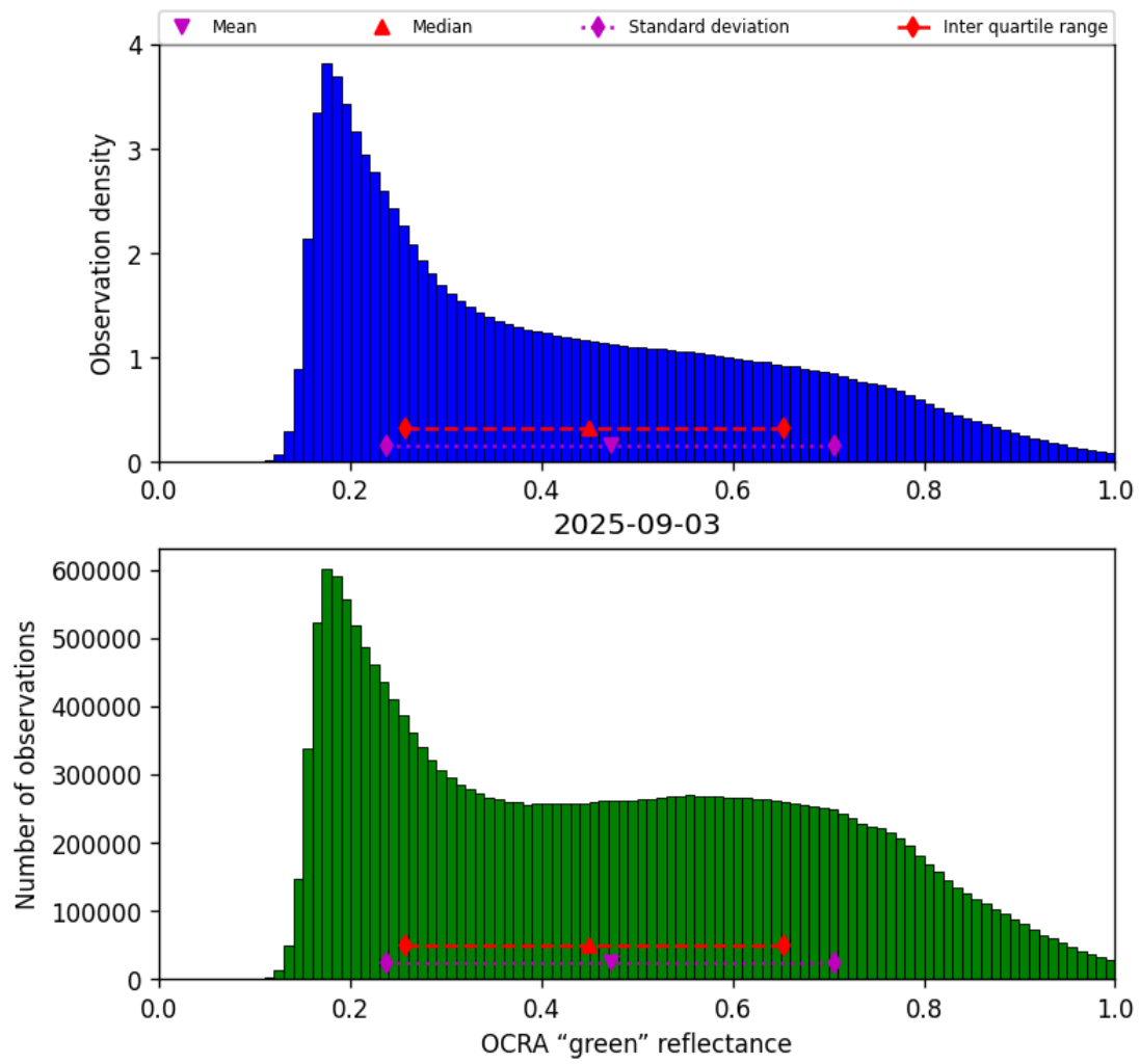
Figure 52: Histogram of “OCRA “green” reflectance” for 2025-09-02 to 2025-09-04
