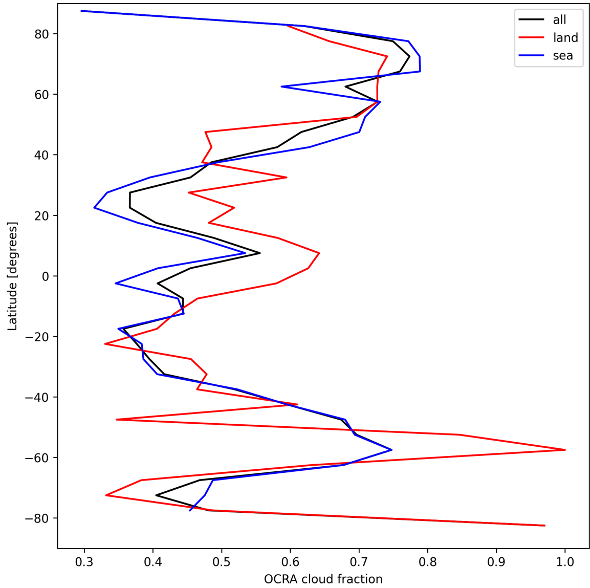
Figure 34: Zonal average of “OCRA cloud fraction” for 2025-09-02 to 2025-09-04.
