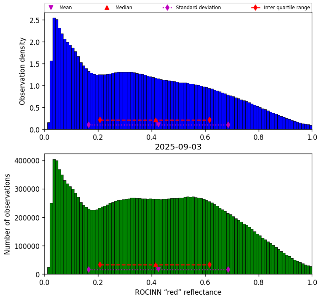
Figure 53: Histogram of "ROCINN "red" reflectance" for 2025-09-02 to 2025-09-04
