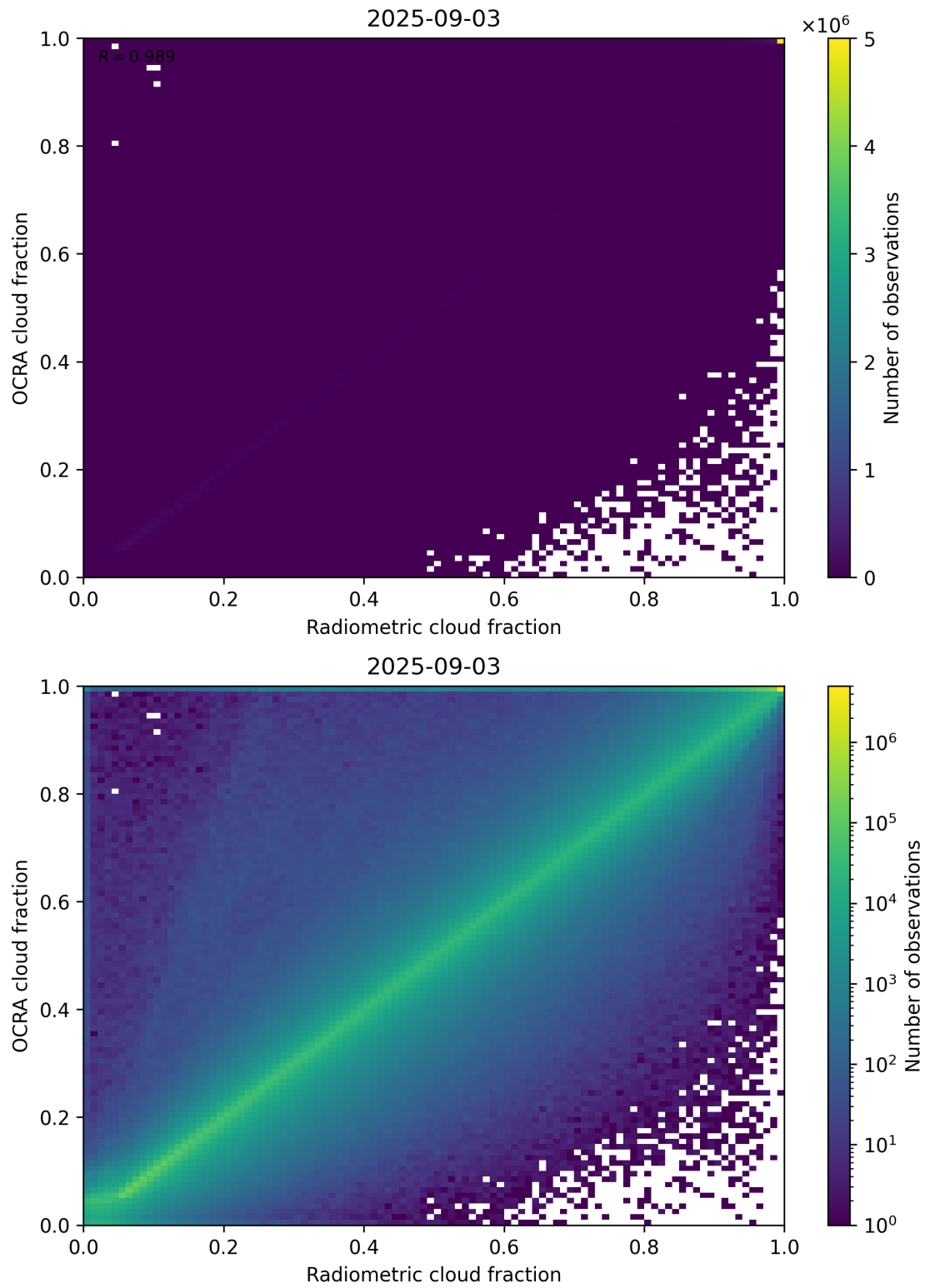
Figure 72: Scatter density plot of “Radiometric cloud fraction” against “OCRA cloud fraction” for 2025-09-02 to 2025-09-04.
