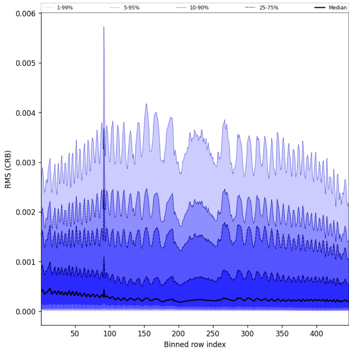
Figure 64: Along track statistics of “RMS (CRB)” for 2025-09-02 to 2025-09-04
