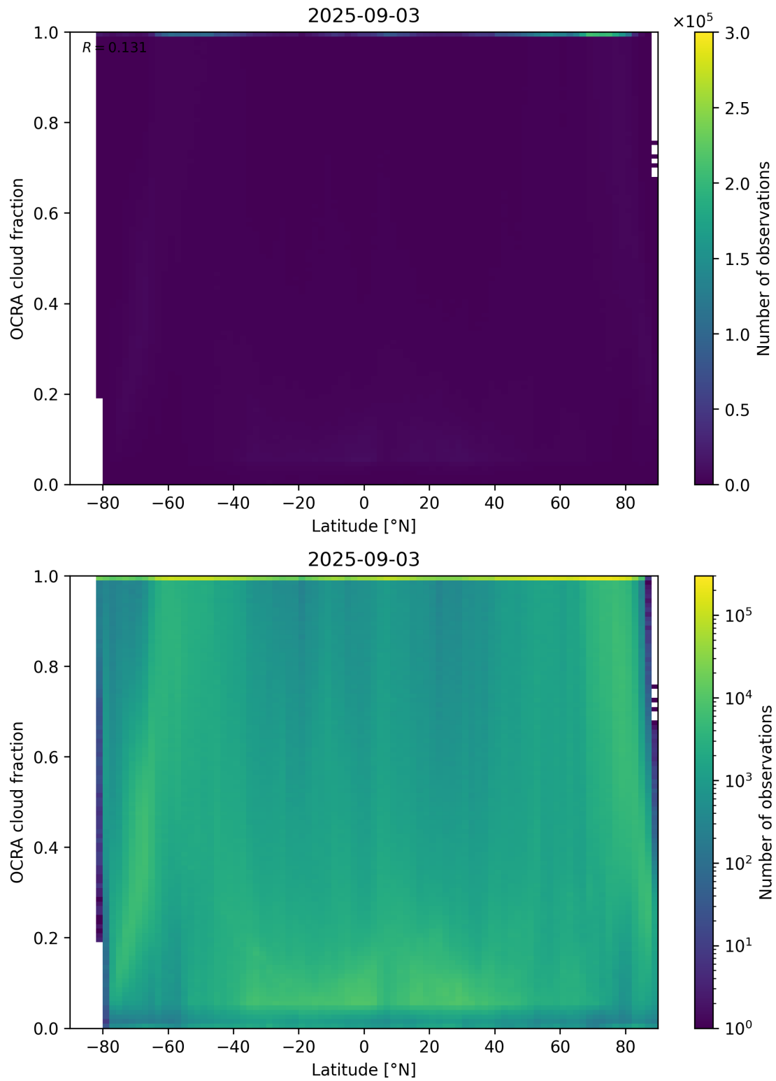
Figure 93: Scatter density plot of “Latitude” against “OCRA cloud fraction” for 2025-09-02 to 2025-09-04.
