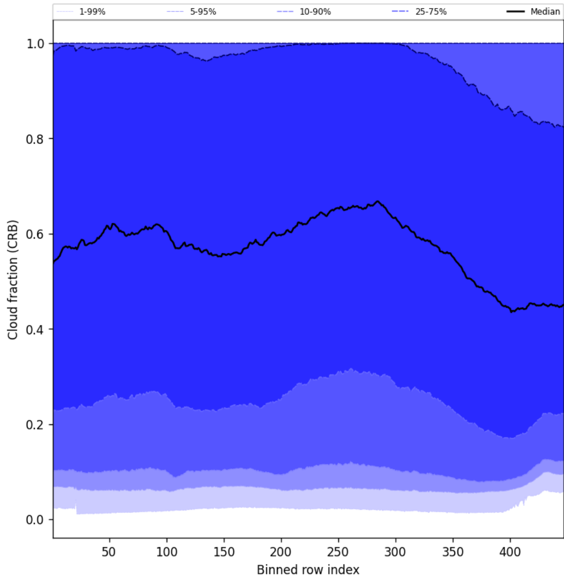
Figure 58: Along track statistics of “Cloud fraction (CRB)” for 2025-09-02 to 2025-09-04
