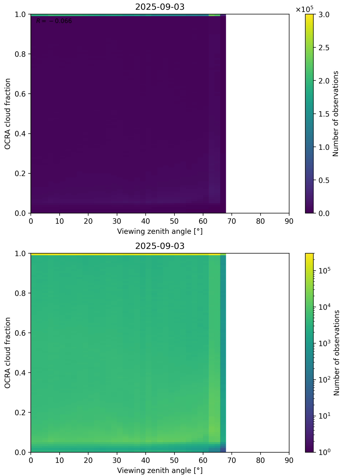
Figure 108: Scatter density plot of “Viewing zenith angle” against “OCRA cloud fraction” for 2025-09-02 to 2025-09-04.
