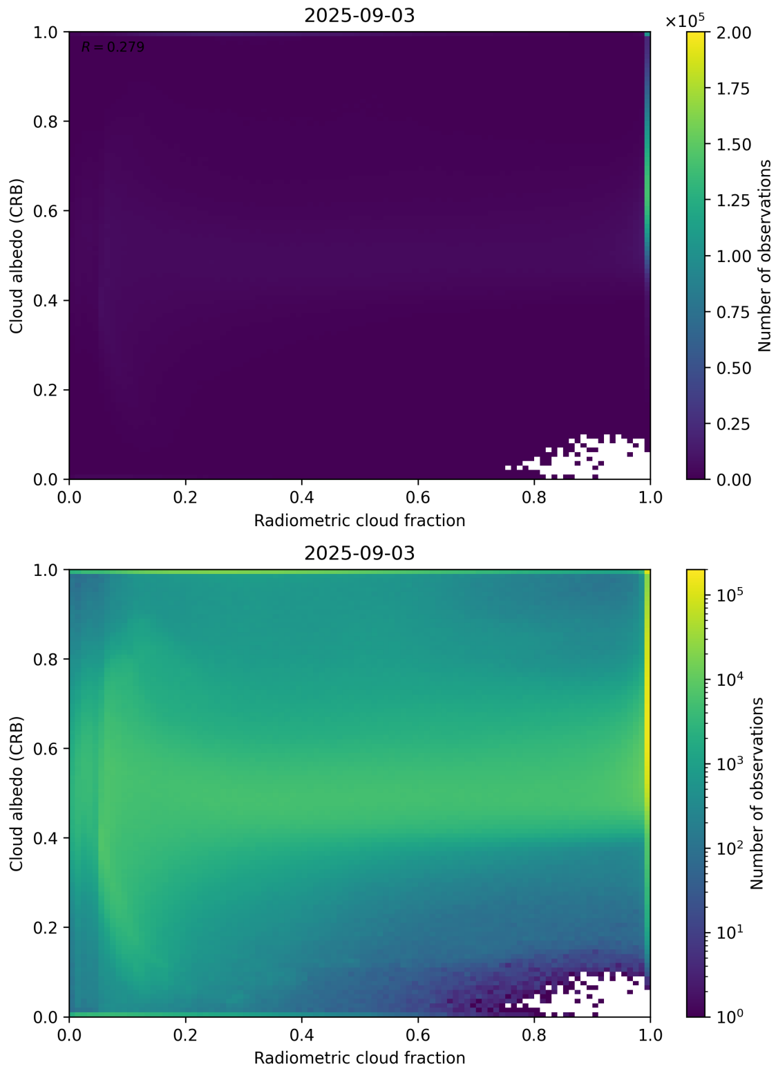
Figure 71: Scatter density plot of “Radiometric cloud fraction” against “Cloud albedo (CRB)” for 2025-09-02 to 2025-09-04.
