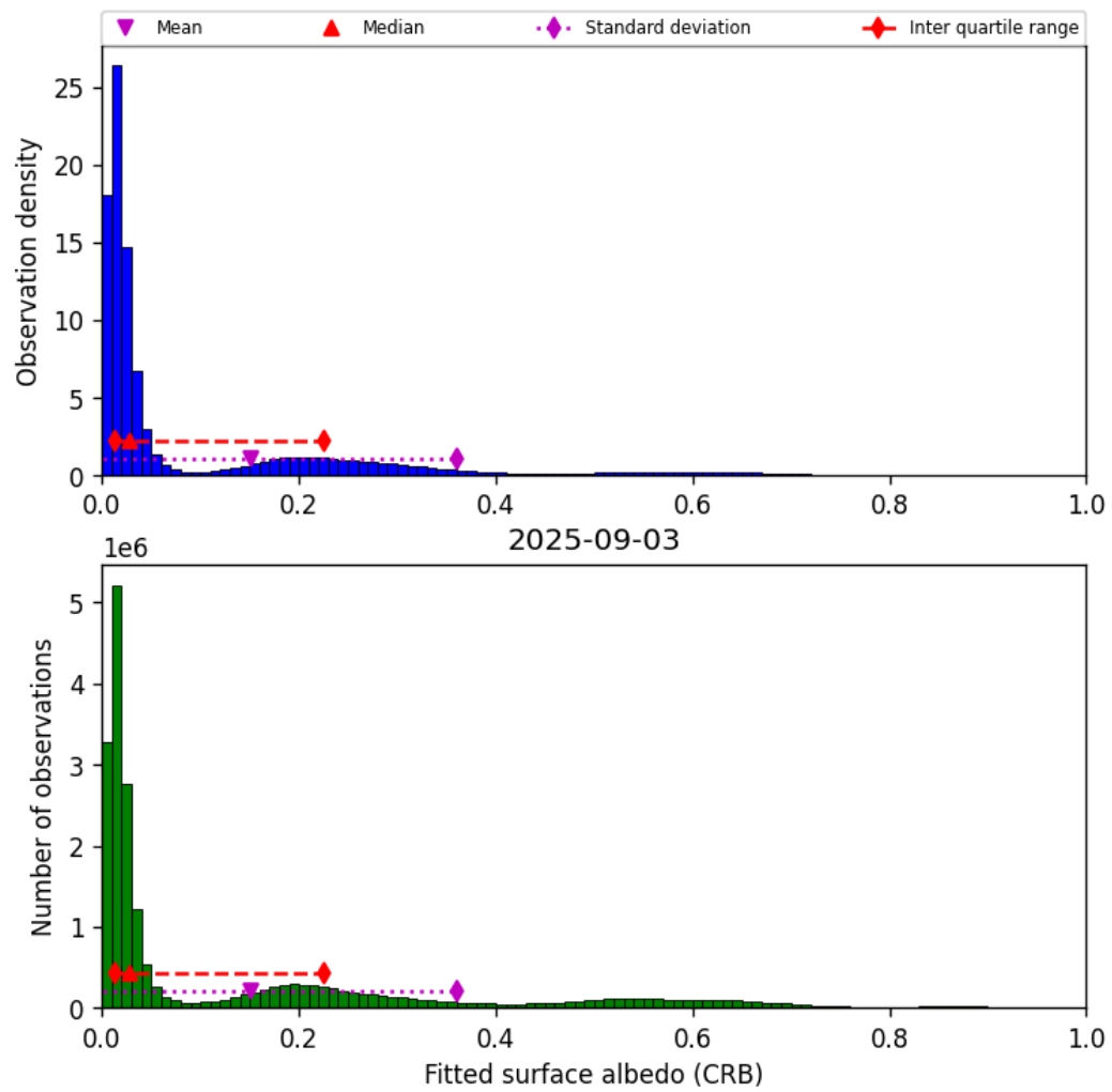
Figure 46: Histogram of “Fitted surface albedo (CRB)” for 2025-09-02 to 2025-09-04
