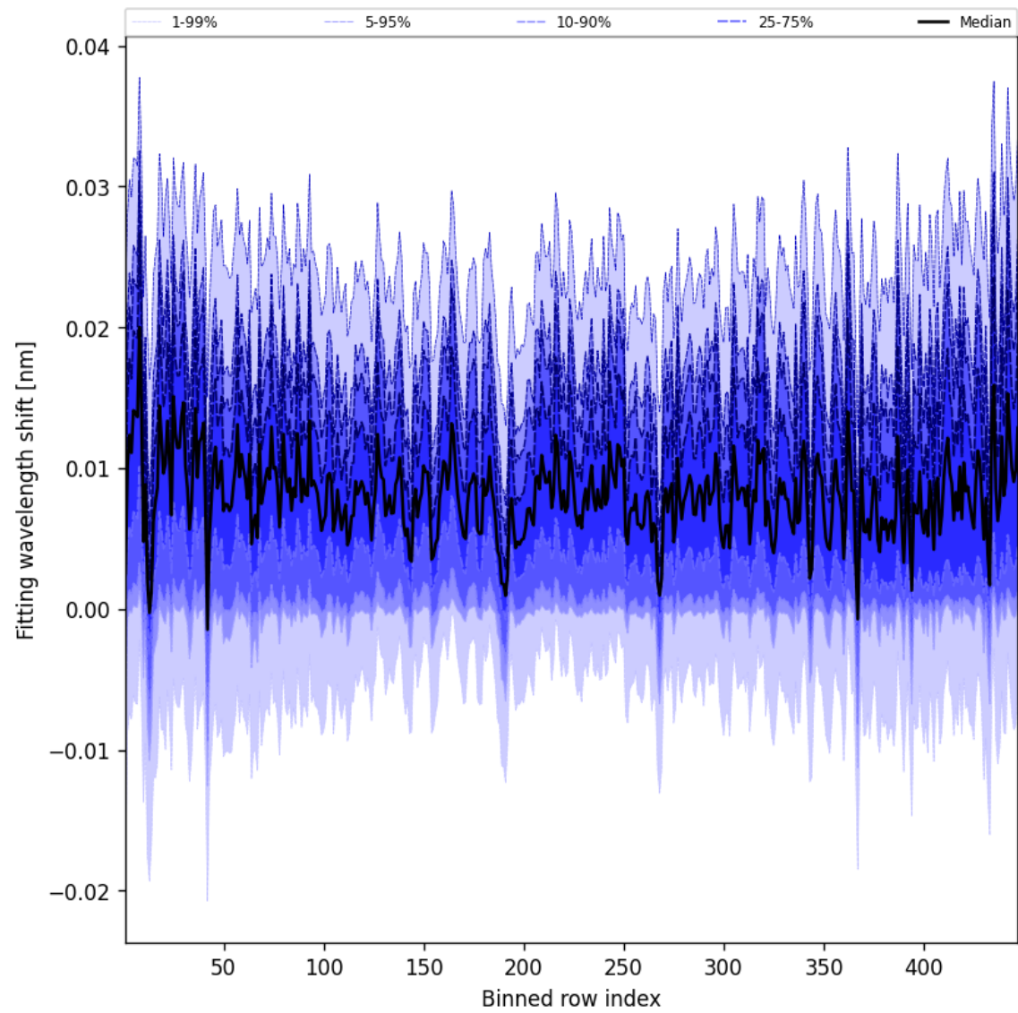
Figure 65: Along track statistics of “Fitting wavelength shift” for 2025-09-02 to 2025-09-04
