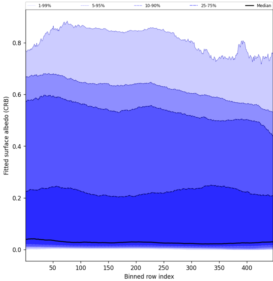
Figure 62: Along track statistics of “Fitted surface albedo (CRB)” for 2025-09-02 to 2025-09-04
