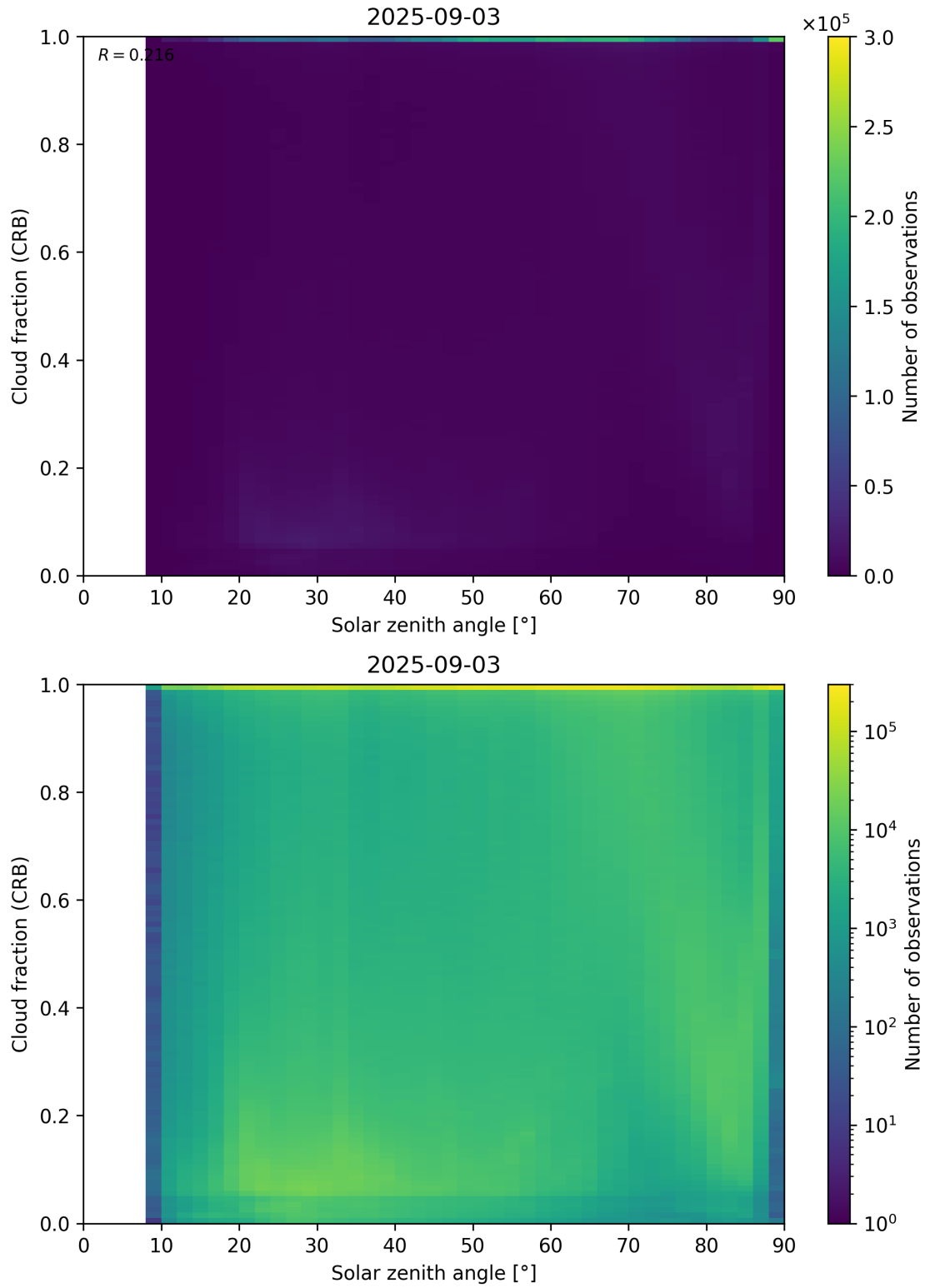
Figure 101: Scatter density plot of “Solar zenith angle” against “Cloud fraction (CRB)” for 2025-09-02 to 2025-09-04.
