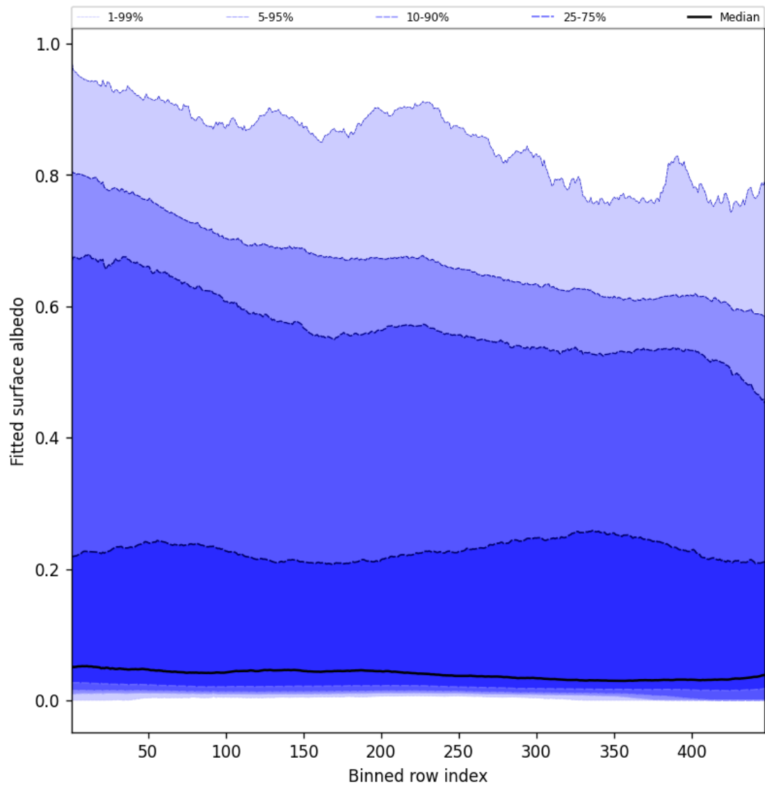
Figure 61: Along track statistics of “Fitted surface albedo” for 2025-09-02 to 2025-09-04
