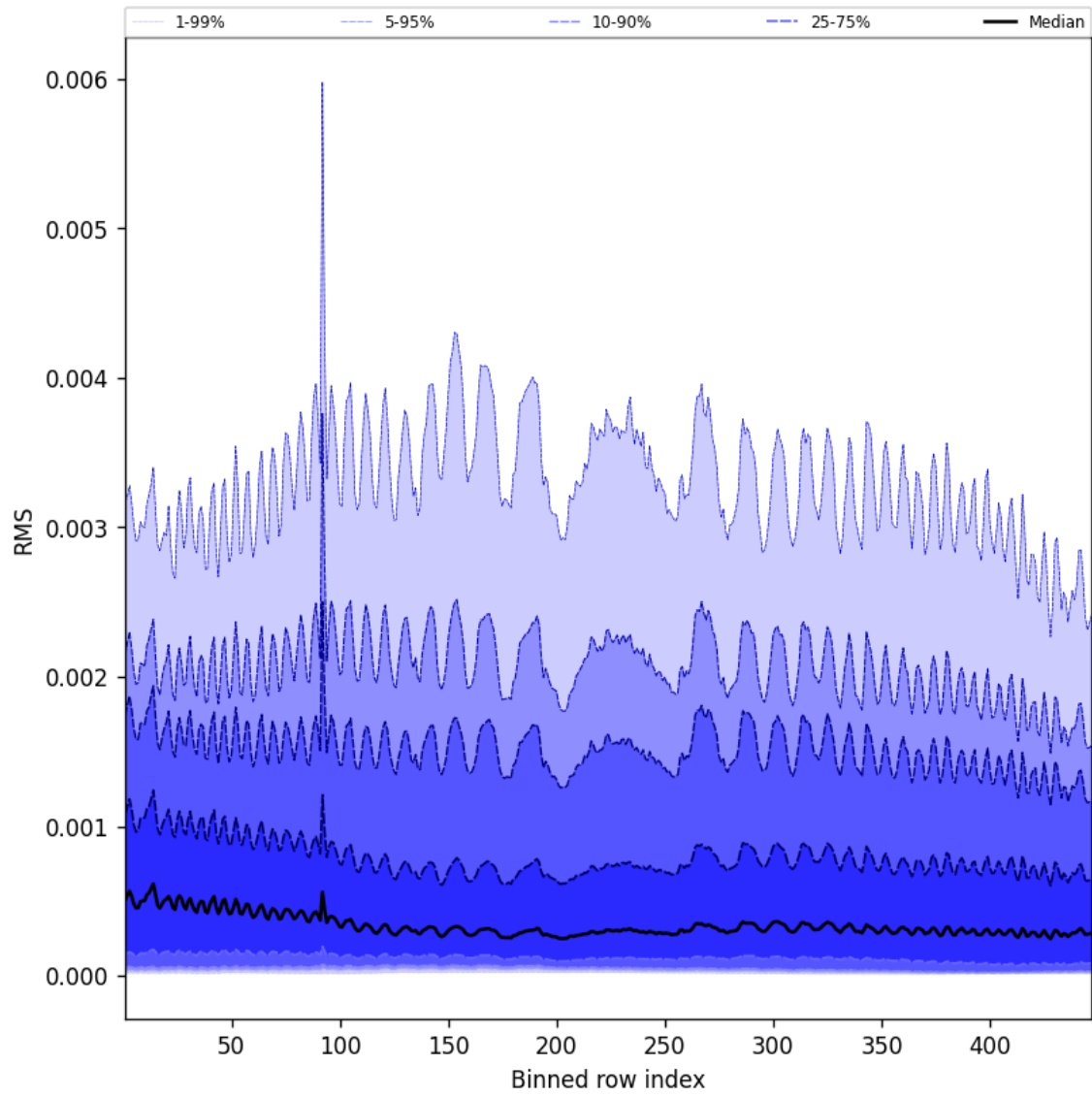
Figure 63: Along track statistics of “RMS” for 2025-09-02 to 2025-09-04
