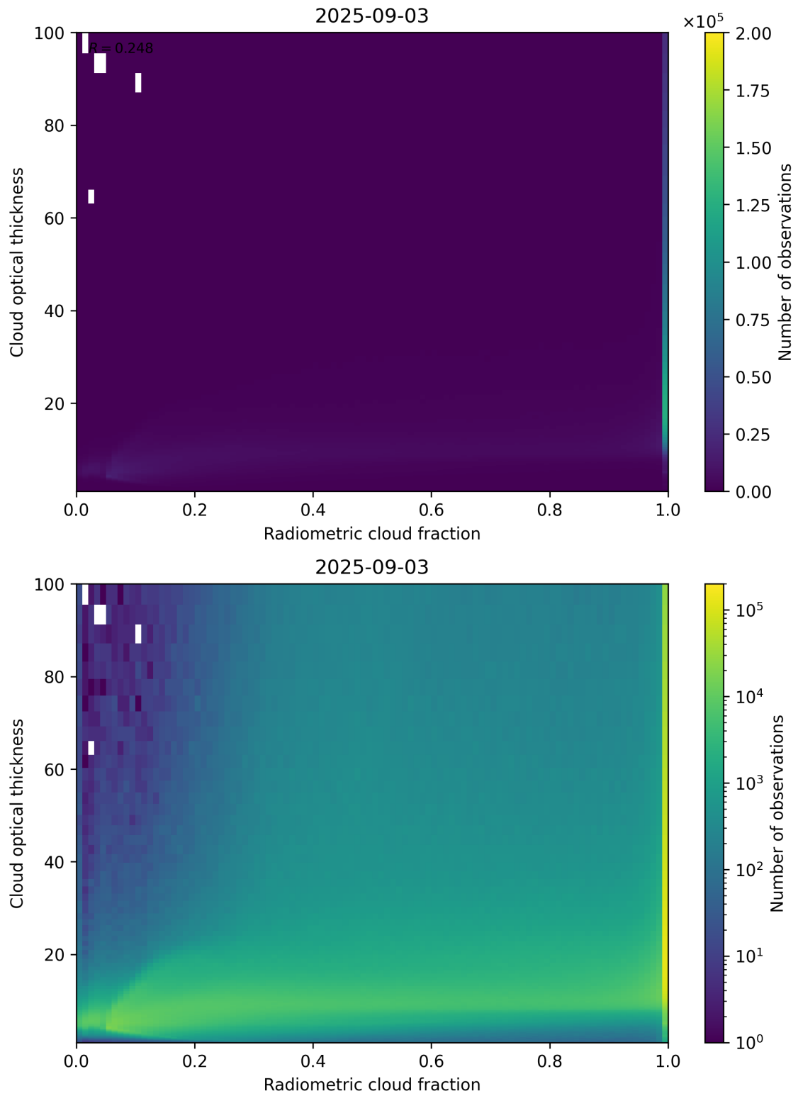
Figure 75: Scatter density plot of “Radiometric cloud fraction” against “Cloud optical thickness” for 2025-09-02 to 2025-09-04.
