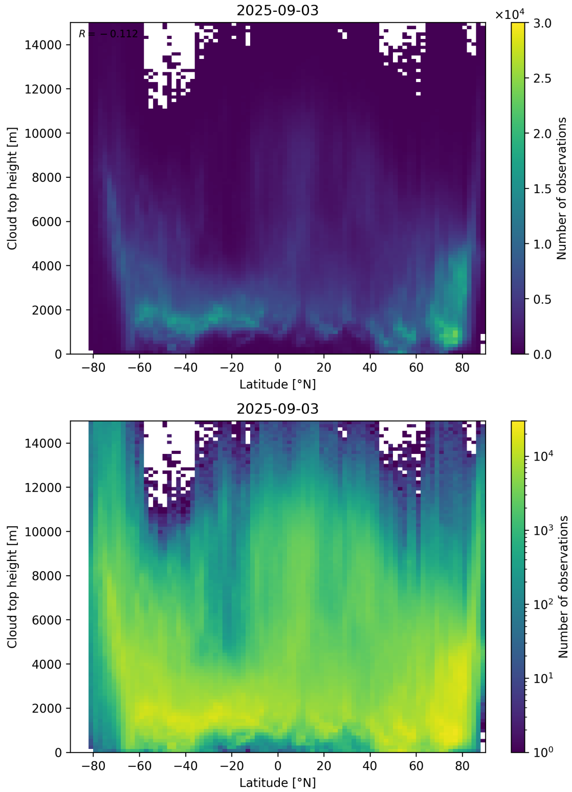
Figure 97: Scatter density plot of “Latitude” against “Cloud top height” for 2025-09-02 to 2025-09-04.
