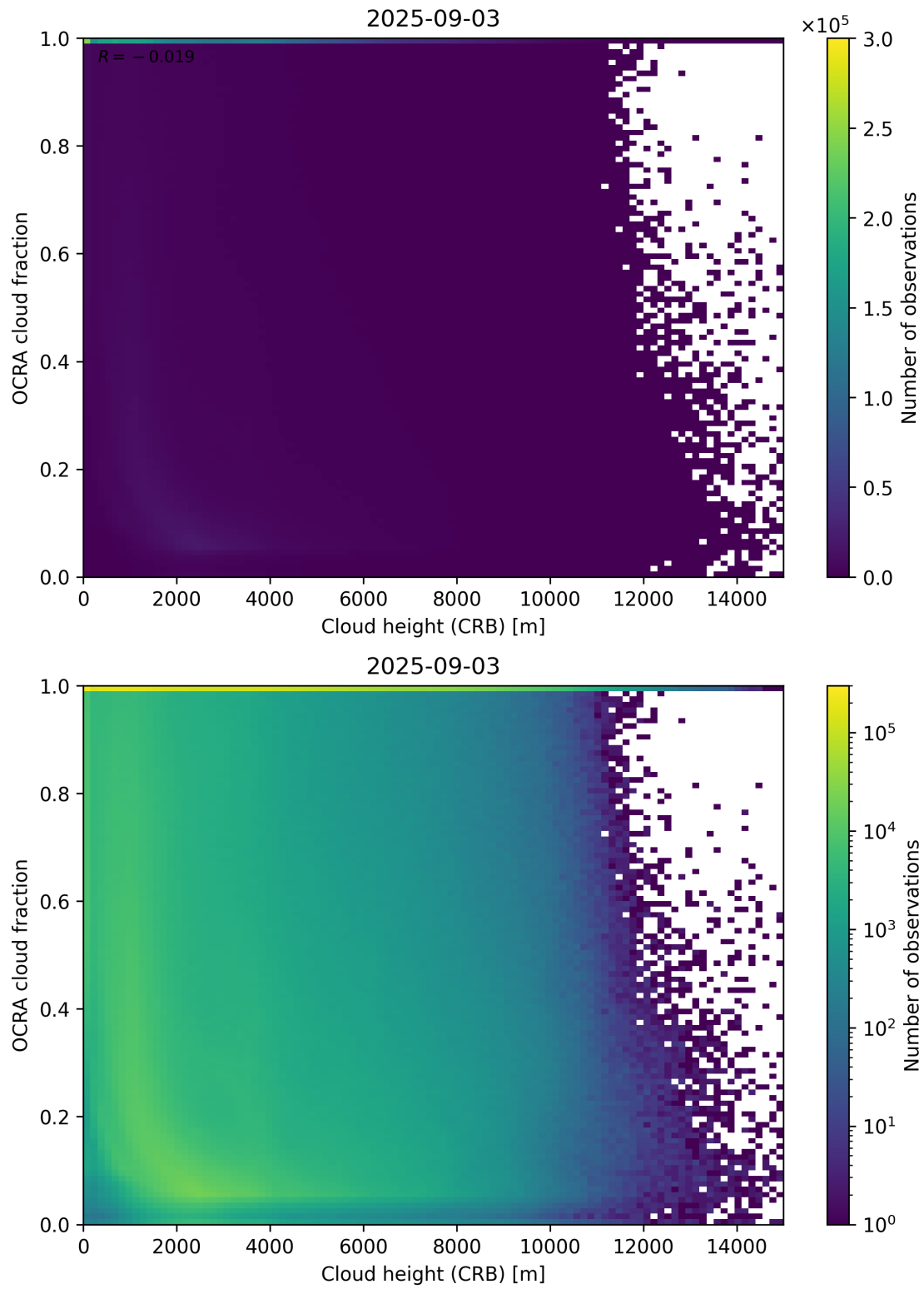
Figure 81: Scatter density plot of “Cloud height (CRB)” against “OCRA cloud fraction” for 2025-09-02 to 2025-09-04.
