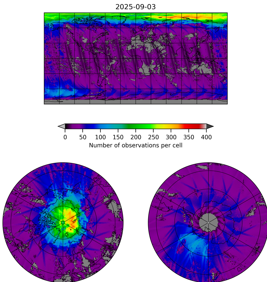
Figure 21: Map of the number of observations for 2025-09-02 to 2025-09-04
