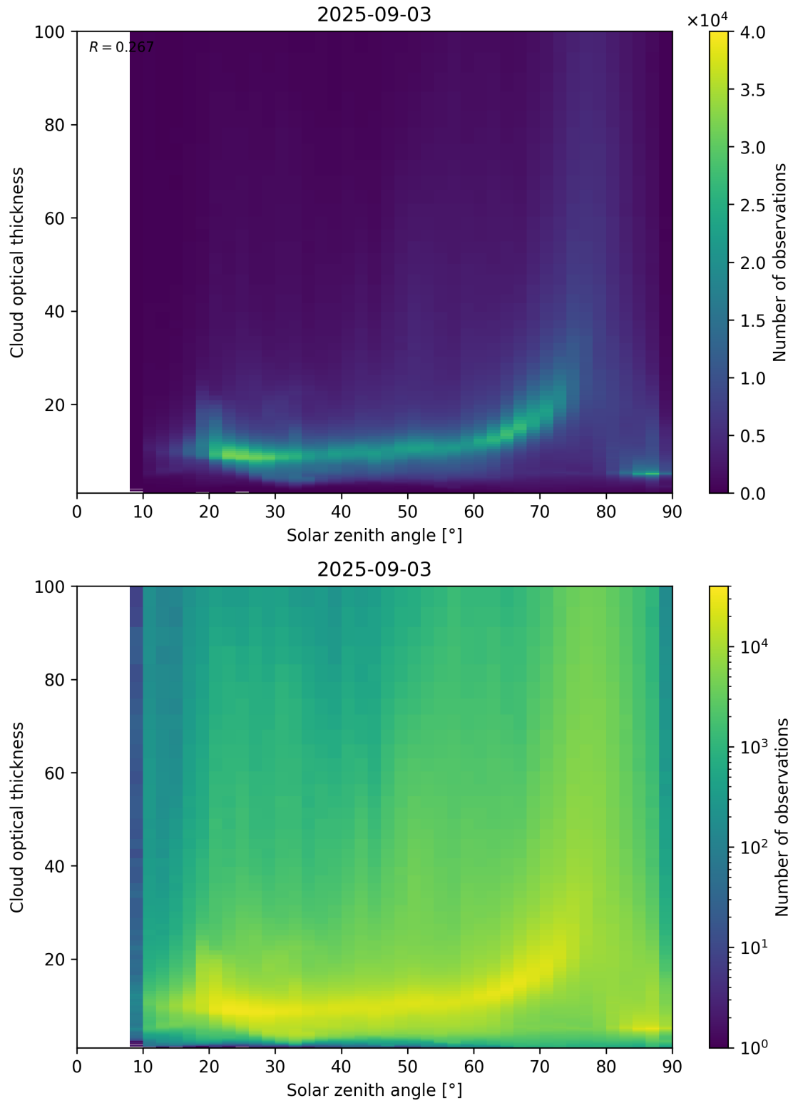
Figure 103: Scatter density plot of “Solar zenith angle” against “Cloud optical thickness” for 2025-09-02 to 2025-09-04.
