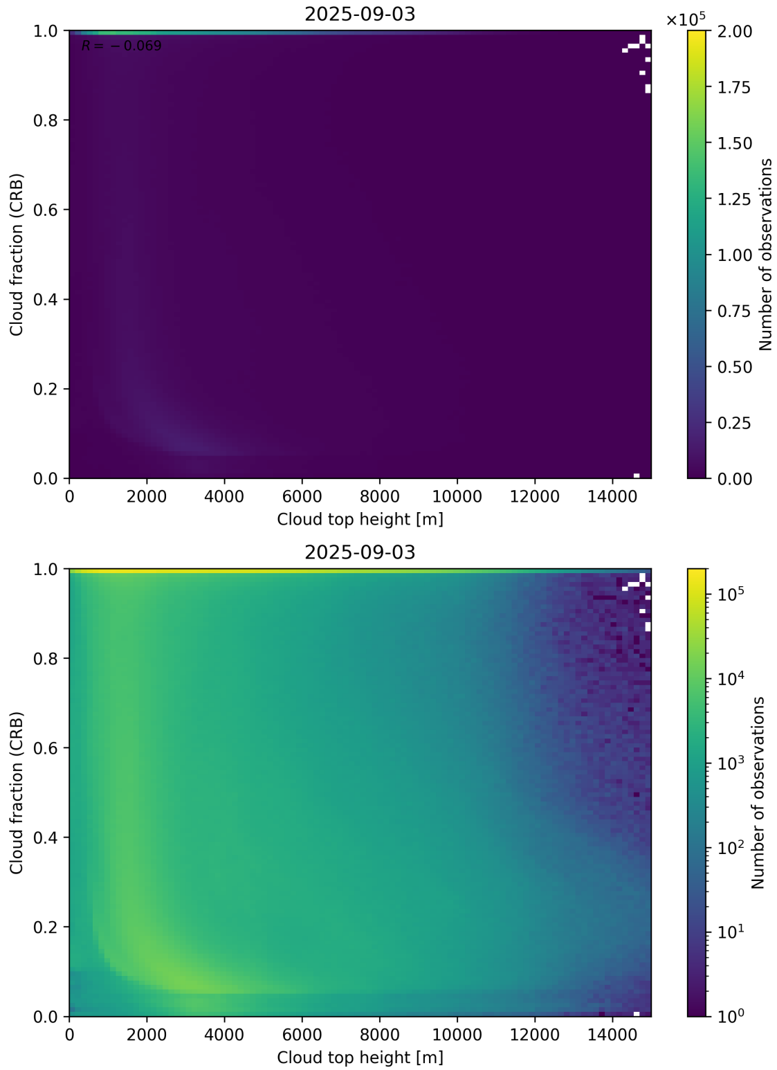
Figure 88: Scatter density plot of “Cloud top height” against “Cloud fraction (CRB)” for 2025-09-02 to 2025-09-04.
