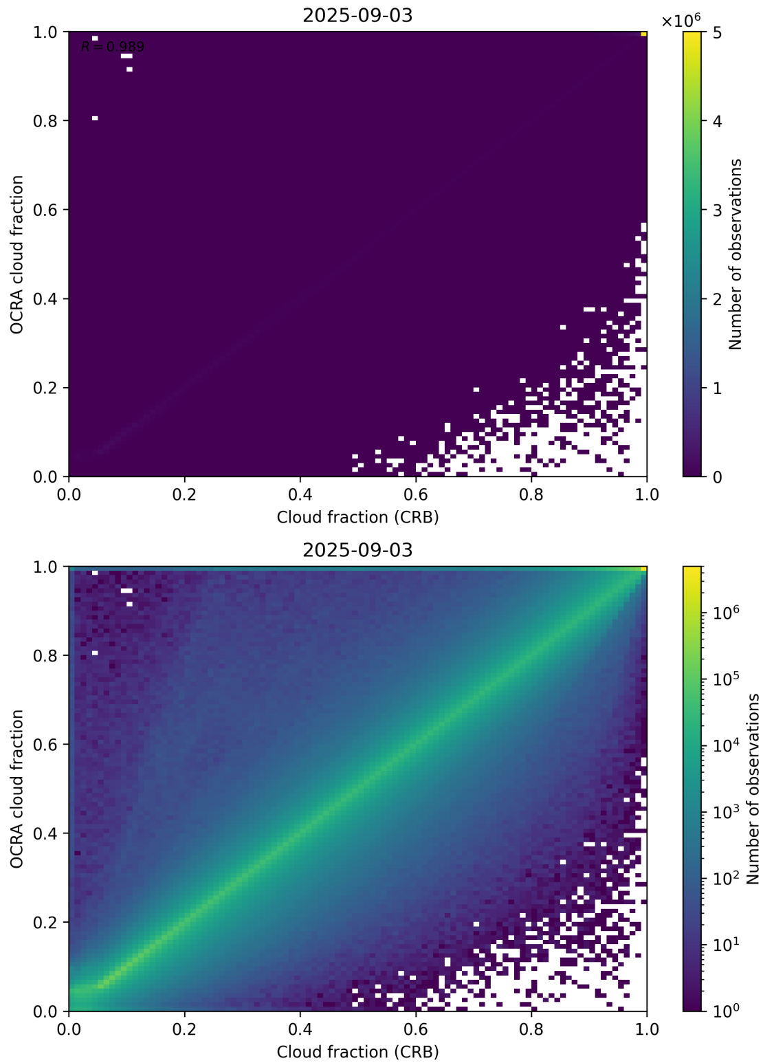
Figure 78: Scatter density plot of “Cloud fraction (CRB)” against “OCRA cloud fraction” for 2025-09-02 to 2025-09-04.
