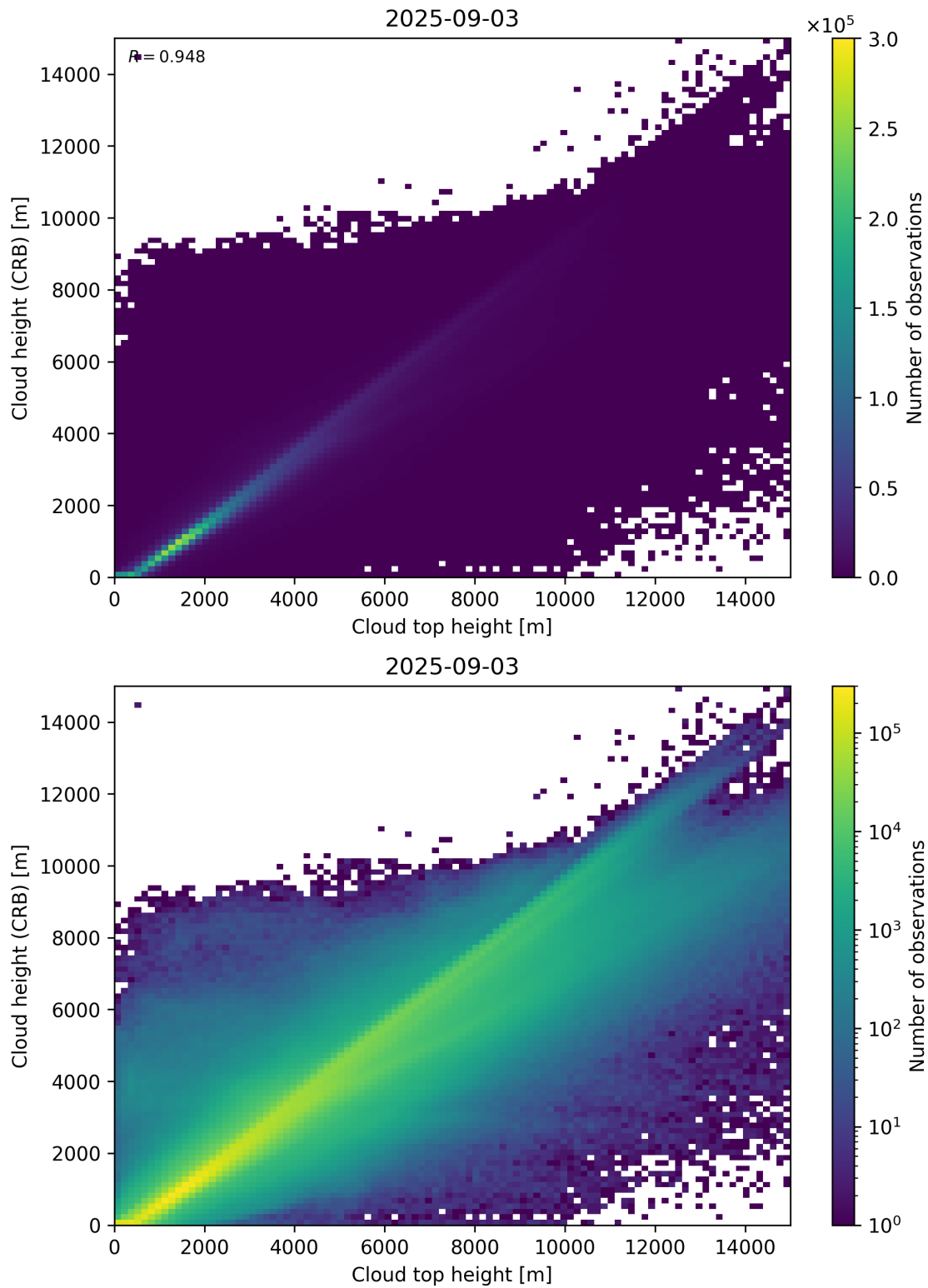
Figure 89: Scatter density plot of “Cloud top height” against “Cloud height (CRB)” for 2025-09-02 to 2025-09-04.
