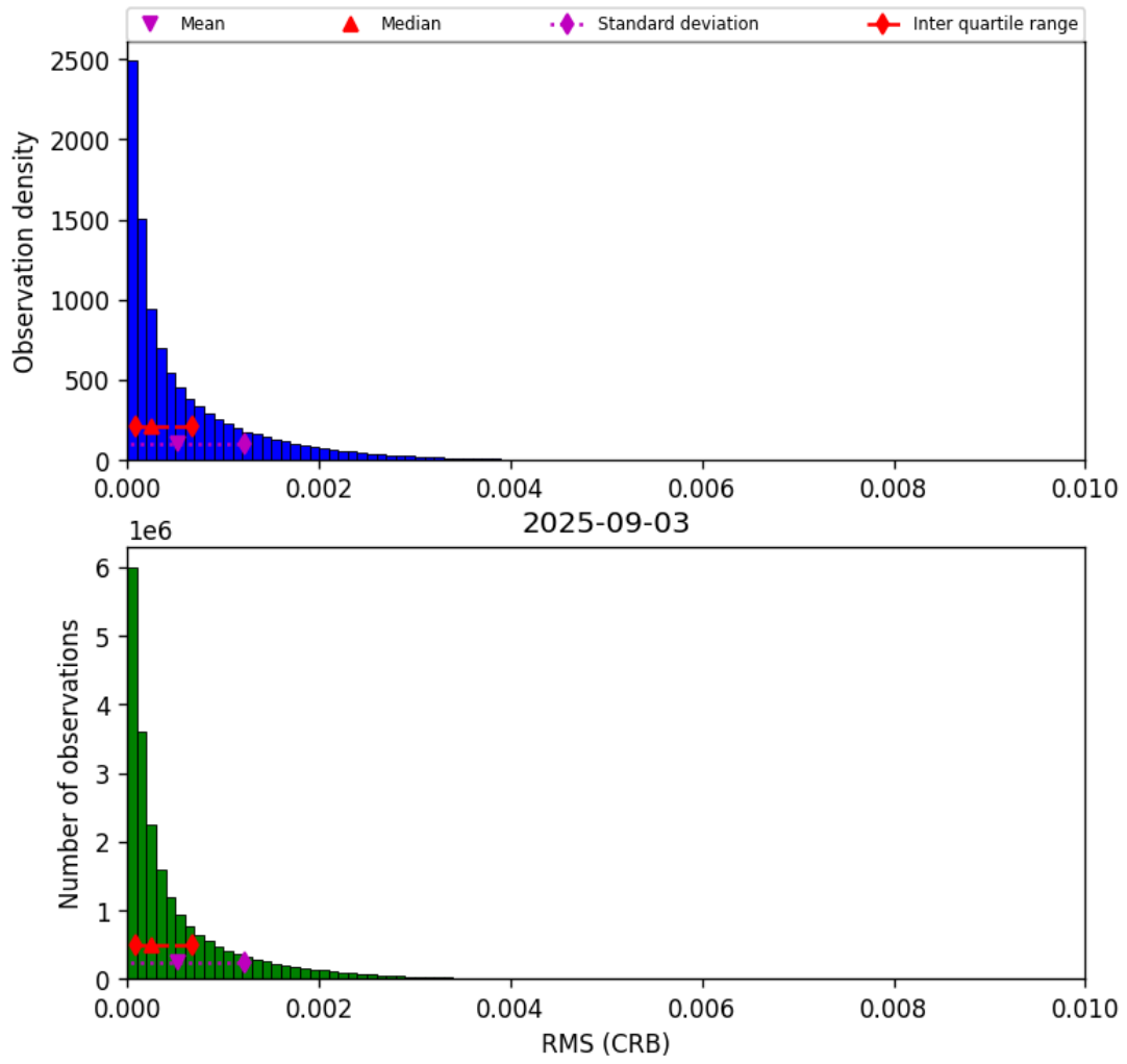
Figure 48: Histogram of “RMS (CRB)” for 2025-09-02 to 2025-09-04
