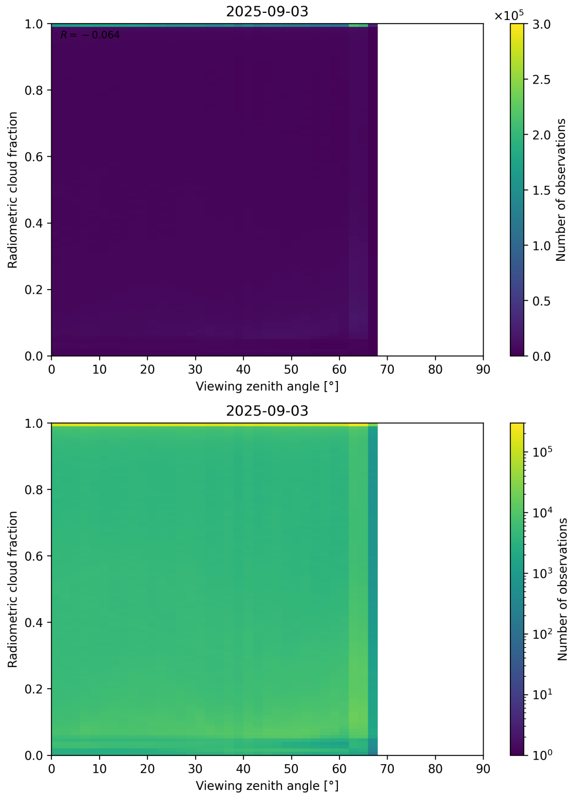
Figure 107: Scatter density plot of “Viewing zenith angle” against “Radiometric cloud fraction” for 2025-09-02 to 2025-09-04.
