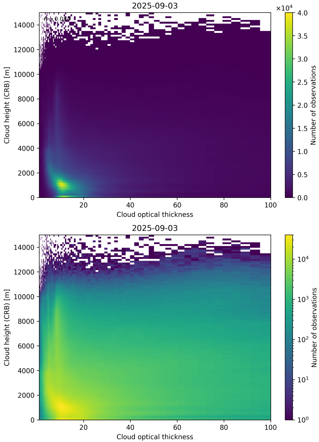
Figure 85: Scatter density plot of “Cloud optical thickness” against “Cloud height (CRB)” for 2025-09-02 to 2025-09-04.
