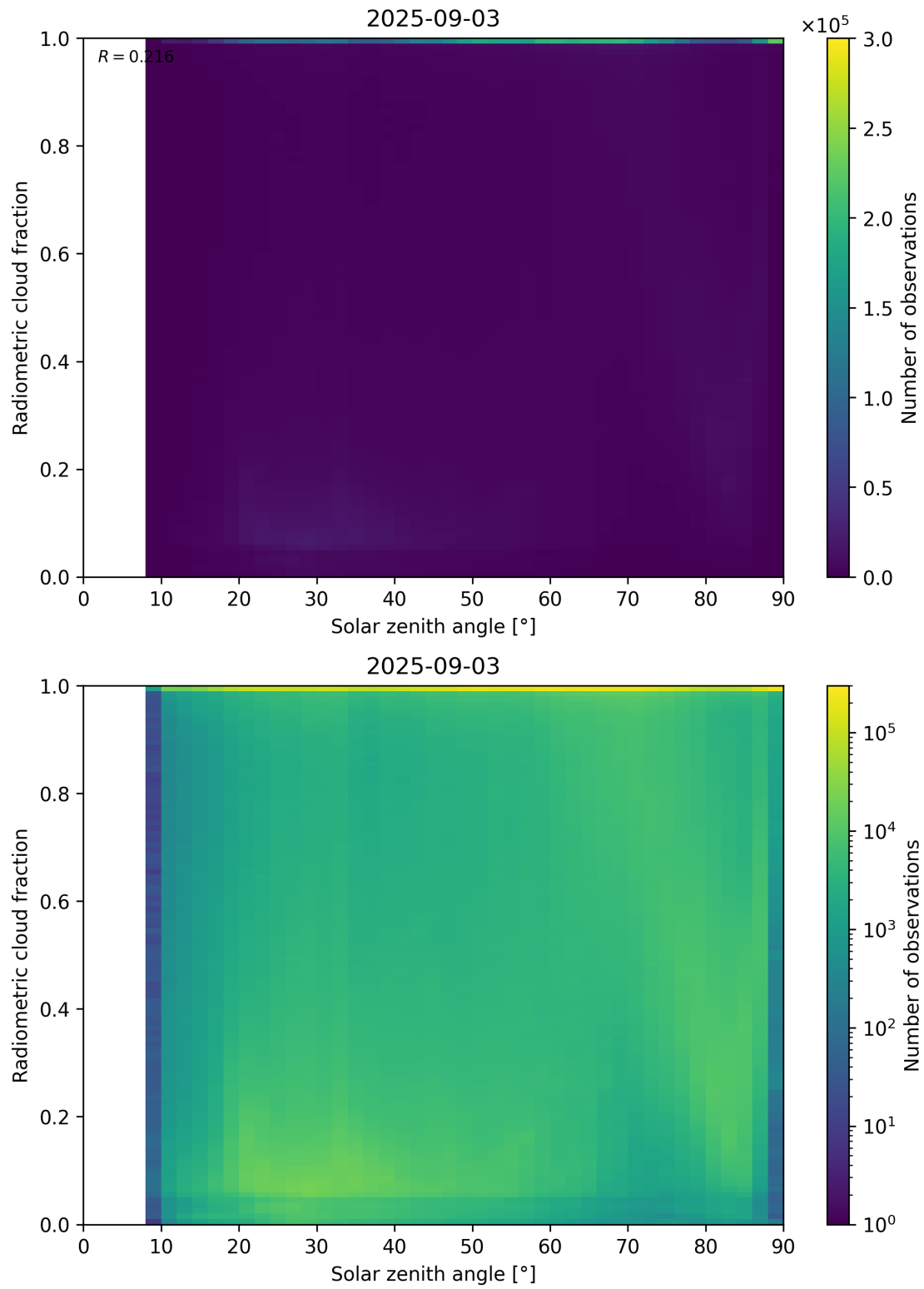
Figure 99: Scatter density plot of “Solar zenith angle” against “Radiometric cloud fraction” for 2025-09-02 to 2025-09-04.
