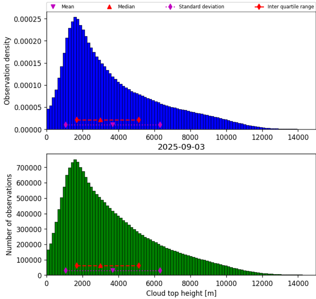
Figure 40: Histogram of “Cloud top height” for 2025-09-02 to 2025-09-04
