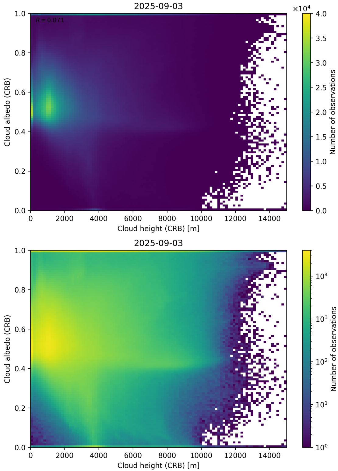
Figure 80: Scatter density plot of “Cloud height (CRB)” against “Cloud albedo (CRB)” for 2025-09-02 to 2025-09-04.
