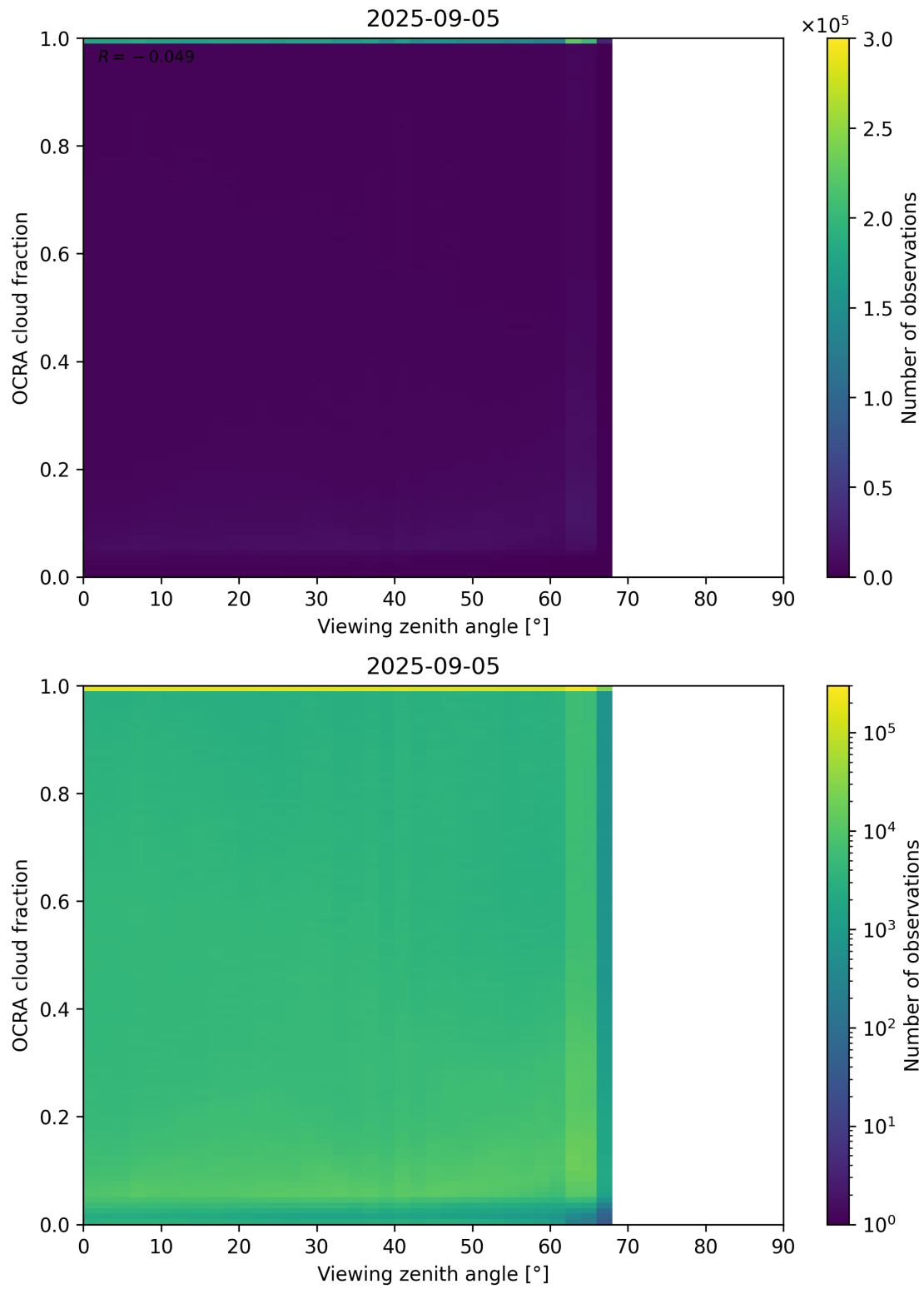
Figure 108: Scatter density plot of “Viewing zenith angle” against “OCRA cloud fraction” for 2025-09-04 to 2025-09-06.
