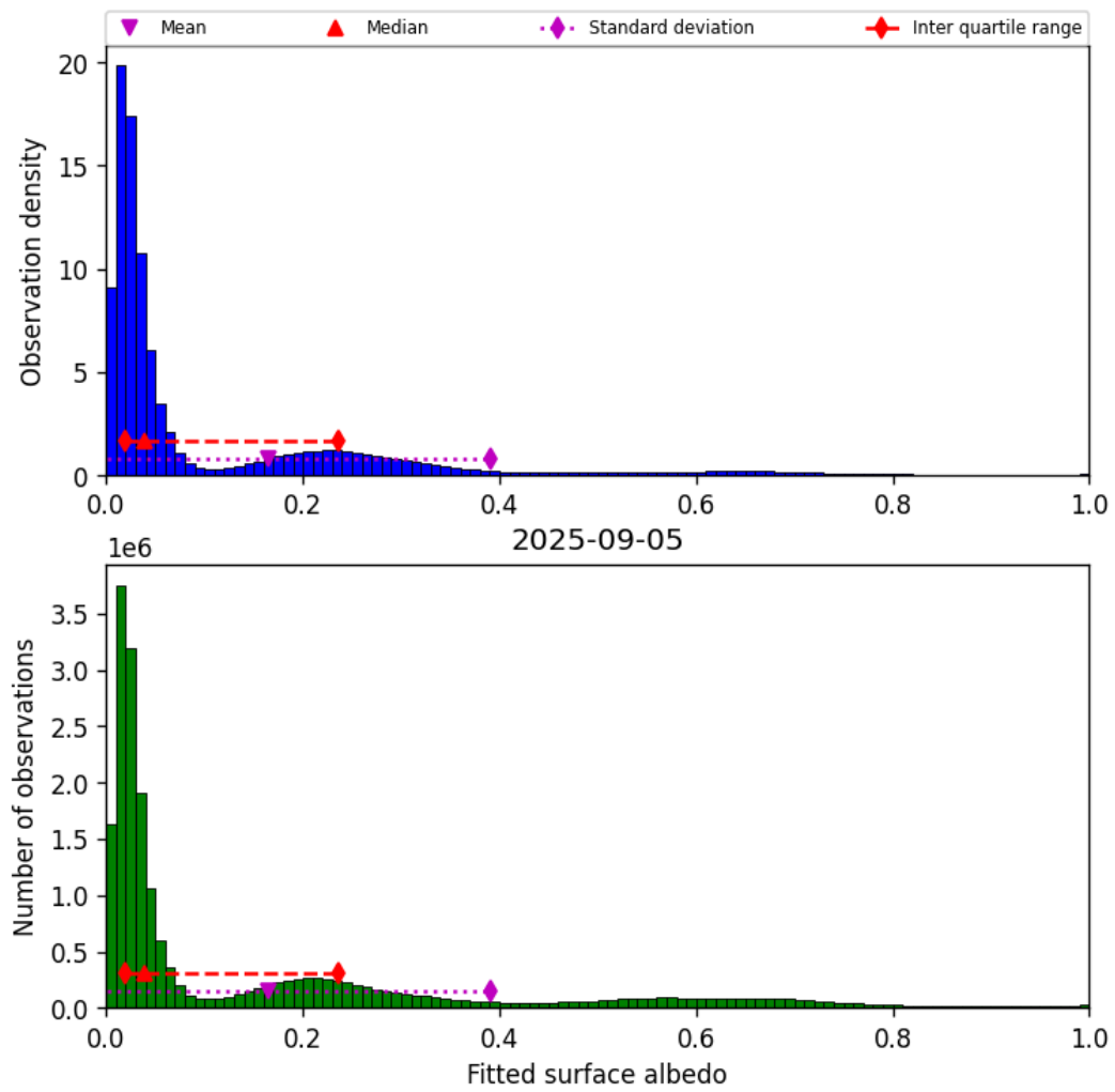
Figure 45: Histogram of “Fitted surface albedo” for 2025-09-04 to 2025-09-06
