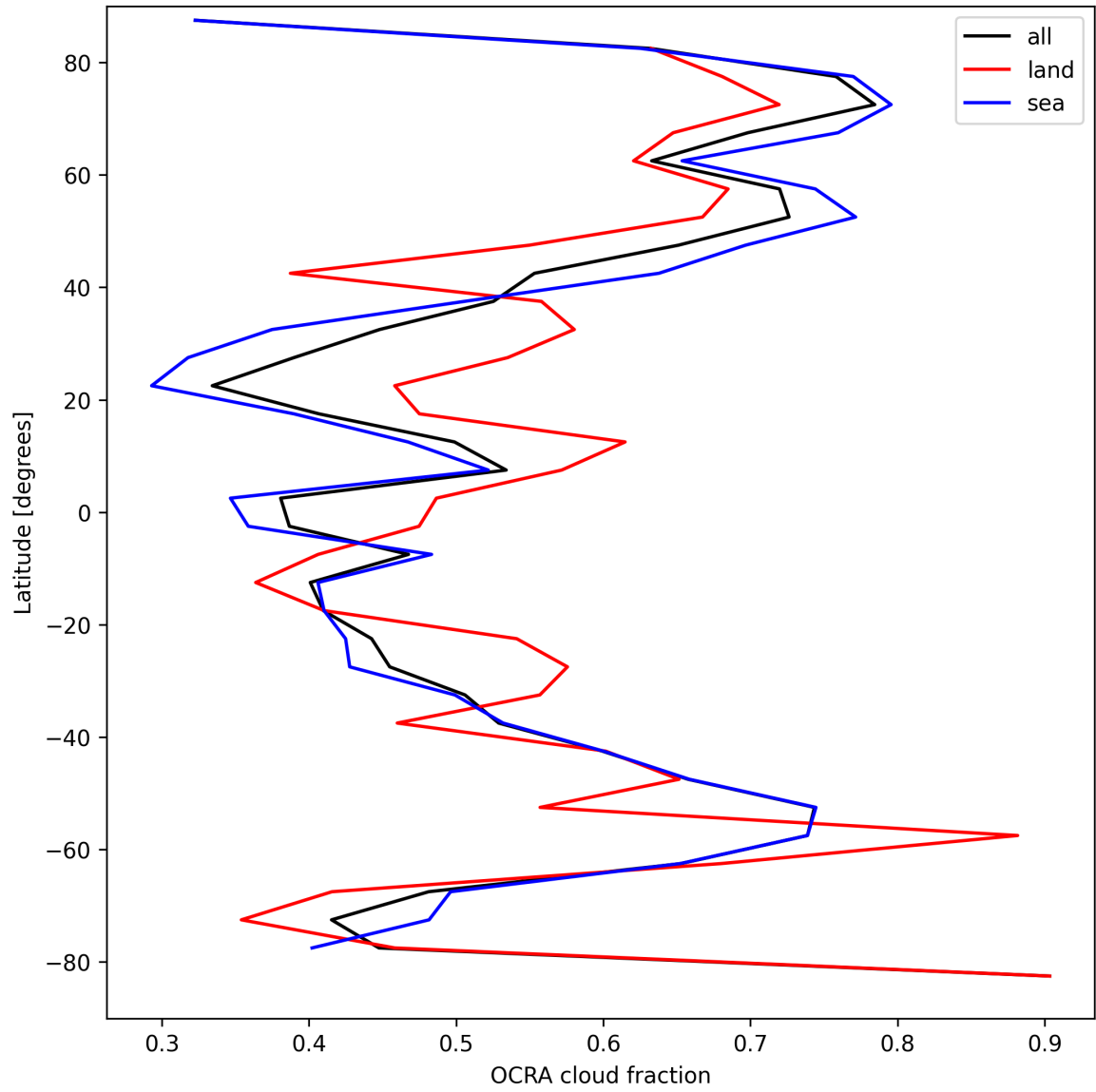
Figure 34: Zonal average of “OCRA cloud fraction” for 2025-09-04 to 2025-09-06.
