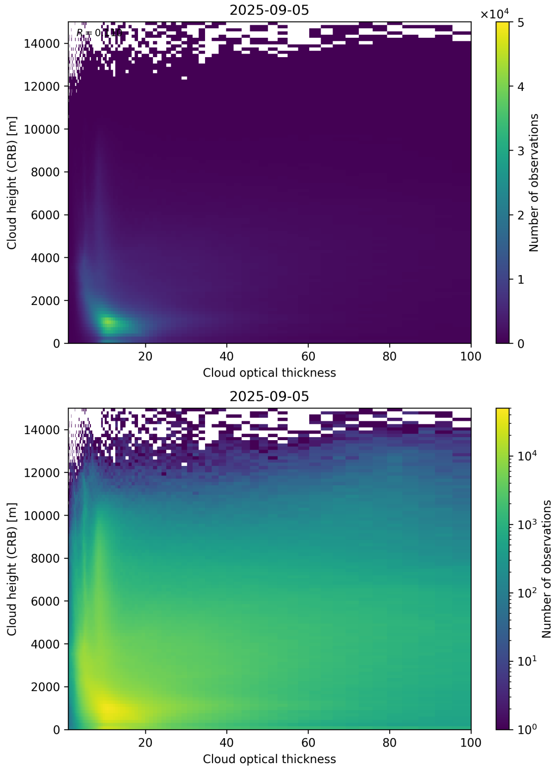
Figure 85: Scatter density plot of “Cloud optical thickness” against “Cloud height (CRB)” for 2025-09-04 to 2025-09-06.
