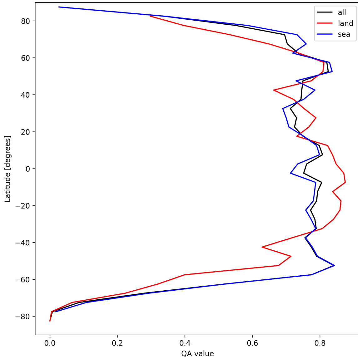
Figure 22: Zonal average of “QA value” for 2025-09-04 to 2025-09-06.
