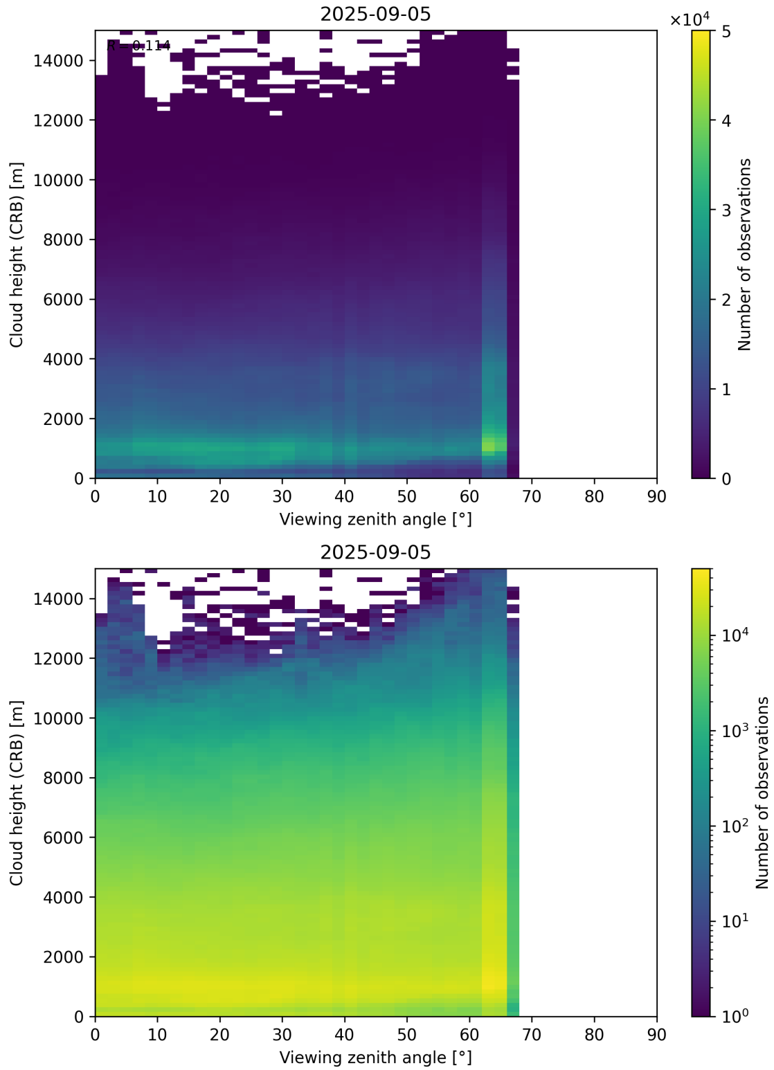
Figure 110: Scatter density plot of “Viewing zenith angle” against “Cloud height (CRB)” for 2025-09-04 to 2025-09-06.
