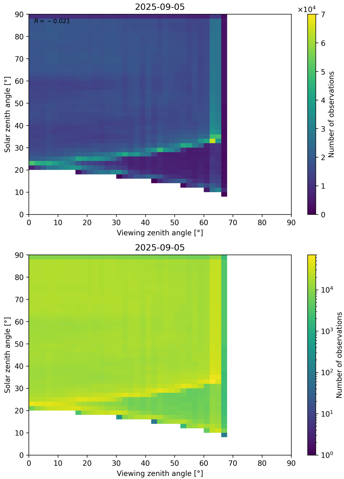
Figure 114: Scatter density plot of “Viewing zenith angle” against “Solar zenith angle” for 2025-09-04 to 2025-09-06.
