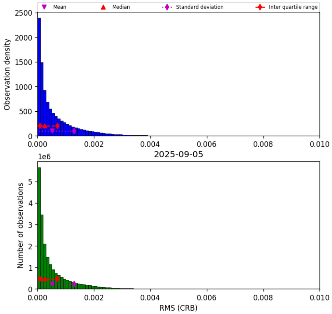
Figure 48: Histogram of “RMS (CRB)” for 2025-09-04 to 2025-09-06
