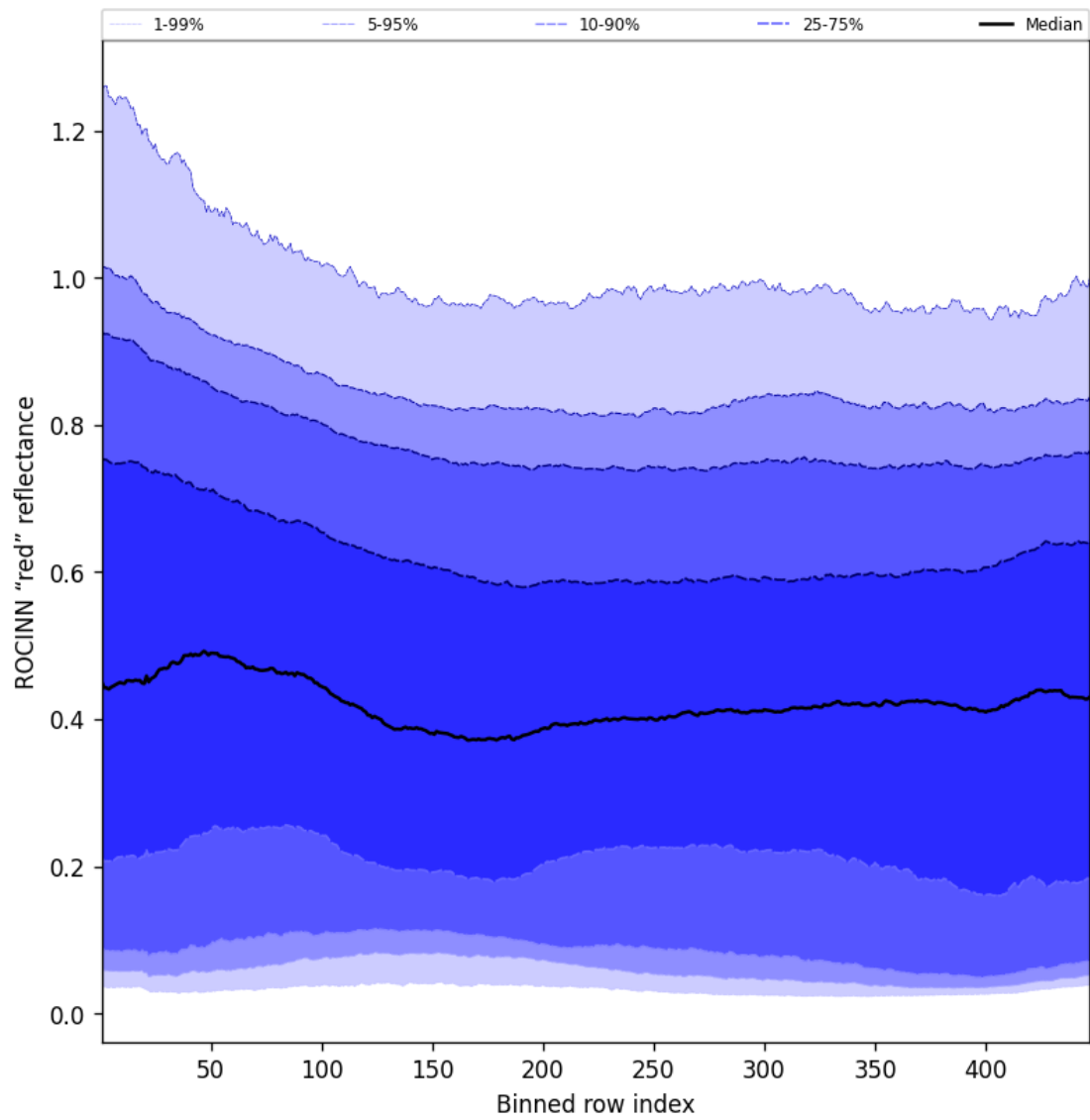
Figure 69: Along track statistics of “ROCINN “red” reflectance” for 2025-09-04 to 2025-09-06
