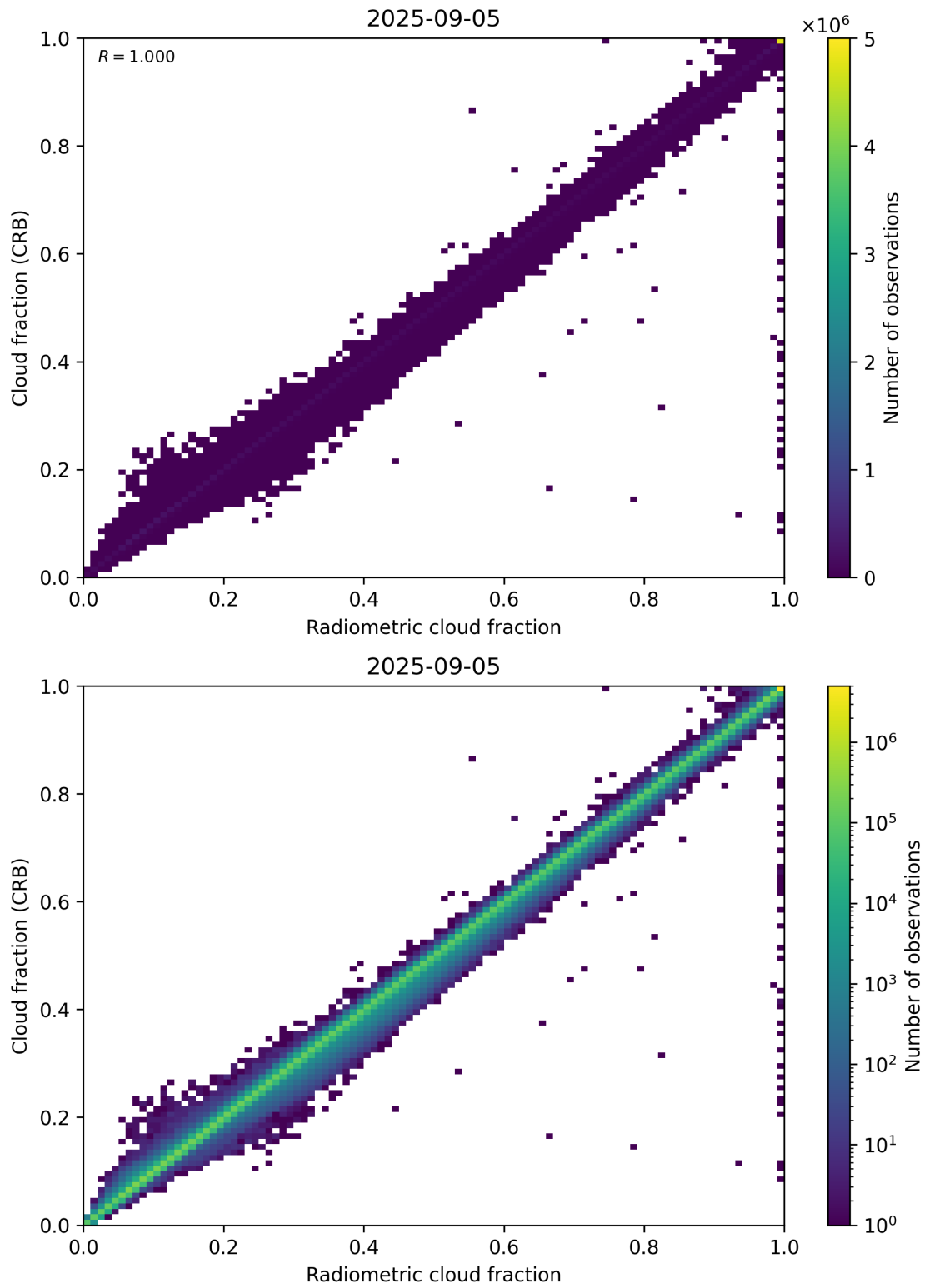
Figure 73: Scatter density plot of “Radiometric cloud fraction” against “Cloud fraction (CRB)” for 2025-09-04 to 2025-09-06.
