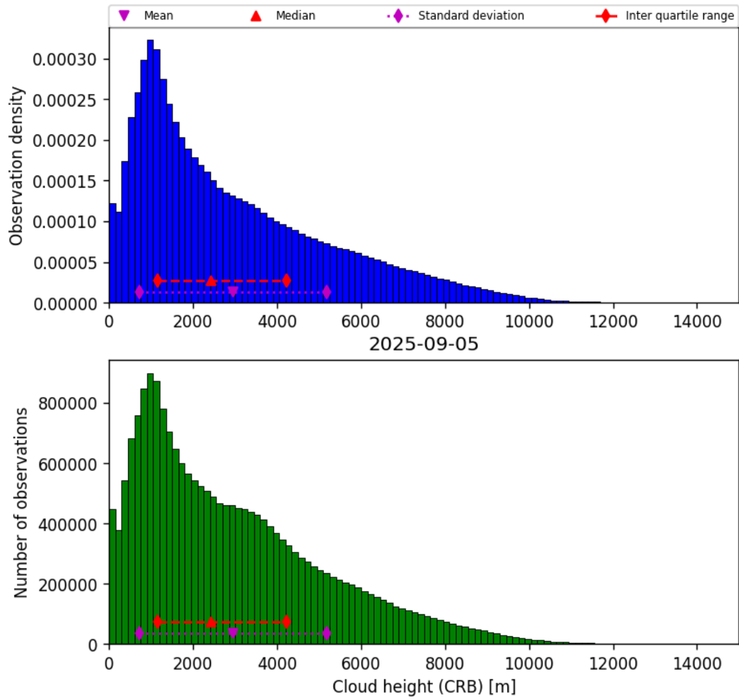
Figure 43: Histogram of “Cloud height (CRB)” for 2025-09-04 to 2025-09-06
