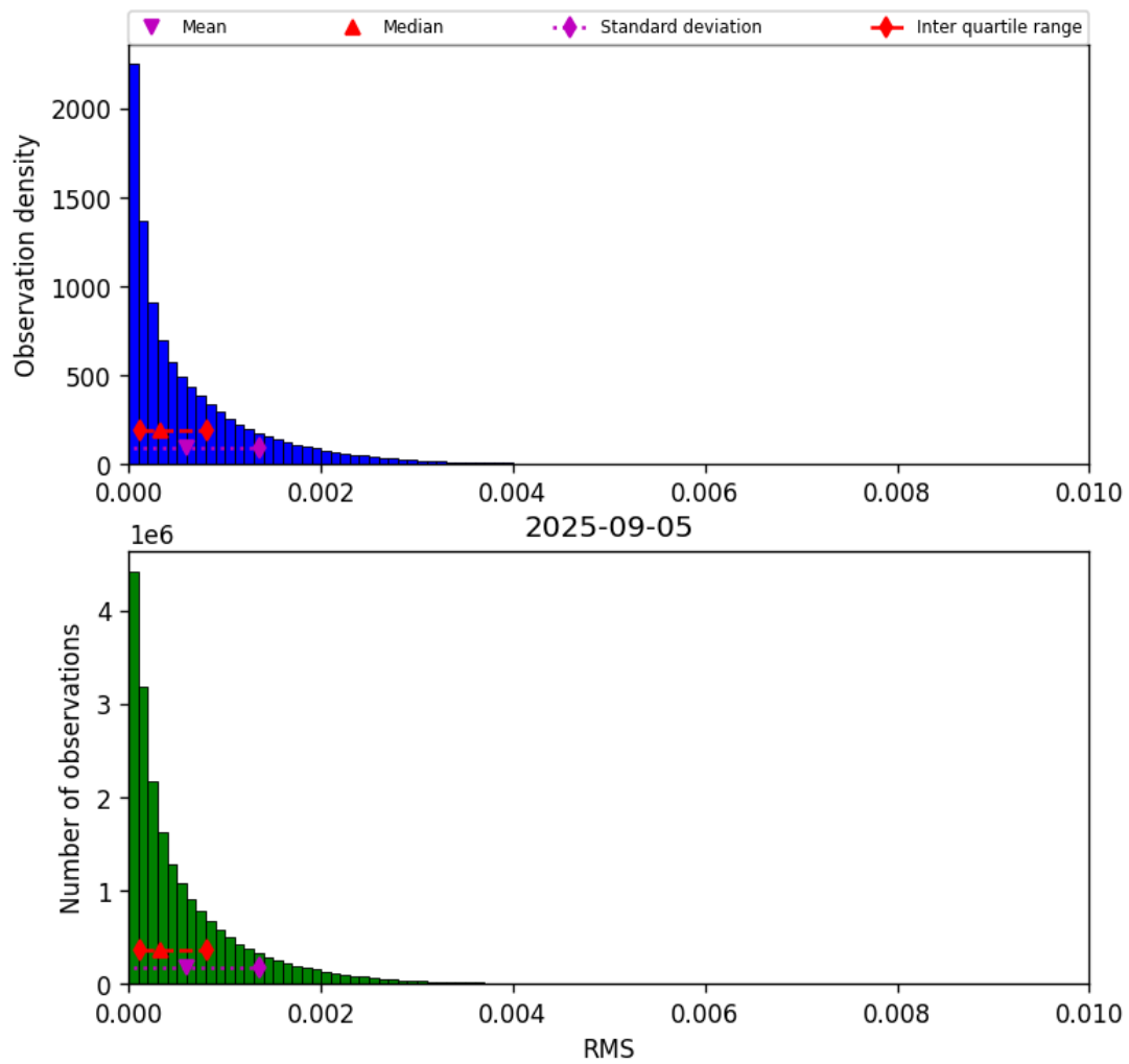
Figure 47: Histogram of “RMS” for 2025-09-04 to 2025-09-06
