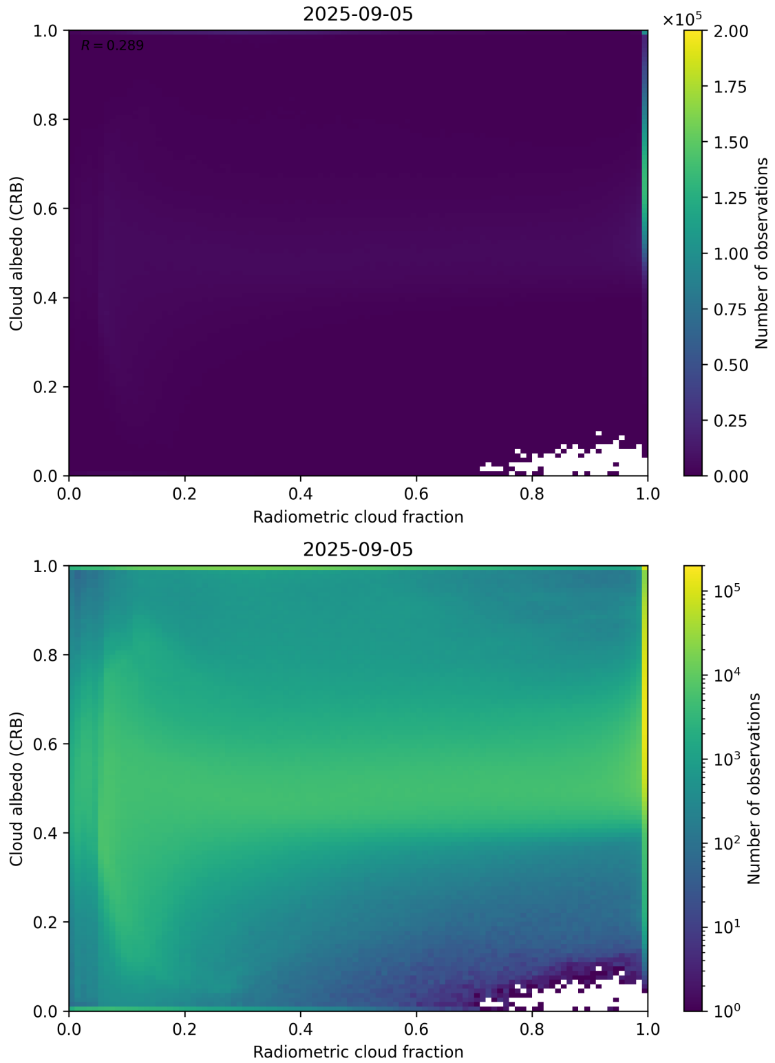
Figure 71: Scatter density plot of “Radiometric cloud fraction” against “Cloud albedo (CRB)” for 2025-09-04 to 2025-09-06.
