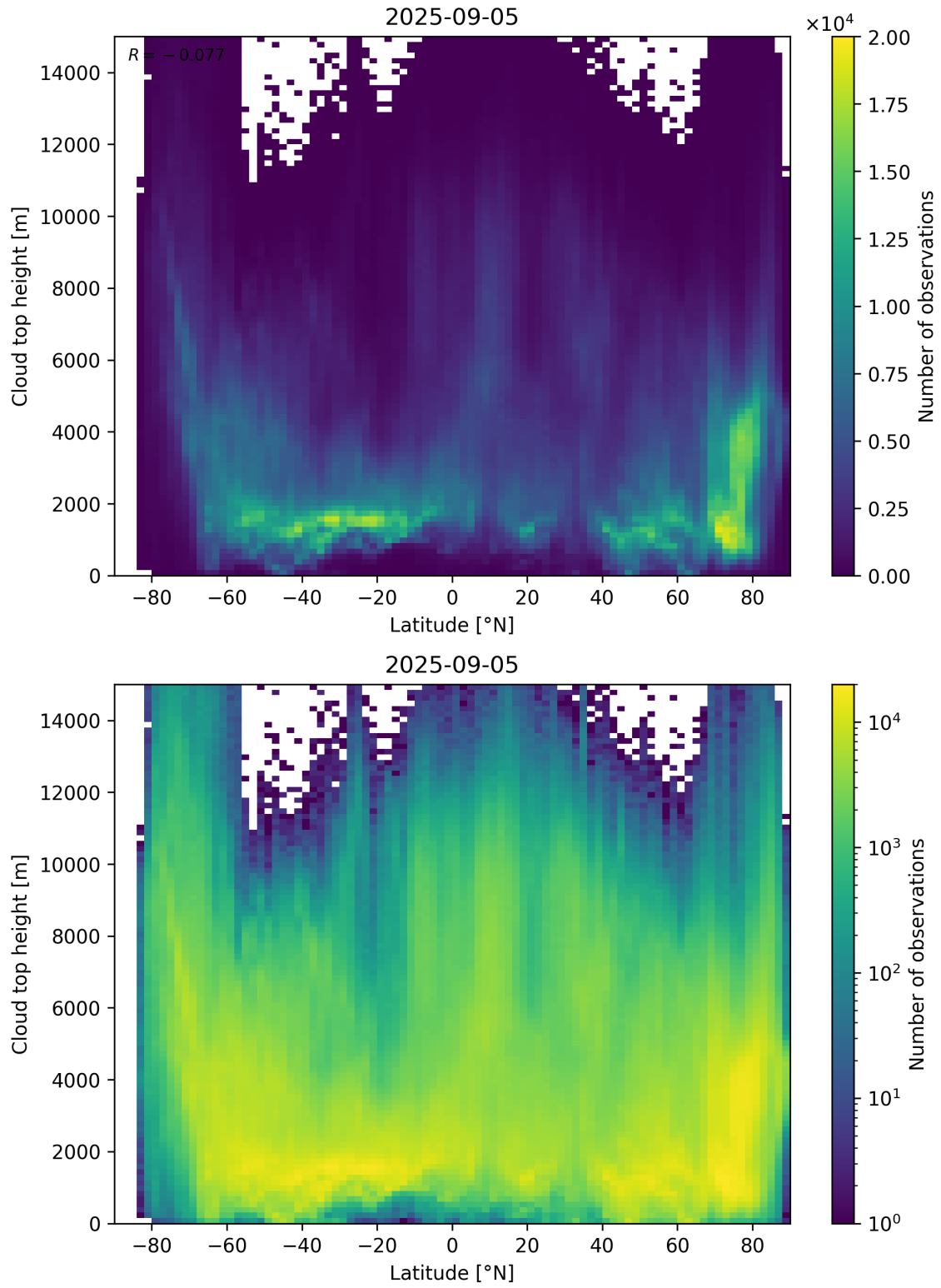
Figure 97: Scatter density plot of “Latitude” against “Cloud top height” for 2025-09-04 to 2025-09-06.
