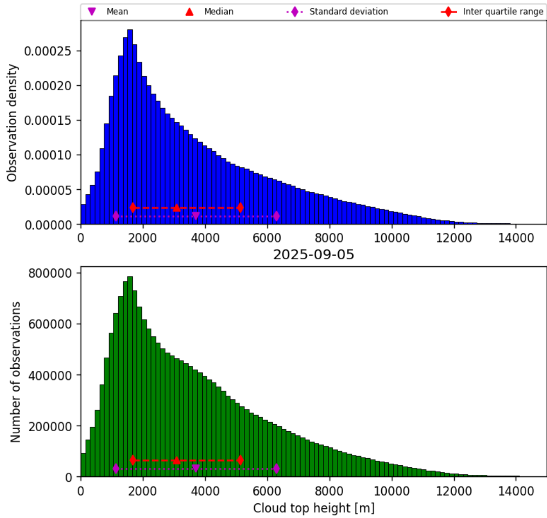
Figure 40: Histogram of “Cloud top height” for 2025-09-04 to 2025-09-06
