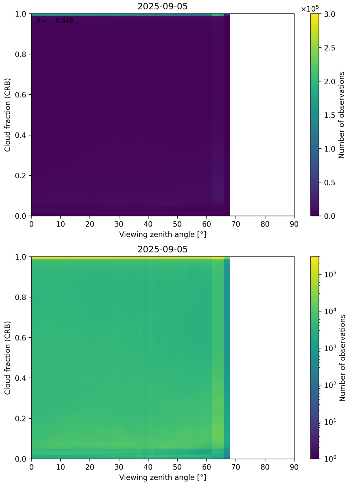
Figure 109: Scatter density plot of “Viewing zenith angle” against “Cloud fraction (CRB)” for 2025-09-04 to 2025-09-06.
