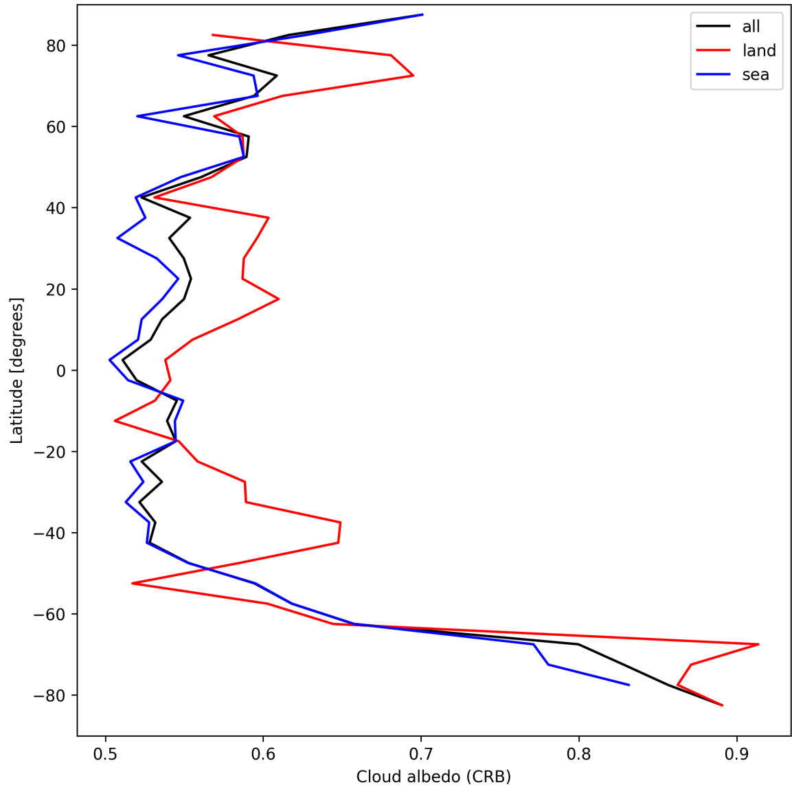
Figure 28: Zonal average of “Cloud albedo (CRB)” for 2025-09-04 to 2025-09-06.
