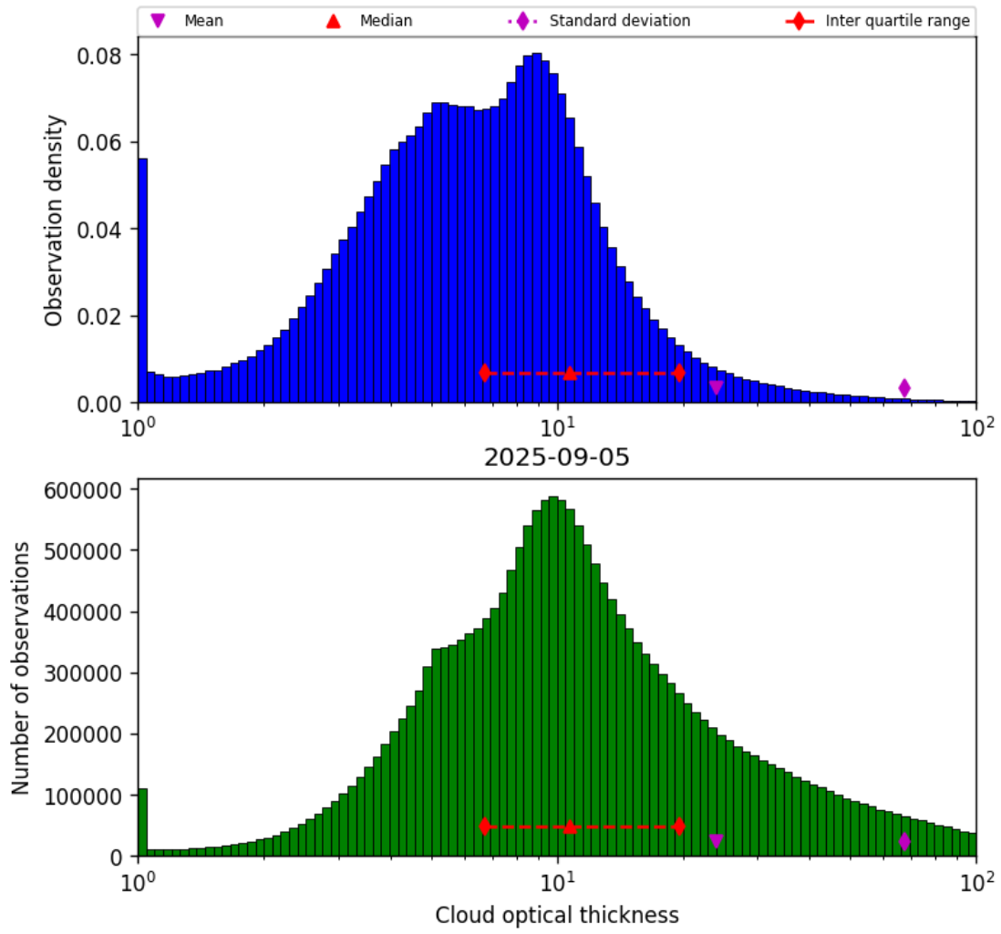
Figure 41: Histogram of “Cloud optical thickness” for 2025-09-04 to 2025-09-06
