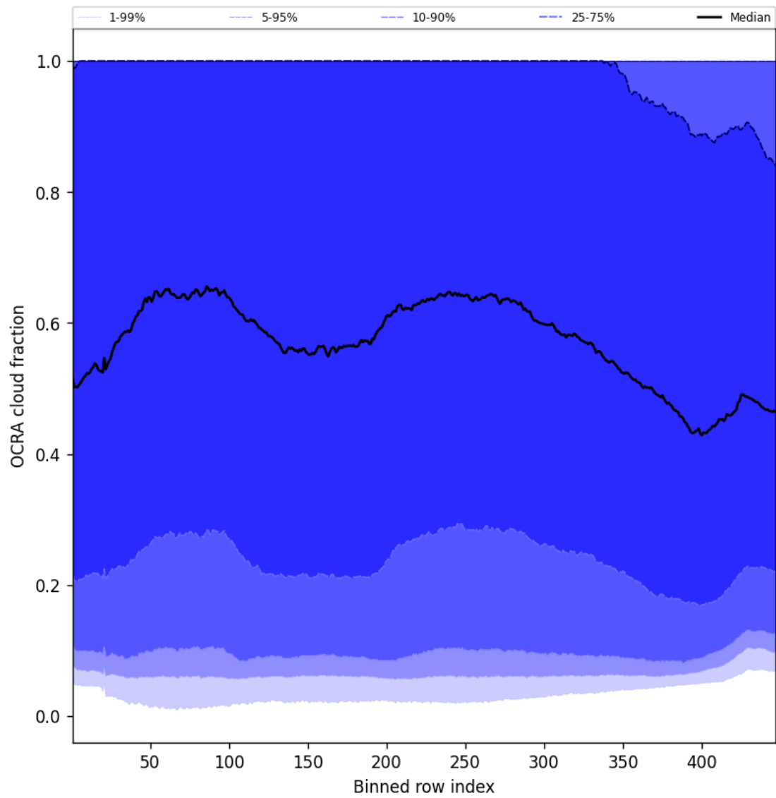
Figure 66: Along track statistics of “OCRA cloud fraction” for 2025-09-04 to 2025-09-06
