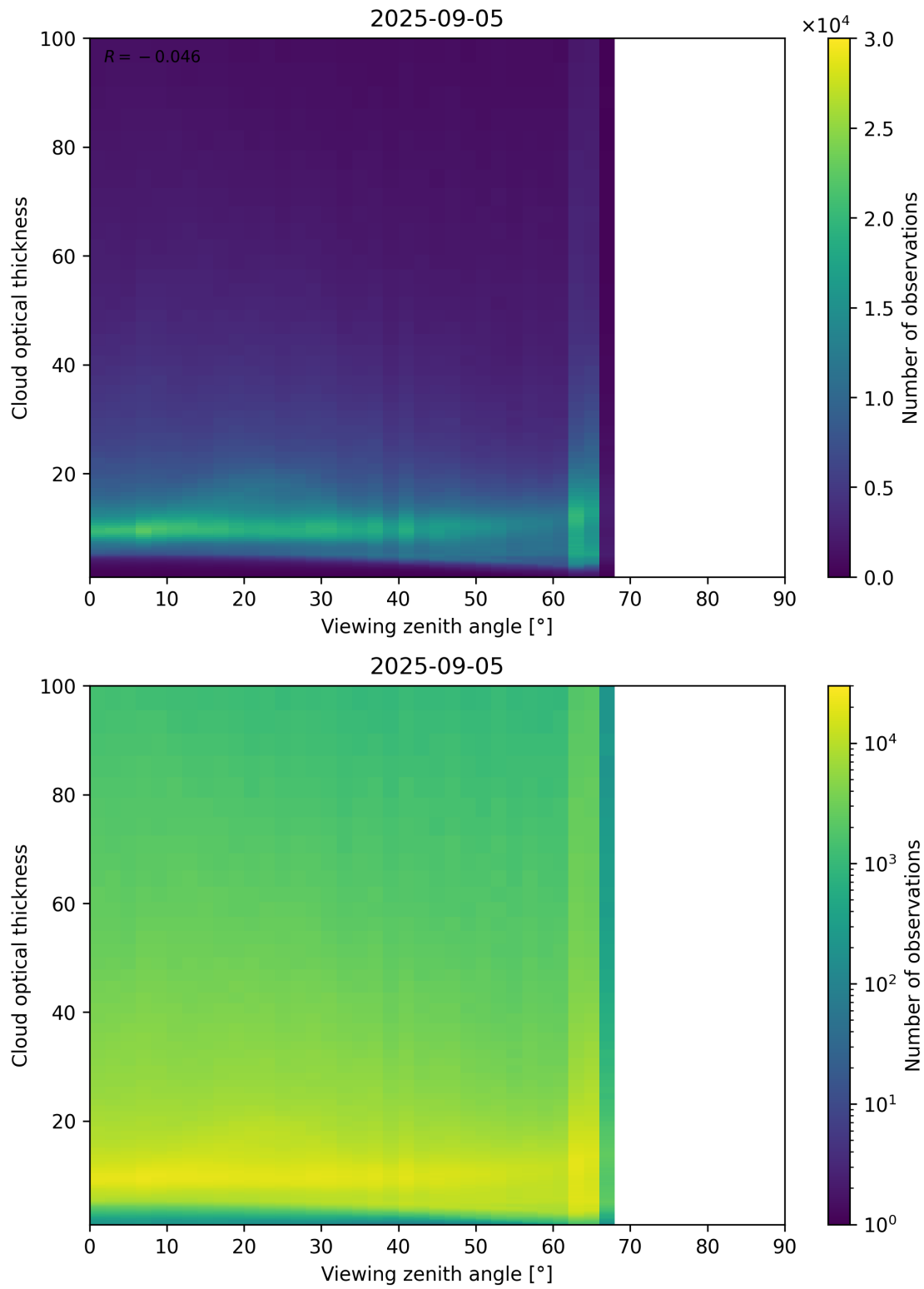
Figure 111: Scatter density plot of “Viewing zenith angle” against “Cloud optical thickness” for 2025-09-04 to 2025-09-06.
