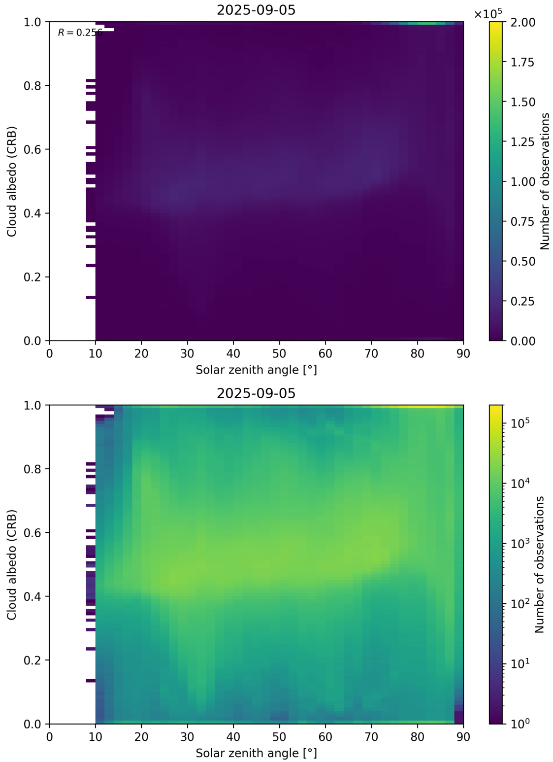
Figure 98: Scatter density plot of “Solar zenith angle” against “Cloud albedo (CRB)” for 2025-09-04 to 2025-09-06.
