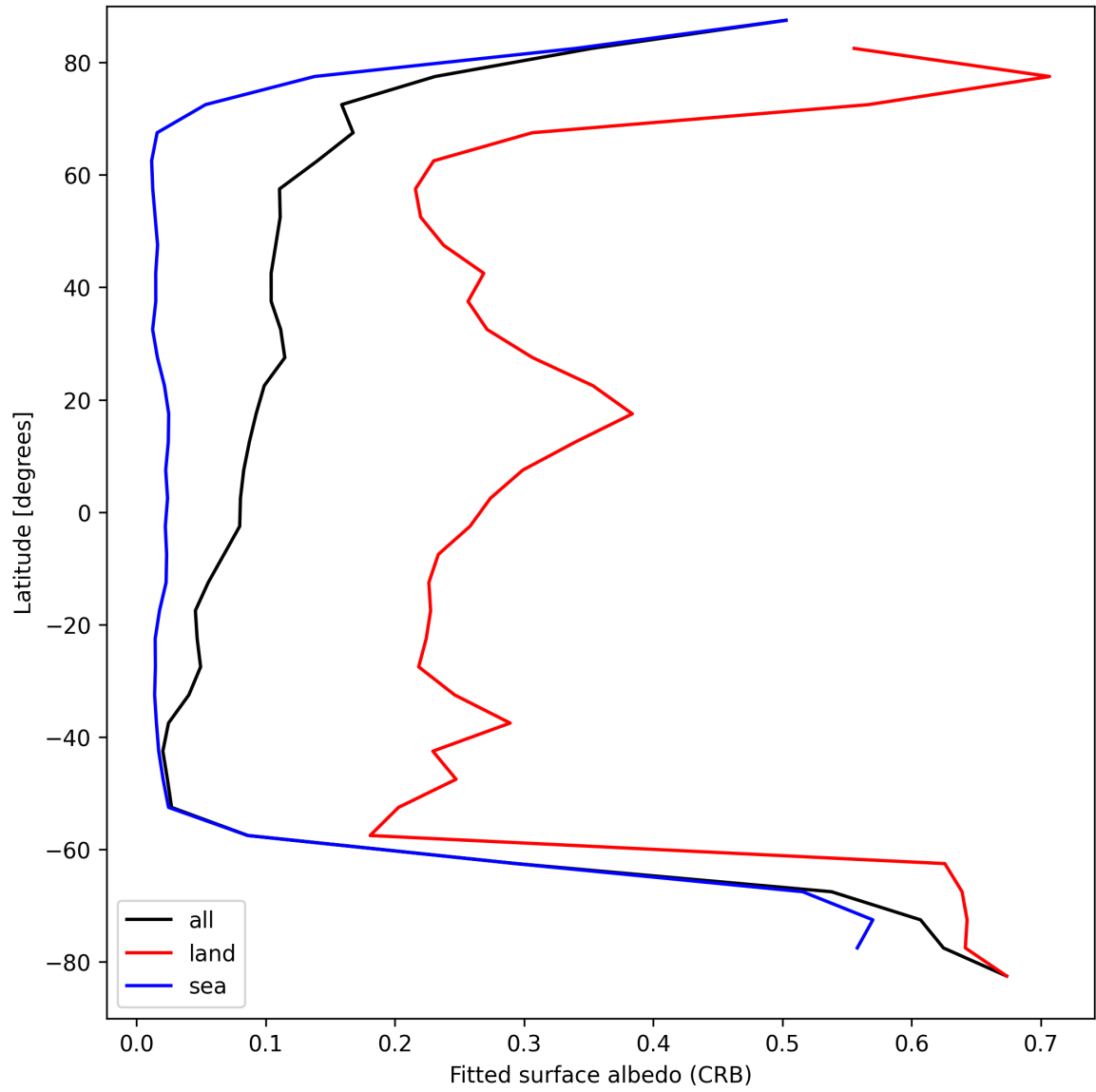
Figure 30: Zonal average of “Fitted surface albedo (CRB)” for 2025-09-04 to 2025-09-06.
