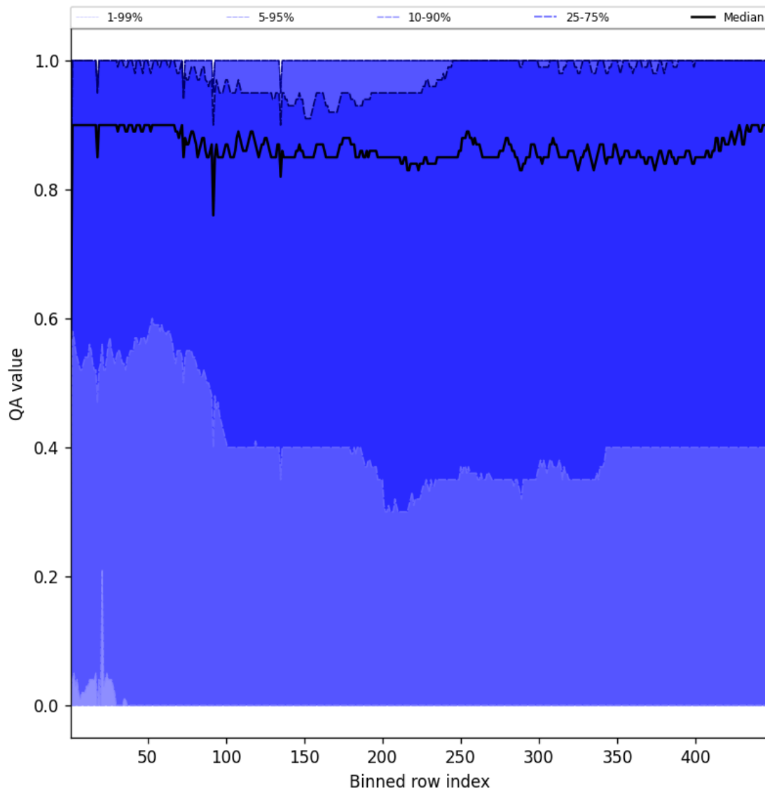
Figure 54: Along track statistics of “QA value” for 2025-09-04 to 2025-09-06
