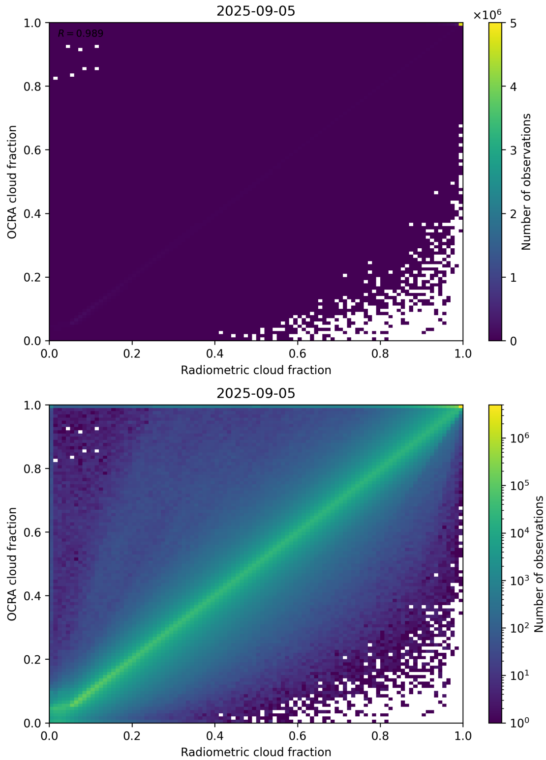
Figure 72: Scatter density plot of “Radiometric cloud fraction” against “OCRA cloud fraction” for 2025-09-04 to 2025-09-06.
