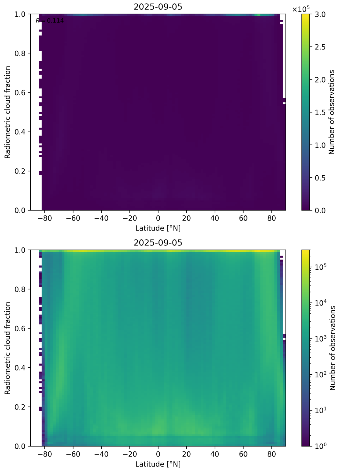
Figure 92: Scatter density plot of “Latitude” against “Radiometric cloud fraction” for 2025-09-04 to 2025-09-06.
