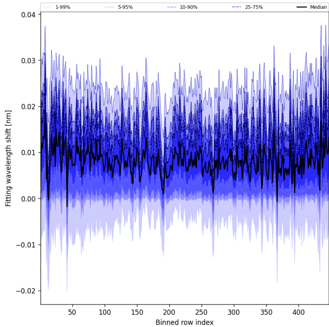
Figure 65: Along track statistics of “Fitting wavelength shift” for 2025-09-04 to 2025-09-06
