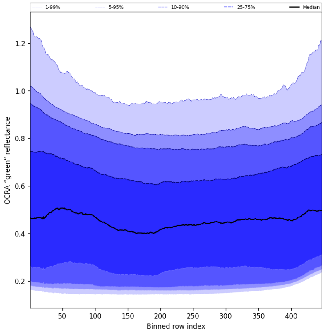
Figure 68: Along track statistics of “OCRA “green” reflectance” for 2025-09-04 to 2025-09-06
