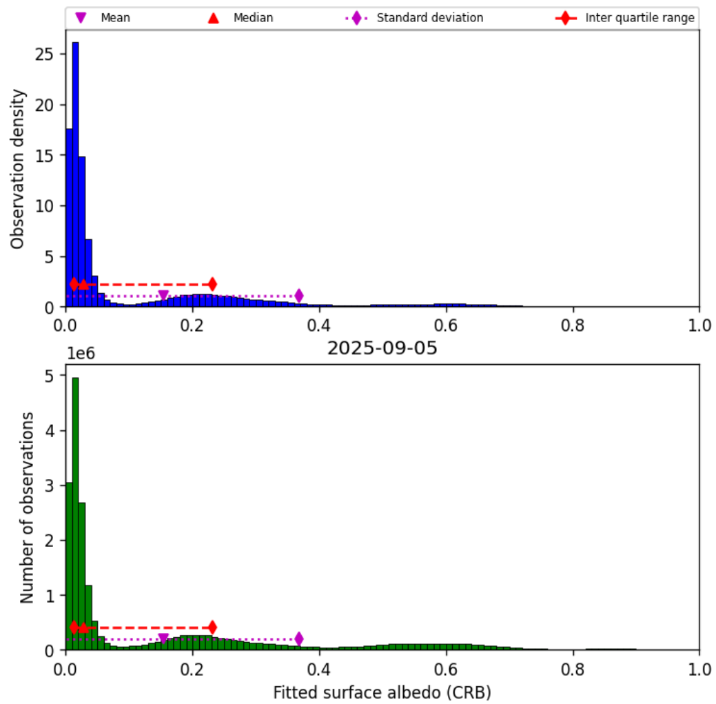
Figure 46: Histogram of “Fitted surface albedo (CRB)” for 2025-09-04 to 2025-09-06
