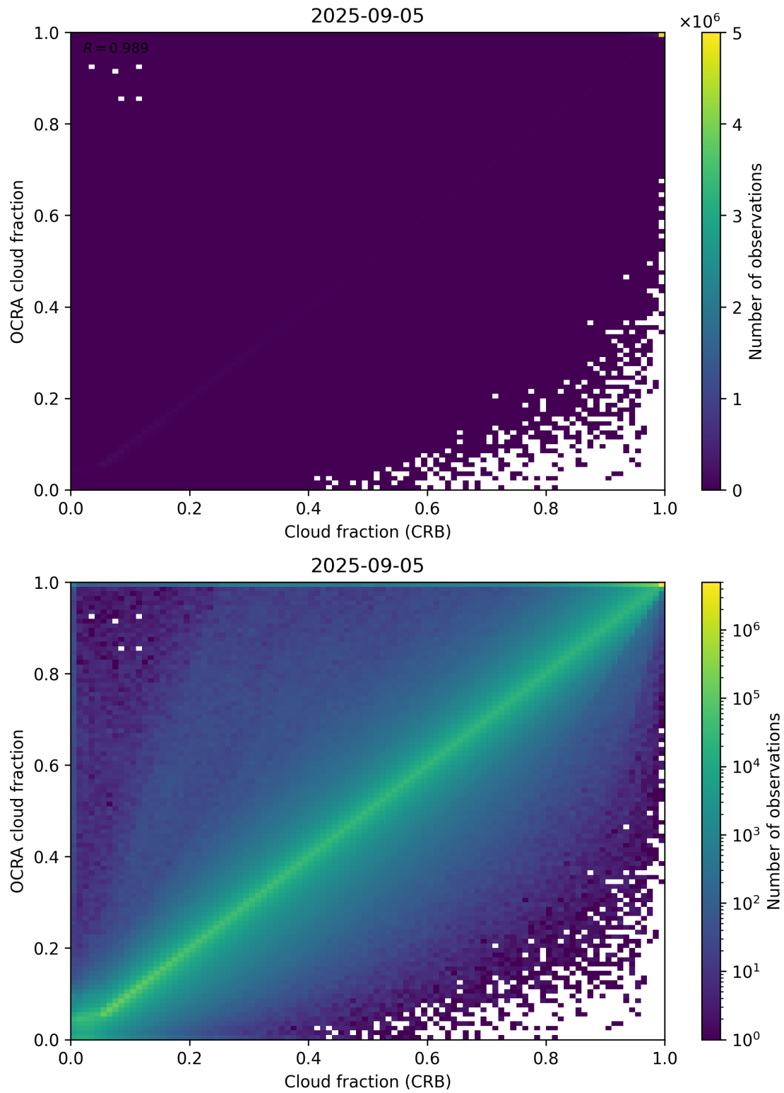
Figure 78: Scatter density plot of “Cloud fraction (CRB)” against “OCRA cloud fraction” for 2025-09-04 to 2025-09-06.
