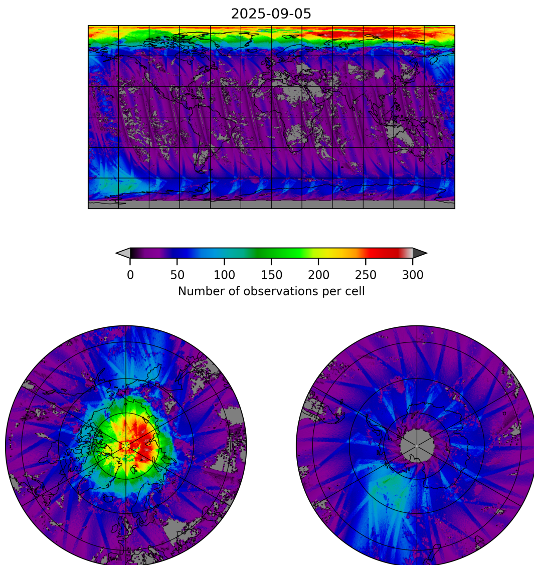
Figure 21: Map of the number of observations for 2025-09-04 to 2025-09-06
