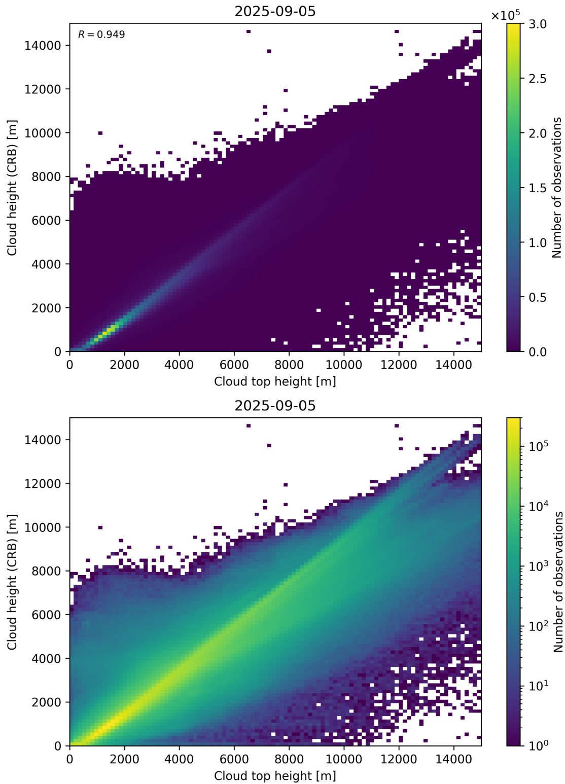
Figure 89: Scatter density plot of “Cloud top height” against “Cloud height (CRB)” for 2025-09-04 to 2025-09-06.
