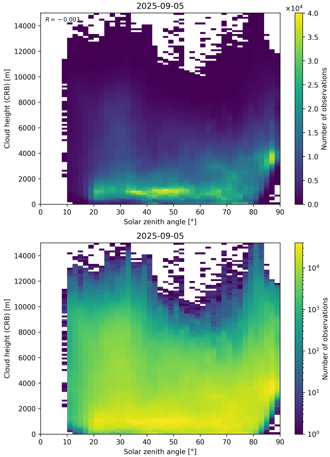
Figure 102: Scatter density plot of “Solar zenith angle” against “Cloud height (CRB)” for 2025-09-04 to 2025-09-06.
