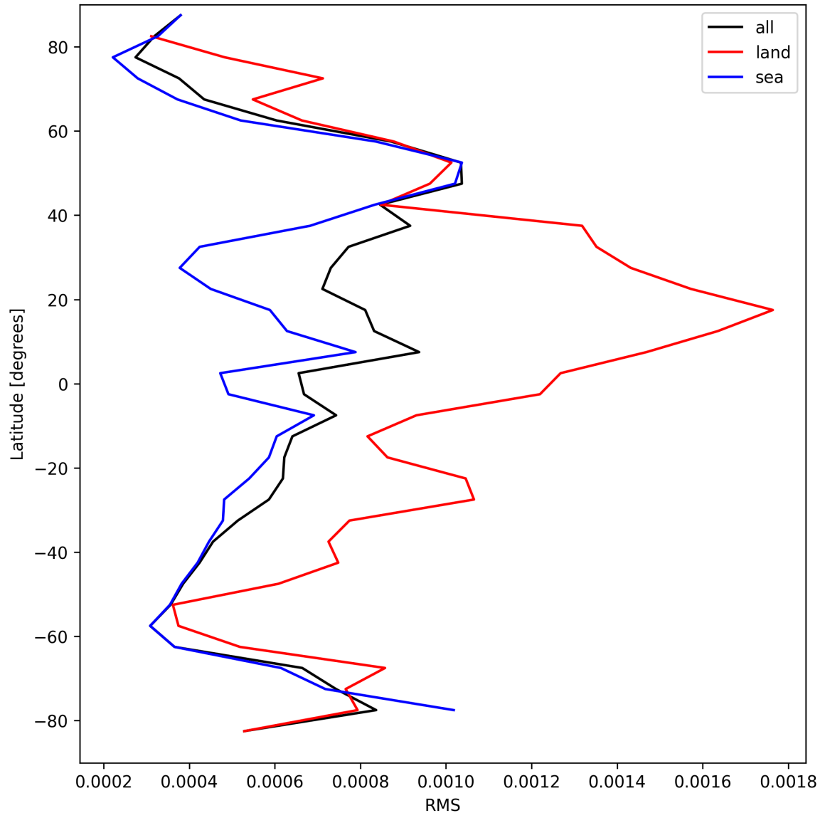
Figure 31: Zonal average of “RMS” for 2025-09-04 to 2025-09-06.
