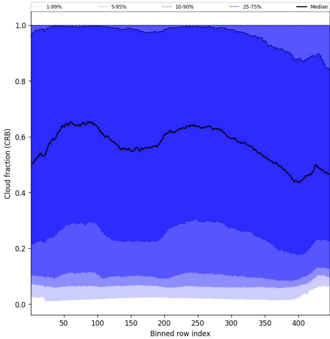
Figure 58: Along track statistics of “Cloud fraction (CRB)” for 2025-09-04 to 2025-09-06
