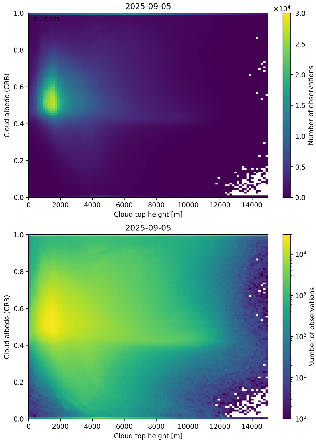
Figure 86: Scatter density plot of “Cloud top height” against “Cloud albedo (CRB)” for 2025-09-04 to 2025-09-06.
