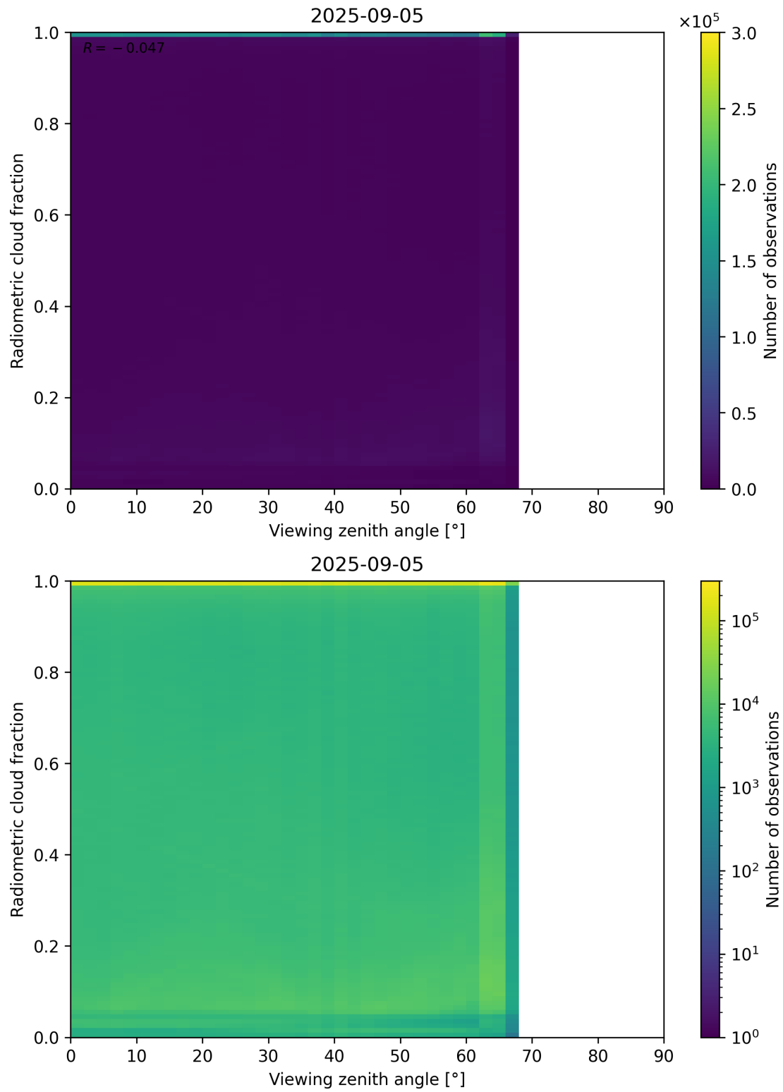
Figure 107: Scatter density plot of “Viewing zenith angle” against “Radiometric cloud fraction” for 2025-09-04 to 2025-09-06.
