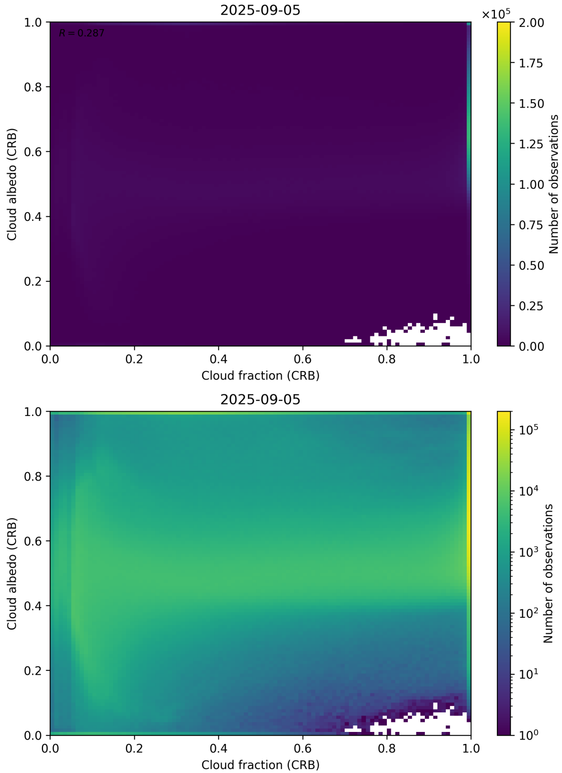
Figure 77: Scatter density plot of “Cloud fraction (CRB)” against “Cloud albedo (CRB)” for 2025-09-04 to 2025-09-06.
