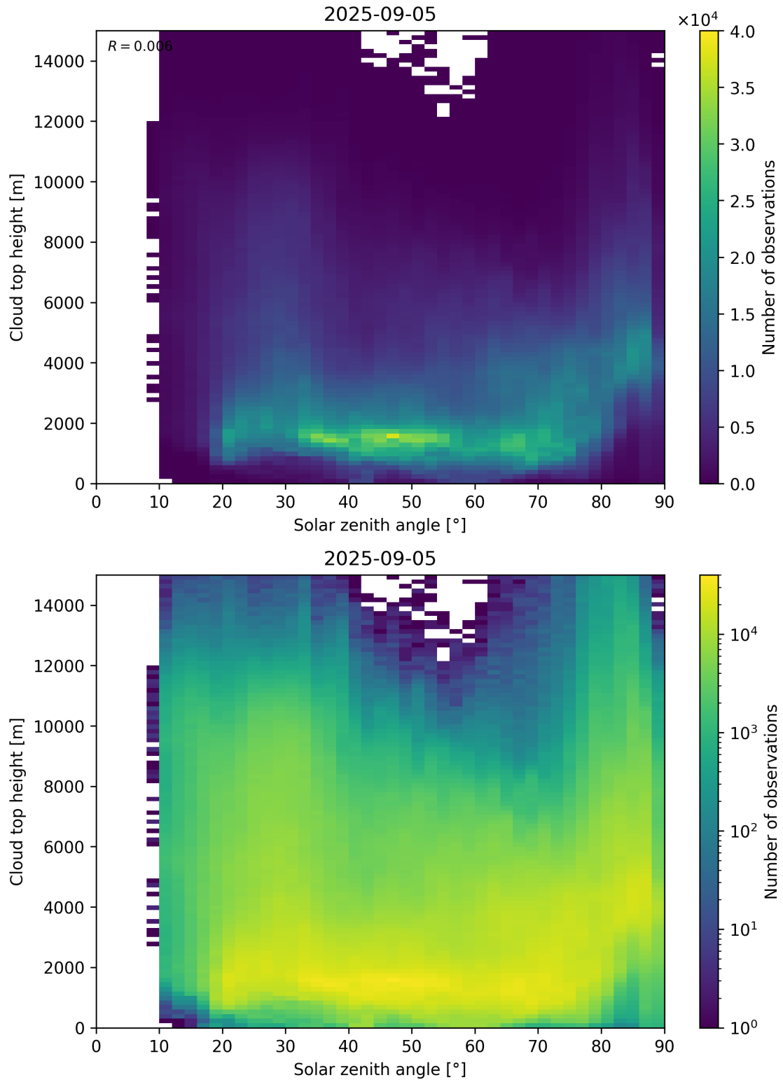
Figure 104: Scatter density plot of “Solar zenith angle” against “Cloud top height” for 2025-09-04 to 2025-09-06.
