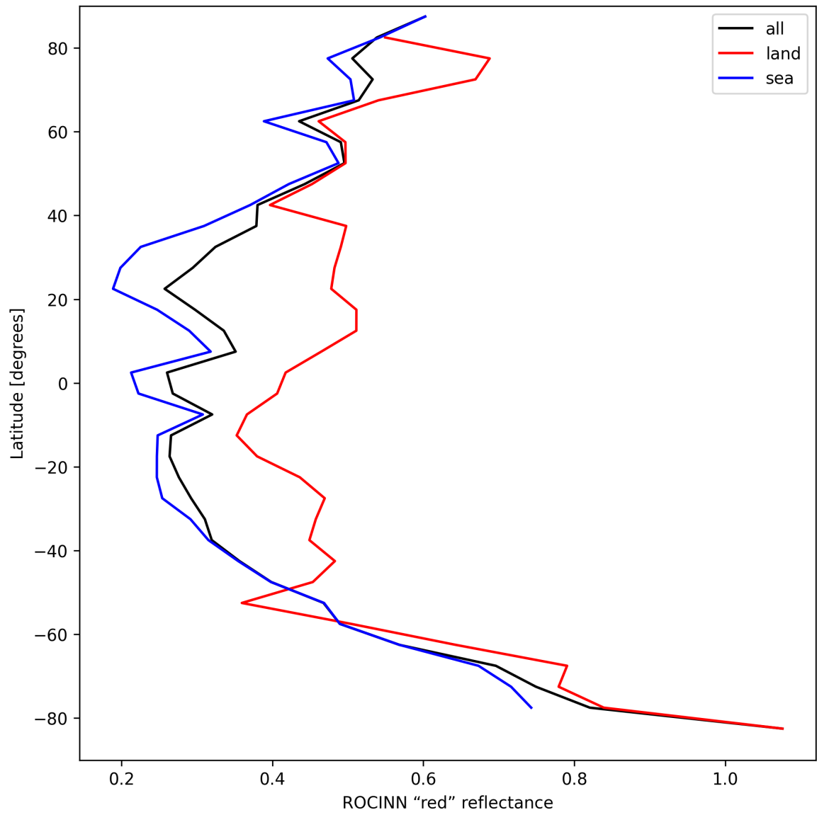
Figure 37: Zonal average of “ROCINN “red” reflectance” for 2025-09-04 to 2025-09-06.
