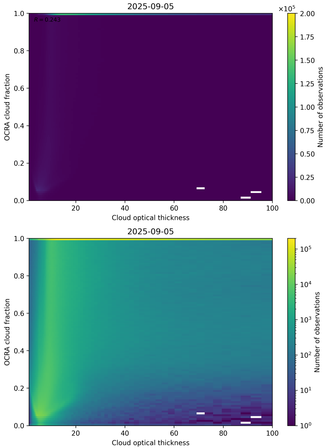
Figure 83: Scatter density plot of “Cloud optical thickness” against “OCRA cloud fraction” for 2025-09-04 to 2025-09-06.
