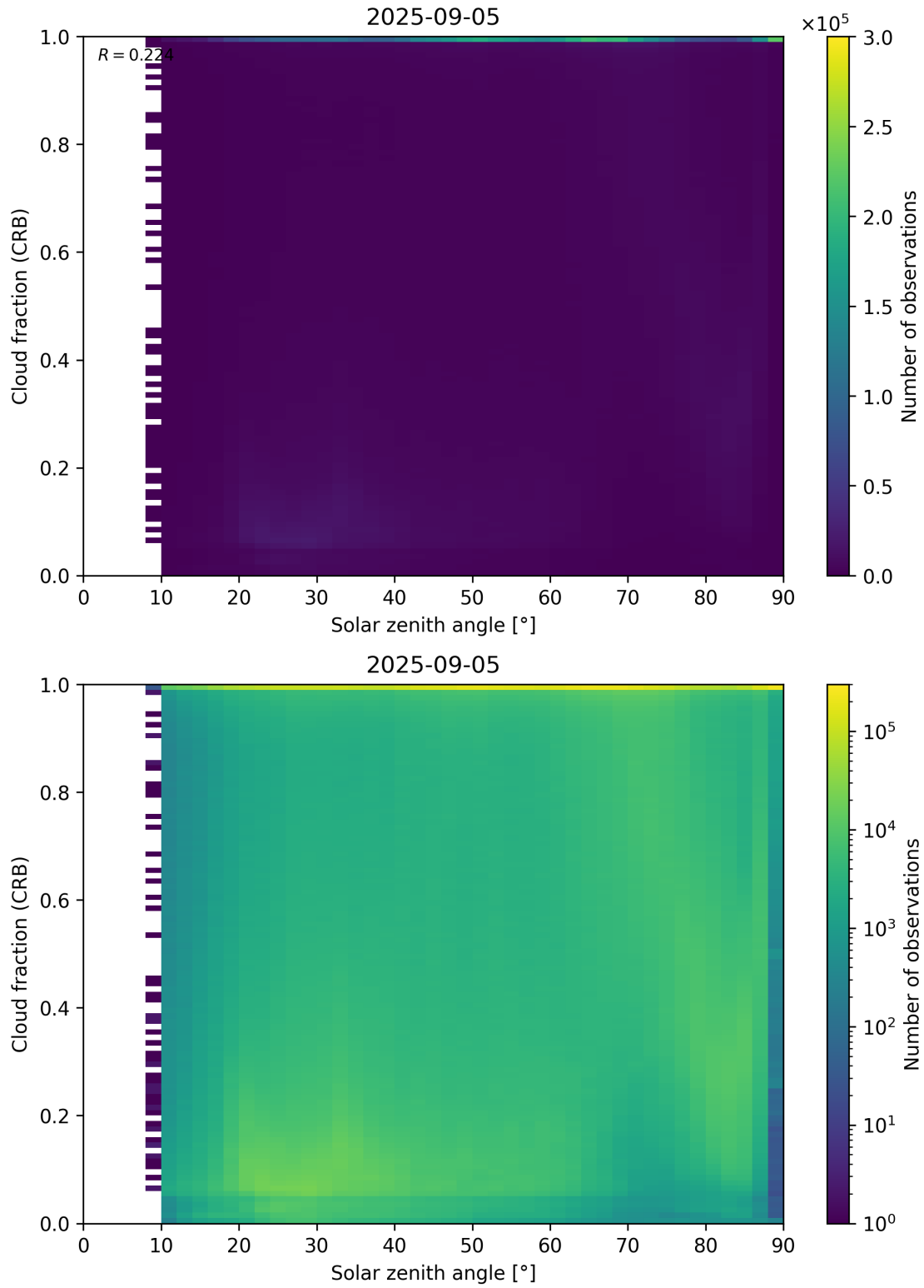
Figure 101: Scatter density plot of “Solar zenith angle” against “Cloud fraction (CRB)” for 2025-09-04 to 2025-09-06.
