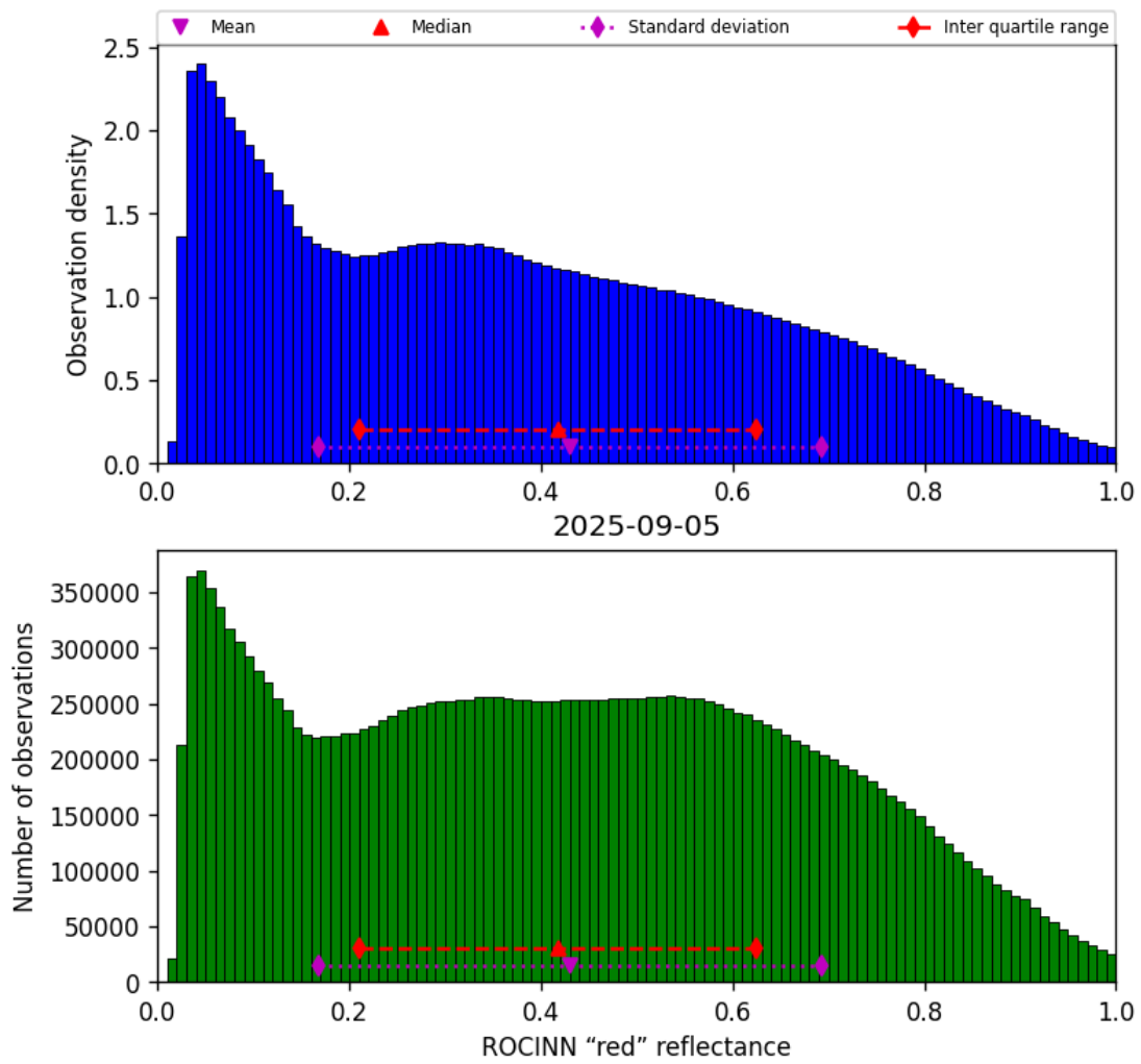
Figure 53: Histogram of “ROCINN “red” reflectance” for 2025-09-04 to 2025-09-06
