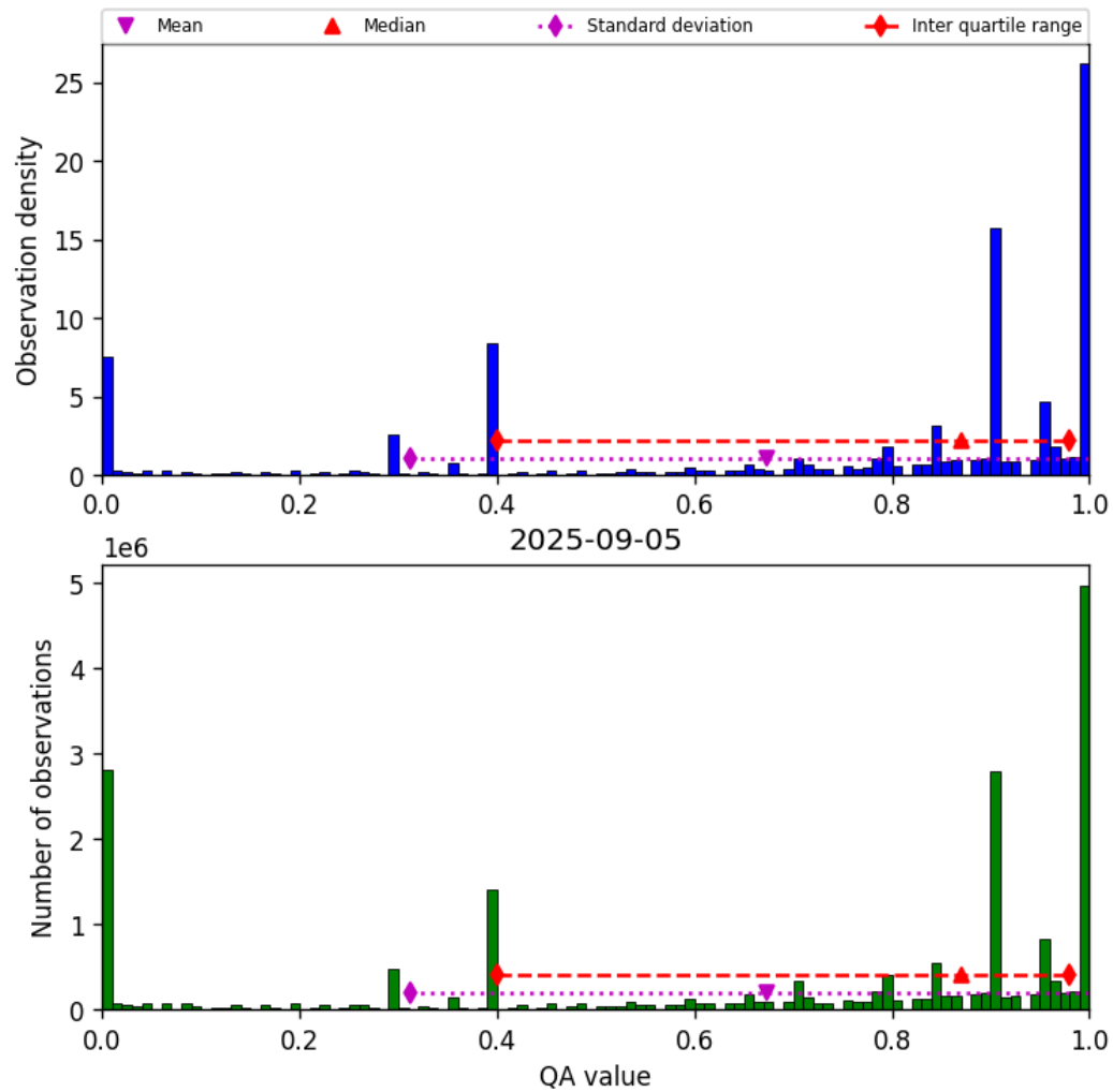
Figure 38: Histogram of “QA value” for 2025-09-04 to 2025-09-06
