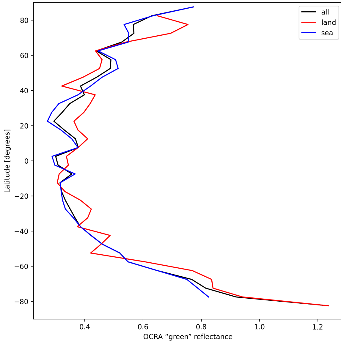
Figure 36: Zonal average of “OCRA “green” reflectance” for 2025-09-04 to 2025-09-06.
