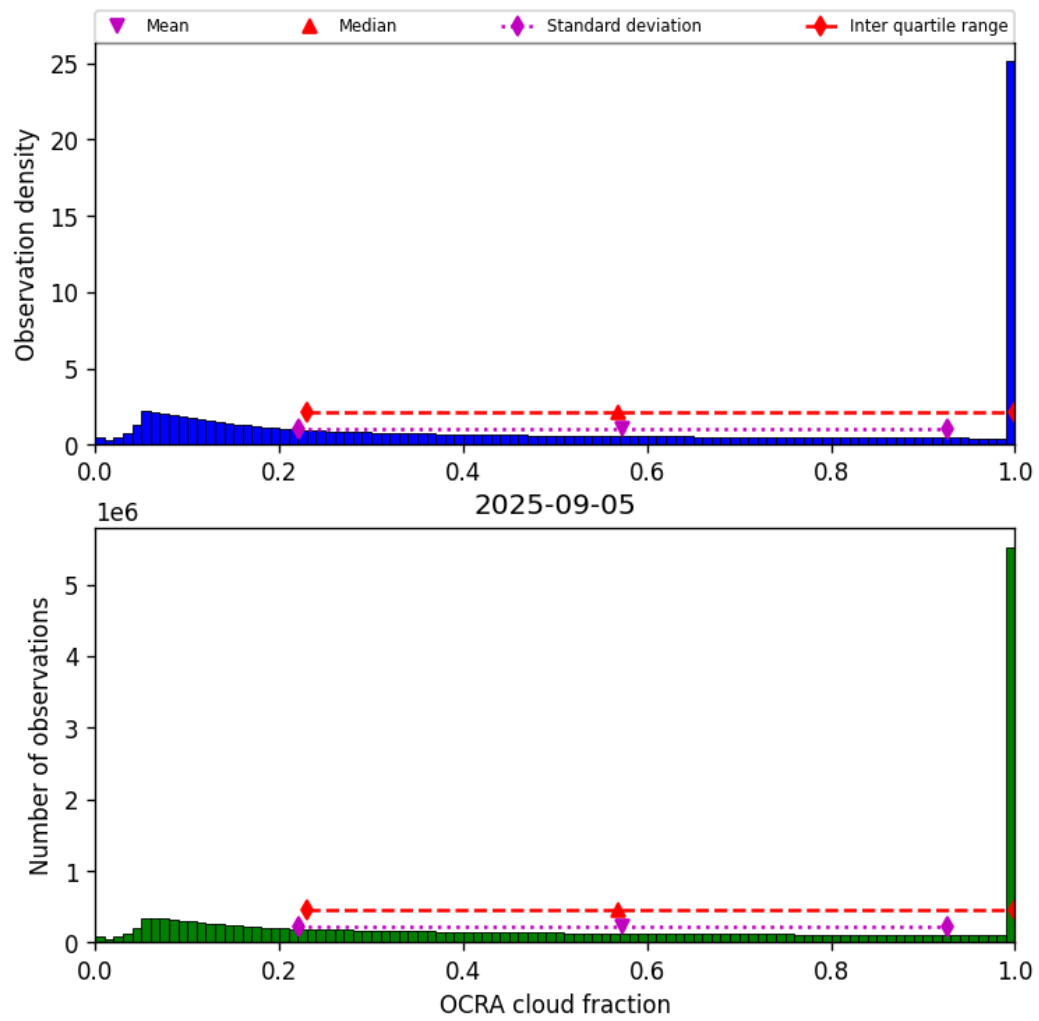
Figure 50: Histogram of “OCRA cloud fraction” for 2025-09-04 to 2025-09-06
