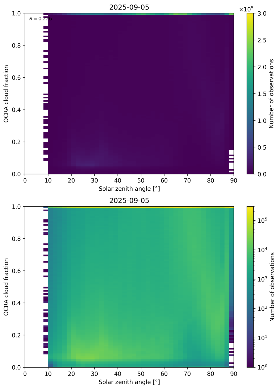
Figure 100: Scatter density plot of “Solar zenith angle” against “OCRA cloud fraction” for 2025-09-04 to 2025-09-06.
