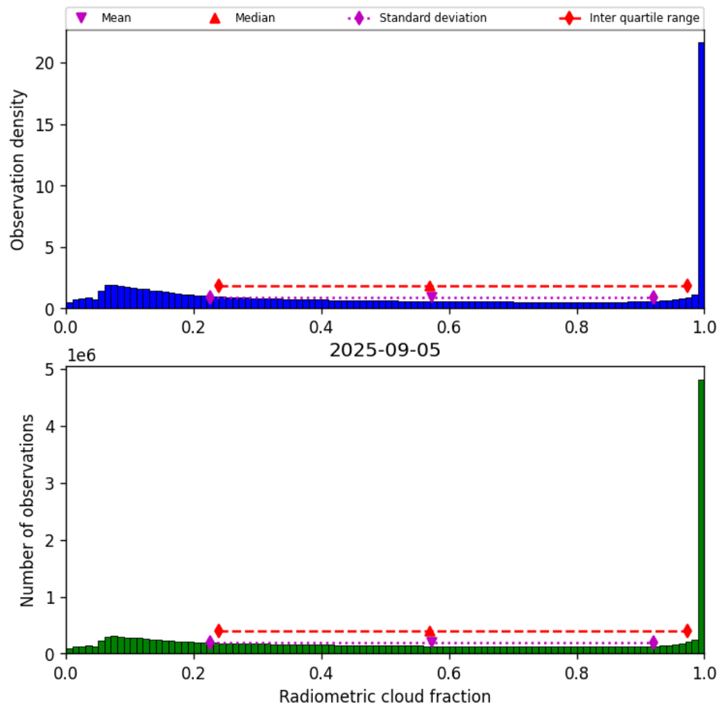
Figure 39: Histogram of “Radiometric cloud fraction” for 2025-09-04 to 2025-09-06
