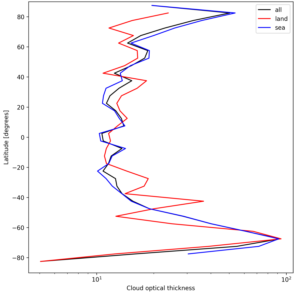
Figure 25: Zonal average of “Cloud optical thickness” for 2025-09-04 to 2025-09-06.
