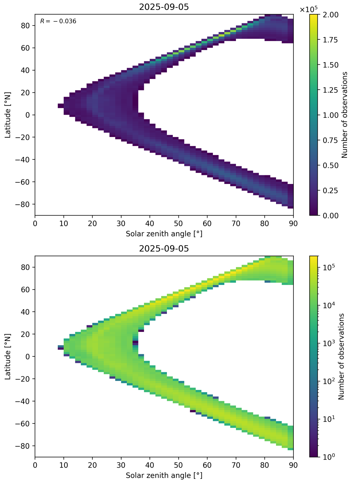
Figure 105: Scatter density plot of “Solar zenith angle” against “Latitude” for 2025-09-04 to 2025-09-06.
