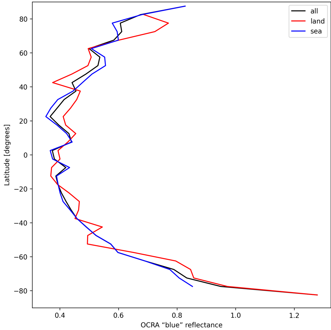
Figure 35: Zonal average of “OCRA “blue” reflectance” for 2025-09-04 to 2025-09-06.
