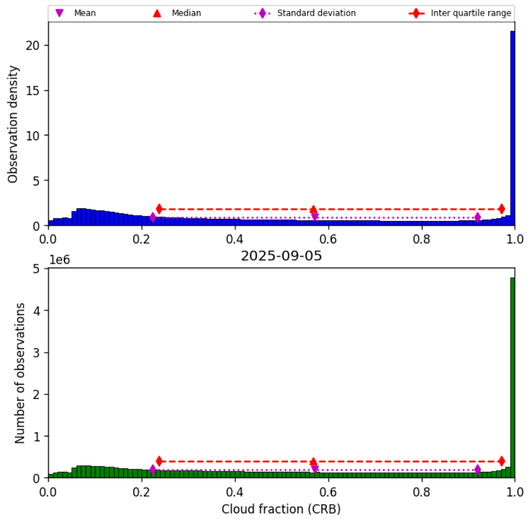
Figure 42: Histogram of “Cloud fraction (CRB)” for 2025-09-04 to 2025-09-06
