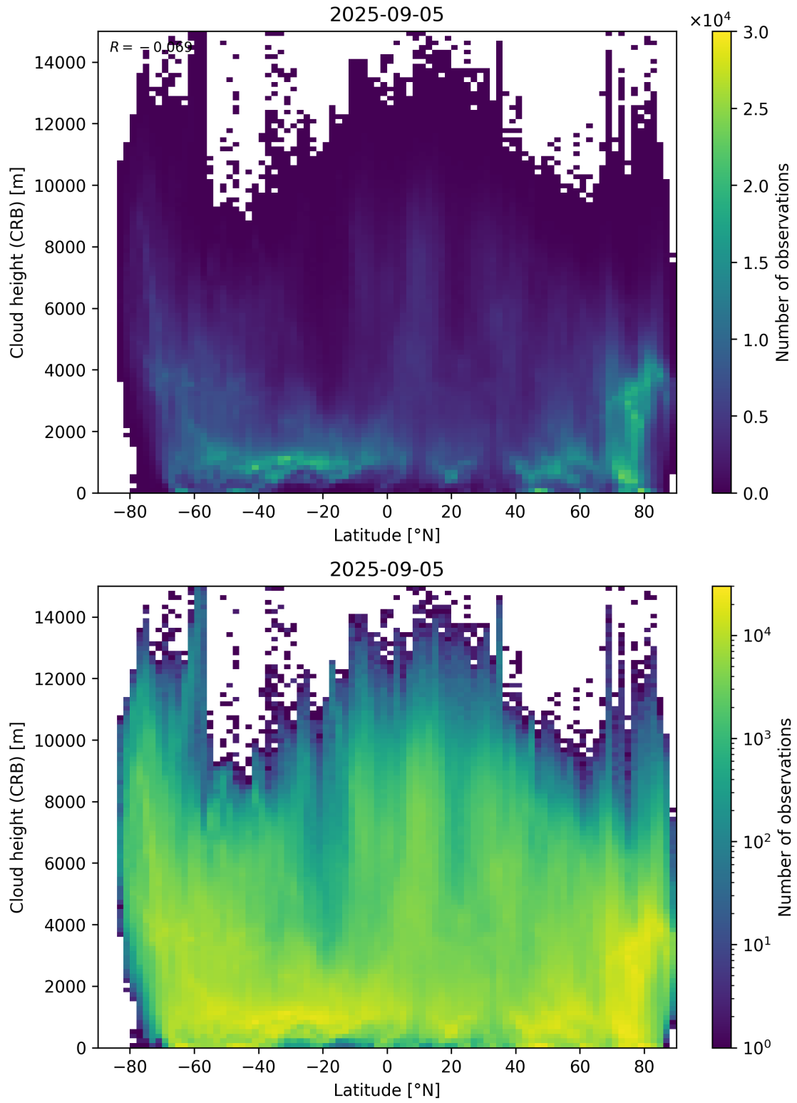
Figure 95: Scatter density plot of “Latitude” against “Cloud height (CRB)” for 2025-09-04 to 2025-09-06.
