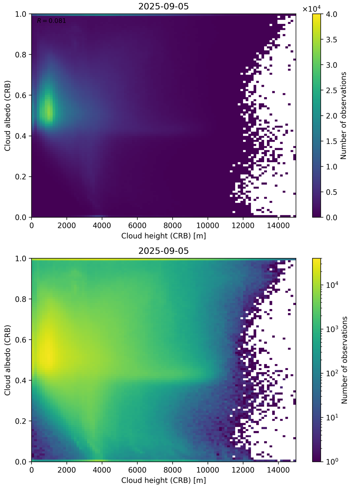
Figure 80: Scatter density plot of “Cloud height (CRB)” against “Cloud albedo (CRB)” for 2025-09-04 to 2025-09-06.
