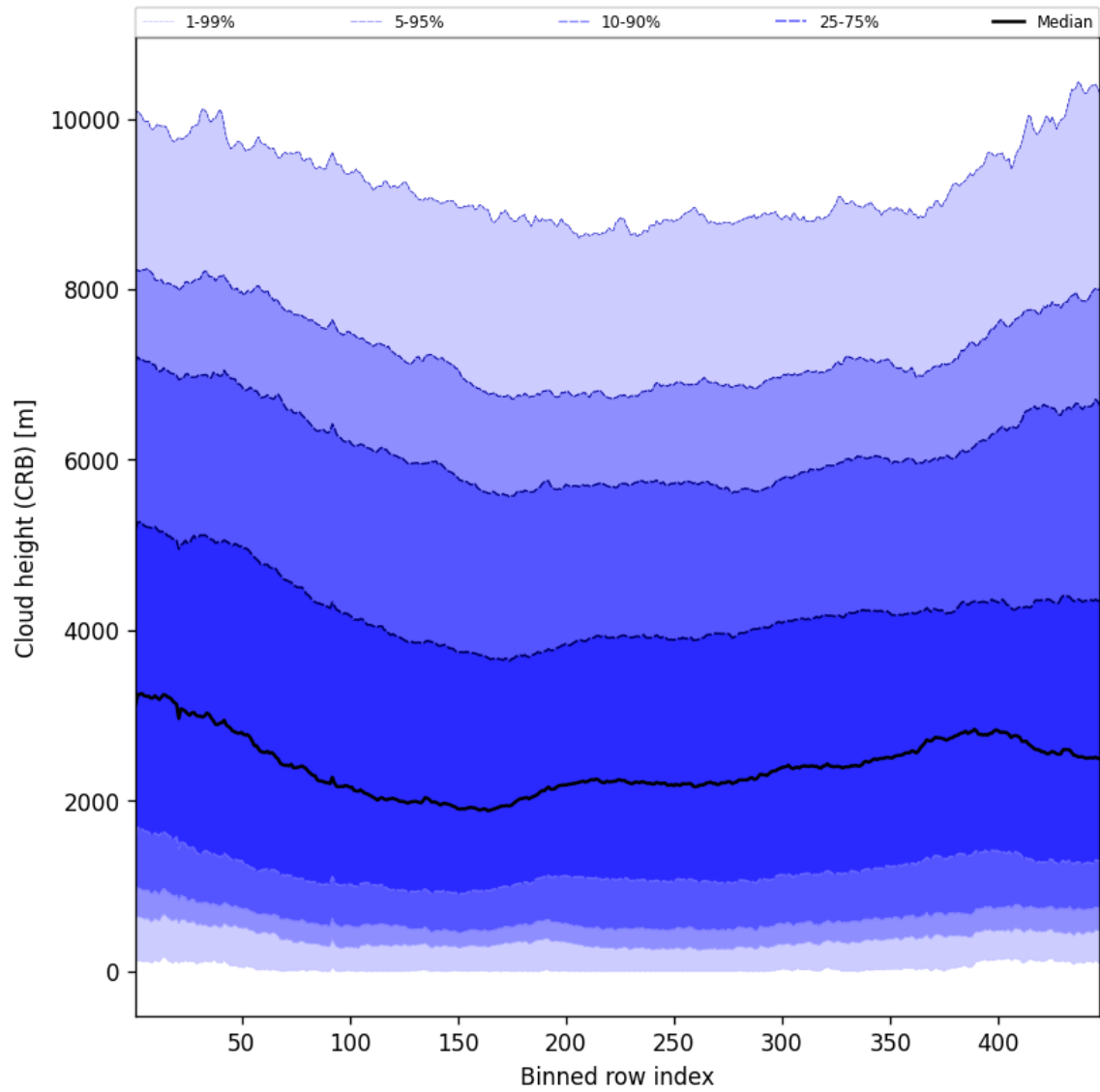
Figure 59: Along track statistics of “Cloud height (CRB)” for 2025-09-04 to 2025-09-06
