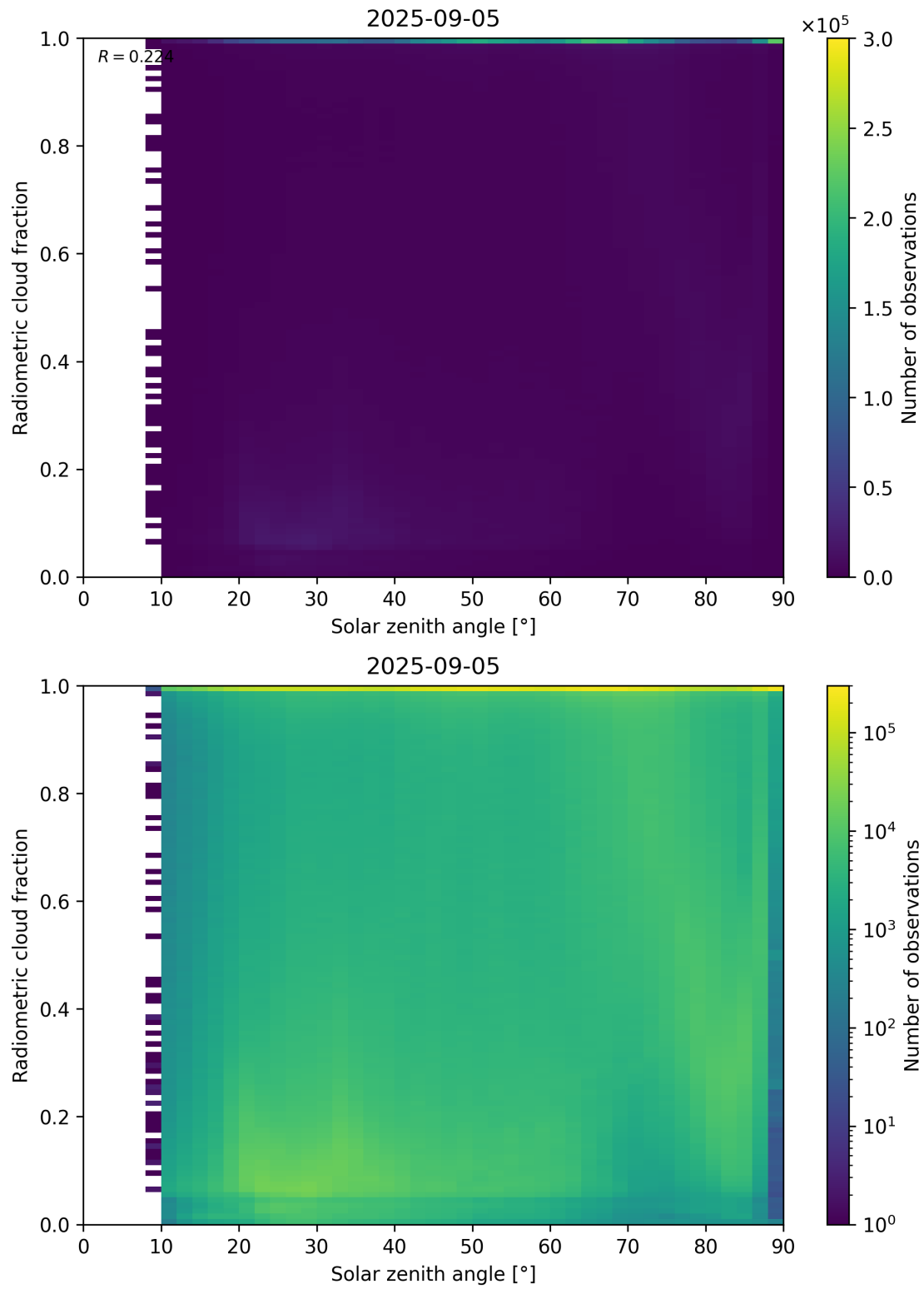
Figure 99: Scatter density plot of “Solar zenith angle” against “Radiometric cloud fraction” for 2025-09-04 to 2025-09-06.
