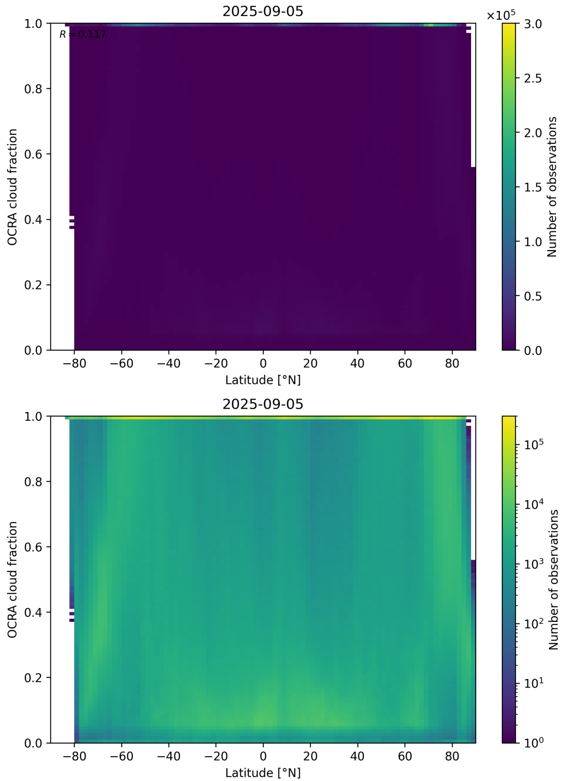
Figure 93: Scatter density plot of “Latitude” against “OCRA cloud fraction” for 2025-09-04 to 2025-09-06.
