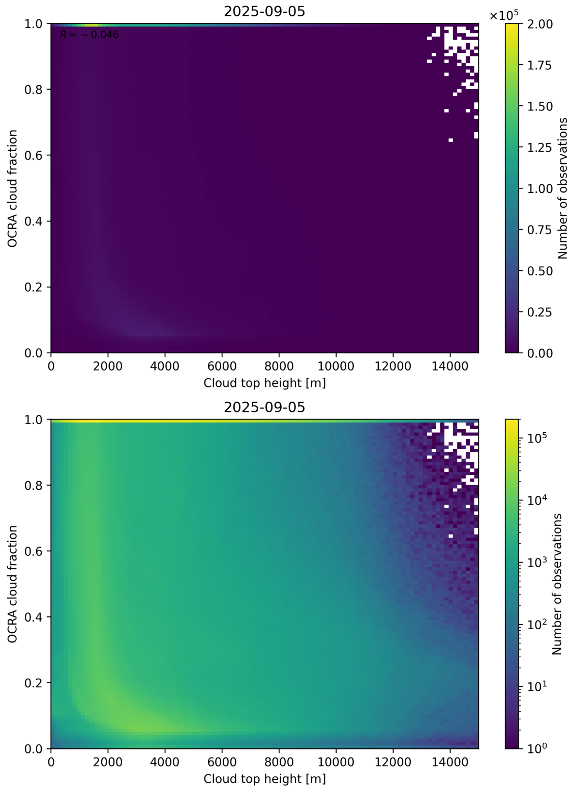
Figure 87: Scatter density plot of “Cloud top height” against “OCRA cloud fraction” for 2025-09-04 to 2025-09-06.
