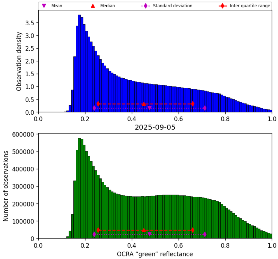
Figure 52: Histogram of “OCRA “green” reflectance” for 2025-09-04 to 2025-09-06
