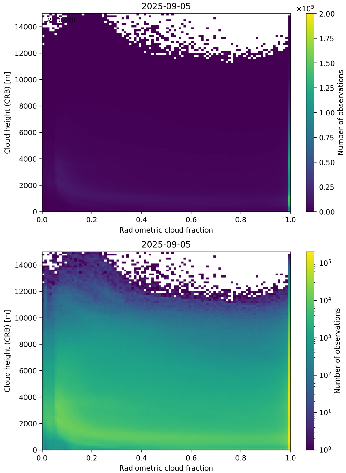
Figure 74: Scatter density plot of “Radiometric cloud fraction” against “Cloud height (CRB)” for 2025-09-04 to 2025-09-06.
