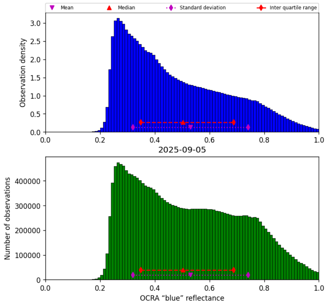
Figure 51: Histogram of “OCRA “blue” reflectance” for 2025-09-04 to 2025-09-06
