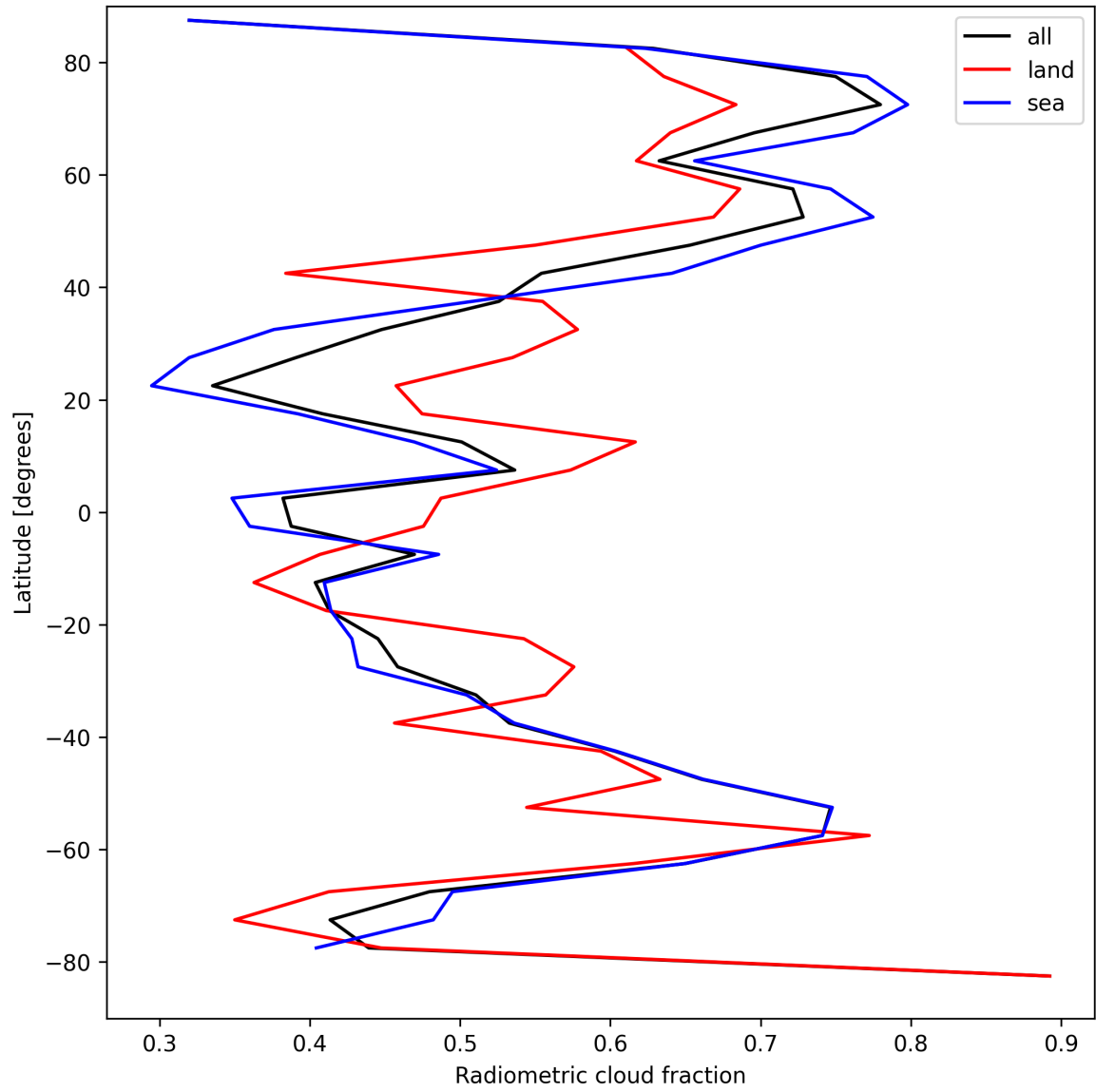
Figure 23: Zonal average of “Radiometric cloud fraction” for 2025-09-04 to 2025-09-06.
