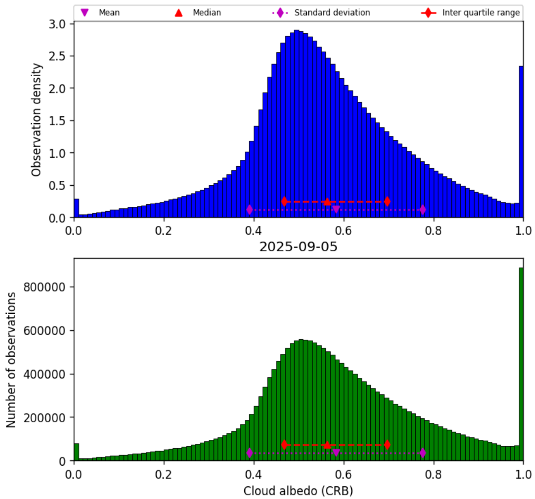
Figure 44: Histogram of “Cloud albedo (CRB)” for 2025-09-04 to 2025-09-06
