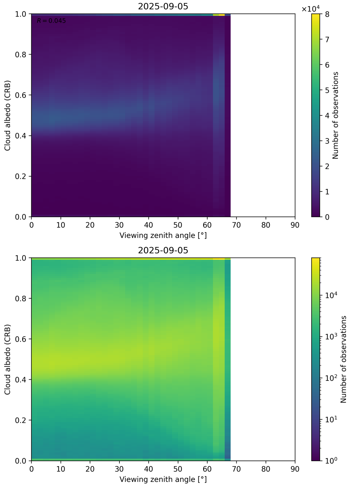
Figure 106: Scatter density plot of “Viewing zenith angle” against “Cloud albedo (CRB)” for 2025-09-04 to 2025-09-06.
