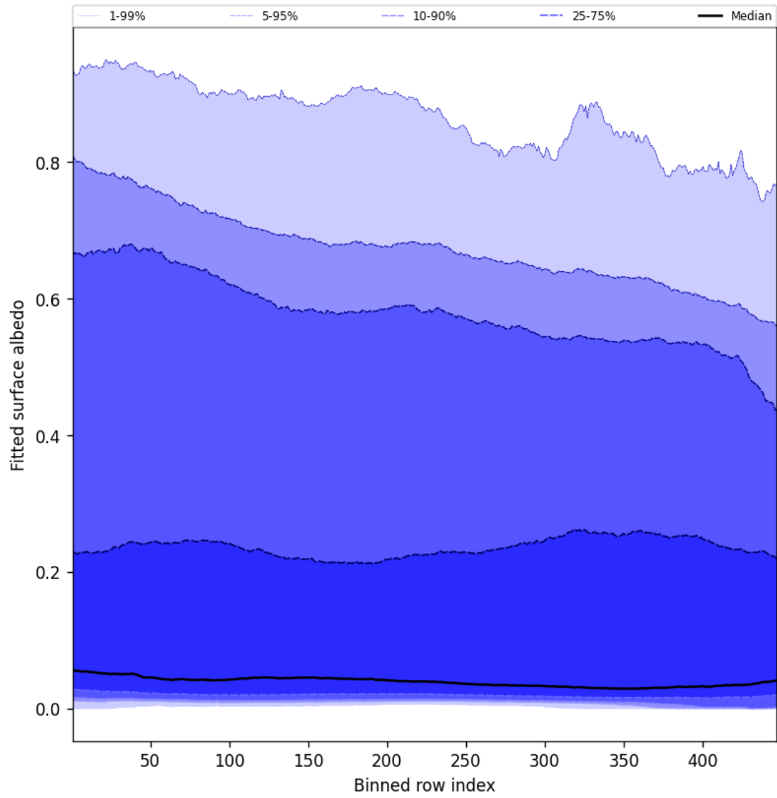
Figure 61: Along track statistics of “Fitted surface albedo” for 2025-09-04 to 2025-09-06
