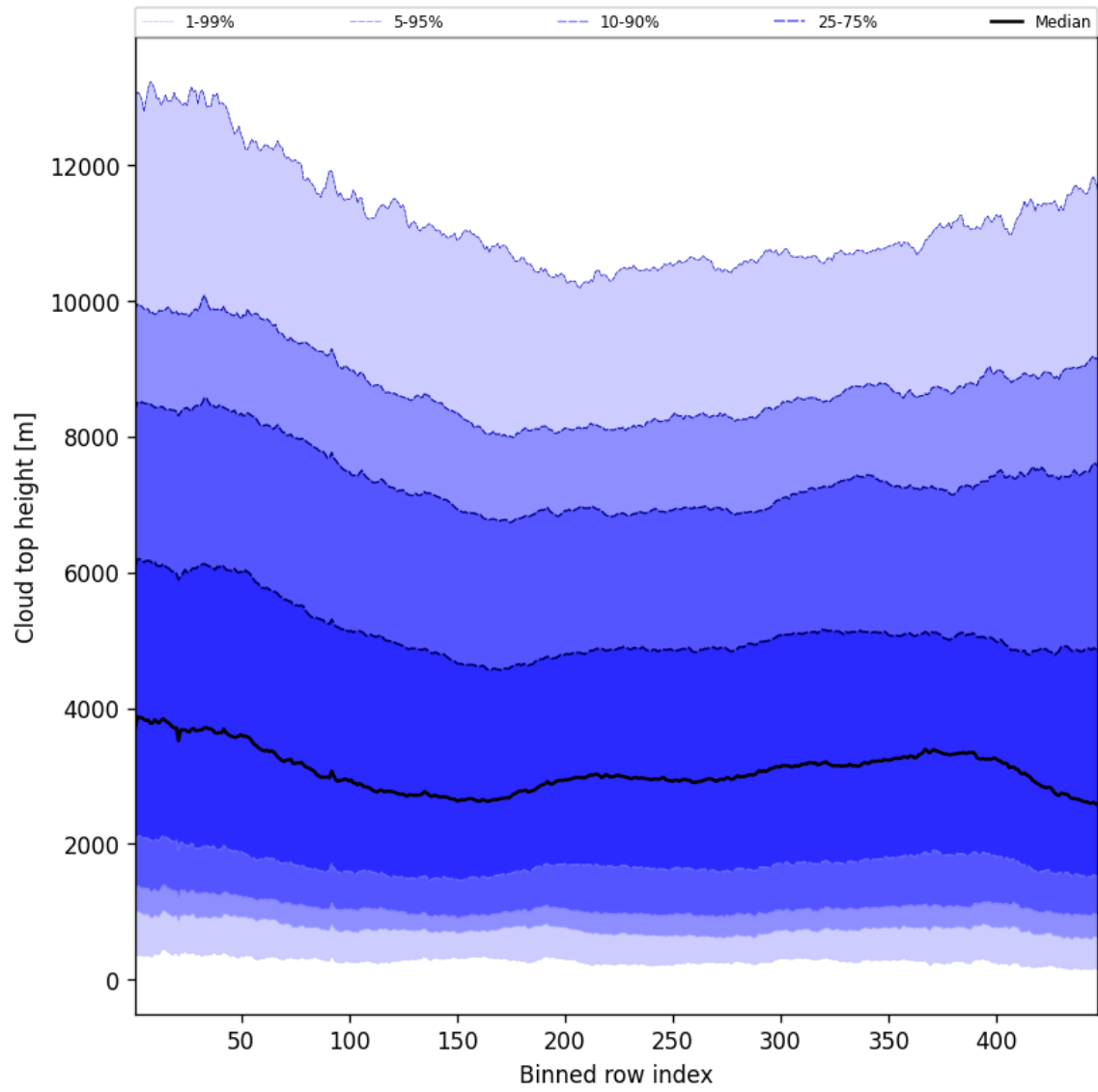
Figure 56: Along track statistics of “Cloud top height” for 2025-09-04 to 2025-09-06
