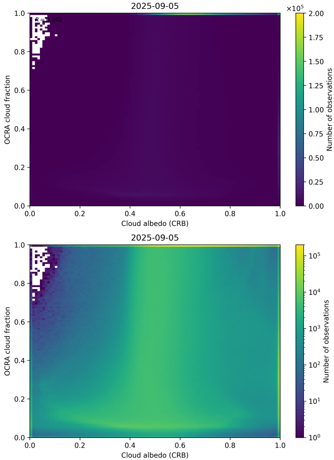
Figure 70: Scatter density plot of “Cloud albedo (CRB)” against “OCRA cloud fraction” for 2025-09-04 to 2025-09-06.
