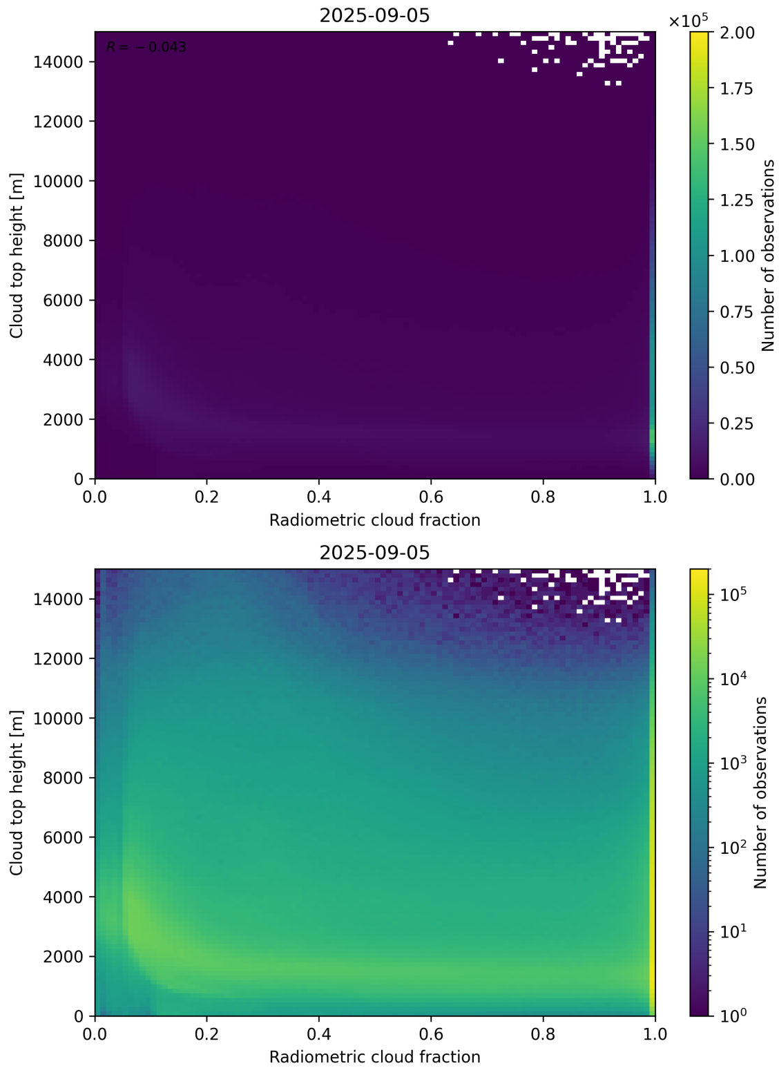
Figure 76: Scatter density plot of “Radiometric cloud fraction” against “Cloud top height” for 2025-09-04 to 2025-09-06.
