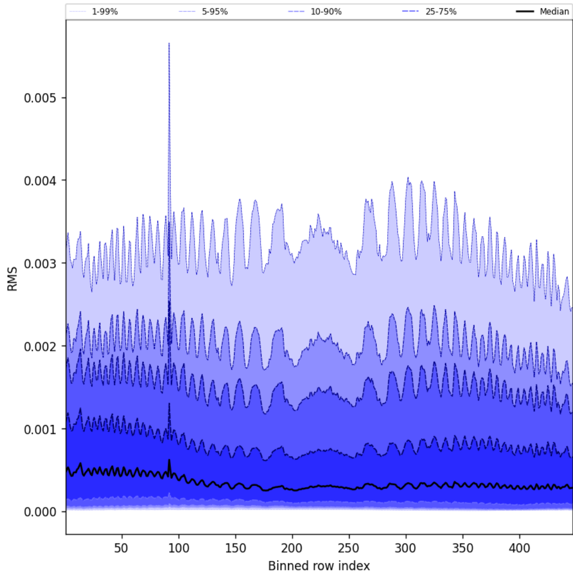
Figure 63: Along track statistics of “RMS” for 2025-09-04 to 2025-09-06
