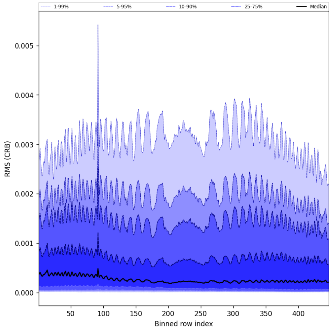
Figure 64: Along track statistics of “RMS (CRB)” for 2025-09-04 to 2025-09-06
