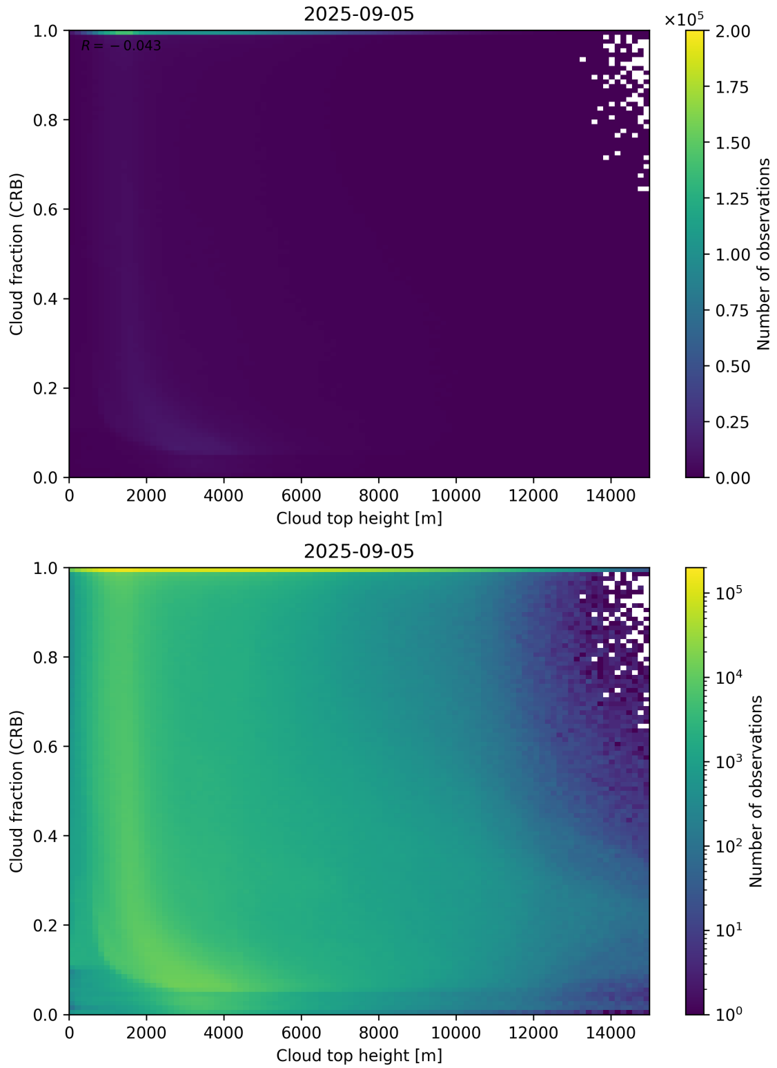
Figure 88: Scatter density plot of “Cloud top height” against “Cloud fraction (CRB)” for 2025-09-04 to 2025-09-06.
