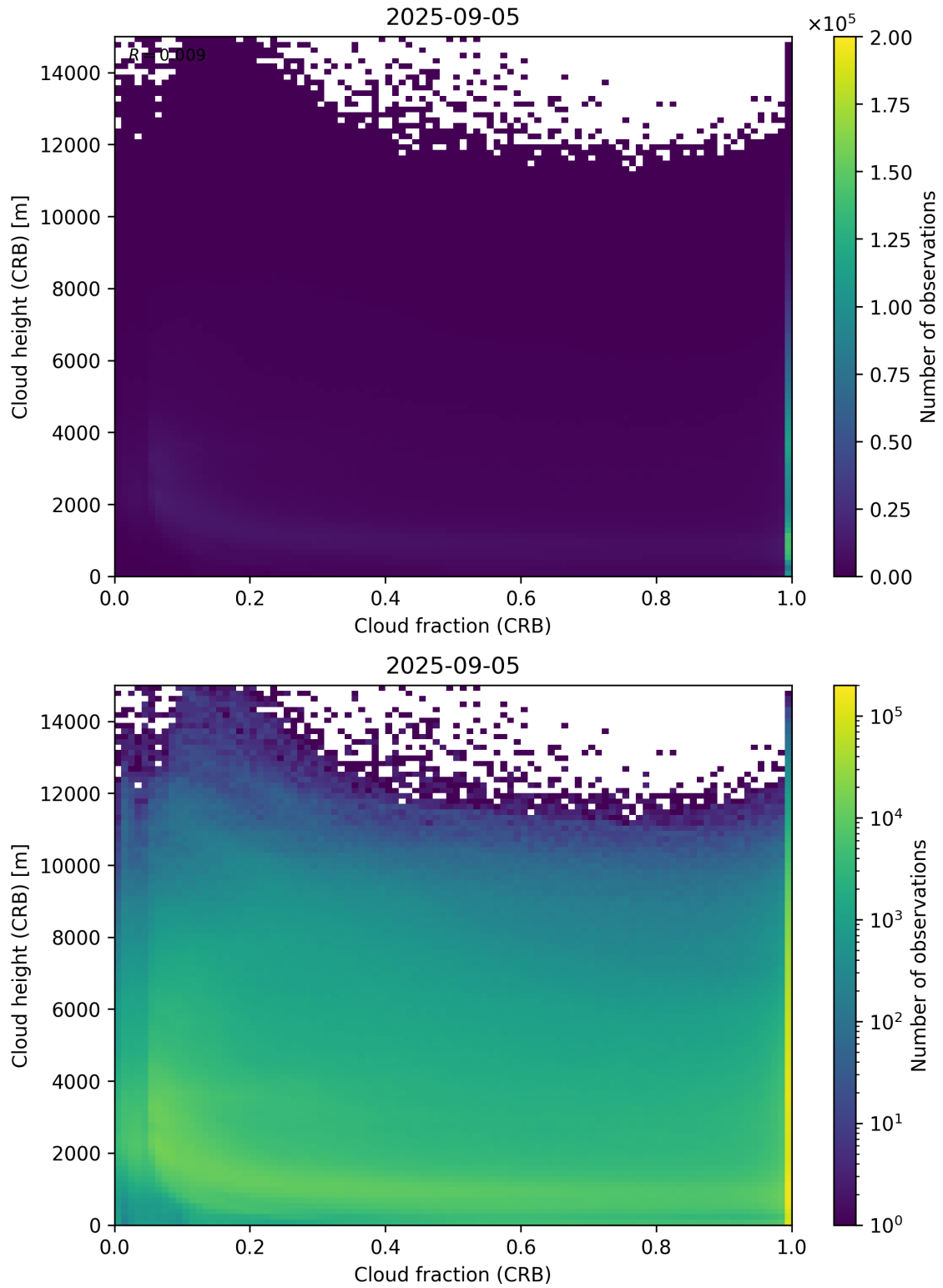
Figure 79: Scatter density plot of “Cloud fraction (CRB)” against “Cloud height (CRB)” for 2025-09-04 to 2025-09-06.
