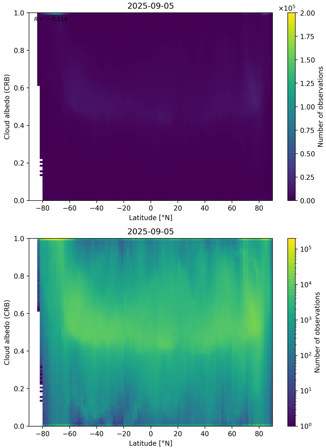
Figure 91: Scatter density plot of “Latitude” against “Cloud albedo (CRB)” for 2025-09-04 to 2025-09-06.
