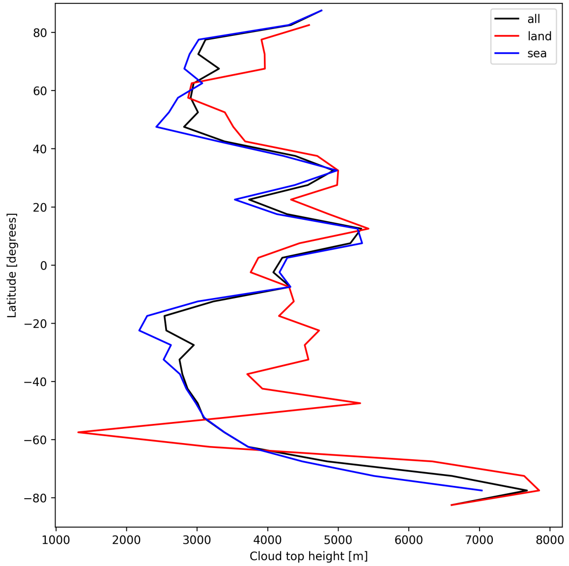
Figure 24: Zonal average of “Cloud top height” for 2025-09-04 to 2025-09-06.
