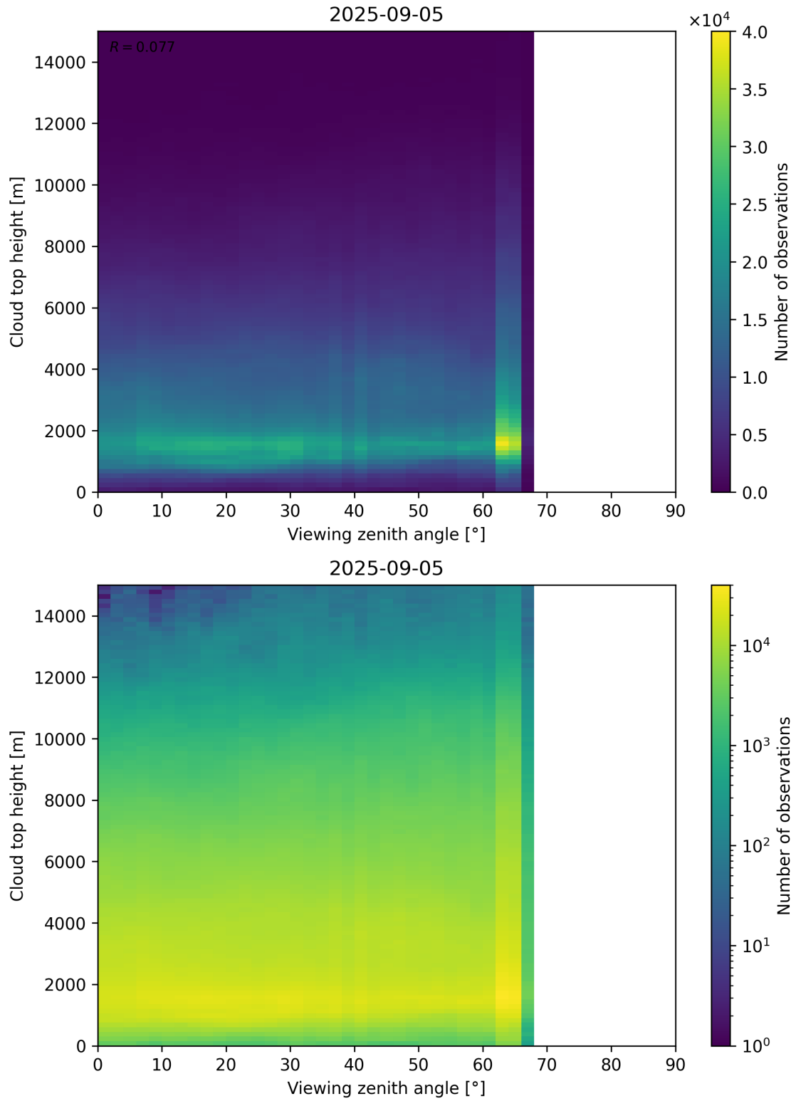
Figure 112: Scatter density plot of “Viewing zenith angle” against “Cloud top height” for 2025-09-04 to 2025-09-06.
