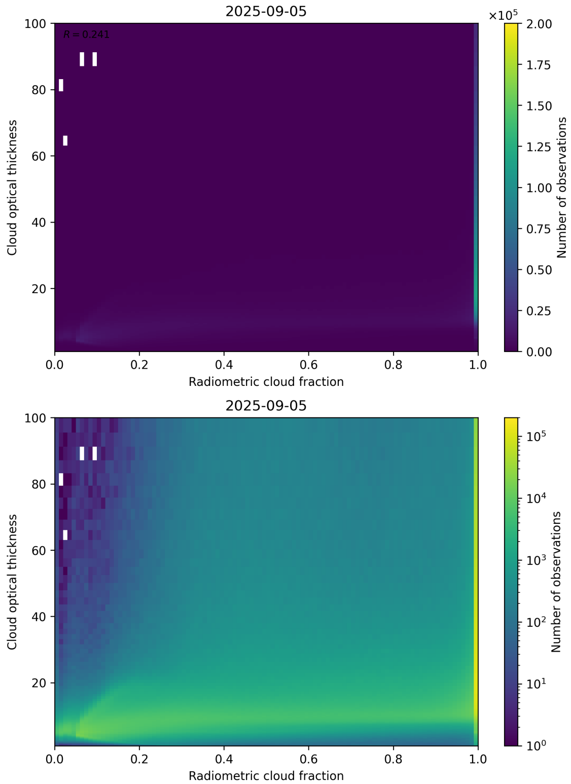
Figure 75: Scatter density plot of “Radiometric cloud fraction” against “Cloud optical thickness” for 2025-09-04 to 2025-09-06.
