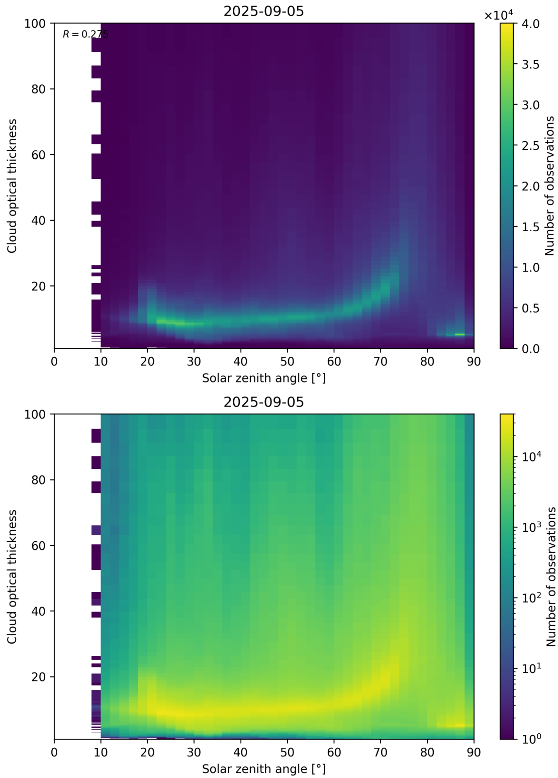
Figure 103: Scatter density plot of “Solar zenith angle” against “Cloud optical thickness” for 2025-09-04 to 2025-09-06.
