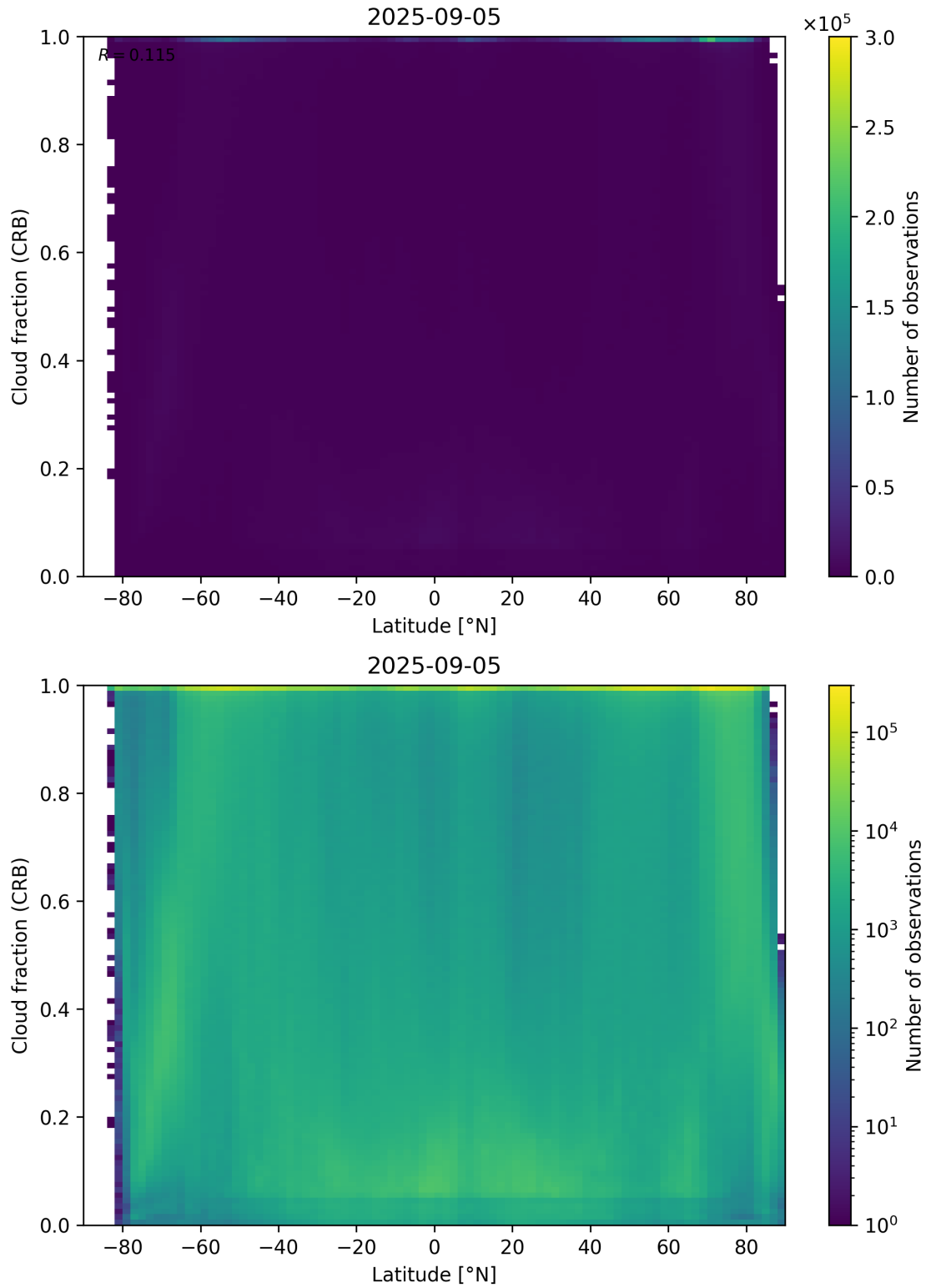
Figure 94: Scatter density plot of “Latitude” against “Cloud fraction (CRB)” for 2025-09-04 to 2025-09-06.
