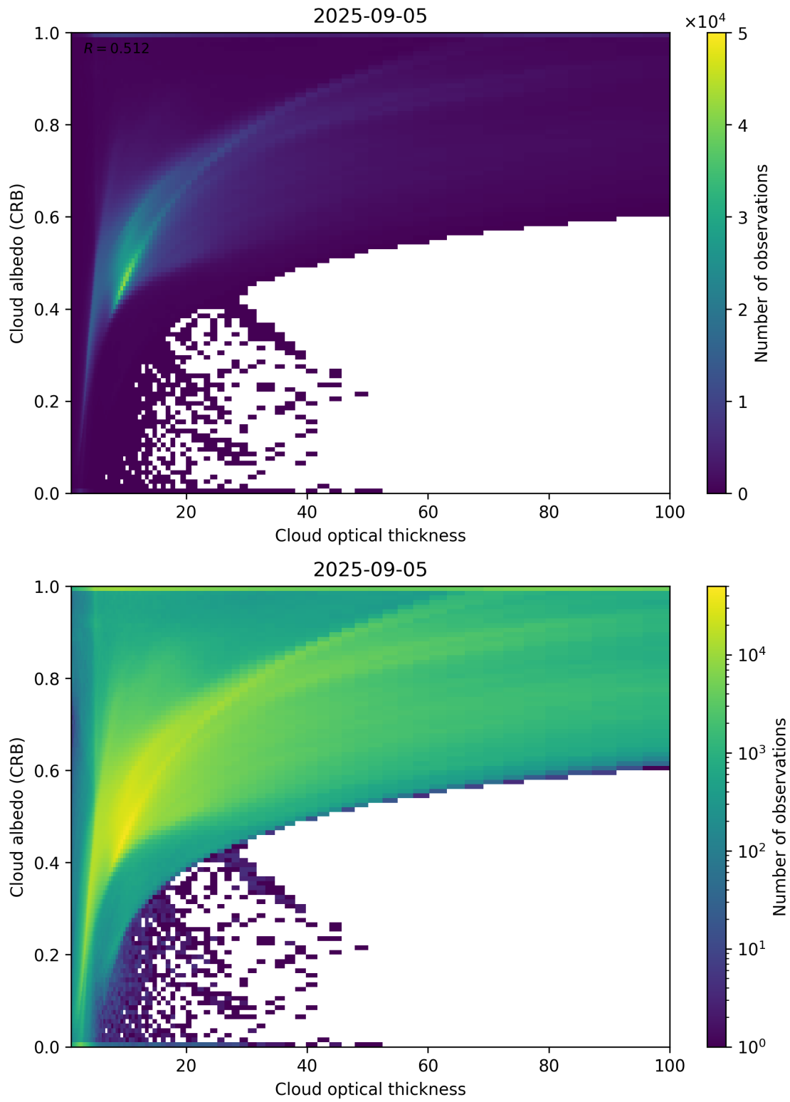
Figure 82: Scatter density plot of “Cloud optical thickness” against “Cloud albedo (CRB)” for 2025-09-04 to 2025-09-06.
