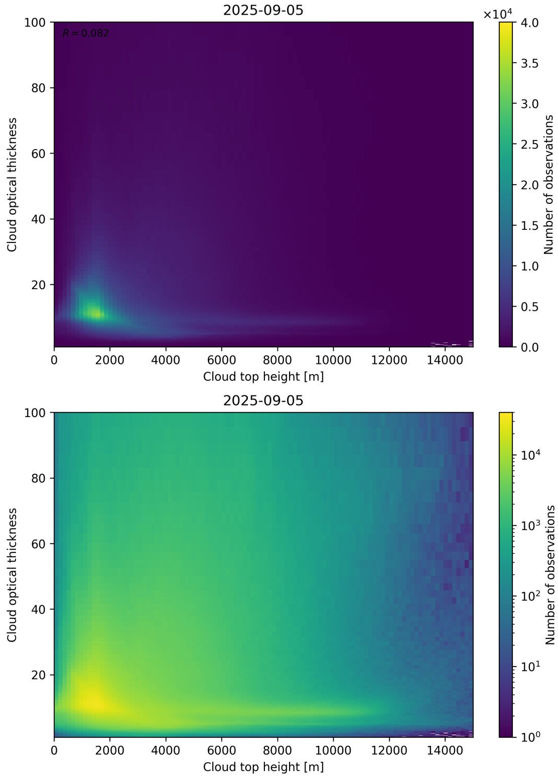
Figure 90: Scatter density plot of “Cloud top height” against “Cloud optical thickness” for 2025-09-04 to 2025-09-06.
