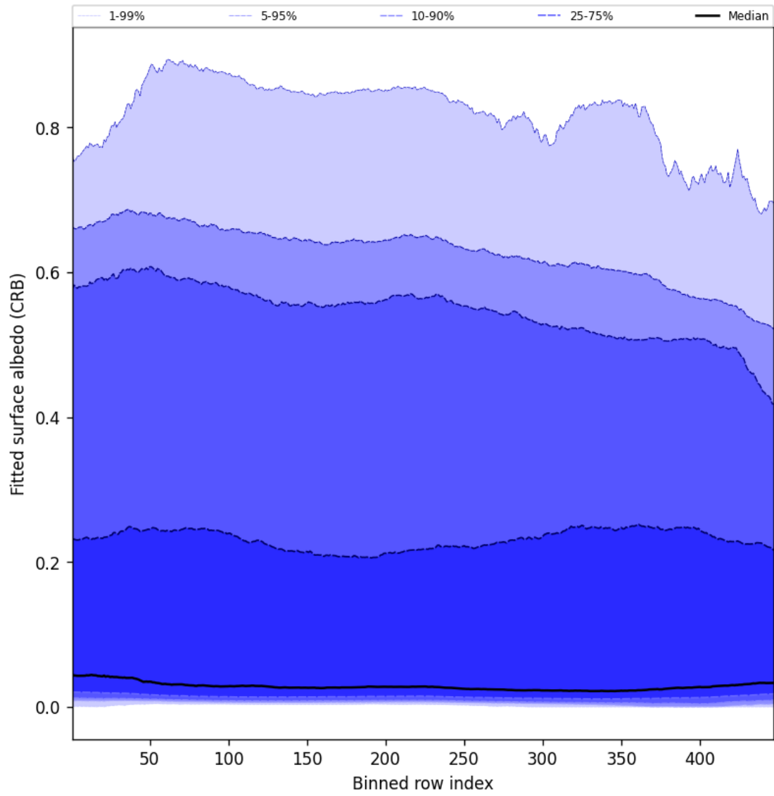
Figure 62: Along track statistics of “Fitted surface albedo (CRB)” for 2025-09-04 to 2025-09-06
