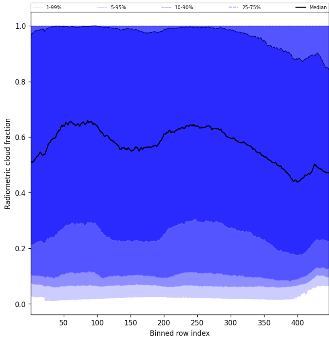
Figure 55: Along track statistics of “Radiometric cloud fraction” for 2025-09-04 to 2025-09-06
