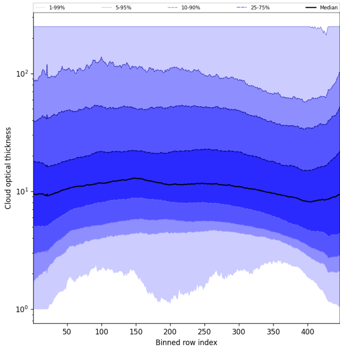
Figure 57: Along track statistics of “Cloud optical thickness” for 2025-09-04 to 2025-09-06
