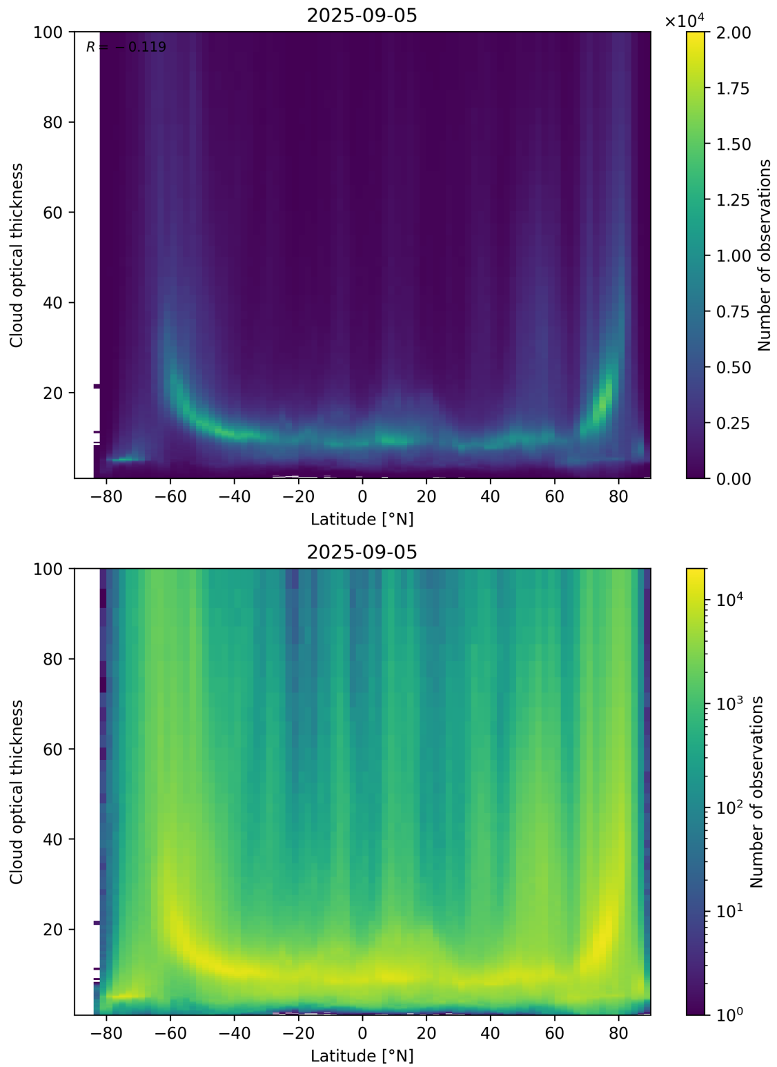
Figure 96: Scatter density plot of “Latitude” against “Cloud optical thickness” for 2025-09-04 to 2025-09-06.
