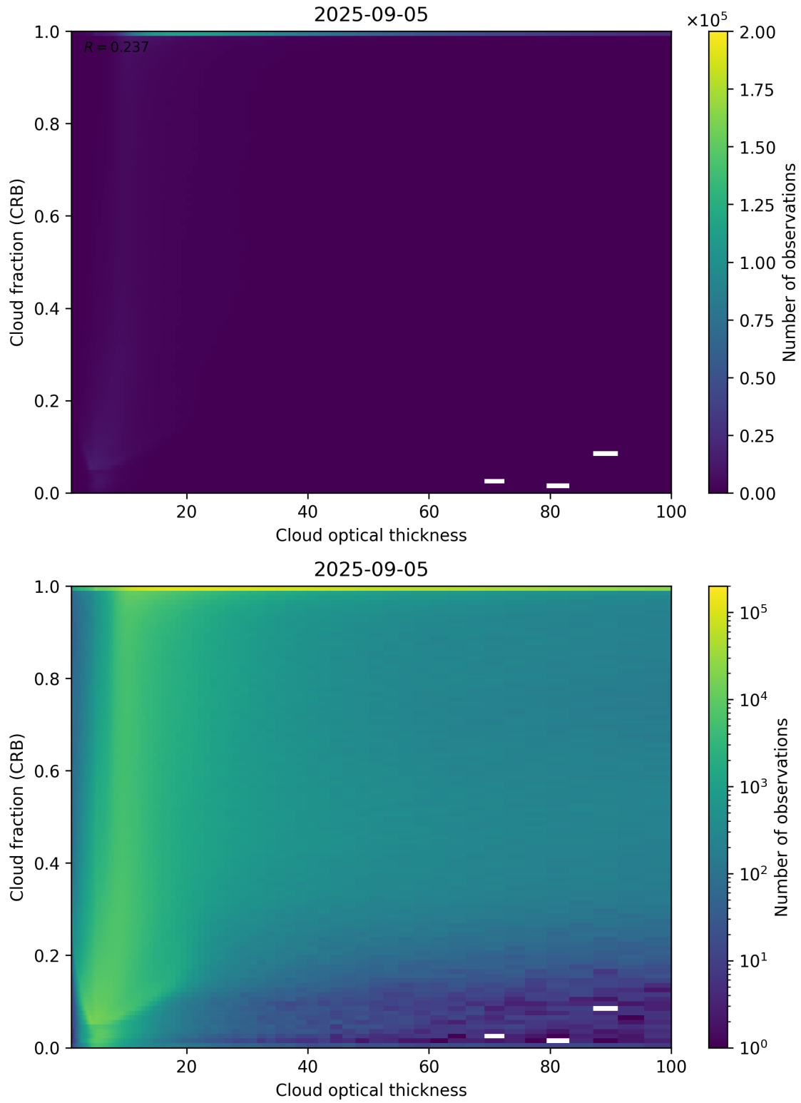
Figure 84: Scatter density plot of “Cloud optical thickness” against “Cloud fraction (CRB)” for 2025-09-04 to 2025-09-06.
