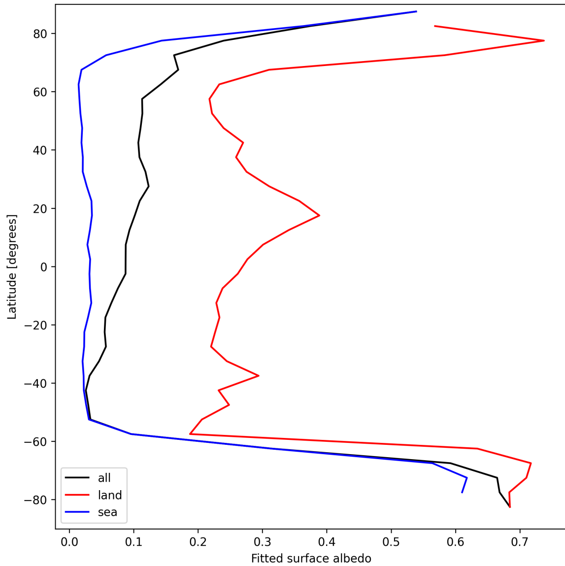
Figure 29: Zonal average of “Fitted surface albedo” for 2025-09-04 to 2025-09-06.
