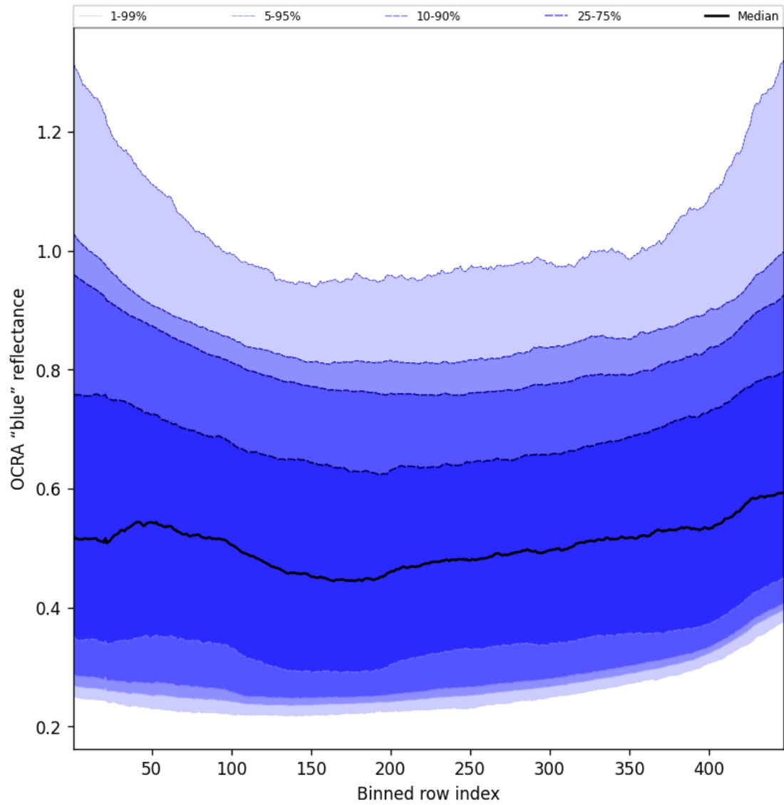
Figure 67: Along track statistics of “OCRA “blue” reflectance” for 2025-09-04 to 2025-09-06
