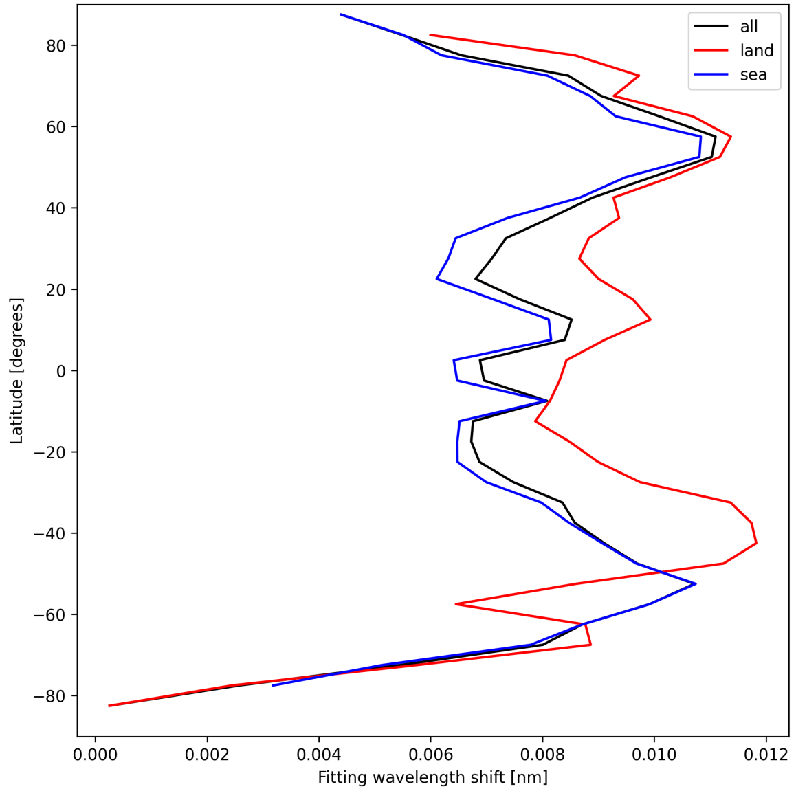
Figure 33: Zonal average of “Fitting wavelength shift” for 2025-09-04 to 2025-09-06.
