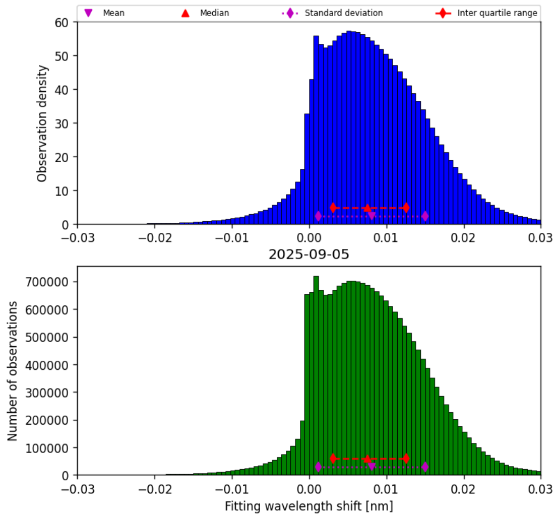
Figure 49: Histogram of “Fitting wavelength shift” for 2025-09-04 to 2025-09-06
