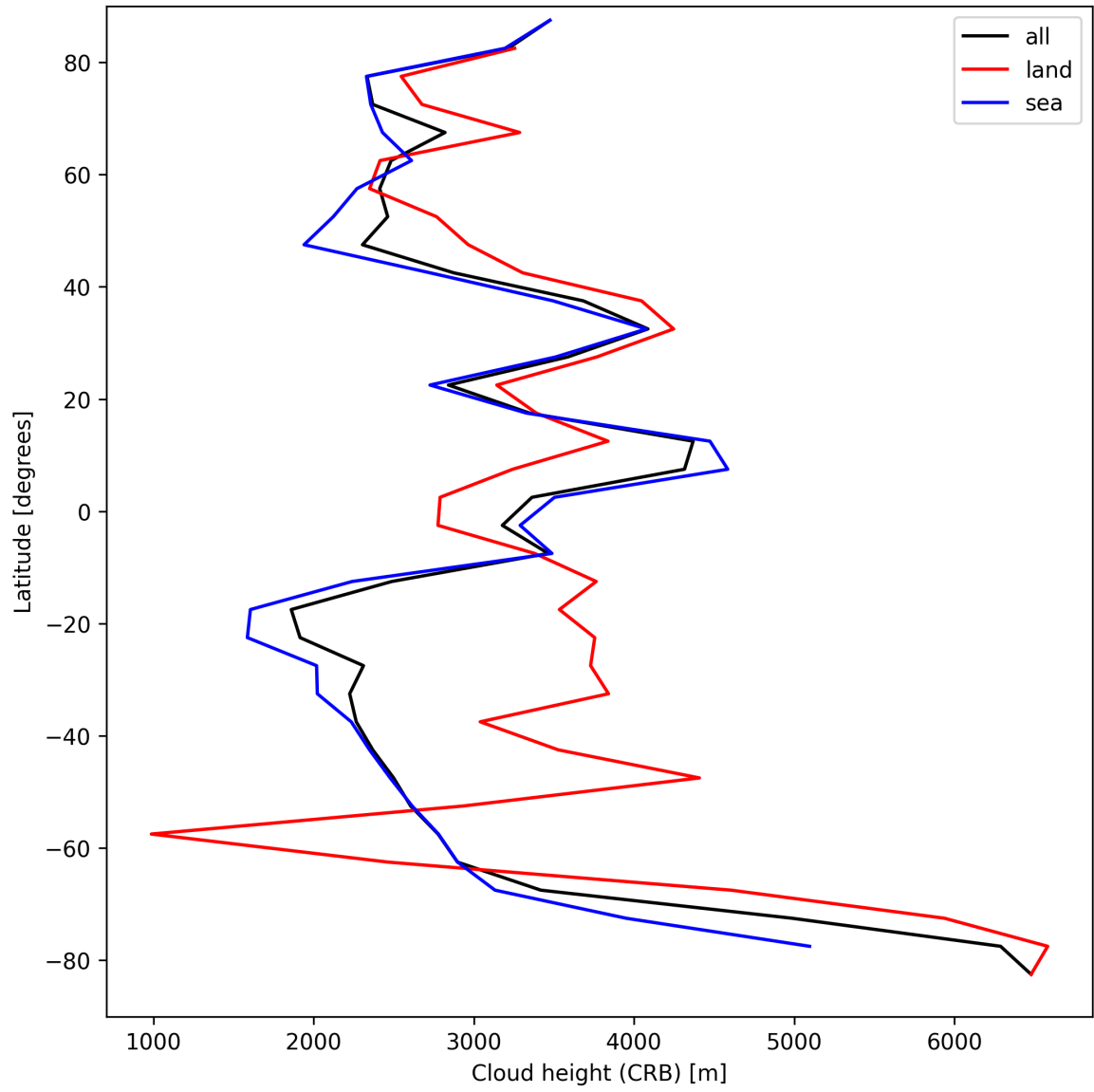
Figure 27: Zonal average of “Cloud height (CRB)” for 2025-09-04 to 2025-09-06.
