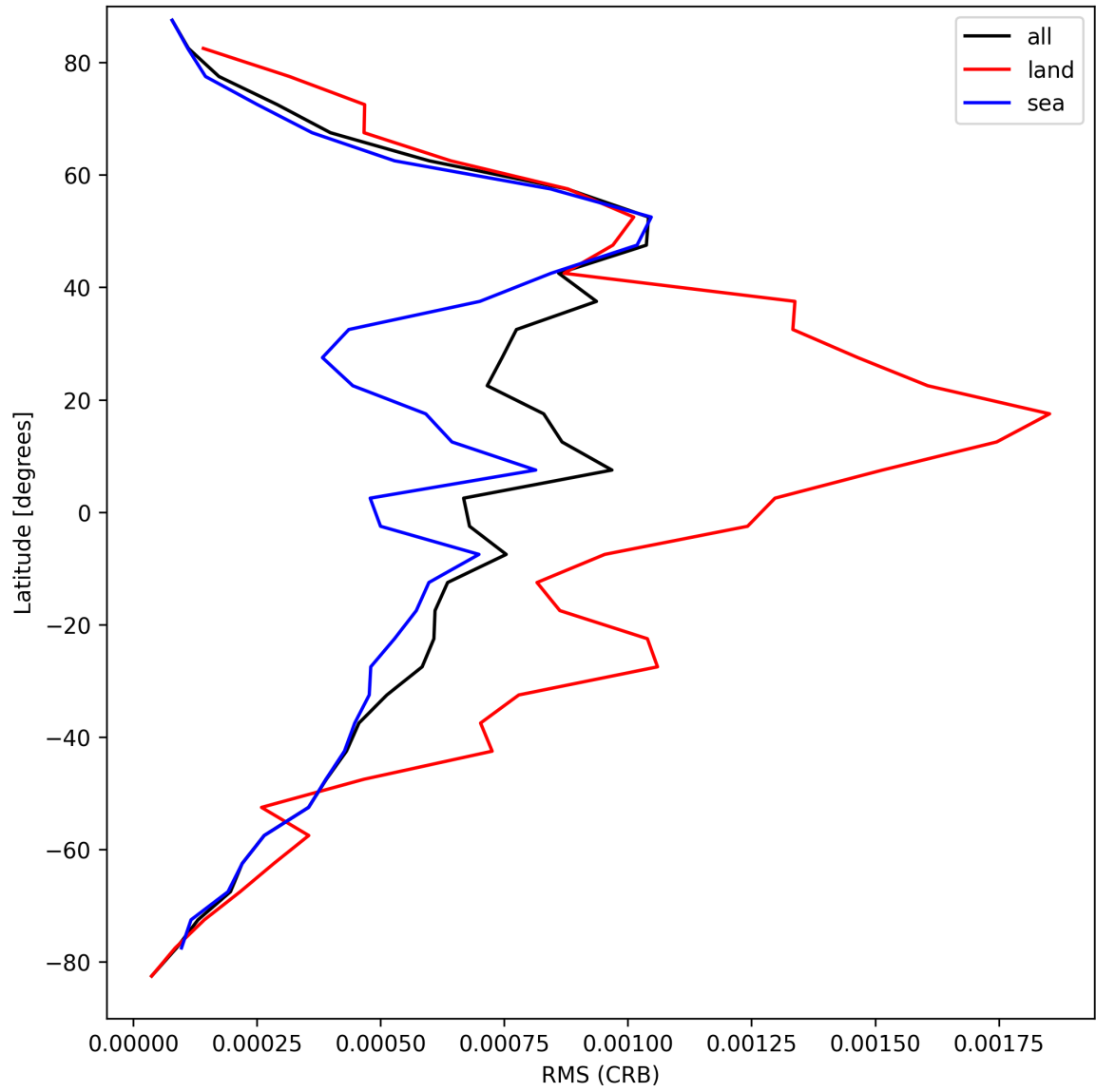
Figure 32: Zonal average of “RMS (CRB)” for 2025-09-04 to 2025-09-06.
