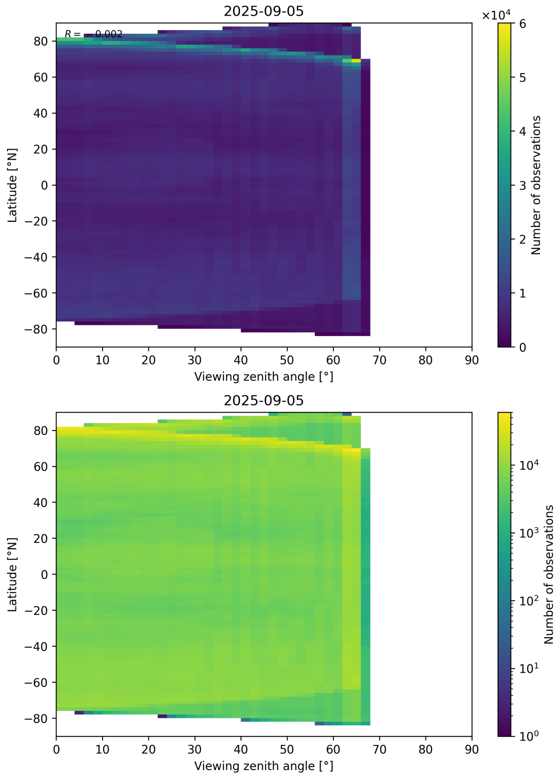
Figure 113: Scatter density plot of “Viewing zenith angle” against “Latitude” for 2025-09-04 to 2025-09-06.
