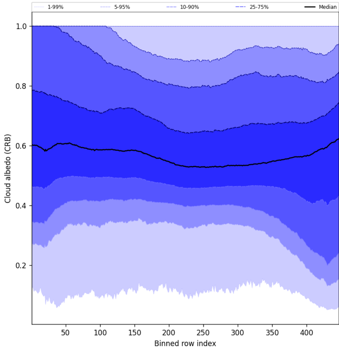
Figure 60: Along track statistics of “Cloud albedo (CRB)” for 2025-09-04 to 2025-09-06
