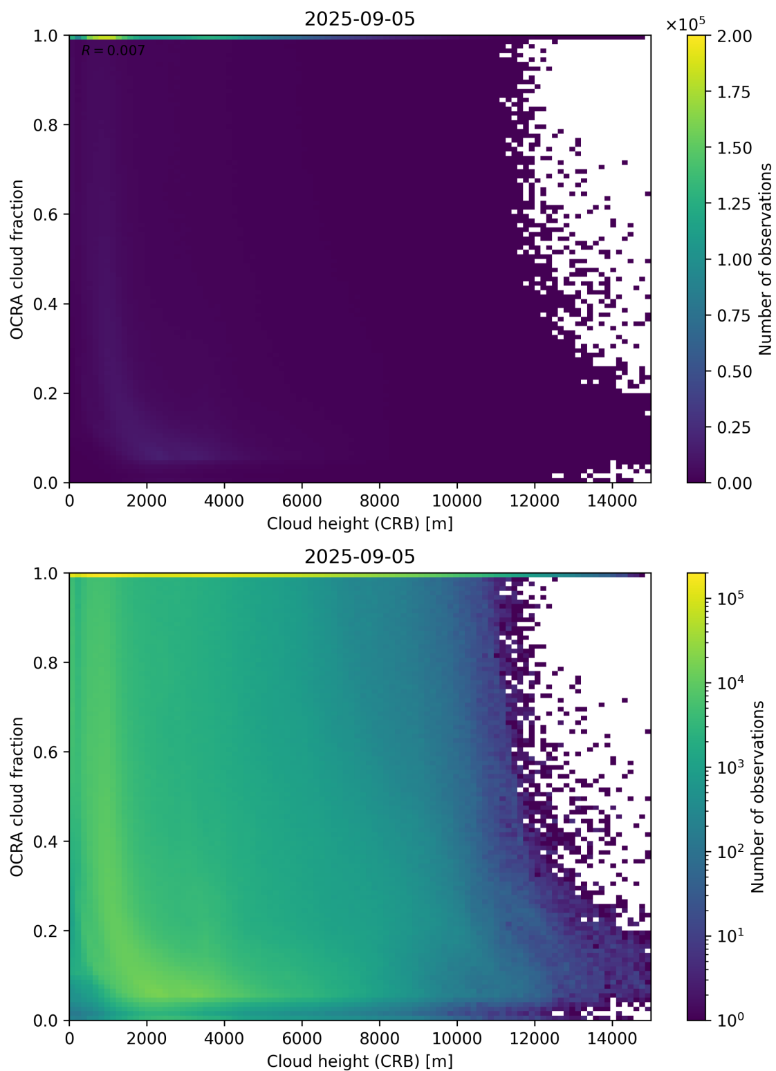
Figure 81: Scatter density plot of “Cloud height (CRB)” against “OCRA cloud fraction” for 2025-09-04 to 2025-09-06.
