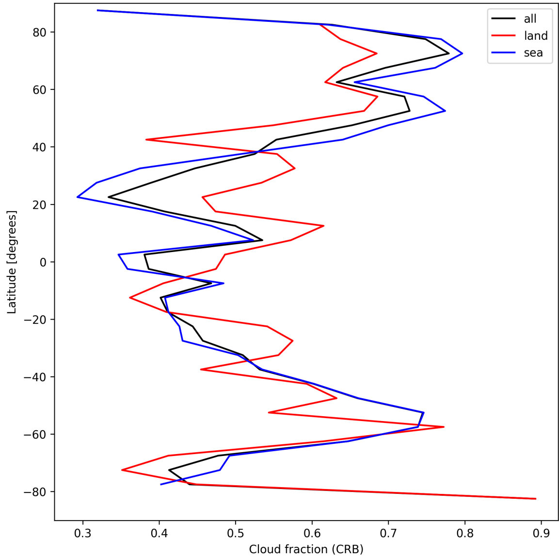
Figure 26: Zonal average of “Cloud fraction (CRB)” for 2025-09-04 to 2025-09-06.
