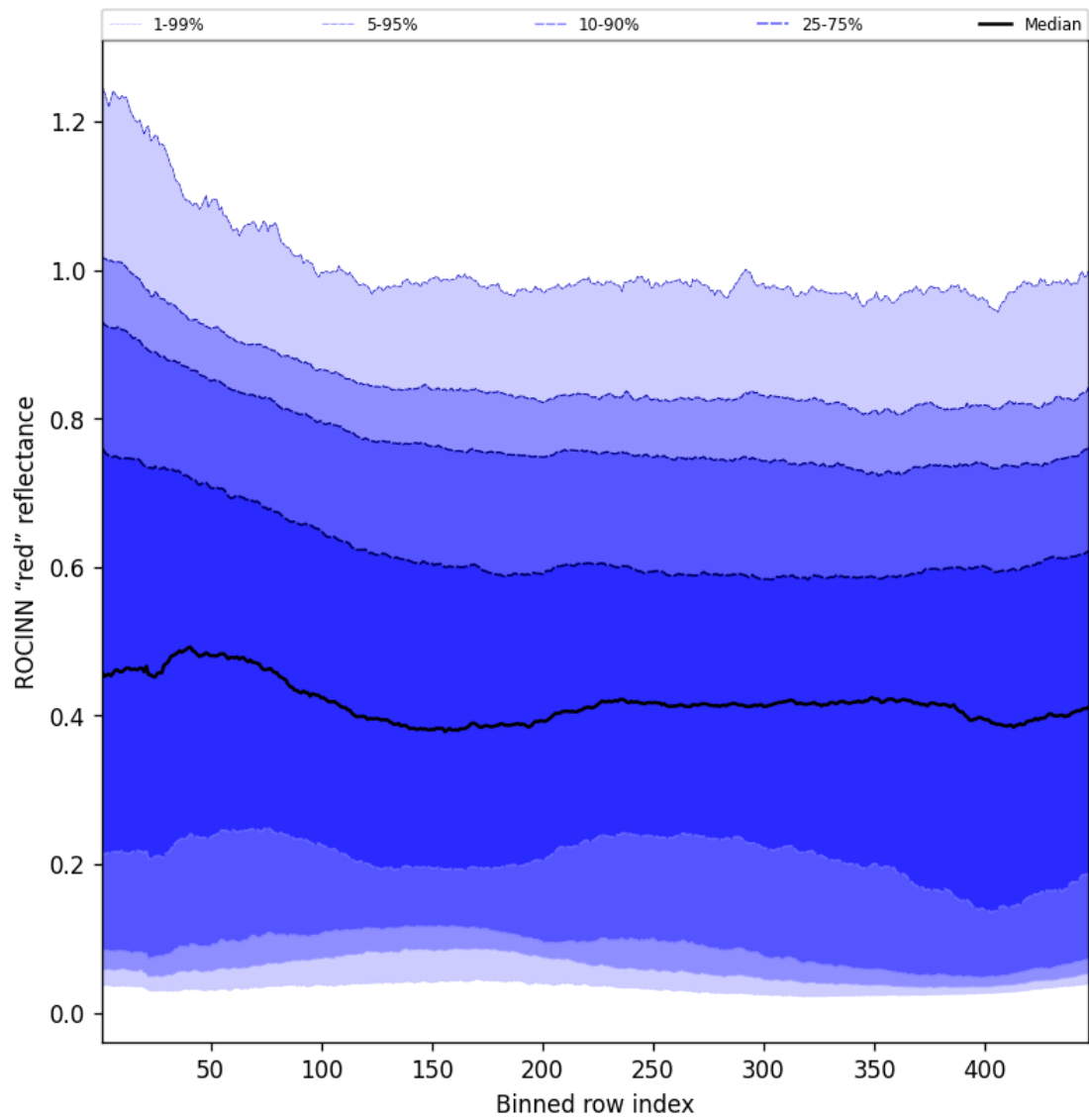
Figure 69: Along track statistics of “ROCINN “red” reflectance” for 2025-09-05 to 2025-09-07
