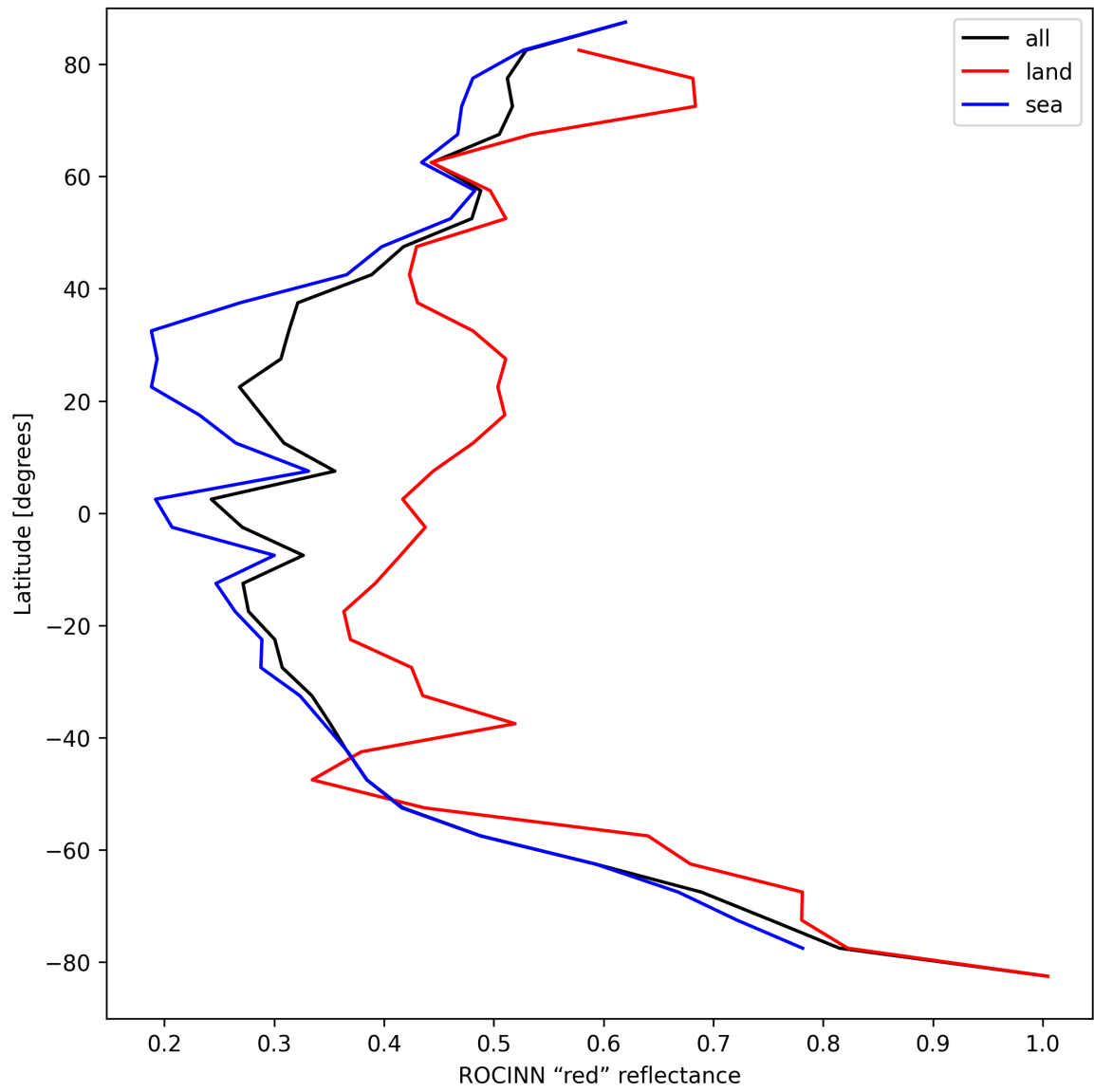
Figure 37: Zonal average of “ROCINN “red” reflectance” for 2025-09-05 to 2025-09-07.
