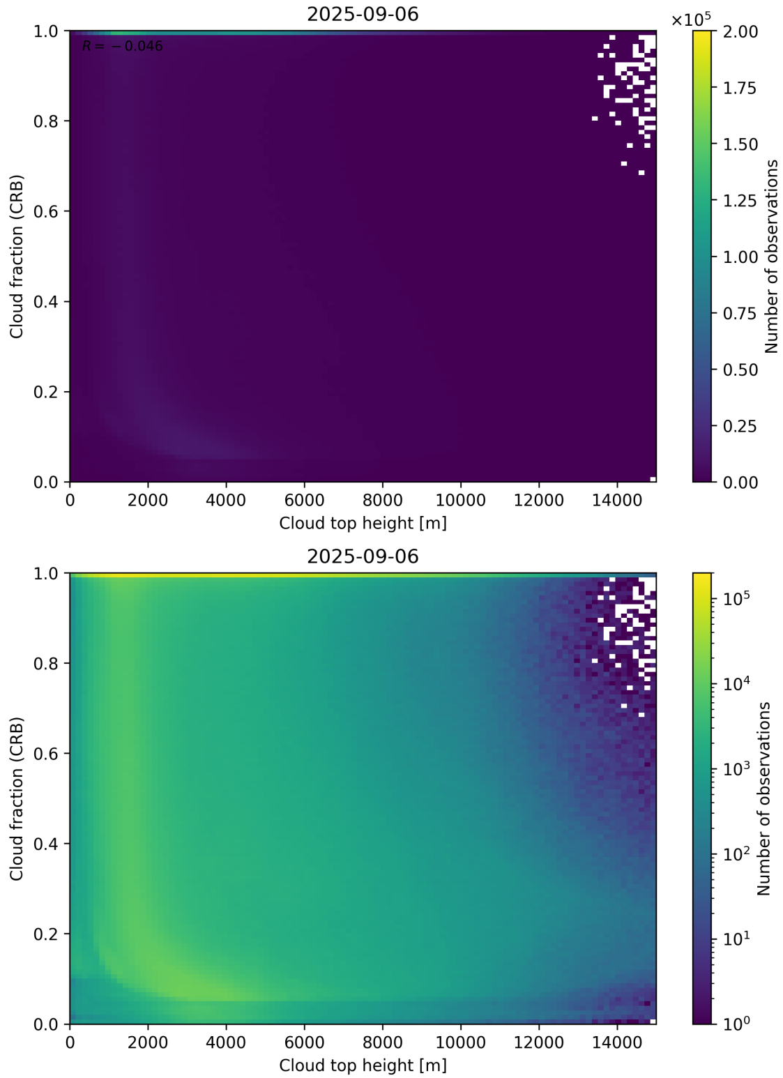
Figure 88: Scatter density plot of “Cloud top height” against “Cloud fraction (CRB)” for 2025-09-05 to 2025-09-07.
