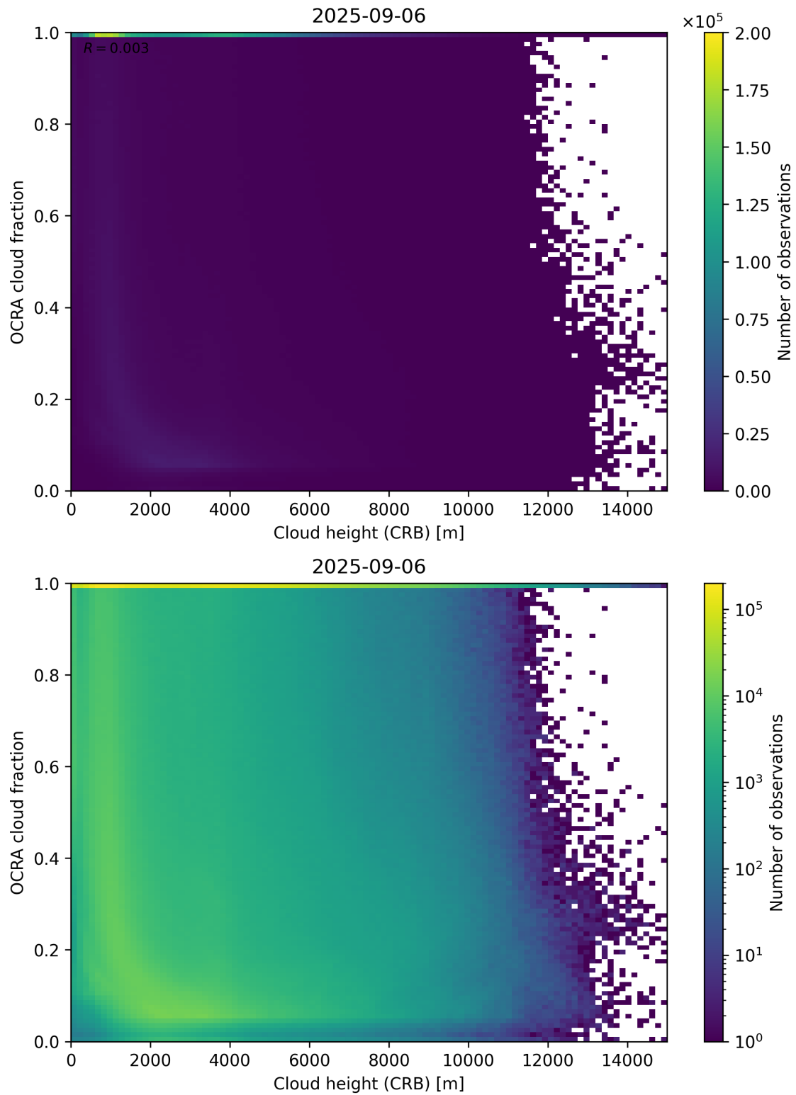
Figure 81: Scatter density plot of “Cloud height (CRB)” against “OCRA cloud fraction” for 2025-09-05 to 2025-09-07.
