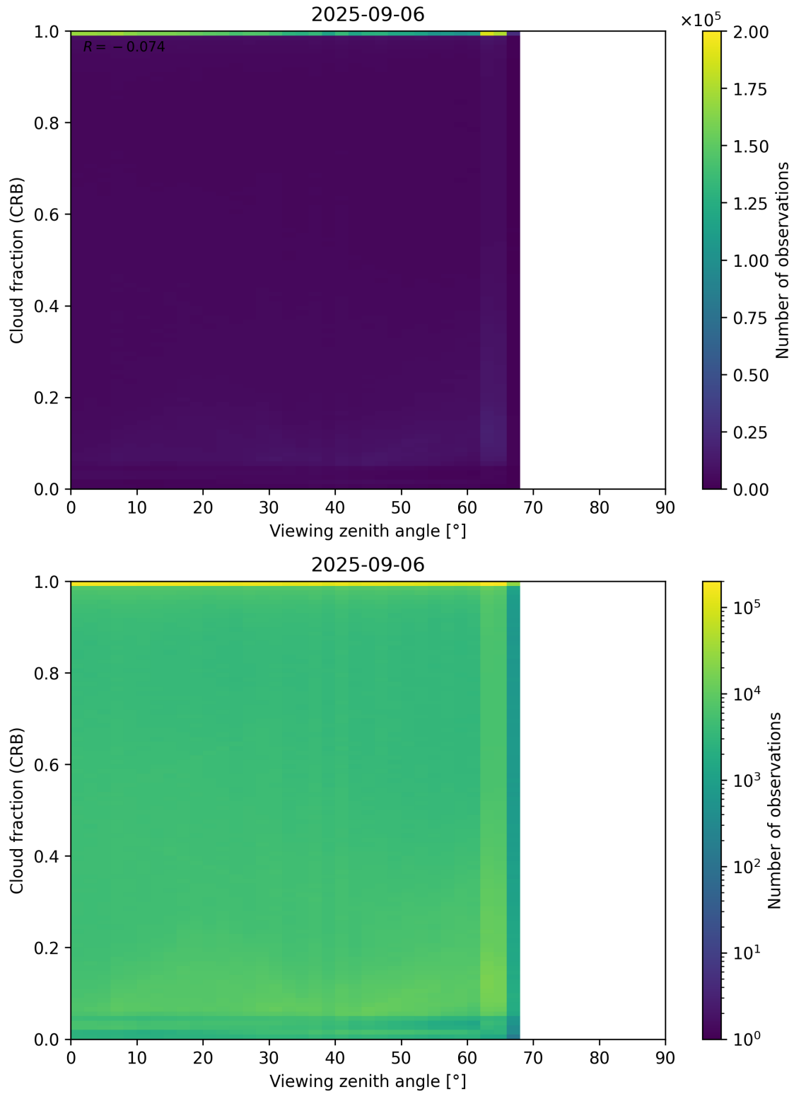
Figure 109: Scatter density plot of “Viewing zenith angle” against “Cloud fraction (CRB)” for 2025-09-05 to 2025-09-07.
