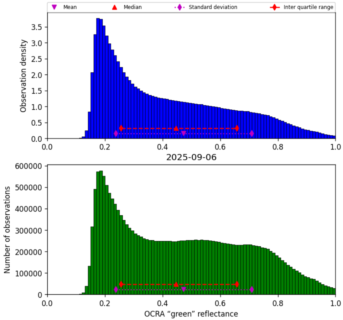
Figure 52: Histogram of “OCRA “green” reflectance” for 2025-09-05 to 2025-09-07
