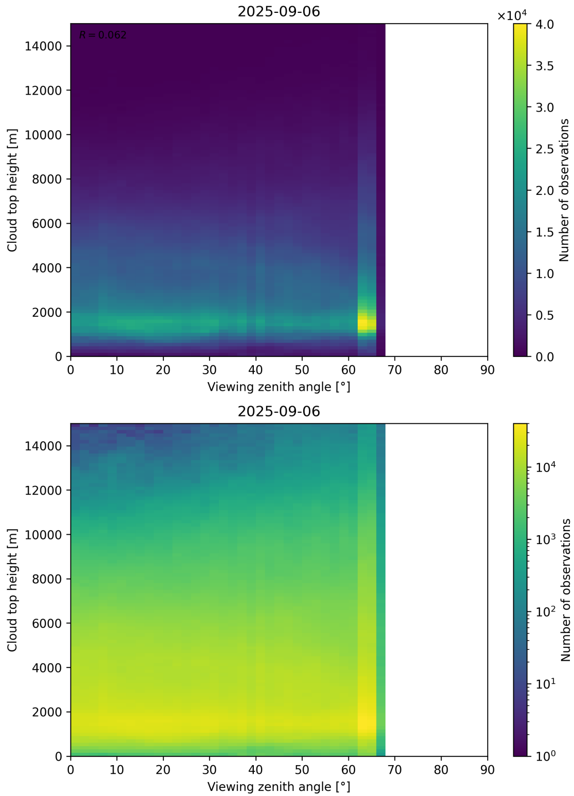
Figure 112: Scatter density plot of “Viewing zenith angle” against “Cloud top height” for 2025-09-05 to 2025-09-07.
