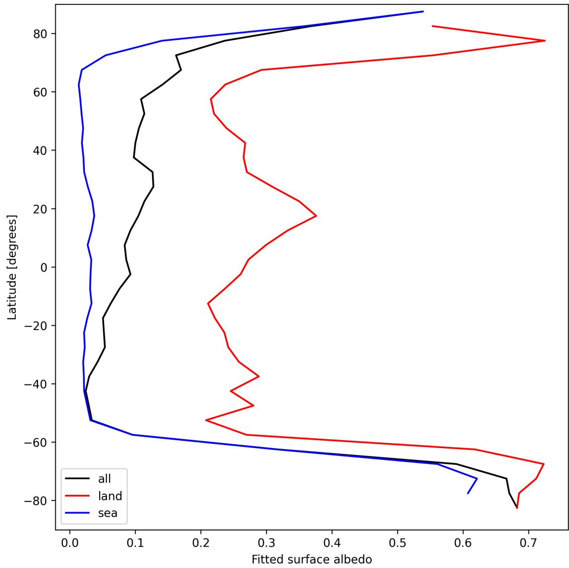
Figure 29: Zonal average of “Fitted surface albedo” for 2025-09-05 to 2025-09-07.
