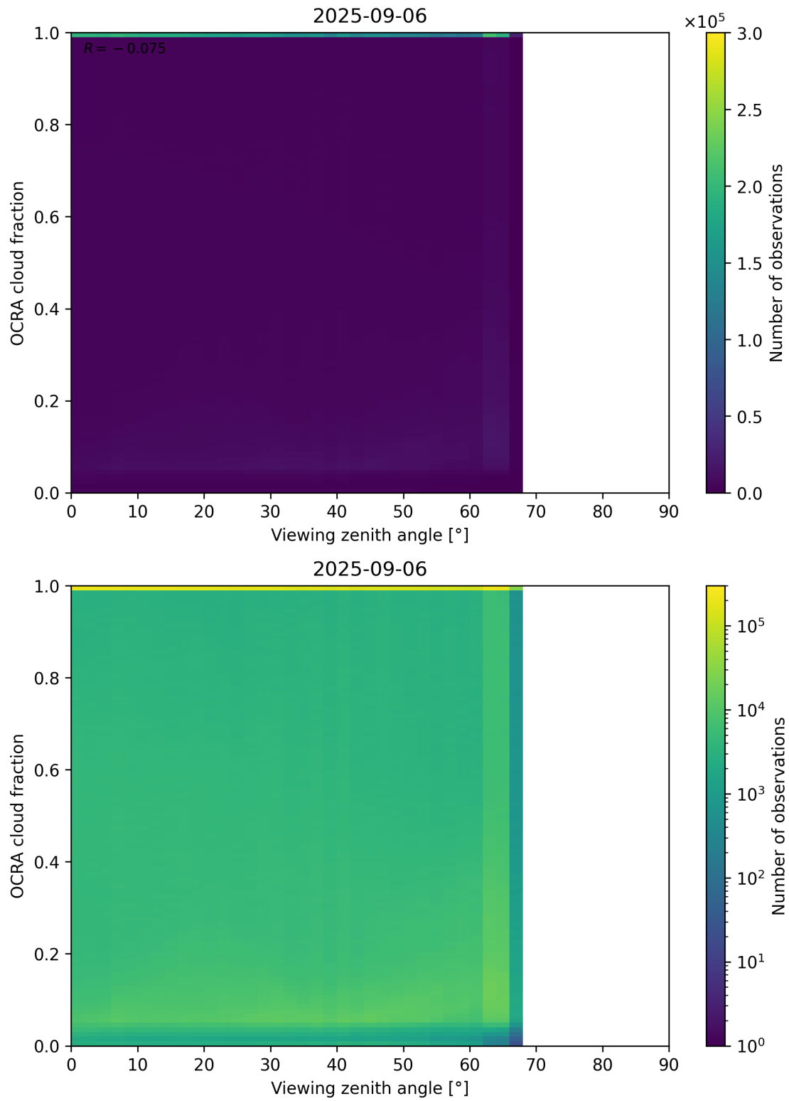
Figure 108: Scatter density plot of “Viewing zenith angle” against “OCRA cloud fraction” for 2025-09-05 to 2025-09-07.
