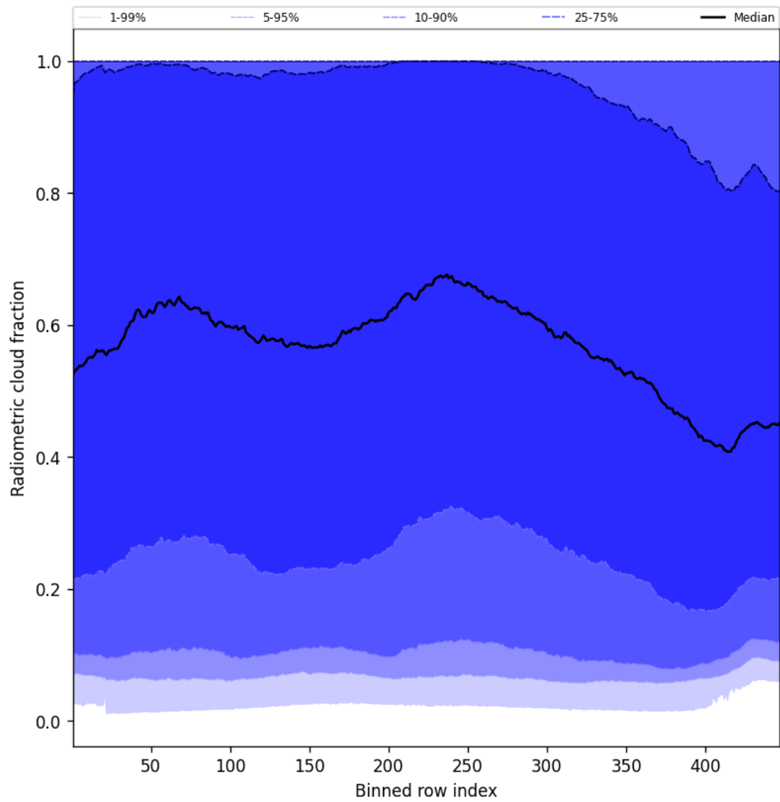
Figure 55: Along track statistics of “Radiometric cloud fraction” for 2025-09-05 to 2025-09-07
