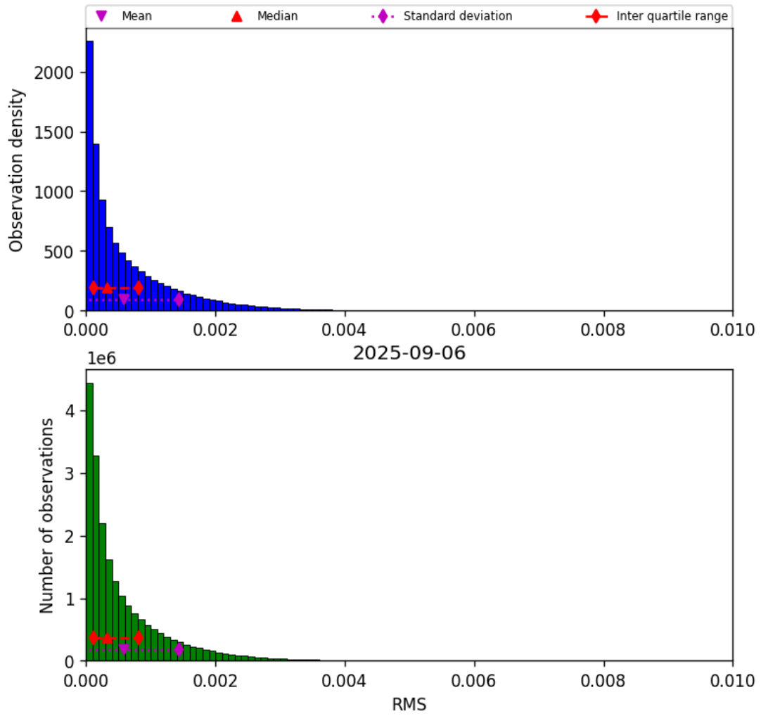
Figure 47: Histogram of “RMS” for 2025-09-05 to 2025-09-07
