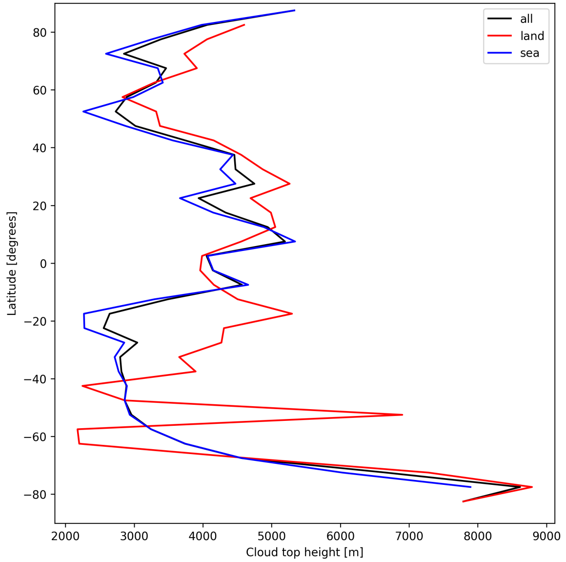
Figure 24: Zonal average of “Cloud top height” for 2025-09-05 to 2025-09-07.
