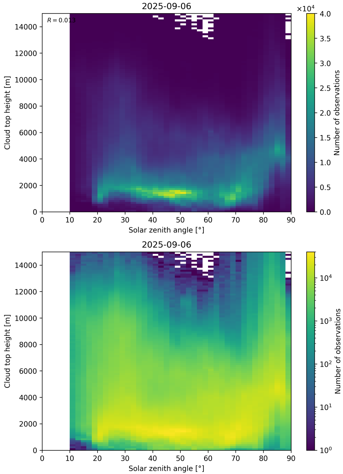
Figure 104: Scatter density plot of “Solar zenith angle” against “Cloud top height” for 2025-09-05 to 2025-09-07.
