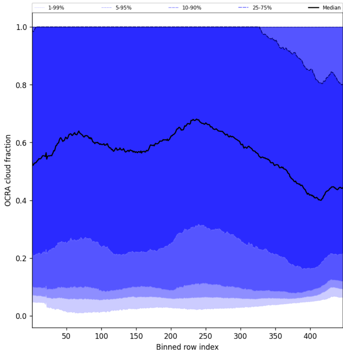
Figure 66: Along track statistics of “OCRA cloud fraction” for 2025-09-05 to 2025-09-07
