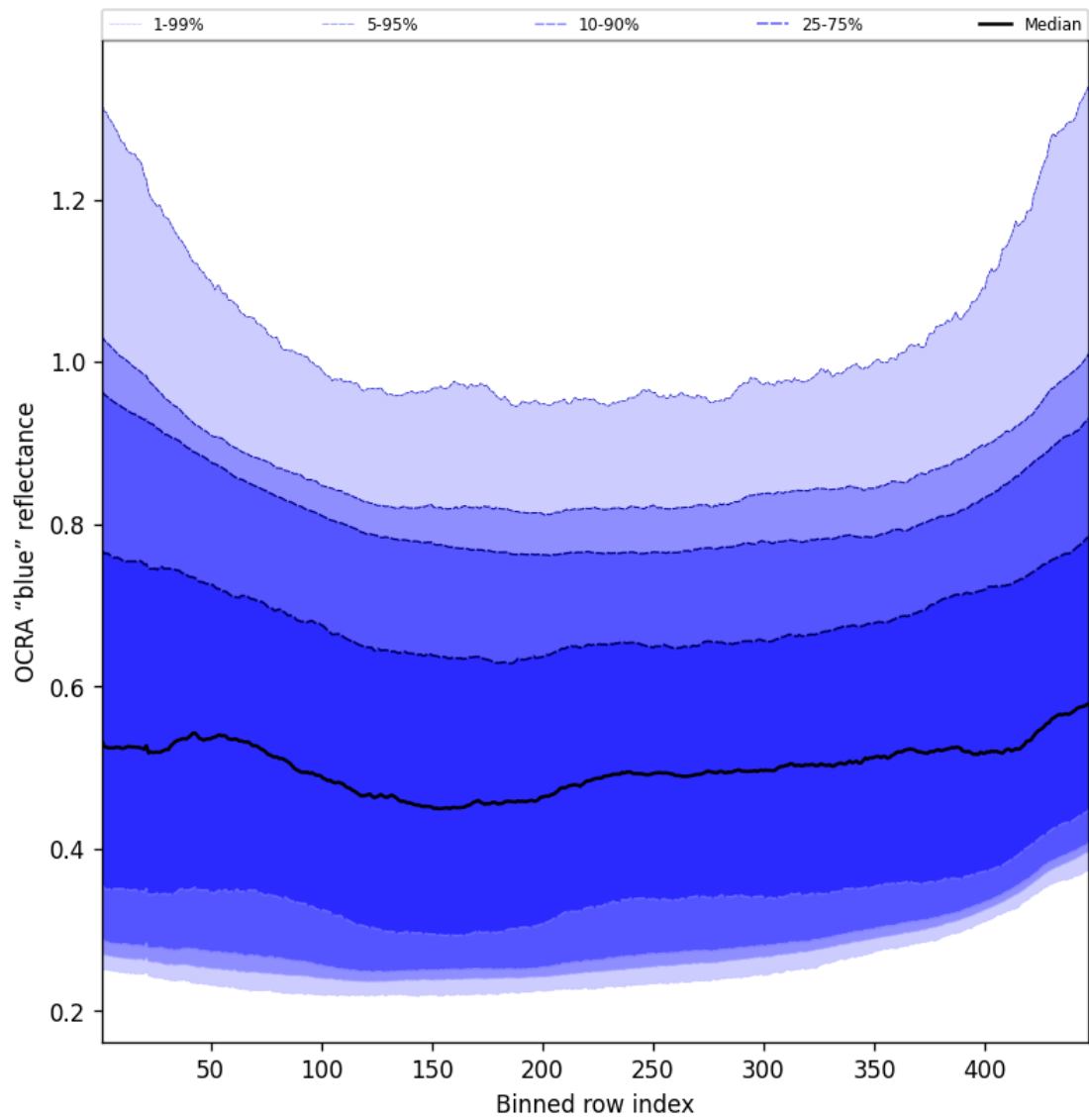
Figure 67: Along track statistics of “OCRA “blue” reflectance” for 2025-09-05 to 2025-09-07
