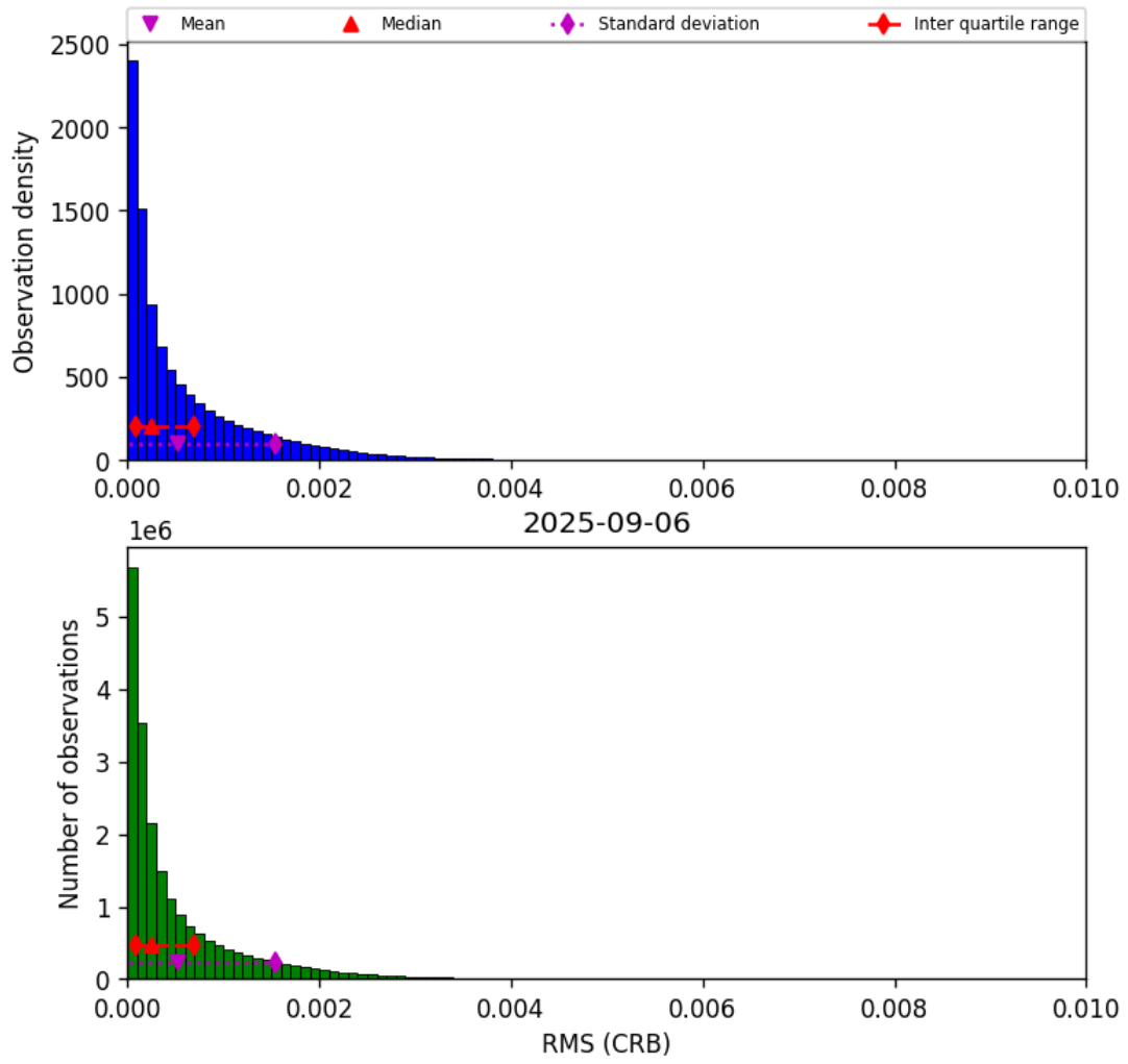
Figure 48: Histogram of “RMS (CRB)” for 2025-09-05 to 2025-09-07
