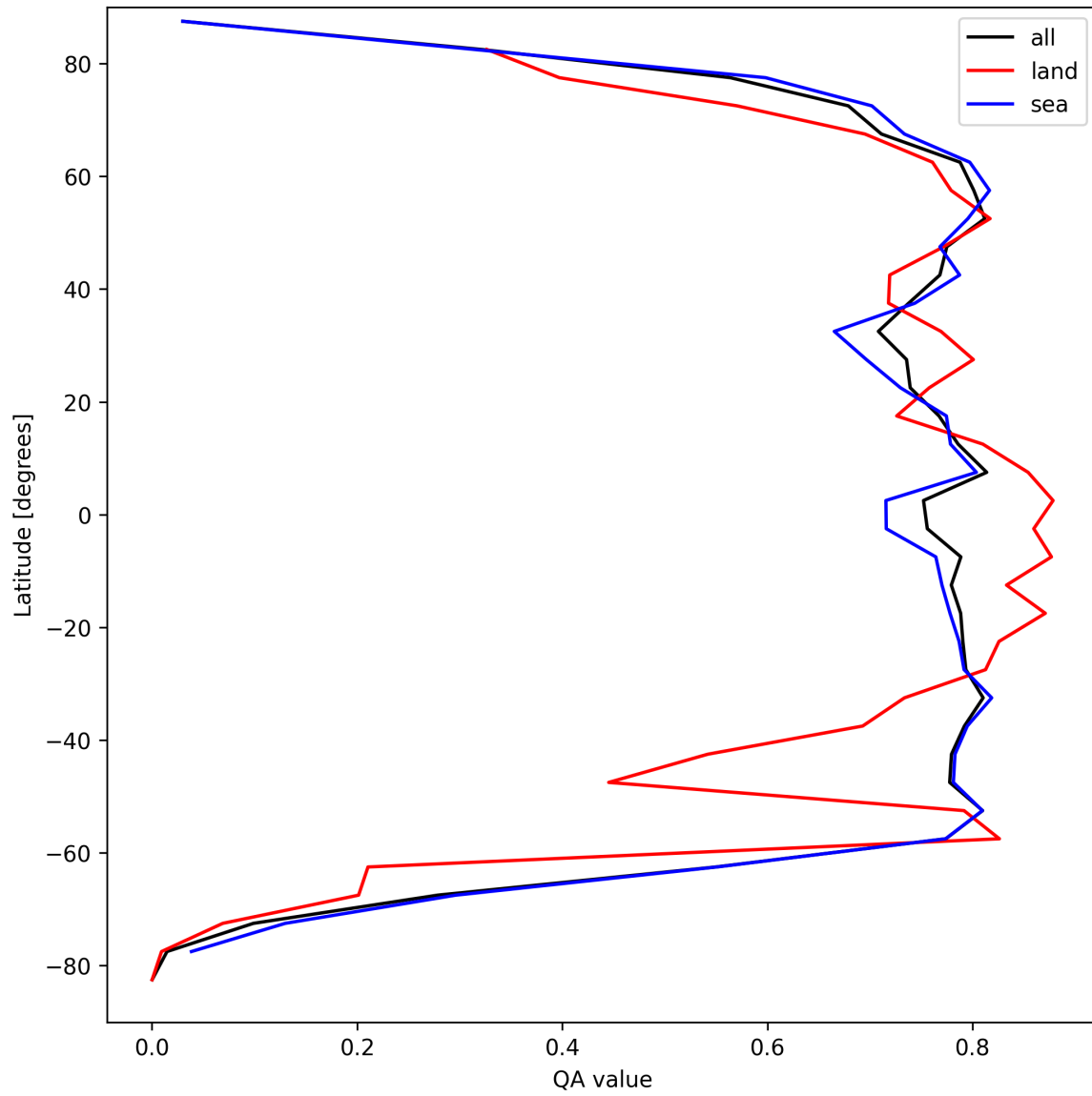
Figure 22: Zonal average of “QA value” for 2025-09-05 to 2025-09-07.
