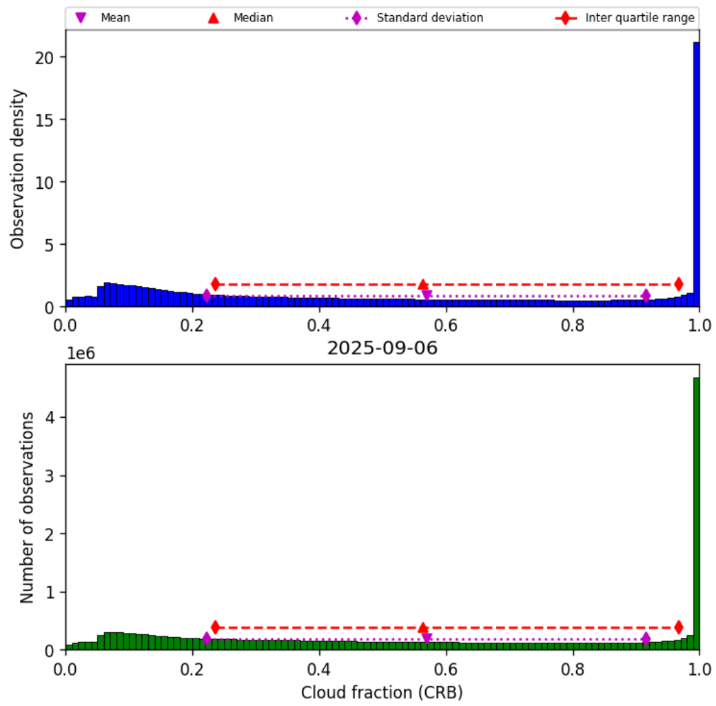
Figure 42: Histogram of “Cloud fraction (CRB)” for 2025-09-05 to 2025-09-07
