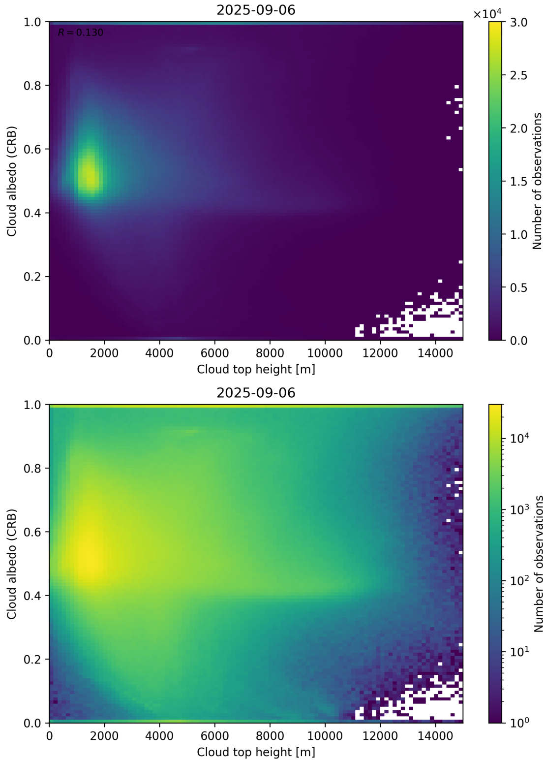
Figure 86: Scatter density plot of “Cloud top height” against “Cloud albedo (CRB)” for 2025-09-05 to 2025-09-07.
