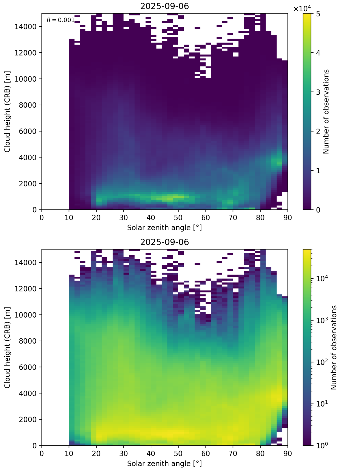
Figure 102: Scatter density plot of “Solar zenith angle” against “Cloud height (CRB)” for 2025-09-05 to 2025-09-07.
