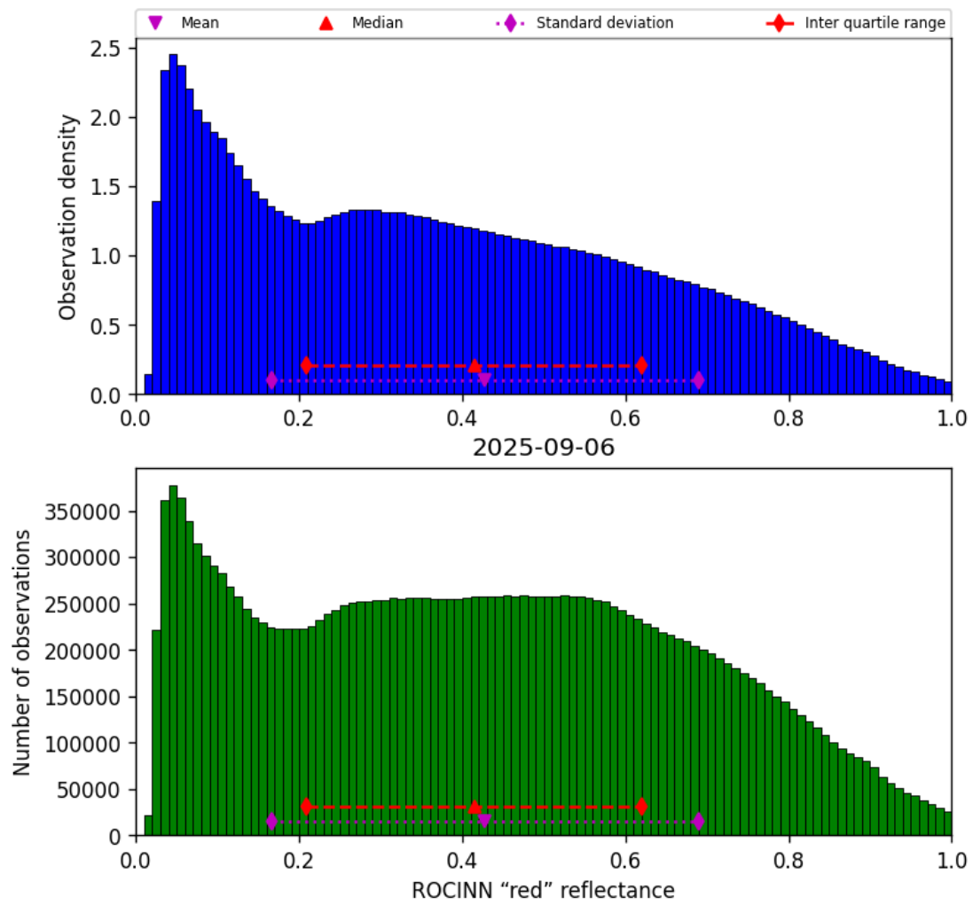
Figure 53: Histogram of “ROCINN “red” reflectance” for 2025-09-05 to 2025-09-07
