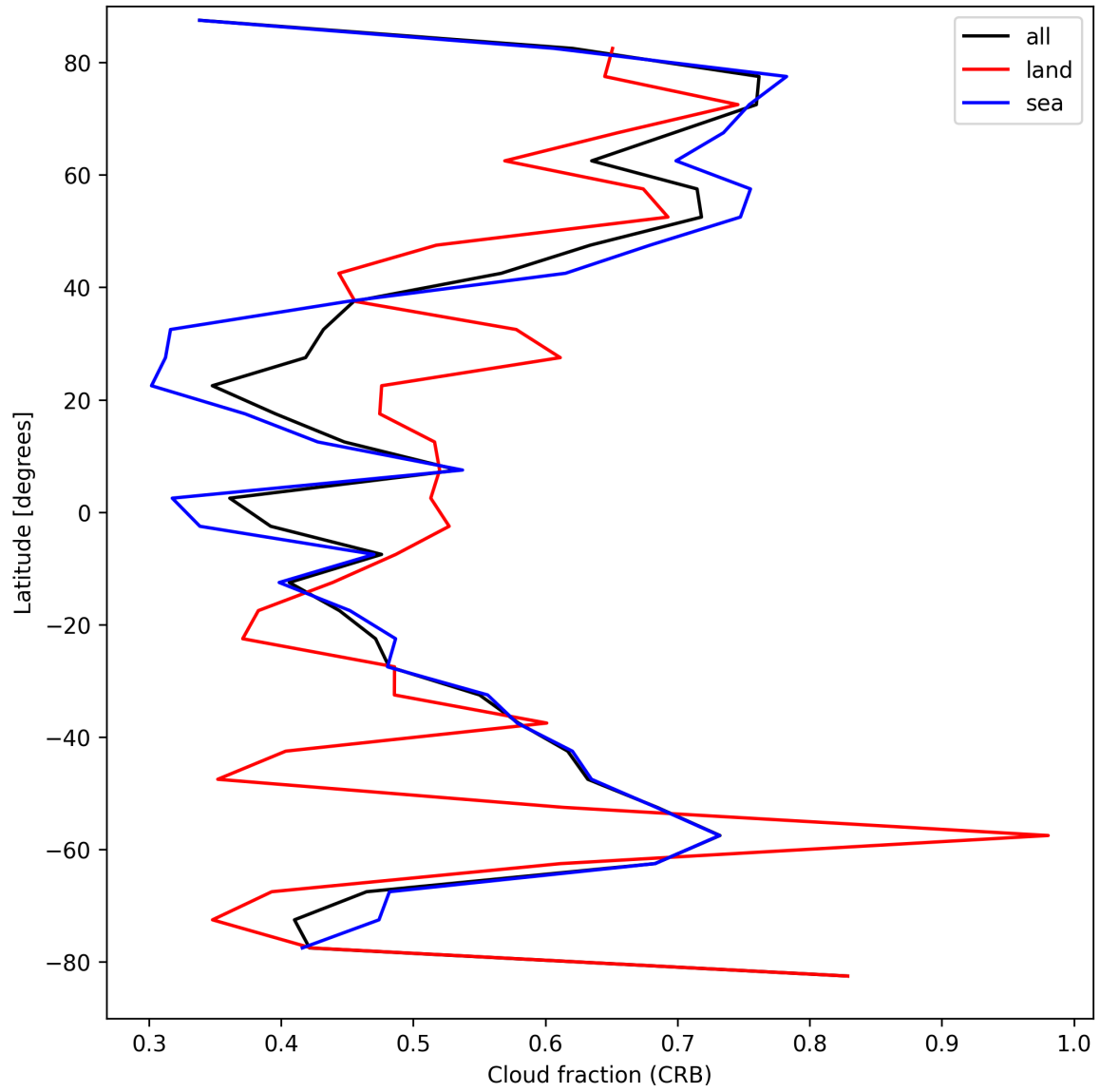
Figure 26: Zonal average of “Cloud fraction (CRB)” for 2025-09-05 to 2025-09-07.
