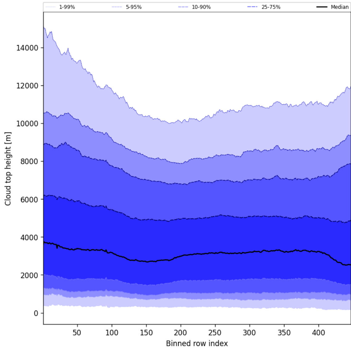
Figure 56: Along track statistics of “Cloud top height” for 2025-09-05 to 2025-09-07
