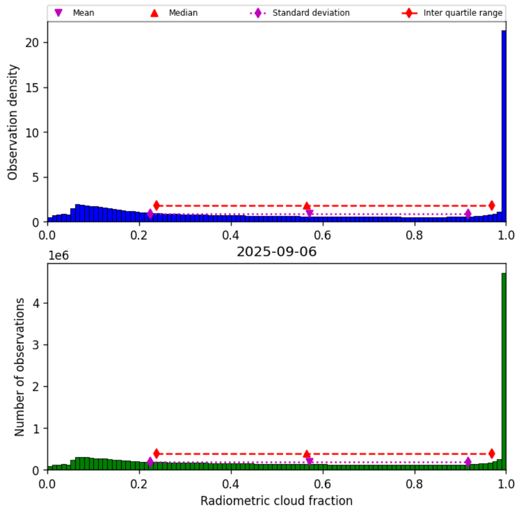
Figure 39: Histogram of “Radiometric cloud fraction” for 2025-09-05 to 2025-09-07
