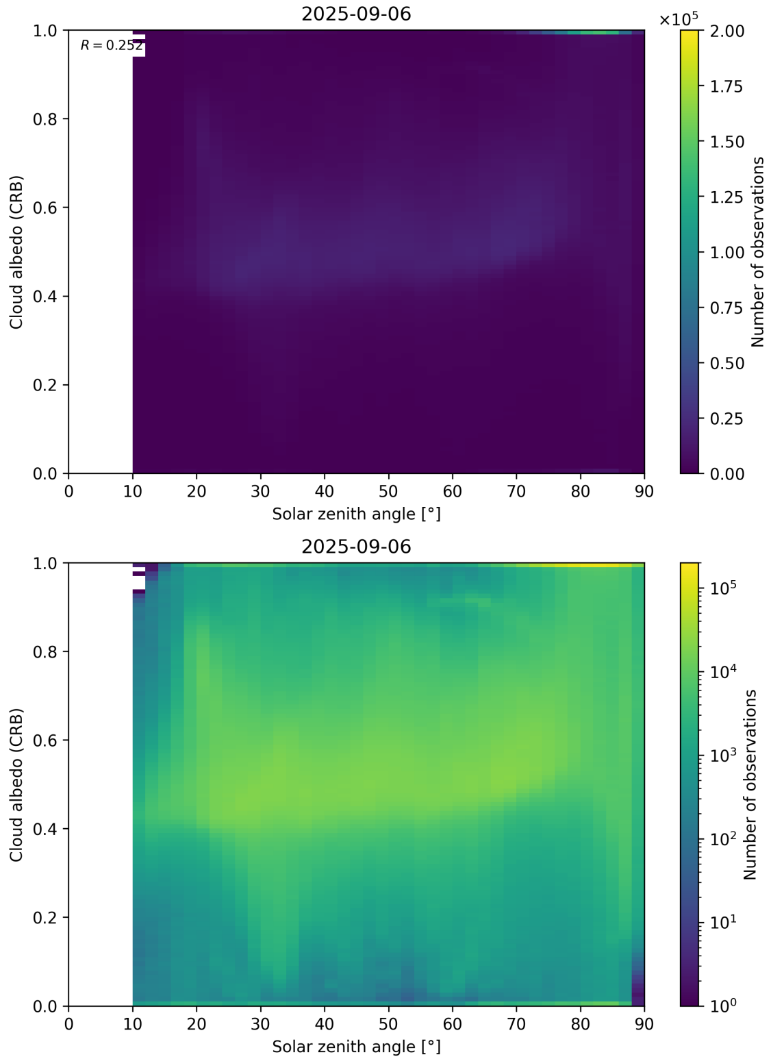
Figure 98: Scatter density plot of “Solar zenith angle” against “Cloud albedo (CRB)” for 2025-09-05 to 2025-09-07.
