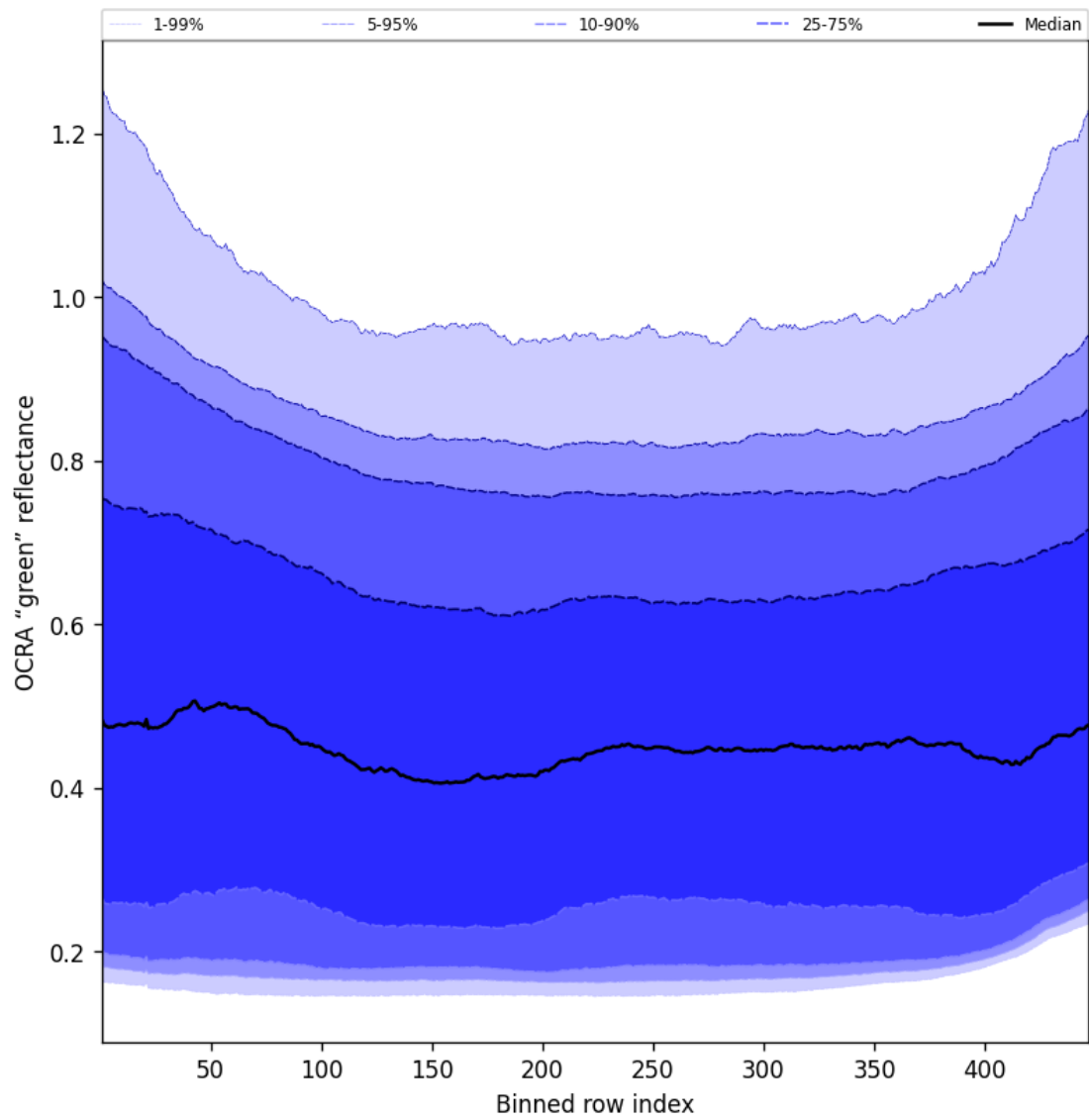
Figure 68: Along track statistics of “OCRA “green” reflectance” for 2025-09-05 to 2025-09-07
