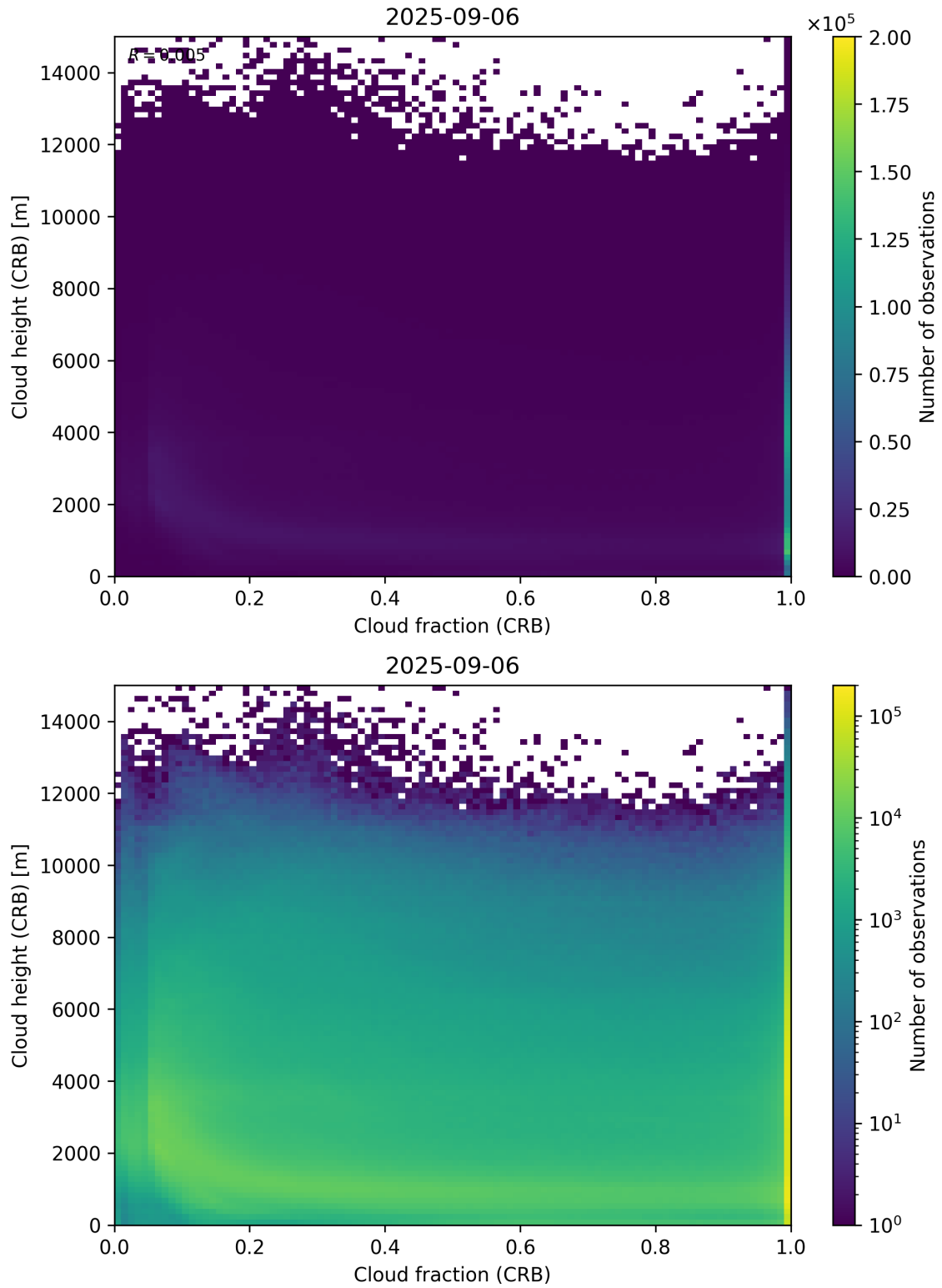
Figure 79: Scatter density plot of “Cloud fraction (CRB)” against “Cloud height (CRB)” for 2025-09-05 to 2025-09-07.
