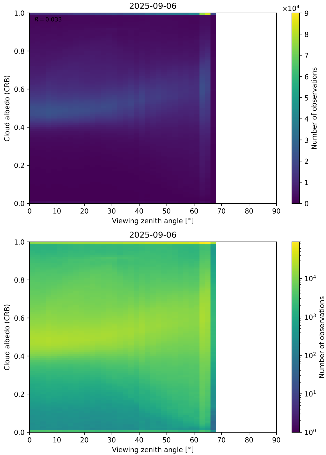
Figure 106: Scatter density plot of “Viewing zenith angle” against “Cloud albedo (CRB)” for 2025-09-05 to 2025-09-07.
