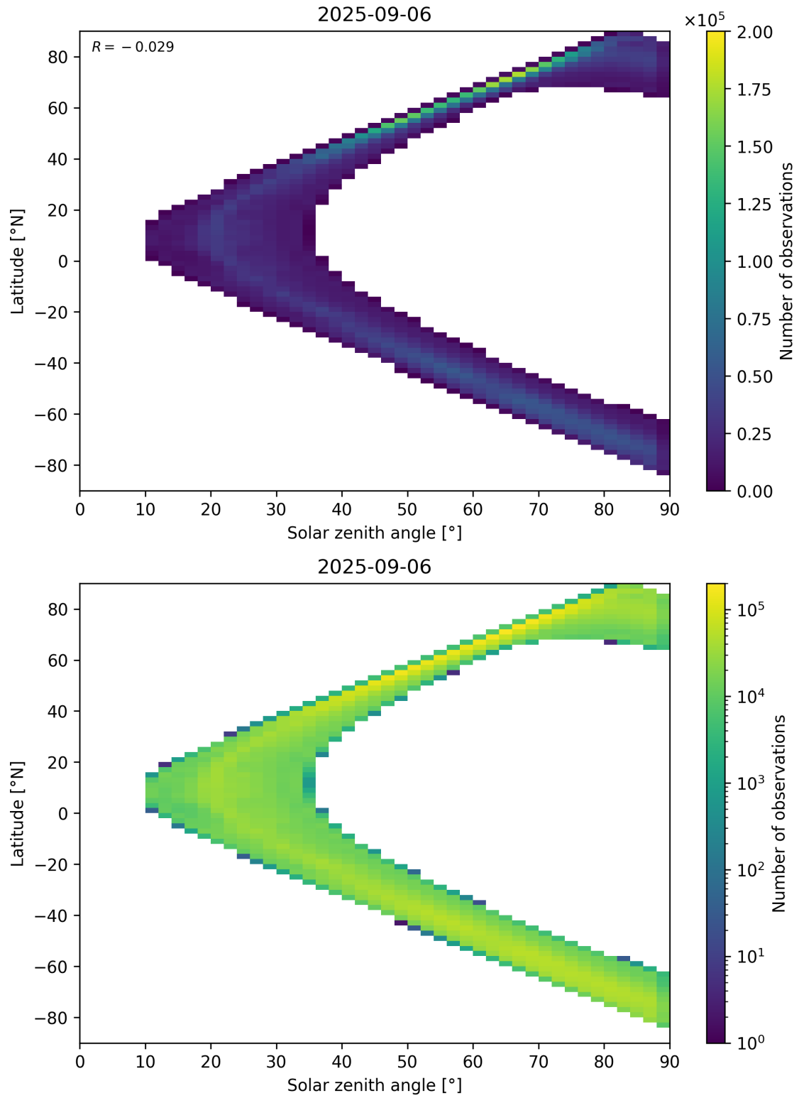
Figure 105: Scatter density plot of “Solar zenith angle” against “Latitude” for 2025-09-05 to 2025-09-07.
