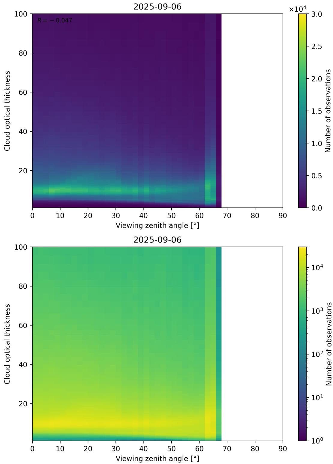
Figure 111: Scatter density plot of “Viewing zenith angle” against “Cloud optical thickness” for 2025-09-05 to 2025-09-07.
