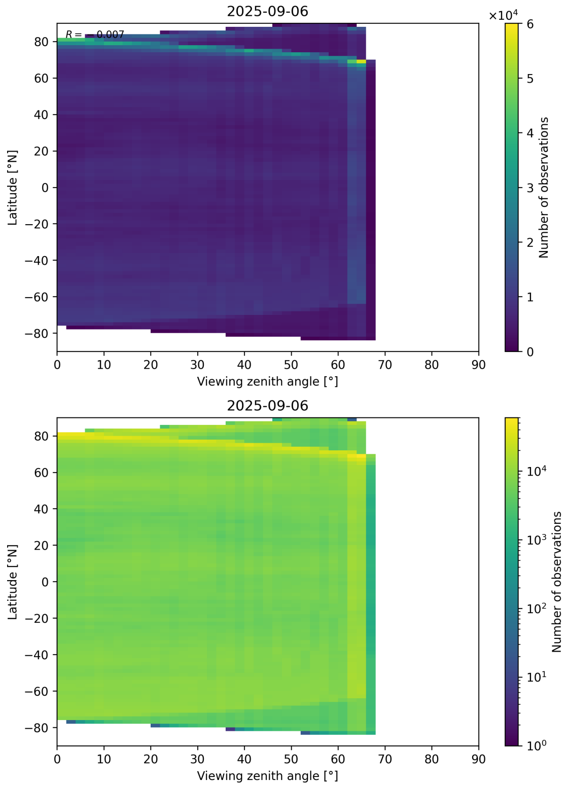
Figure 113: Scatter density plot of “Viewing zenith angle” against “Latitude” for 2025-09-05 to 2025-09-07.
