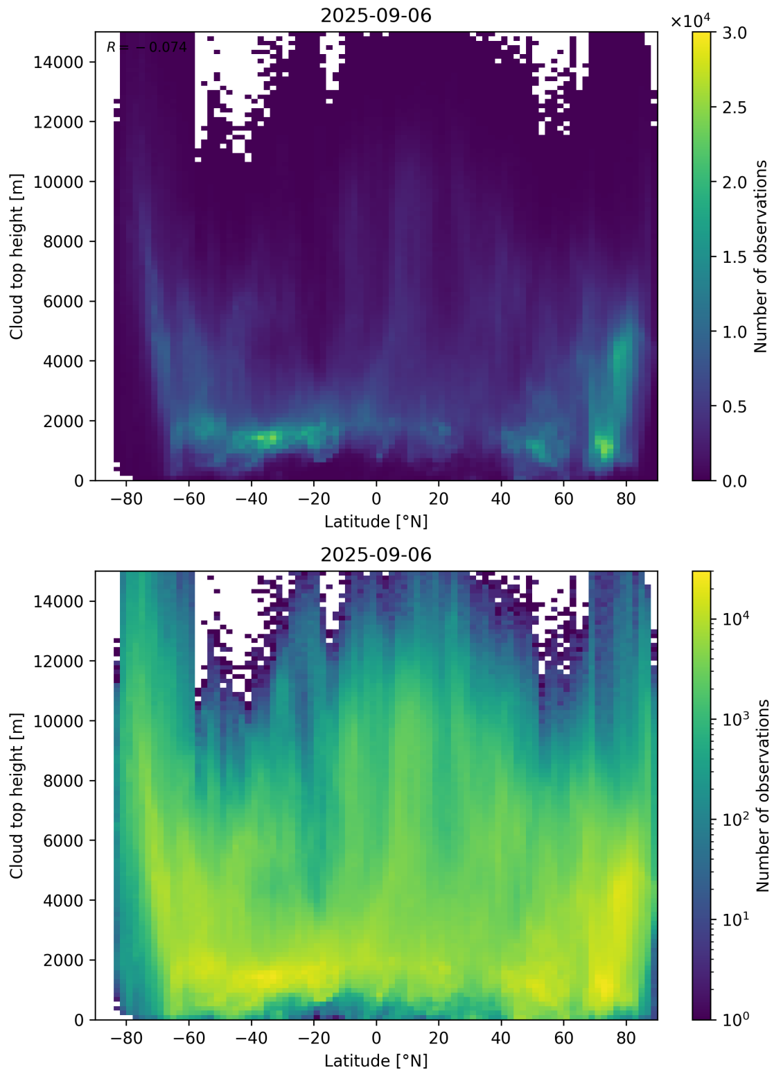
Figure 97: Scatter density plot of “Latitude” against “Cloud top height” for 2025-09-05 to 2025-09-07.
