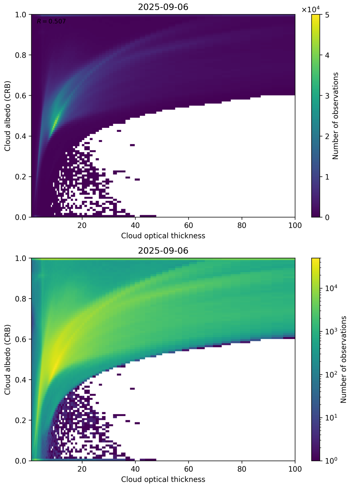
Figure 82: Scatter density plot of “Cloud optical thickness” against “Cloud albedo (CRB)” for 2025-09-05 to 2025-09-07.
