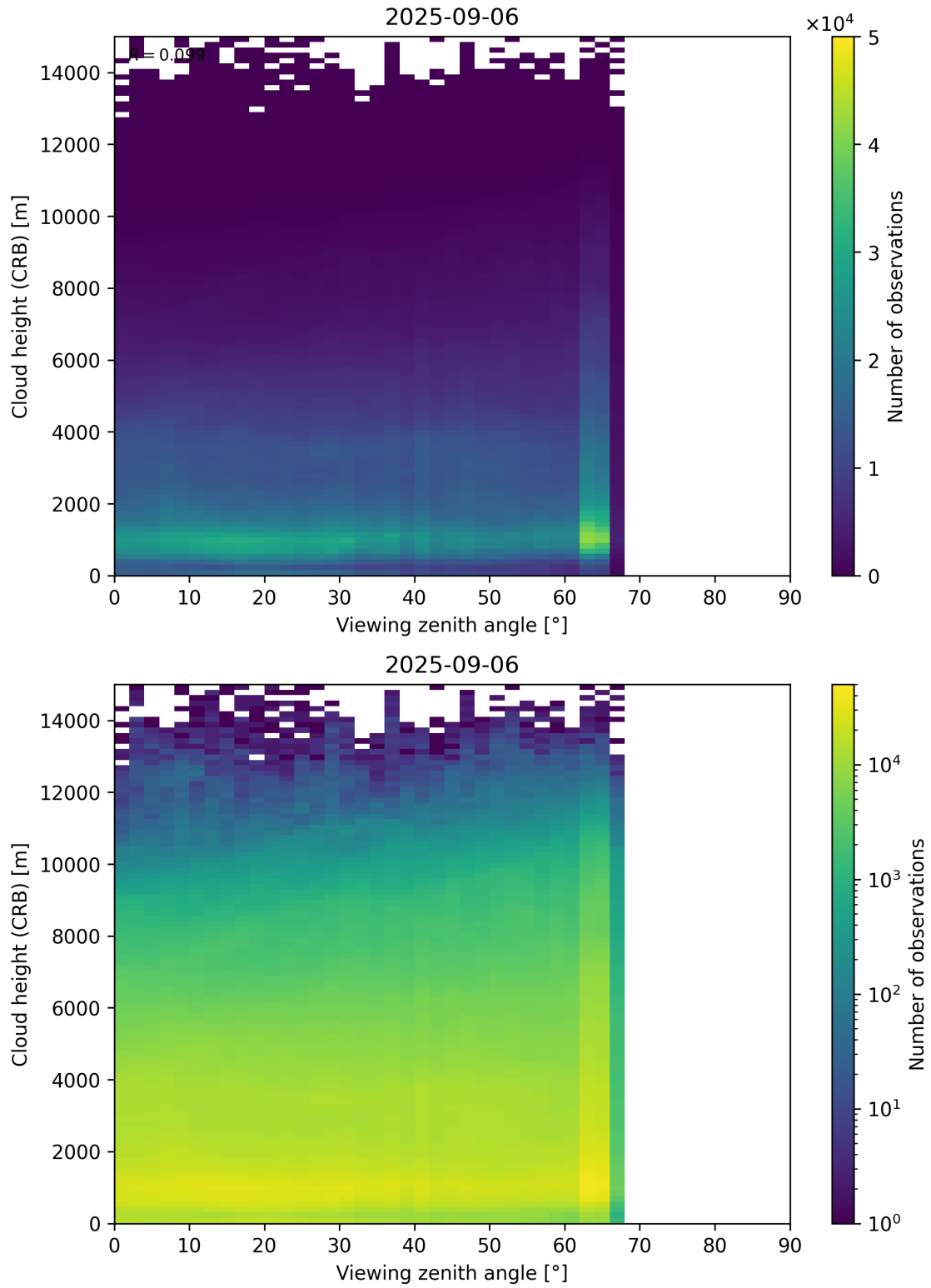
Figure 110: Scatter density plot of “Viewing zenith angle” against “Cloud height (CRB)” for 2025-09-05 to 2025-09-07.
