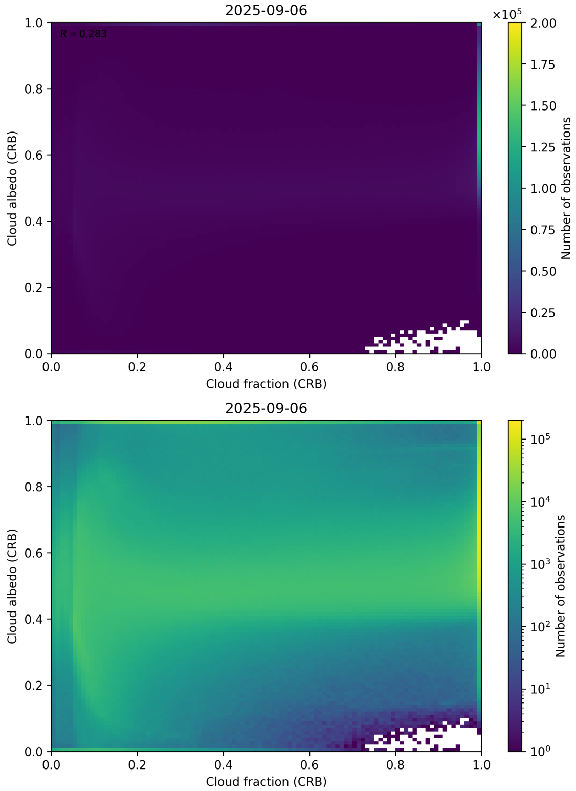
Figure 77: Scatter density plot of “Cloud fraction (CRB)” against “Cloud albedo (CRB)” for 2025-09-05 to 2025-09-07.
