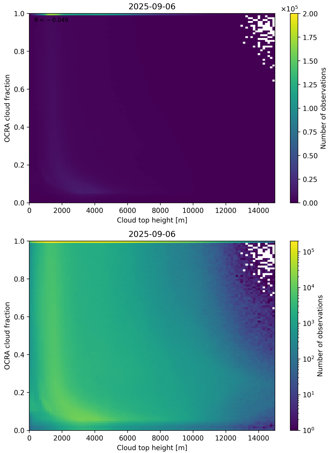
Figure 87: Scatter density plot of “Cloud top height” against “OCRA cloud fraction” for 2025-09-05 to 2025-09-07.
