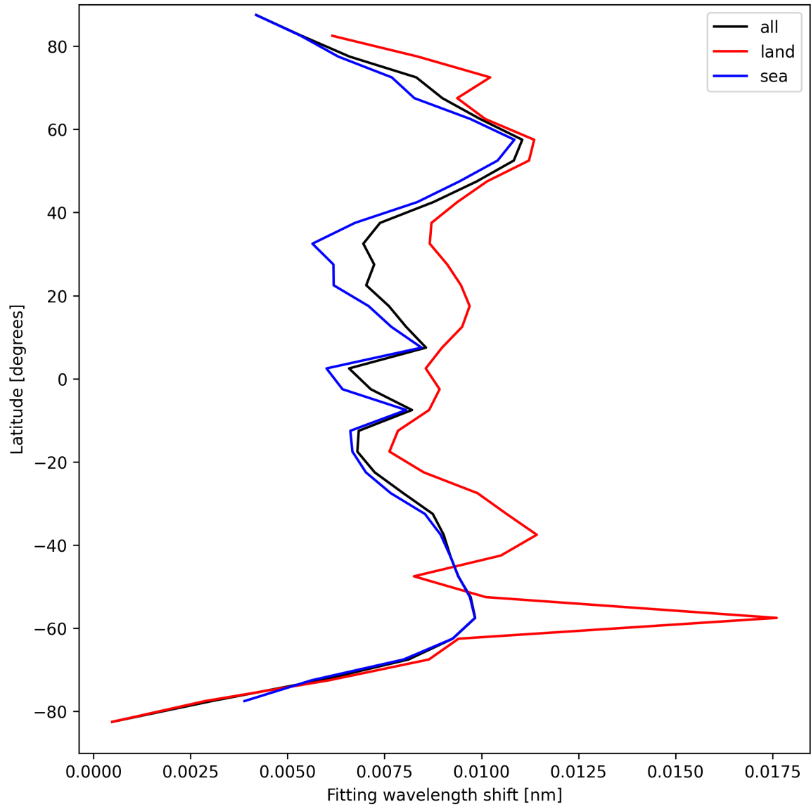
Figure 33: Zonal average of “Fitting wavelength shift” for 2025-09-05 to 2025-09-07.
