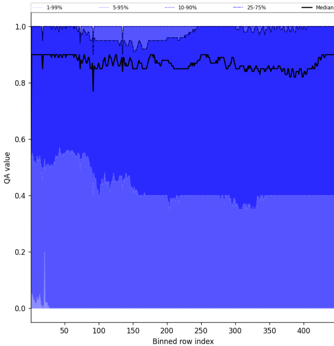
Figure 54: Along track statistics of “QA value” for 2025-09-05 to 2025-09-07
