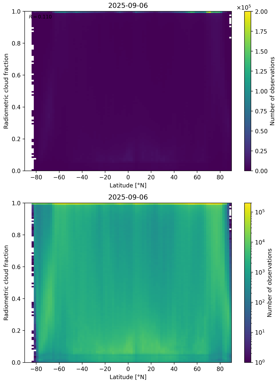
Figure 92: Scatter density plot of “Latitude” against “Radiometric cloud fraction” for 2025-09-05 to 2025-09-07.
