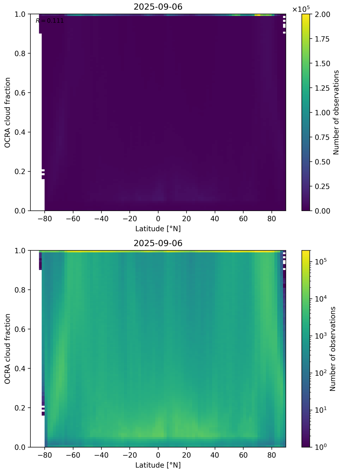
Figure 93: Scatter density plot of “Latitude” against “OCRA cloud fraction” for 2025-09-05 to 2025-09-07.
