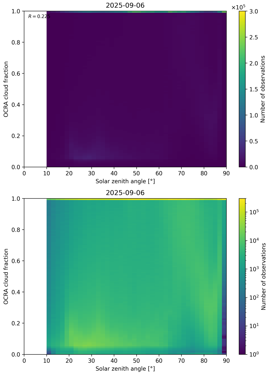
Figure 100: Scatter density plot of “Solar zenith angle” against “OCRA cloud fraction” for 2025-09-05 to 2025-09-07.
