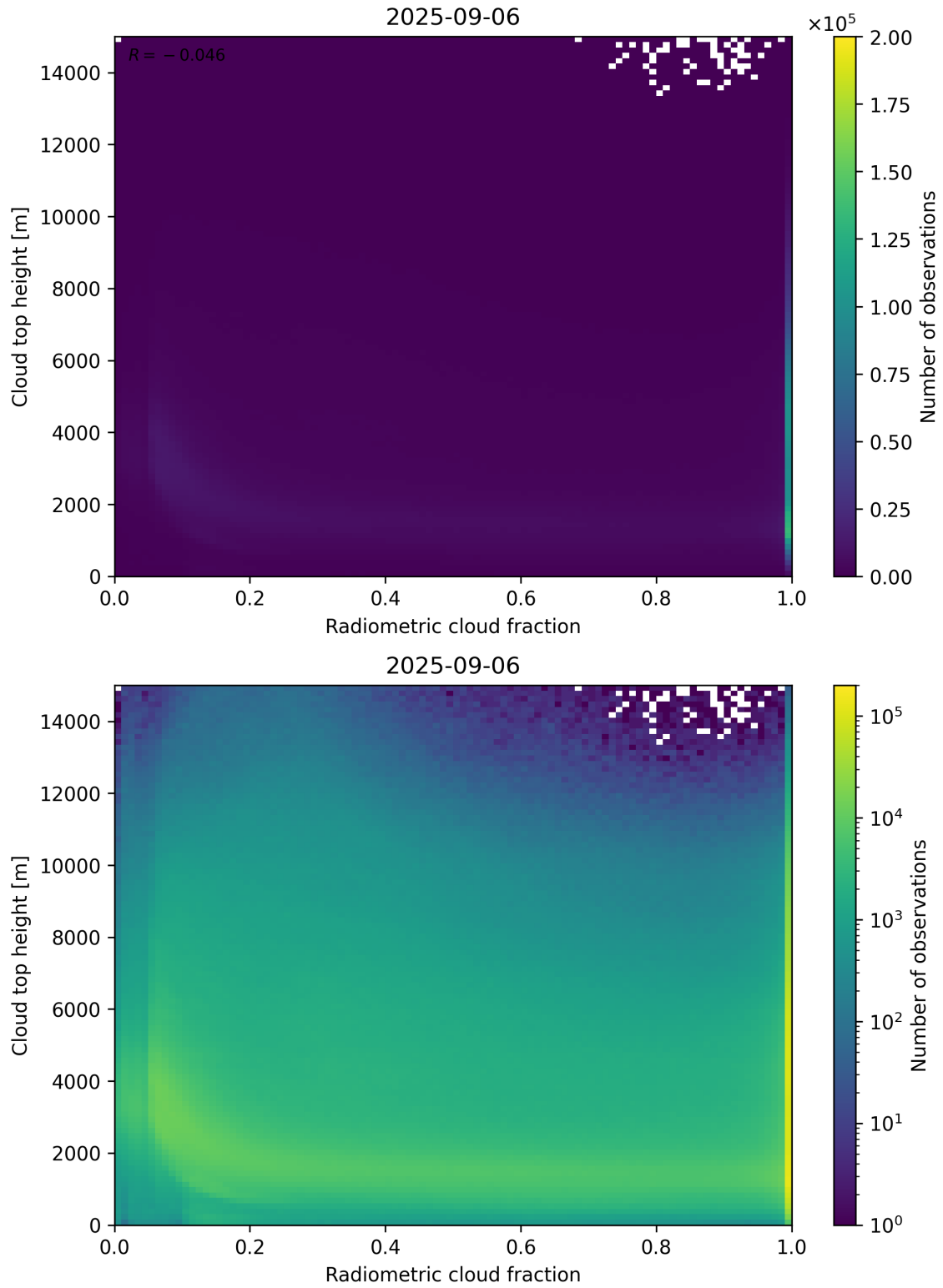
Figure 76: Scatter density plot of “Radiometric cloud fraction” against “Cloud top height” for 2025-09-05 to 2025-09-07.
