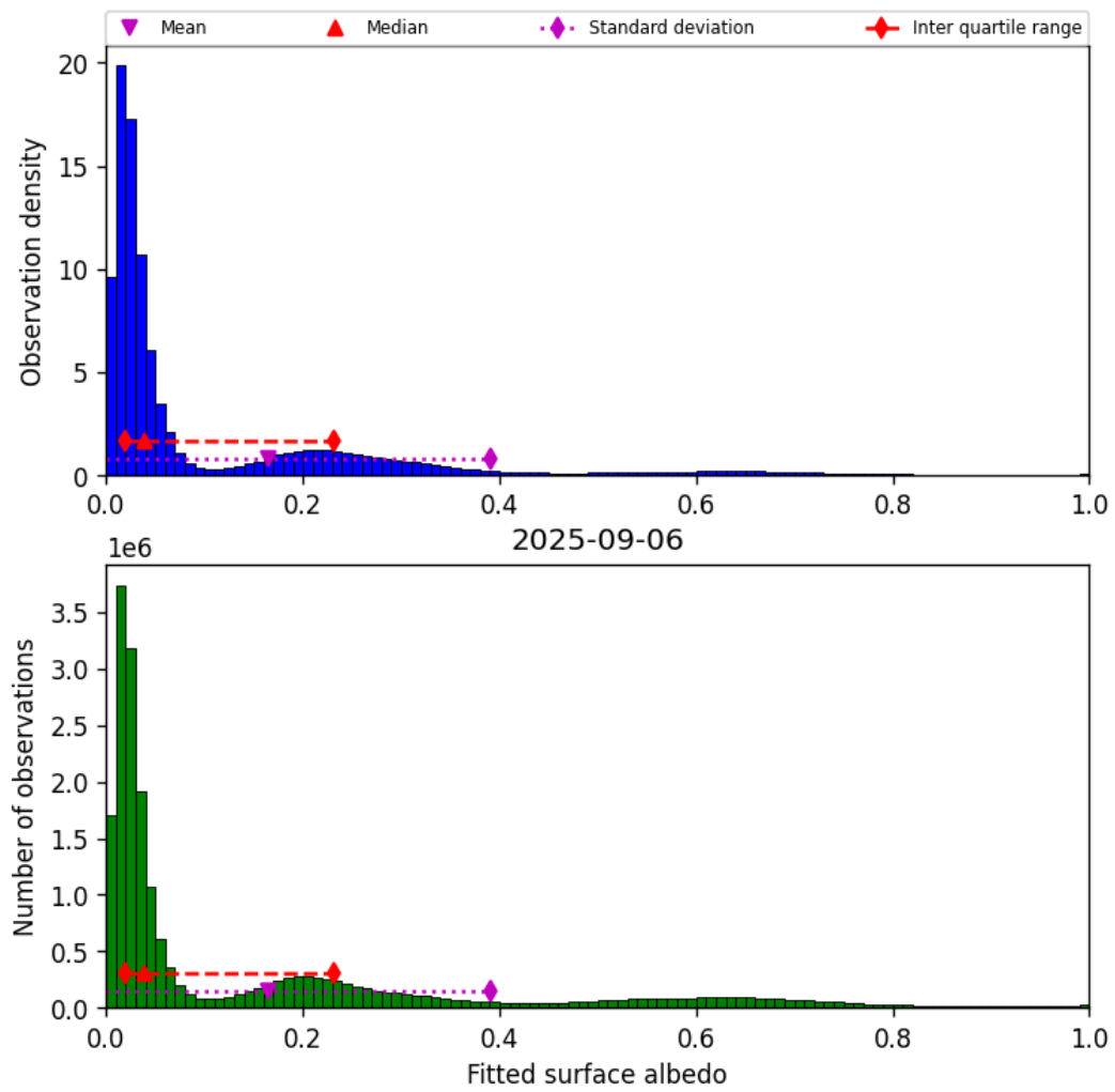
Figure 45: Histogram of “Fitted surface albedo” for 2025-09-05 to 2025-09-07
