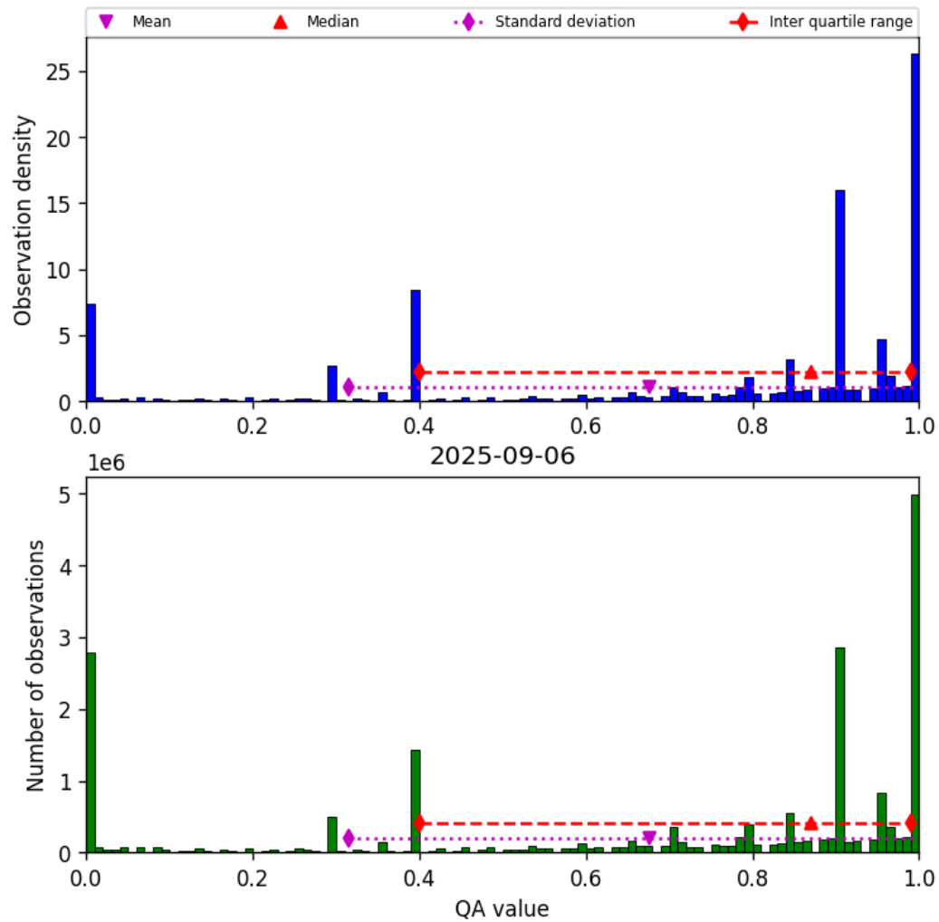
Figure 38: Histogram of “QA value” for 2025-09-05 to 2025-09-07
