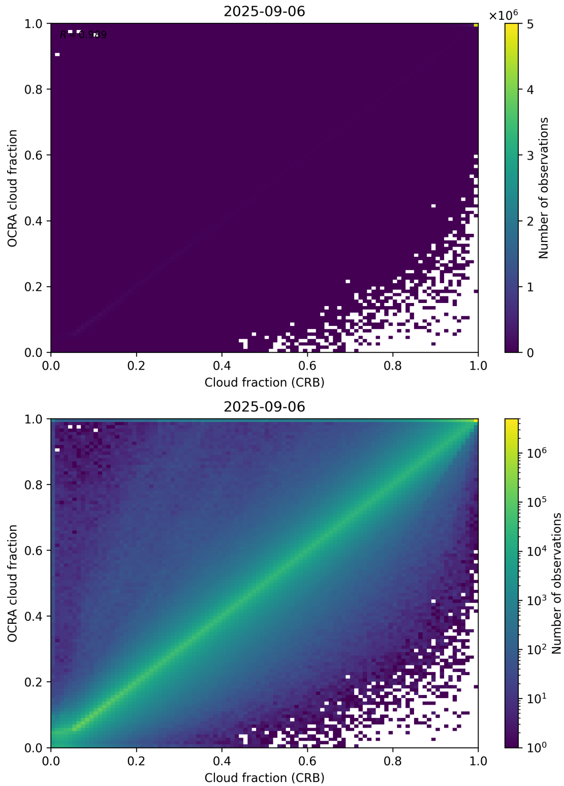
Figure 78: Scatter density plot of “Cloud fraction (CRB)” against “OCRA cloud fraction” for 2025-09-05 to 2025-09-07.
