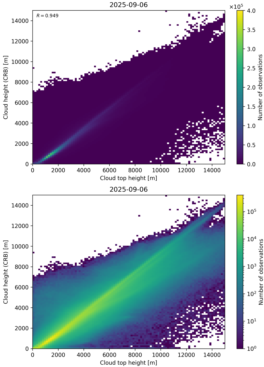
Figure 89: Scatter density plot of “Cloud top height” against “Cloud height (CRB)” for 2025-09-05 to 2025-09-07.
