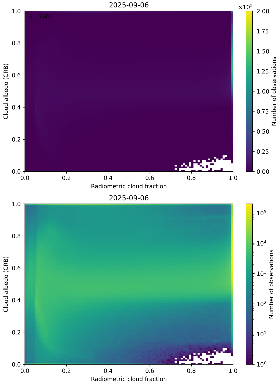
Figure 71: Scatter density plot of “Radiometric cloud fraction” against “Cloud albedo (CRB)” for 2025-09-05 to 2025-09-07.
