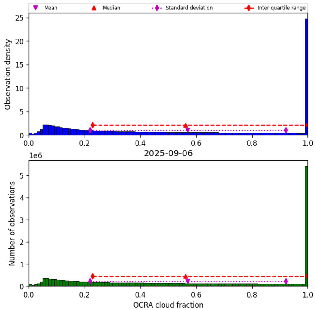
Figure 50: Histogram of “OCRA cloud fraction” for 2025-09-05 to 2025-09-07
