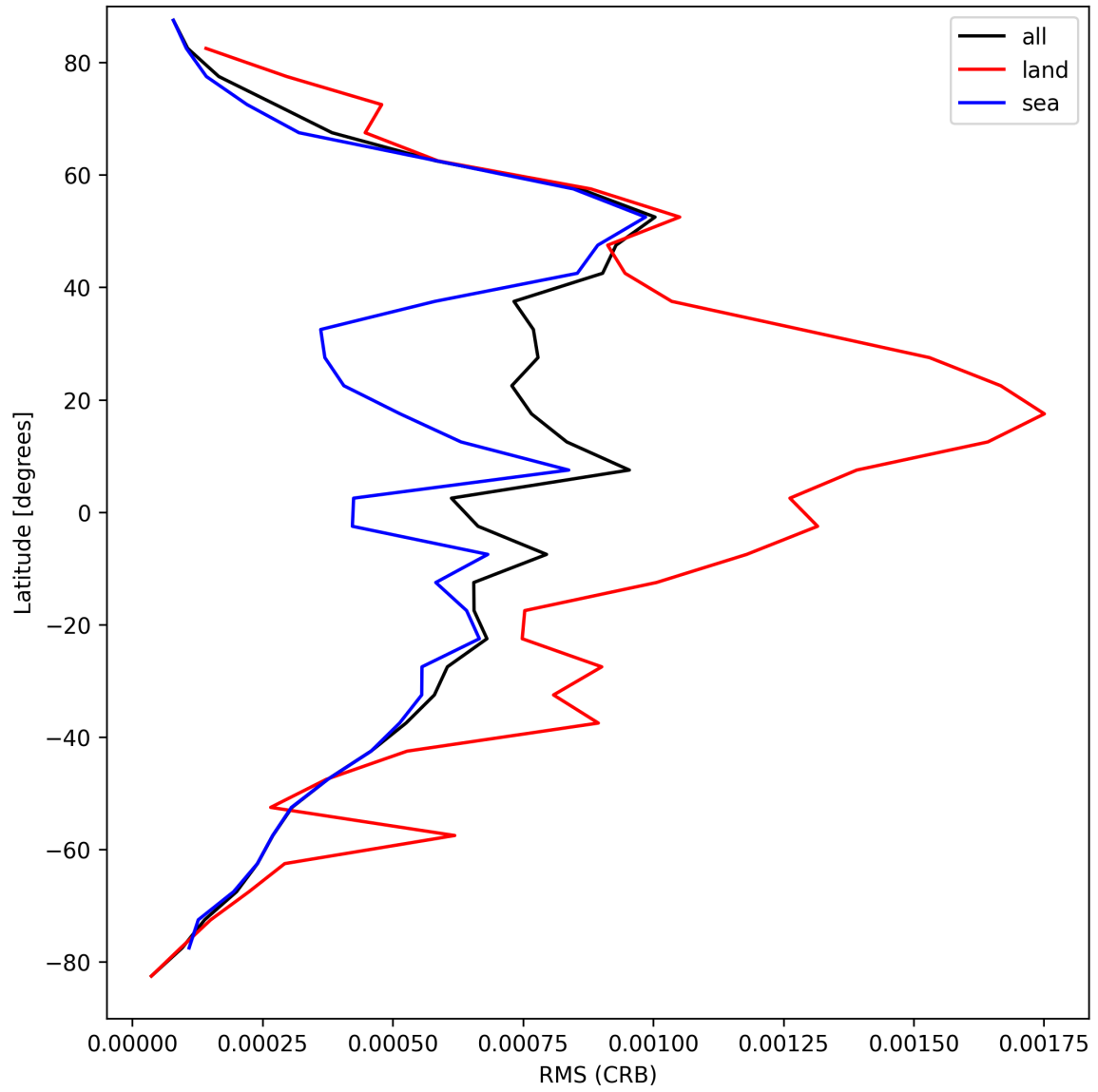
Figure 32: Zonal average of “RMS (CRB)” for 2025-09-05 to 2025-09-07.
