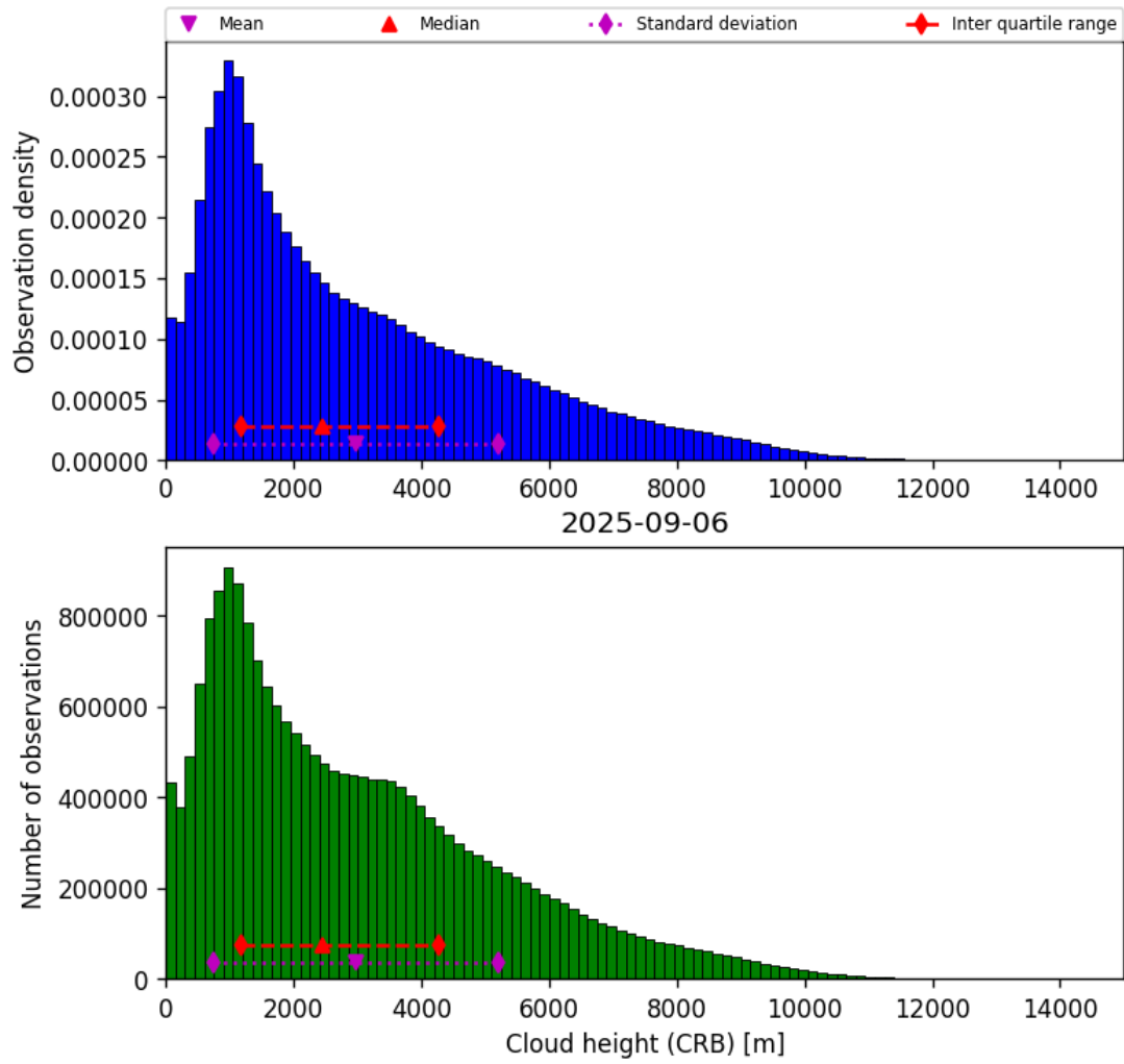
Figure 43: Histogram of “Cloud height (CRB)” for 2025-09-05 to 2025-09-07
