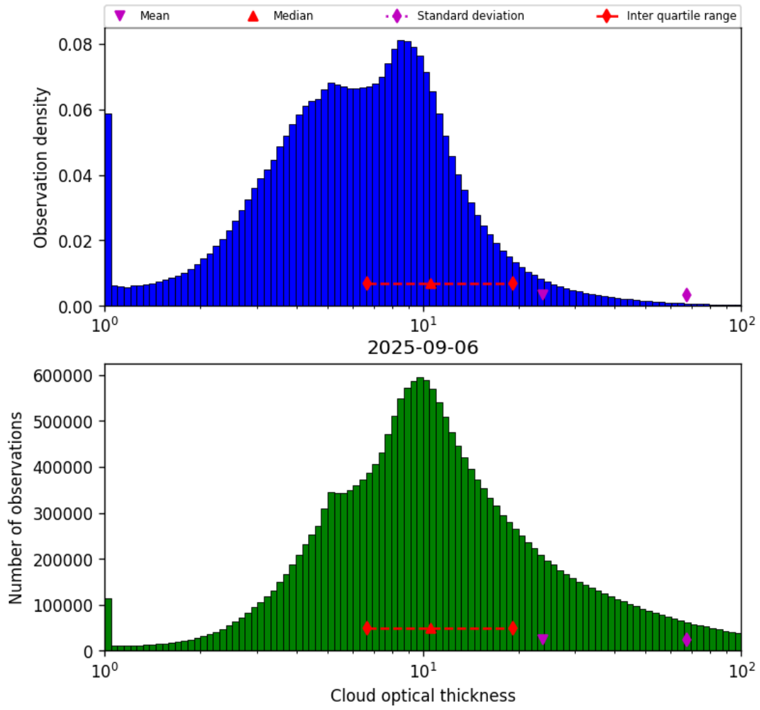
Figure 41: Histogram of “Cloud optical thickness” for 2025-09-05 to 2025-09-07
