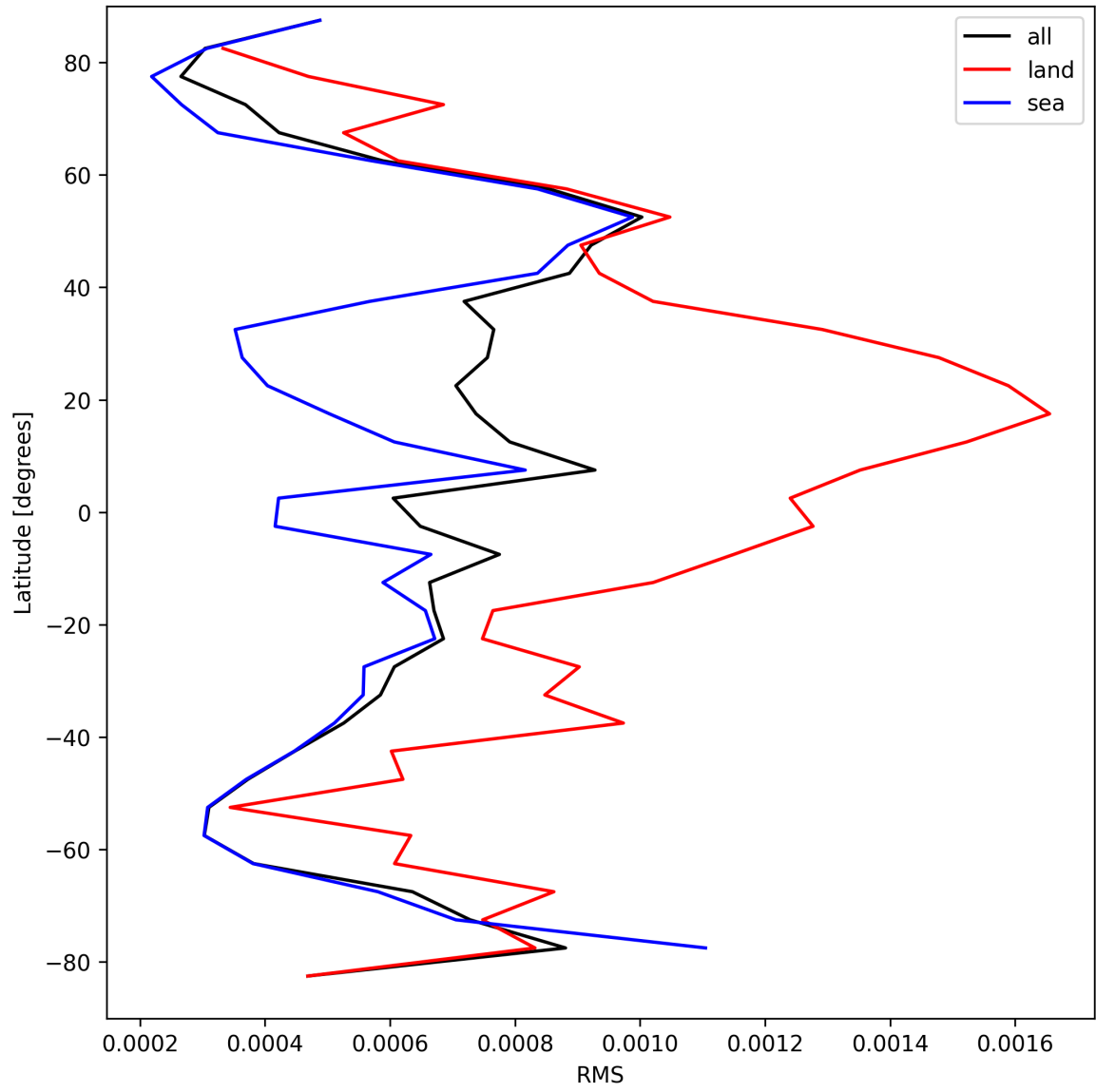
Figure 31: Zonal average of “RMS” for 2025-09-05 to 2025-09-07.
