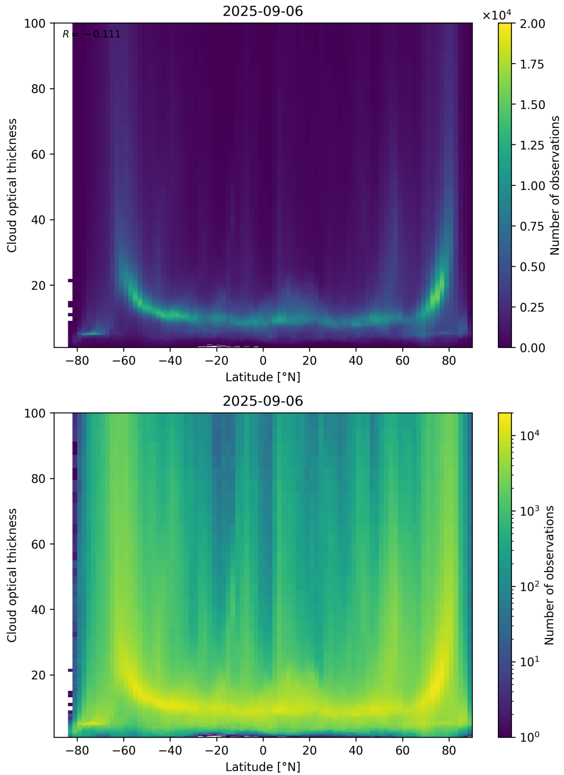
Figure 96: Scatter density plot of “Latitude” against “Cloud optical thickness” for 2025-09-05 to 2025-09-07.
