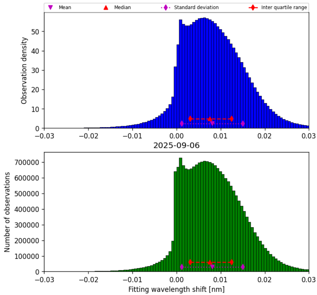
Figure 49: Histogram of “Fitting wavelength shift” for 2025-09-05 to 2025-09-07
