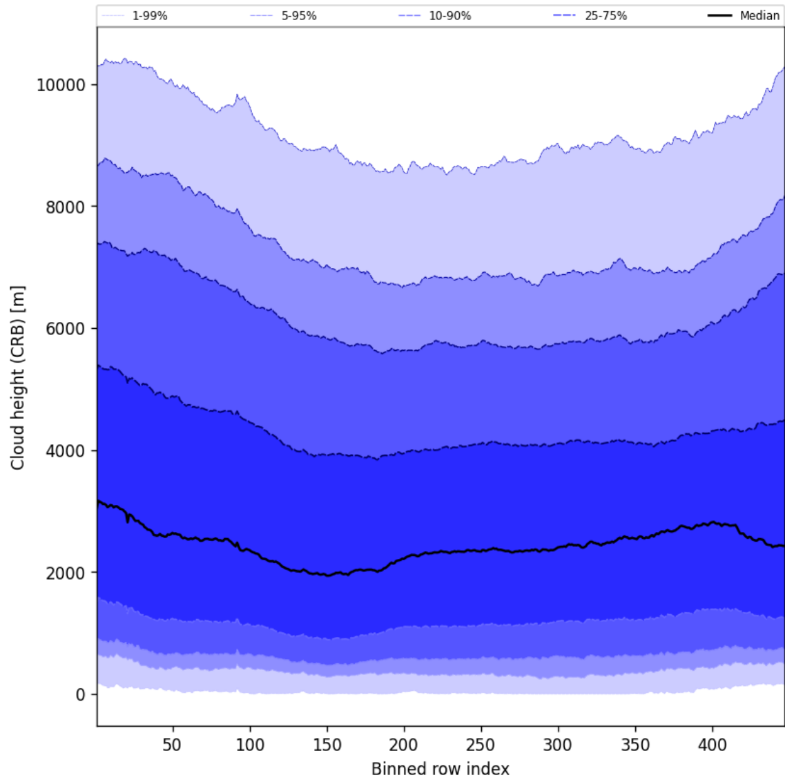
Figure 59: Along track statistics of “Cloud height (CRB)” for 2025-09-05 to 2025-09-07
