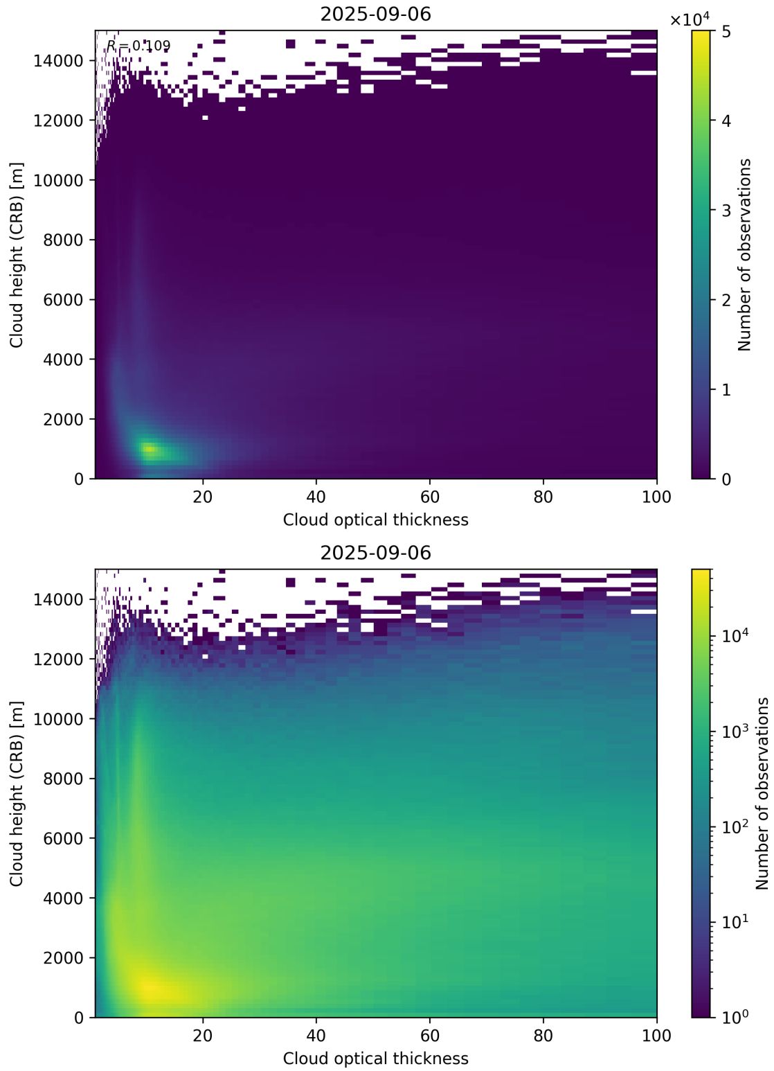
Figure 85: Scatter density plot of “Cloud optical thickness” against “Cloud height (CRB)” for 2025-09-05 to 2025-09-07.
