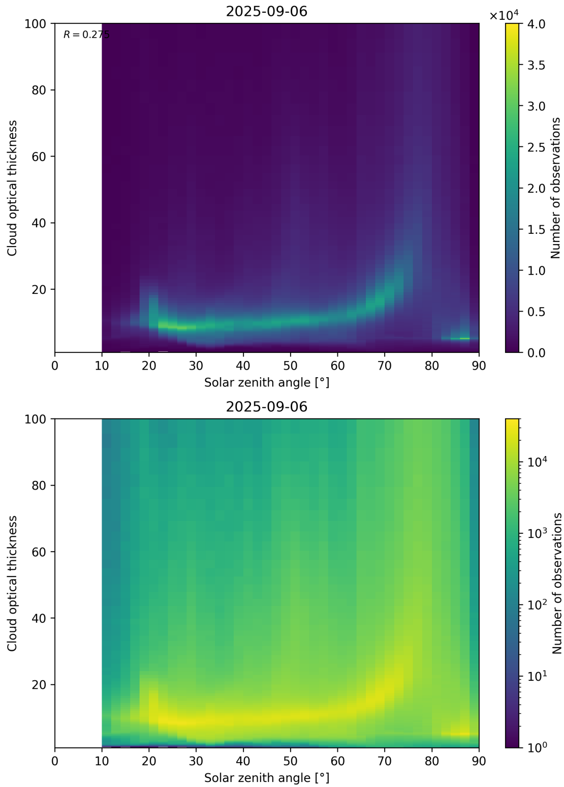
Figure 103: Scatter density plot of “Solar zenith angle” against “Cloud optical thickness” for 2025-09-05 to 2025-09-07.
