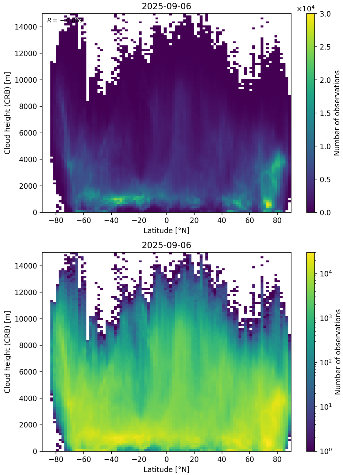
Figure 95: Scatter density plot of “Latitude” against “Cloud height (CRB)” for 2025-09-05 to 2025-09-07.
