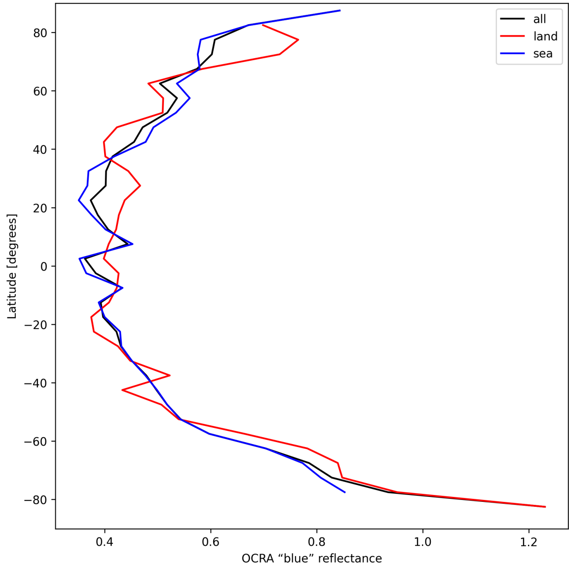
Figure 35: Zonal average of "OCRA "blue" reflectance" for 2025-09-05 to 2025-09-07.
