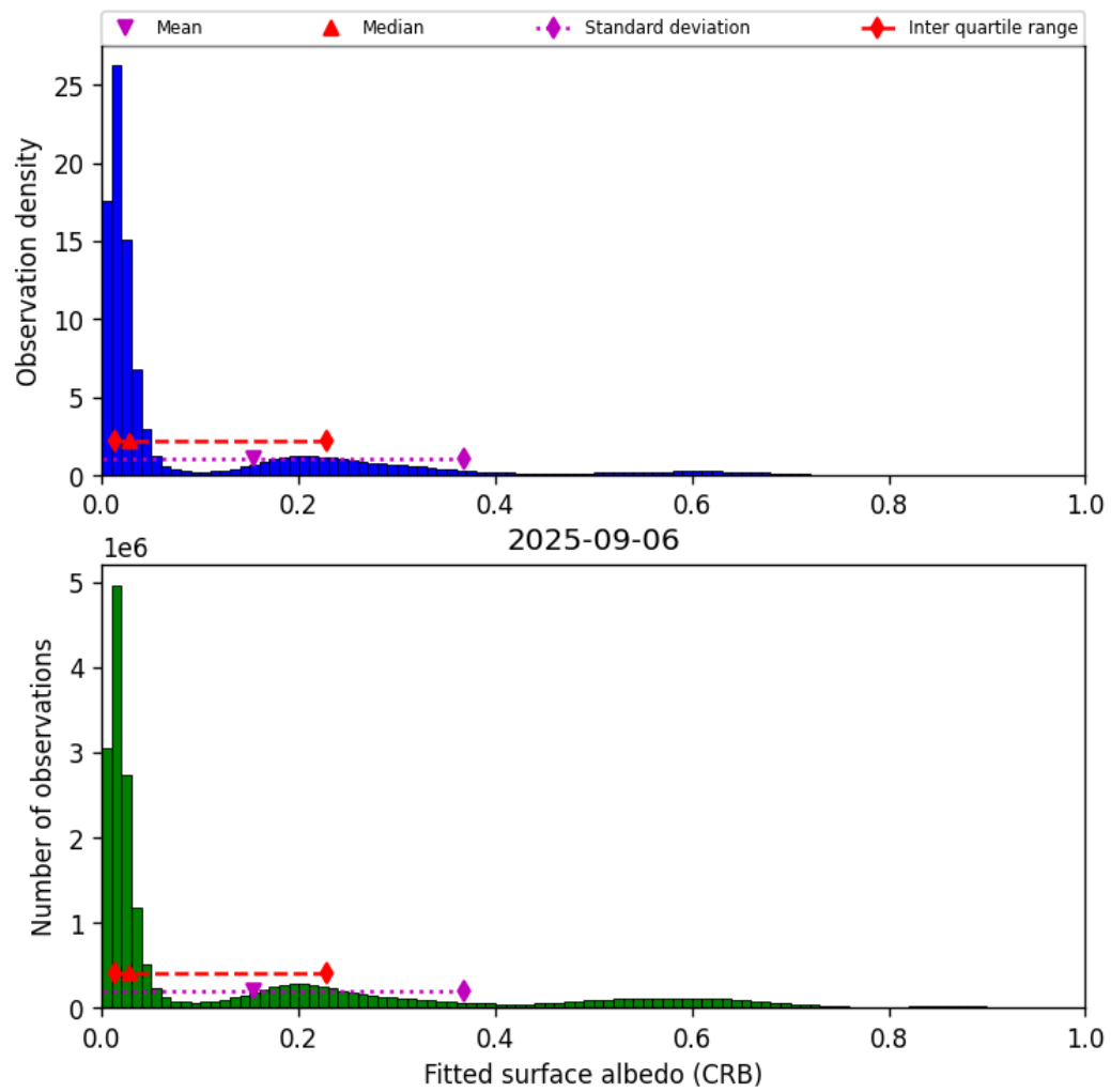
Figure 46: Histogram of “Fitted surface albedo (CRB)” for 2025-09-05 to 2025-09-07
