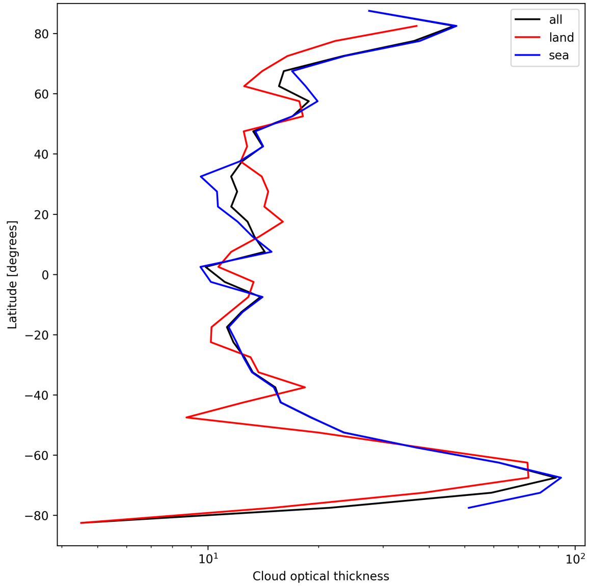
Figure 25: Zonal average of “Cloud optical thickness” for 2025-09-05 to 2025-09-07.
