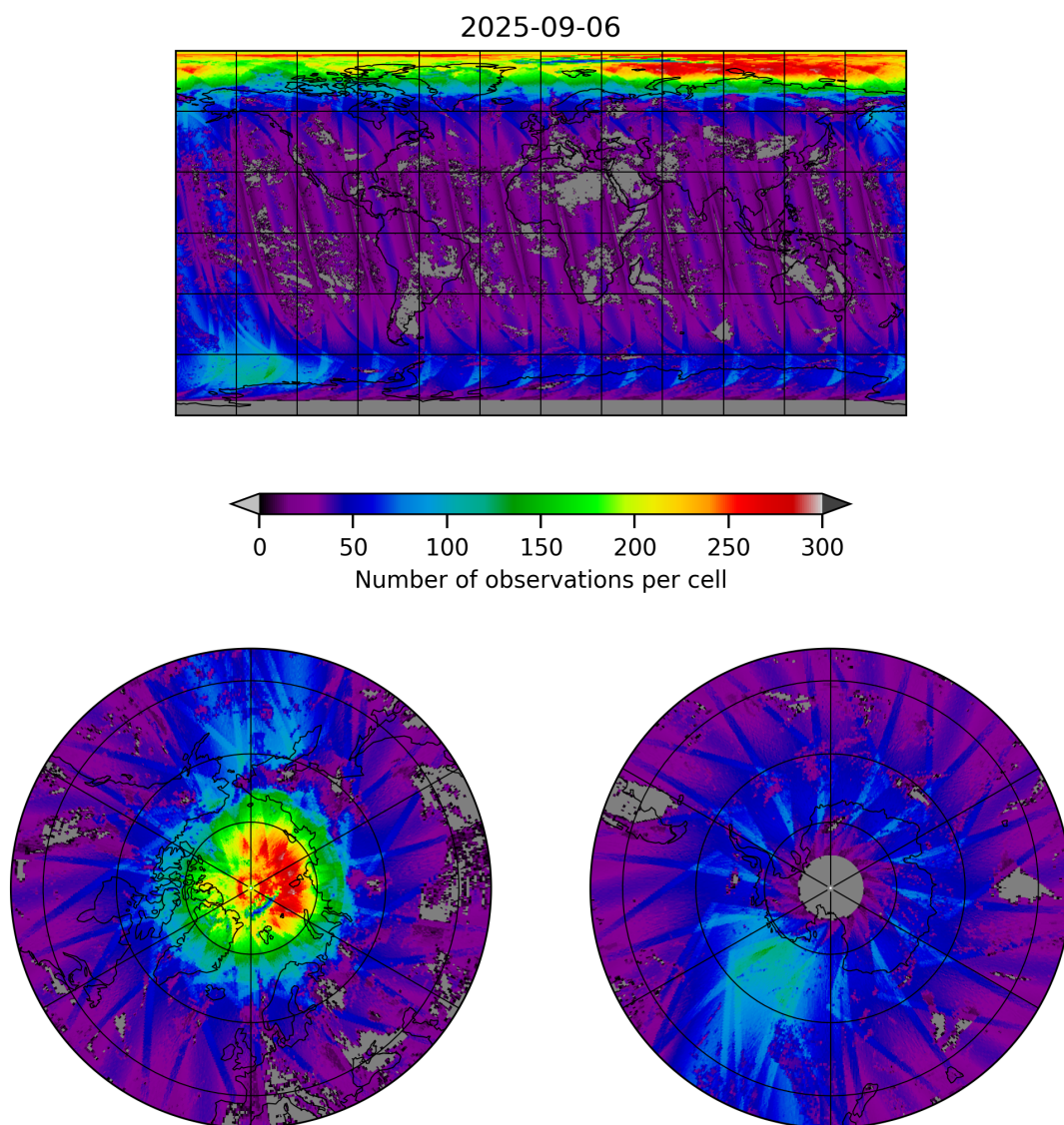
Figure 21: Map of the number of observations for 2025-09-05 to 2025-09-07
