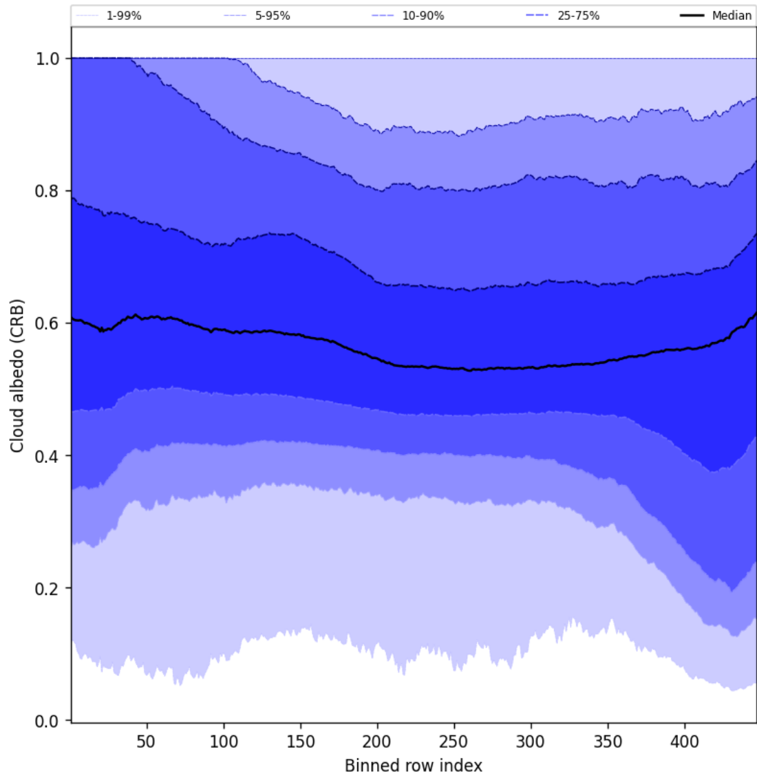
Figure 60: Along track statistics of “Cloud albedo (CRB)” for 2025-09-05 to 2025-09-07
