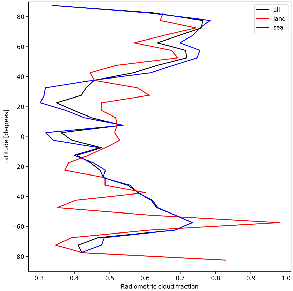
Figure 23: Zonal average of “Radiometric cloud fraction” for 2025-09-05 to 2025-09-07.
