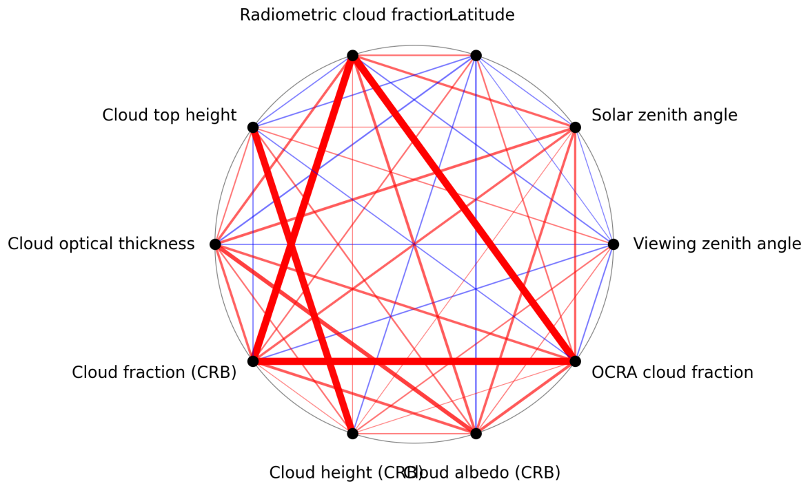
Figure 1: Map of correlation graph for 2025-09-05 to 2025-09-07.
