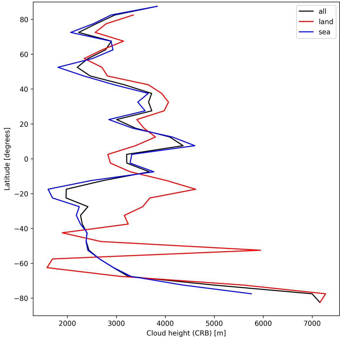
Figure 27: Zonal average of “Cloud height (CRB)” for 2025-09-05 to 2025-09-07.
