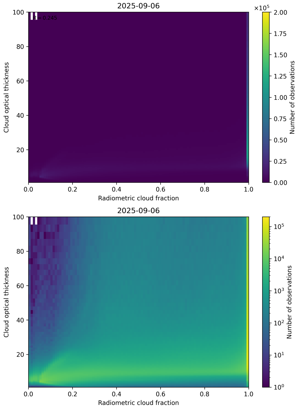
Figure 75: Scatter density plot of “Radiometric cloud fraction” against “Cloud optical thickness” for 2025-09-05 to 2025-09-07.
