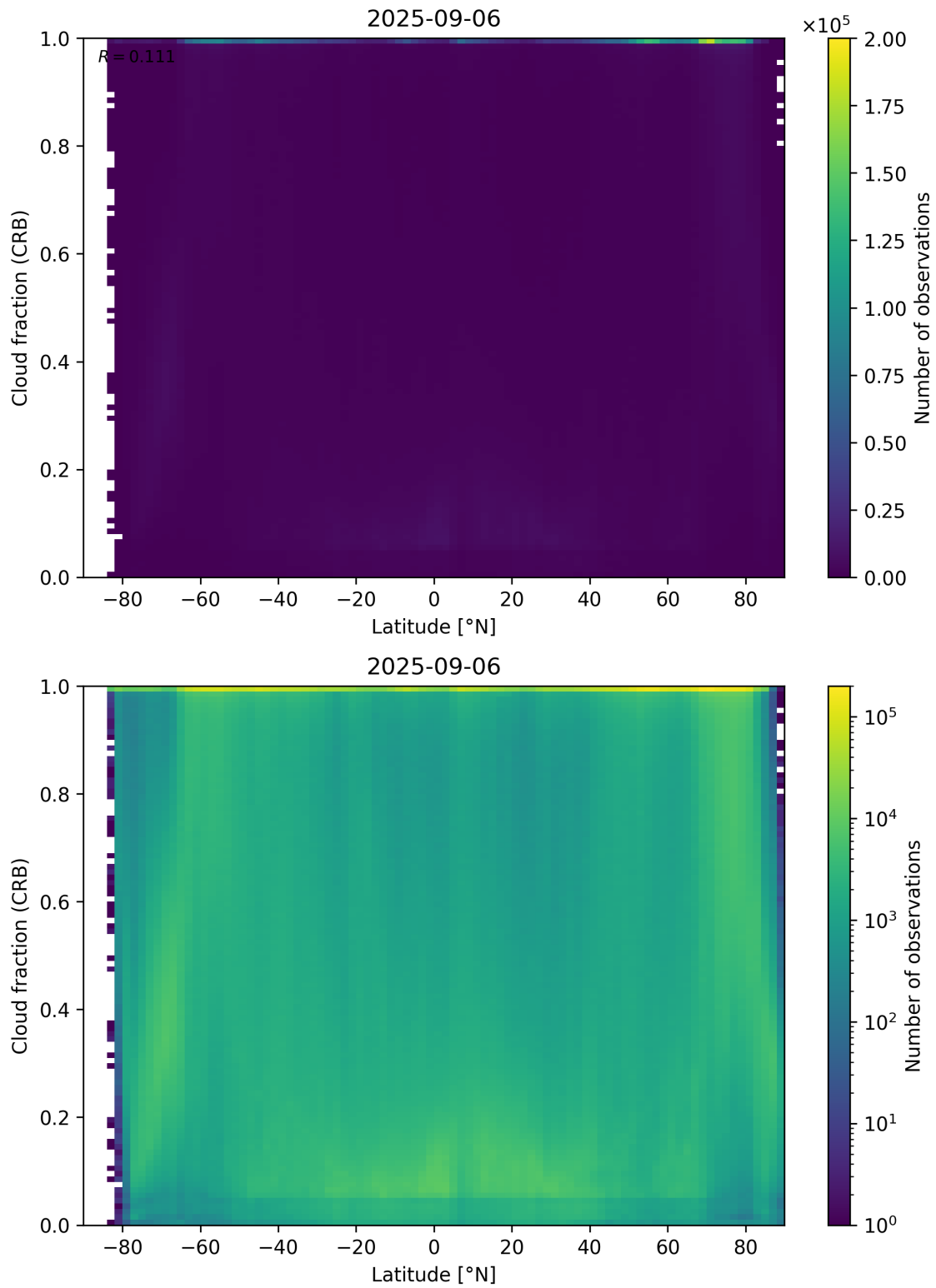
Figure 94: Scatter density plot of “Latitude” against “Cloud fraction (CRB)” for 2025-09-05 to 2025-09-07.
