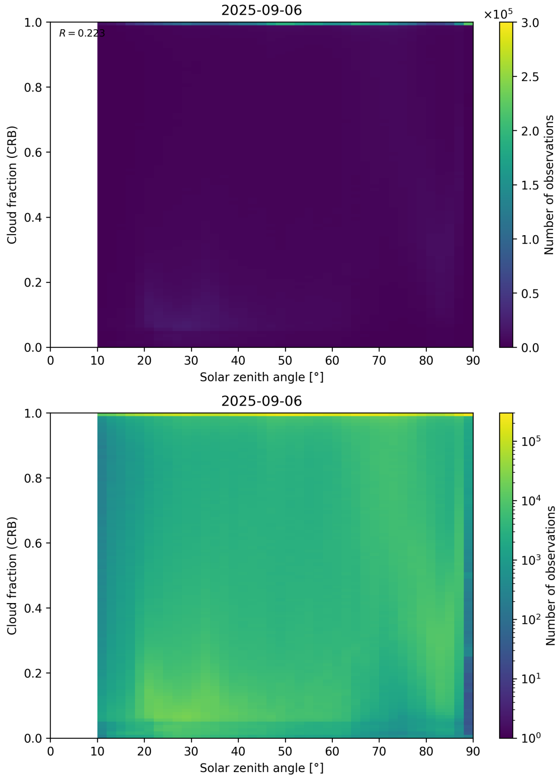
Figure 101: Scatter density plot of “Solar zenith angle” against “Cloud fraction (CRB)” for 2025-09-05 to 2025-09-07.
