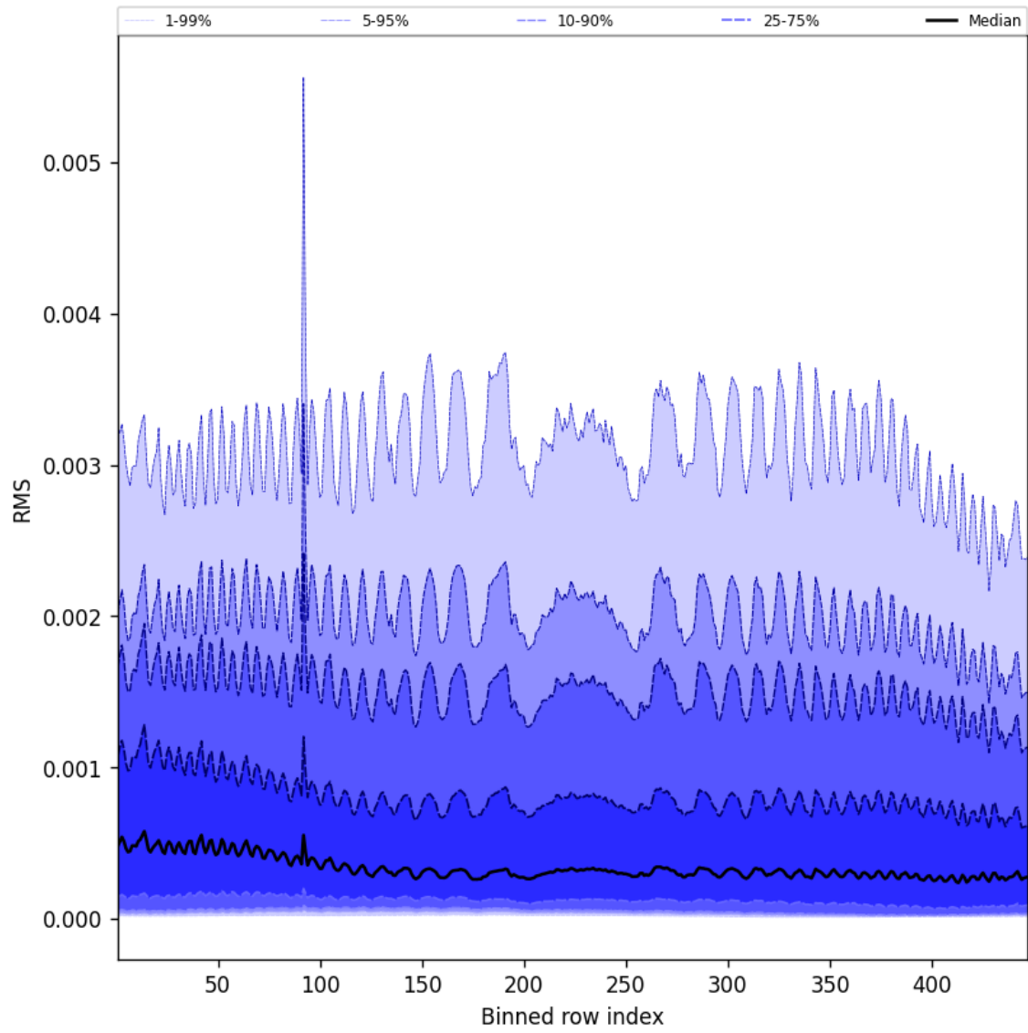
Figure 63: Along track statistics of “RMS” for 2025-09-05 to 2025-09-07
