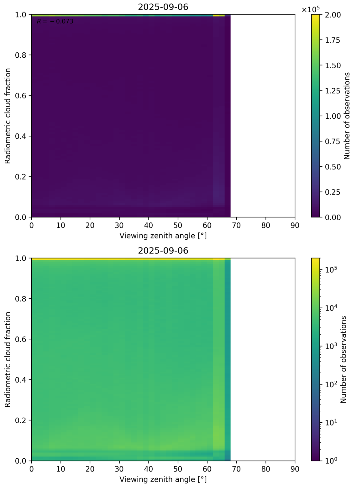
Figure 107: Scatter density plot of “Viewing zenith angle” against “Radiometric cloud fraction” for 2025-09-05 to 2025-09-07.
