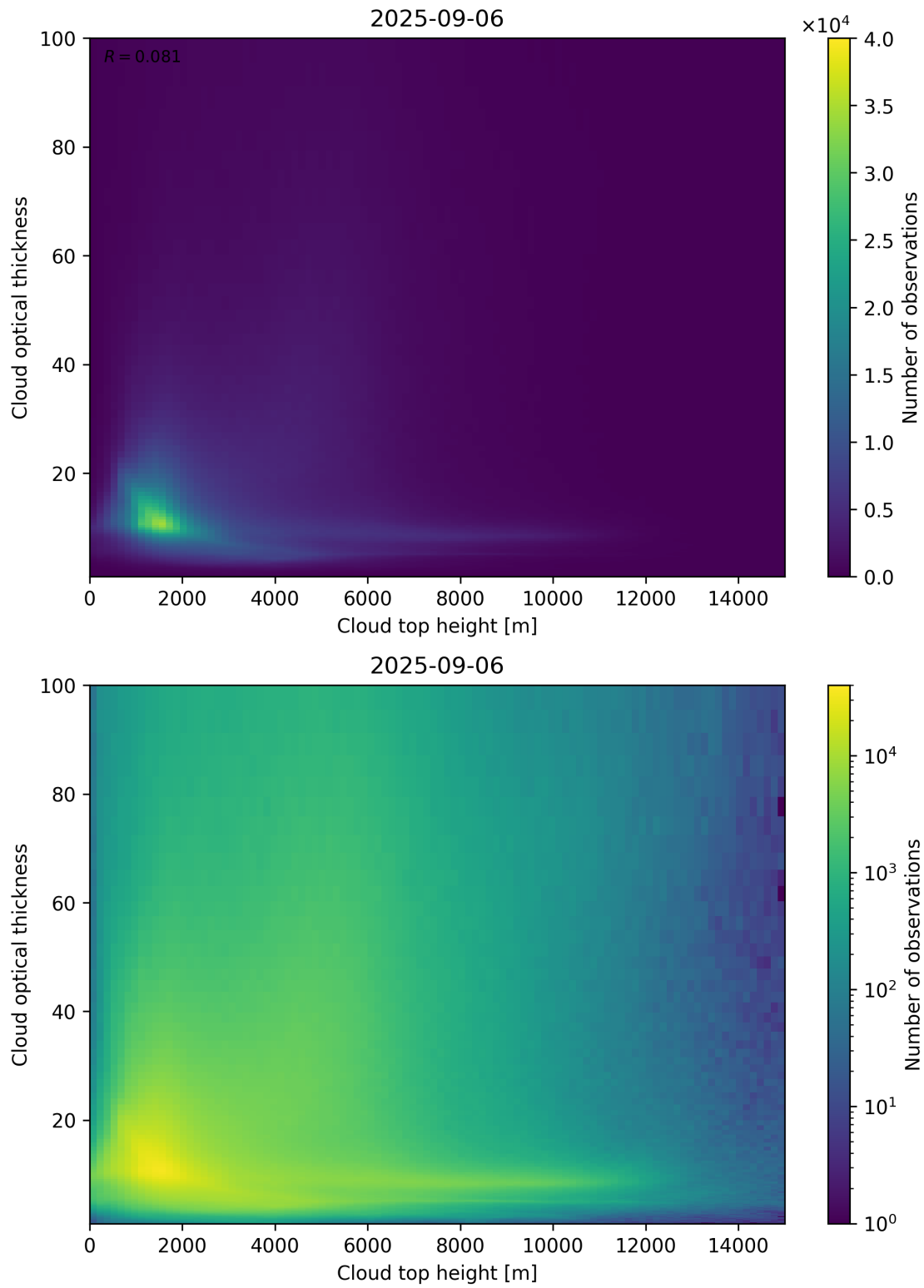
Figure 90: Scatter density plot of “Cloud top height” against “Cloud optical thickness” for 2025-09-05 to 2025-09-07.
