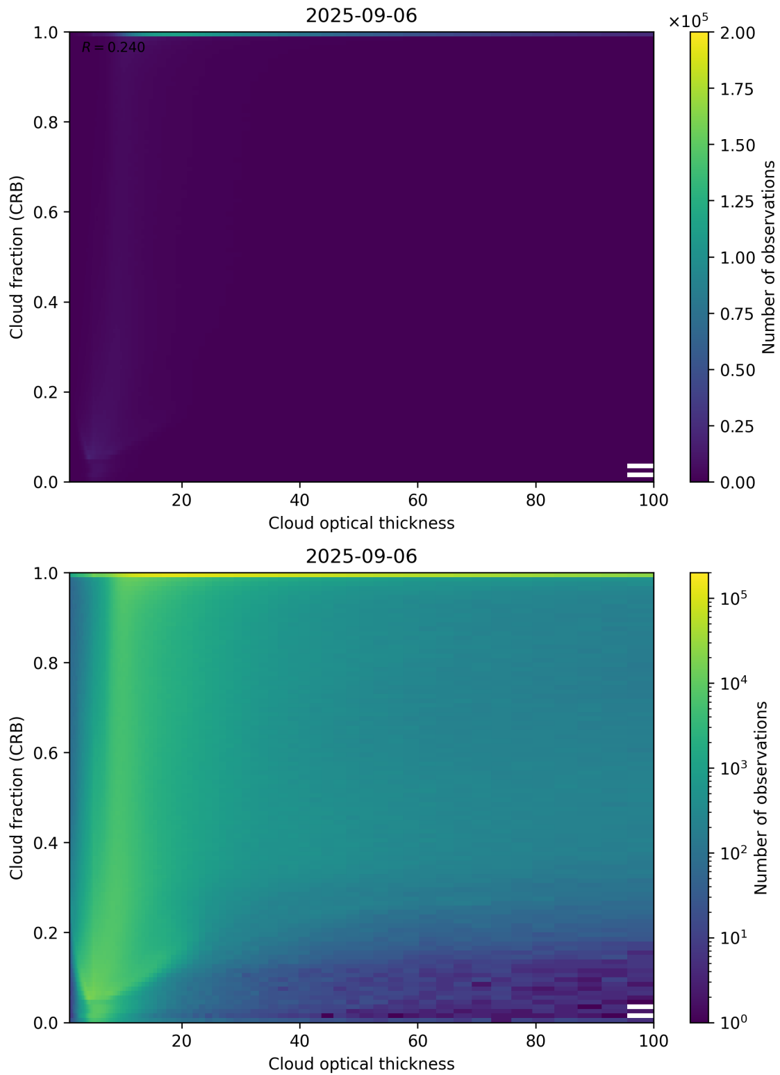
Figure 84: Scatter density plot of “Cloud optical thickness” against “Cloud fraction (CRB)” for 2025-09-05 to 2025-09-07.
