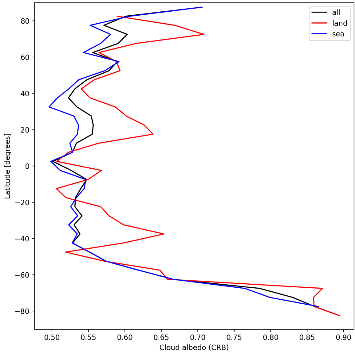
Figure 28: Zonal average of “Cloud albedo (CRB)” for 2025-09-05 to 2025-09-07.
