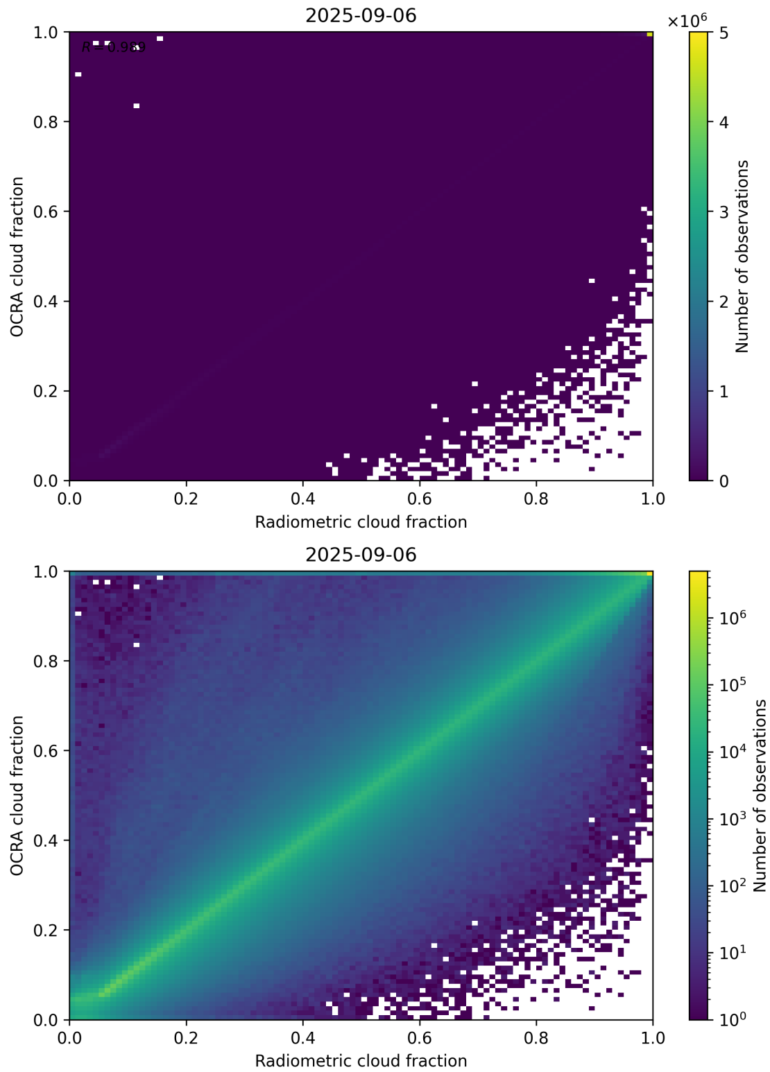
Figure 72: Scatter density plot of “Radiometric cloud fraction” against “OCRA cloud fraction” for 2025-09-05 to 2025-09-07.
