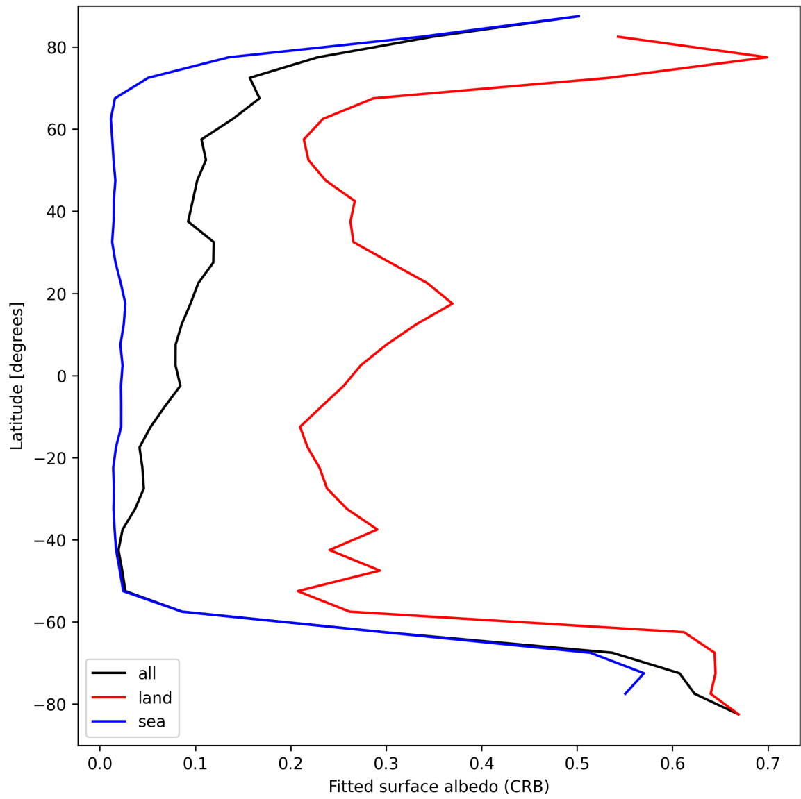
Figure 30: Zonal average of “Fitted surface albedo (CRB)” for 2025-09-05 to 2025-09-07.
