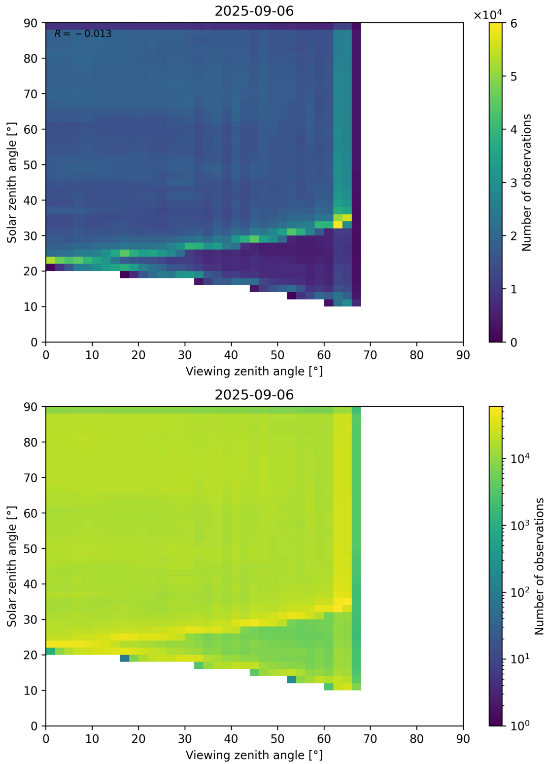
Figure 114: Scatter density plot of “Viewing zenith angle” against “Solar zenith angle” for 2025-09-05 to 2025-09-07.
