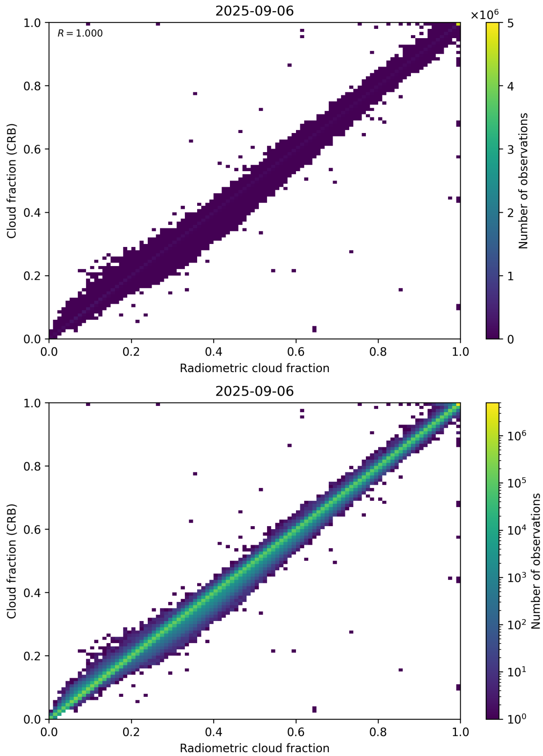
Figure 73: Scatter density plot of “Radiometric cloud fraction” against “Cloud fraction (CRB)” for 2025-09-05 to 2025-09-07.
