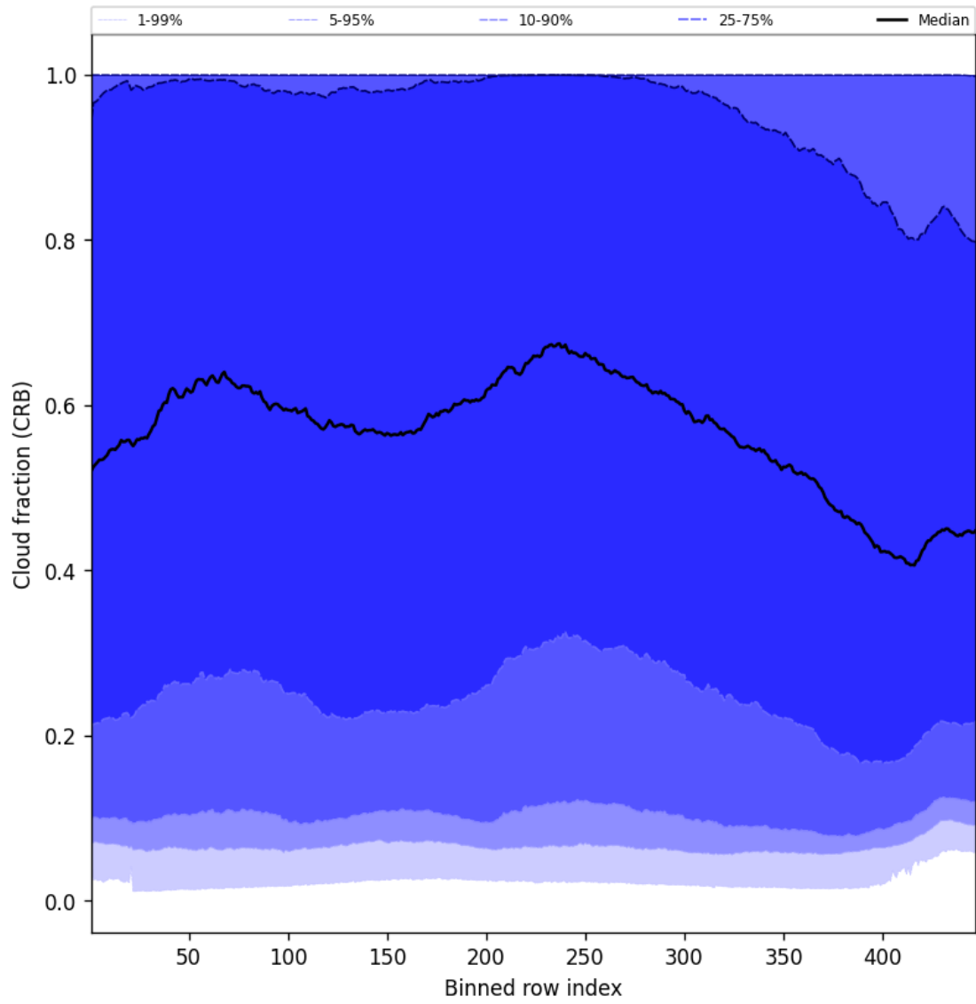
Figure 58: Along track statistics of “Cloud fraction (CRB)” for 2025-09-05 to 2025-09-07
