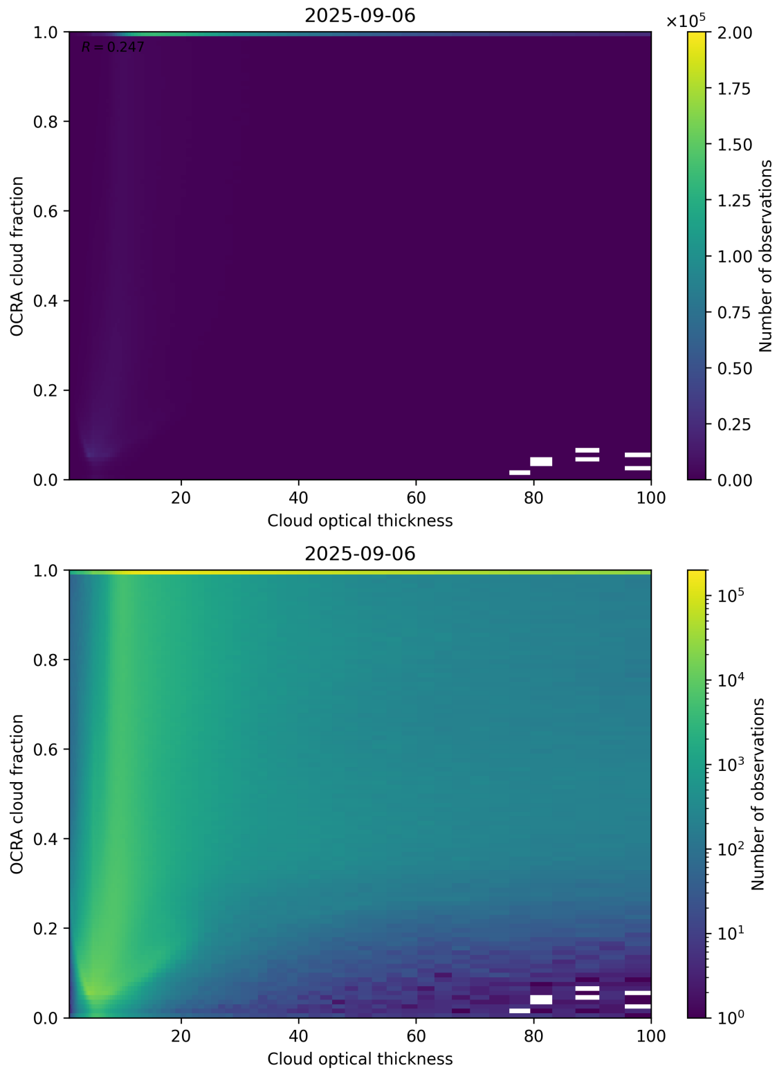
Figure 83: Scatter density plot of “Cloud optical thickness” against “OCRA cloud fraction” for 2025-09-05 to 2025-09-07.
