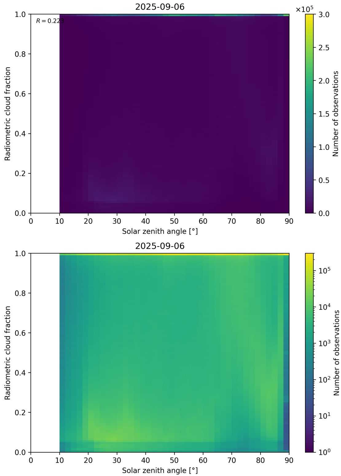
Figure 99: Scatter density plot of “Solar zenith angle” against “Radiometric cloud fraction” for 2025-09-05 to 2025-09-07.
