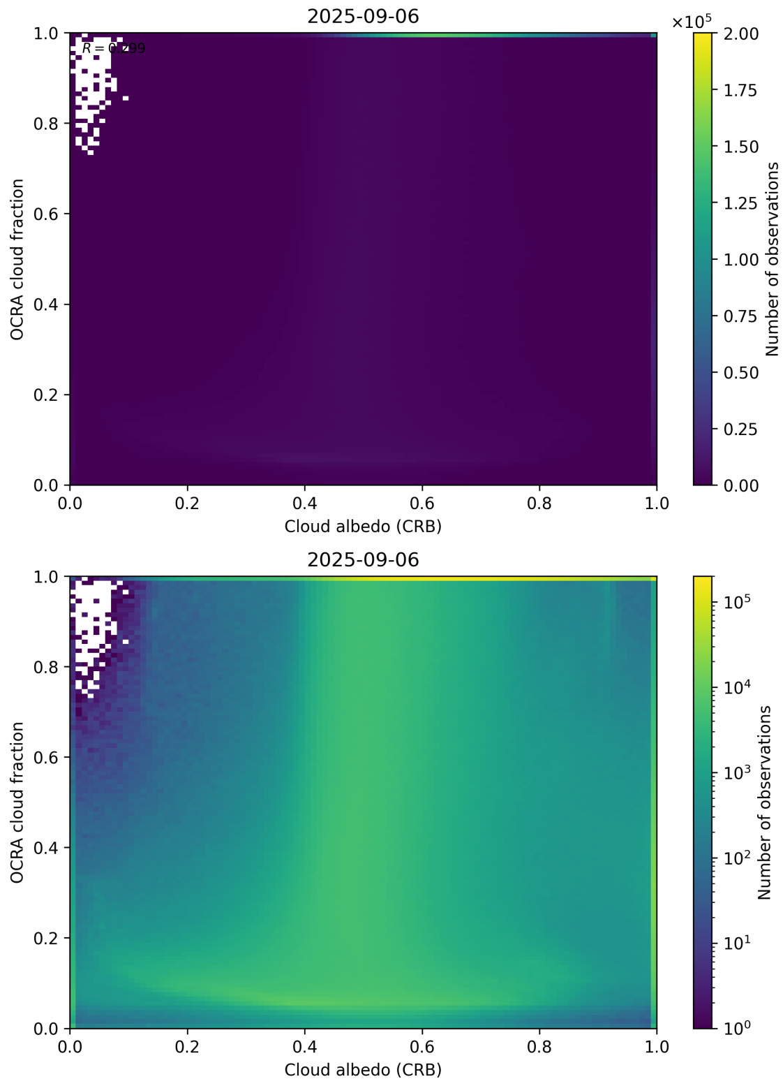
Figure 70: Scatter density plot of “Cloud albedo (CRB)” against “OCRA cloud fraction” for 2025-09-05 to 2025-09-07.
