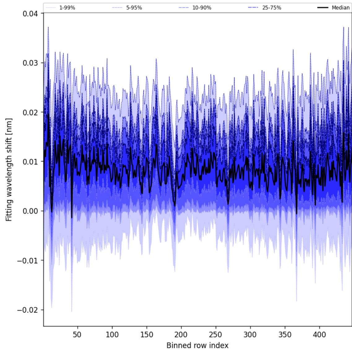
Figure 65: Along track statistics of “Fitting wavelength shift” for 2025-09-05 to 2025-09-07
