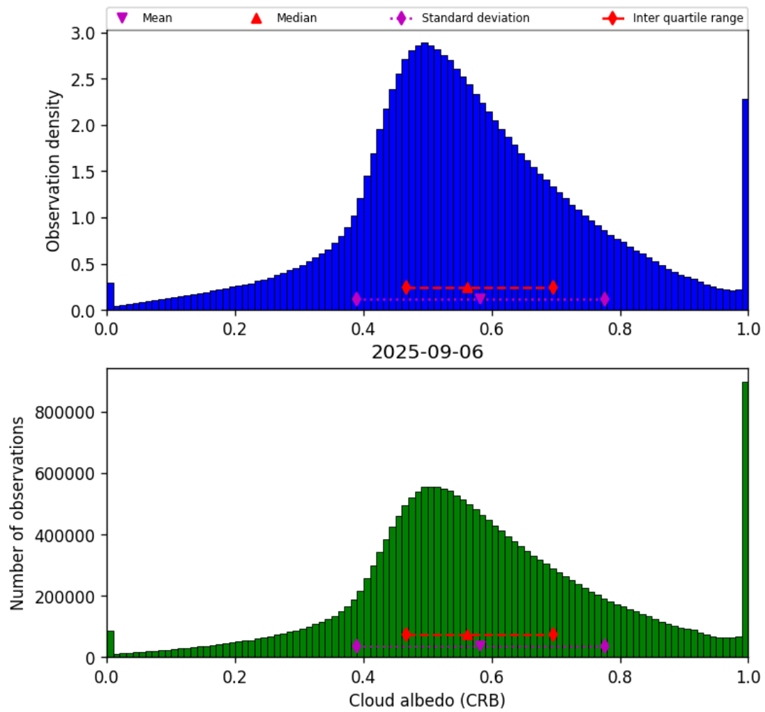
Figure 44: Histogram of “Cloud albedo (CRB)” for 2025-09-05 to 2025-09-07
