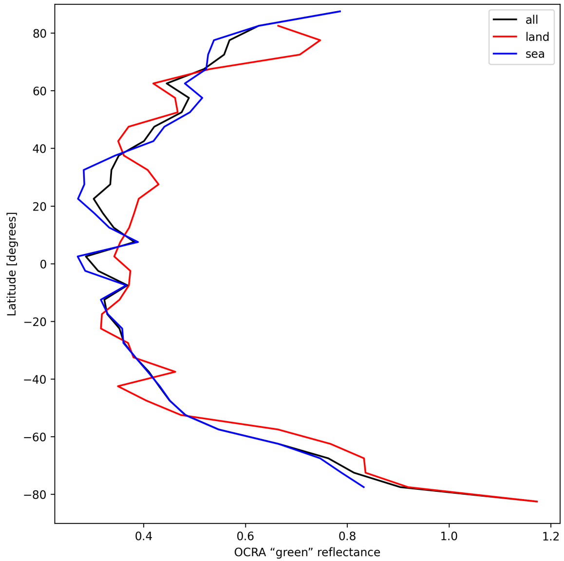
Figure 36: Zonal average of “OCRA “green” reflectance” for 2025-09-05 to 2025-09-07.
