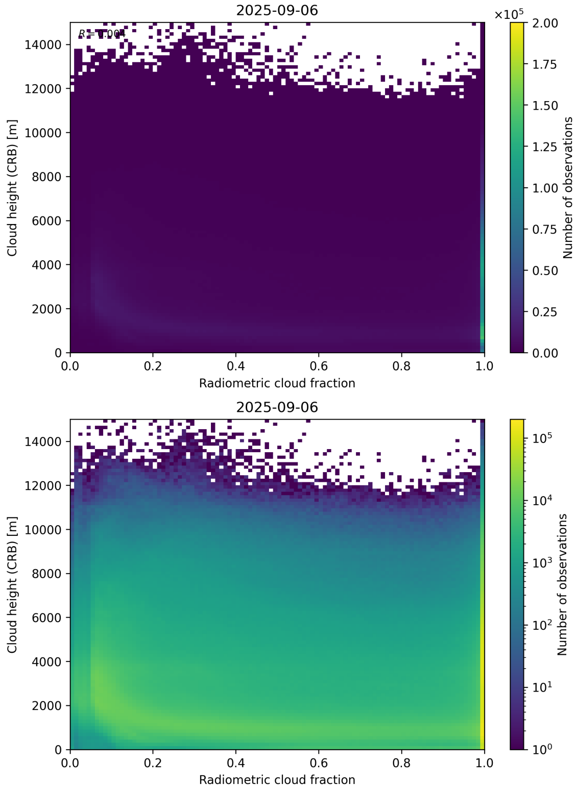
Figure 74: Scatter density plot of “Radiometric cloud fraction” against “Cloud height (CRB)” for 2025-09-05 to 2025-09-07.
