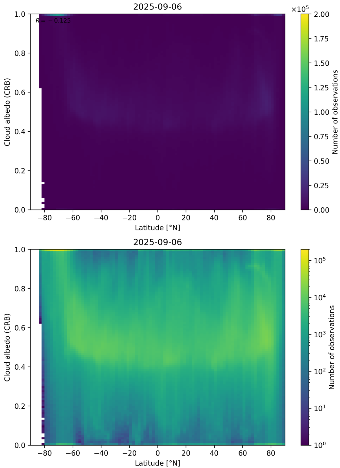
Figure 91: Scatter density plot of “Latitude” against “Cloud albedo (CRB)” for 2025-09-05 to 2025-09-07.
