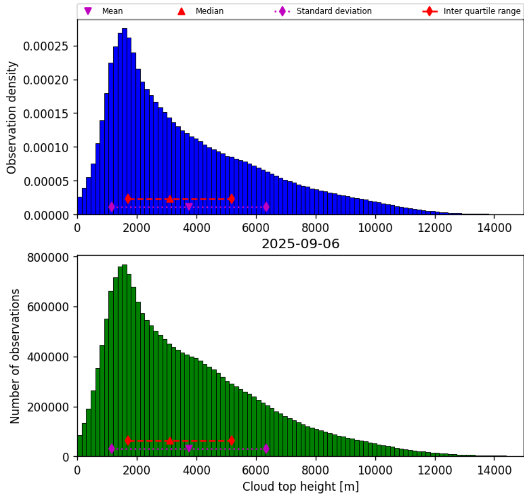
Figure 40: Histogram of “Cloud top height” for 2025-09-05 to 2025-09-07
