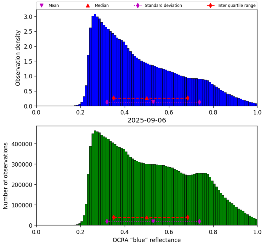
Figure 51: Histogram of “OCRA “blue” reflectance” for 2025-09-05 to 2025-09-07
