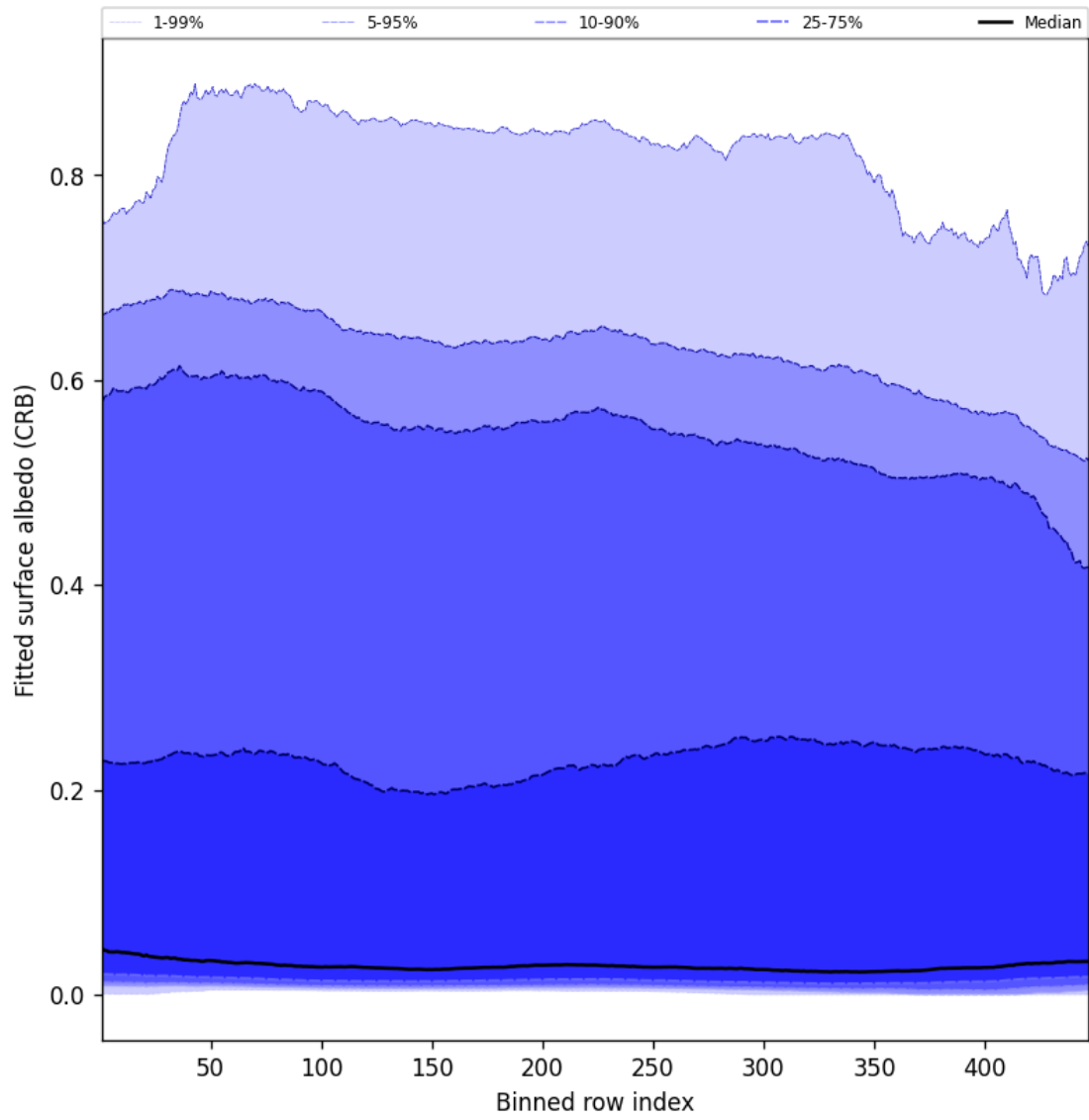
Figure 62: Along track statistics of “Fitted surface albedo (CRB)” for 2025-09-05 to 2025-09-07
