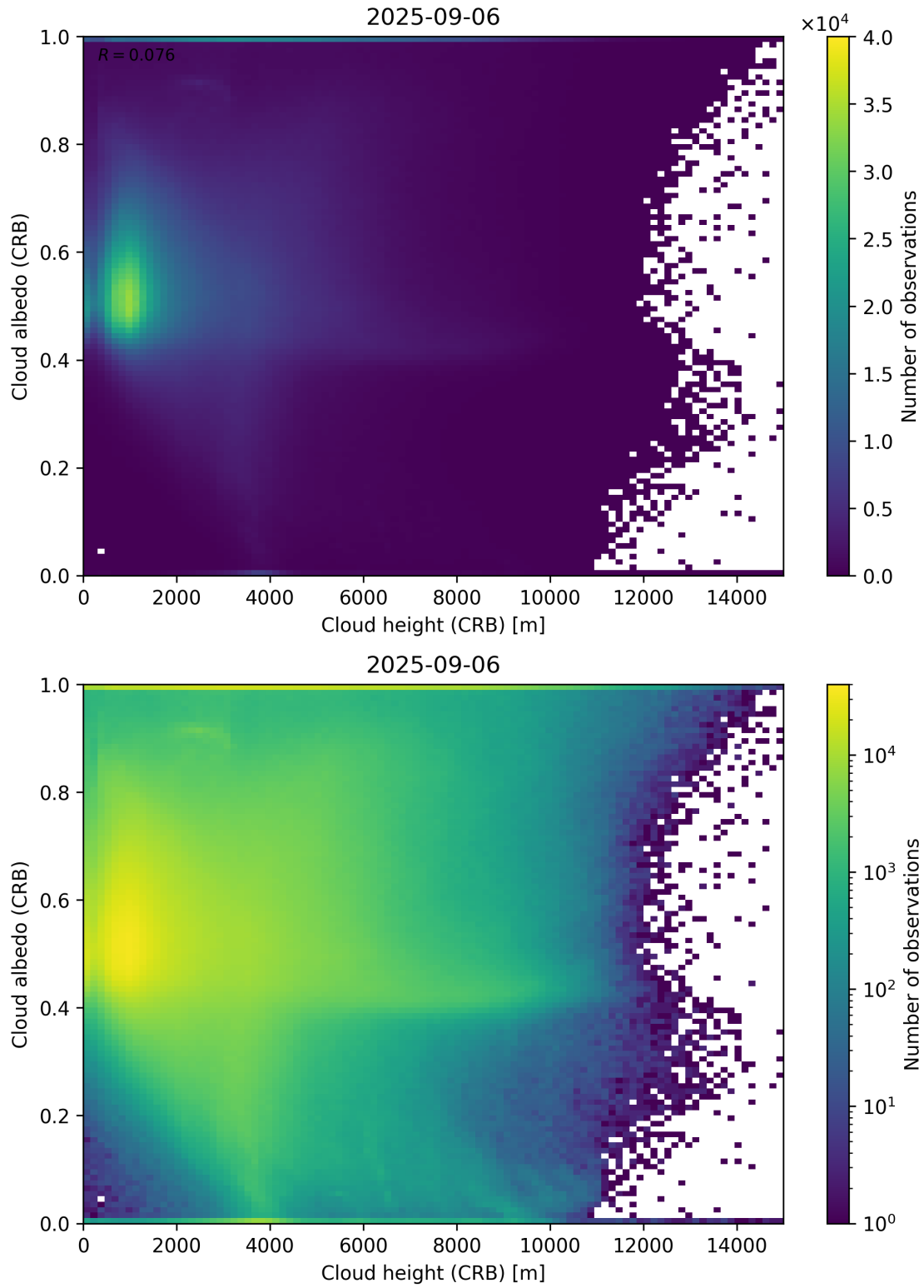
Figure 80: Scatter density plot of “Cloud height (CRB)” against “Cloud albedo (CRB)” for 2025-09-05 to 2025-09-07.
