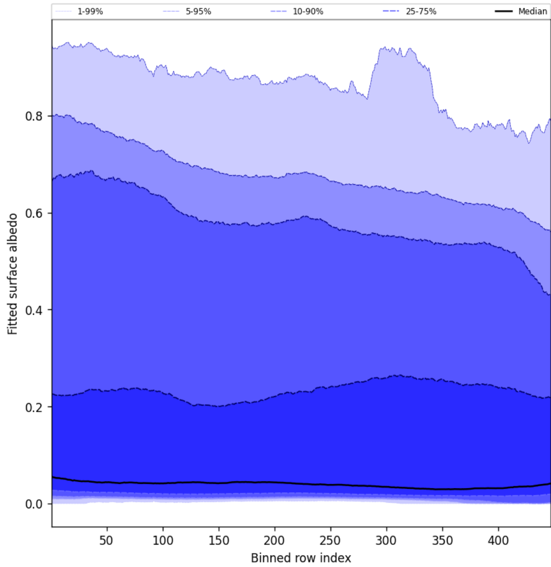
Figure 61: Along track statistics of “Fitted surface albedo” for 2025-09-05 to 2025-09-07
