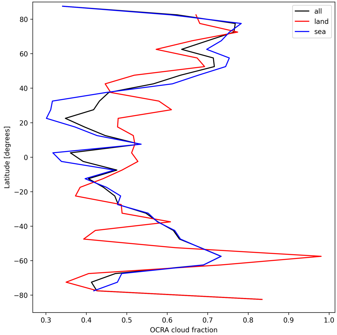
Figure 34: Zonal average of “OCRA cloud fraction” for 2025-09-05 to 2025-09-07.
