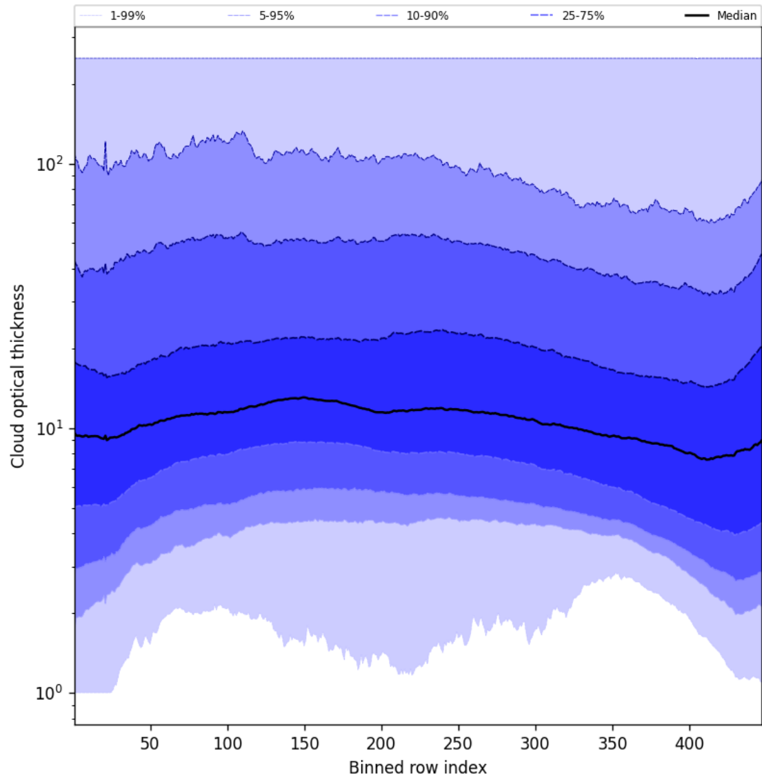
Figure 57: Along track statistics of “Cloud optical thickness” for 2025-09-05 to 2025-09-07
