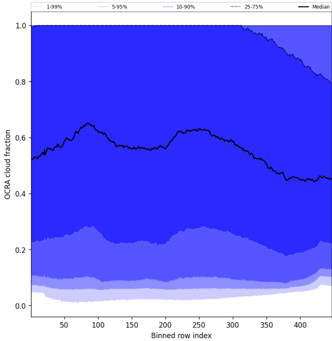
Figure 66: Along track statistics of “OCRA cloud fraction” for 2025-09-07 to 2025-09-09
