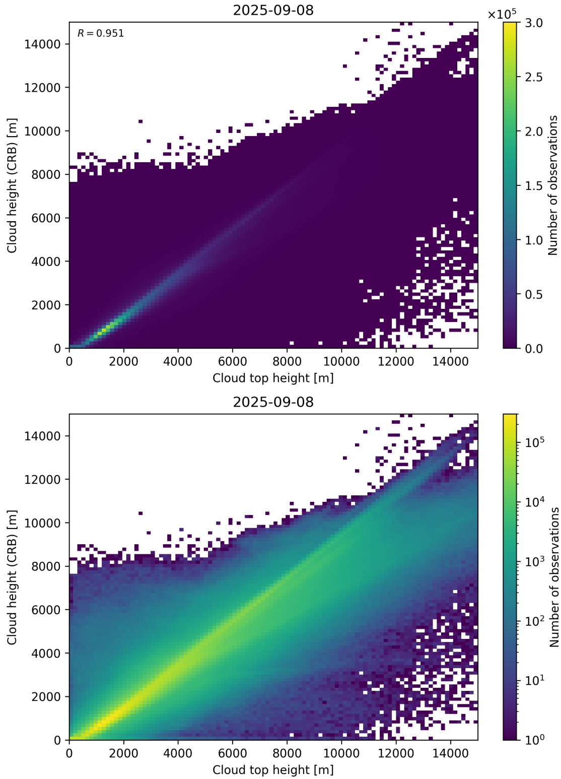
Figure 89: Scatter density plot of “Cloud top height” against “Cloud height (CRB)” for 2025-09-07 to 2025-09-09.
