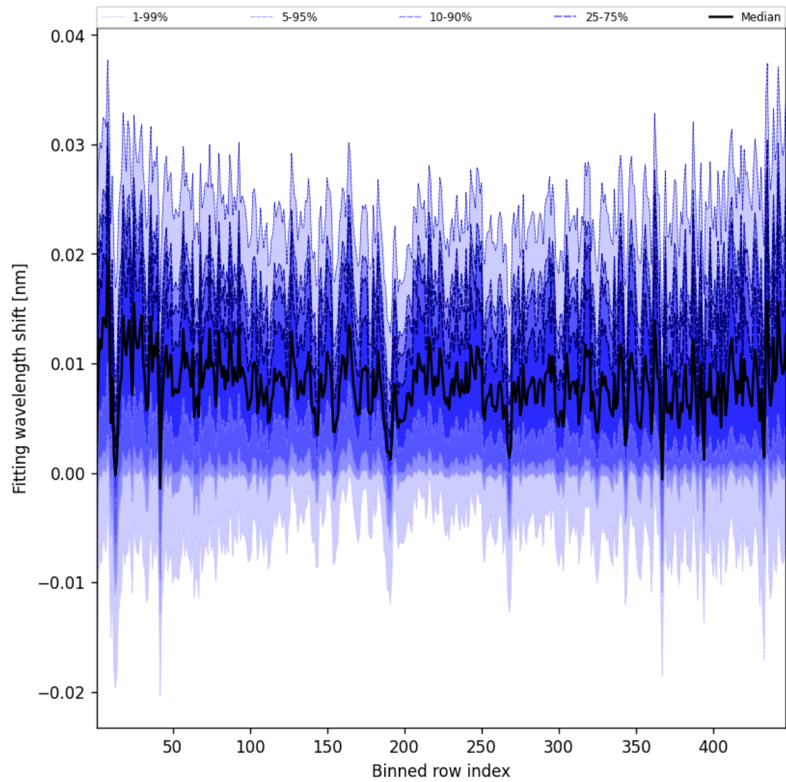
Figure 65: Along track statistics of “Fitting wavelength shift” for 2025-09-07 to 2025-09-09
