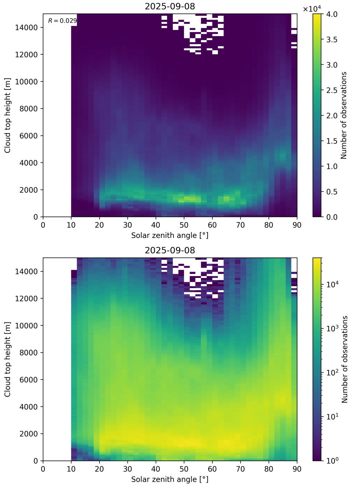
Figure 104: Scatter density plot of “Solar zenith angle” against “Cloud top height” for 2025-09-07 to 2025-09-09.
