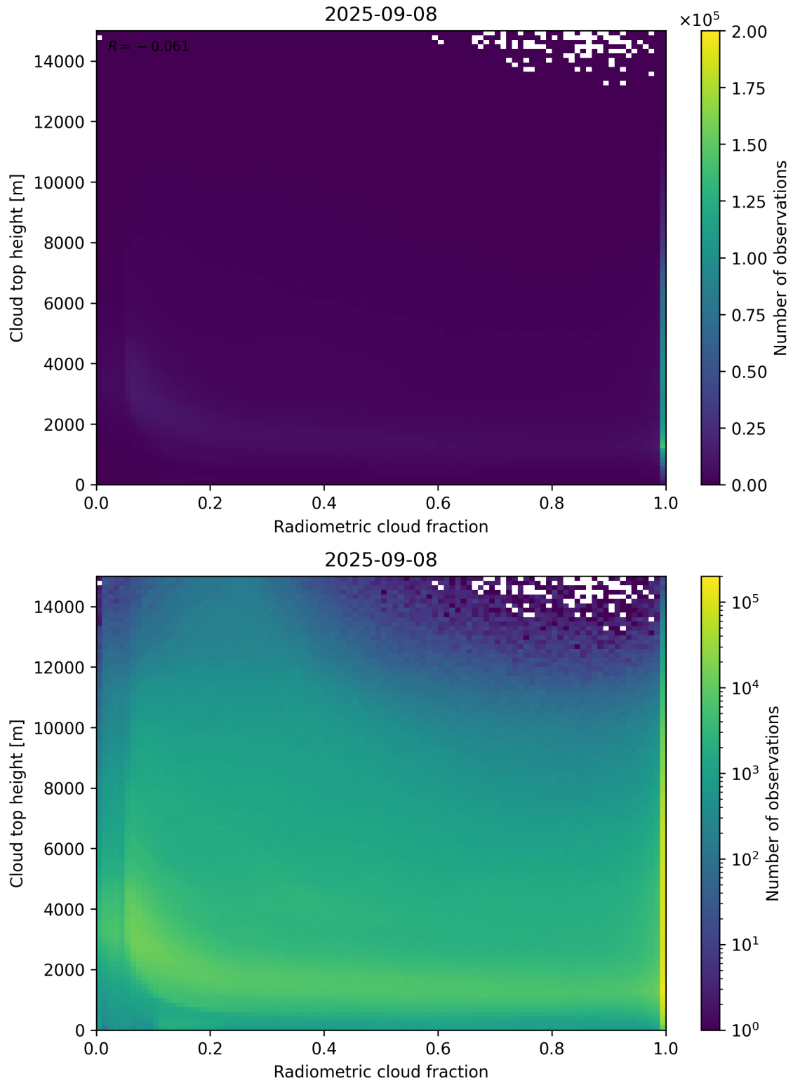
Figure 76: Scatter density plot of “Radiometric cloud fraction” against “Cloud top height” for 2025-09-07 to 2025-09-09.
