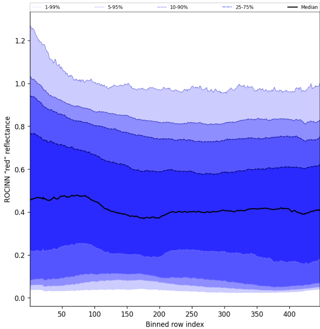
Figure 69: Along track statistics of “ROCINN “red” reflectance” for 2025-09-07 to 2025-09-09
