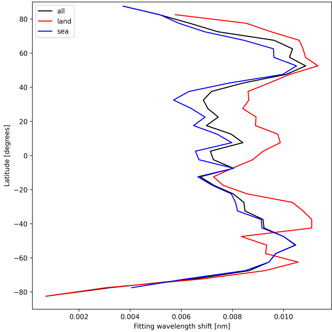
Figure 33: Zonal average of “Fitting wavelength shift” for 2025-09-07 to 2025-09-09.
