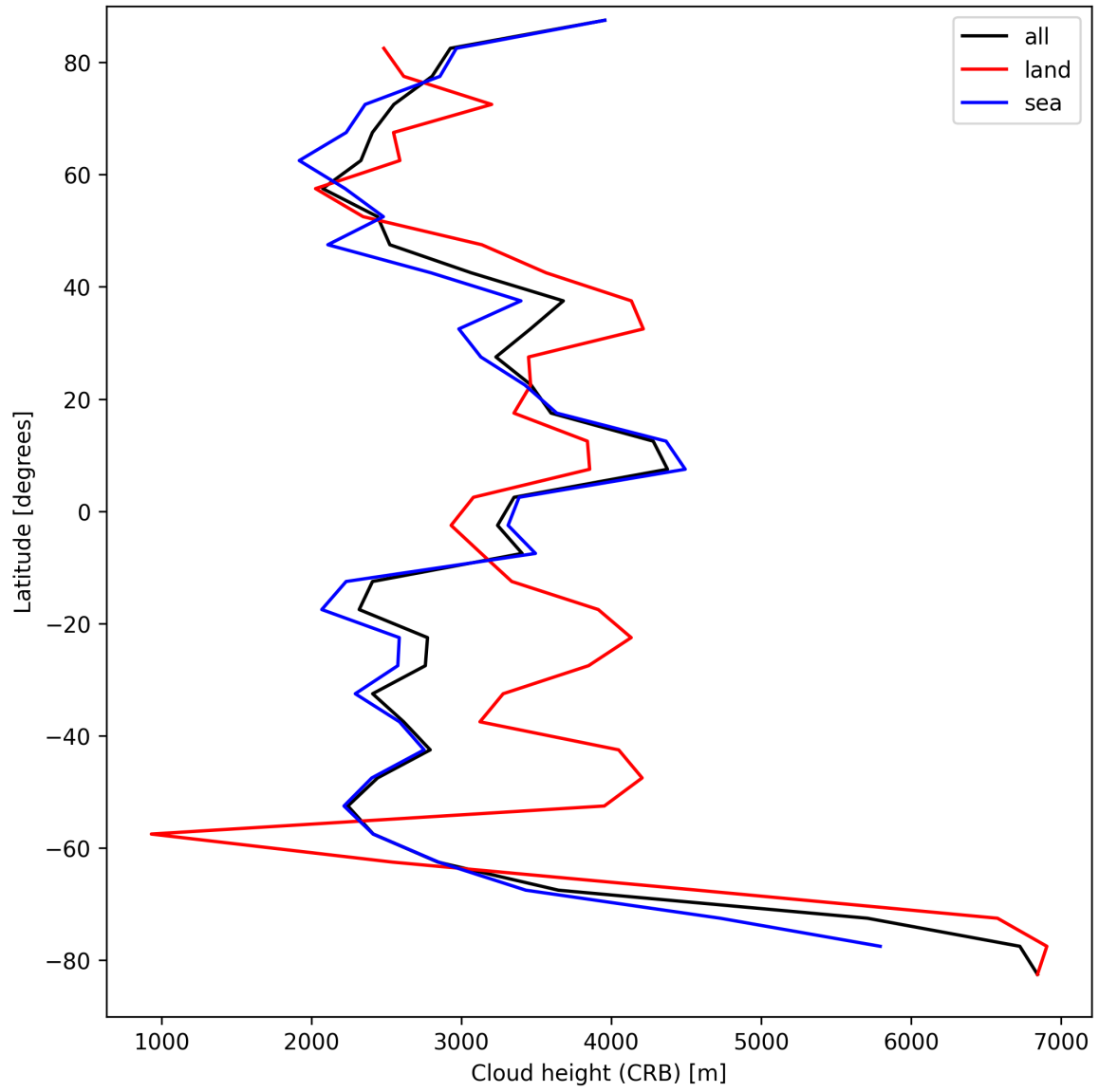
Figure 27: Zonal average of “Cloud height (CRB)” for 2025-09-07 to 2025-09-09.
