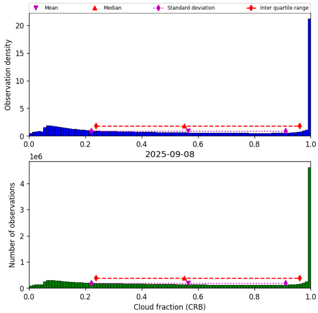
Figure 42: Histogram of “Cloud fraction (CRB)” for 2025-09-07 to 2025-09-09
