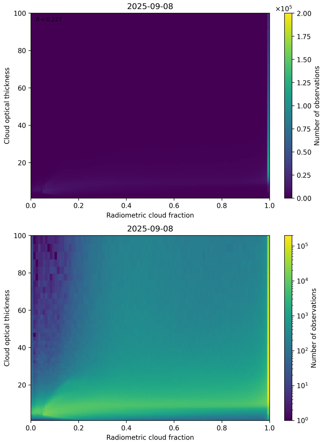
Figure 75: Scatter density plot of “Radiometric cloud fraction” against “Cloud optical thickness” for 2025-09-07 to 2025-09-09.
