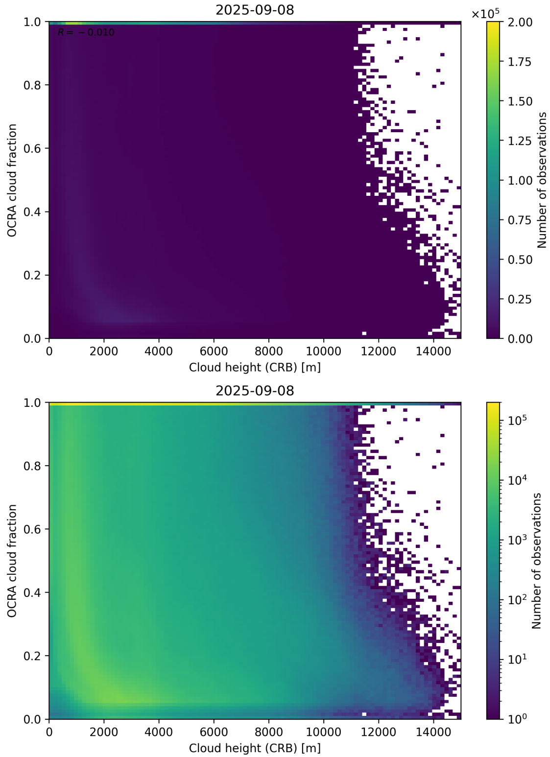
Figure 81: Scatter density plot of “Cloud height (CRB)” against “OCRA cloud fraction” for 2025-09-07 to 2025-09-09.
