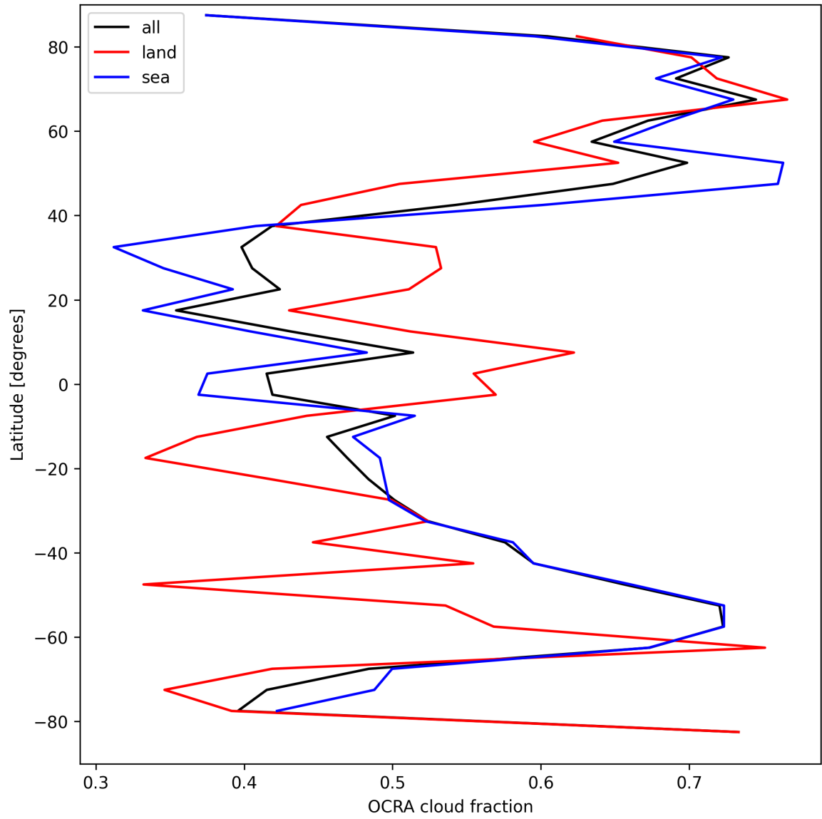
Figure 34: Zonal average of “OCRA cloud fraction” for 2025-09-07 to 2025-09-09.
