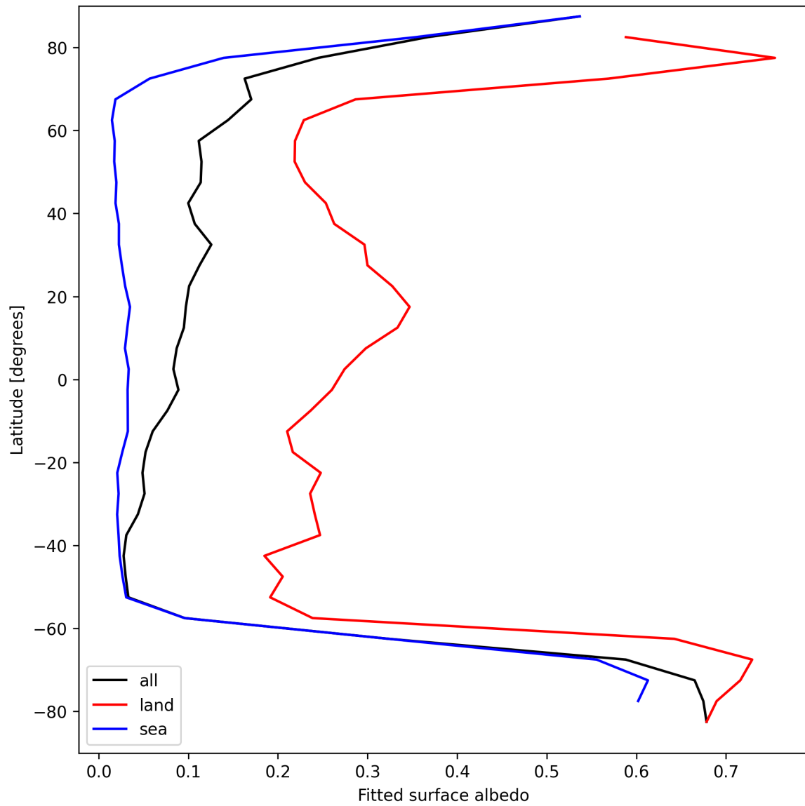
Figure 29: Zonal average of “Fitted surface albedo” for 2025-09-07 to 2025-09-09.
