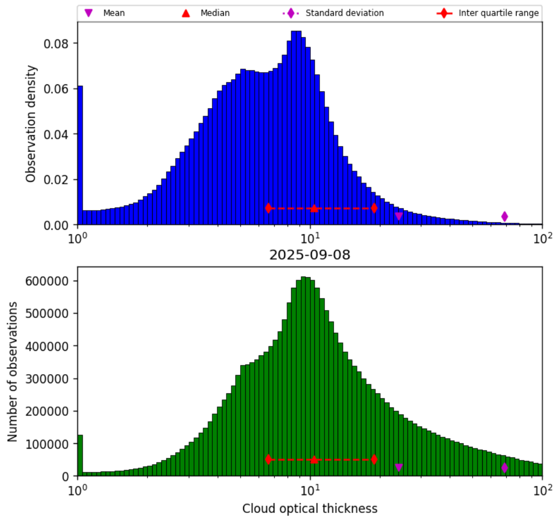
Figure 41: Histogram of “Cloud optical thickness” for 2025-09-07 to 2025-09-09
