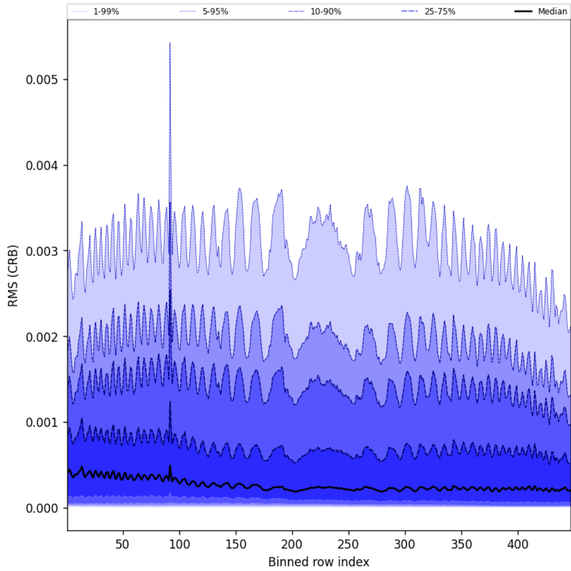
Figure 64: Along track statistics of “RMS (CRB)” for 2025-09-07 to 2025-09-09
