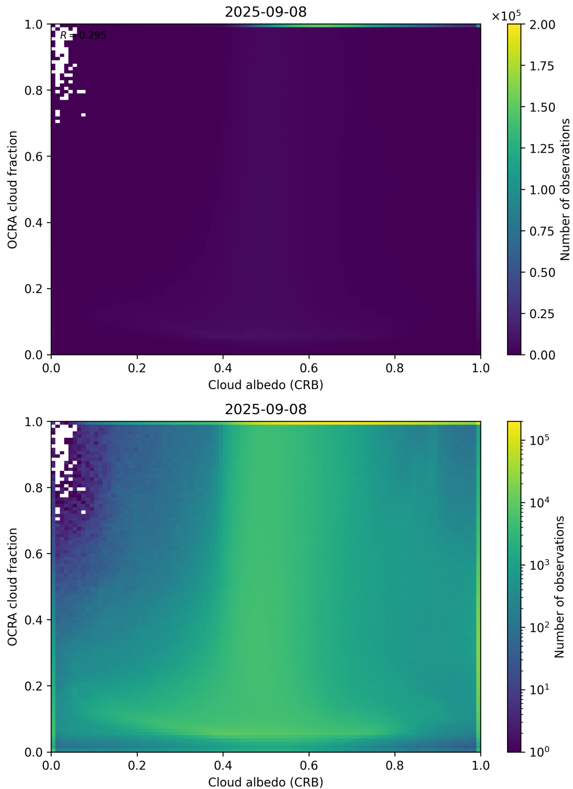
Figure 70: Scatter density plot of “Cloud albedo (CRB)” against “OCRA cloud fraction” for 2025-09-07 to 2025-09-09.
