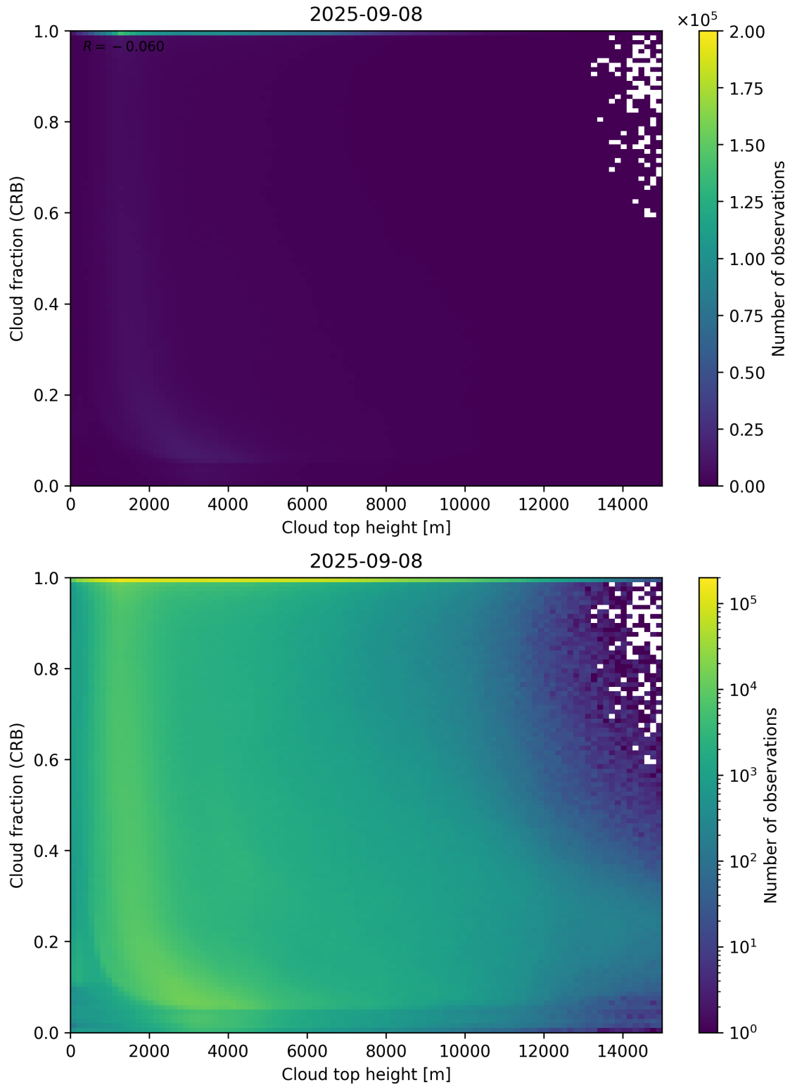
Figure 88: Scatter density plot of “Cloud top height” against “Cloud fraction (CRB)” for 2025-09-07 to 2025-09-09.
