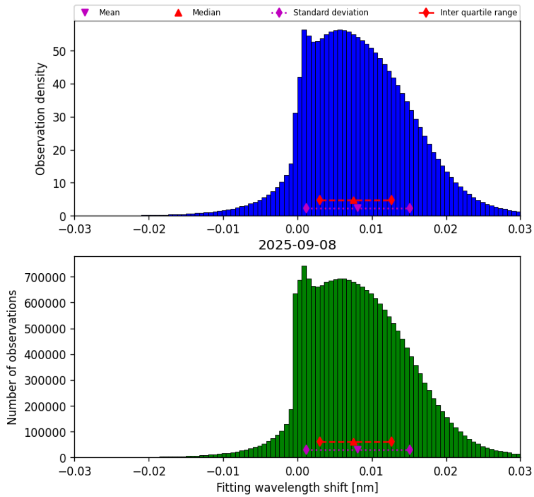
Figure 49: Histogram of “Fitting wavelength shift” for 2025-09-07 to 2025-09-09
