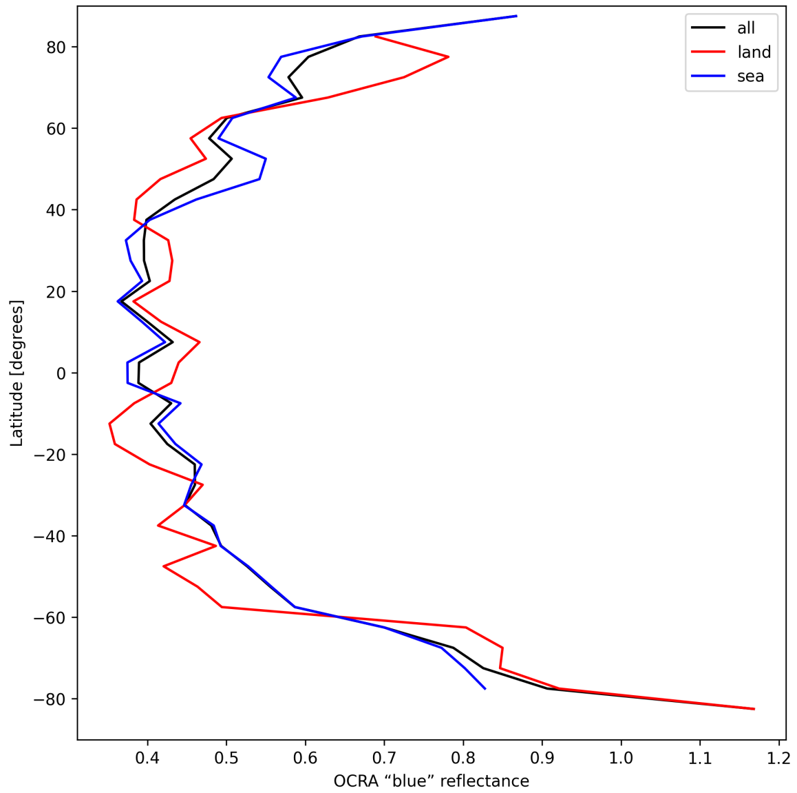
Figure 35: Zonal average of “OCRA “blue” reflectance” for 2025-09-07 to 2025-09-09.
