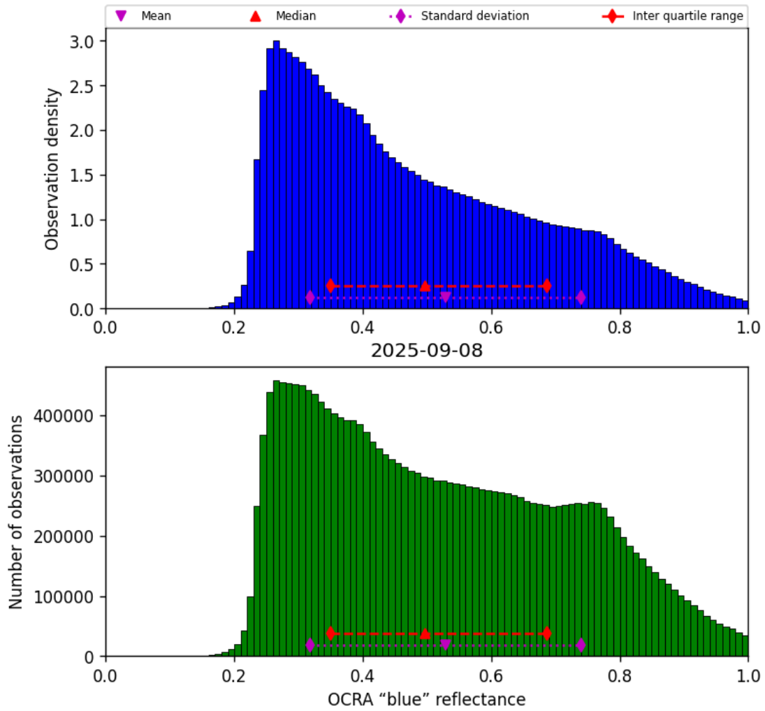
Figure 51: Histogram of “OCRA “blue” reflectance” for 2025-09-07 to 2025-09-09
