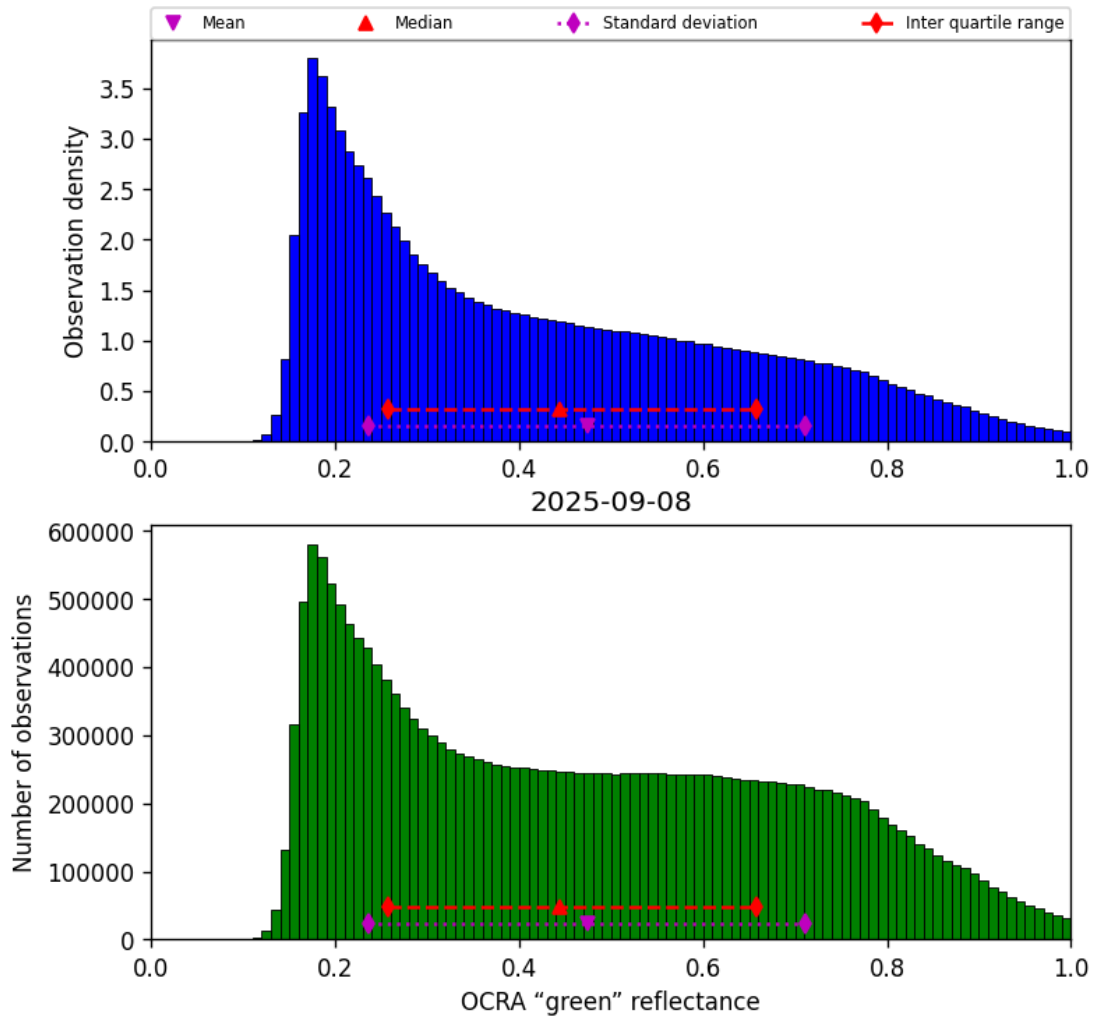
Figure 52: Histogram of “OCRA “green” reflectance” for 2025-09-07 to 2025-09-09
