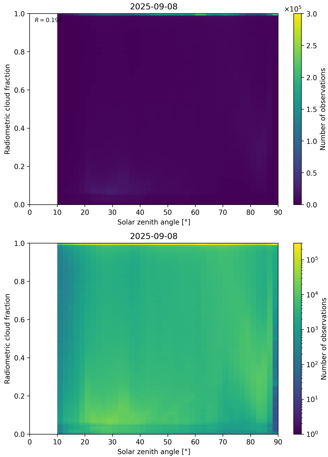
Figure 99: Scatter density plot of “Solar zenith angle” against “Radiometric cloud fraction” for 2025-09-07 to 2025-09-09.
