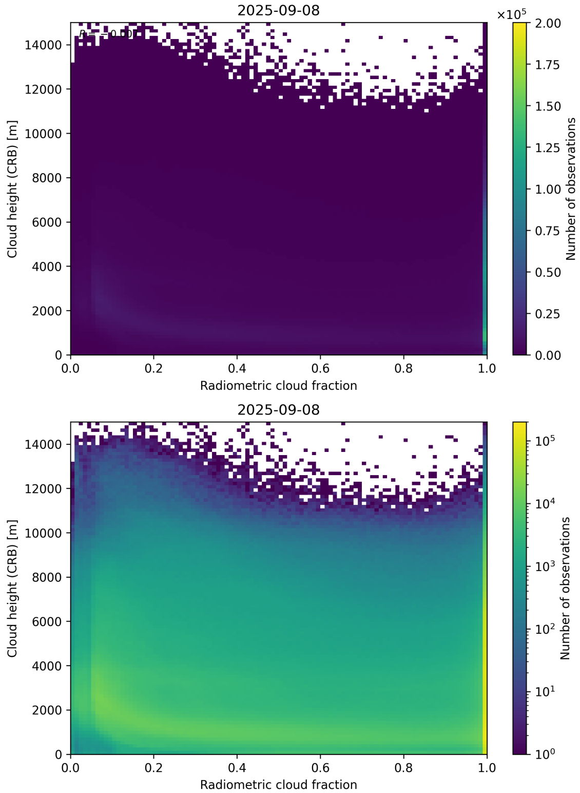
Figure 74: Scatter density plot of “Radiometric cloud fraction” against “Cloud height (CRB)” for 2025-09-07 to 2025-09-09.
