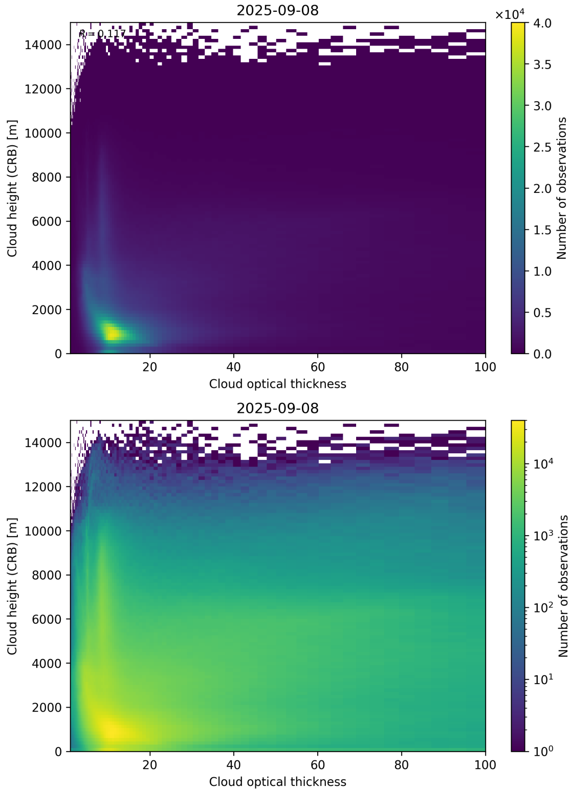
Figure 85: Scatter density plot of “Cloud optical thickness” against “Cloud height (CRB)” for 2025-09-07 to 2025-09-09.
