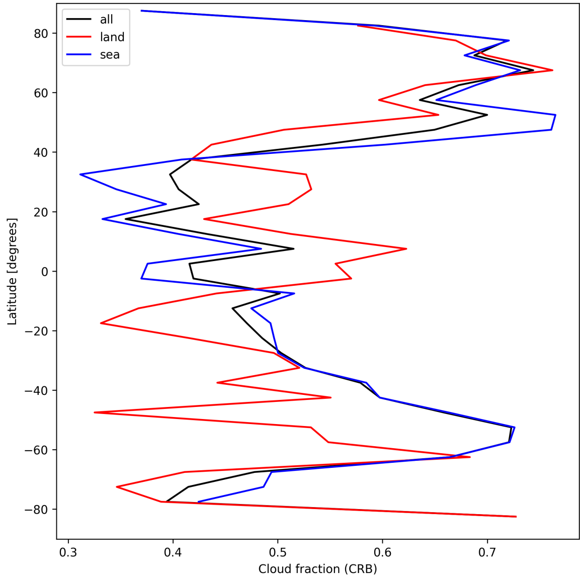
Figure 26: Zonal average of “Cloud fraction (CRB)” for 2025-09-07 to 2025-09-09.
