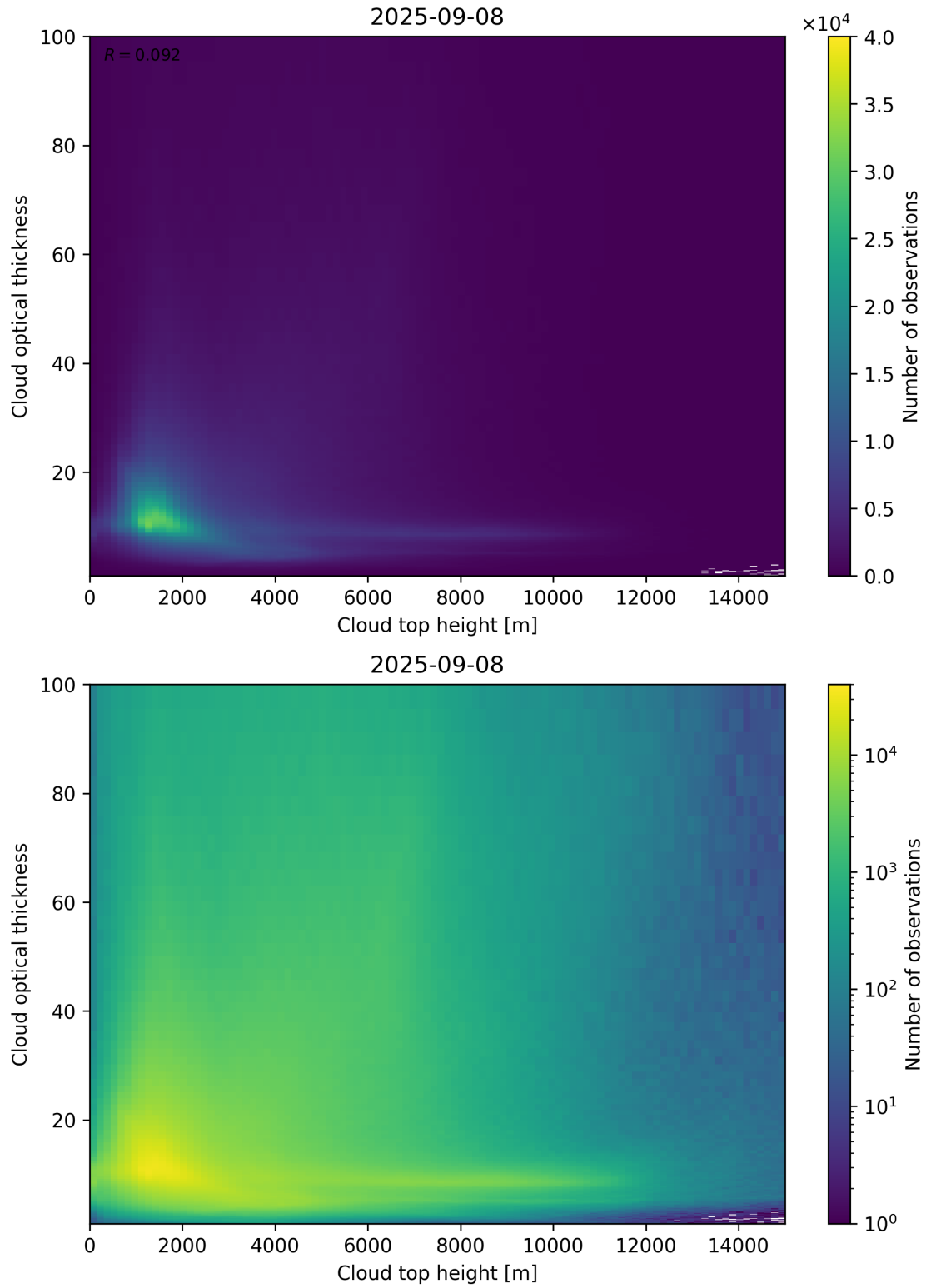
Figure 90: Scatter density plot of “Cloud top height” against “Cloud optical thickness” for 2025-09-07 to 2025-09-09.
