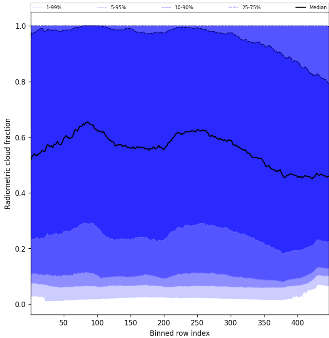
Figure 55: Along track statistics of “Radiometric cloud fraction” for 2025-09-07 to 2025-09-09
