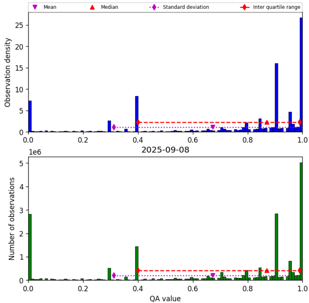
Figure 38: Histogram of “QA value” for 2025-09-07 to 2025-09-09
