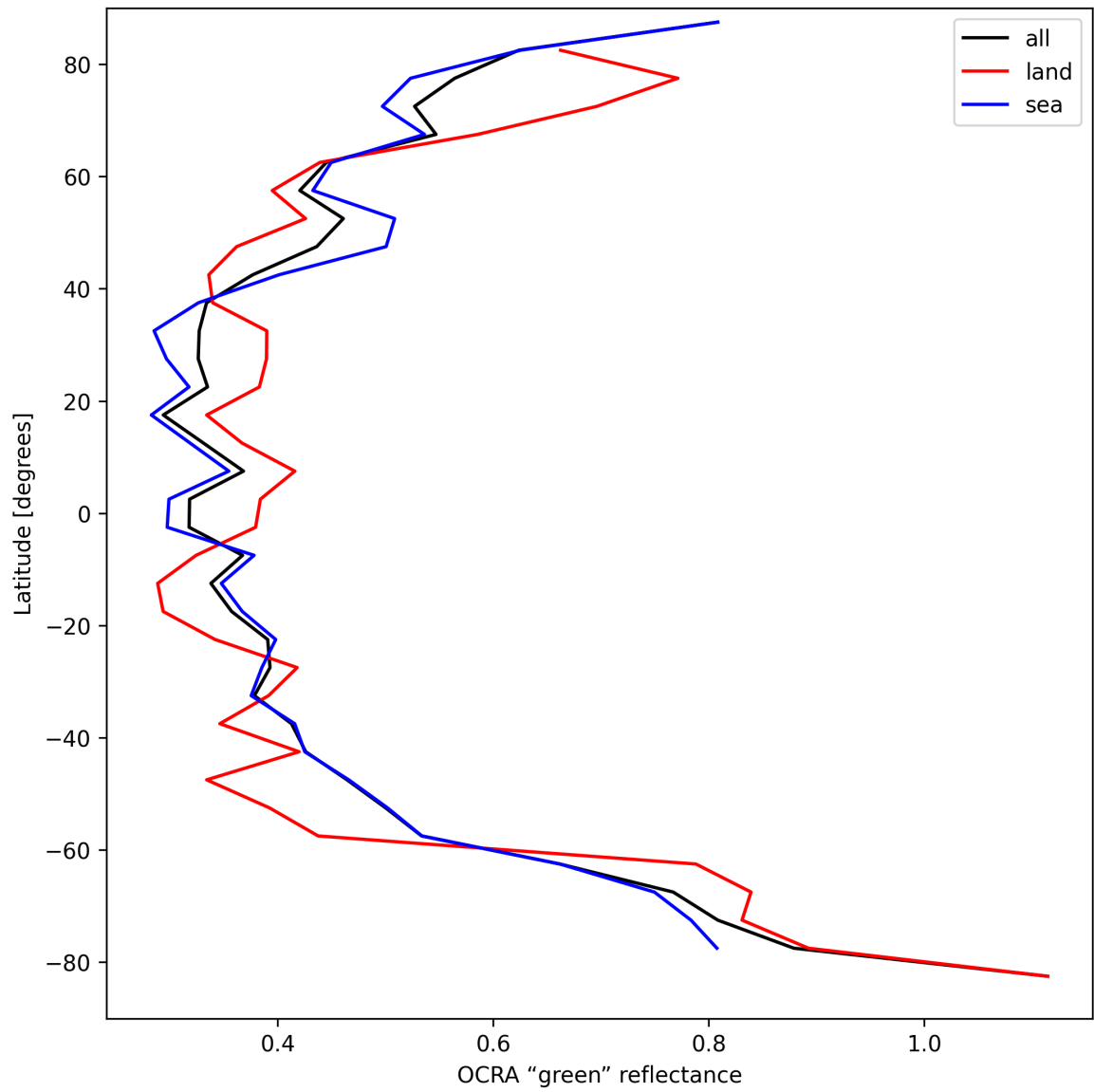
Figure 36: Zonal average of “OCRA “green” reflectance” for 2025-09-07 to 2025-09-09.
