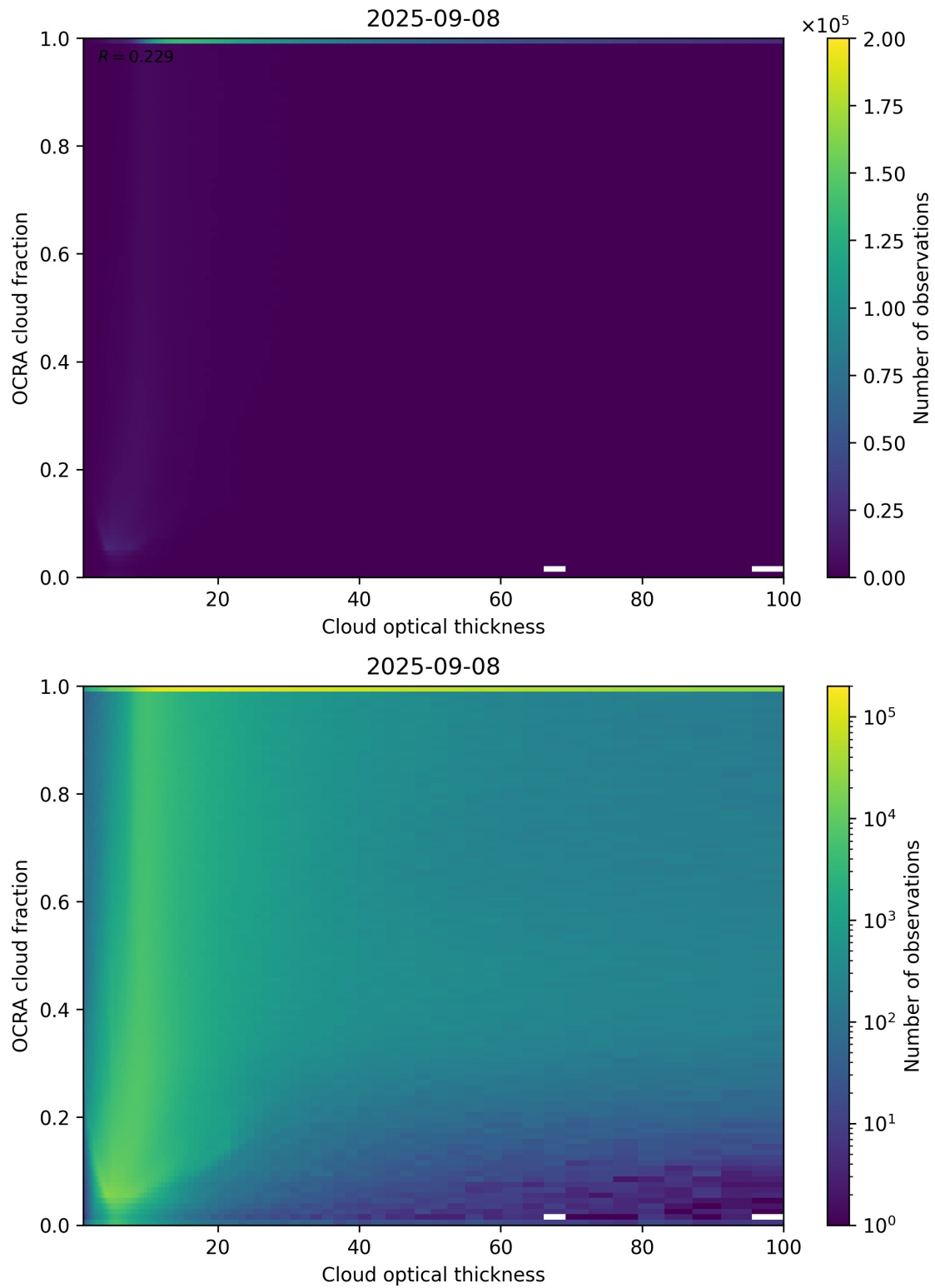
Figure 83: Scatter density plot of “Cloud optical thickness” against “OCRA cloud fraction” for 2025-09-07 to 2025-09-09.
