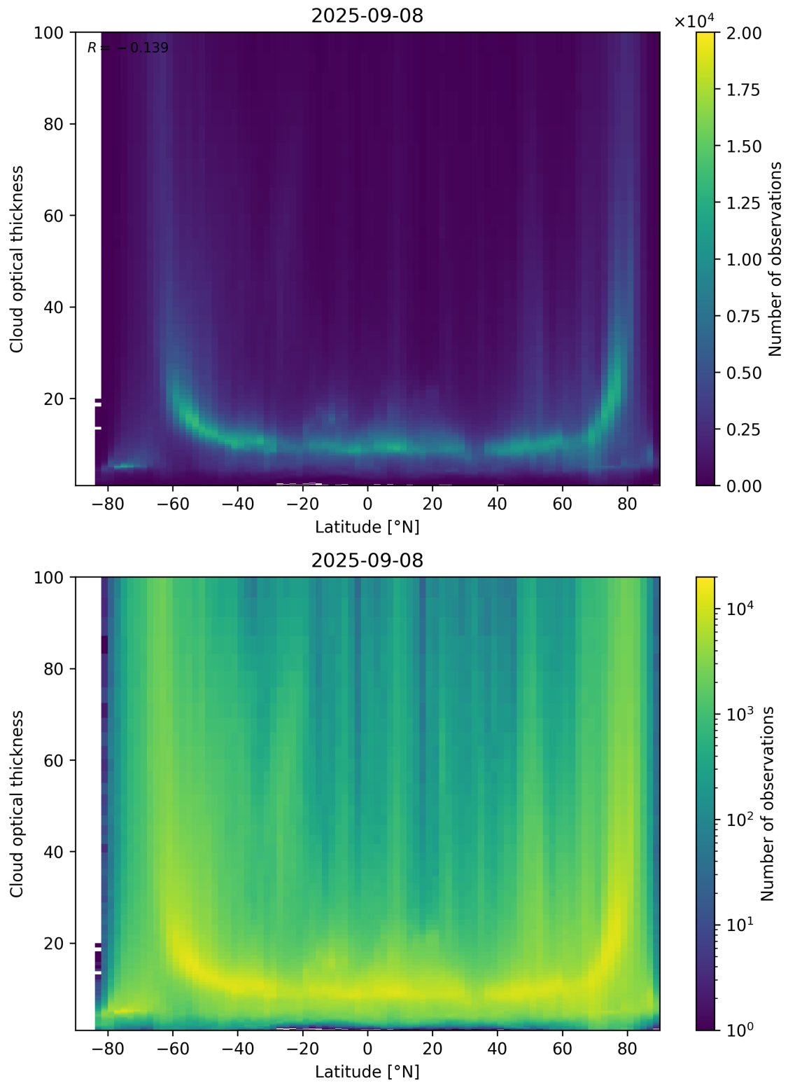
Figure 96: Scatter density plot of “Latitude” against “Cloud optical thickness” for 2025-09-07 to 2025-09-09.
