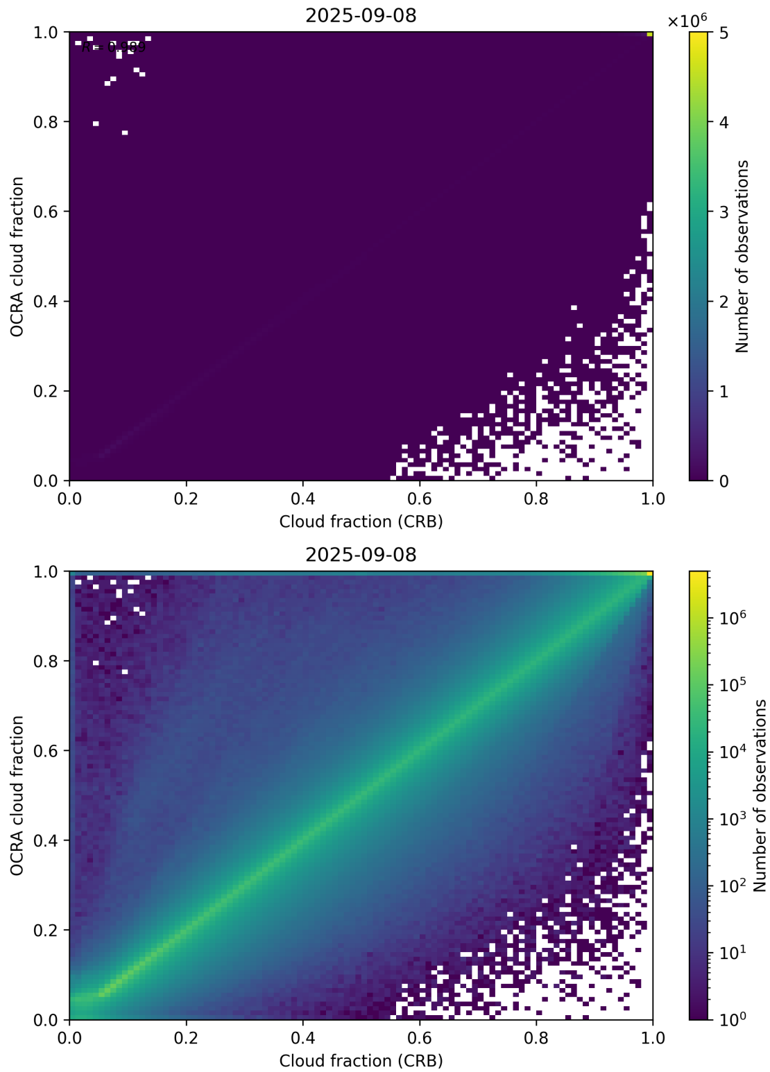
Figure 78: Scatter density plot of “Cloud fraction (CRB)” against “OCRA cloud fraction” for 2025-09-07 to 2025-09-09.
