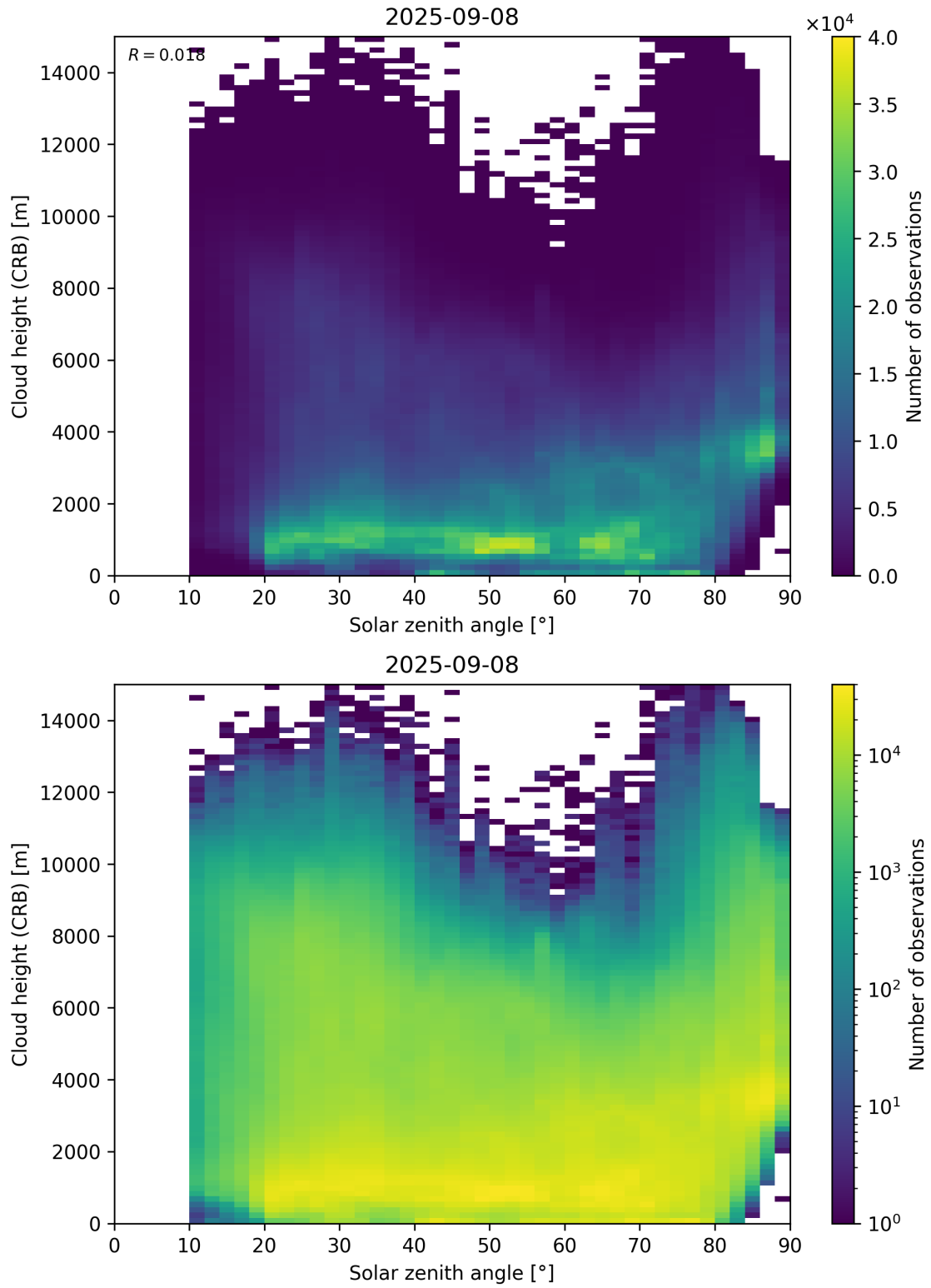
Figure 102: Scatter density plot of “Solar zenith angle” against “Cloud height (CRB)” for 2025-09-07 to 2025-09-09.
