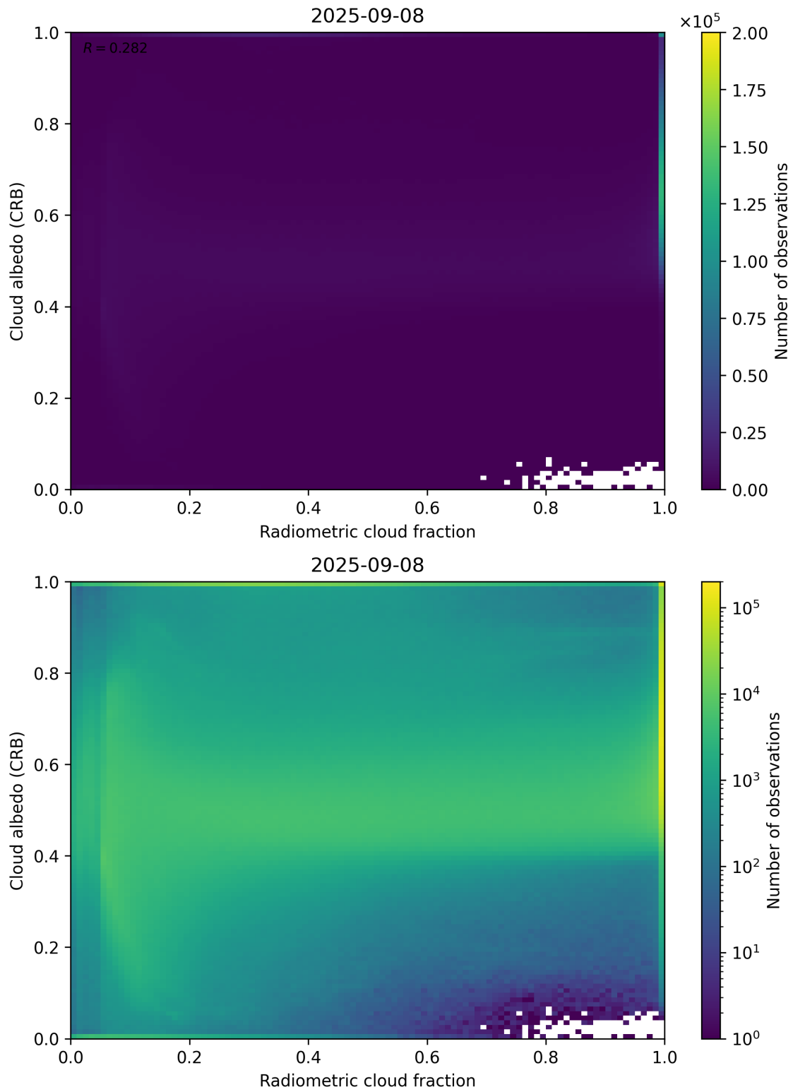
Figure 71: Scatter density plot of “Radiometric cloud fraction” against “Cloud albedo (CRB)” for 2025-09-07 to 2025-09-09.
