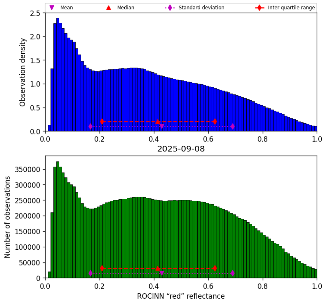
Figure 53: Histogram of “ROCINN “red” reflectance” for 2025-09-07 to 2025-09-09
