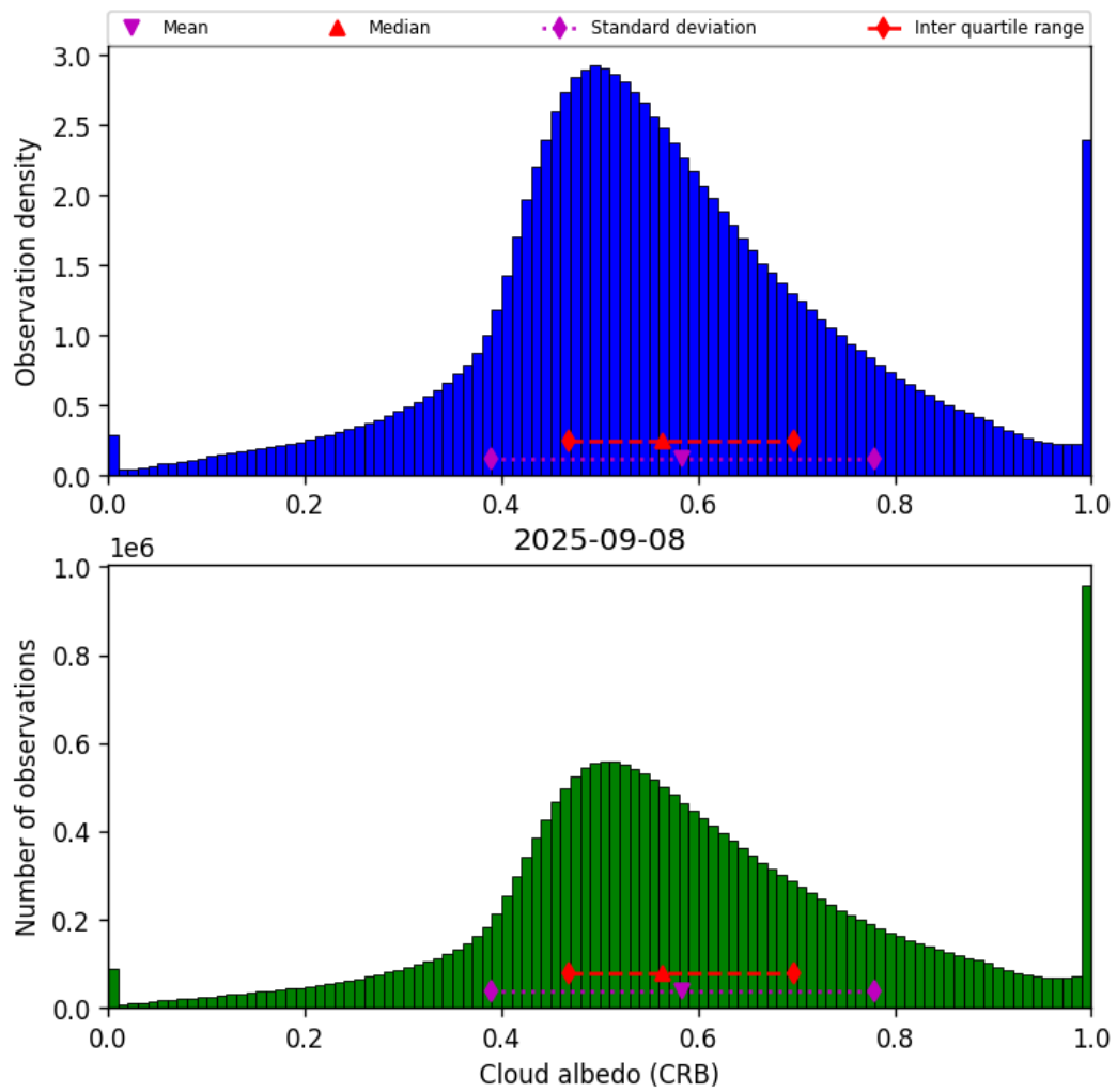
Figure 44: Histogram of “Cloud albedo (CRB)” for 2025-09-07 to 2025-09-09
