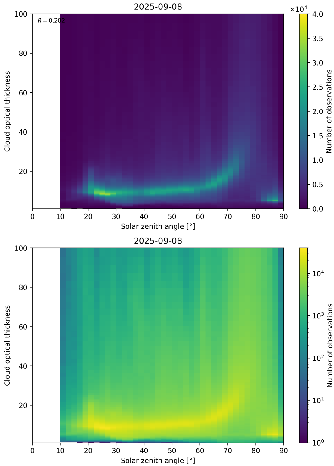
Figure 103: Scatter density plot of “Solar zenith angle” against “Cloud optical thickness” for 2025-09-07 to 2025-09-09.
