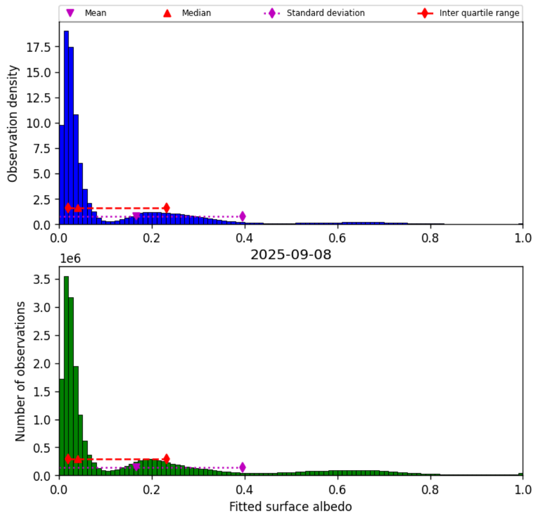
Figure 45: Histogram of “Fitted surface albedo” for 2025-09-07 to 2025-09-09
