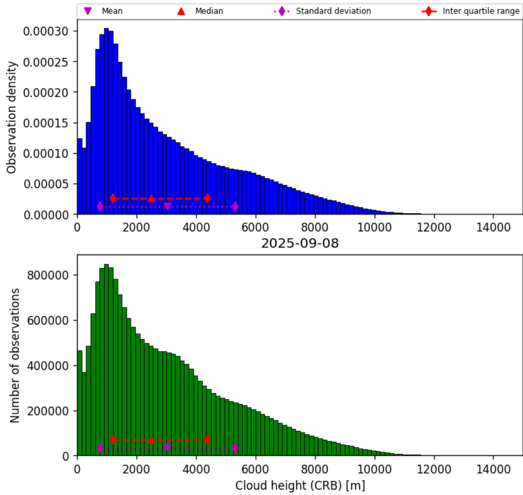
Figure 43: Histogram of “Cloud height (CRB)” for 2025-09-07 to 2025-09-09
