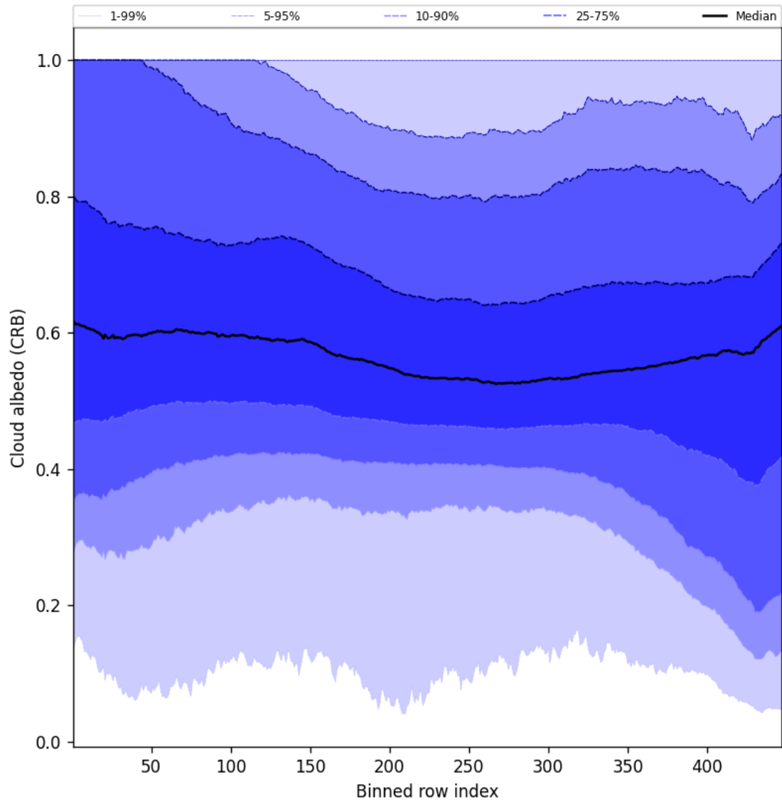
Figure 60: Along track statistics of “Cloud albedo (CRB)” for 2025-09-07 to 2025-09-09
