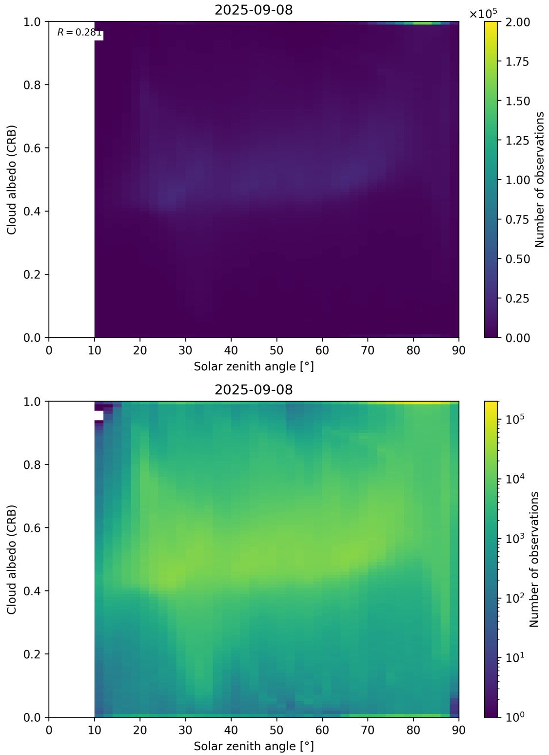
Figure 98: Scatter density plot of “Solar zenith angle” against “Cloud albedo (CRB)” for 2025-09-07 to 2025-09-09.
