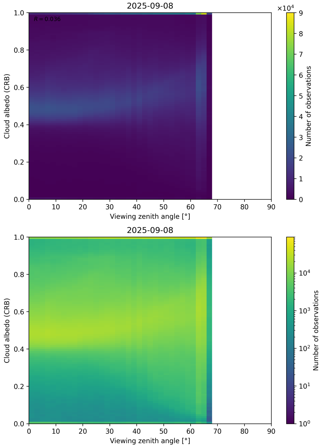
Figure 106: Scatter density plot of “Viewing zenith angle” against “Cloud albedo (CRB)” for 2025-09-07 to 2025-09-09.
