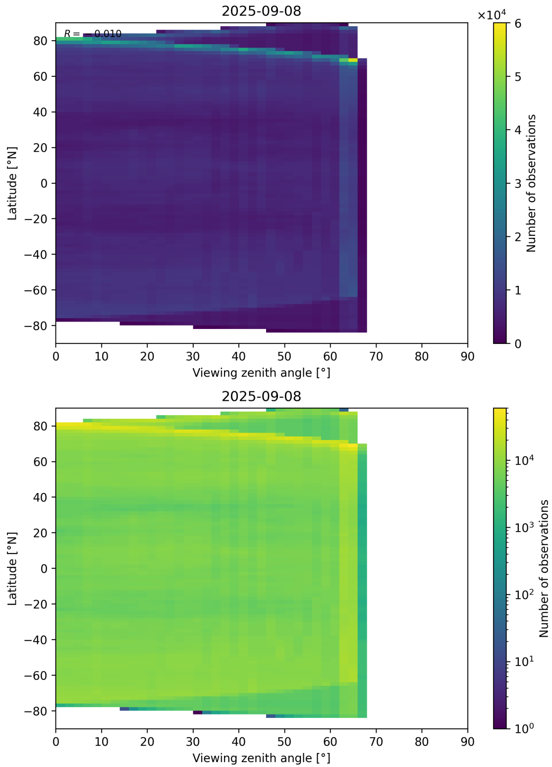
Figure 113: Scatter density plot of “Viewing zenith angle” against “Latitude” for 2025-09-07 to 2025-09-09.
