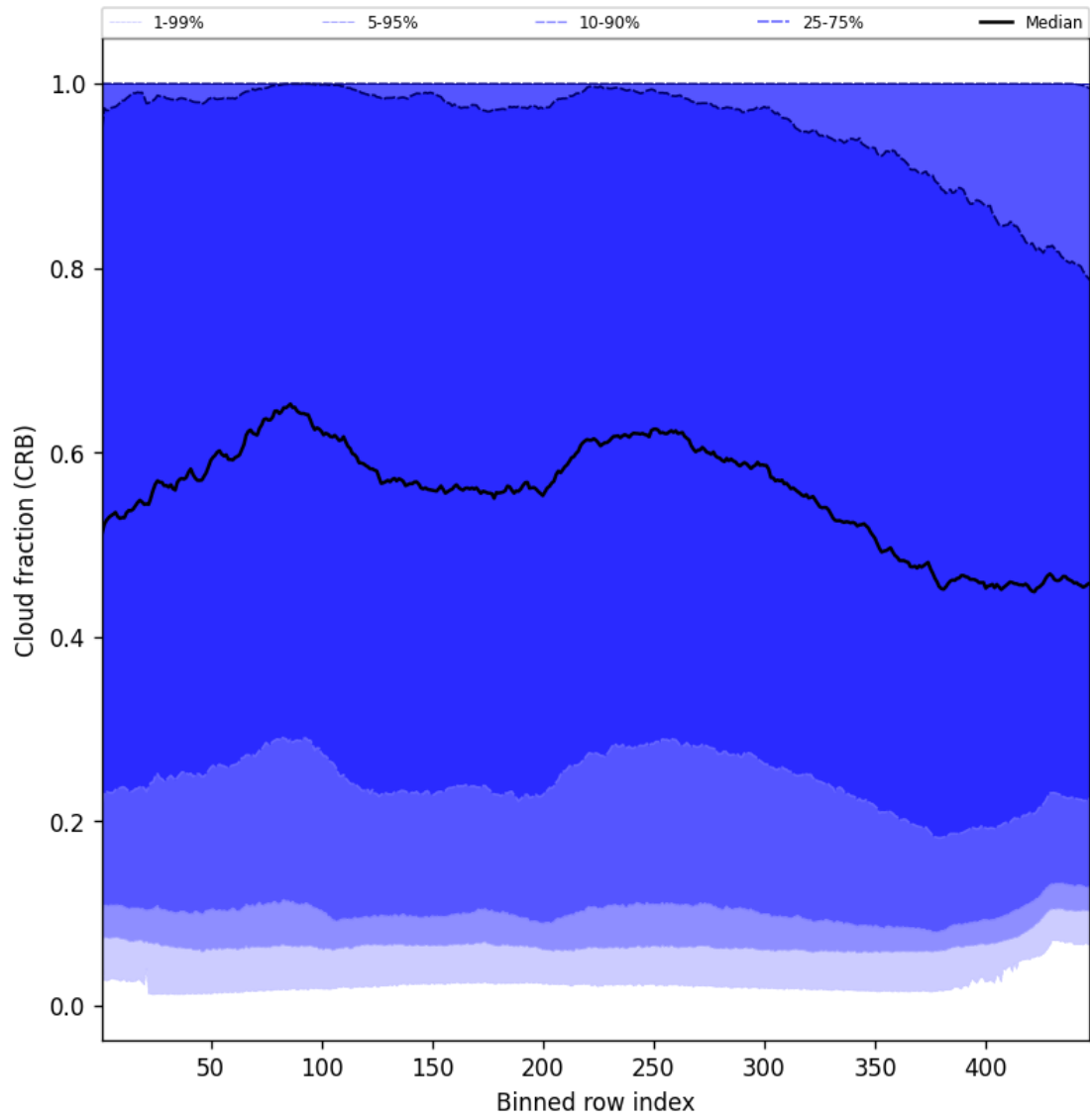
Figure 58: Along track statistics of “Cloud fraction (CRB)” for 2025-09-07 to 2025-09-09
