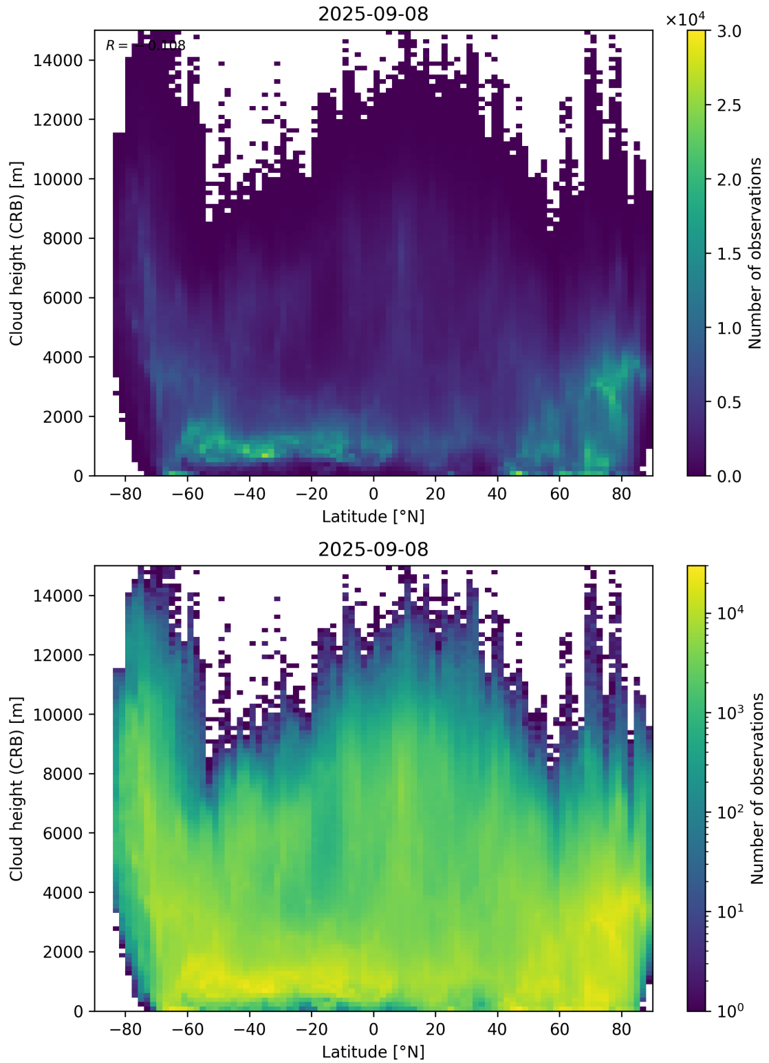
Figure 95: Scatter density plot of “Latitude” against “Cloud height (CRB)” for 2025-09-07 to 2025-09-09.
