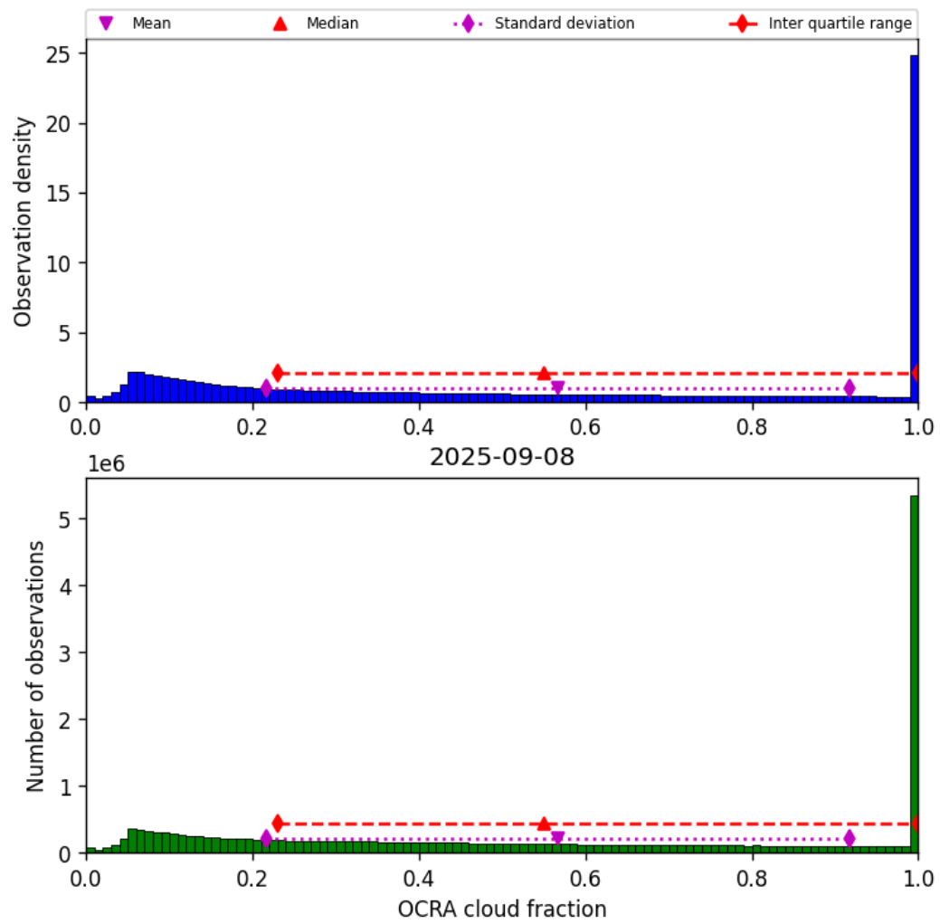
Figure 50: Histogram of “OCRA cloud fraction” for 2025-09-07 to 2025-09-09
