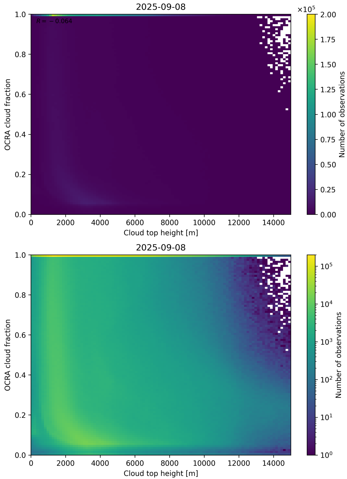
Figure 87: Scatter density plot of “Cloud top height” against “OCRA cloud fraction” for 2025-09-07 to 2025-09-09.
