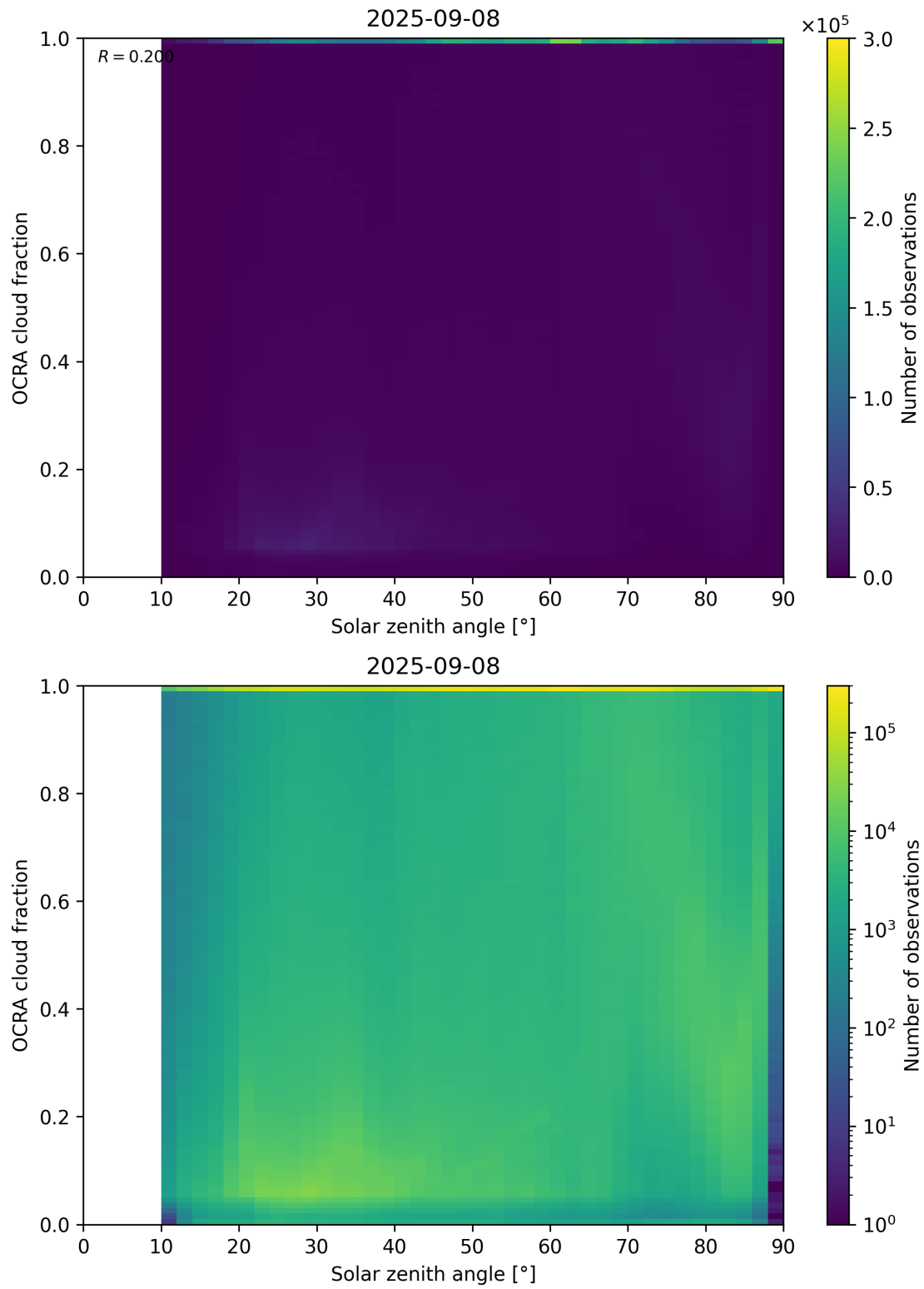
Figure 100: Scatter density plot of “Solar zenith angle” against “OCRA cloud fraction” for 2025-09-07 to 2025-09-09.
