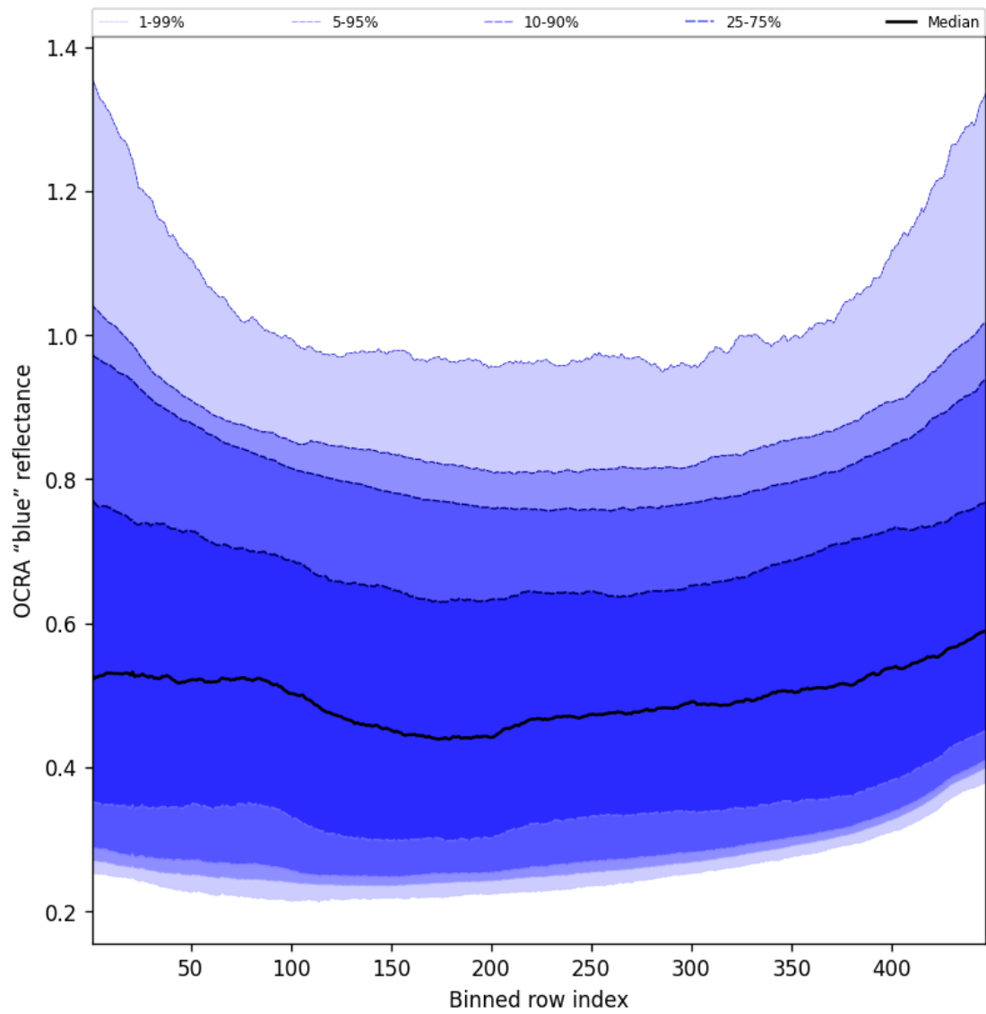
Figure 67: Along track statistics of “OCRA “blue” reflectance” for 2025-09-07 to 2025-09-09
