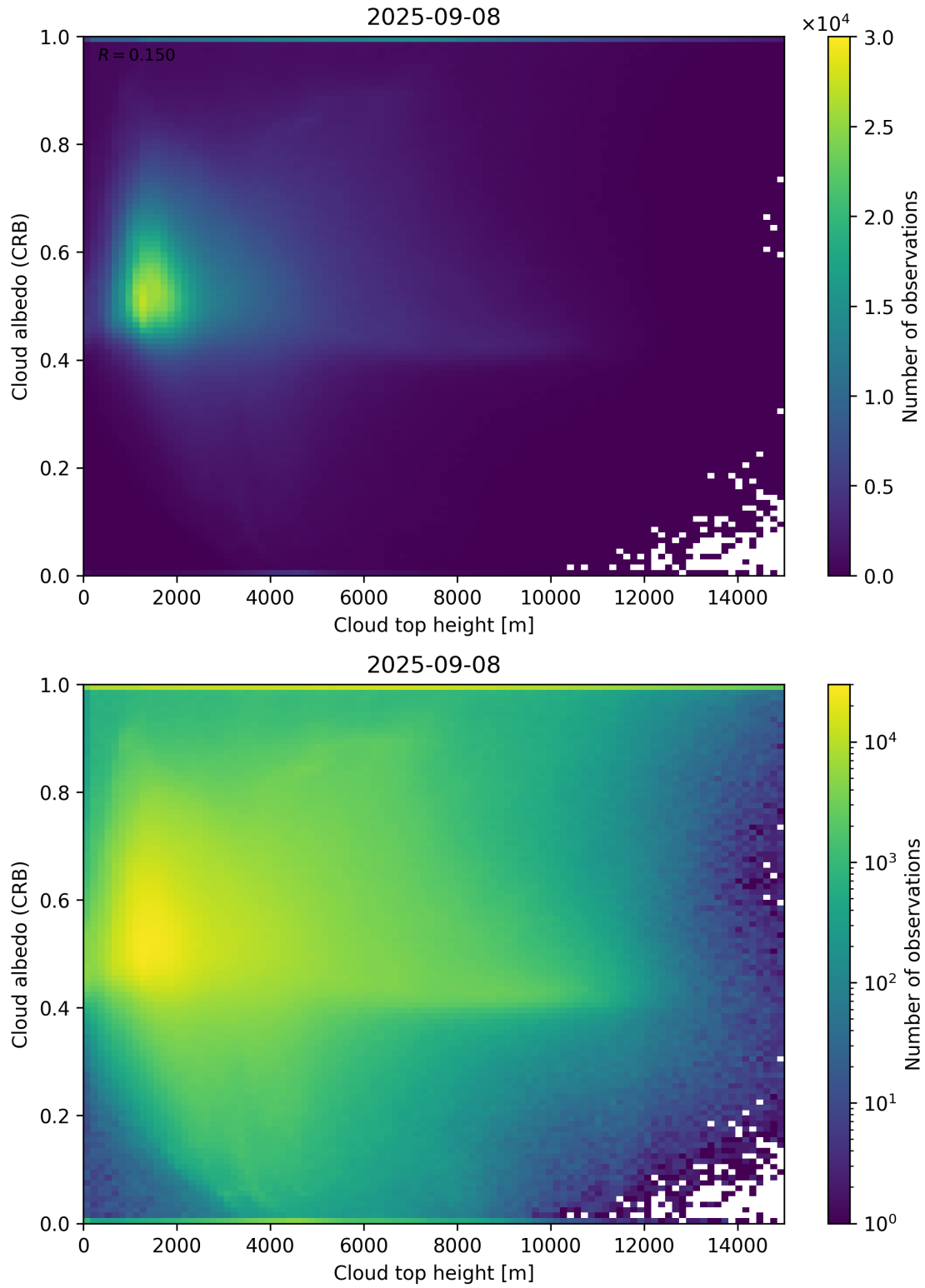
Figure 86: Scatter density plot of “Cloud top height” against “Cloud albedo (CRB)” for 2025-09-07 to 2025-09-09.
