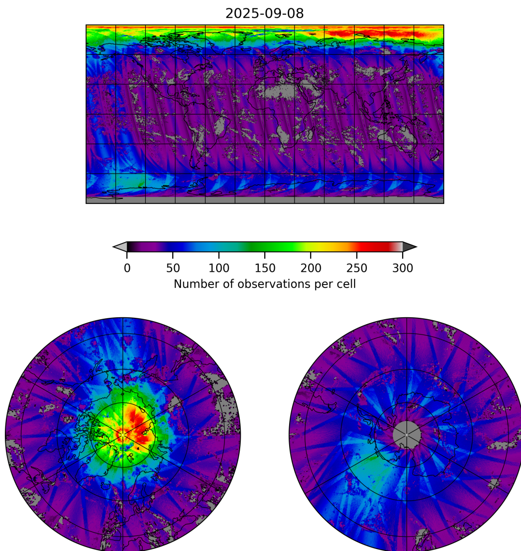
Figure 21: Map of the number of observations for 2025-09-07 to 2025-09-09
