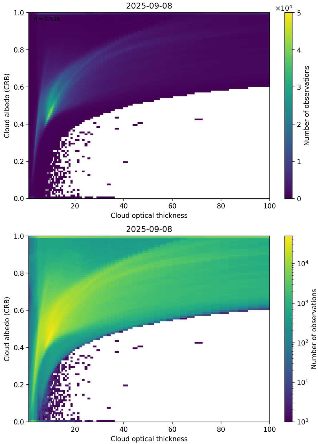
Figure 82: Scatter density plot of “Cloud optical thickness” against “Cloud albedo (CRB)” for 2025-09-07 to 2025-09-09.
