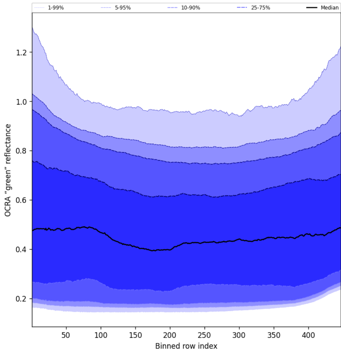
Figure 68: Along track statistics of “OCRA “green” reflectance” for 2025-09-07 to 2025-09-09
