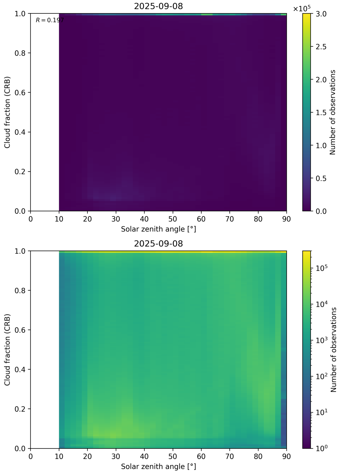
Figure 101: Scatter density plot of “Solar zenith angle” against “Cloud fraction (CRB)” for 2025-09-07 to 2025-09-09.
