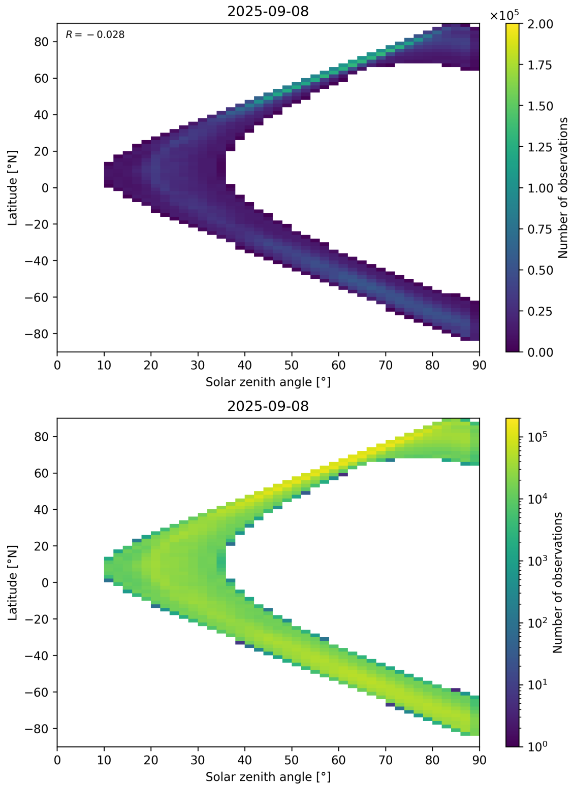
Figure 105: Scatter density plot of “Solar zenith angle” against “Latitude” for 2025-09-07 to 2025-09-09.
