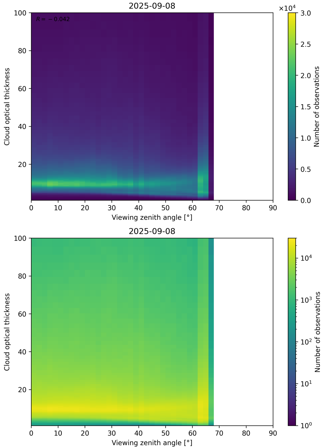
Figure 111: Scatter density plot of “Viewing zenith angle” against “Cloud optical thickness” for 2025-09-07 to 2025-09-09.
