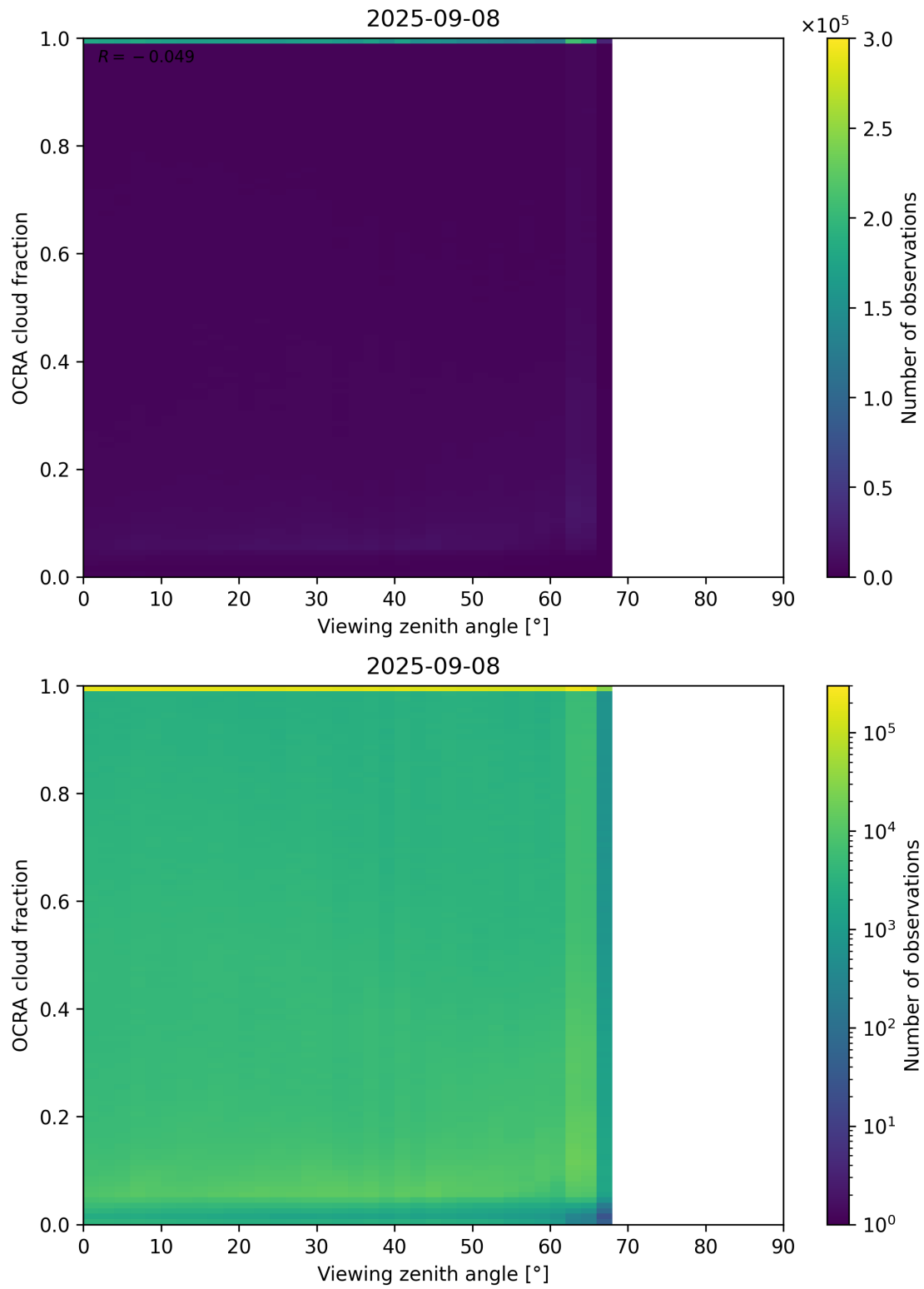
Figure 108: Scatter density plot of “Viewing zenith angle” against “OCRA cloud fraction” for 2025-09-07 to 2025-09-09.
