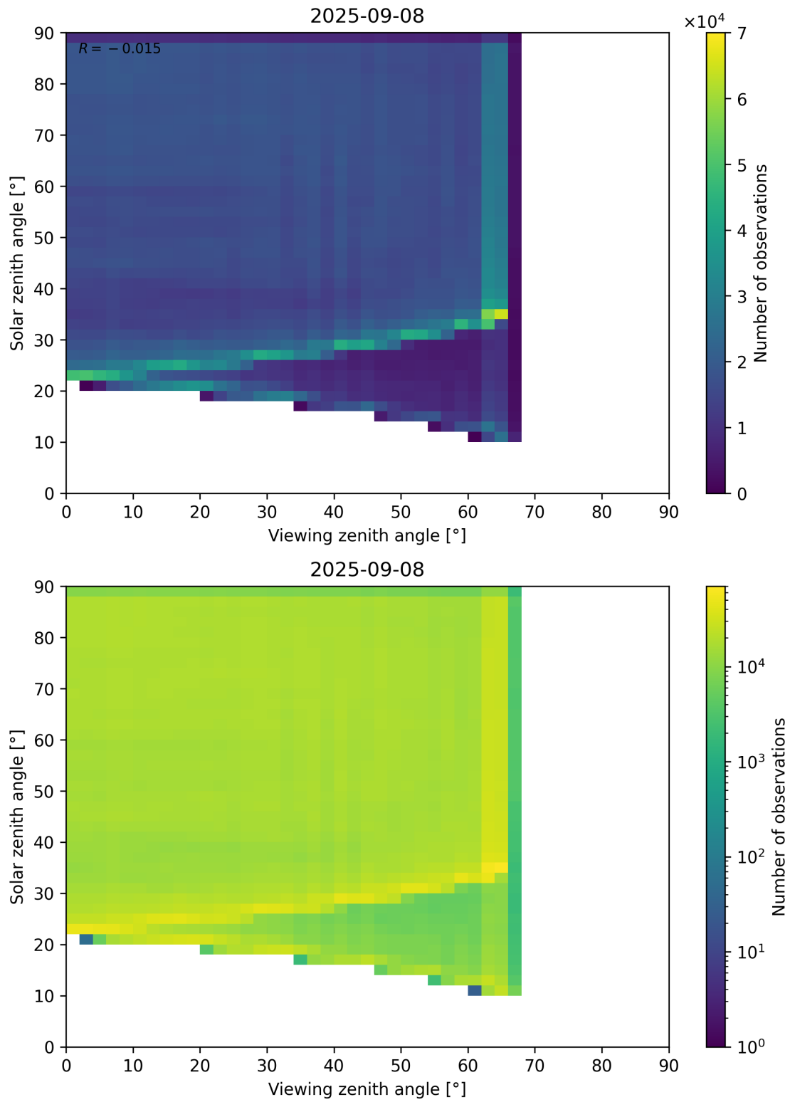
Figure 114: Scatter density plot of “Viewing zenith angle” against “Solar zenith angle” for 2025-09-07 to 2025-09-09.
