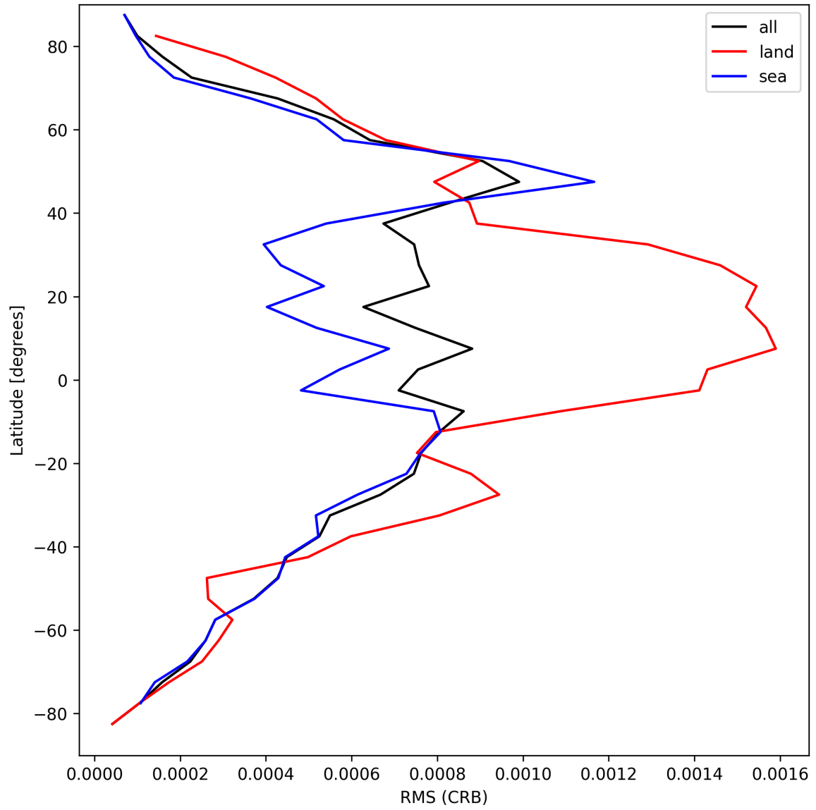
Figure 32: Zonal average of “RMS (CRB)” for 2025-09-07 to 2025-09-09.
