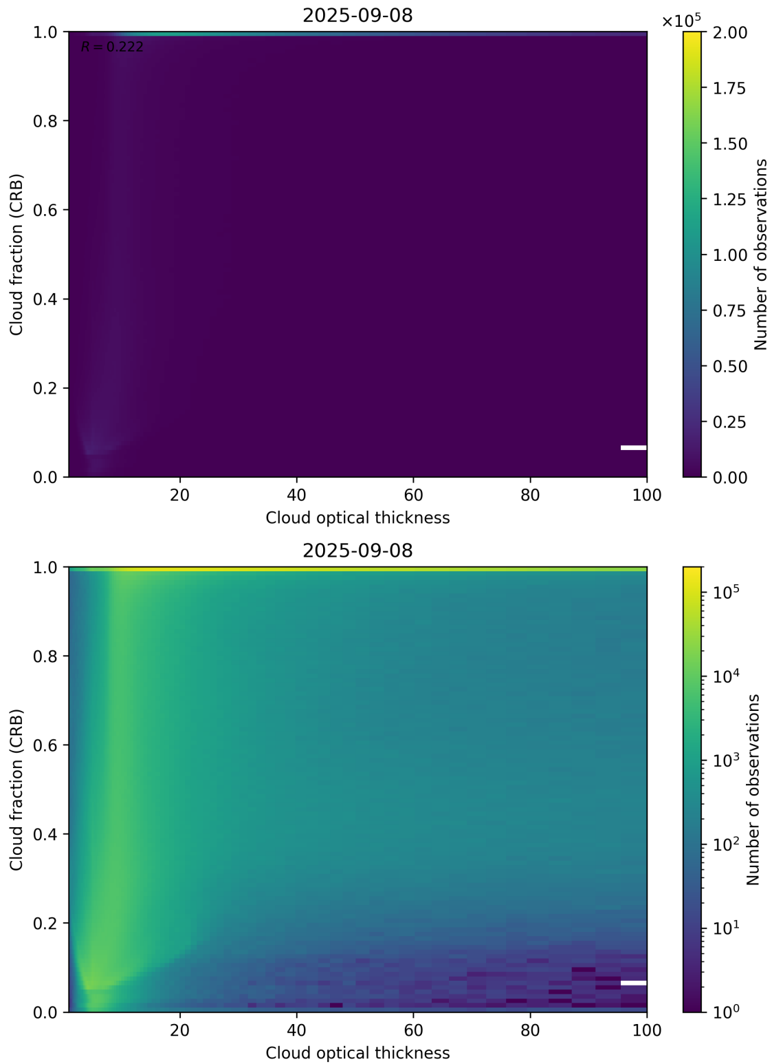
Figure 84: Scatter density plot of “Cloud optical thickness” against “Cloud fraction (CRB)” for 2025-09-07 to 2025-09-09.
