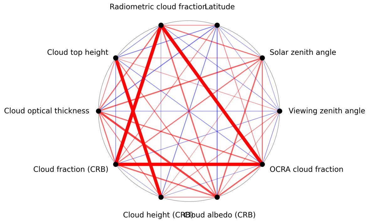
Figure 1: Map of correlation graph for 2025-09-07 to 2025-09-09.
