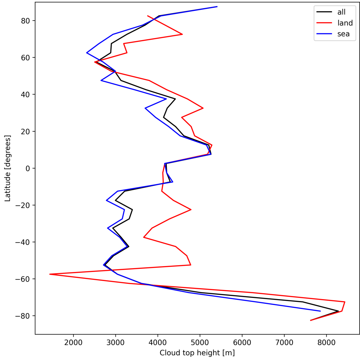
Figure 24: Zonal average of “Cloud top height” for 2025-09-07 to 2025-09-09.
