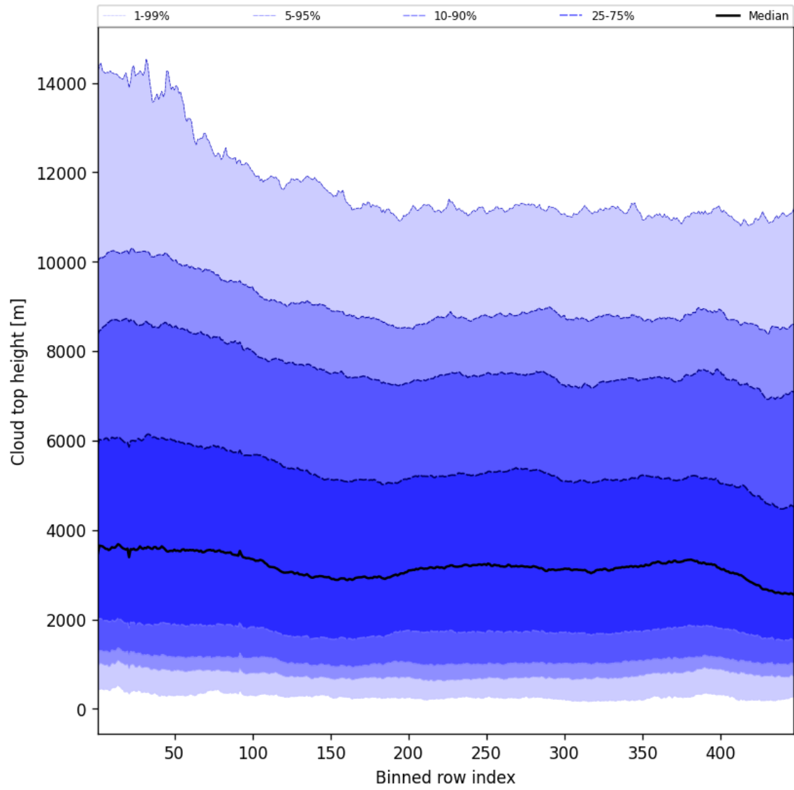
Figure 56: Along track statistics of “Cloud top height” for 2025-09-07 to 2025-09-09
