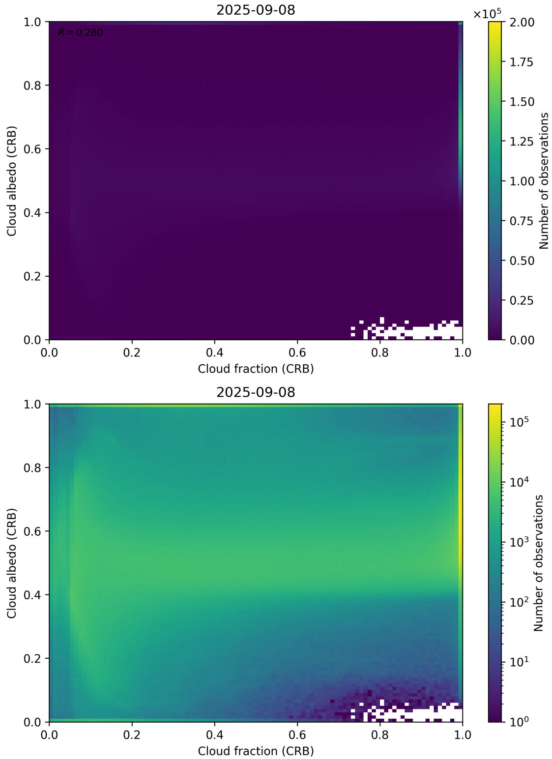
Figure 77: Scatter density plot of “Cloud fraction (CRB)” against “Cloud albedo (CRB)” for 2025-09-07 to 2025-09-09.
