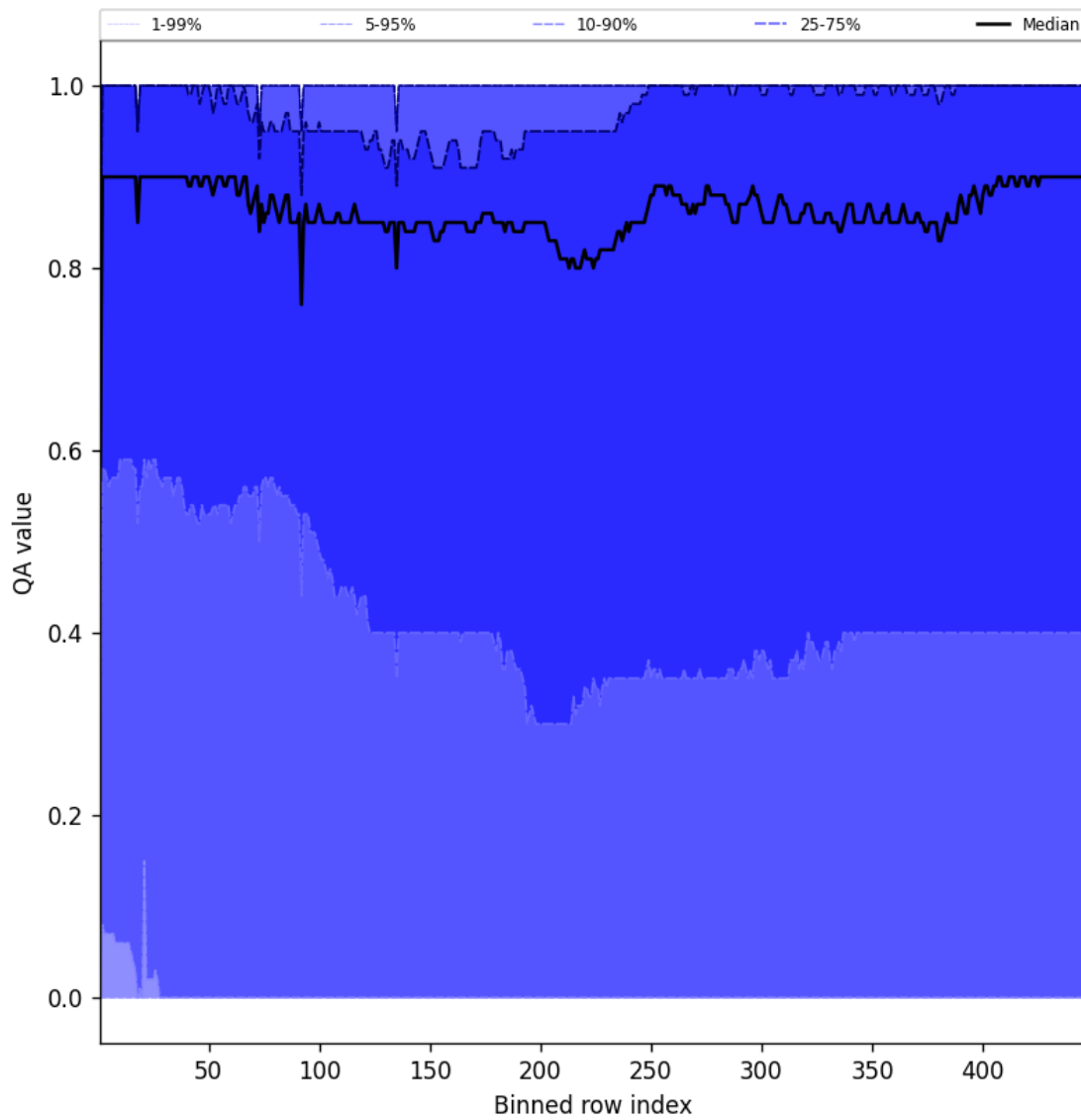
Figure 54: Along track statistics of “QA value” for 2025-09-07 to 2025-09-09
