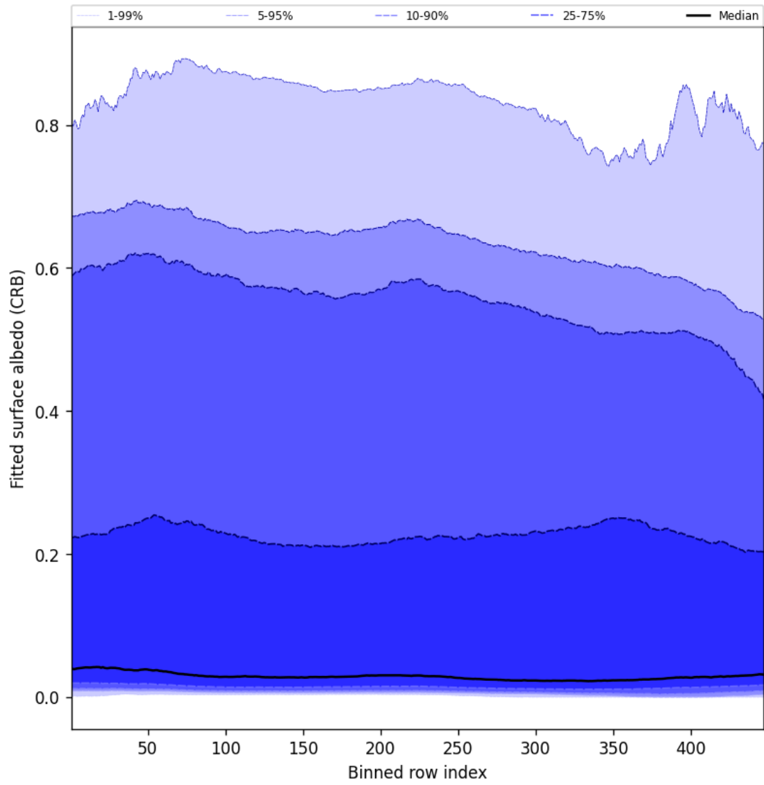
Figure 62: Along track statistics of “Fitted surface albedo (CRB)” for 2025-09-07 to 2025-09-09
