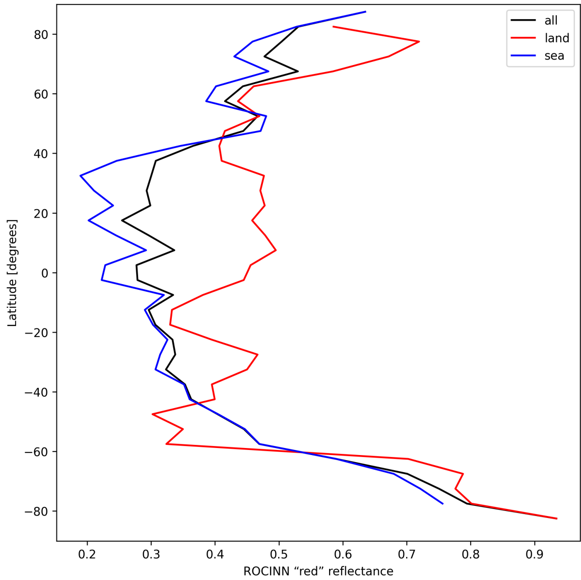
Figure 37: Zonal average of “ROCINN “red” reflectance” for 2025-09-07 to 2025-09-09.
