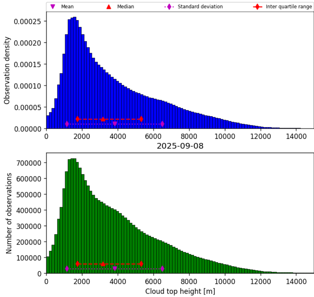
Figure 40: Histogram of “Cloud top height” for 2025-09-07 to 2025-09-09
