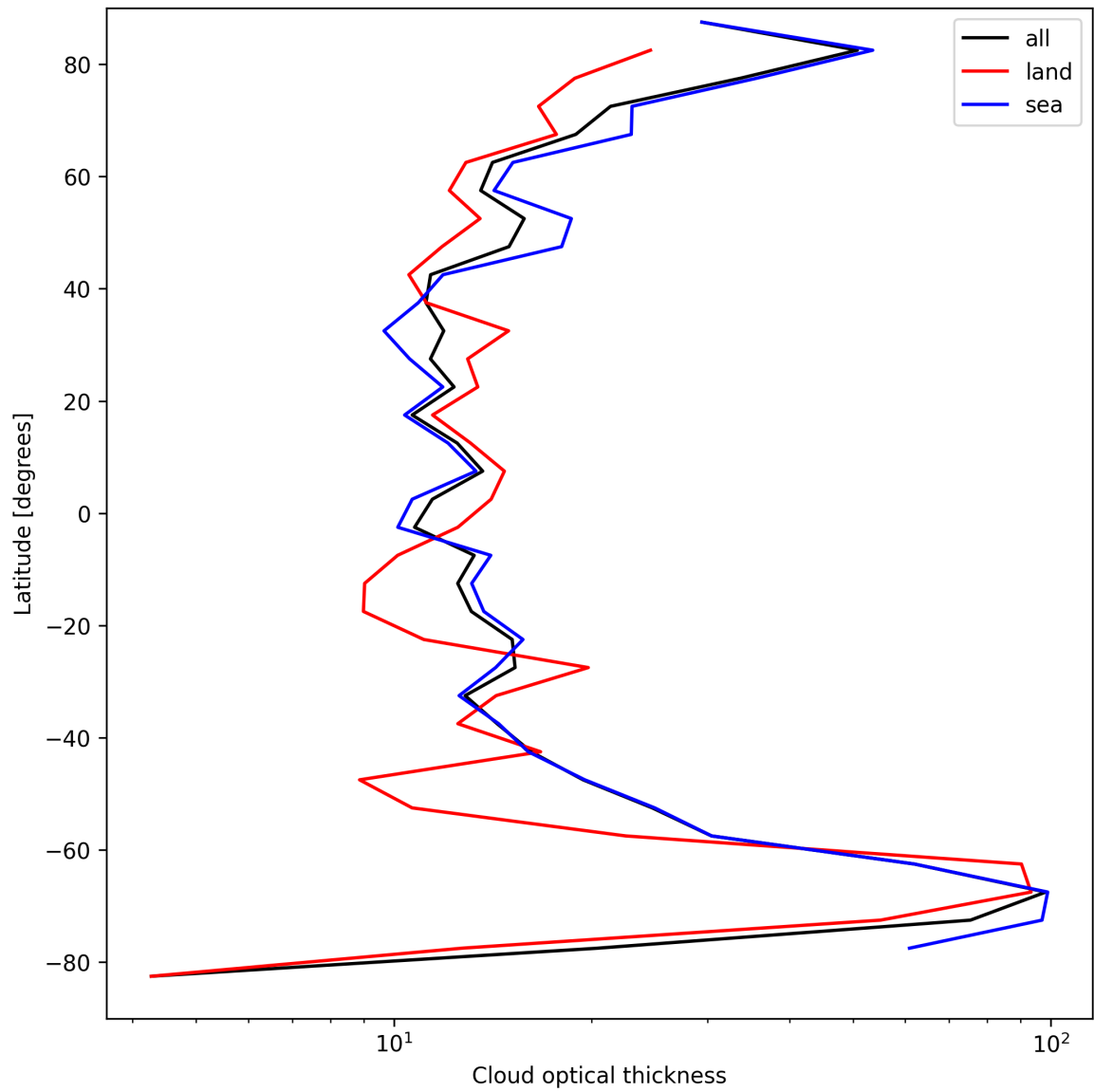
Figure 25: Zonal average of “Cloud optical thickness” for 2025-09-07 to 2025-09-09.
