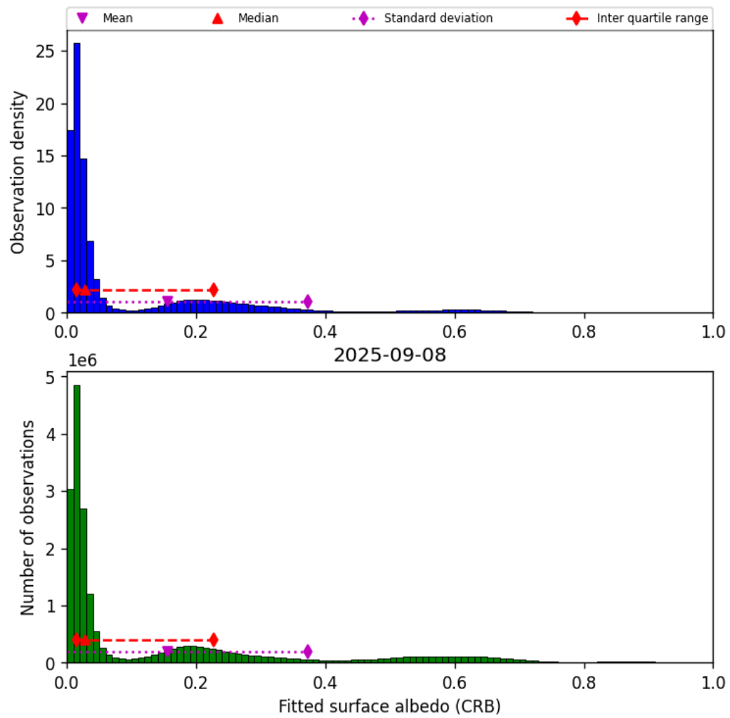
Figure 46: Histogram of “Fitted surface albedo (CRB)” for 2025-09-07 to 2025-09-09
