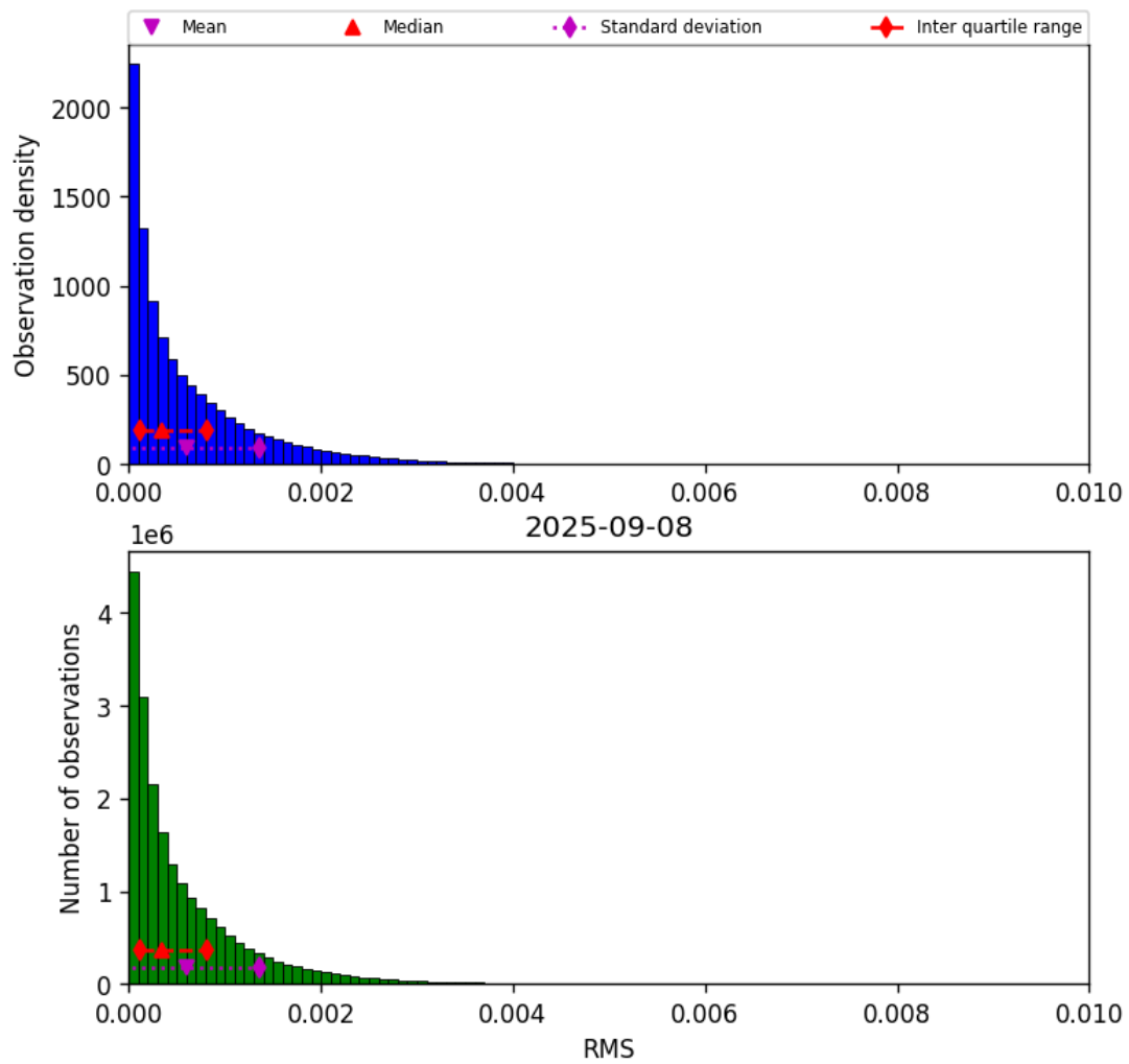
Figure 47: Histogram of “RMS” for 2025-09-07 to 2025-09-09
