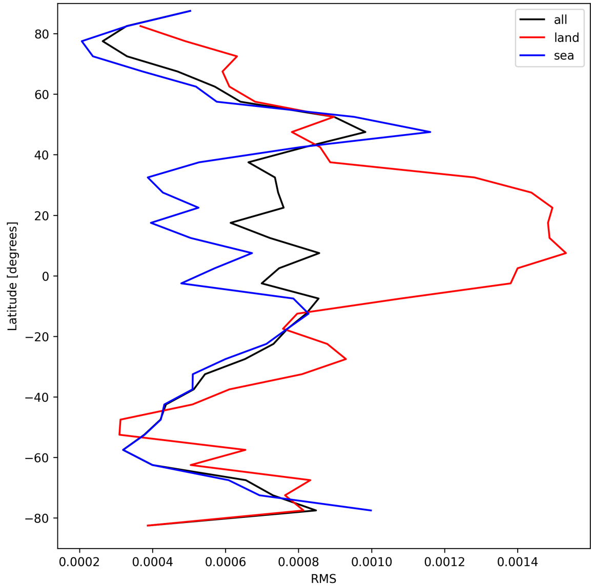
Figure 31: Zonal average of “RMS” for 2025-09-07 to 2025-09-09.
