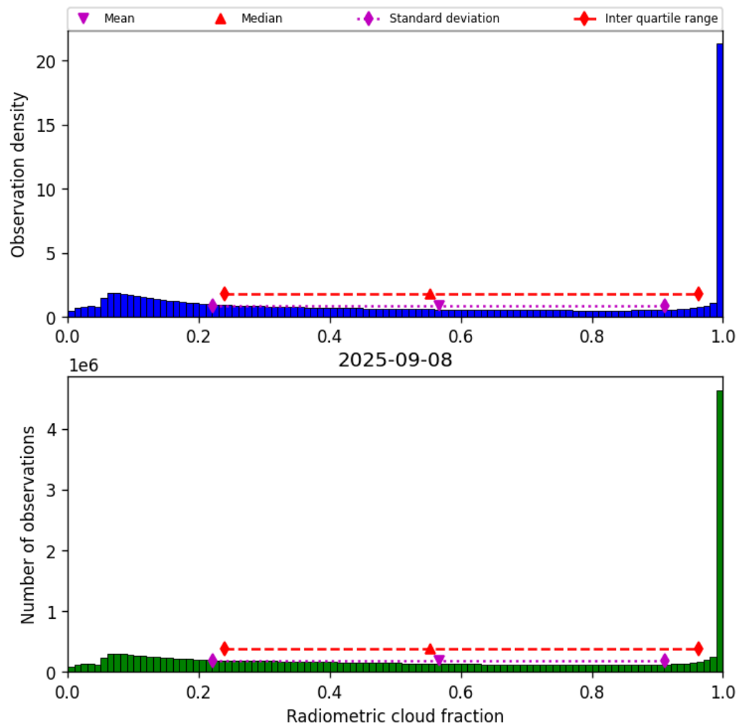
Figure 39: Histogram of “Radiometric cloud fraction” for 2025-09-07 to 2025-09-09
