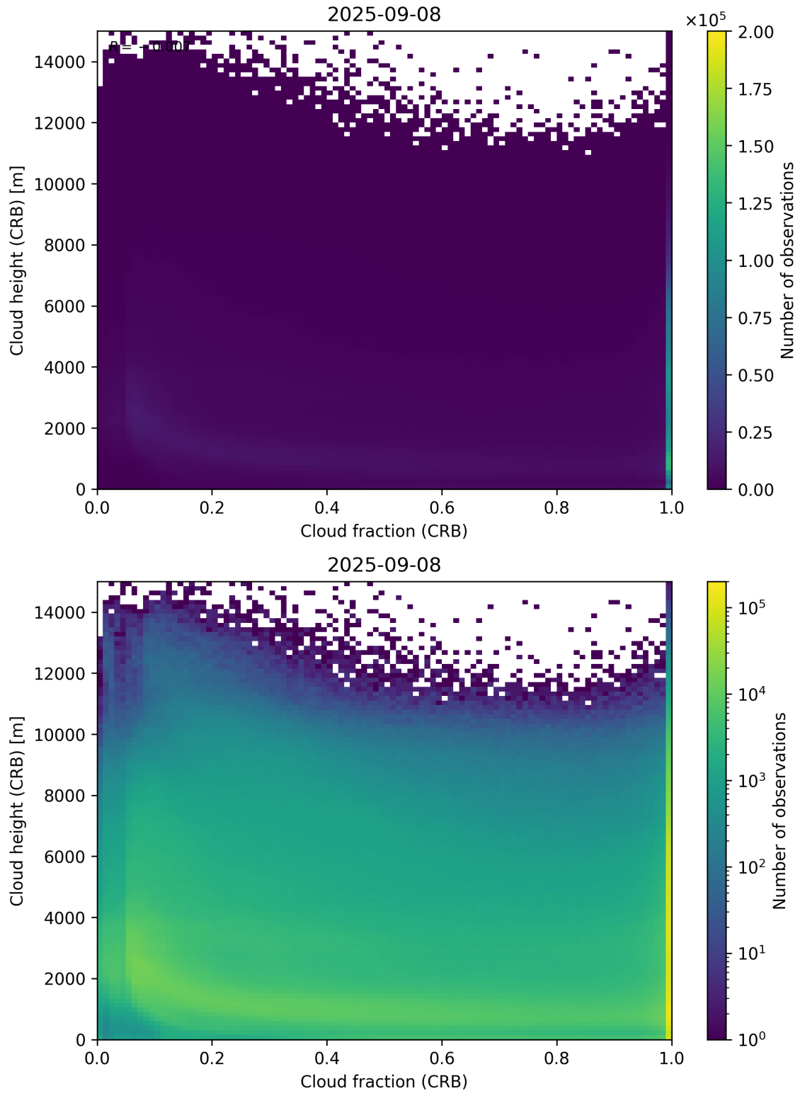
Figure 79: Scatter density plot of “Cloud fraction (CRB)” against “Cloud height (CRB)” for 2025-09-07 to 2025-09-09.
