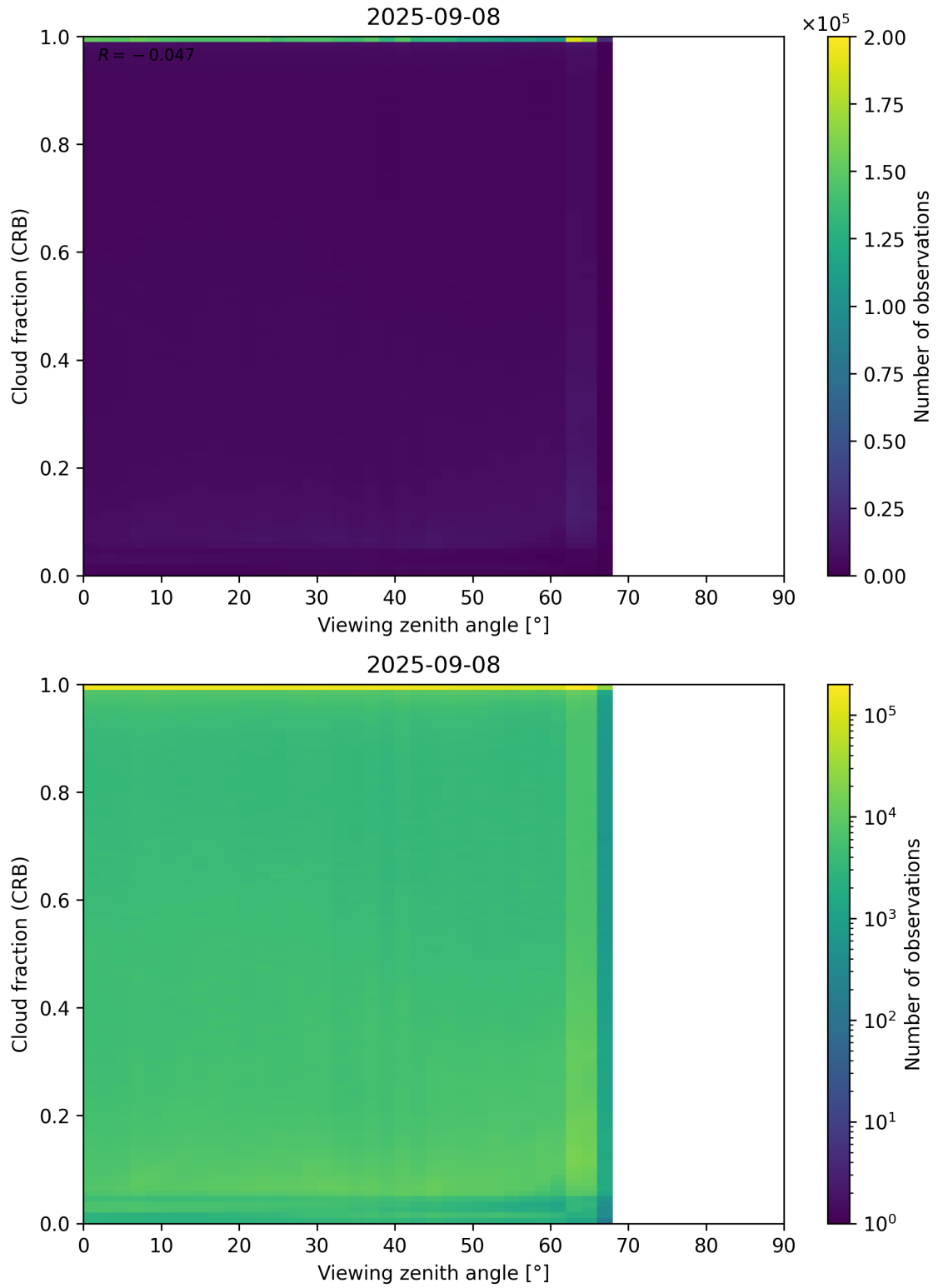
Figure 109: Scatter density plot of “Viewing zenith angle” against “Cloud fraction (CRB)” for 2025-09-07 to 2025-09-09.
