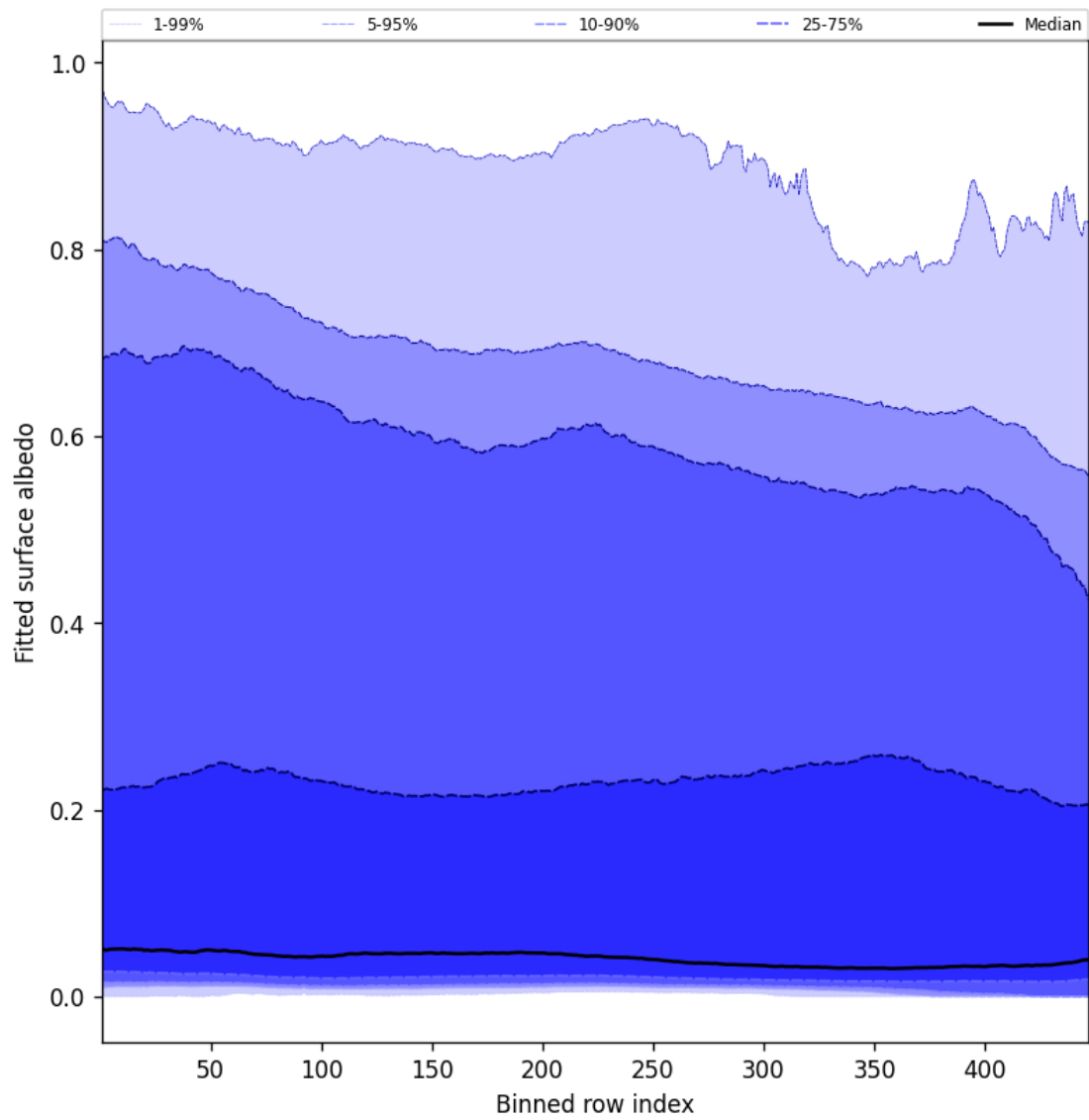
Figure 61: Along track statistics of “Fitted surface albedo” for 2025-09-07 to 2025-09-09
