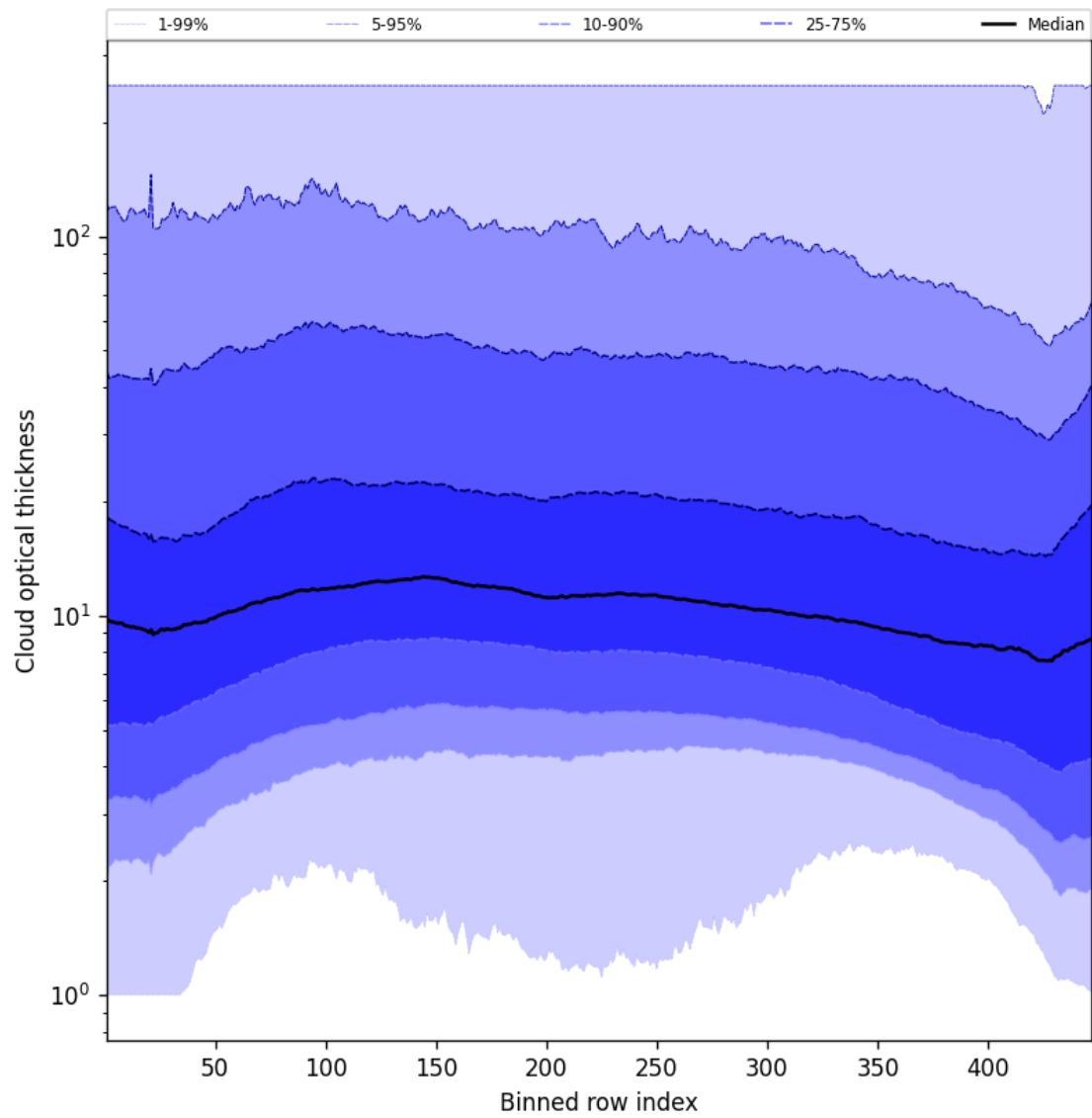
Figure 57: Along track statistics of “Cloud optical thickness” for 2025-09-07 to 2025-09-09
