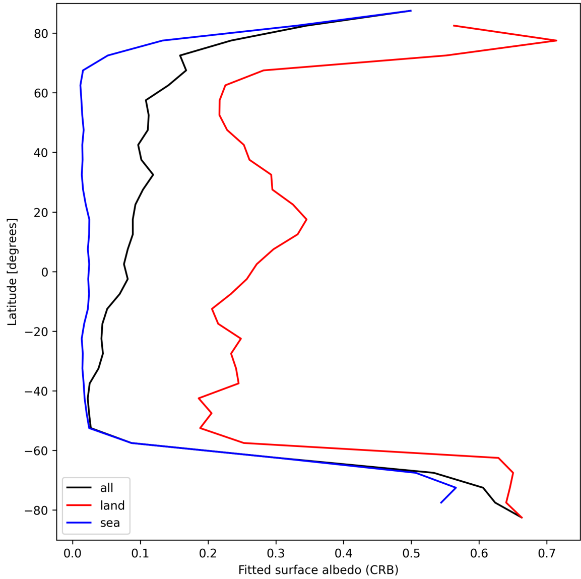
Figure 30: Zonal average of “Fitted surface albedo (CRB)” for 2025-09-07 to 2025-09-09.
