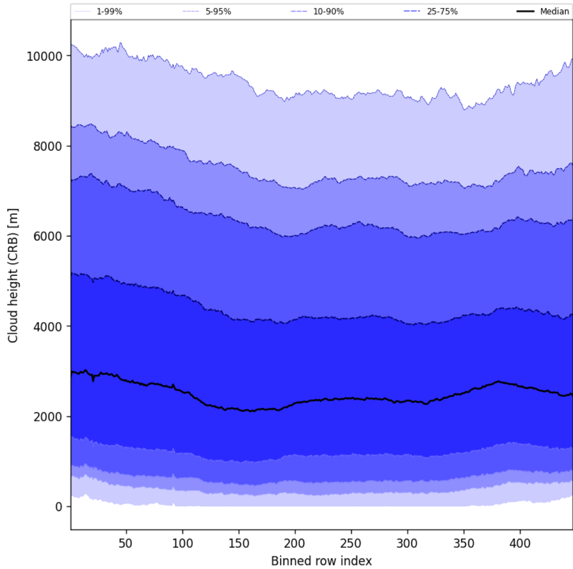
Figure 59: Along track statistics of “Cloud height (CRB)” for 2025-09-07 to 2025-09-09
