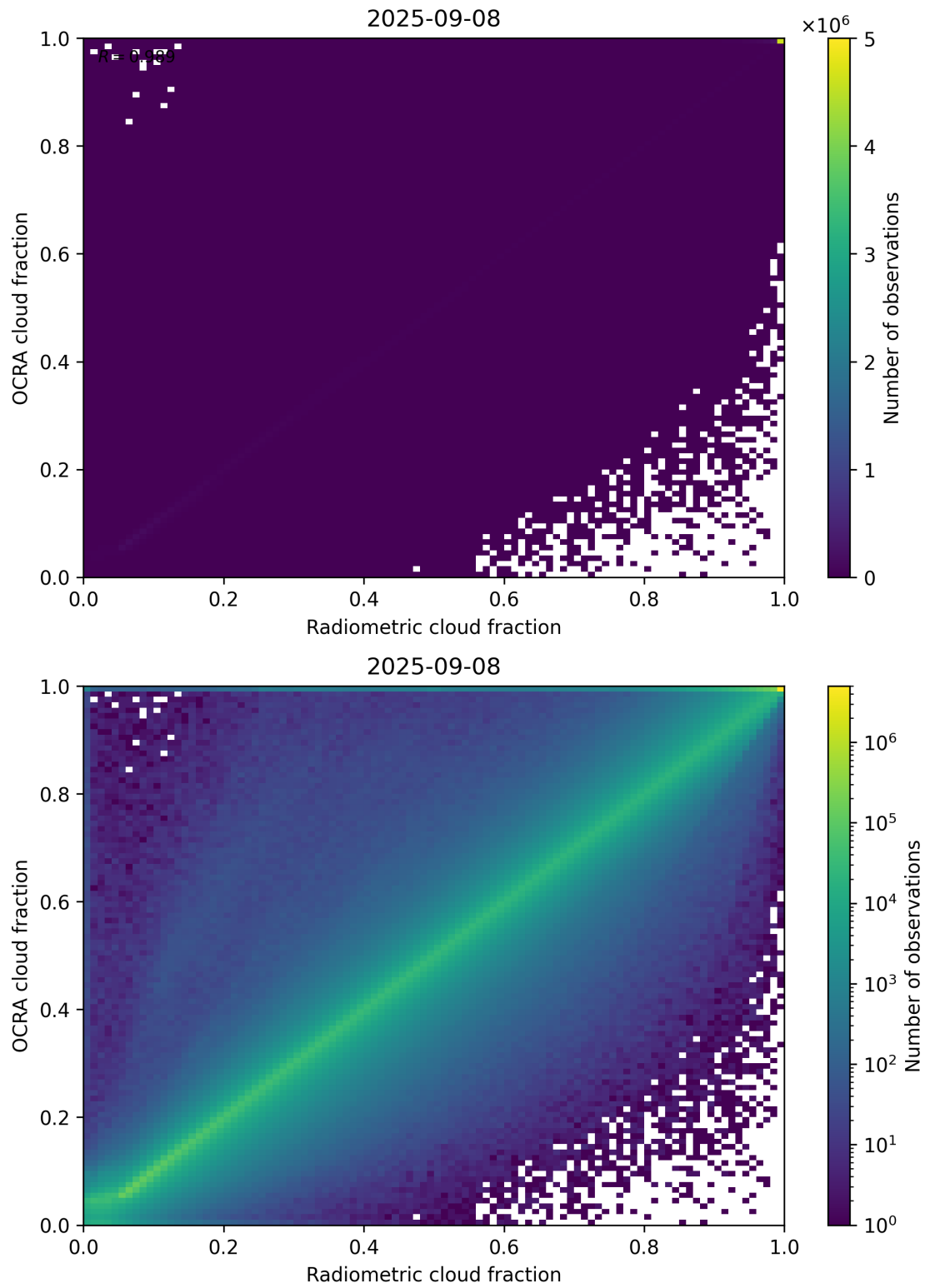
Figure 72: Scatter density plot of “Radiometric cloud fraction” against “OCRA cloud fraction” for 2025-09-07 to 2025-09-09.
