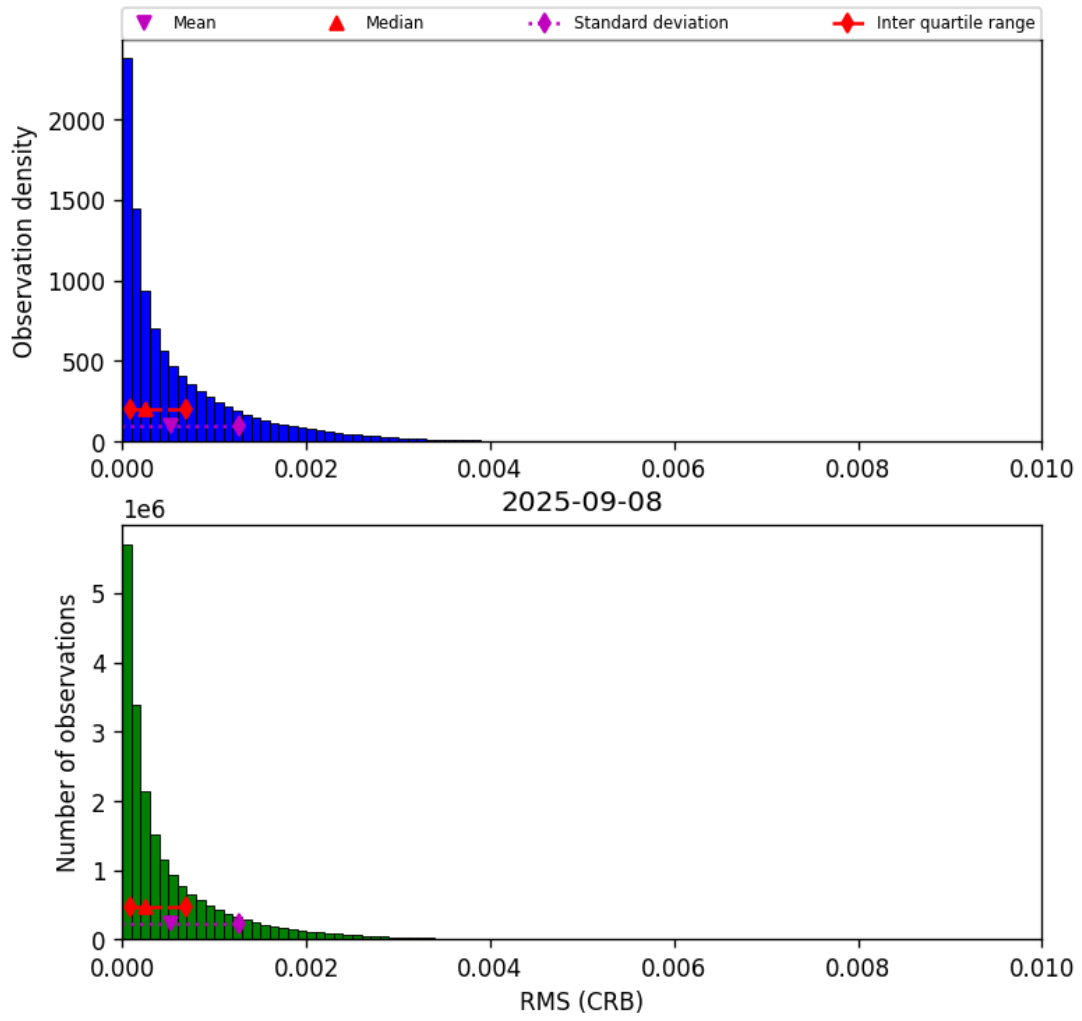
Figure 48: Histogram of “RMS (CRB)” for 2025-09-07 to 2025-09-09
