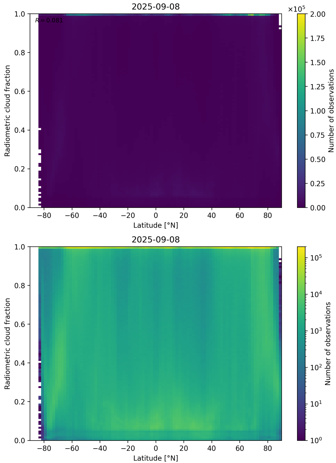
Figure 92: Scatter density plot of “Latitude” against “Radiometric cloud fraction” for 2025-09-07 to 2025-09-09.
