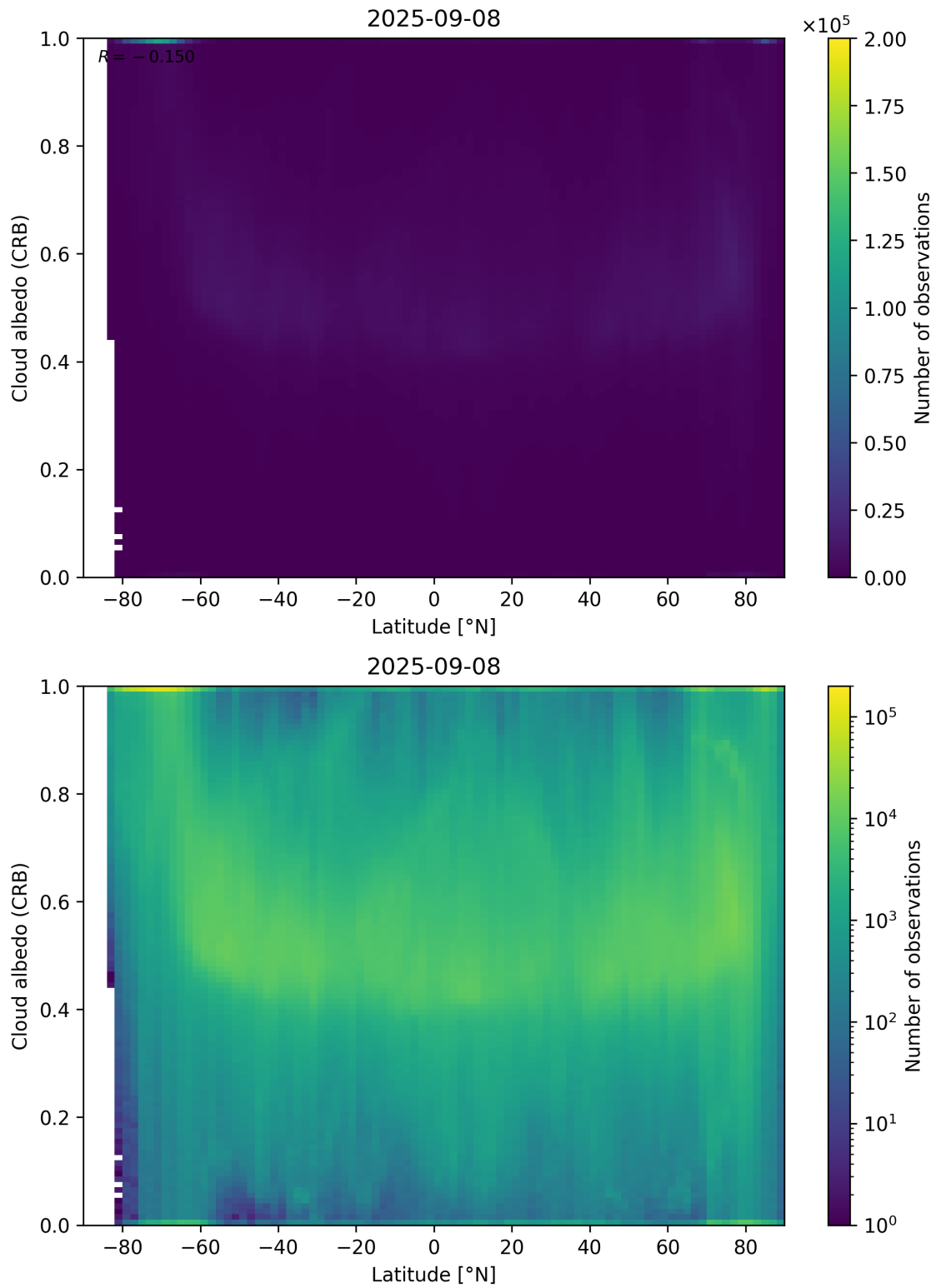
Figure 91: Scatter density plot of “Latitude” against “Cloud albedo (CRB)” for 2025-09-07 to 2025-09-09.
