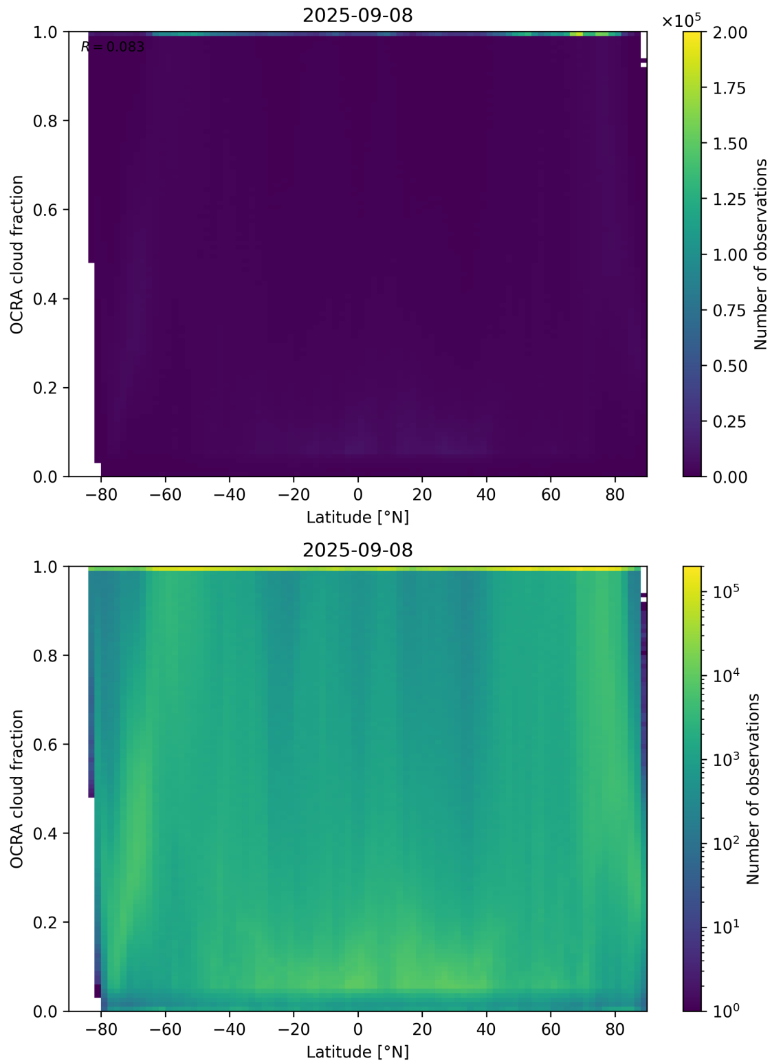
Figure 93: Scatter density plot of “Latitude” against “OCRA cloud fraction” for 2025-09-07 to 2025-09-09.
