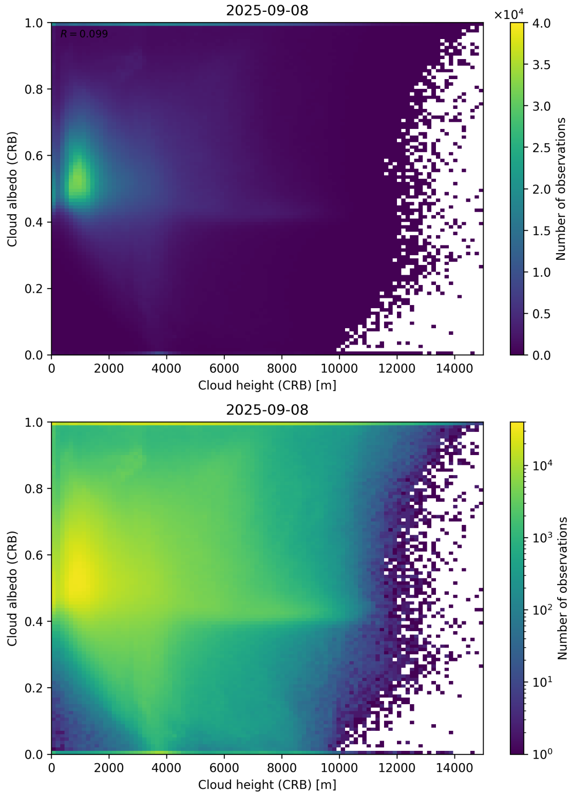
Figure 80: Scatter density plot of “Cloud height (CRB)” against “Cloud albedo (CRB)” for 2025-09-07 to 2025-09-09.
