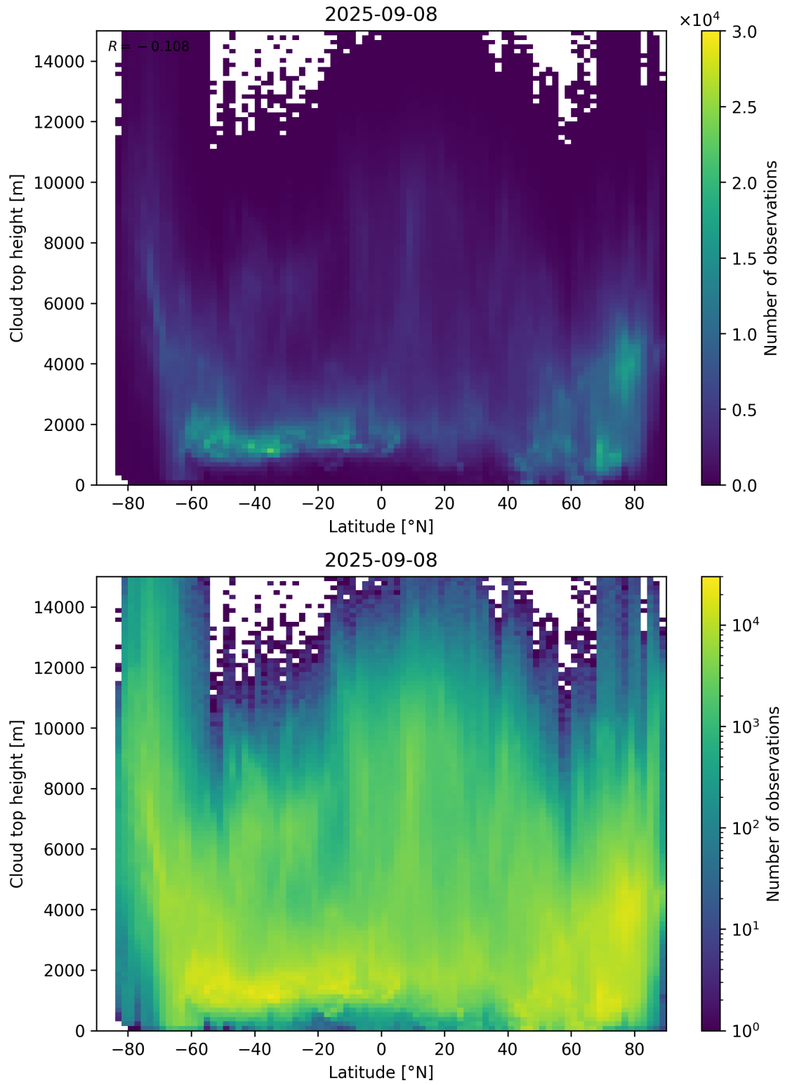
Figure 97: Scatter density plot of “Latitude” against “Cloud top height” for 2025-09-07 to 2025-09-09.
