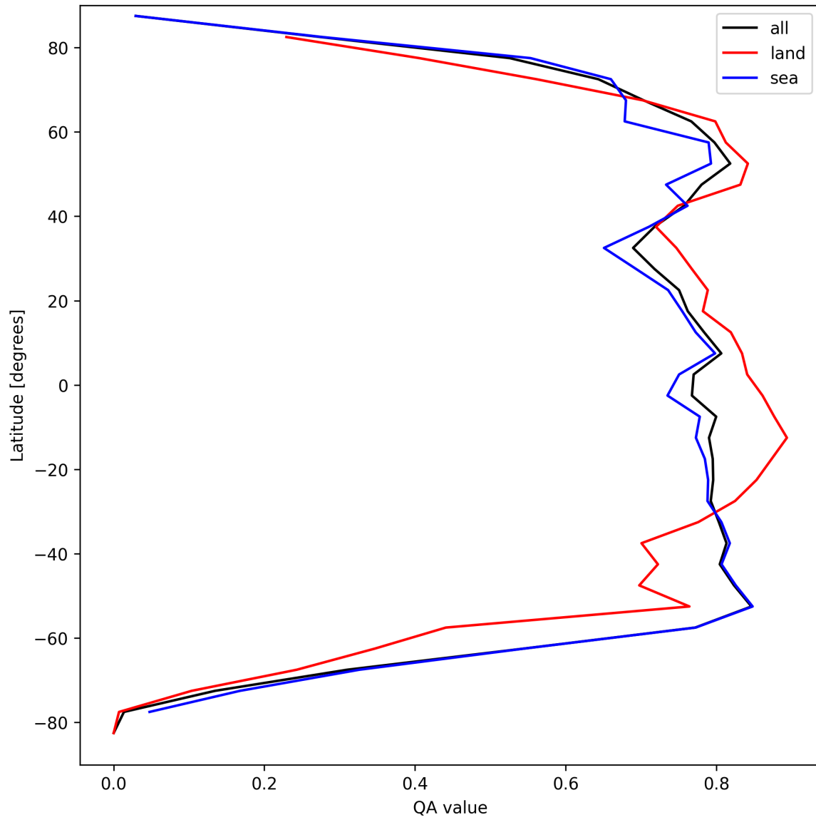
Figure 22: Zonal average of “QA value” for 2025-09-07 to 2025-09-09.
