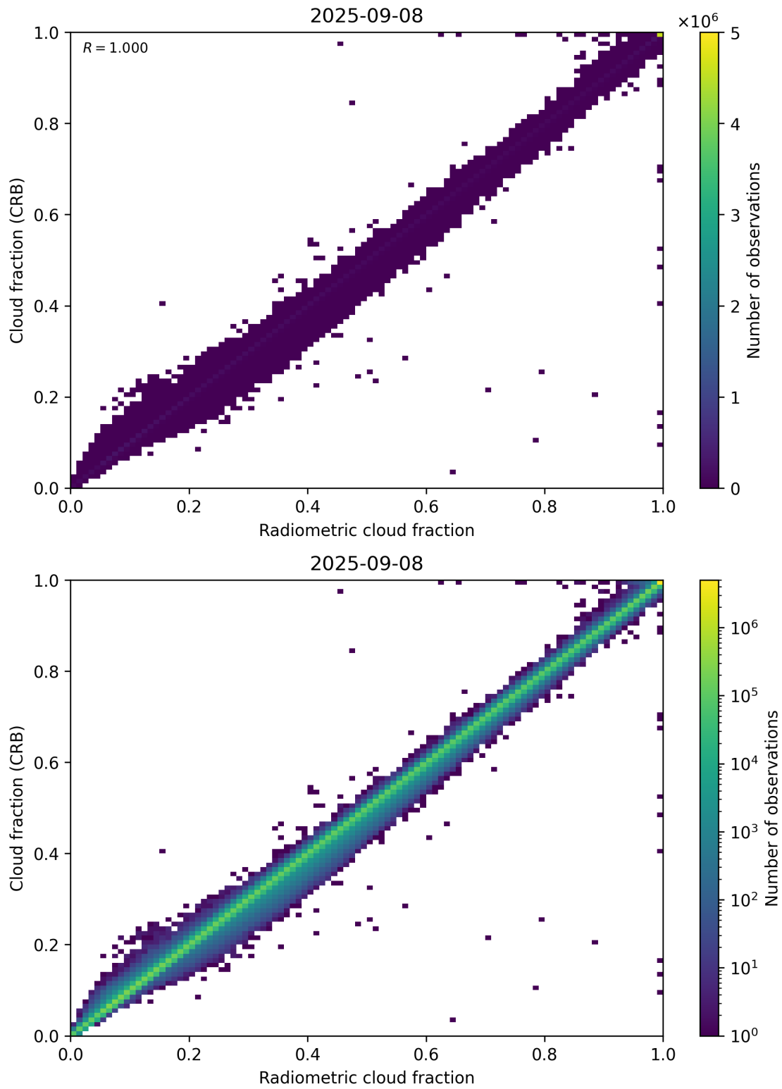
Figure 73: Scatter density plot of “Radiometric cloud fraction” against “Cloud fraction (CRB)” for 2025-09-07 to 2025-09-09.
