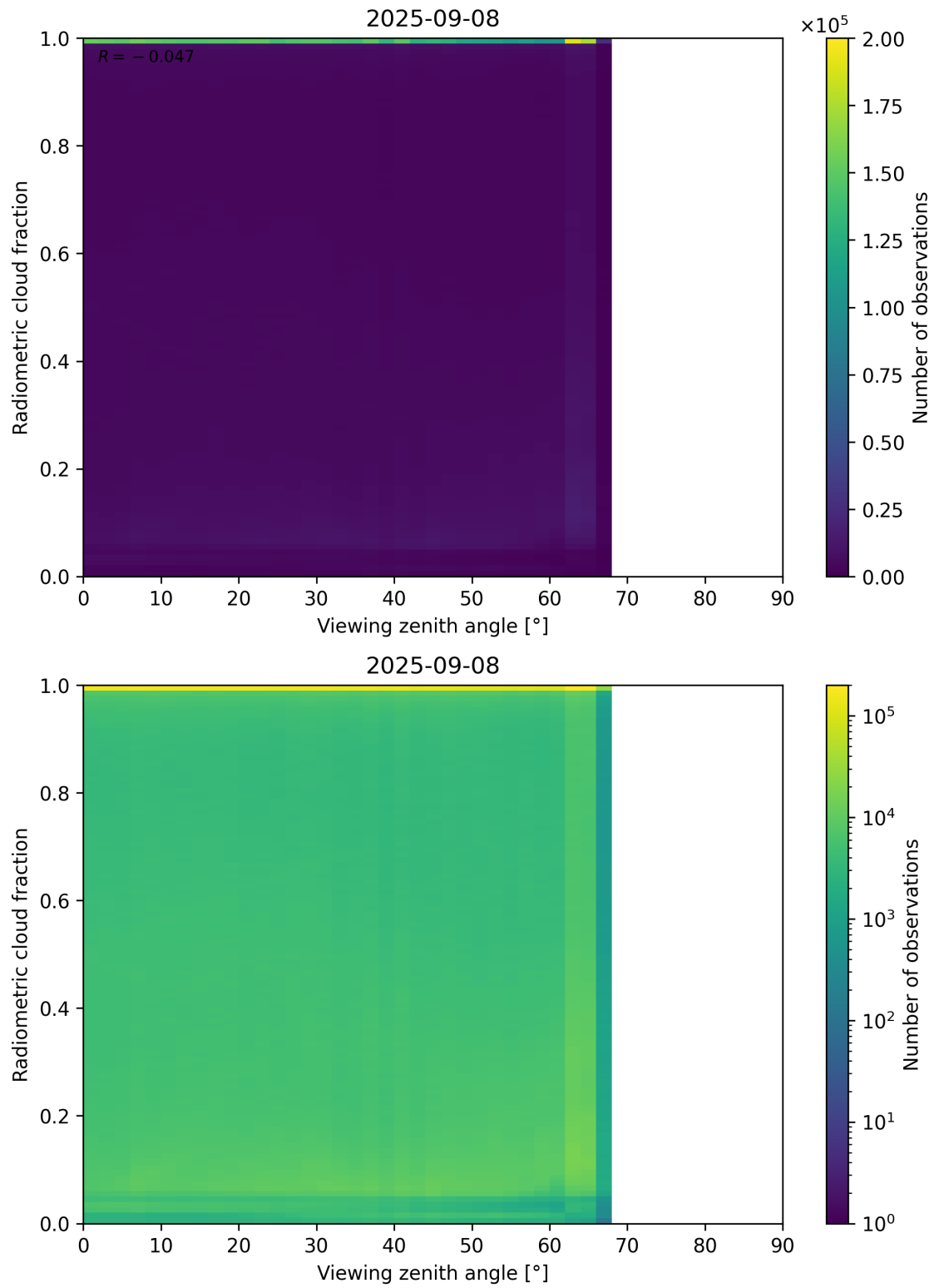
Figure 107: Scatter density plot of “Viewing zenith angle” against “Radiometric cloud fraction” for 2025-09-07 to 2025-09-09.
