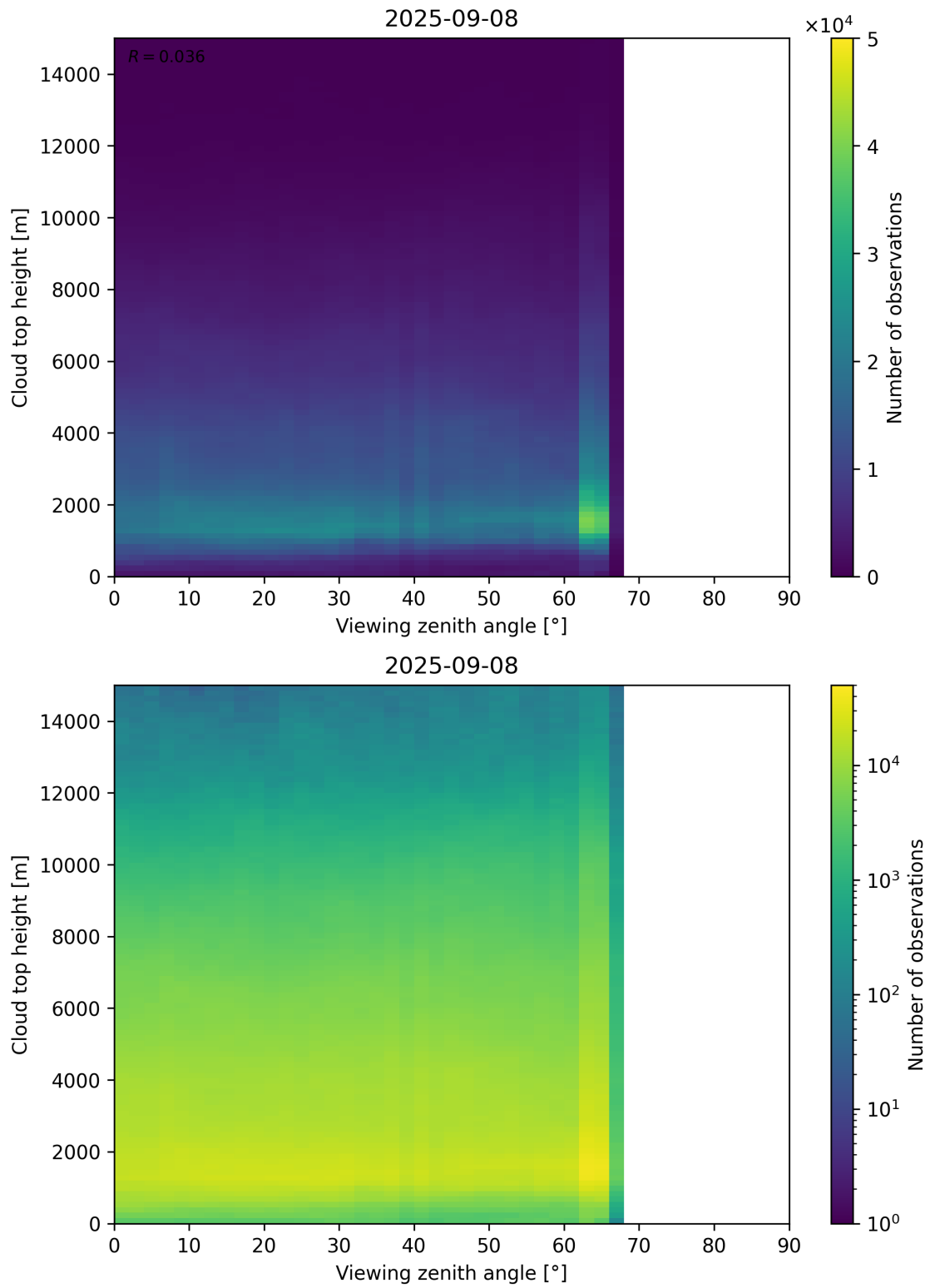
Figure 112: Scatter density plot of “Viewing zenith angle” against “Cloud top height” for 2025-09-07 to 2025-09-09.
