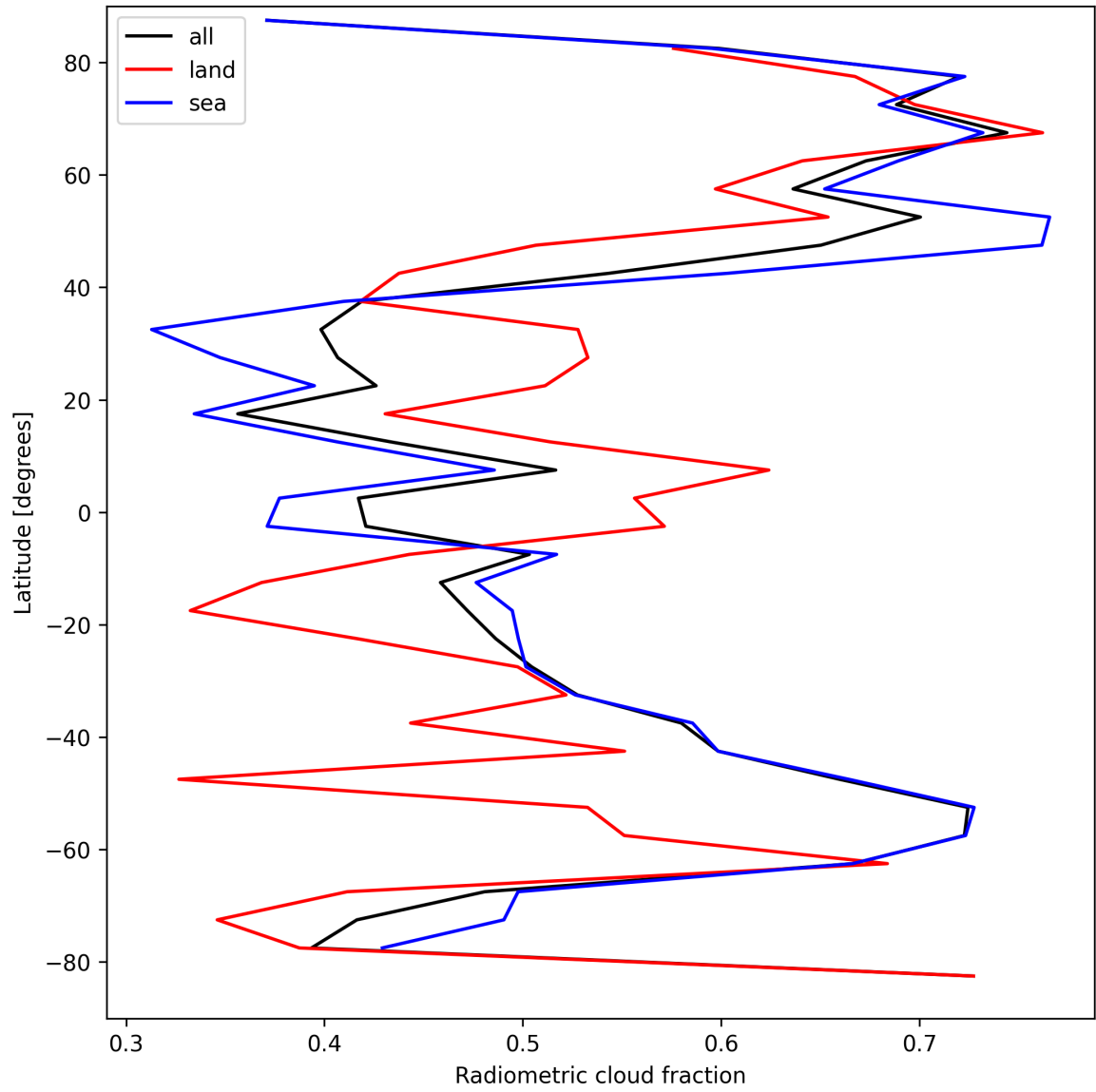
Figure 23: Zonal average of “Radiometric cloud fraction” for 2025-09-07 to 2025-09-09.
