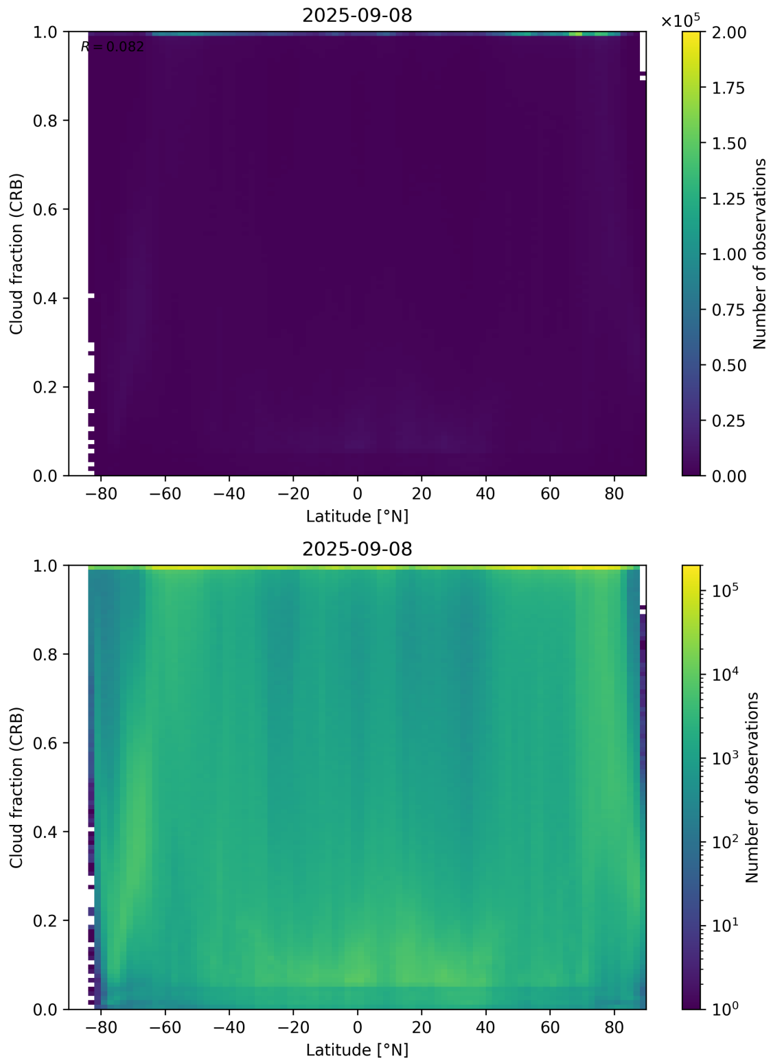
Figure 94: Scatter density plot of “Latitude” against “Cloud fraction (CRB)” for 2025-09-07 to 2025-09-09.
