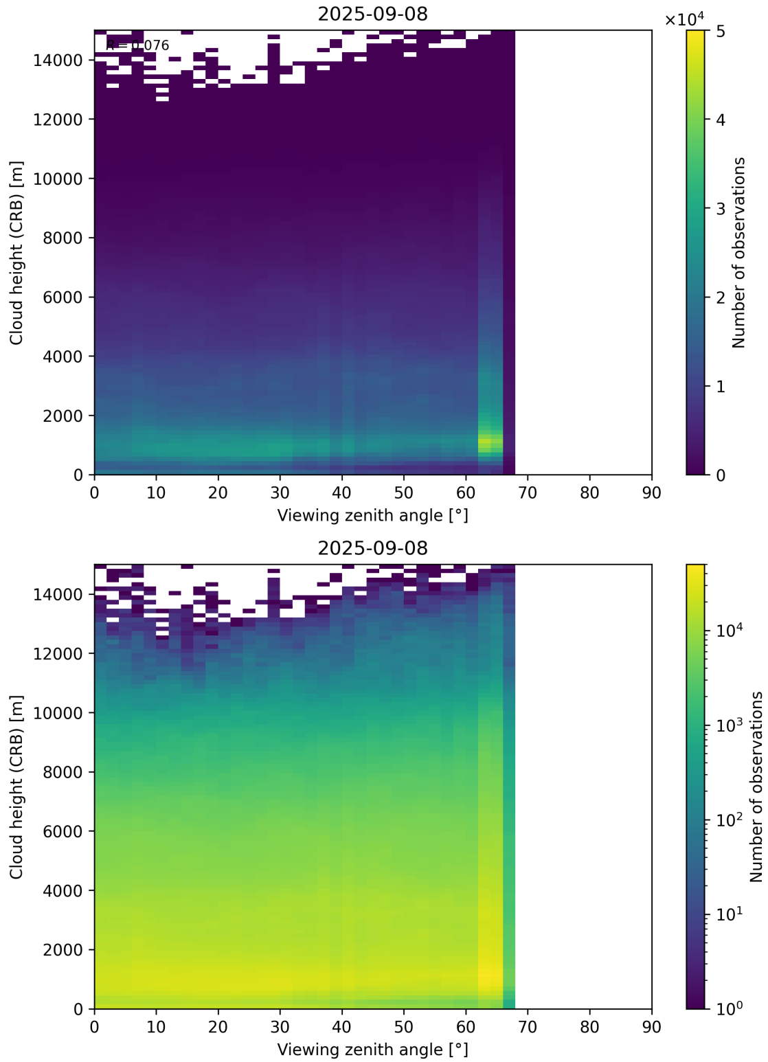
Figure 110: Scatter density plot of “Viewing zenith angle” against “Cloud height (CRB)” for 2025-09-07 to 2025-09-09.
