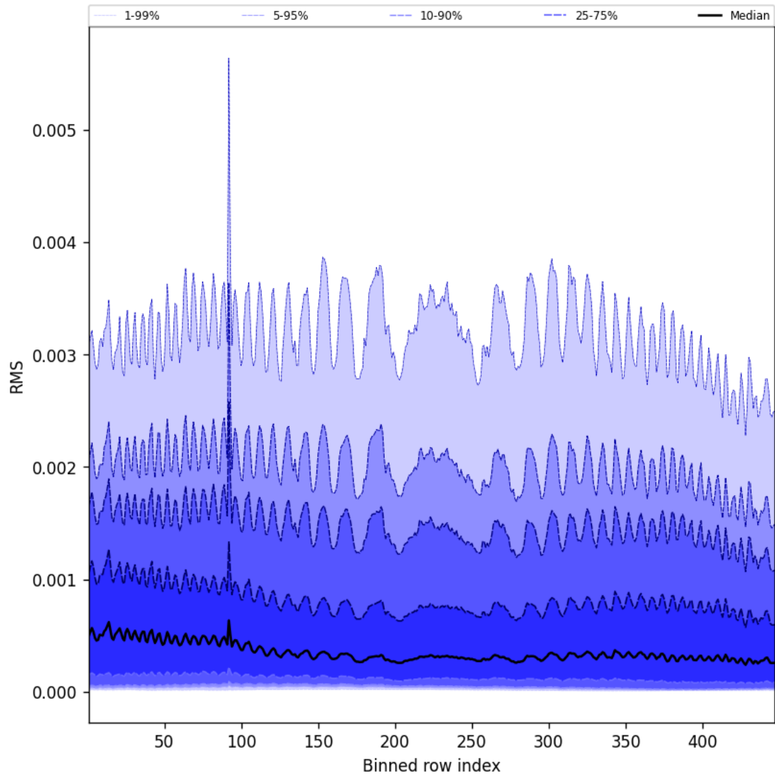
Figure 63: Along track statistics of “RMS” for 2025-09-07 to 2025-09-09
