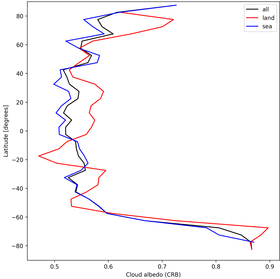
Figure 28: Zonal average of “Cloud albedo (CRB)” for 2025-09-07 to 2025-09-09.
