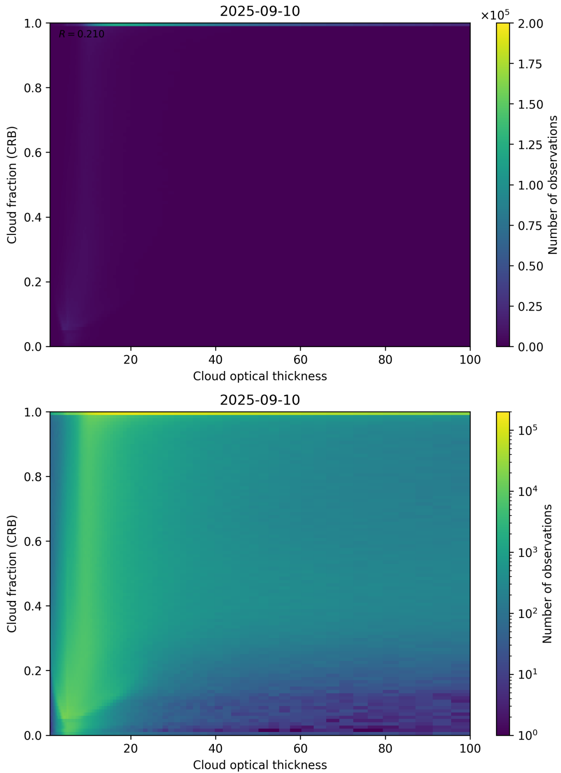
Figure 84: Scatter density plot of “Cloud optical thickness” against “Cloud fraction (CRB)” for 2025-09-10 to 2025-09-11.
