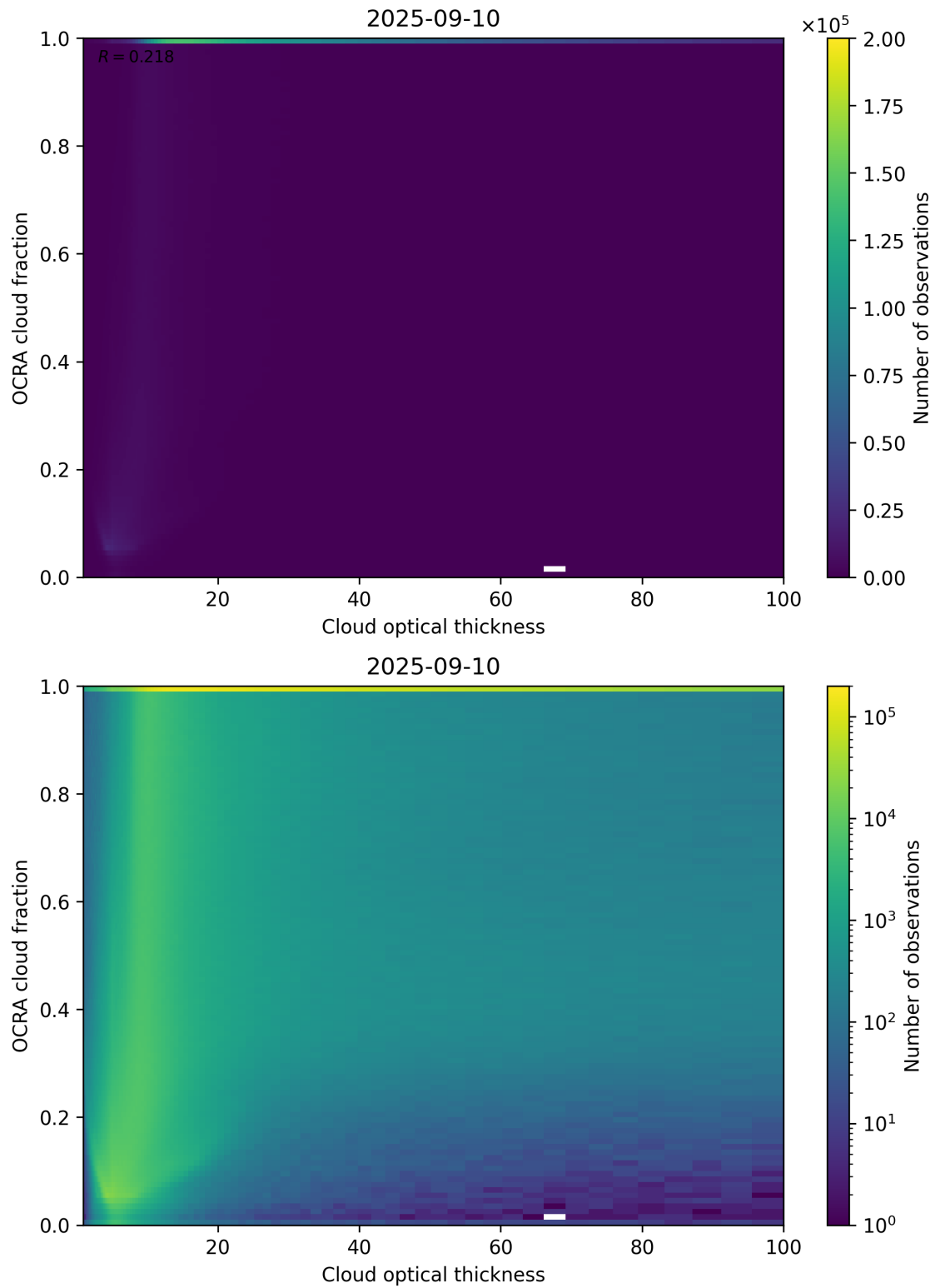
Figure 83: Scatter density plot of “Cloud optical thickness” against “OCRA cloud fraction” for 2025-09-10 to 2025-09-11.
