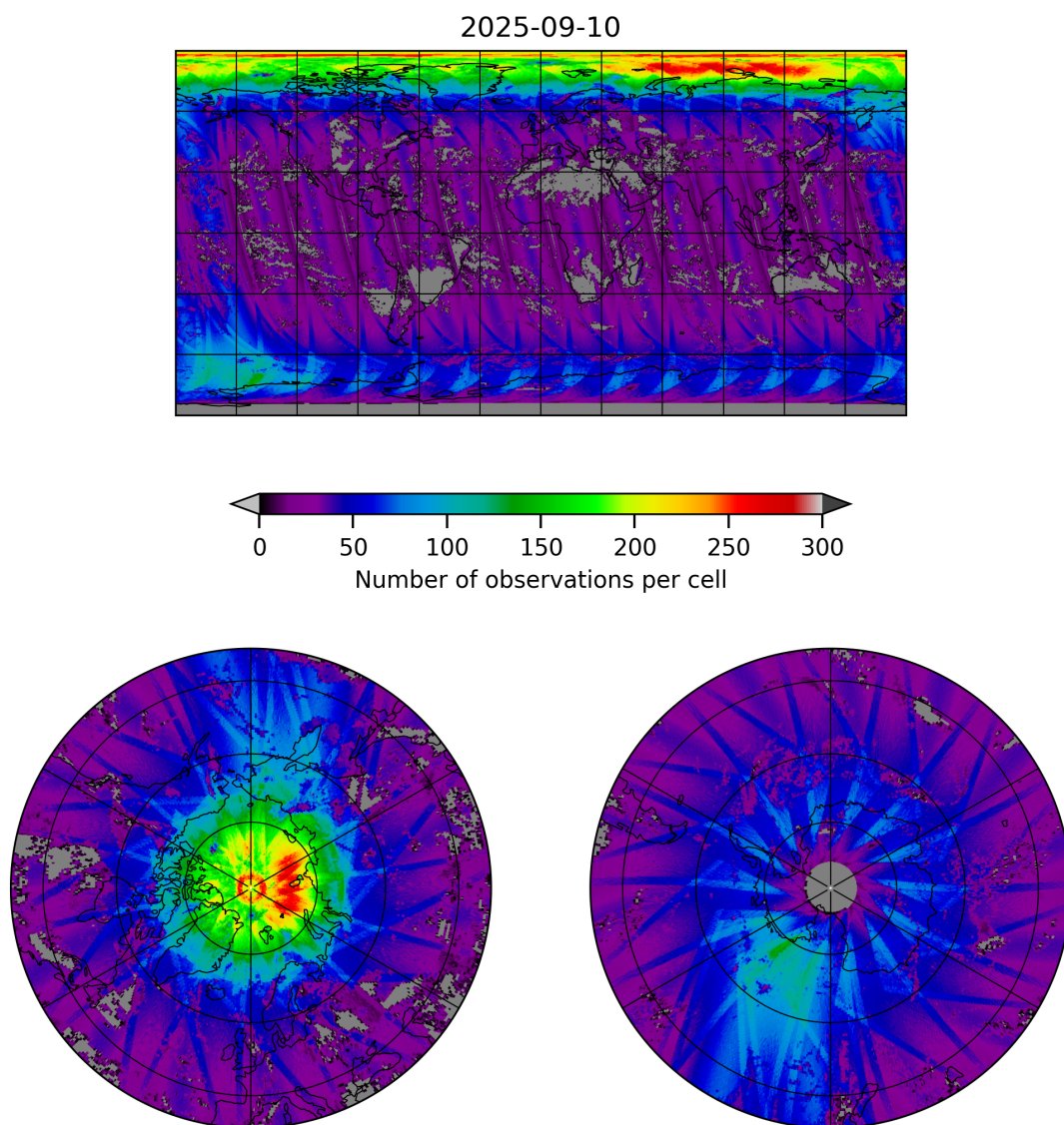
Figure 21: Map of the number of observations for 2025-09-10 to 2025-09-11
