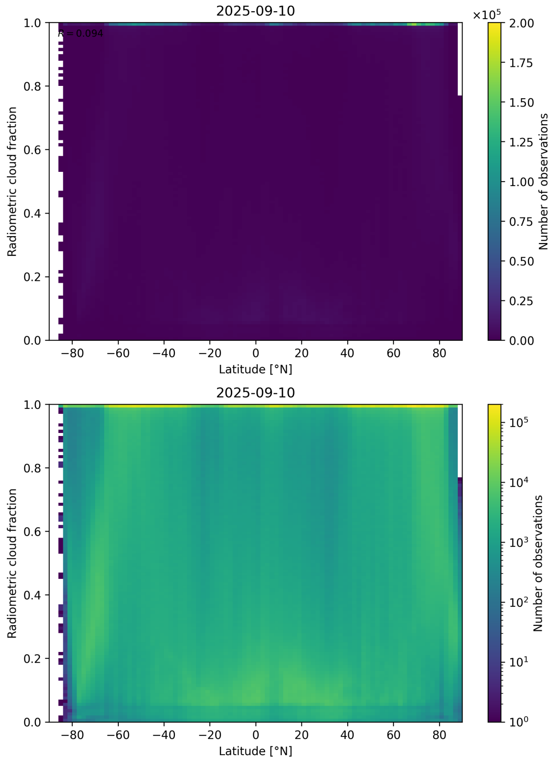
Figure 92: Scatter density plot of “Latitude” against “Radiometric cloud fraction” for 2025-09-10 to 2025-09-11.
