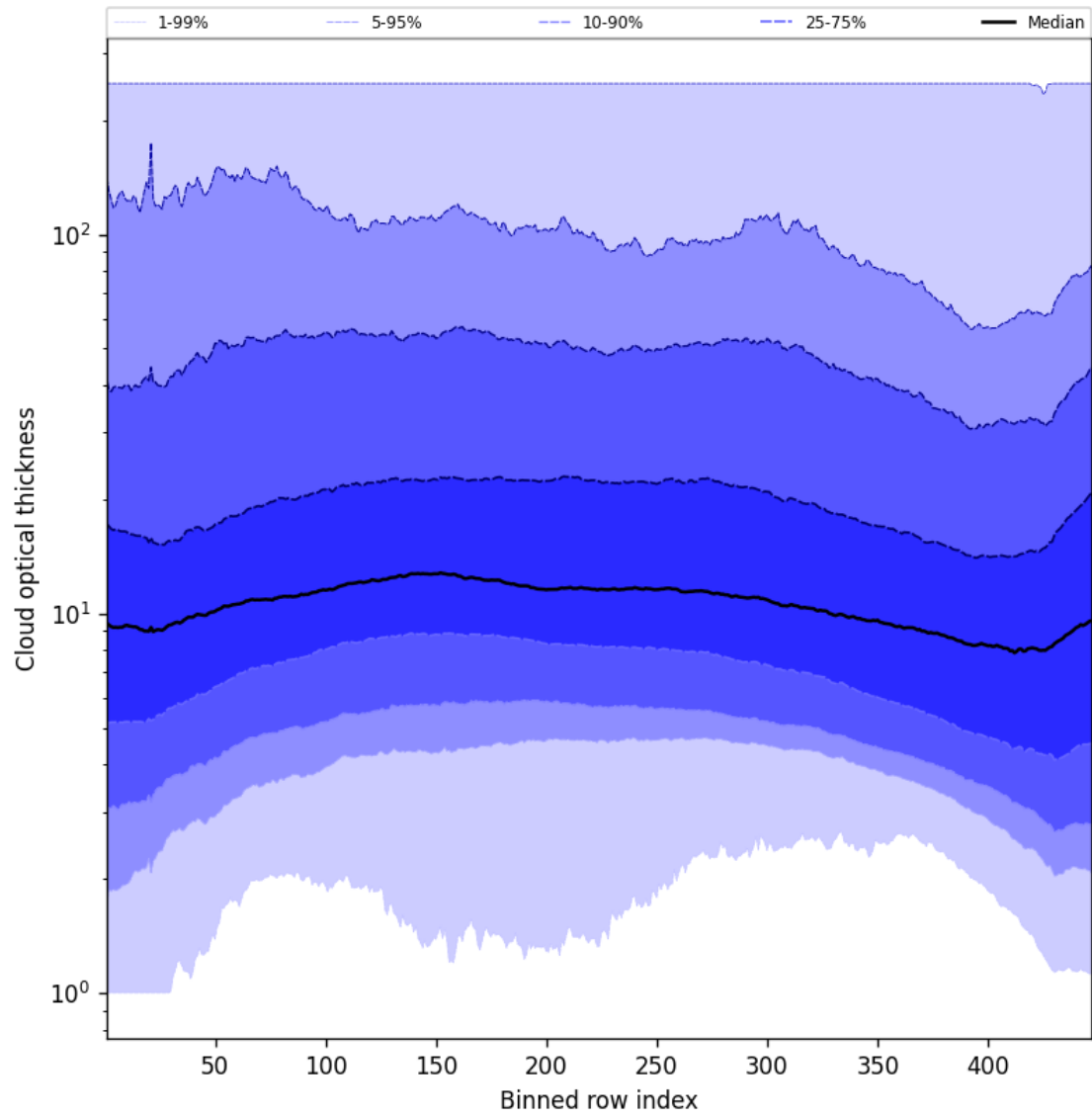
Figure 57: Along track statistics of “Cloud optical thickness” for 2025-09-10 to 2025-09-11
