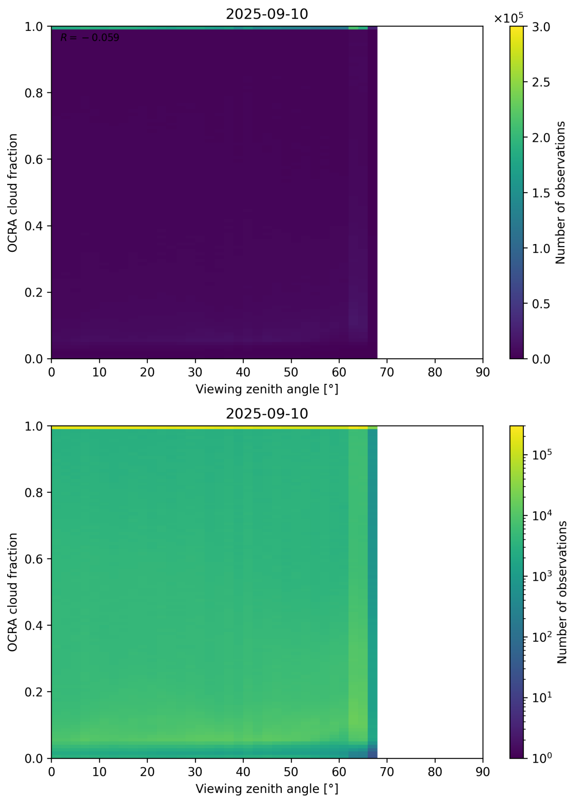
Figure 108: Scatter density plot of “Viewing zenith angle” against “OCRA cloud fraction” for 2025-09-10 to 2025-09-11.
