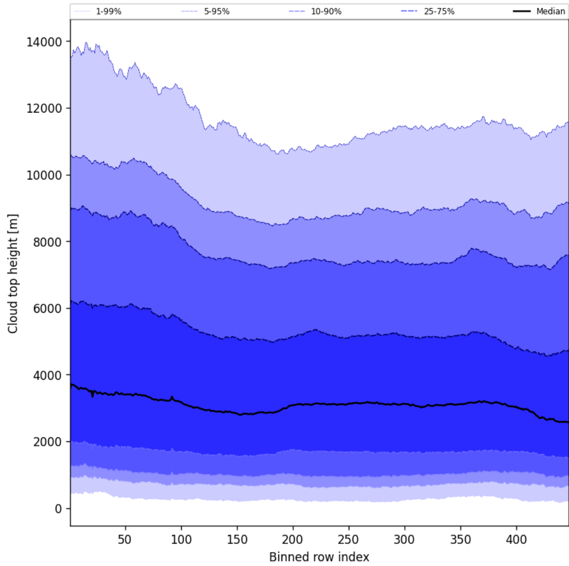
Figure 56: Along track statistics of “Cloud top height” for 2025-09-10 to 2025-09-11
