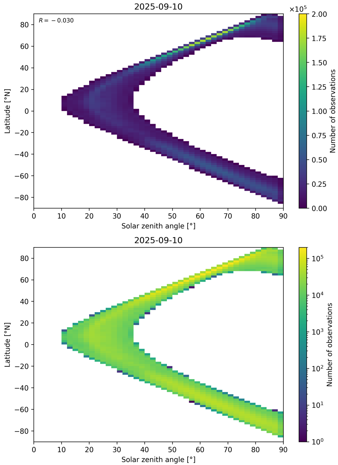
Figure 105: Scatter density plot of “Solar zenith angle” against “Latitude” for 2025-09-10 to 2025-09-11.
