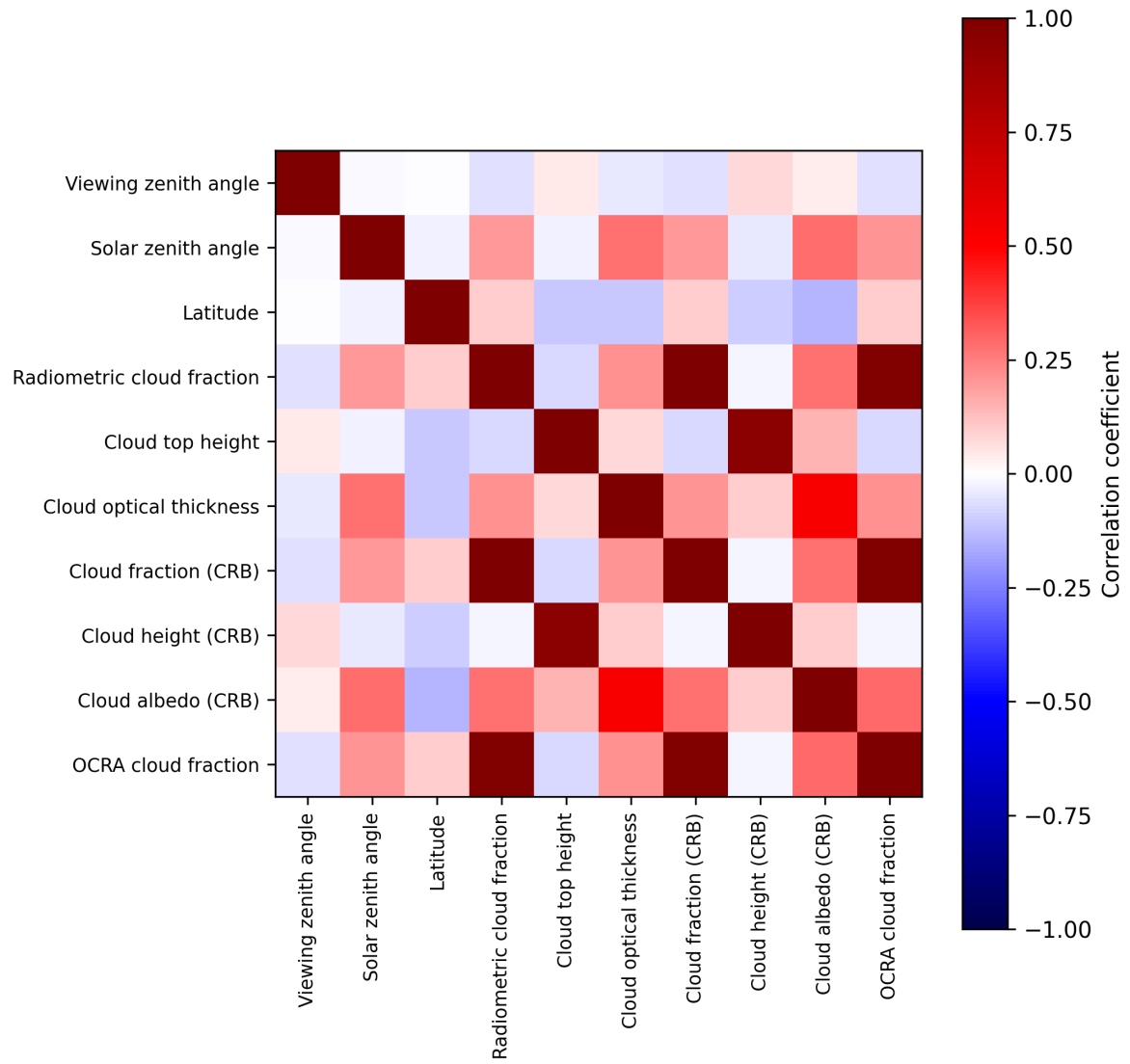
Figure 2: Map of correlation matrix for 2025-09-10 to 2025-09-11.
