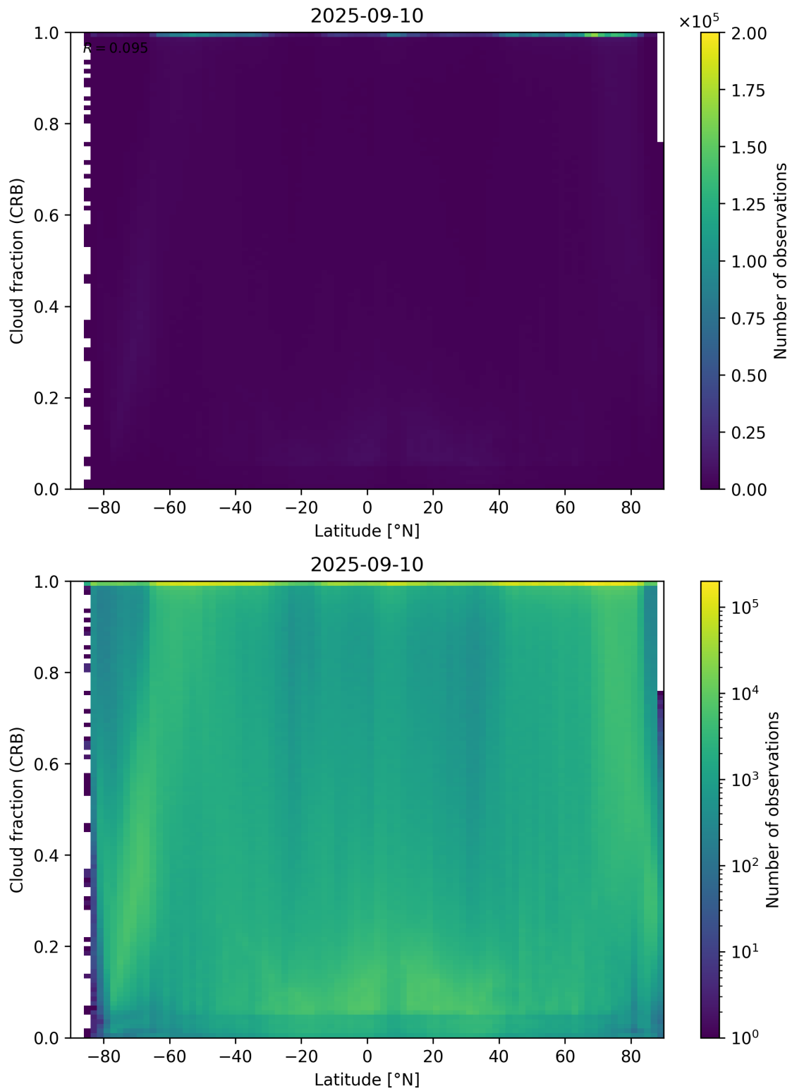
Figure 94: Scatter density plot of “Latitude” against “Cloud fraction (CRB)” for 2025-09-10 to 2025-09-11.
