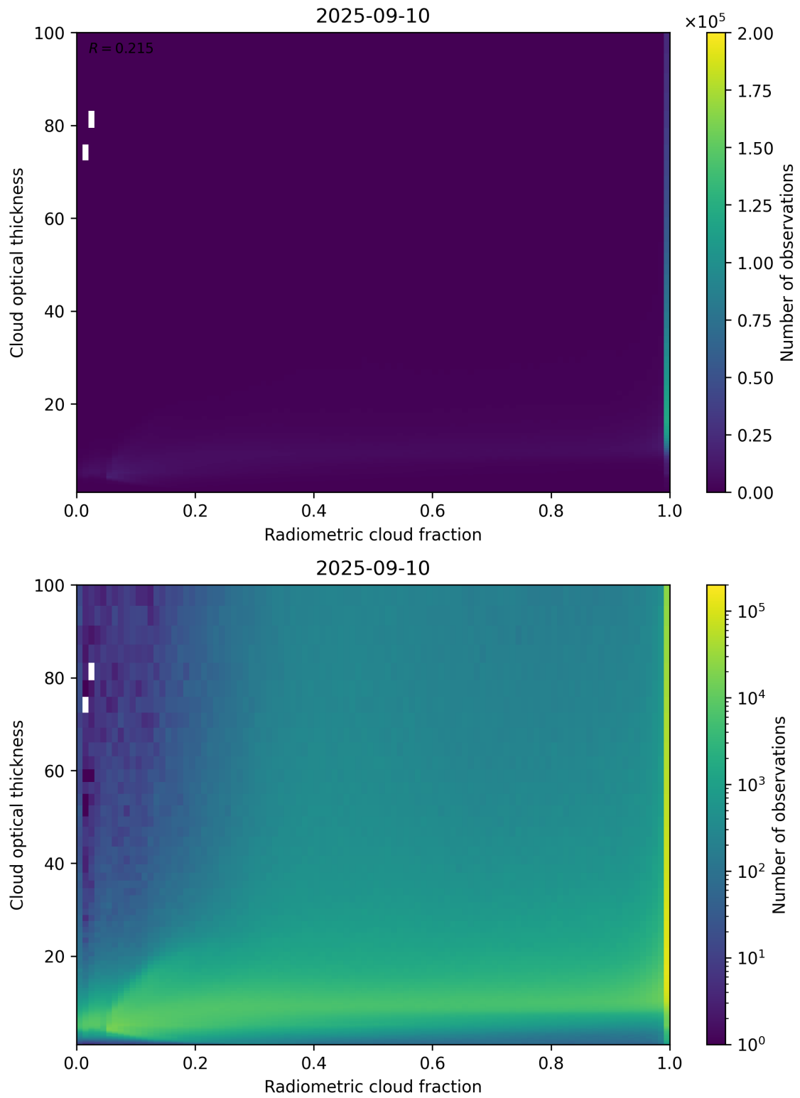
Figure 75: Scatter density plot of “Radiometric cloud fraction” against “Cloud optical thickness” for 2025-09-10 to 2025-09-11.
