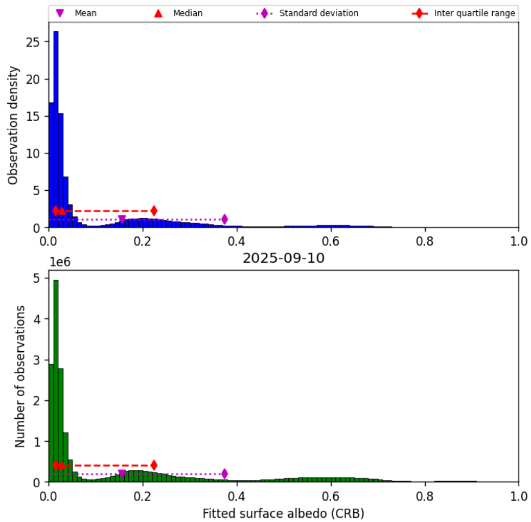
Figure 46: Histogram of “Fitted surface albedo (CRB)” for 2025-09-10 to 2025-09-11
