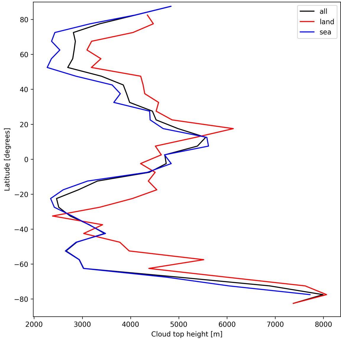
Figure 24: Zonal average of “Cloud top height” for 2025-09-10 to 2025-09-11.
