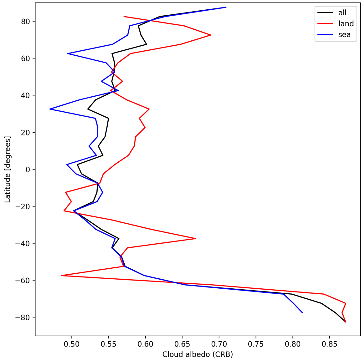
Figure 28: Zonal average of “Cloud albedo (CRB)” for 2025-09-10 to 2025-09-11.
