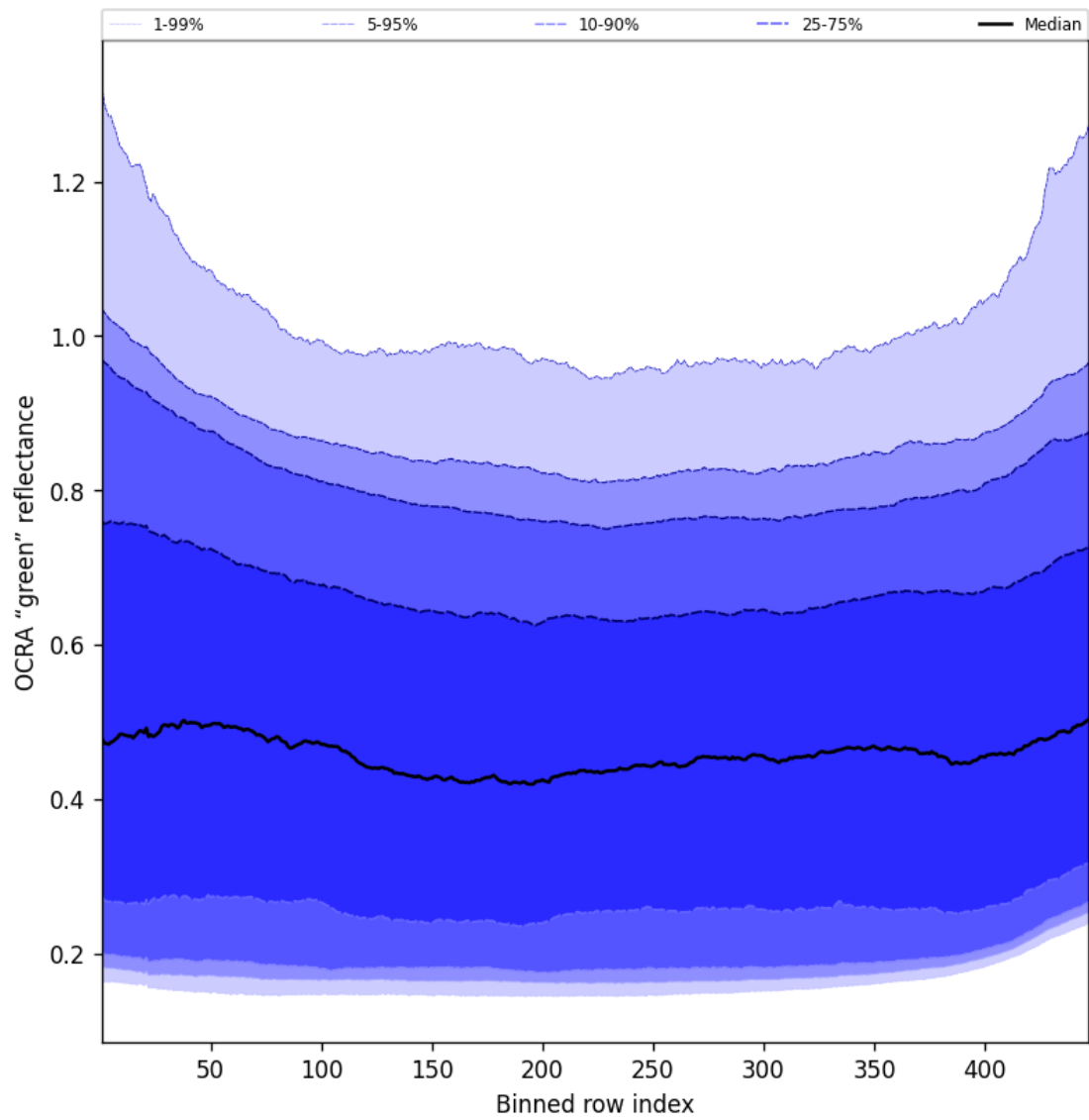
Figure 68: Along track statistics of “OCRA “green” reflectance” for 2025-09-10 to 2025-09-11
