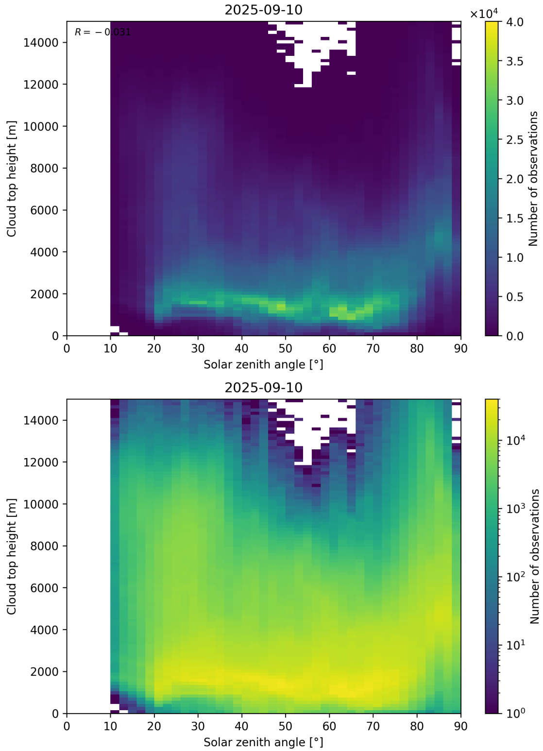
Figure 104: Scatter density plot of “Solar zenith angle” against “Cloud top height” for 2025-09-10 to 2025-09-11.
