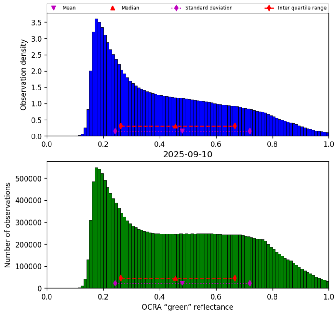
Figure 52: Histogram of “OCRA “green” reflectance” for 2025-09-10 to 2025-09-11
