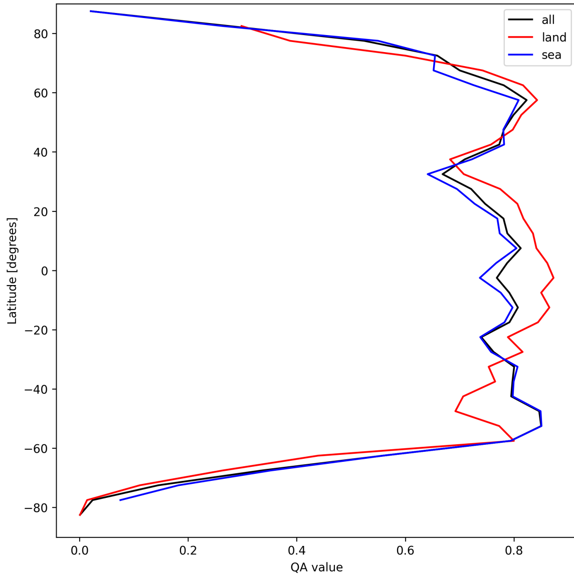
Figure 22: Zonal average of “QA value” for 2025-09-10 to 2025-09-11.
