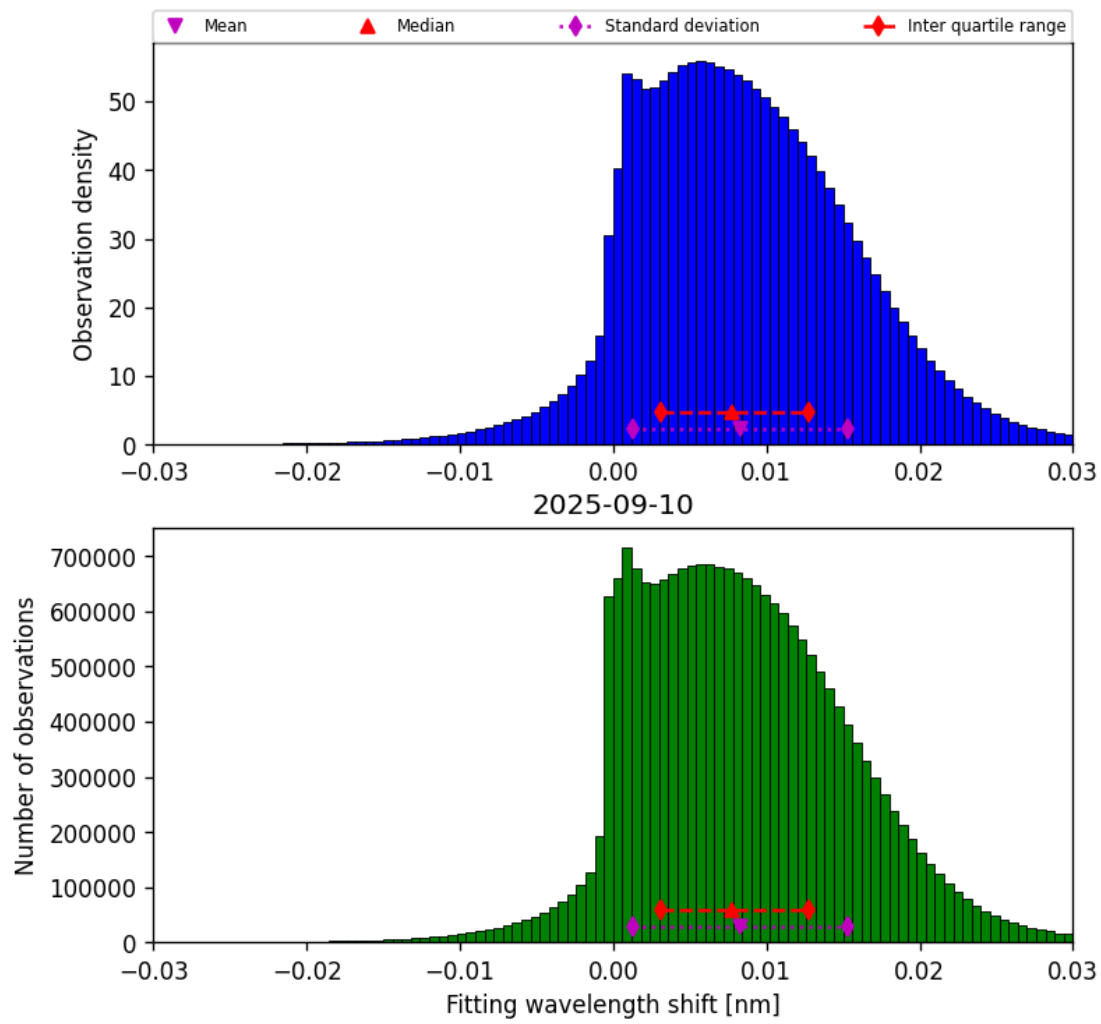
Figure 49: Histogram of “Fitting wavelength shift” for 2025-09-10 to 2025-09-11
