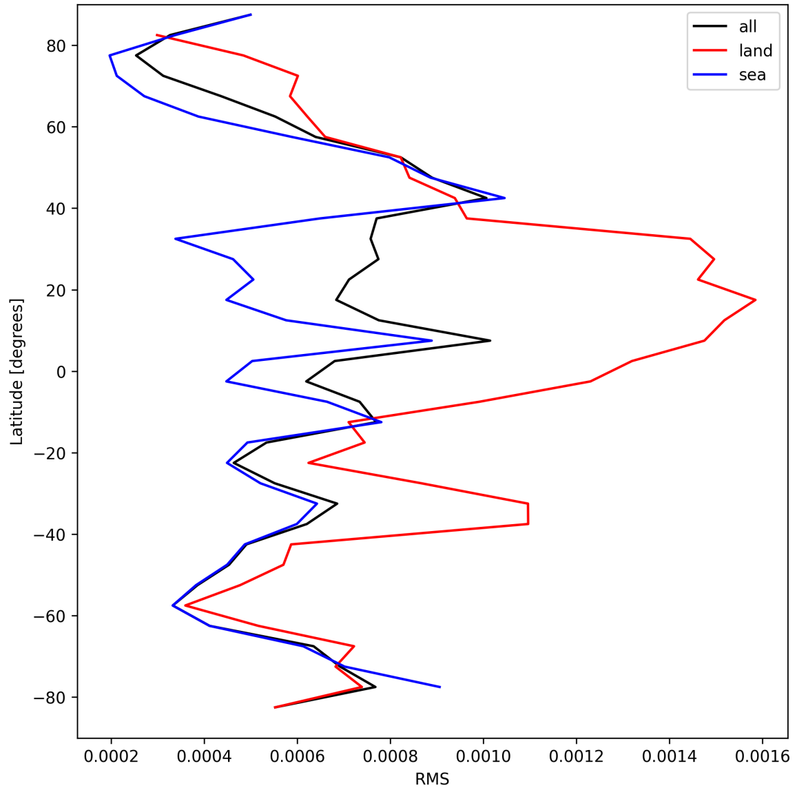
Figure 31: Zonal average of “RMS” for 2025-09-10 to 2025-09-11.
