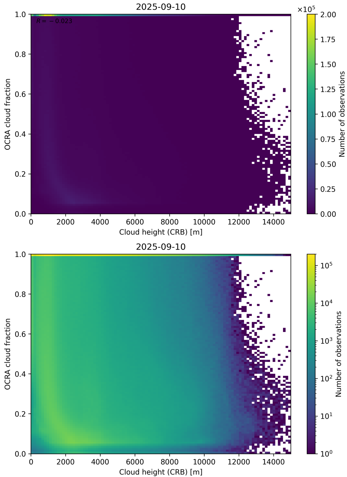
Figure 81: Scatter density plot of “Cloud height (CRB)” against “OCRA cloud fraction” for 2025-09-10 to 2025-09-11.
