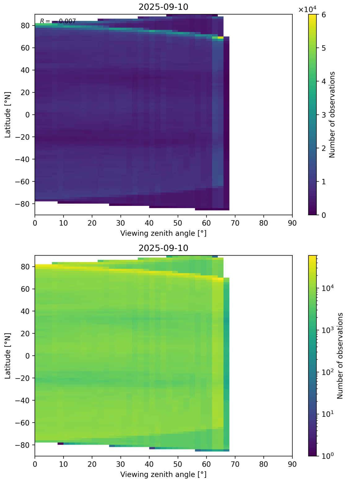
Figure 113: Scatter density plot of “Viewing zenith angle” against “Latitude” for 2025-09-10 to 2025-09-11.
