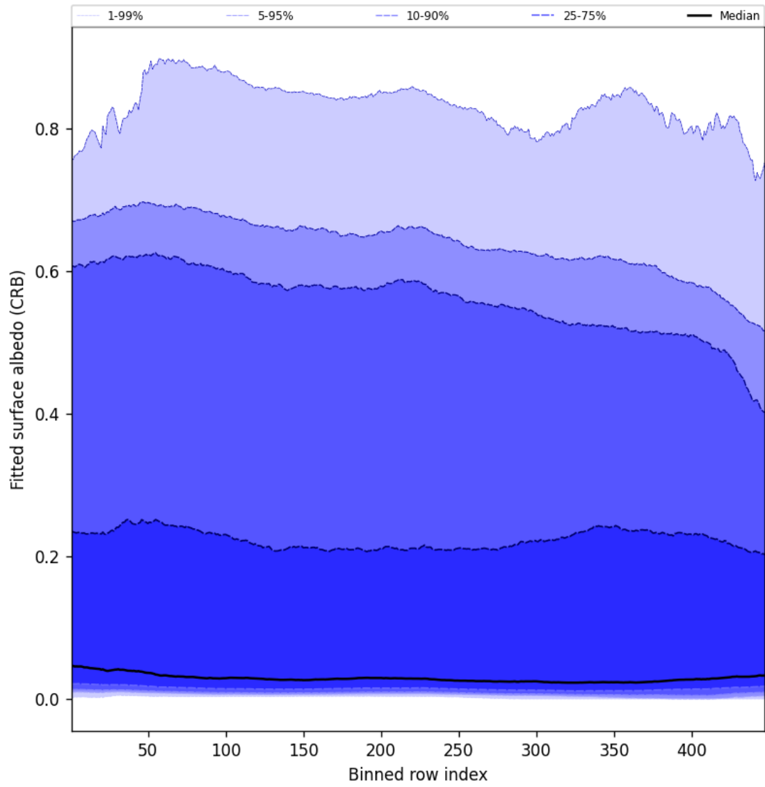
Figure 62: Along track statistics of “Fitted surface albedo (CRB)” for 2025-09-10 to 2025-09-11
