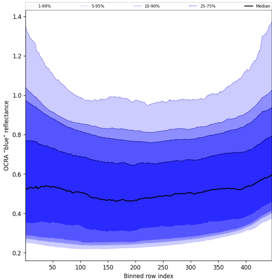
Figure 67: Along track statistics of "OCRA "blue" reflectance" for 2025-09-10 to 2025-09-11
