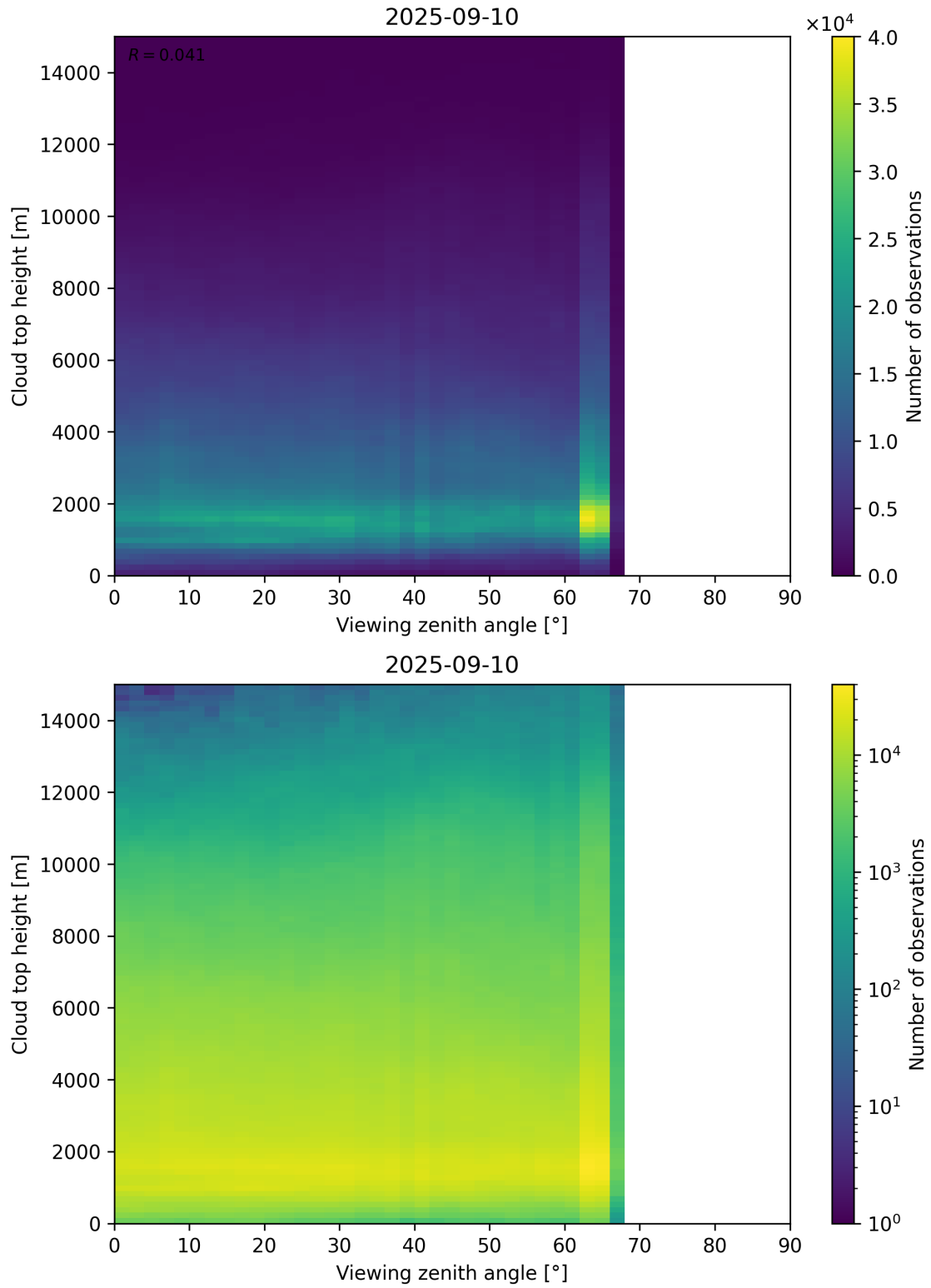
Figure 112: Scatter density plot of “Viewing zenith angle” against “Cloud top height” for 2025-09-10 to 2025-09-11.
