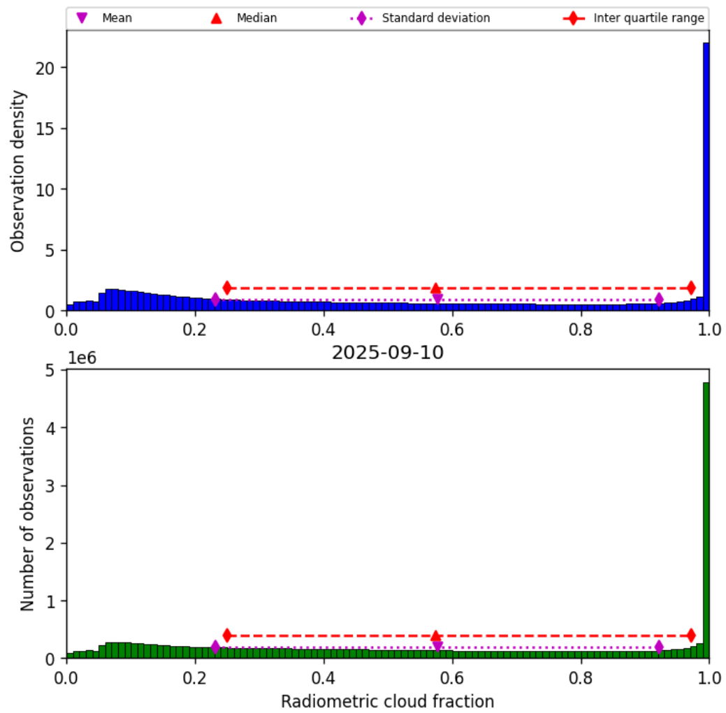
Figure 39: Histogram of “Radiometric cloud fraction” for 2025-09-10 to 2025-09-11
