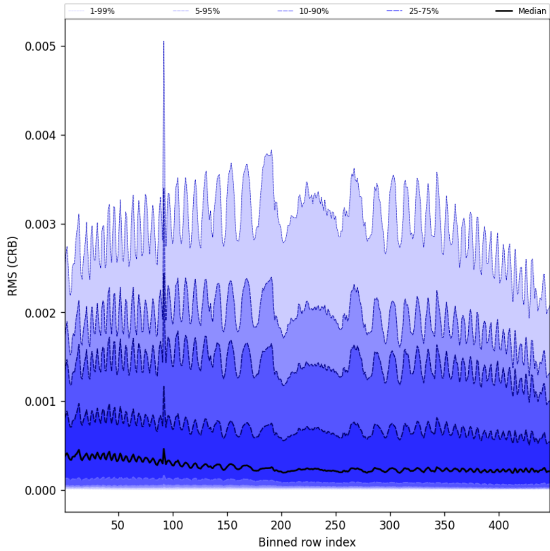
Figure 64: Along track statistics of “RMS (CRB)” for 2025-09-10 to 2025-09-11
