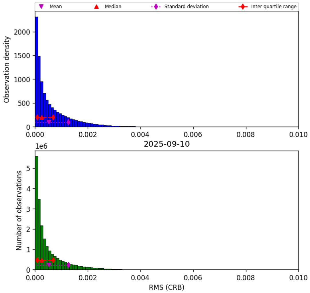
Figure 48: Histogram of "RMS (CRB)" for 2025-09-10 to 2025-09-11
