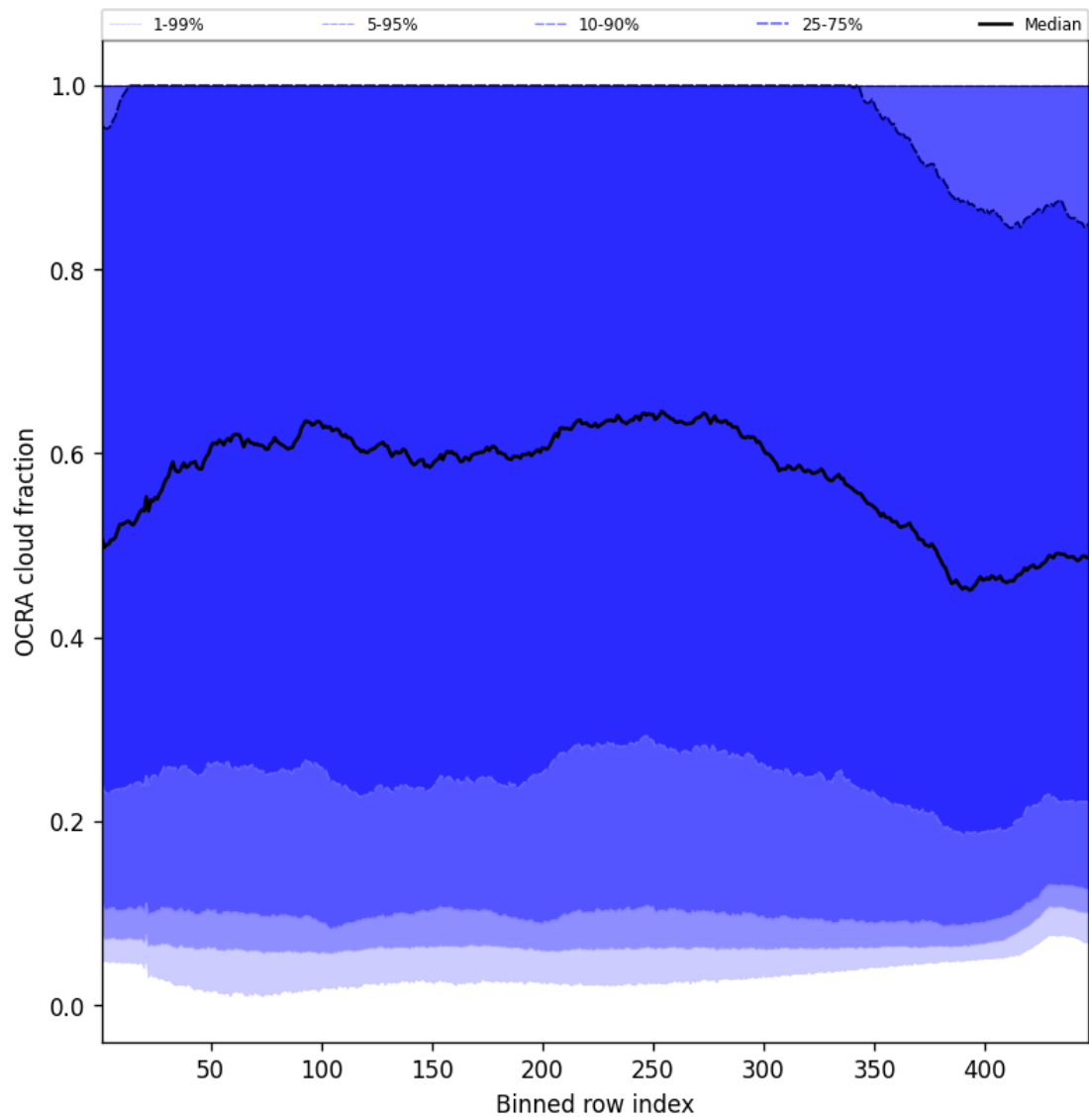
Figure 66: Along track statistics of “OCRA cloud fraction” for 2025-09-10 to 2025-09-11
