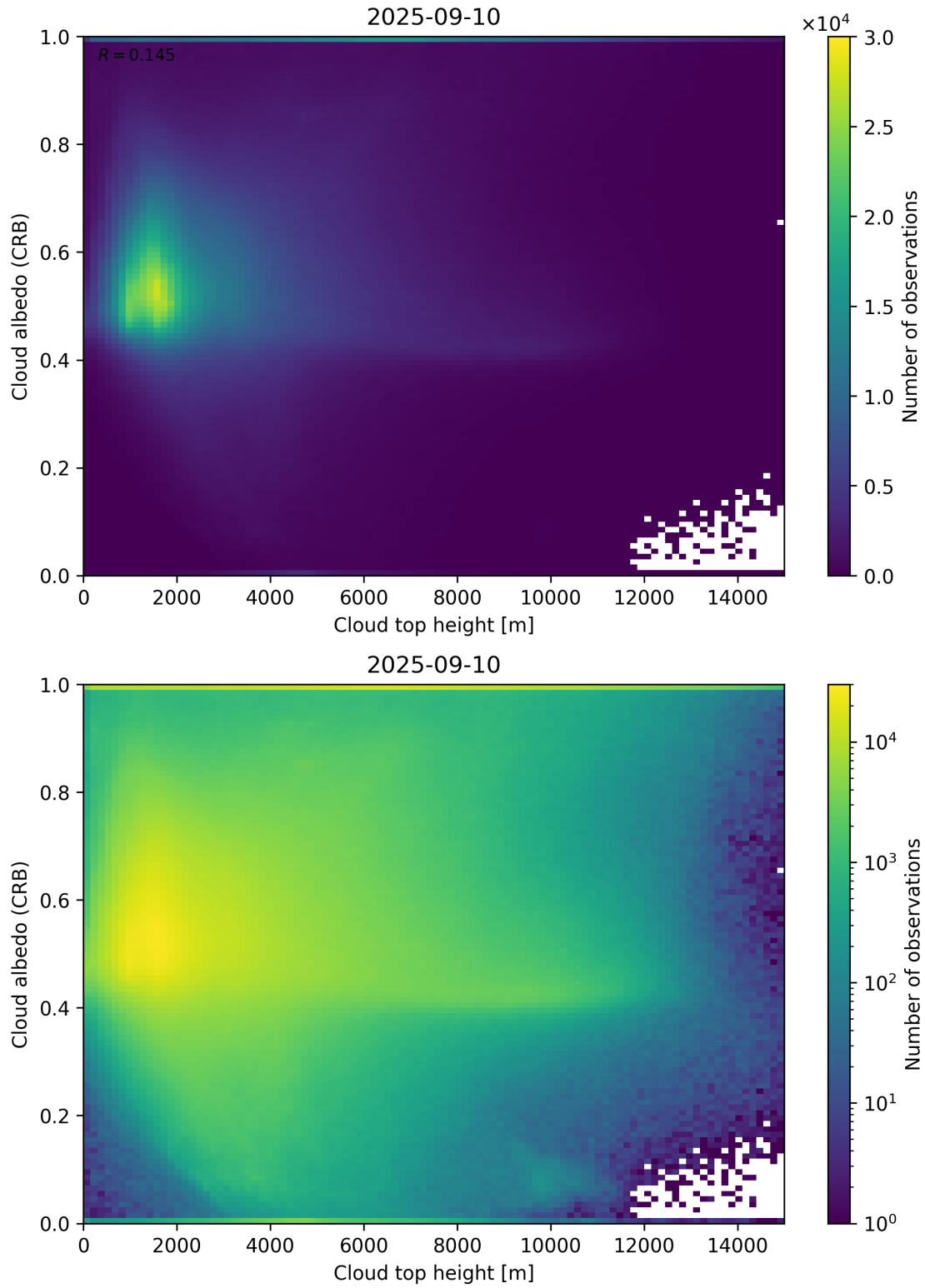
Figure 86: Scatter density plot of “Cloud top height” against “Cloud albedo (CRB)” for 2025-09-10 to 2025-09-11.
