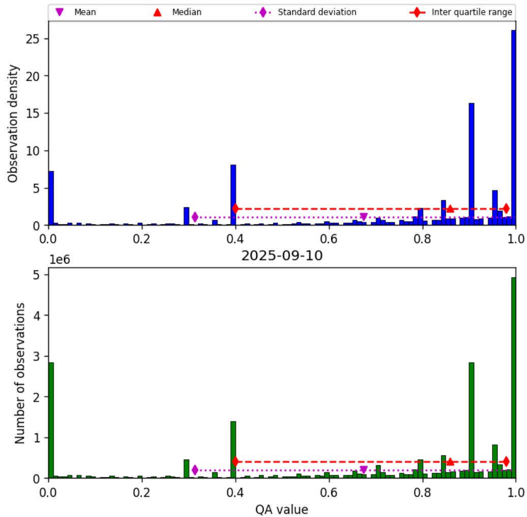
Figure 38: Histogram of “QA value” for 2025-09-10 to 2025-09-11
