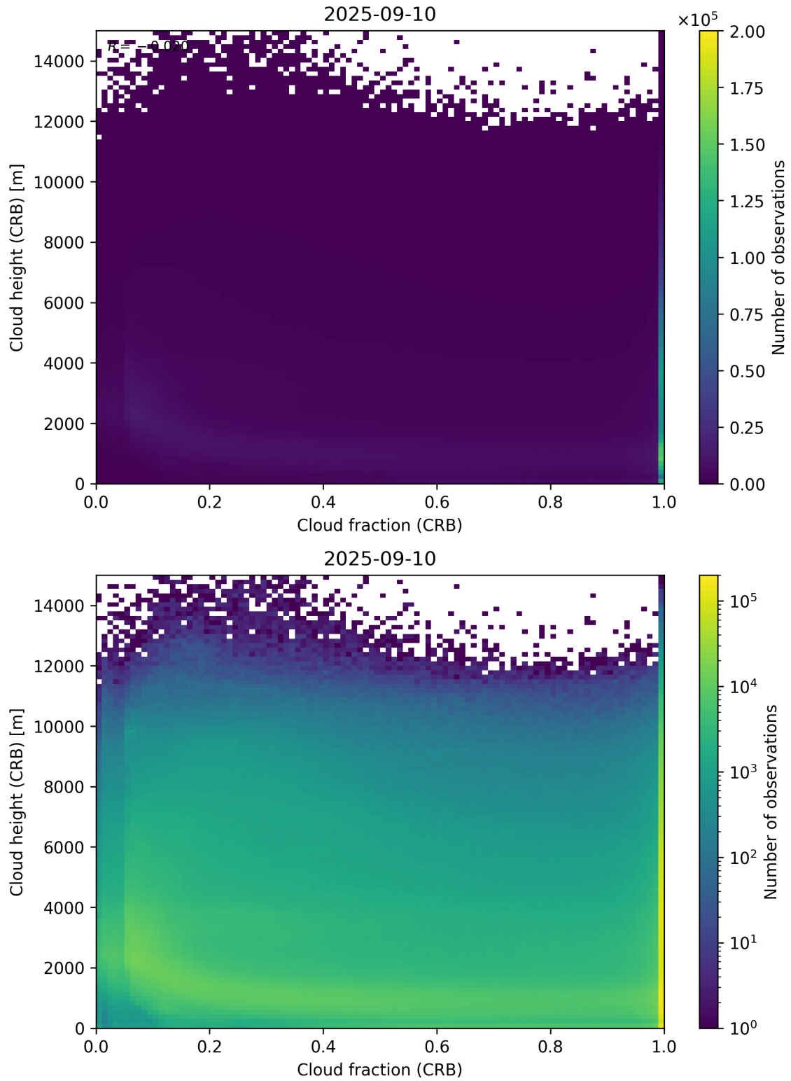
Figure 79: Scatter density plot of “Cloud fraction (CRB)” against “Cloud height (CRB)” for 2025-09-10 to 2025-09-11.
