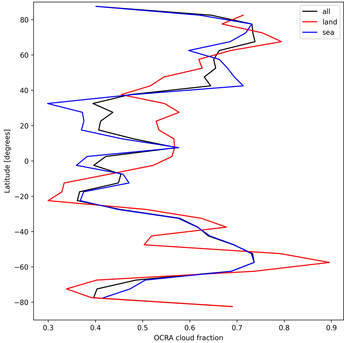
Figure 34: Zonal average of “OCRA cloud fraction” for 2025-09-10 to 2025-09-11.
