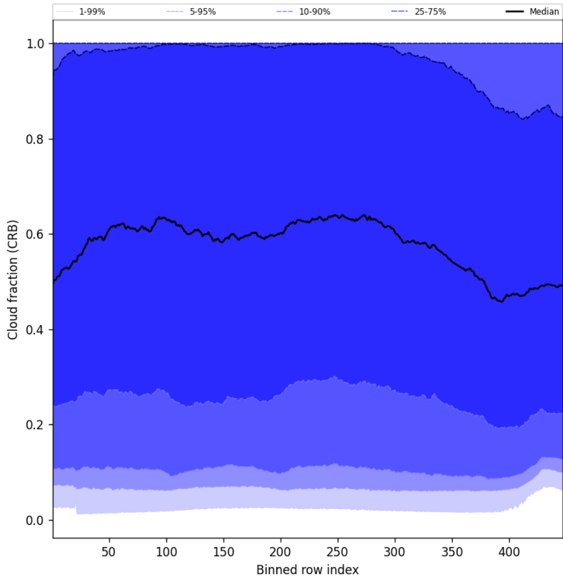
Figure 58: Along track statistics of “Cloud fraction (CRB)” for 2025-09-10 to 2025-09-11
