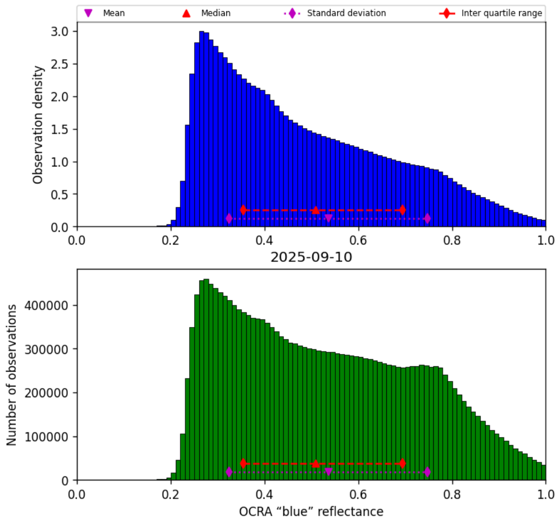
Figure 51: Histogram of “OCRA “blue” reflectance” for 2025-09-10 to 2025-09-11
