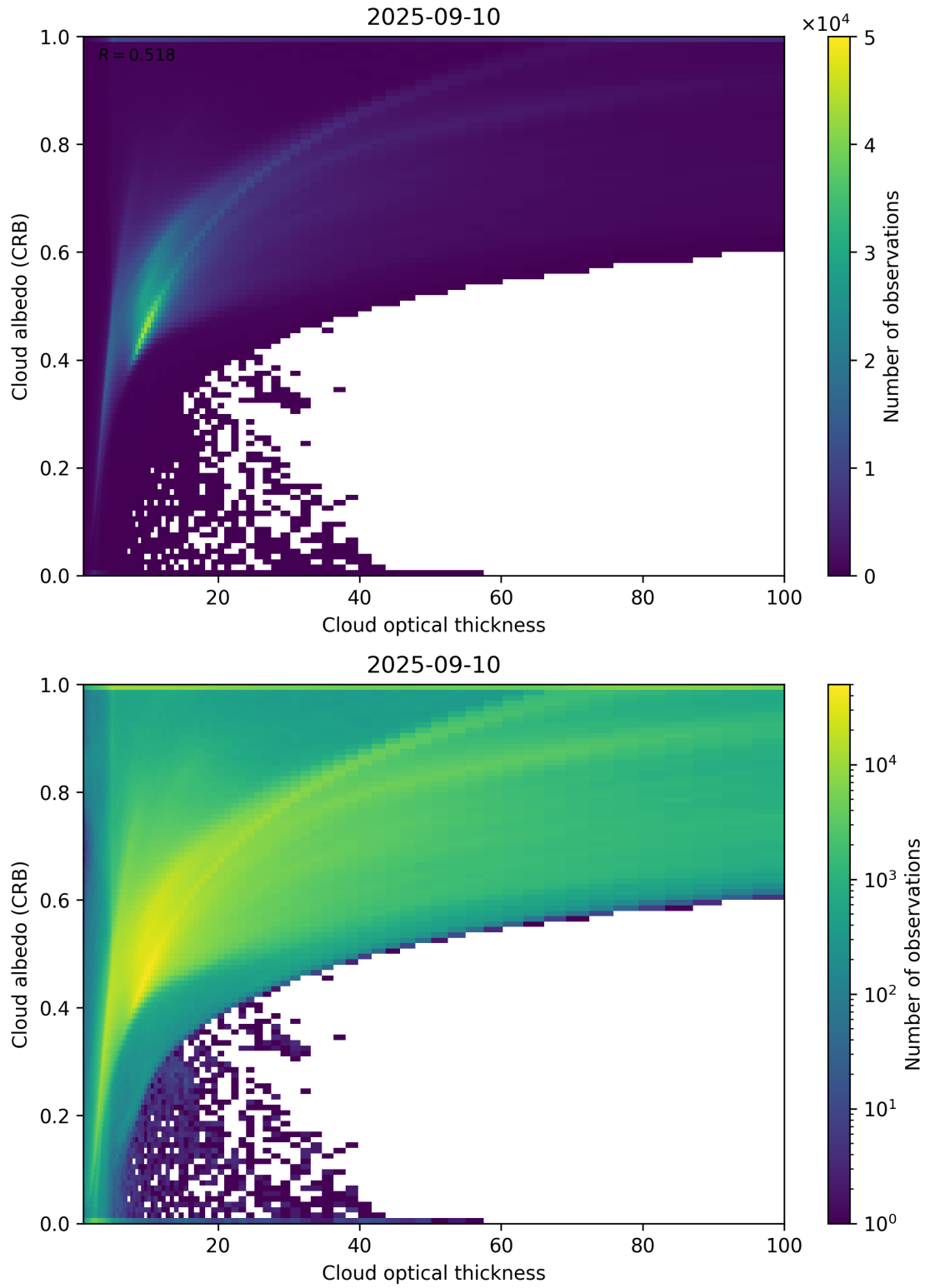
Figure 82: Scatter density plot of “Cloud optical thickness” against “Cloud albedo (CRB)” for 2025-09-10 to 2025-09-11.
