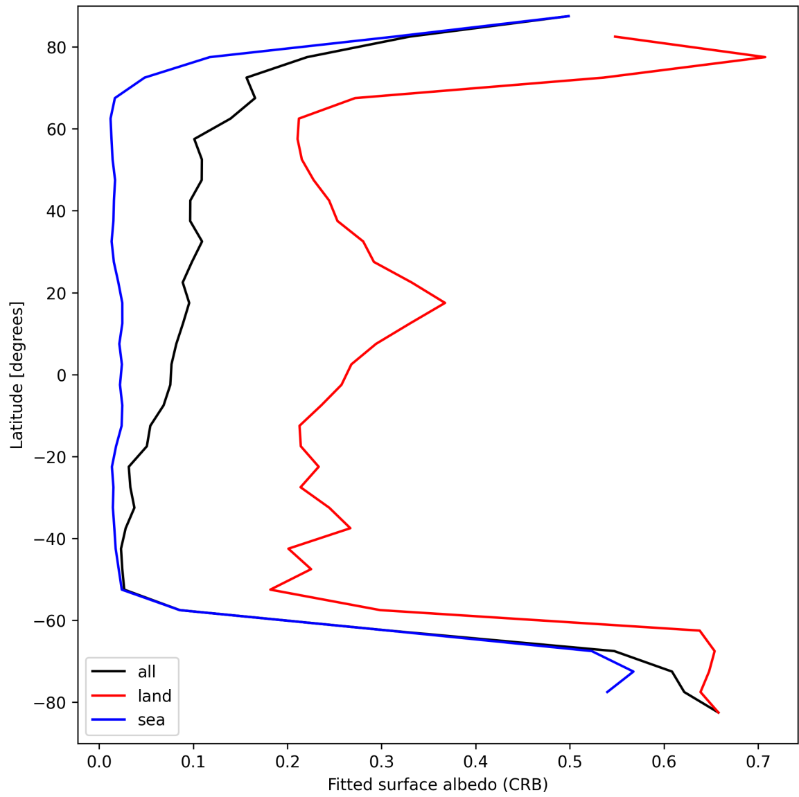
Figure 30: Zonal average of “Fitted surface albedo (CRB)” for 2025-09-10 to 2025-09-11.
