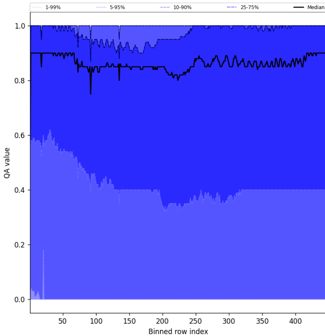
Figure 54: Along track statistics of “QA value” for 2025-09-10 to 2025-09-11
