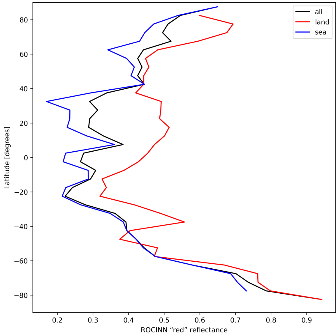
Figure 37: Zonal average of “ROCINN “red” reflectance” for 2025-09-10 to 2025-09-11.
