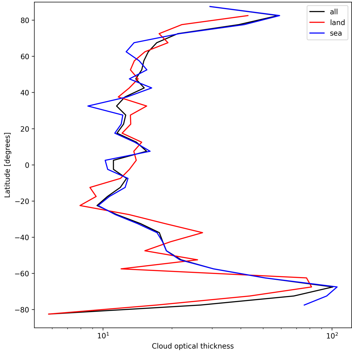
Figure 25: Zonal average of “Cloud optical thickness” for 2025-09-10 to 2025-09-11.
