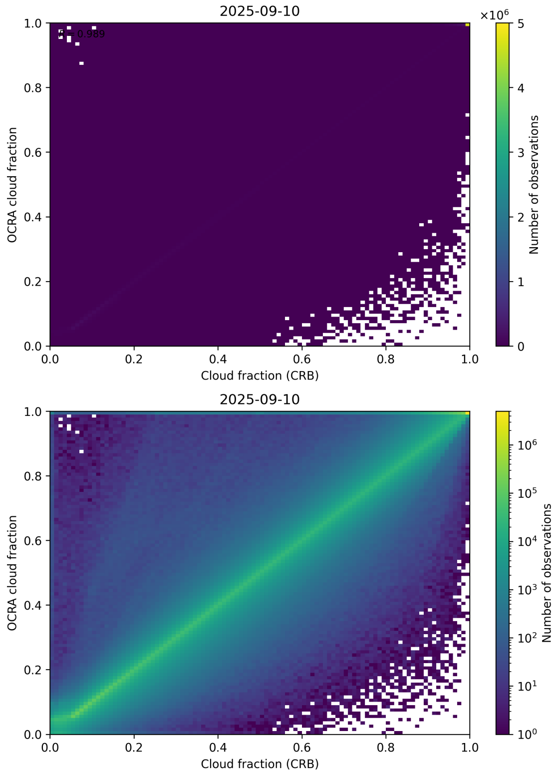
Figure 78: Scatter density plot of “Cloud fraction (CRB)” against “OCRA cloud fraction” for 2025-09-10 to 2025-09-11.
