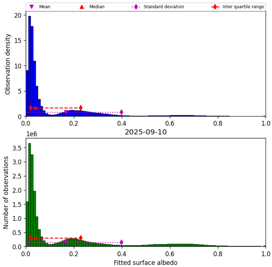
Figure 45: Histogram of “Fitted surface albedo” for 2025-09-10 to 2025-09-11
