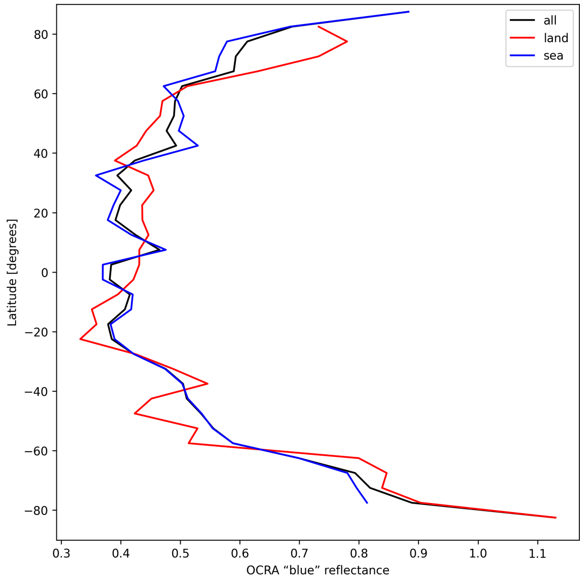
Figure 35: Zonal average of “OCRA “blue” reflectance” for 2025-09-10 to 2025-09-11.
