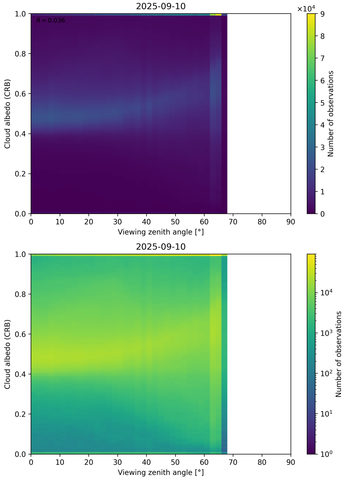
Figure 106: Scatter density plot of “Viewing zenith angle” against “Cloud albedo (CRB)” for 2025-09-10 to 2025-09-11.
