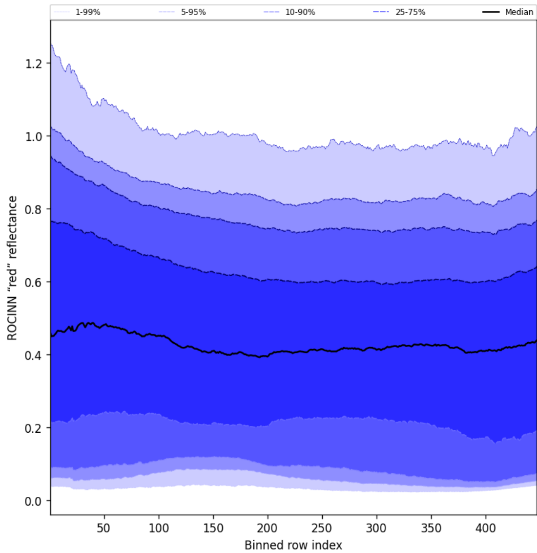
Figure 69: Along track statistics of “ROCINN “red” reflectance” for 2025-09-10 to 2025-09-11
