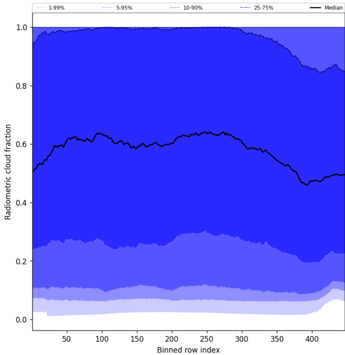
Figure 55: Along track statistics of “Radiometric cloud fraction” for 2025-09-10 to 2025-09-11
