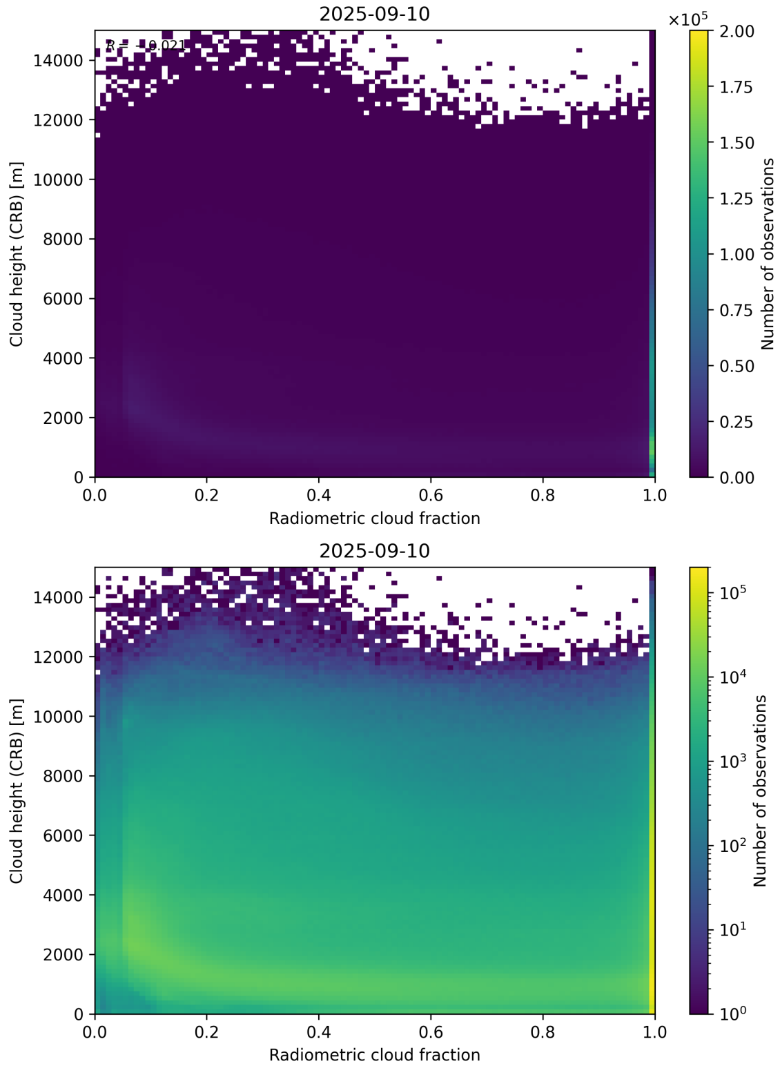
Figure 74: Scatter density plot of “Radiometric cloud fraction” against “Cloud height (CRB)” for 2025-09-10 to 2025-09-11.
