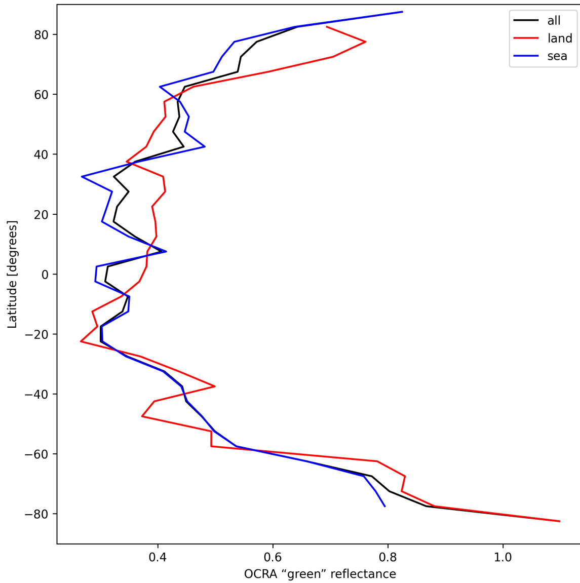
Figure 36: Zonal average of “OCRA “green” reflectance” for 2025-09-10 to 2025-09-11.
