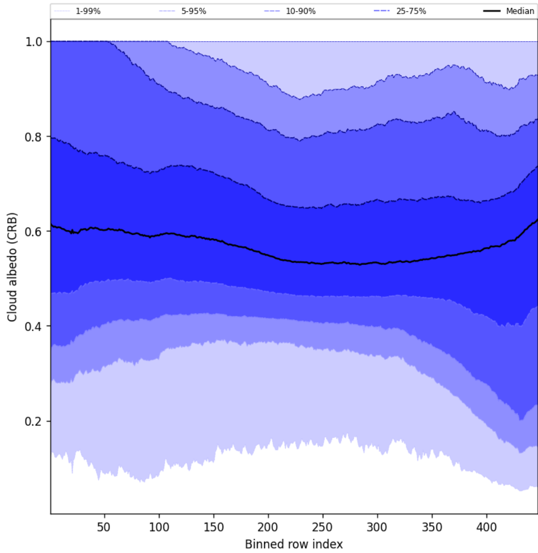
Figure 60: Along track statistics of “Cloud albedo (CRB)” for 2025-09-10 to 2025-09-11
