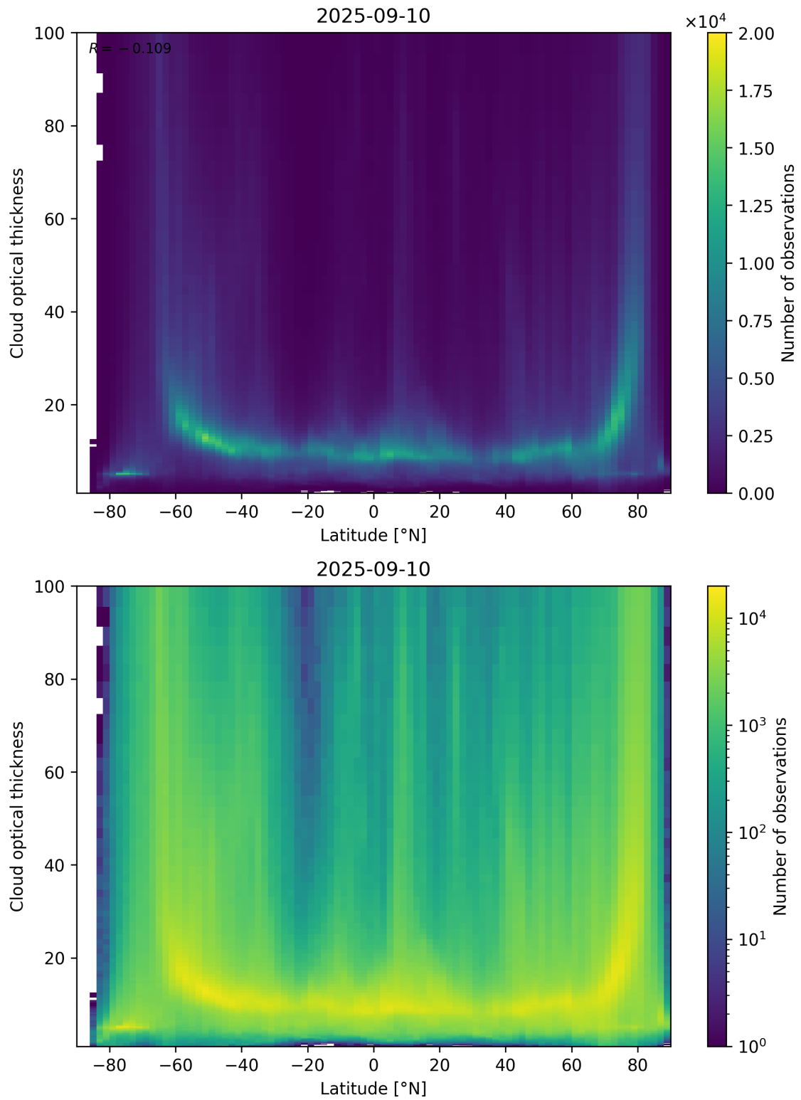
Figure 96: Scatter density plot of “Latitude” against “Cloud optical thickness” for 2025-09-10 to 2025-09-11.
