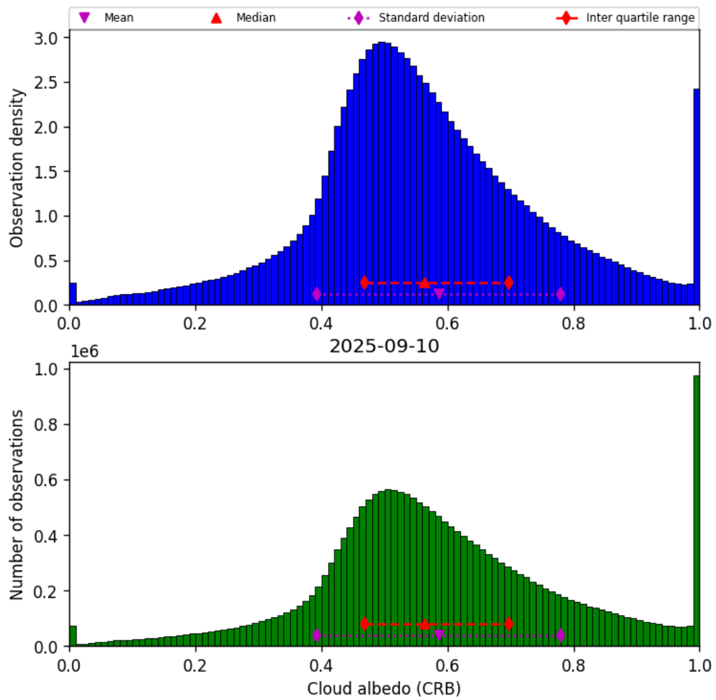
Figure 44: Histogram of “Cloud albedo (CRB)” for 2025-09-10 to 2025-09-11
