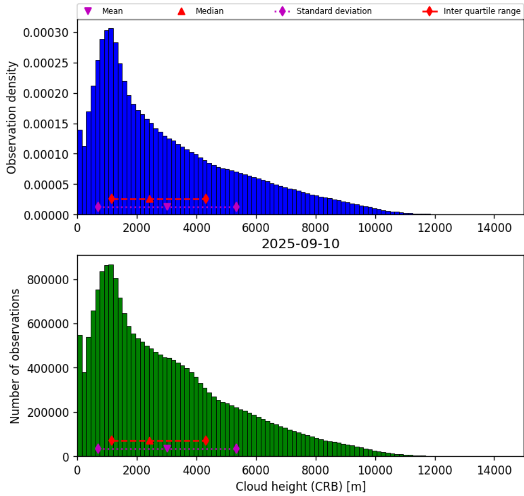
Figure 43: Histogram of “Cloud height (CRB)” for 2025-09-10 to 2025-09-11
