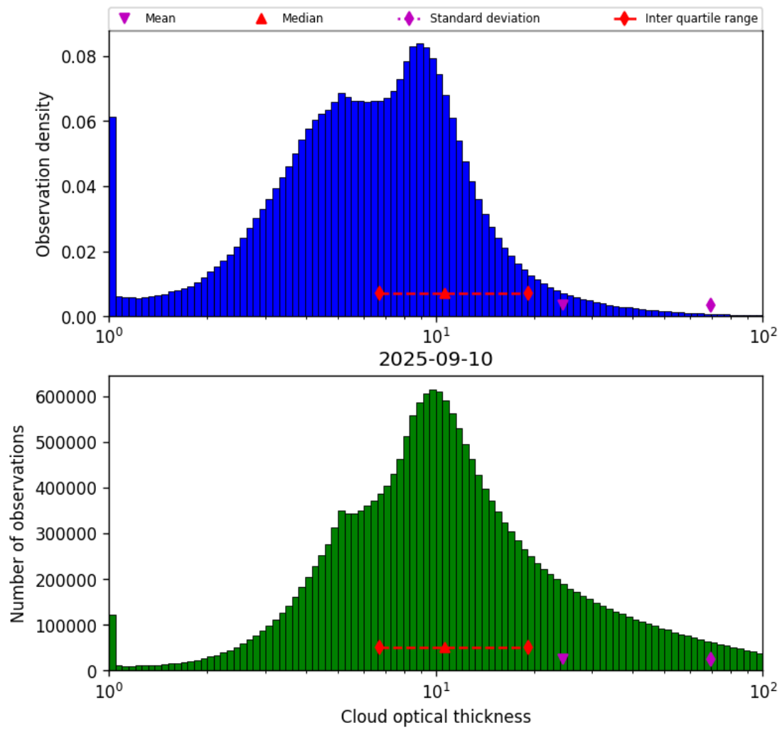
Figure 41: Histogram of “Cloud optical thickness” for 2025-09-10 to 2025-09-11
