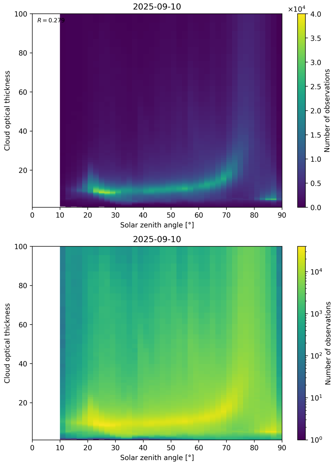
Figure 103: Scatter density plot of “Solar zenith angle” against “Cloud optical thickness” for 2025-09-10 to 2025-09-11.
