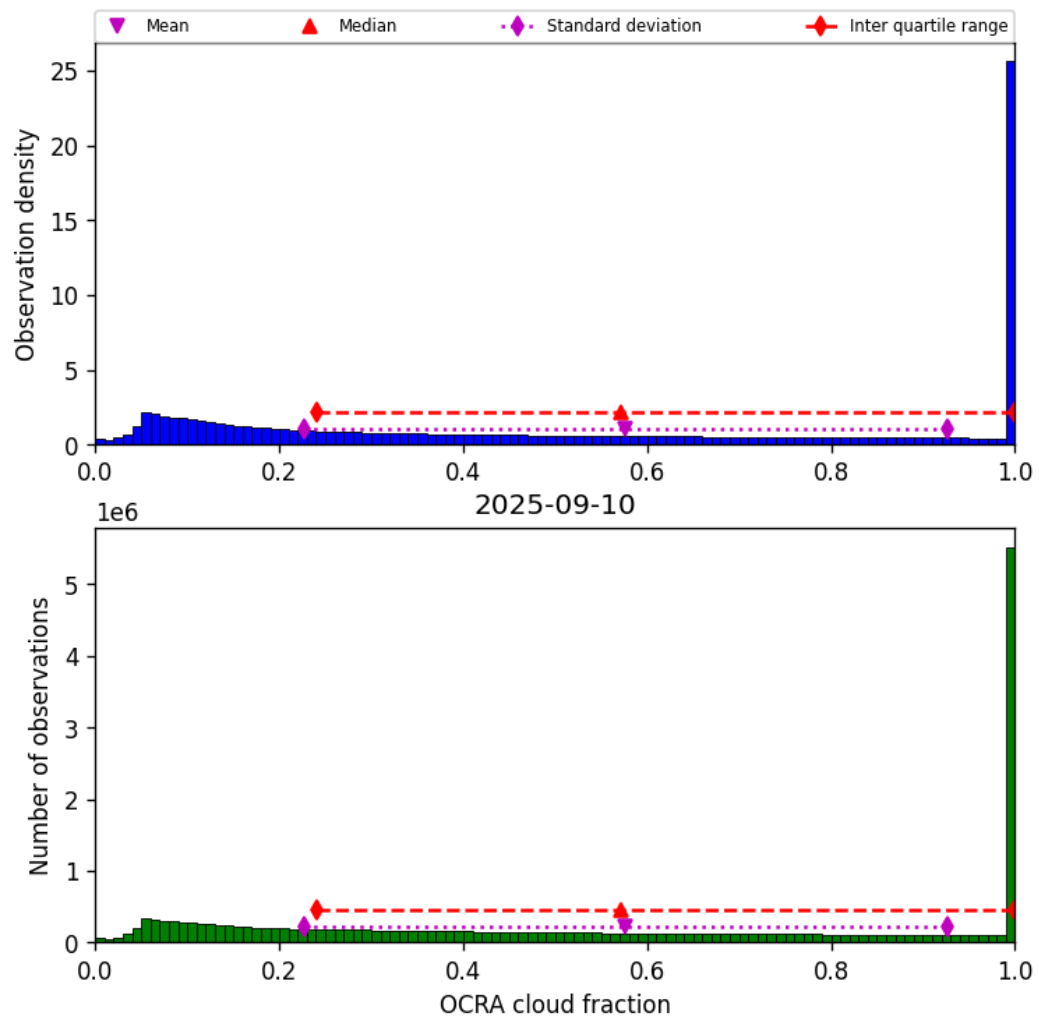
Figure 50: Histogram of “OCRA cloud fraction” for 2025-09-10 to 2025-09-11
