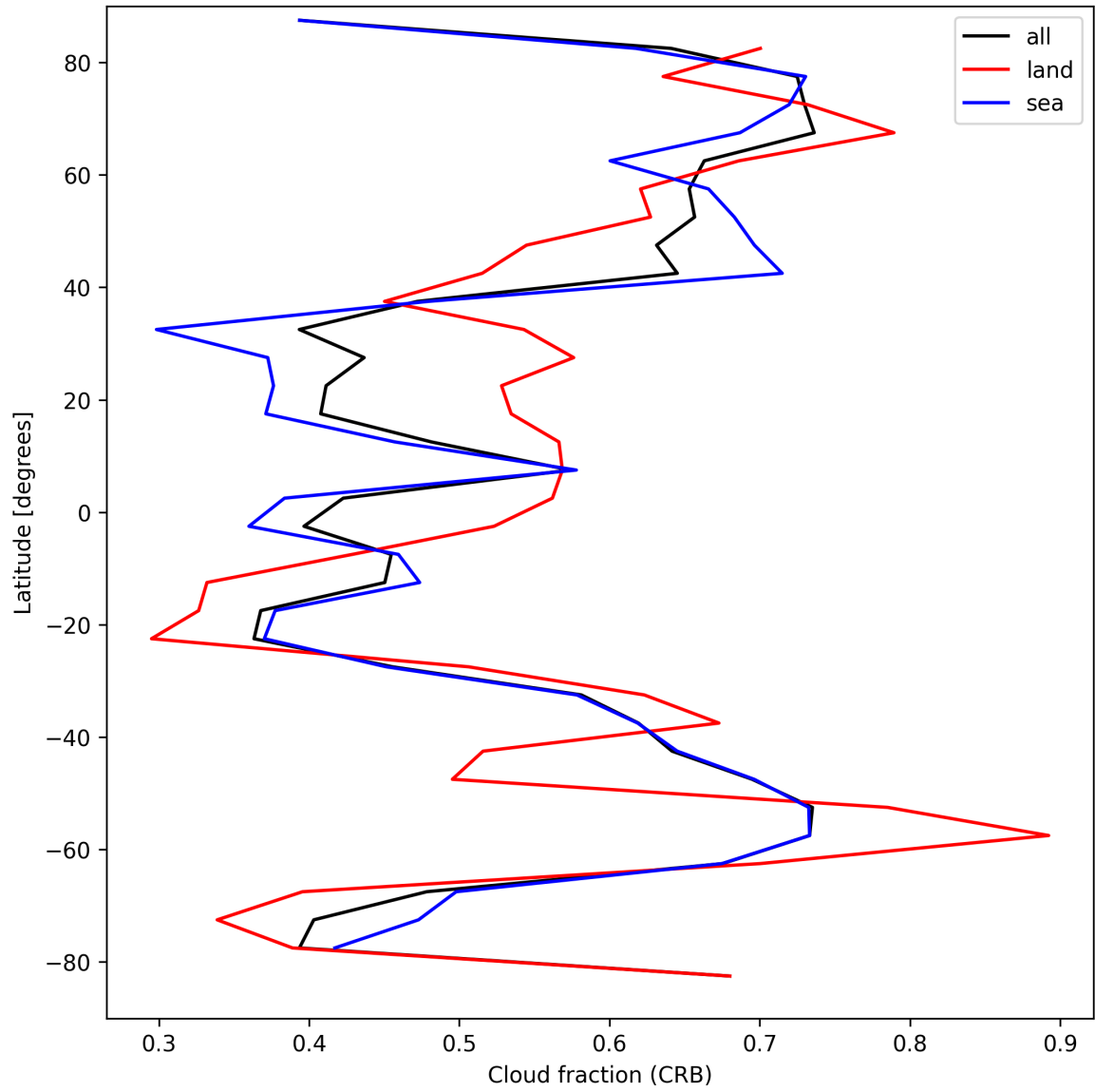
Figure 26: Zonal average of “Cloud fraction (CRB)” for 2025-09-10 to 2025-09-11.
