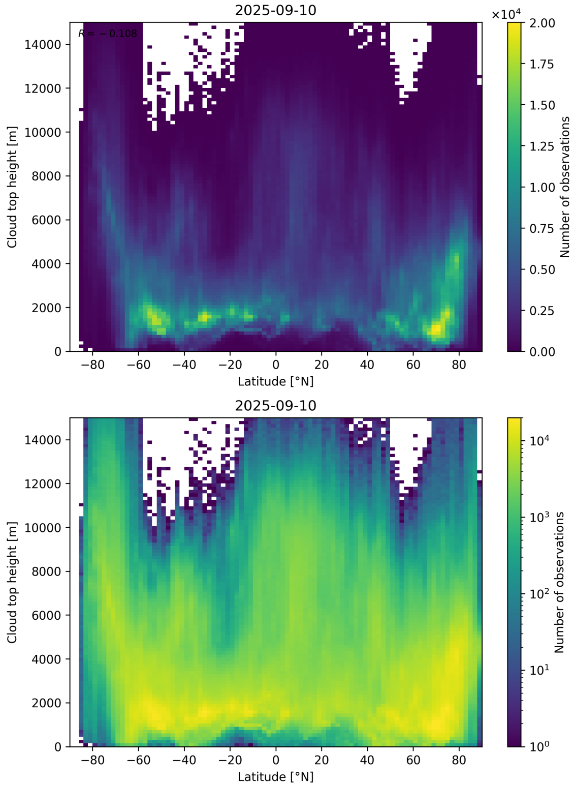
Figure 97: Scatter density plot of “Latitude” against “Cloud top height” for 2025-09-10 to 2025-09-11.
