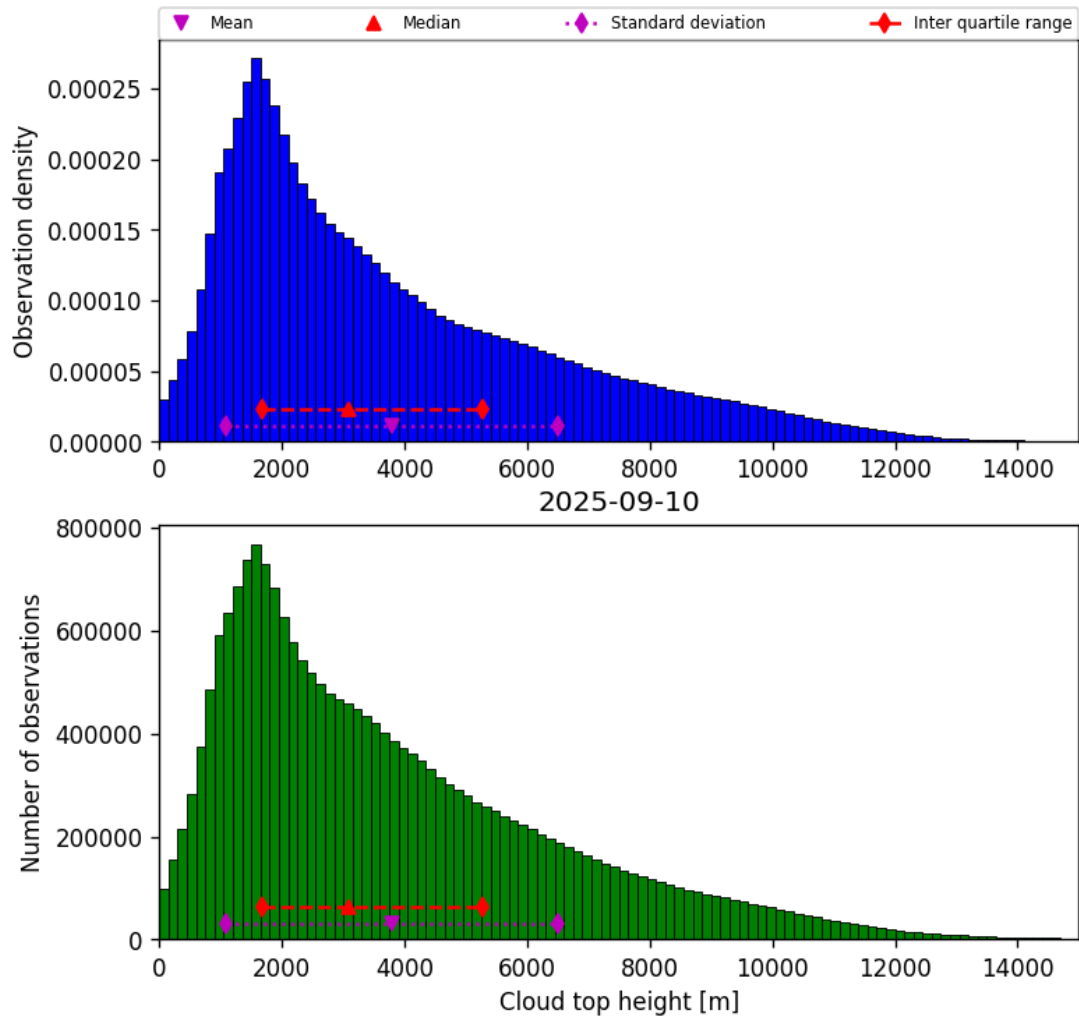
Figure 40: Histogram of “Cloud top height” for 2025-09-10 to 2025-09-11
