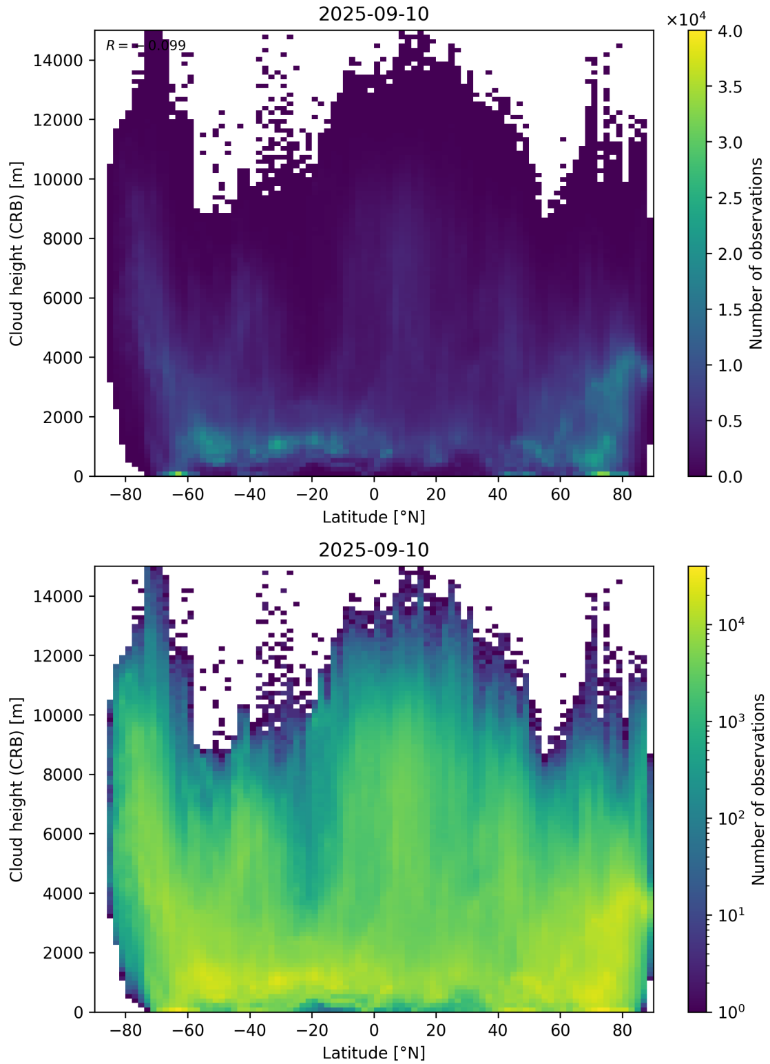
Figure 95: Scatter density plot of “Latitude” against “Cloud height (CRB)” for 2025-09-10 to 2025-09-11.
