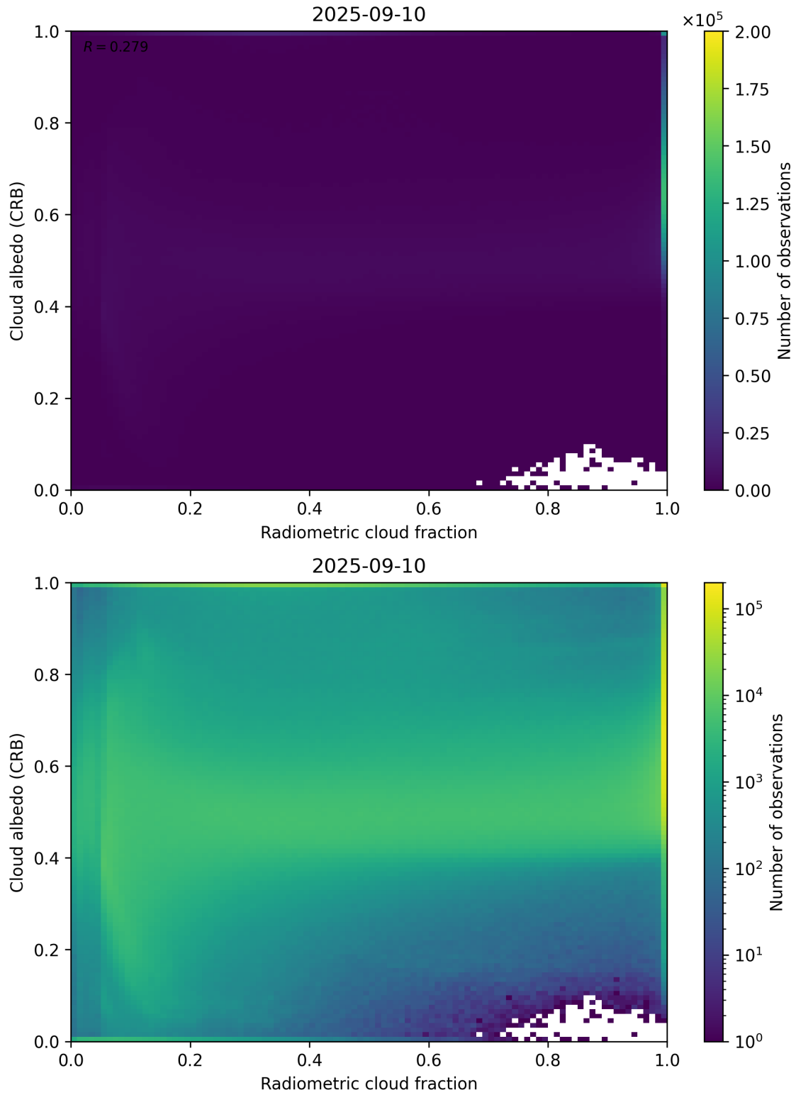
Figure 71: Scatter density plot of “Radiometric cloud fraction” against “Cloud albedo (CRB)” for 2025-09-10 to 2025-09-11.
