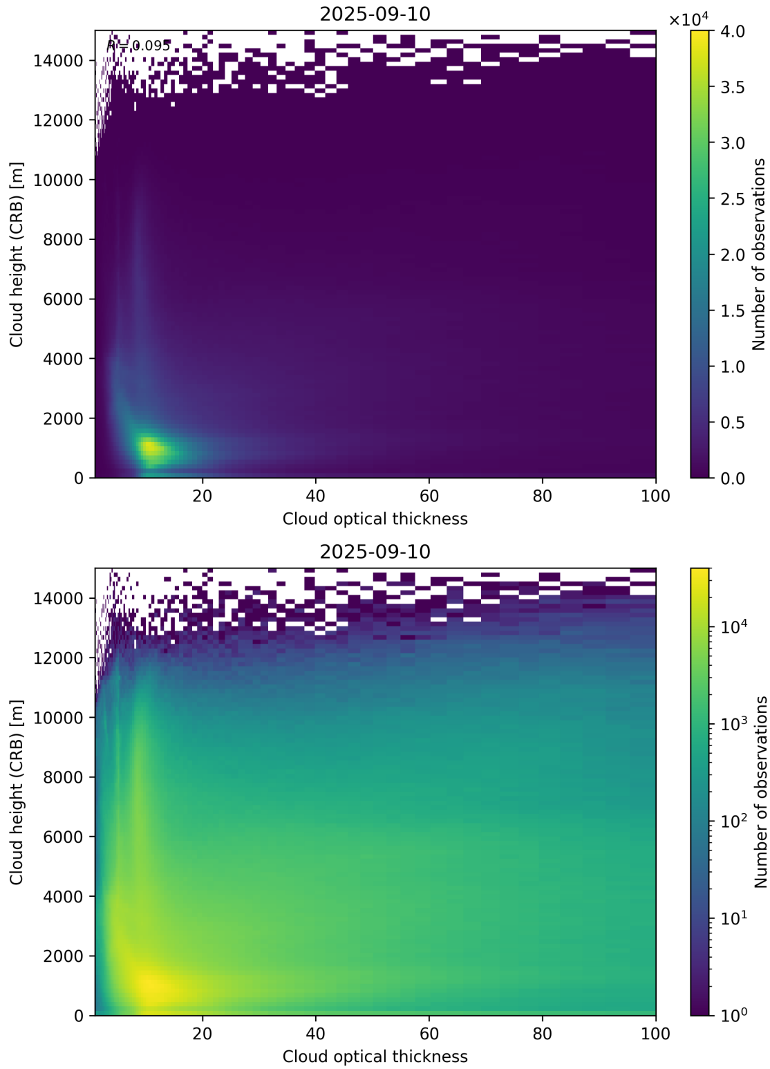
Figure 85: Scatter density plot of “Cloud optical thickness” against “Cloud height (CRB)” for 2025-09-10 to 2025-09-11.
