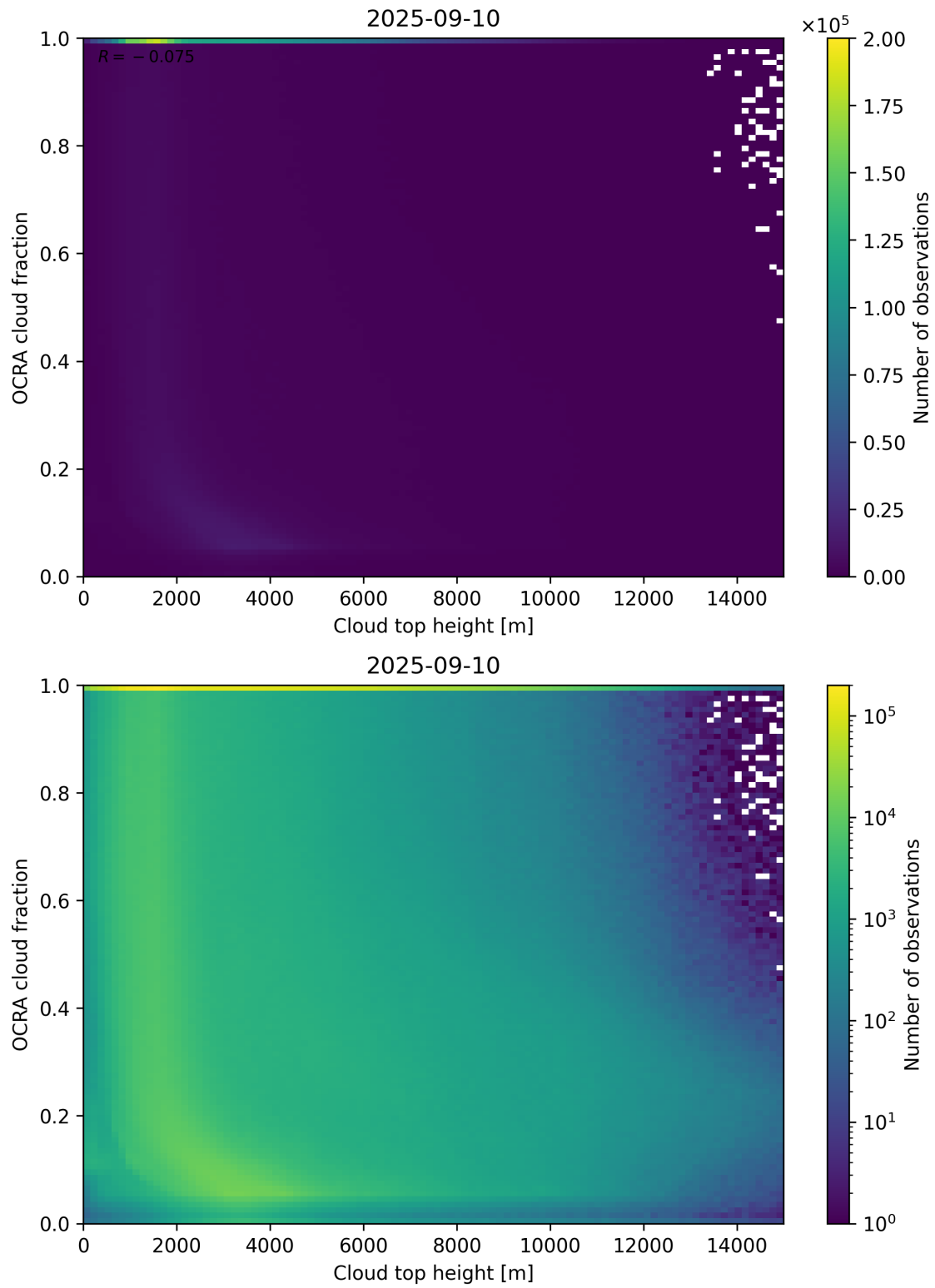
Figure 87: Scatter density plot of “Cloud top height” against “OCRA cloud fraction” for 2025-09-10 to 2025-09-11.
