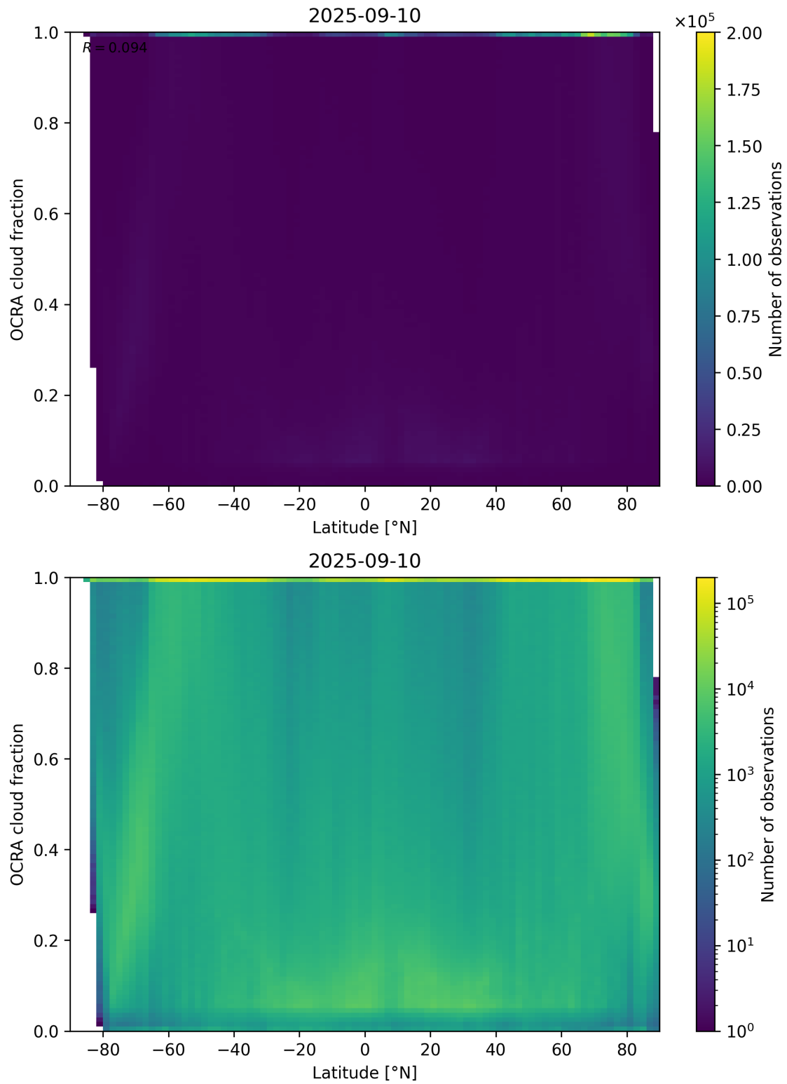
Figure 93: Scatter density plot of “Latitude” against “OCRA cloud fraction” for 2025-09-10 to 2025-09-11.
