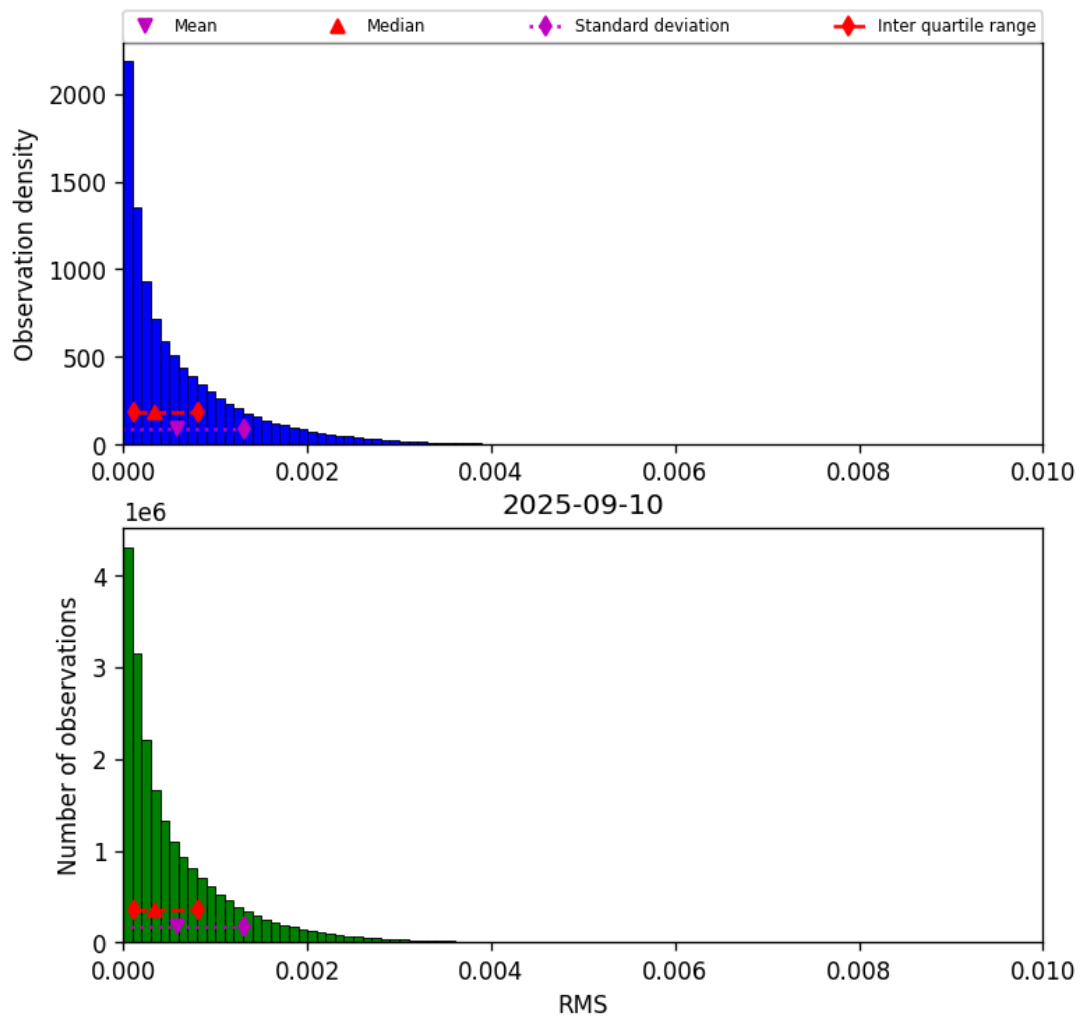
Figure 47: Histogram of “RMS” for 2025-09-10 to 2025-09-11
