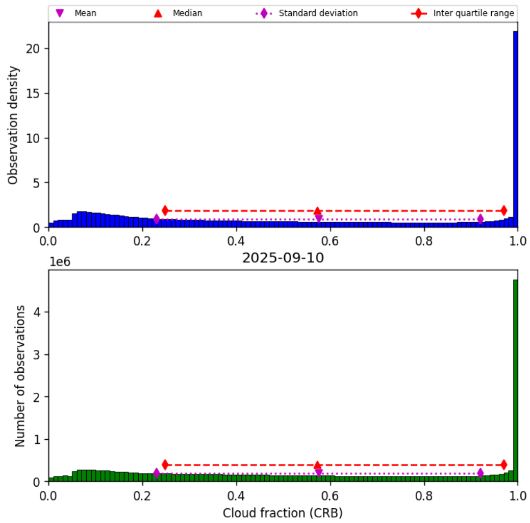
Figure 42: Histogram of “Cloud fraction (CRB)” for 2025-09-10 to 2025-09-11
