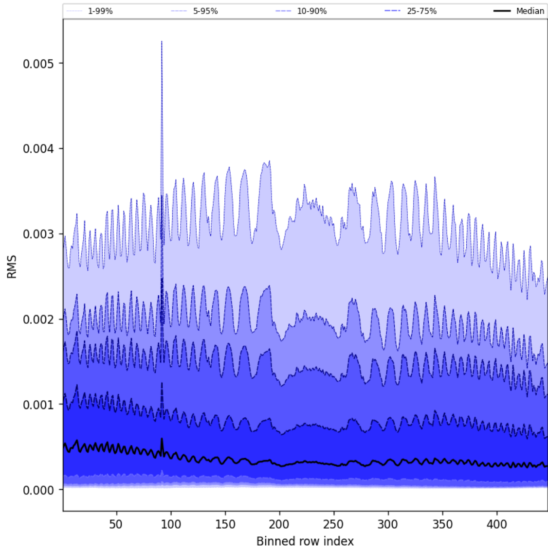
Figure 63: Along track statistics of “RMS” for 2025-09-10 to 2025-09-11
