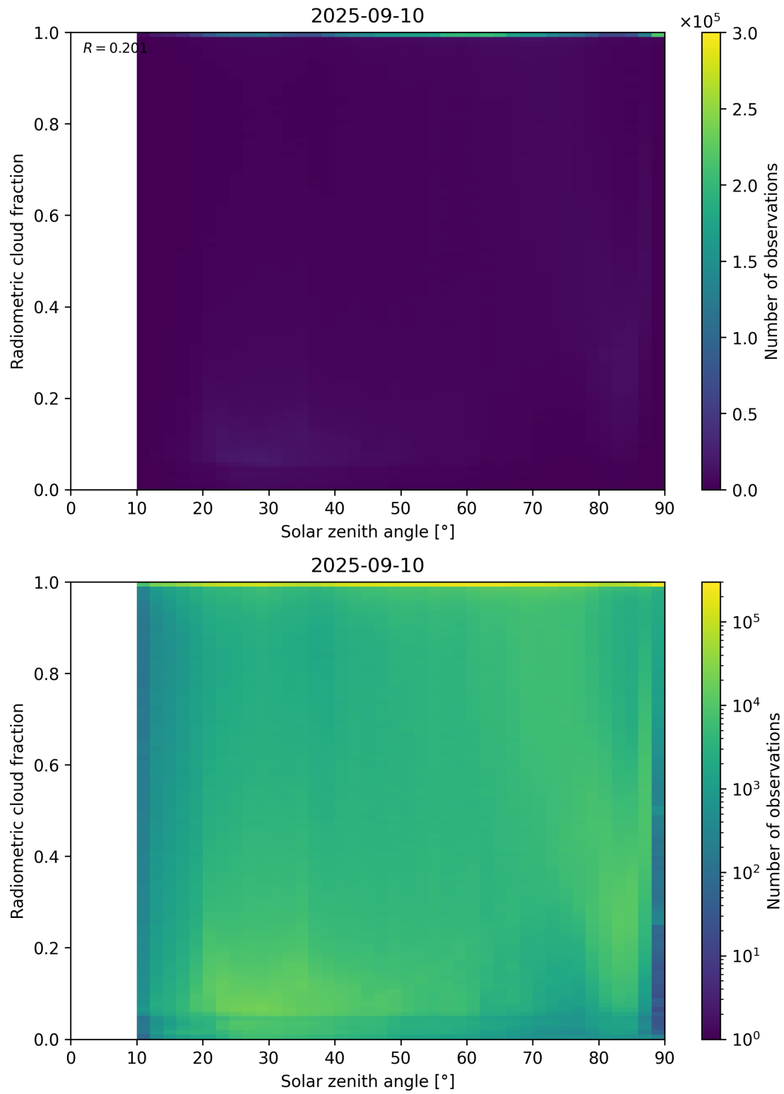
Figure 99: Scatter density plot of “Solar zenith angle” against “Radiometric cloud fraction” for 2025-09-10 to 2025-09-11.
