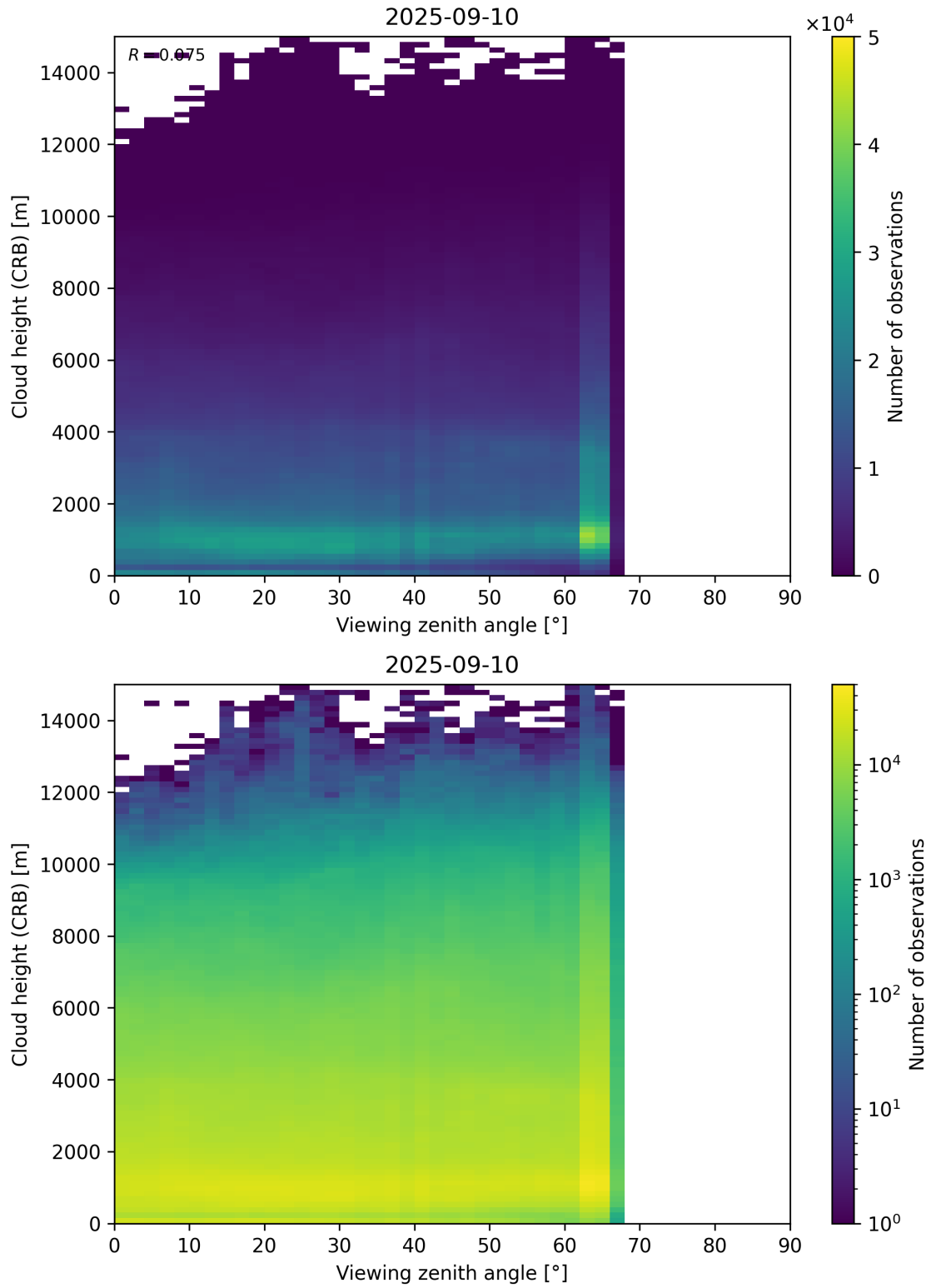
Figure 110: Scatter density plot of “Viewing zenith angle” against “Cloud height (CRB)” for 2025-09-10 to 2025-09-11.
