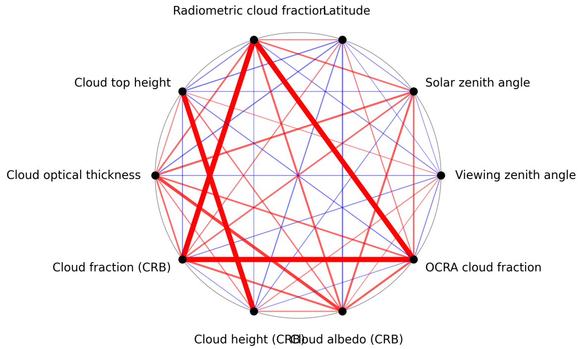
Figure 1: Map of correlation graph for 2025-09-10 to 2025-09-11.
