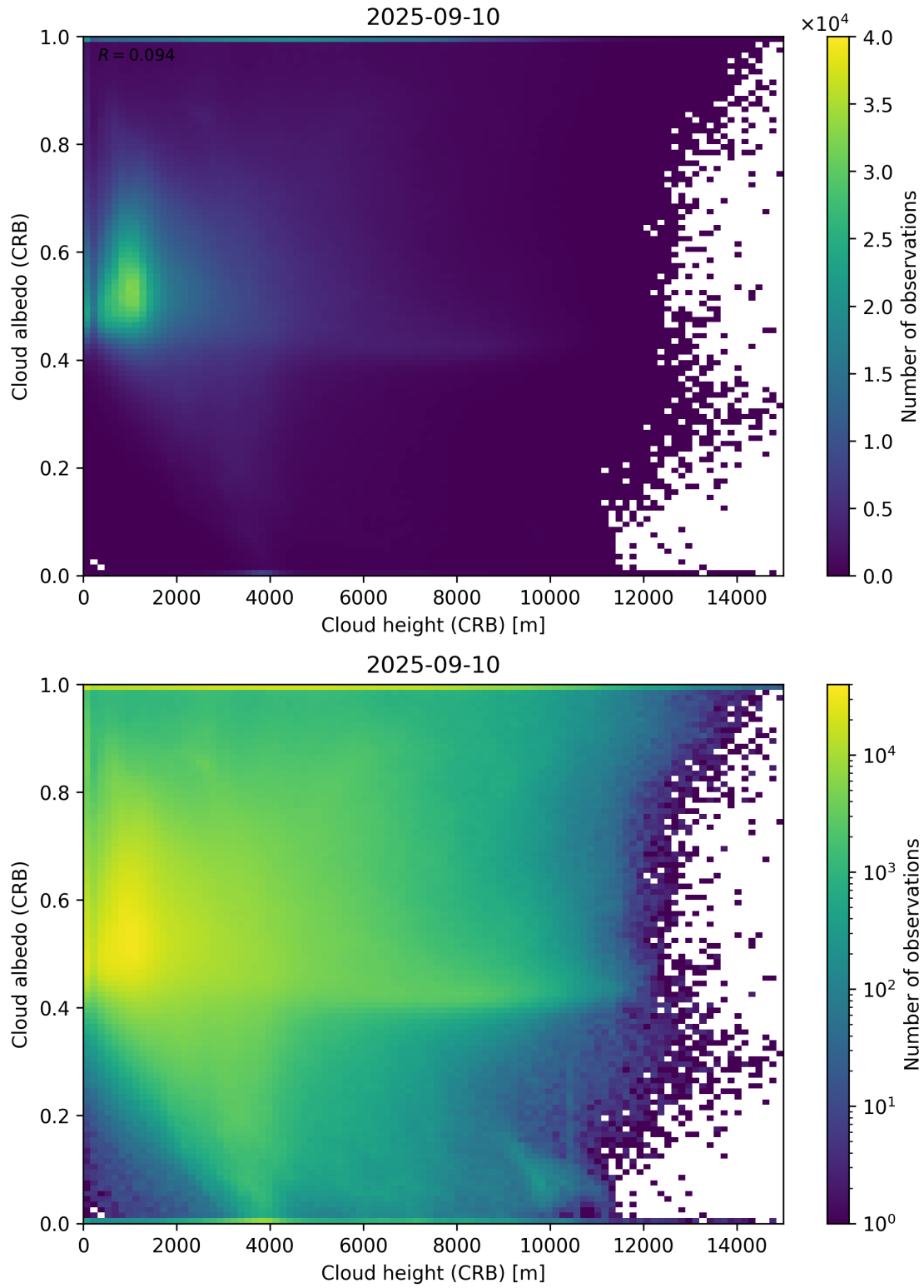
Figure 80: Scatter density plot of “Cloud height (CRB)” against “Cloud albedo (CRB)” for 2025-09-10 to 2025-09-11.
