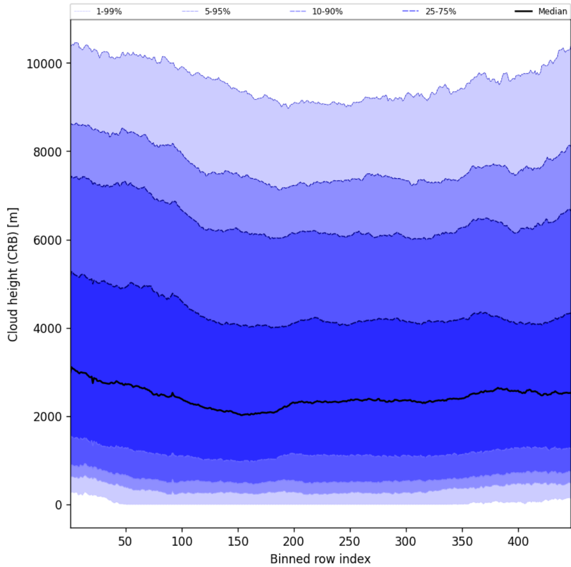
Figure 59: Along track statistics of “Cloud height (CRB)” for 2025-09-10 to 2025-09-11
