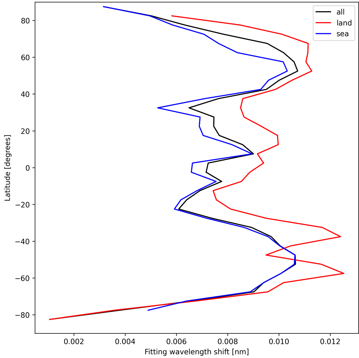
Figure 33: Zonal average of “Fitting wavelength shift” for 2025-09-10 to 2025-09-11.
