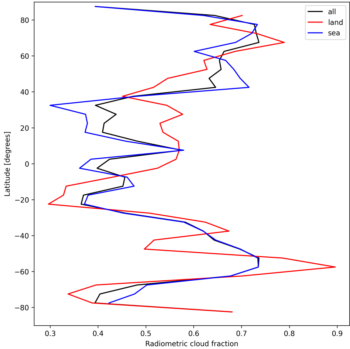
Figure 23: Zonal average of “Radiometric cloud fraction” for 2025-09-10 to 2025-09-11.
