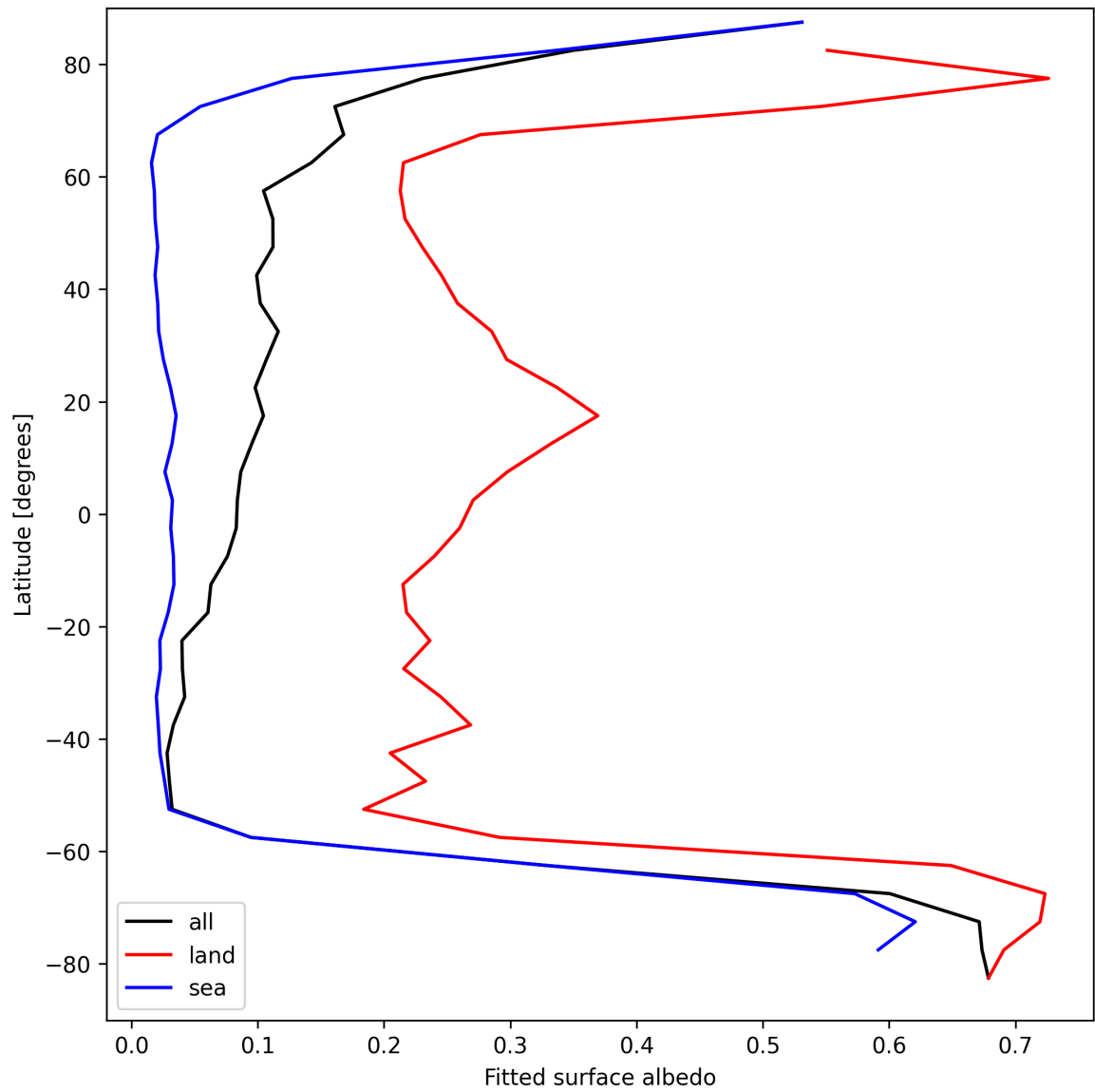
Figure 29: Zonal average of “Fitted surface albedo” for 2025-09-10 to 2025-09-11.
