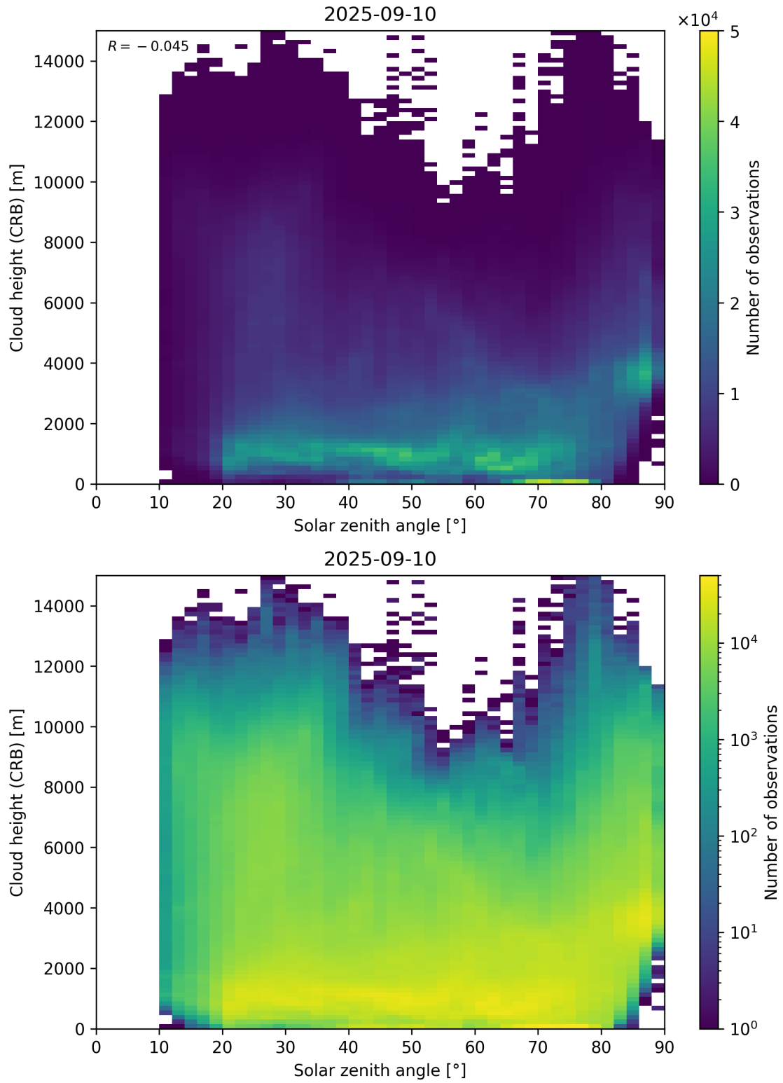
Figure 102: Scatter density plot of “Solar zenith angle” against “Cloud height (CRB)” for 2025-09-10 to 2025-09-11.
