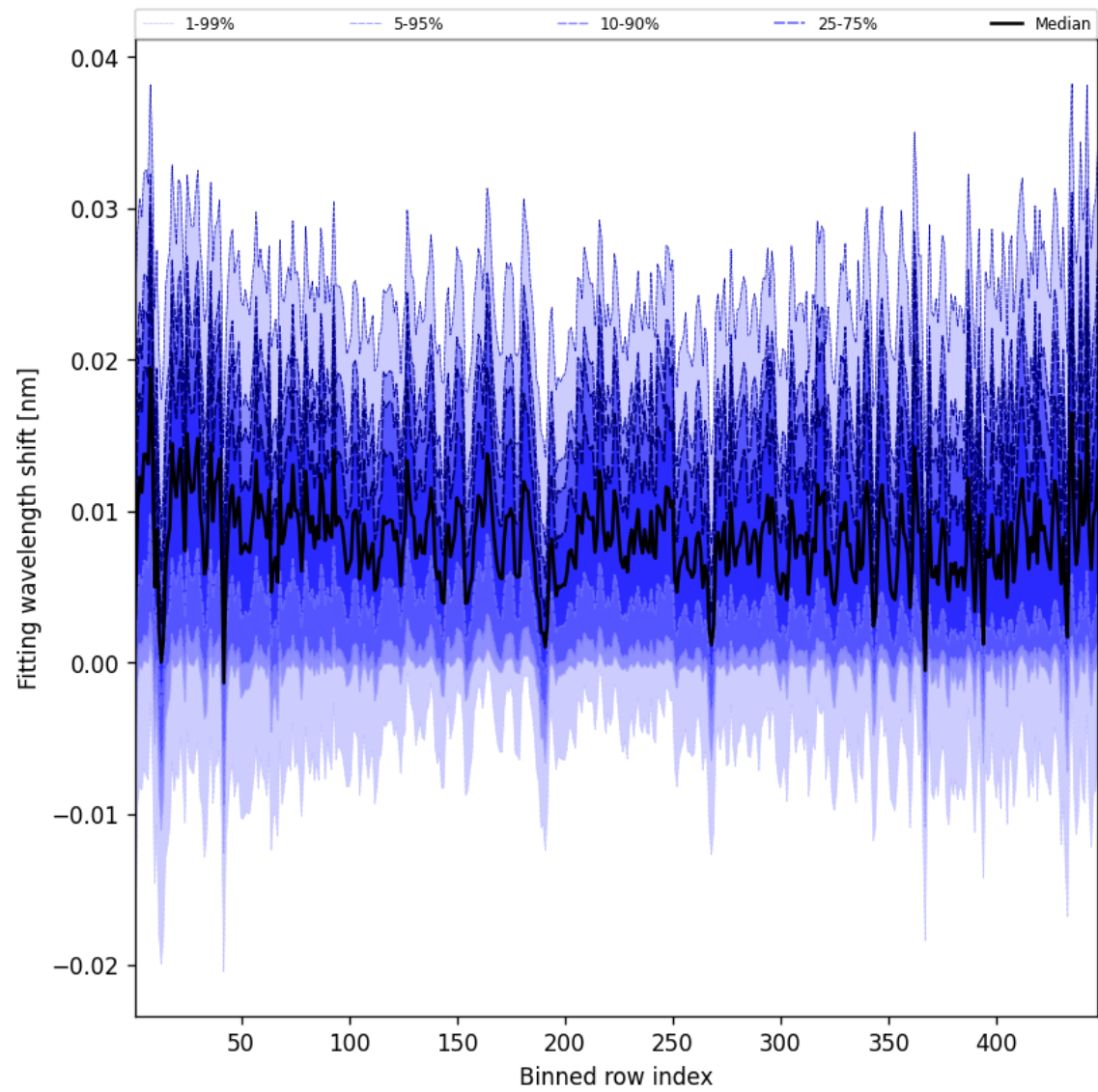
Figure 65: Along track statistics of “Fitting wavelength shift” for 2025-09-10 to 2025-09-11
