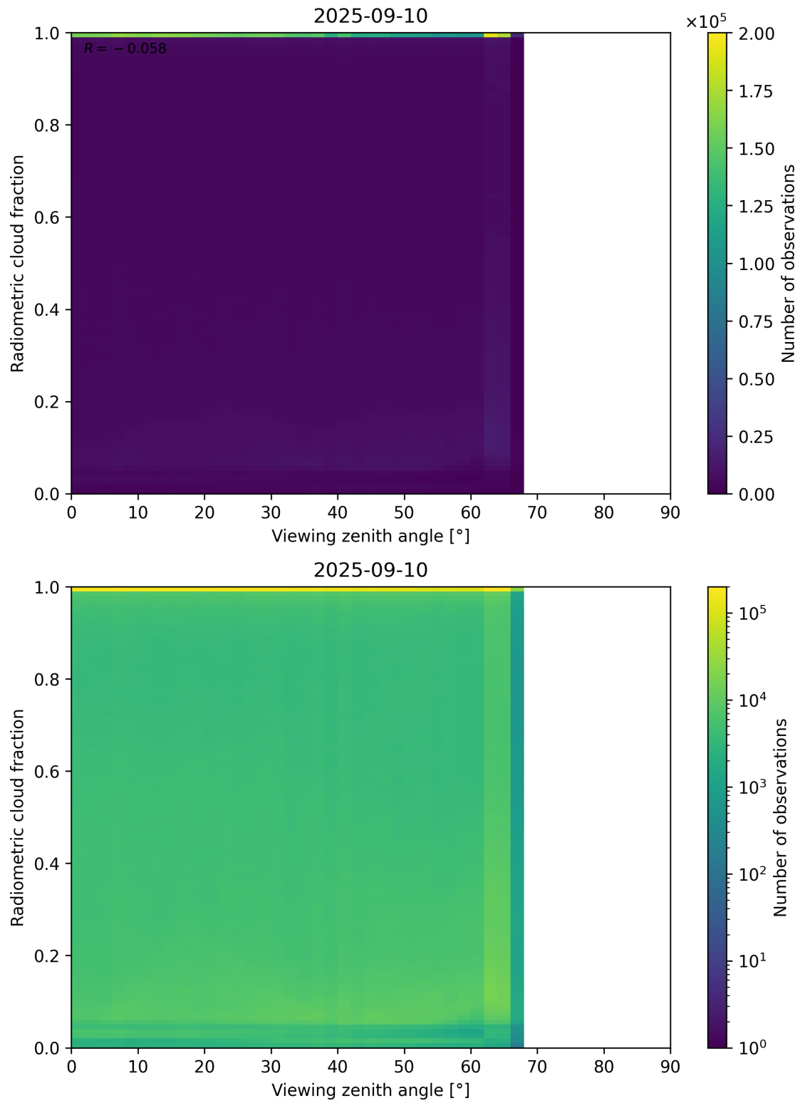
Figure 107: Scatter density plot of “Viewing zenith angle” against “Radiometric cloud fraction” for 2025-09-10 to 2025-09-11.
