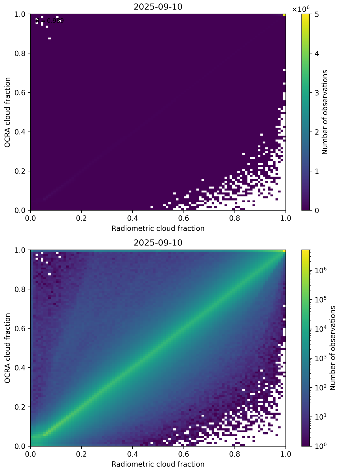
Figure 72: Scatter density plot of “Radiometric cloud fraction” against “OCRA cloud fraction” for 2025-09-10 to 2025-09-11.
