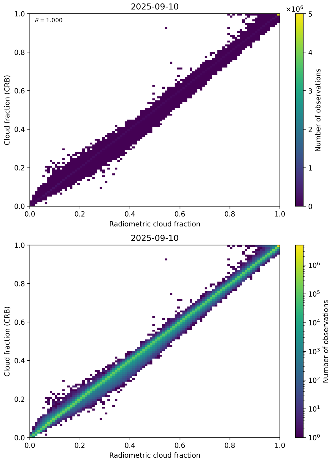
Figure 73: Scatter density plot of “Radiometric cloud fraction” against “Cloud fraction (CRB)” for 2025-09-10 to 2025-09-11.
