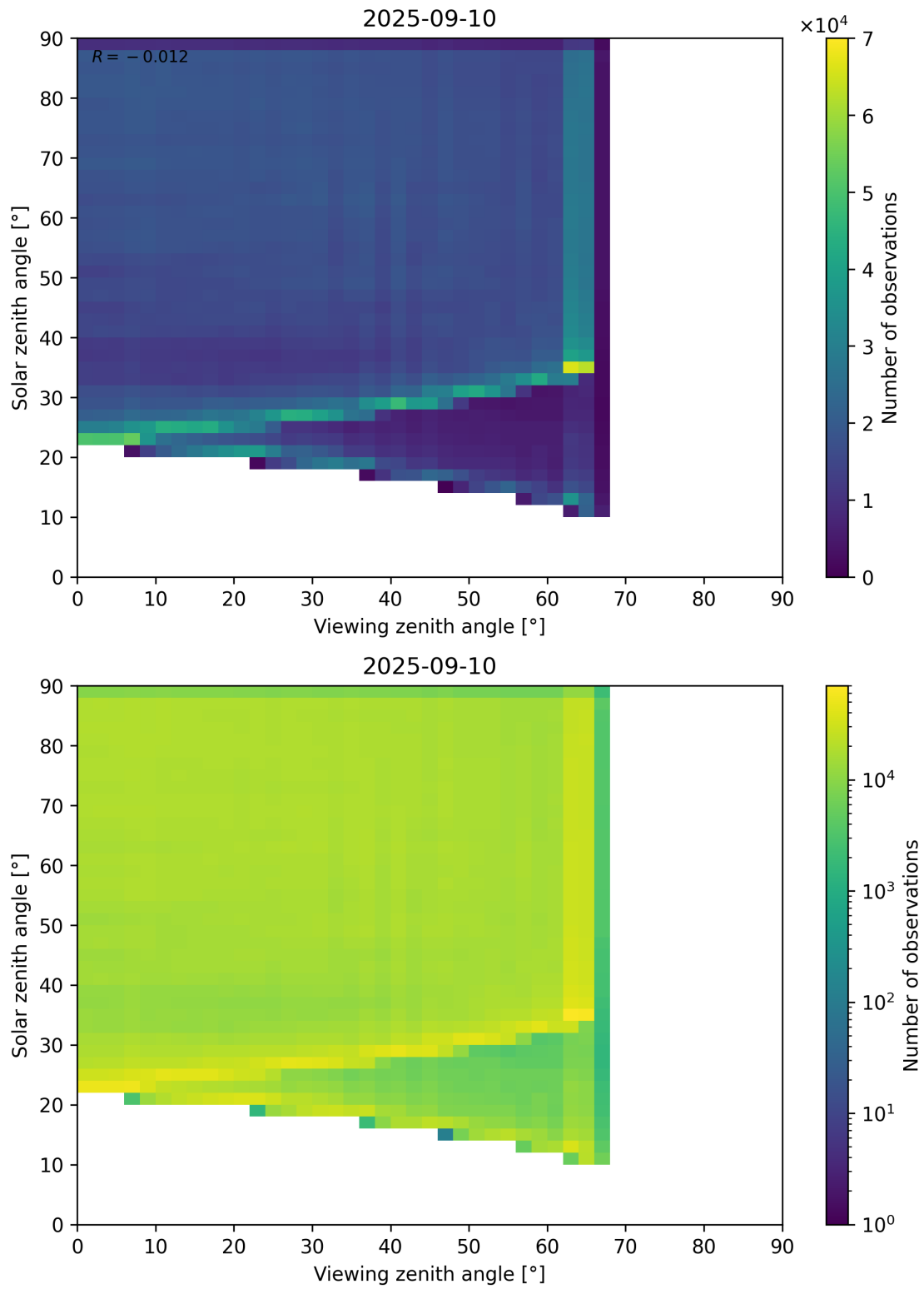
Figure 114: Scatter density plot of “Viewing zenith angle” against “Solar zenith angle” for 2025-09-10 to 2025-09-11.
