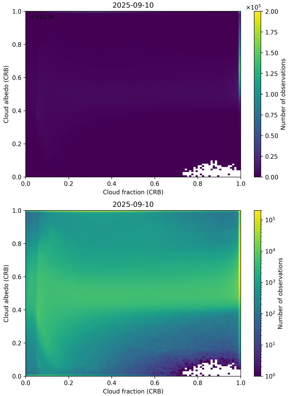
Figure 77: Scatter density plot of “Cloud fraction (CRB)” against “Cloud albedo (CRB)” for 2025-09-10 to 2025-09-11.
