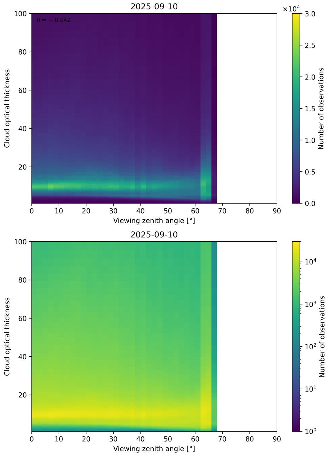
Figure 111: Scatter density plot of “Viewing zenith angle” against “Cloud optical thickness” for 2025-09-10 to 2025-09-11.
