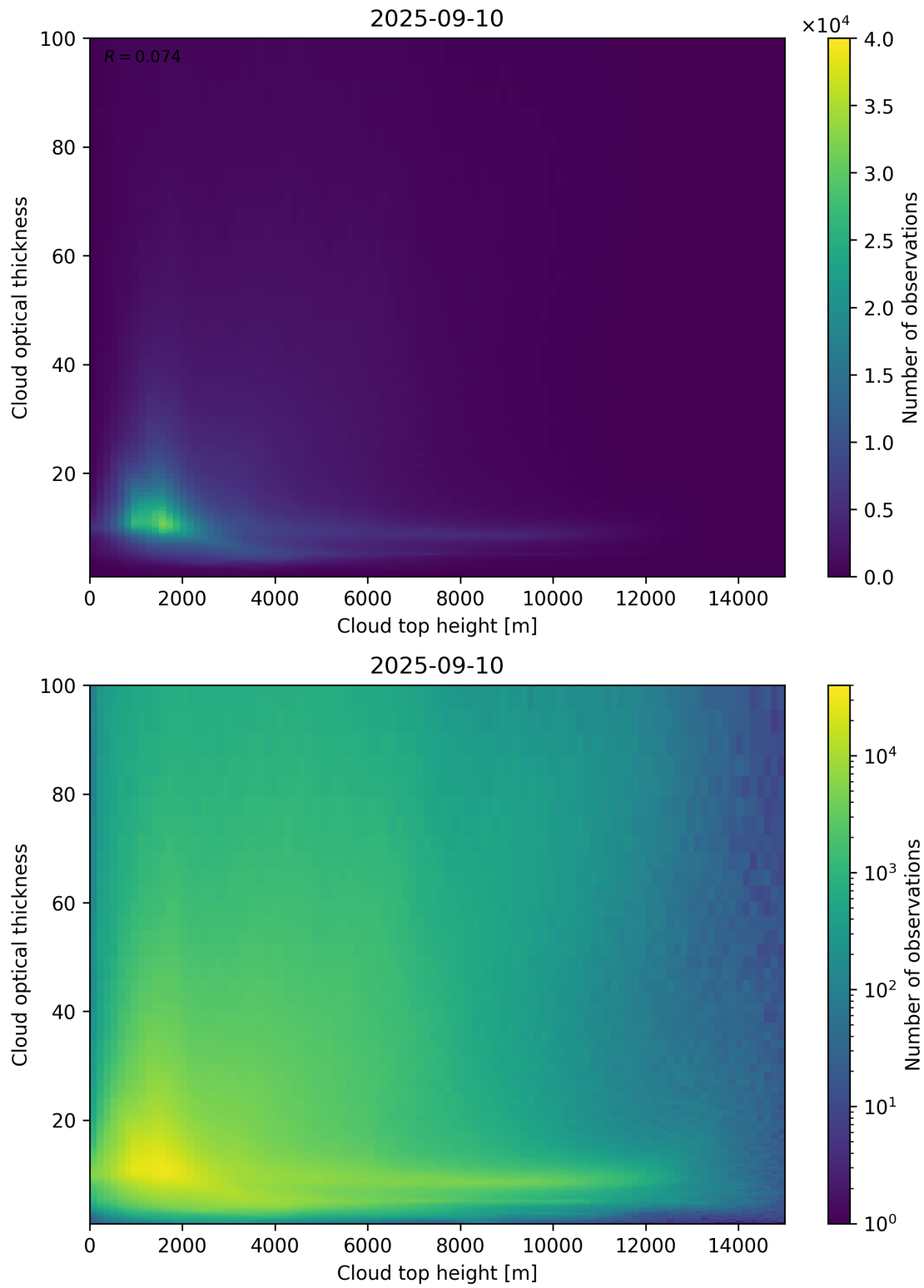
Figure 90: Scatter density plot of “Cloud top height” against “Cloud optical thickness” for 2025-09-10 to 2025-09-11.
