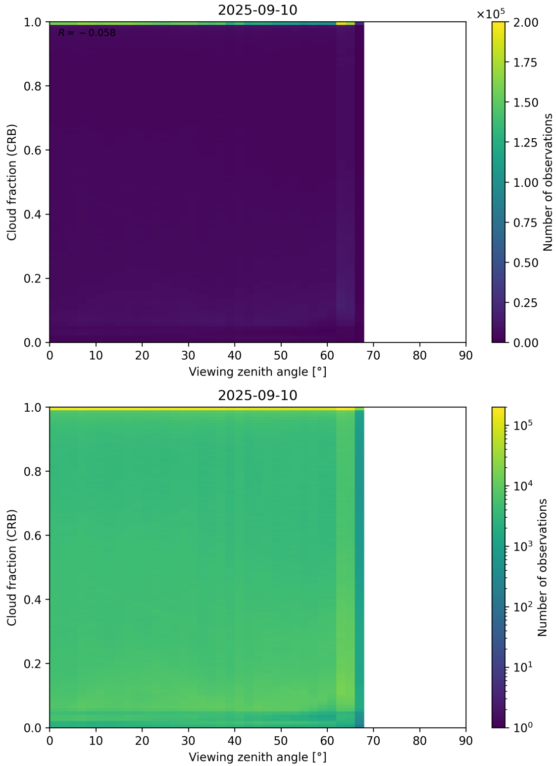
Figure 109: Scatter density plot of “Viewing zenith angle” against “Cloud fraction (CRB)” for 2025-09-10 to 2025-09-11.
