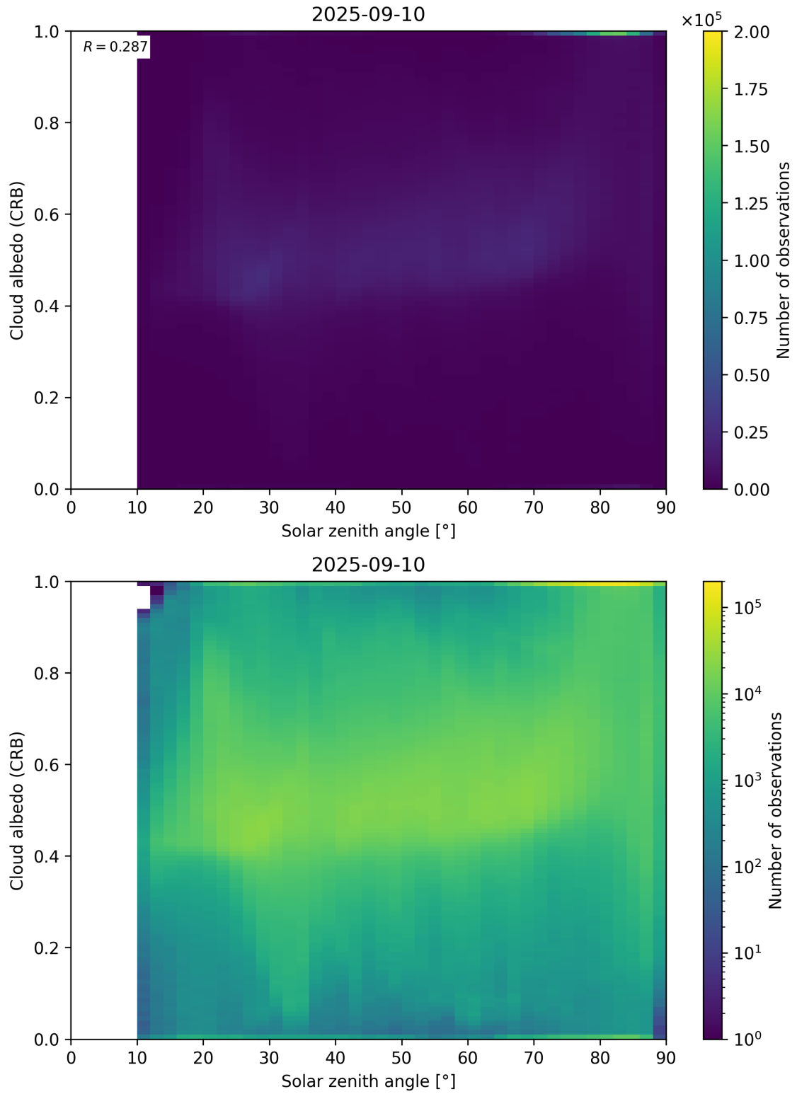
Figure 98: Scatter density plot of “Solar zenith angle” against “Cloud albedo (CRB)” for 2025-09-10 to 2025-09-11.
