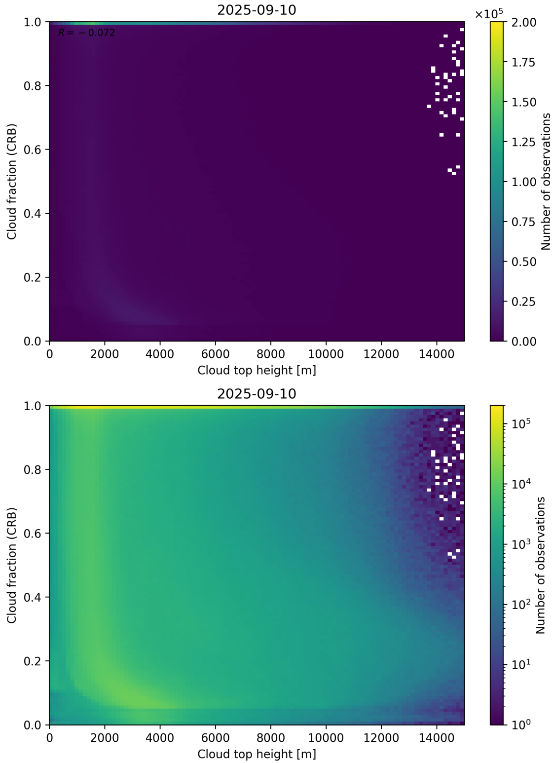
Figure 88: Scatter density plot of “Cloud top height” against “Cloud fraction (CRB)” for 2025-09-10 to 2025-09-11.
