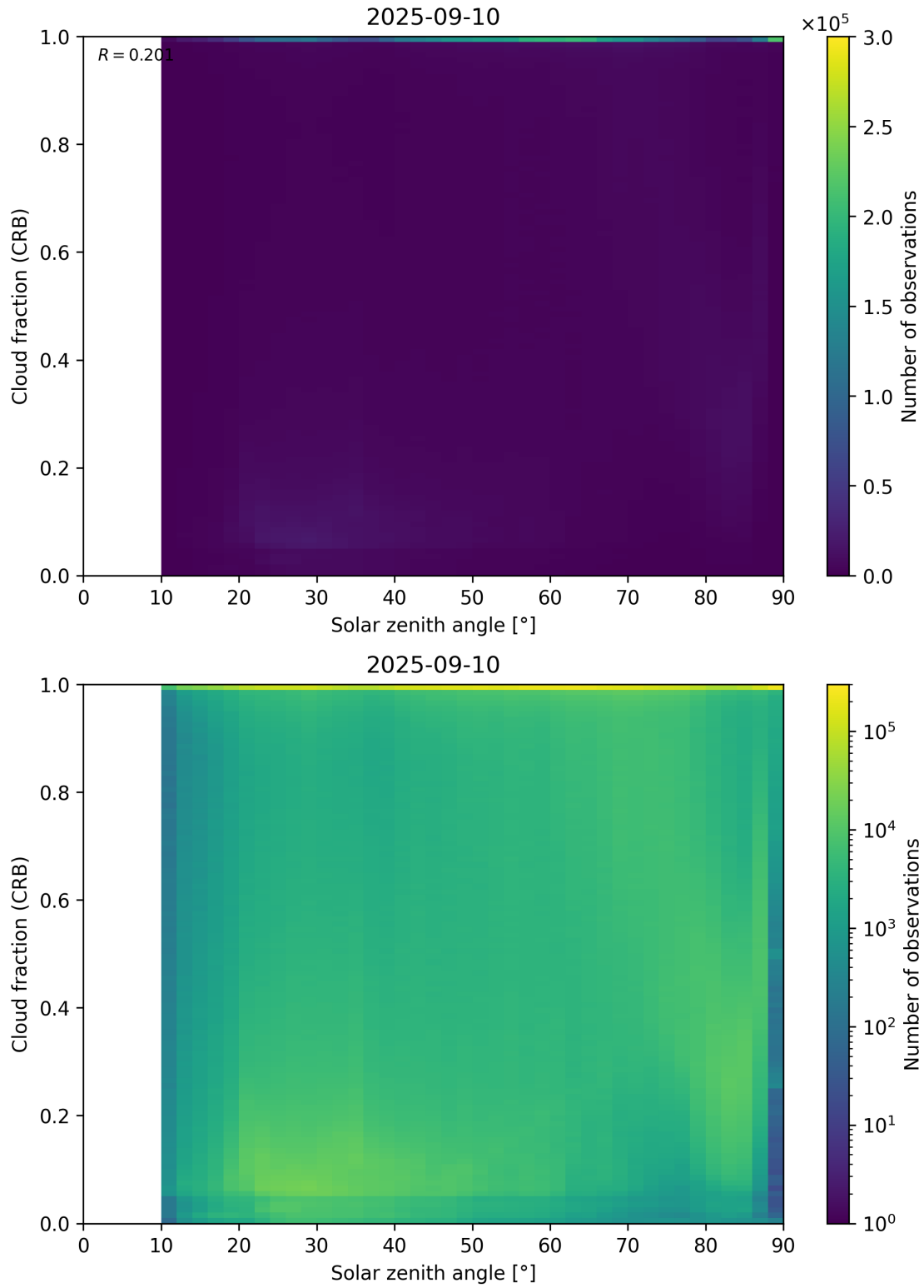
Figure 101: Scatter density plot of “Solar zenith angle” against “Cloud fraction (CRB)” for 2025-09-10 to 2025-09-11.
