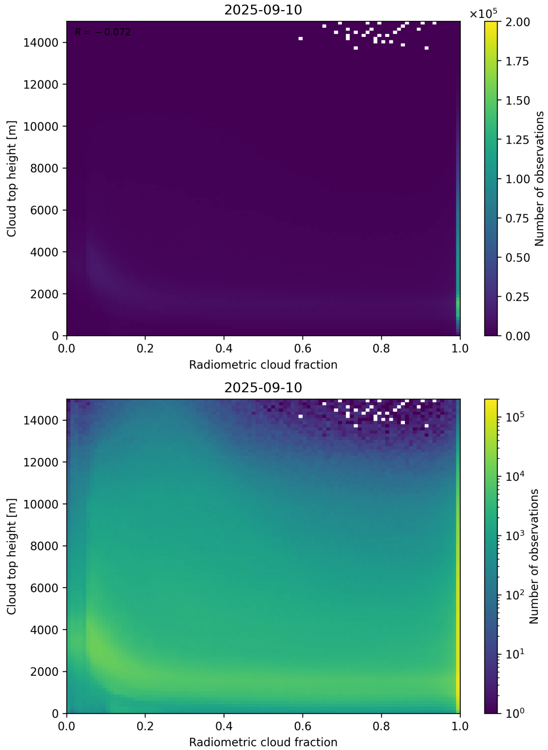
Figure 76: Scatter density plot of “Radiometric cloud fraction” against “Cloud top height” for 2025-09-10 to 2025-09-11.
