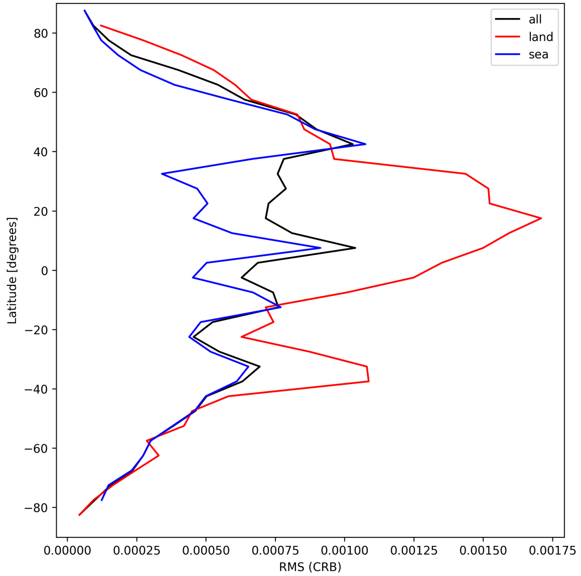
Figure 32: Zonal average of “RMS (CRB)” for 2025-09-10 to 2025-09-11.
