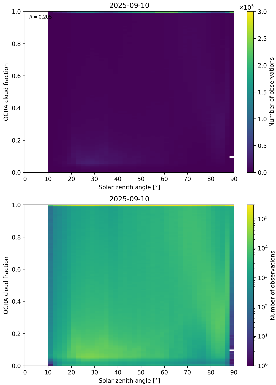
Figure 100: Scatter density plot of “Solar zenith angle” against “OCRA cloud fraction” for 2025-09-10 to 2025-09-11.
