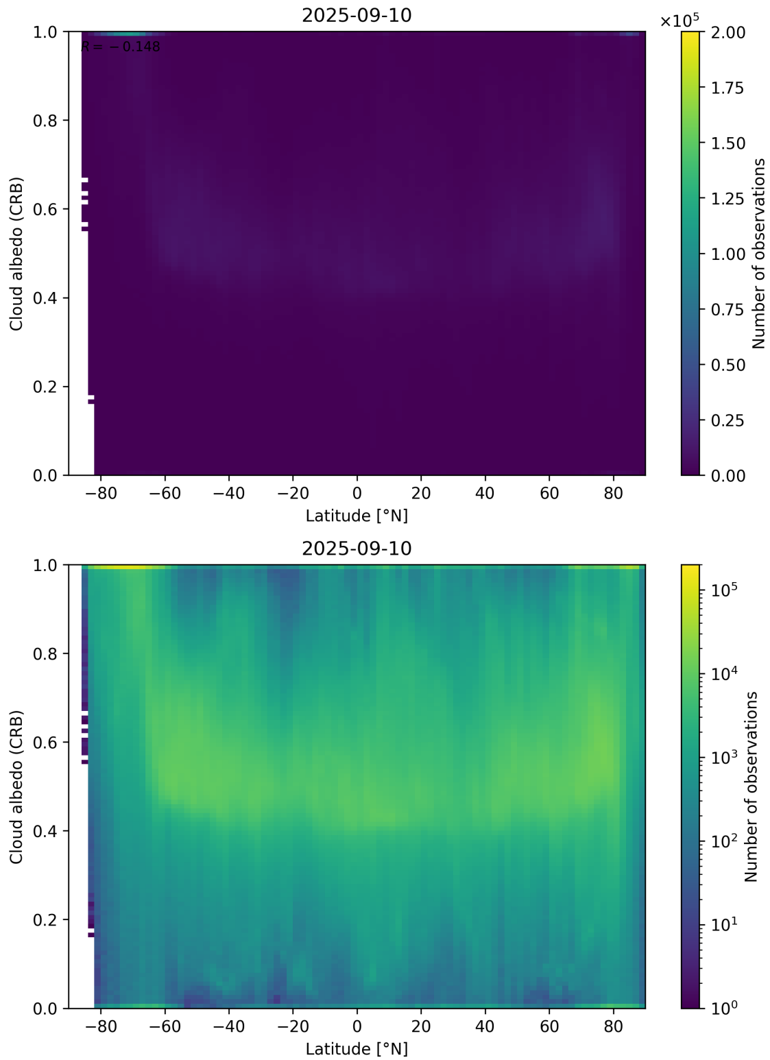
Figure 91: Scatter density plot of “Latitude” against “Cloud albedo (CRB)” for 2025-09-10 to 2025-09-11.
