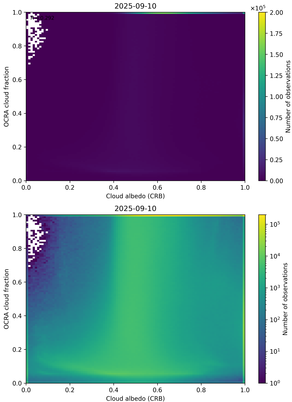
Figure 70: Scatter density plot of “Cloud albedo (CRB)” against “OCRA cloud fraction” for 2025-09-10 to 2025-09-11.
