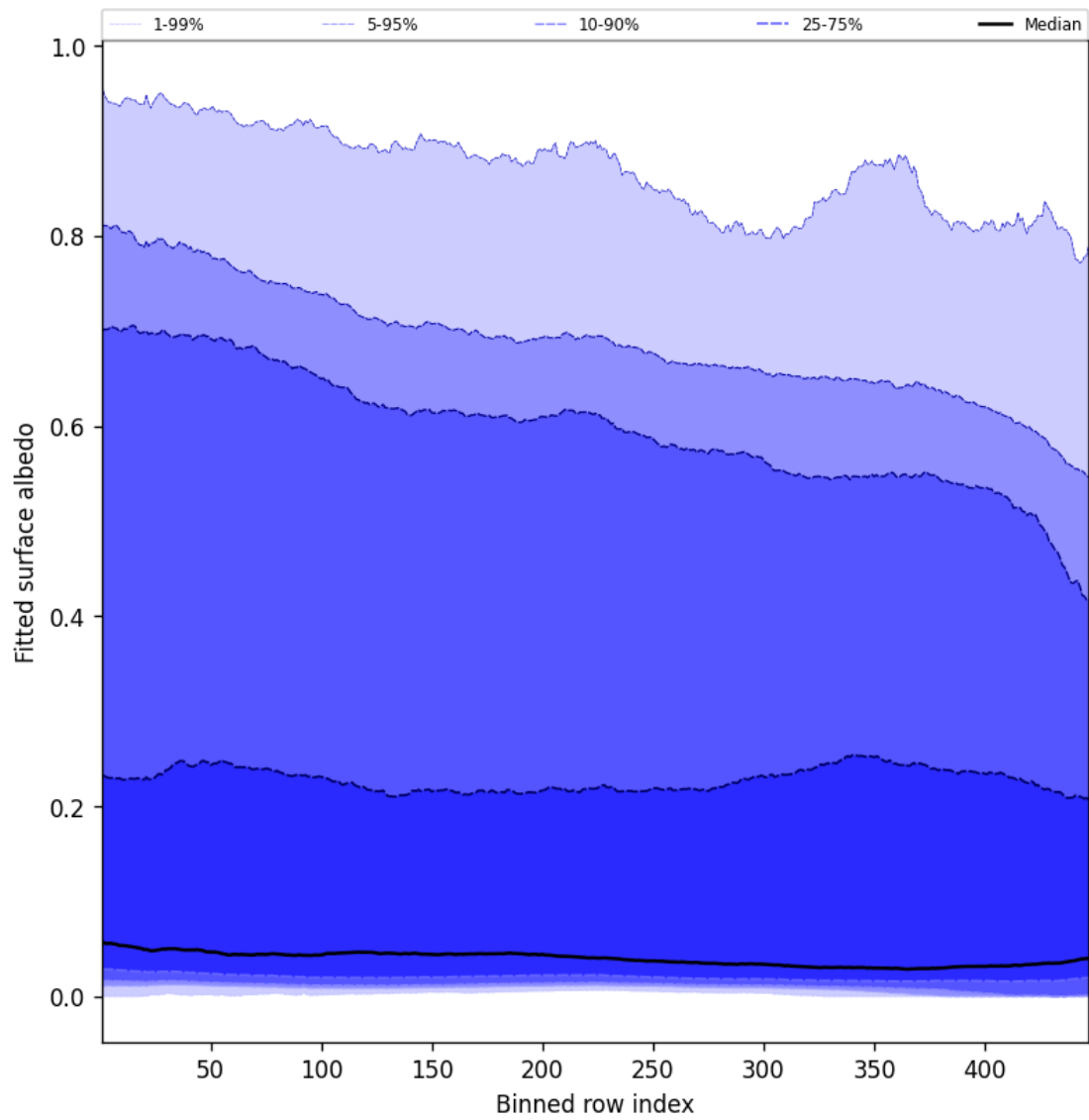
Figure 61: Along track statistics of “Fitted surface albedo” for 2025-09-10 to 2025-09-11
