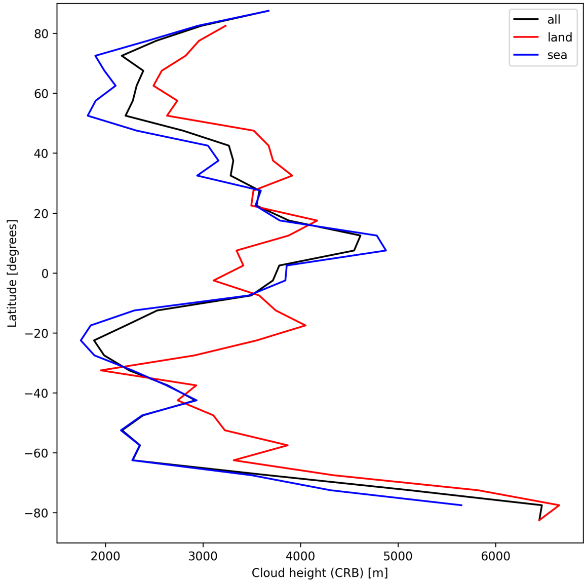
Figure 27: Zonal average of “Cloud height (CRB)” for 2025-09-10 to 2025-09-11.
