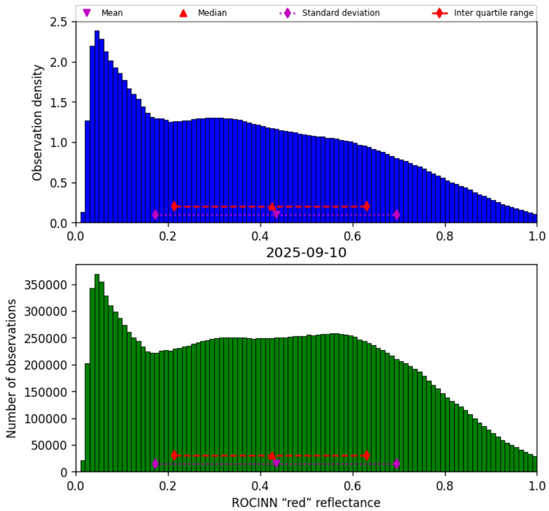
Figure 53: Histogram of “ROCINN “red” reflectance” for 2025-09-10 to 2025-09-11
