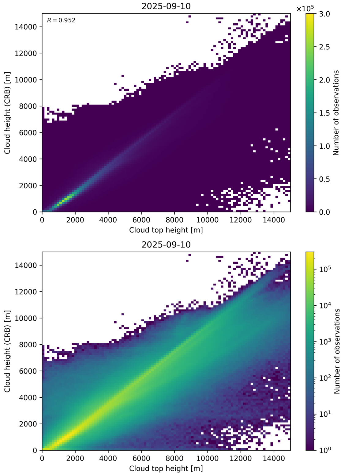
Figure 89: Scatter density plot of “Cloud top height” against “Cloud height (CRB)” for 2025-09-10 to 2025-09-11.
