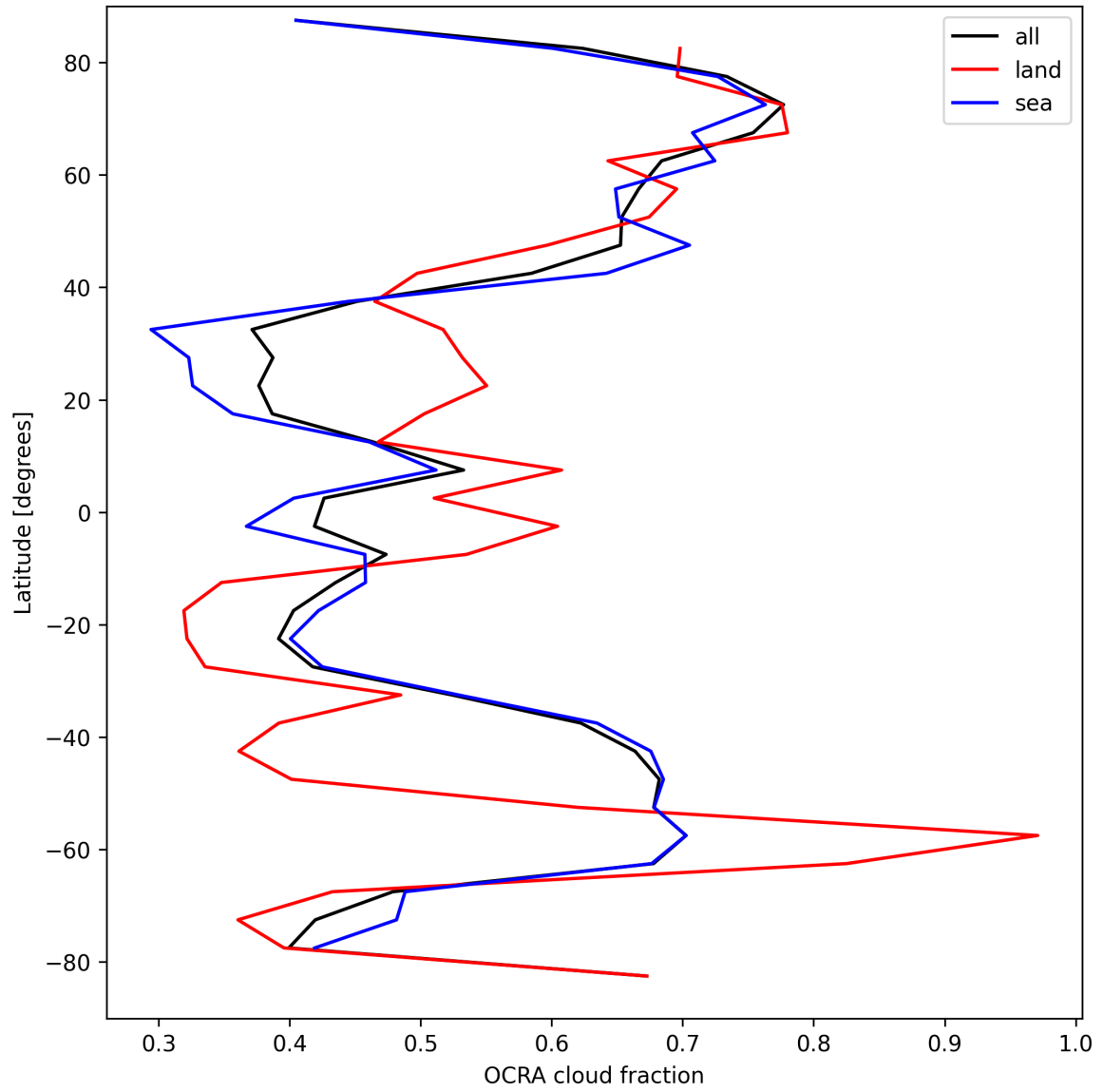
Figure 34: Zonal average of “OCRA cloud fraction” for 2025-09-10 to 2025-09-12.
