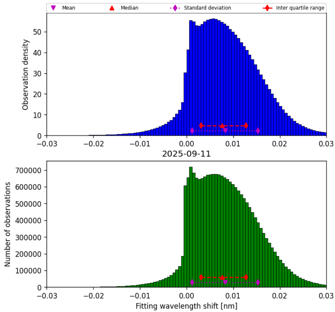
Figure 49: Histogram of “Fitting wavelength shift” for 2025-09-10 to 2025-09-12
