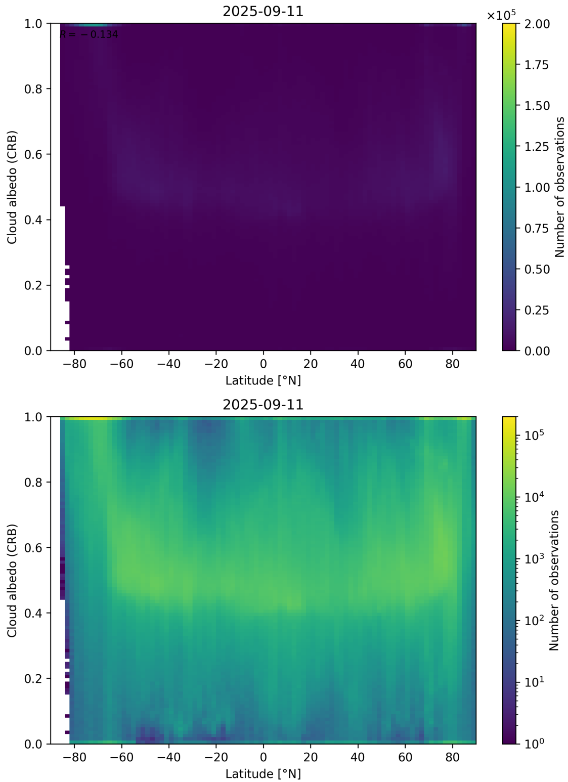
Figure 91: Scatter density plot of “Latitude” against “Cloud albedo (CRB)” for 2025-09-10 to 2025-09-12.
