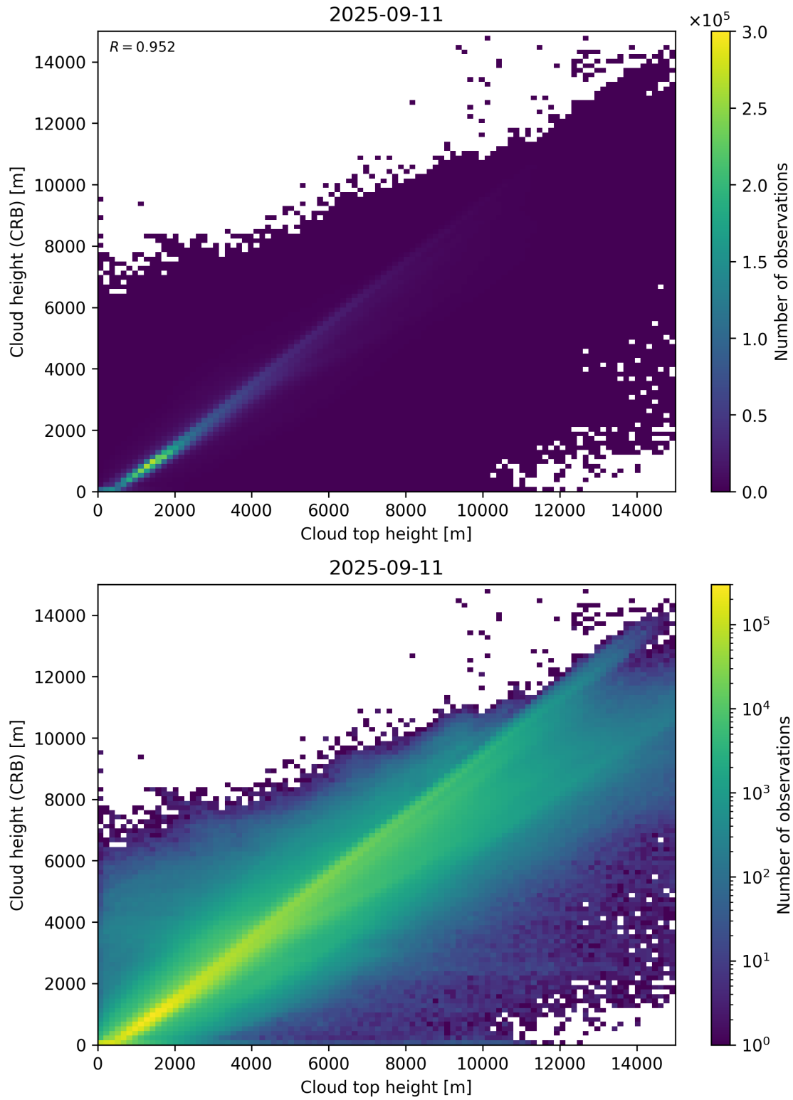
Figure 89: Scatter density plot of “Cloud top height” against “Cloud height (CRB)” for 2025-09-10 to 2025-09-12.
