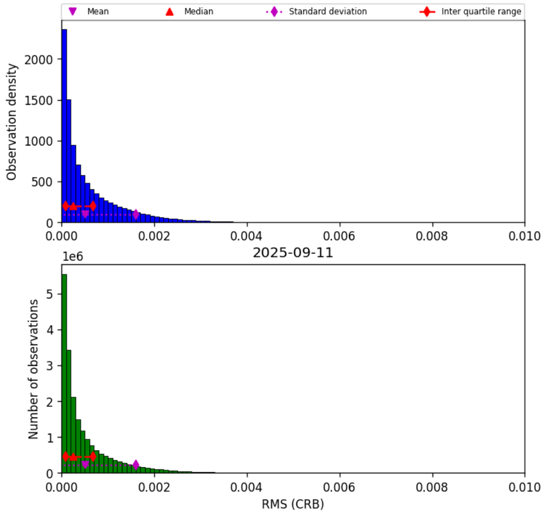
Figure 48: Histogram of “RMS (CRB)” for 2025-09-10 to 2025-09-12
