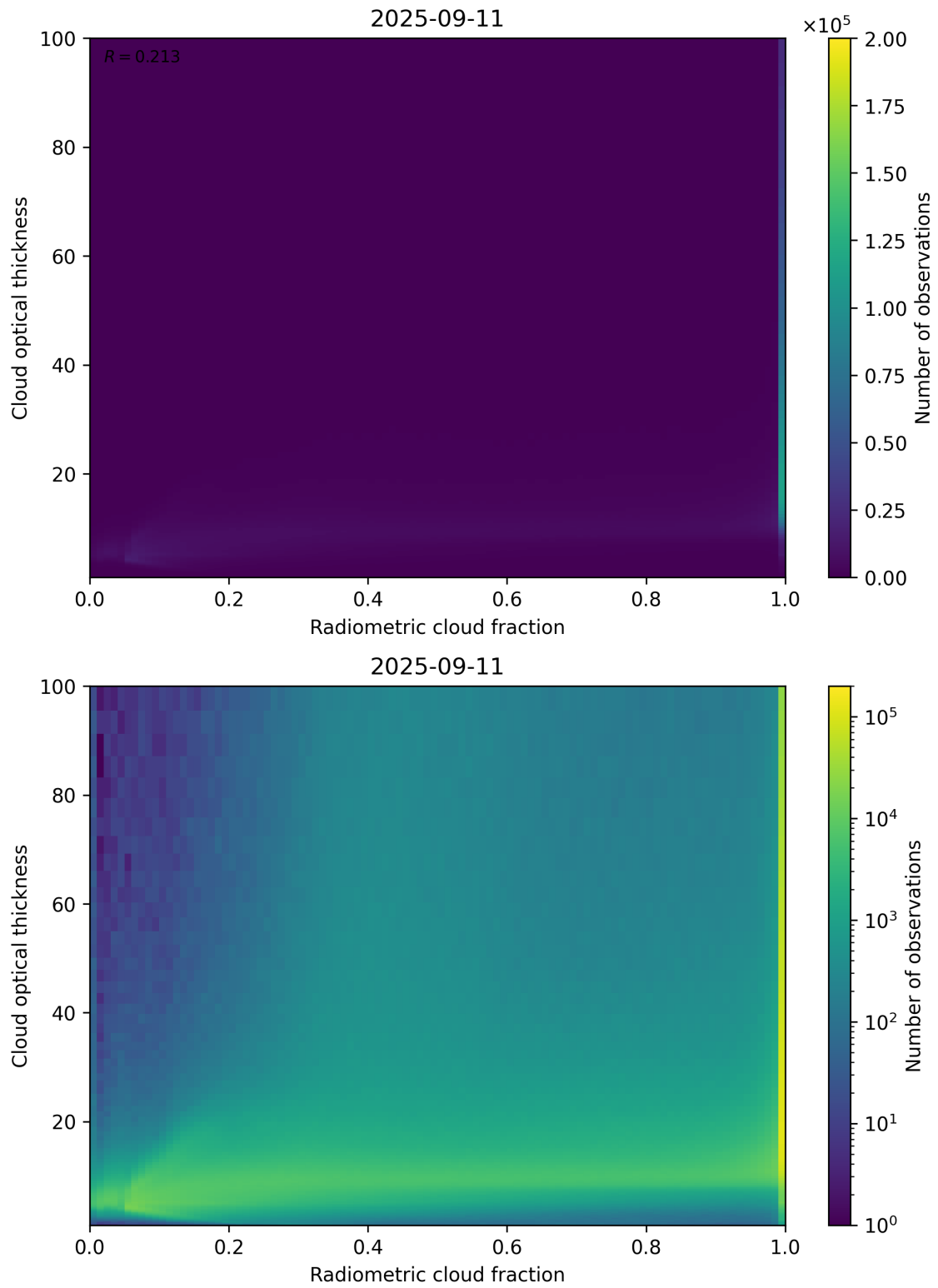
Figure 75: Scatter density plot of “Radiometric cloud fraction” against “Cloud optical thickness” for 2025-09-10 to 2025-09-12.
