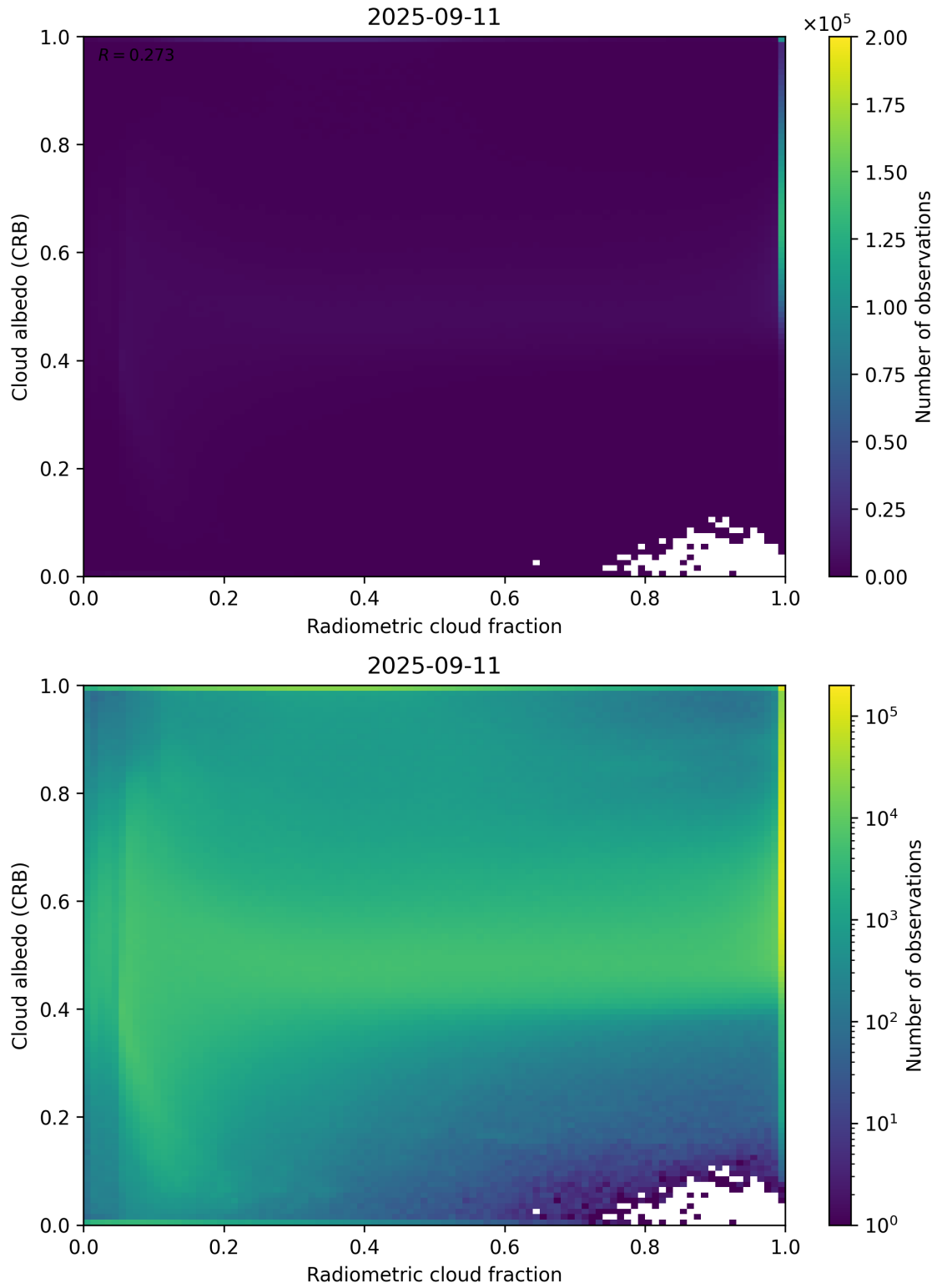
Figure 71: Scatter density plot of “Radiometric cloud fraction” against “Cloud albedo (CRB)” for 2025-09-10 to 2025-09-12.
