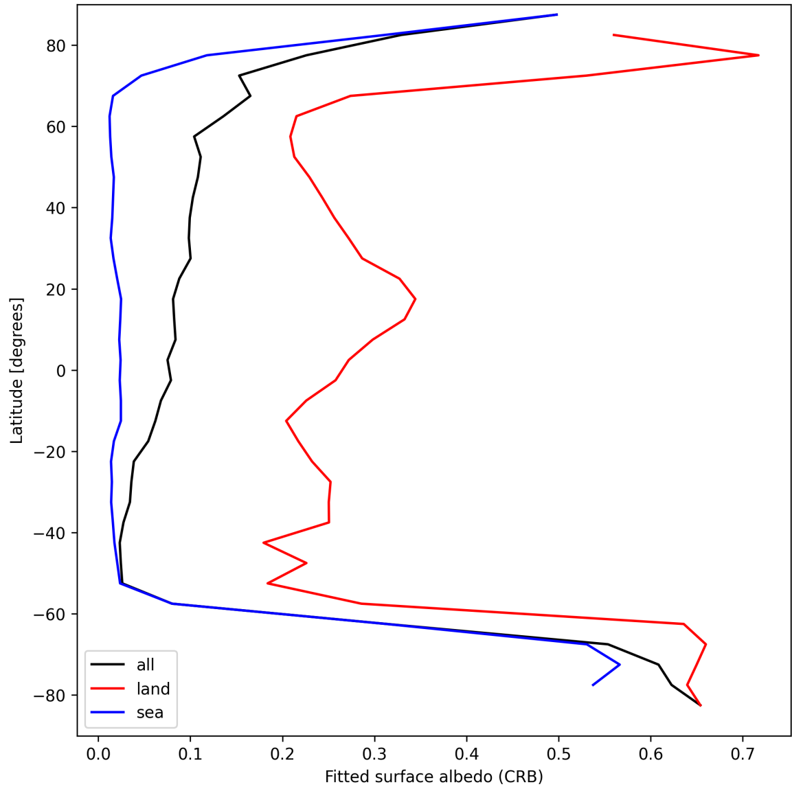
Figure 30: Zonal average of “Fitted surface albedo (CRB)” for 2025-09-10 to 2025-09-12.
