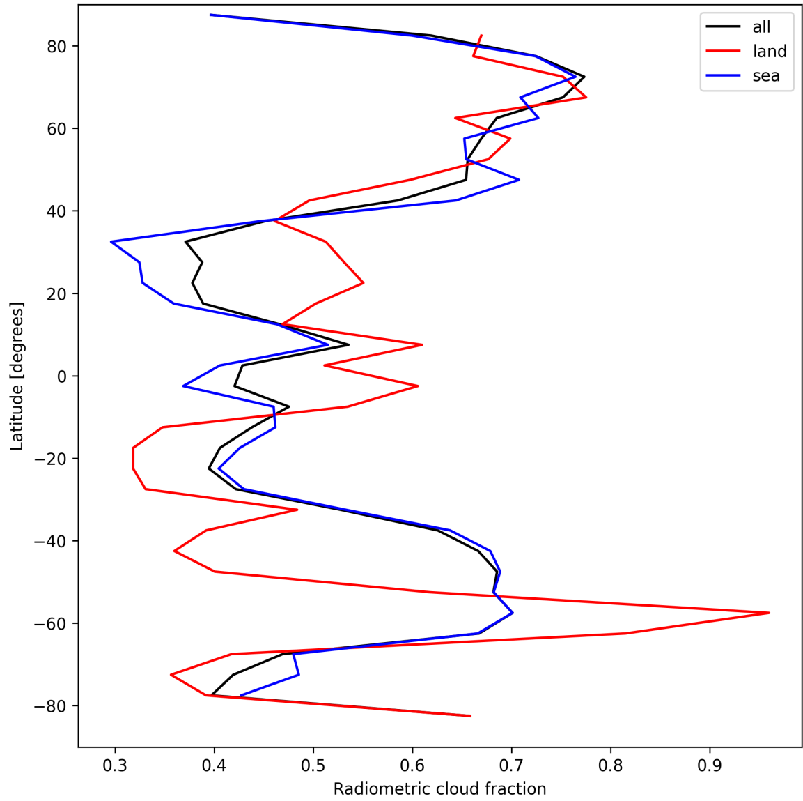
Figure 23: Zonal average of “Radiometric cloud fraction” for 2025-09-10 to 2025-09-12.
