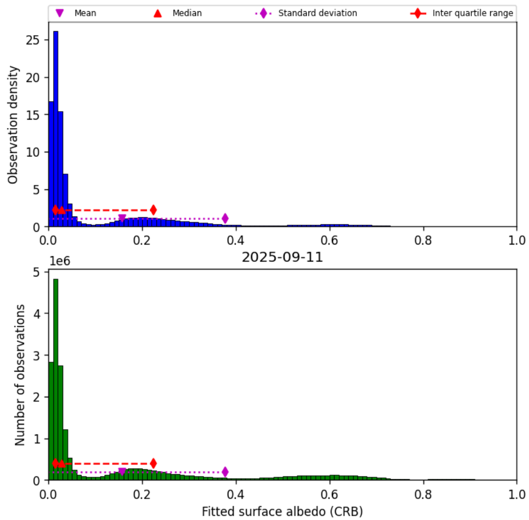
Figure 46: Histogram of “Fitted surface albedo (CRB)” for 2025-09-10 to 2025-09-12
