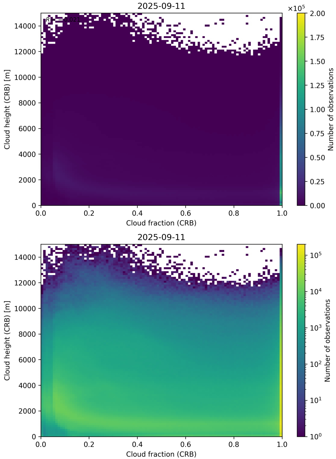
Figure 79: Scatter density plot of “Cloud fraction (CRB)” against “Cloud height (CRB)” for 2025-09-10 to 2025-09-12.
