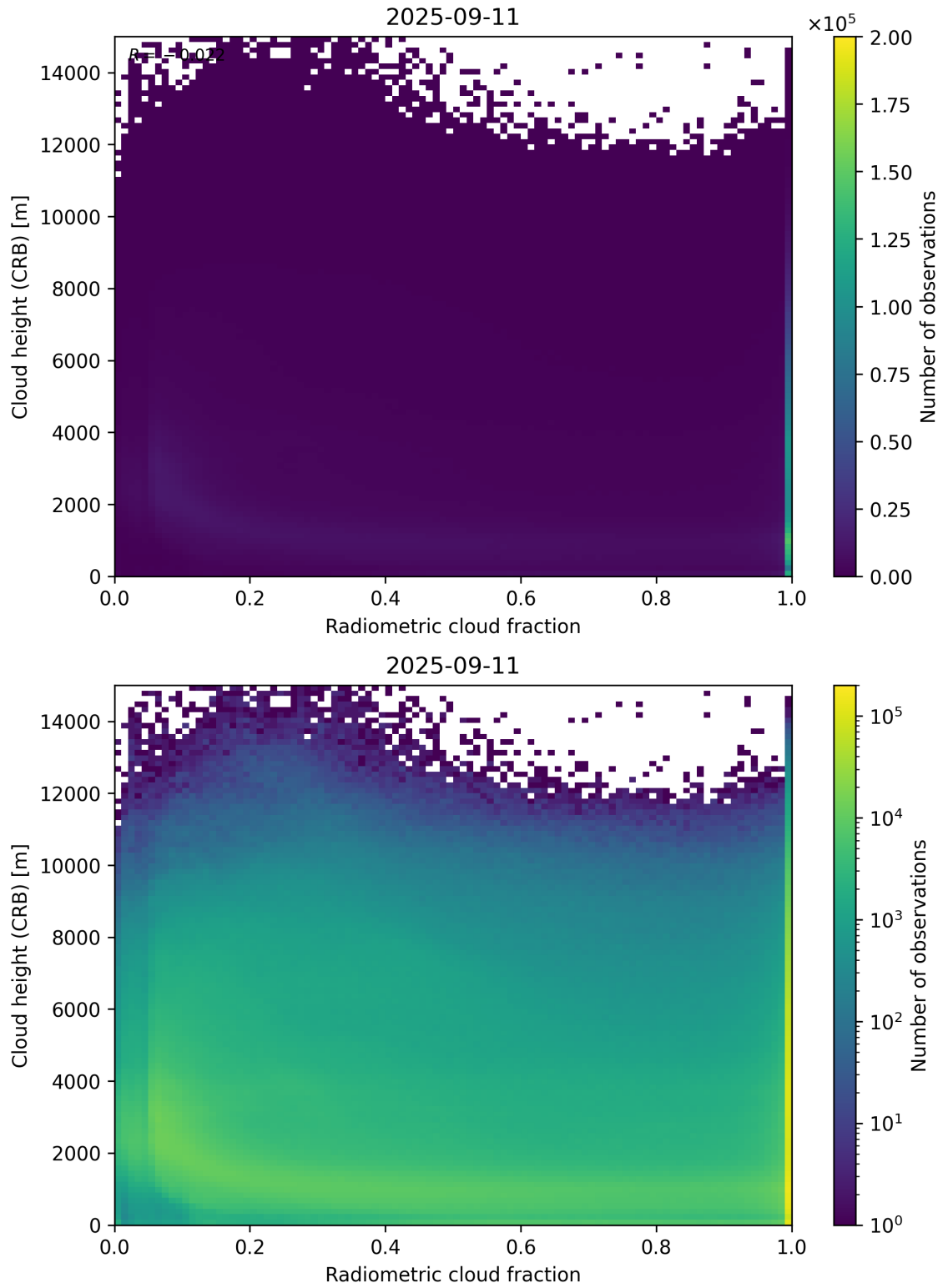
Figure 74: Scatter density plot of “Radiometric cloud fraction” against “Cloud height (CRB)” for 2025-09-10 to 2025-09-12.
