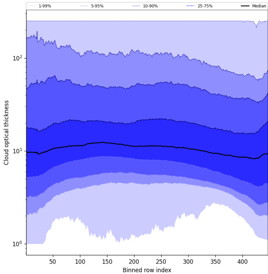
Figure 57: Along track statistics of “Cloud optical thickness” for 2025-09-10 to 2025-09-12
