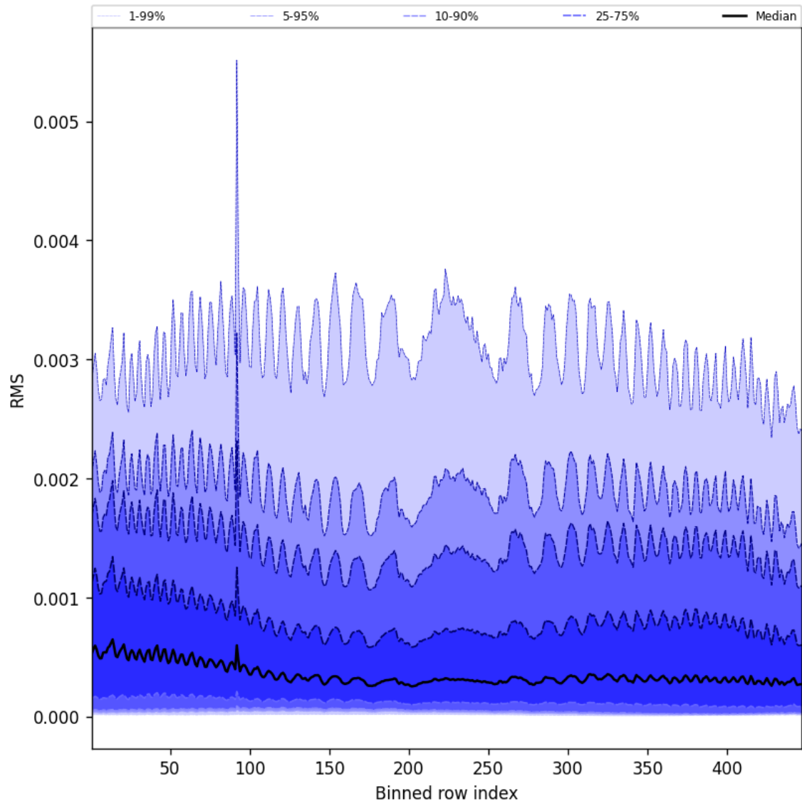
Figure 63: Along track statistics of “RMS” for 2025-09-10 to 2025-09-12
