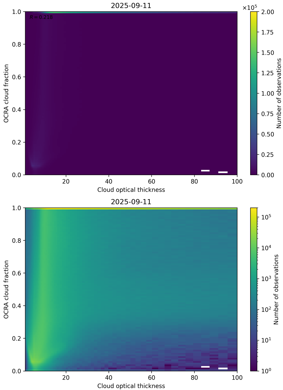
Figure 83: Scatter density plot of “Cloud optical thickness” against “OCRA cloud fraction” for 2025-09-10 to 2025-09-12.
