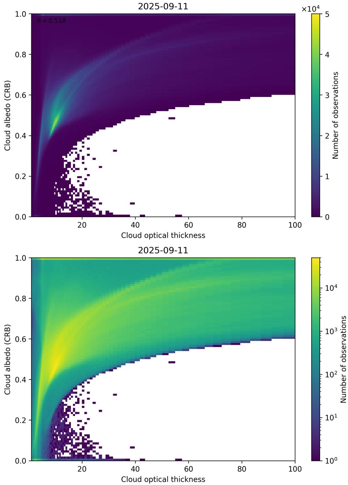
Figure 82: Scatter density plot of “Cloud optical thickness” against “Cloud albedo (CRB)” for 2025-09-10 to 2025-09-12.
