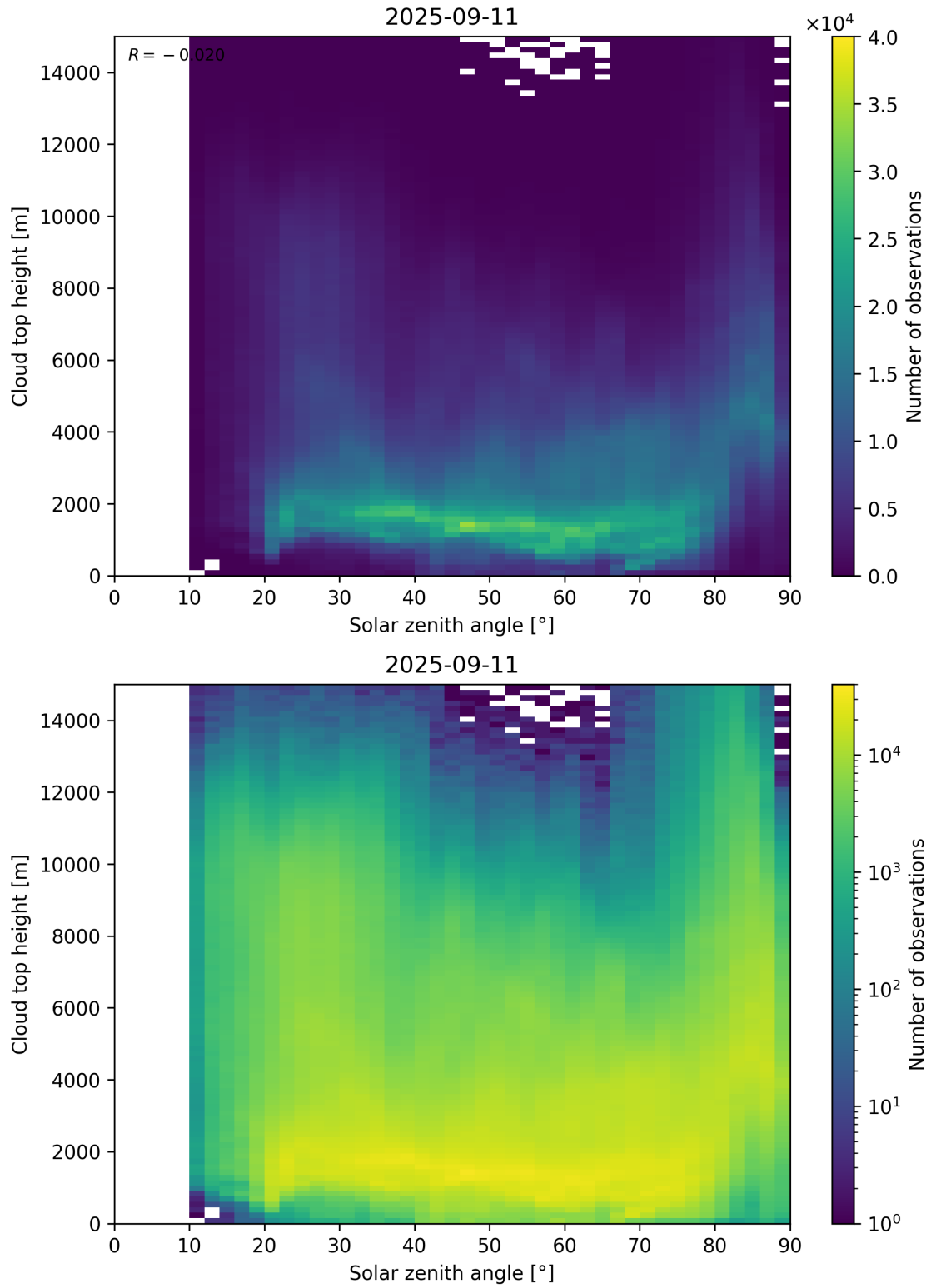
Figure 104: Scatter density plot of “Solar zenith angle” against “Cloud top height” for 2025-09-10 to 2025-09-12.
