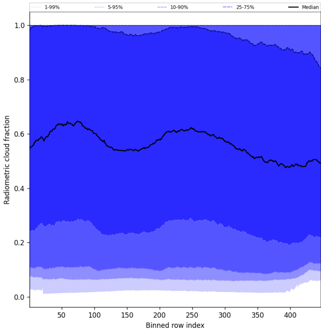
Figure 55: Along track statistics of “Radiometric cloud fraction” for 2025-09-10 to 2025-09-12
