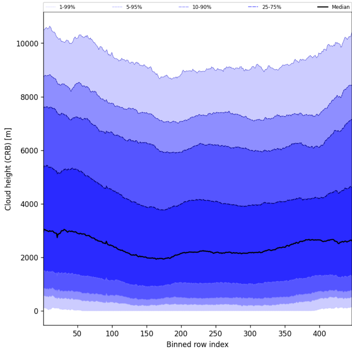
Figure 59: Along track statistics of “Cloud height (CRB)” for 2025-09-10 to 2025-09-12
