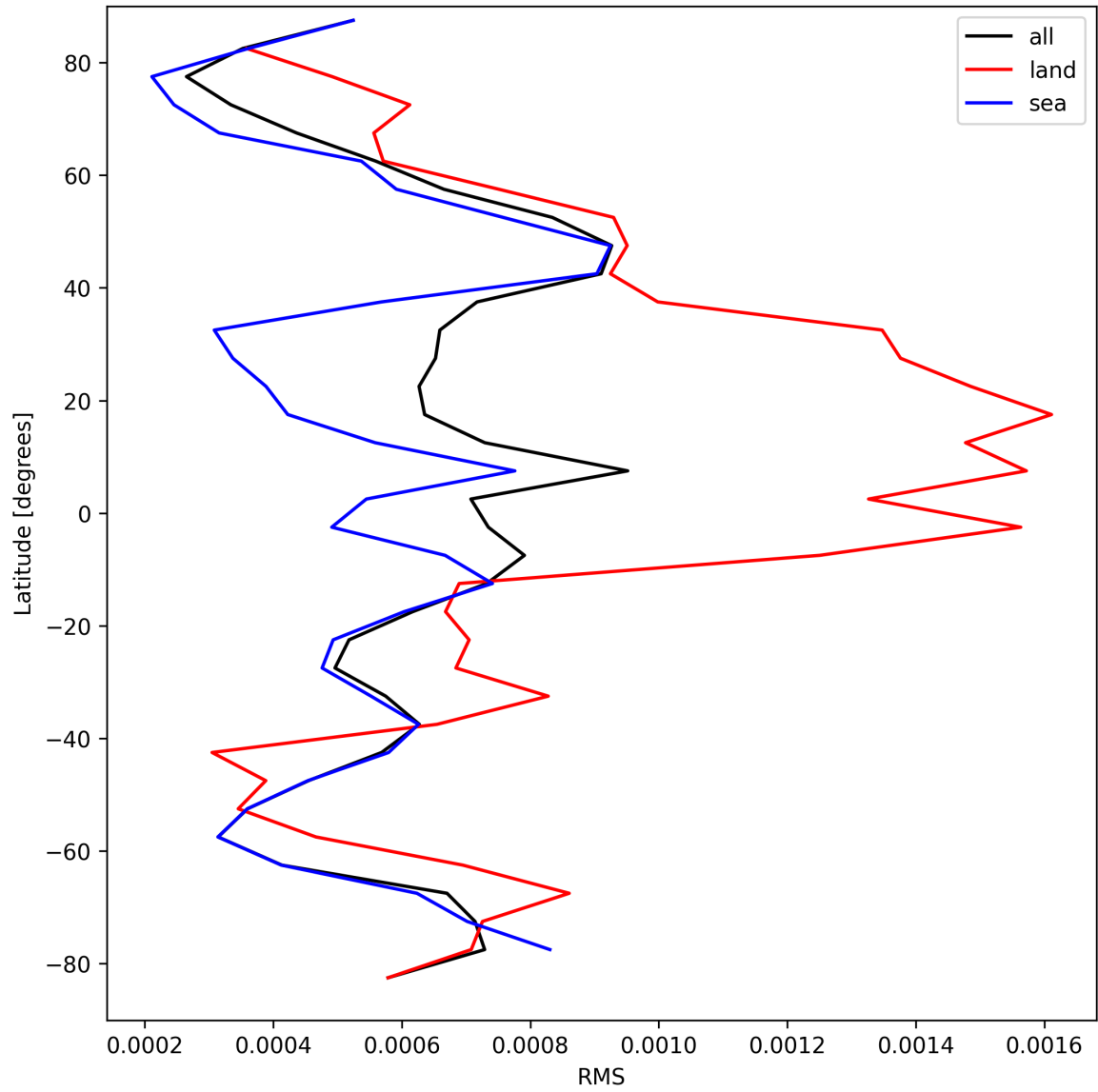
Figure 31: Zonal average of “RMS” for 2025-09-10 to 2025-09-12.
