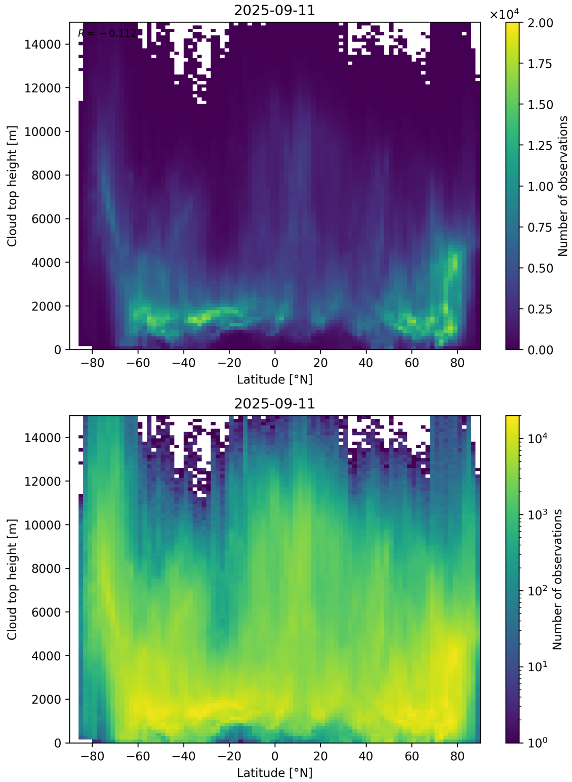
Figure 97: Scatter density plot of “Latitude” against “Cloud top height” for 2025-09-10 to 2025-09-12.
