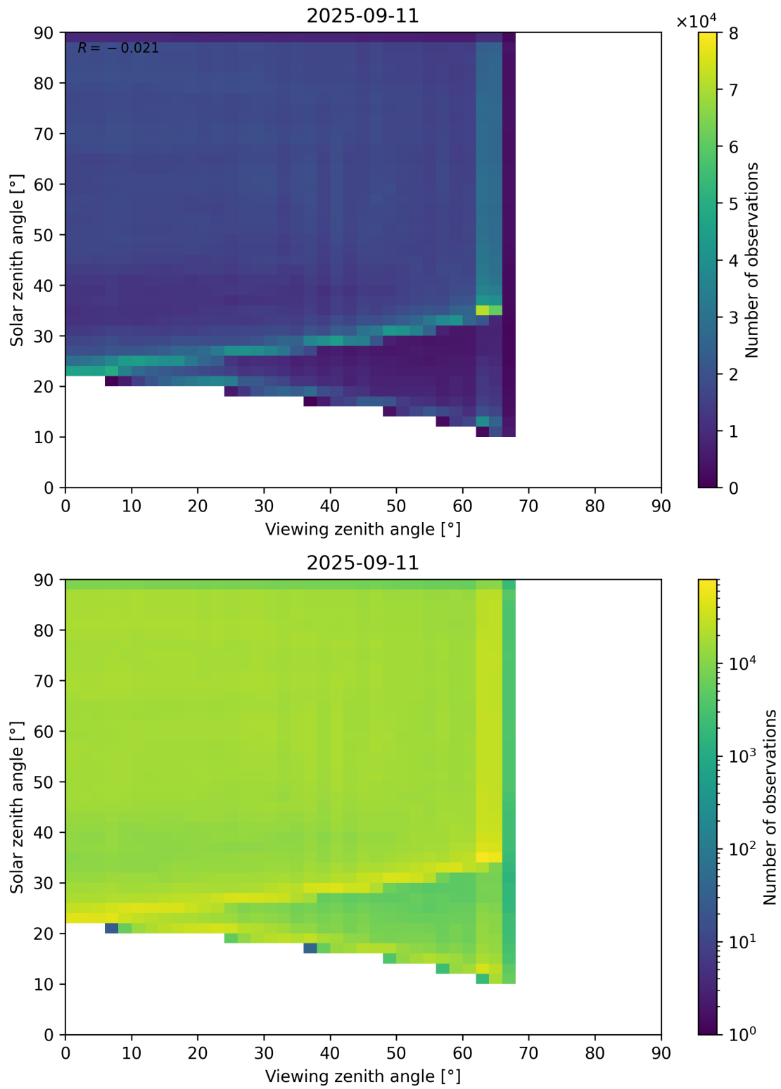
Figure 114: Scatter density plot of “Viewing zenith angle” against “Solar zenith angle” for 2025-09-10 to 2025-09-12.
