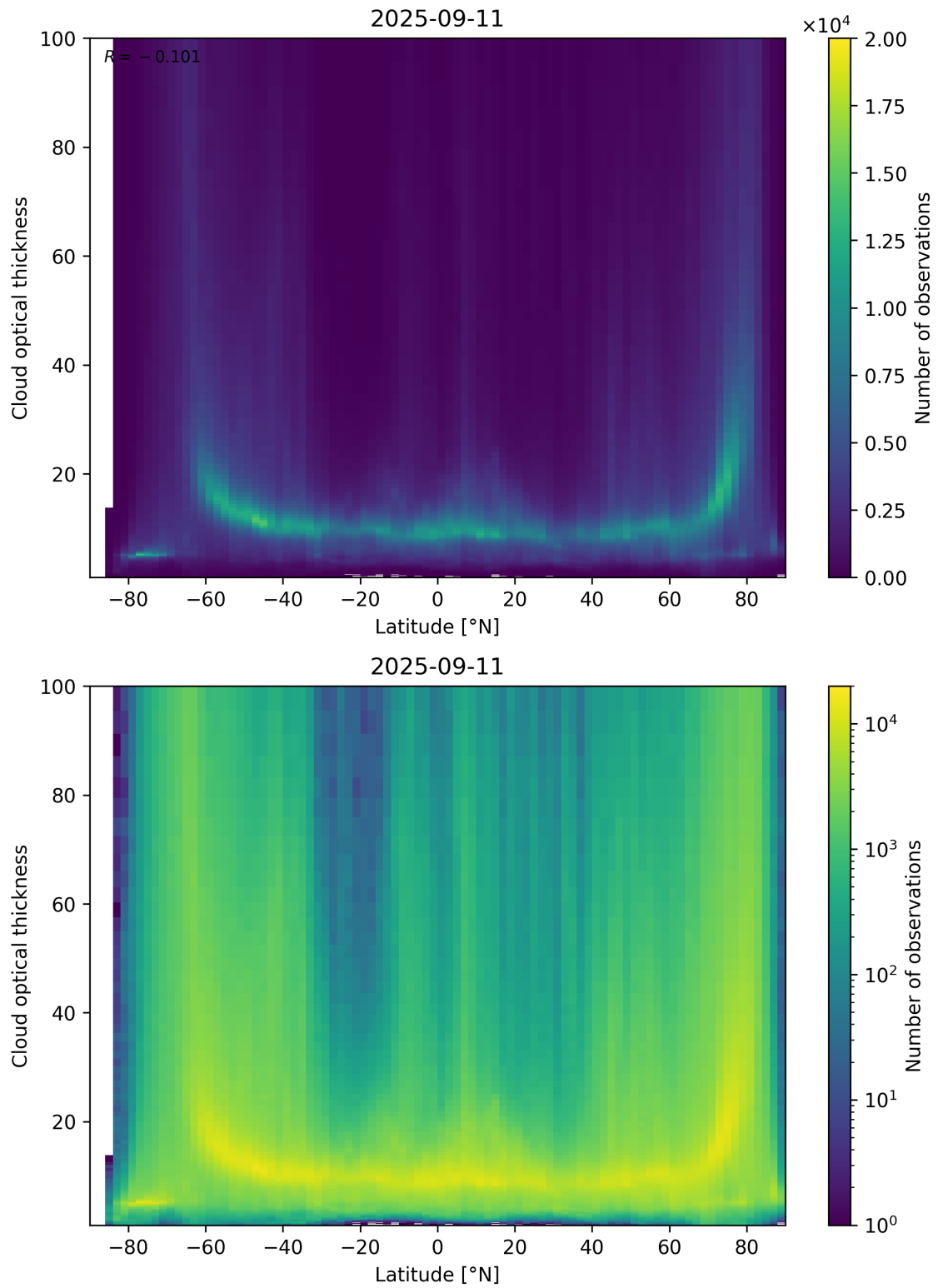
Figure 96: Scatter density plot of “Latitude” against “Cloud optical thickness” for 2025-09-10 to 2025-09-12.
