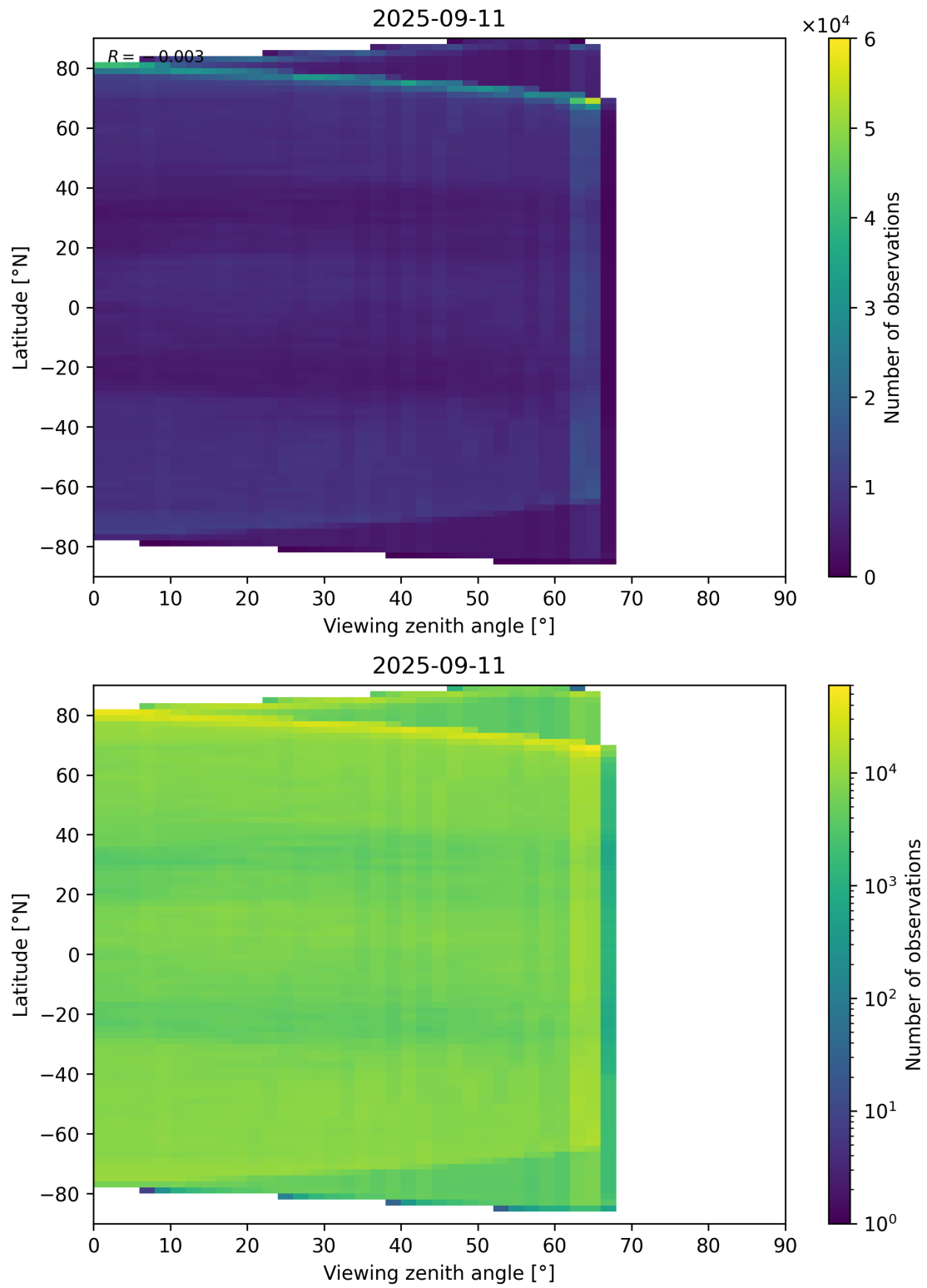
Figure 113: Scatter density plot of “Viewing zenith angle” against “Latitude” for 2025-09-10 to 2025-09-12.
