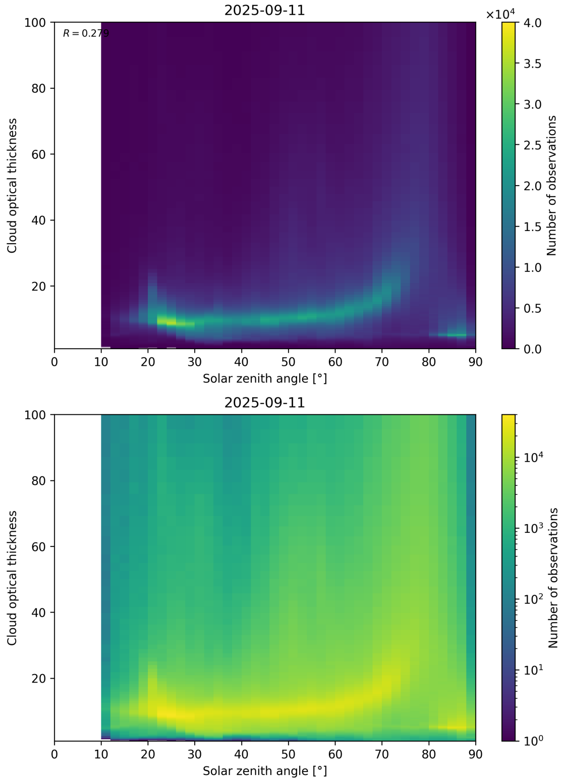
Figure 103: Scatter density plot of “Solar zenith angle” against “Cloud optical thickness” for 2025-09-10 to 2025-09-12.
