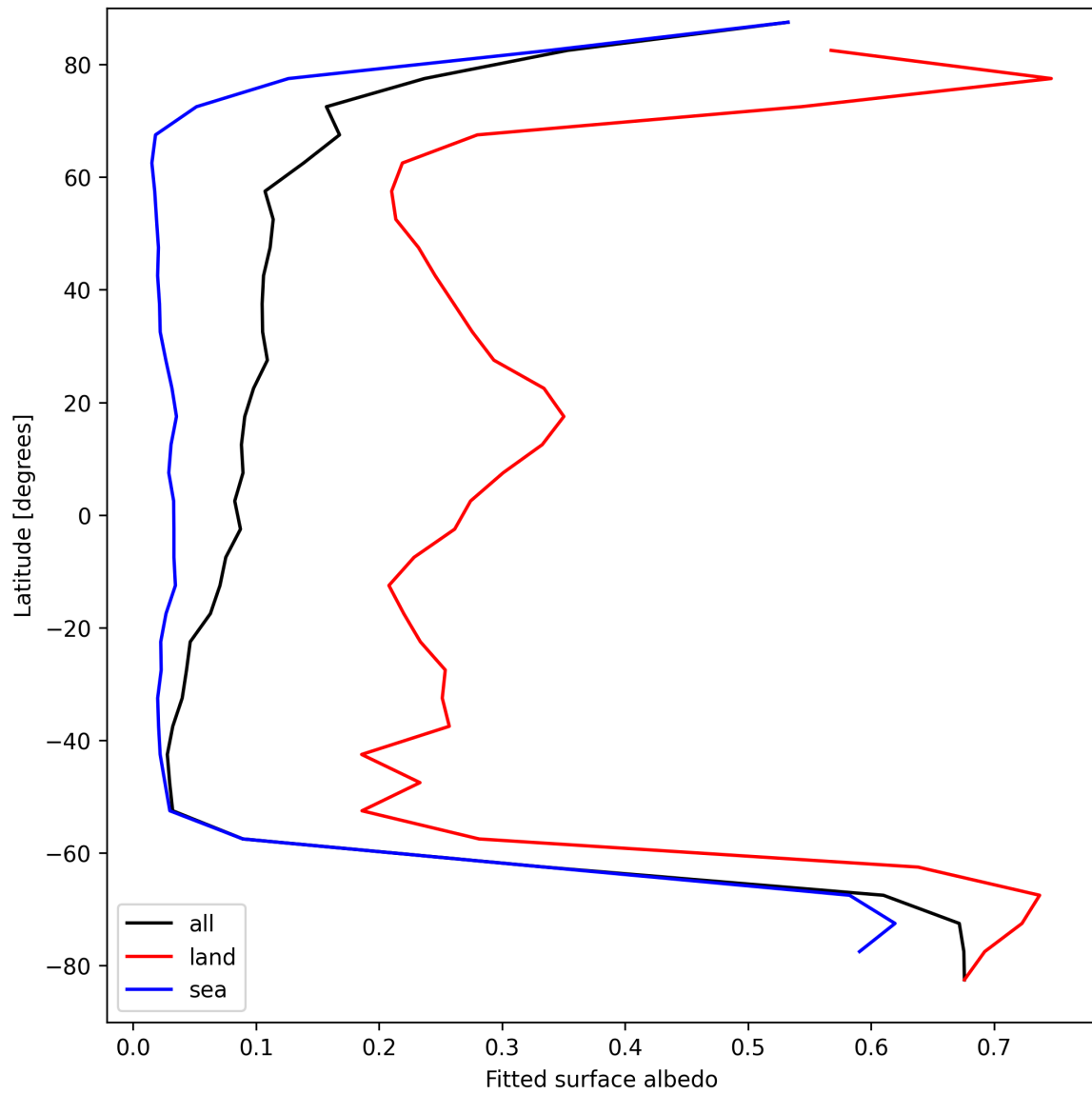
Figure 29: Zonal average of “Fitted surface albedo” for 2025-09-10 to 2025-09-12.
