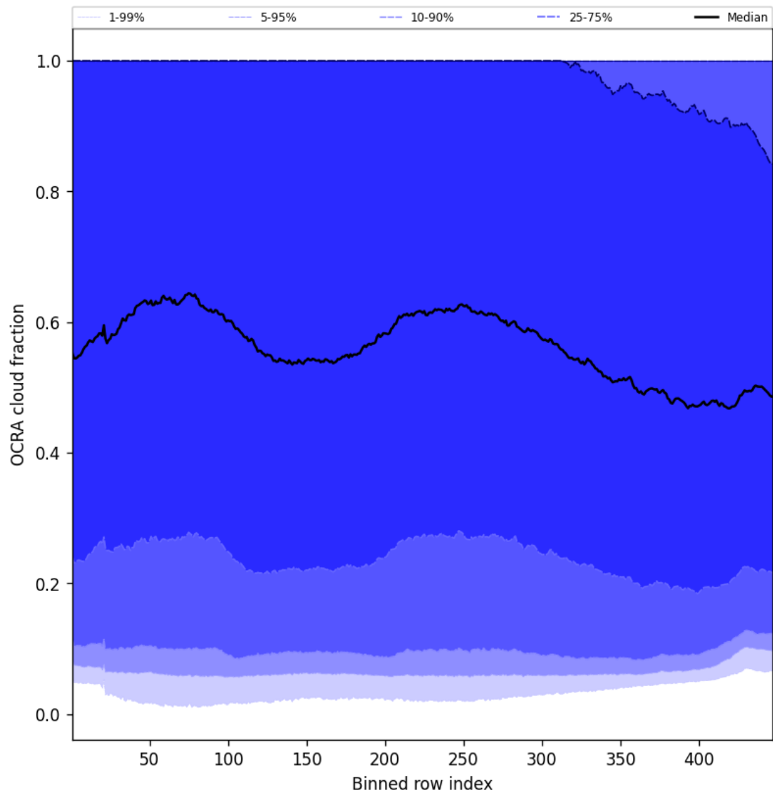
Figure 66: Along track statistics of “OCRA cloud fraction” for 2025-09-10 to 2025-09-12
