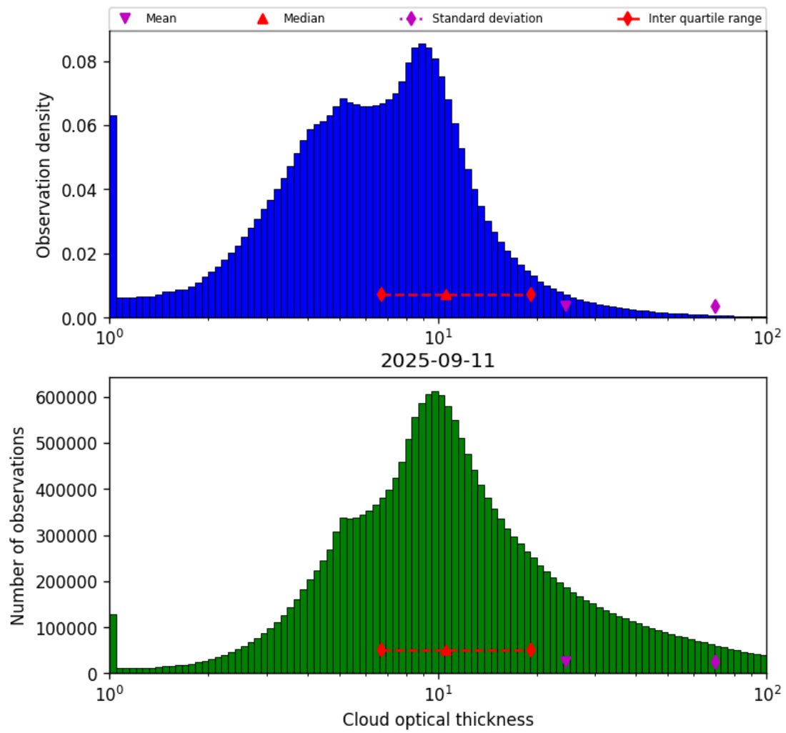
Figure 41: Histogram of “Cloud optical thickness” for 2025-09-10 to 2025-09-12
