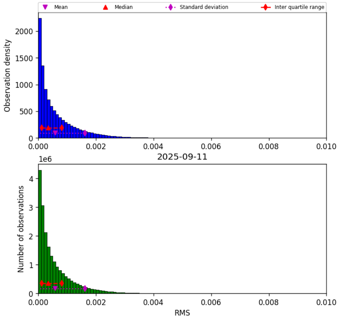
Figure 47: Histogram of “RMS” for 2025-09-10 to 2025-09-12
