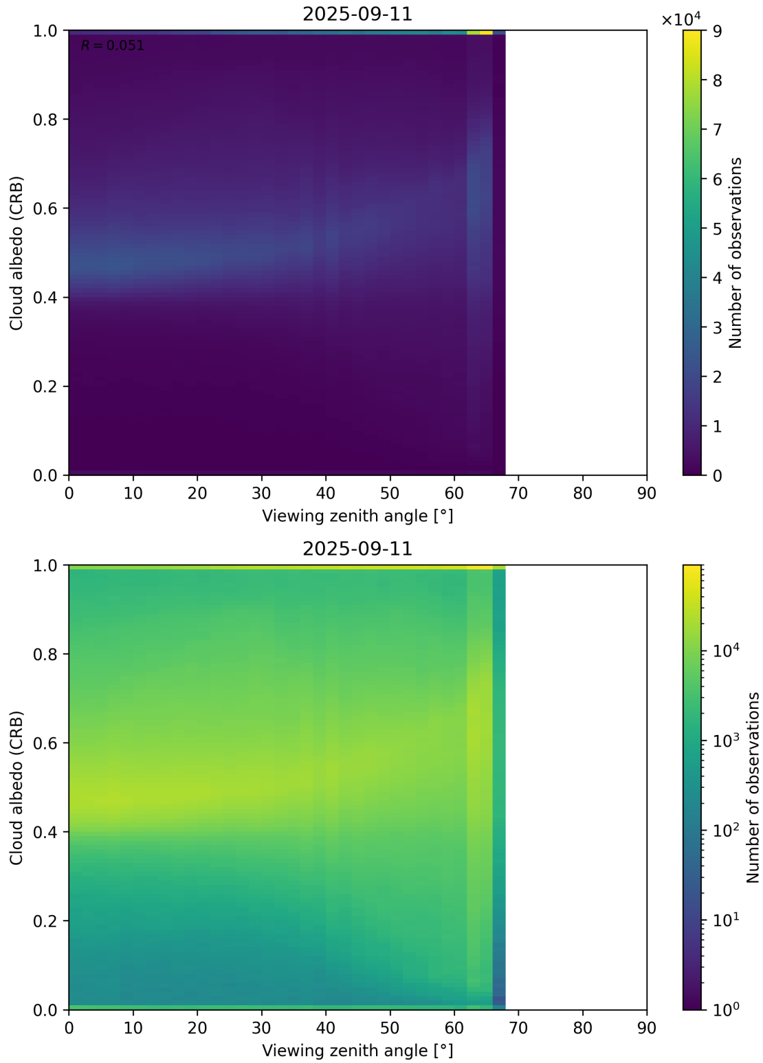
Figure 106: Scatter density plot of “Viewing zenith angle” against “Cloud albedo (CRB)” for 2025-09-10 to 2025-09-12.
