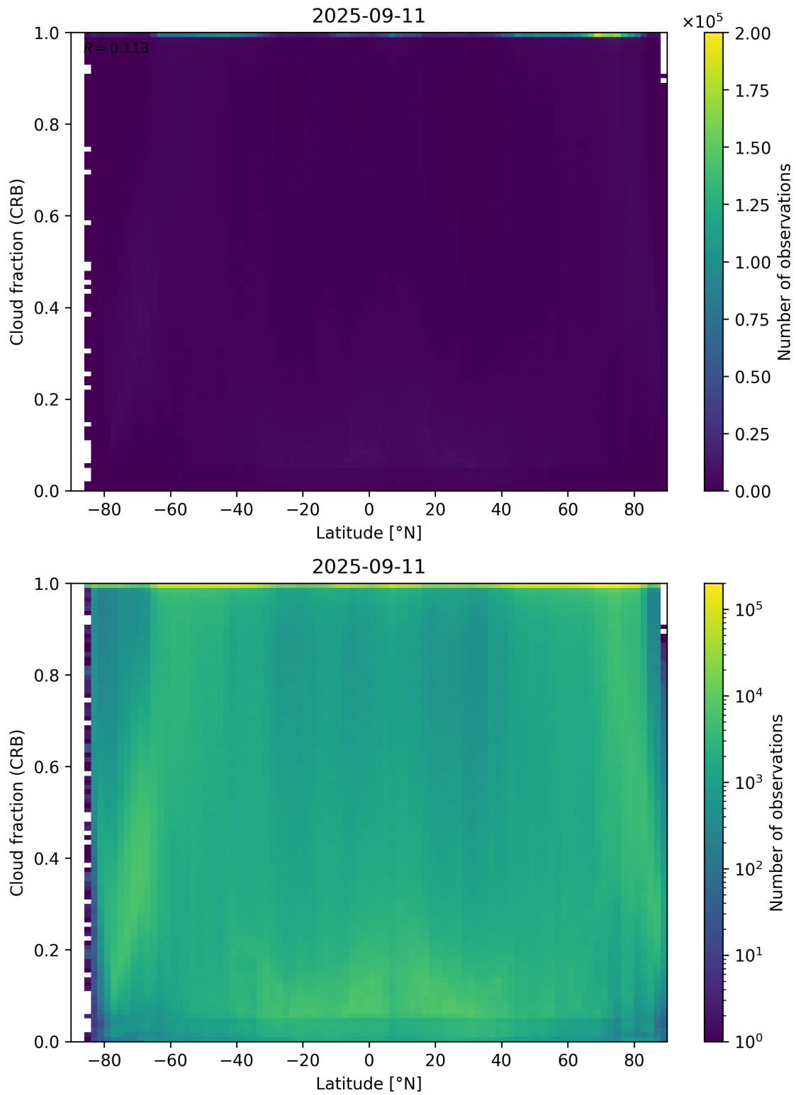
Figure 94: Scatter density plot of “Latitude” against “Cloud fraction (CRB)” for 2025-09-10 to 2025-09-12.
