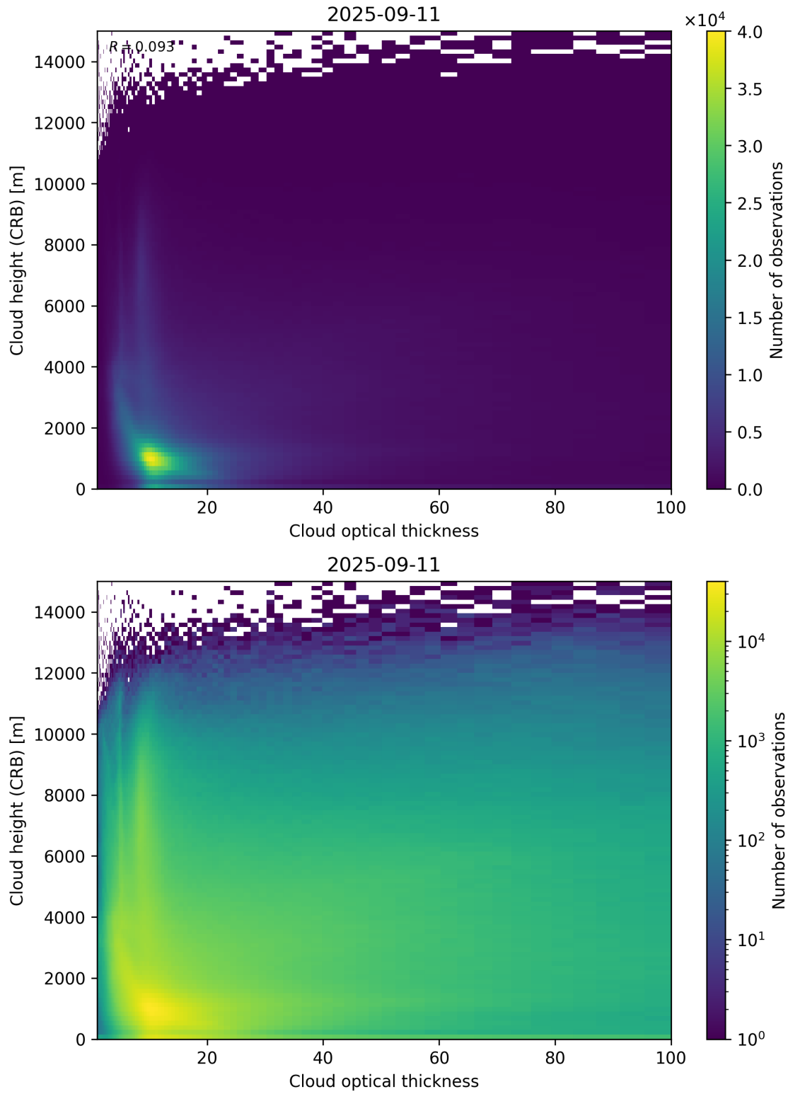
Figure 85: Scatter density plot of “Cloud optical thickness” against “Cloud height (CRB)” for 2025-09-10 to 2025-09-12.
