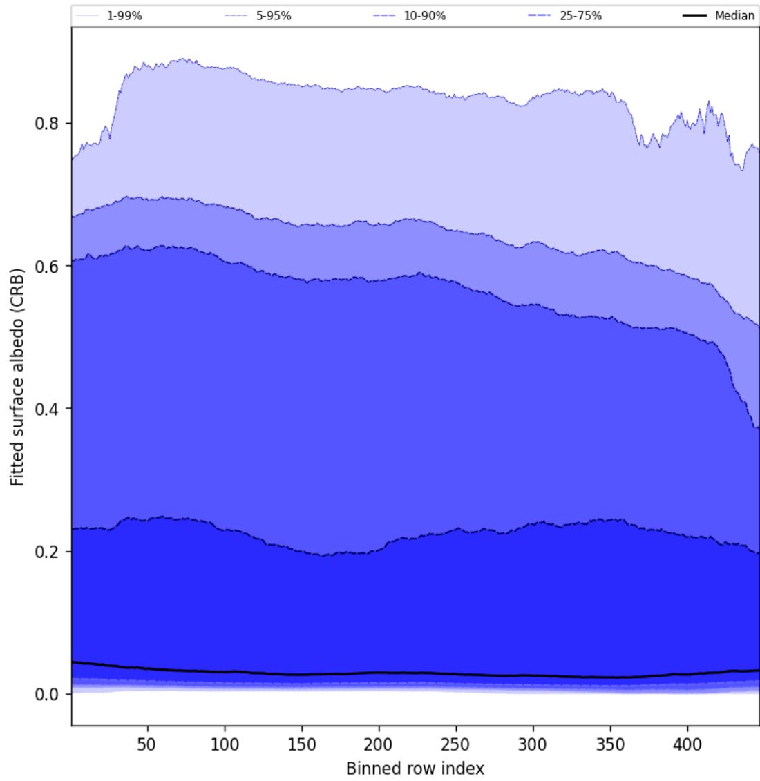
Figure 62: Along track statistics of “Fitted surface albedo (CRB)” for 2025-09-10 to 2025-09-12
