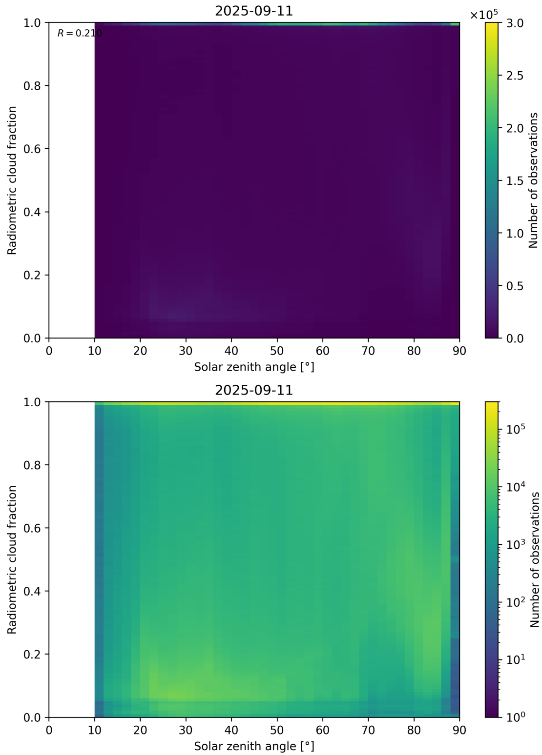
Figure 99: Scatter density plot of “Solar zenith angle” against “Radiometric cloud fraction” for 2025-09-10 to 2025-09-12.
