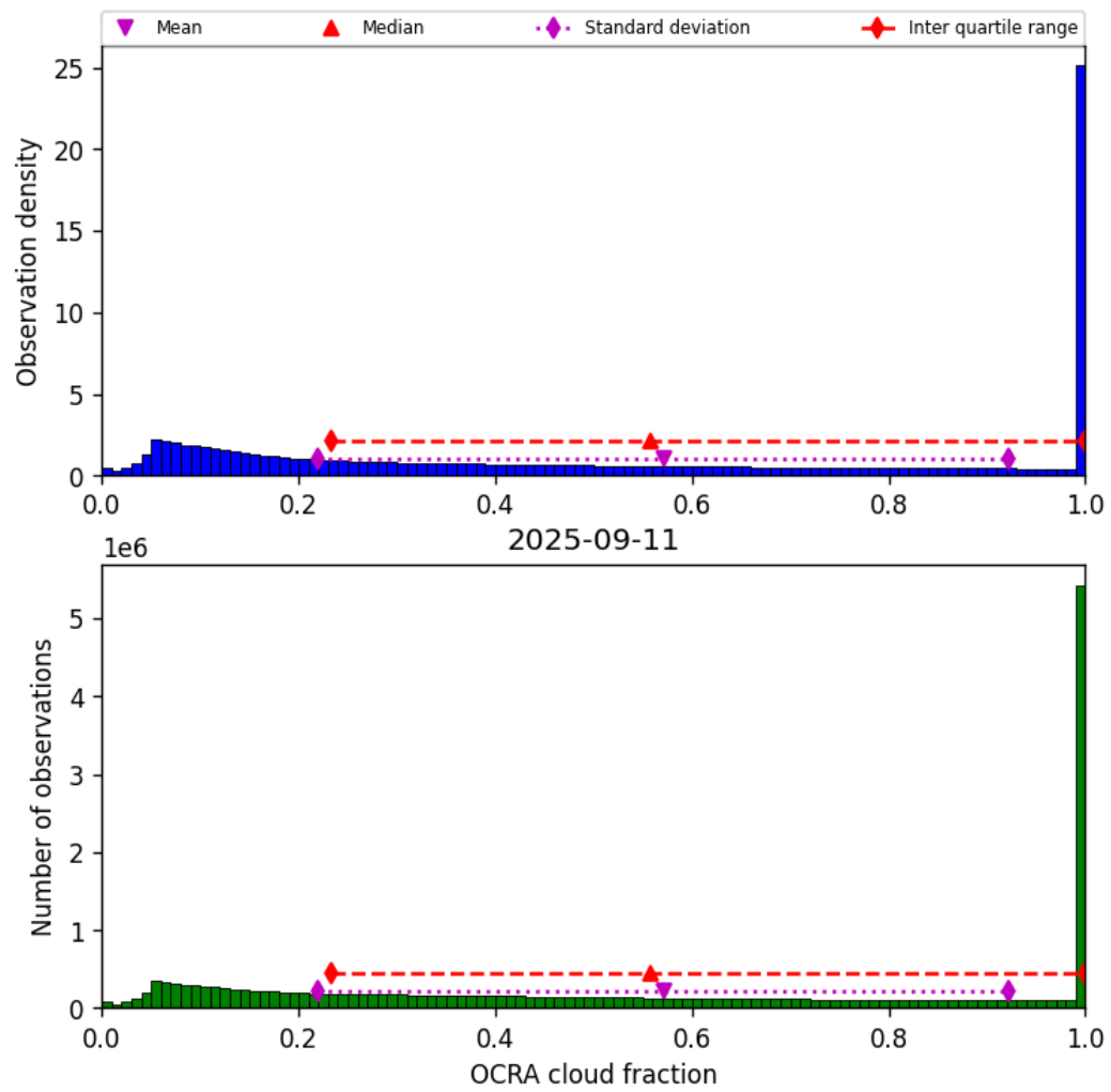
Figure 50: Histogram of “OCRA cloud fraction” for 2025-09-10 to 2025-09-12
