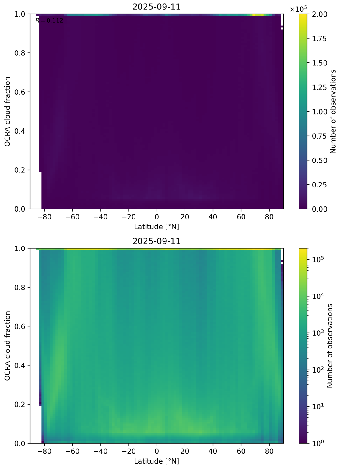
Figure 93: Scatter density plot of “Latitude” against “OCRA cloud fraction” for 2025-09-10 to 2025-09-12.
