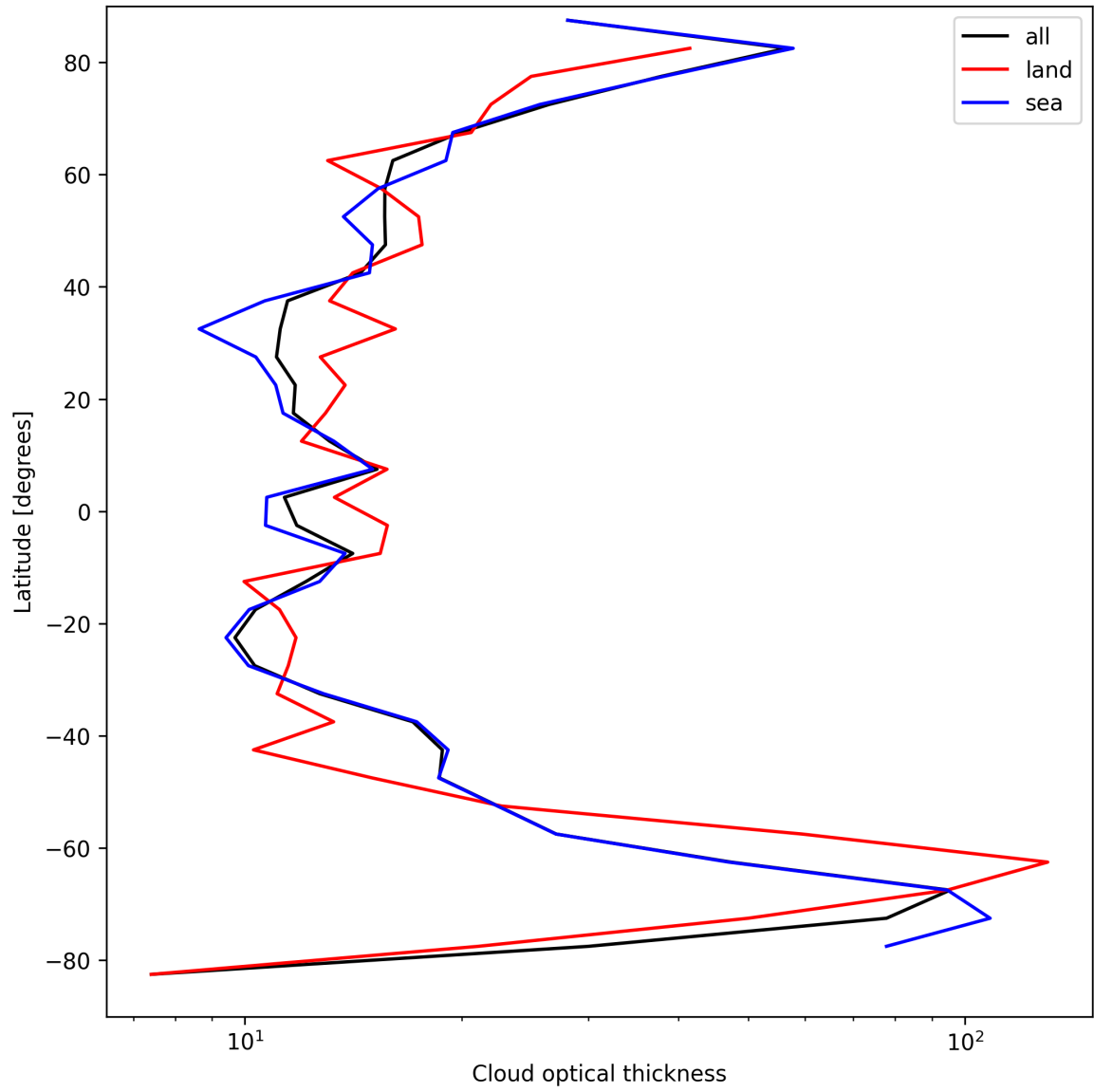
Figure 25: Zonal average of “Cloud optical thickness” for 2025-09-10 to 2025-09-12.
