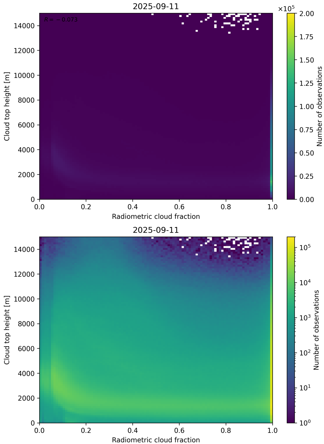
Figure 76: Scatter density plot of “Radiometric cloud fraction” against “Cloud top height” for 2025-09-10 to 2025-09-12.
