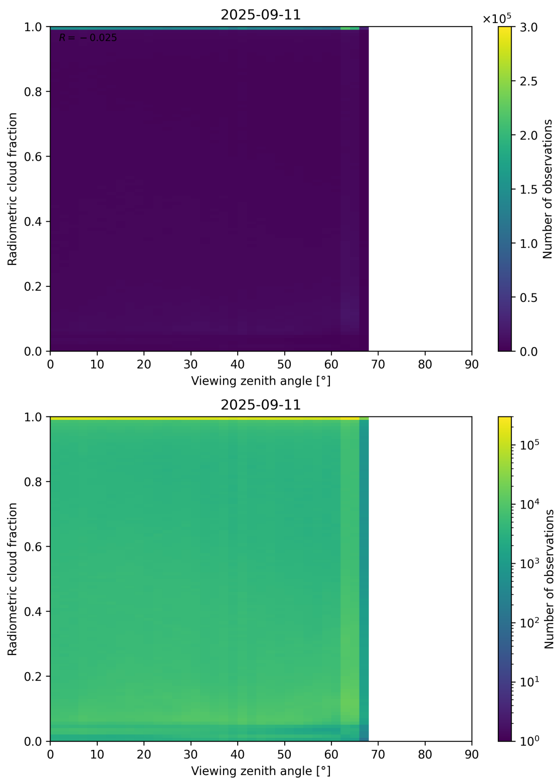
Figure 107: Scatter density plot of “Viewing zenith angle” against “Radiometric cloud fraction” for 2025-09-10 to 2025-09-12.
