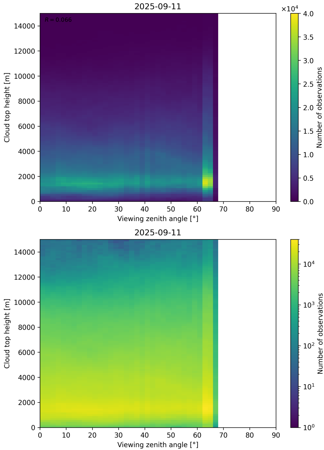
Figure 112: Scatter density plot of “Viewing zenith angle” against “Cloud top height” for 2025-09-10 to 2025-09-12.
