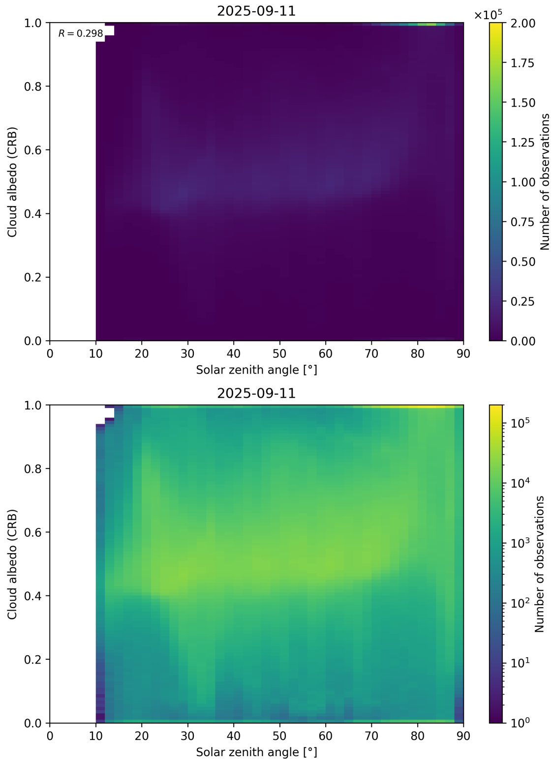
Figure 98: Scatter density plot of “Solar zenith angle” against “Cloud albedo (CRB)” for 2025-09-10 to 2025-09-12.
