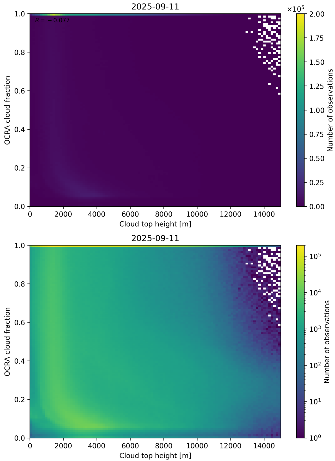
Figure 87: Scatter density plot of “Cloud top height” against “OCRA cloud fraction” for 2025-09-10 to 2025-09-12.
