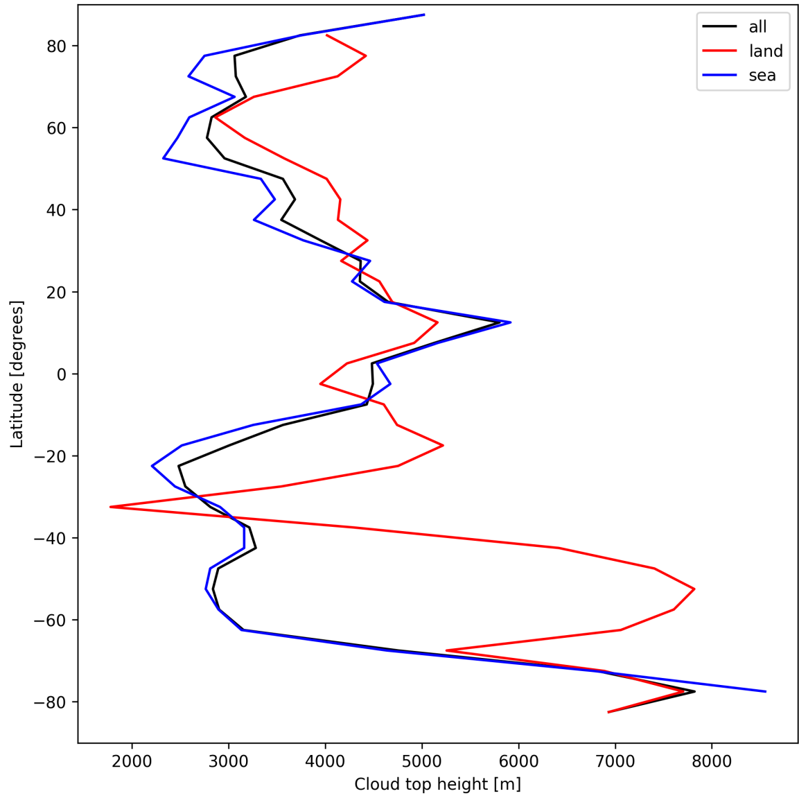
Figure 24: Zonal average of “Cloud top height” for 2025-09-10 to 2025-09-12.
