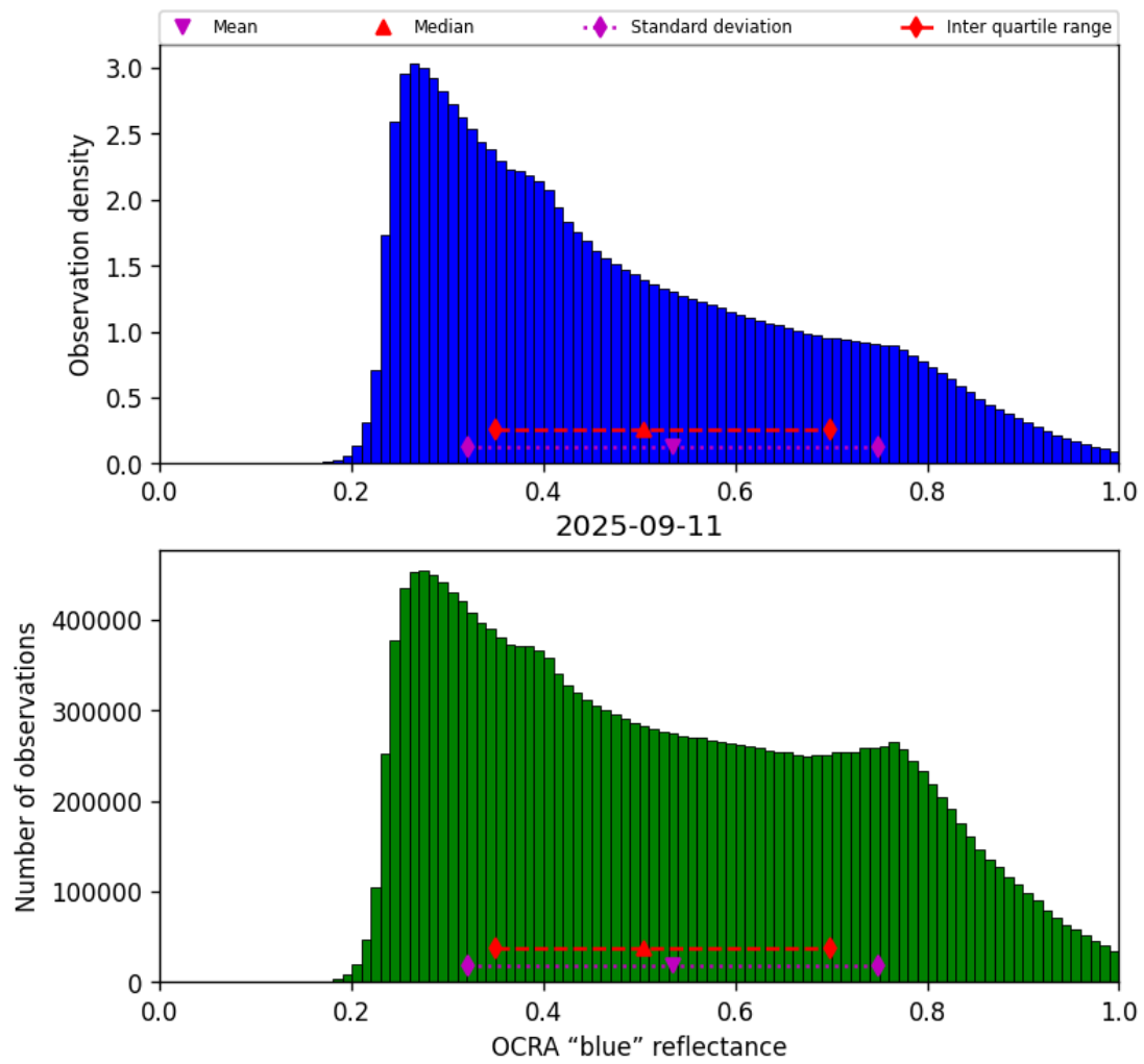
Figure 51: Histogram of “OCRA “blue” reflectance” for 2025-09-10 to 2025-09-12
