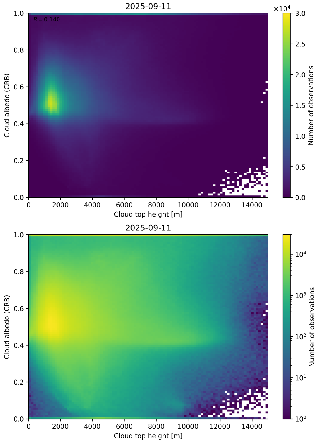
Figure 86: Scatter density plot of “Cloud top height” against “Cloud albedo (CRB)” for 2025-09-10 to 2025-09-12.
