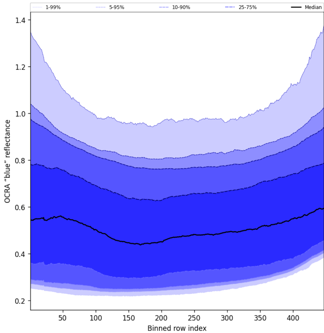
Figure 67: Along track statistics of “OCRA “blue” reflectance” for 2025-09-10 to 2025-09-12
