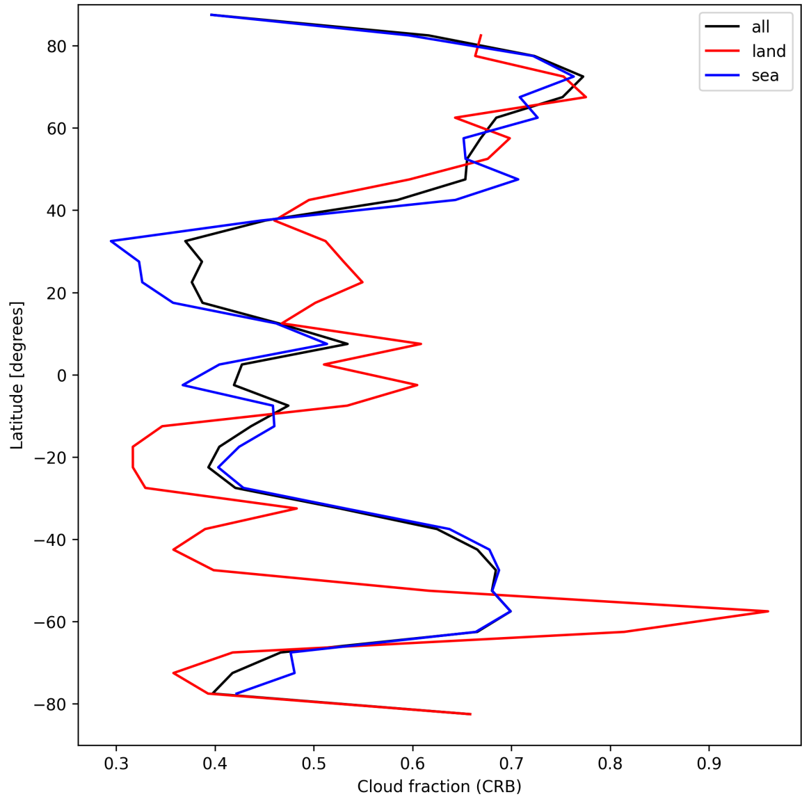
Figure 26: Zonal average of “Cloud fraction (CRB)” for 2025-09-10 to 2025-09-12.
