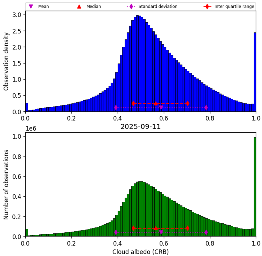
Figure 44: Histogram of “Cloud albedo (CRB)” for 2025-09-10 to 2025-09-12
