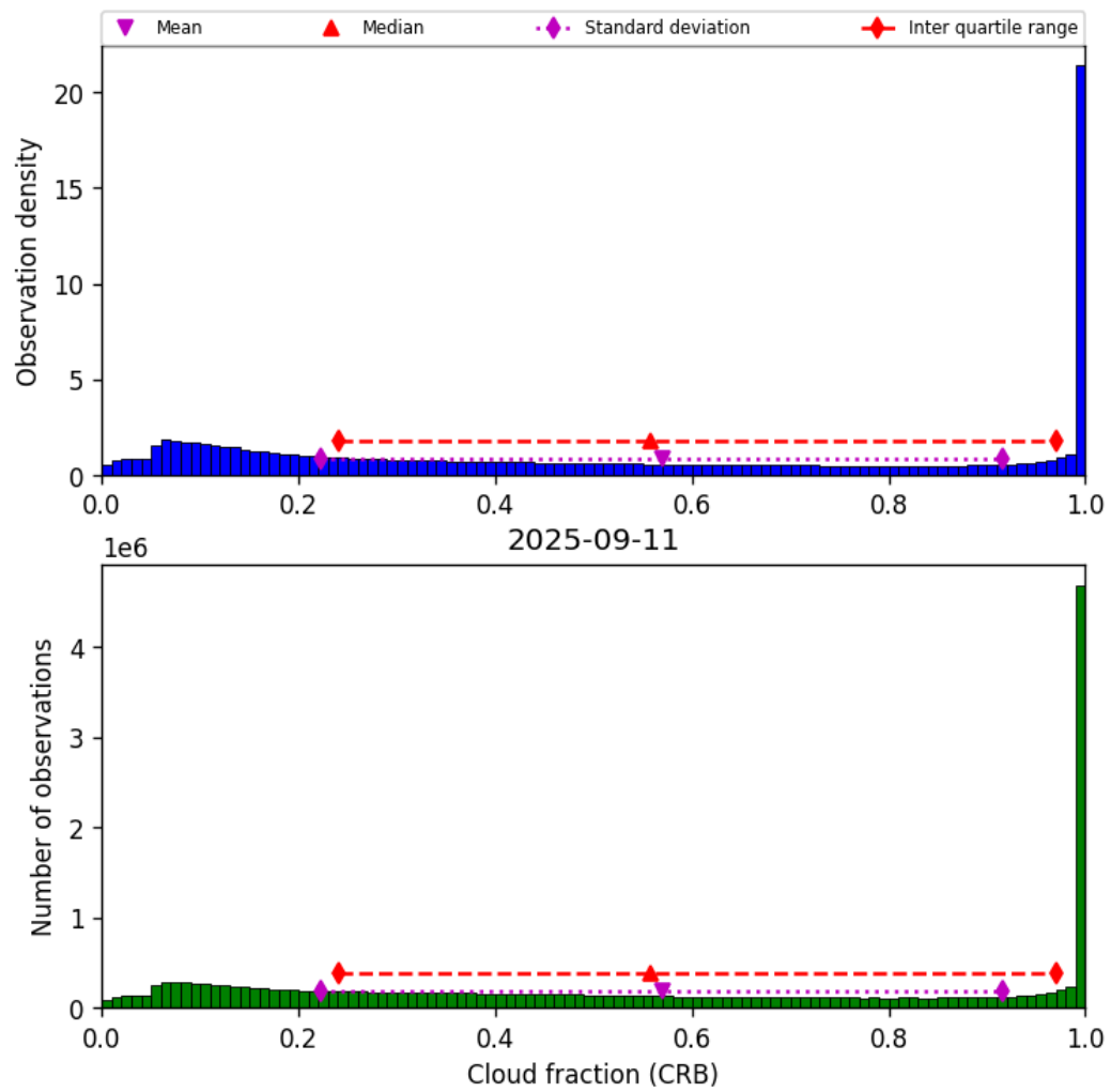
Figure 42: Histogram of “Cloud fraction (CRB)” for 2025-09-10 to 2025-09-12
