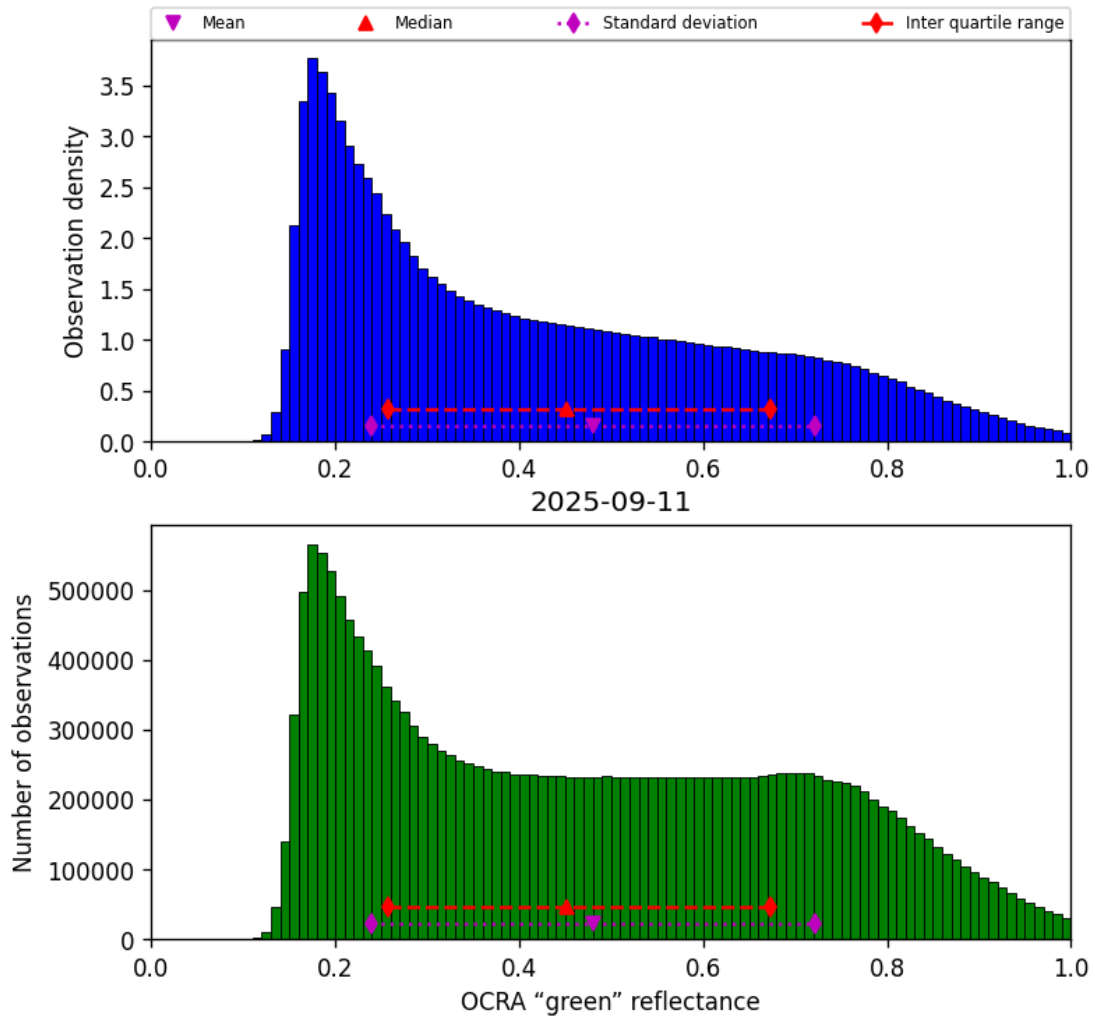
Figure 52: Histogram of “OCRA “green” reflectance” for 2025-09-10 to 2025-09-12
