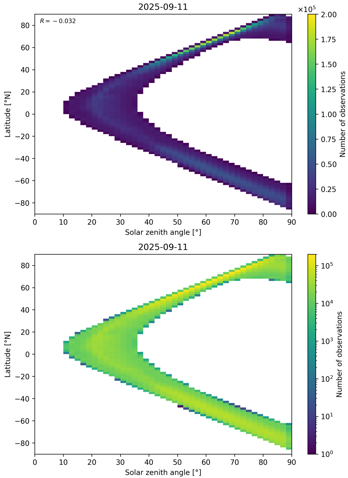
Figure 105: Scatter density plot of “Solar zenith angle” against “Latitude” for 2025-09-10 to 2025-09-12.
