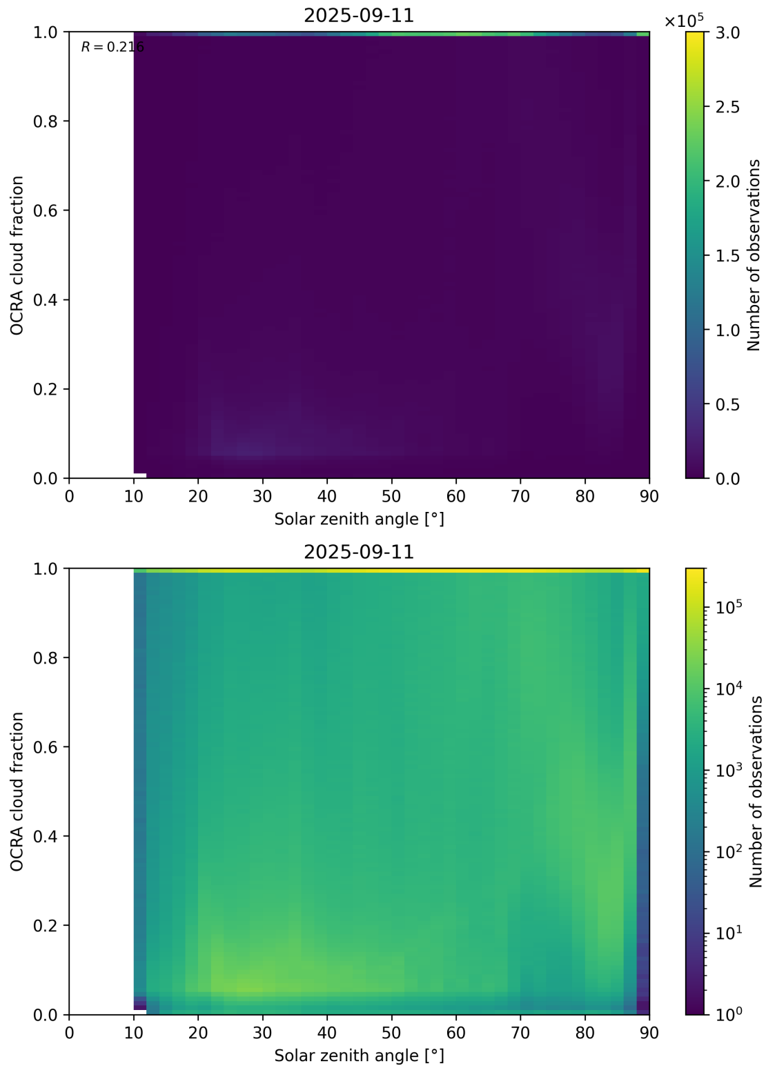
Figure 100: Scatter density plot of “Solar zenith angle” against “OCRA cloud fraction” for 2025-09-10 to 2025-09-12.
