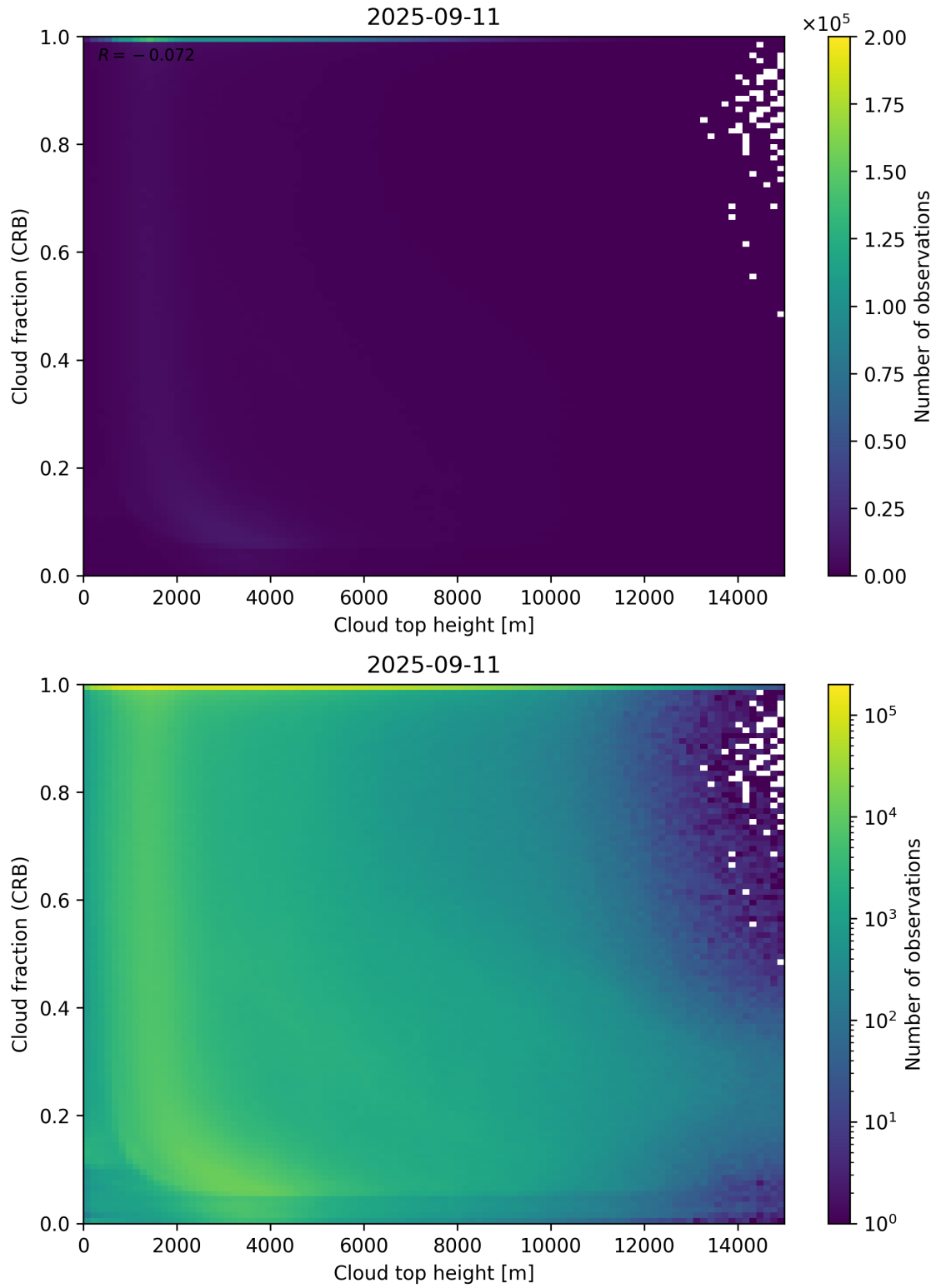
Figure 88: Scatter density plot of “Cloud top height” against “Cloud fraction (CRB)” for 2025-09-10 to 2025-09-12.
