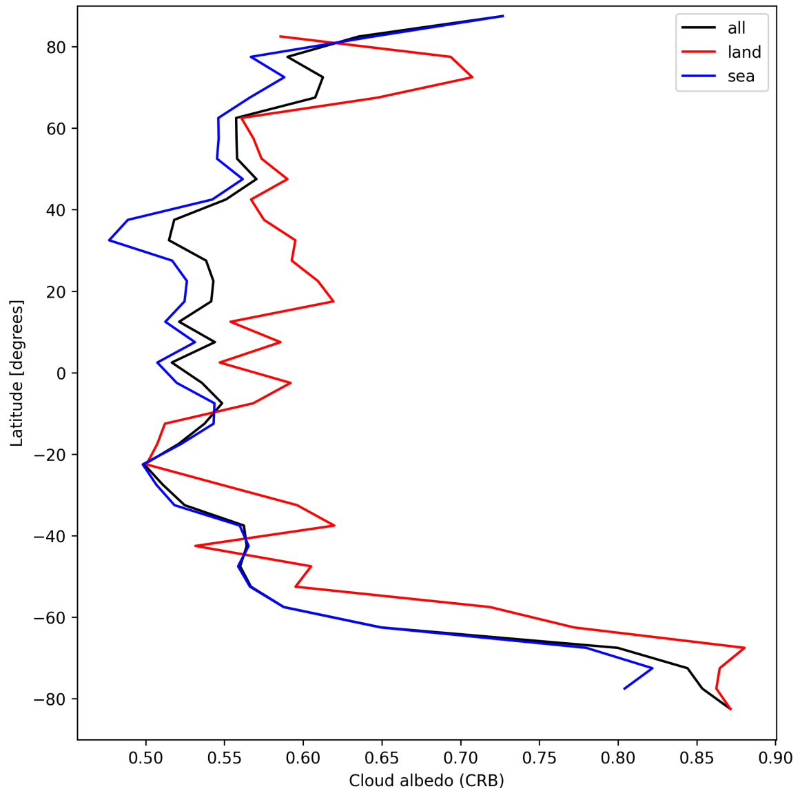
Figure 28: Zonal average of “Cloud albedo (CRB)” for 2025-09-10 to 2025-09-12.
