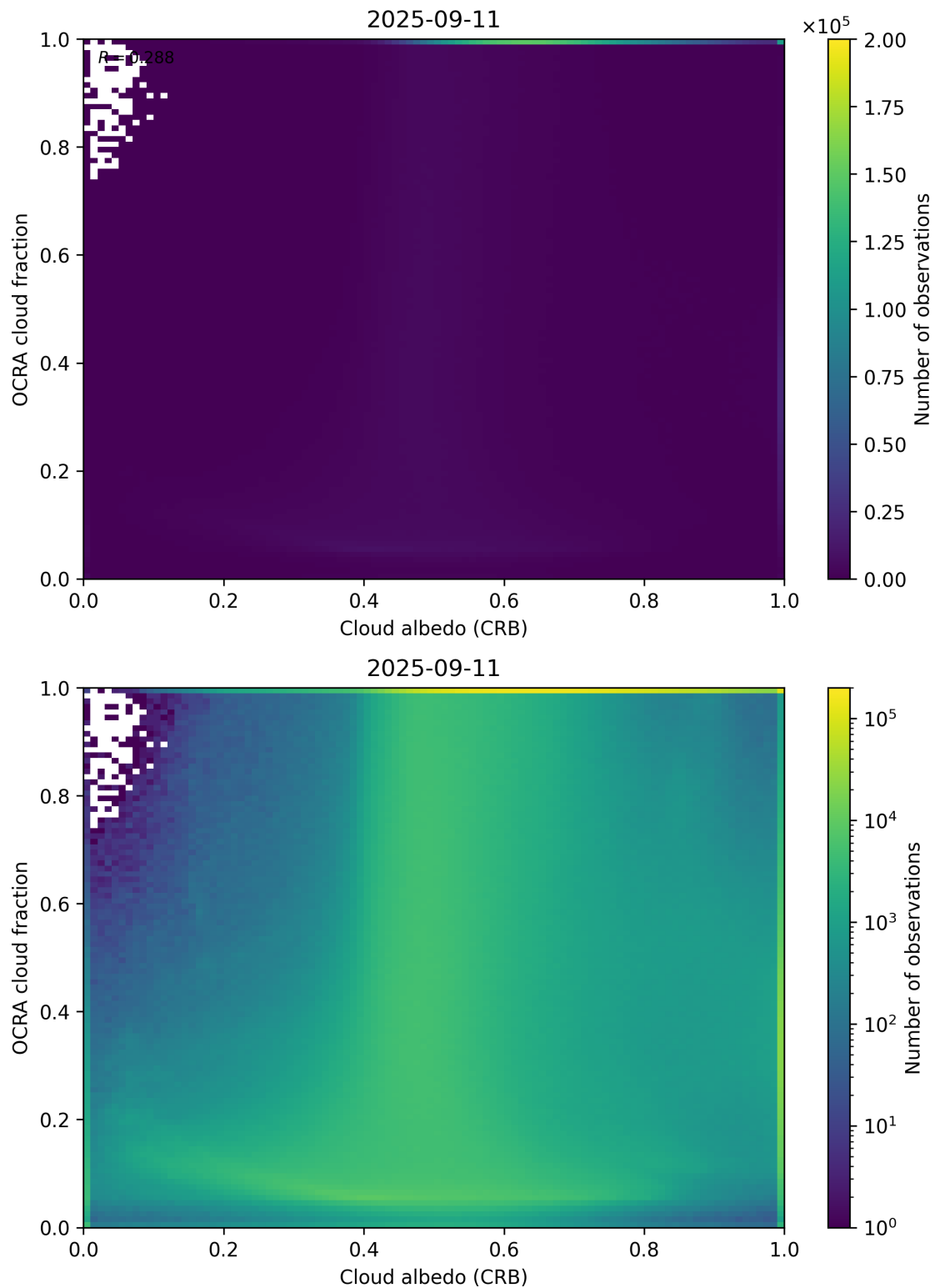
Figure 70: Scatter density plot of “Cloud albedo (CRB)” against “OCRA cloud fraction” for 2025-09-10 to 2025-09-12.
