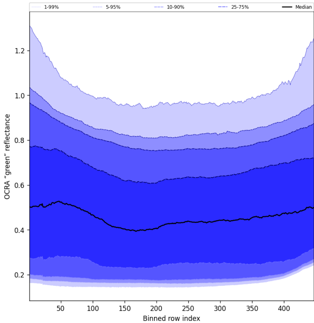
Figure 68: Along track statistics of "OCRA "green" reflectance" for 2025-09-10 to 2025-09-12
