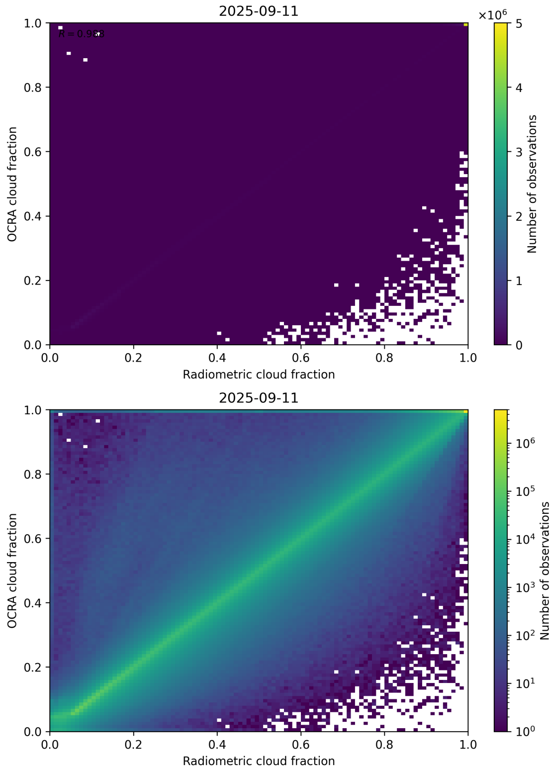
Figure 72: Scatter density plot of “Radiometric cloud fraction” against “OCRA cloud fraction” for 2025-09-10 to 2025-09-12.
