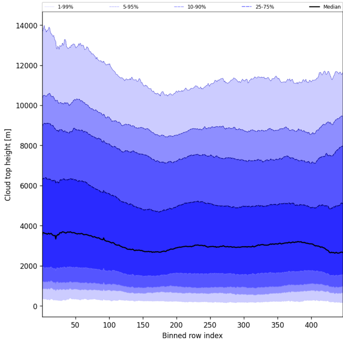
Figure 56: Along track statistics of “Cloud top height” for 2025-09-10 to 2025-09-12
