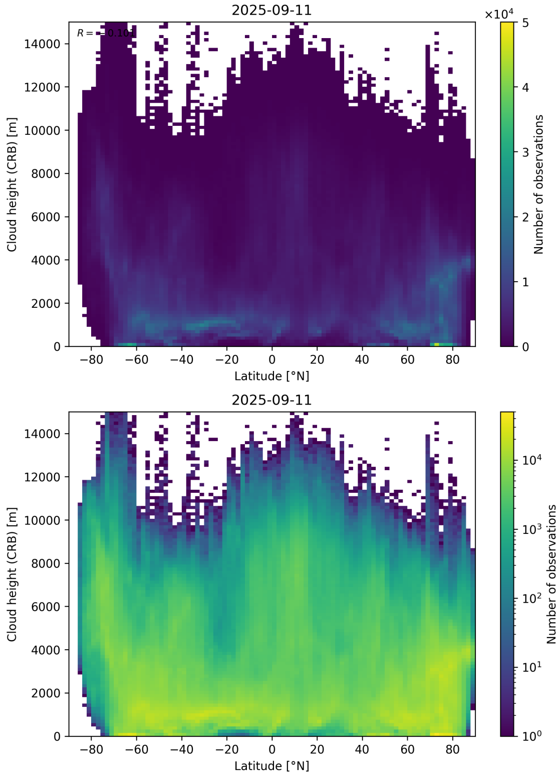
Figure 95: Scatter density plot of “Latitude” against “Cloud height (CRB)” for 2025-09-10 to 2025-09-12.
