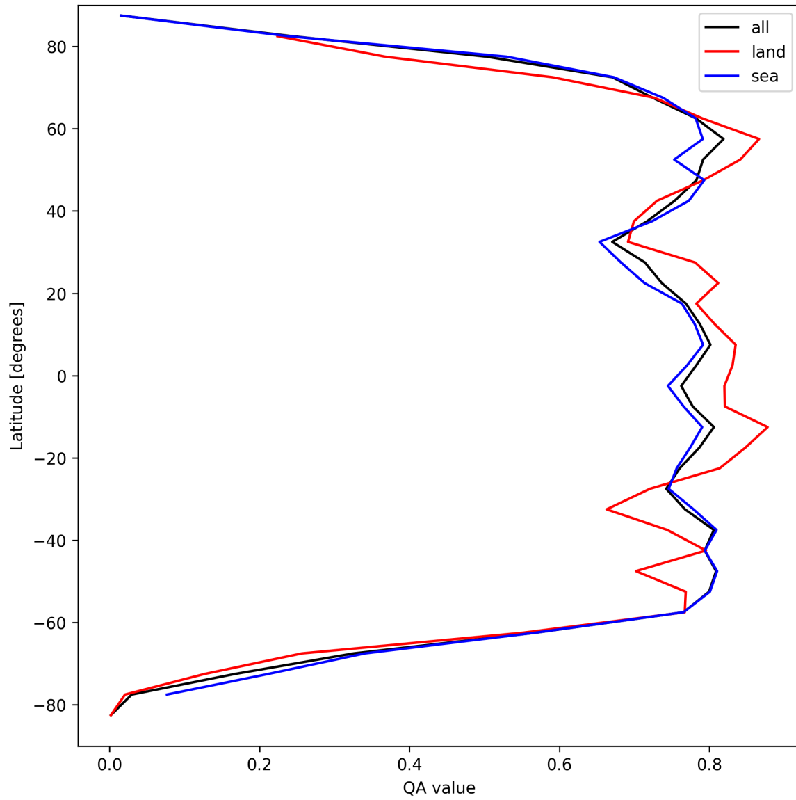
Figure 22: Zonal average of “QA value” for 2025-09-10 to 2025-09-12.
