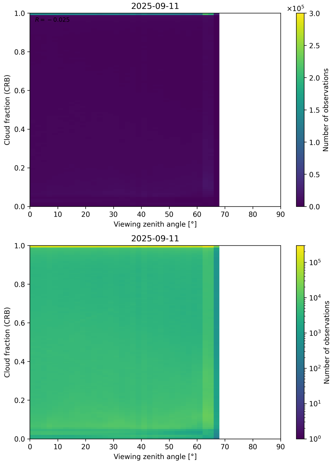
Figure 109: Scatter density plot of “Viewing zenith angle” against “Cloud fraction (CRB)” for 2025-09-10 to 2025-09-12.
