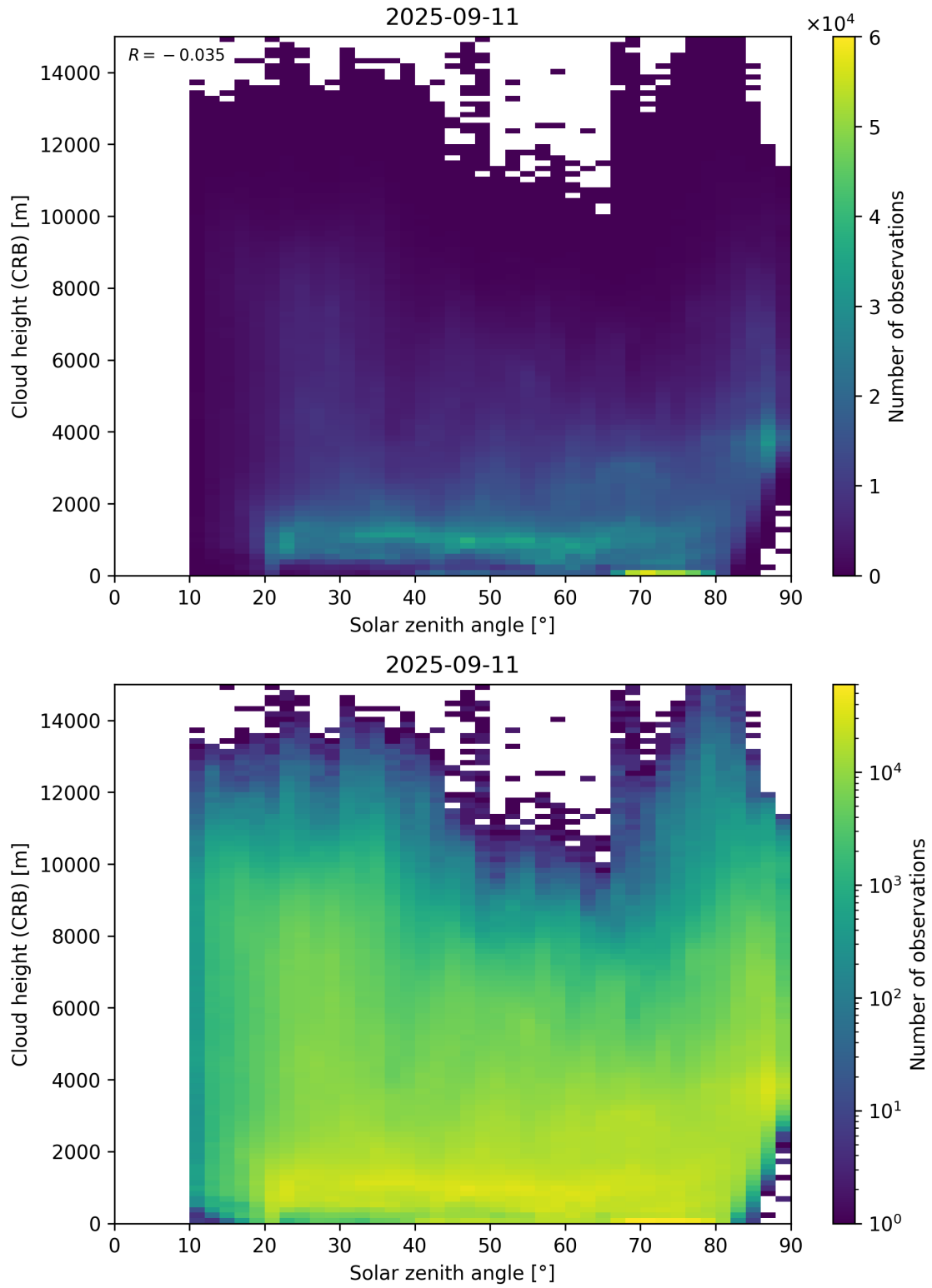
Figure 102: Scatter density plot of “Solar zenith angle” against “Cloud height (CRB)” for 2025-09-10 to 2025-09-12.
