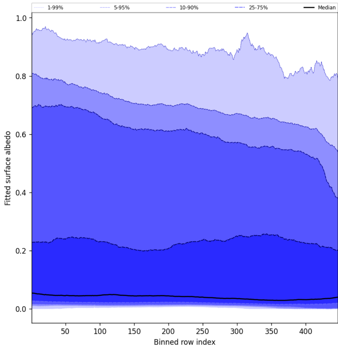
Figure 61: Along track statistics of “Fitted surface albedo” for 2025-09-10 to 2025-09-12
