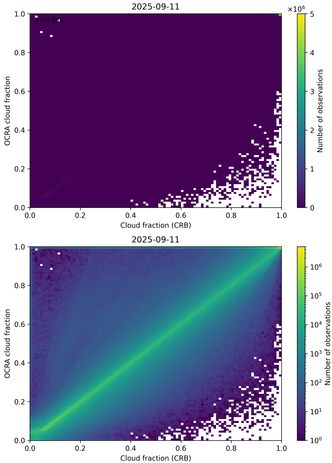
Figure 78: Scatter density plot of “Cloud fraction (CRB)” against “OCRA cloud fraction” for 2025-09-10 to 2025-09-12.
