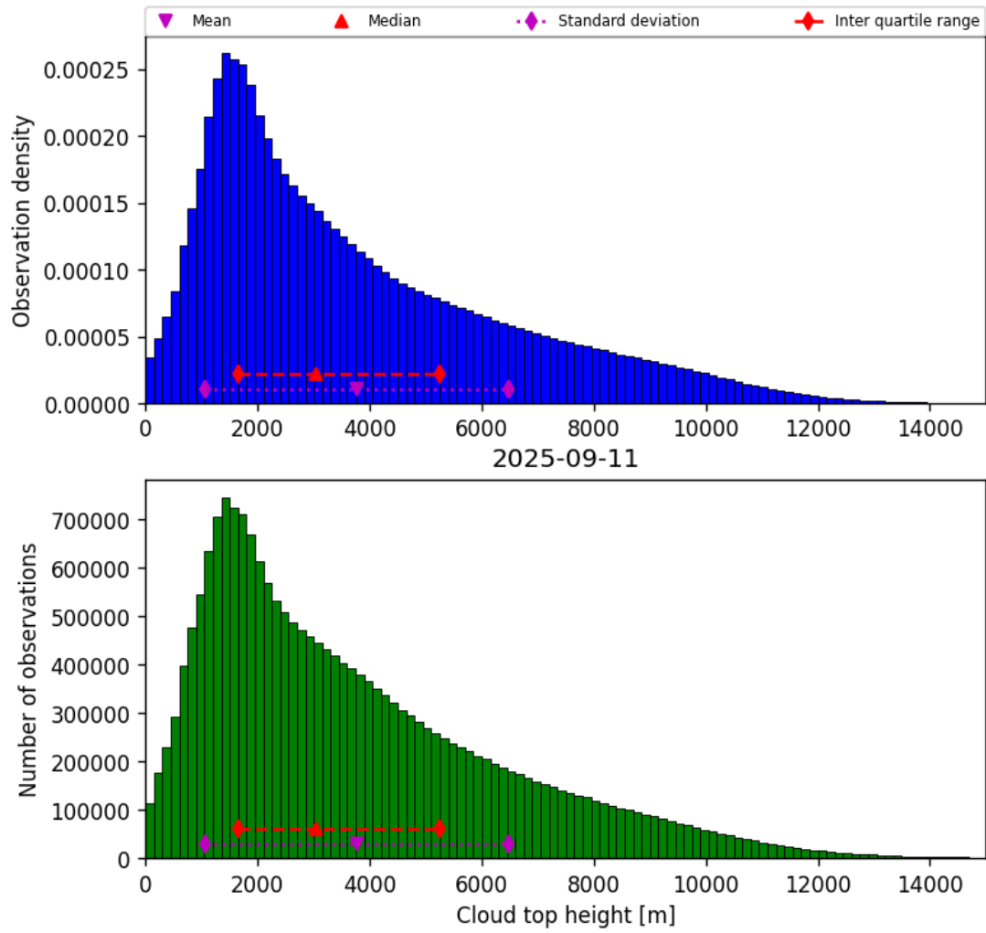
Figure 40: Histogram of “Cloud top height” for 2025-09-10 to 2025-09-12
