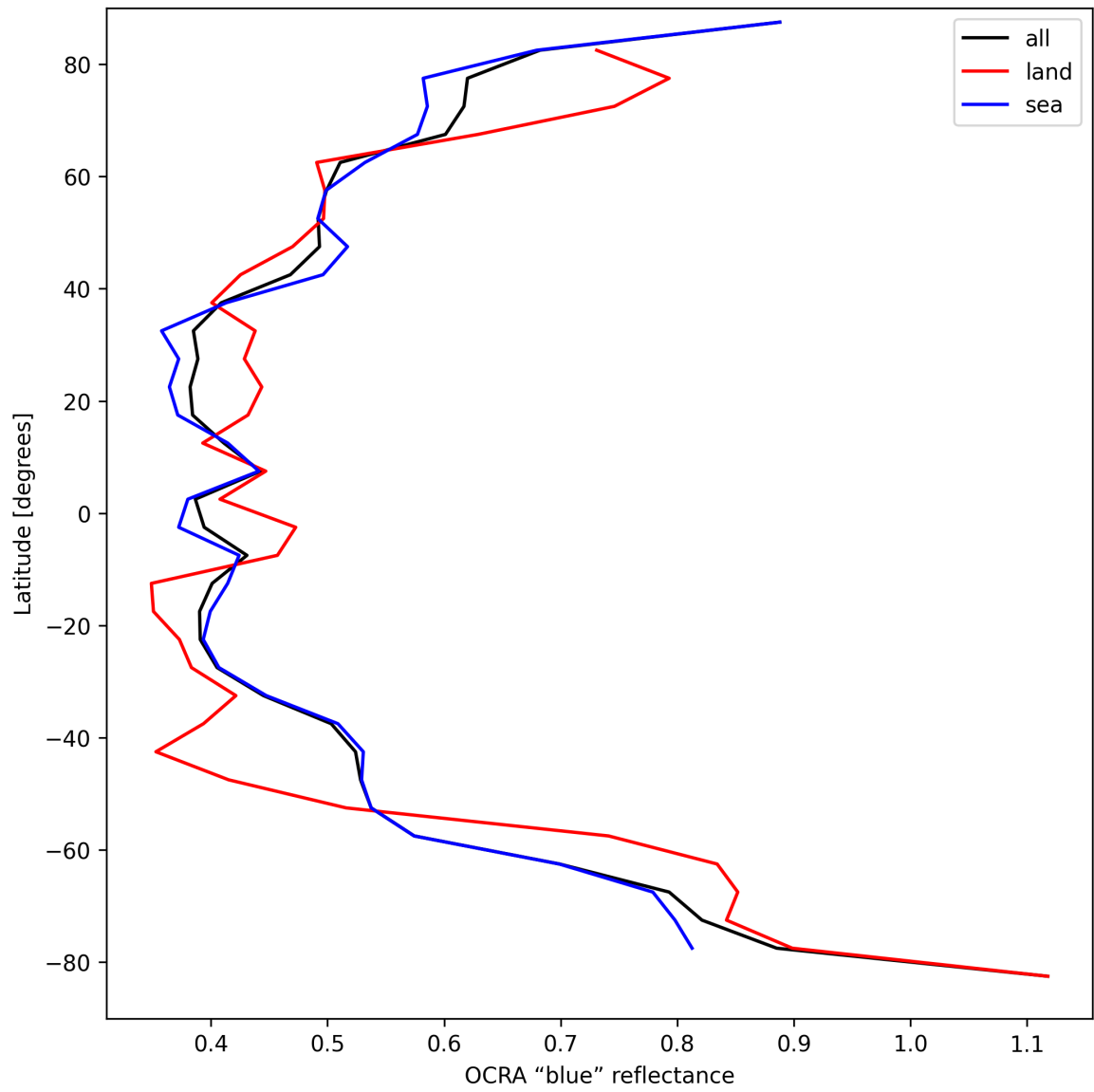
Figure 35: Zonal average of “OCRA “blue” reflectance” for 2025-09-10 to 2025-09-12.
