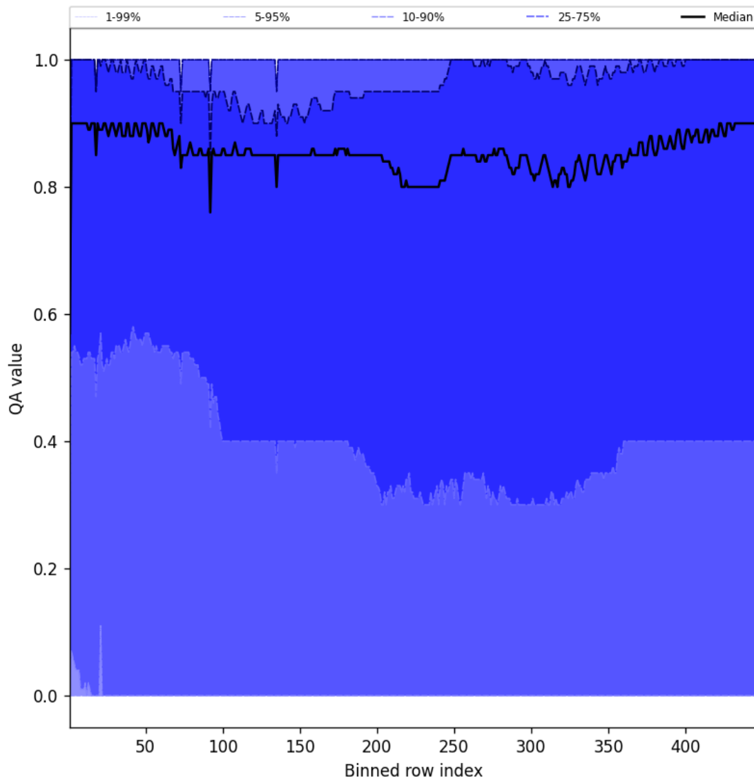
Figure 54: Along track statistics of “QA value” for 2025-09-10 to 2025-09-12
