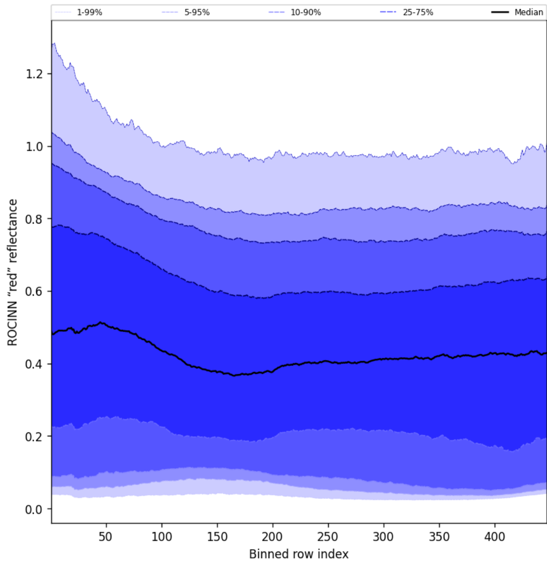
Figure 69: Along track statistics of “ROCINN “red” reflectance” for 2025-09-10 to 2025-09-12
