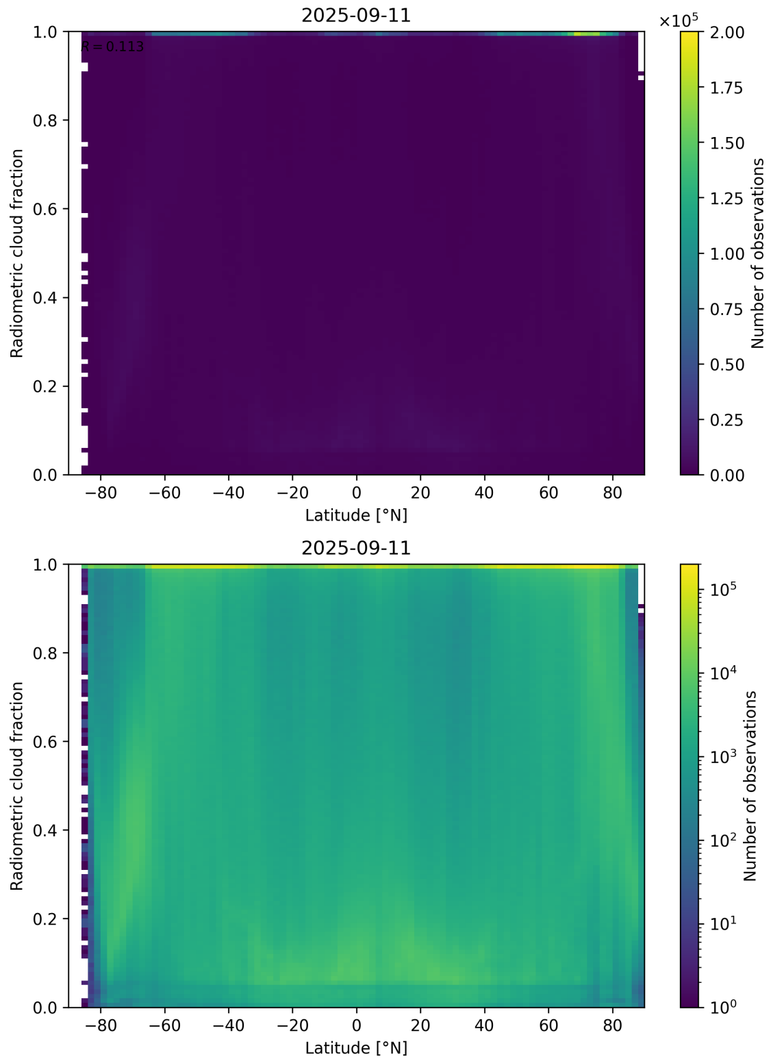
Figure 92: Scatter density plot of “Latitude” against “Radiometric cloud fraction” for 2025-09-10 to 2025-09-12.
