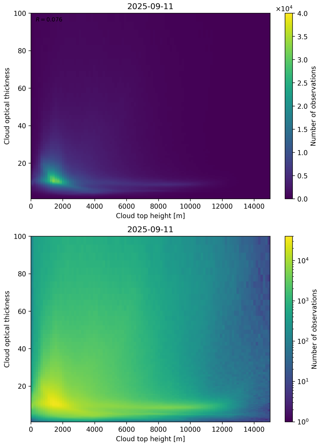
Figure 90: Scatter density plot of “Cloud top height” against “Cloud optical thickness” for 2025-09-10 to 2025-09-12.
