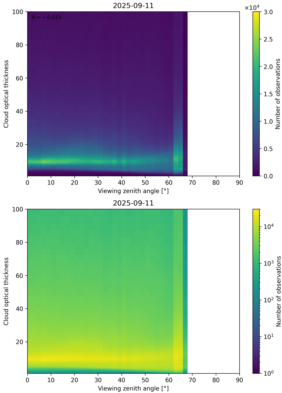
Figure 111: Scatter density plot of “Viewing zenith angle” against “Cloud optical thickness” for 2025-09-10 to 2025-09-12.
