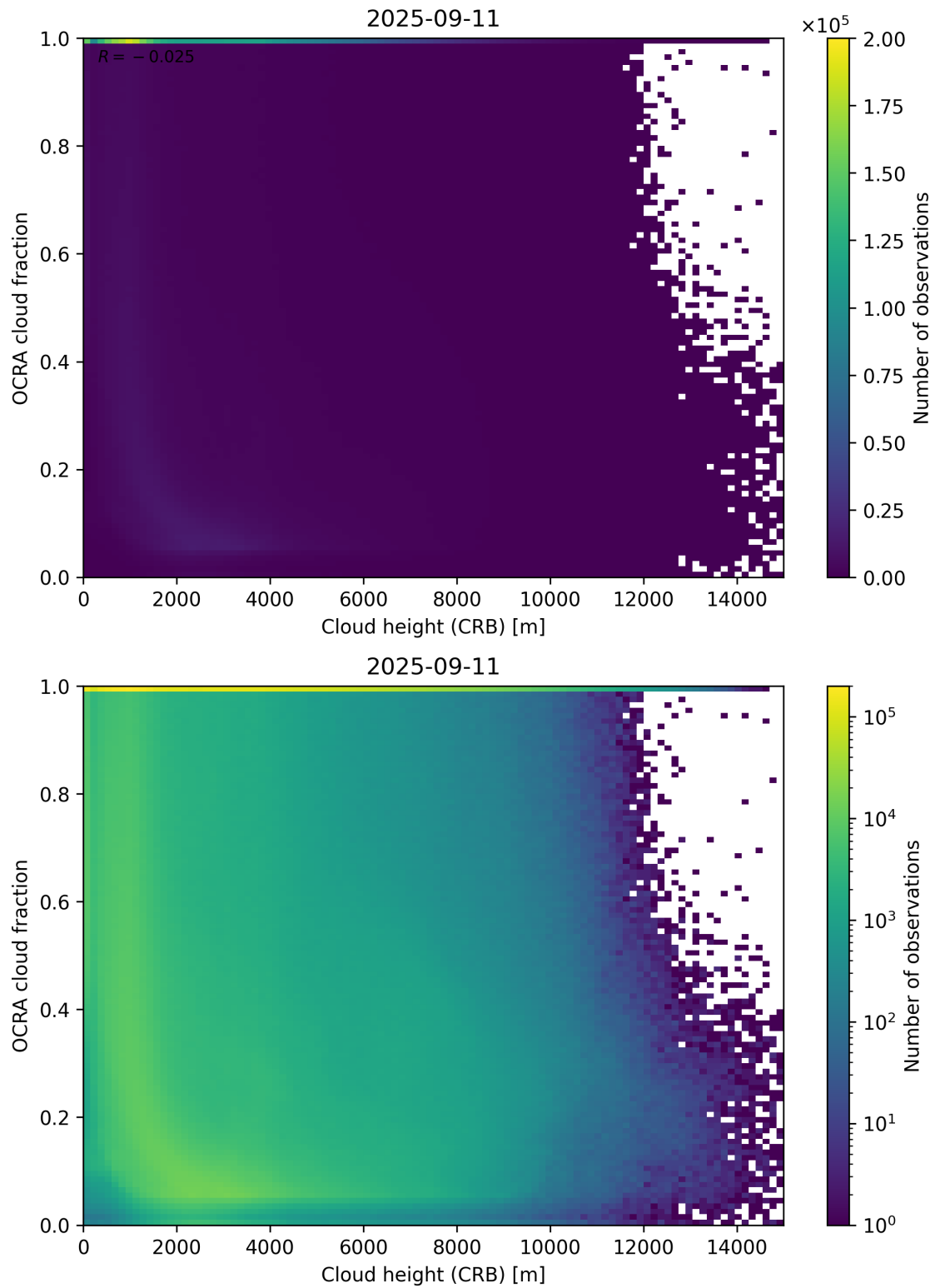
Figure 81: Scatter density plot of “Cloud height (CRB)” against “OCRA cloud fraction” for 2025-09-10 to 2025-09-12.
