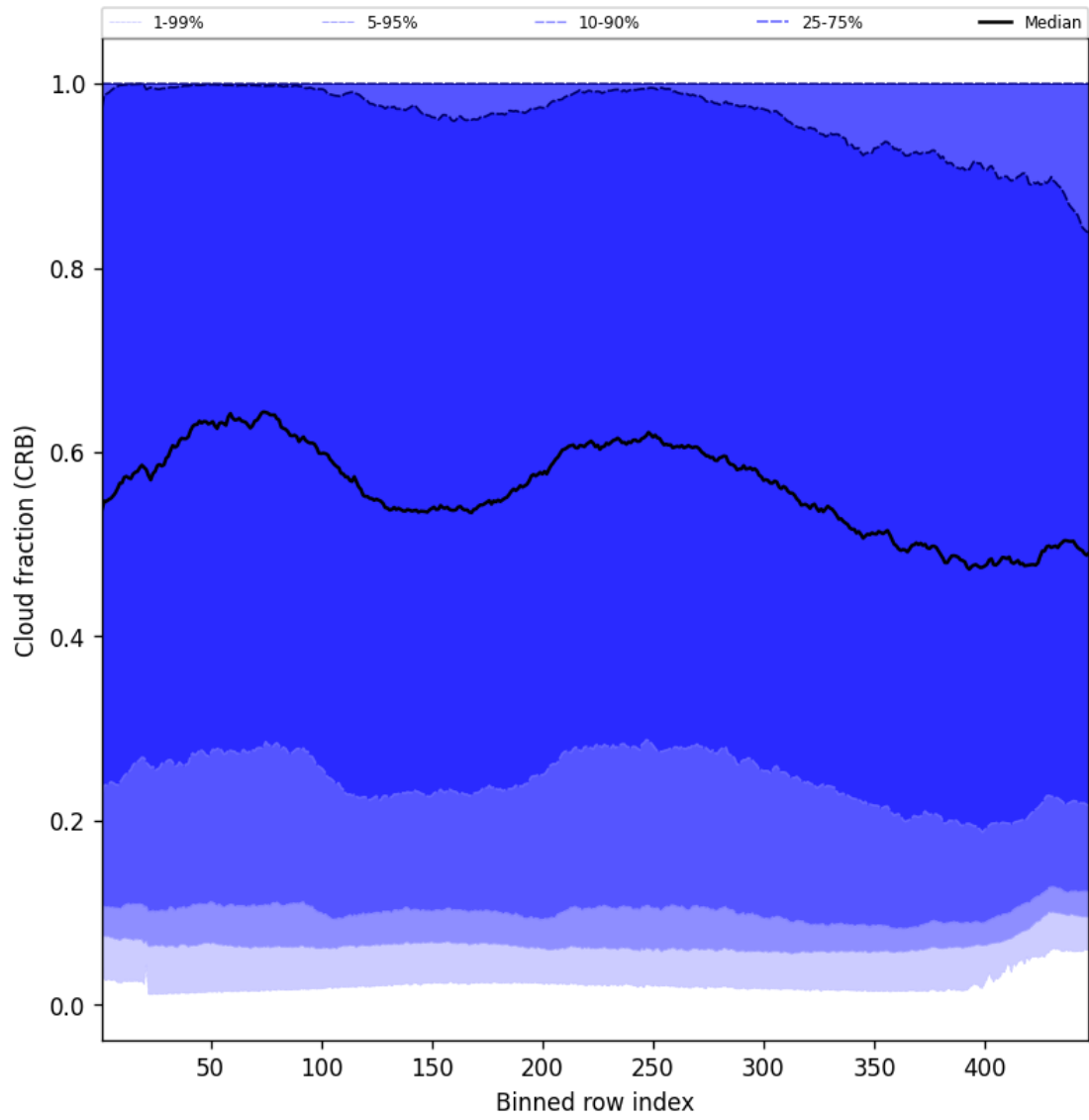
Figure 58: Along track statistics of “Cloud fraction (CRB)” for 2025-09-10 to 2025-09-12
