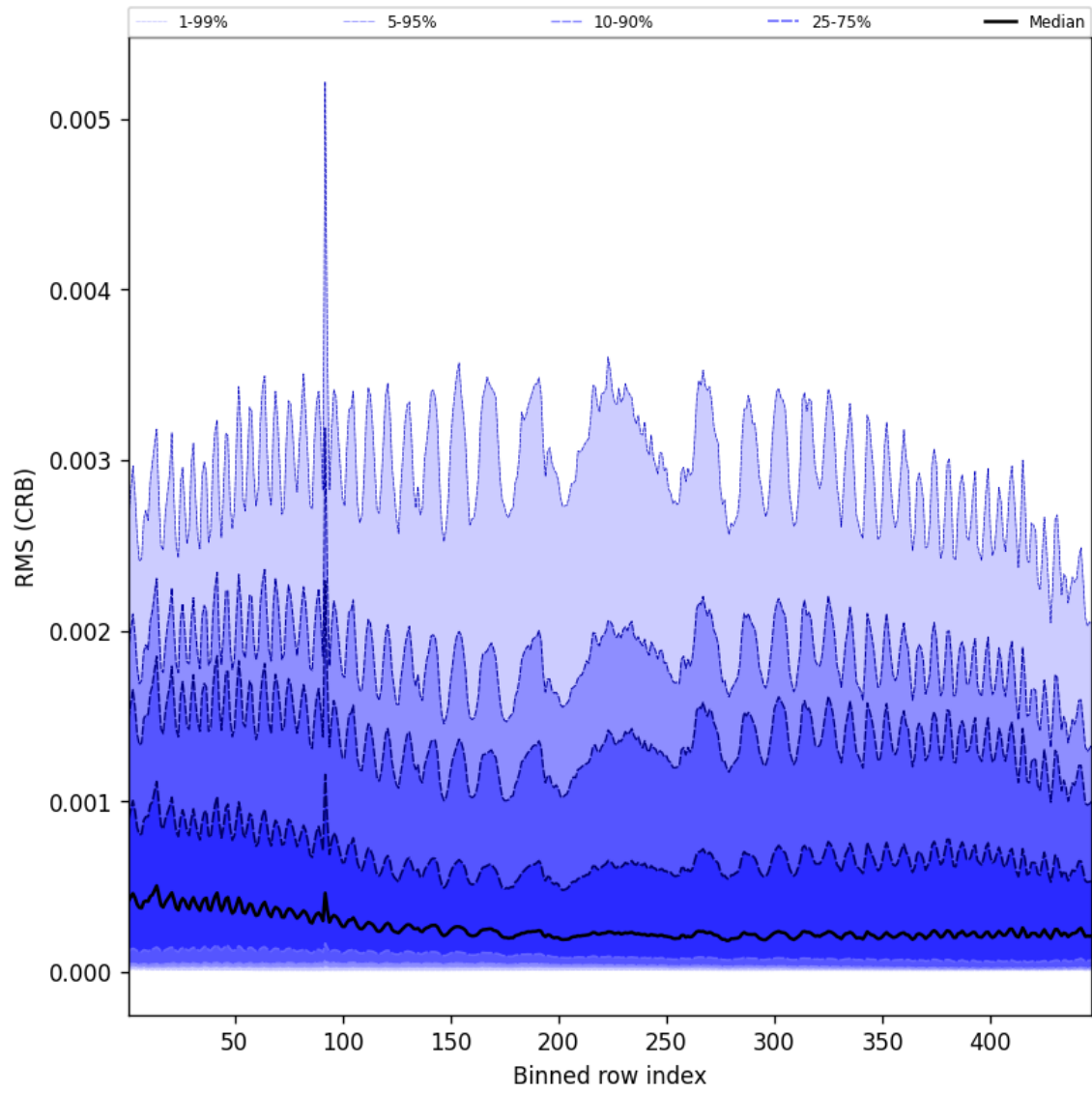
Figure 64: Along track statistics of “RMS (CRB)” for 2025-09-10 to 2025-09-12
