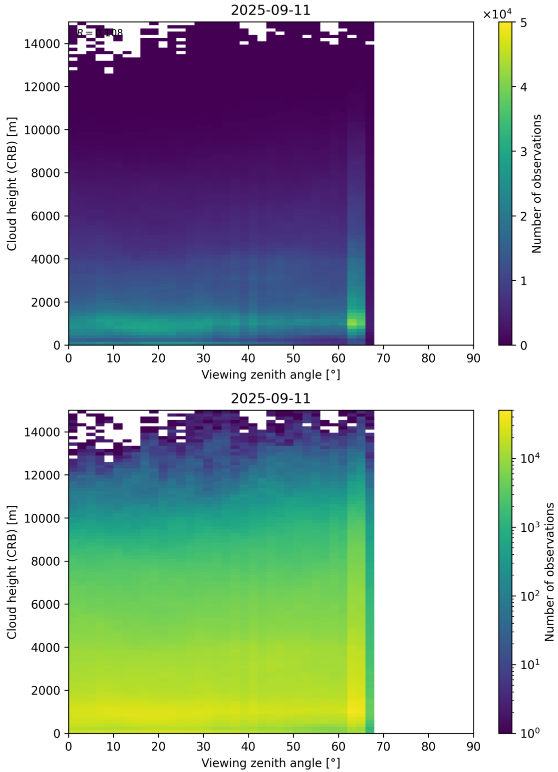
Figure 110: Scatter density plot of “Viewing zenith angle” against “Cloud height (CRB)” for 2025-09-10 to 2025-09-12.
