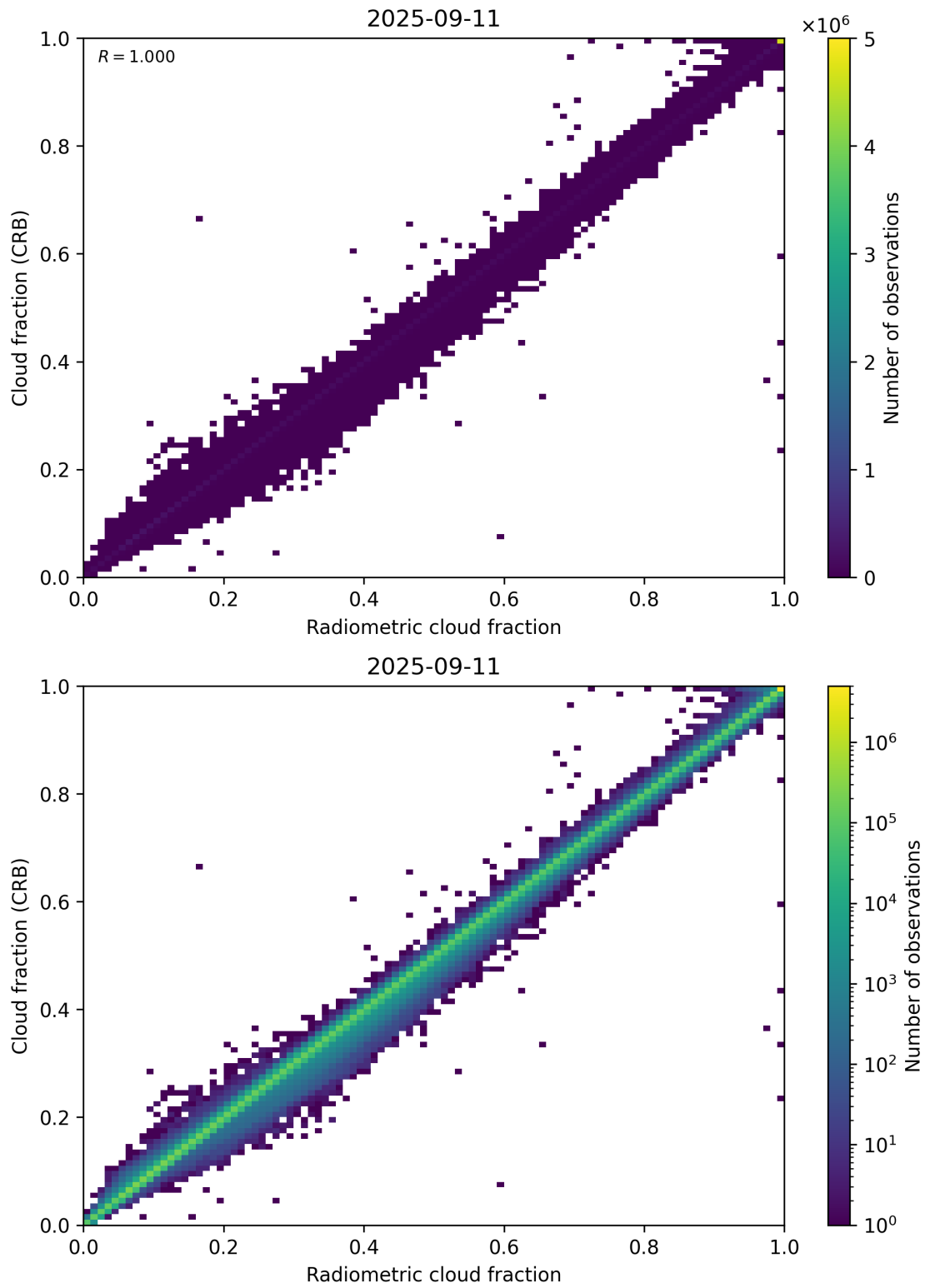
Figure 73: Scatter density plot of “Radiometric cloud fraction” against “Cloud fraction (CRB)” for 2025-09-10 to 2025-09-12.
