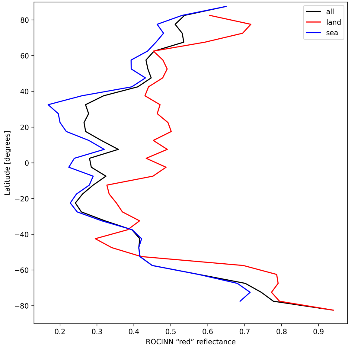
Figure 37: Zonal average of “ROCINN “red” reflectance” for 2025-09-10 to 2025-09-12.
