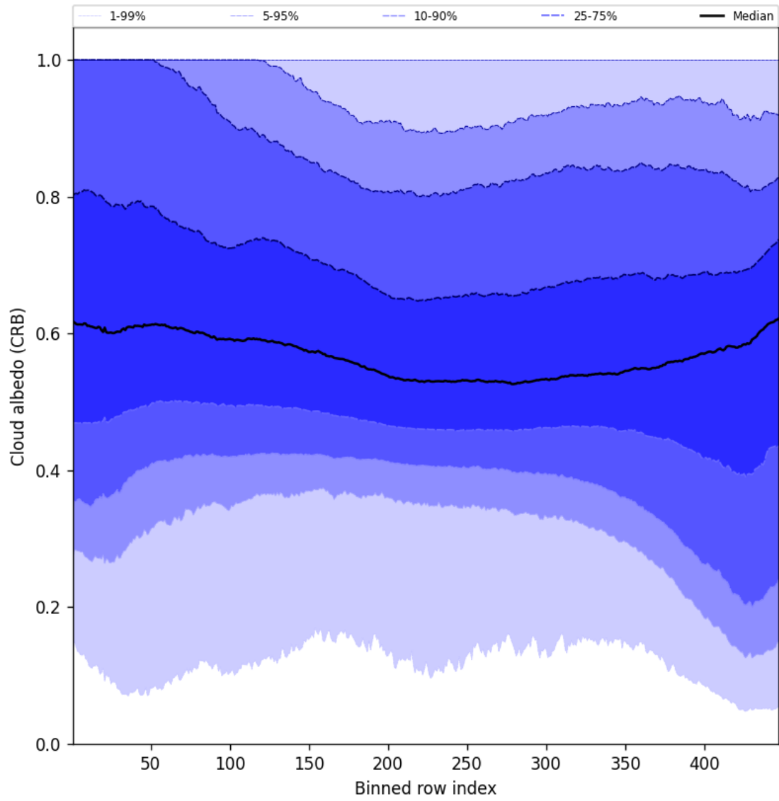
Figure 60: Along track statistics of “Cloud albedo (CRB)” for 2025-09-10 to 2025-09-12
