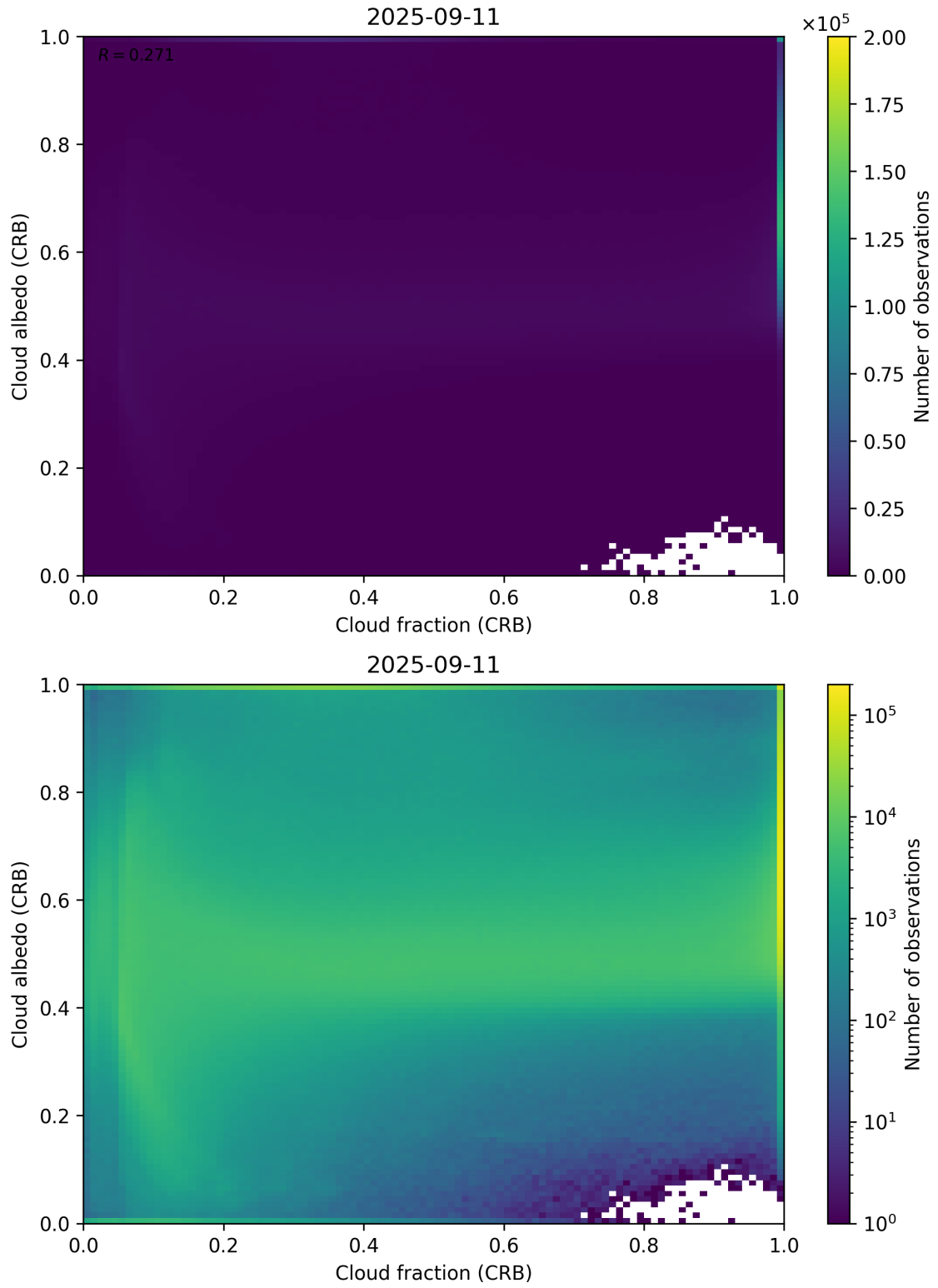
Figure 77: Scatter density plot of “Cloud fraction (CRB)” against “Cloud albedo (CRB)” for 2025-09-10 to 2025-09-12.
