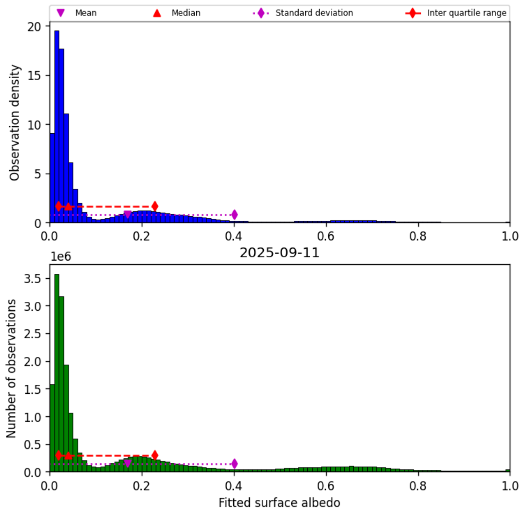
Figure 45: Histogram of “Fitted surface albedo” for 2025-09-10 to 2025-09-12
