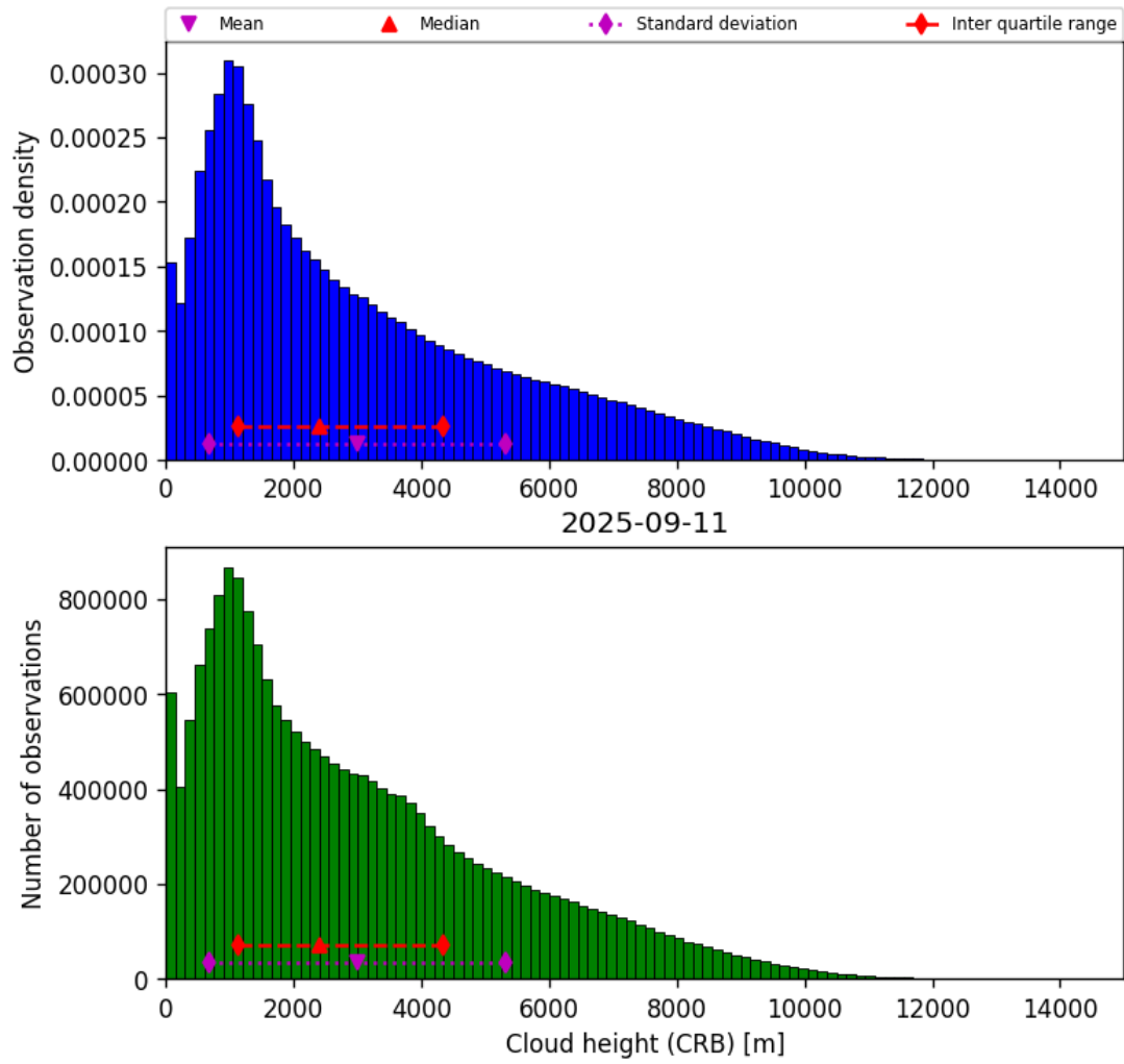
Figure 43: Histogram of “Cloud height (CRB)” for 2025-09-10 to 2025-09-12
