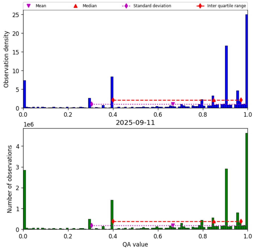
Figure 38: Histogram of “QA value” for 2025-09-10 to 2025-09-12
