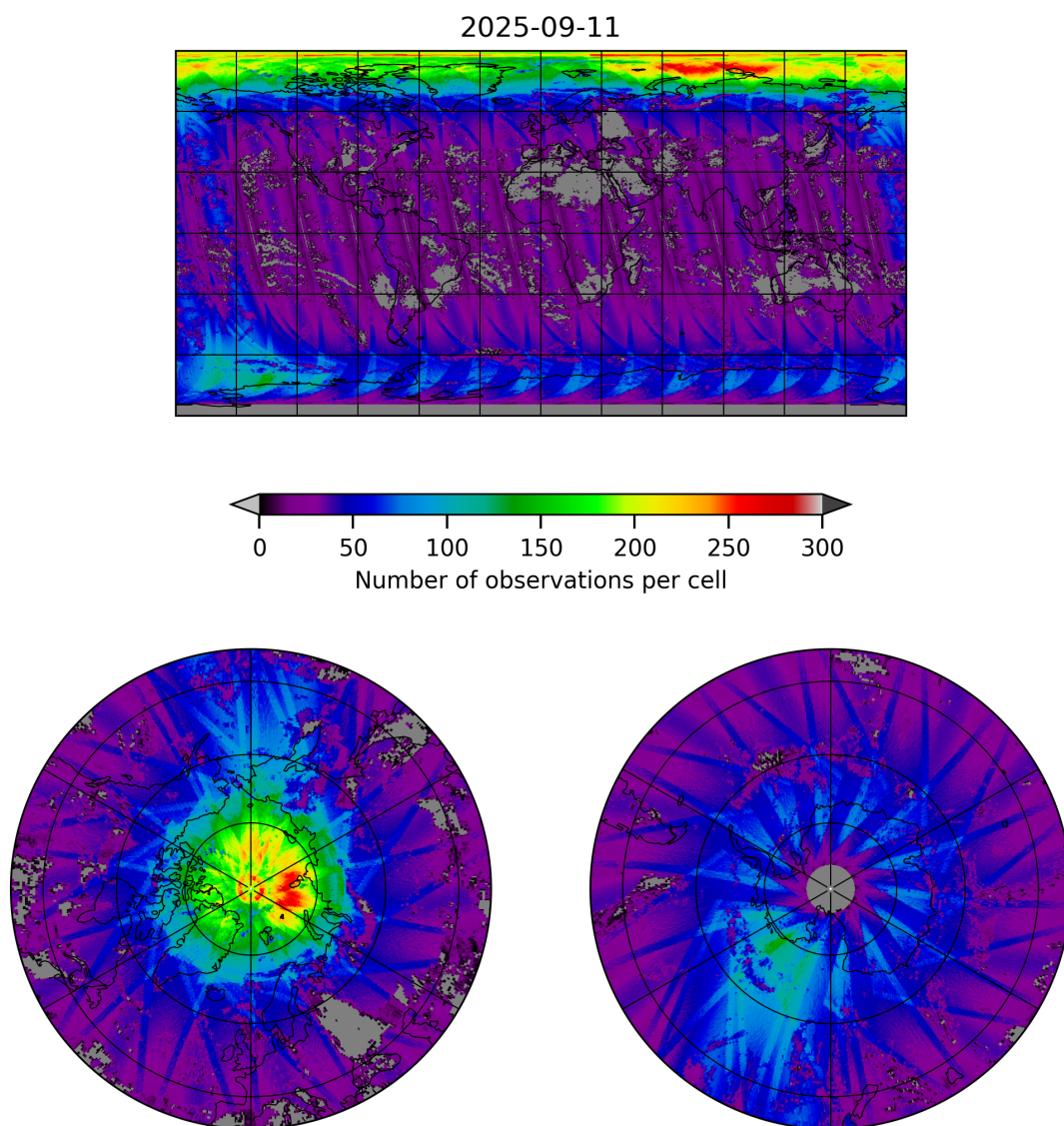
Figure 21: Map of the number of observations for 2025-09-10 to 2025-09-12
