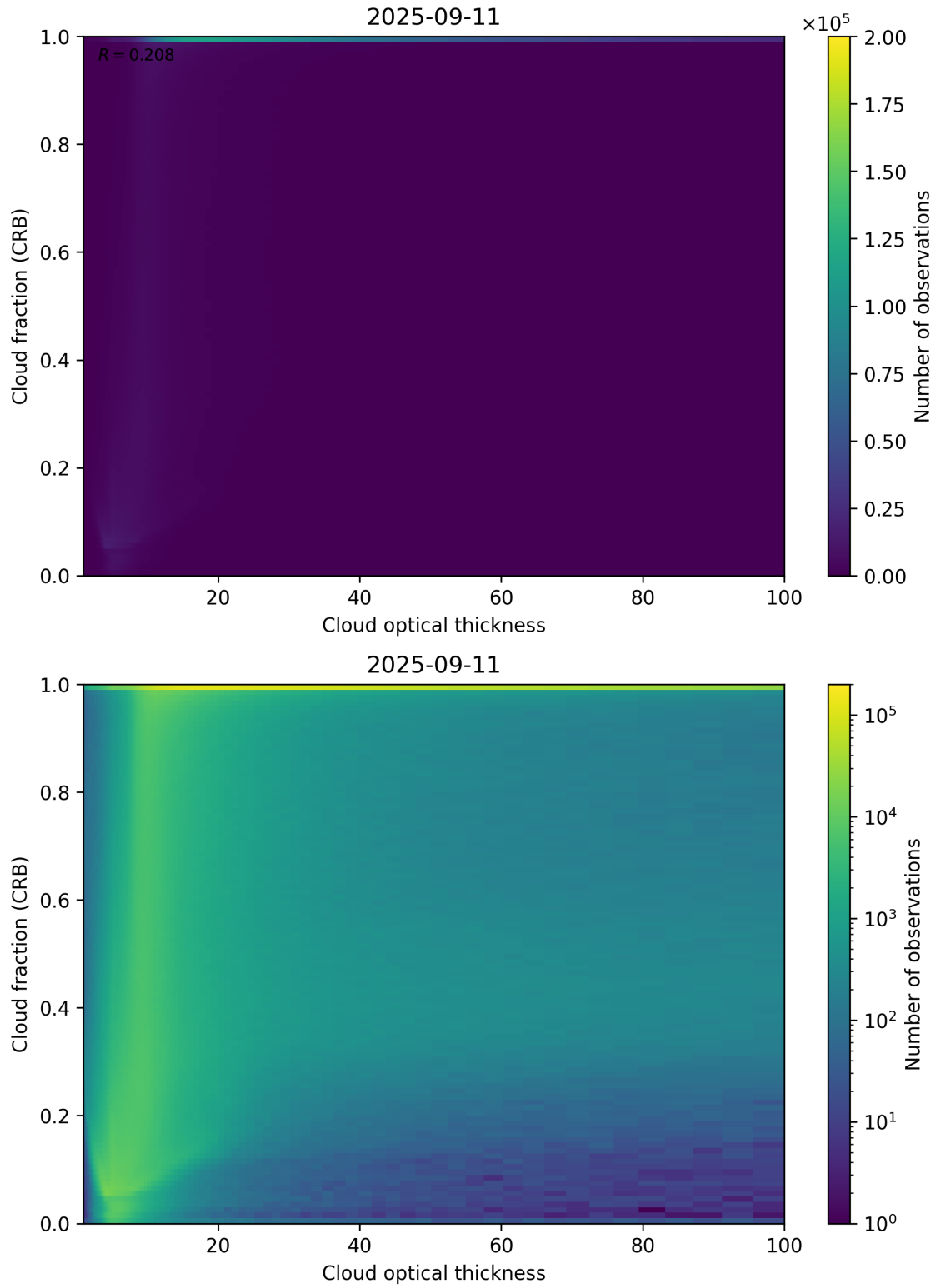
Figure 84: Scatter density plot of “Cloud optical thickness” against “Cloud fraction (CRB)” for 2025-09-10 to 2025-09-12.
