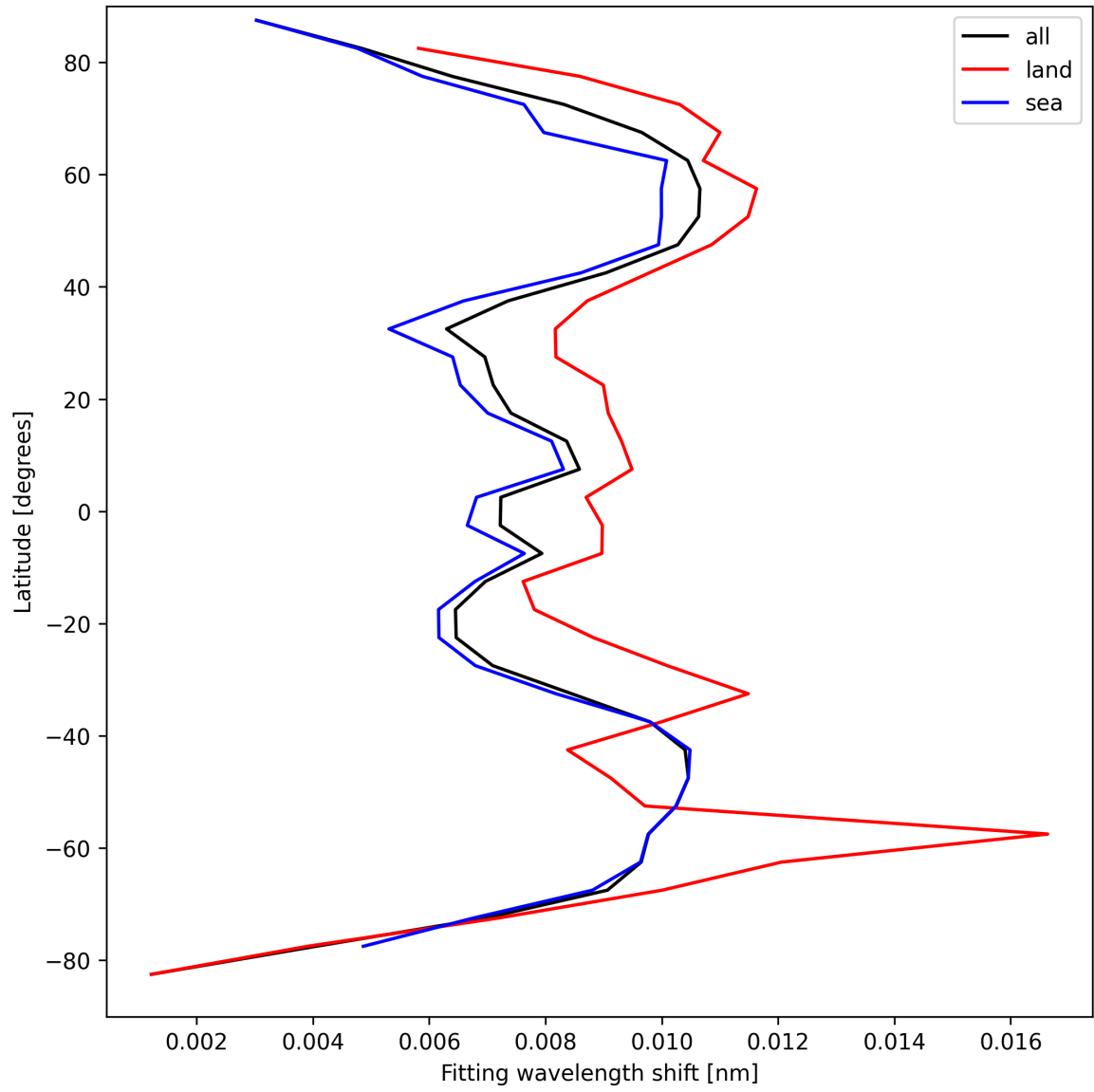
Figure 33: Zonal average of “Fitting wavelength shift” for 2025-09-10 to 2025-09-12.
