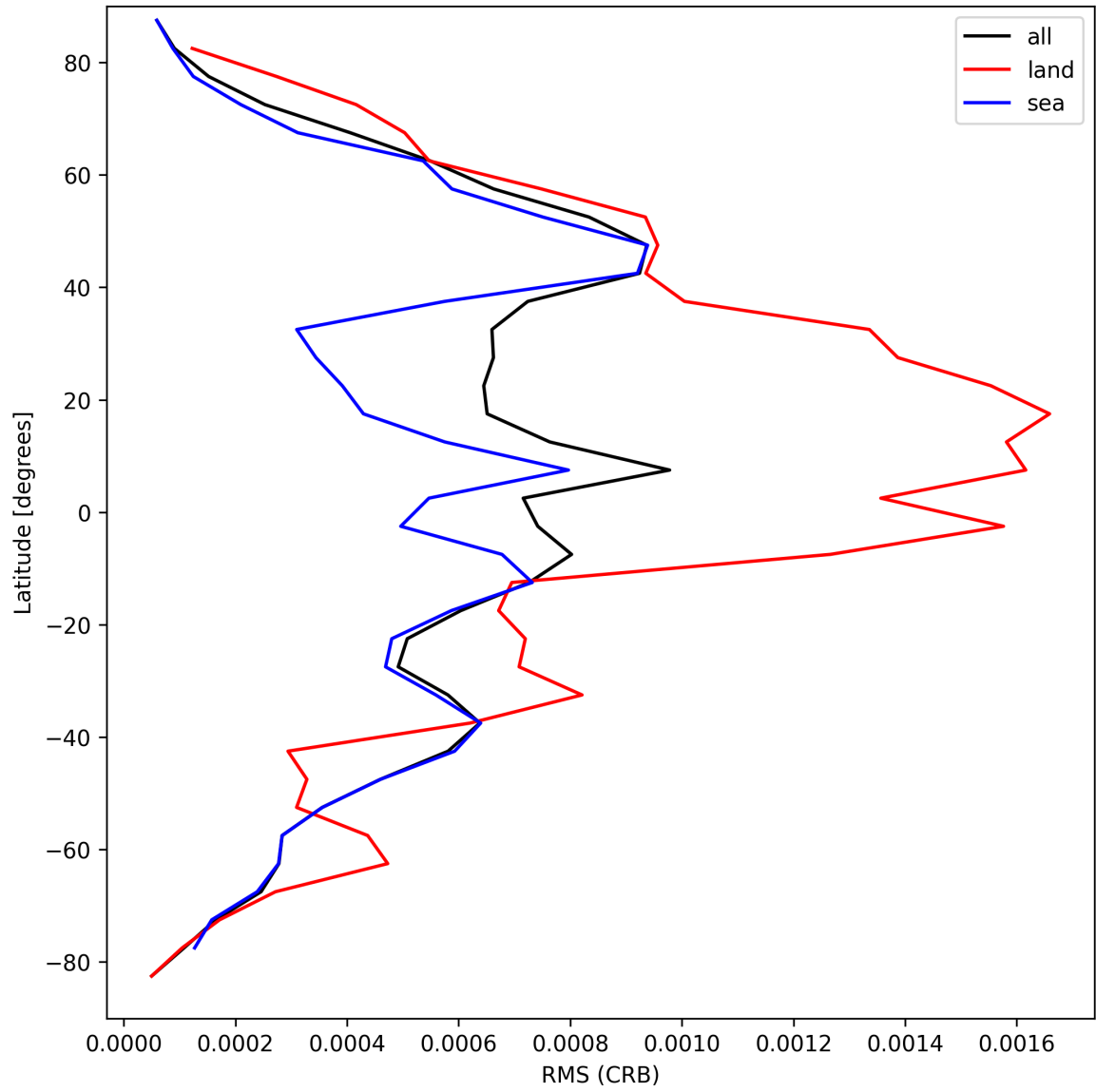
Figure 32: Zonal average of “RMS (CRB)” for 2025-09-10 to 2025-09-12.
