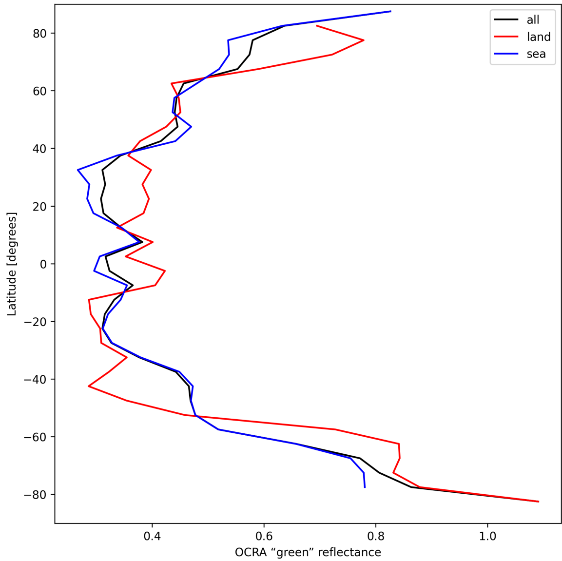
Figure 36: Zonal average of “OCRA “green” reflectance” for 2025-09-10 to 2025-09-12.
