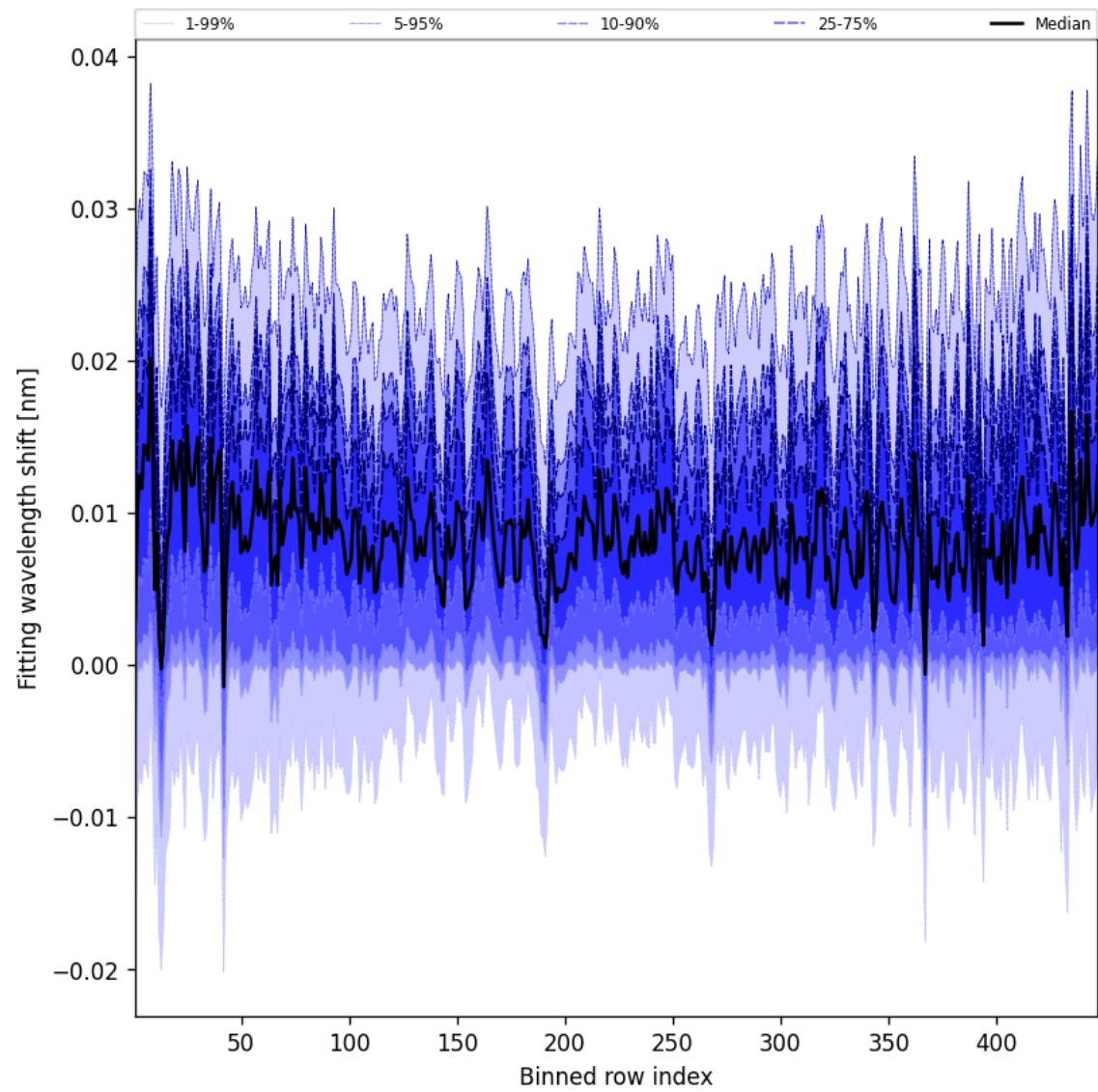
Figure 65: Along track statistics of “Fitting wavelength shift” for 2025-09-10 to 2025-09-12
