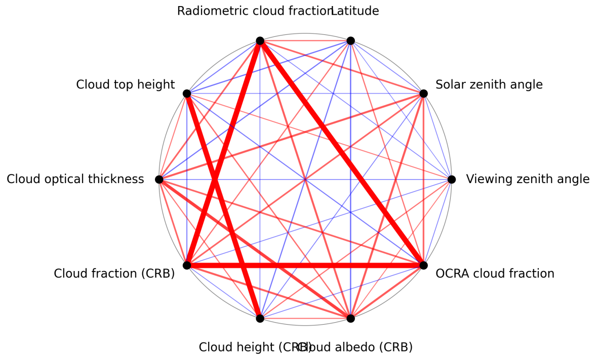
Figure 1: Map of correlation graph for 2025-09-10 to 2025-09-12.
