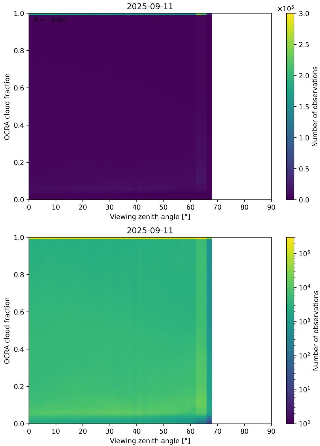
Figure 108: Scatter density plot of “Viewing zenith angle” against “OCRA cloud fraction” for 2025-09-10 to 2025-09-12.
