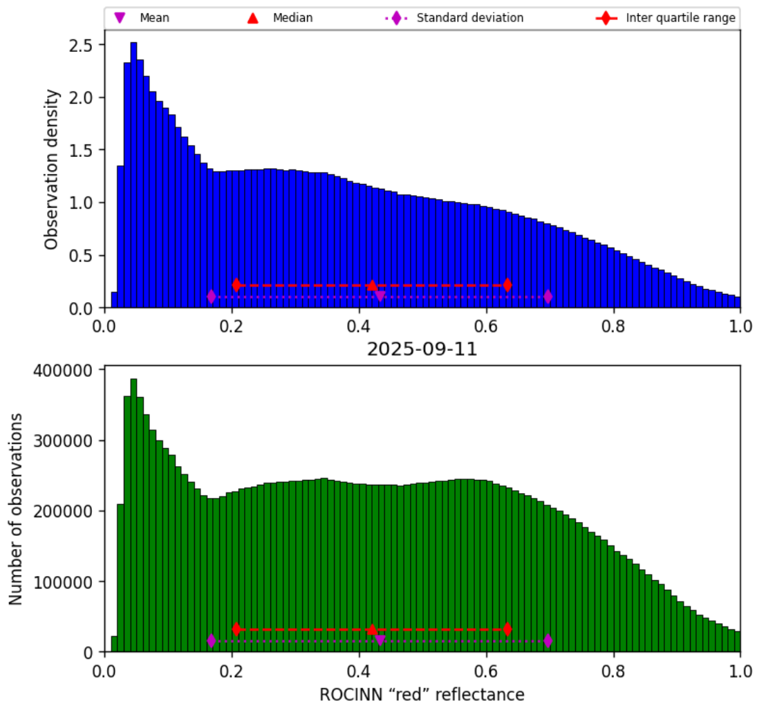
Figure 53: Histogram of “ROCINN “red” reflectance” for 2025-09-10 to 2025-09-12
