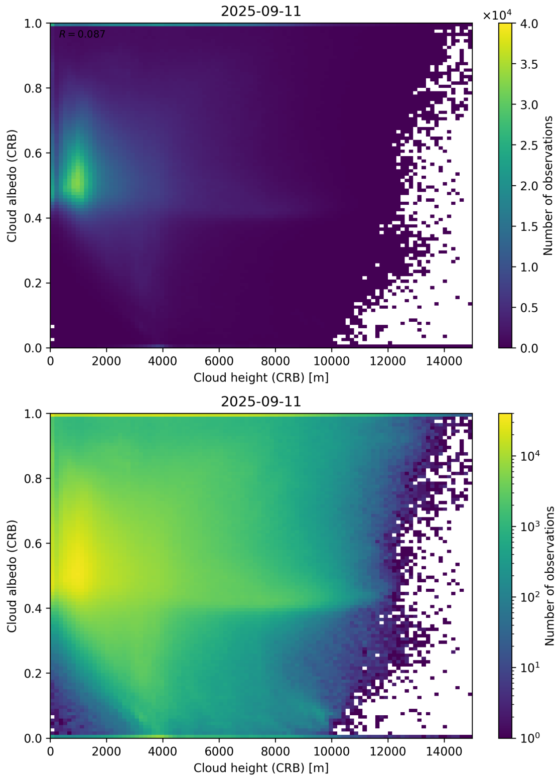
Figure 80: Scatter density plot of “Cloud height (CRB)” against “Cloud albedo (CRB)” for 2025-09-10 to 2025-09-12.
