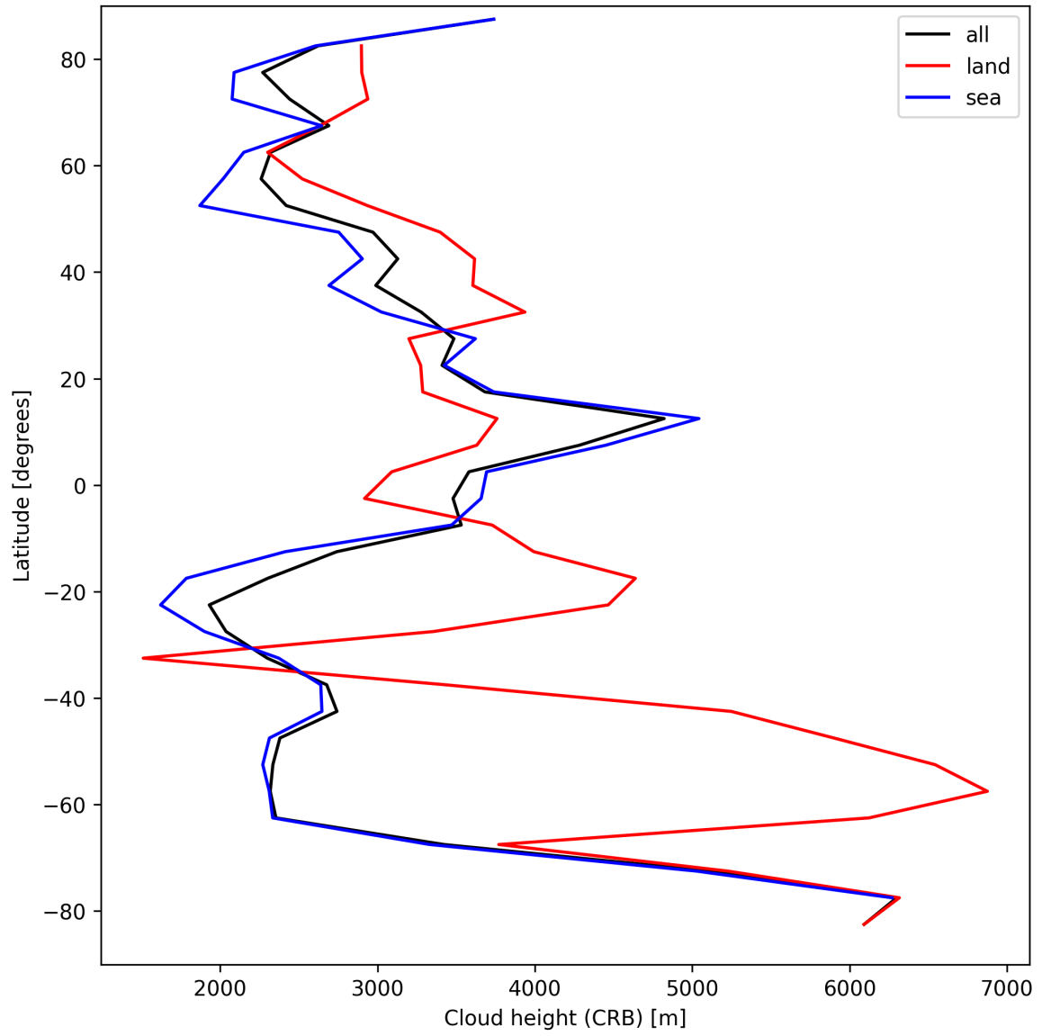
Figure 27: Zonal average of “Cloud height (CRB)” for 2025-09-10 to 2025-09-12.
