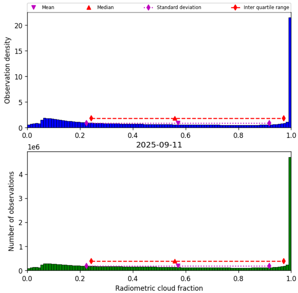
Figure 39: Histogram of “Radiometric cloud fraction” for 2025-09-10 to 2025-09-12
