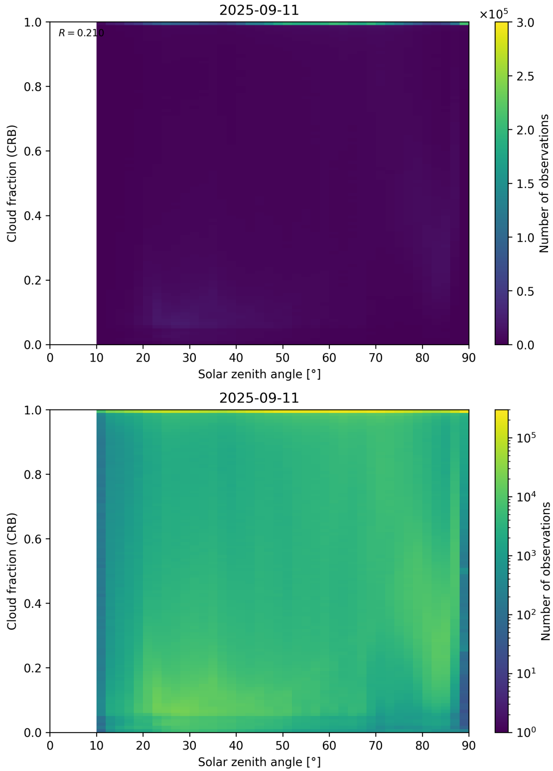
Figure 101: Scatter density plot of “Solar zenith angle” against “Cloud fraction (CRB)” for 2025-09-10 to 2025-09-12.
