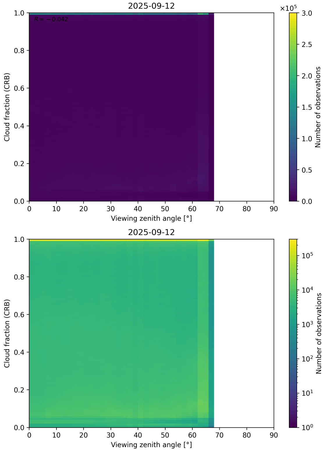
Figure 109: Scatter density plot of “Viewing zenith angle” against “Cloud fraction (CRB)” for 2025-09-11 to 2025-09-13.
