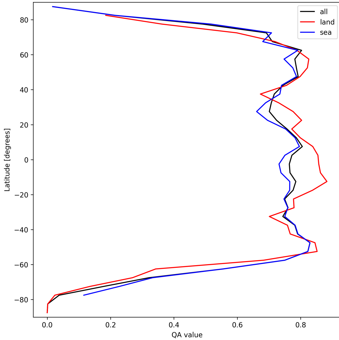
Figure 22: Zonal average of “QA value” for 2025-09-11 to 2025-09-13.
