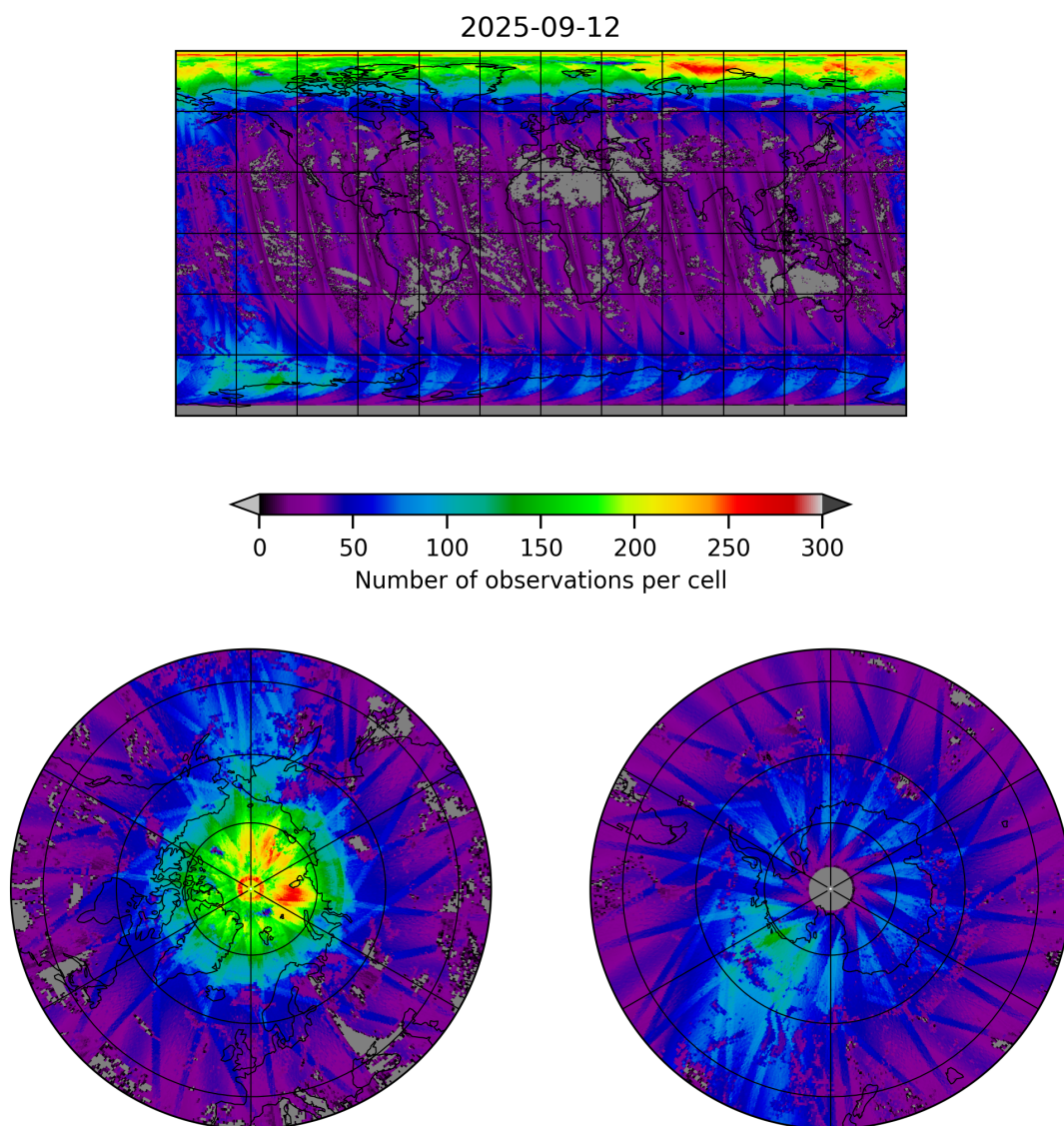
Figure 21: Map of the number of observations for 2025-09-11 to 2025-09-13
