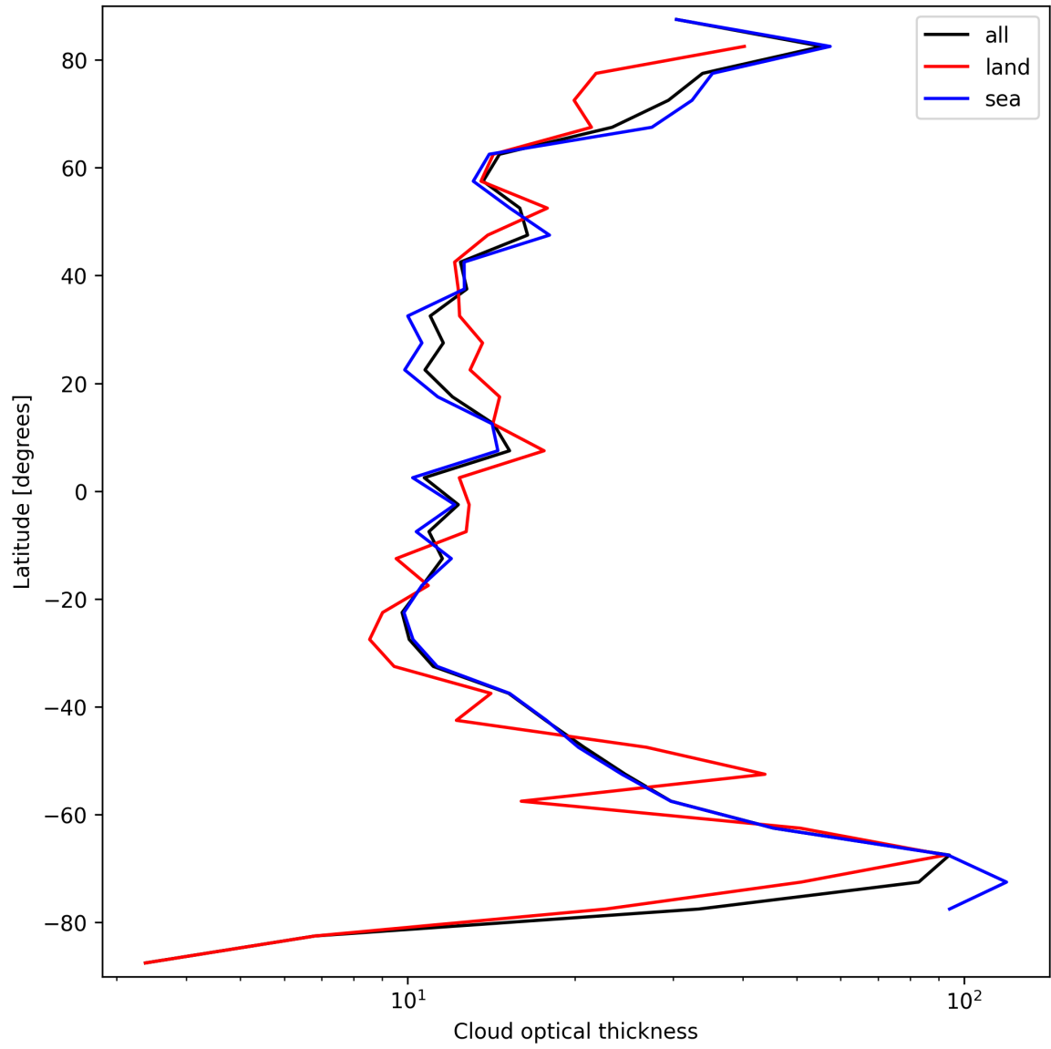
Figure 25: Zonal average of “Cloud optical thickness” for 2025-09-11 to 2025-09-13.
