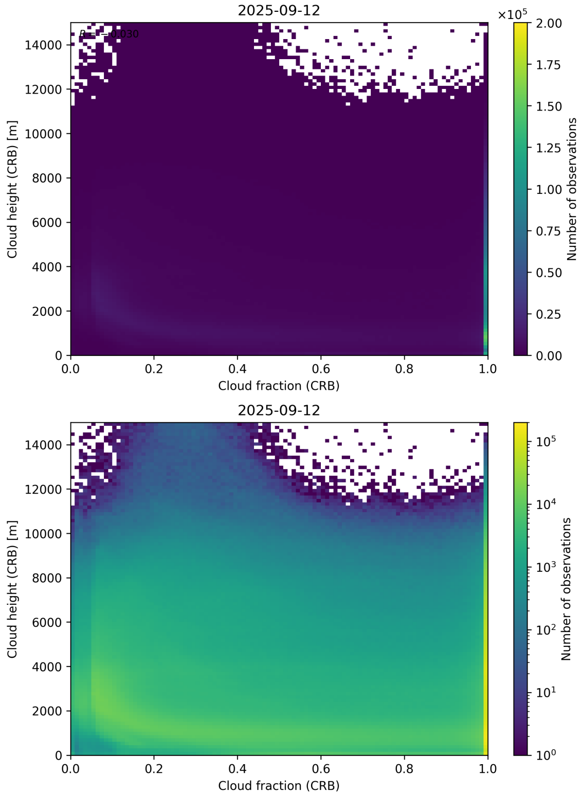
Figure 79: Scatter density plot of “Cloud fraction (CRB)” against “Cloud height (CRB)” for 2025-09-11 to 2025-09-13.
