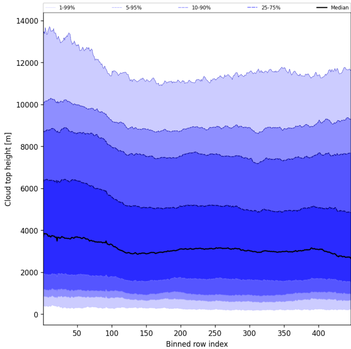
Figure 56: Along track statistics of “Cloud top height” for 2025-09-11 to 2025-09-13
