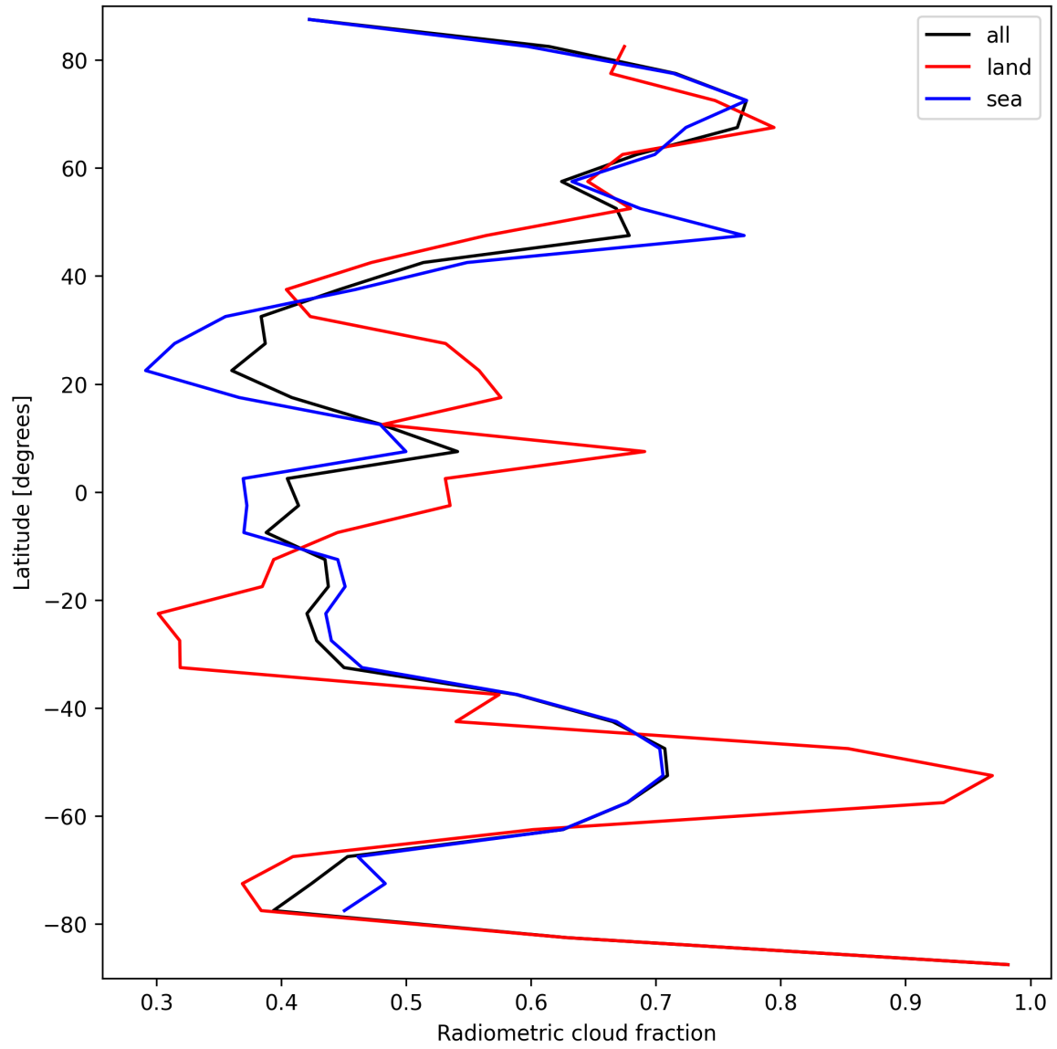
Figure 23: Zonal average of “Radiometric cloud fraction” for 2025-09-11 to 2025-09-13.
