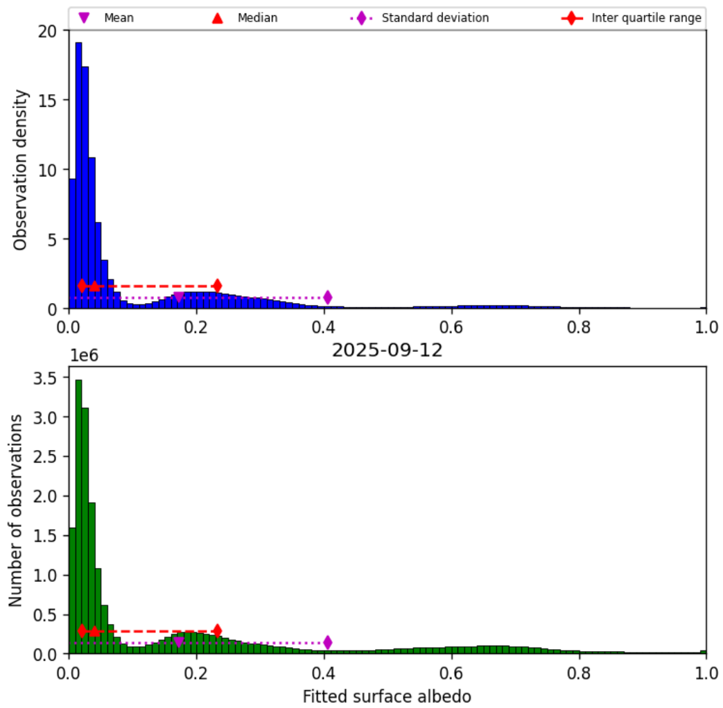
Figure 45: Histogram of “Fitted surface albedo” for 2025-09-11 to 2025-09-13
