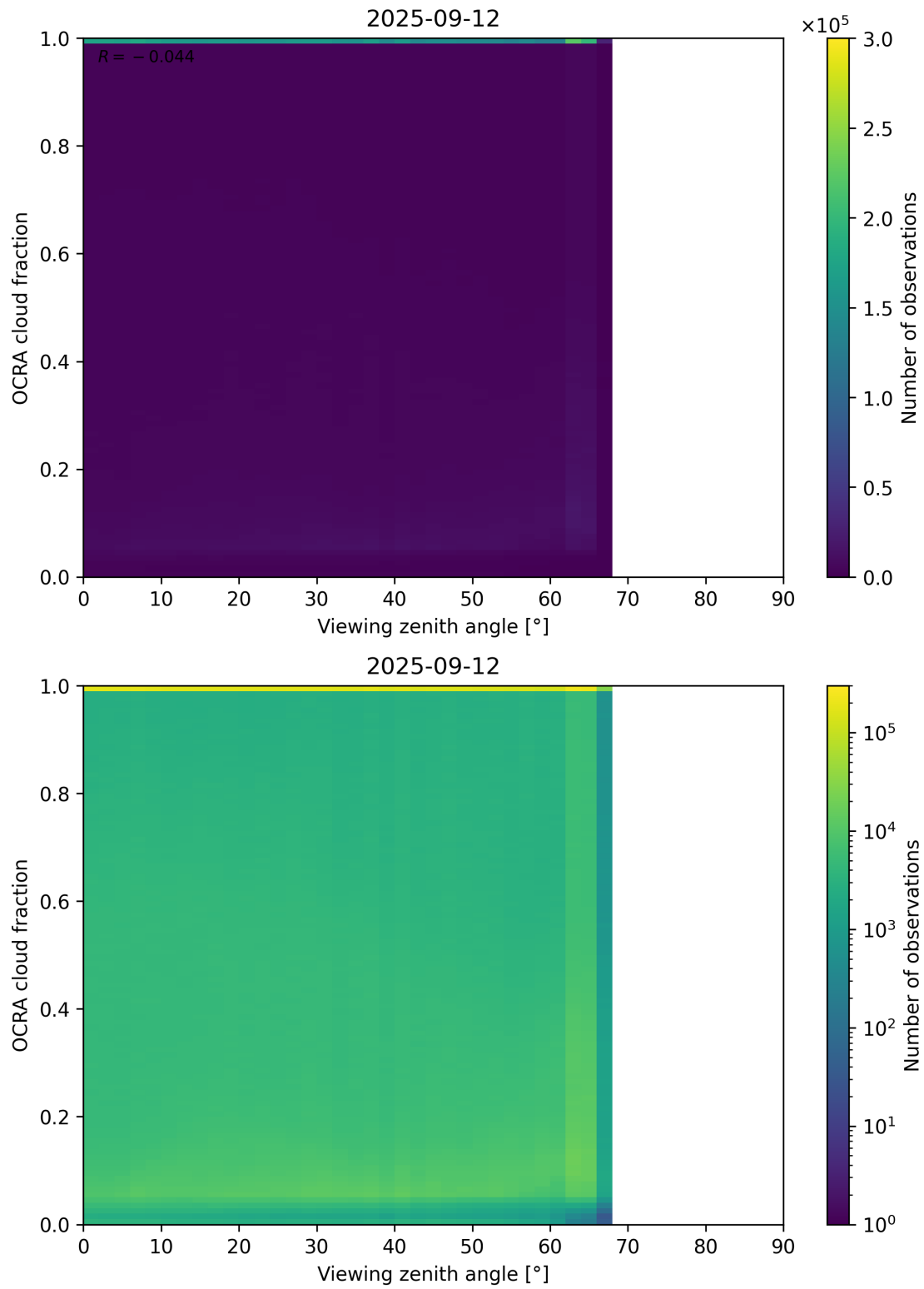
Figure 108: Scatter density plot of “Viewing zenith angle” against “OCRA cloud fraction” for 2025-09-11 to 2025-09-13.
