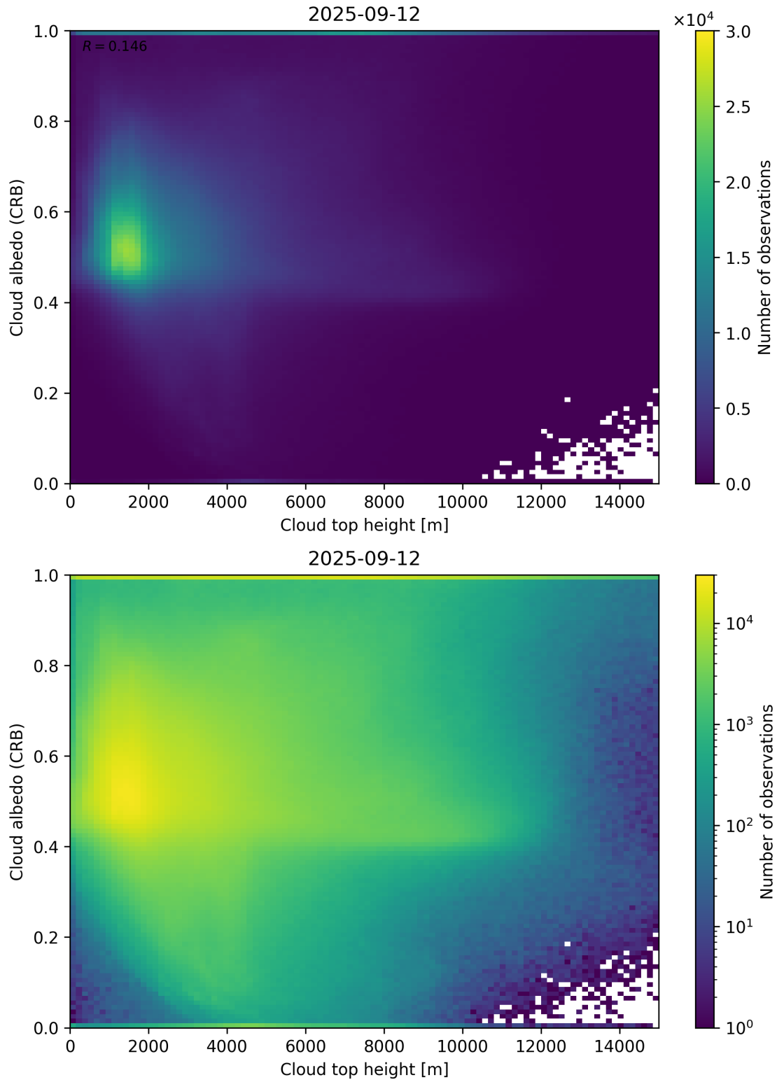
Figure 86: Scatter density plot of “Cloud top height” against “Cloud albedo (CRB)” for 2025-09-11 to 2025-09-13.
