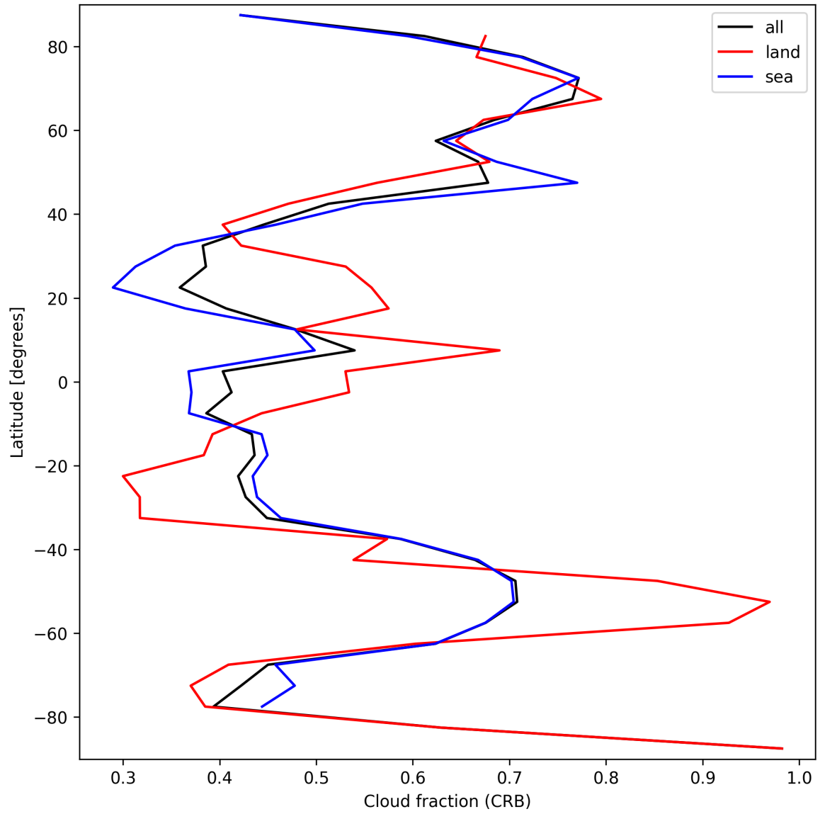
Figure 26: Zonal average of “Cloud fraction (CRB)” for 2025-09-11 to 2025-09-13.
