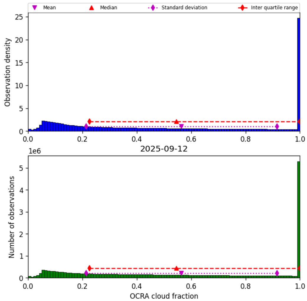
Figure 50: Histogram of “OCRA cloud fraction” for 2025-09-11 to 2025-09-13
