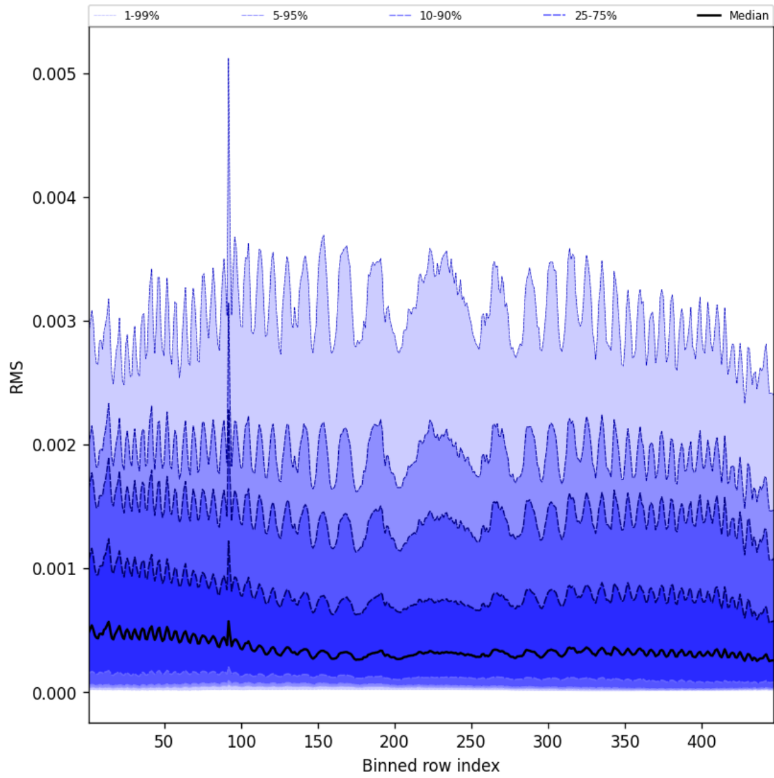
Figure 63: Along track statistics of “RMS” for 2025-09-11 to 2025-09-13
