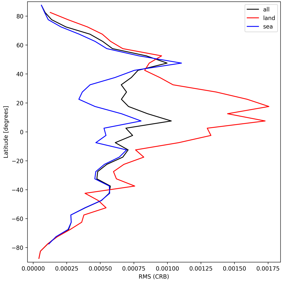
Figure 32: Zonal average of “RMS (CRB)” for 2025-09-11 to 2025-09-13.
