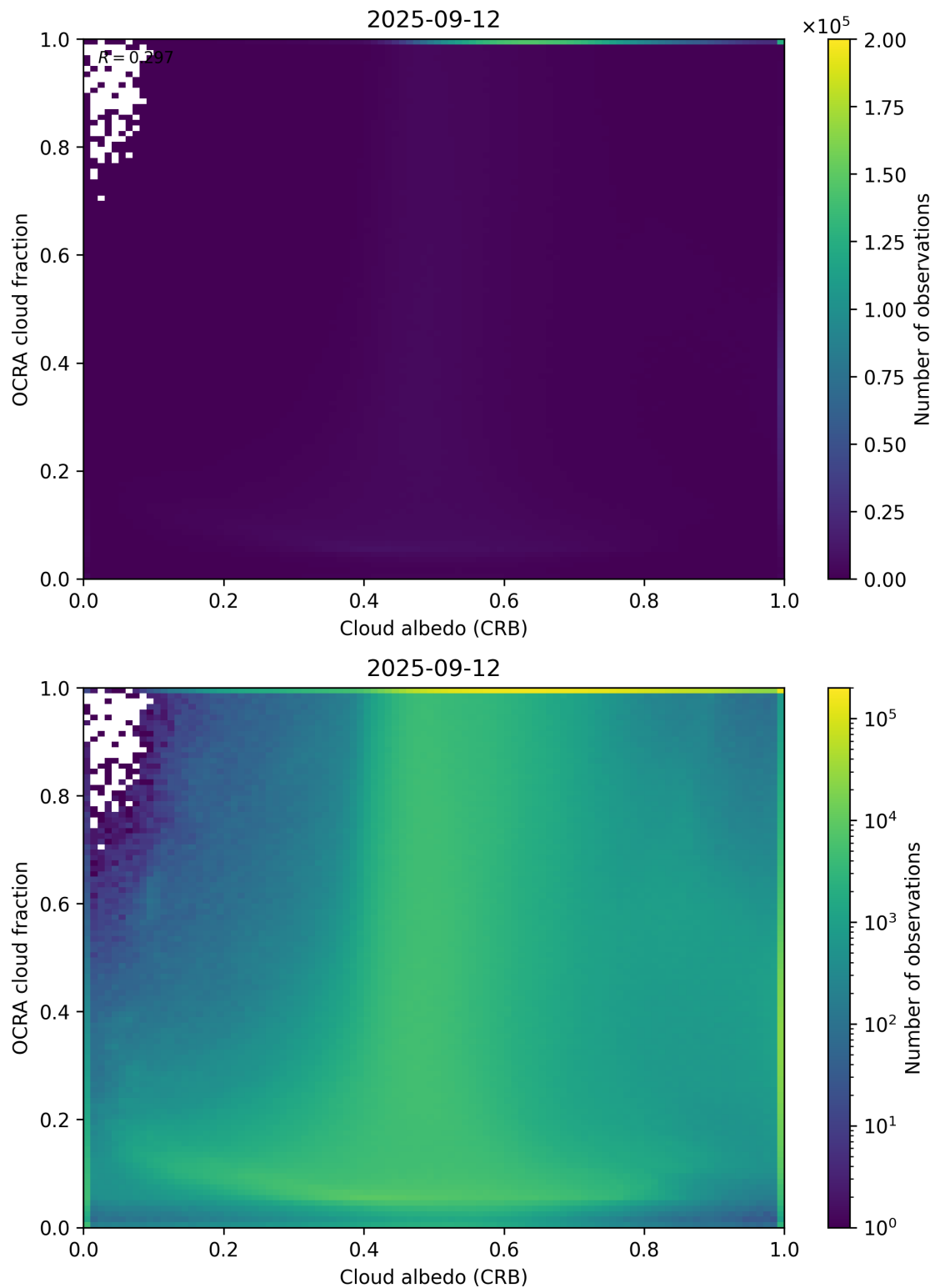
Figure 70: Scatter density plot of “Cloud albedo (CRB)” against “OCRA cloud fraction” for 2025-09-11 to 2025-09-13.
