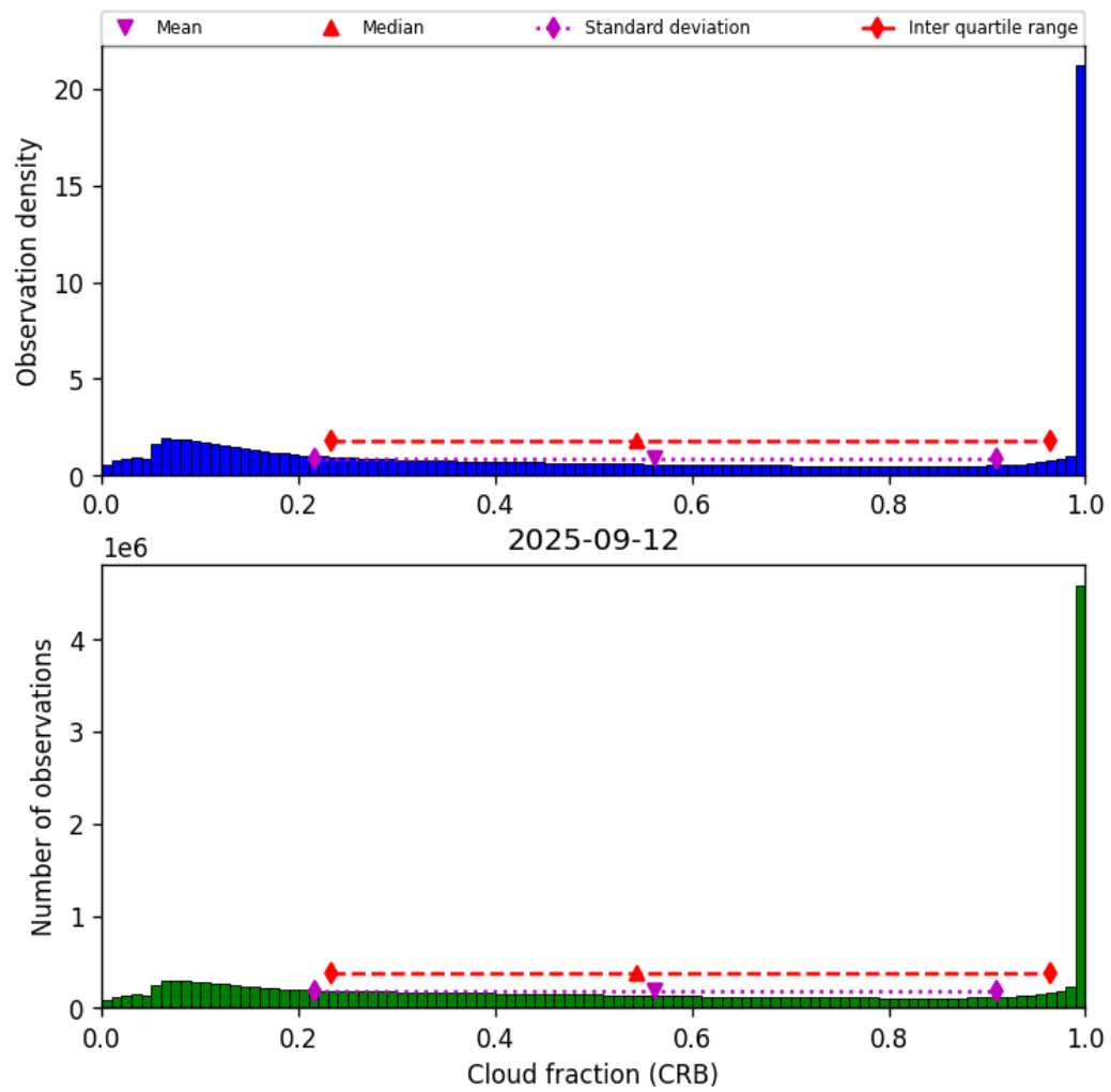
Figure 42: Histogram of “Cloud fraction (CRB)” for 2025-09-11 to 2025-09-13
