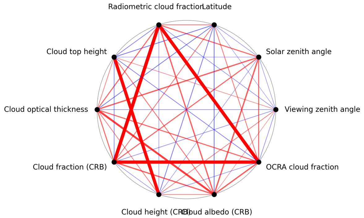
Figure 1: Map of correlation graph for 2025-09-11 to 2025-09-13.
