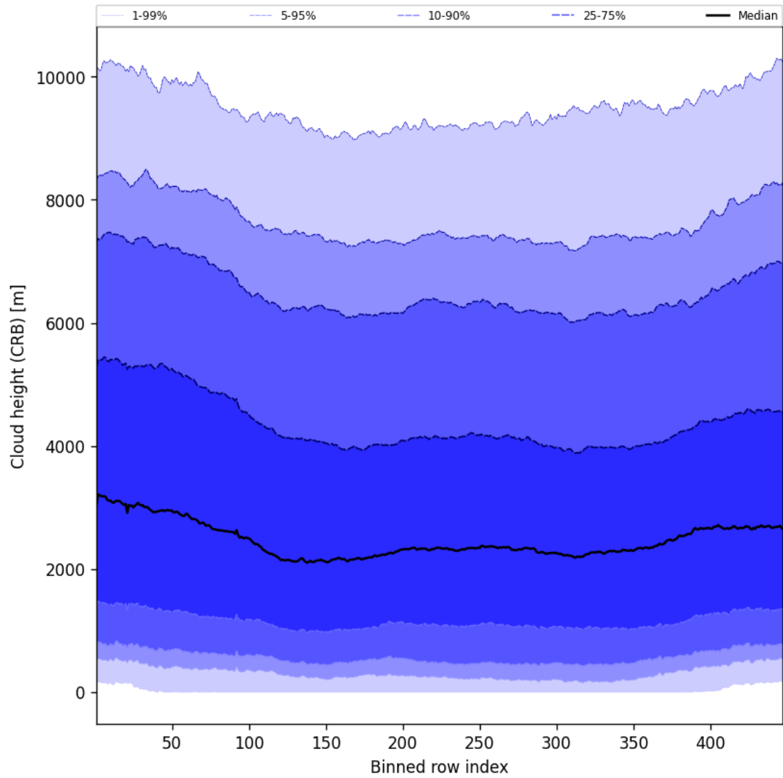
Figure 59: Along track statistics of “Cloud height (CRB)” for 2025-09-11 to 2025-09-13
