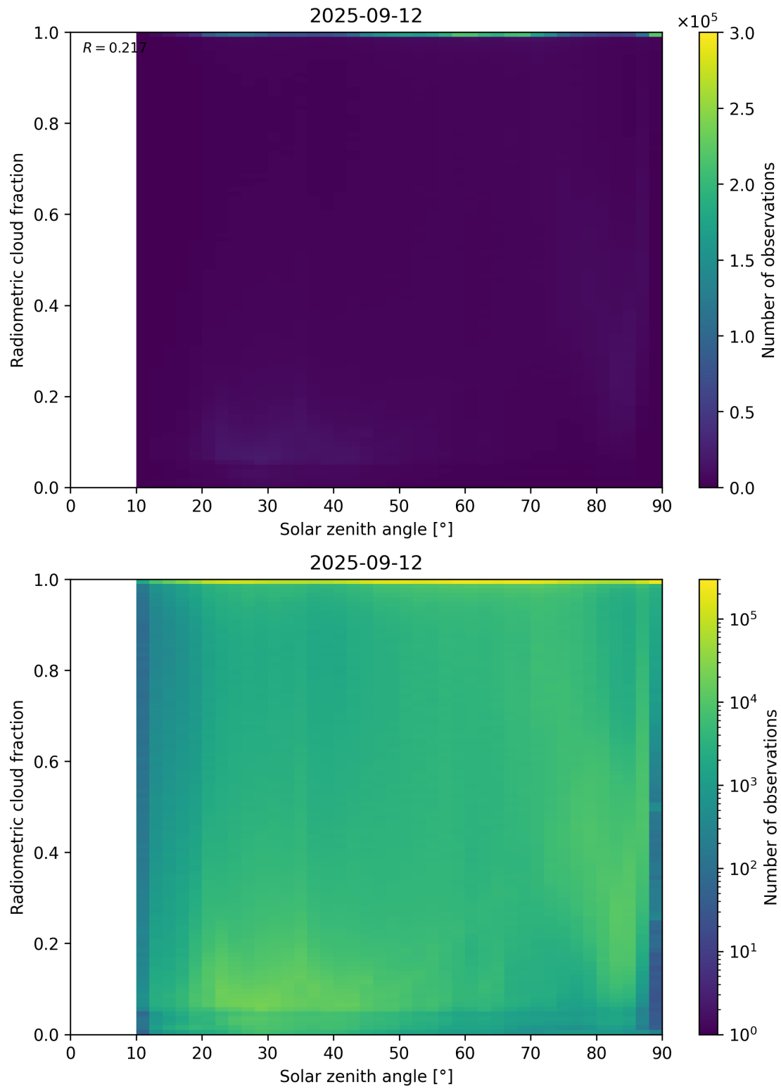
Figure 99: Scatter density plot of “Solar zenith angle” against “Radiometric cloud fraction” for 2025-09-11 to 2025-09-13.
