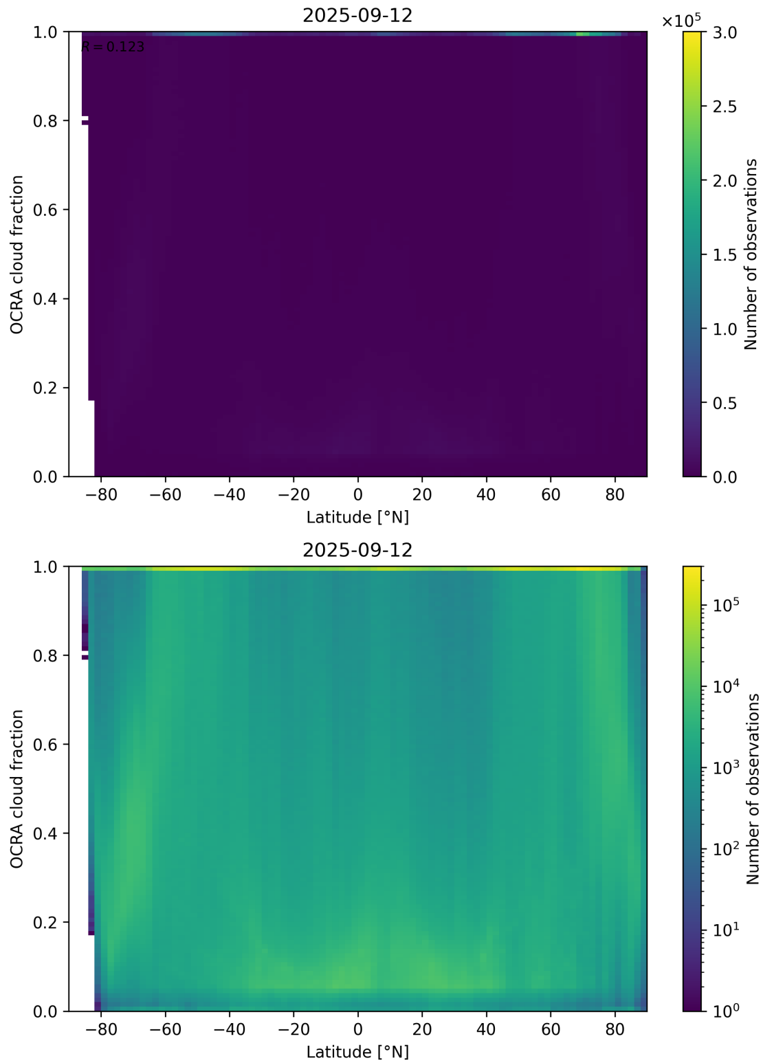
Figure 93: Scatter density plot of “Latitude” against “OCRA cloud fraction” for 2025-09-11 to 2025-09-13.
