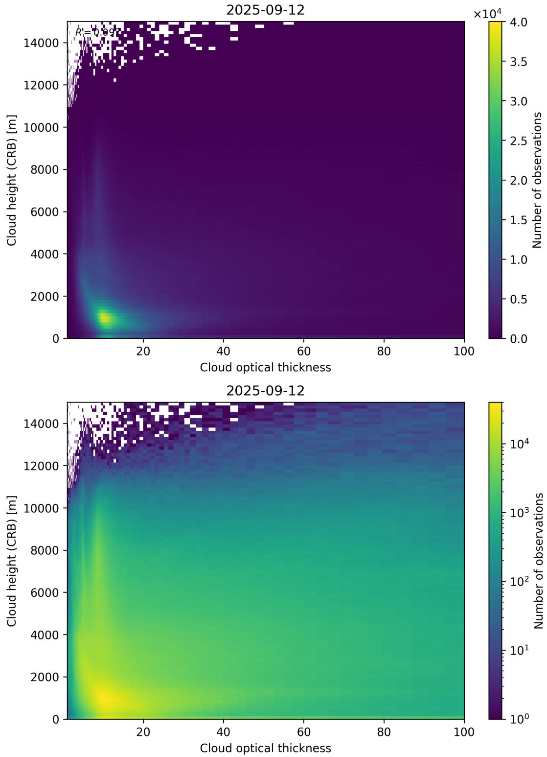
Figure 85: Scatter density plot of “Cloud optical thickness” against “Cloud height (CRB)” for 2025-09-11 to 2025-09-13.
