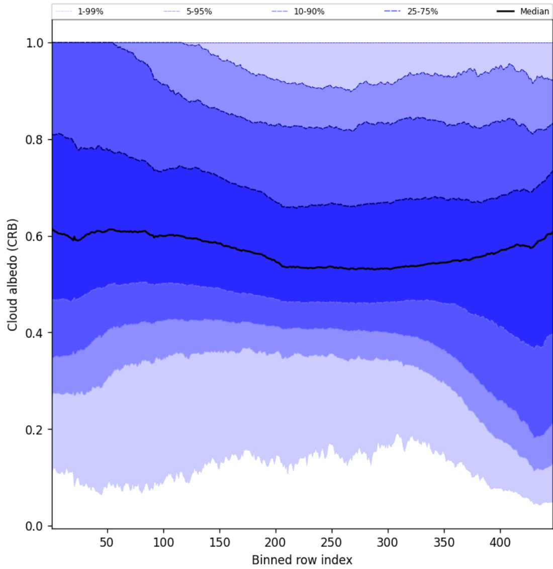
Figure 60: Along track statistics of “Cloud albedo (CRB)” for 2025-09-11 to 2025-09-13
