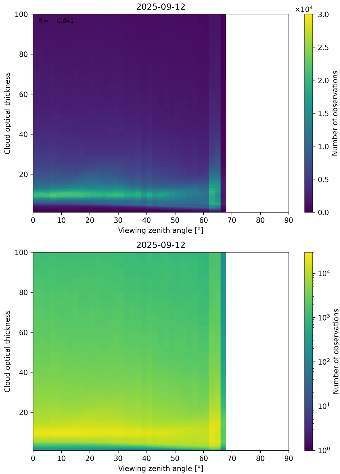
Figure 111: Scatter density plot of “Viewing zenith angle” against “Cloud optical thickness” for 2025-09-11 to 2025-09-13.
