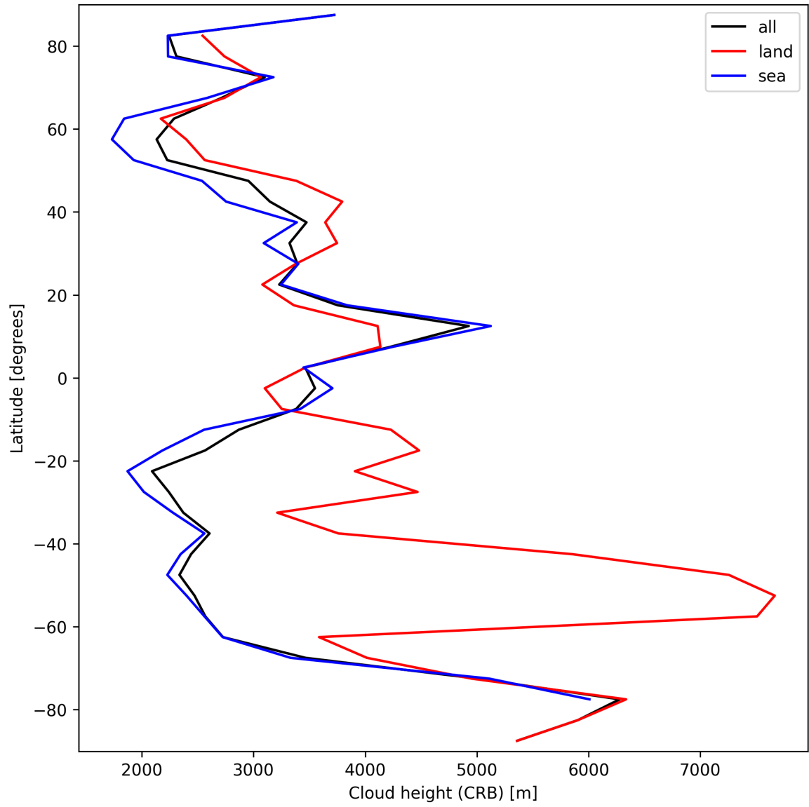
Figure 27: Zonal average of “Cloud height (CRB)” for 2025-09-11 to 2025-09-13.
