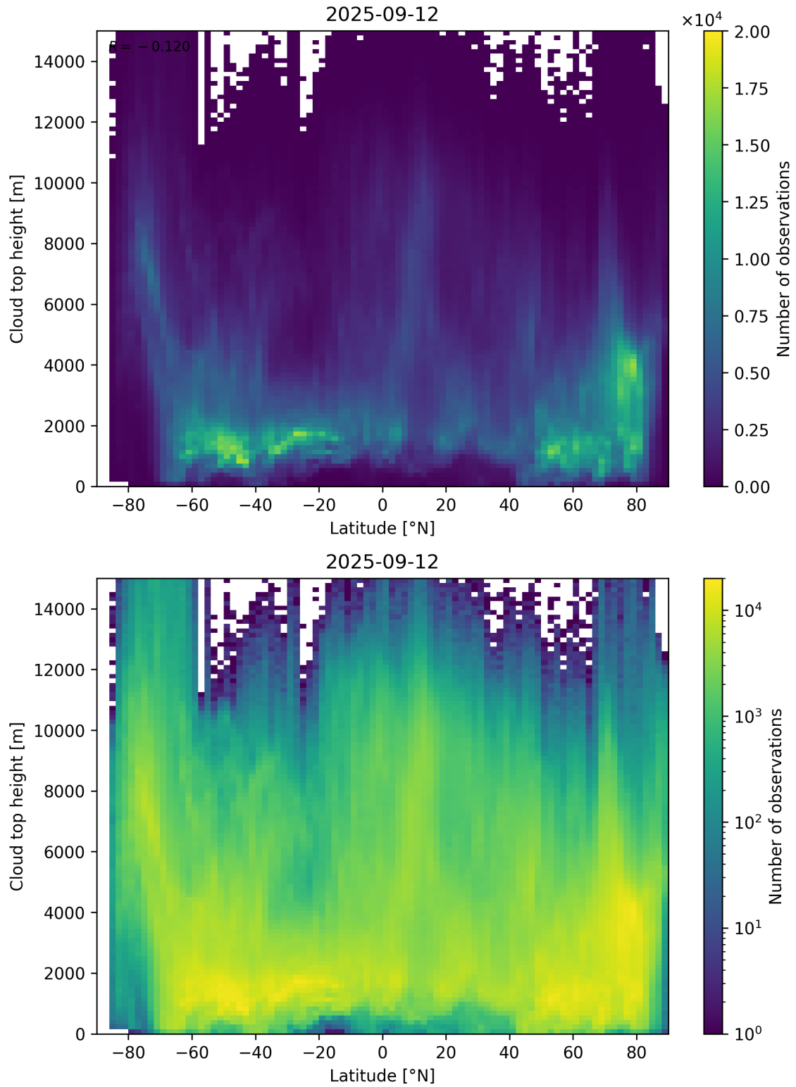
Figure 97: Scatter density plot of “Latitude” against “Cloud top height” for 2025-09-11 to 2025-09-13.
