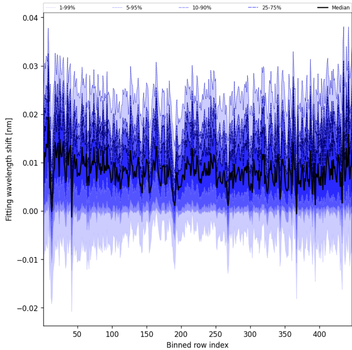
Figure 65: Along track statistics of “Fitting wavelength shift” for 2025-09-11 to 2025-09-13
