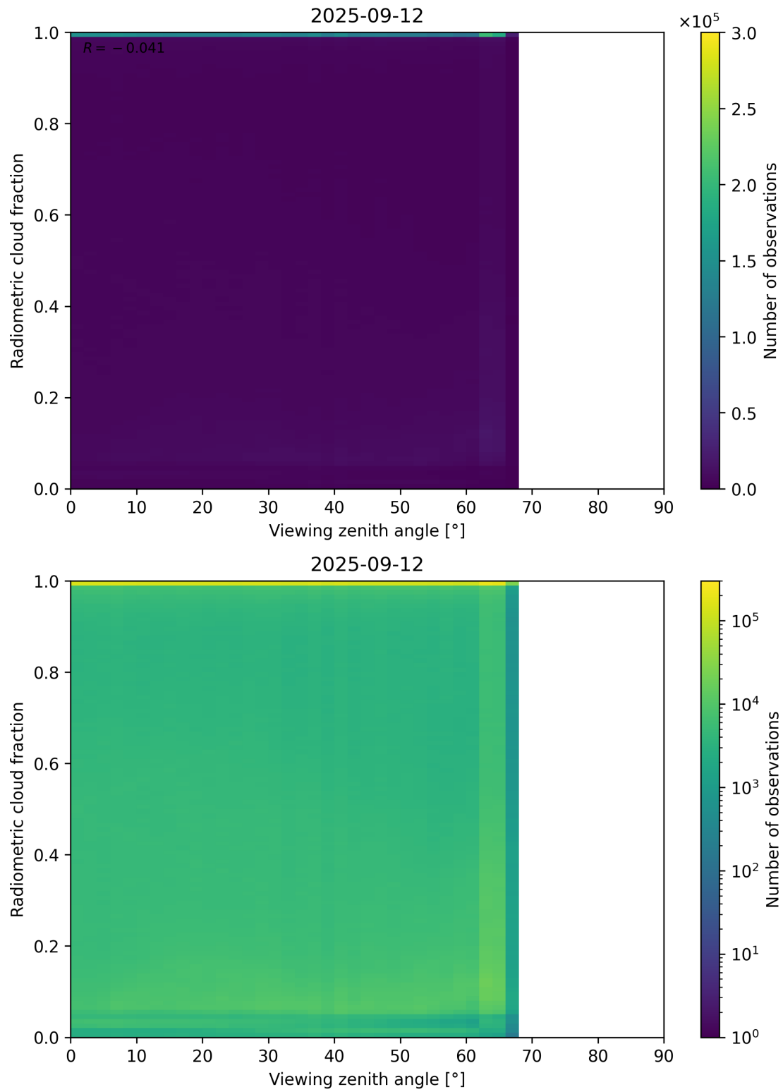
Figure 107: Scatter density plot of “Viewing zenith angle” against “Radiometric cloud fraction” for 2025-09-11 to 2025-09-13.
