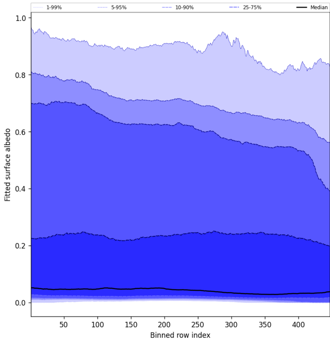
Figure 61: Along track statistics of “Fitted surface albedo” for 2025-09-11 to 2025-09-13
