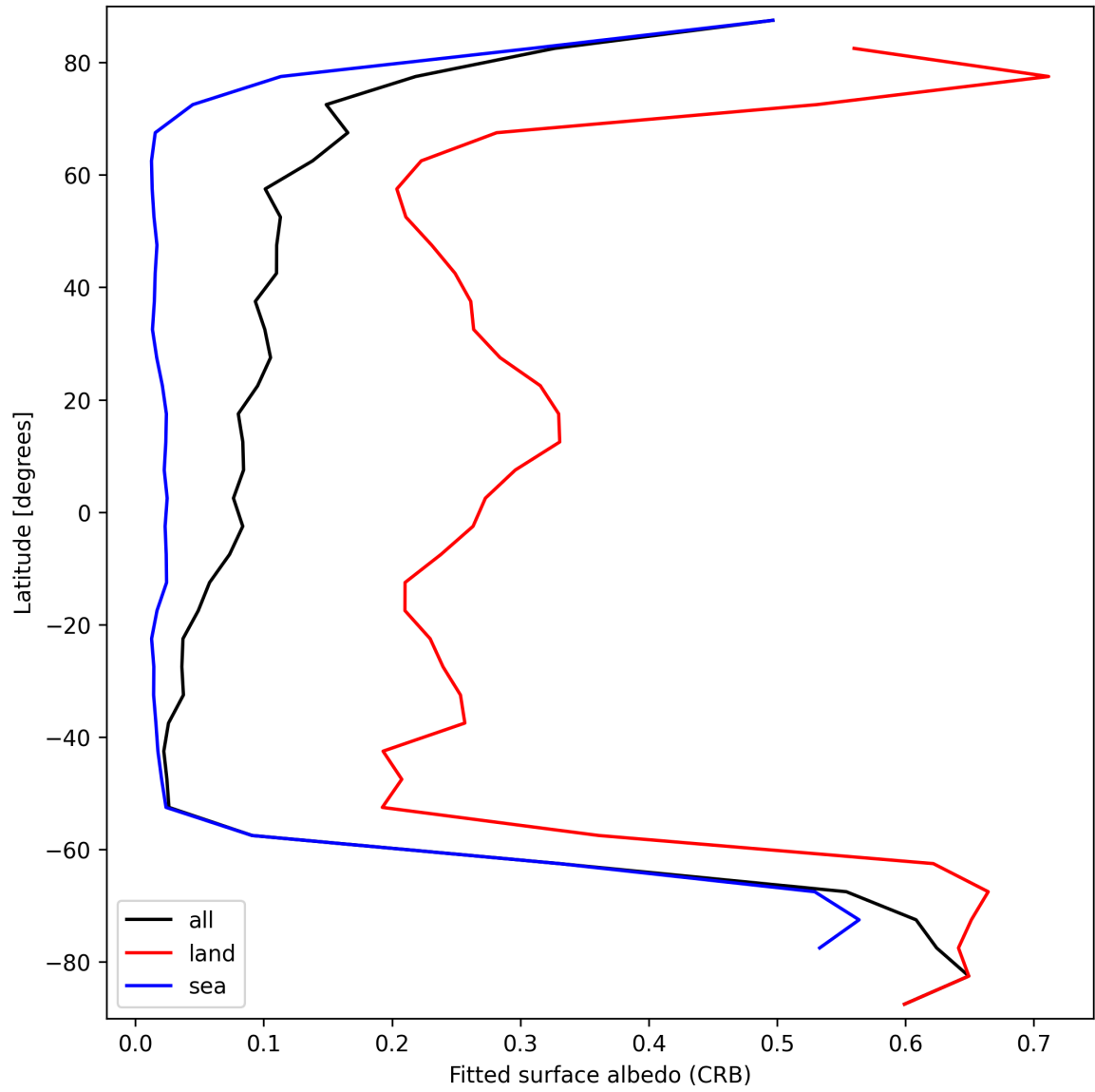
Figure 30: Zonal average of “Fitted surface albedo (CRB)” for 2025-09-11 to 2025-09-13.
