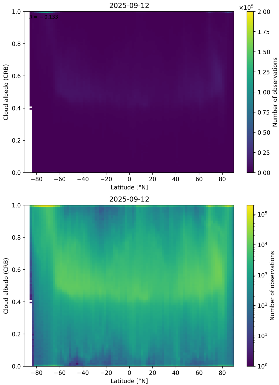
Figure 91: Scatter density plot of “Latitude” against “Cloud albedo (CRB)” for 2025-09-11 to 2025-09-13.
