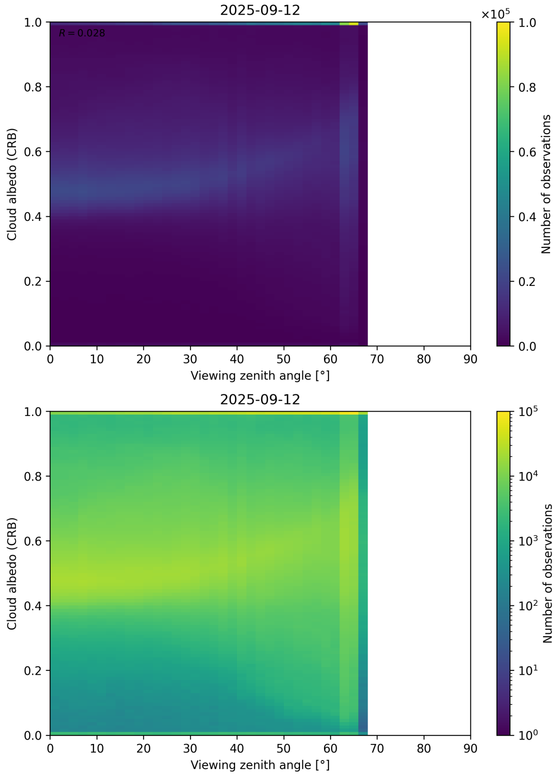
Figure 106: Scatter density plot of “Viewing zenith angle” against “Cloud albedo (CRB)” for 2025-09-11 to 2025-09-13.
