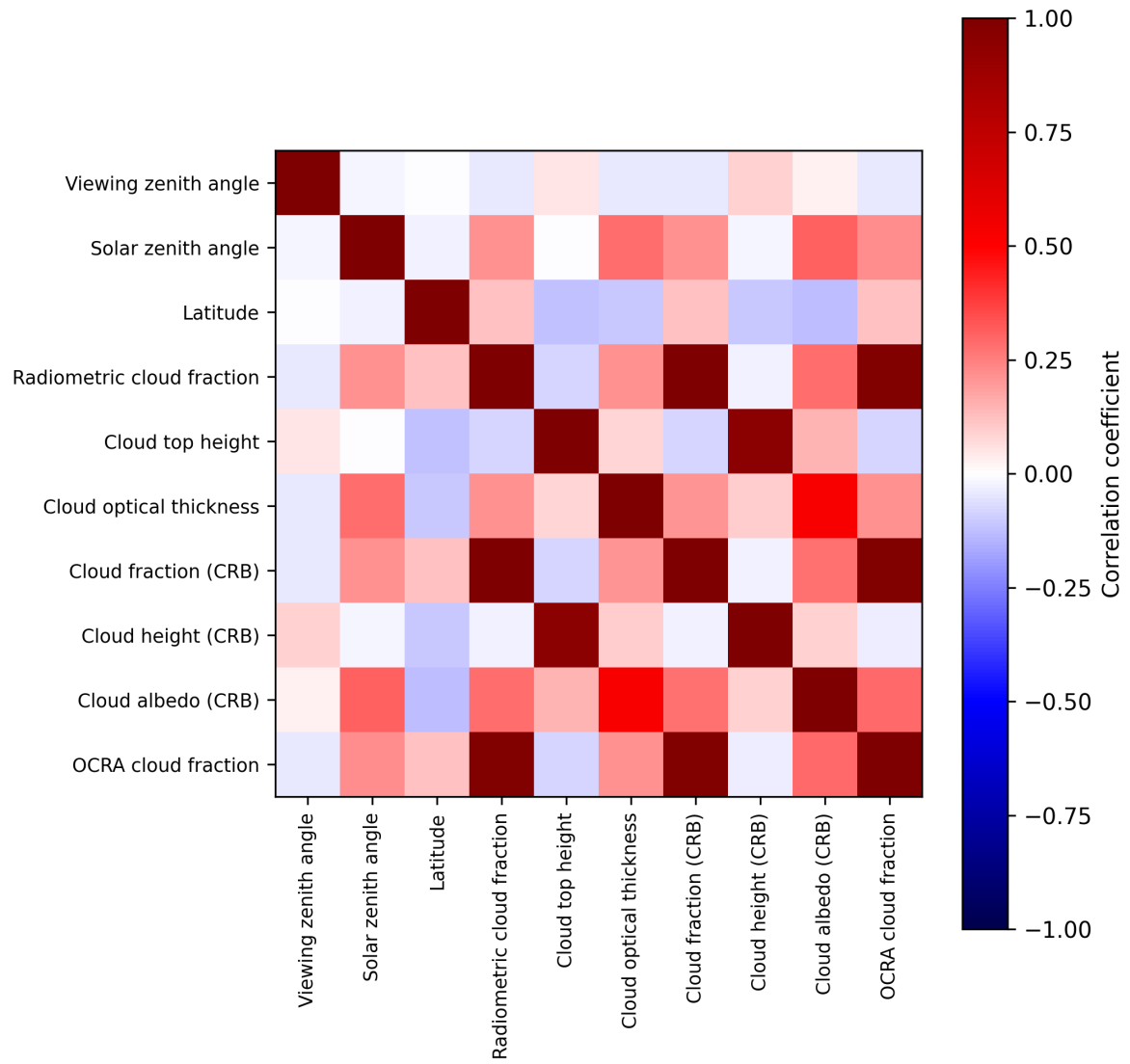
Figure 2: Map of correlation matrix for 2025-09-11 to 2025-09-13.
