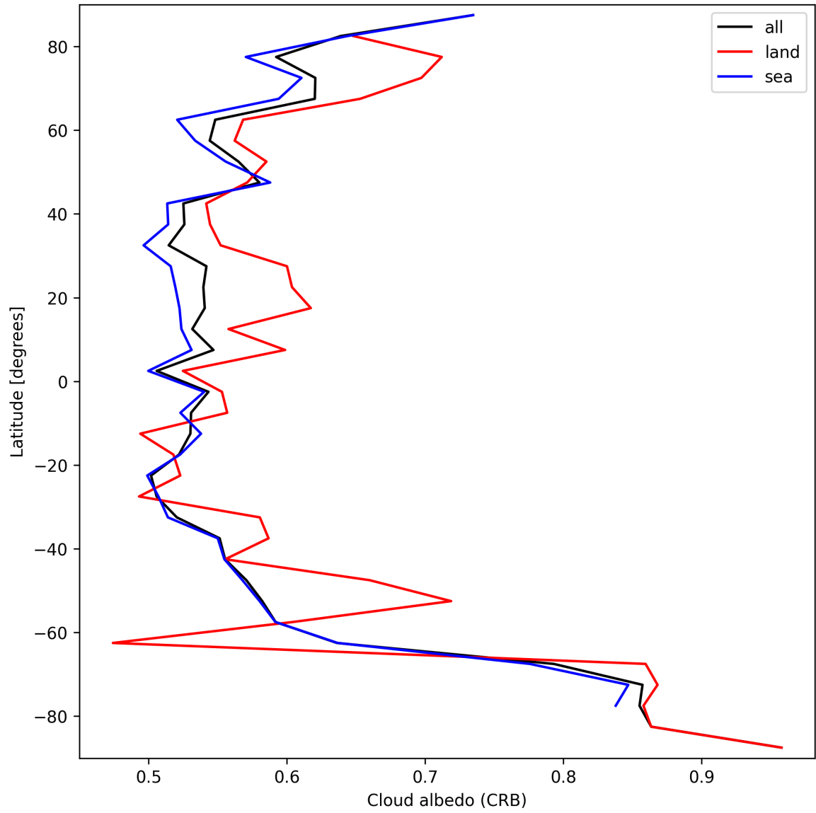
Figure 28: Zonal average of “Cloud albedo (CRB)” for 2025-09-11 to 2025-09-13.
