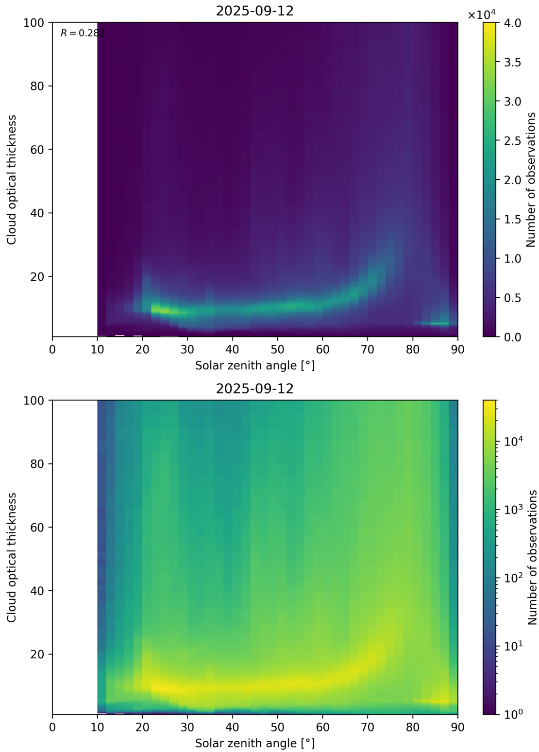
Figure 103: Scatter density plot of “Solar zenith angle” against “Cloud optical thickness” for 2025-09-11 to 2025-09-13.
