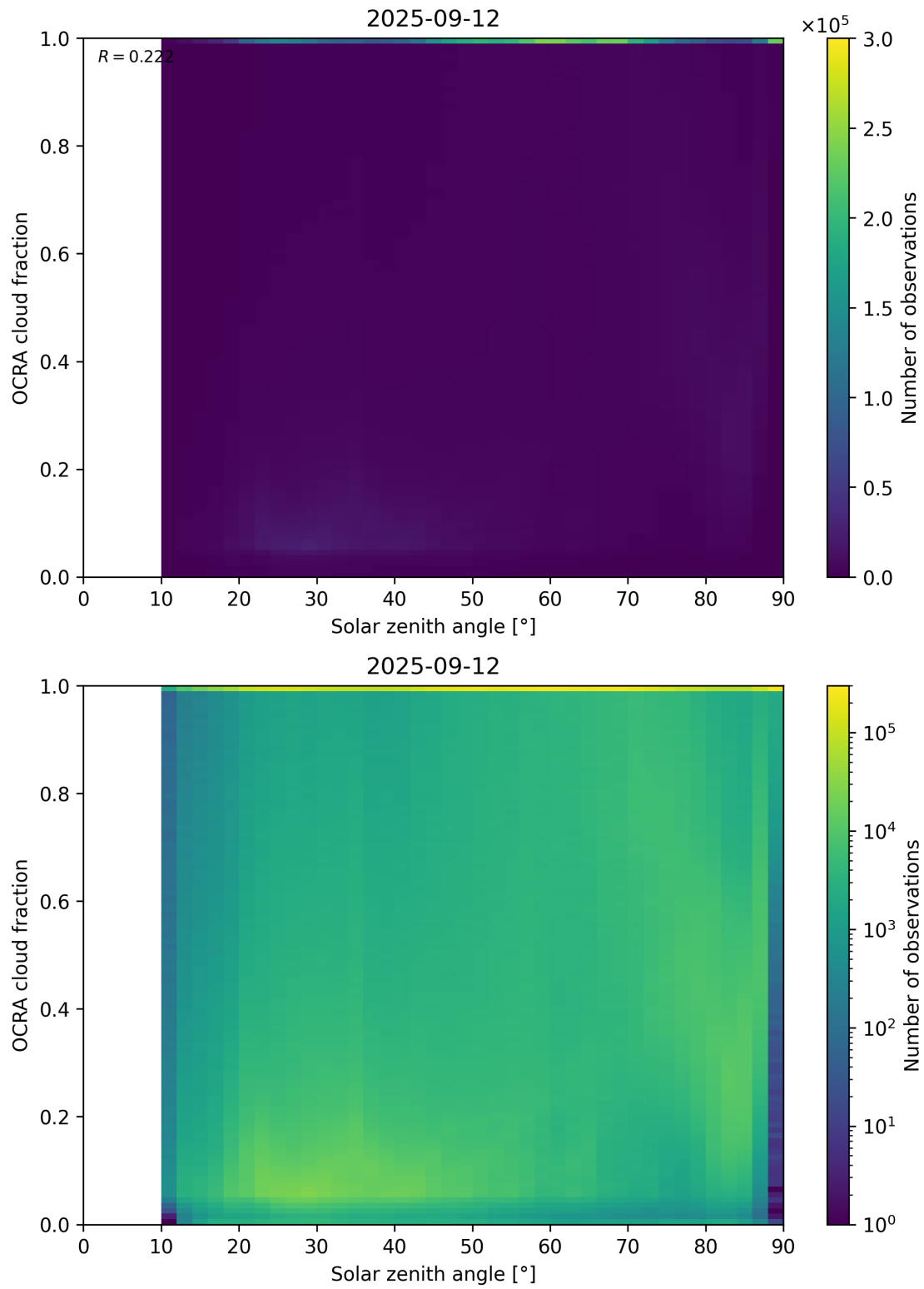
Figure 100: Scatter density plot of “Solar zenith angle” against “OCRA cloud fraction” for 2025-09-11 to 2025-09-13.
