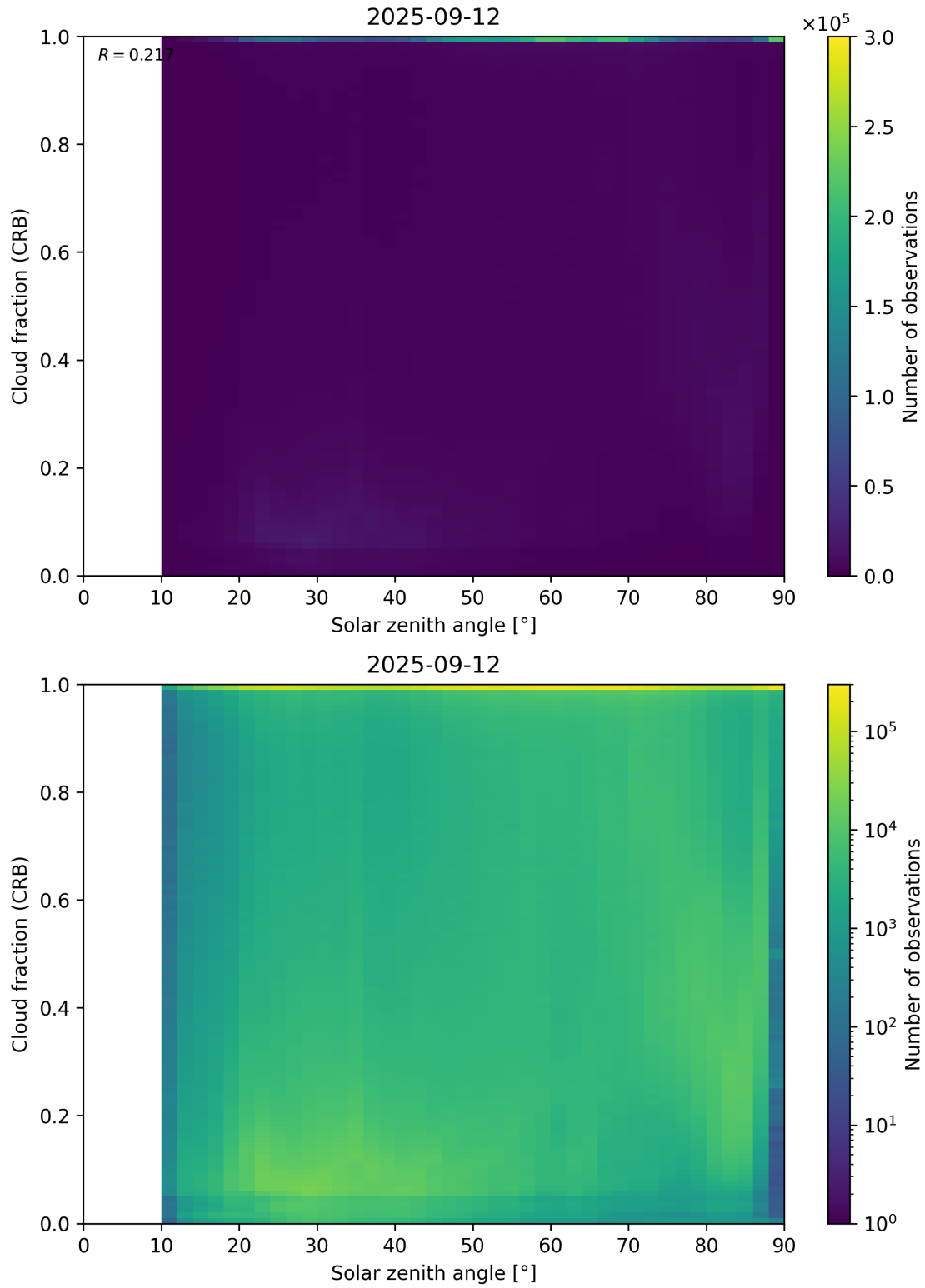
Figure 101: Scatter density plot of “Solar zenith angle” against “Cloud fraction (CRB)” for 2025-09-11 to 2025-09-13.
