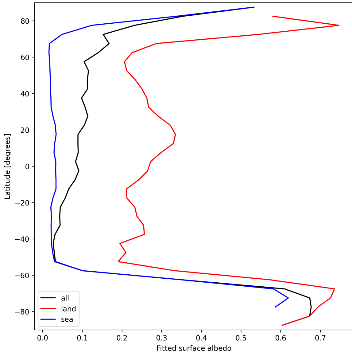
Figure 29: Zonal average of “Fitted surface albedo” for 2025-09-11 to 2025-09-13.
