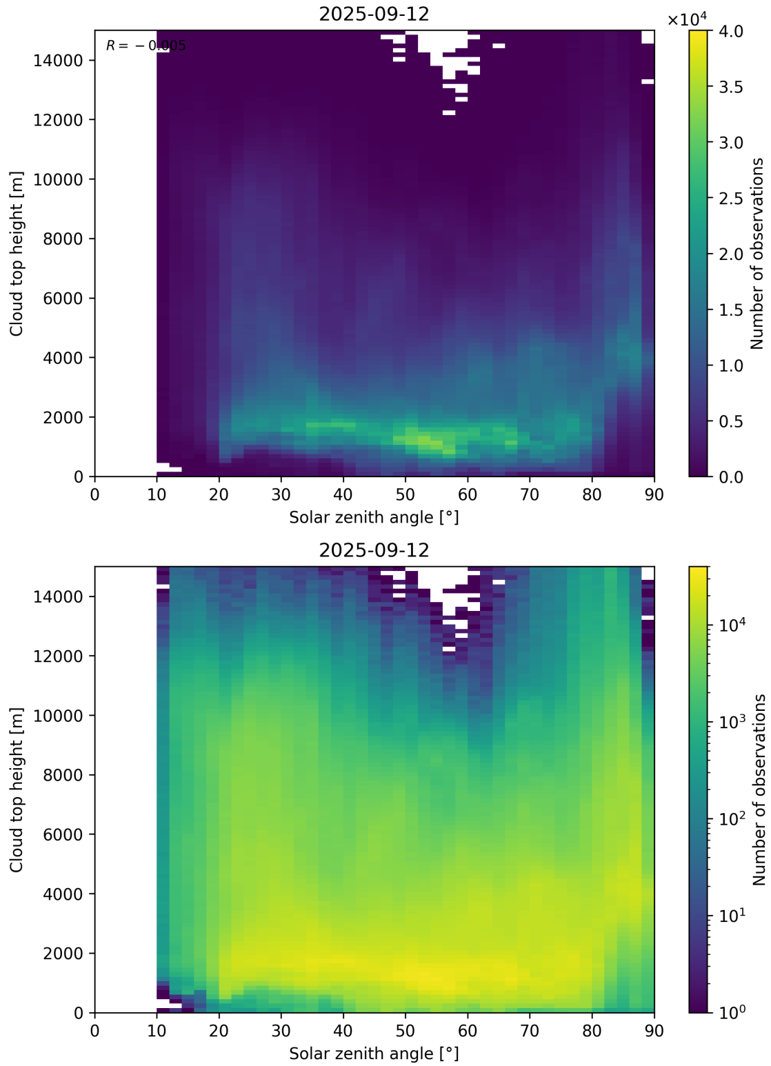
Figure 104: Scatter density plot of “Solar zenith angle” against “Cloud top height” for 2025-09-11 to 2025-09-13.
