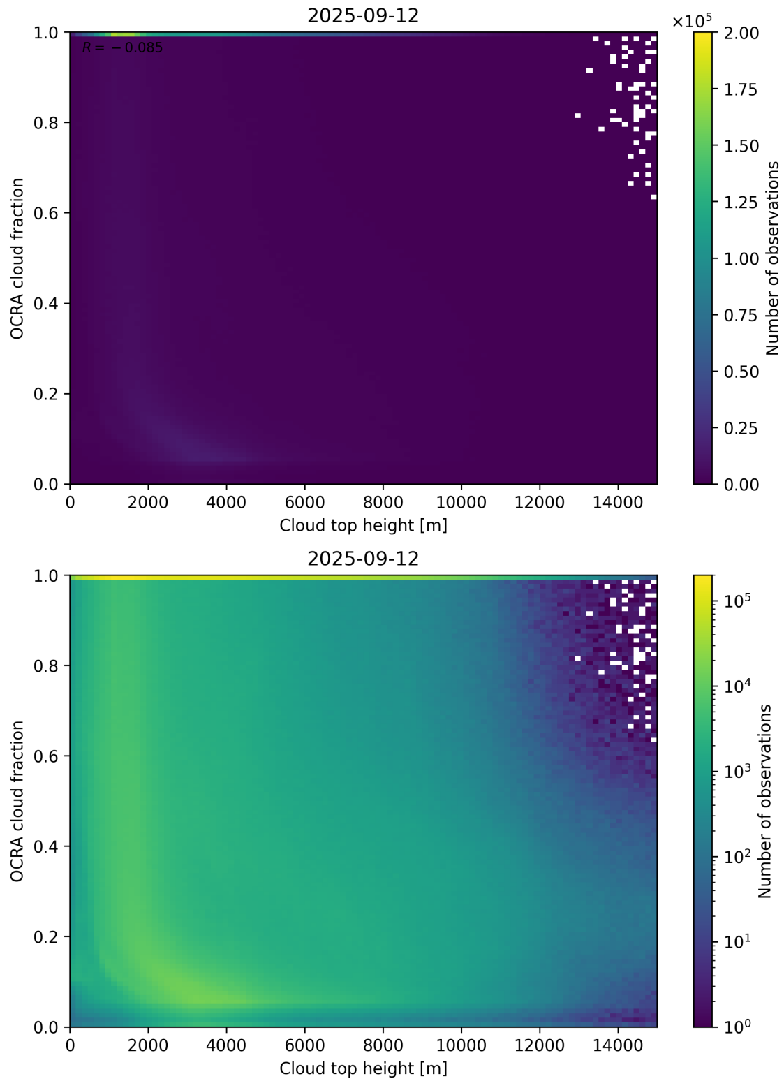
Figure 87: Scatter density plot of “Cloud top height” against “OCRA cloud fraction” for 2025-09-11 to 2025-09-13.
