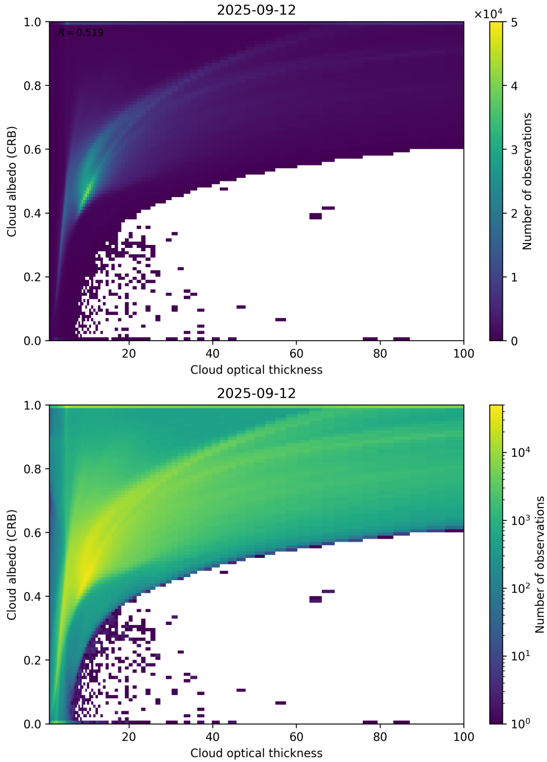
Figure 82: Scatter density plot of “Cloud optical thickness” against “Cloud albedo (CRB)” for 2025-09-11 to 2025-09-13.
