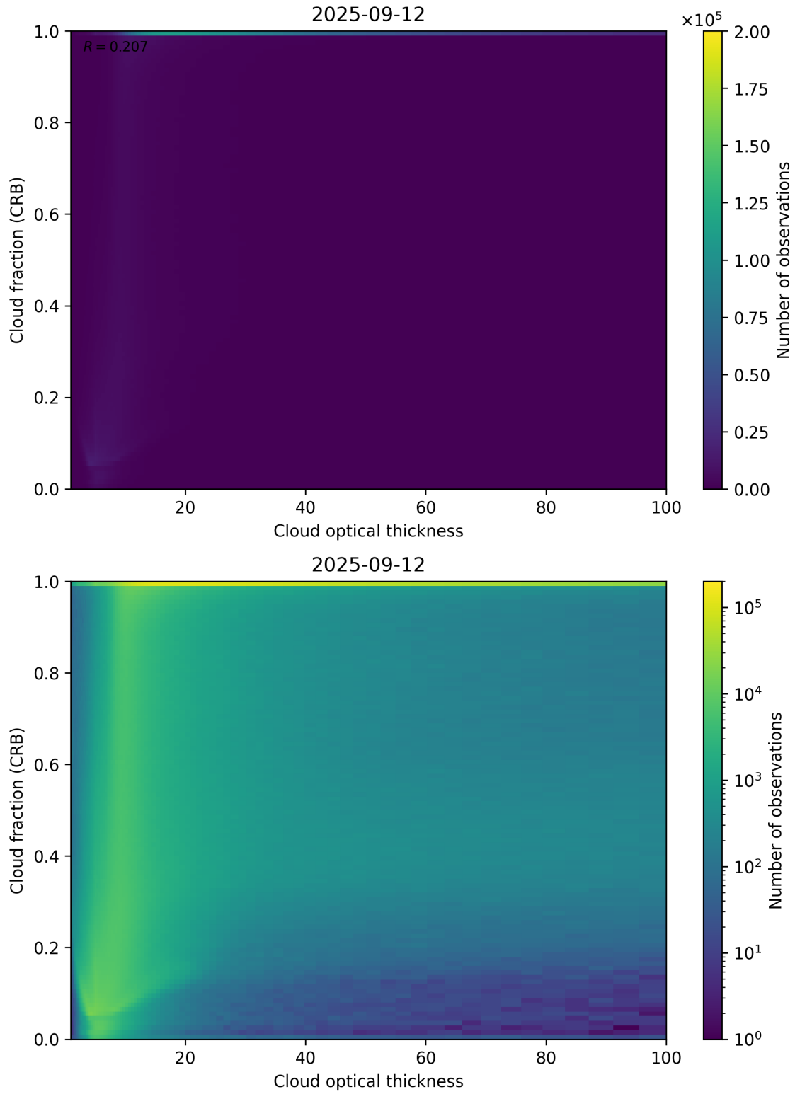
Figure 84: Scatter density plot of “Cloud optical thickness” against “Cloud fraction (CRB)” for 2025-09-11 to 2025-09-13.
