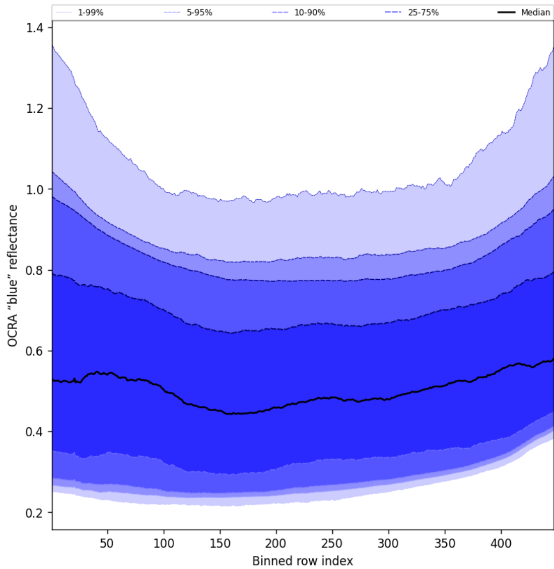
Figure 67: Along track statistics of “OCRA “blue” reflectance” for 2025-09-11 to 2025-09-13
