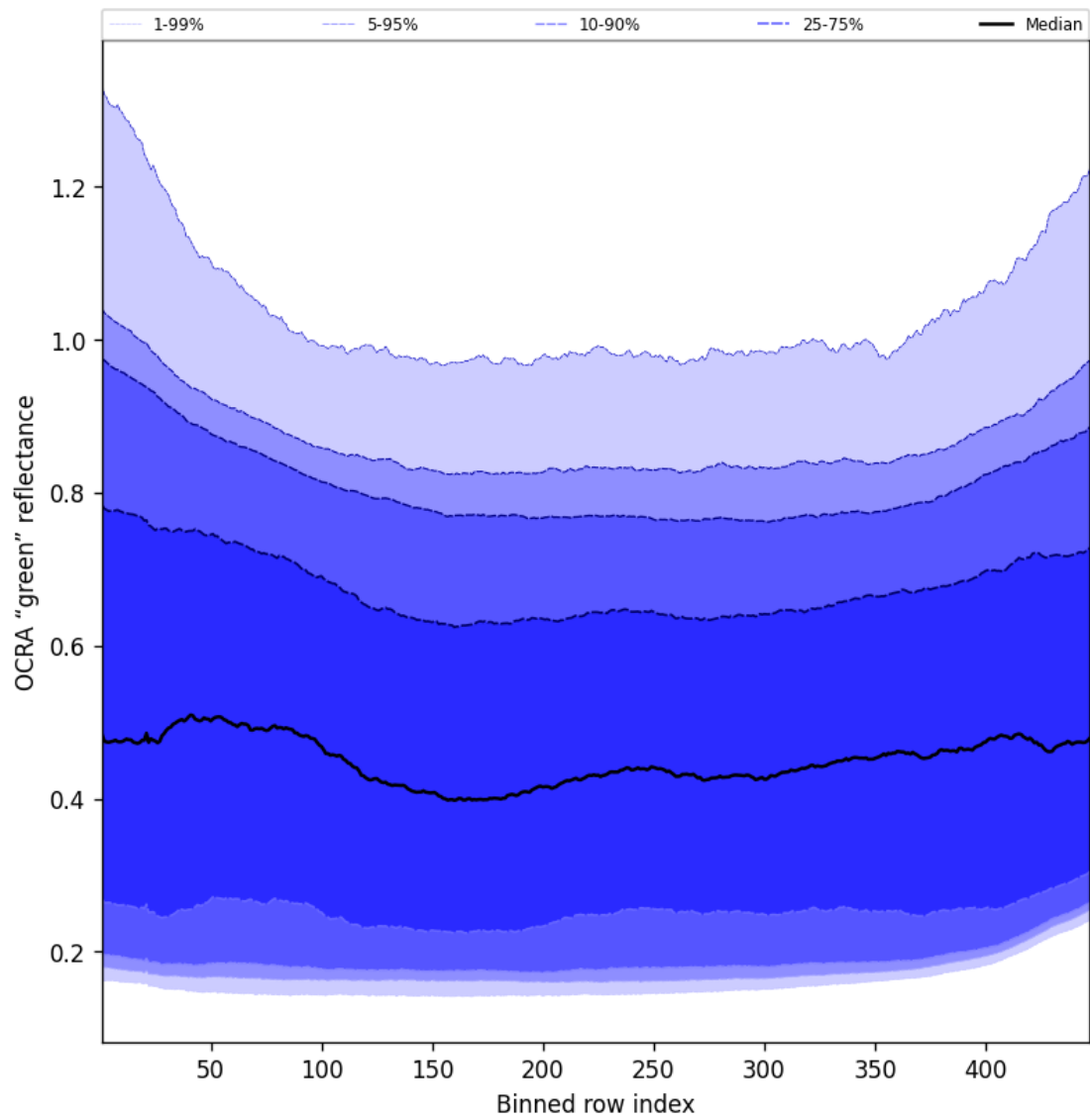
Figure 68: Along track statistics of “OCRA “green” reflectance” for 2025-09-11 to 2025-09-13
