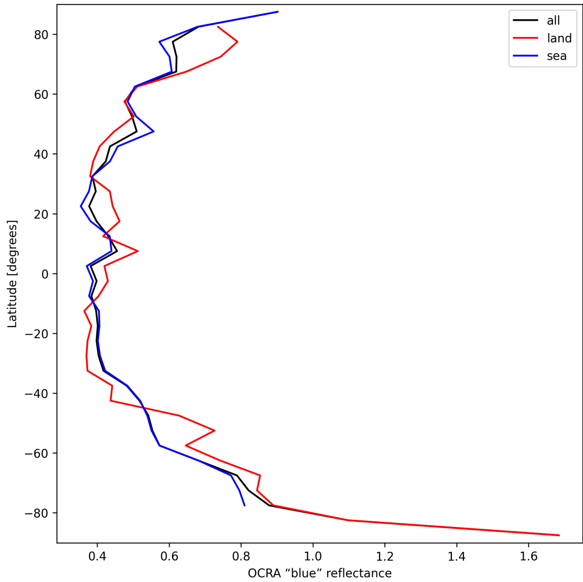
Figure 35: Zonal average of “OCRA “blue” reflectance” for 2025-09-11 to 2025-09-13.
