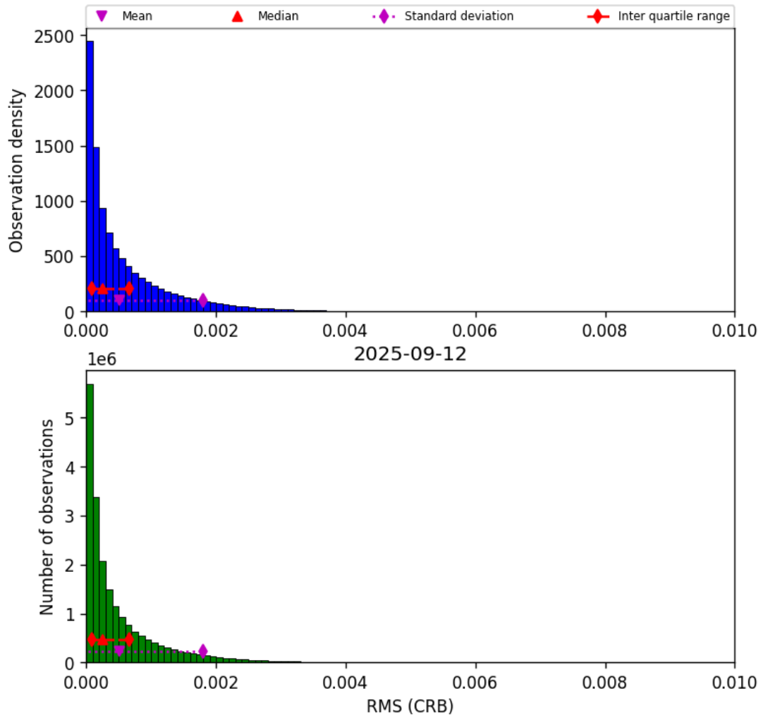
Figure 48: Histogram of “RMS (CRB)” for 2025-09-11 to 2025-09-13
