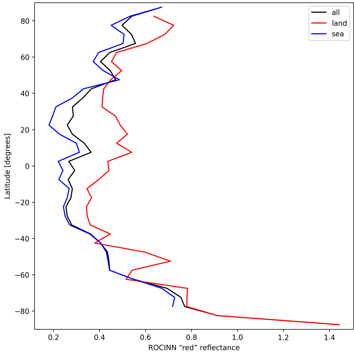
Figure 37: Zonal average of “ROCINN “red” reflectance” for 2025-09-11 to 2025-09-13.
