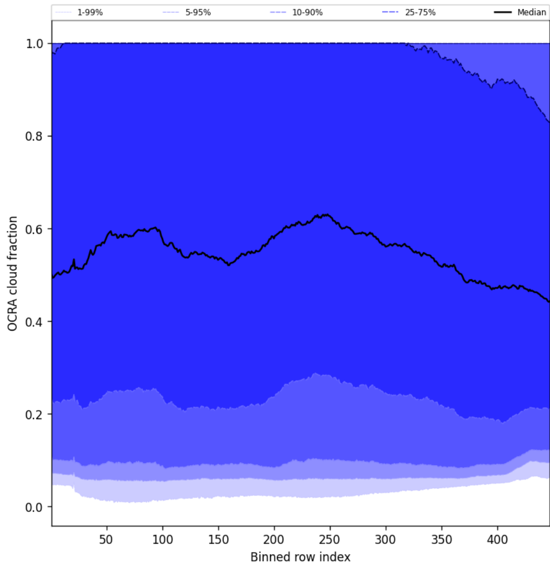
Figure 66: Along track statistics of “OCRA cloud fraction” for 2025-09-11 to 2025-09-13
