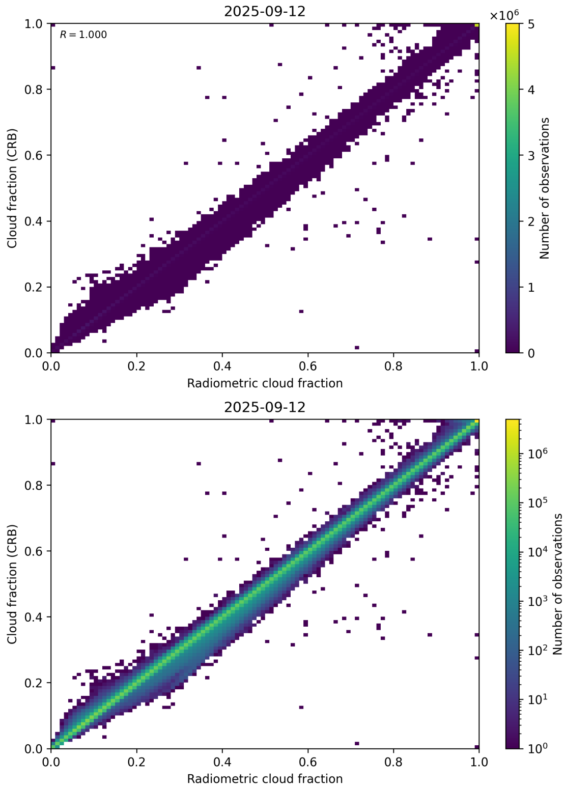
Figure 73: Scatter density plot of “Radiometric cloud fraction” against “Cloud fraction (CRB)” for 2025-09-11 to 2025-09-13.
