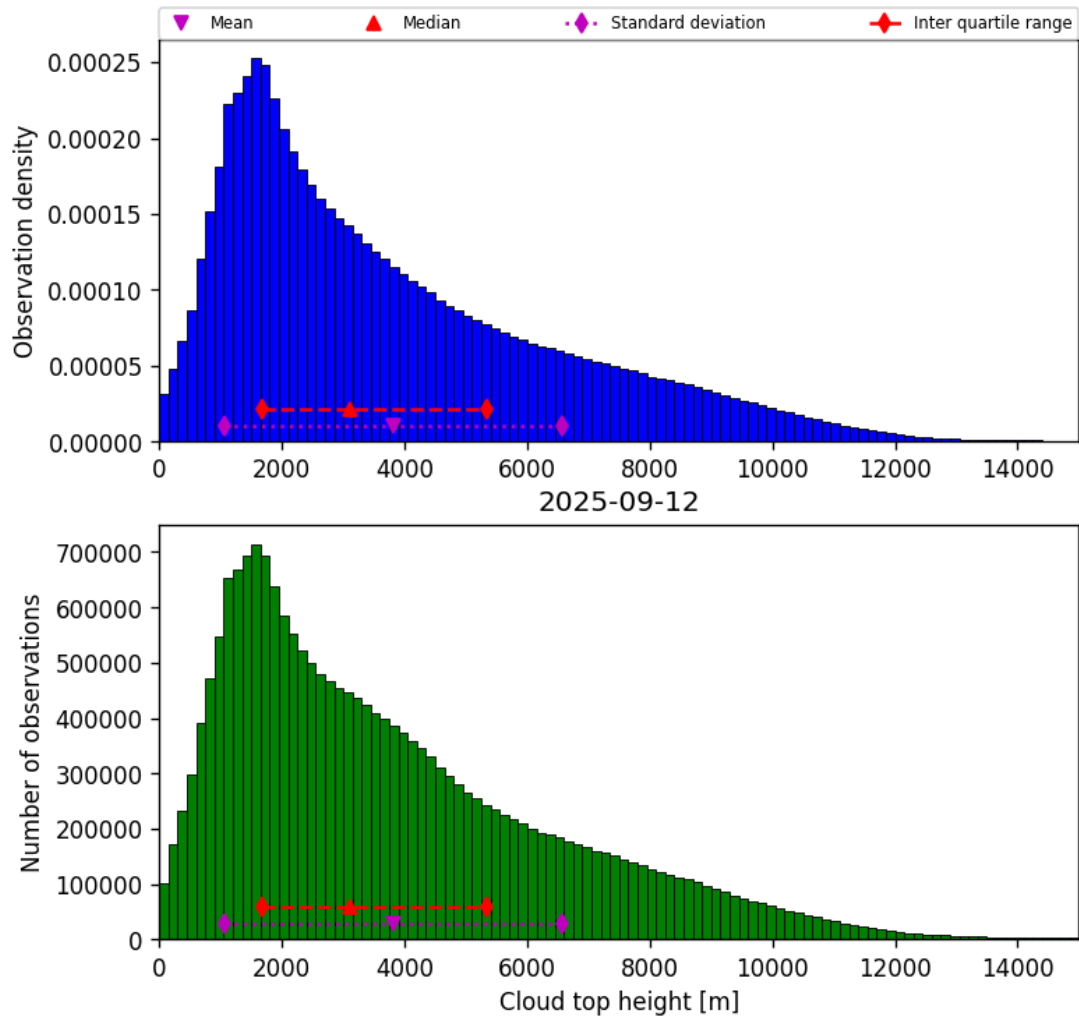
Figure 40: Histogram of “Cloud top height” for 2025-09-11 to 2025-09-13
