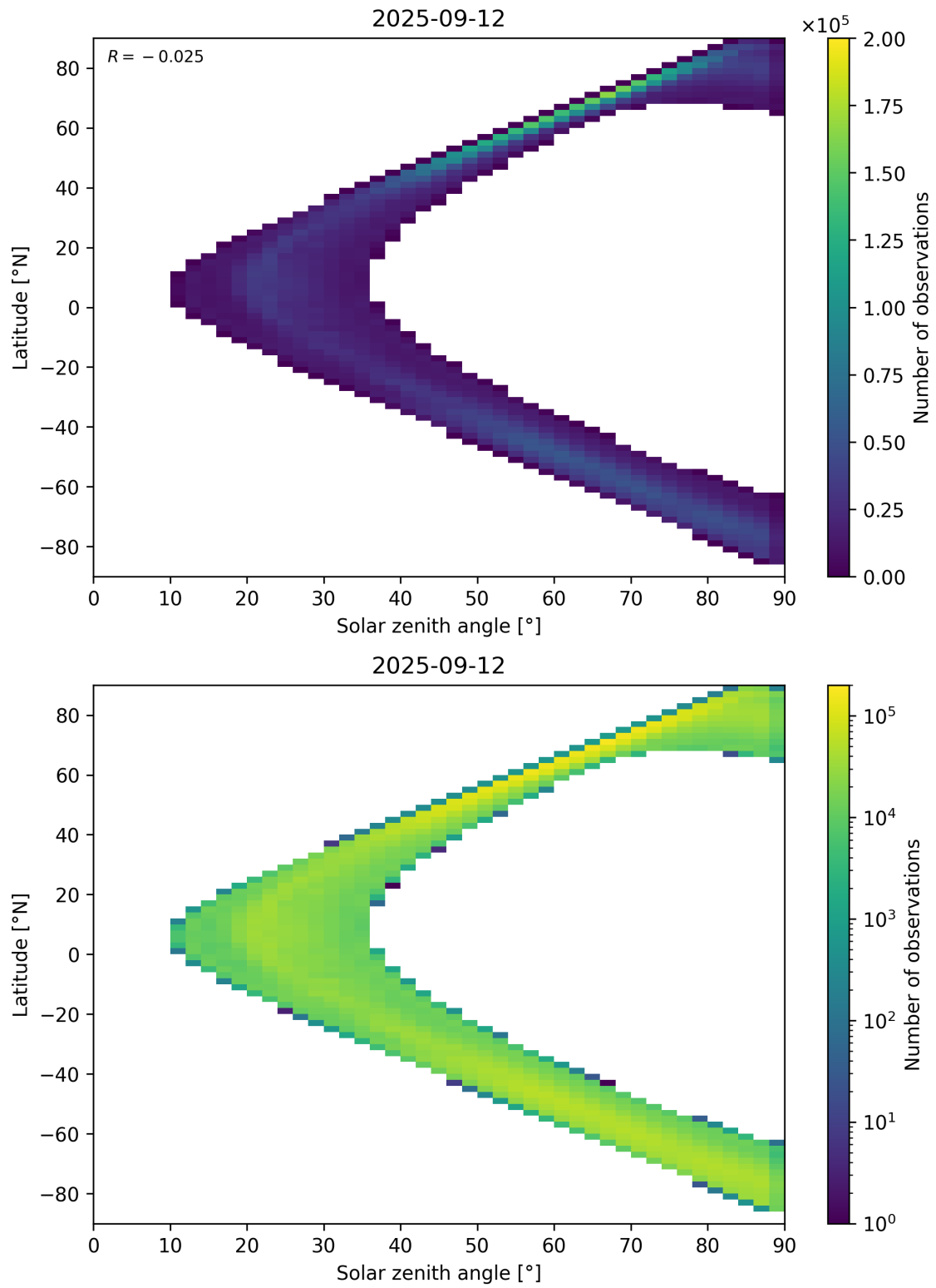
Figure 105: Scatter density plot of “Solar zenith angle” against “Latitude” for 2025-09-11 to 2025-09-13.
