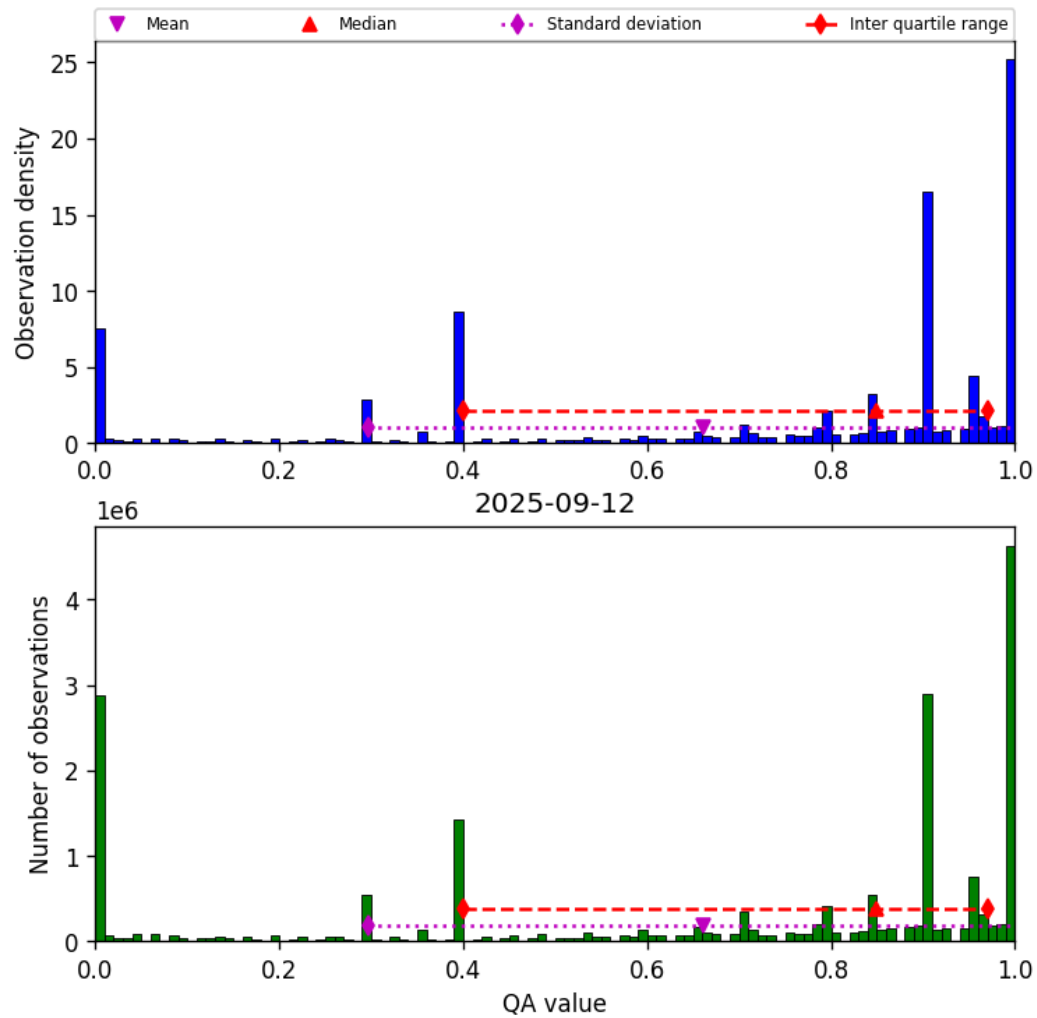
Figure 38: Histogram of “QA value” for 2025-09-11 to 2025-09-13
