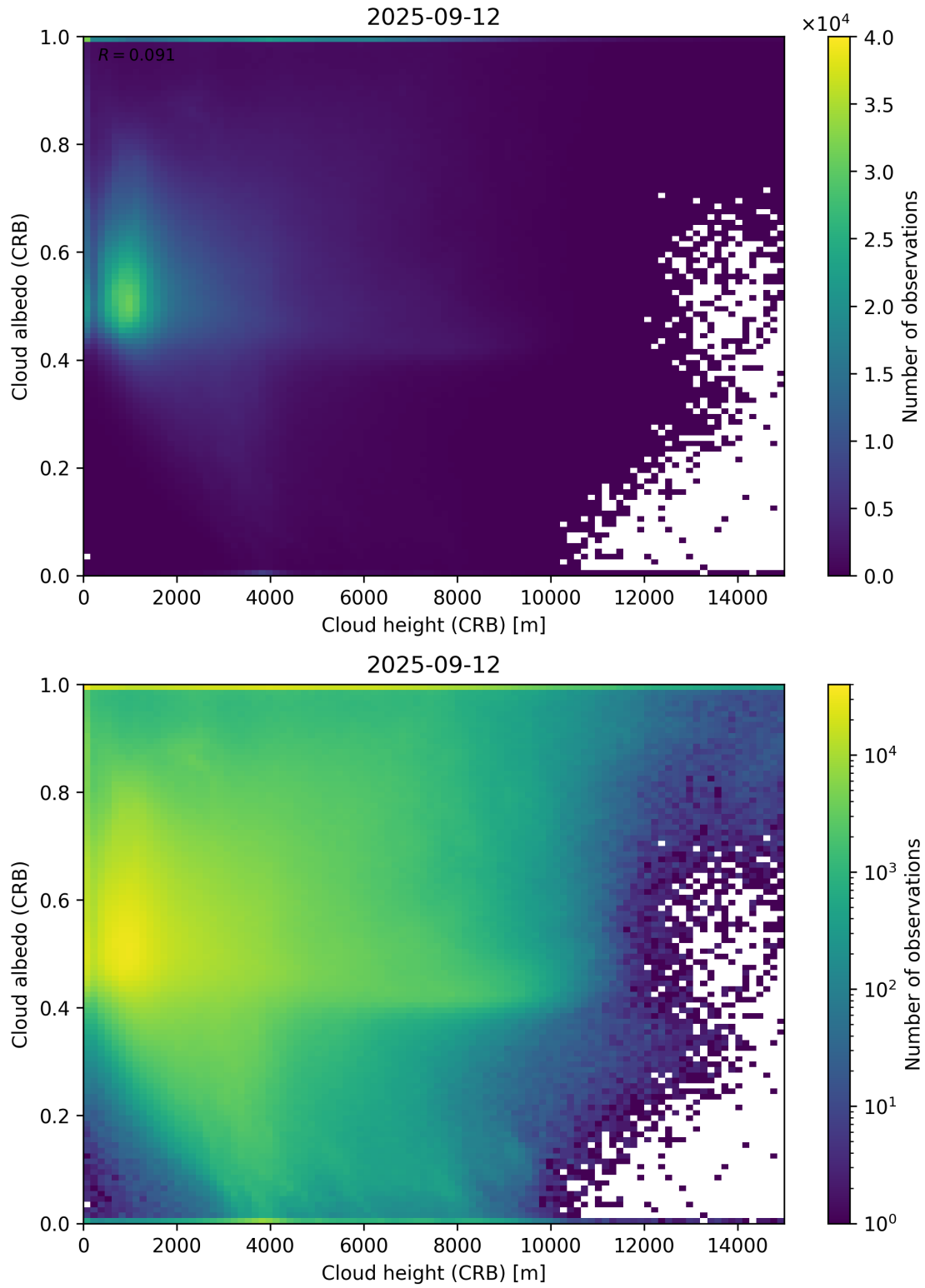
Figure 80: Scatter density plot of “Cloud height (CRB)” against “Cloud albedo (CRB)” for 2025-09-11 to 2025-09-13.
