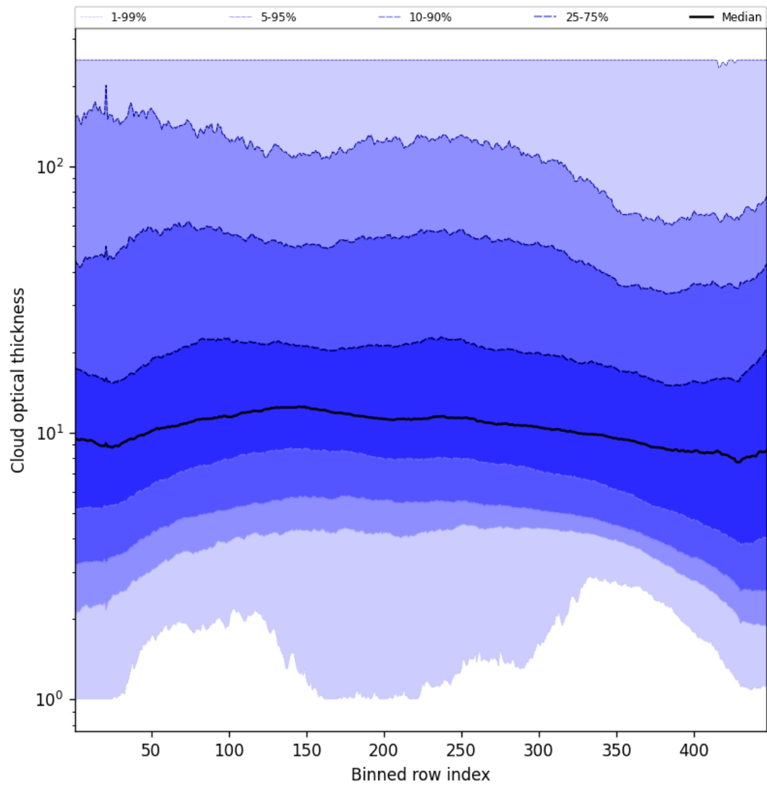
Figure 57: Along track statistics of “Cloud optical thickness” for 2025-09-11 to 2025-09-13
