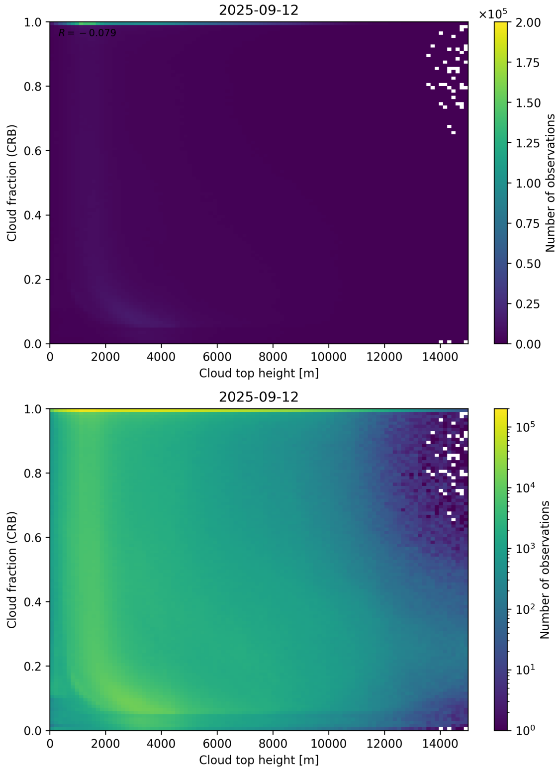
Figure 88: Scatter density plot of “Cloud top height” against “Cloud fraction (CRB)” for 2025-09-11 to 2025-09-13.
