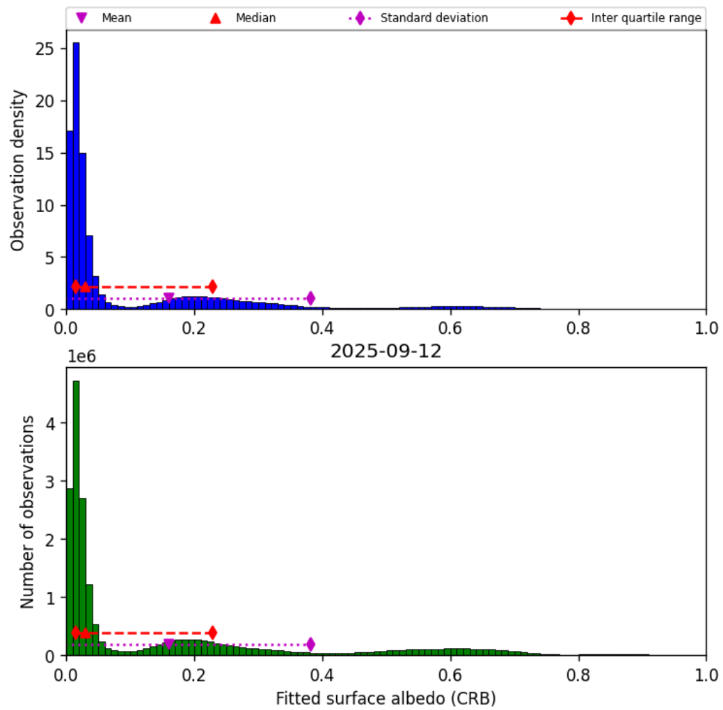
Figure 46: Histogram of “Fitted surface albedo (CRB)” for 2025-09-11 to 2025-09-13
