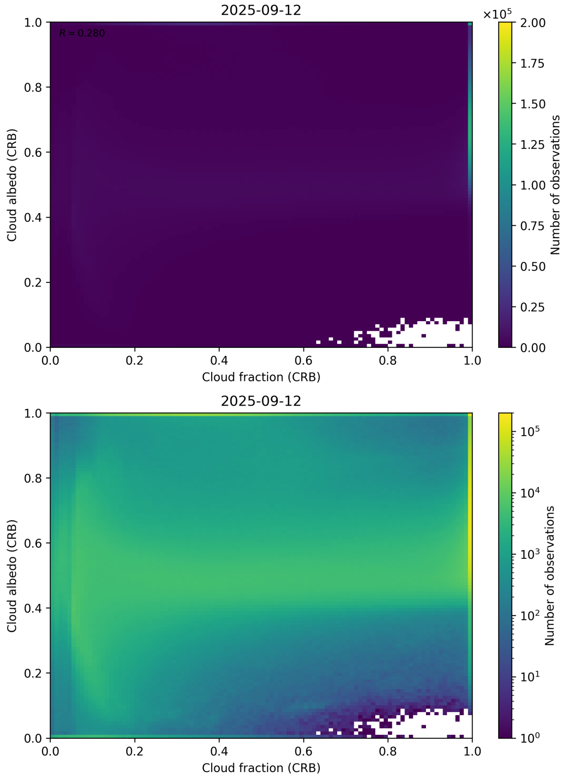
Figure 77: Scatter density plot of “Cloud fraction (CRB)” against “Cloud albedo (CRB)” for 2025-09-11 to 2025-09-13.
