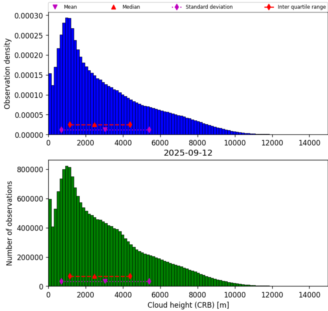
Figure 43: Histogram of “Cloud height (CRB)” for 2025-09-11 to 2025-09-13
