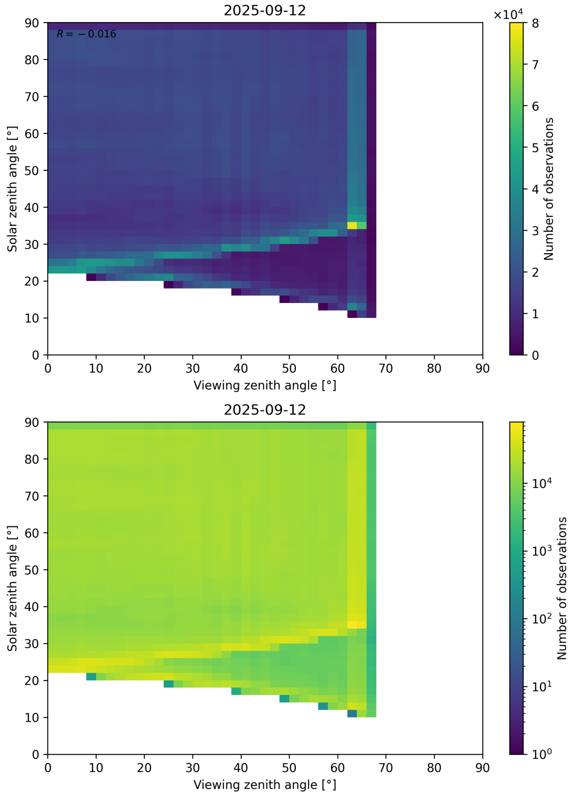
Figure 114: Scatter density plot of “Viewing zenith angle” against “Solar zenith angle” for 2025-09-11 to 2025-09-13.
