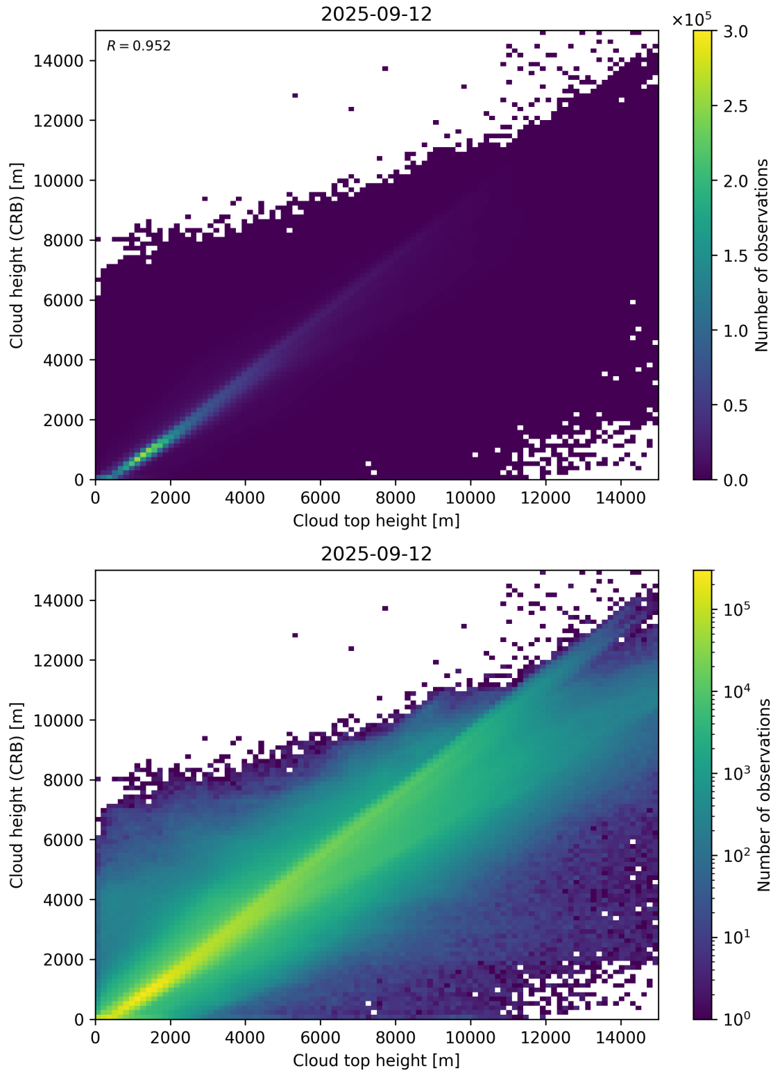
Figure 89: Scatter density plot of “Cloud top height” against “Cloud height (CRB)” for 2025-09-11 to 2025-09-13.
