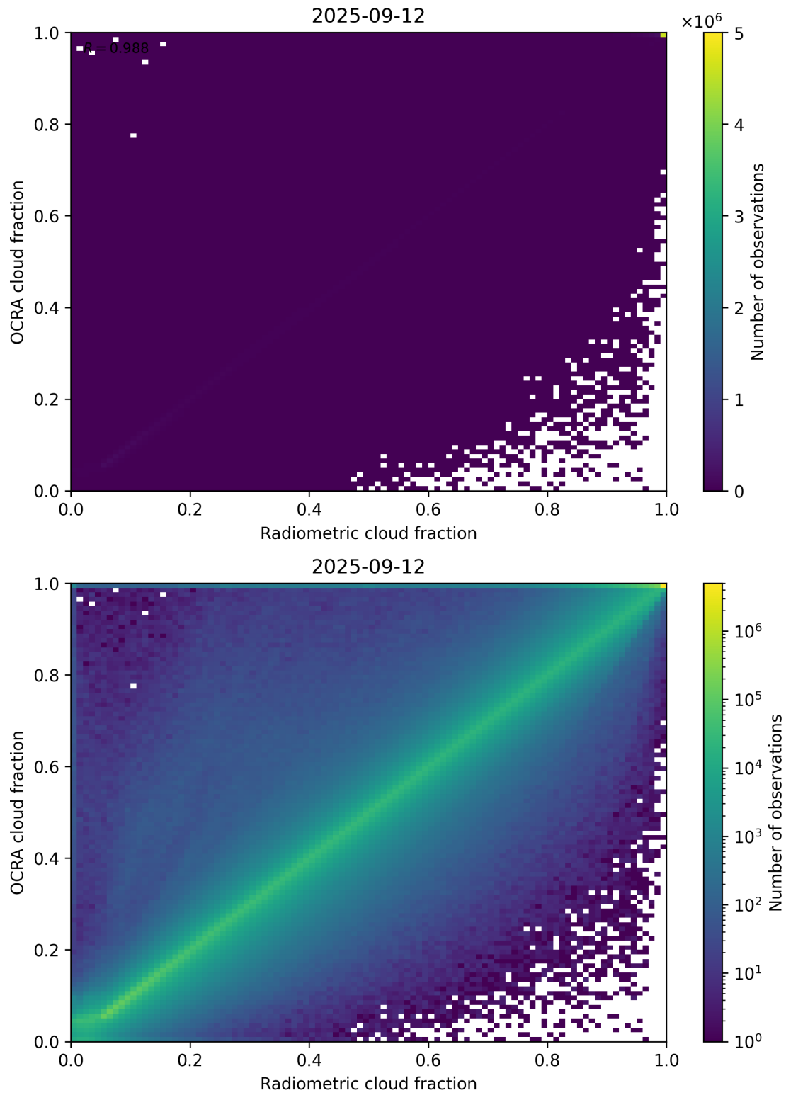
Figure 72: Scatter density plot of “Radiometric cloud fraction” against “OCRA cloud fraction” for 2025-09-11 to 2025-09-13.
