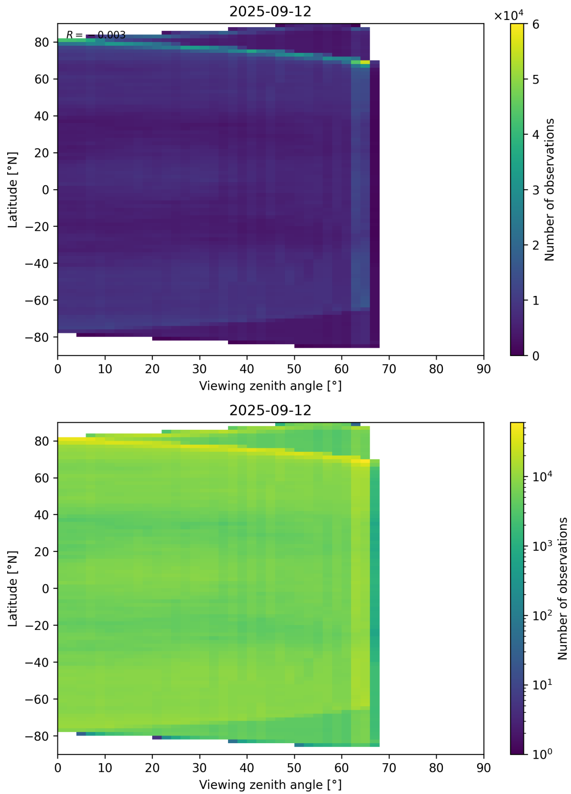
Figure 113: Scatter density plot of “Viewing zenith angle” against “Latitude” for 2025-09-11 to 2025-09-13.
