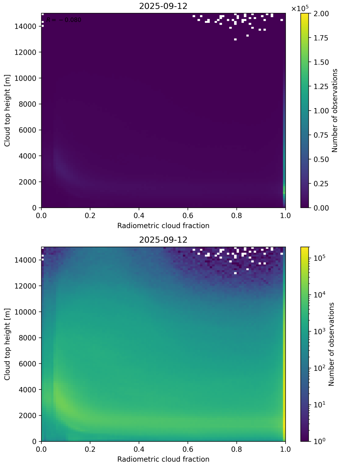
Figure 76: Scatter density plot of “Radiometric cloud fraction” against “Cloud top height” for 2025-09-11 to 2025-09-13.
