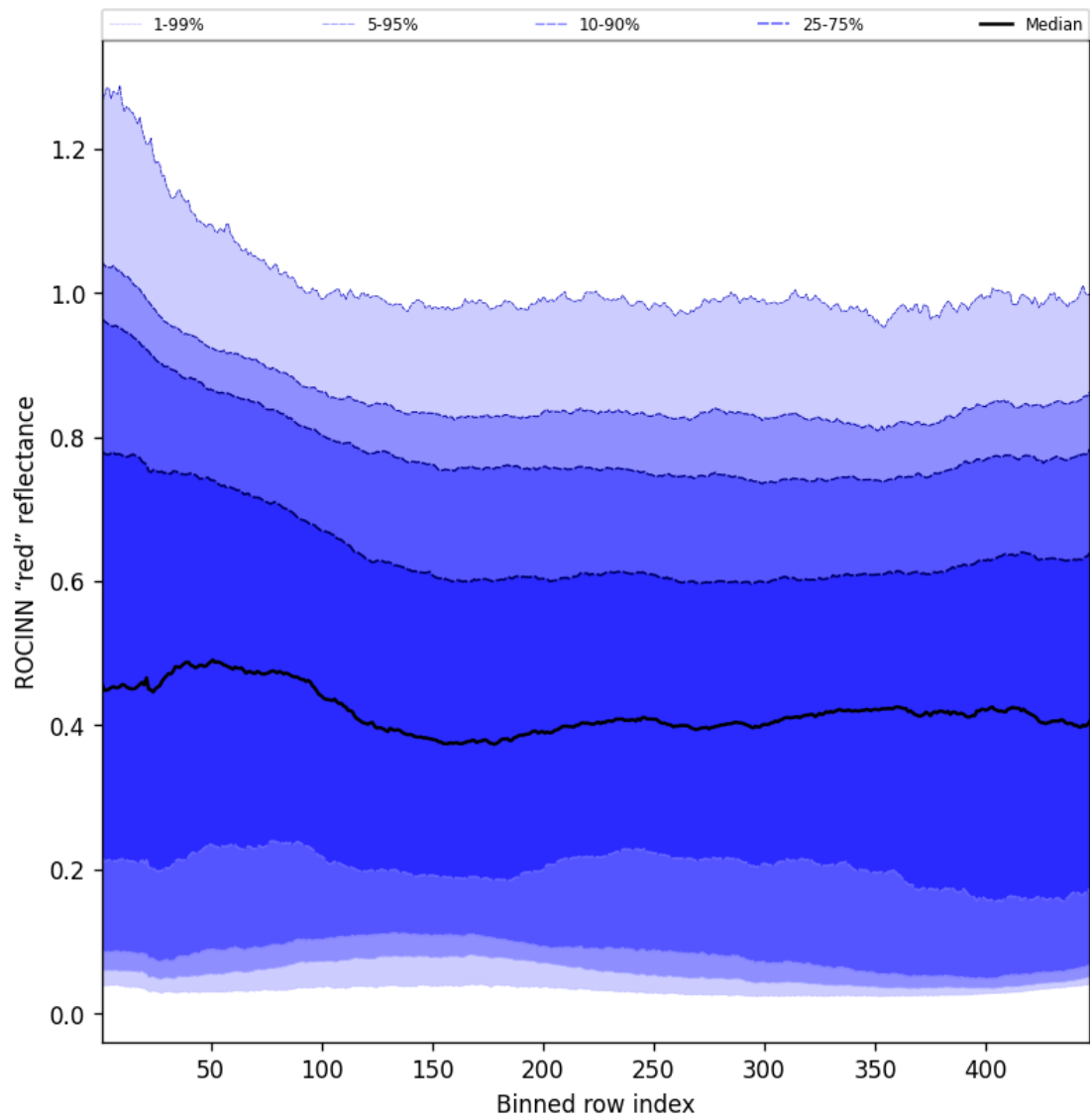
Figure 69: Along track statistics of "ROCINN "red" reflectance" for 2025-09-11 to 2025-09-13
