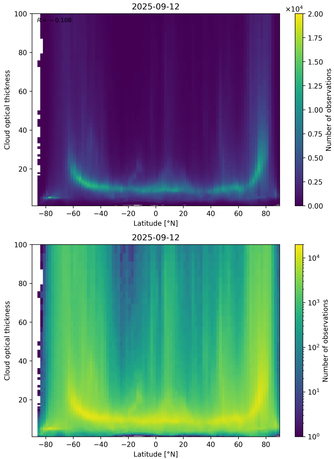
Figure 96: Scatter density plot of “Latitude” against “Cloud optical thickness” for 2025-09-11 to 2025-09-13.
