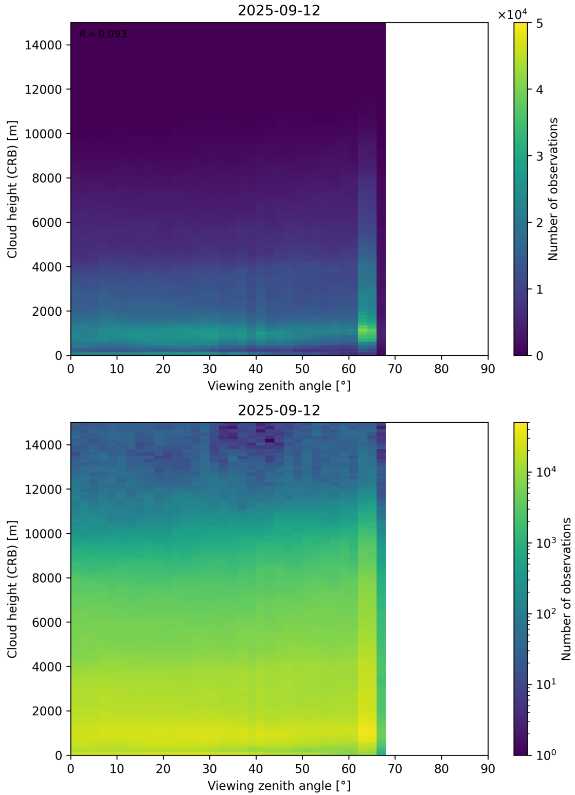
Figure 110: Scatter density plot of “Viewing zenith angle” against “Cloud height (CRB)” for 2025-09-11 to 2025-09-13.
