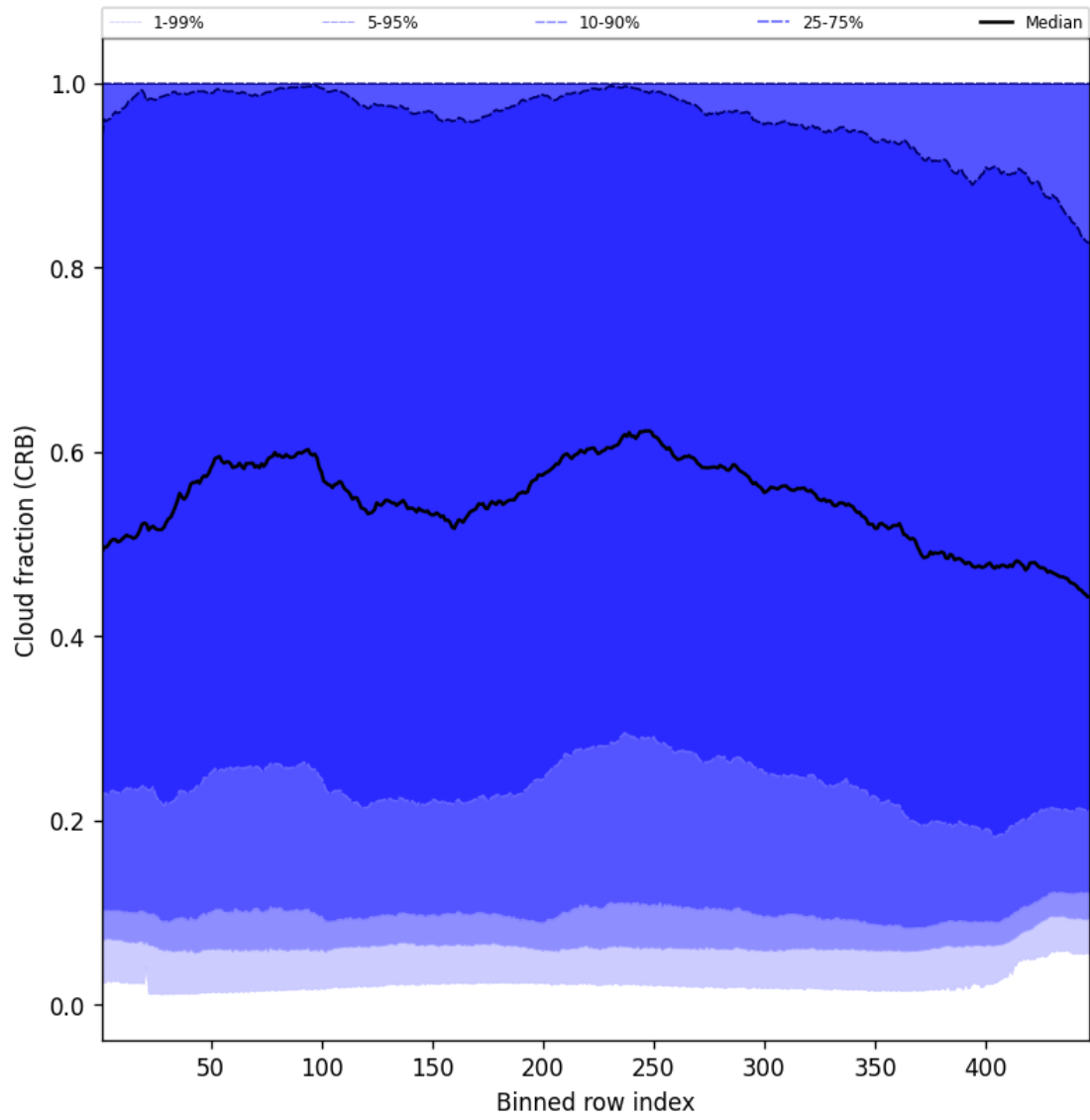
Figure 58: Along track statistics of “Cloud fraction (CRB)” for 2025-09-11 to 2025-09-13
