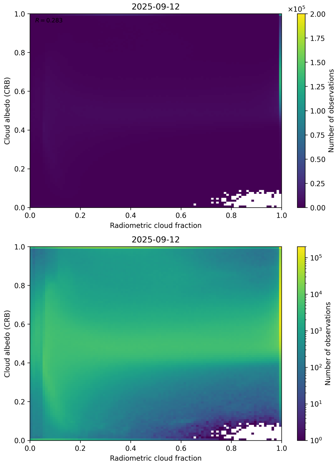
Figure 71: Scatter density plot of “Radiometric cloud fraction” against “Cloud albedo (CRB)” for 2025-09-11 to 2025-09-13.
