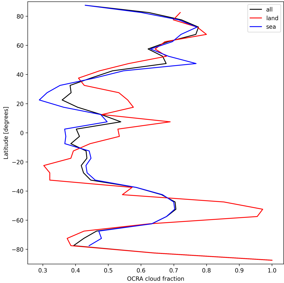
Figure 34: Zonal average of “OCRA cloud fraction” for 2025-09-11 to 2025-09-13.
