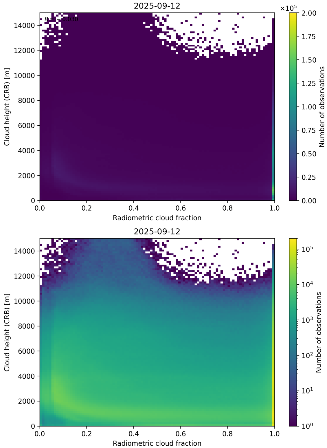
Figure 74: Scatter density plot of “Radiometric cloud fraction” against “Cloud height (CRB)” for 2025-09-11 to 2025-09-13.
