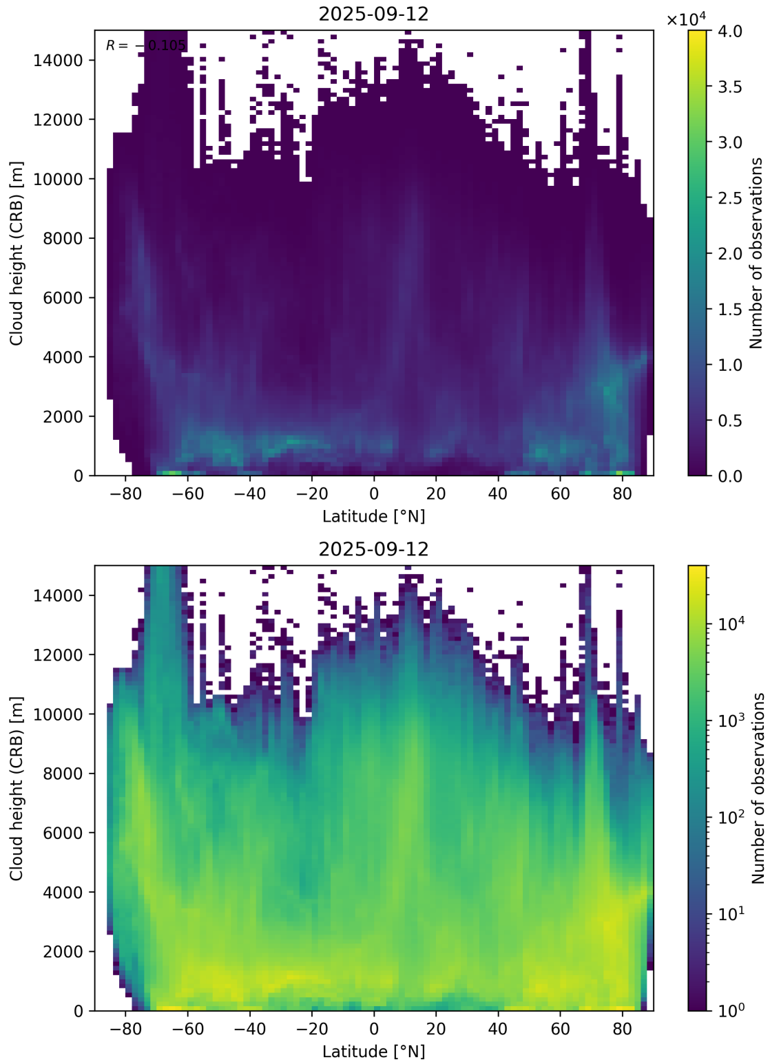
Figure 95: Scatter density plot of “Latitude” against “Cloud height (CRB)” for 2025-09-11 to 2025-09-13.
