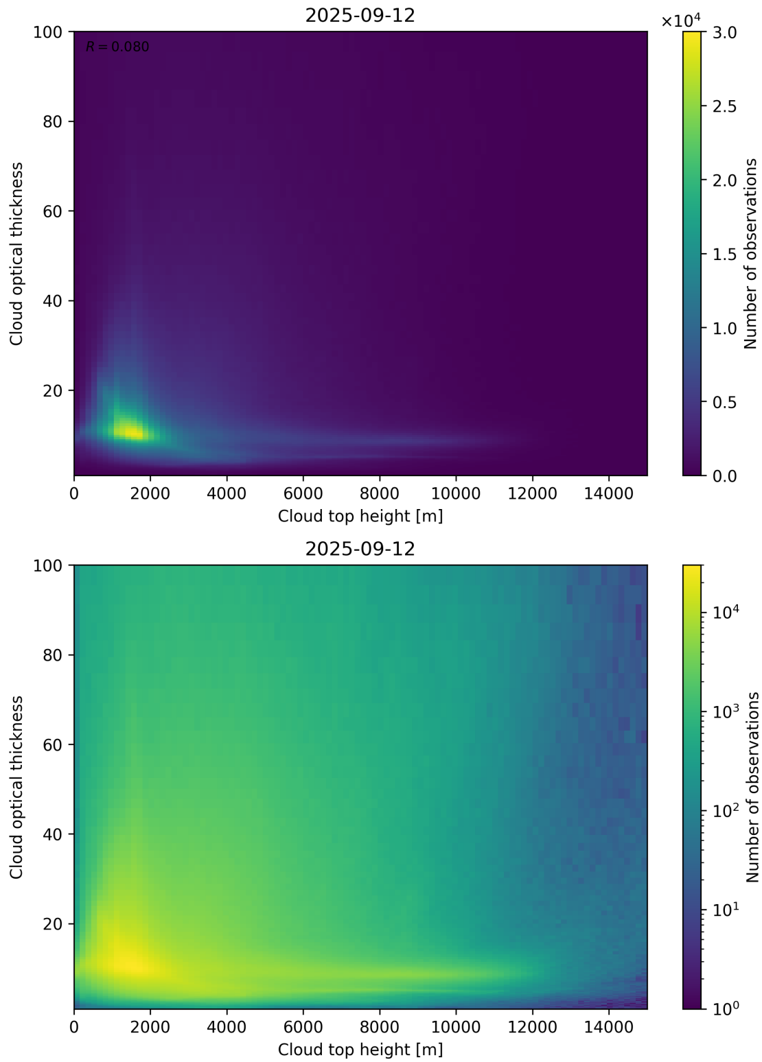
Figure 90: Scatter density plot of “Cloud top height” against “Cloud optical thickness” for 2025-09-11 to 2025-09-13.
