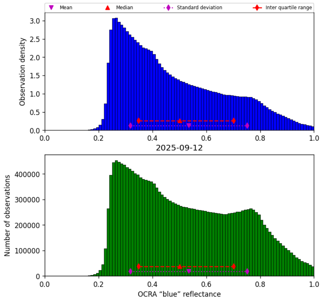
Figure 51: Histogram of “OCRA “blue” reflectance” for 2025-09-11 to 2025-09-13
