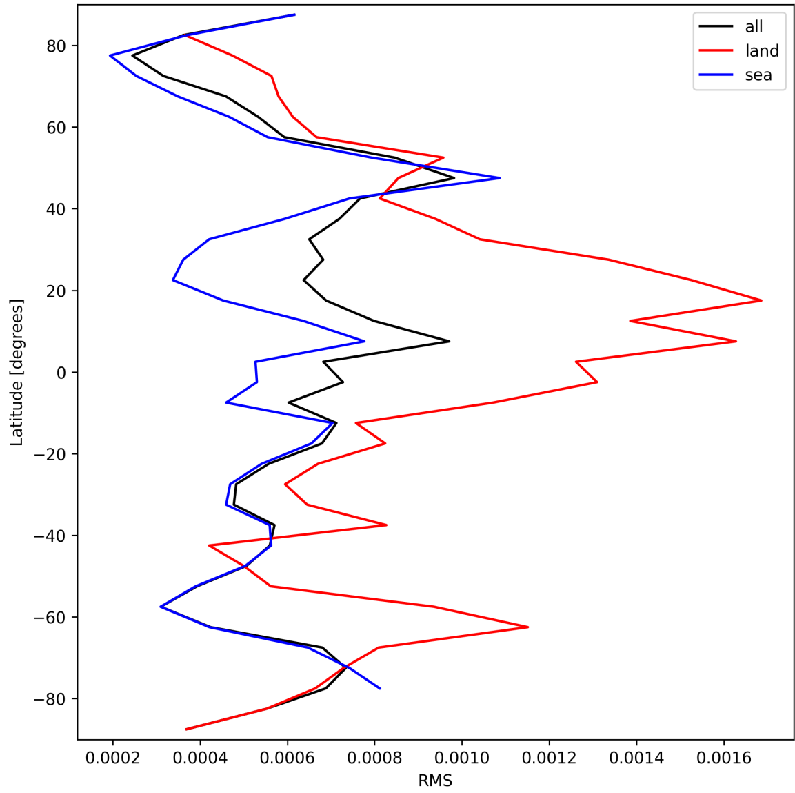
Figure 31: Zonal average of “RMS” for 2025-09-11 to 2025-09-13.
