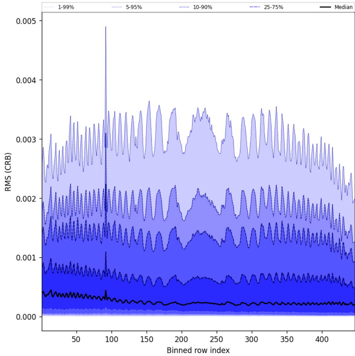
Figure 64: Along track statistics of “RMS (CRB)” for 2025-09-11 to 2025-09-13
