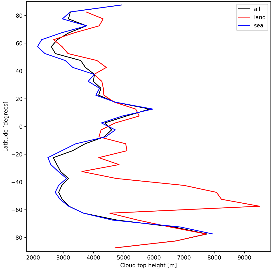
Figure 24: Zonal average of “Cloud top height” for 2025-09-11 to 2025-09-13.
