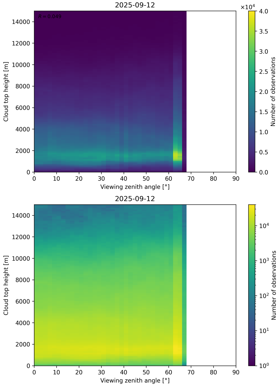
Figure 112: Scatter density plot of “Viewing zenith angle” against “Cloud top height” for 2025-09-11 to 2025-09-13.
