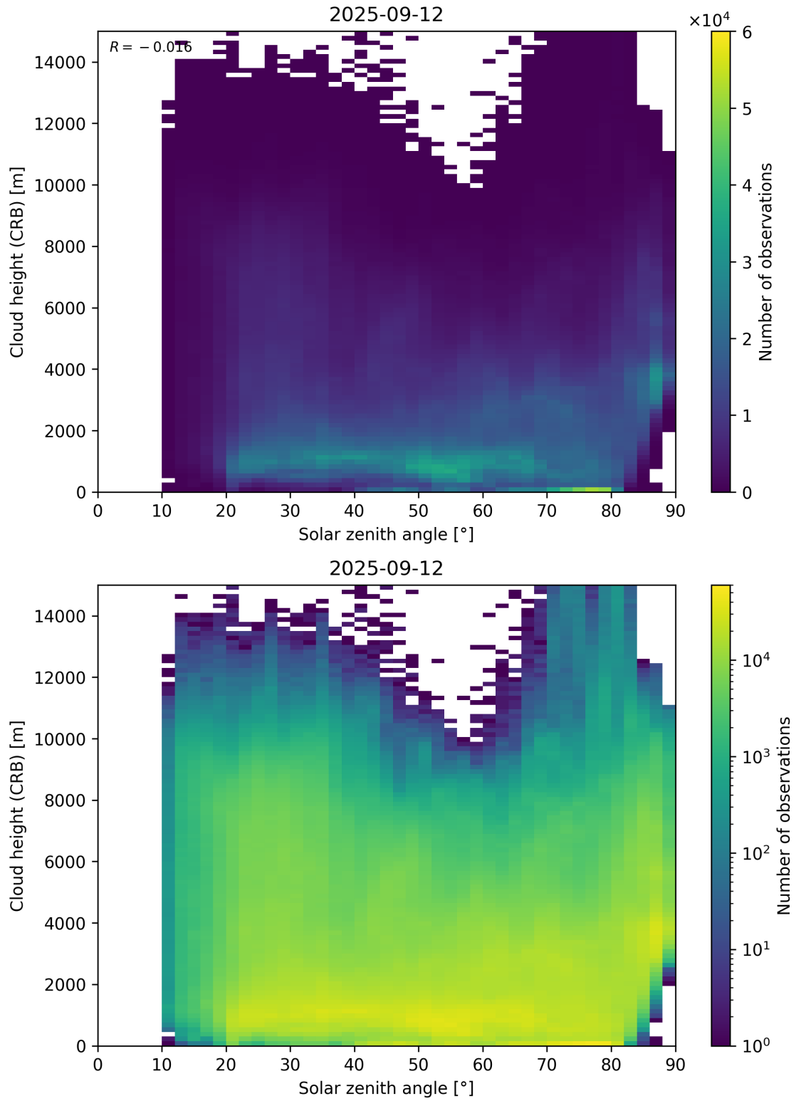
Figure 102: Scatter density plot of “Solar zenith angle” against “Cloud height (CRB)” for 2025-09-11 to 2025-09-13.
