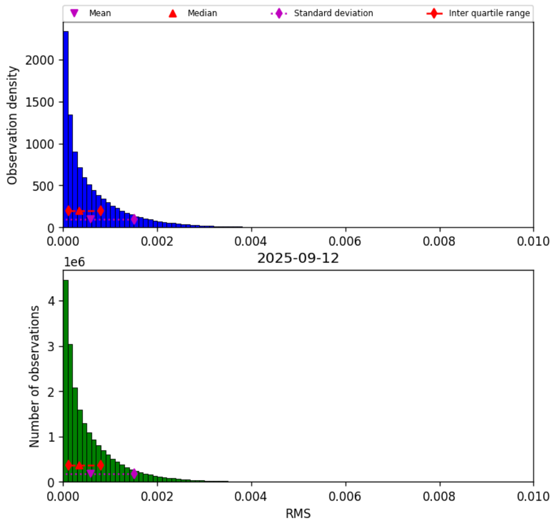
Figure 47: Histogram of “RMS” for 2025-09-11 to 2025-09-13
