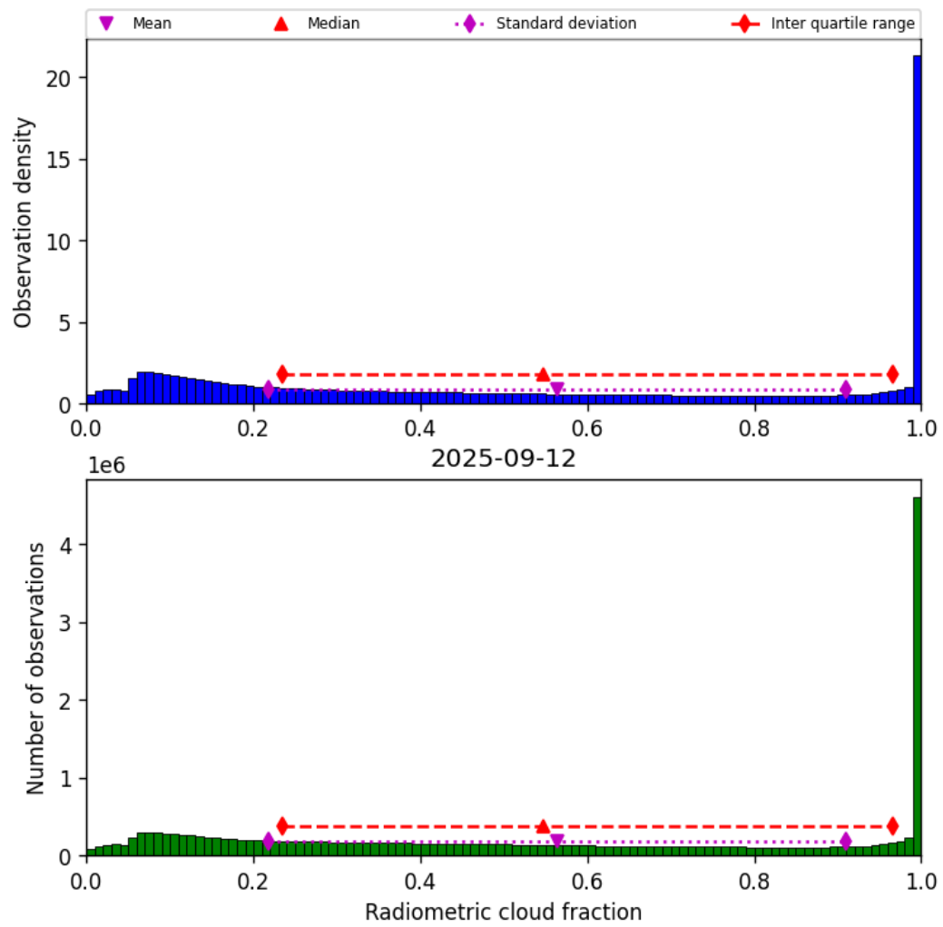
Figure 39: Histogram of “Radiometric cloud fraction” for 2025-09-11 to 2025-09-13
