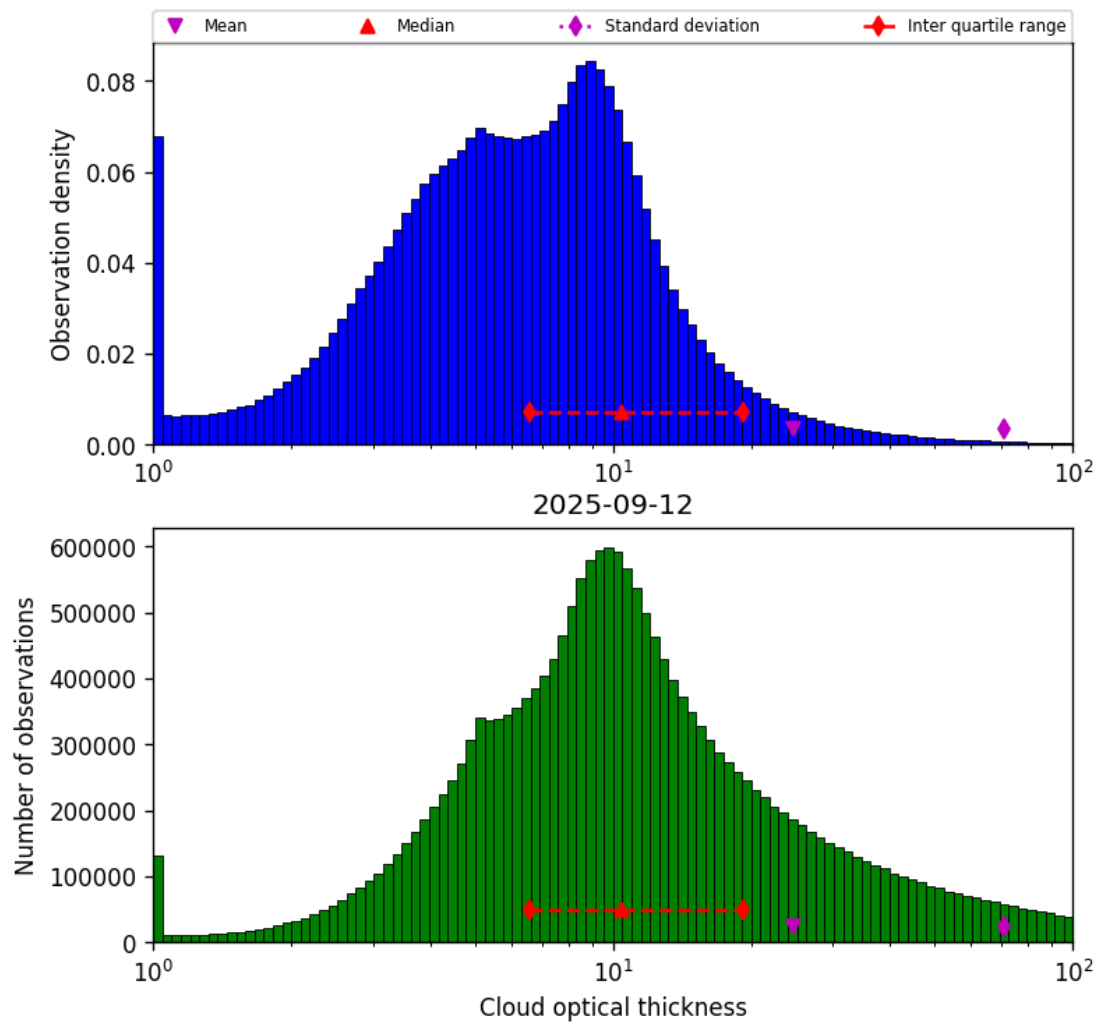
Figure 41: Histogram of “Cloud optical thickness” for 2025-09-11 to 2025-09-13
