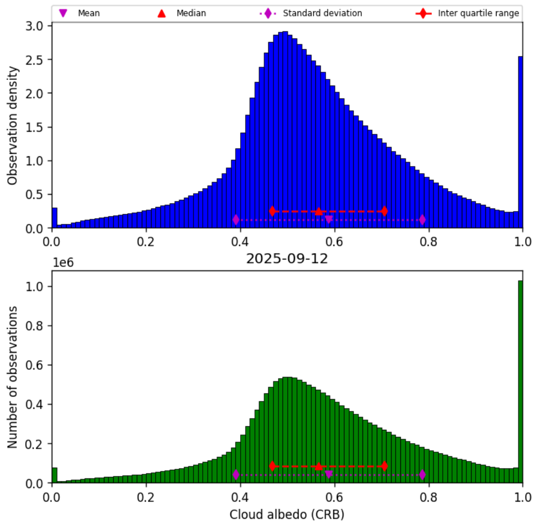
Figure 44: Histogram of “Cloud albedo (CRB)” for 2025-09-11 to 2025-09-13
