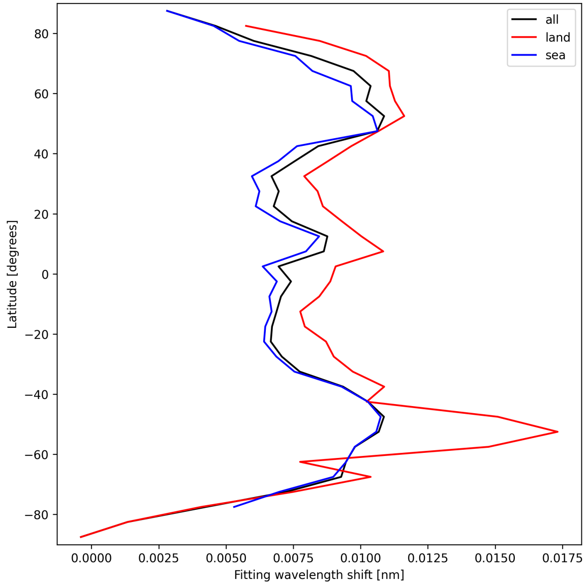
Figure 33: Zonal average of “Fitting wavelength shift” for 2025-09-11 to 2025-09-13.
