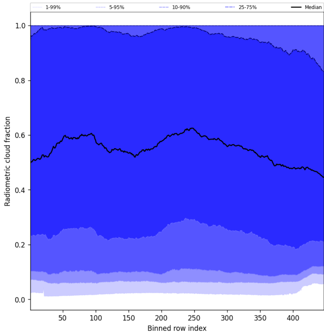
Figure 55: Along track statistics of “Radiometric cloud fraction” for 2025-09-11 to 2025-09-13
