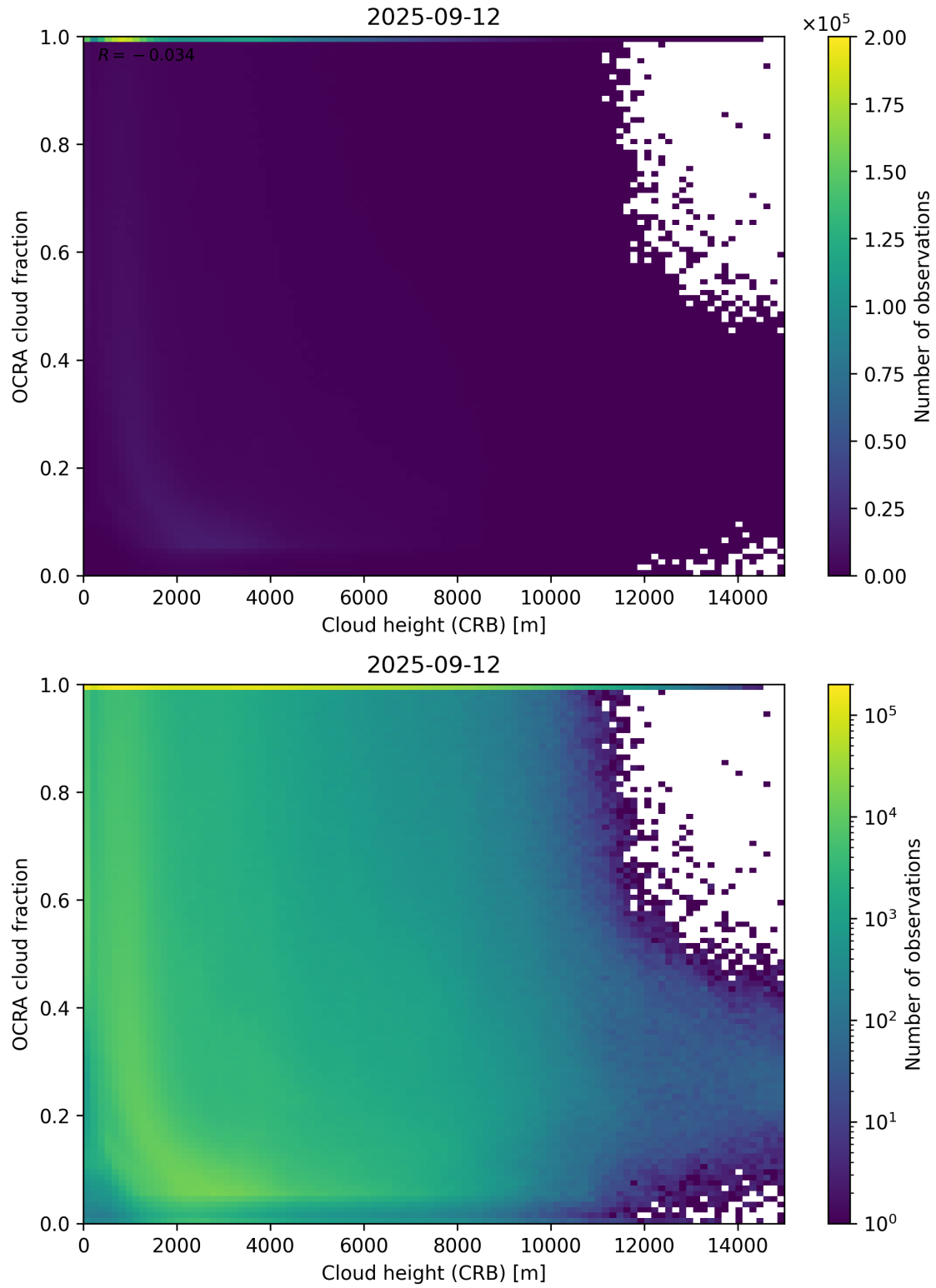
Figure 81: Scatter density plot of “Cloud height (CRB)” against “OCRA cloud fraction” for 2025-09-11 to 2025-09-13.
