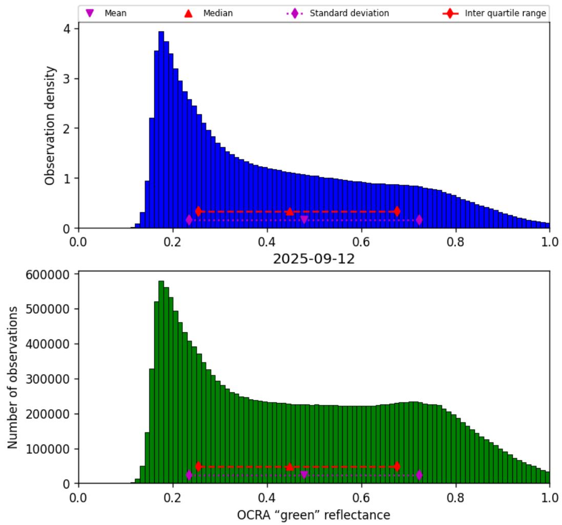
Figure 52: Histogram of “OCRA “green” reflectance” for 2025-09-11 to 2025-09-13
