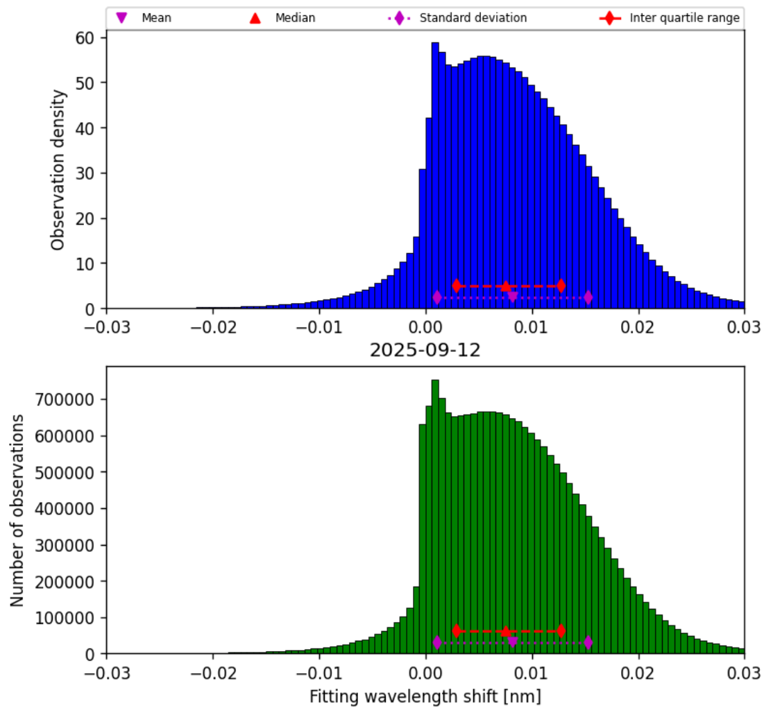
Figure 49: Histogram of “Fitting wavelength shift” for 2025-09-11 to 2025-09-13
