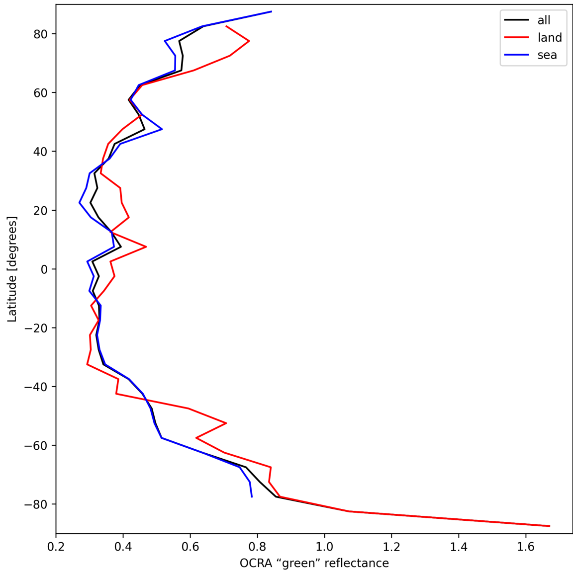
Figure 36: Zonal average of “OCRA “green” reflectance” for 2025-09-11 to 2025-09-13.
