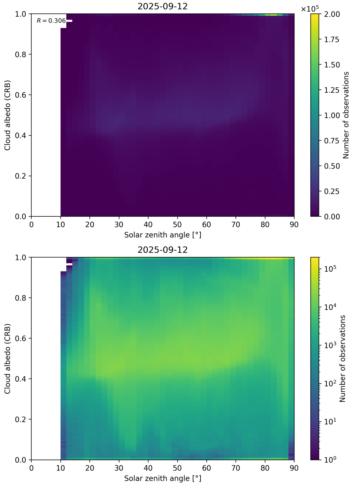
Figure 98: Scatter density plot of “Solar zenith angle” against “Cloud albedo (CRB)” for 2025-09-11 to 2025-09-13.
