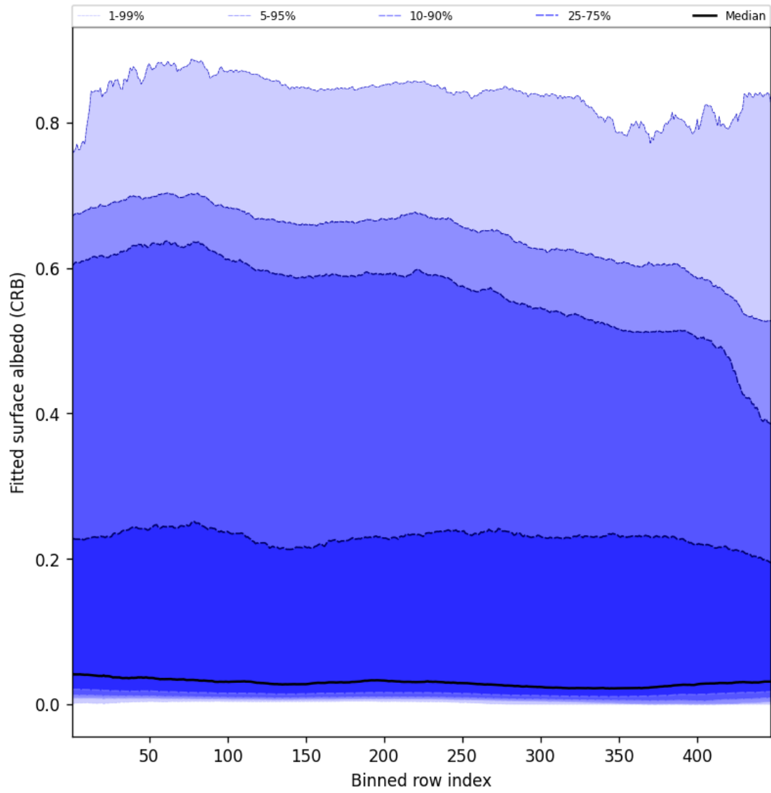
Figure 62: Along track statistics of “Fitted surface albedo (CRB)” for 2025-09-11 to 2025-09-13
