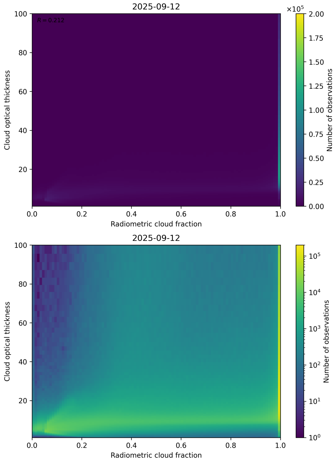
Figure 75: Scatter density plot of “Radiometric cloud fraction” against “Cloud optical thickness” for 2025-09-11 to 2025-09-13.
