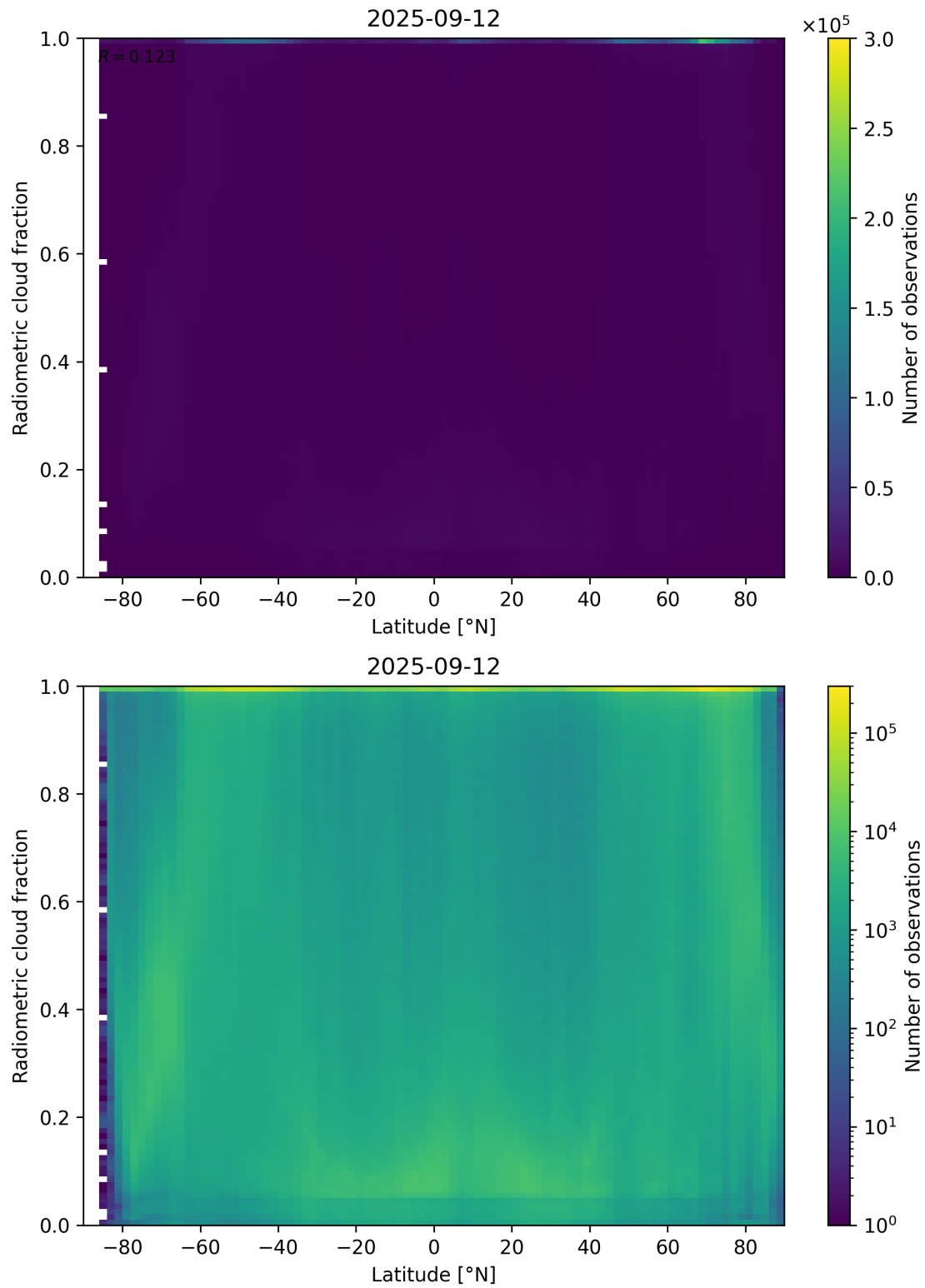
Figure 92: Scatter density plot of “Latitude” against “Radiometric cloud fraction” for 2025-09-11 to 2025-09-13.
