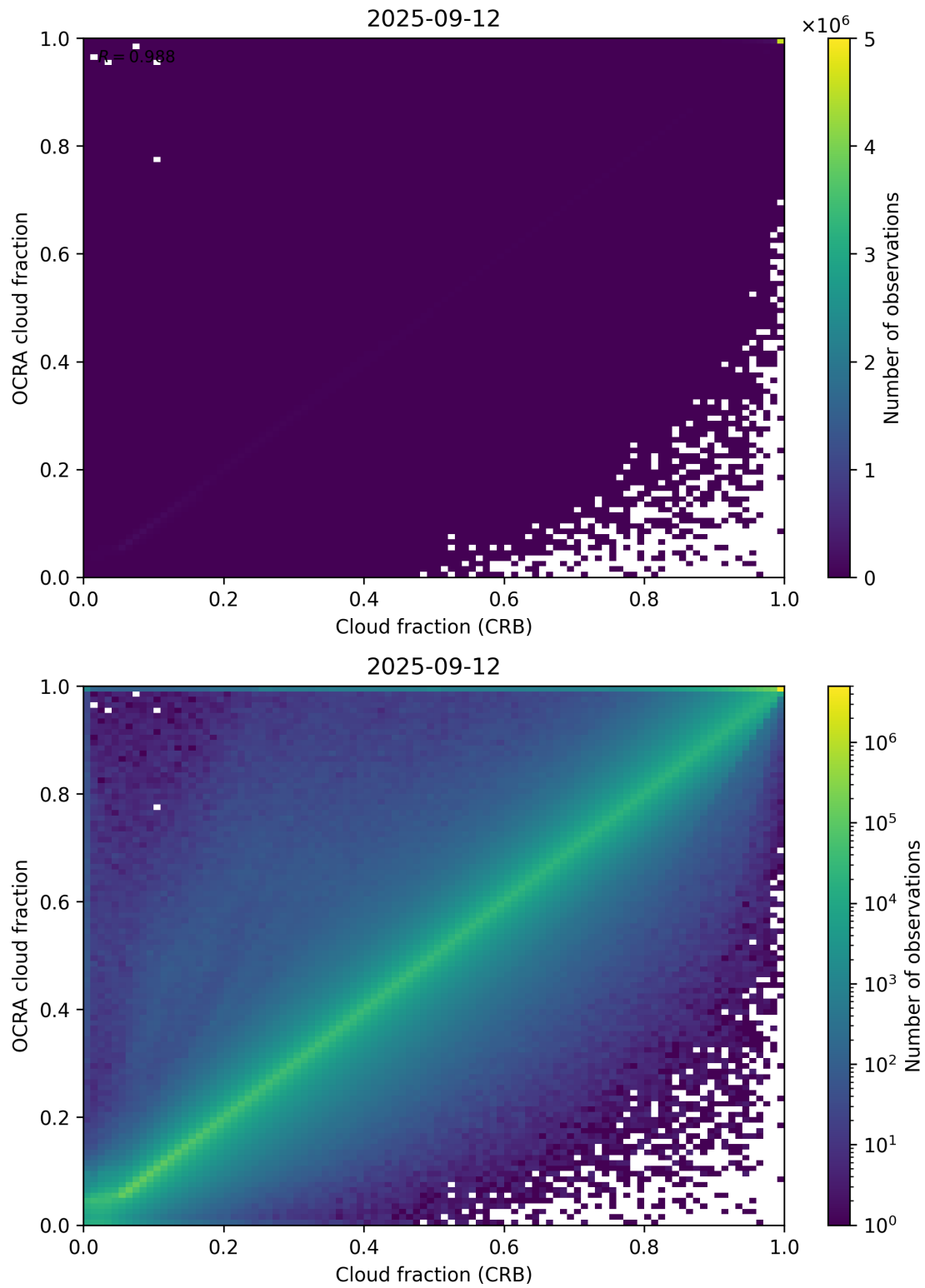
Figure 78: Scatter density plot of “Cloud fraction (CRB)” against “OCRA cloud fraction” for 2025-09-11 to 2025-09-13.
