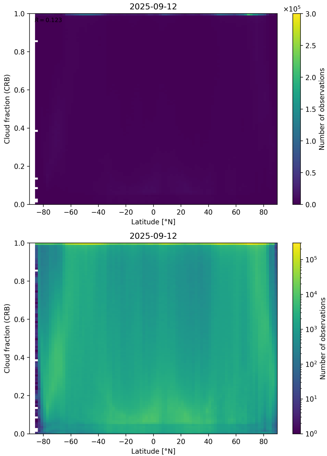
Figure 94: Scatter density plot of “Latitude” against “Cloud fraction (CRB)” for 2025-09-11 to 2025-09-13.
