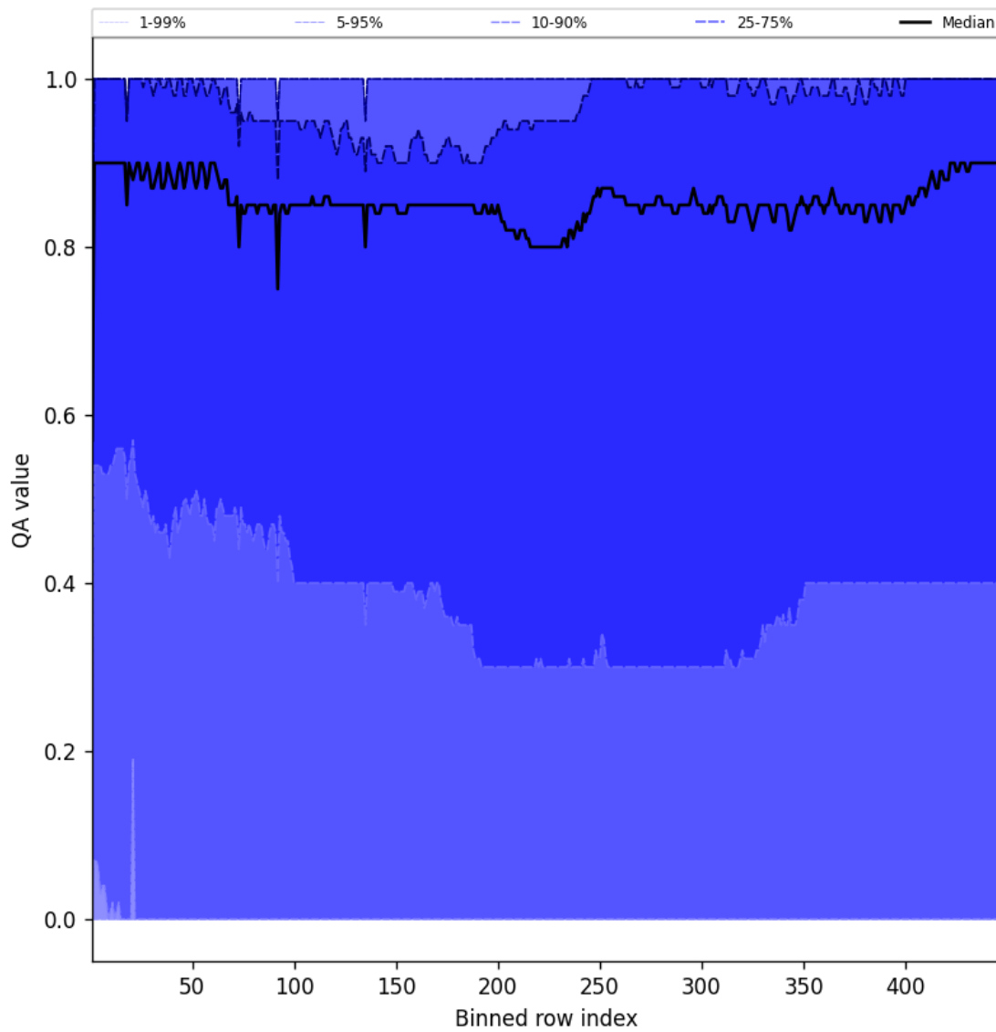
Figure 54: Along track statistics of “QA value” for 2025-09-12 to 2025-09-14
