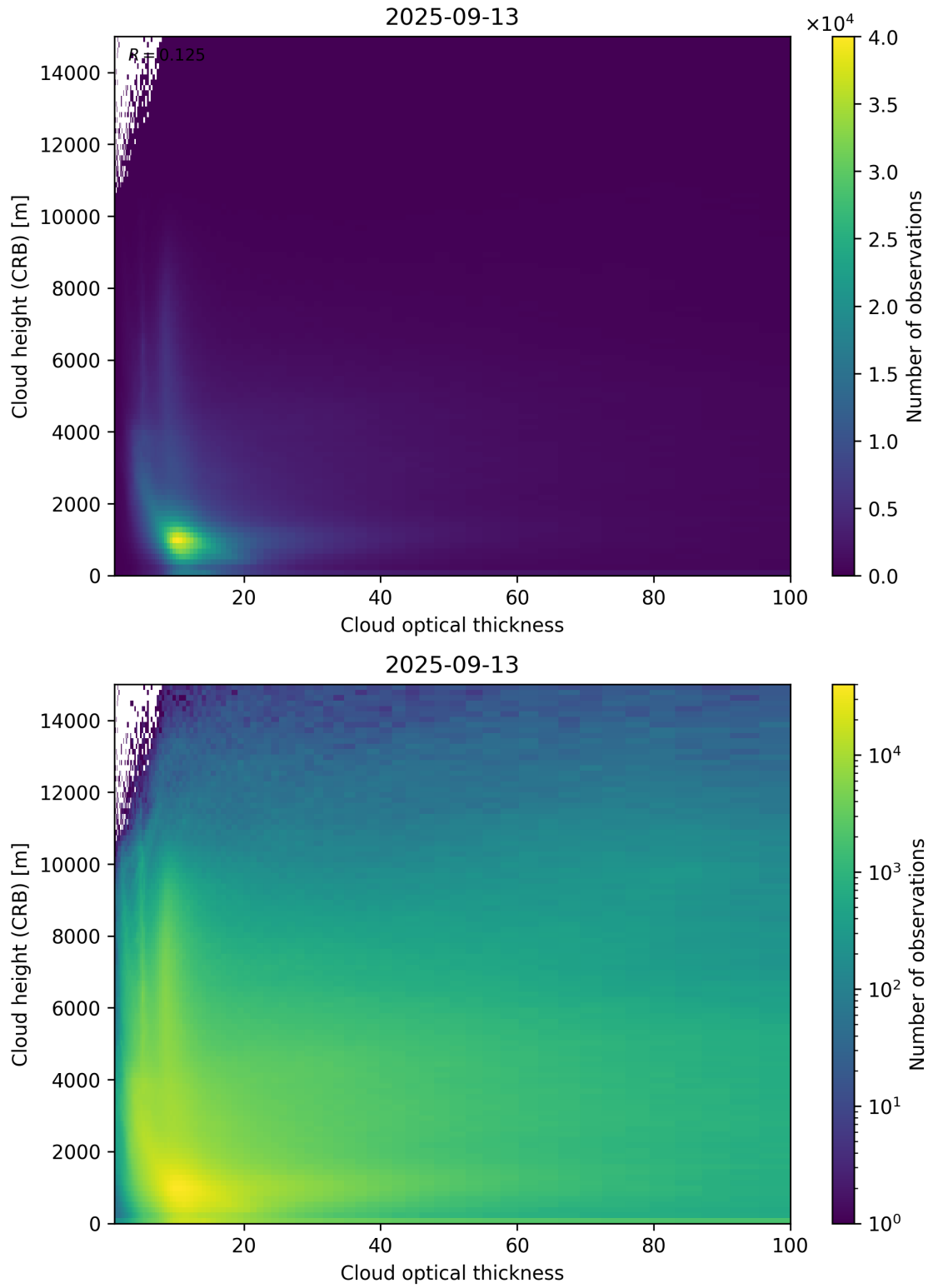
Figure 85: Scatter density plot of “Cloud optical thickness” against “Cloud height (CRB)” for 2025-09-12 to 2025-09-14.
