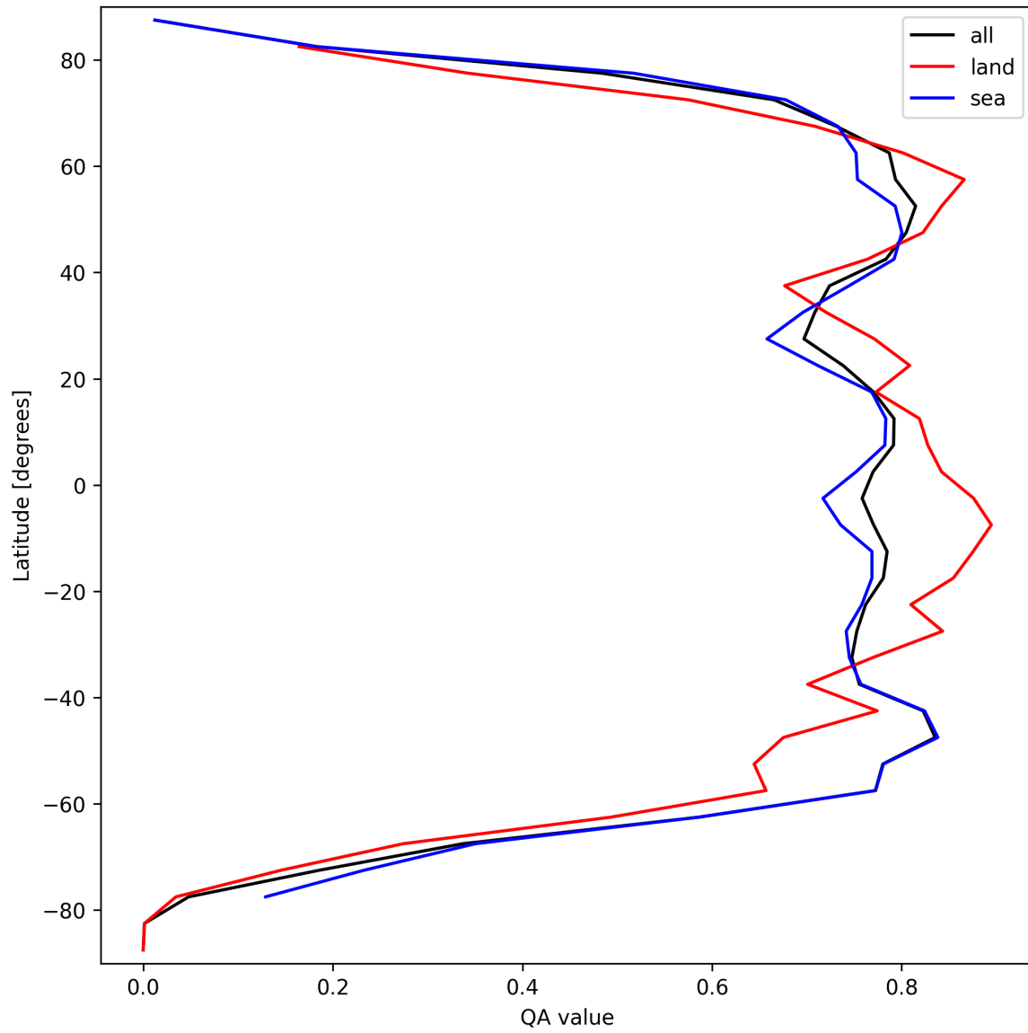
Figure 22: Zonal average of “QA value” for 2025-09-12 to 2025-09-14.
