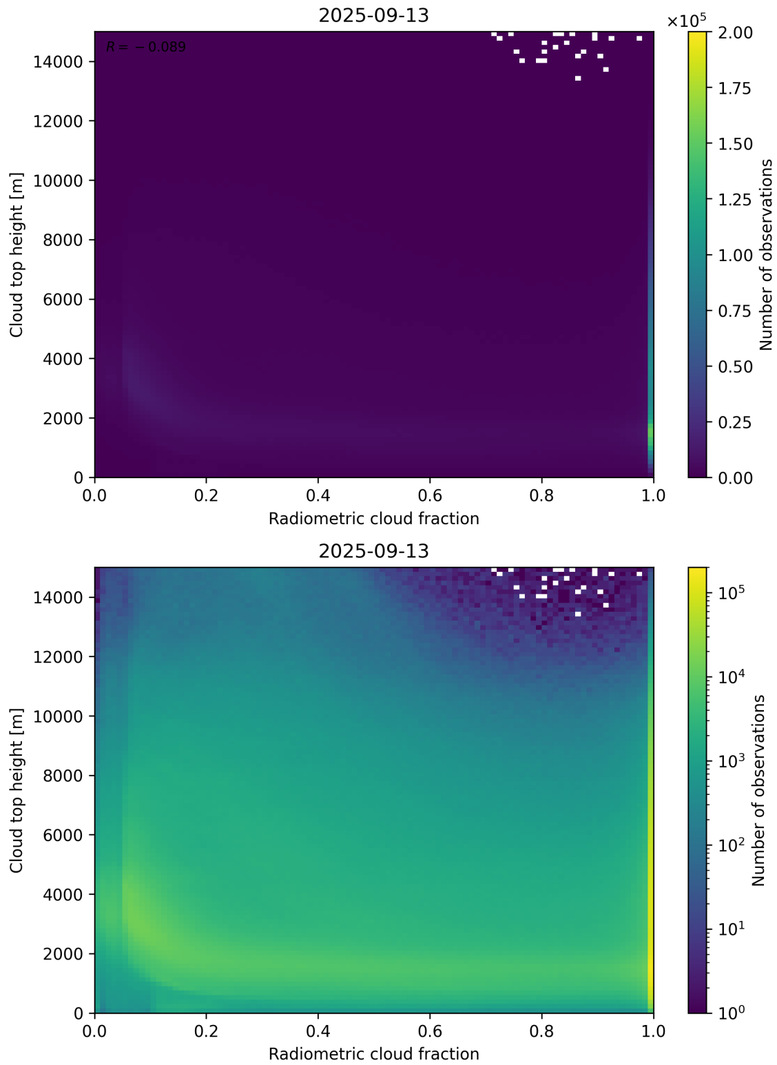
Figure 76: Scatter density plot of “Radiometric cloud fraction” against “Cloud top height” for 2025-09-12 to 2025-09-14.
