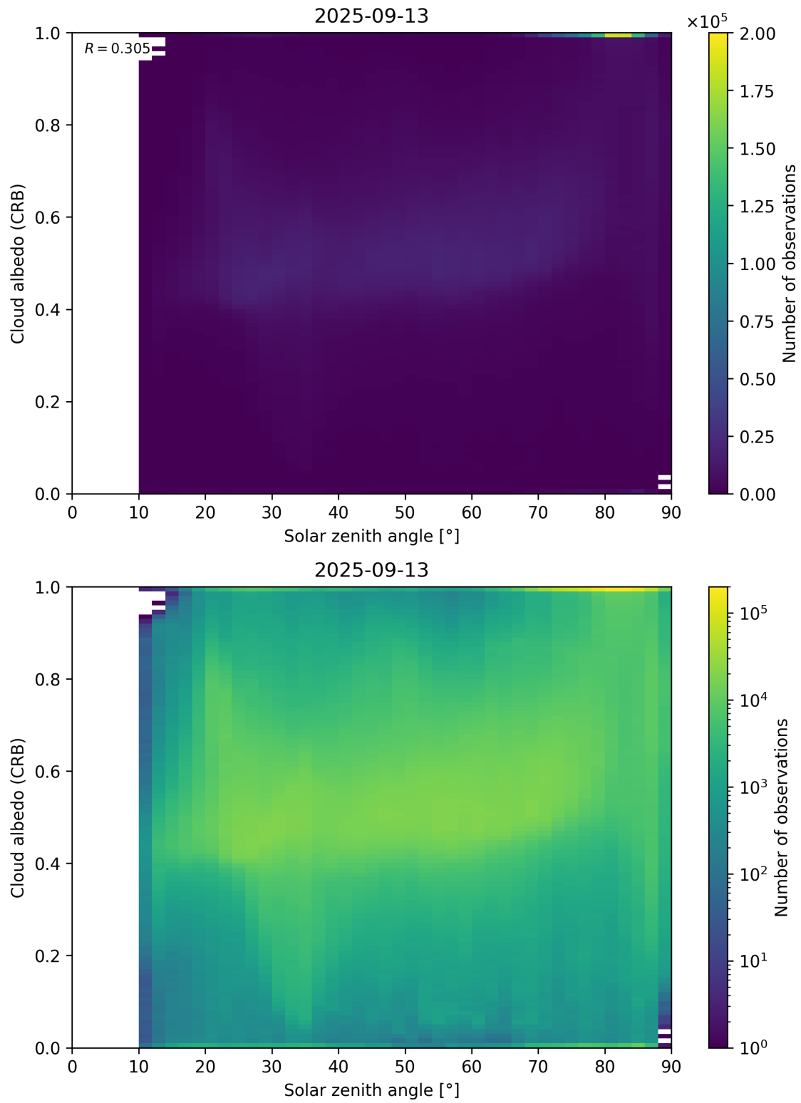
Figure 98: Scatter density plot of “Solar zenith angle” against “Cloud albedo (CRB)” for 2025-09-12 to 2025-09-14.
