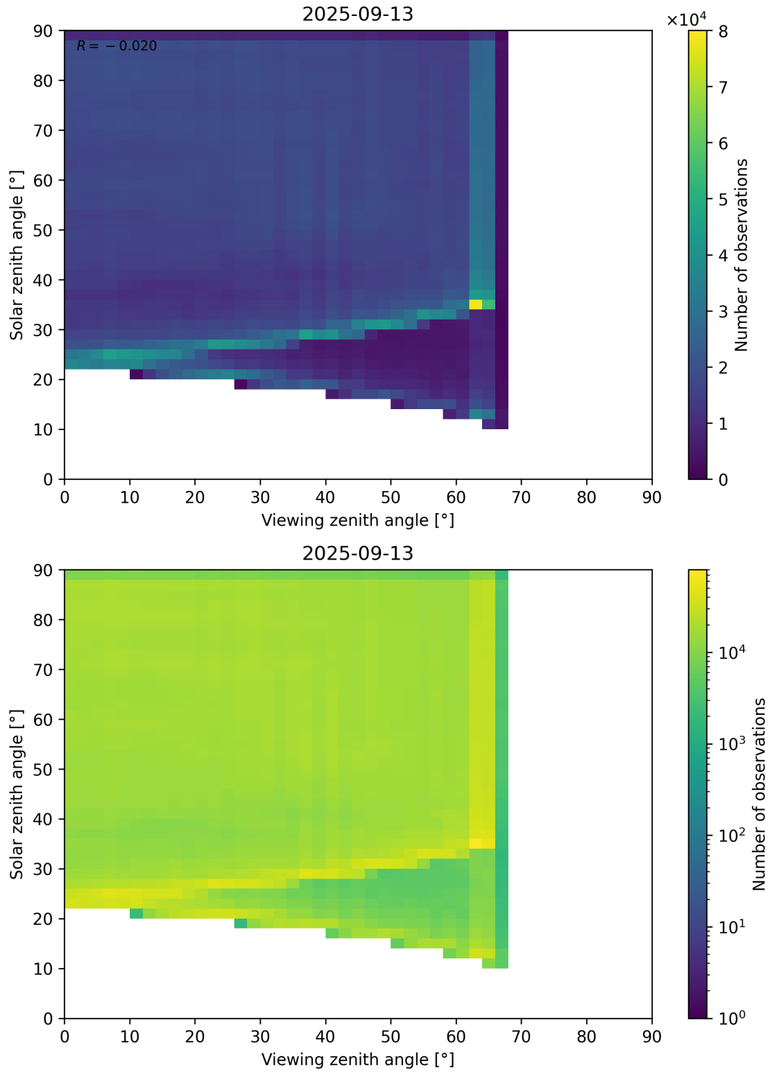
Figure 114: Scatter density plot of “Viewing zenith angle” against “Solar zenith angle” for 2025-09-12 to 2025-09-14.
