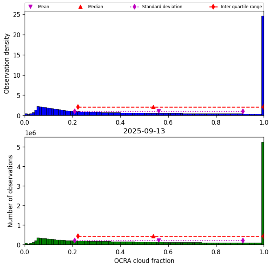
Figure 50: Histogram of “OCRA cloud fraction” for 2025-09-12 to 2025-09-14
