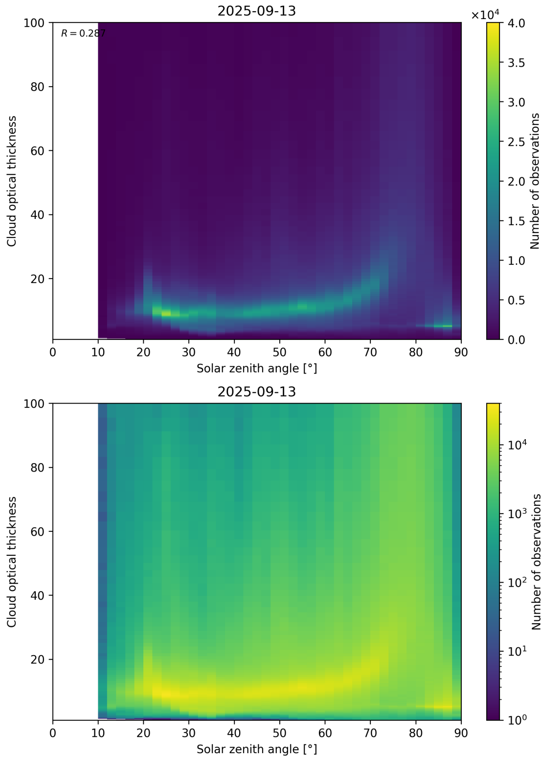
Figure 103: Scatter density plot of “Solar zenith angle” against “Cloud optical thickness” for 2025-09-12 to 2025-09-14.
