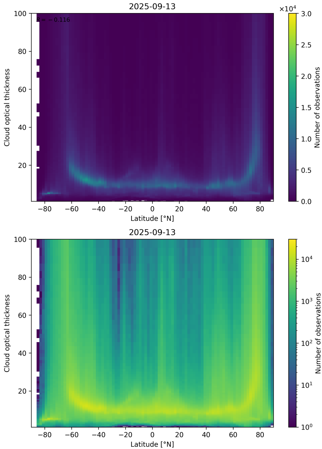
Figure 96: Scatter density plot of “Latitude” against “Cloud optical thickness” for 2025-09-12 to 2025-09-14.
