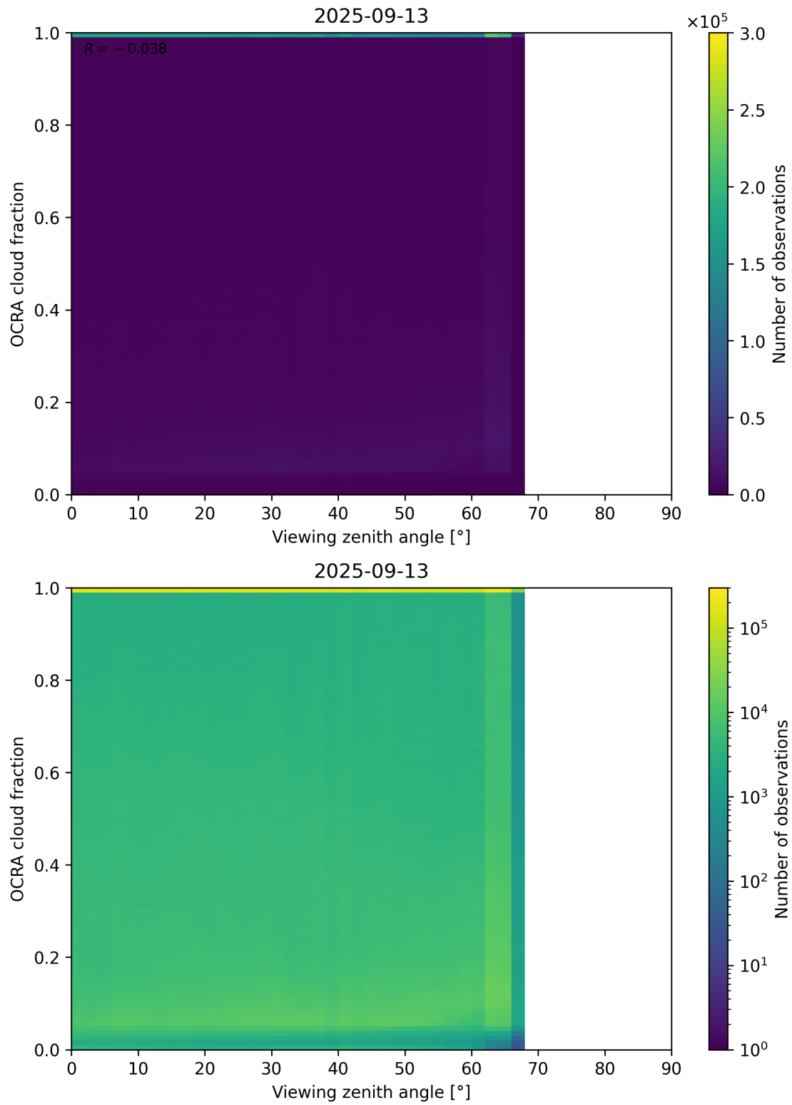
Figure 108: Scatter density plot of “Viewing zenith angle” against “OCRA cloud fraction” for 2025-09-12 to 2025-09-14.
