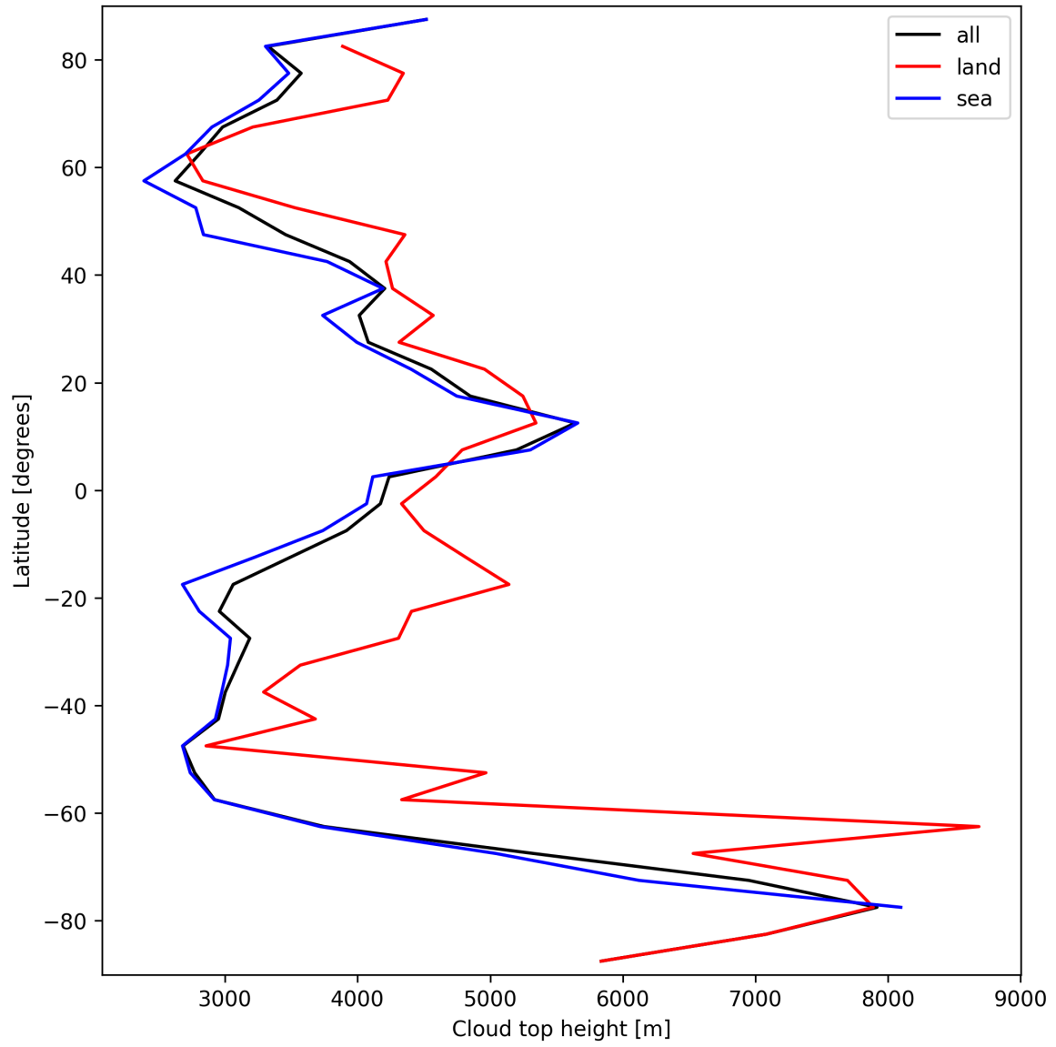
Figure 24: Zonal average of “Cloud top height” for 2025-09-12 to 2025-09-14.
