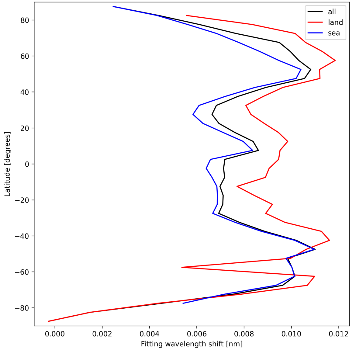
Figure 33: Zonal average of “Fitting wavelength shift” for 2025-09-12 to 2025-09-14.
