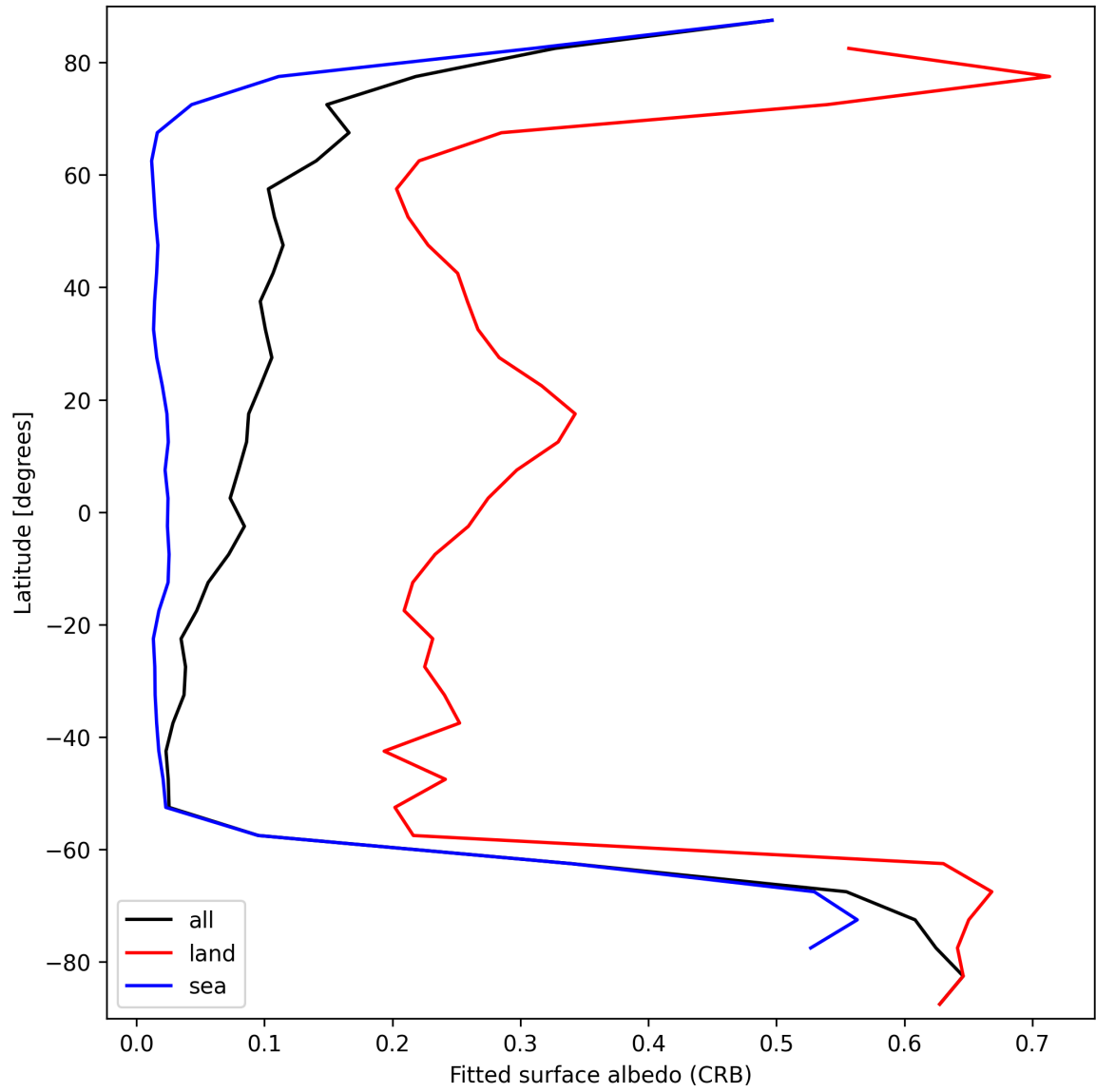
Figure 30: Zonal average of “Fitted surface albedo (CRB)” for 2025-09-12 to 2025-09-14.
