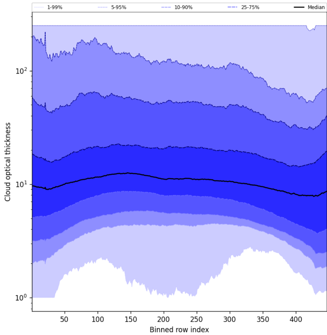
Figure 57: Along track statistics of “Cloud optical thickness” for 2025-09-12 to 2025-09-14
