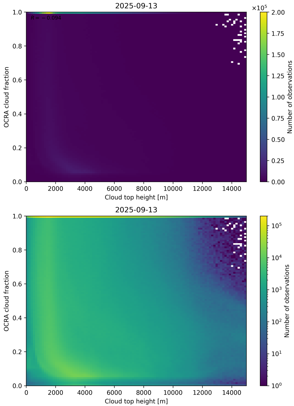
Figure 87: Scatter density plot of “Cloud top height” against “OCRA cloud fraction” for 2025-09-12 to 2025-09-14.
