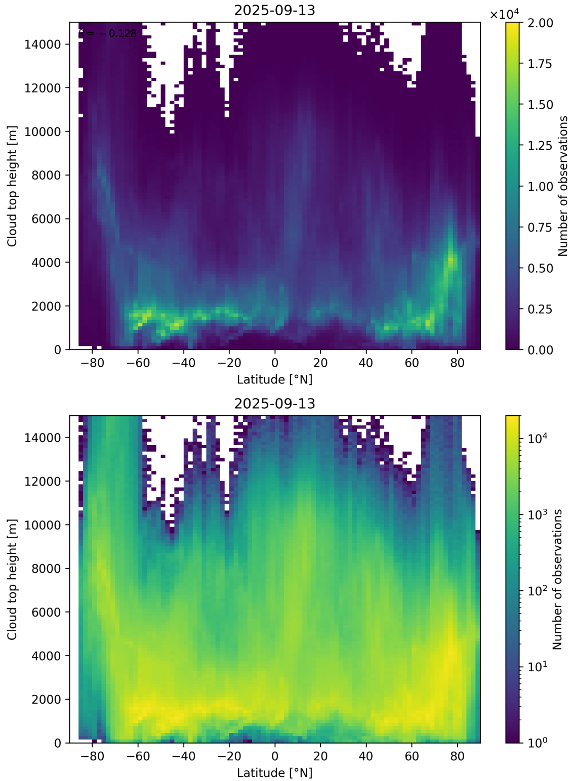
Figure 97: Scatter density plot of “Latitude” against “Cloud top height” for 2025-09-12 to 2025-09-14.
