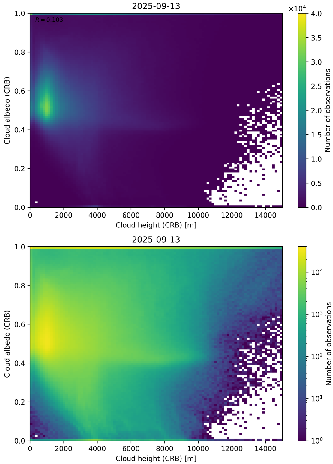
Figure 80: Scatter density plot of “Cloud height (CRB)” against “Cloud albedo (CRB)” for 2025-09-12 to 2025-09-14.
