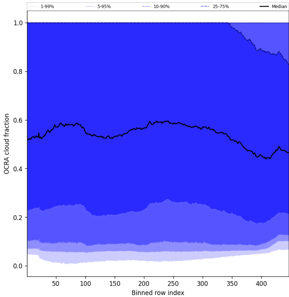
Figure 66: Along track statistics of “OCRA cloud fraction” for 2025-09-12 to 2025-09-14
