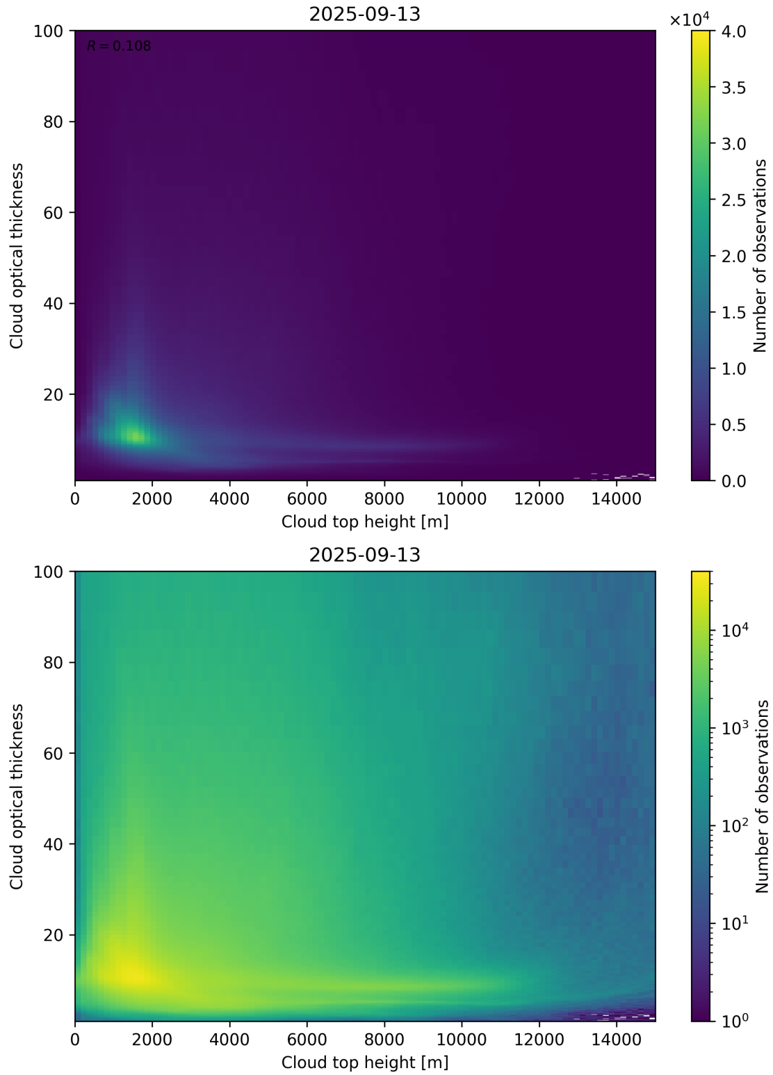
Figure 90: Scatter density plot of “Cloud top height” against “Cloud optical thickness” for 2025-09-12 to 2025-09-14.
