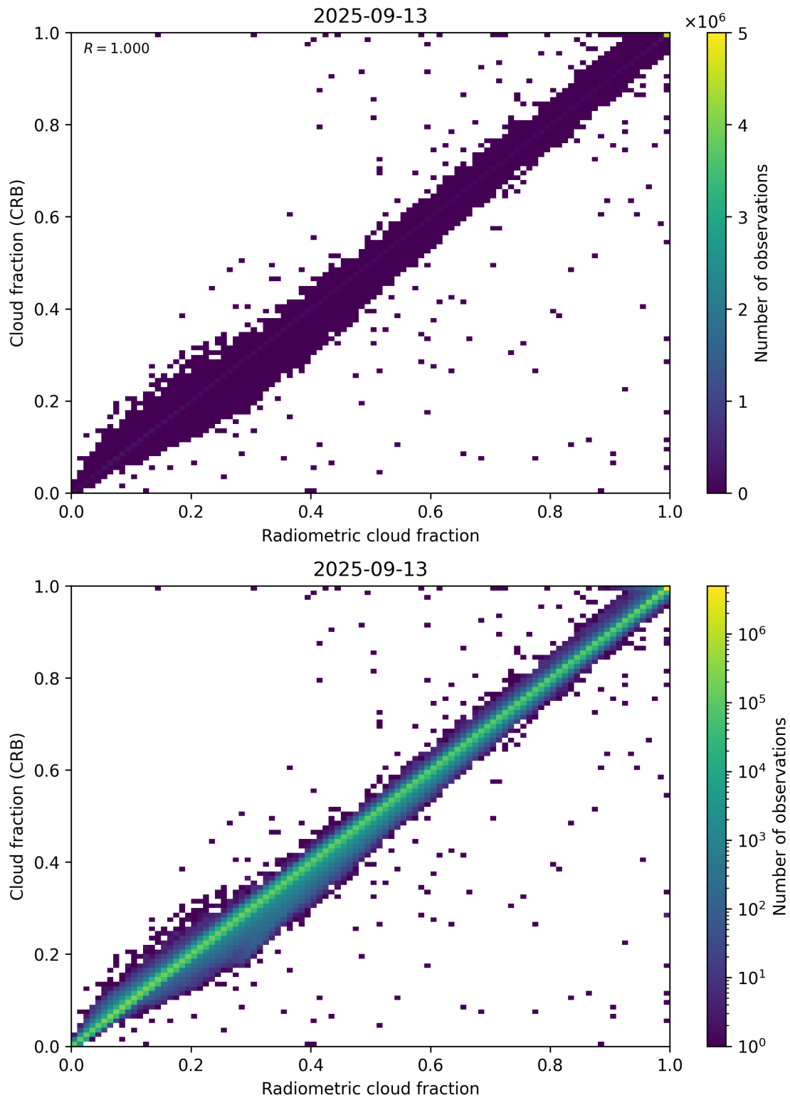
Figure 73: Scatter density plot of “Radiometric cloud fraction” against “Cloud fraction (CRB)” for 2025-09-12 to 2025-09-14.
