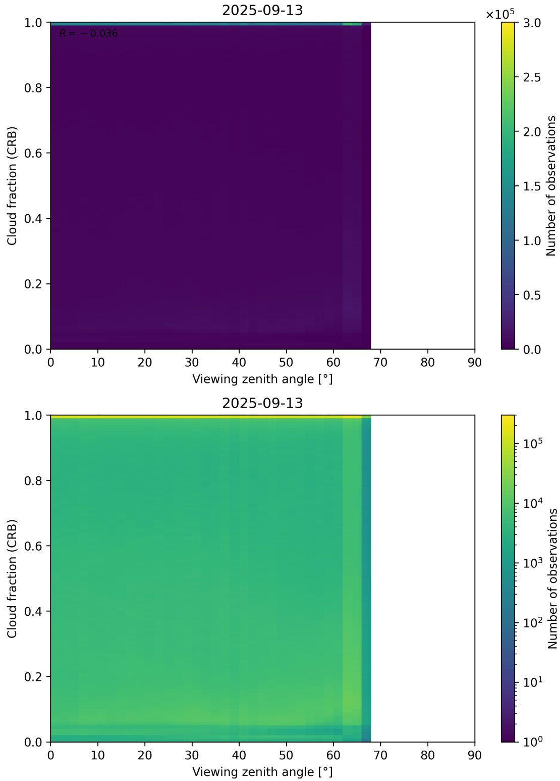
Figure 109: Scatter density plot of “Viewing zenith angle” against “Cloud fraction (CRB)” for 2025-09-12 to 2025-09-14.
