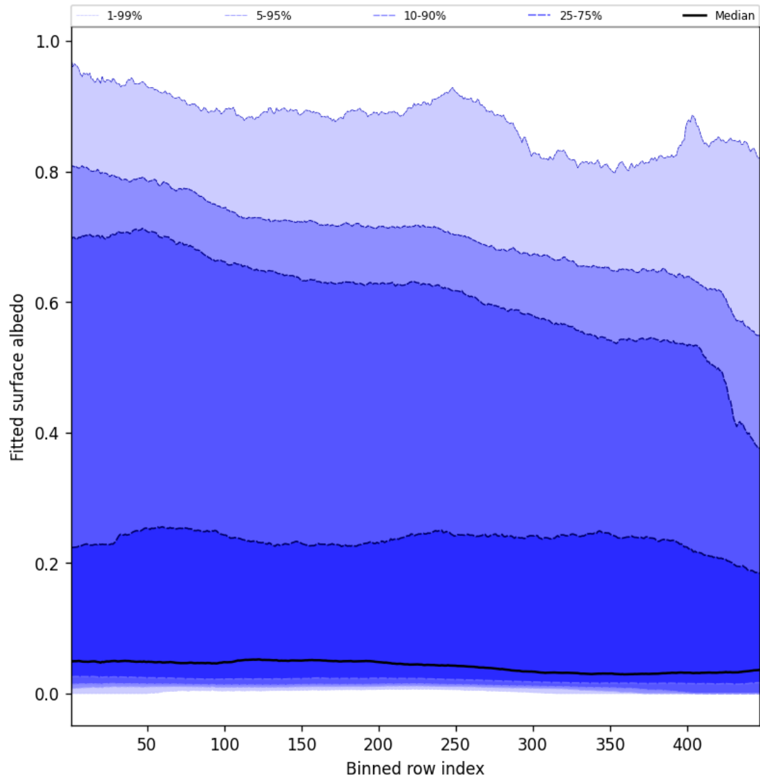
Figure 61: Along track statistics of “Fitted surface albedo” for 2025-09-12 to 2025-09-14
