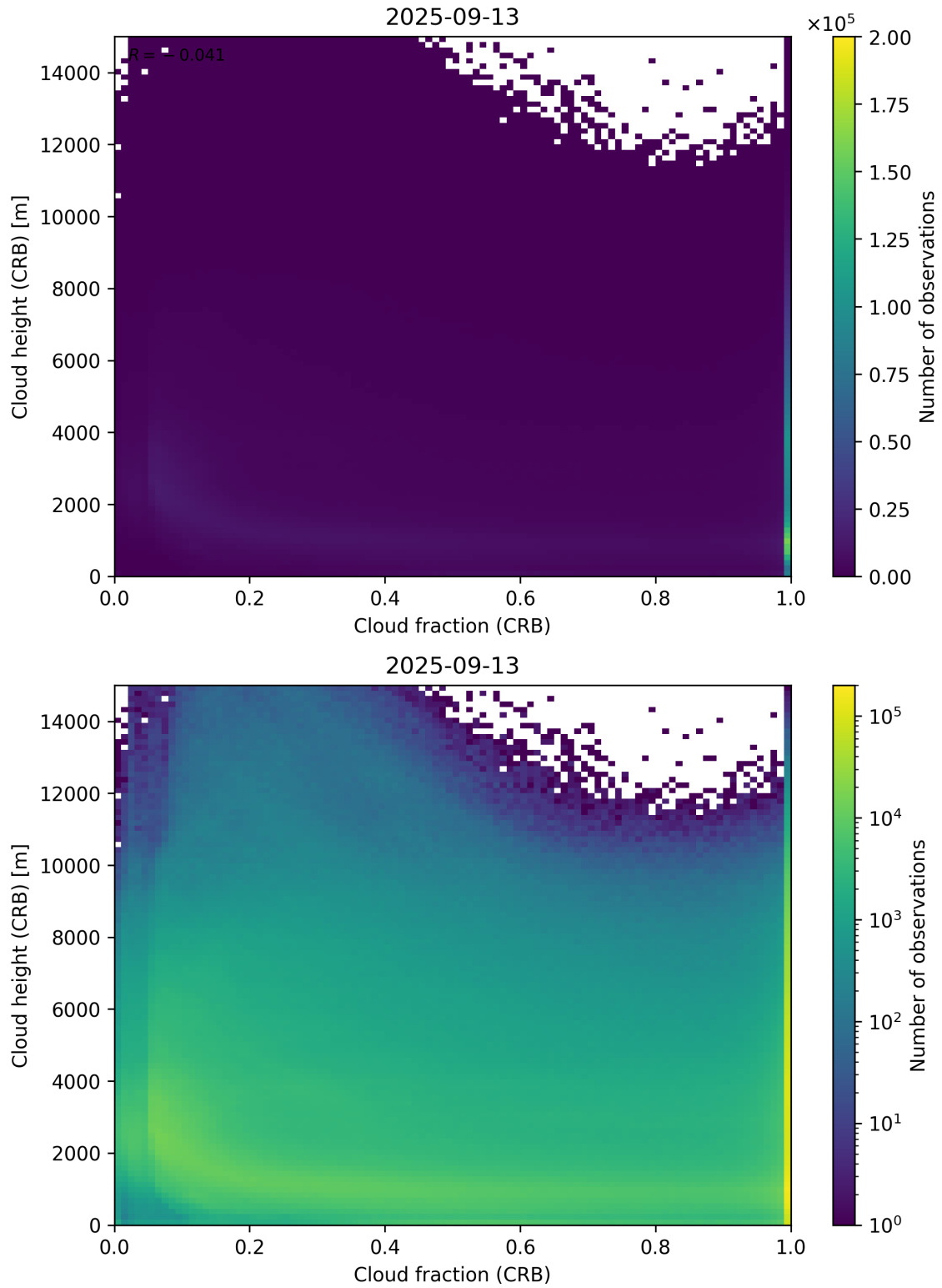
Figure 79: Scatter density plot of “Cloud fraction (CRB)” against “Cloud height (CRB)” for 2025-09-12 to 2025-09-14.
