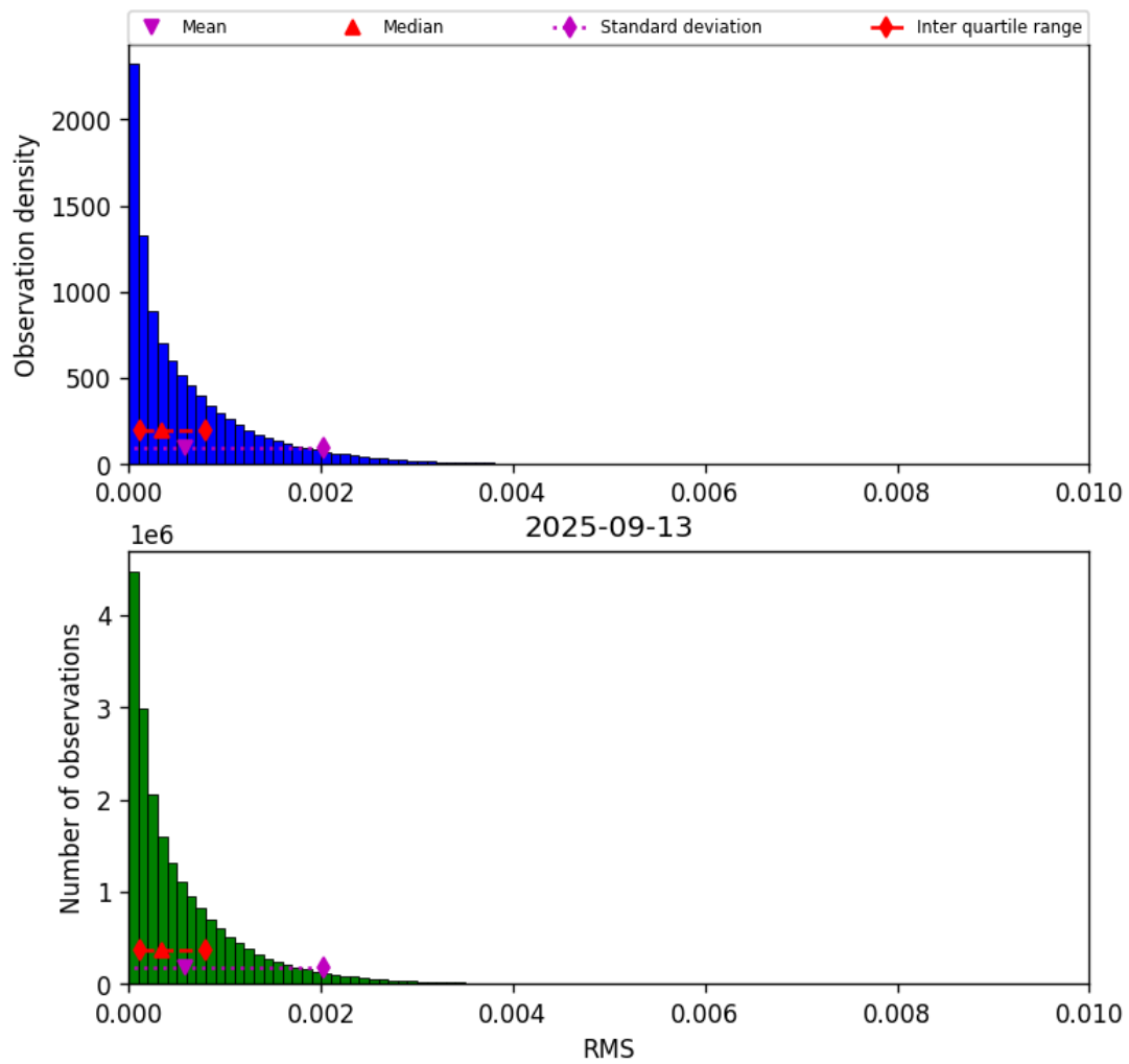
Figure 47: Histogram of “RMS” for 2025-09-12 to 2025-09-14
