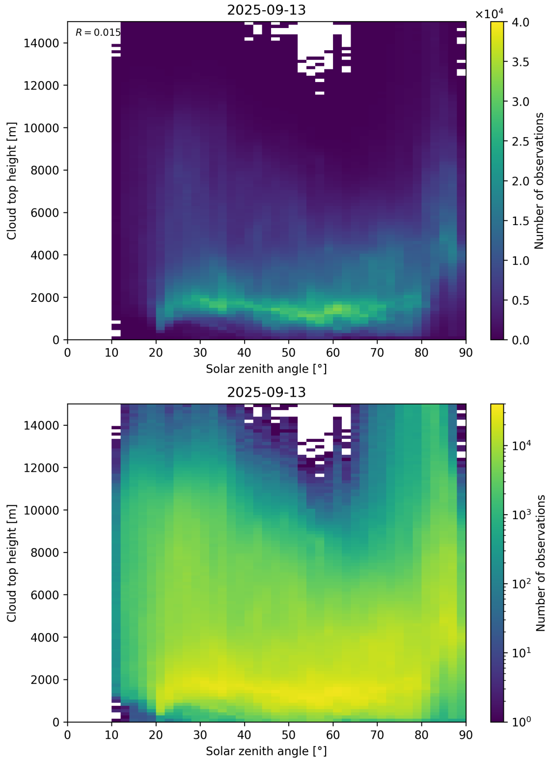
Figure 104: Scatter density plot of “Solar zenith angle” against “Cloud top height” for 2025-09-12 to 2025-09-14.
