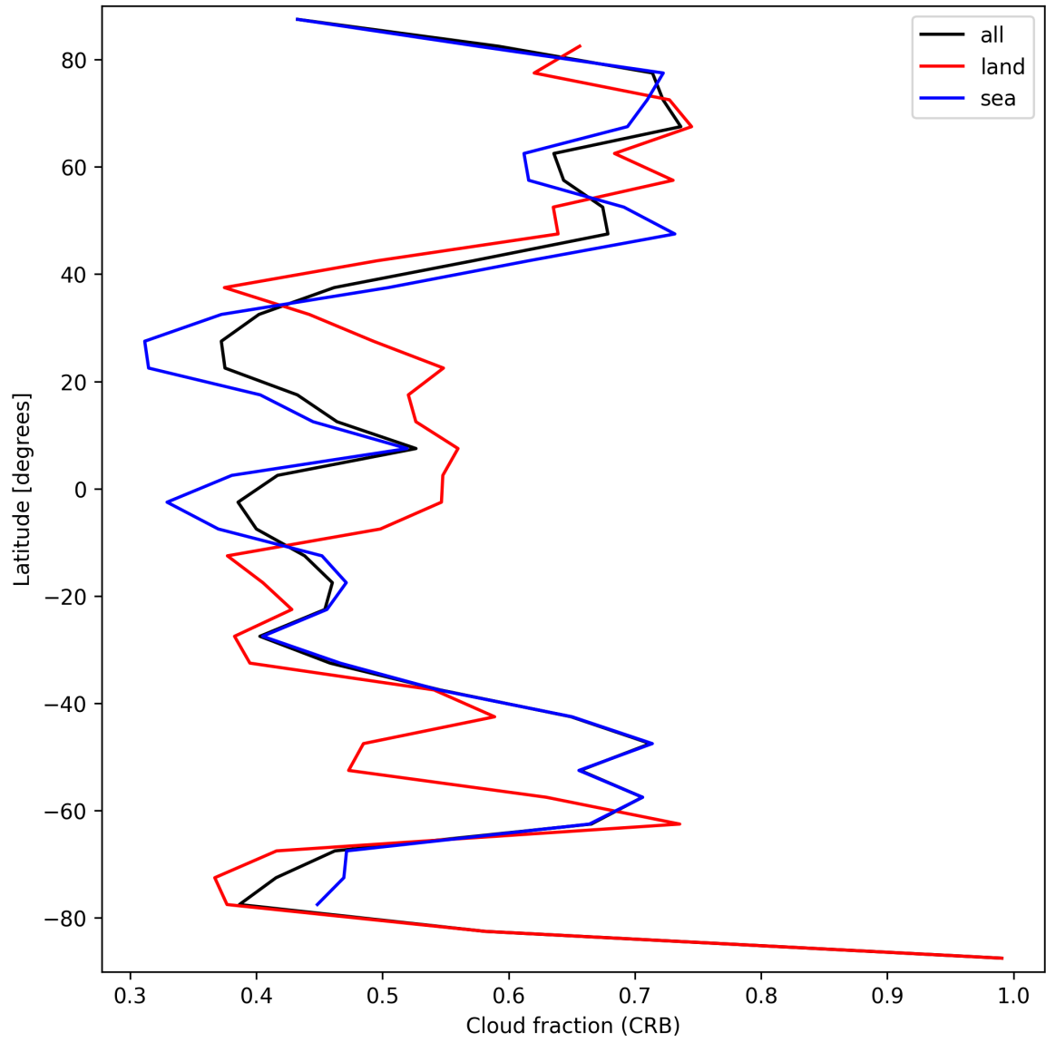
Figure 26: Zonal average of “Cloud fraction (CRB)” for 2025-09-12 to 2025-09-14.
