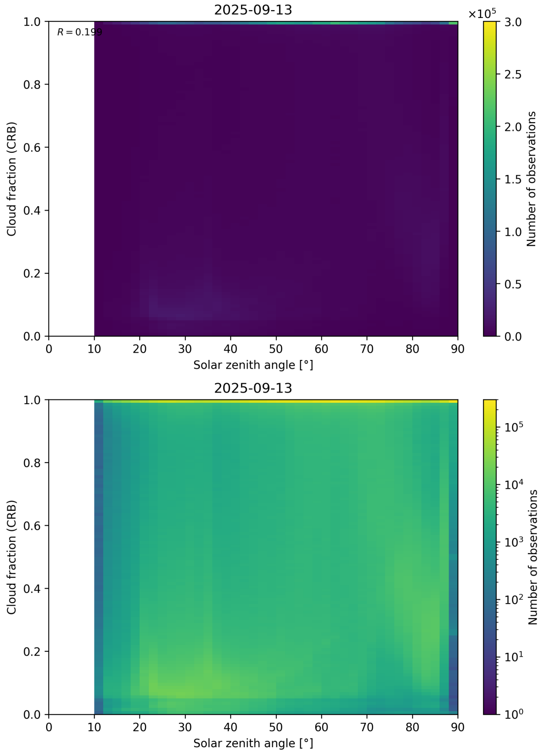
Figure 101: Scatter density plot of “Solar zenith angle” against “Cloud fraction (CRB)” for 2025-09-12 to 2025-09-14.
