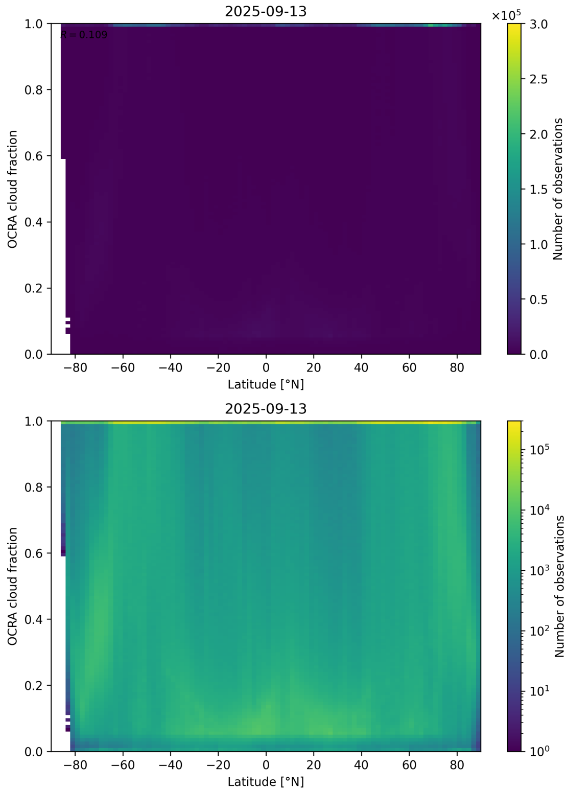
Figure 93: Scatter density plot of “Latitude” against “OCRA cloud fraction” for 2025-09-12 to 2025-09-14.
