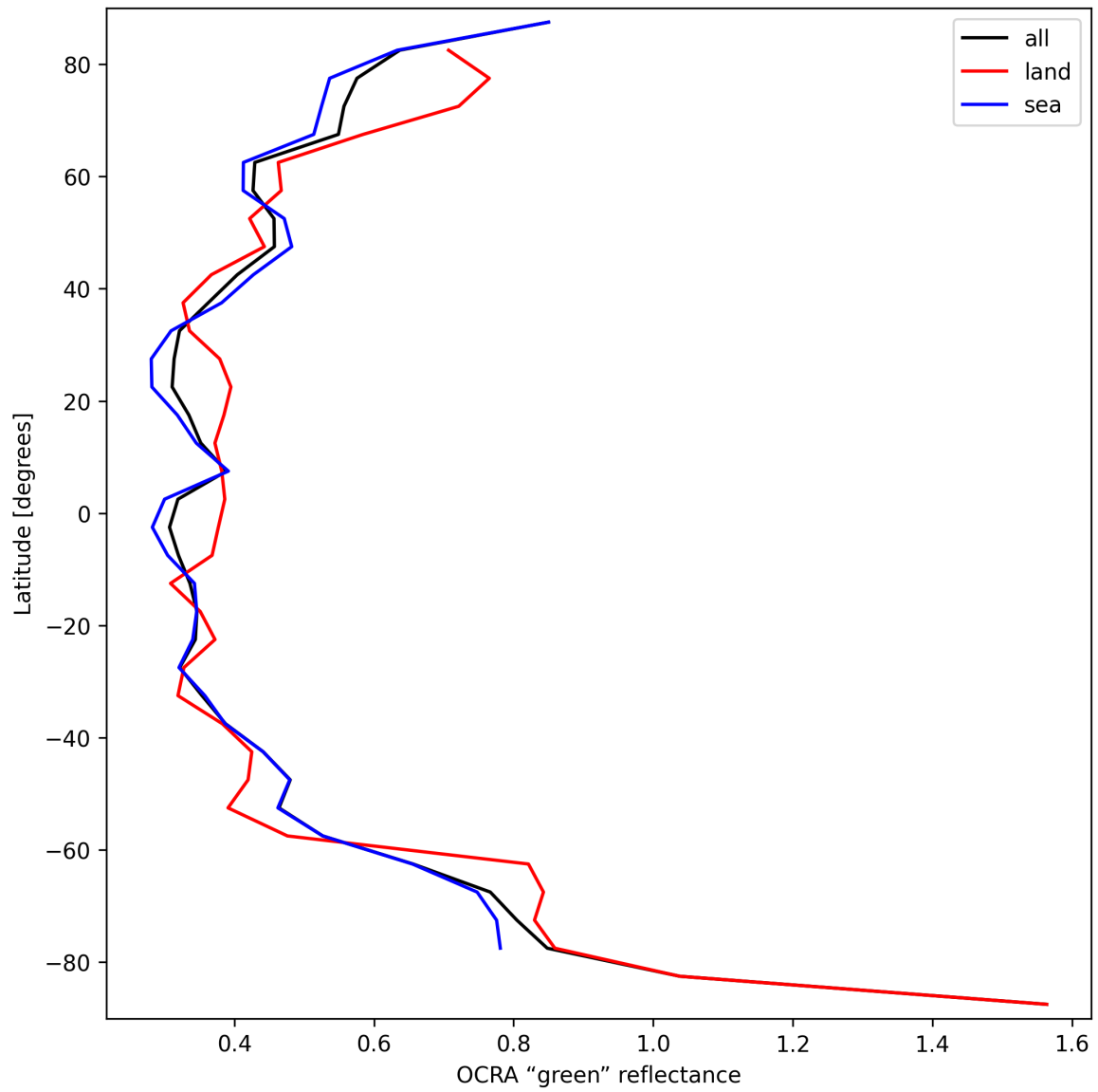
Figure 36: Zonal average of “OCRA “green” reflectance” for 2025-09-12 to 2025-09-14.
