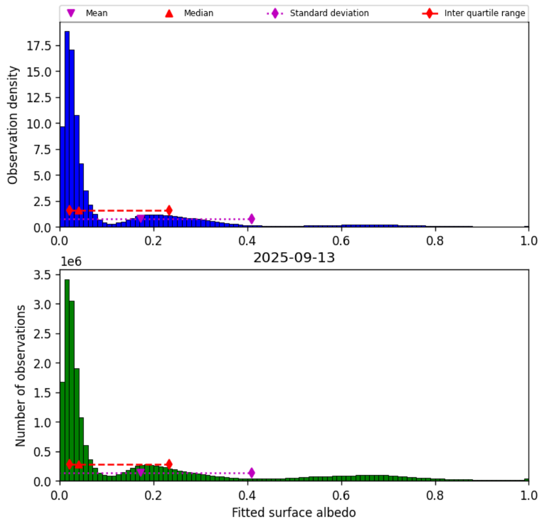
Figure 45: Histogram of “Fitted surface albedo” for 2025-09-12 to 2025-09-14
