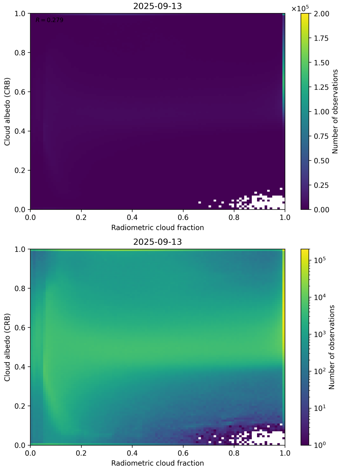
Figure 71: Scatter density plot of “Radiometric cloud fraction” against “Cloud albedo (CRB)” for 2025-09-12 to 2025-09-14.
