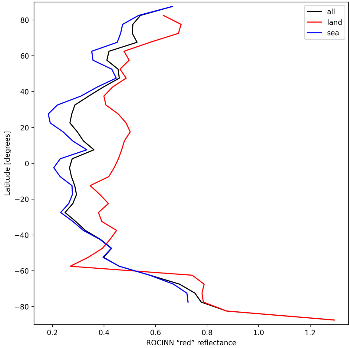
Figure 37: Zonal average of “ROCINN “red” reflectance” for 2025-09-12 to 2025-09-14.
