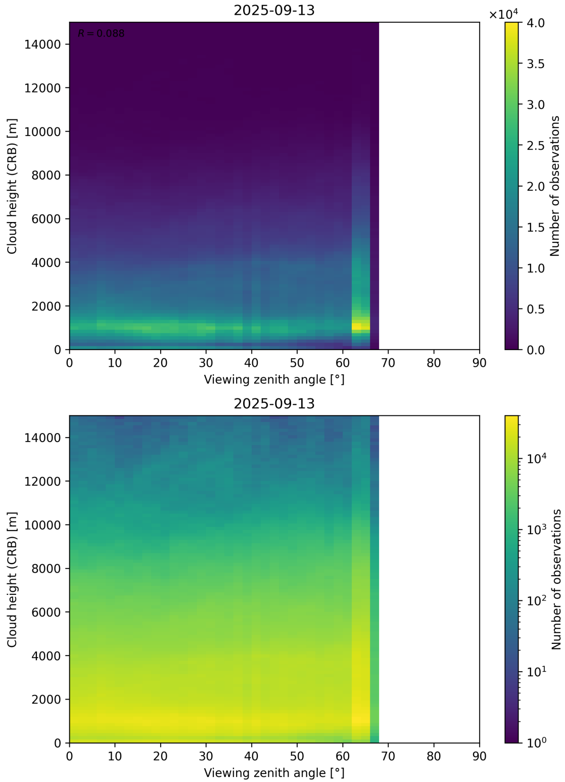
Figure 110: Scatter density plot of “Viewing zenith angle” against “Cloud height (CRB)” for 2025-09-12 to 2025-09-14.
