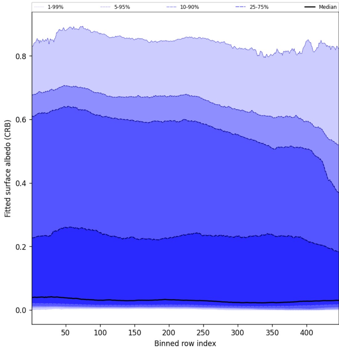
Figure 62: Along track statistics of “Fitted surface albedo (CRB)” for 2025-09-12 to 2025-09-14
