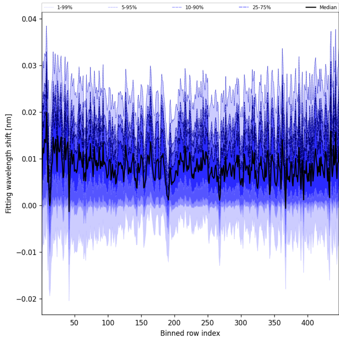
Figure 65: Along track statistics of “Fitting wavelength shift” for 2025-09-12 to 2025-09-14
