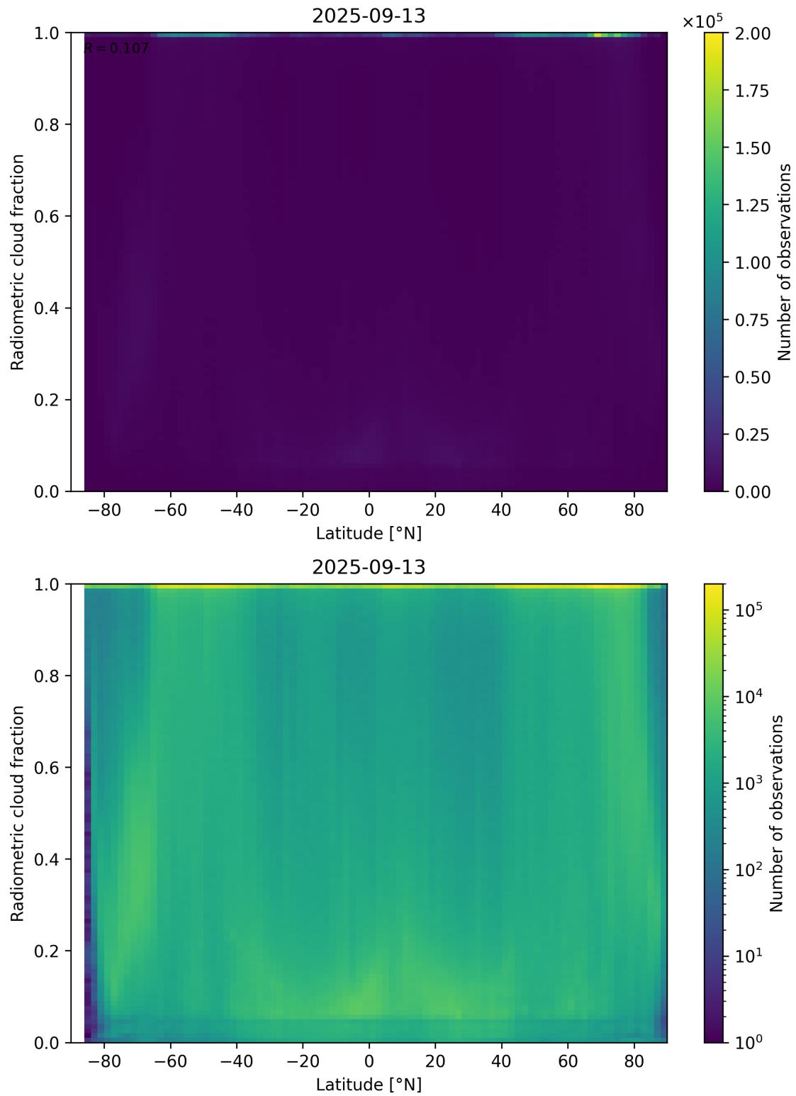
Figure 92: Scatter density plot of “Latitude” against “Radiometric cloud fraction” for 2025-09-12 to 2025-09-14.
