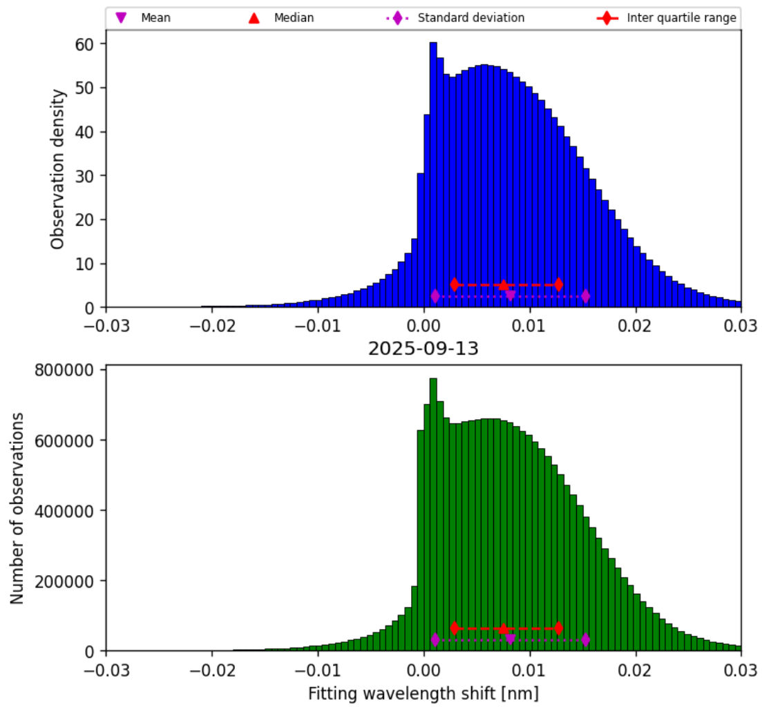
Figure 49: Histogram of “Fitting wavelength shift” for 2025-09-12 to 2025-09-14
