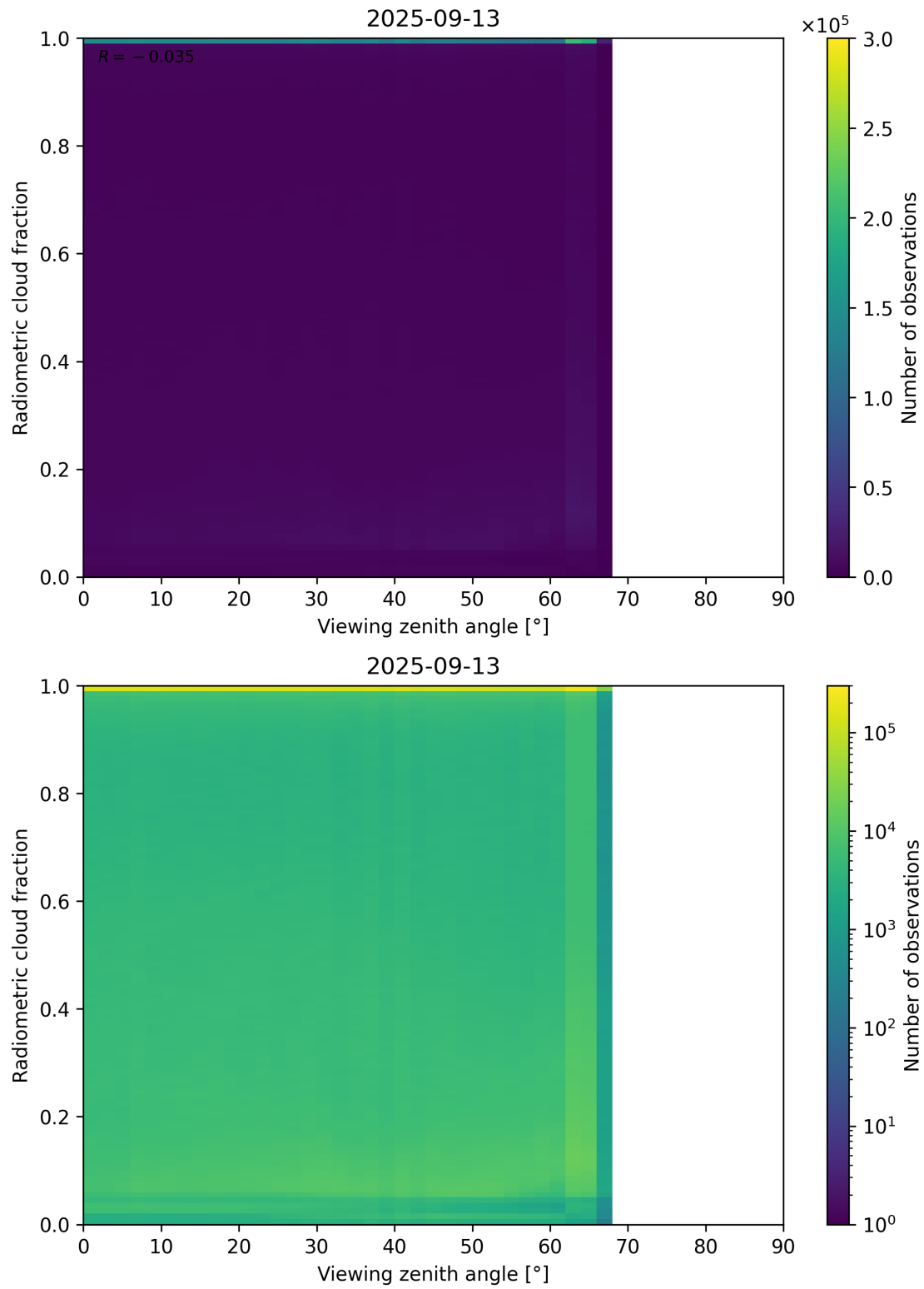
Figure 107: Scatter density plot of “Viewing zenith angle” against “Radiometric cloud fraction” for 2025-09-12 to 2025-09-14.
