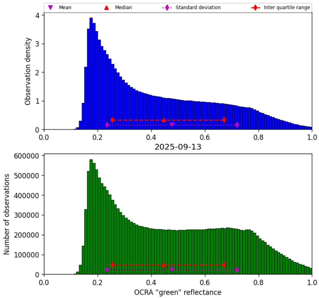
Figure 52: Histogram of “OCRA “green” reflectance” for 2025-09-12 to 2025-09-14
