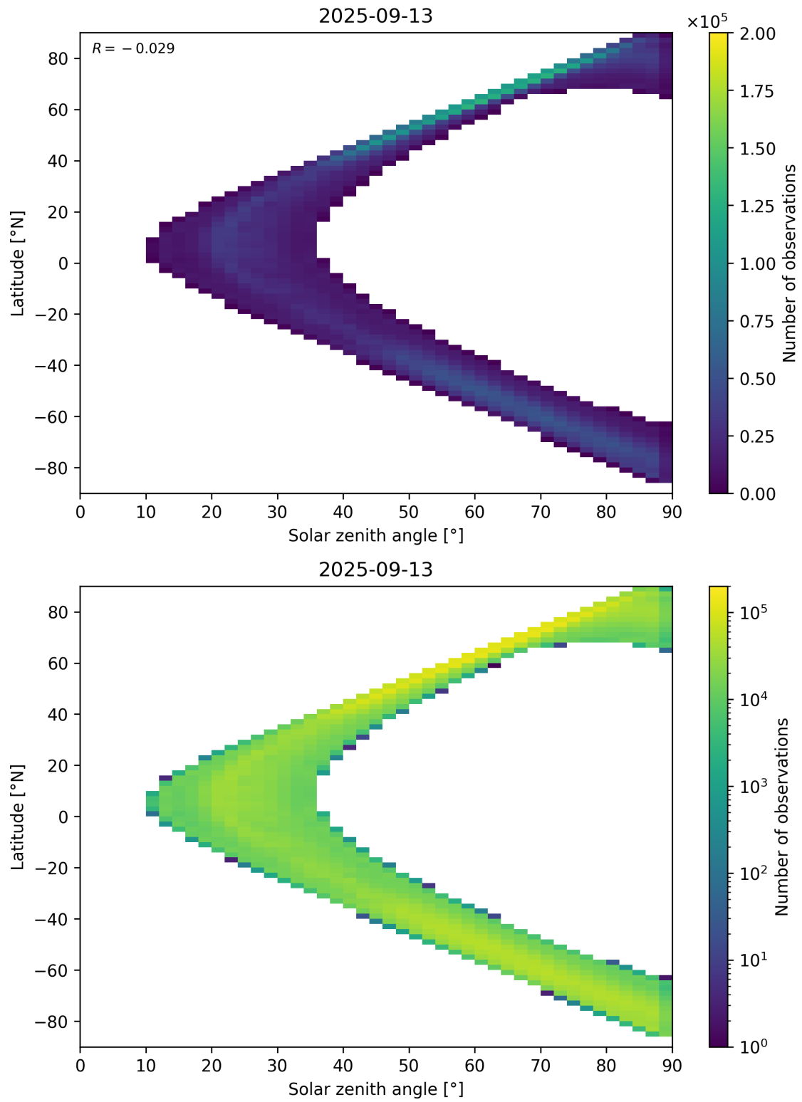
Figure 105: Scatter density plot of “Solar zenith angle” against “Latitude” for 2025-09-12 to 2025-09-14.
