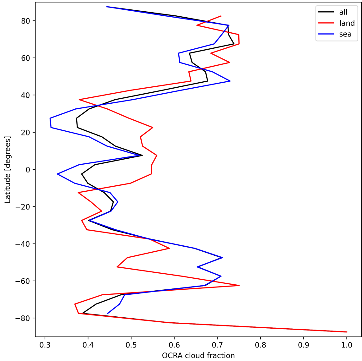
Figure 34: Zonal average of “OCRA cloud fraction” for 2025-09-12 to 2025-09-14.
