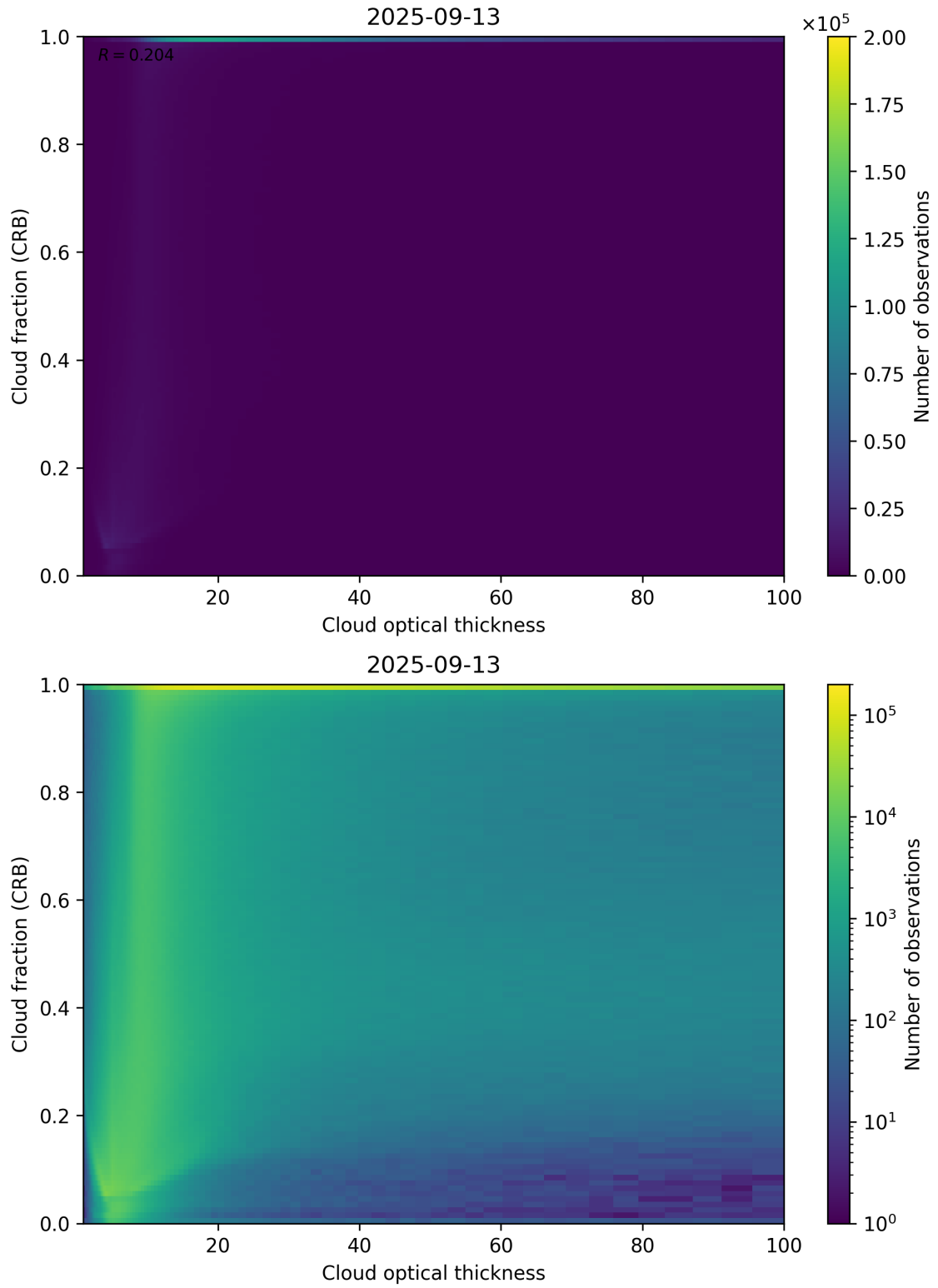
Figure 84: Scatter density plot of “Cloud optical thickness” against “Cloud fraction (CRB)” for 2025-09-12 to 2025-09-14.
