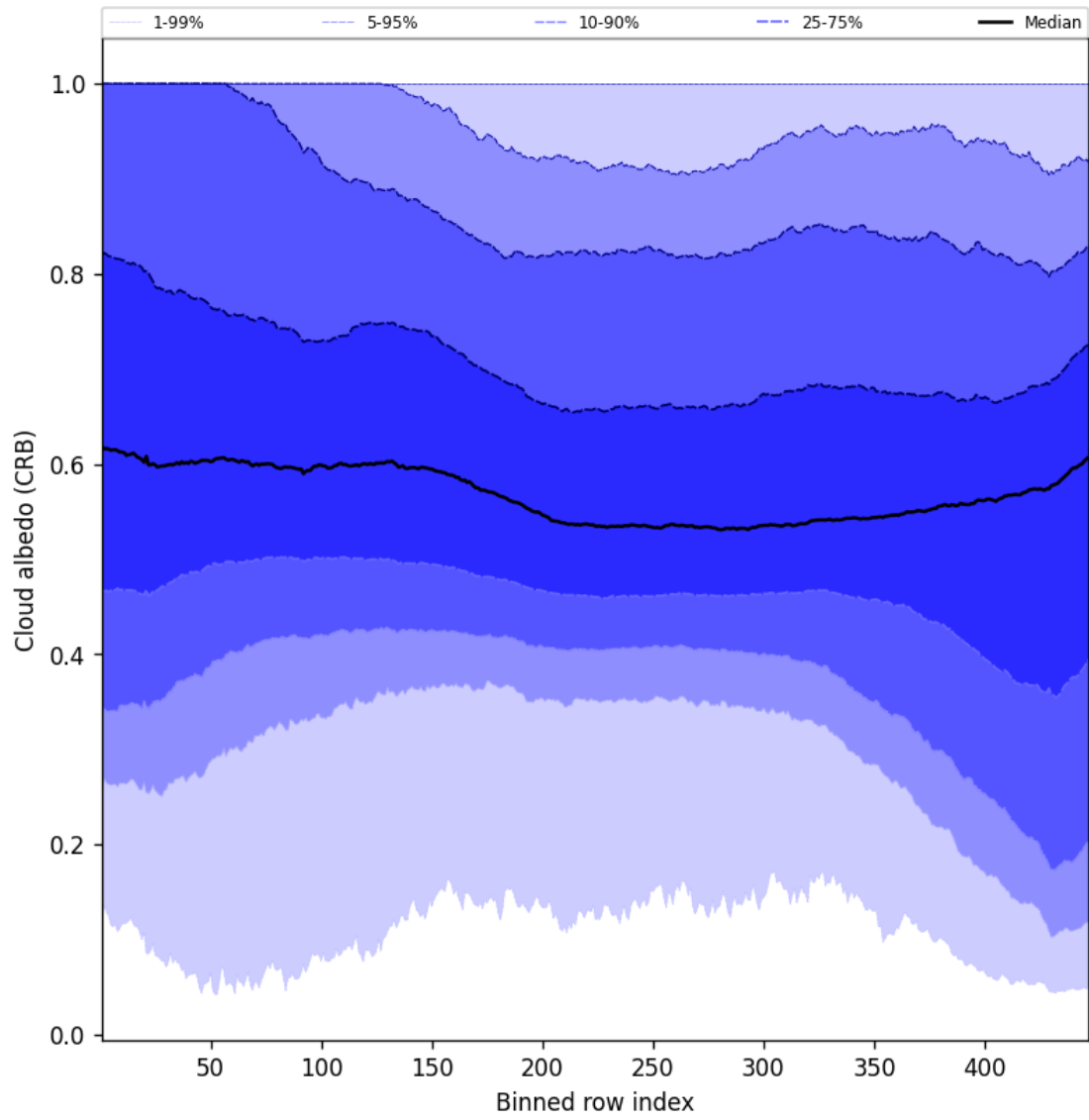
Figure 60: Along track statistics of “Cloud albedo (CRB)” for 2025-09-12 to 2025-09-14
