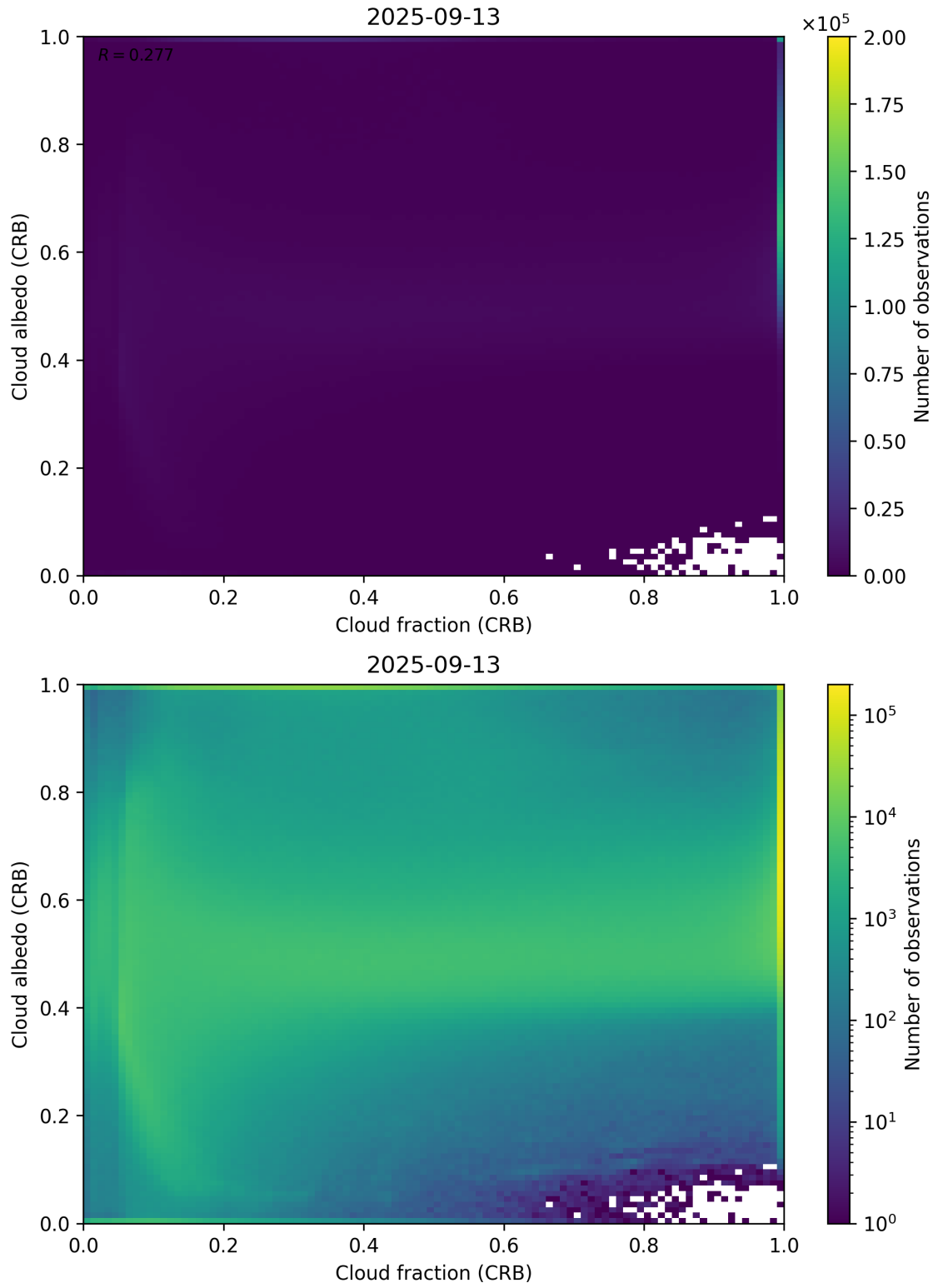
Figure 77: Scatter density plot of “Cloud fraction (CRB)” against “Cloud albedo (CRB)” for 2025-09-12 to 2025-09-14.
