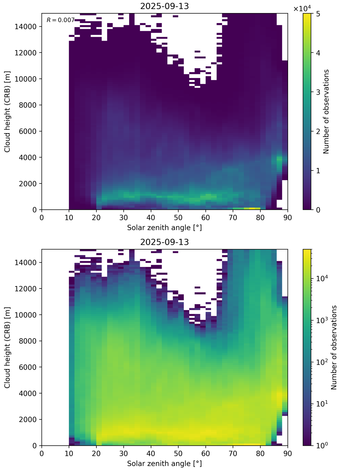
Figure 102: Scatter density plot of “Solar zenith angle” against “Cloud height (CRB)” for 2025-09-12 to 2025-09-14.
