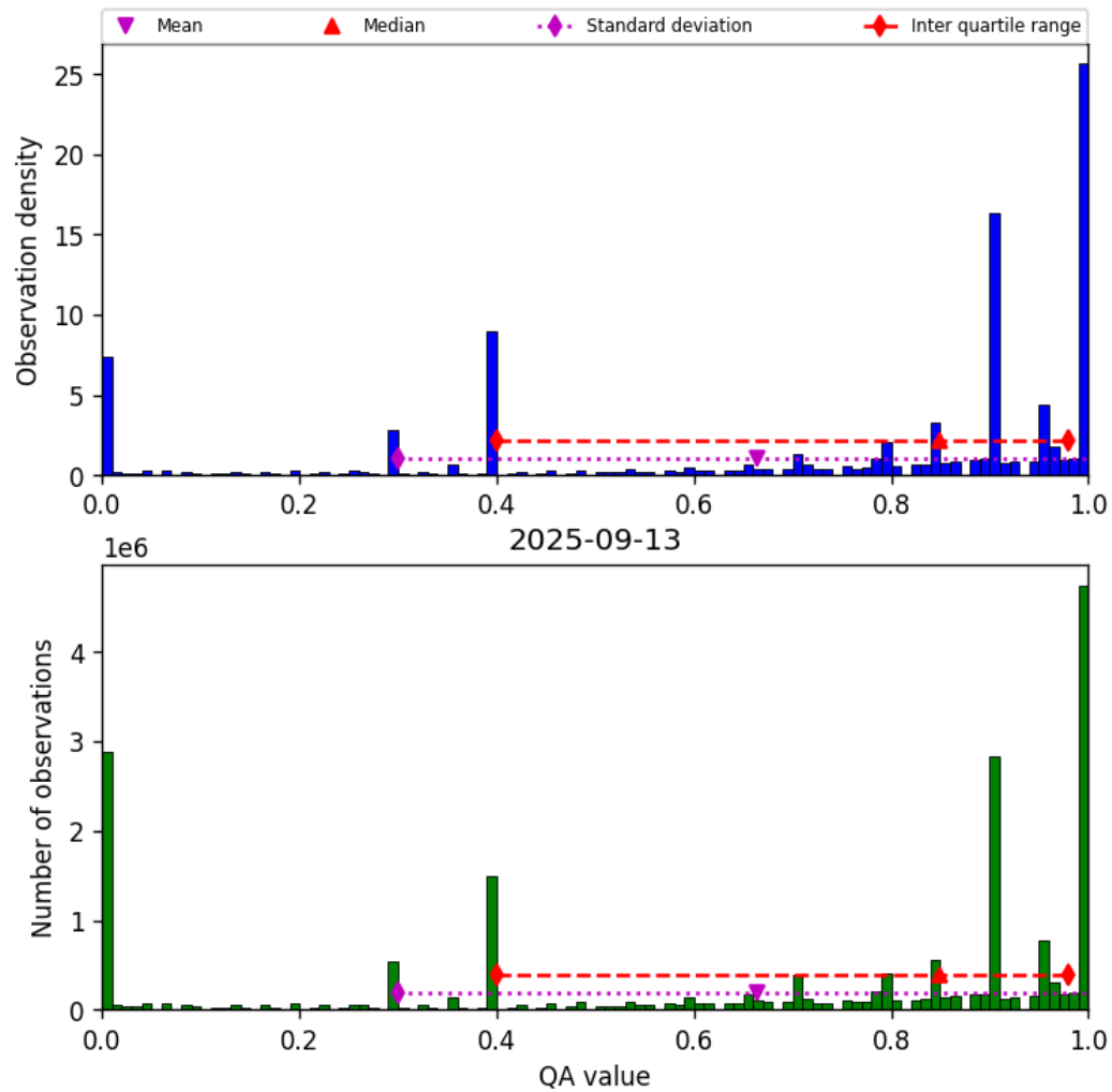
Figure 38: Histogram of “QA value” for 2025-09-12 to 2025-09-14
