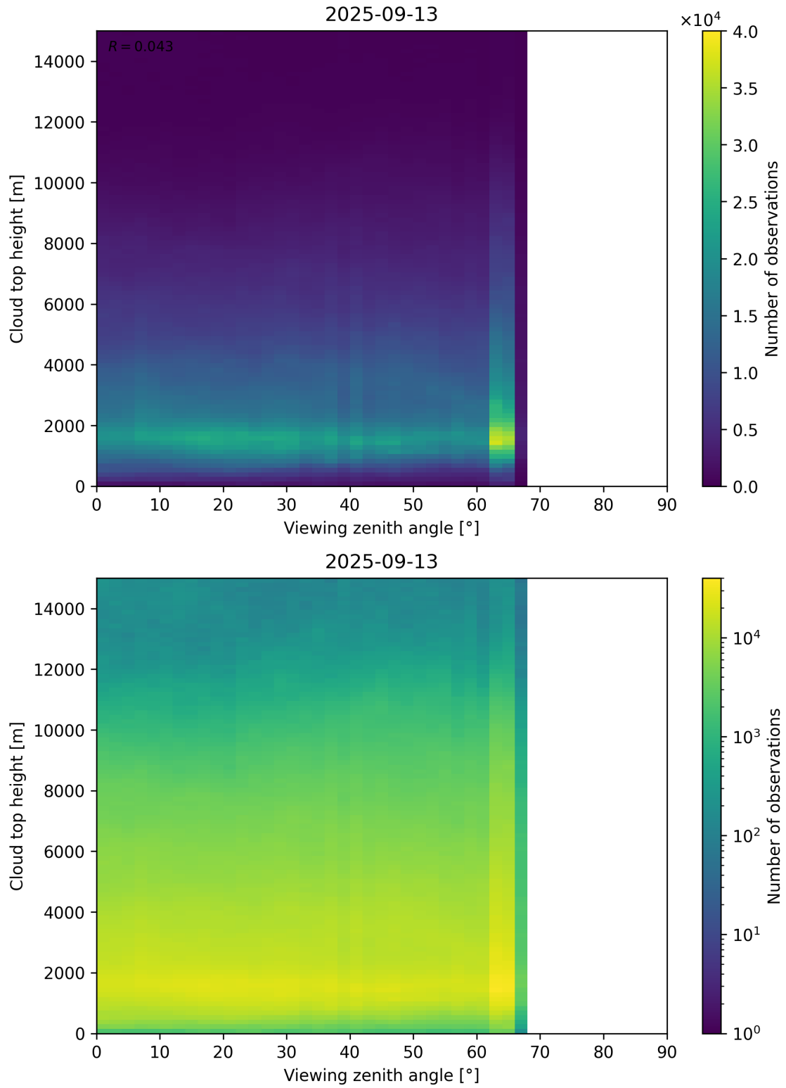
Figure 112: Scatter density plot of “Viewing zenith angle” against “Cloud top height” for 2025-09-12 to 2025-09-14.
