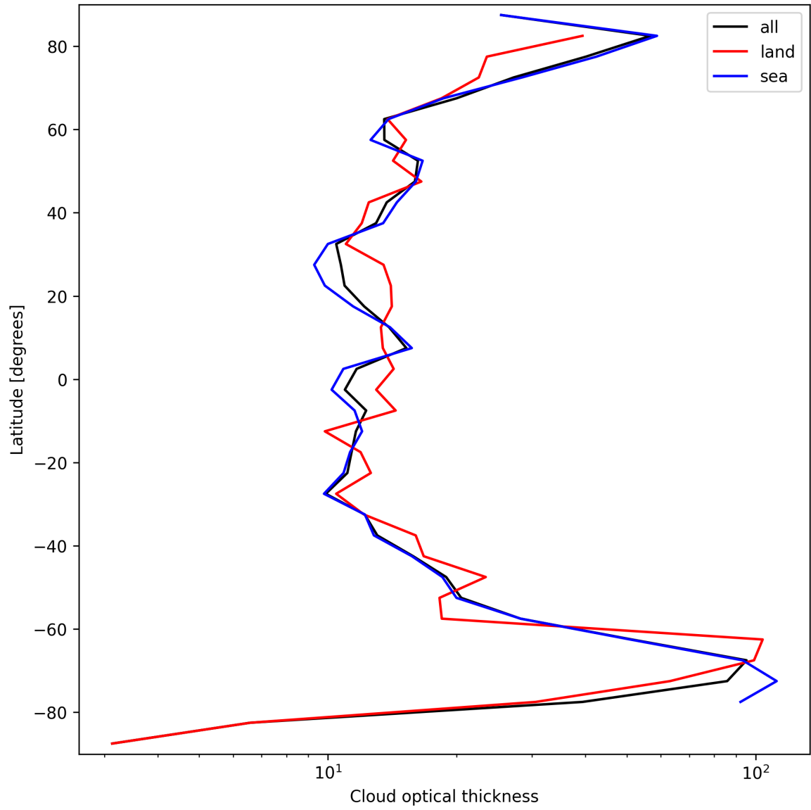
Figure 25: Zonal average of “Cloud optical thickness” for 2025-09-12 to 2025-09-14.
