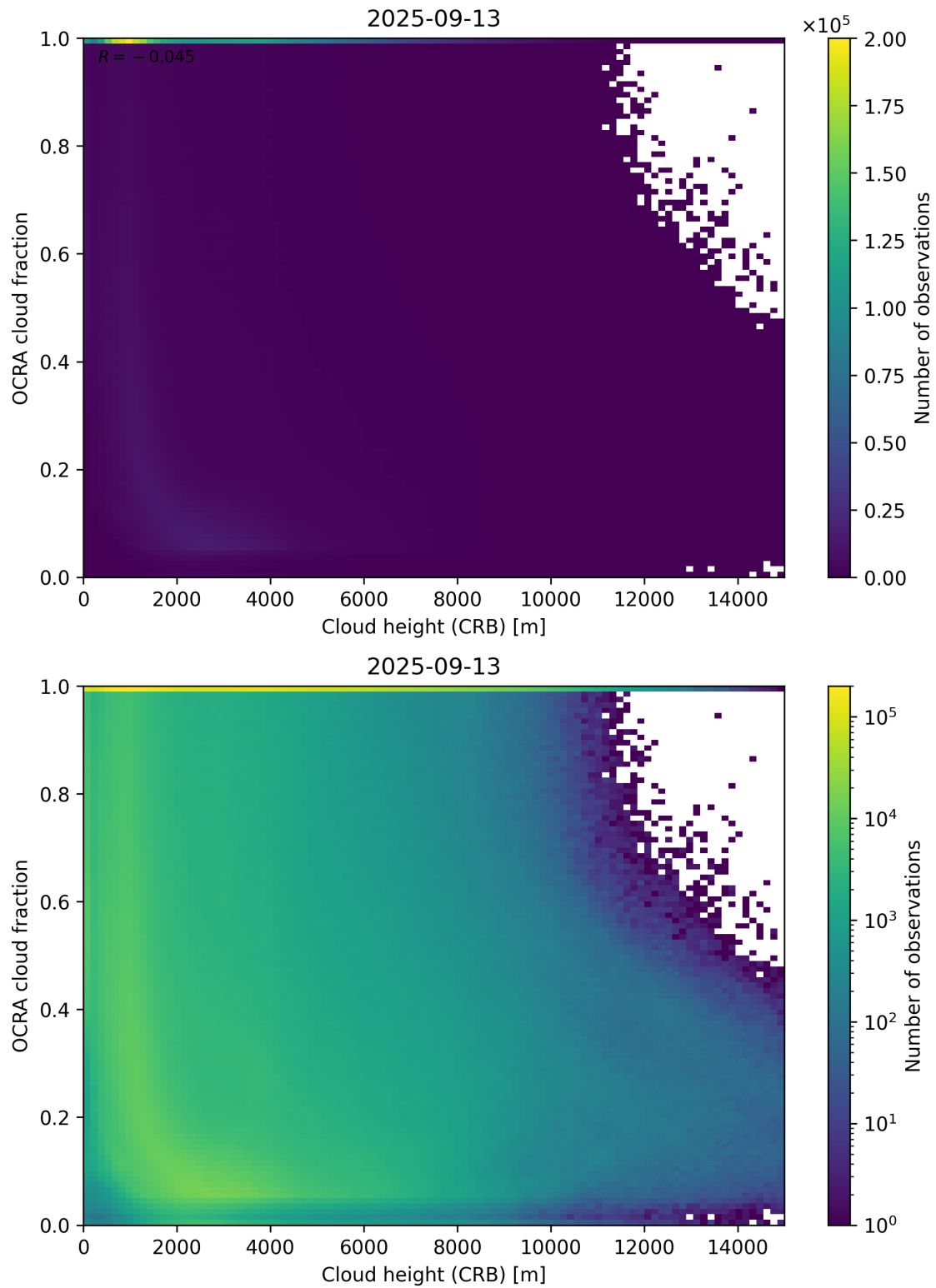
Figure 81: Scatter density plot of “Cloud height (CRB)” against “OCRA cloud fraction” for 2025-09-12 to 2025-09-14.
