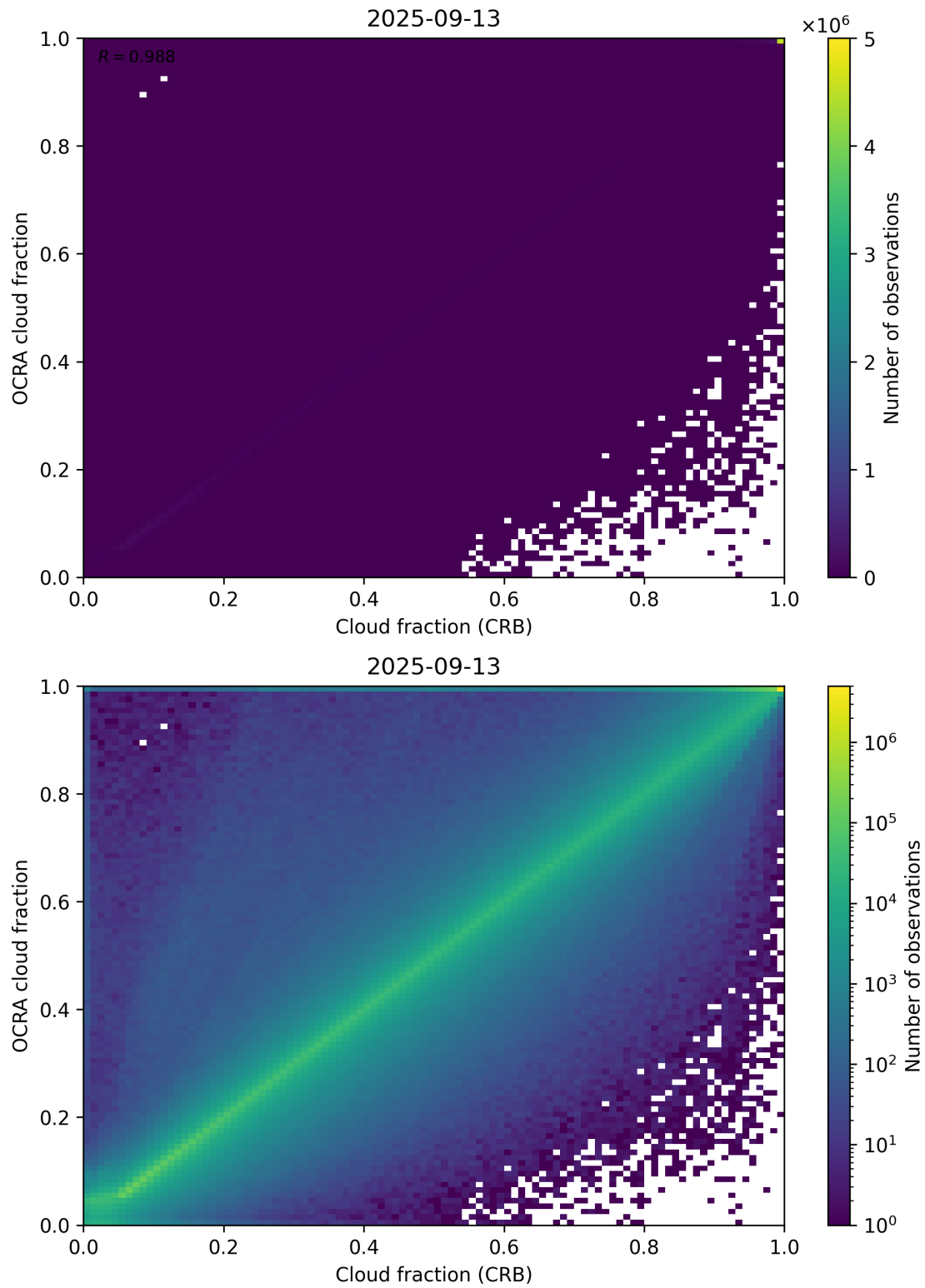
Figure 78: Scatter density plot of “Cloud fraction (CRB)” against “OCRA cloud fraction” for 2025-09-12 to 2025-09-14.
