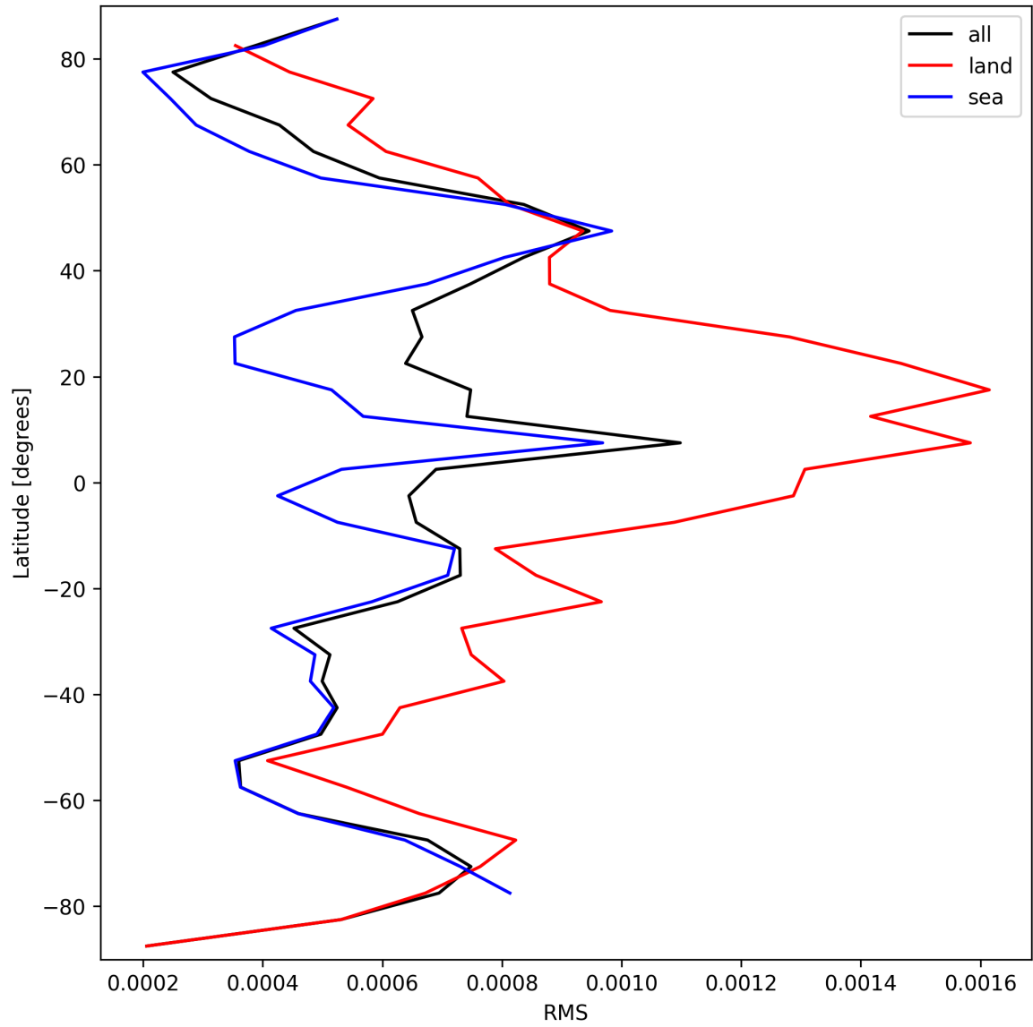
Figure 31: Zonal average of “RMS” for 2025-09-12 to 2025-09-14.
