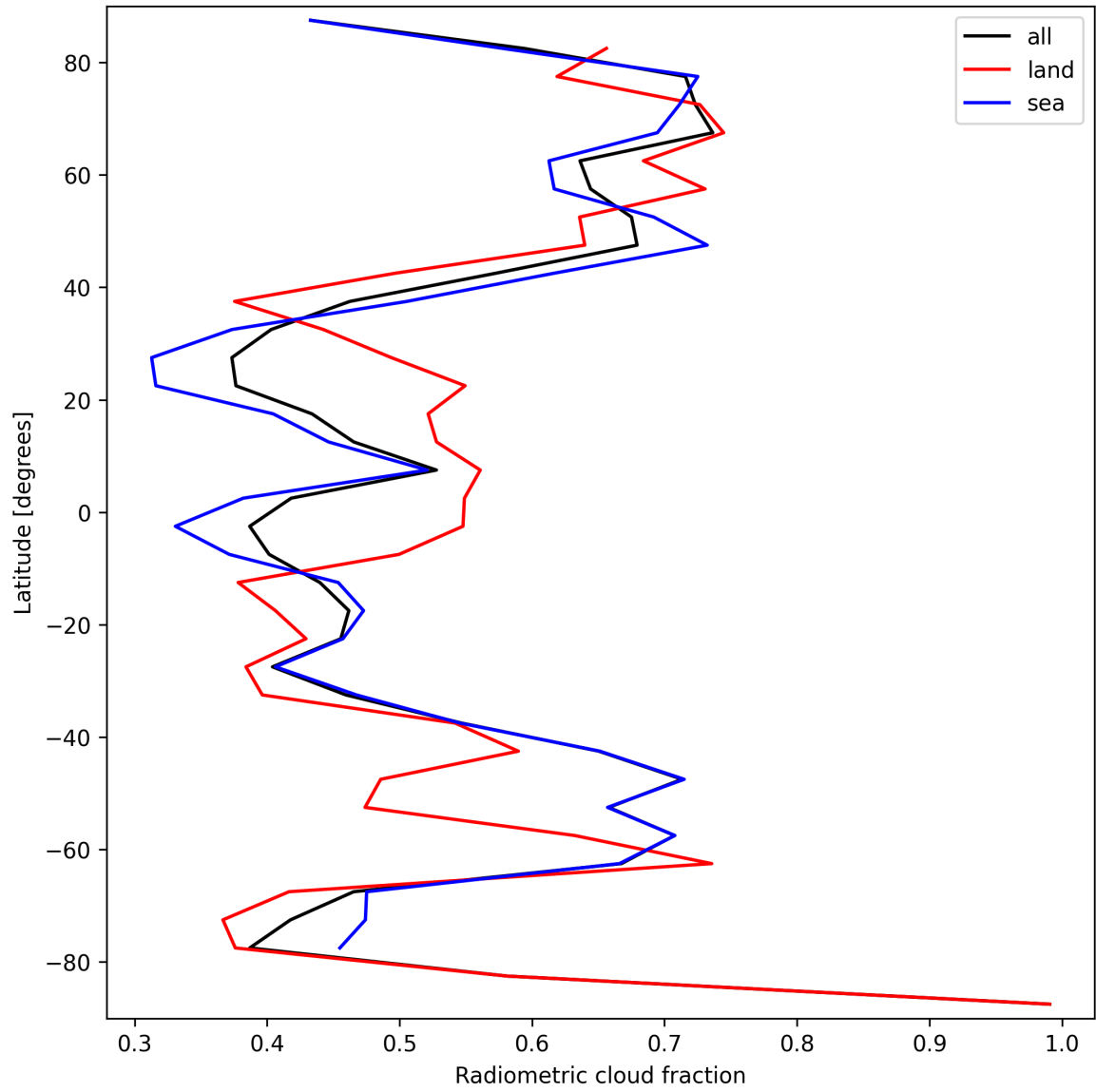
Figure 23: Zonal average of “Radiometric cloud fraction” for 2025-09-12 to 2025-09-14.
