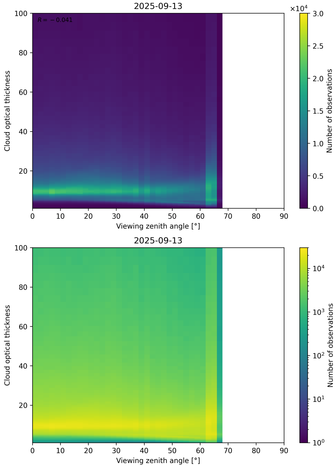
Figure 111: Scatter density plot of “Viewing zenith angle” against “Cloud optical thickness” for 2025-09-12 to 2025-09-14.
