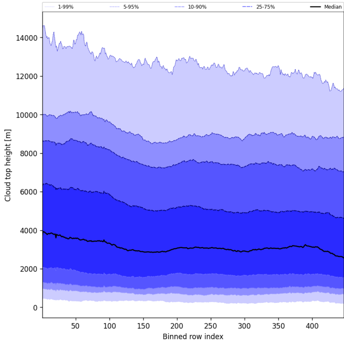
Figure 56: Along track statistics of “Cloud top height” for 2025-09-12 to 2025-09-14
