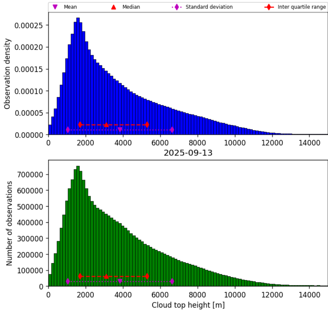
Figure 40: Histogram of “Cloud top height” for 2025-09-12 to 2025-09-14
