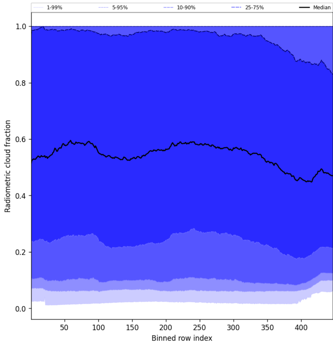
Figure 55: Along track statistics of “Radiometric cloud fraction” for 2025-09-12 to 2025-09-14
