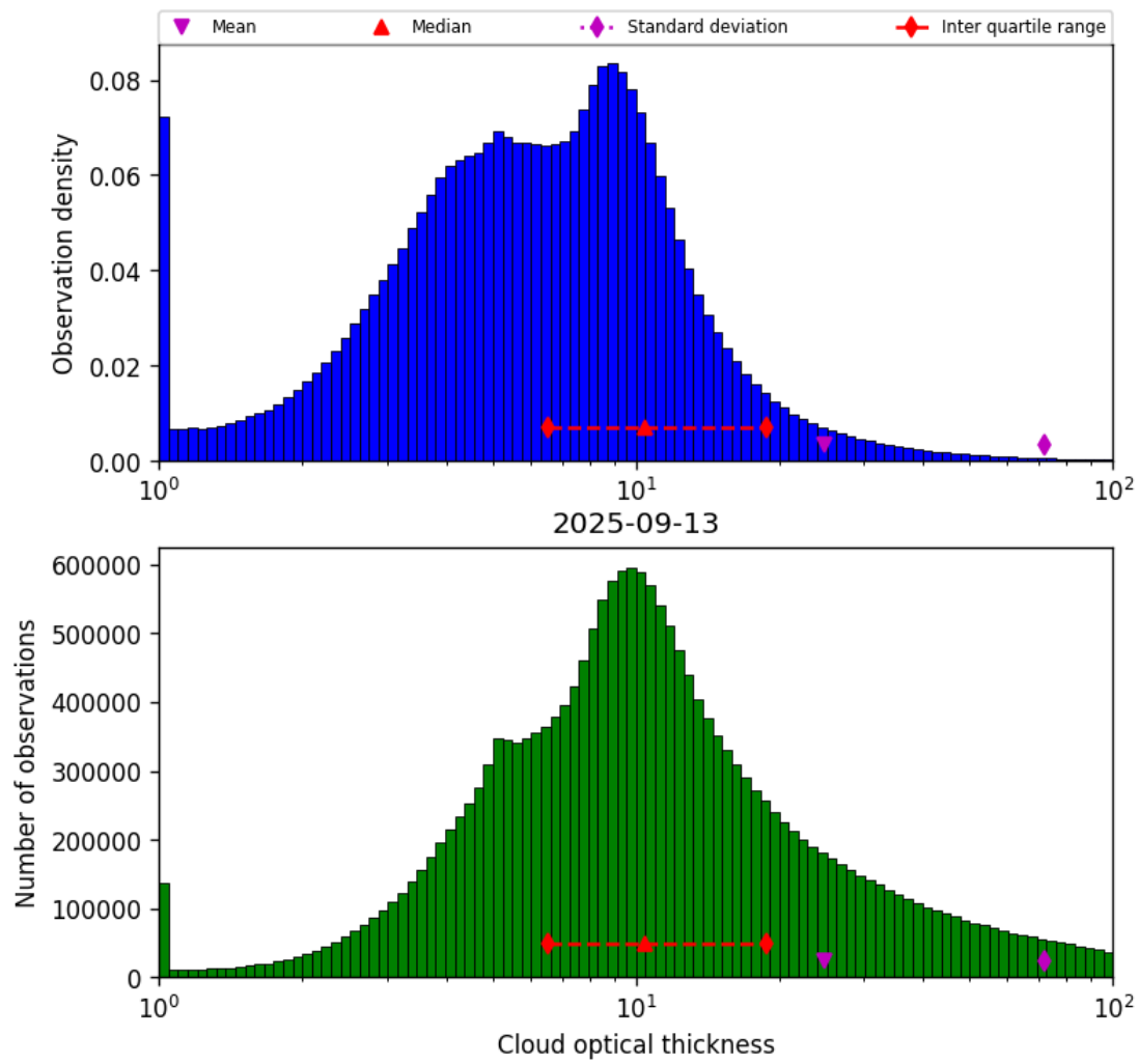
Figure 41: Histogram of “Cloud optical thickness” for 2025-09-12 to 2025-09-14
