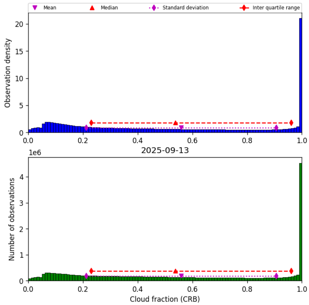
Figure 42: Histogram of “Cloud fraction (CRB)” for 2025-09-12 to 2025-09-14
