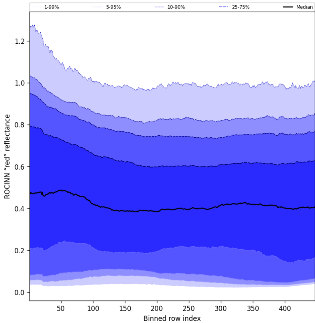
Figure 69: Along track statistics of “ROCINN “red” reflectance” for 2025-09-12 to 2025-09-14
