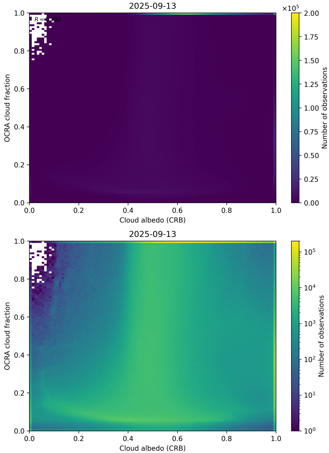
Figure 70: Scatter density plot of “Cloud albedo (CRB)” against “OCRA cloud fraction” for 2025-09-12 to 2025-09-14.
