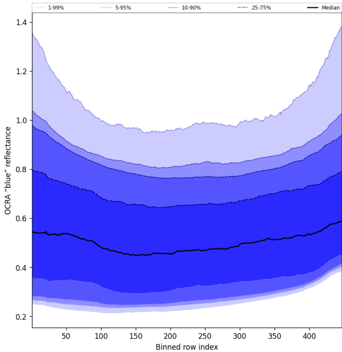
Figure 67: Along track statistics of “OCRA “blue” reflectance” for 2025-09-12 to 2025-09-14
