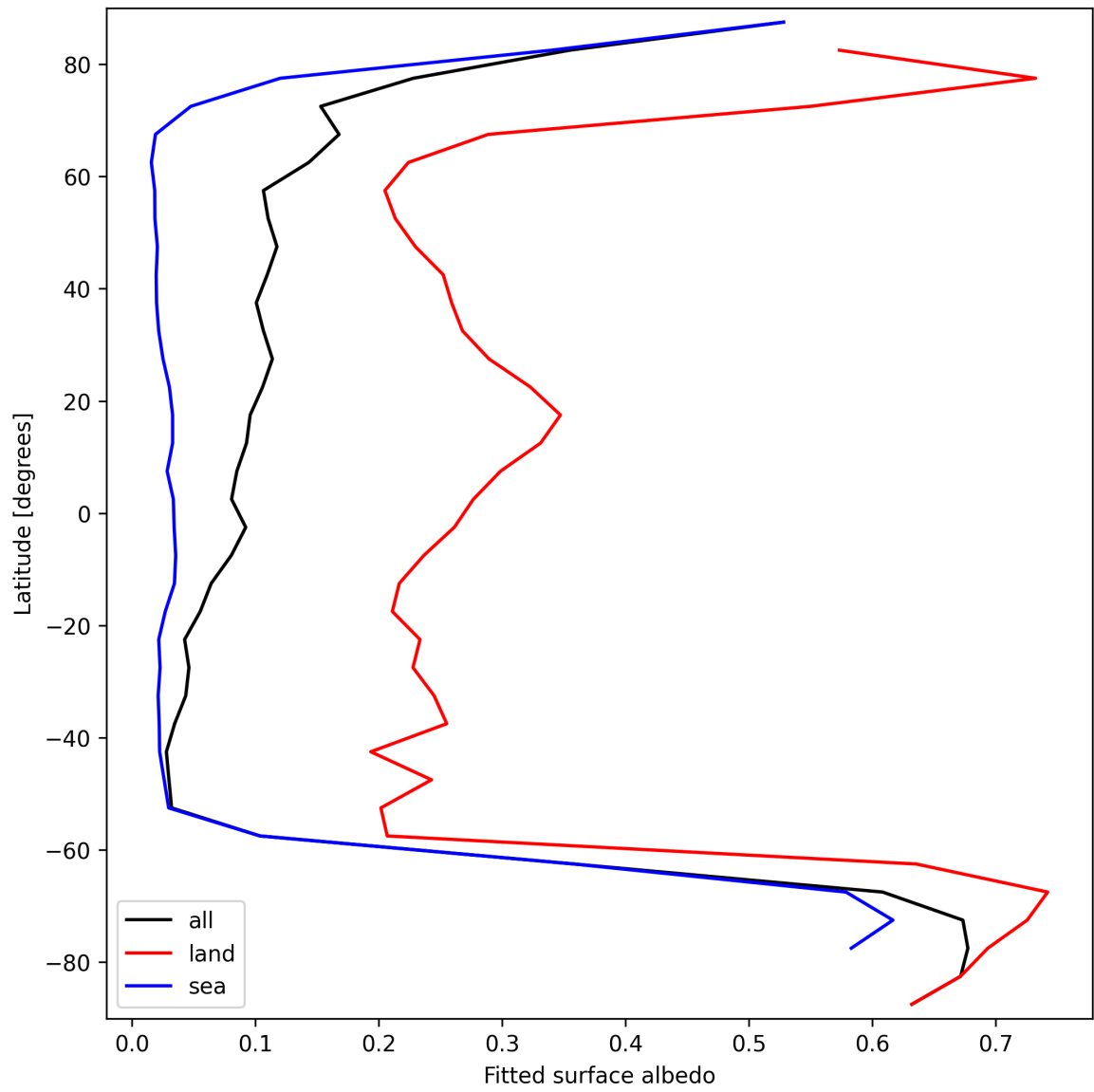
Figure 29: Zonal average of “Fitted surface albedo” for 2025-09-12 to 2025-09-14.
