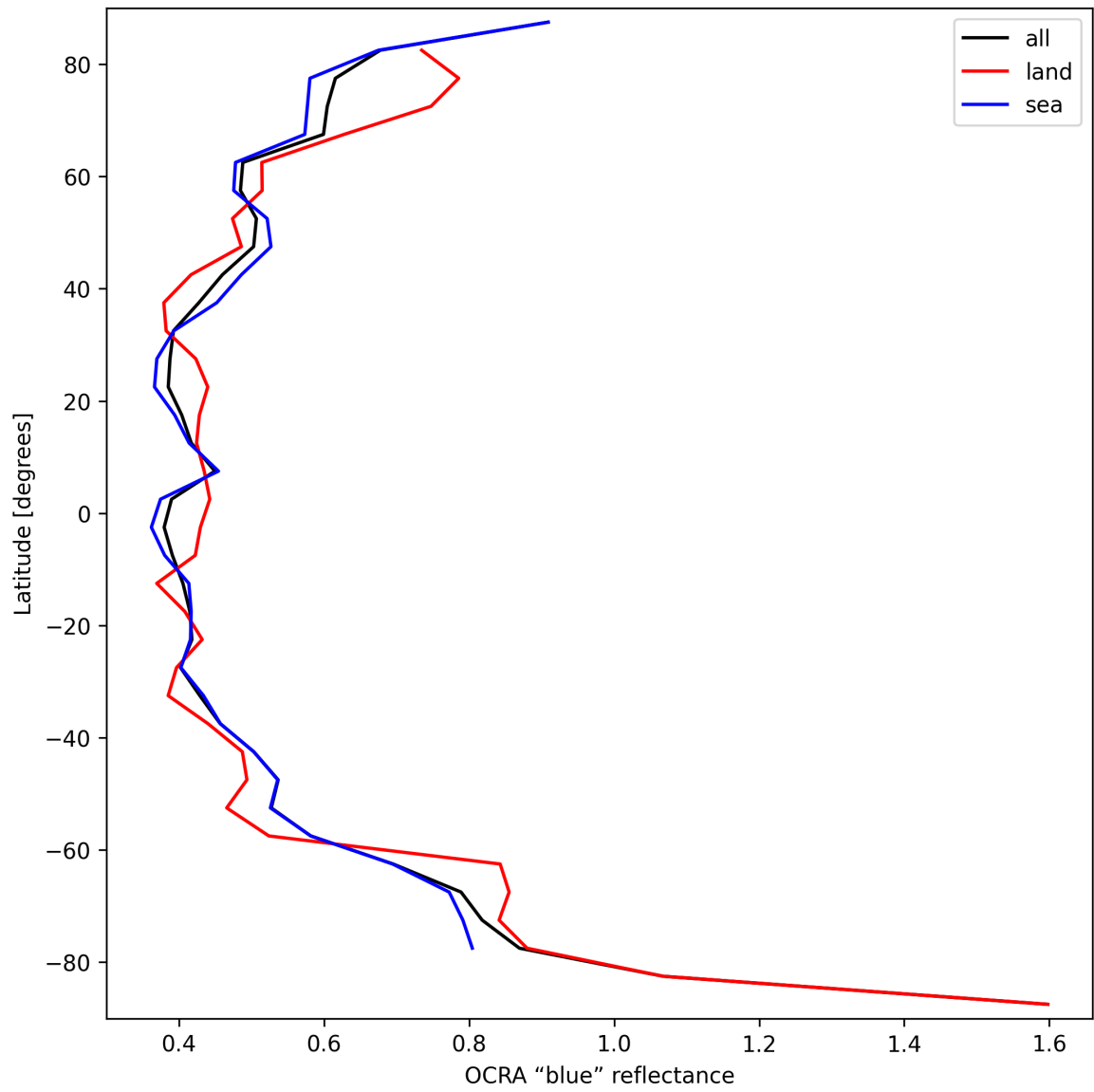
Figure 35: Zonal average of “OCRA “blue” reflectance” for 2025-09-12 to 2025-09-14.
