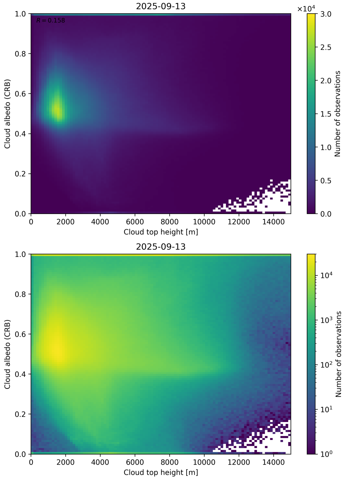
Figure 86: Scatter density plot of “Cloud top height” against “Cloud albedo (CRB)” for 2025-09-12 to 2025-09-14.
