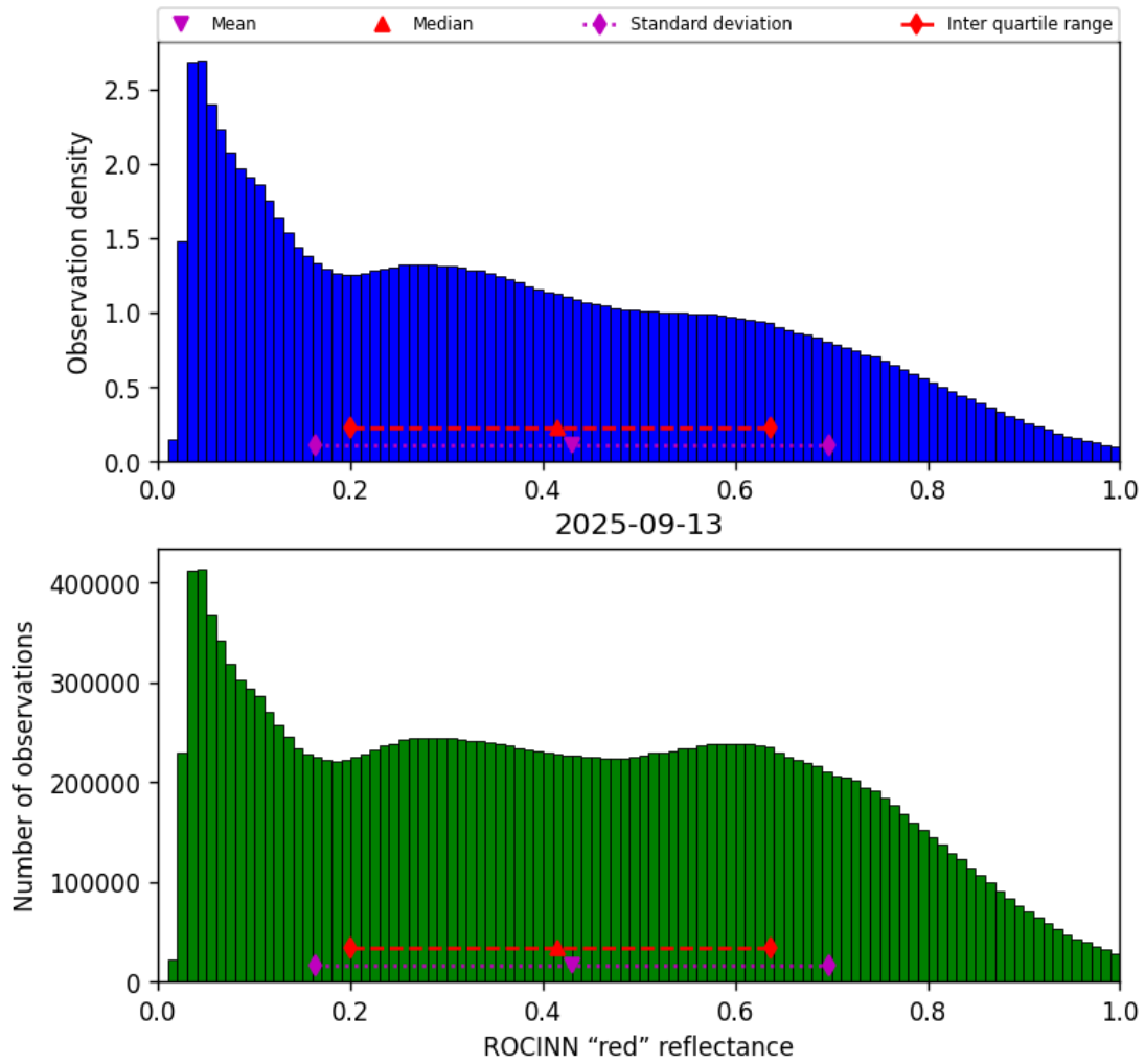
Figure 53: Histogram of “ROCINN “red” reflectance” for 2025-09-12 to 2025-09-14
