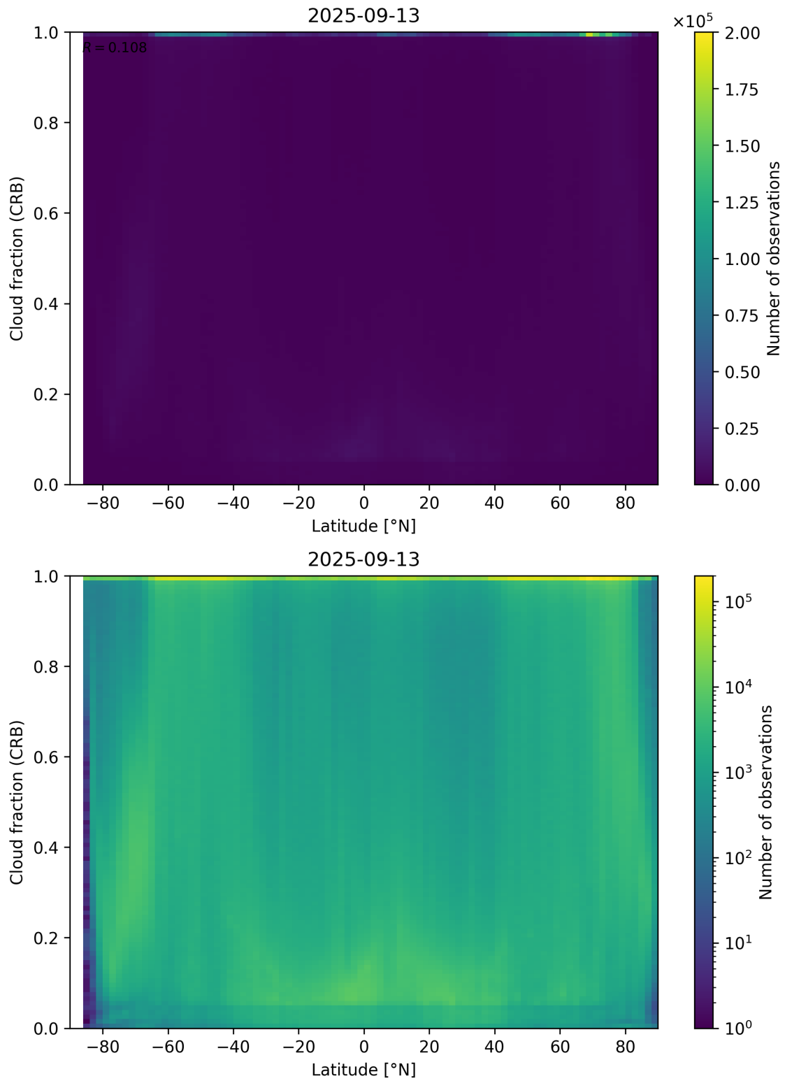
Figure 94: Scatter density plot of “Latitude” against “Cloud fraction (CRB)” for 2025-09-12 to 2025-09-14.
