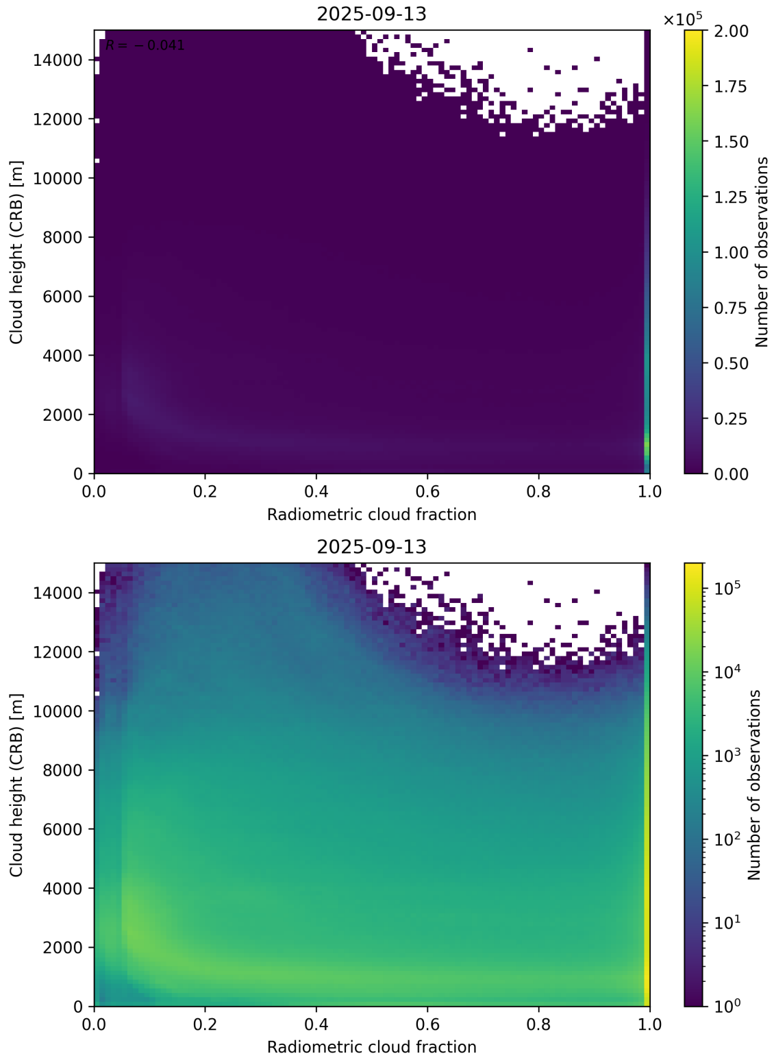
Figure 74: Scatter density plot of “Radiometric cloud fraction” against “Cloud height (CRB)” for 2025-09-12 to 2025-09-14.
