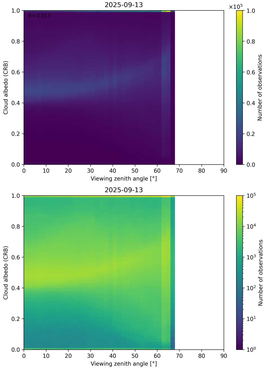
Figure 106: Scatter density plot of “Viewing zenith angle” against “Cloud albedo (CRB)” for 2025-09-12 to 2025-09-14.
