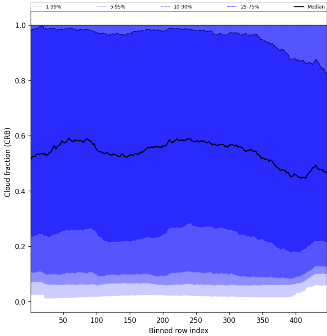
Figure 58: Along track statistics of “Cloud fraction (CRB)” for 2025-09-12 to 2025-09-14
