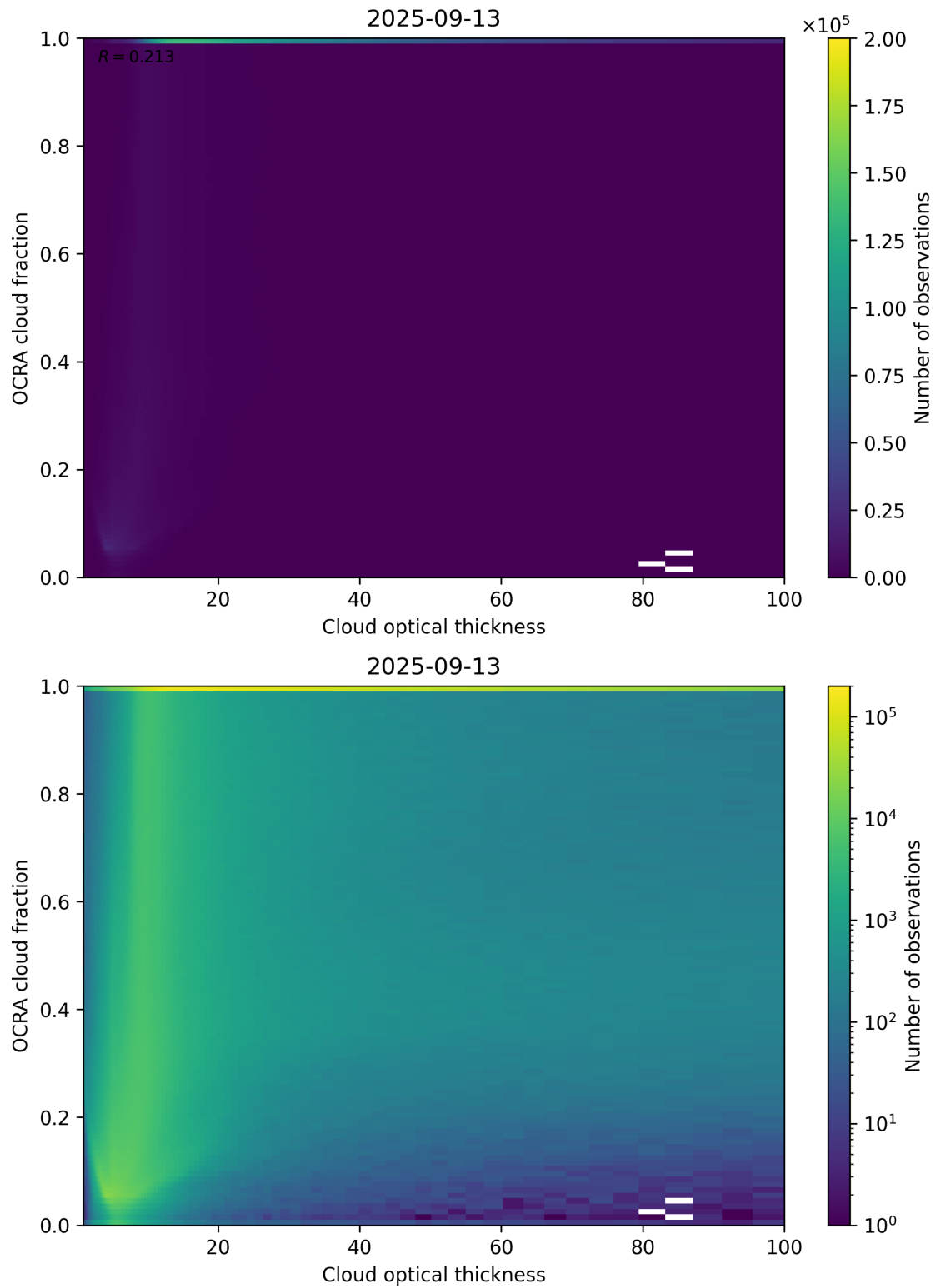
Figure 83: Scatter density plot of “Cloud optical thickness” against “OCRA cloud fraction” for 2025-09-12 to 2025-09-14.
