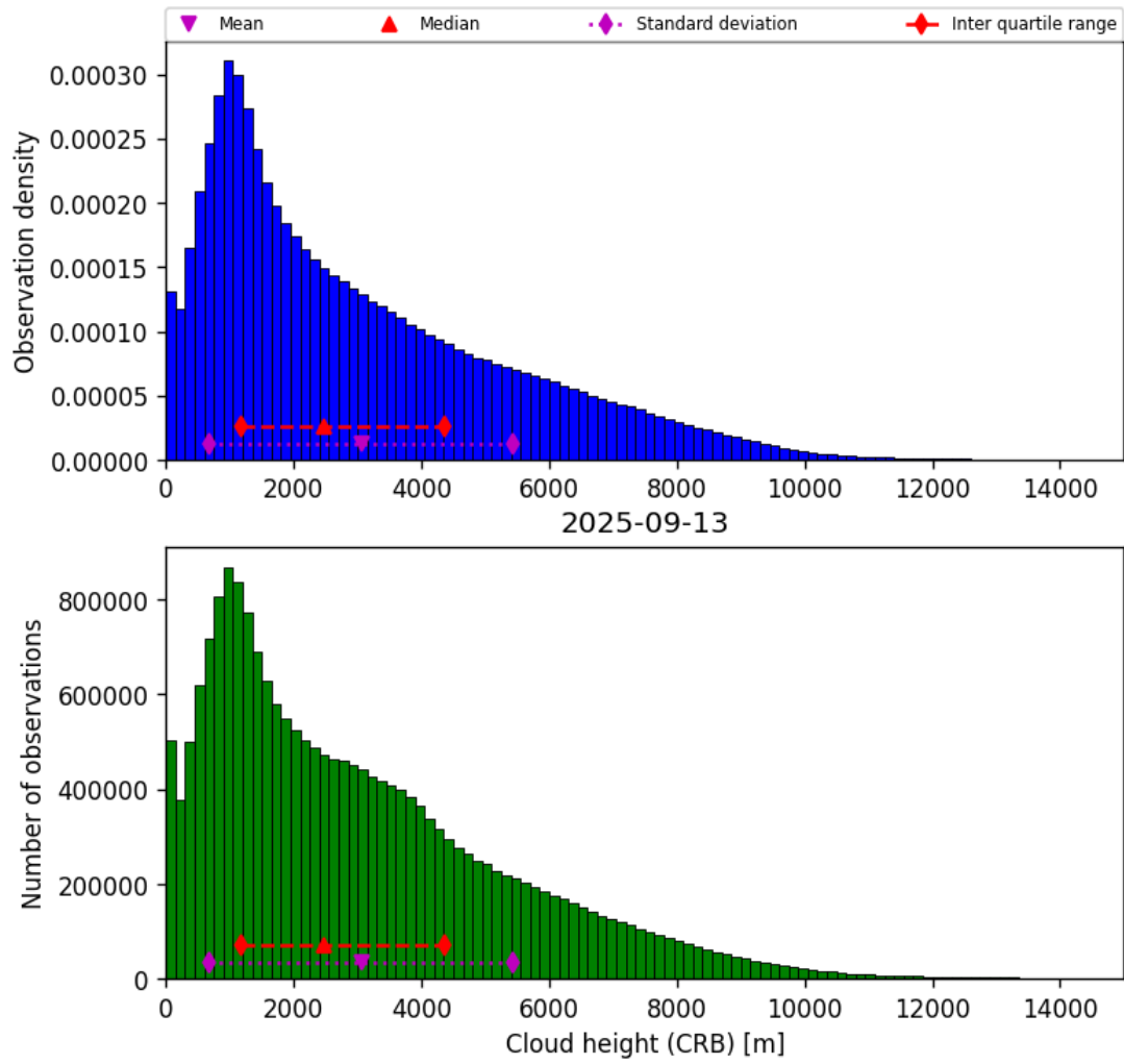
Figure 43: Histogram of “Cloud height (CRB)” for 2025-09-12 to 2025-09-14
