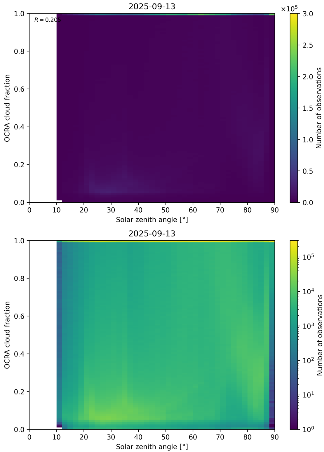
Figure 100: Scatter density plot of “Solar zenith angle” against “OCRA cloud fraction” for 2025-09-12 to 2025-09-14.
