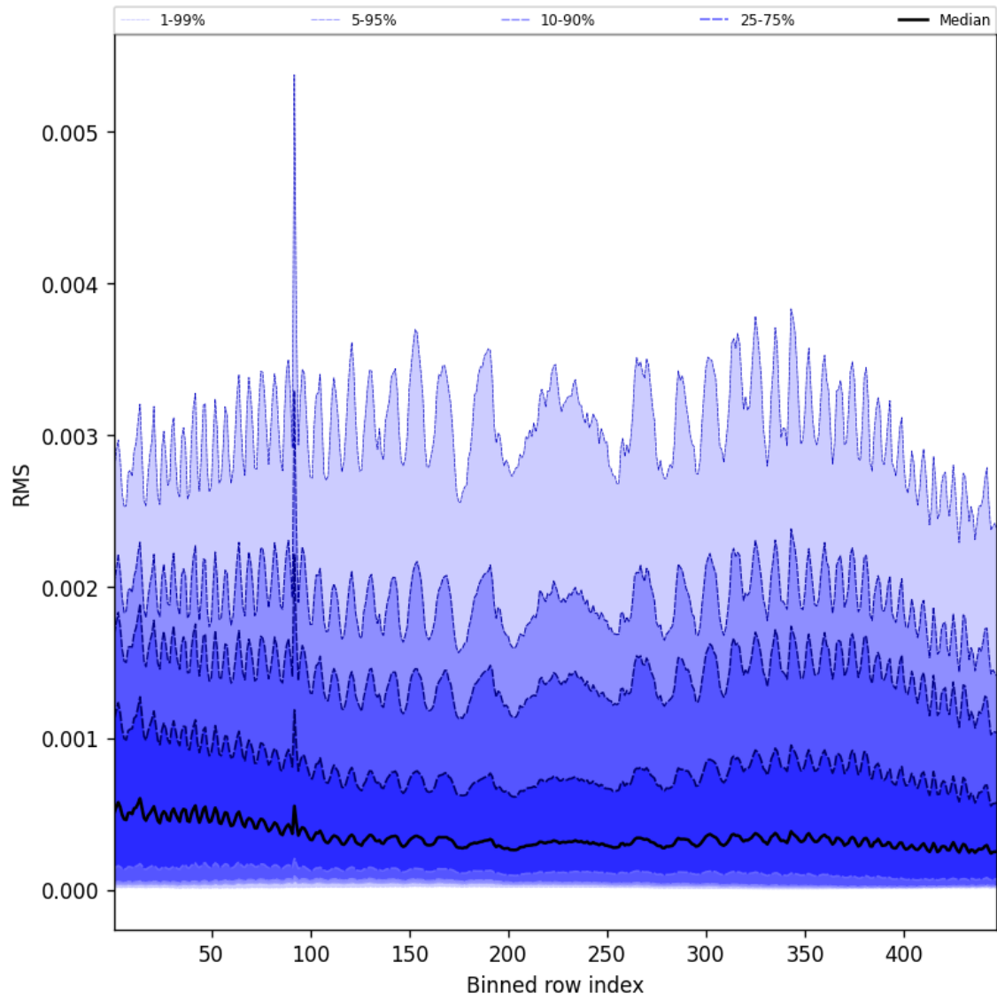
Figure 63: Along track statistics of “RMS” for 2025-09-12 to 2025-09-14
