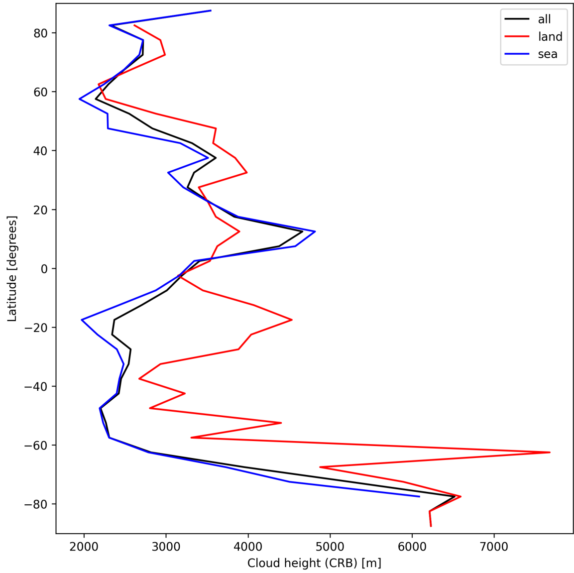
Figure 27: Zonal average of “Cloud height (CRB)” for 2025-09-12 to 2025-09-14.
