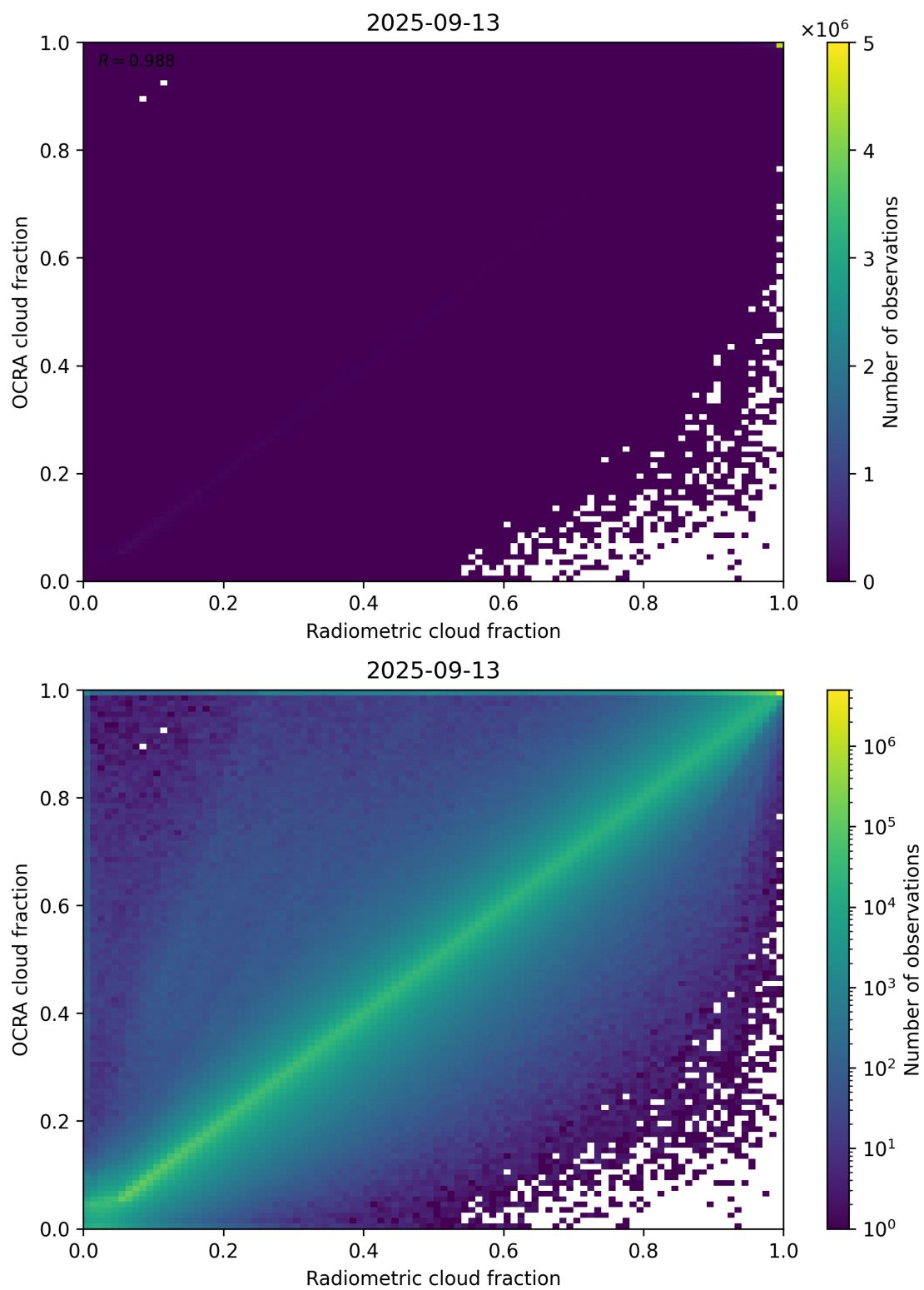
Figure 72: Scatter density plot of “Radiometric cloud fraction” against “OCRA cloud fraction” for 2025-09-12 to 2025-09-14.
