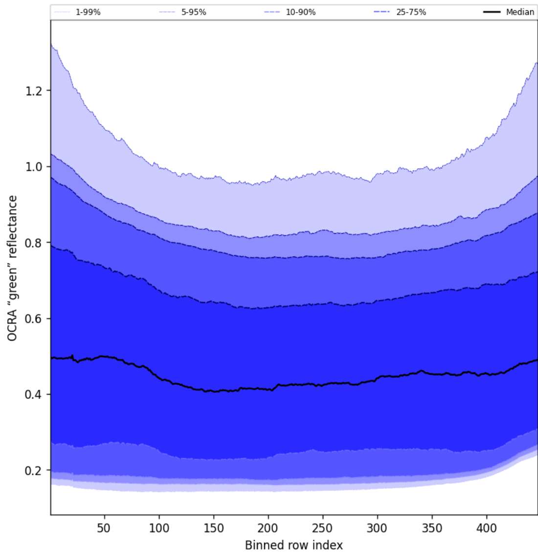
Figure 68: Along track statistics of "OCRA "green" reflectance" for 2025-09-12 to 2025-09-14
