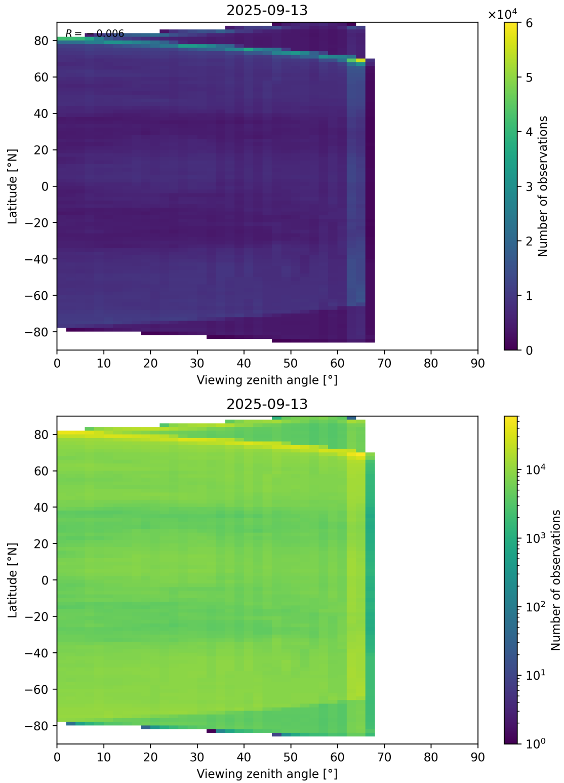
Figure 113: Scatter density plot of “Viewing zenith angle” against “Latitude” for 2025-09-12 to 2025-09-14.
