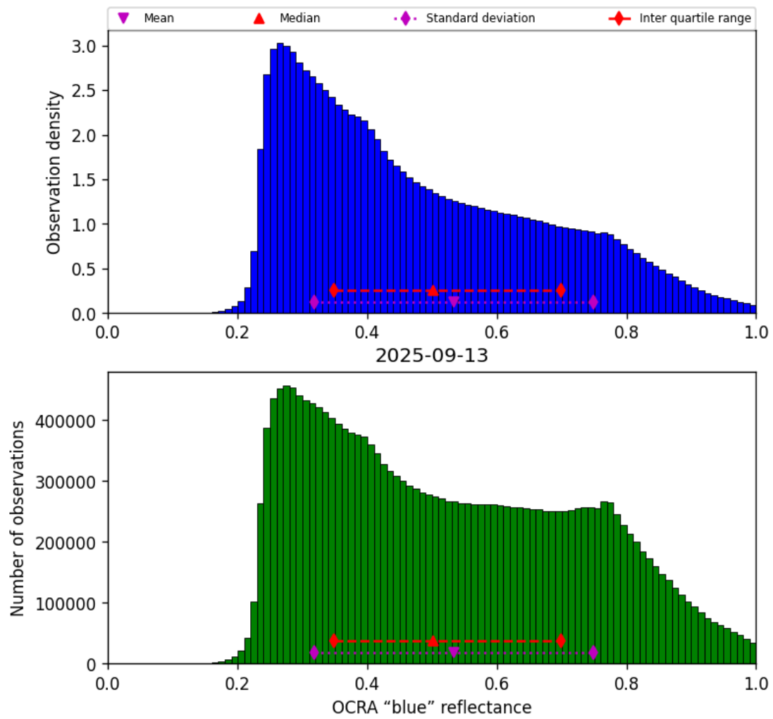
Figure 51: Histogram of “OCRA “blue” reflectance” for 2025-09-12 to 2025-09-14
