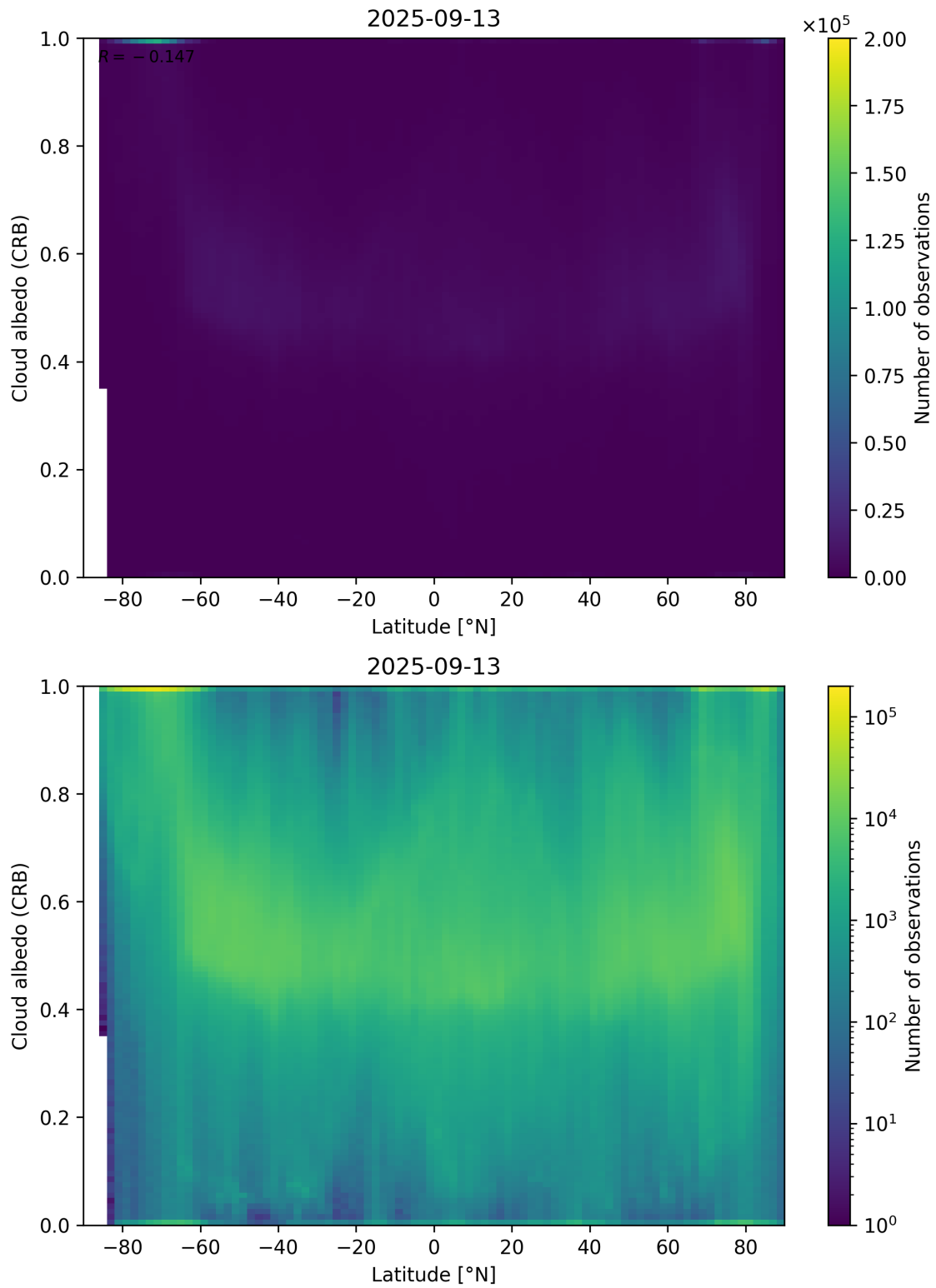
Figure 91: Scatter density plot of “Latitude” against “Cloud albedo (CRB)” for 2025-09-12 to 2025-09-14.
