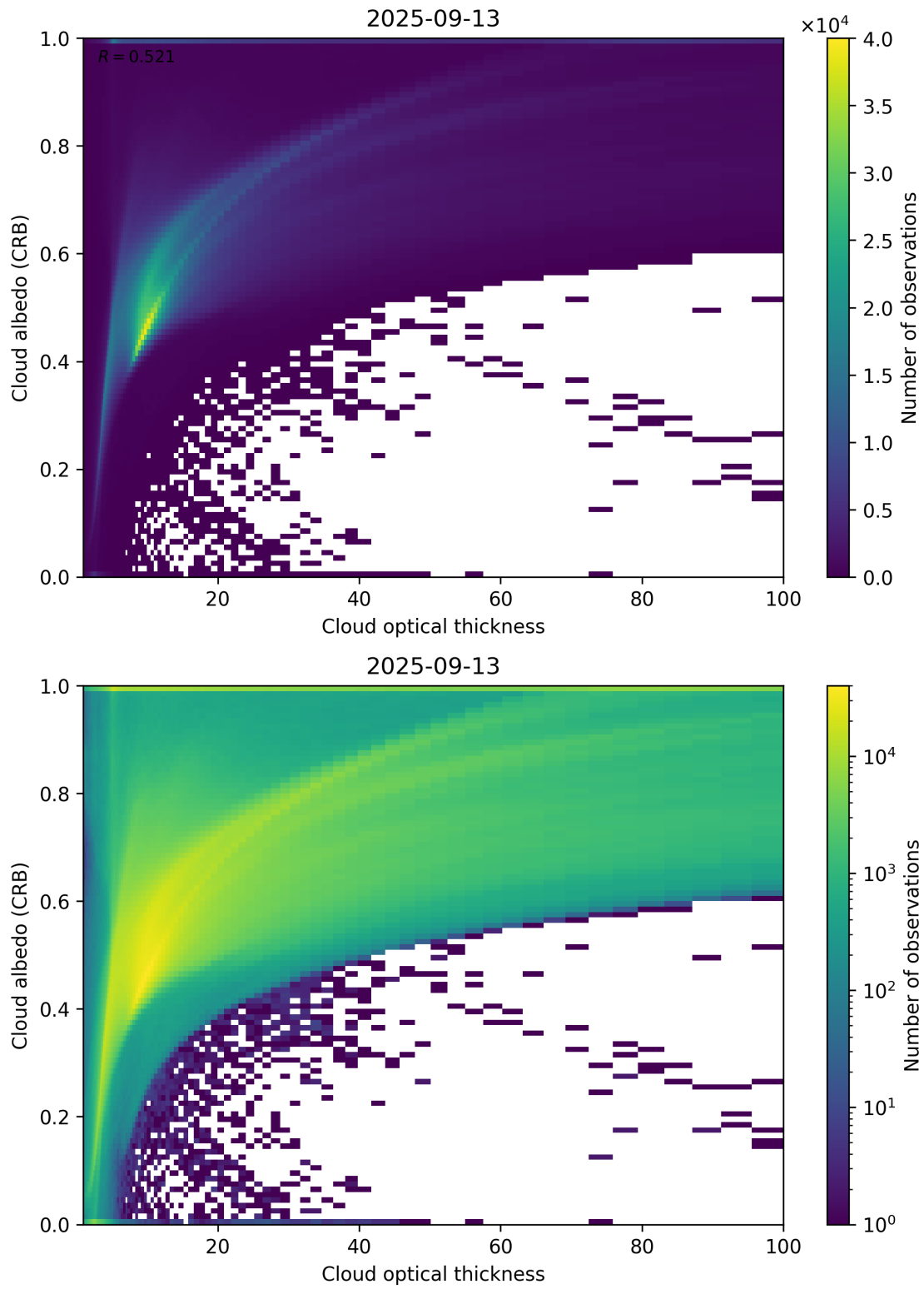
Figure 82: Scatter density plot of “Cloud optical thickness” against “Cloud albedo (CRB)” for 2025-09-12 to 2025-09-14.
