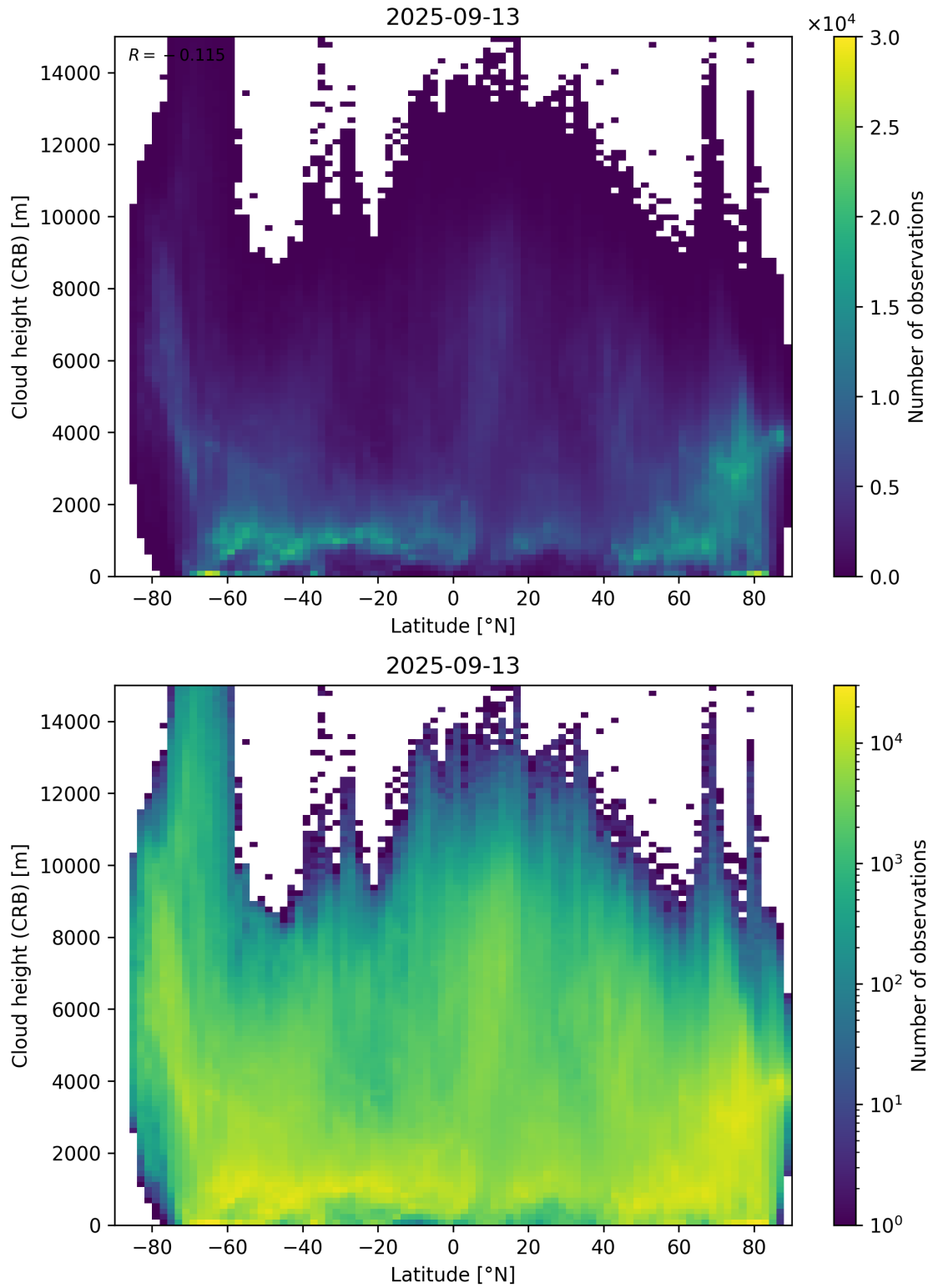
Figure 95: Scatter density plot of “Latitude” against “Cloud height (CRB)” for 2025-09-12 to 2025-09-14.
