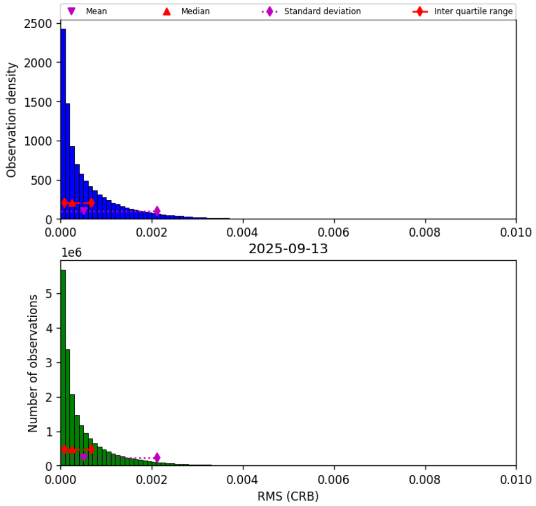
Figure 48: Histogram of “RMS (CRB)” for 2025-09-12 to 2025-09-14
