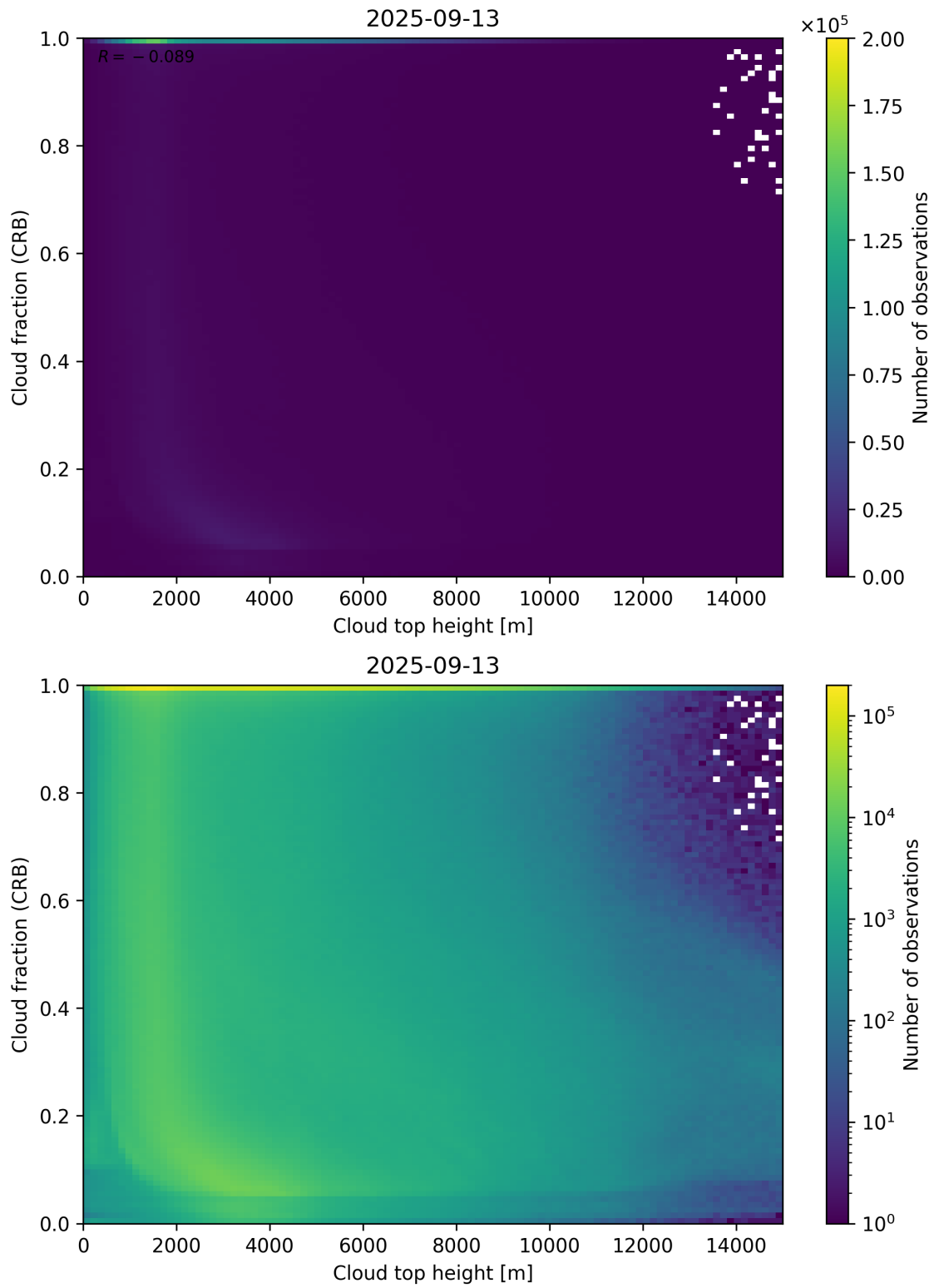
Figure 88: Scatter density plot of “Cloud top height” against “Cloud fraction (CRB)” for 2025-09-12 to 2025-09-14.
