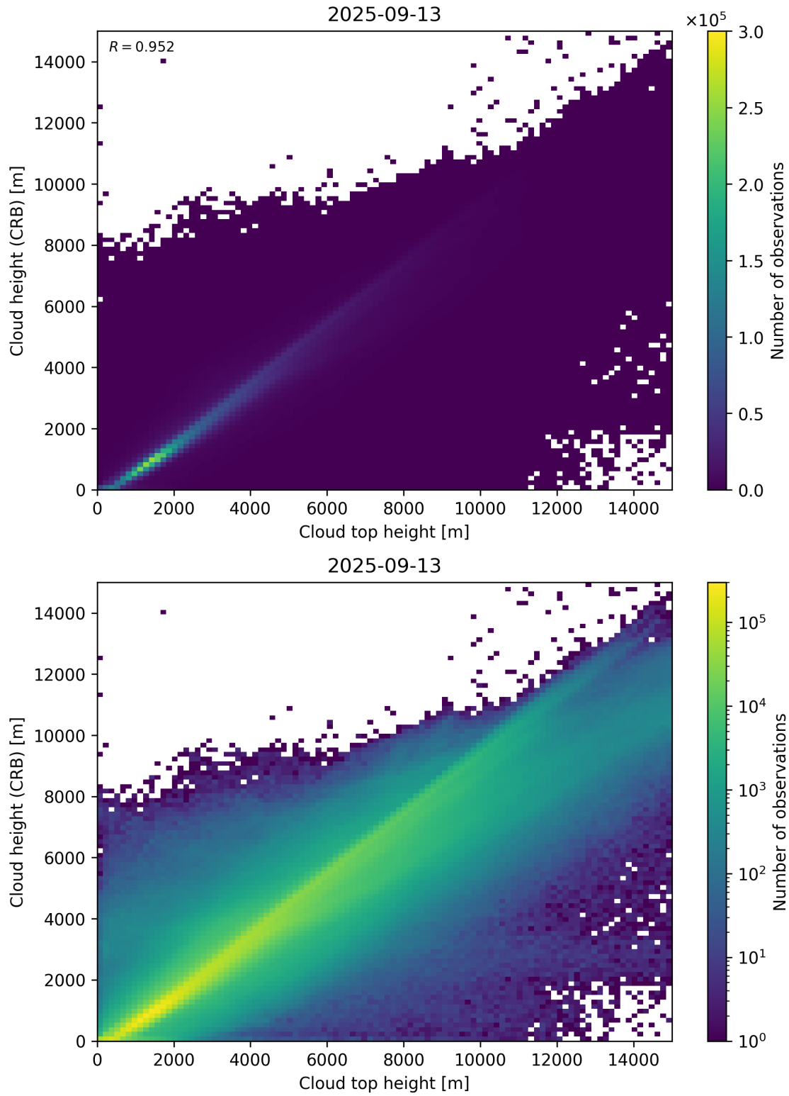
Figure 89: Scatter density plot of “Cloud top height” against “Cloud height (CRB)” for 2025-09-12 to 2025-09-14.
