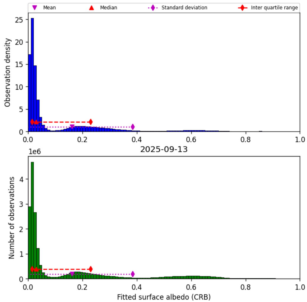
Figure 46: Histogram of “Fitted surface albedo (CRB)” for 2025-09-12 to 2025-09-14
