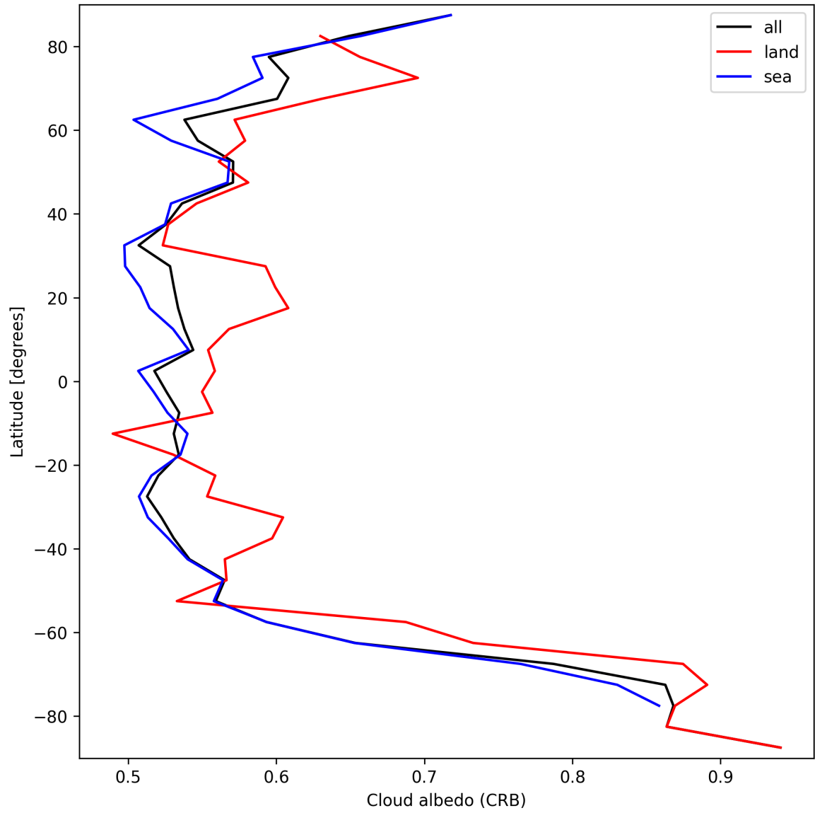
Figure 28: Zonal average of “Cloud albedo (CRB)” for 2025-09-12 to 2025-09-14.
