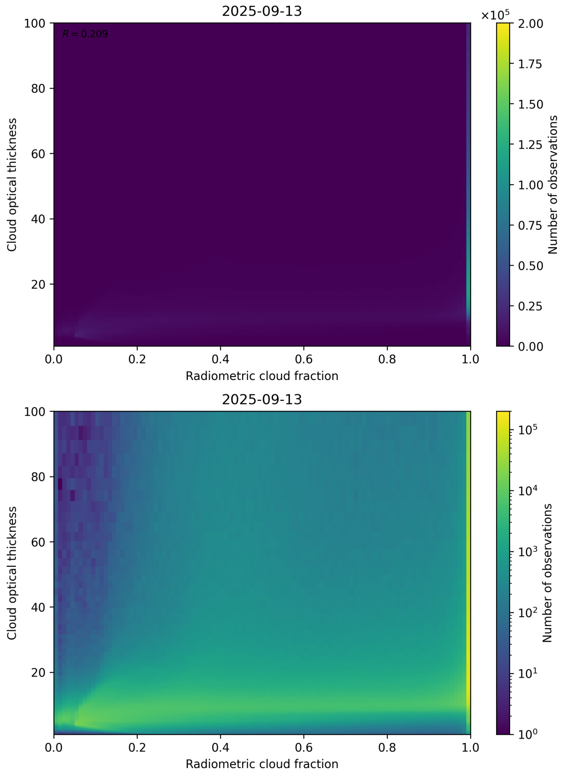
Figure 75: Scatter density plot of “Radiometric cloud fraction” against “Cloud optical thickness” for 2025-09-12 to 2025-09-14.
