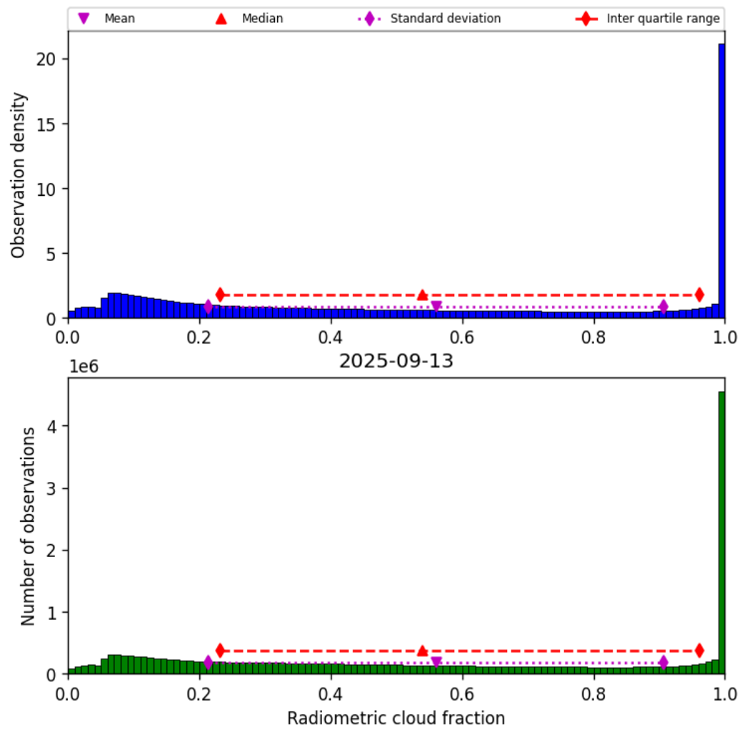
Figure 39: Histogram of “Radiometric cloud fraction” for 2025-09-12 to 2025-09-14
