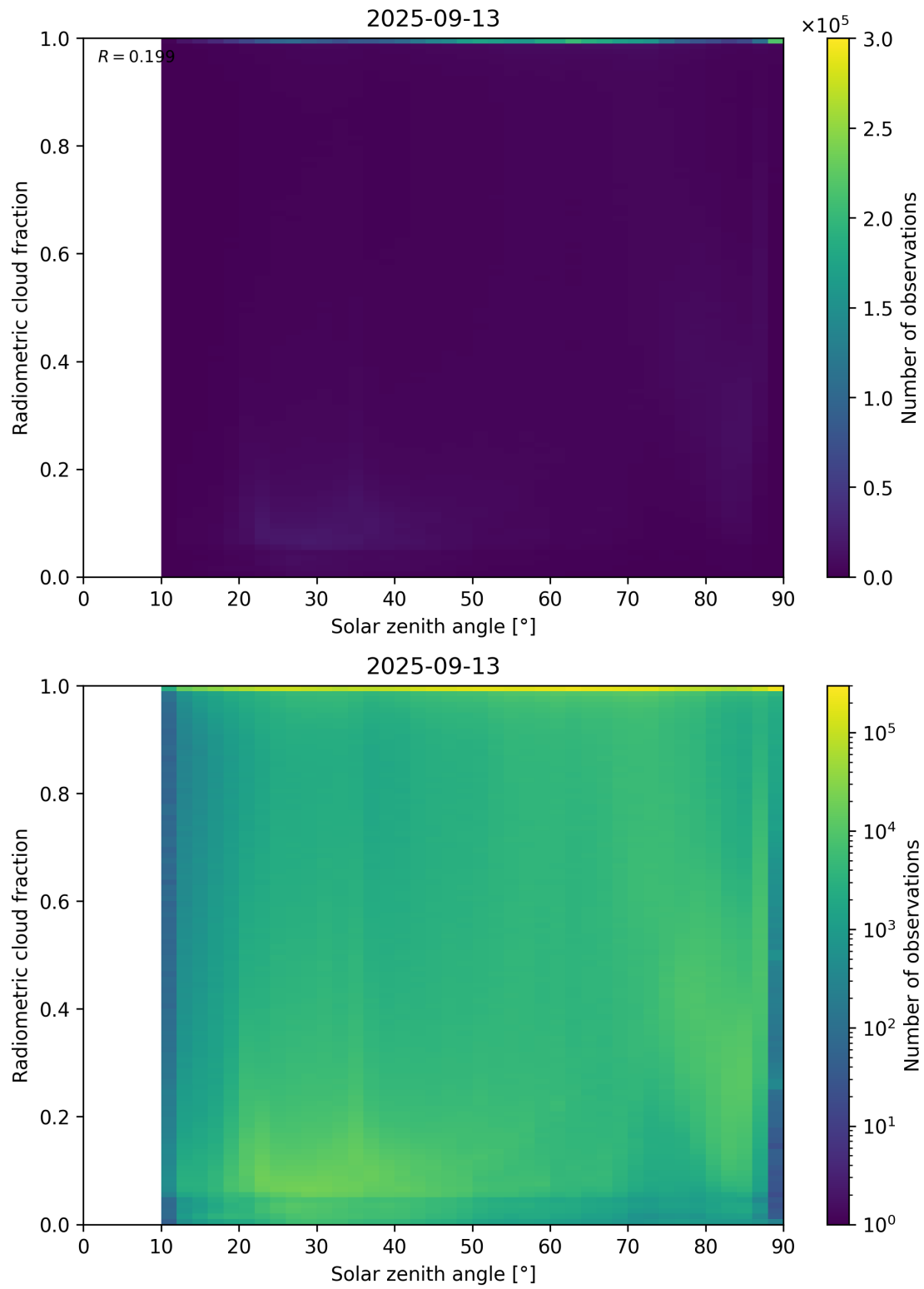
Figure 99: Scatter density plot of “Solar zenith angle” against “Radiometric cloud fraction” for 2025-09-12 to 2025-09-14.
