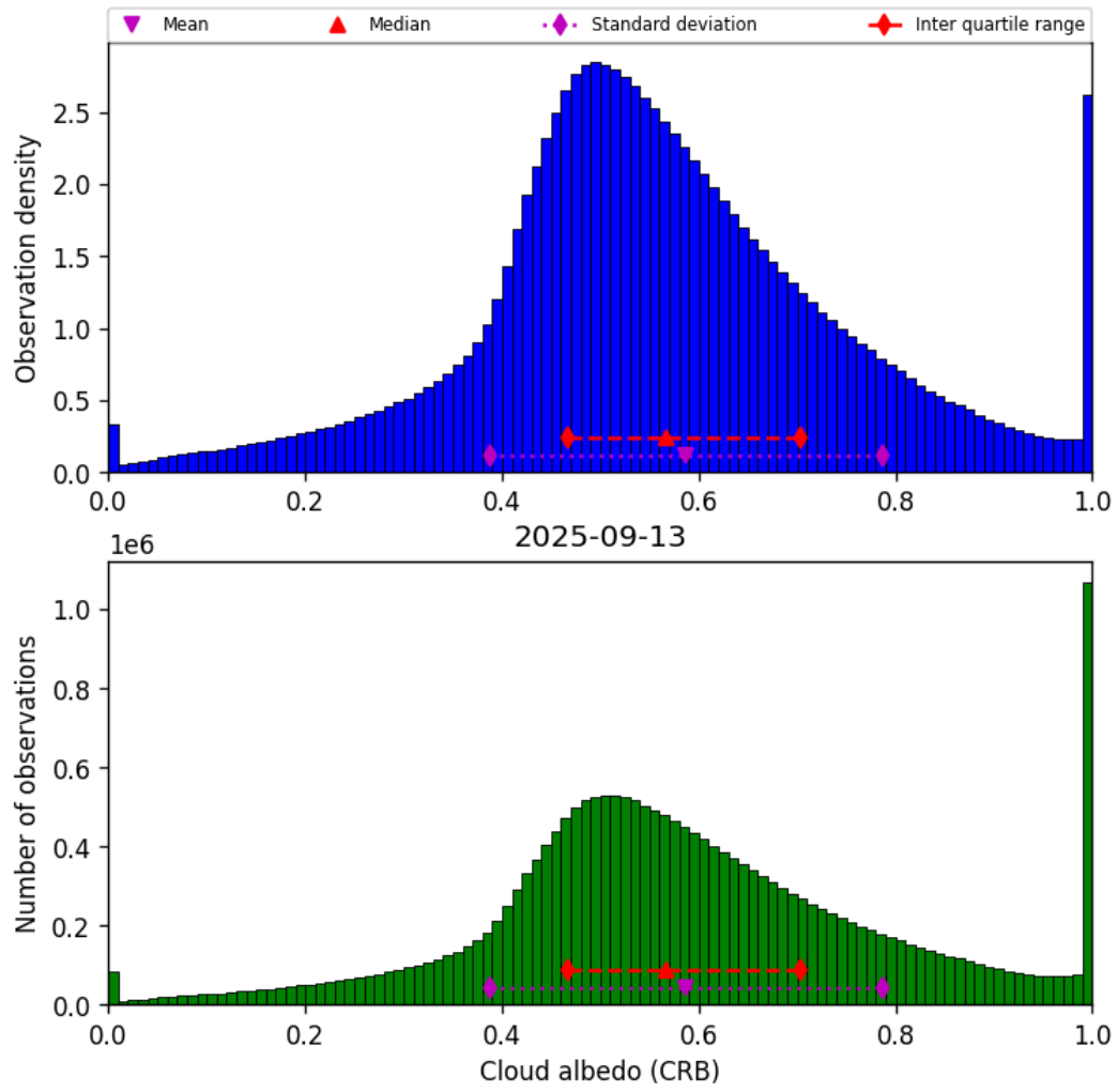
Figure 44: Histogram of “Cloud albedo (CRB)” for 2025-09-12 to 2025-09-14
