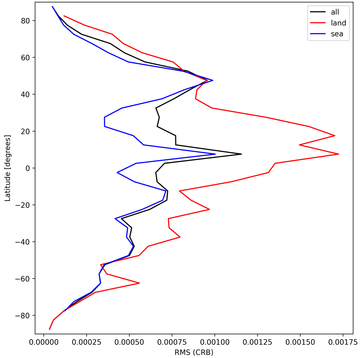
Figure 32: Zonal average of “RMS (CRB)” for 2025-09-12 to 2025-09-14.
