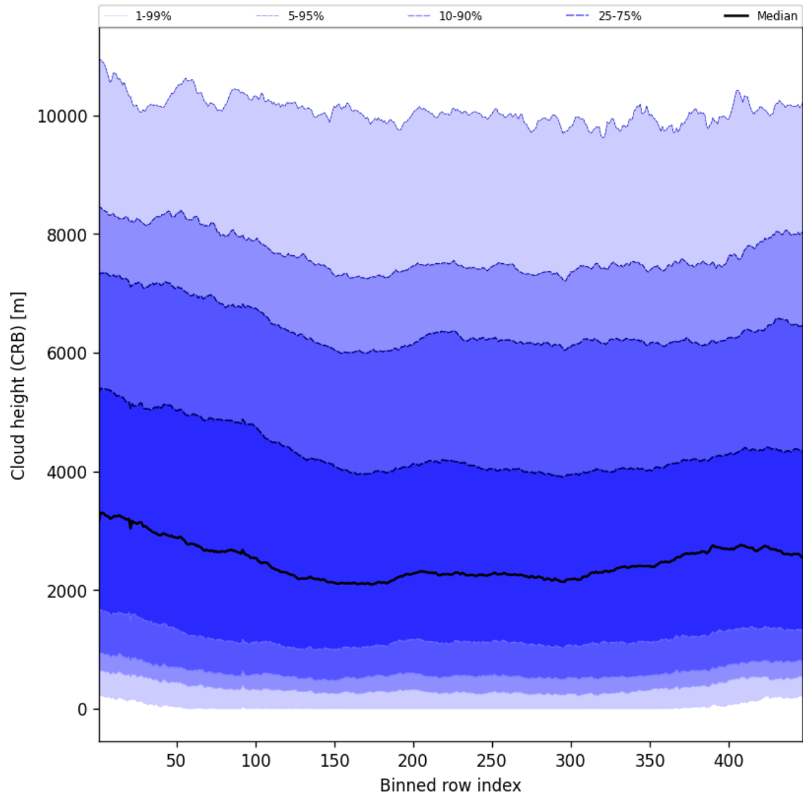
Figure 59: Along track statistics of “Cloud height (CRB)” for 2025-09-12 to 2025-09-14
