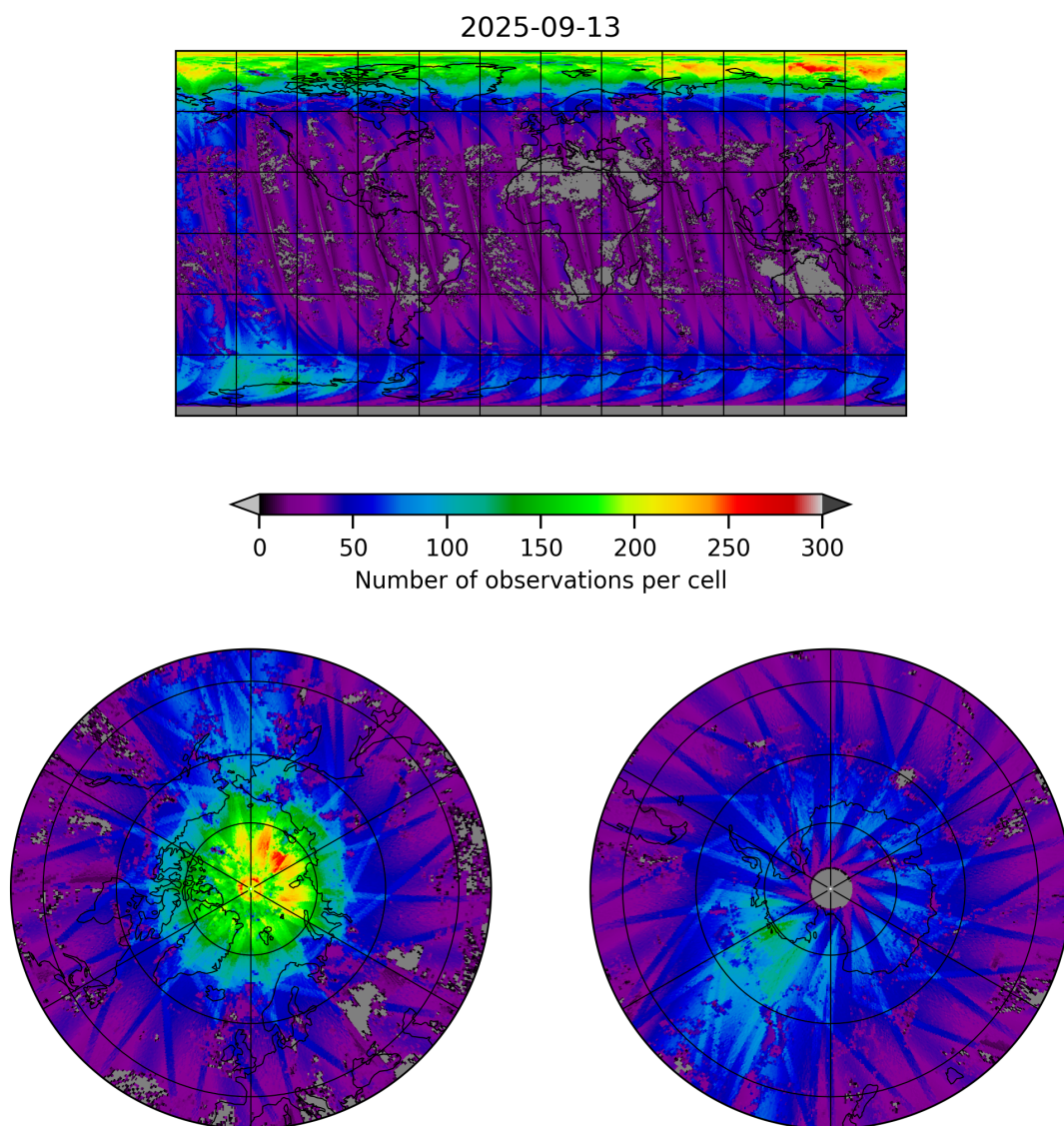
Figure 21: Map of the number of observations for 2025-09-12 to 2025-09-14
