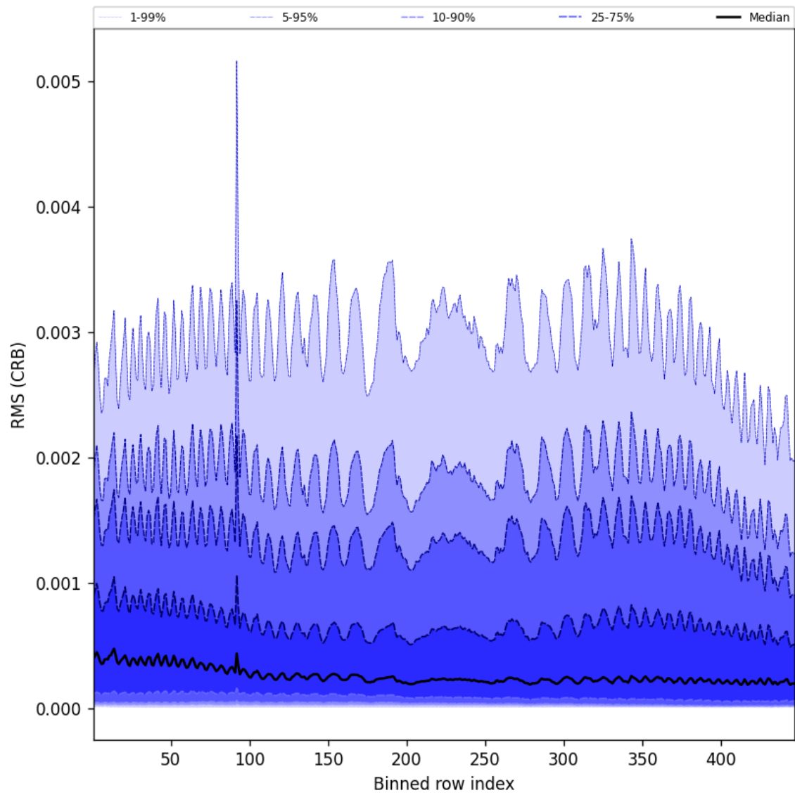
Figure 64: Along track statistics of “RMS (CRB)” for 2025-09-12 to 2025-09-14
