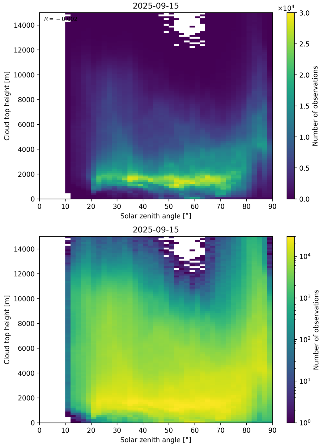
Figure 104: Scatter density plot of “Solar zenith angle” against “Cloud top height” for 2025-09-15 to 2025-09-16.
