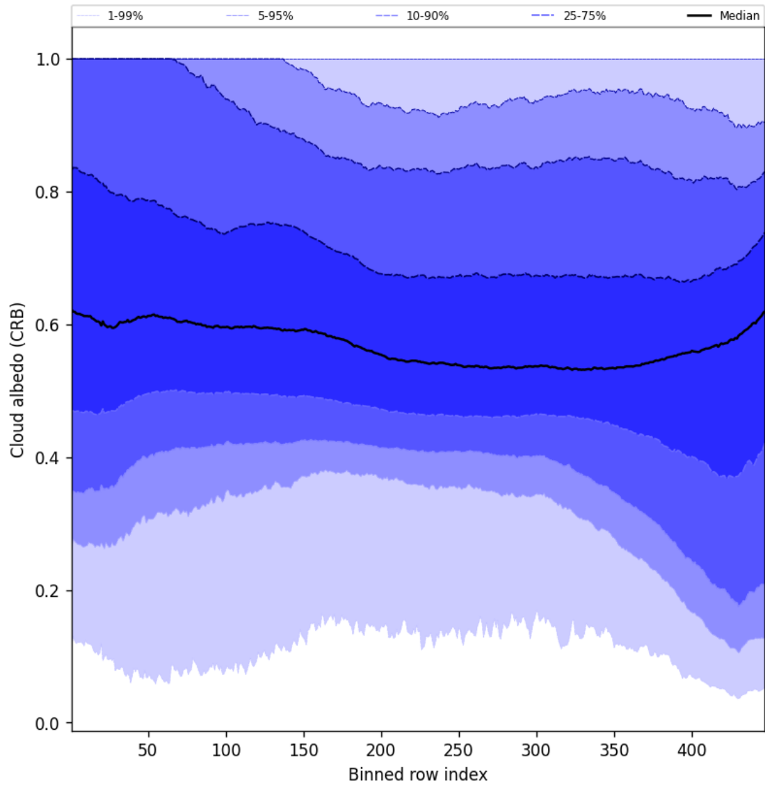
Figure 60: Along track statistics of “Cloud albedo (CRB)” for 2025-09-15 to 2025-09-16
