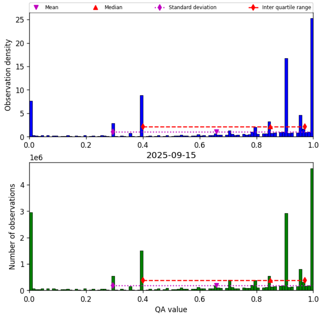
Figure 38: Histogram of “QA value” for 2025-09-15 to 2025-09-16
