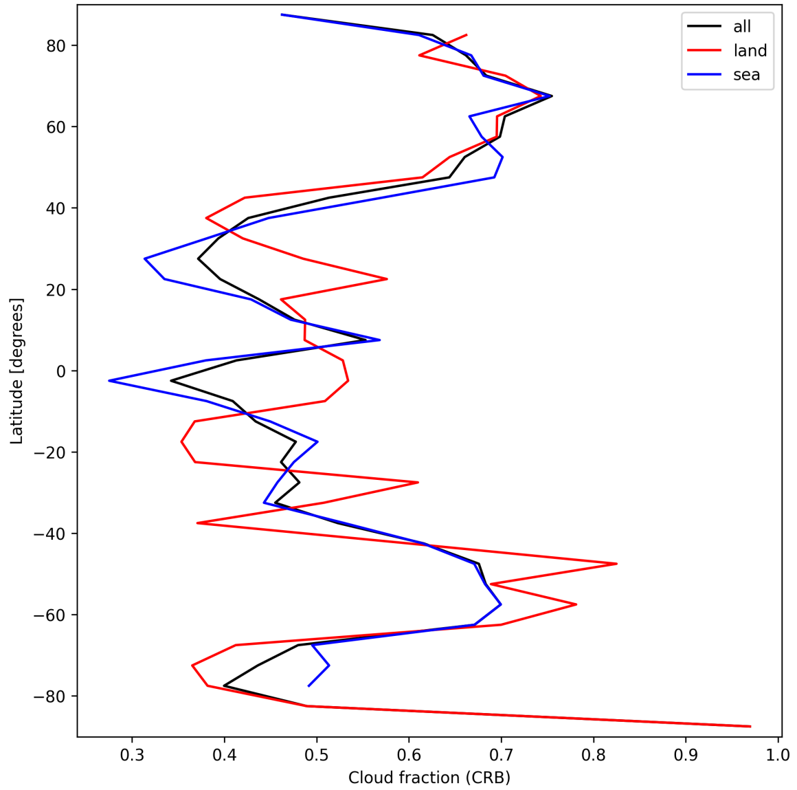
Figure 26: Zonal average of “Cloud fraction (CRB)” for 2025-09-15 to 2025-09-16.
