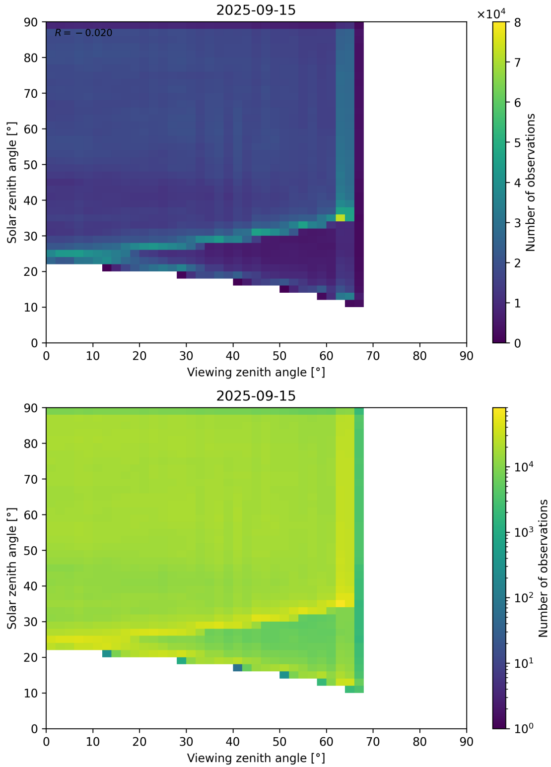
Figure 114: Scatter density plot of “Viewing zenith angle” against “Solar zenith angle” for 2025-09-15 to 2025-09-16.
