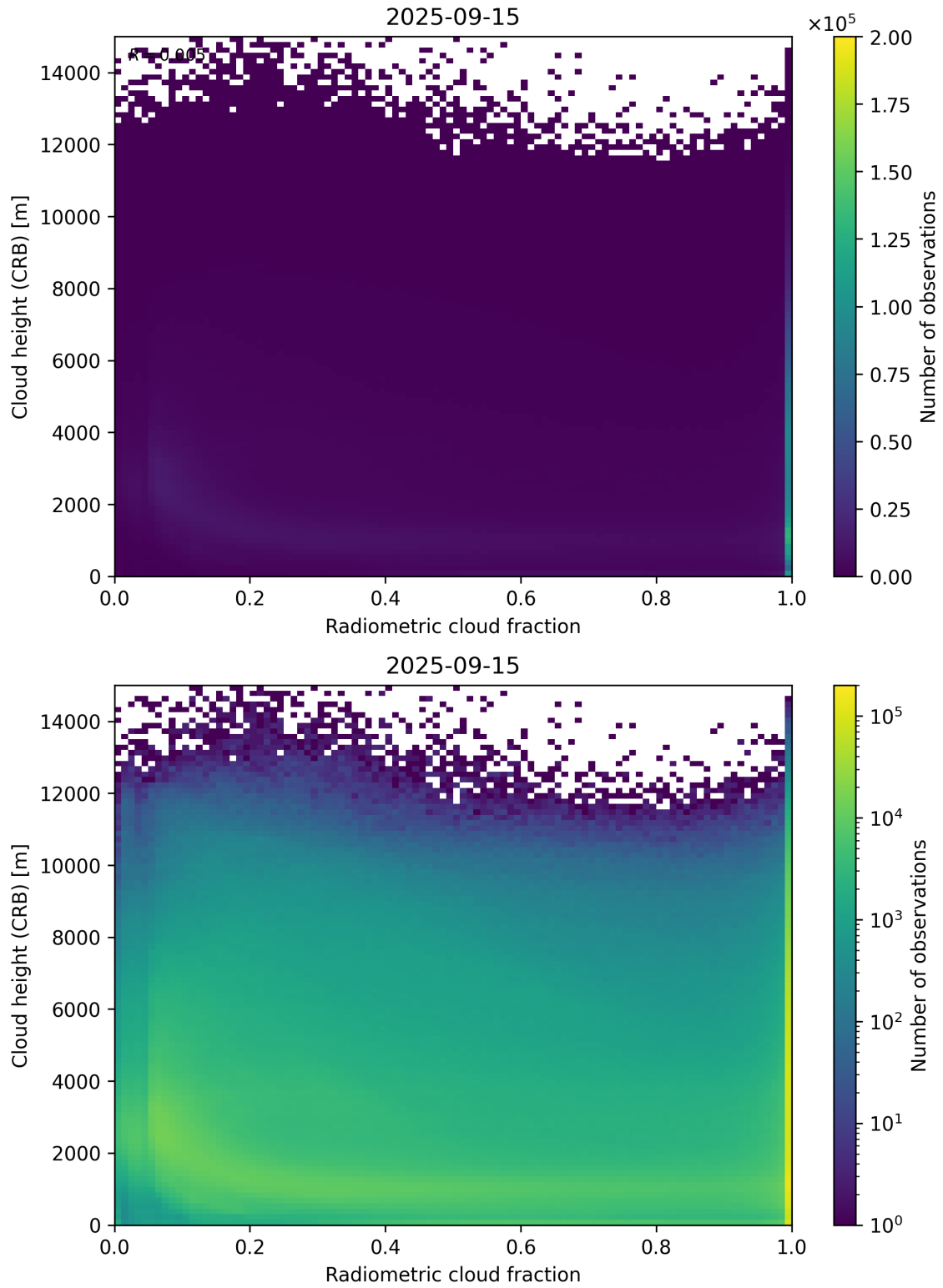
Figure 74: Scatter density plot of “Radiometric cloud fraction” against “Cloud height (CRB)” for 2025-09-15 to 2025-09-16.
