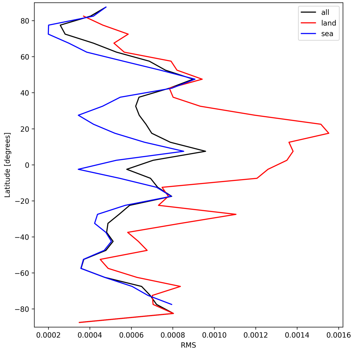
Figure 31: Zonal average of “RMS” for 2025-09-15 to 2025-09-16.
