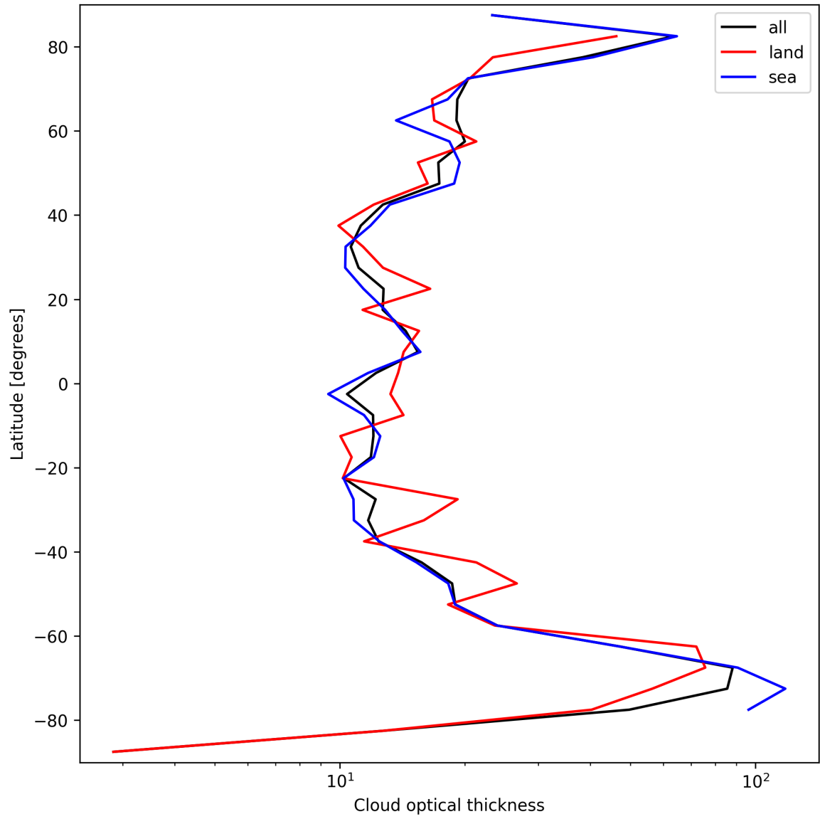
Figure 25: Zonal average of “Cloud optical thickness” for 2025-09-15 to 2025-09-16.
