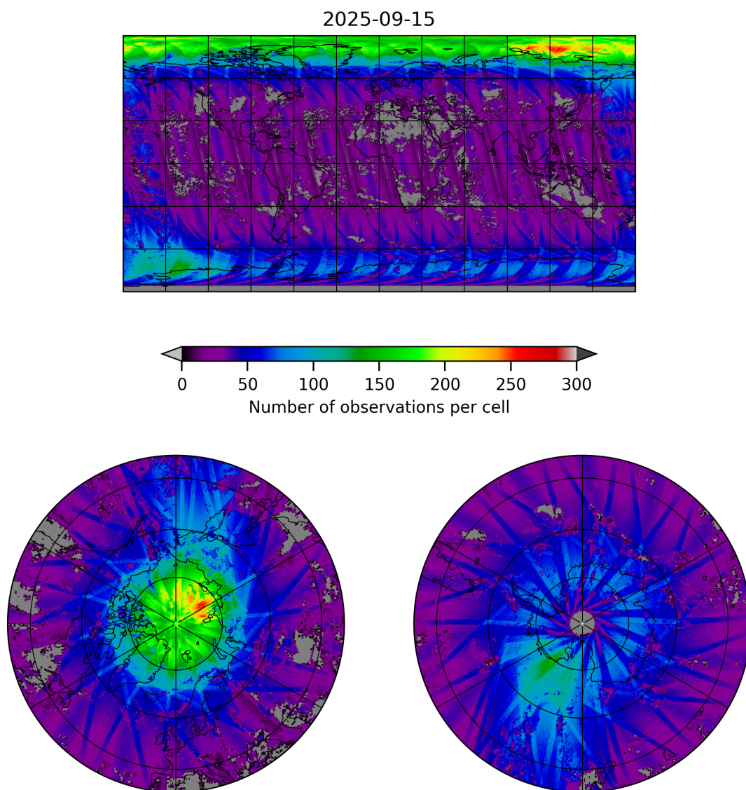
Figure 21: Map of the number of observations for 2025-09-15 to 2025-09-16
