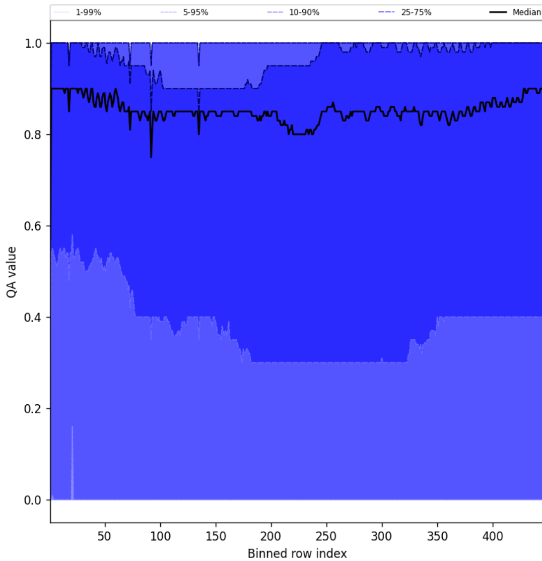
Figure 54: Along track statistics of “QA value” for 2025-09-15 to 2025-09-16
