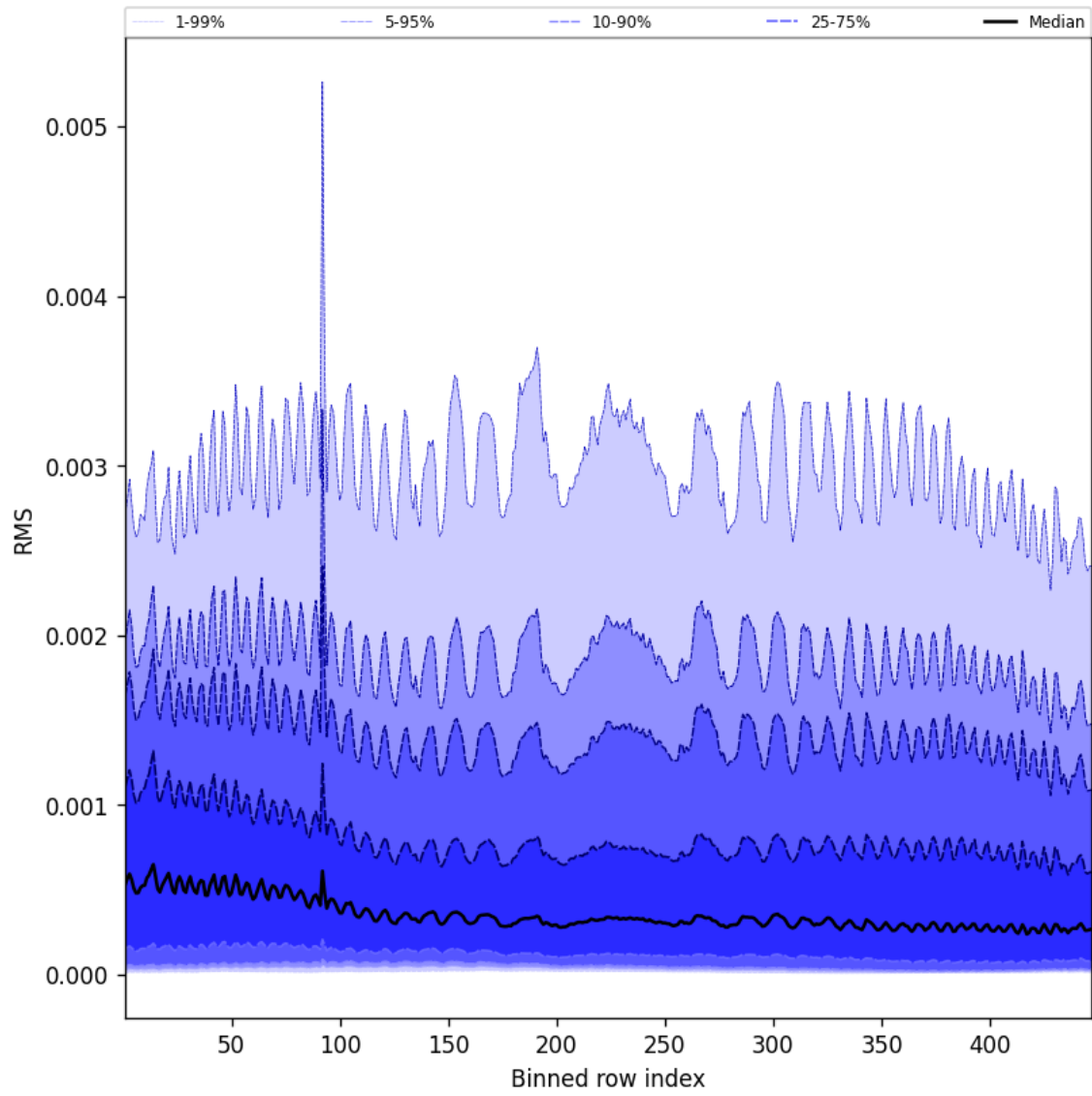
Figure 63: Along track statistics of “RMS” for 2025-09-15 to 2025-09-16
