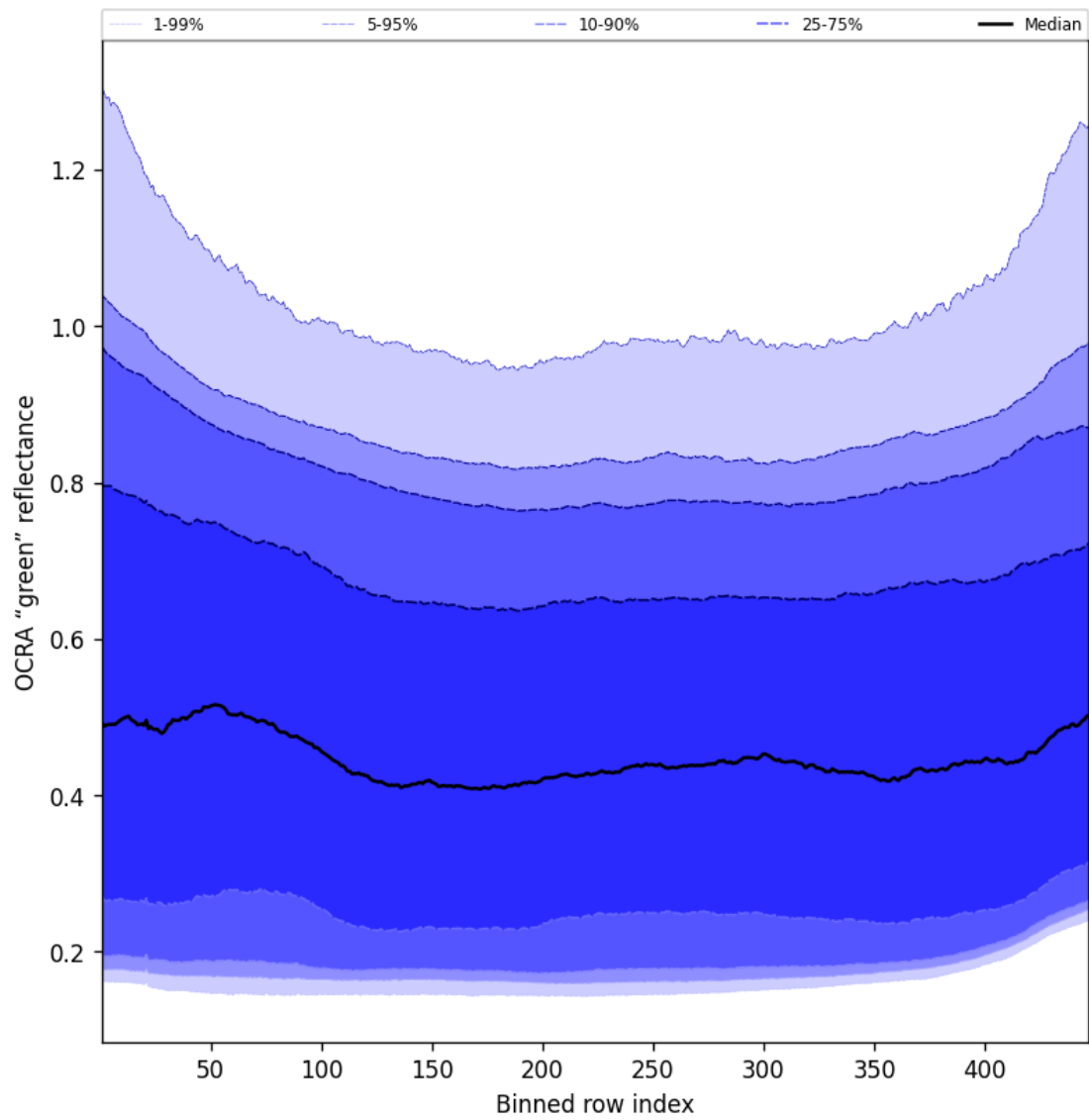
Figure 68: Along track statistics of “OCRA “green” reflectance” for 2025-09-15 to 2025-09-16
