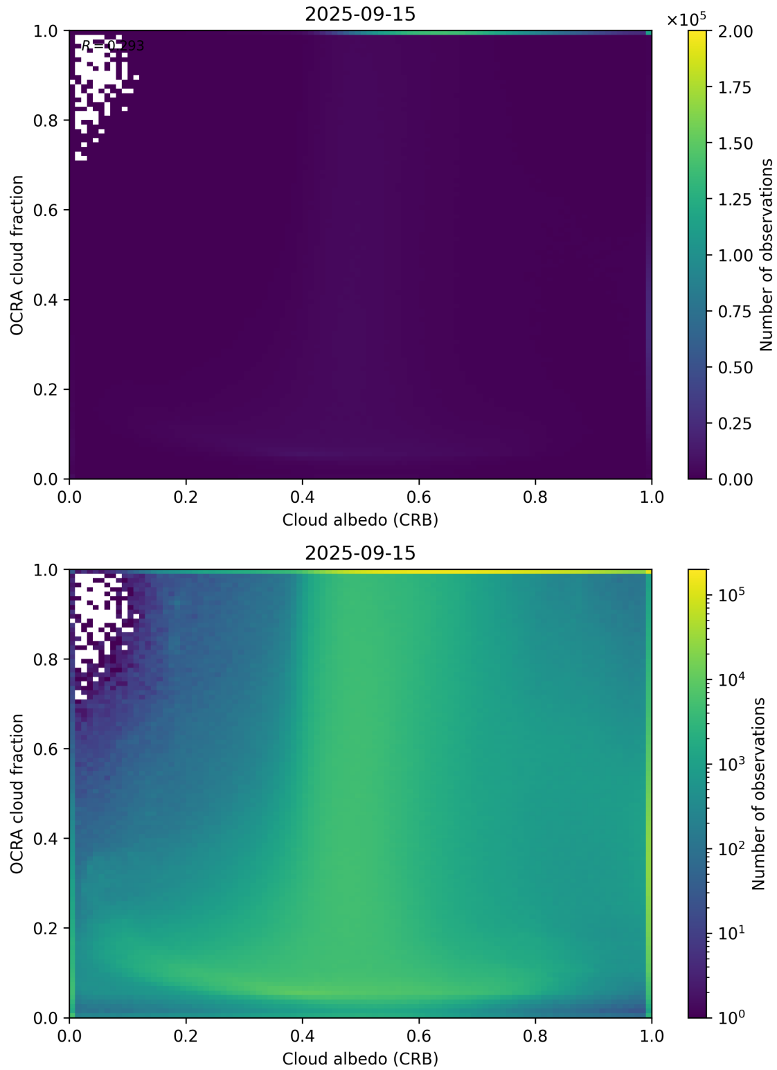
Figure 70: Scatter density plot of “Cloud albedo (CRB)” against “OCRA cloud fraction” for 2025-09-15 to 2025-09-16.
