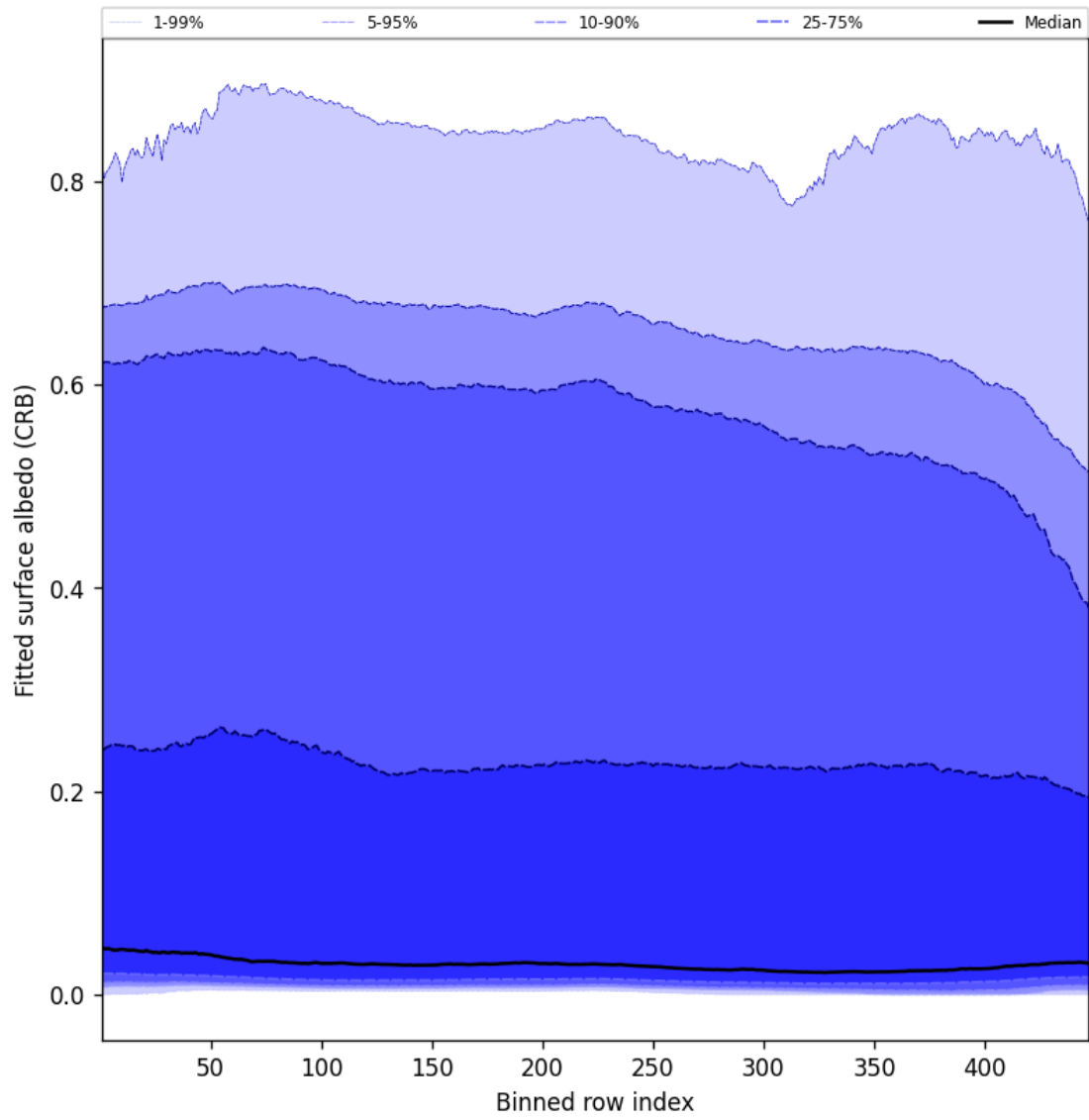
Figure 62: Along track statistics of “Fitted surface albedo (CRB)” for 2025-09-15 to 2025-09-16
