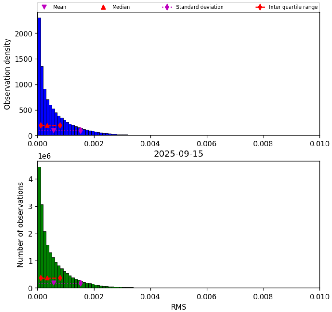
Figure 47: Histogram of “RMS” for 2025-09-15 to 2025-09-16
