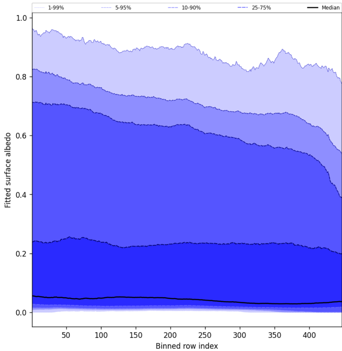
Figure 61: Along track statistics of “Fitted surface albedo” for 2025-09-15 to 2025-09-16
