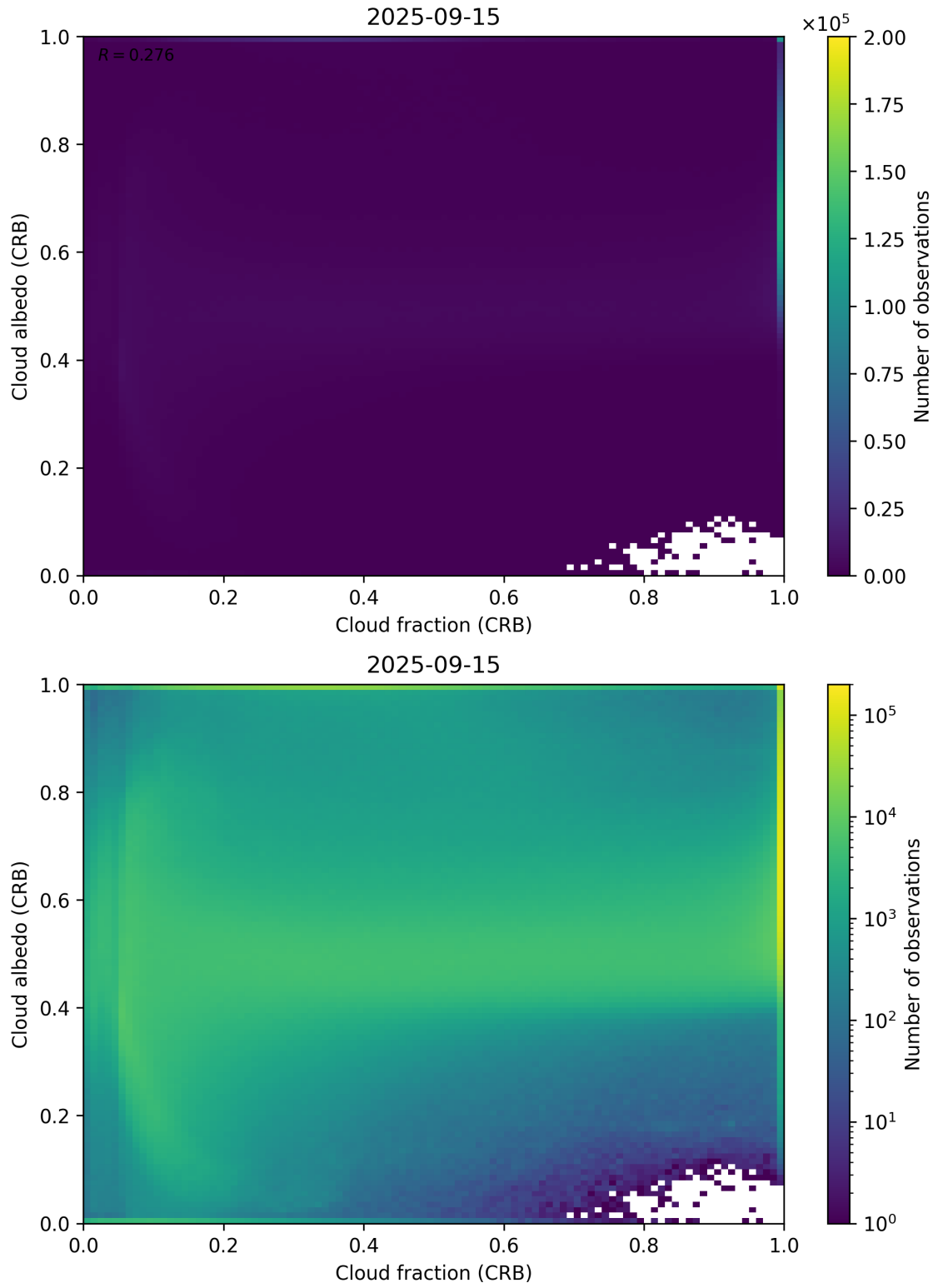
Figure 77: Scatter density plot of “Cloud fraction (CRB)” against “Cloud albedo (CRB)” for 2025-09-15 to 2025-09-16.
