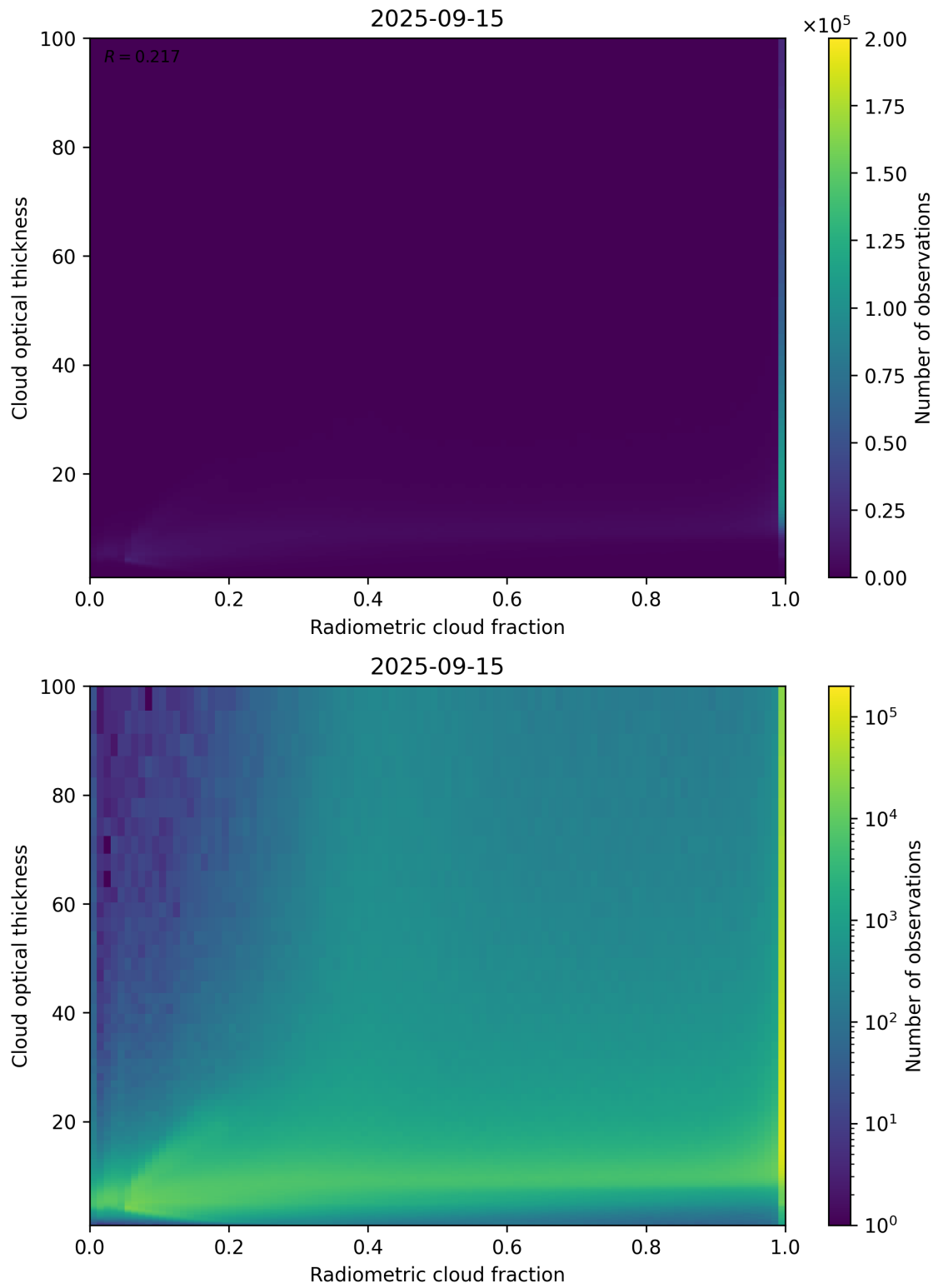
Figure 75: Scatter density plot of “Radiometric cloud fraction” against “Cloud optical thickness” for 2025-09-15 to 2025-09-16.
