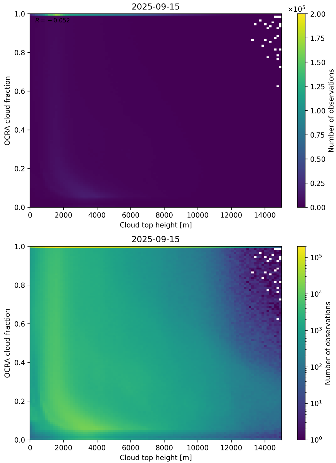
Figure 87: Scatter density plot of “Cloud top height” against “OCRA cloud fraction” for 2025-09-15 to 2025-09-16.
