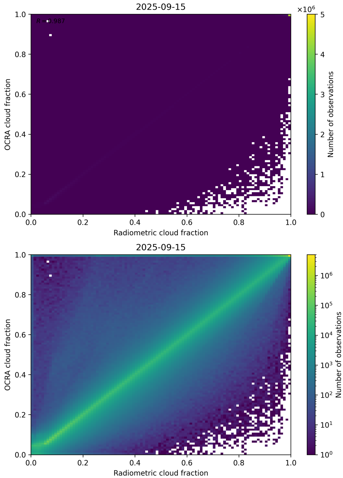
Figure 72: Scatter density plot of “Radiometric cloud fraction” against “OCRA cloud fraction” for 2025-09-15 to 2025-09-16.
