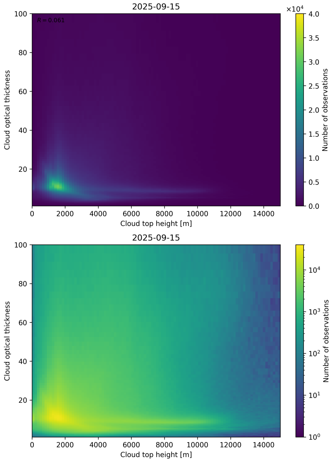
Figure 90: Scatter density plot of “Cloud top height” against “Cloud optical thickness” for 2025-09-15 to 2025-09-16.
