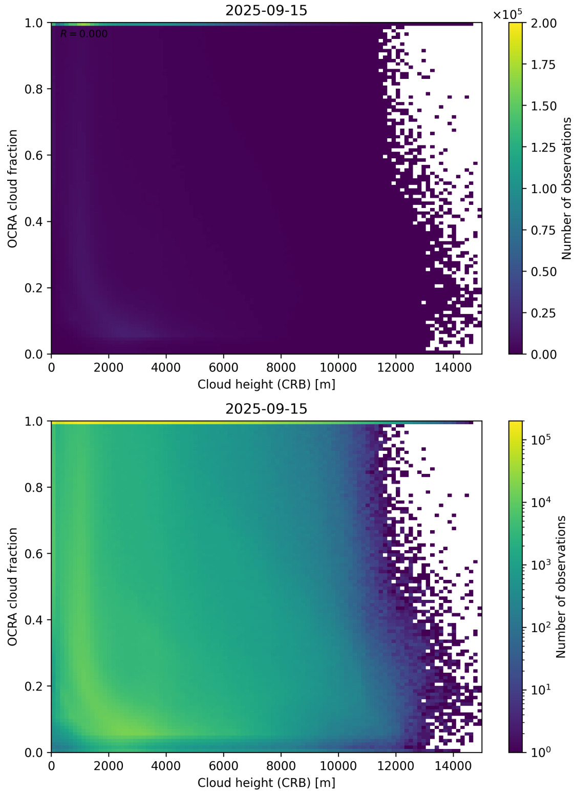
Figure 81: Scatter density plot of “Cloud height (CRB)” against “OCRA cloud fraction” for 2025-09-15 to 2025-09-16.
