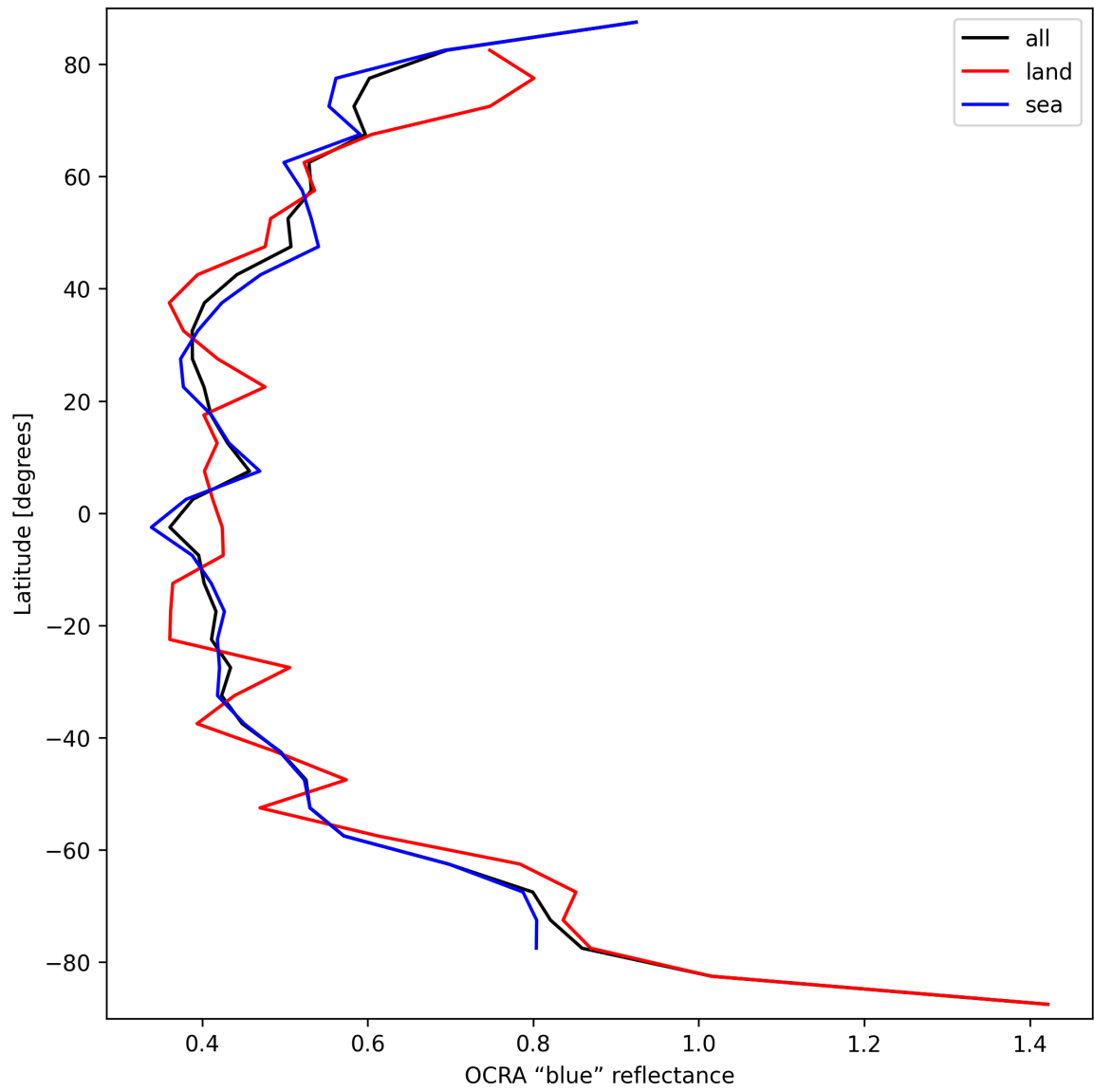
Figure 35: Zonal average of “OCRA “blue” reflectance” for 2025-09-15 to 2025-09-16.
