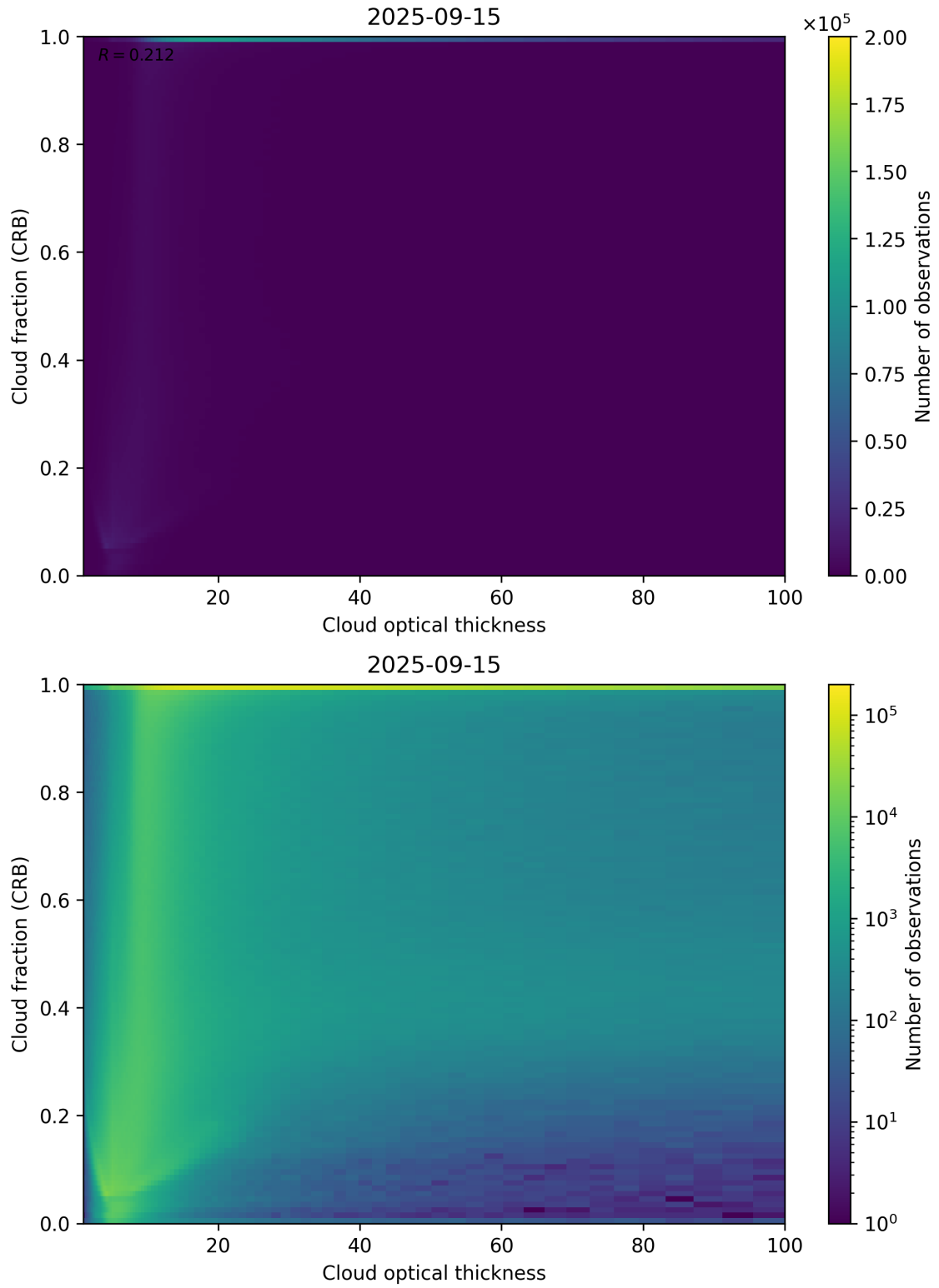
Figure 84: Scatter density plot of “Cloud optical thickness” against “Cloud fraction (CRB)” for 2025-09-15 to 2025-09-16.
