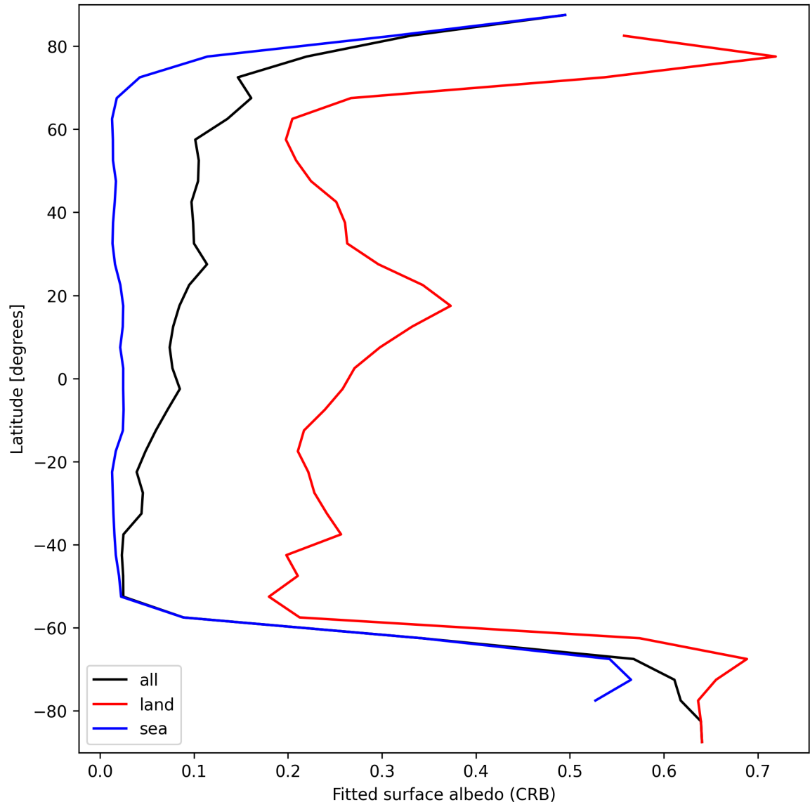
Figure 30: Zonal average of “Fitted surface albedo (CRB)” for 2025-09-15 to 2025-09-16.
