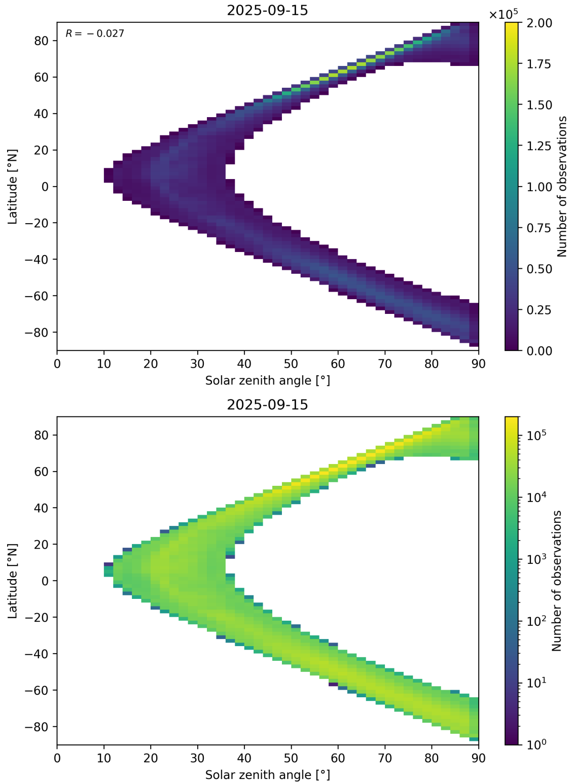
Figure 105: Scatter density plot of “Solar zenith angle” against “Latitude” for 2025-09-15 to 2025-09-16.
