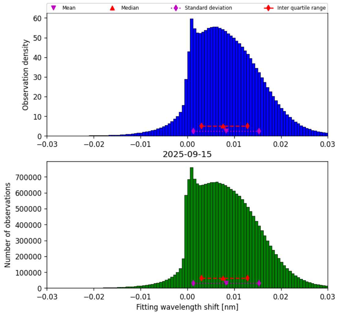
Figure 49: Histogram of “Fitting wavelength shift” for 2025-09-15 to 2025-09-16
