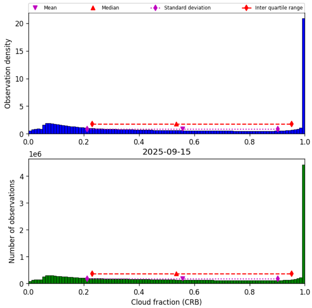
Figure 42: Histogram of “Cloud fraction (CRB)” for 2025-09-15 to 2025-09-16
