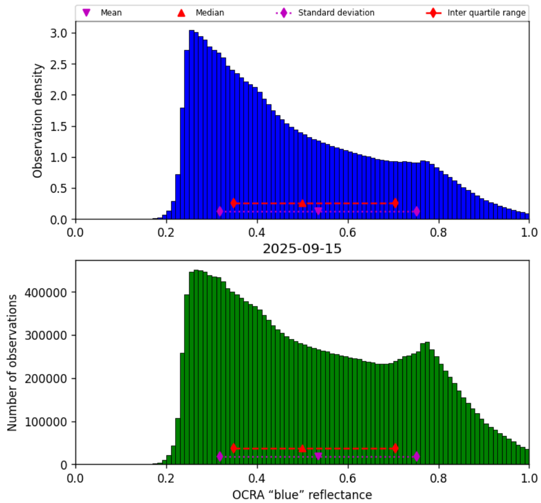
Figure 51: Histogram of “OCRA “blue” reflectance” for 2025-09-15 to 2025-09-16
