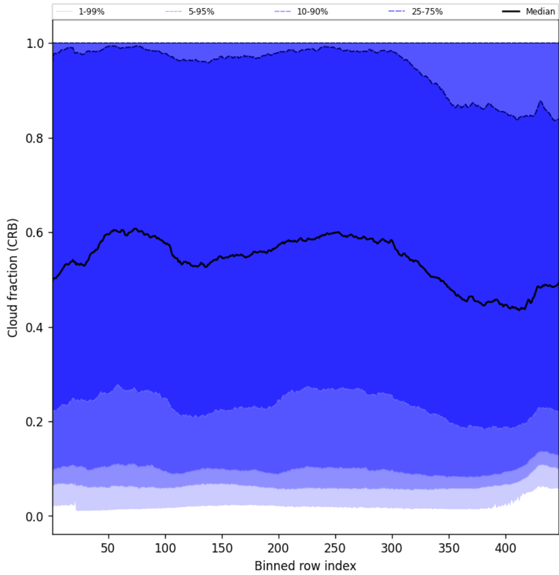
Figure 58: Along track statistics of “Cloud fraction (CRB)” for 2025-09-15 to 2025-09-16
