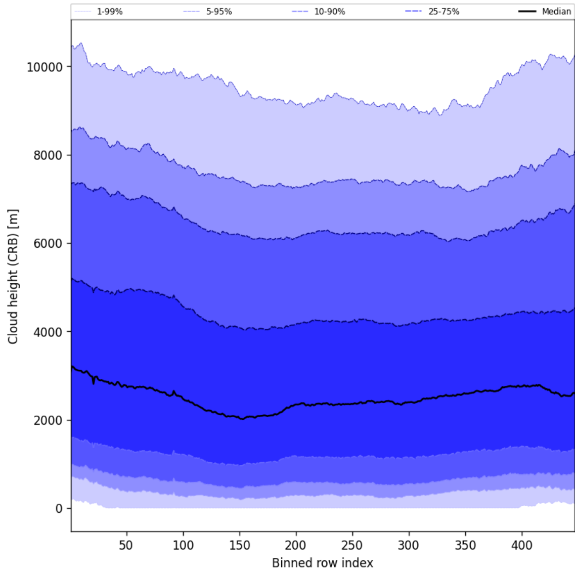
Figure 59: Along track statistics of “Cloud height (CRB)” for 2025-09-15 to 2025-09-16
