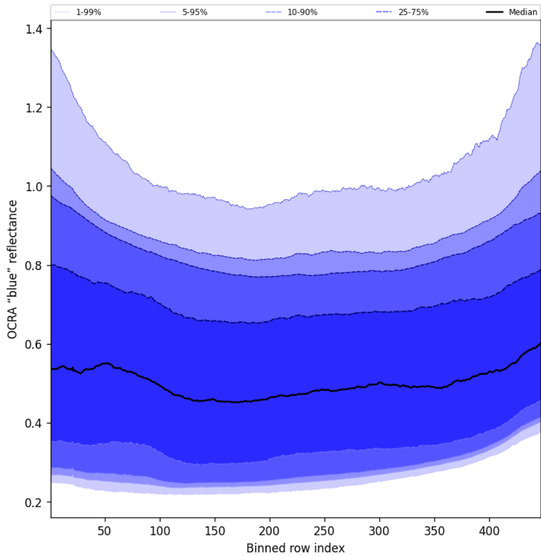
Figure 67: Along track statistics of “OCRA “blue” reflectance” for 2025-09-15 to 2025-09-16
