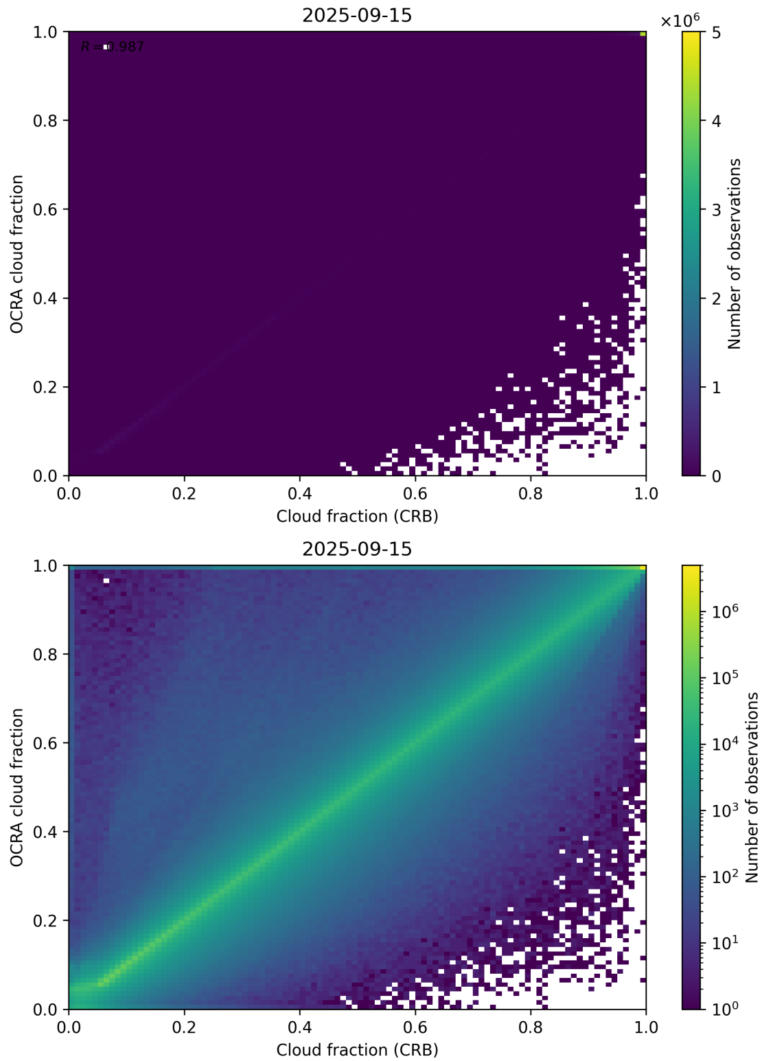
Figure 78: Scatter density plot of “Cloud fraction (CRB)” against “OCRA cloud fraction” for 2025-09-15 to 2025-09-16.
