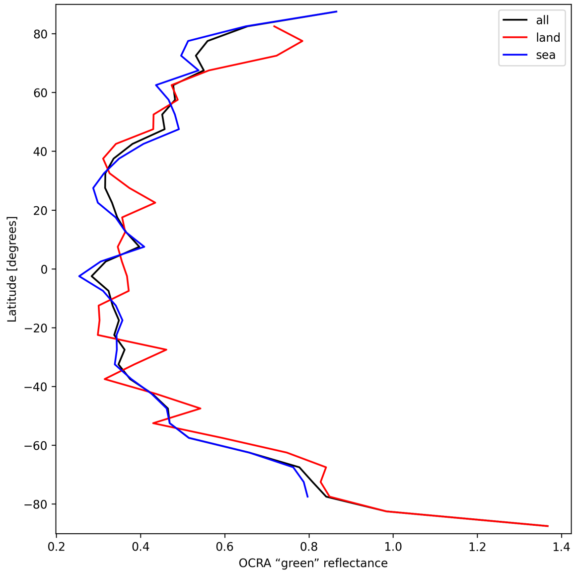
Figure 36: Zonal average of “OCRA “green” reflectance” for 2025-09-15 to 2025-09-16.
