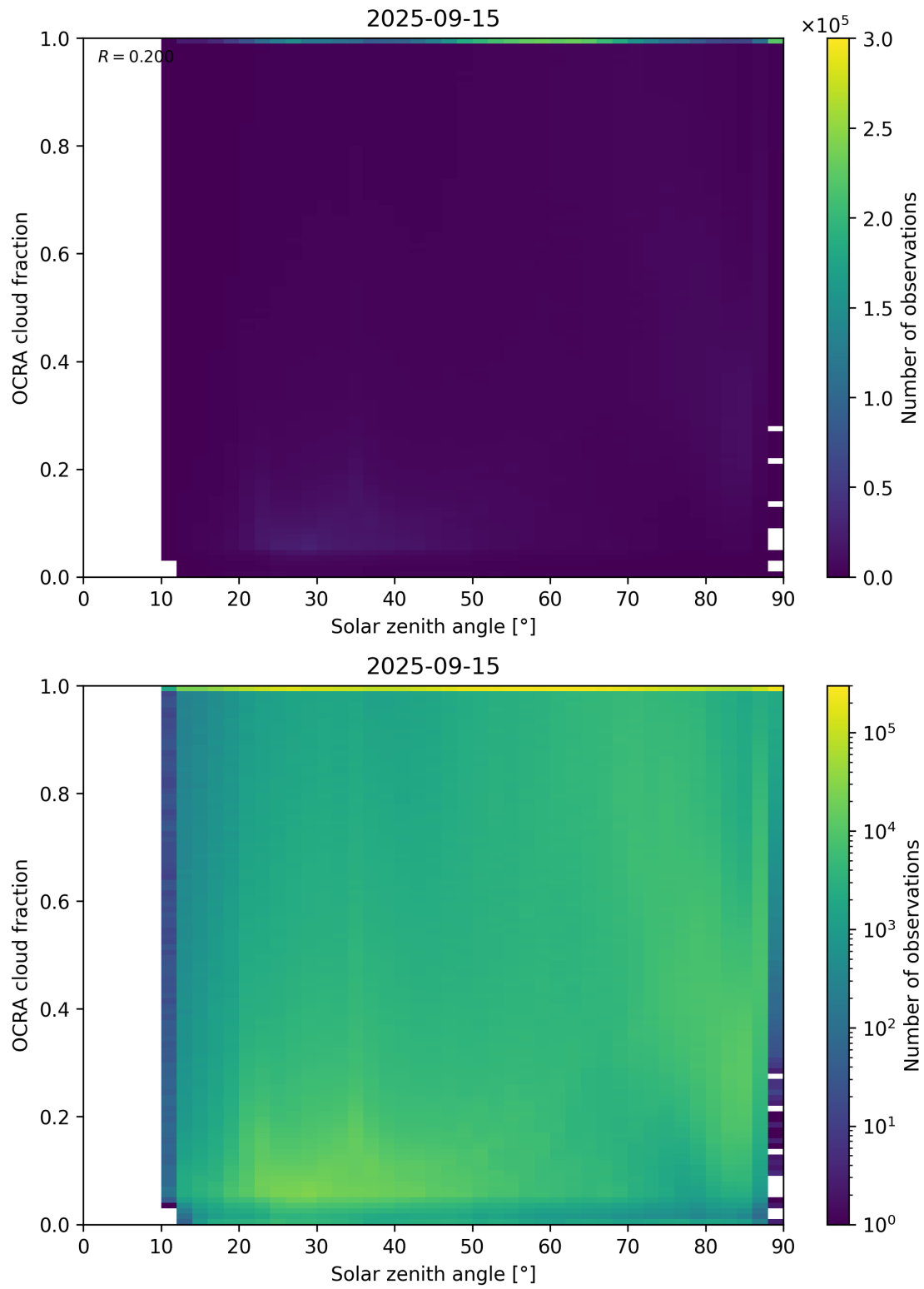
Figure 100: Scatter density plot of “Solar zenith angle” against “OCRA cloud fraction” for 2025-09-15 to 2025-09-16.
