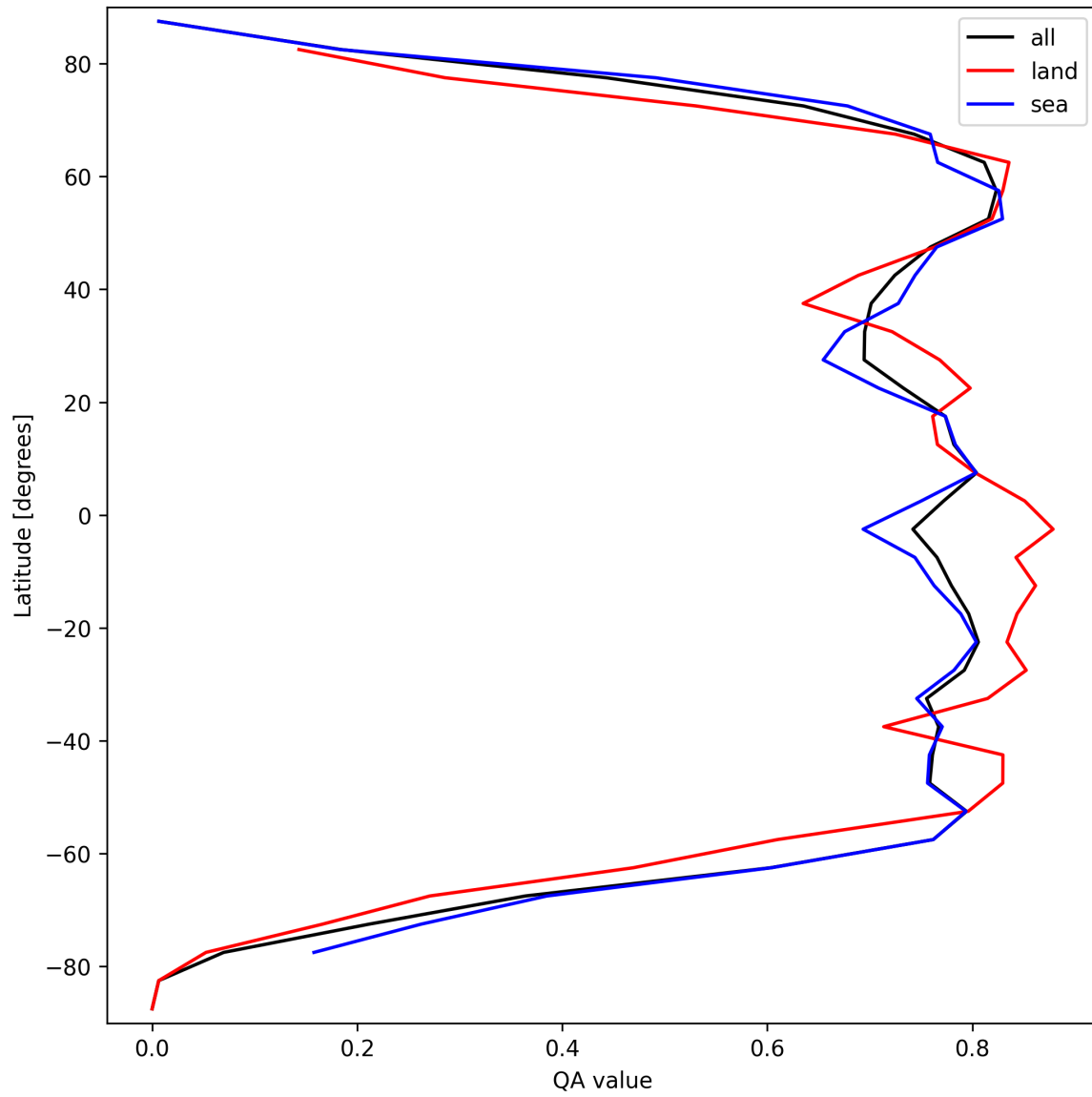
Figure 22: Zonal average of “QA value” for 2025-09-15 to 2025-09-16.
