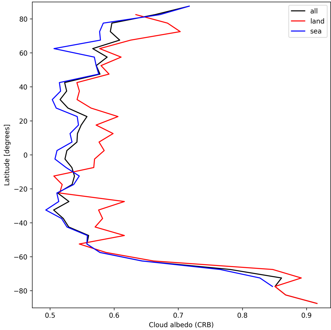
Figure 28: Zonal average of “Cloud albedo (CRB)” for 2025-09-15 to 2025-09-16.
