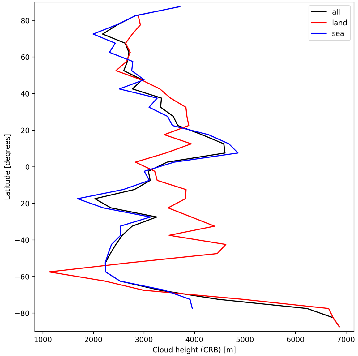
Figure 27: Zonal average of “Cloud height (CRB)” for 2025-09-15 to 2025-09-16.
