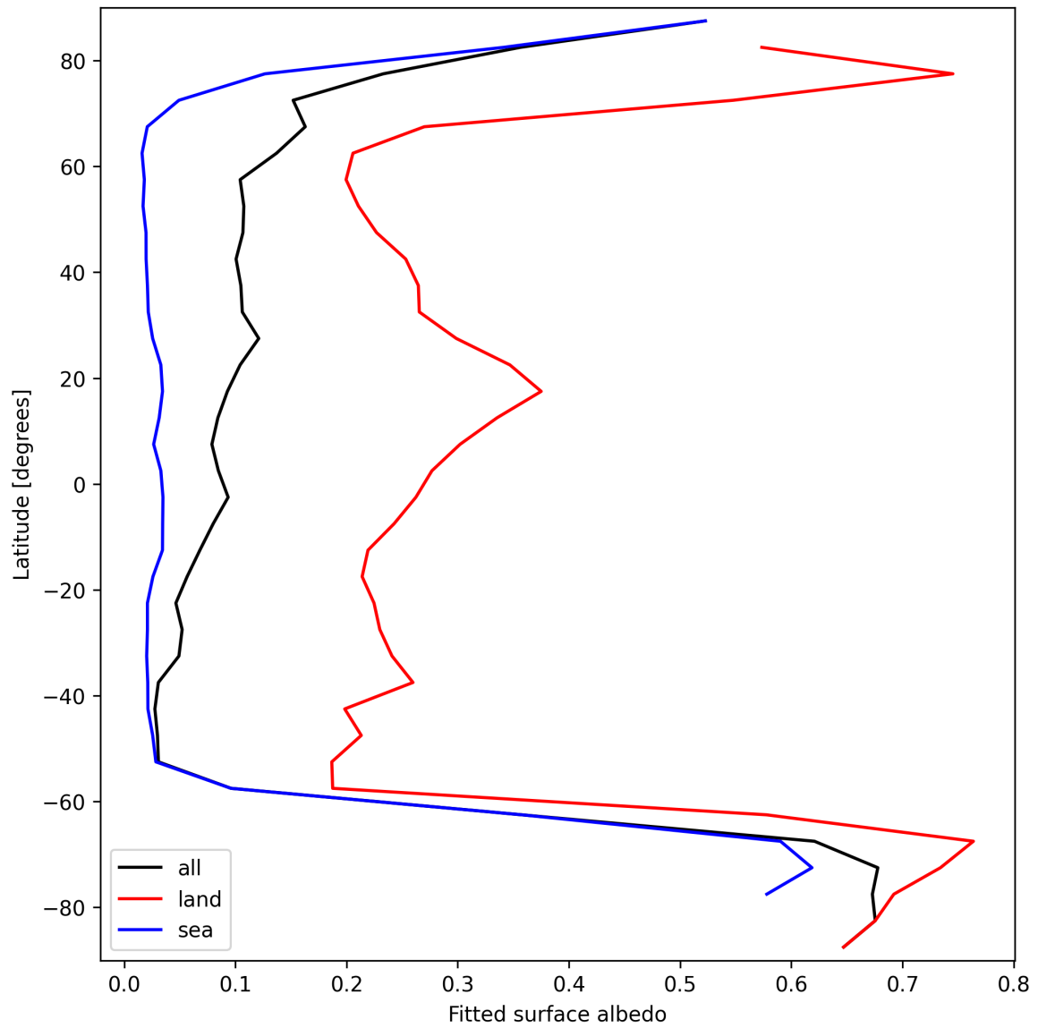
Figure 29: Zonal average of “Fitted surface albedo” for 2025-09-15 to 2025-09-16.
