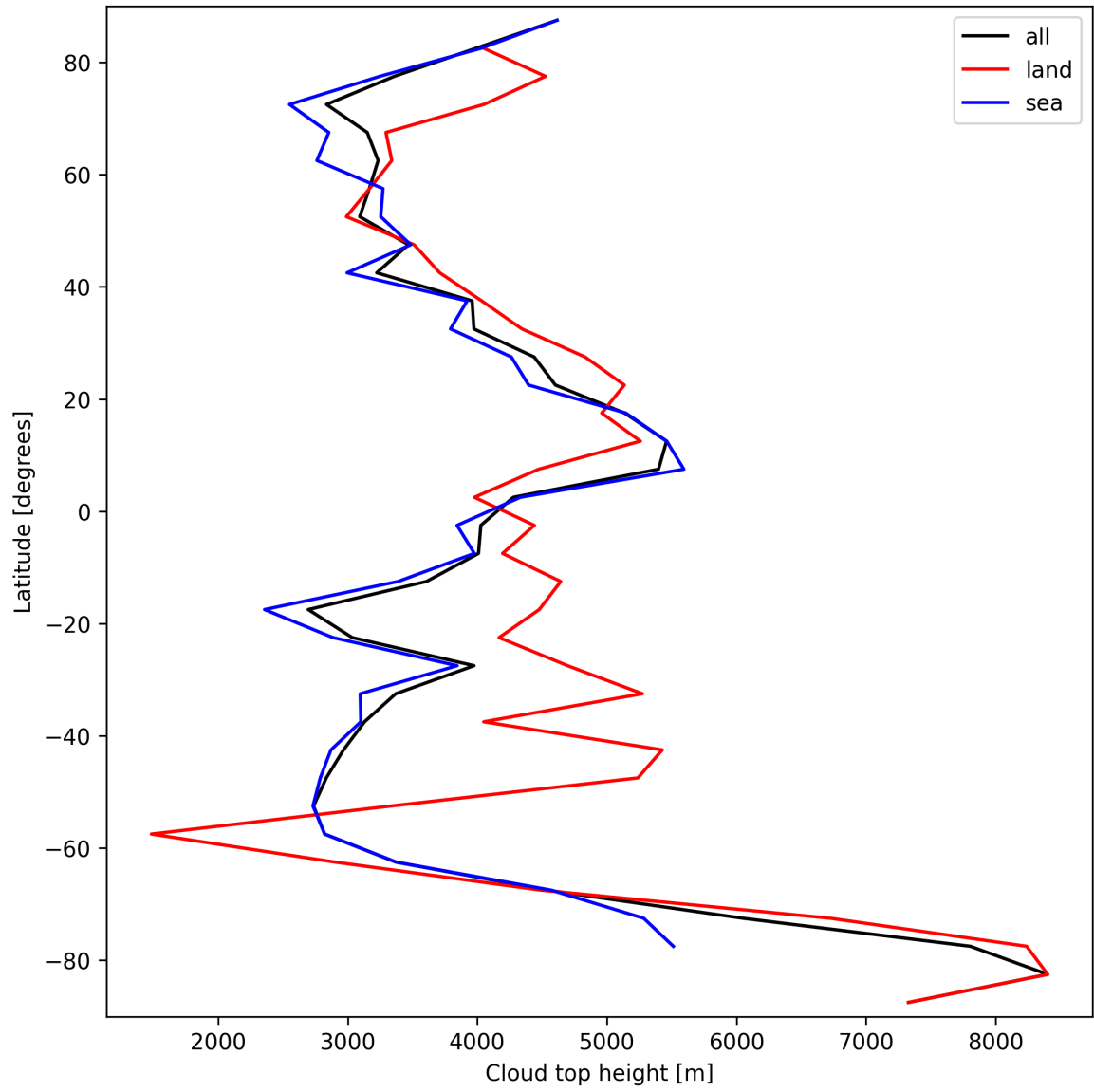
Figure 24: Zonal average of “Cloud top height” for 2025-09-15 to 2025-09-16.
