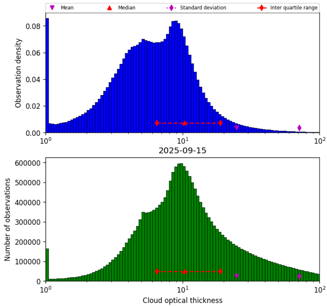
Figure 41: Histogram of “Cloud optical thickness” for 2025-09-15 to 2025-09-16
