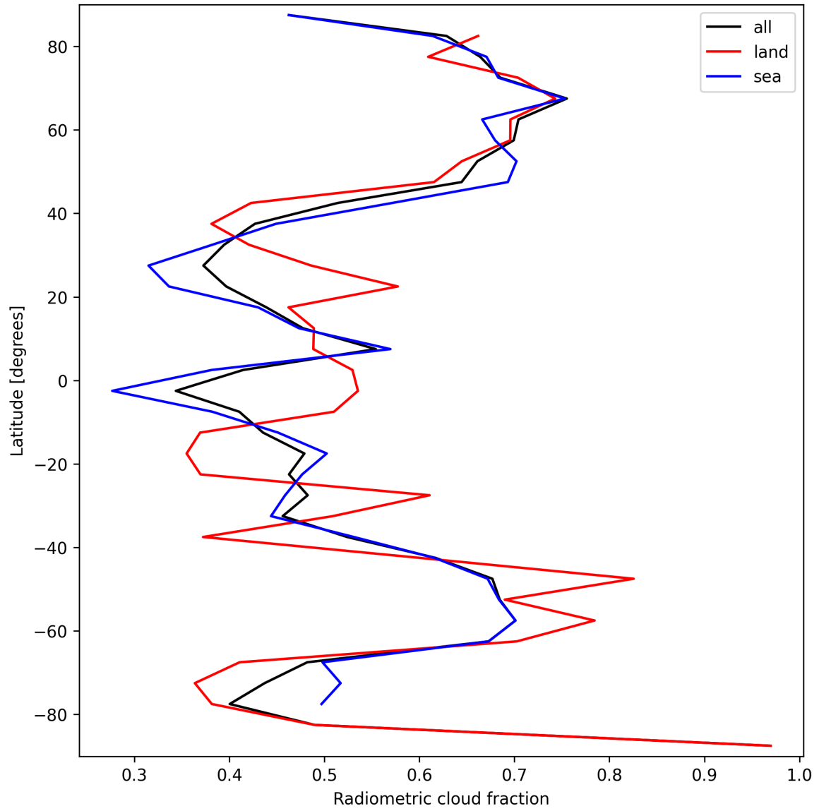
Figure 23: Zonal average of “Radiometric cloud fraction” for 2025-09-15 to 2025-09-16.
