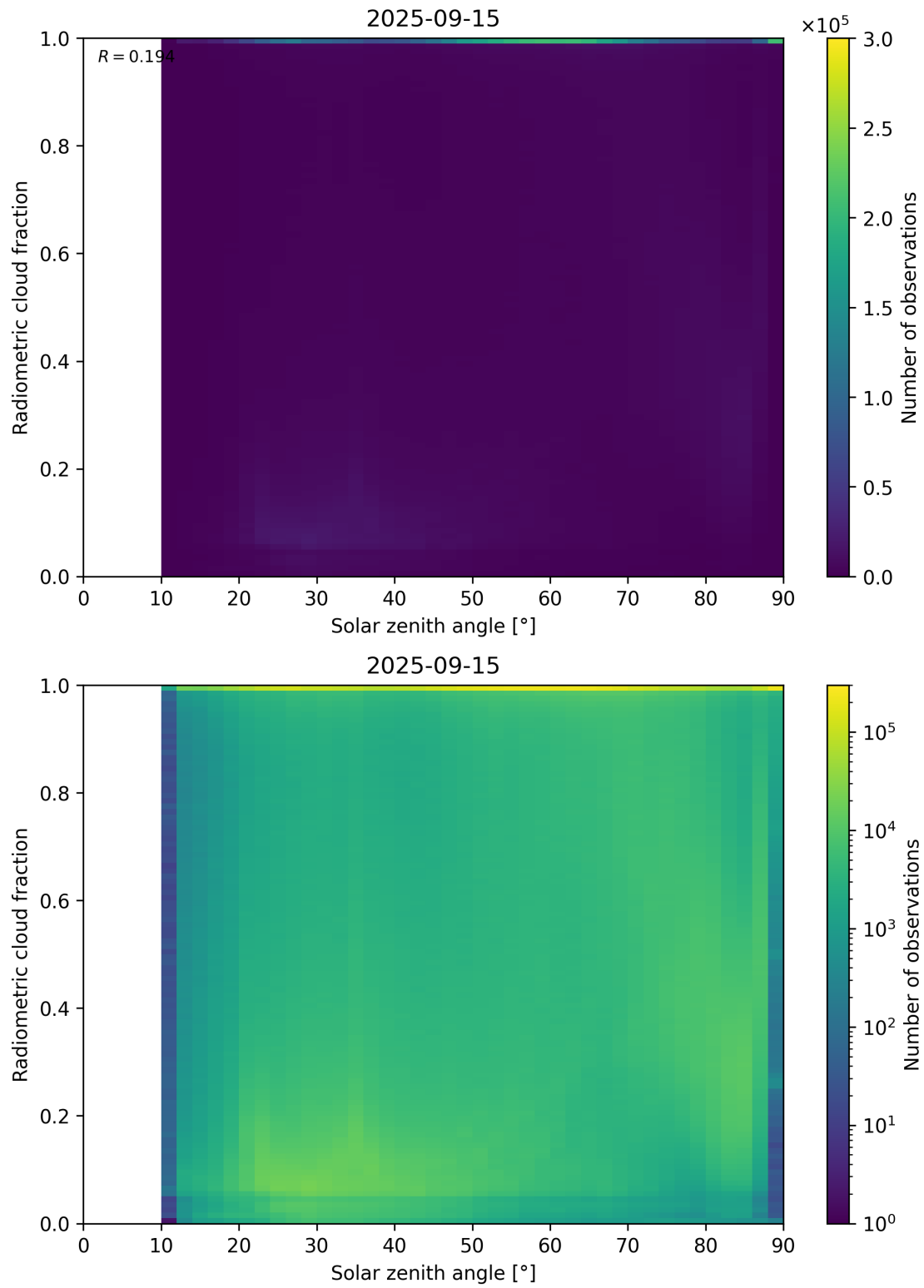
Figure 99: Scatter density plot of “Solar zenith angle” against “Radiometric cloud fraction” for 2025-09-15 to 2025-09-16.
