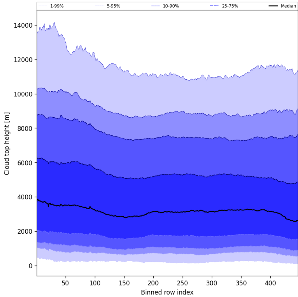
Figure 56: Along track statistics of “Cloud top height” for 2025-09-15 to 2025-09-16
