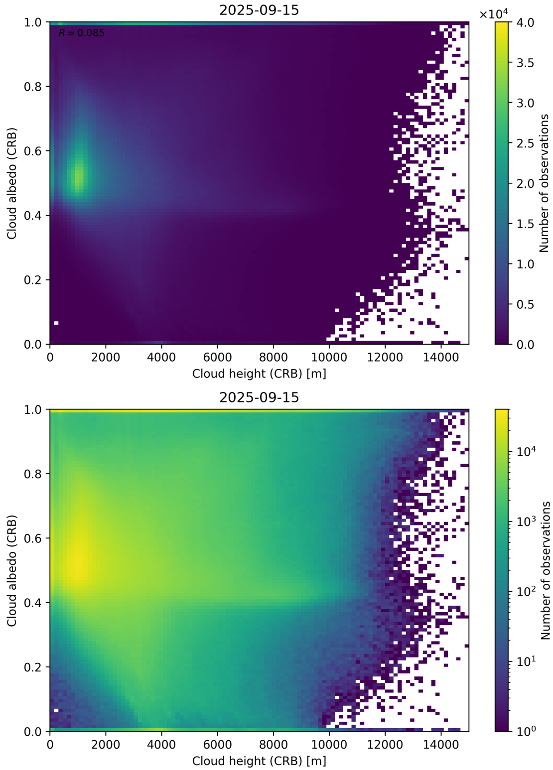
Figure 80: Scatter density plot of “Cloud height (CRB)” against “Cloud albedo (CRB)” for 2025-09-15 to 2025-09-16.
