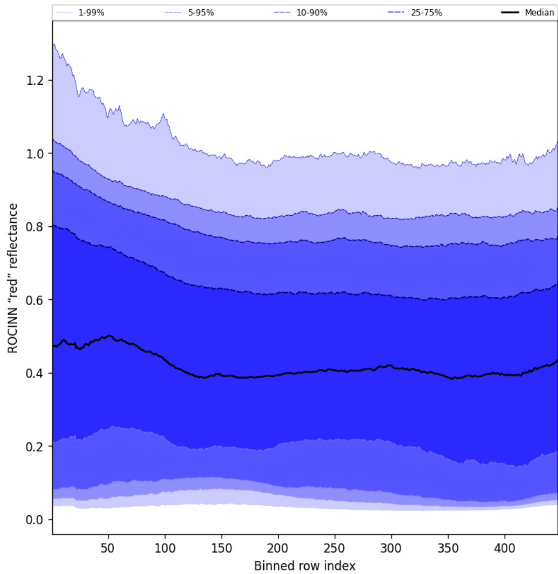
Figure 69: Along track statistics of “ROCINN “red” reflectance” for 2025-09-15 to 2025-09-16
