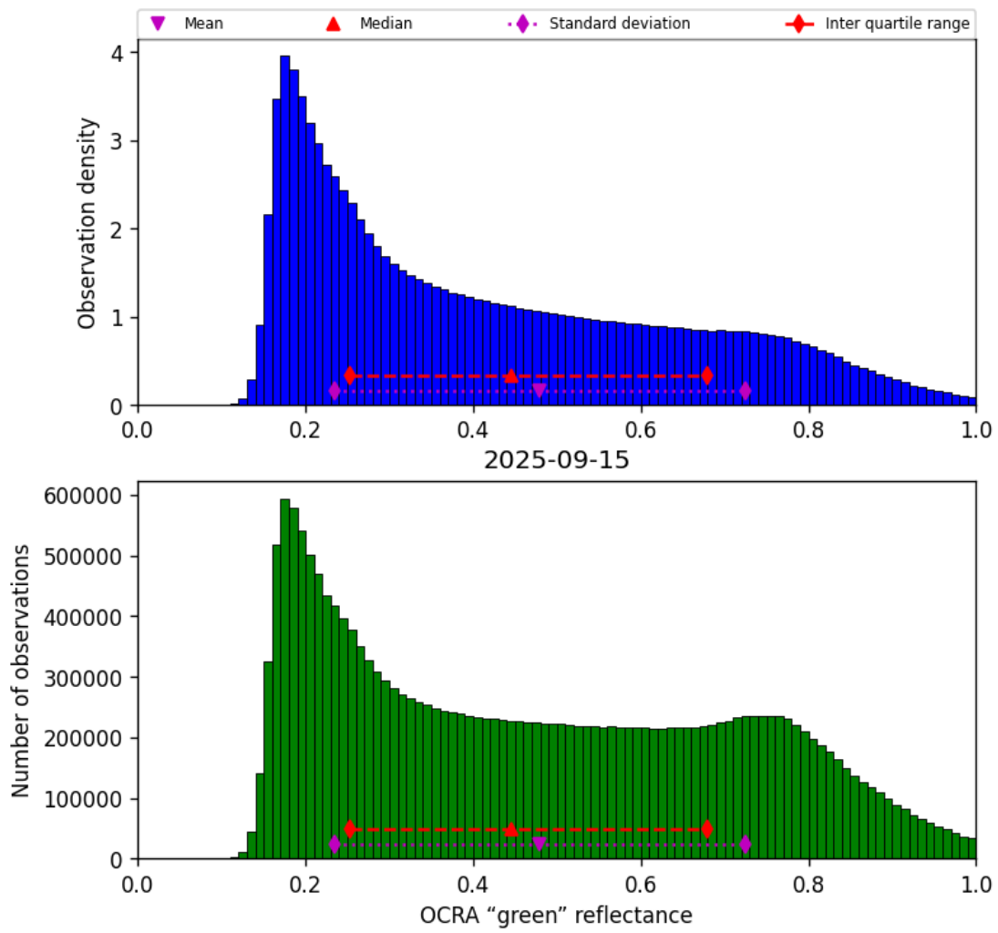
Figure 52: Histogram of “OCRA “green” reflectance” for 2025-09-15 to 2025-09-16
