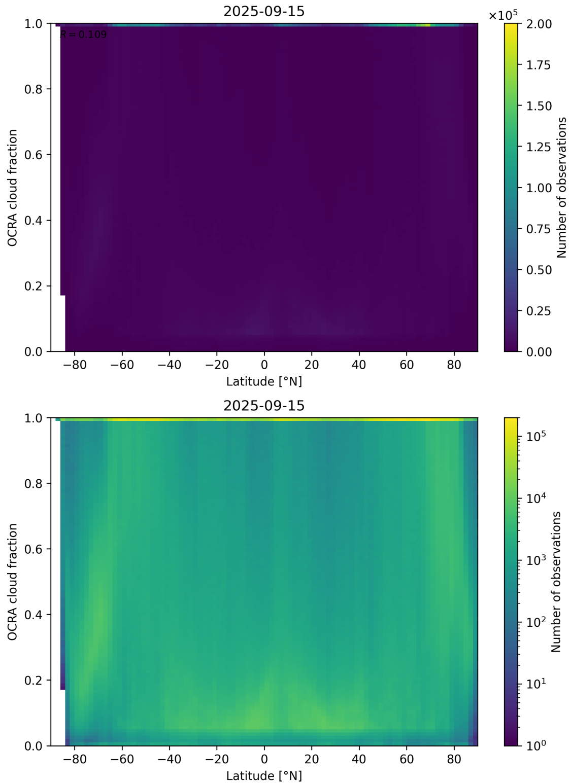
Figure 93: Scatter density plot of “Latitude” against “OCRA cloud fraction” for 2025-09-15 to 2025-09-16.
