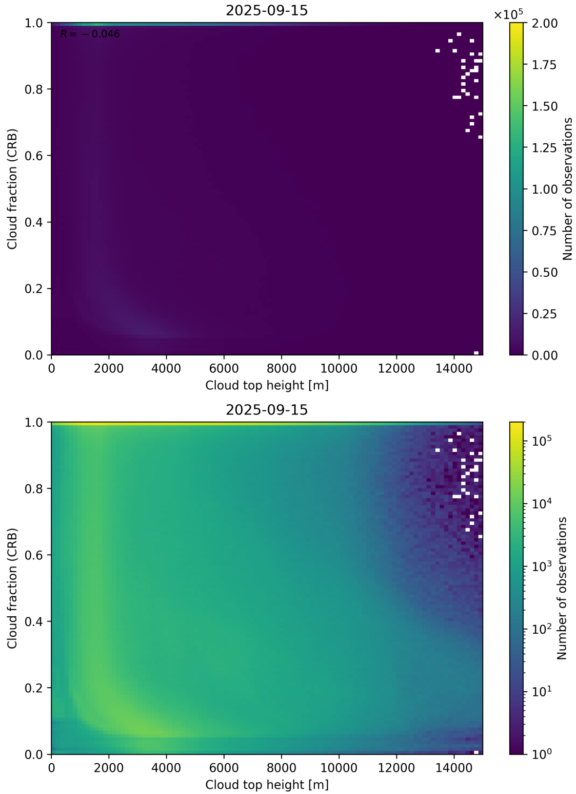
Figure 88: Scatter density plot of “Cloud top height” against “Cloud fraction (CRB)” for 2025-09-15 to 2025-09-16.
