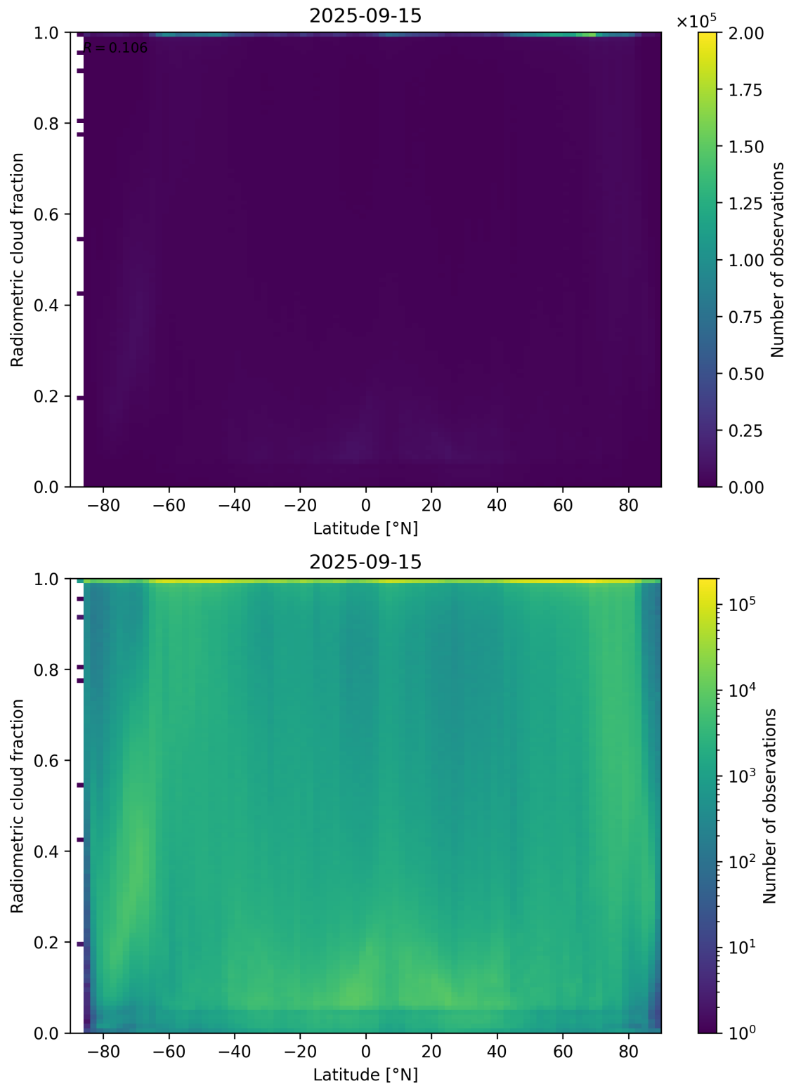
Figure 92: Scatter density plot of “Latitude” against “Radiometric cloud fraction” for 2025-09-15 to 2025-09-16.
