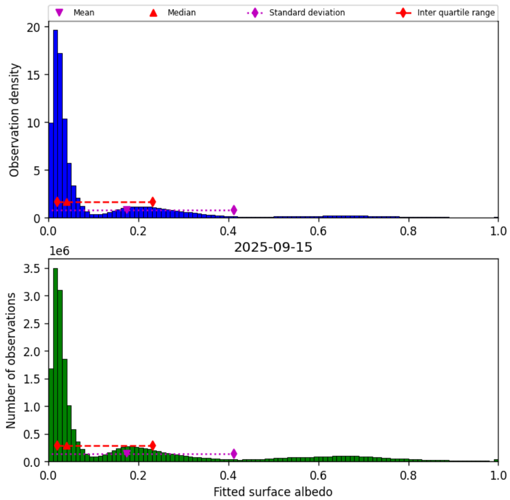
Figure 45: Histogram of “Fitted surface albedo” for 2025-09-15 to 2025-09-16
