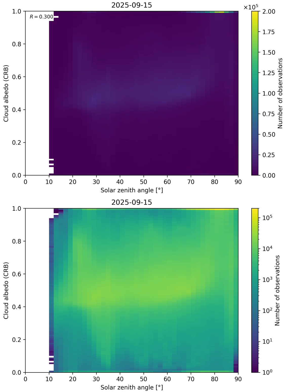
Figure 98: Scatter density plot of “Solar zenith angle” against “Cloud albedo (CRB)” for 2025-09-15 to 2025-09-16.
