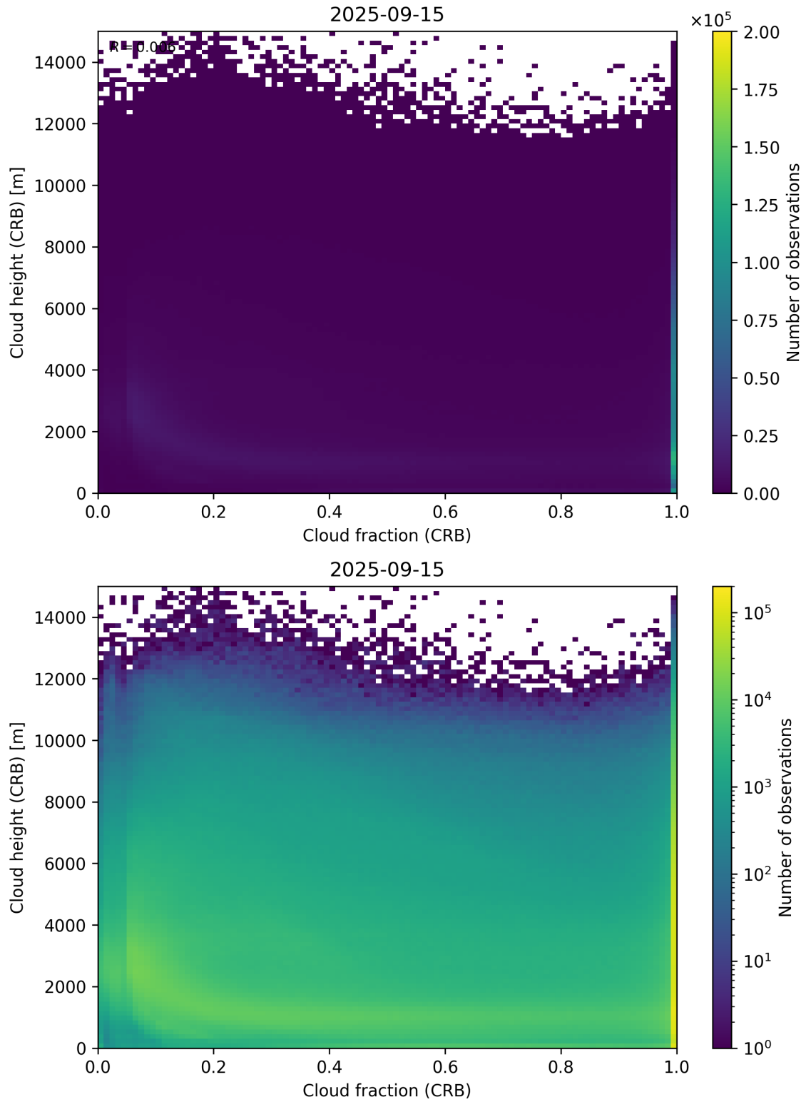
Figure 79: Scatter density plot of “Cloud fraction (CRB)” against “Cloud height (CRB)” for 2025-09-15 to 2025-09-16.
