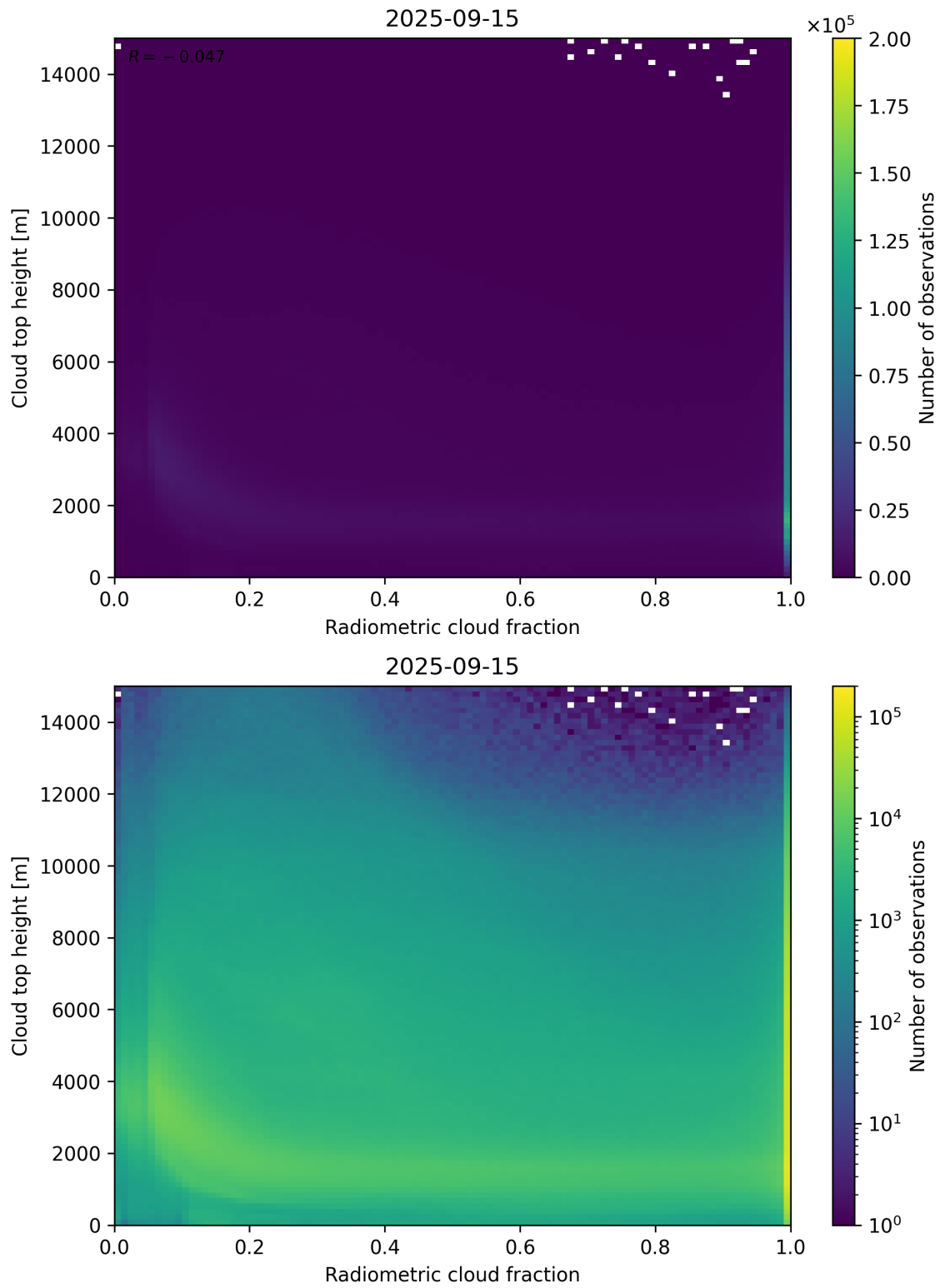
Figure 76: Scatter density plot of “Radiometric cloud fraction” against “Cloud top height” for 2025-09-15 to 2025-09-16.
