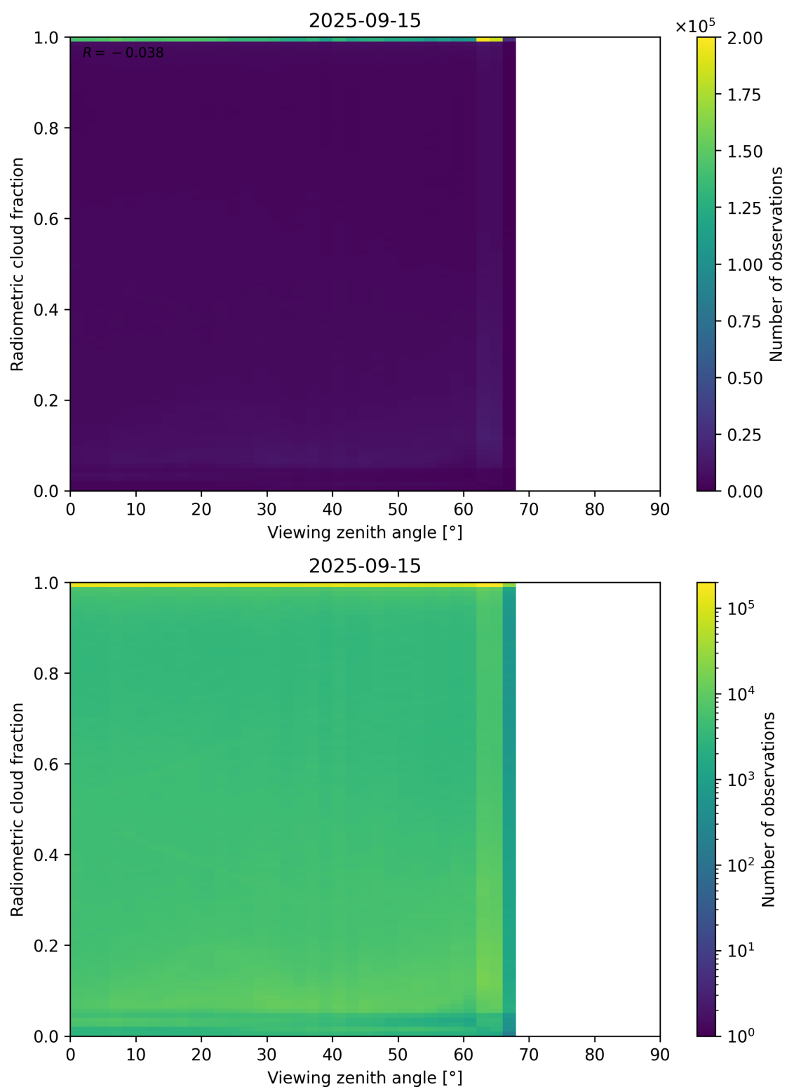
Figure 107: Scatter density plot of “Viewing zenith angle” against “Radiometric cloud fraction” for 2025-09-15 to 2025-09-16.
