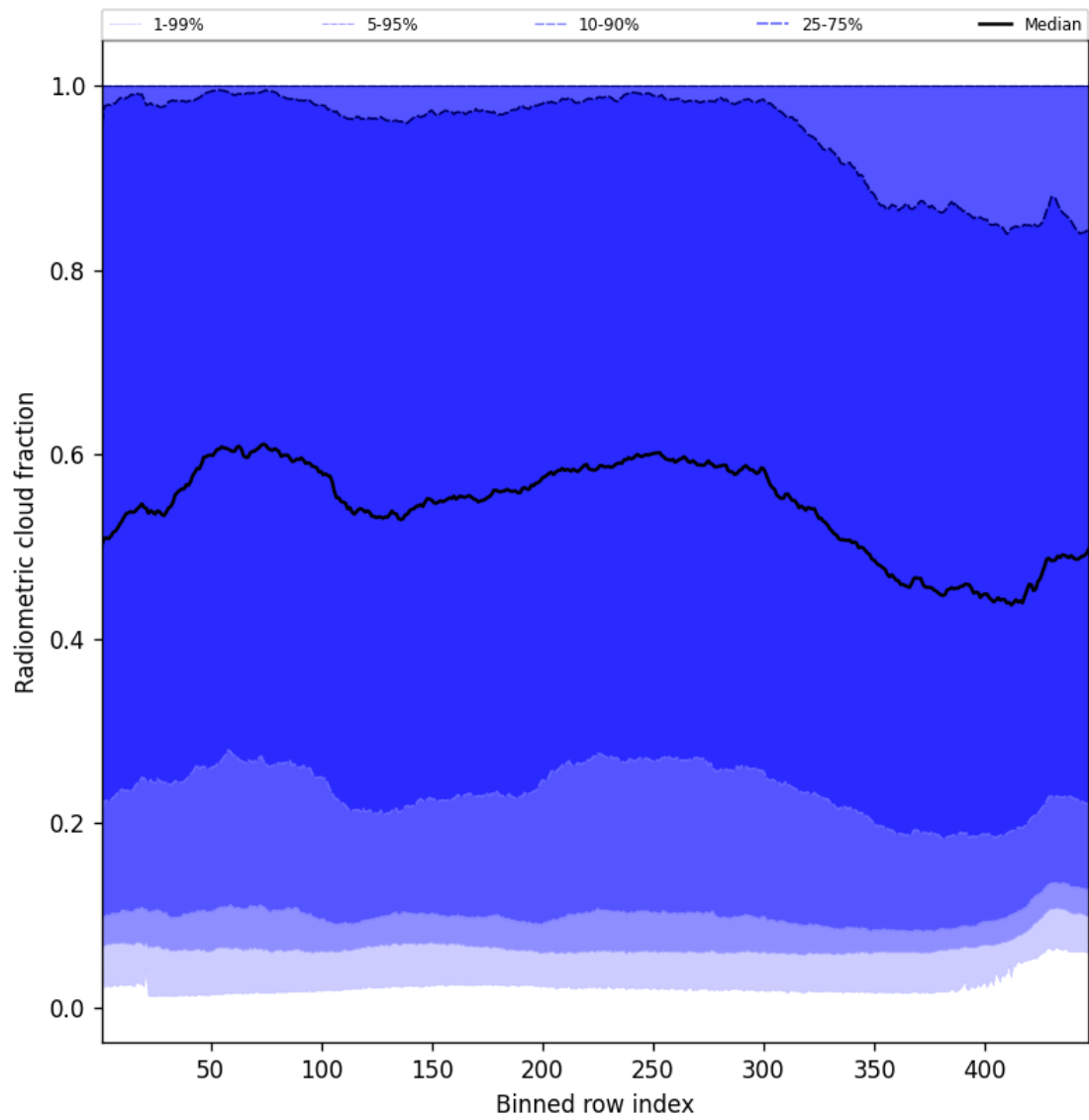
Figure 55: Along track statistics of “Radiometric cloud fraction” for 2025-09-15 to 2025-09-16
