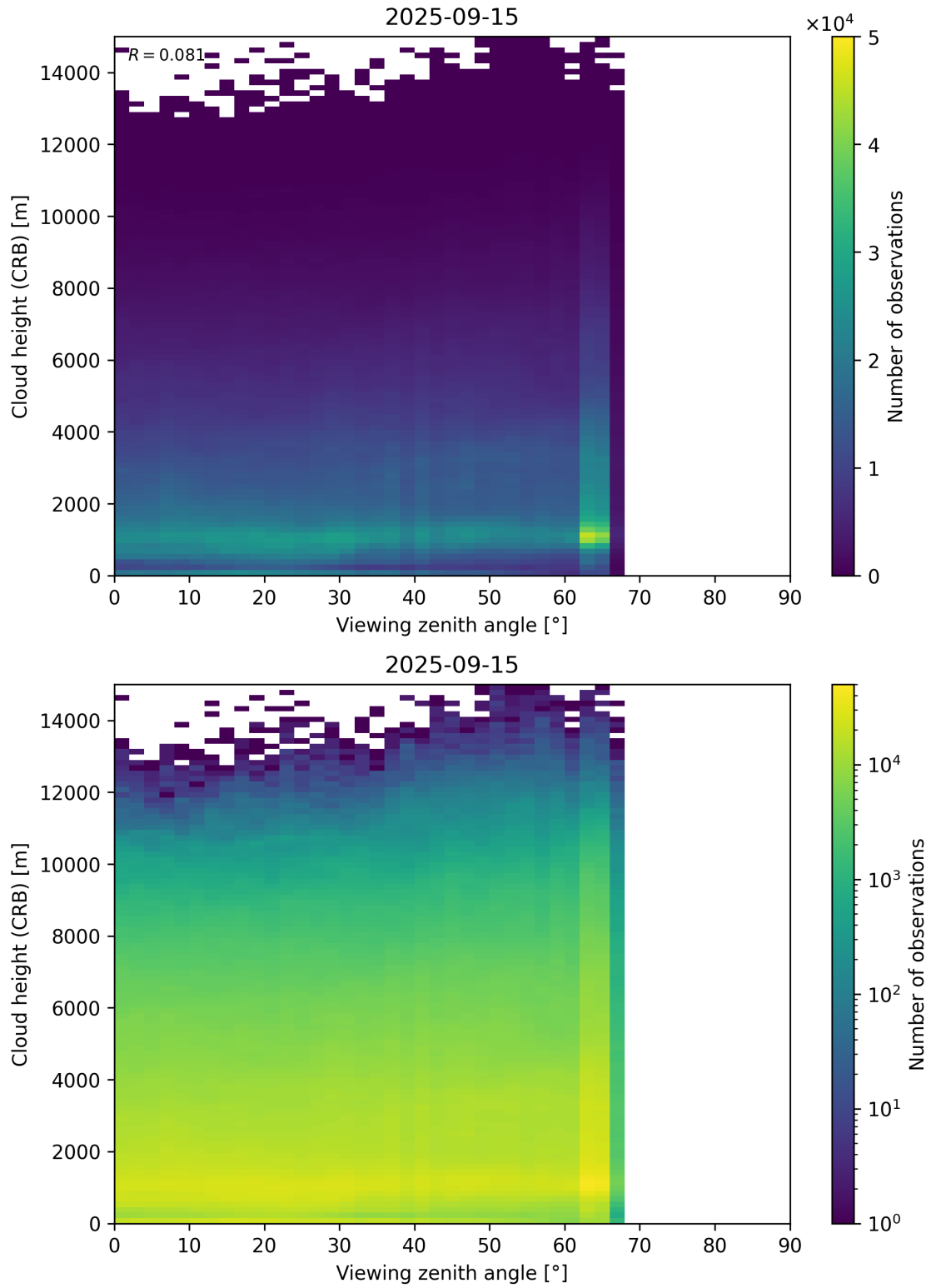
Figure 110: Scatter density plot of “Viewing zenith angle” against “Cloud height (CRB)” for 2025-09-15 to 2025-09-16.
