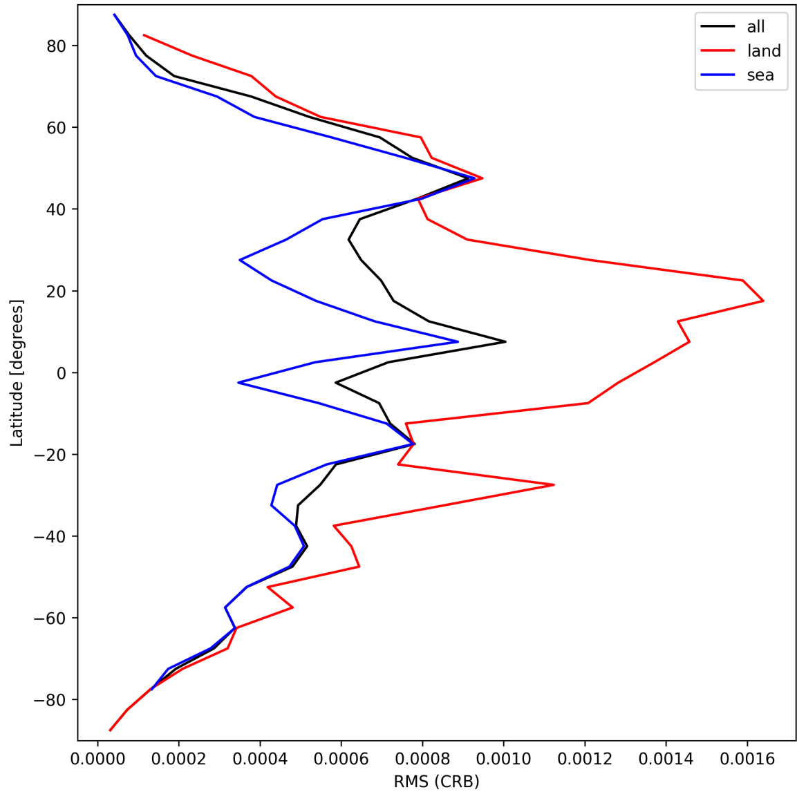
Figure 32: Zonal average of “RMS (CRB)” for 2025-09-15 to 2025-09-16.
