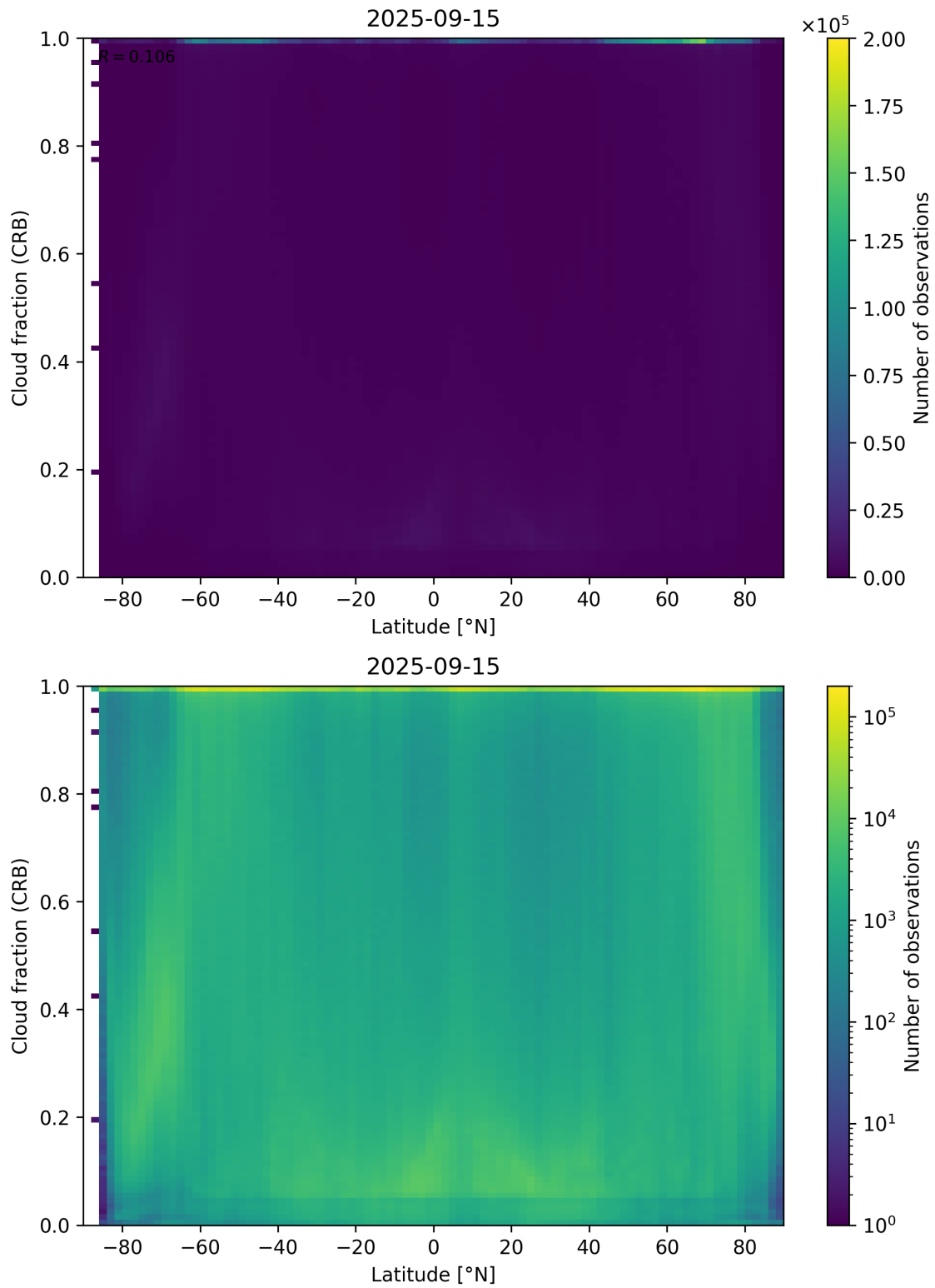
Figure 94: Scatter density plot of “Latitude” against “Cloud fraction (CRB)” for 2025-09-15 to 2025-09-16.
