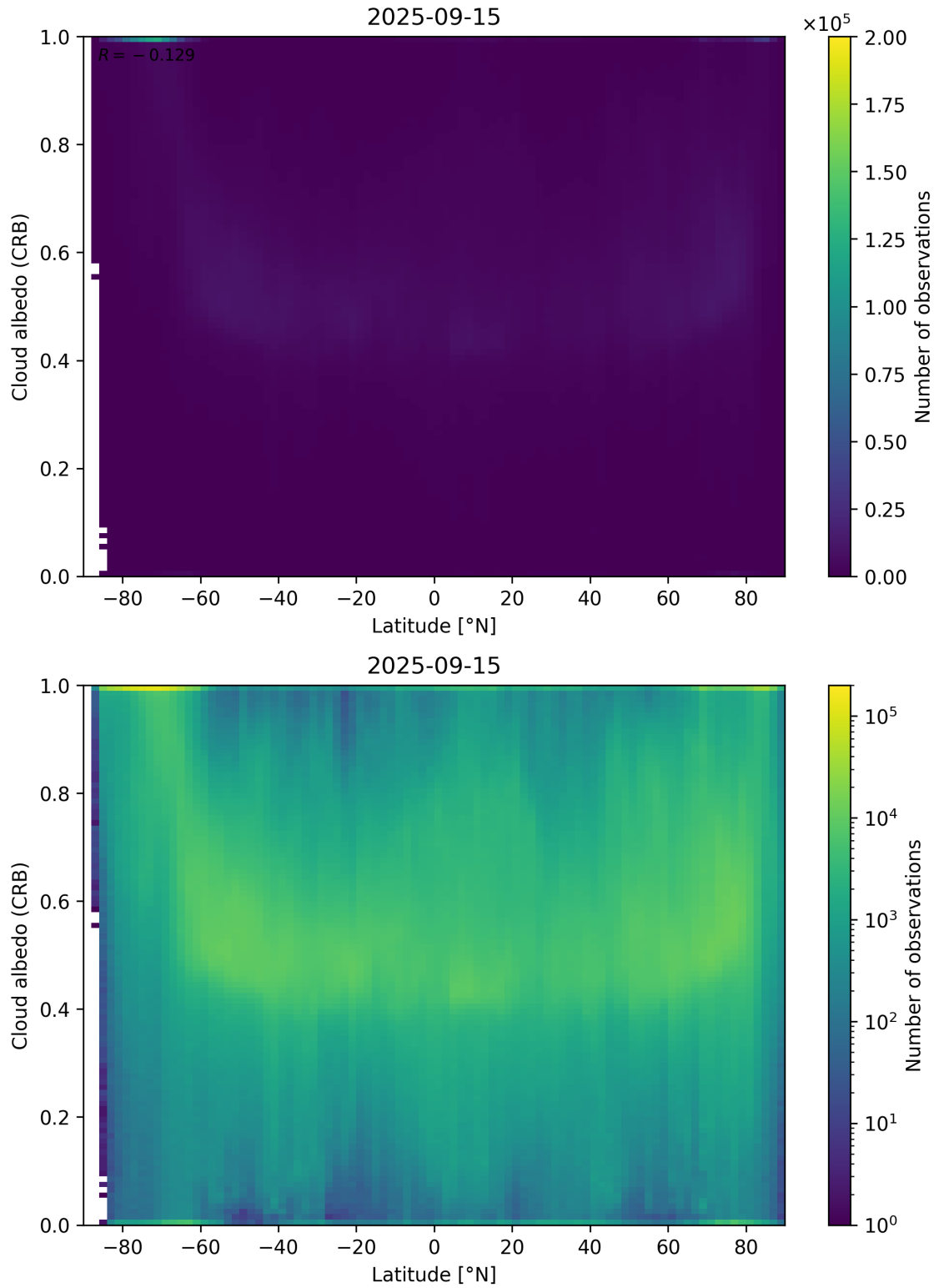
Figure 91: Scatter density plot of “Latitude” against “Cloud albedo (CRB)” for 2025-09-15 to 2025-09-16.
