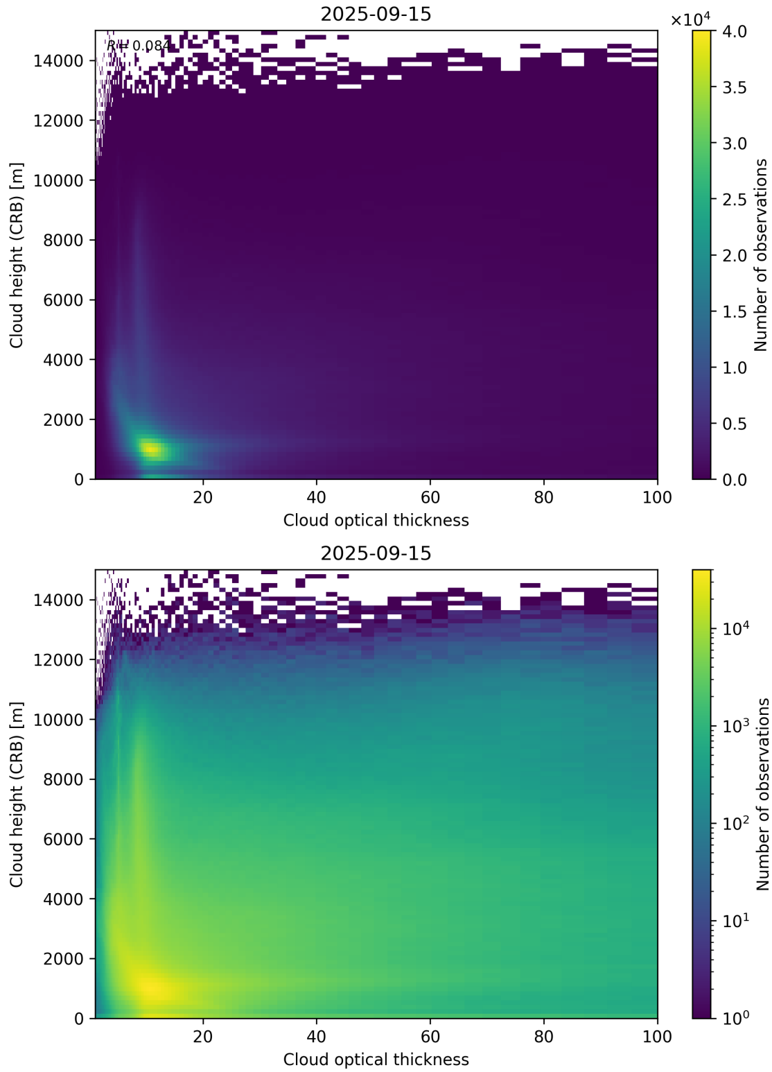
Figure 85: Scatter density plot of “Cloud optical thickness” against “Cloud height (CRB)” for 2025-09-15 to 2025-09-16.
