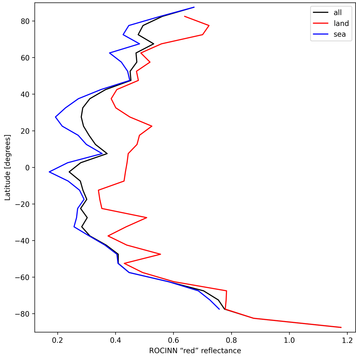
Figure 37: Zonal average of “ROCINN “red” reflectance” for 2025-09-15 to 2025-09-16.
