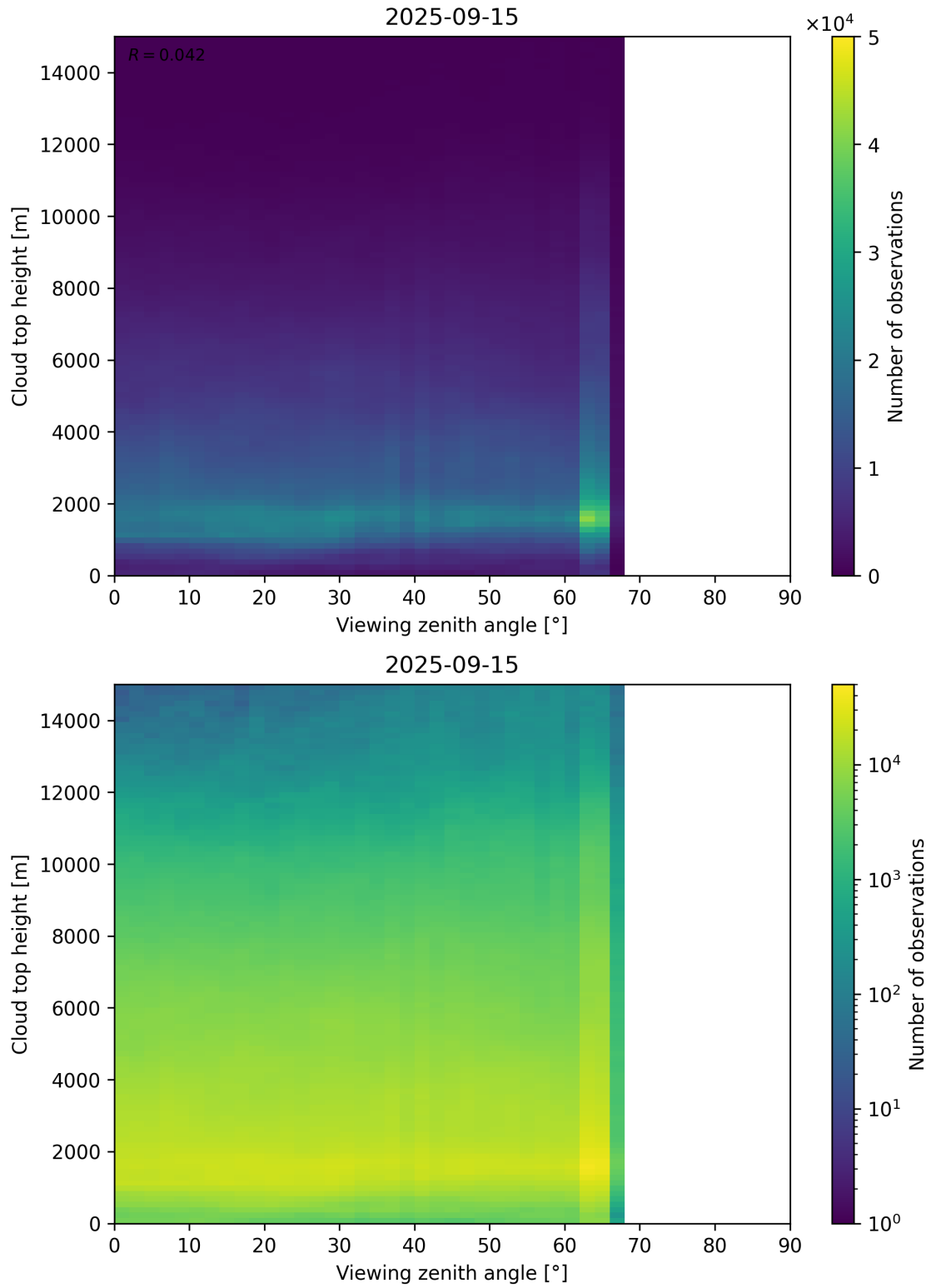
Figure 112: Scatter density plot of “Viewing zenith angle” against “Cloud top height” for 2025-09-15 to 2025-09-16.
