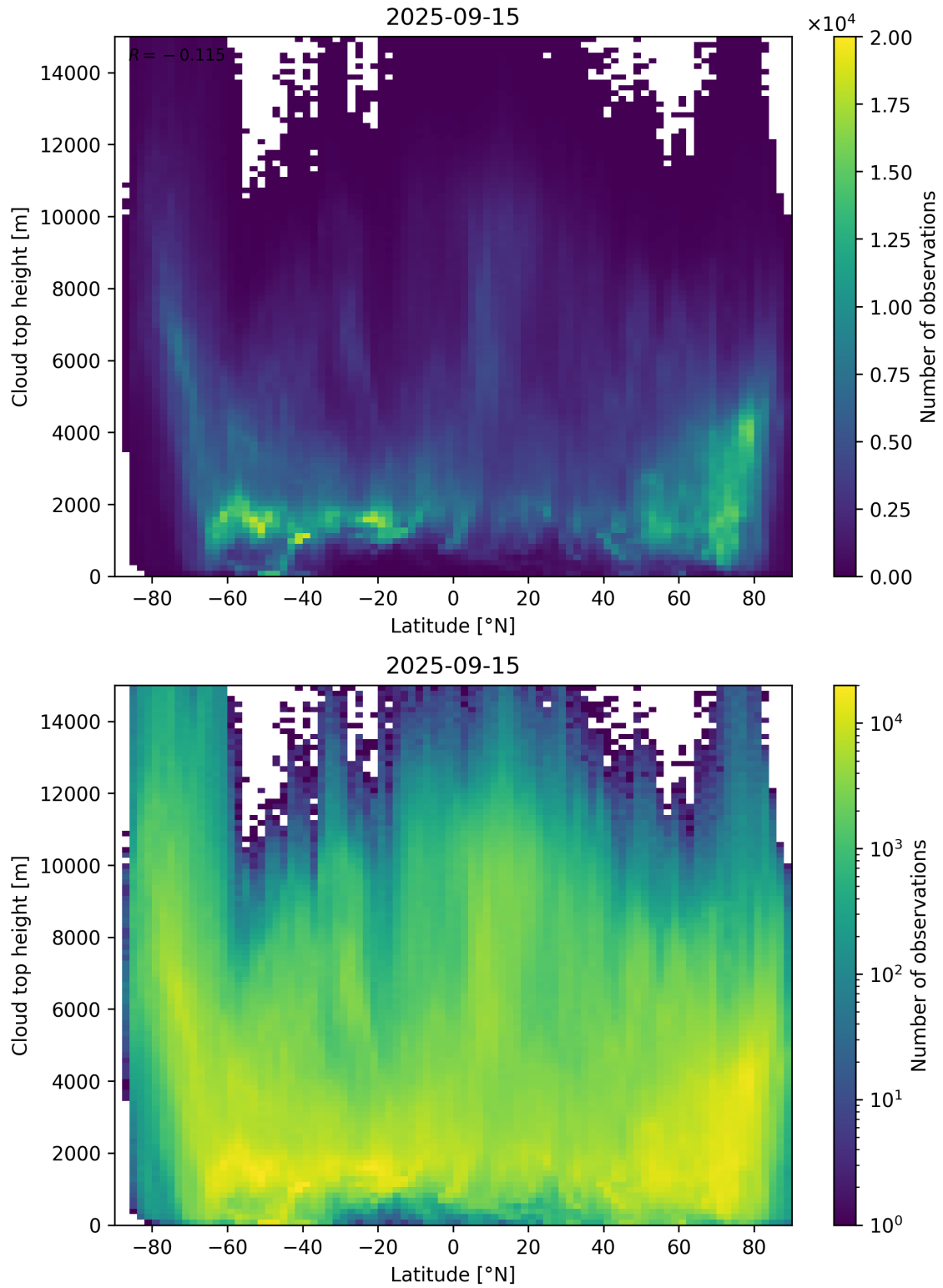
Figure 97: Scatter density plot of “Latitude” against “Cloud top height” for 2025-09-15 to 2025-09-16.
