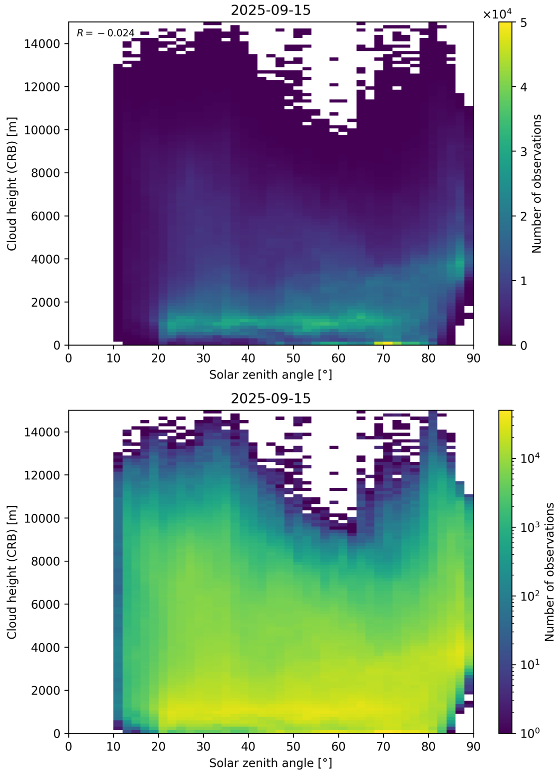
Figure 102: Scatter density plot of “Solar zenith angle” against “Cloud height (CRB)” for 2025-09-15 to 2025-09-16.
