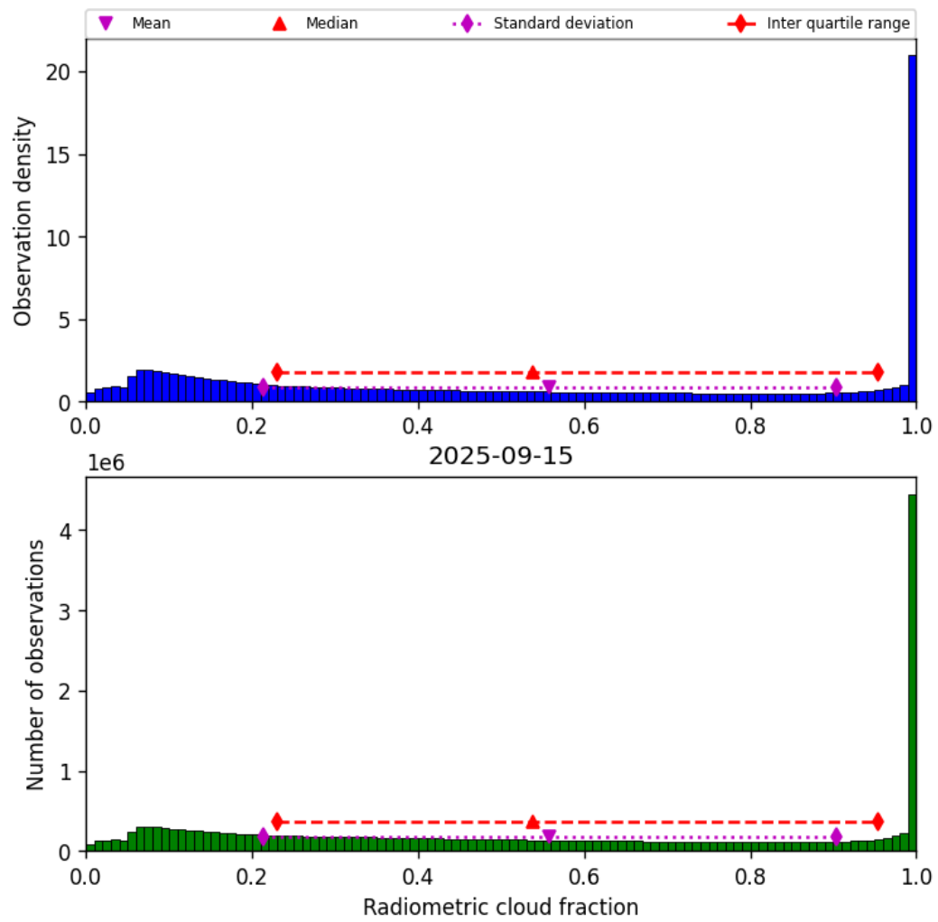
Figure 39: Histogram of “Radiometric cloud fraction” for 2025-09-15 to 2025-09-16
