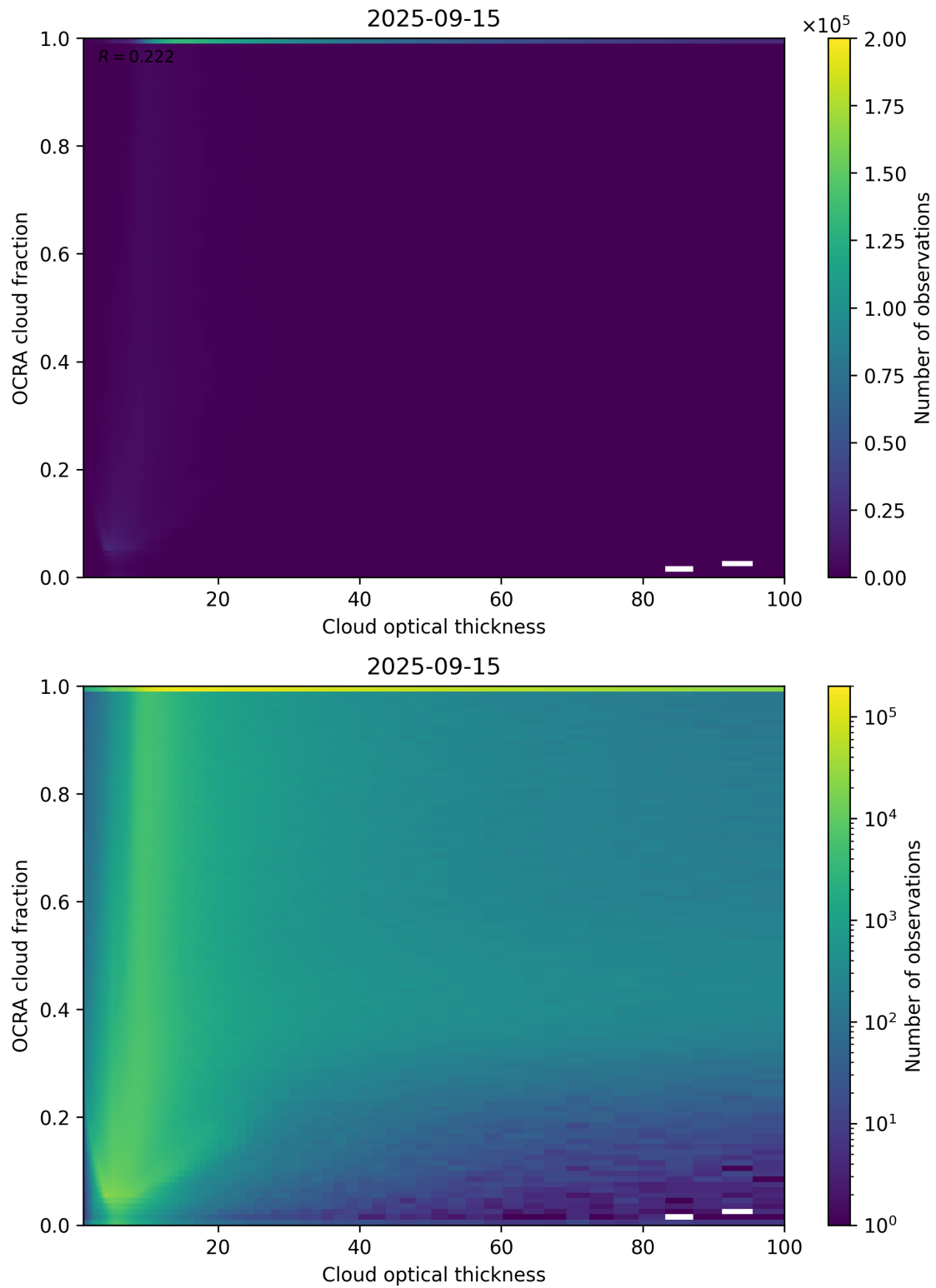
Figure 83: Scatter density plot of “Cloud optical thickness” against “OCRA cloud fraction” for 2025-09-15 to 2025-09-16.
