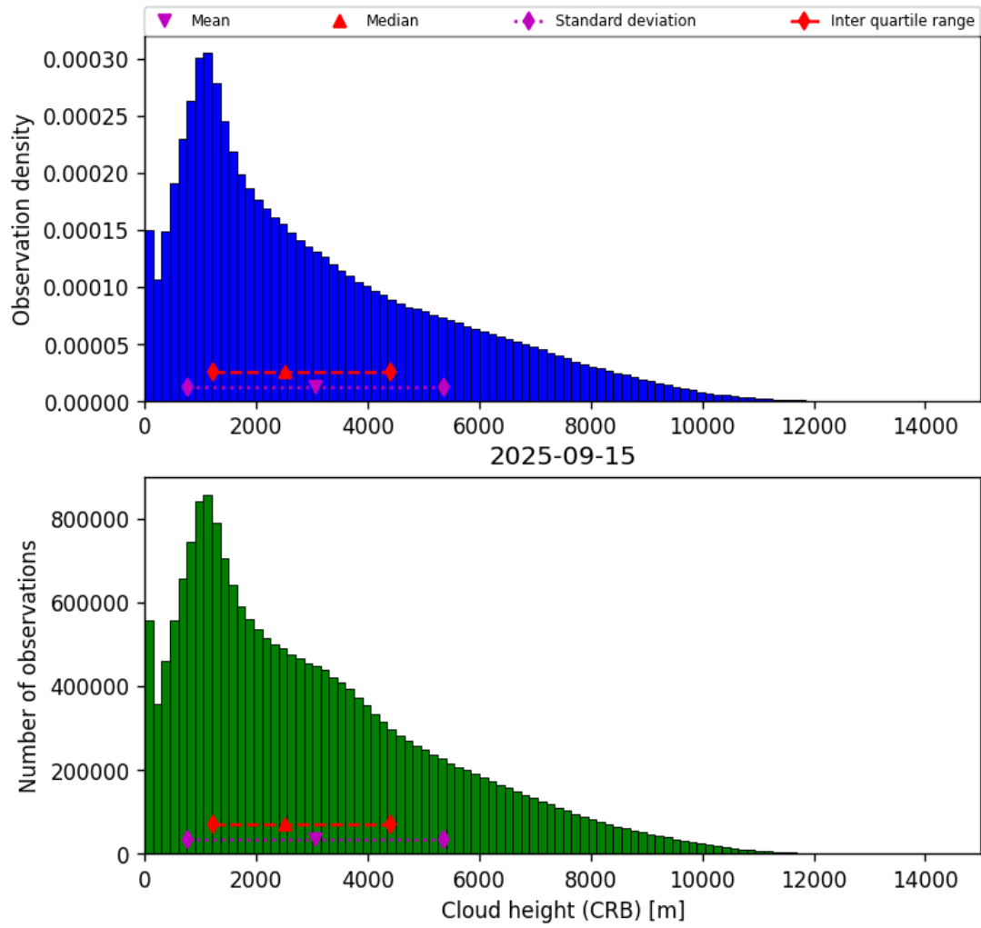
Figure 43: Histogram of “Cloud height (CRB)” for 2025-09-15 to 2025-09-16
