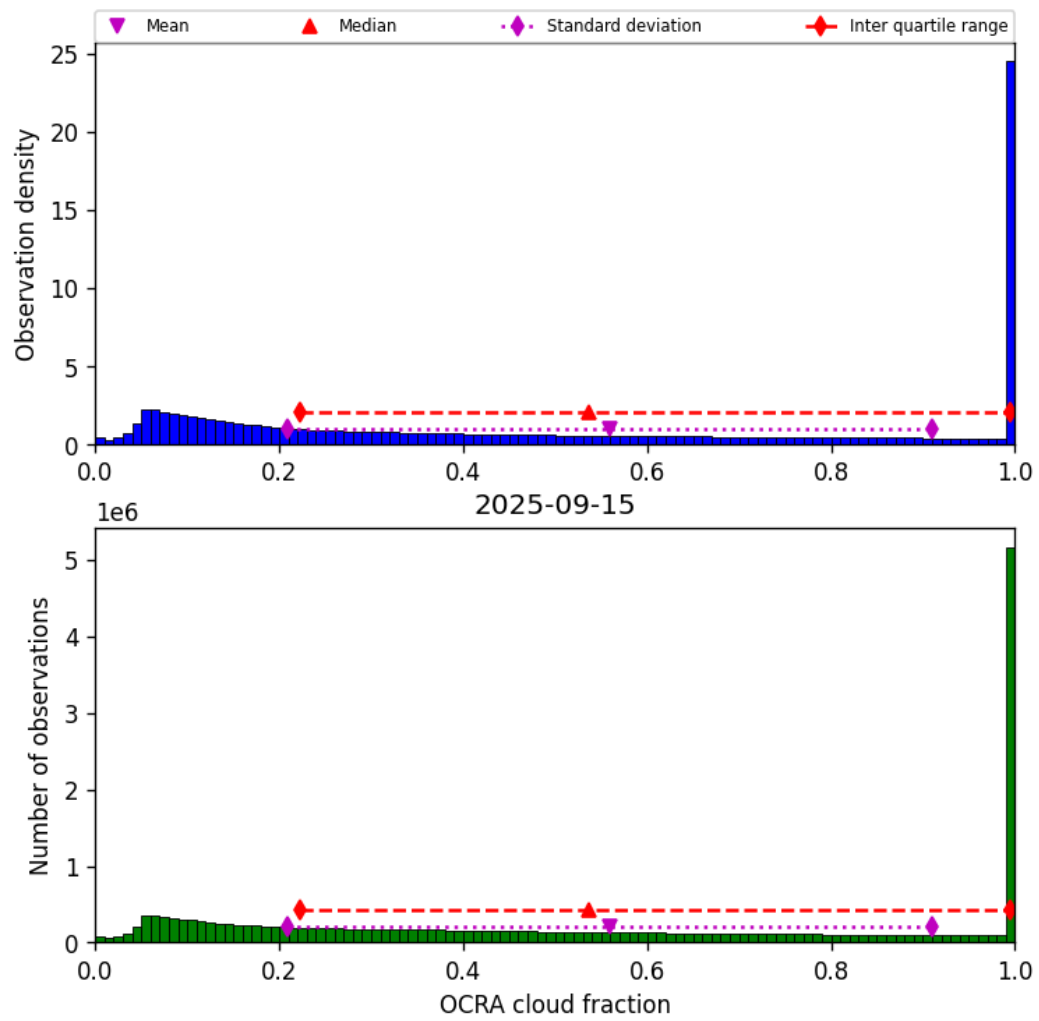
Figure 50: Histogram of “OCRA cloud fraction” for 2025-09-15 to 2025-09-16
