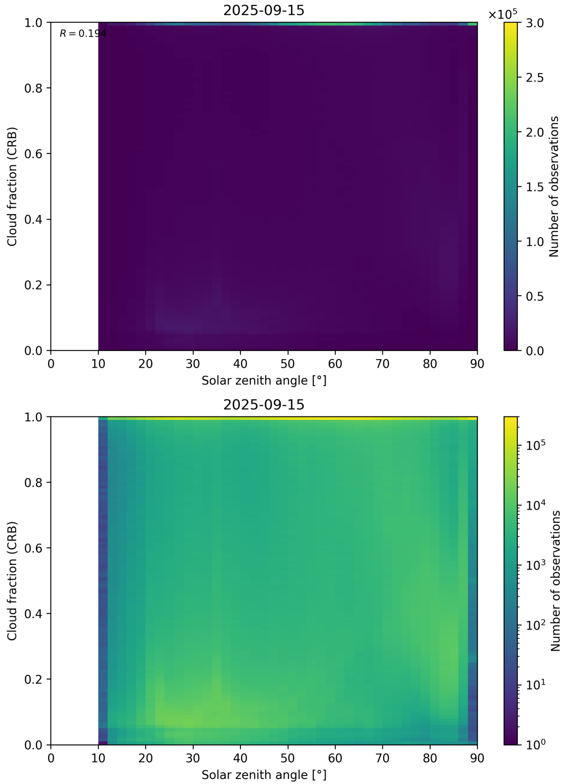
Figure 101: Scatter density plot of “Solar zenith angle” against “Cloud fraction (CRB)” for 2025-09-15 to 2025-09-16.
