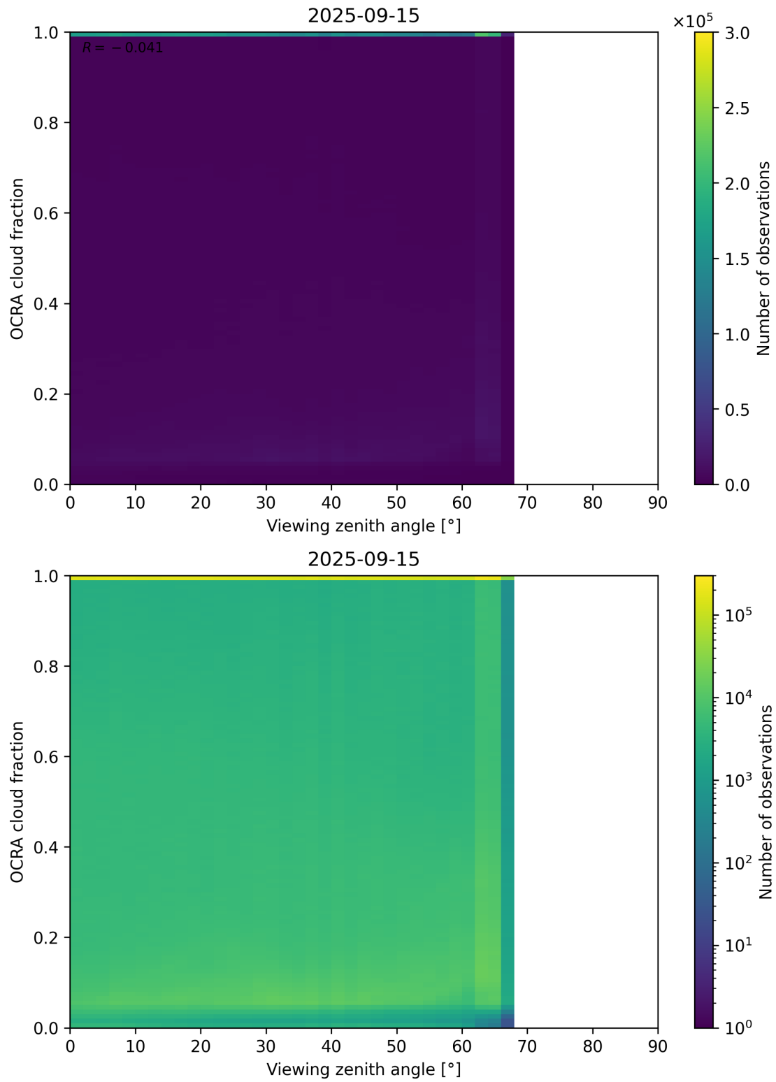
Figure 108: Scatter density plot of “Viewing zenith angle” against “OCRA cloud fraction” for 2025-09-15 to 2025-09-16.
