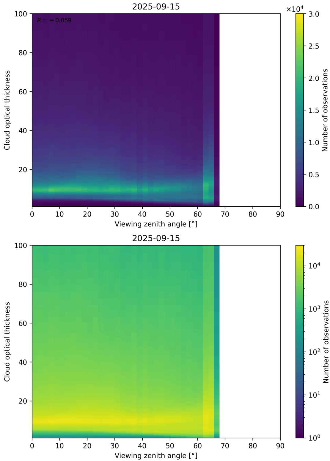
Figure 111: Scatter density plot of “Viewing zenith angle” against “Cloud optical thickness” for 2025-09-15 to 2025-09-16.
