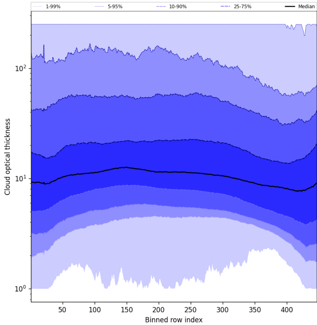
Figure 57: Along track statistics of “Cloud optical thickness” for 2025-09-15 to 2025-09-16
