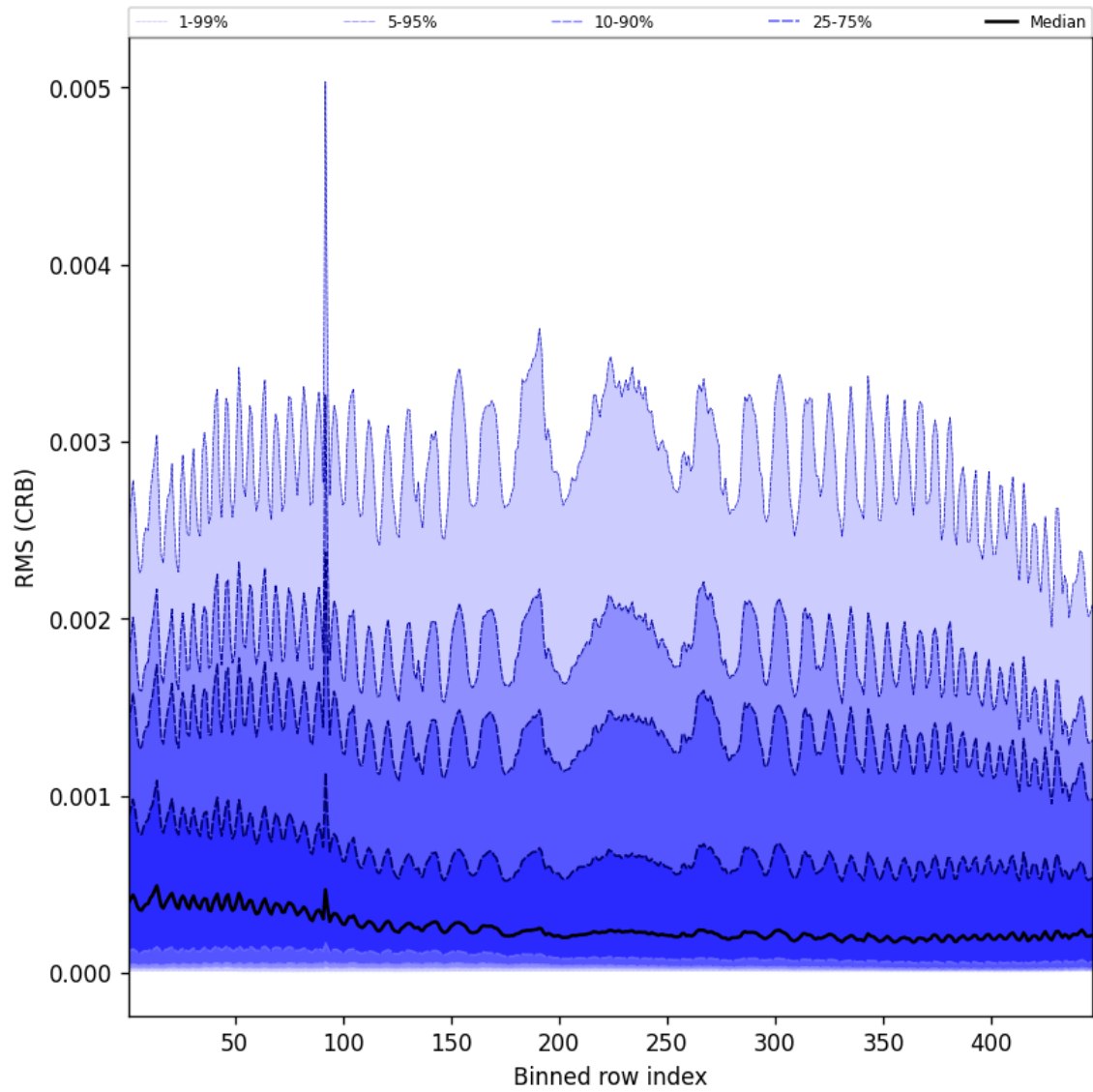
Figure 64: Along track statistics of “RMS (CRB)” for 2025-09-15 to 2025-09-16
