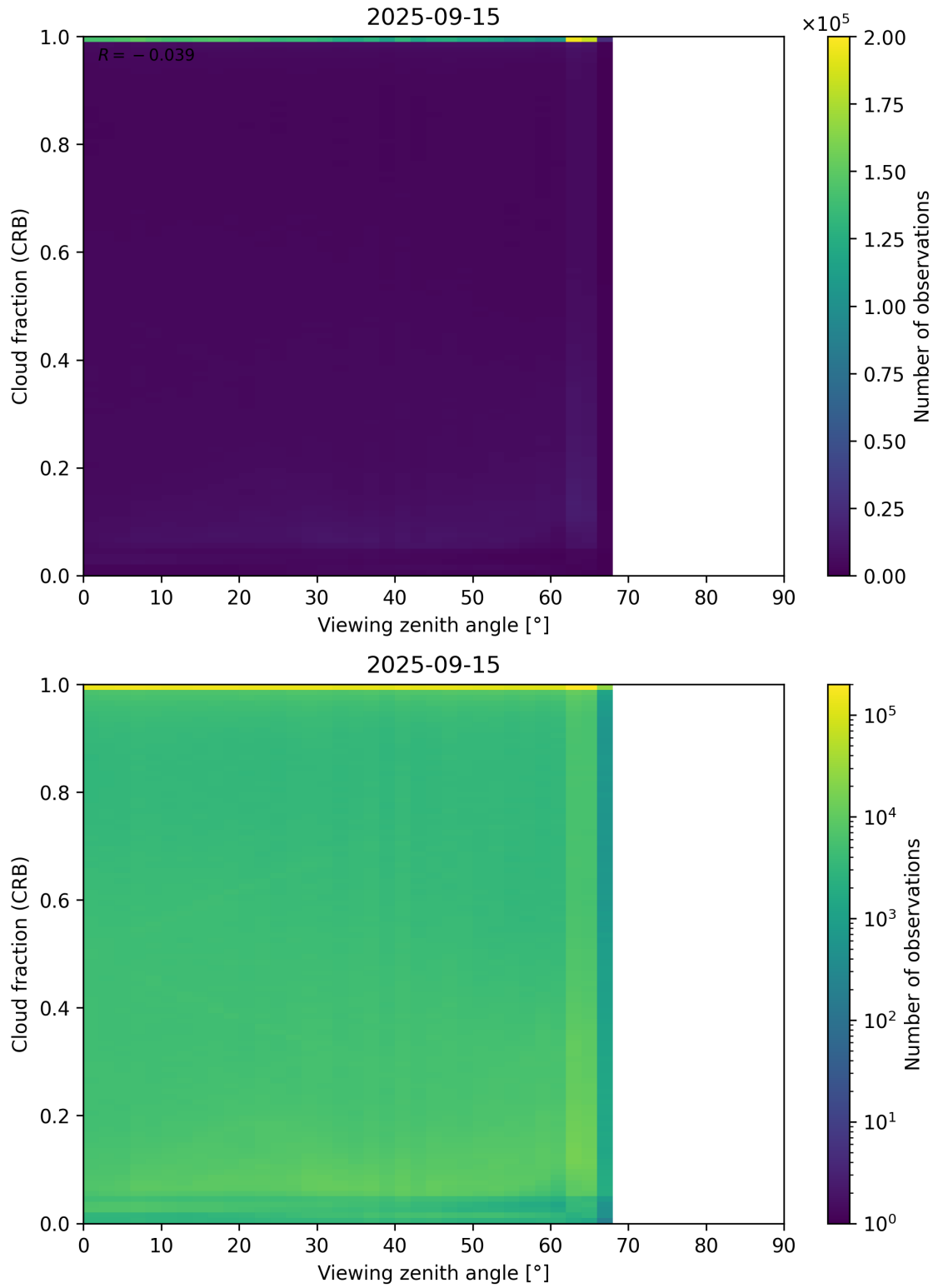
Figure 109: Scatter density plot of “Viewing zenith angle” against “Cloud fraction (CRB)” for 2025-09-15 to 2025-09-16.
