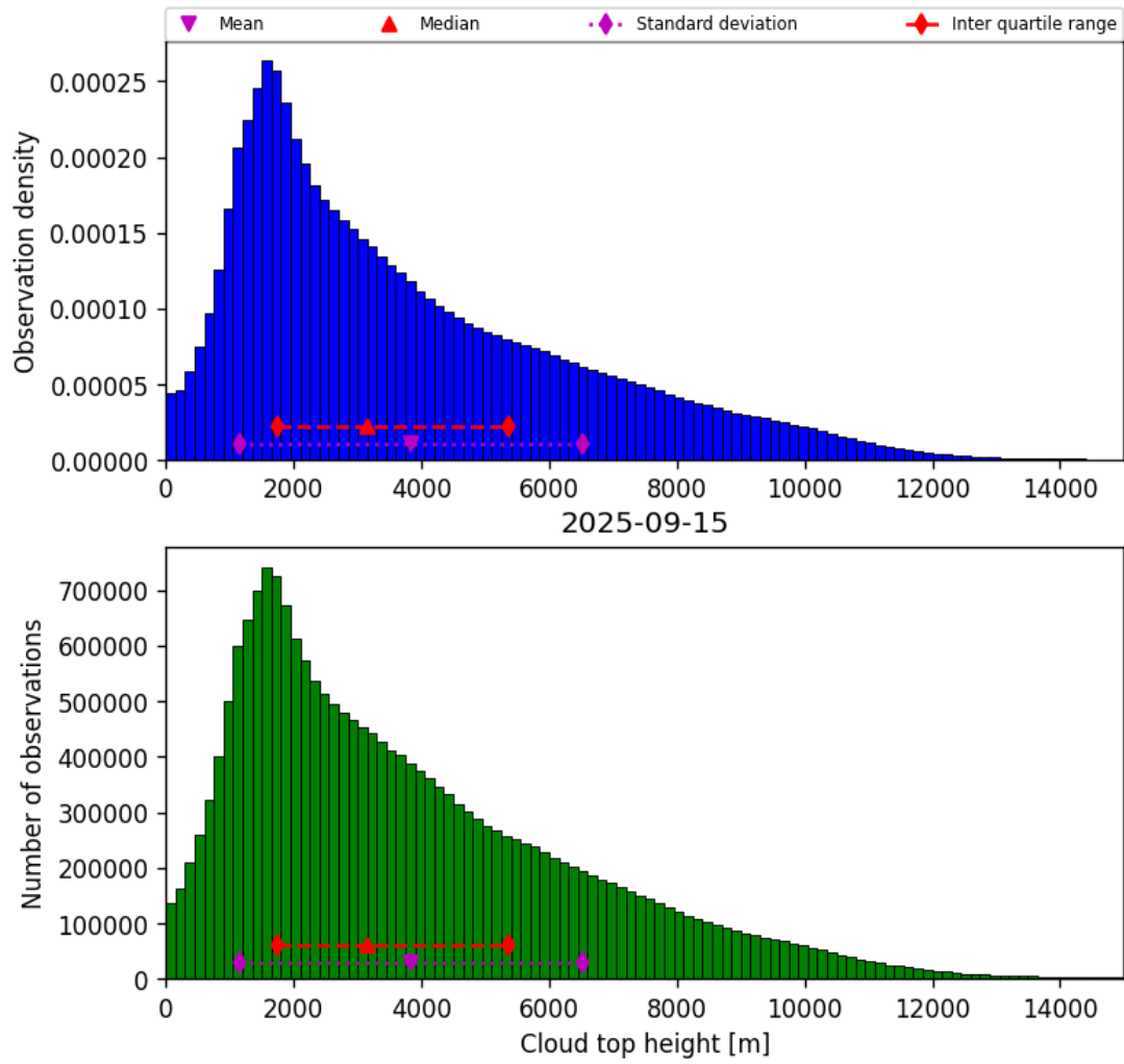
Figure 40: Histogram of “Cloud top height” for 2025-09-15 to 2025-09-16
