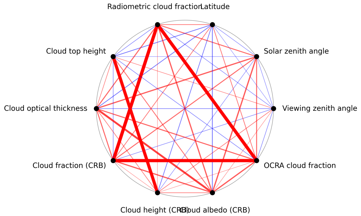
Figure 1: Map of correlation graph for 2025-09-15 to 2025-09-16.
