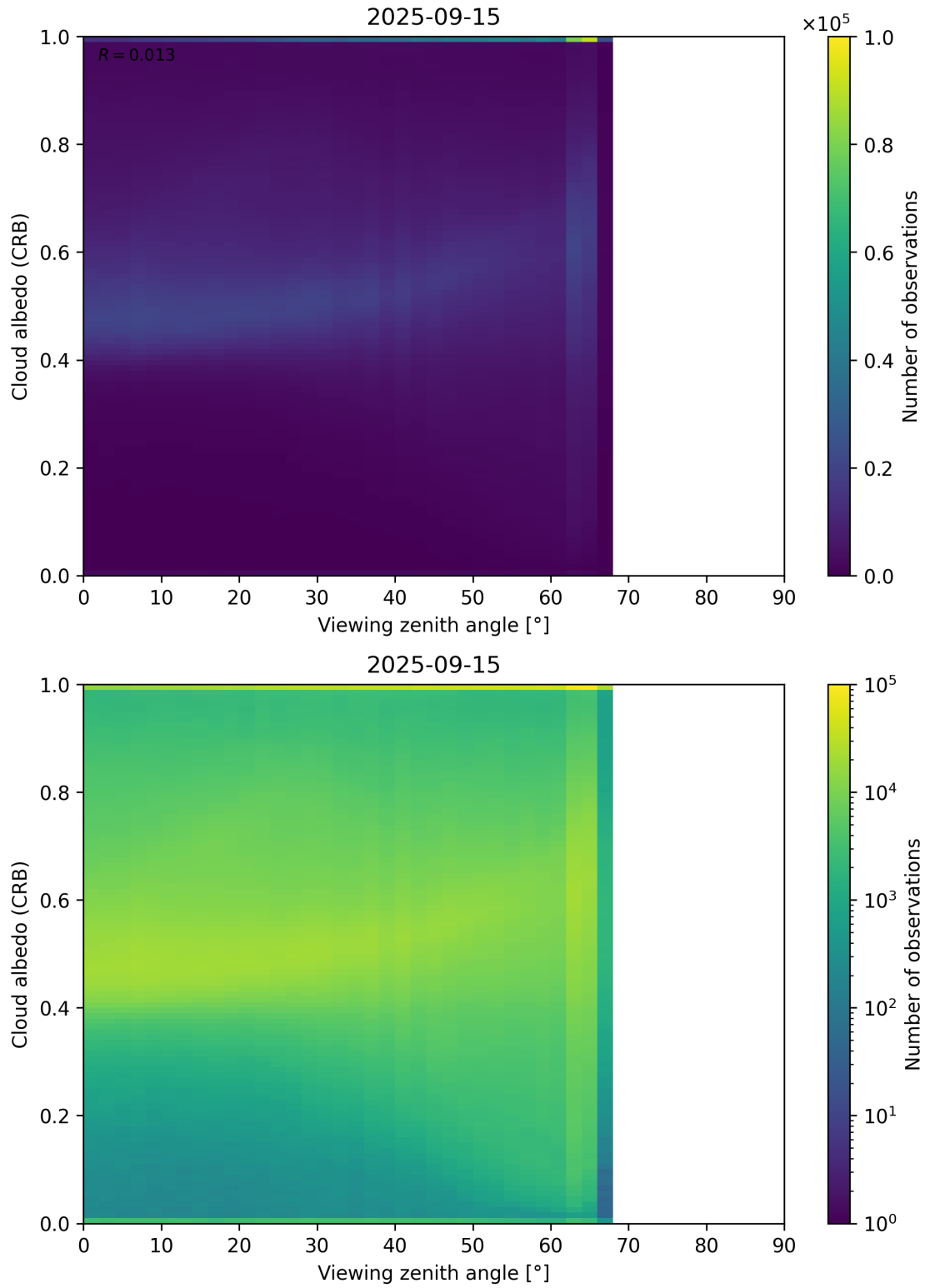
Figure 106: Scatter density plot of “Viewing zenith angle” against “Cloud albedo (CRB)” for 2025-09-15 to 2025-09-16.
