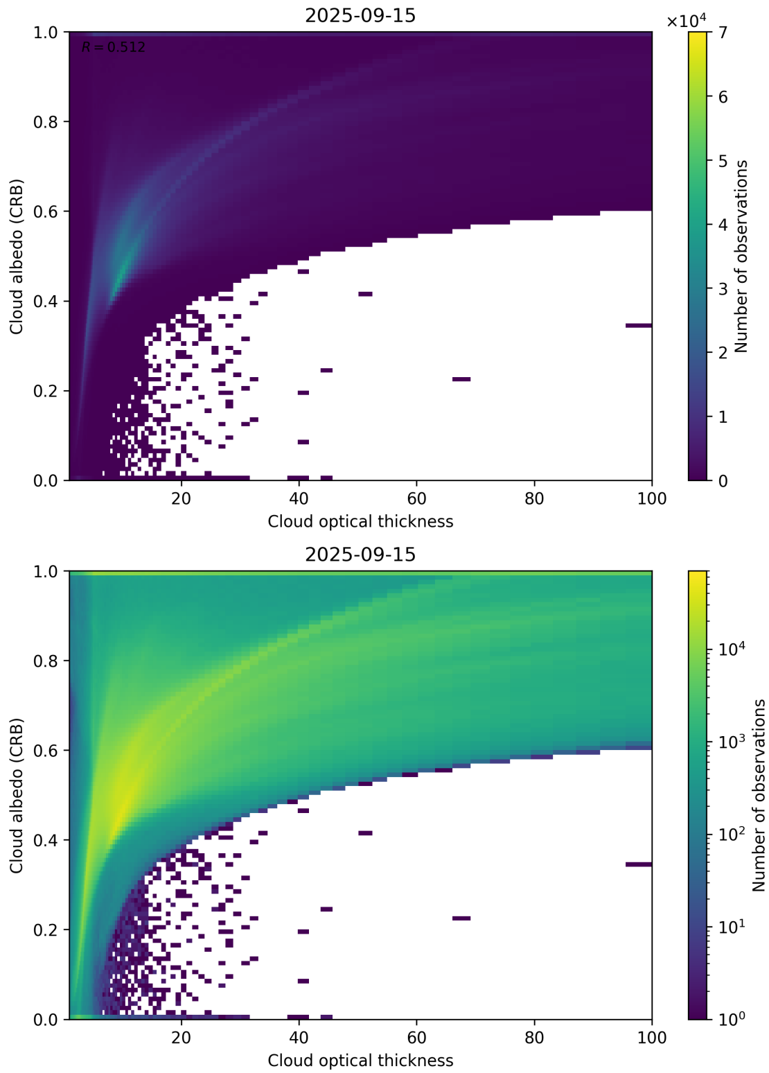
Figure 82: Scatter density plot of “Cloud optical thickness” against “Cloud albedo (CRB)” for 2025-09-15 to 2025-09-16.
