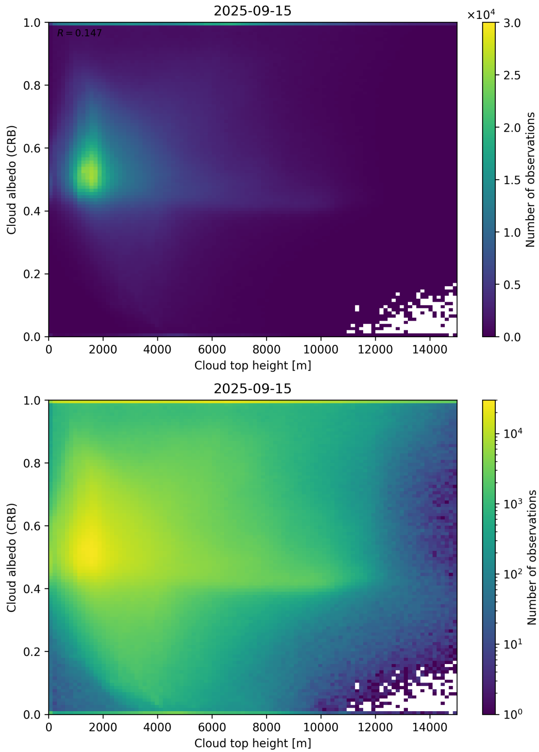
Figure 86: Scatter density plot of “Cloud top height” against “Cloud albedo (CRB)” for 2025-09-15 to 2025-09-16.
