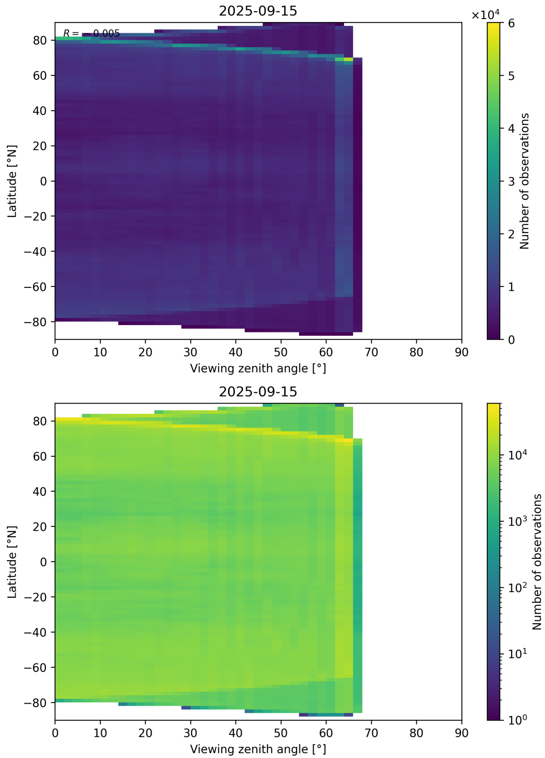
Figure 113: Scatter density plot of “Viewing zenith angle” against “Latitude” for 2025-09-15 to 2025-09-16.
