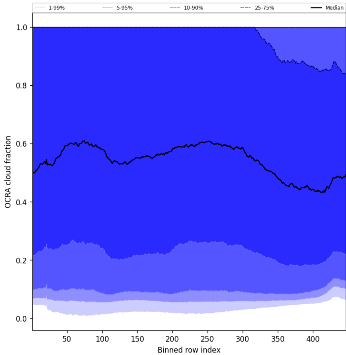
Figure 66: Along track statistics of “OCRA cloud fraction” for 2025-09-15 to 2025-09-16
