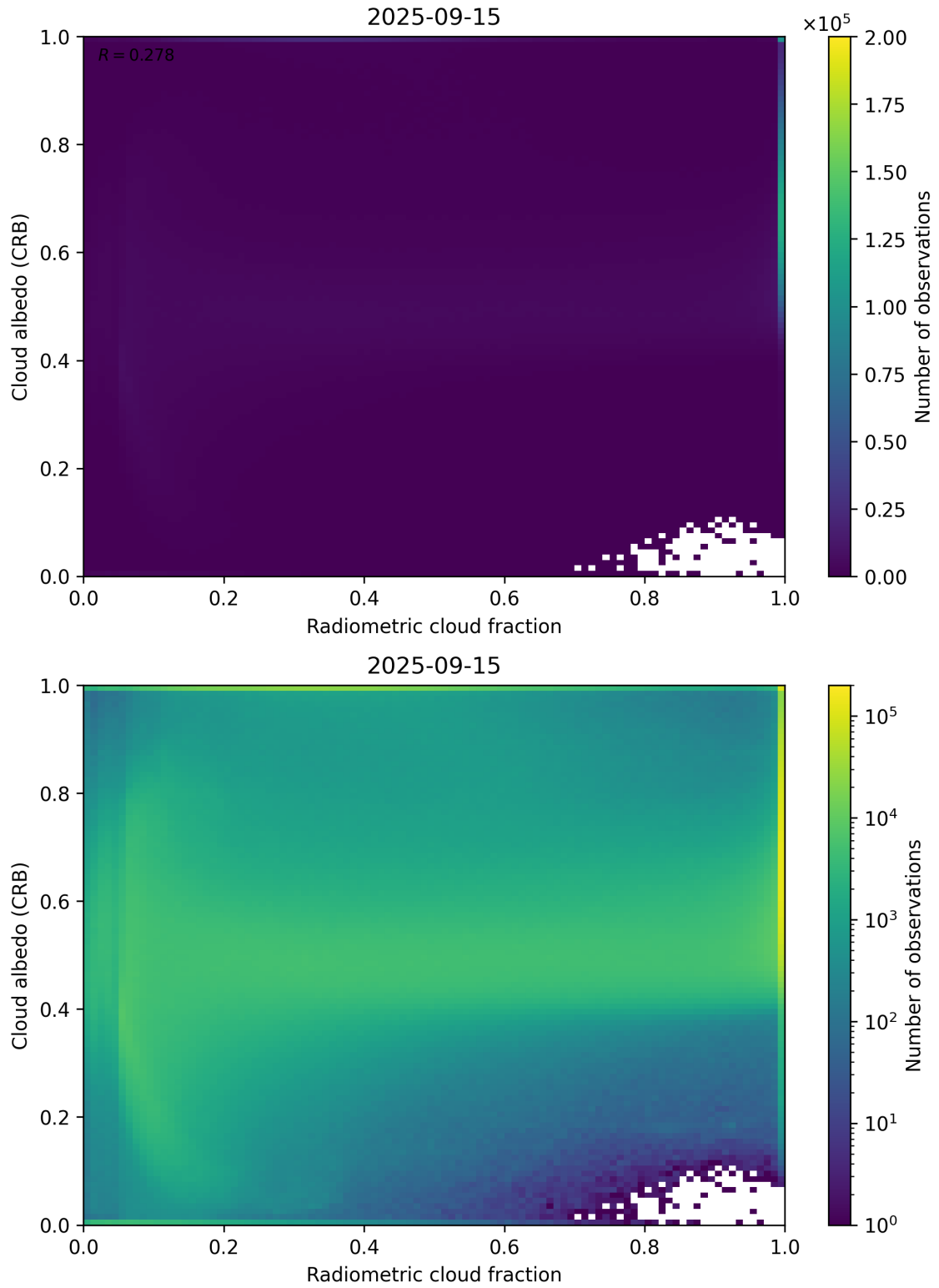
Figure 71: Scatter density plot of “Radiometric cloud fraction” against “Cloud albedo (CRB)” for 2025-09-15 to 2025-09-16.
