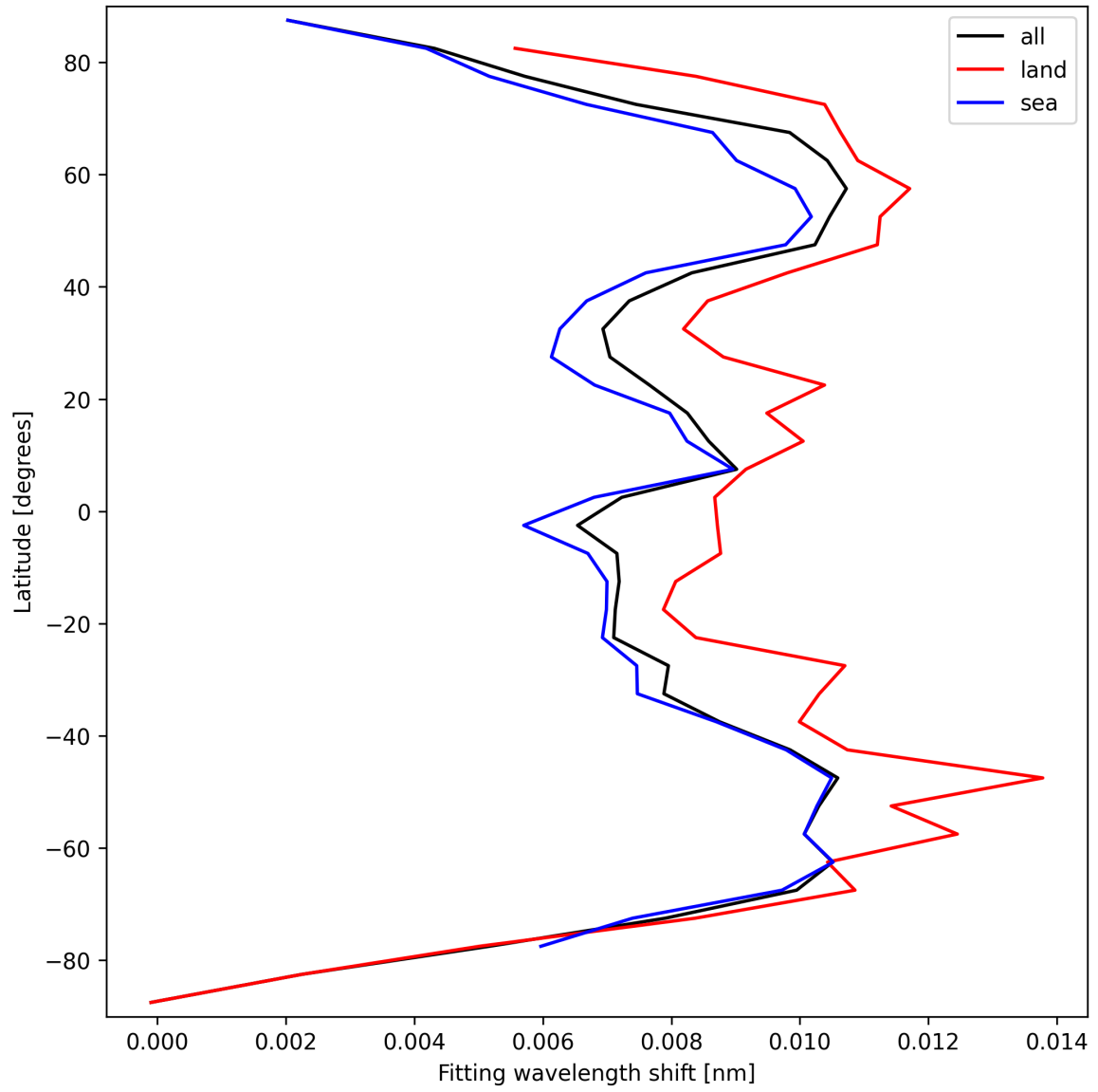
Figure 33: Zonal average of “Fitting wavelength shift” for 2025-09-15 to 2025-09-16.
