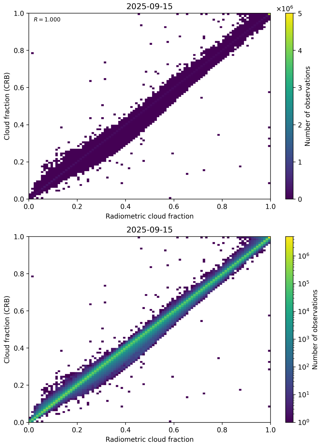
Figure 73: Scatter density plot of “Radiometric cloud fraction” against “Cloud fraction (CRB)” for 2025-09-15 to 2025-09-16.
