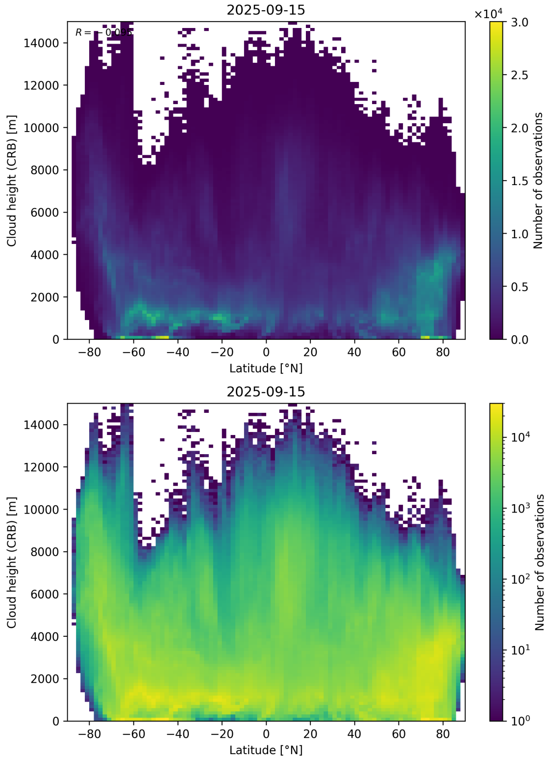
Figure 95: Scatter density plot of “Latitude” against “Cloud height (CRB)” for 2025-09-15 to 2025-09-16.
