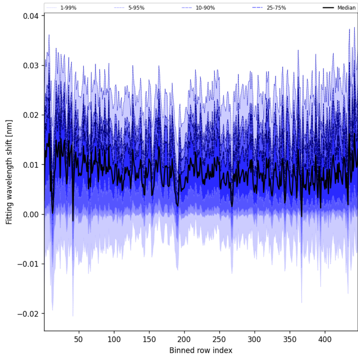
Figure 65: Along track statistics of “Fitting wavelength shift” for 2025-09-15 to 2025-09-16
