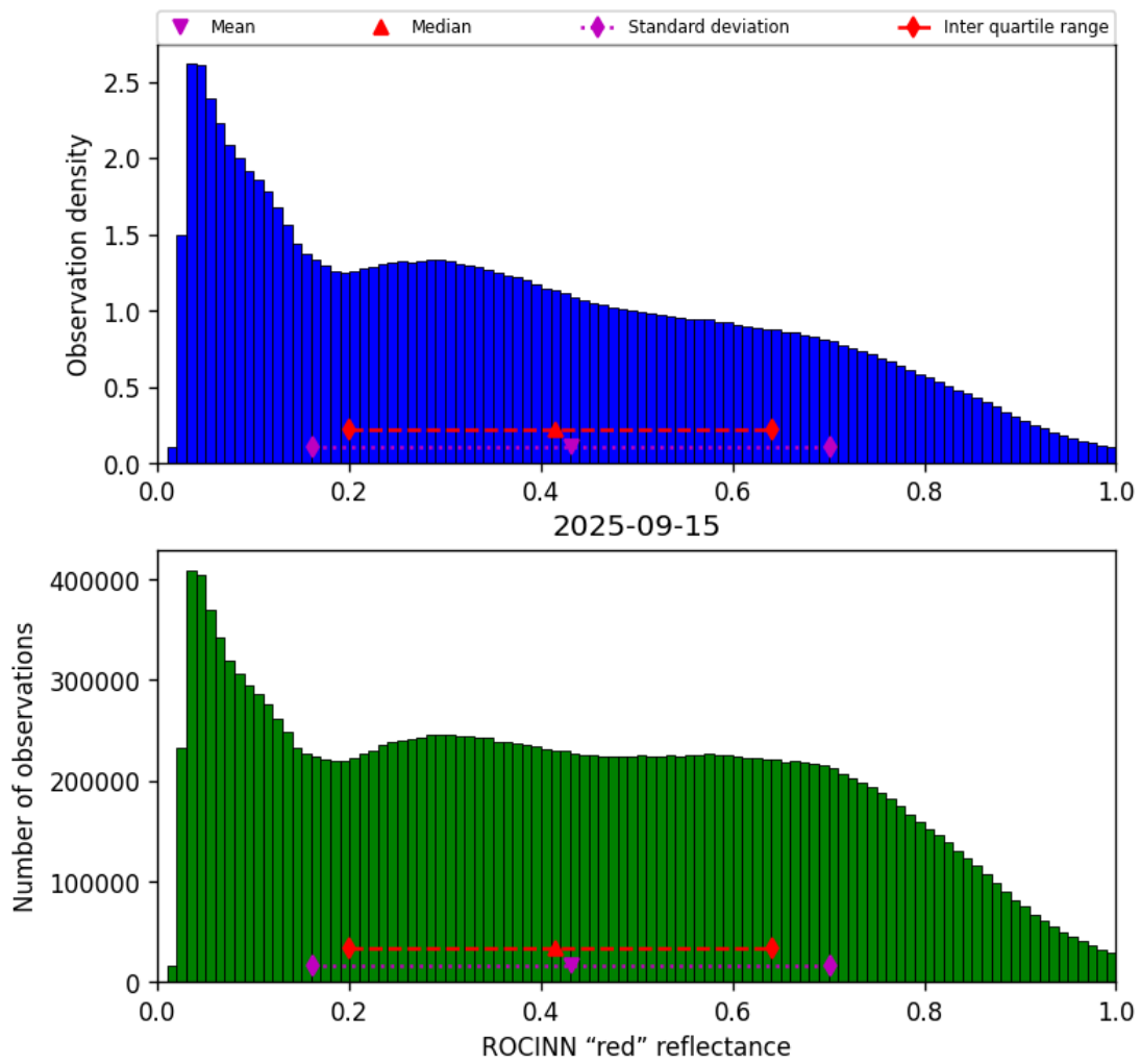
Figure 53: Histogram of “ROCINN “red” reflectance” for 2025-09-15 to 2025-09-16
