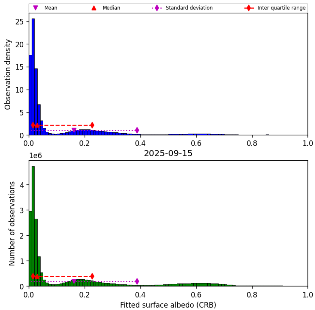
Figure 46: Histogram of “Fitted surface albedo (CRB)” for 2025-09-15 to 2025-09-16
