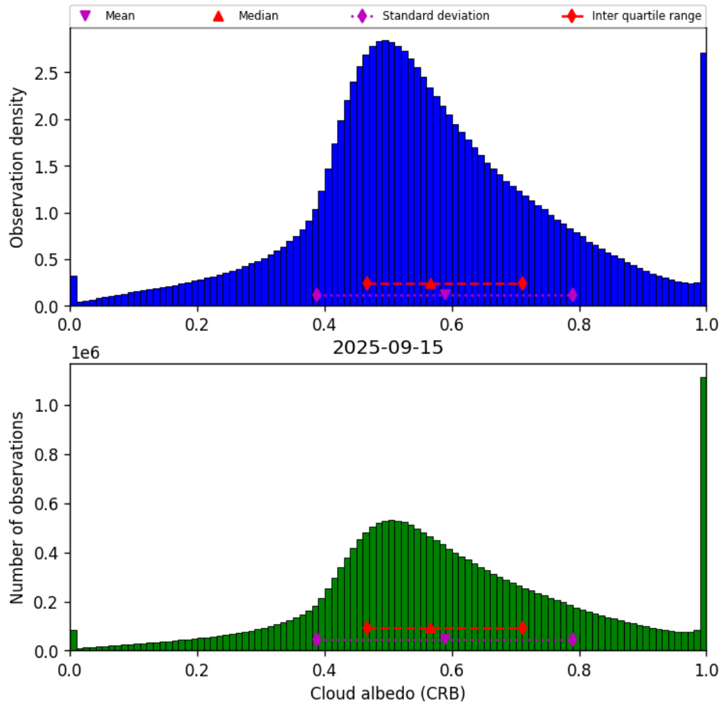
Figure 44: Histogram of “Cloud albedo (CRB)” for 2025-09-15 to 2025-09-16
