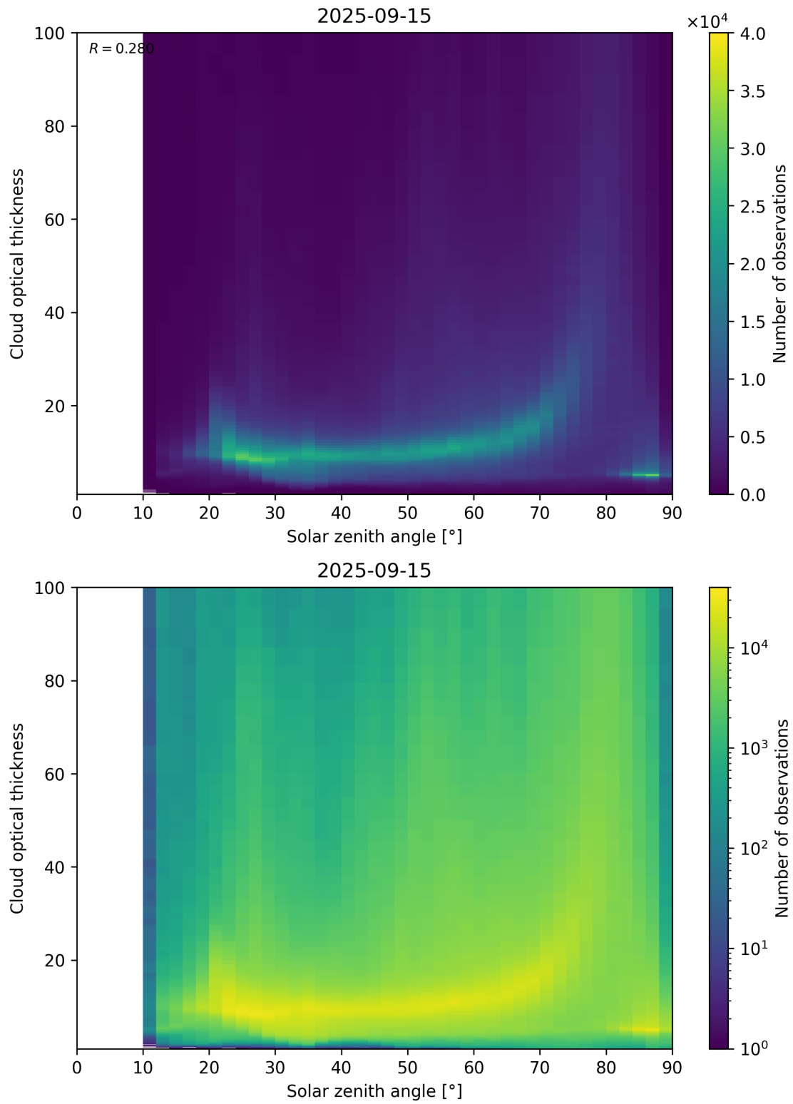
Figure 103: Scatter density plot of “Solar zenith angle” against “Cloud optical thickness” for 2025-09-15 to 2025-09-16.
