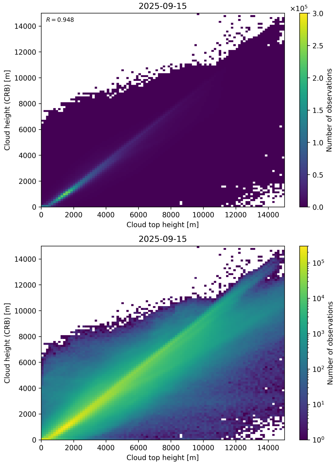
Figure 89: Scatter density plot of “Cloud top height” against “Cloud height (CRB)” for 2025-09-15 to 2025-09-16.
