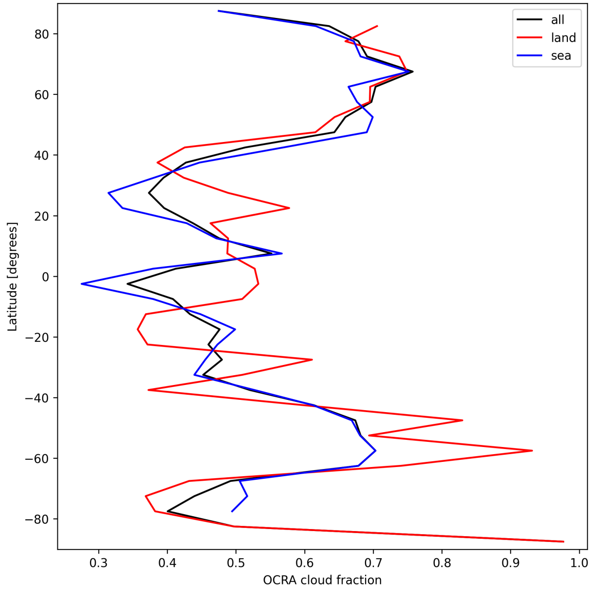
Figure 34: Zonal average of “OCRA cloud fraction” for 2025-09-15 to 2025-09-16.
