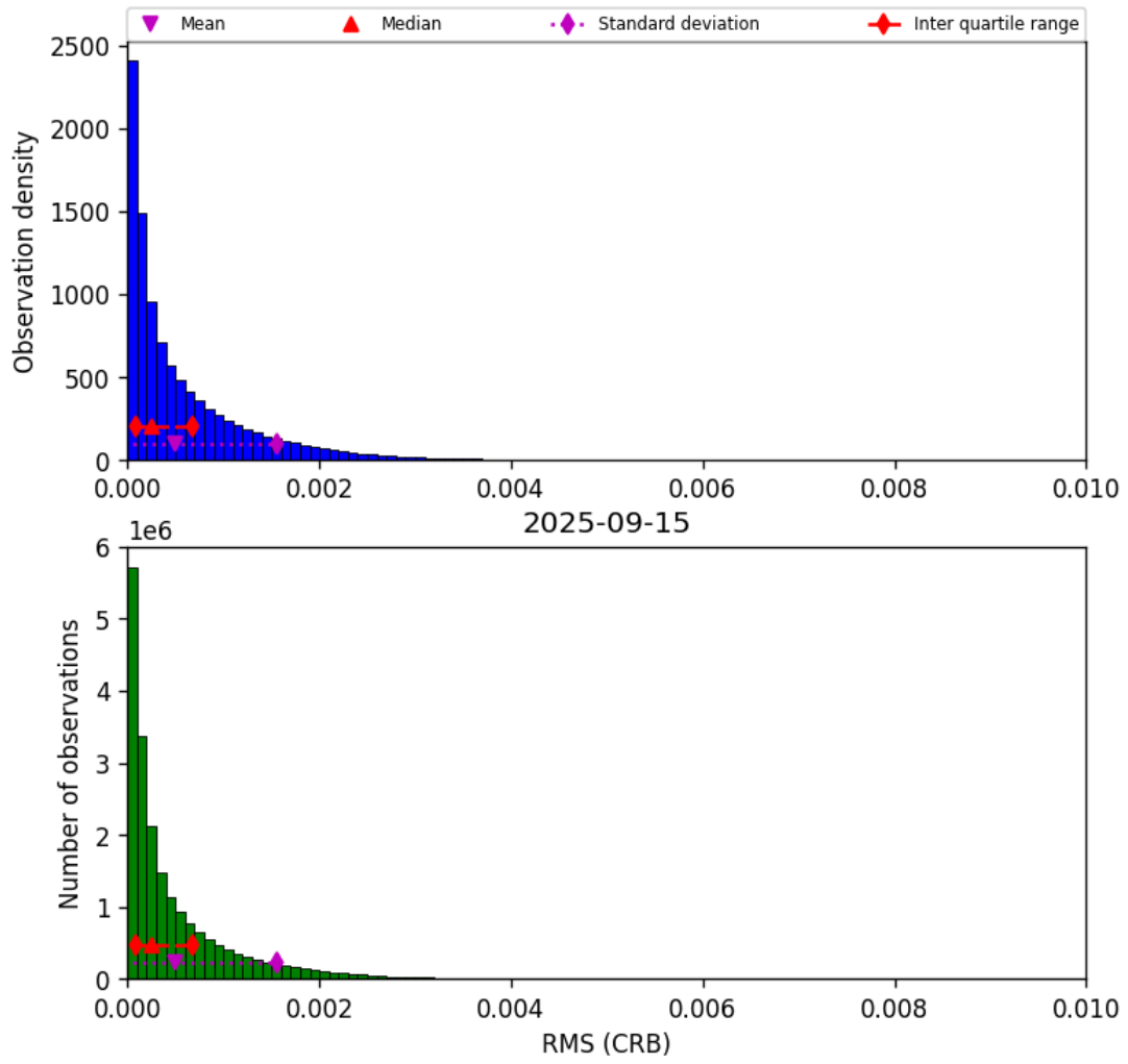
Figure 48: Histogram of “RMS (CRB)” for 2025-09-15 to 2025-09-16
