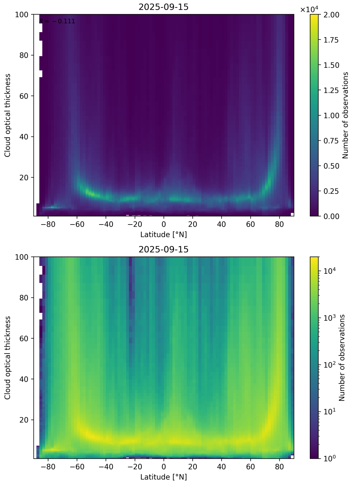
Figure 96: Scatter density plot of “Latitude” against “Cloud optical thickness” for 2025-09-15 to 2025-09-16.
