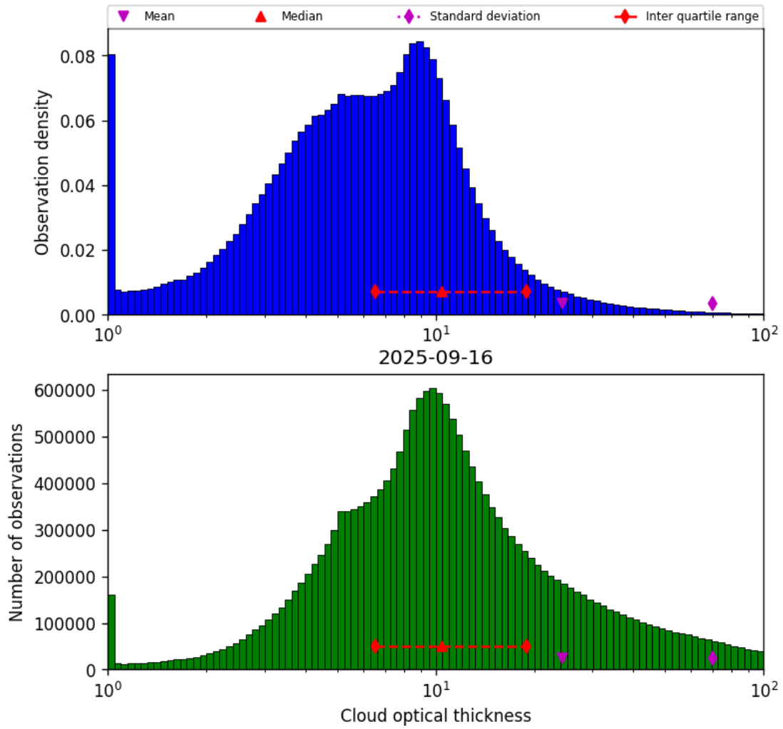
Figure 41: Histogram of “Cloud optical thickness” for 2025-09-15 to 2025-09-17
