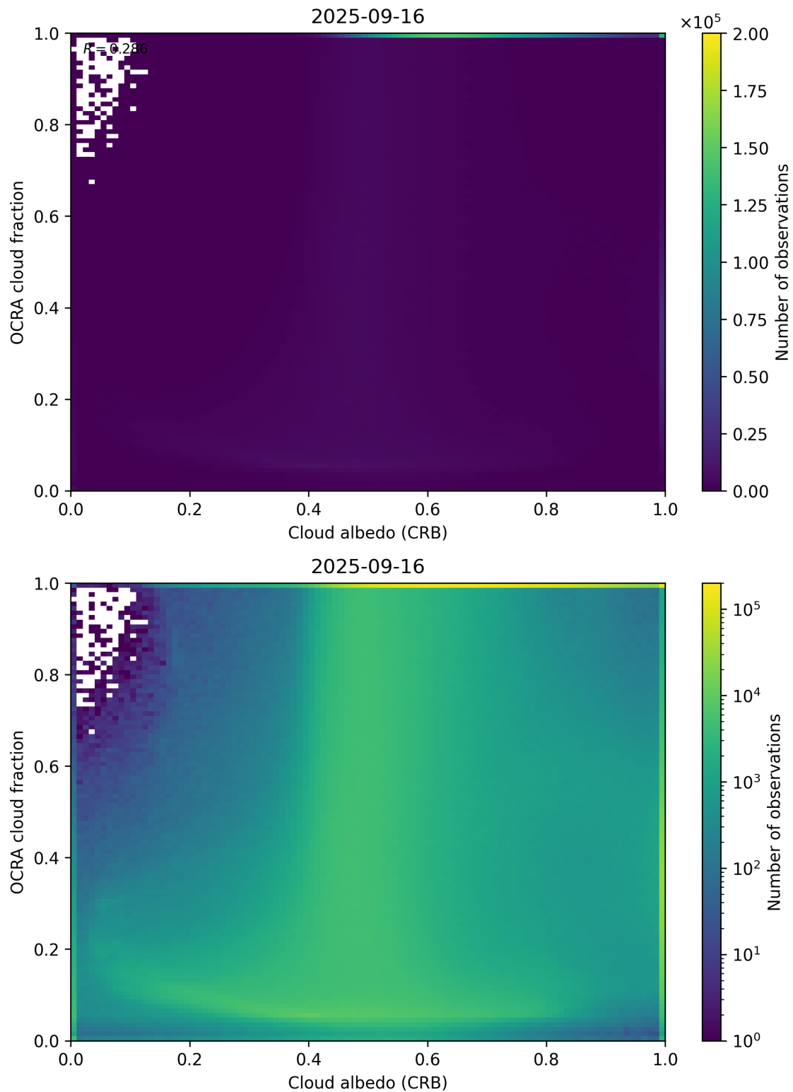
Figure 70: Scatter density plot of “Cloud albedo (CRB)” against “OCRA cloud fraction” for 2025-09-15 to 2025-09-17.
