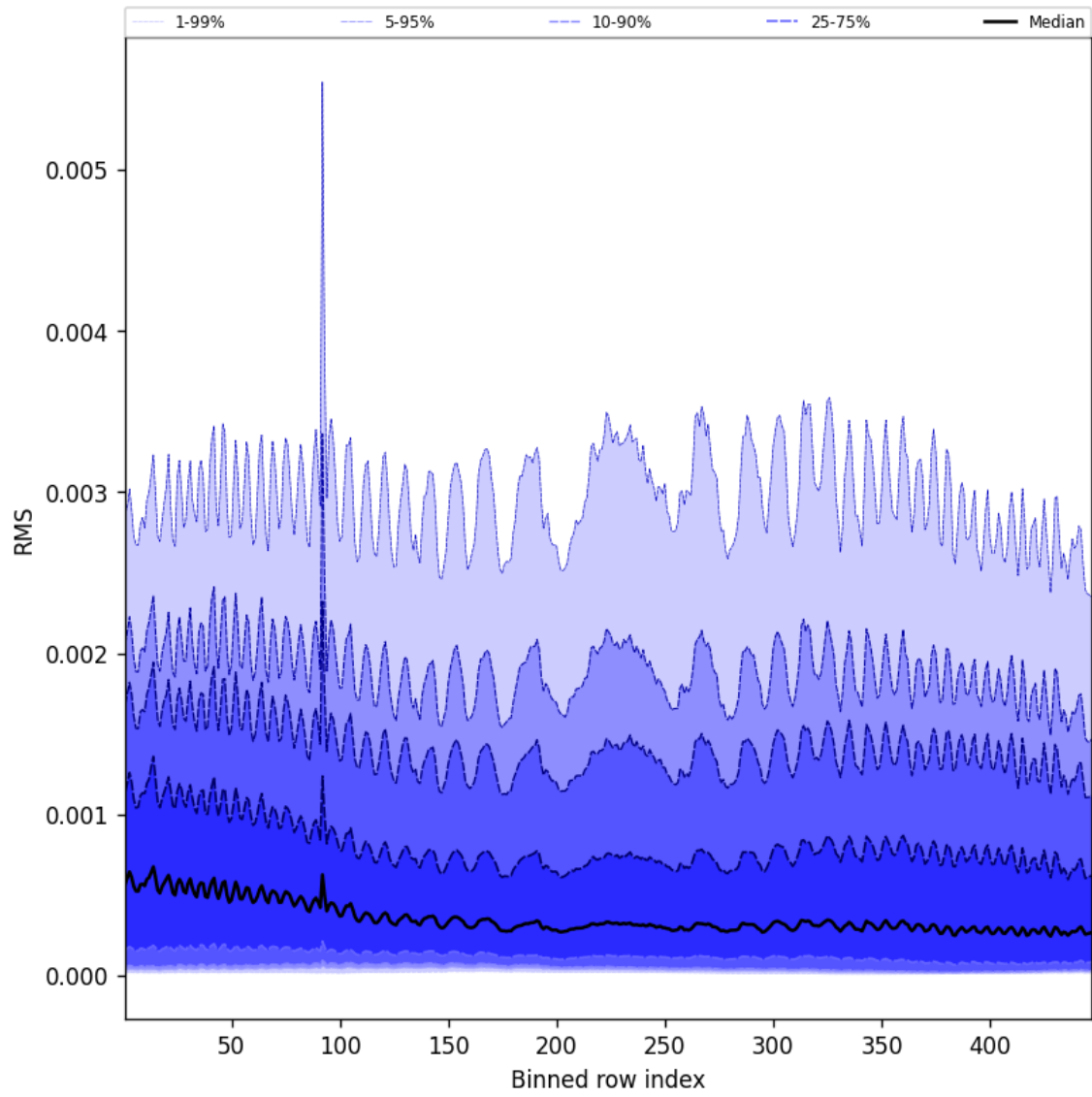
Figure 63: Along track statistics of “RMS” for 2025-09-15 to 2025-09-17
