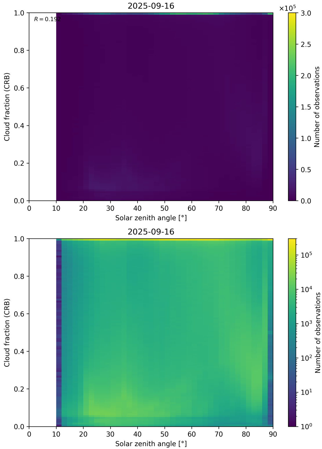
Figure 101: Scatter density plot of “Solar zenith angle” against “Cloud fraction (CRB)” for 2025-09-15 to 2025-09-17.
