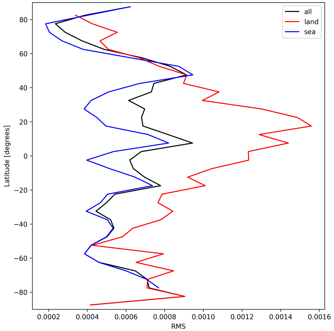
Figure 31: Zonal average of “RMS” for 2025-09-15 to 2025-09-17.
