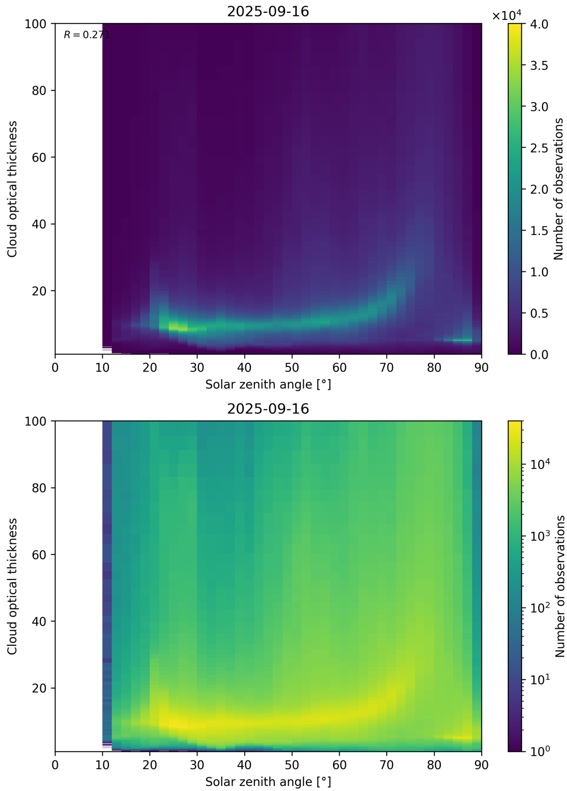
Figure 103: Scatter density plot of “Solar zenith angle” against “Cloud optical thickness” for 2025-09-15 to 2025-09-17.
