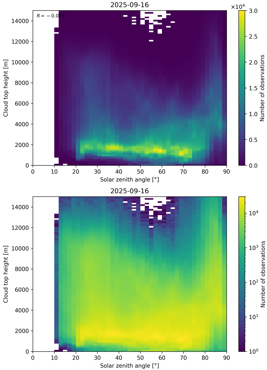
Figure 104: Scatter density plot of “Solar zenith angle” against “Cloud top height” for 2025-09-15 to 2025-09-17.
