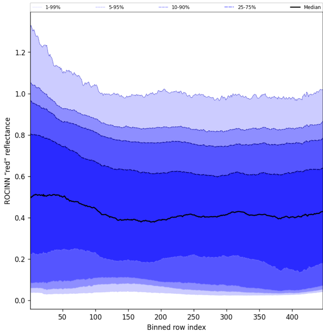
Figure 69: Along track statistics of “ROCINN “red” reflectance” for 2025-09-15 to 2025-09-17
