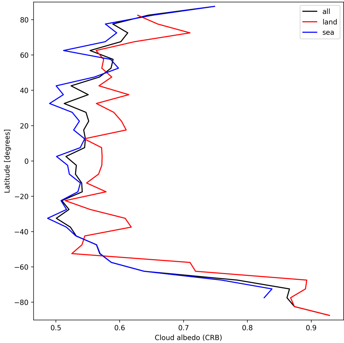
Figure 28: Zonal average of “Cloud albedo (CRB)” for 2025-09-15 to 2025-09-17.
