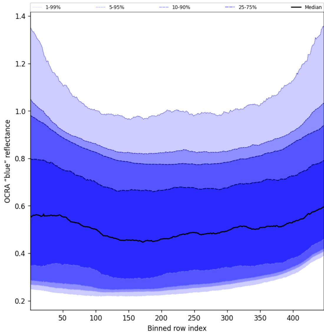
Figure 67: Along track statistics of “OCRA “blue” reflectance” for 2025-09-15 to 2025-09-17
