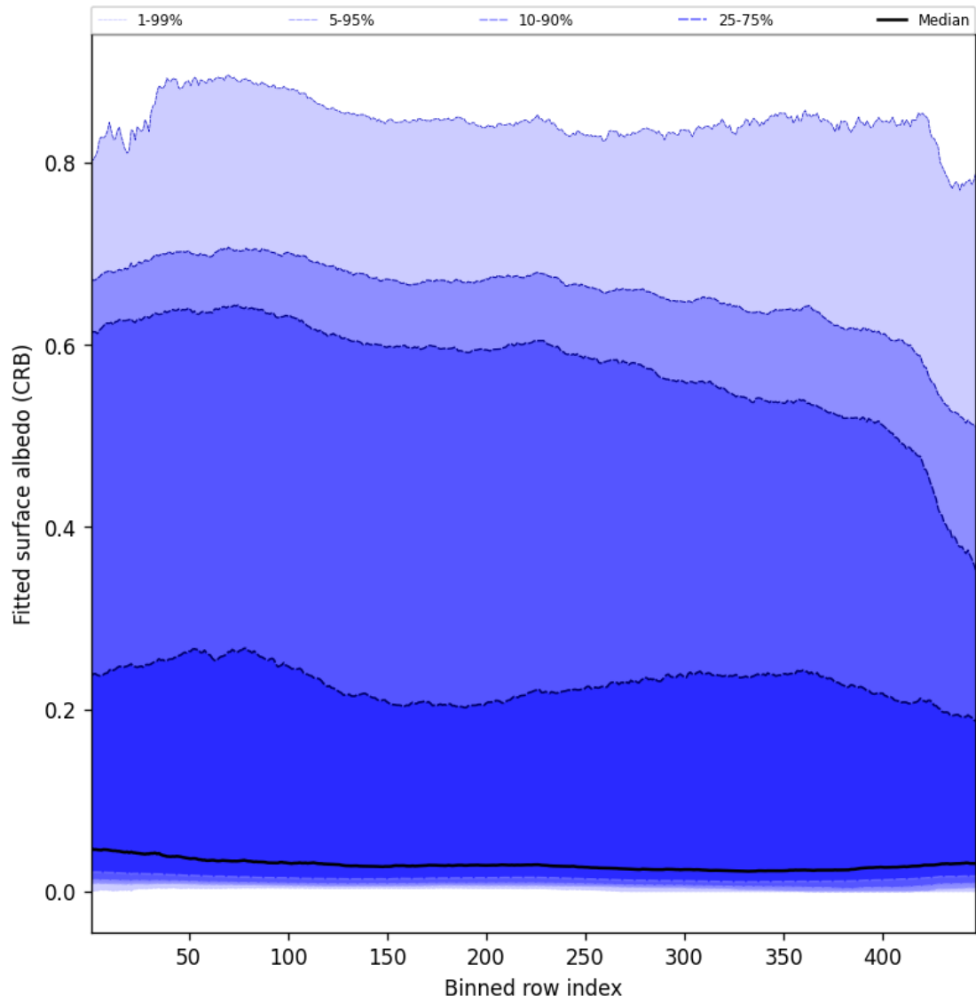
Figure 62: Along track statistics of “Fitted surface albedo (CRB)” for 2025-09-15 to 2025-09-17
