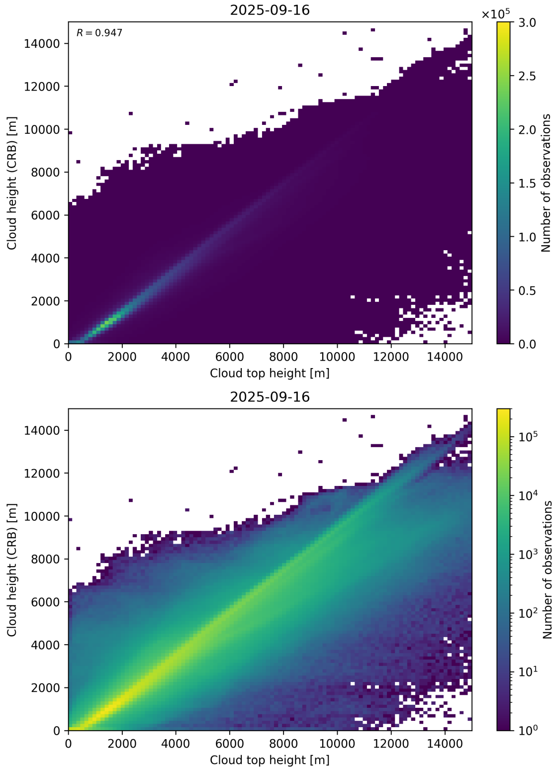
Figure 89: Scatter density plot of “Cloud top height” against “Cloud height (CRB)” for 2025-09-15 to 2025-09-17.
