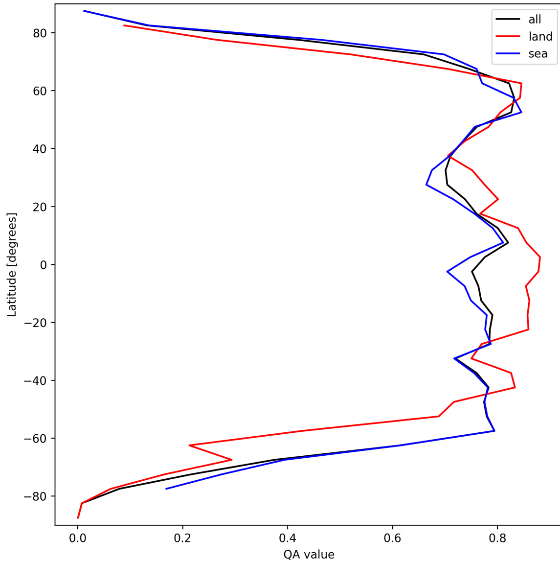
Figure 22: Zonal average of “QA value” for 2025-09-15 to 2025-09-17.
