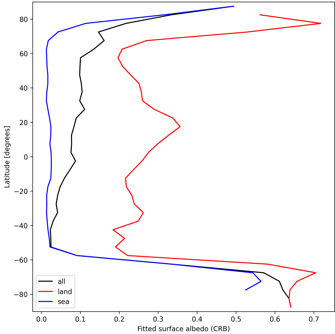
Figure 30: Zonal average of “Fitted surface albedo (CRB)” for 2025-09-15 to 2025-09-17.
