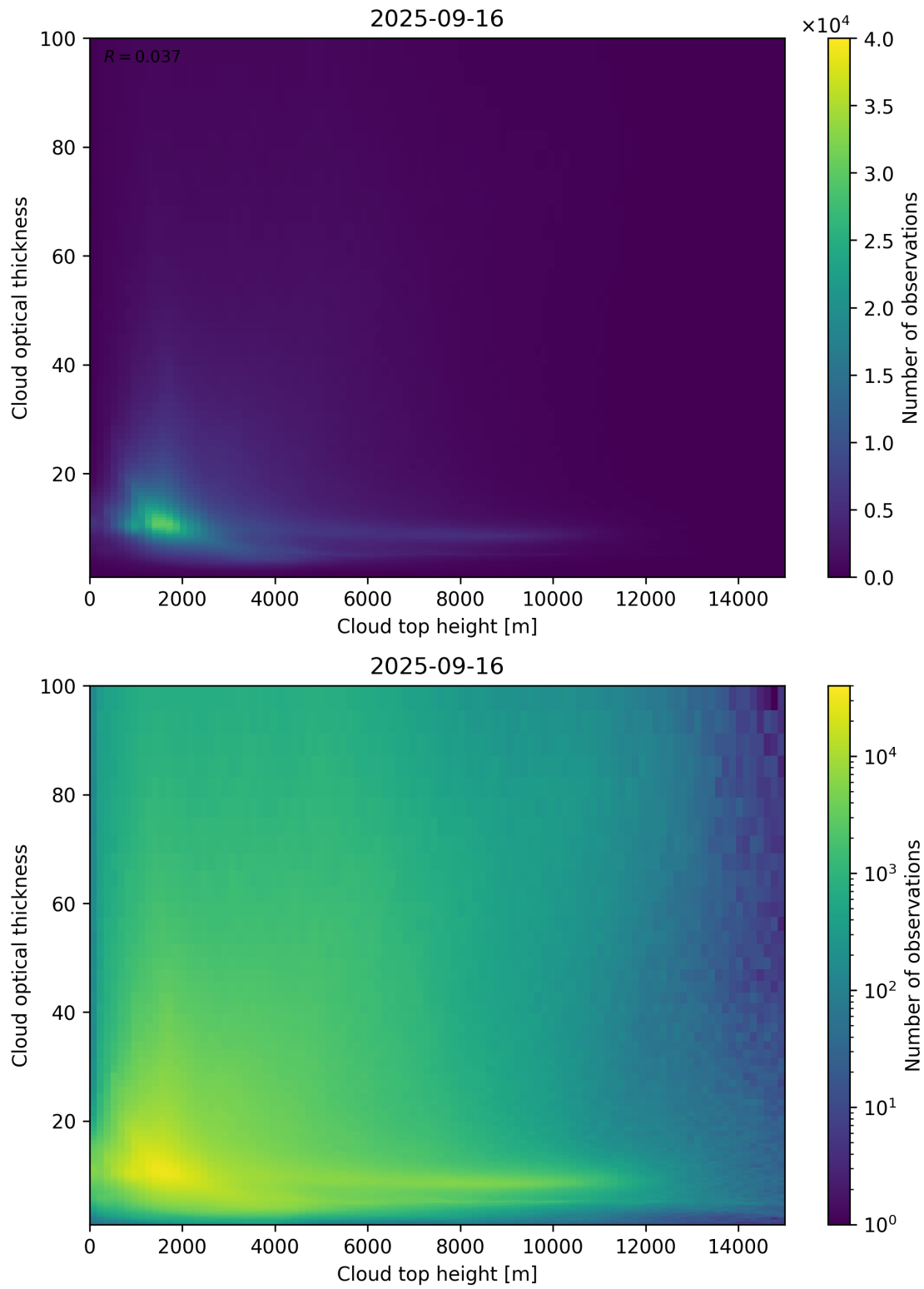
Figure 90: Scatter density plot of “Cloud top height” against “Cloud optical thickness” for 2025-09-15 to 2025-09-17.
