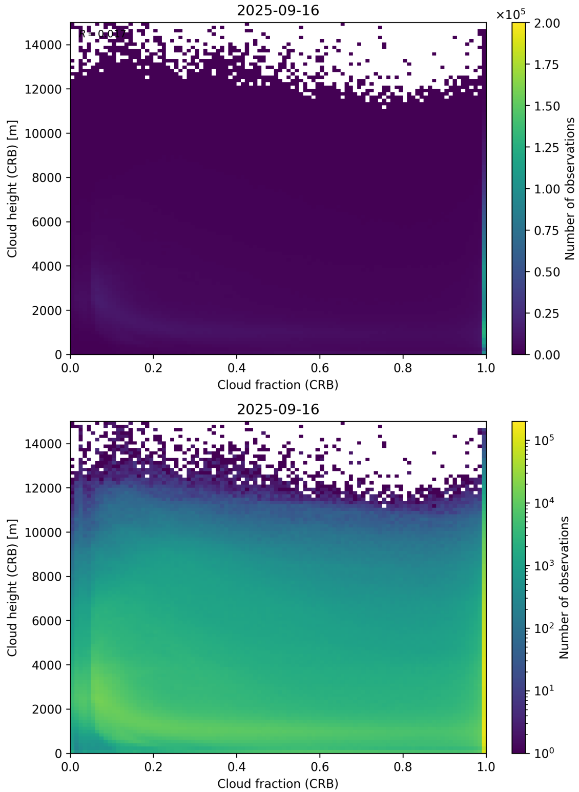
Figure 79: Scatter density plot of “Cloud fraction (CRB)” against “Cloud height (CRB)” for 2025-09-15 to 2025-09-17.
