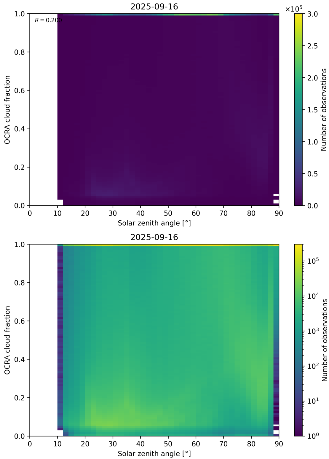
Figure 100: Scatter density plot of “Solar zenith angle” against “OCRA cloud fraction” for 2025-09-15 to 2025-09-17.
