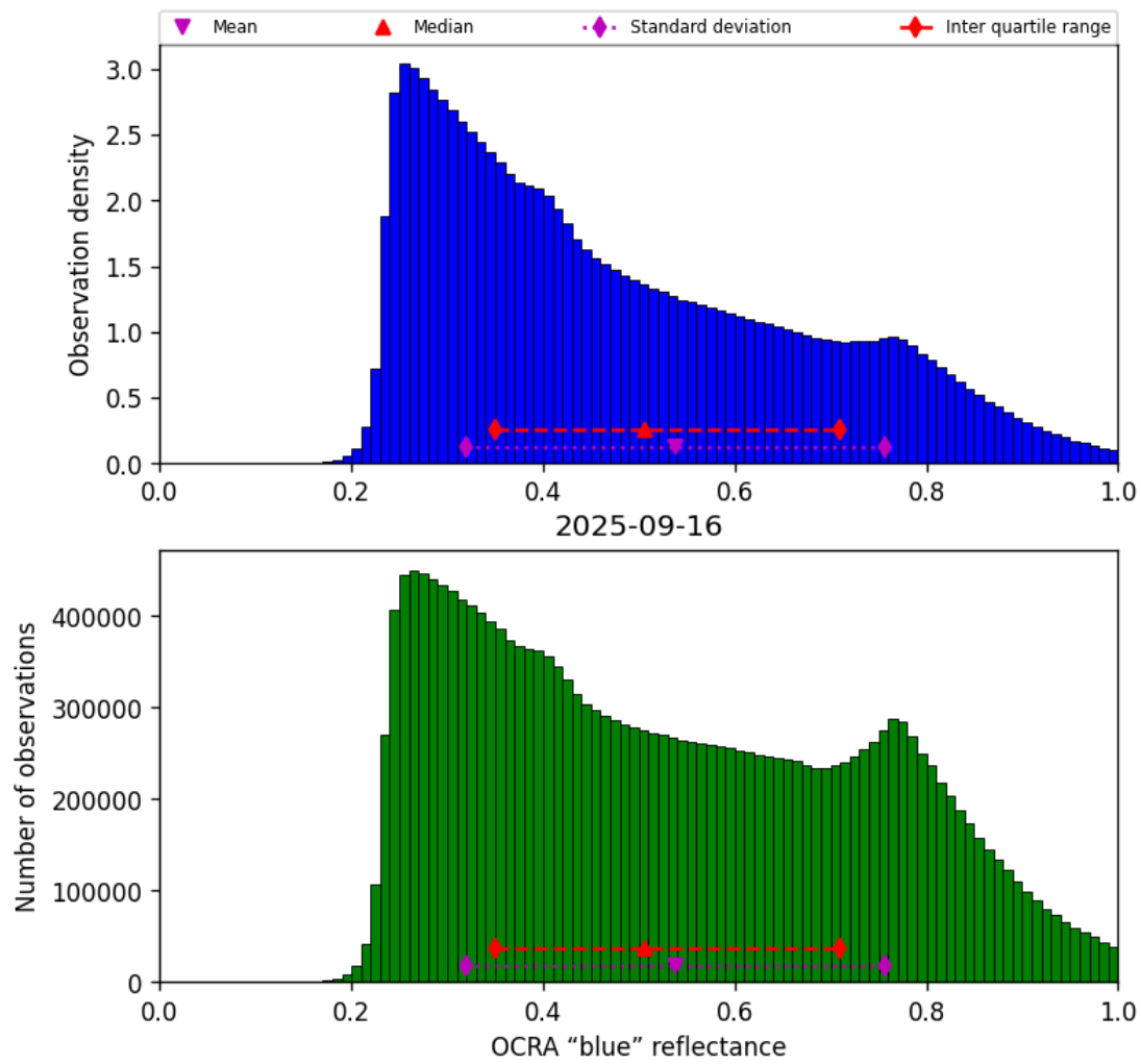
Figure 51: Histogram of “OCRA “blue” reflectance” for 2025-09-15 to 2025-09-17
