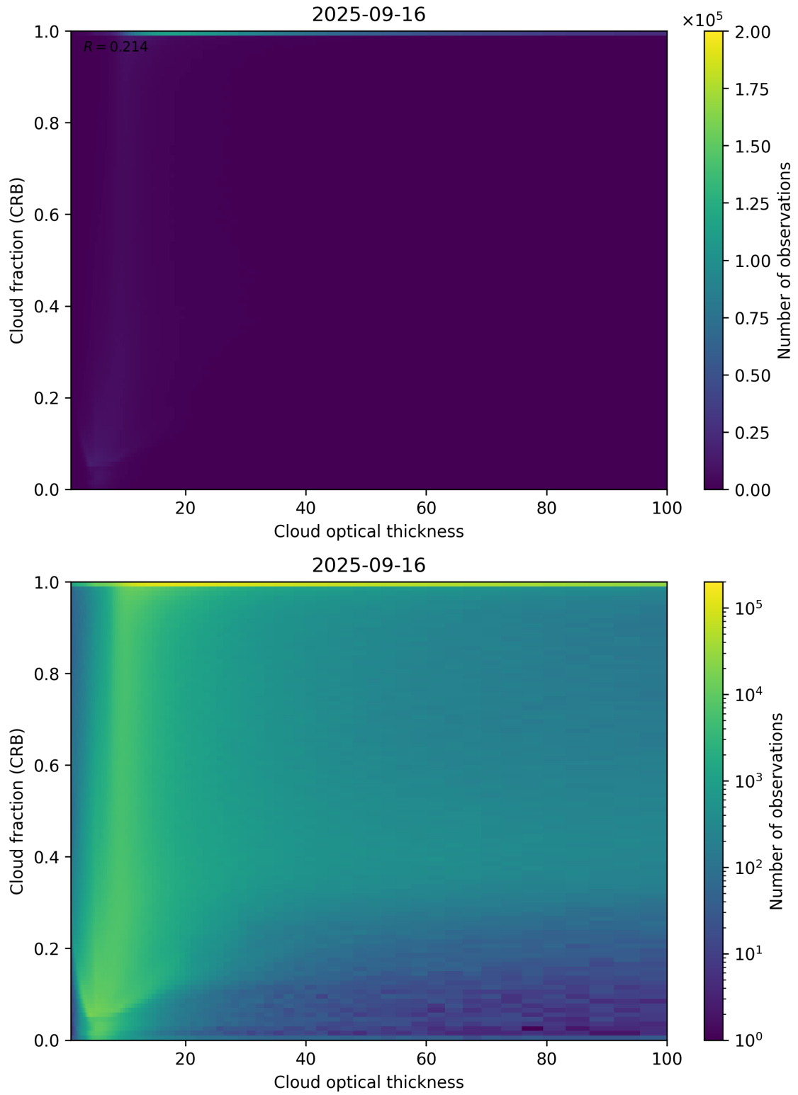
Figure 84: Scatter density plot of “Cloud optical thickness” against “Cloud fraction (CRB)” for 2025-09-15 to 2025-09-17.
