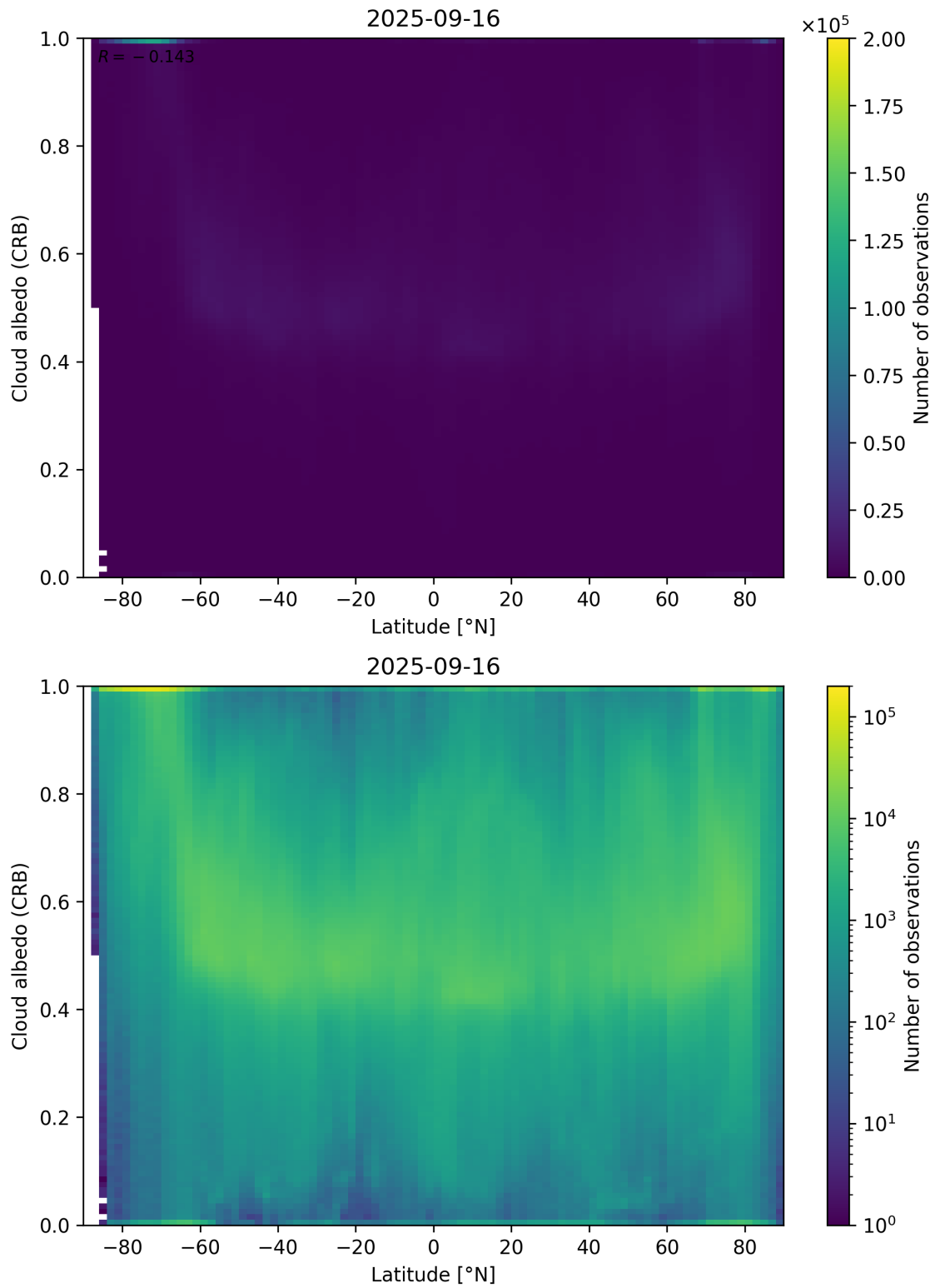
Figure 91: Scatter density plot of “Latitude” against “Cloud albedo (CRB)” for 2025-09-15 to 2025-09-17.
