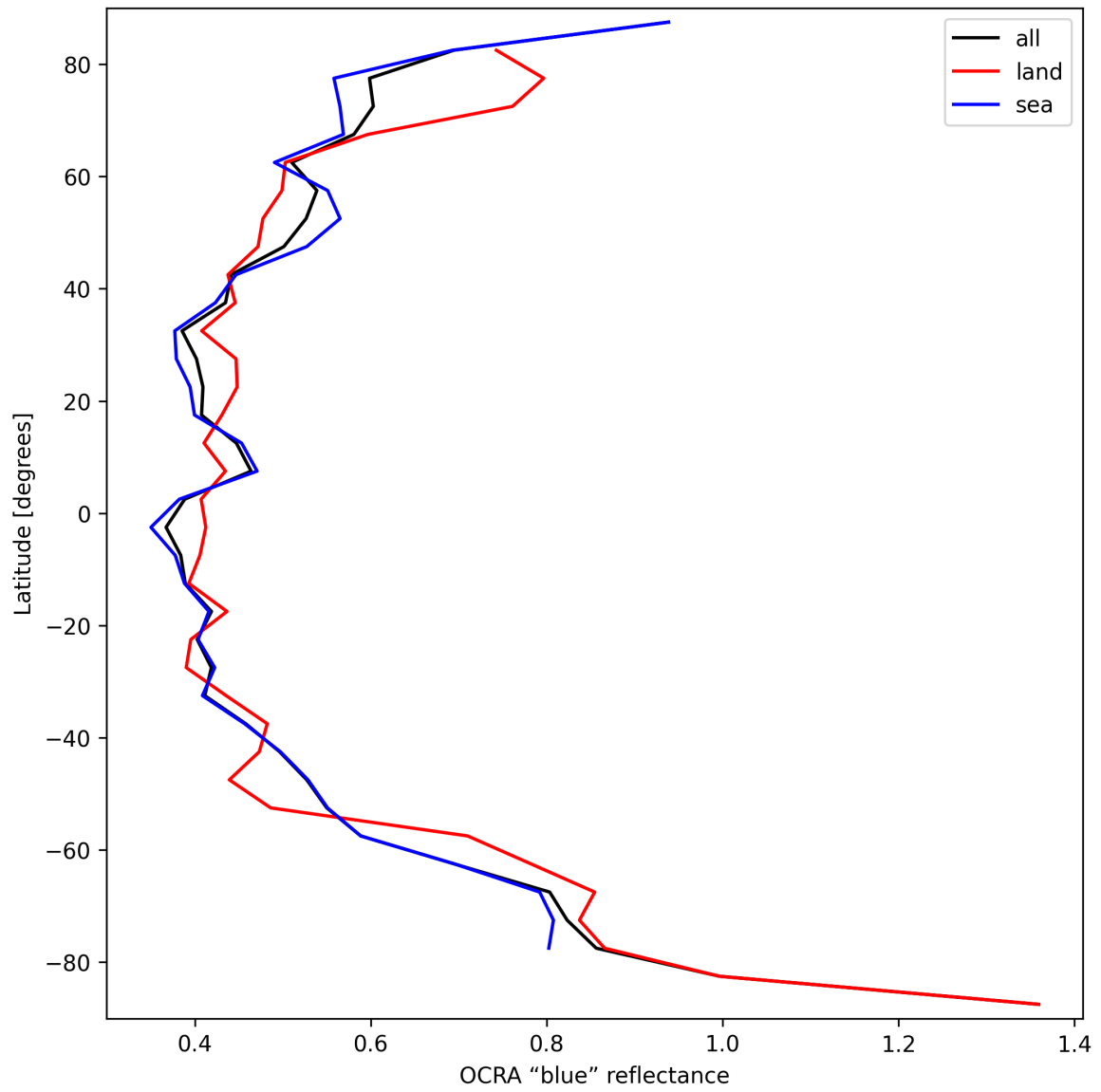
Figure 35: Zonal average of "OCRA "blue" reflectance" for 2025-09-15 to 2025-09-17.
