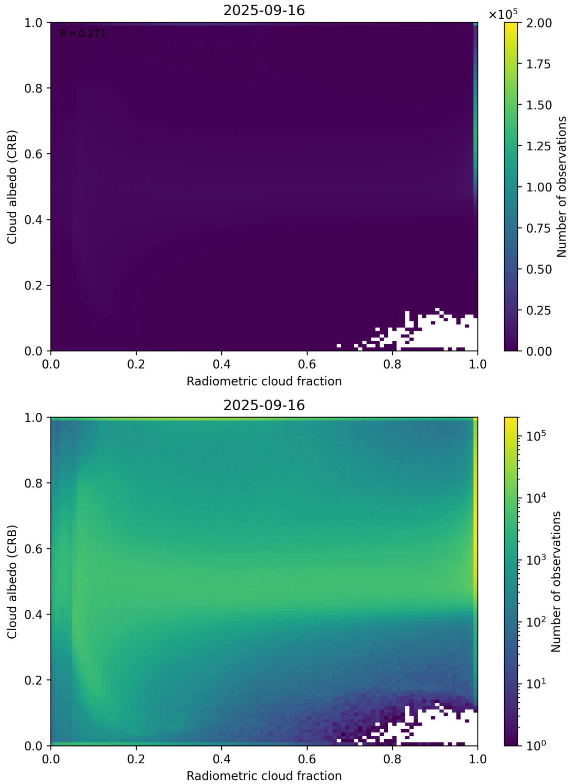
Figure 71: Scatter density plot of “Radiometric cloud fraction” against “Cloud albedo (CRB)” for 2025-09-15 to 2025-09-17.
