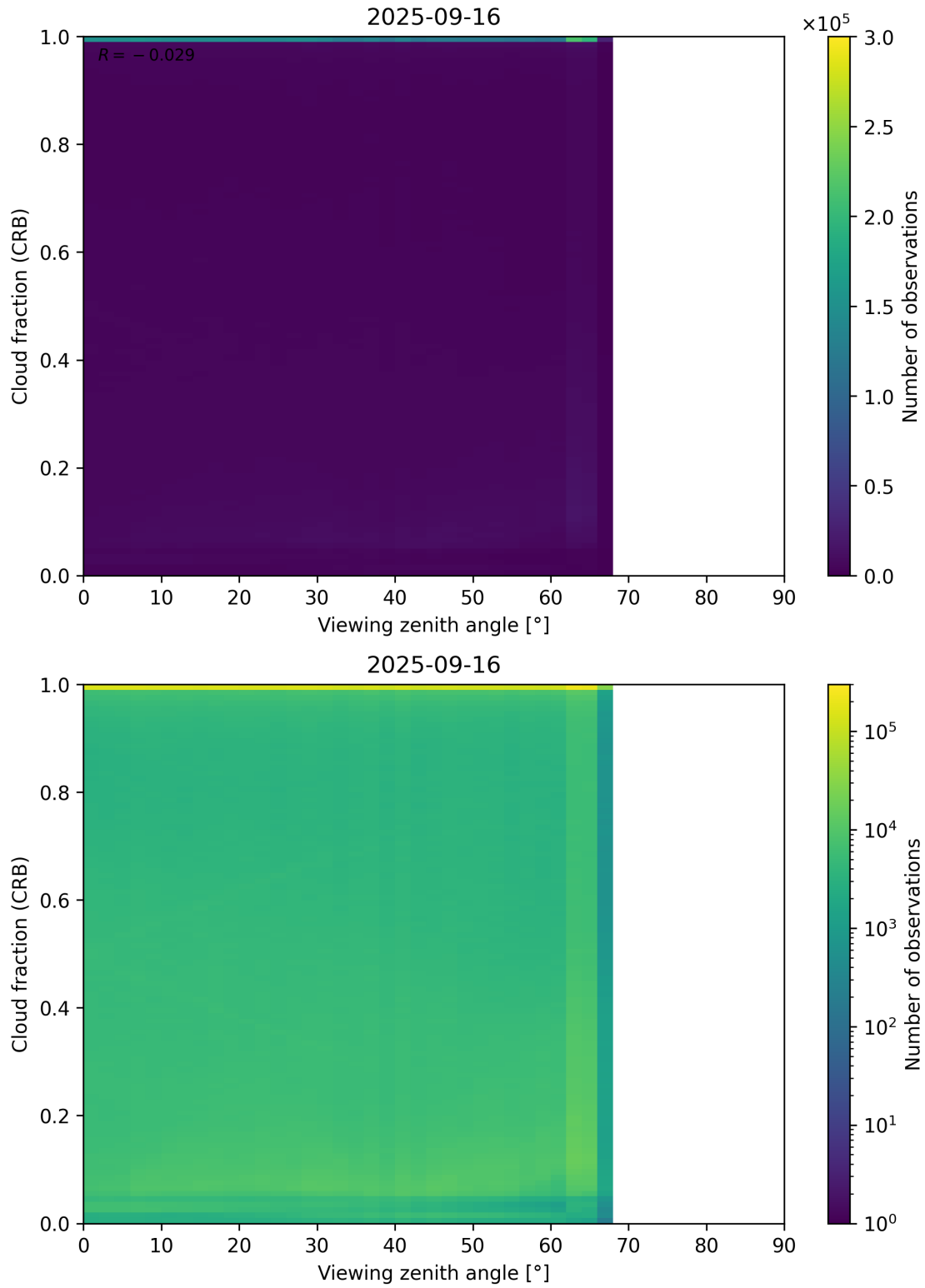
Figure 109: Scatter density plot of “Viewing zenith angle” against “Cloud fraction (CRB)” for 2025-09-15 to 2025-09-17.
