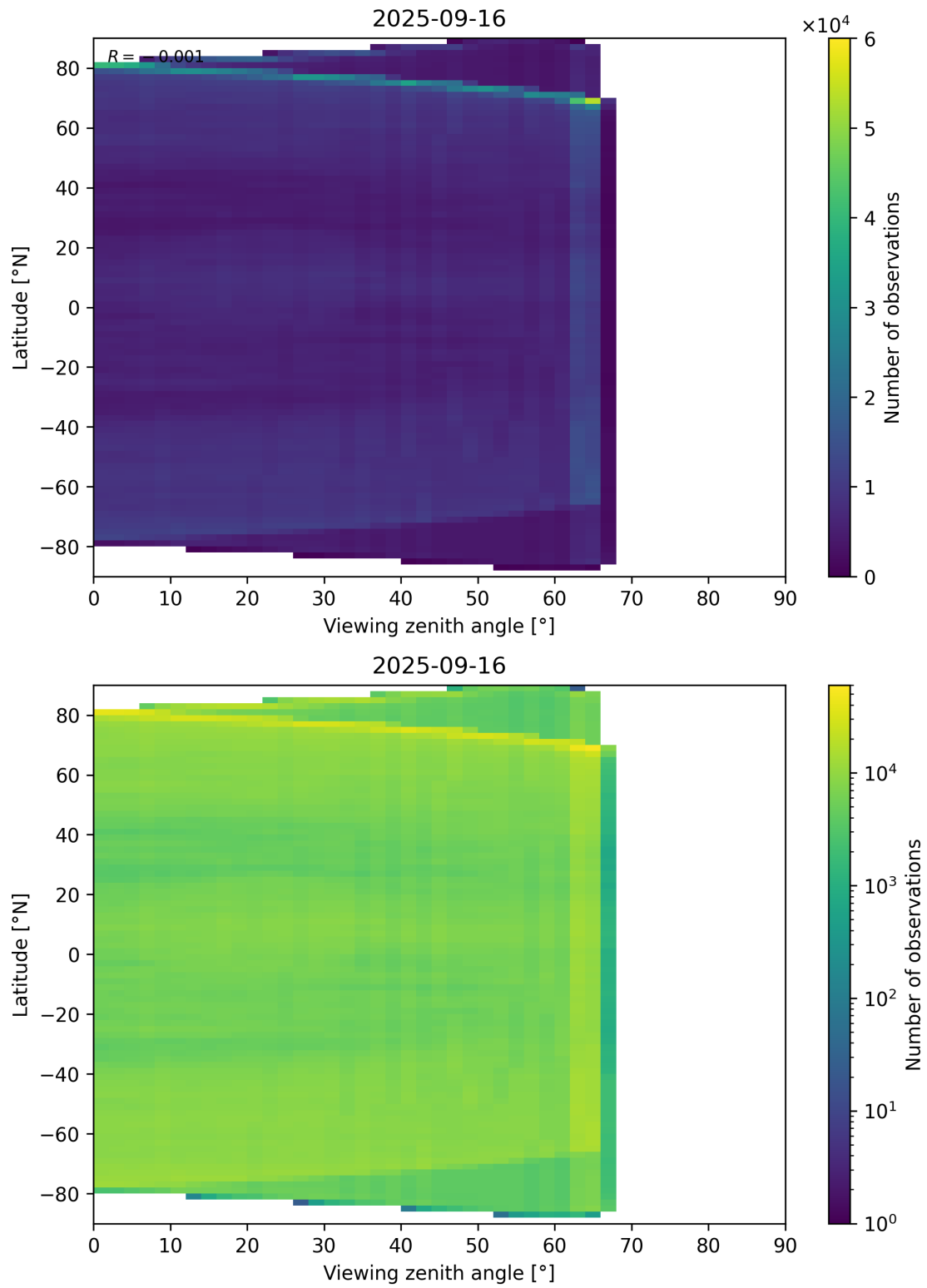
Figure 113: Scatter density plot of “Viewing zenith angle” against “Latitude” for 2025-09-15 to 2025-09-17.
