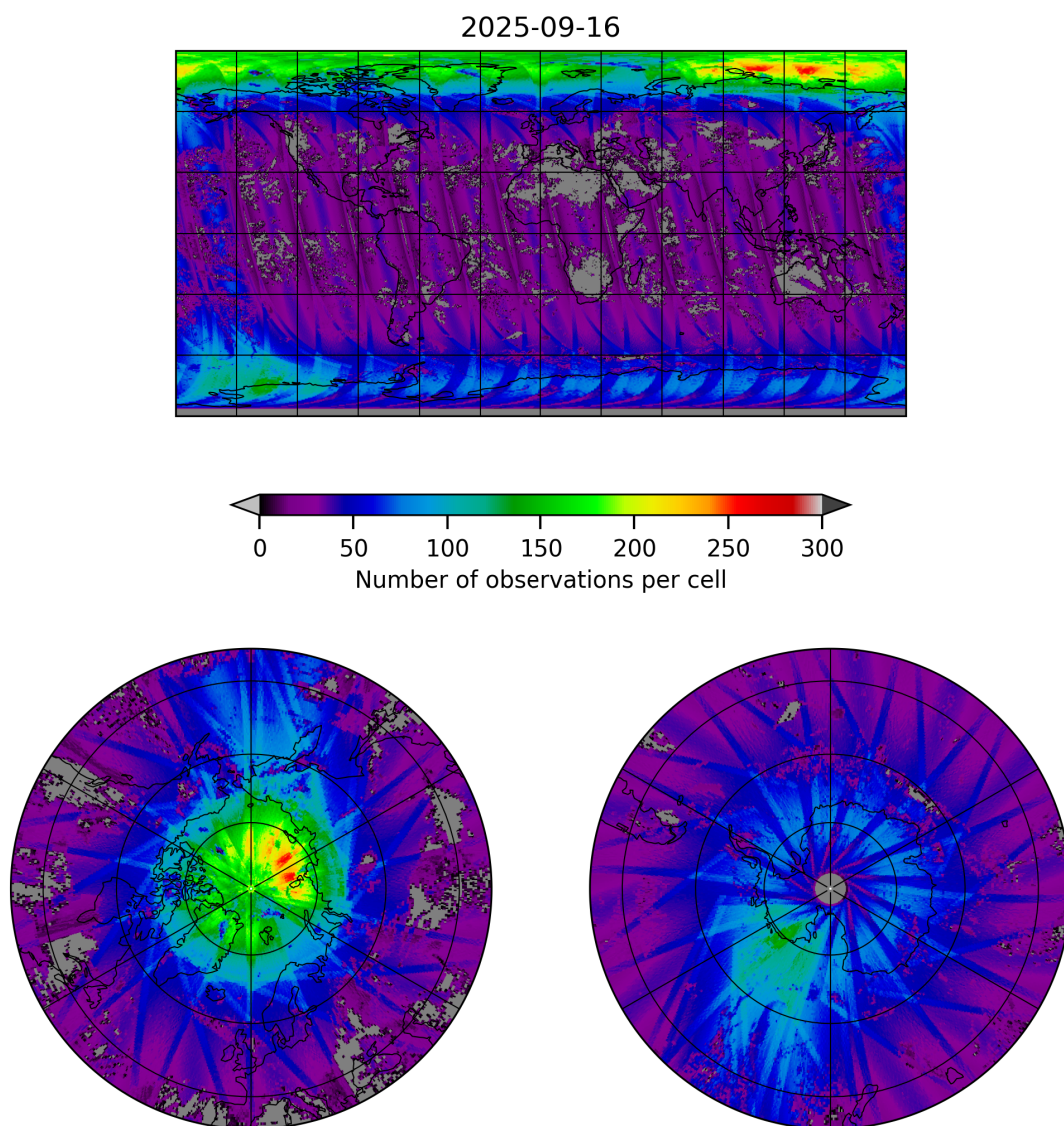
Figure 21: Map of the number of observations for 2025-09-15 to 2025-09-17
