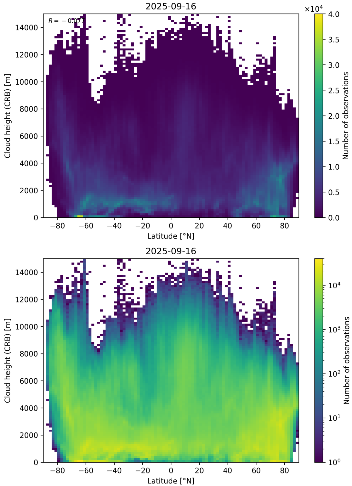
Figure 95: Scatter density plot of “Latitude” against “Cloud height (CRB)” for 2025-09-15 to 2025-09-17.
