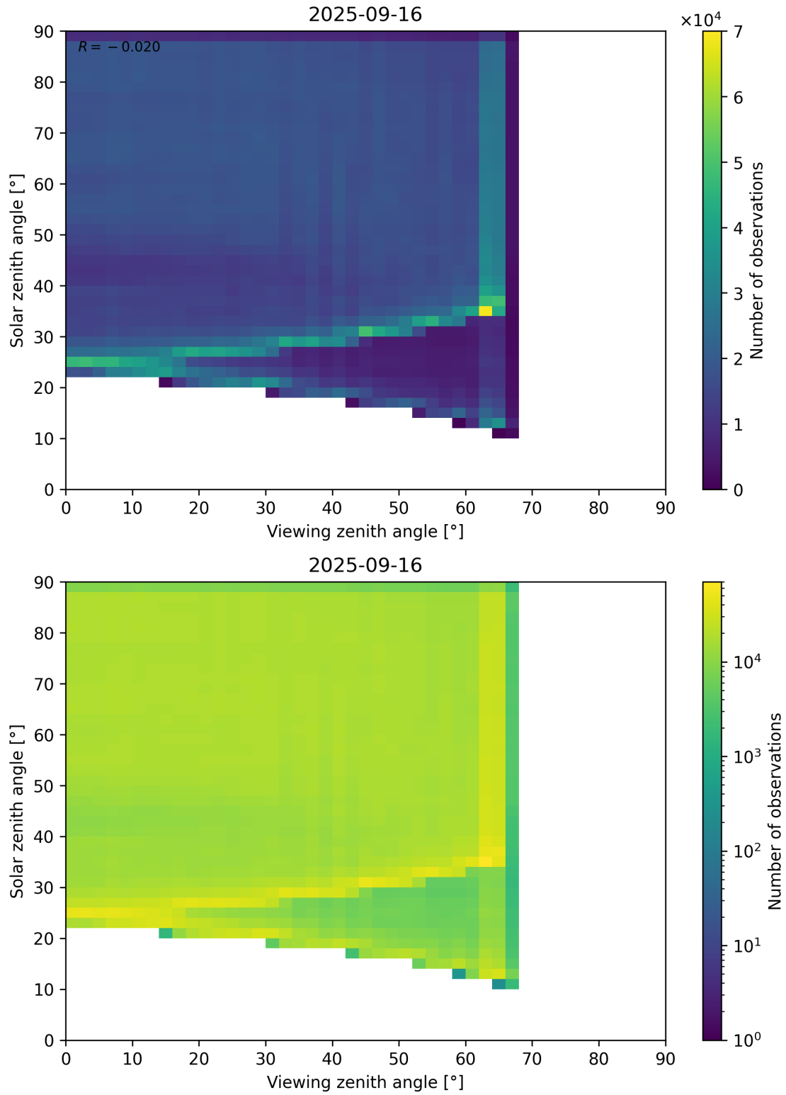
Figure 114: Scatter density plot of “Viewing zenith angle” against “Solar zenith angle” for 2025-09-15 to 2025-09-17.
