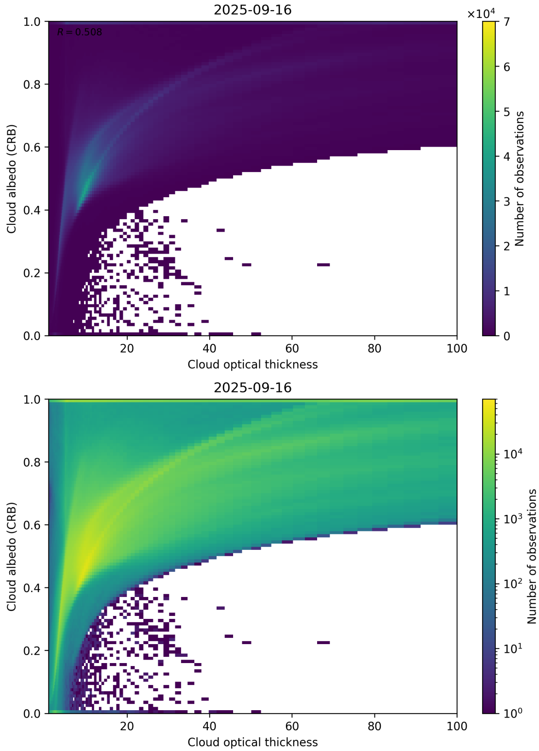
Figure 82: Scatter density plot of “Cloud optical thickness” against “Cloud albedo (CRB)” for 2025-09-15 to 2025-09-17.
