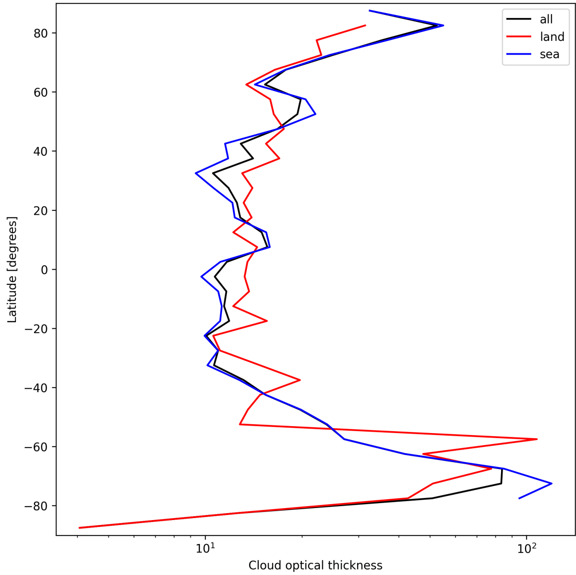
Figure 25: Zonal average of “Cloud optical thickness” for 2025-09-15 to 2025-09-17.
