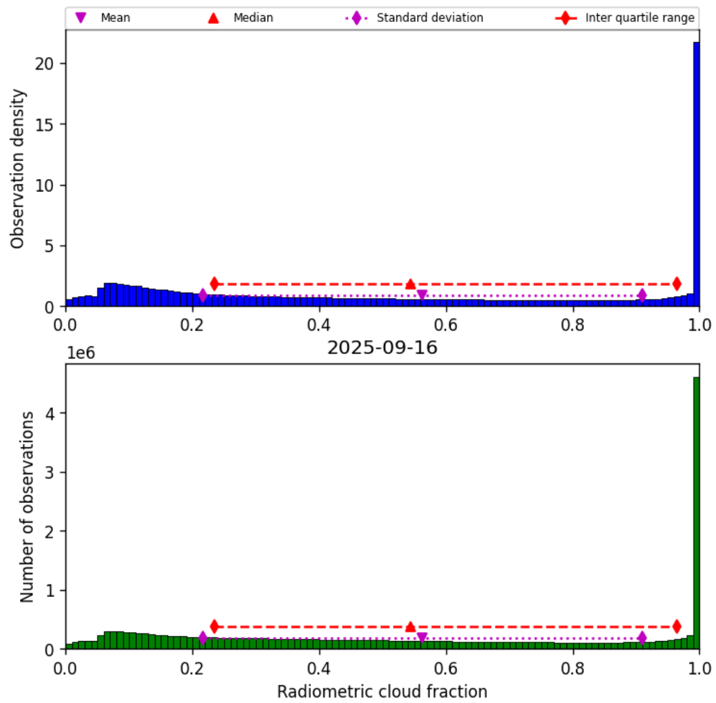
Figure 39: Histogram of “Radiometric cloud fraction” for 2025-09-15 to 2025-09-17
