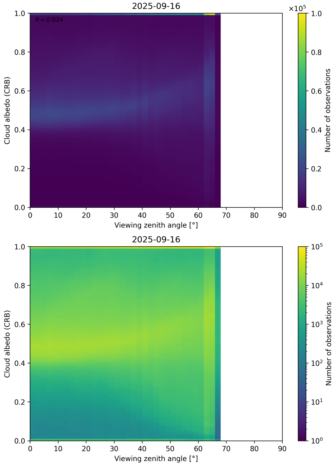
Figure 106: Scatter density plot of “Viewing zenith angle” against “Cloud albedo (CRB)” for 2025-09-15 to 2025-09-17.
