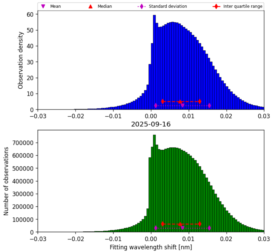
Figure 49: Histogram of “Fitting wavelength shift” for 2025-09-15 to 2025-09-17
