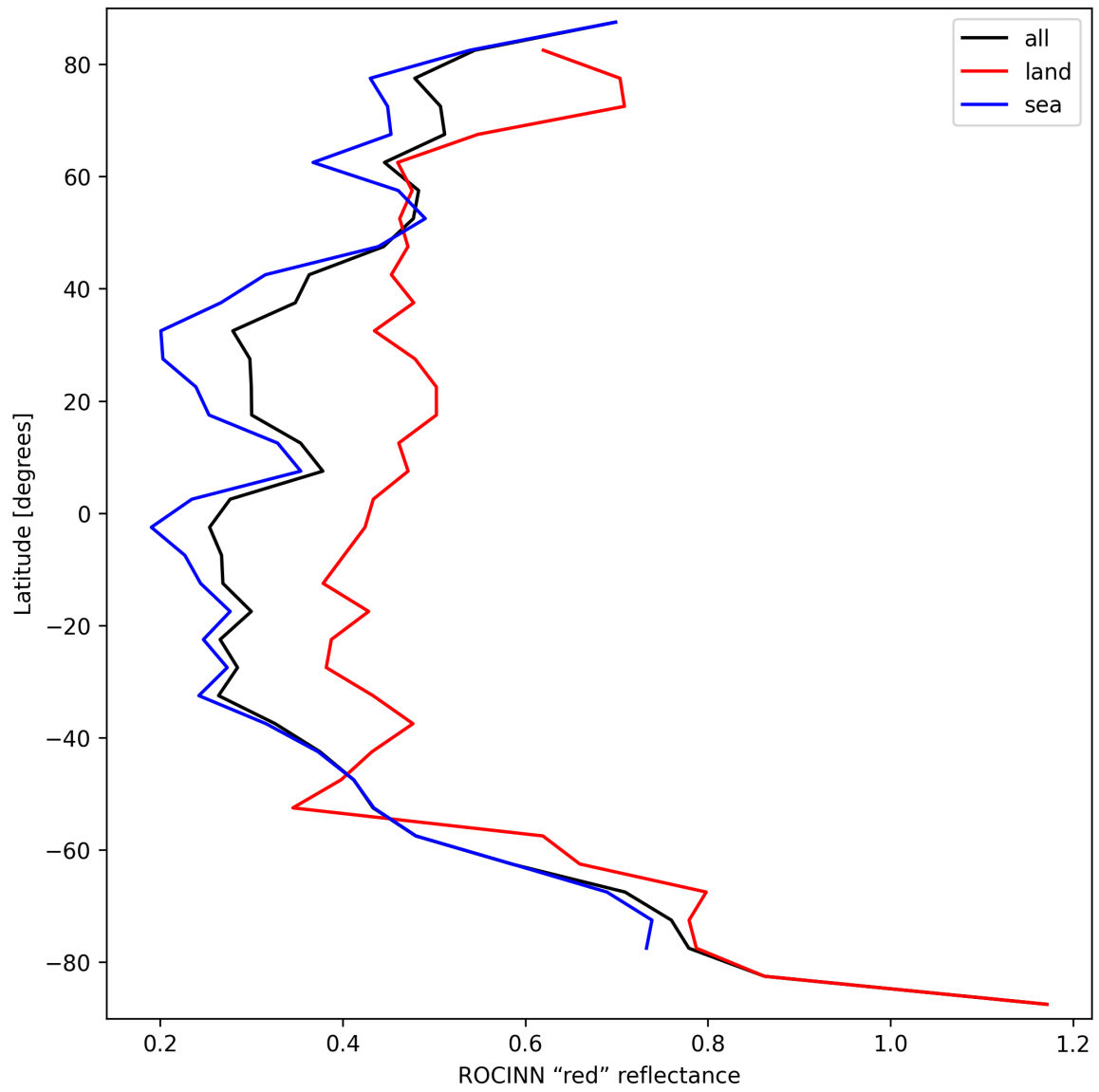
Figure 37: Zonal average of “ROCINN “red” reflectance” for 2025-09-15 to 2025-09-17.
