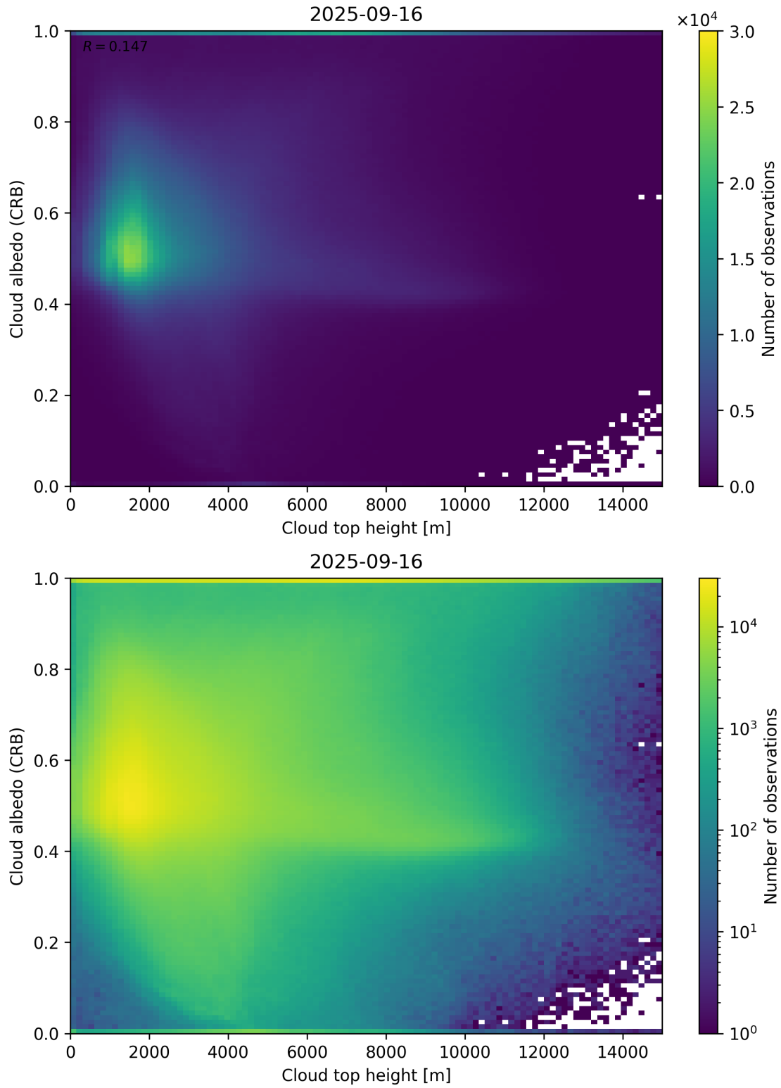
Figure 86: Scatter density plot of “Cloud top height” against “Cloud albedo (CRB)” for 2025-09-15 to 2025-09-17.
