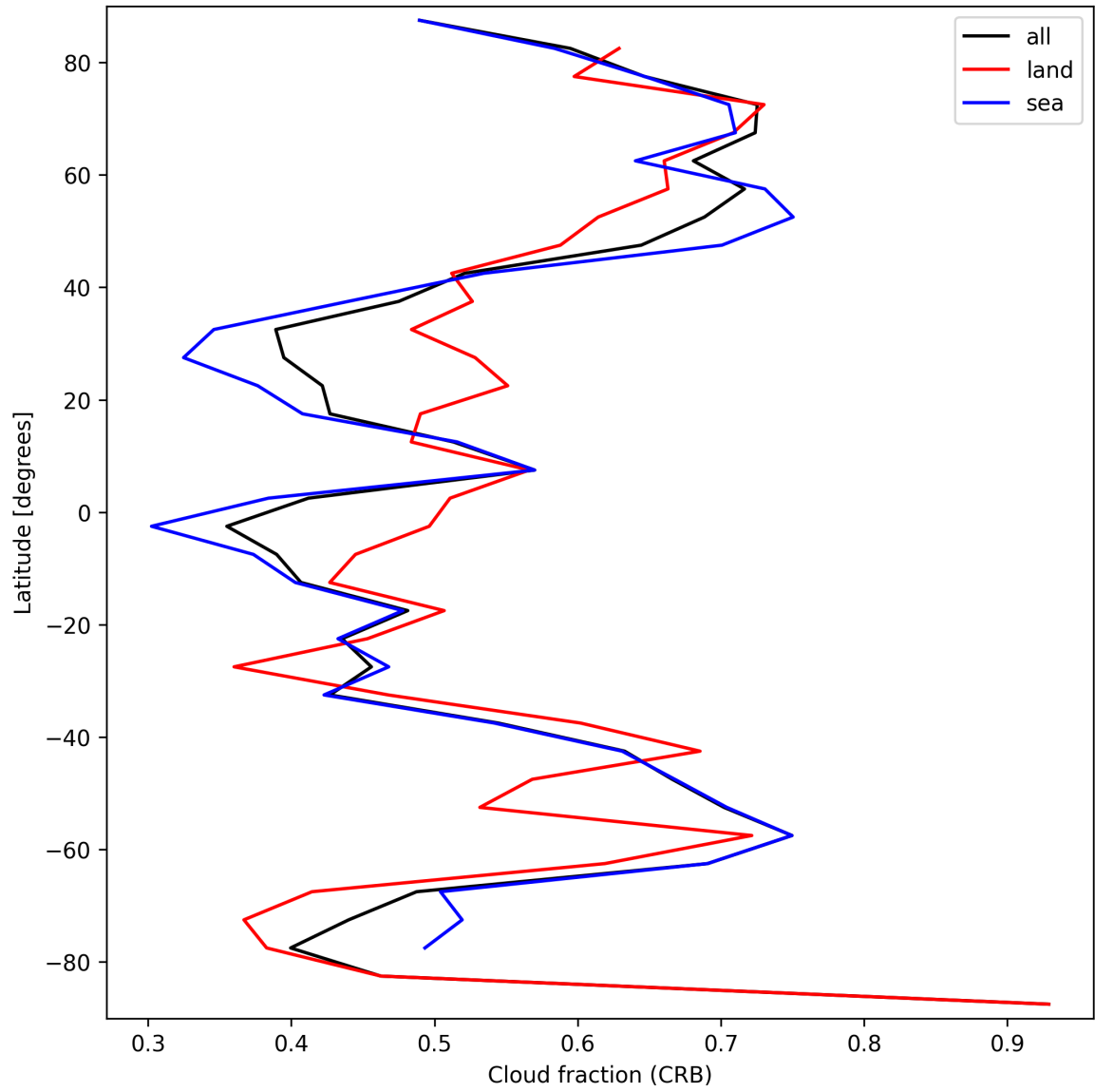
Figure 26: Zonal average of “Cloud fraction (CRB)” for 2025-09-15 to 2025-09-17.
