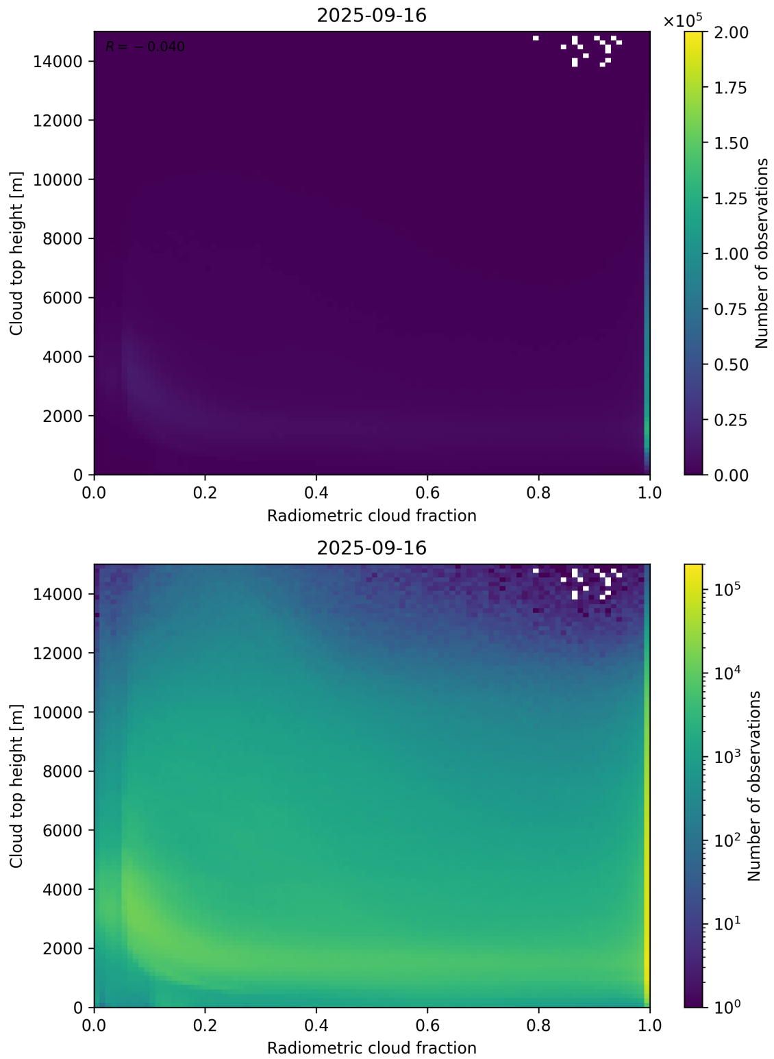
Figure 76: Scatter density plot of “Radiometric cloud fraction” against “Cloud top height” for 2025-09-15 to 2025-09-17.
