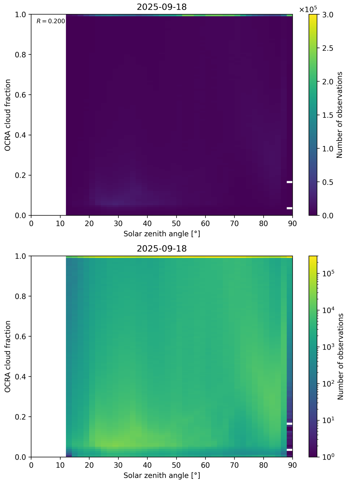
Figure 100: Scatter density plot of “Solar zenith angle” against “OCRA cloud fraction” for 2025-09-17 to 2025-09-19.
