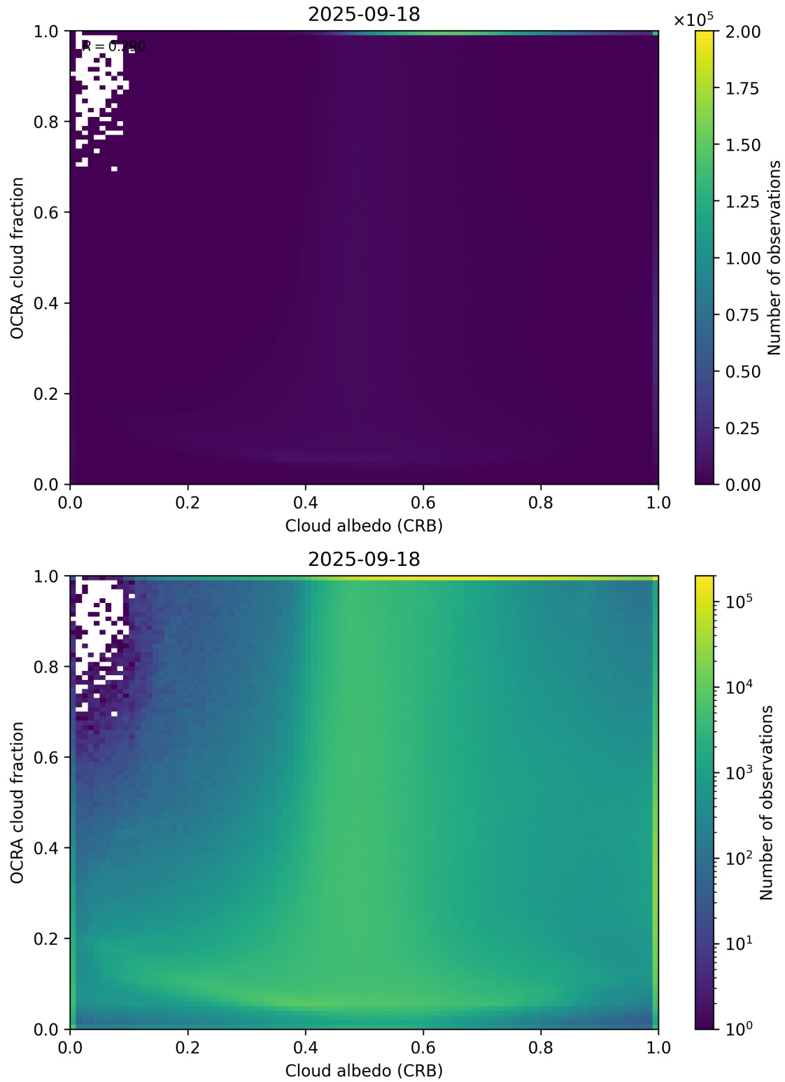
Figure 70: Scatter density plot of “Cloud albedo (CRB)” against “OCRA cloud fraction” for 2025-09-17 to 2025-09-19.
