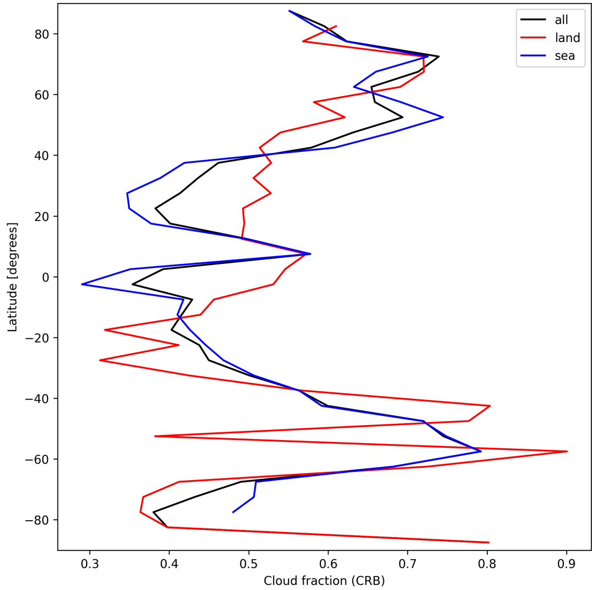
Figure 26: Zonal average of “Cloud fraction (CRB)” for 2025-09-17 to 2025-09-19.
