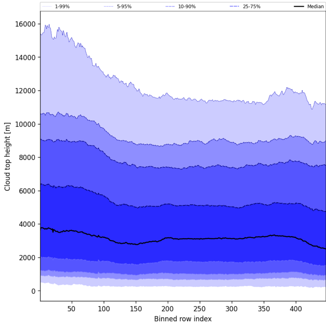
Figure 56: Along track statistics of “Cloud top height” for 2025-09-17 to 2025-09-19
