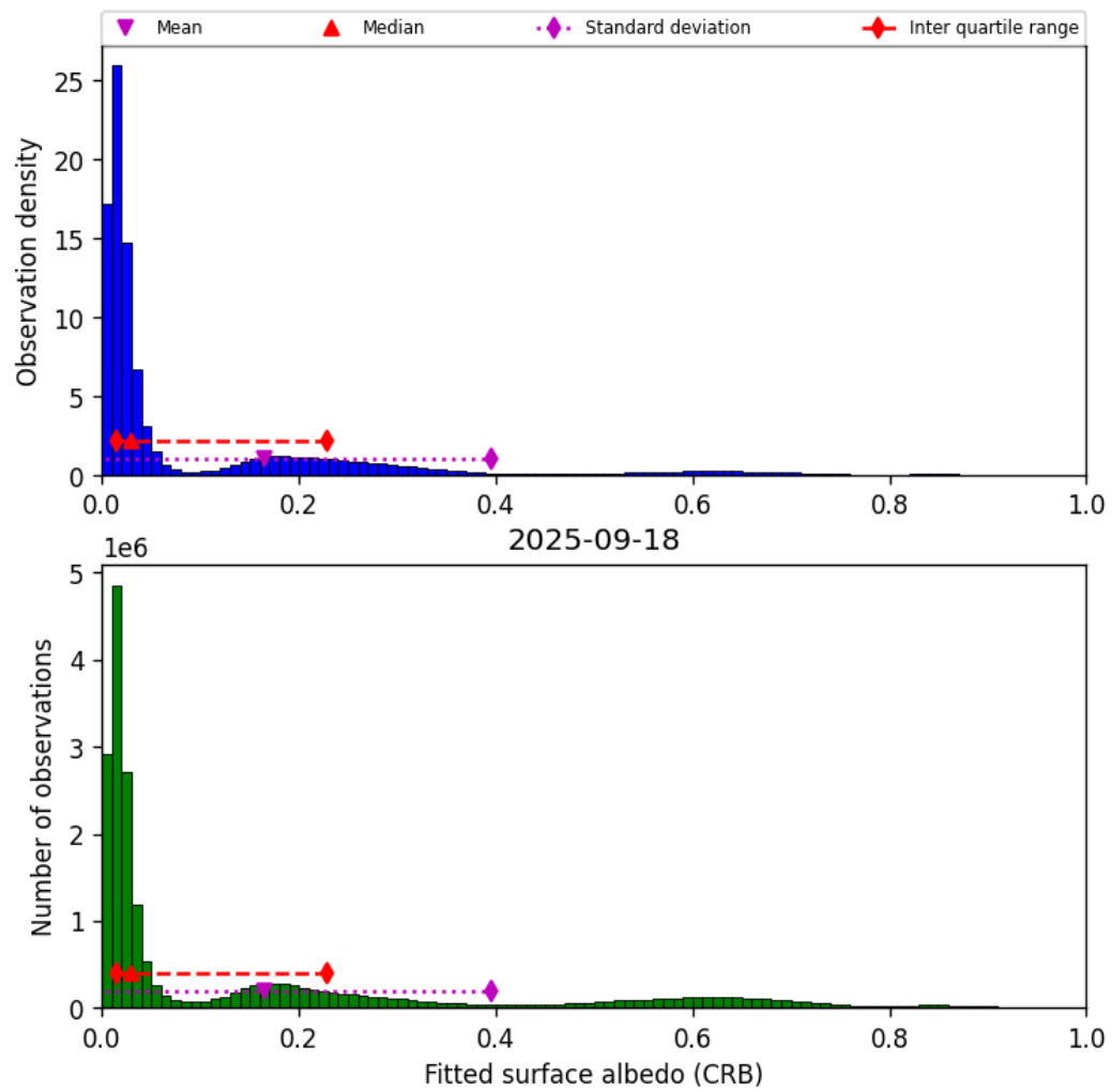
Figure 46: Histogram of “Fitted surface albedo (CRB)” for 2025-09-17 to 2025-09-19
