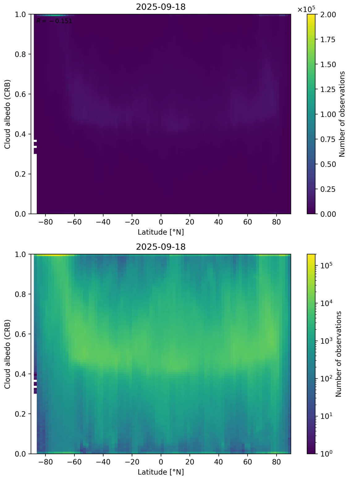
Figure 91: Scatter density plot of “Latitude” against “Cloud albedo (CRB)” for 2025-09-17 to 2025-09-19.
