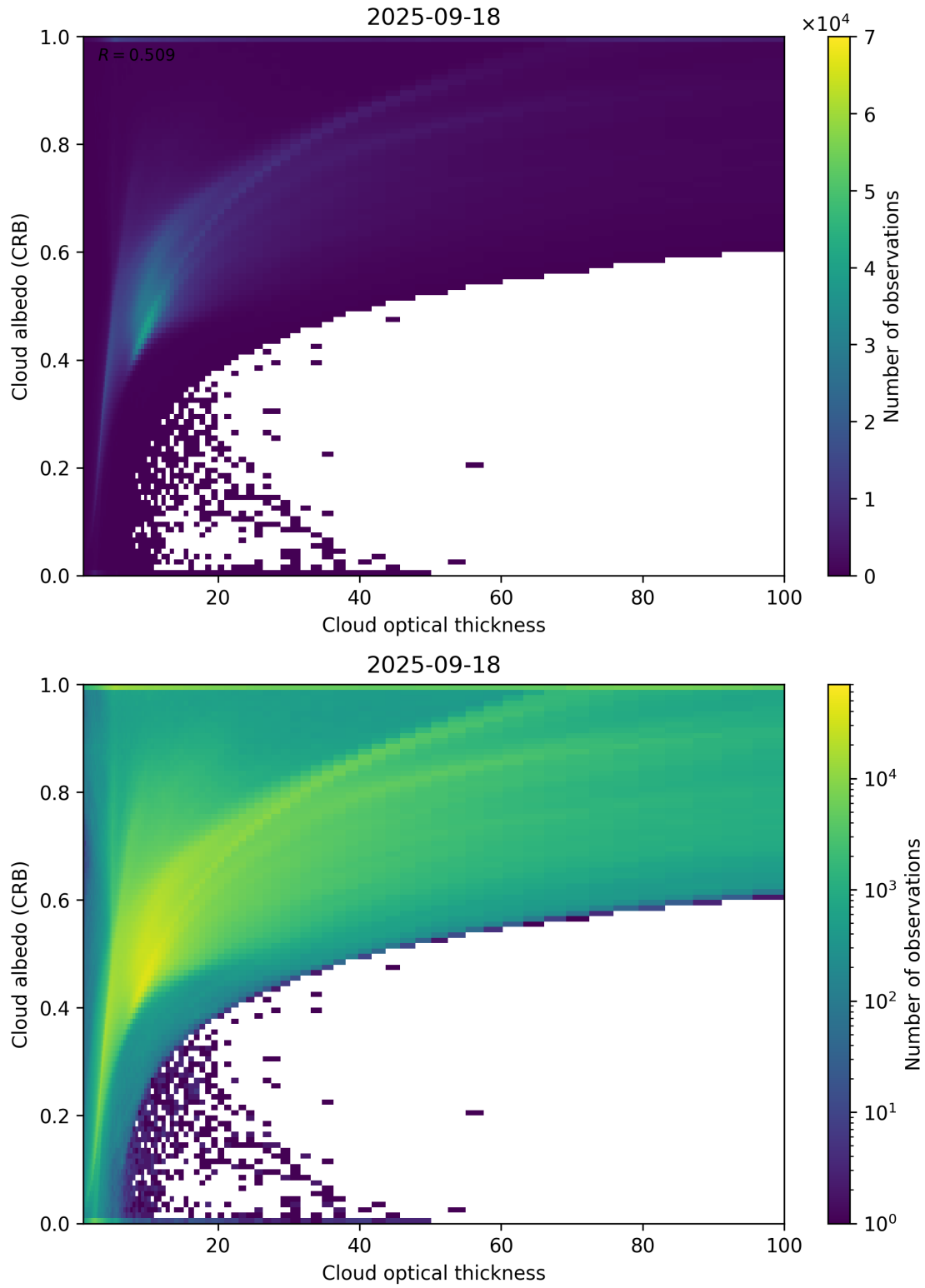
Figure 82: Scatter density plot of “Cloud optical thickness” against “Cloud albedo (CRB)” for 2025-09-17 to 2025-09-19.
