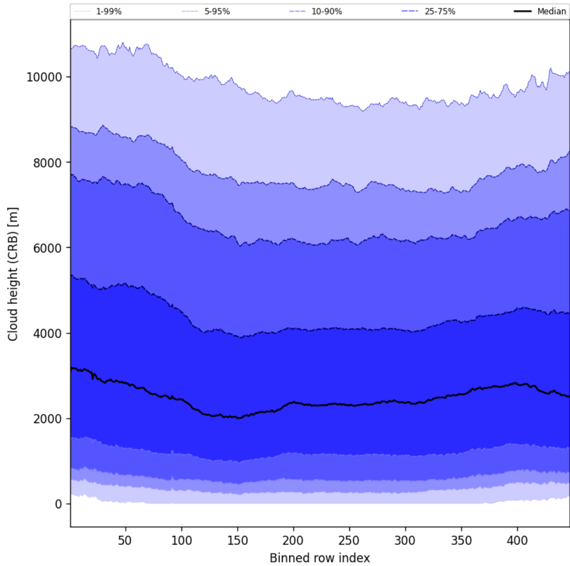
Figure 59: Along track statistics of “Cloud height (CRB)” for 2025-09-17 to 2025-09-19
