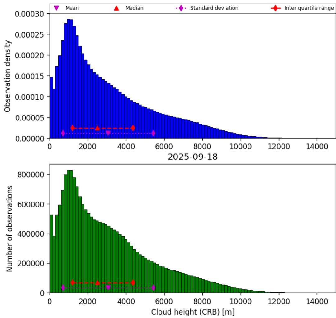
Figure 43: Histogram of “Cloud height (CRB)” for 2025-09-17 to 2025-09-19
