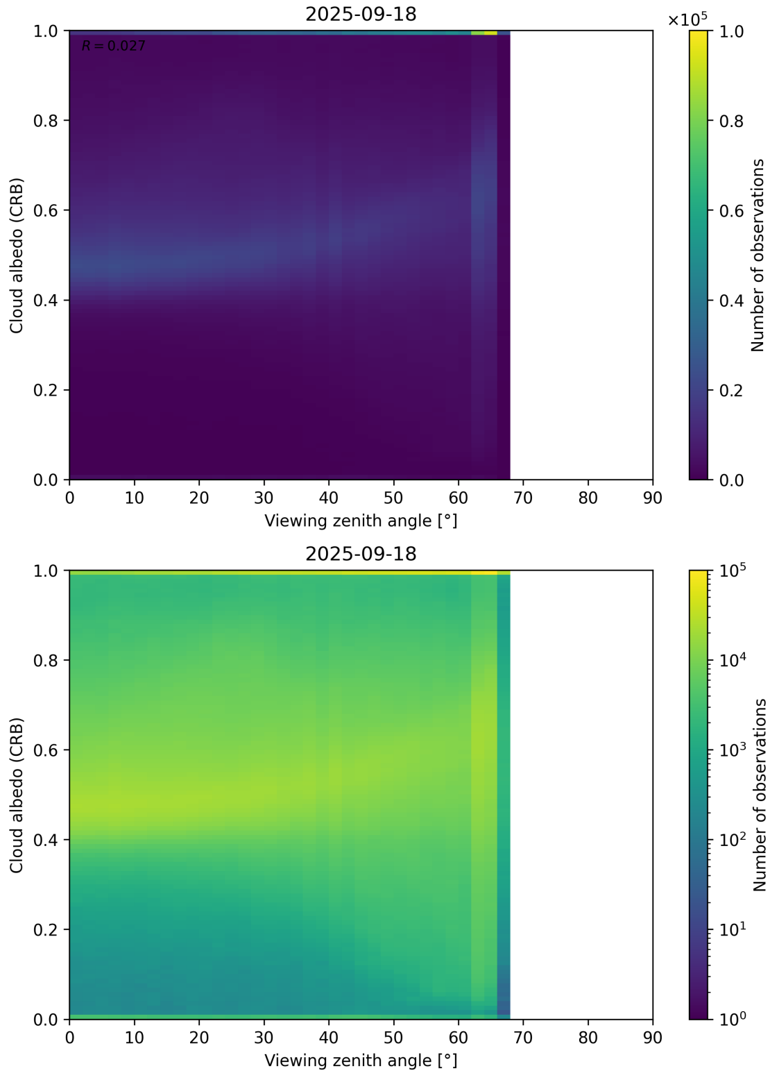
Figure 106: Scatter density plot of “Viewing zenith angle” against “Cloud albedo (CRB)” for 2025-09-17 to 2025-09-19.
