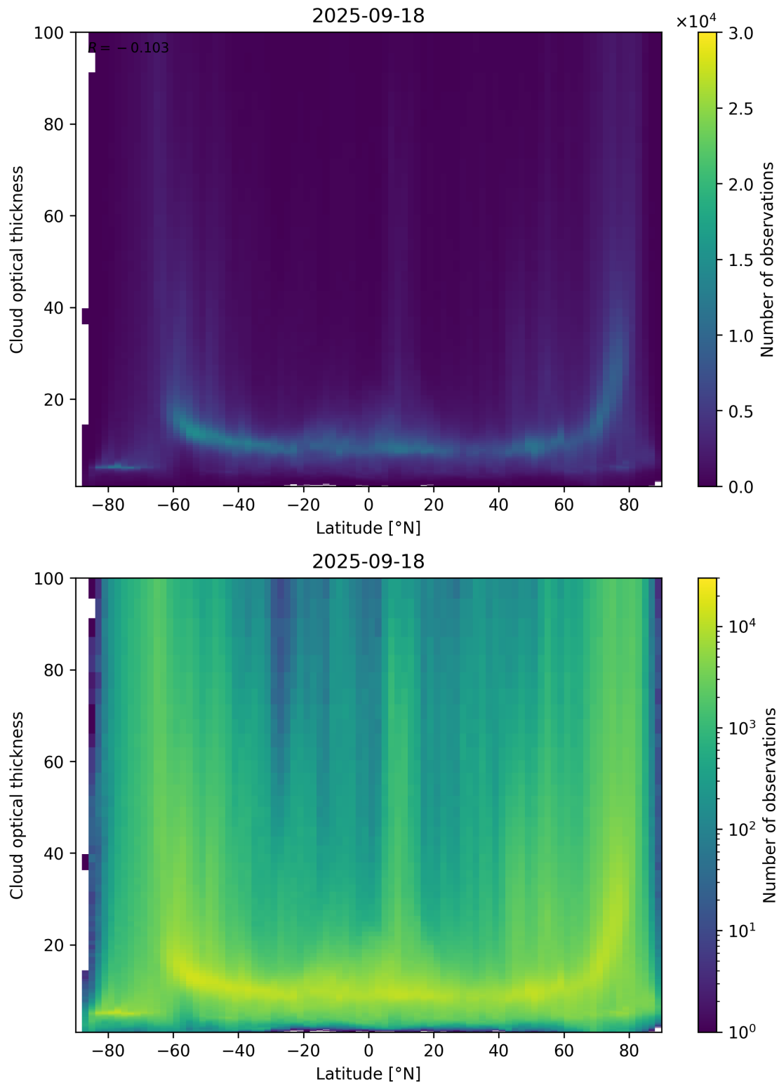
Figure 96: Scatter density plot of “Latitude” against “Cloud optical thickness” for 2025-09-17 to 2025-09-19.
