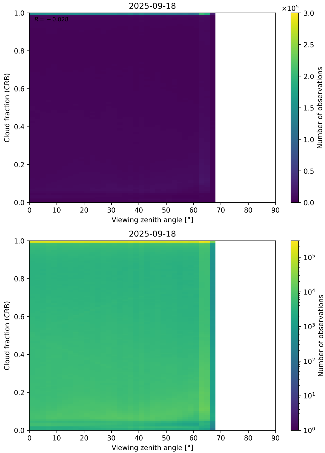
Figure 109: Scatter density plot of “Viewing zenith angle” against “Cloud fraction (CRB)” for 2025-09-17 to 2025-09-19.
