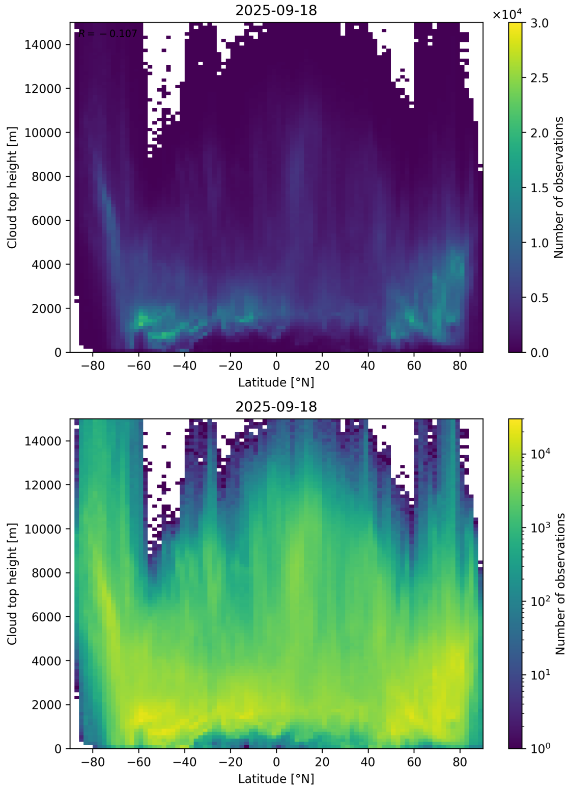
Figure 97: Scatter density plot of “Latitude” against “Cloud top height” for 2025-09-17 to 2025-09-19.
