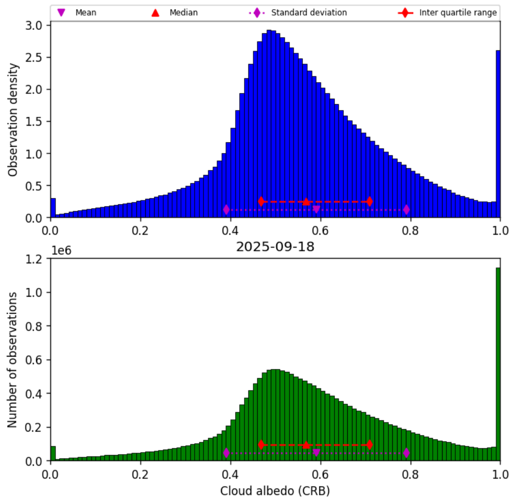
Figure 44: Histogram of “Cloud albedo (CRB)” for 2025-09-17 to 2025-09-19
