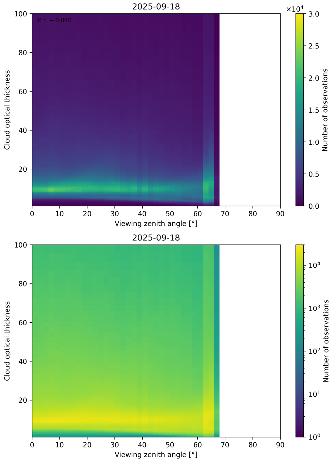
Figure 111: Scatter density plot of “Viewing zenith angle” against “Cloud optical thickness” for 2025-09-17 to 2025-09-19.
