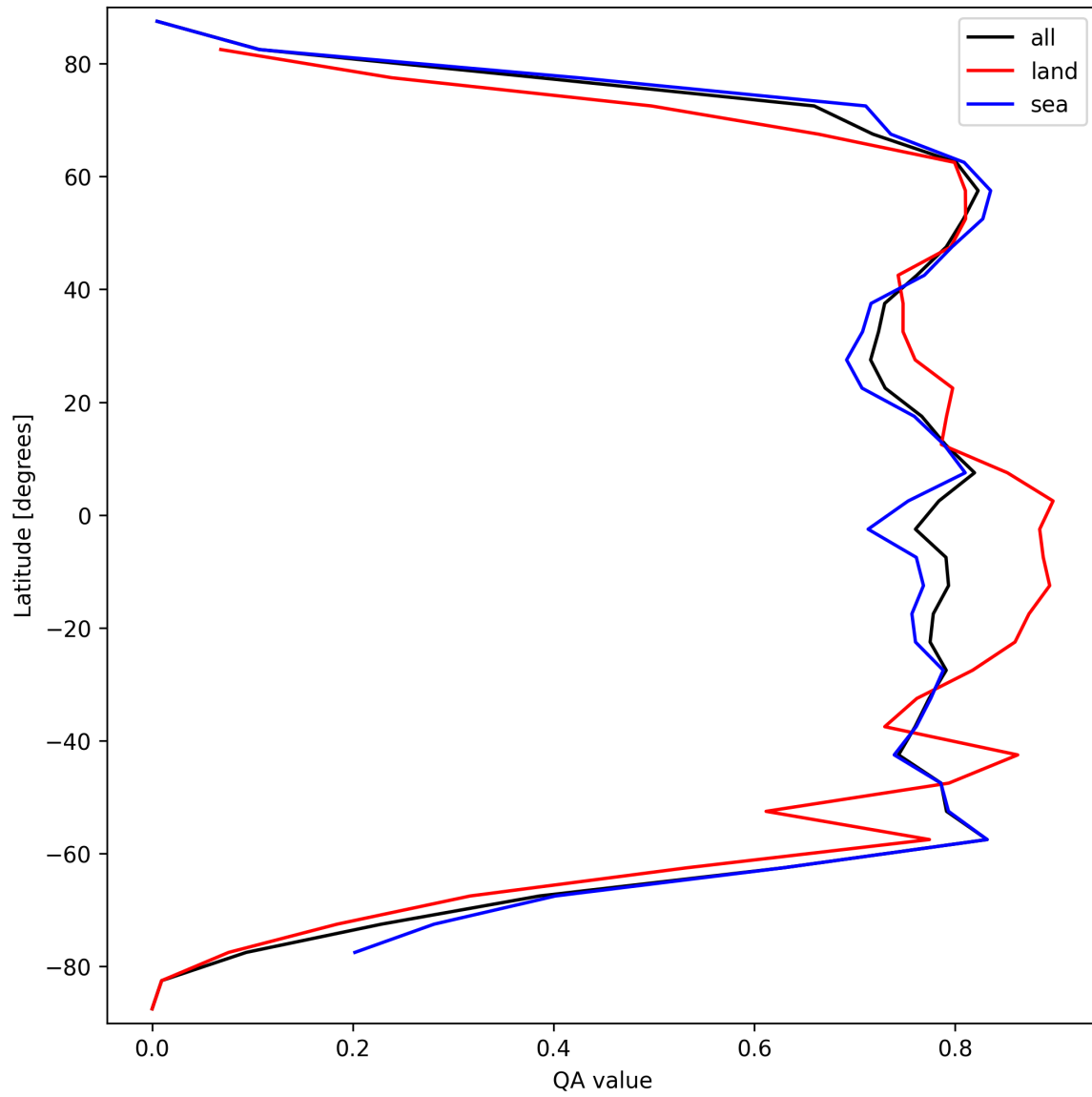
Figure 22: Zonal average of “QA value” for 2025-09-17 to 2025-09-19.
