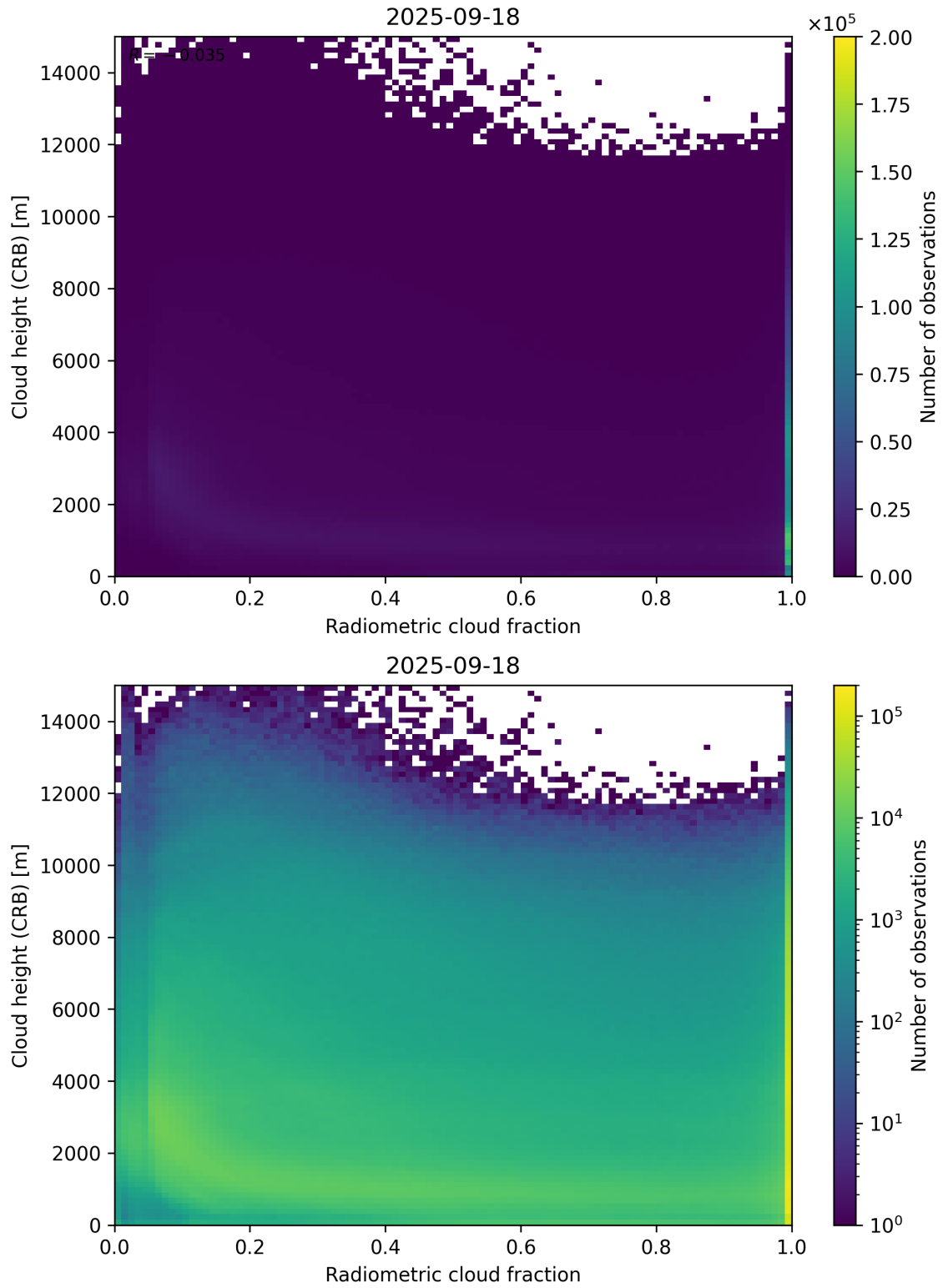
Figure 74: Scatter density plot of “Radiometric cloud fraction” against “Cloud height (CRB)” for 2025-09-17 to 2025-09-19.
