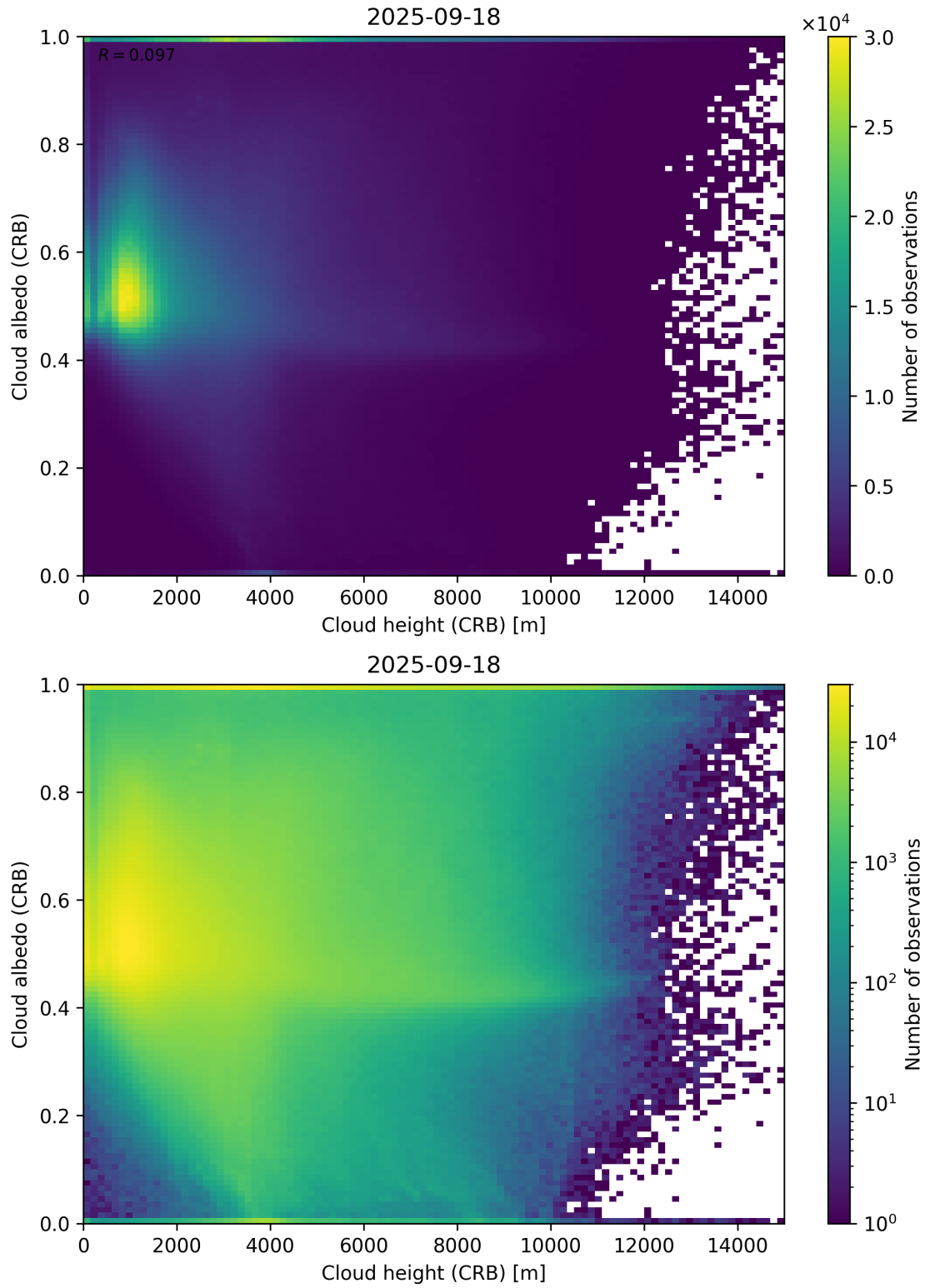
Figure 80: Scatter density plot of “Cloud height (CRB)” against “Cloud albedo (CRB)” for 2025-09-17 to 2025-09-19.
