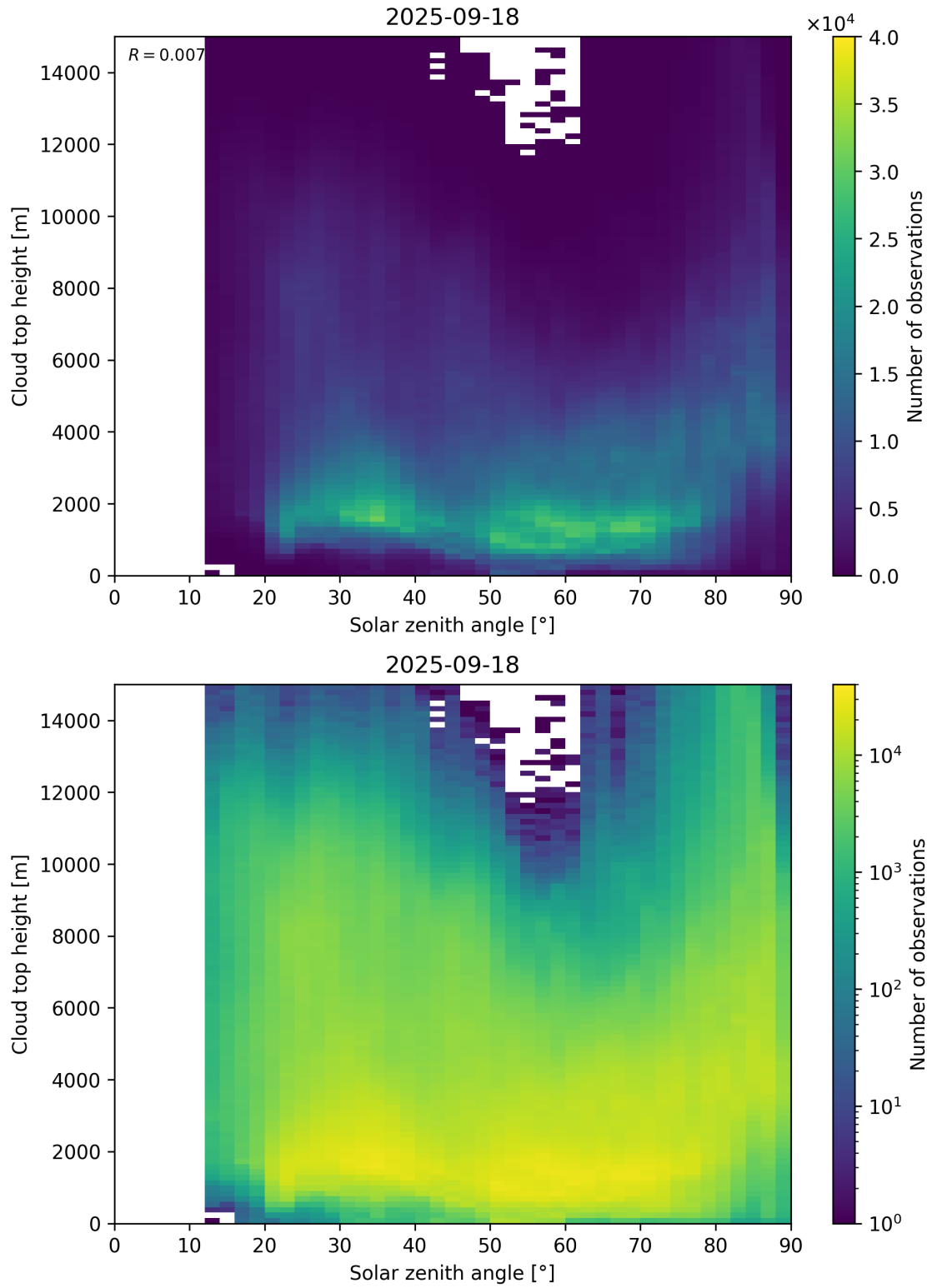
Figure 104: Scatter density plot of “Solar zenith angle” against “Cloud top height” for 2025-09-17 to 2025-09-19.
