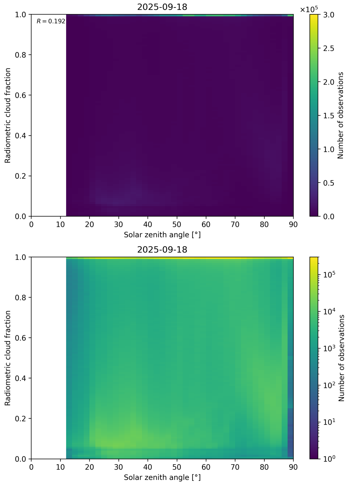
Figure 99: Scatter density plot of “Solar zenith angle” against “Radiometric cloud fraction” for 2025-09-17 to 2025-09-19.
