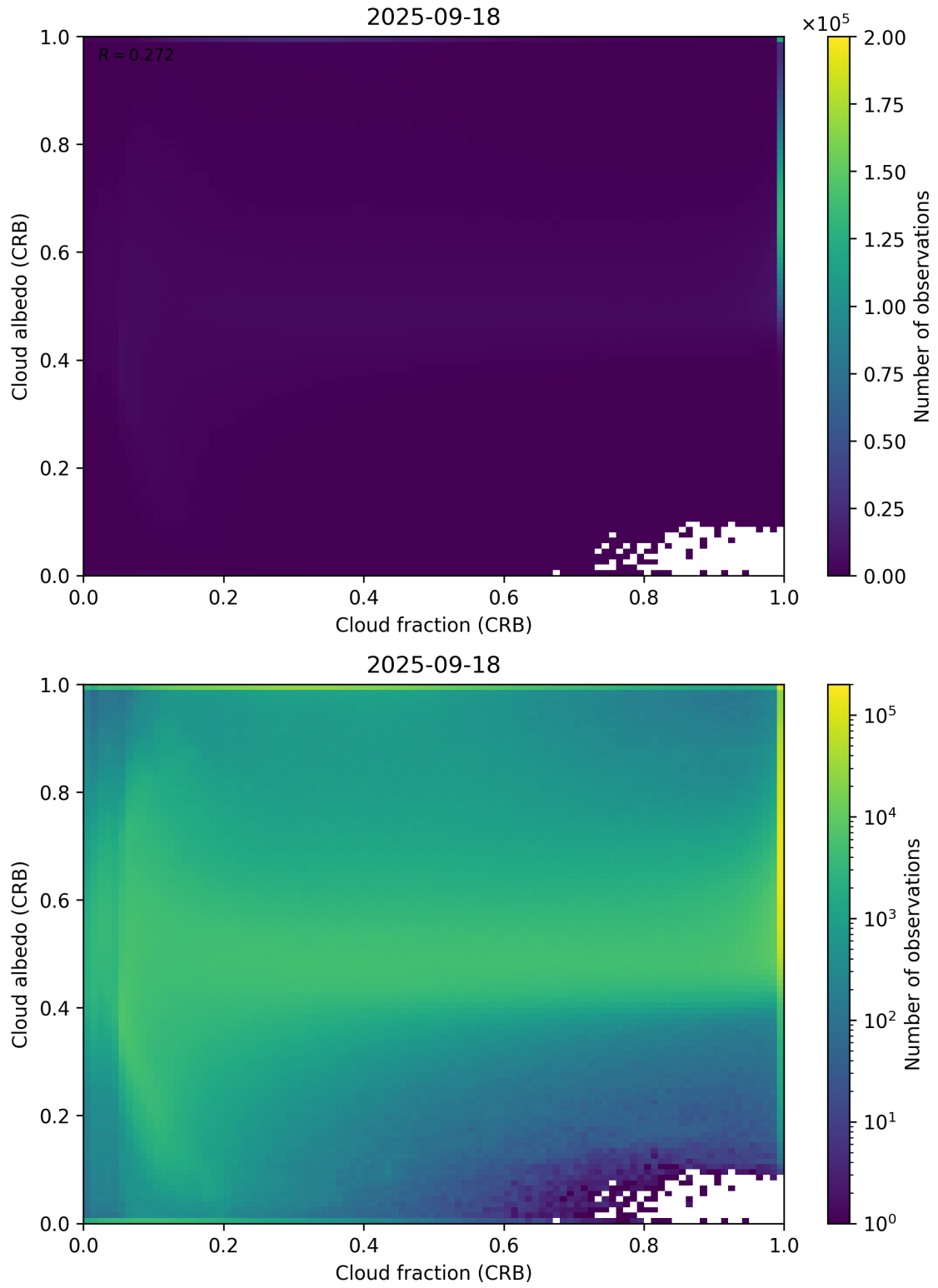
Figure 77: Scatter density plot of “Cloud fraction (CRB)” against “Cloud albedo (CRB)” for 2025-09-17 to 2025-09-19.
