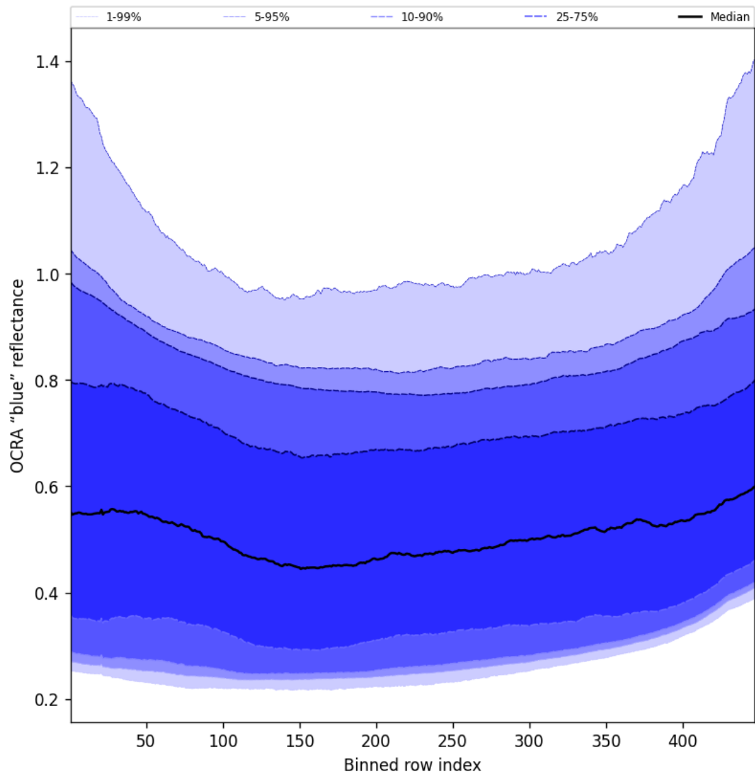
Figure 67: Along track statistics of “OCRA “blue” reflectance” for 2025-09-17 to 2025-09-19
