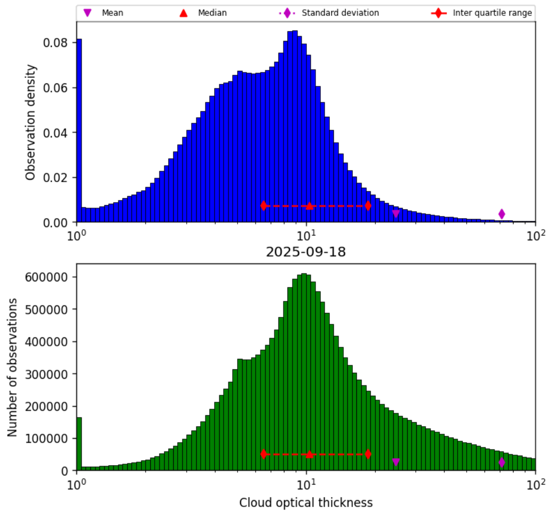
Figure 41: Histogram of “Cloud optical thickness” for 2025-09-17 to 2025-09-19
