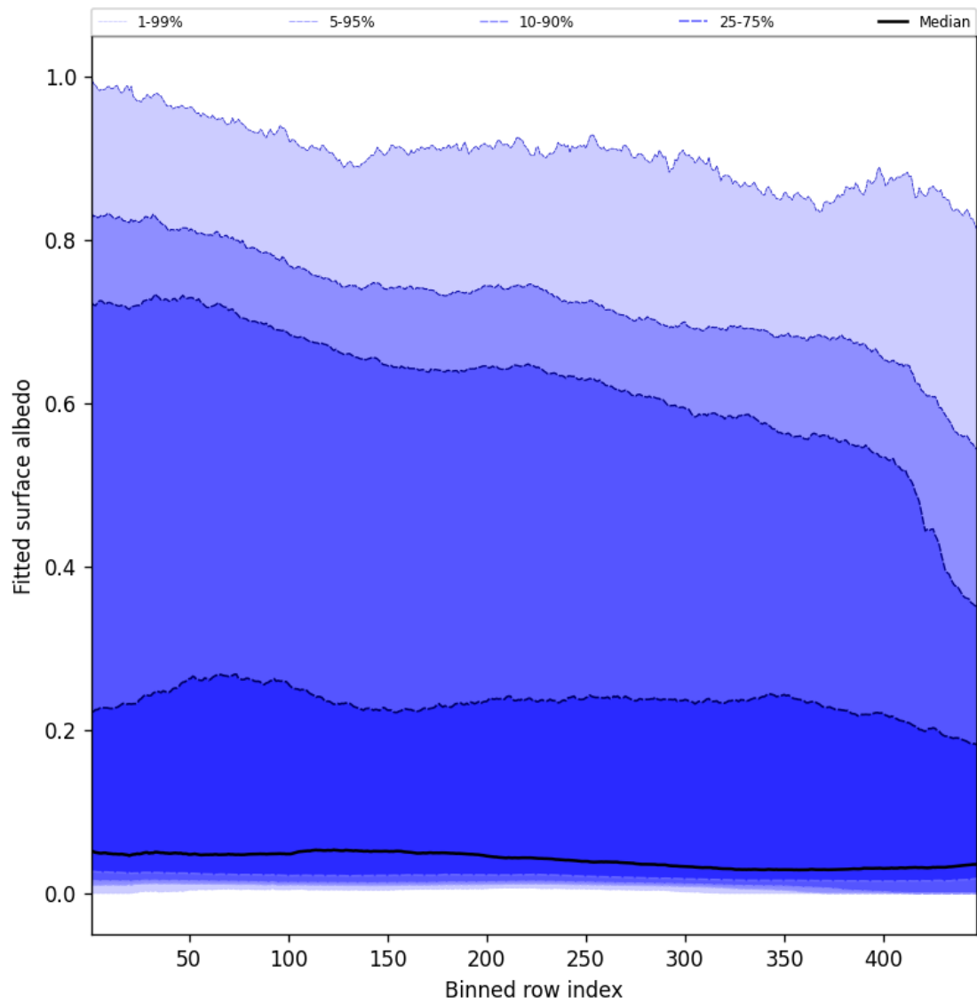
Figure 61: Along track statistics of “Fitted surface albedo” for 2025-09-17 to 2025-09-19
