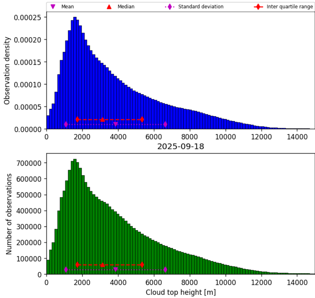
Figure 40: Histogram of “Cloud top height” for 2025-09-17 to 2025-09-19
