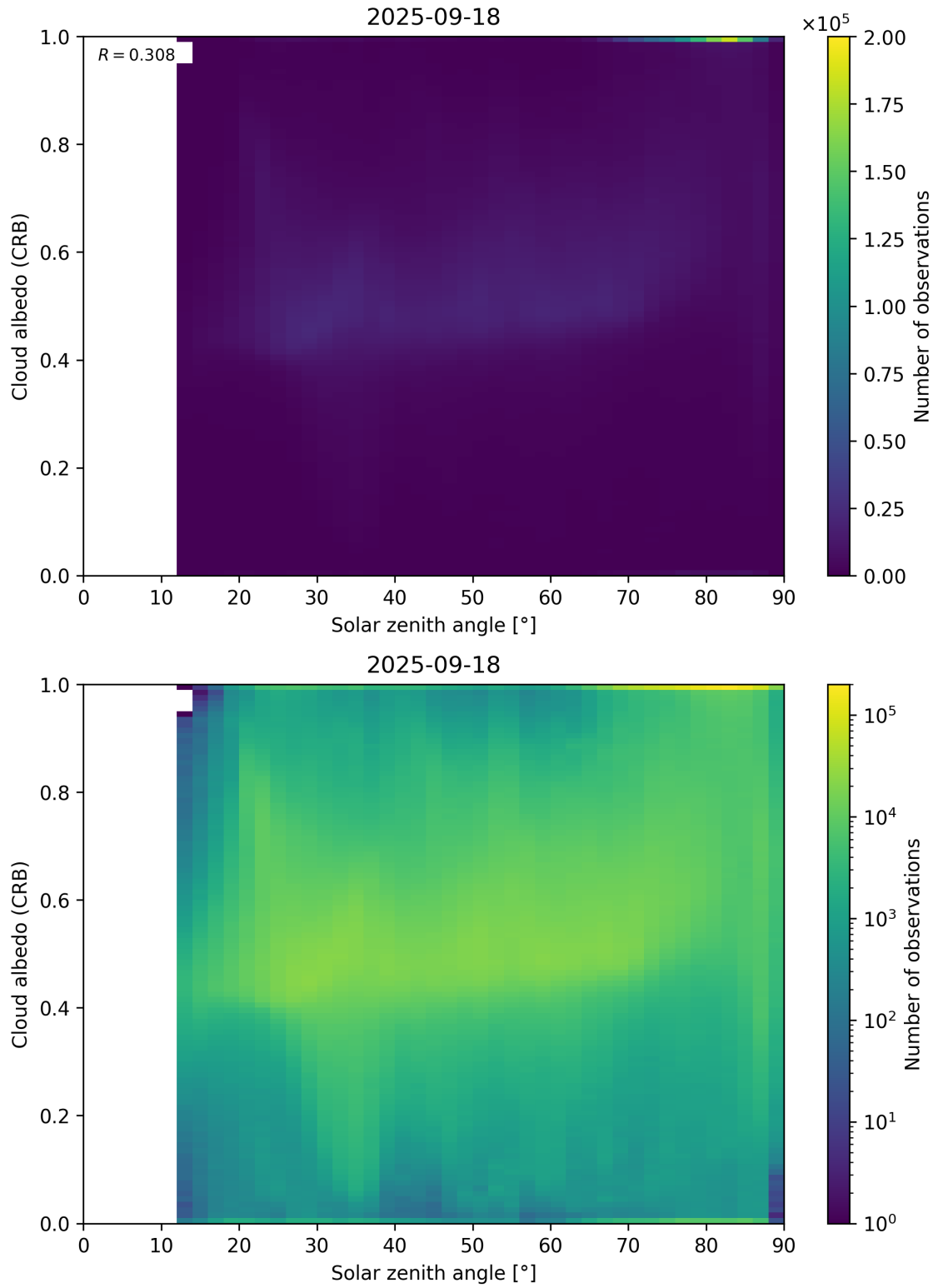
Figure 98: Scatter density plot of “Solar zenith angle” against “Cloud albedo (CRB)” for 2025-09-17 to 2025-09-19.
