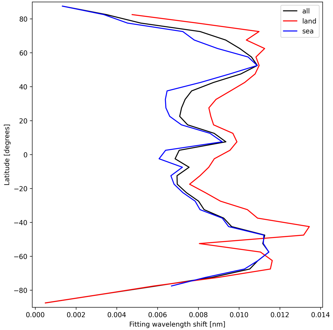
Figure 33: Zonal average of “Fitting wavelength shift” for 2025-09-17 to 2025-09-19.
