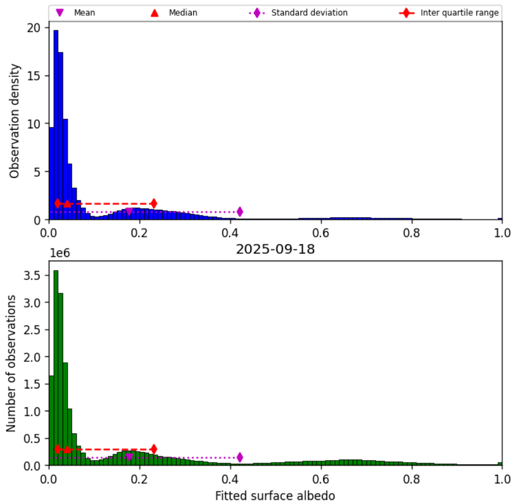
Figure 45: Histogram of “Fitted surface albedo” for 2025-09-17 to 2025-09-19
