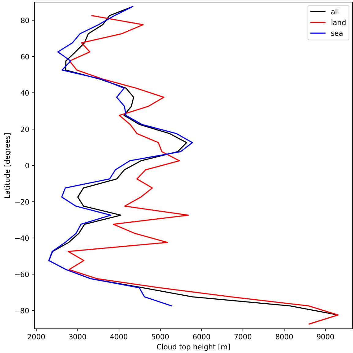
Figure 24: Zonal average of “Cloud top height” for 2025-09-17 to 2025-09-19.
