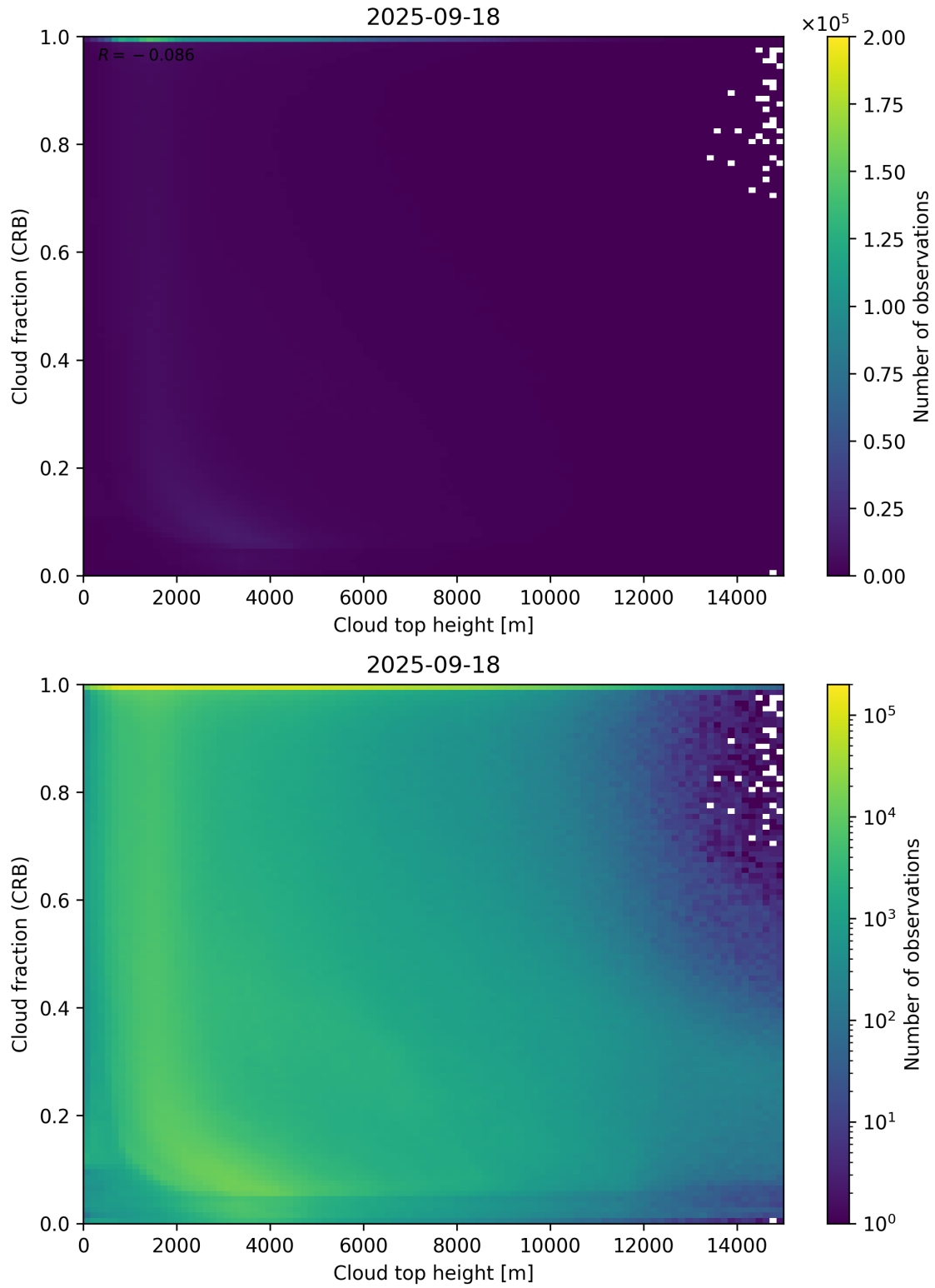
Figure 88: Scatter density plot of “Cloud top height” against “Cloud fraction (CRB)” for 2025-09-17 to 2025-09-19.
