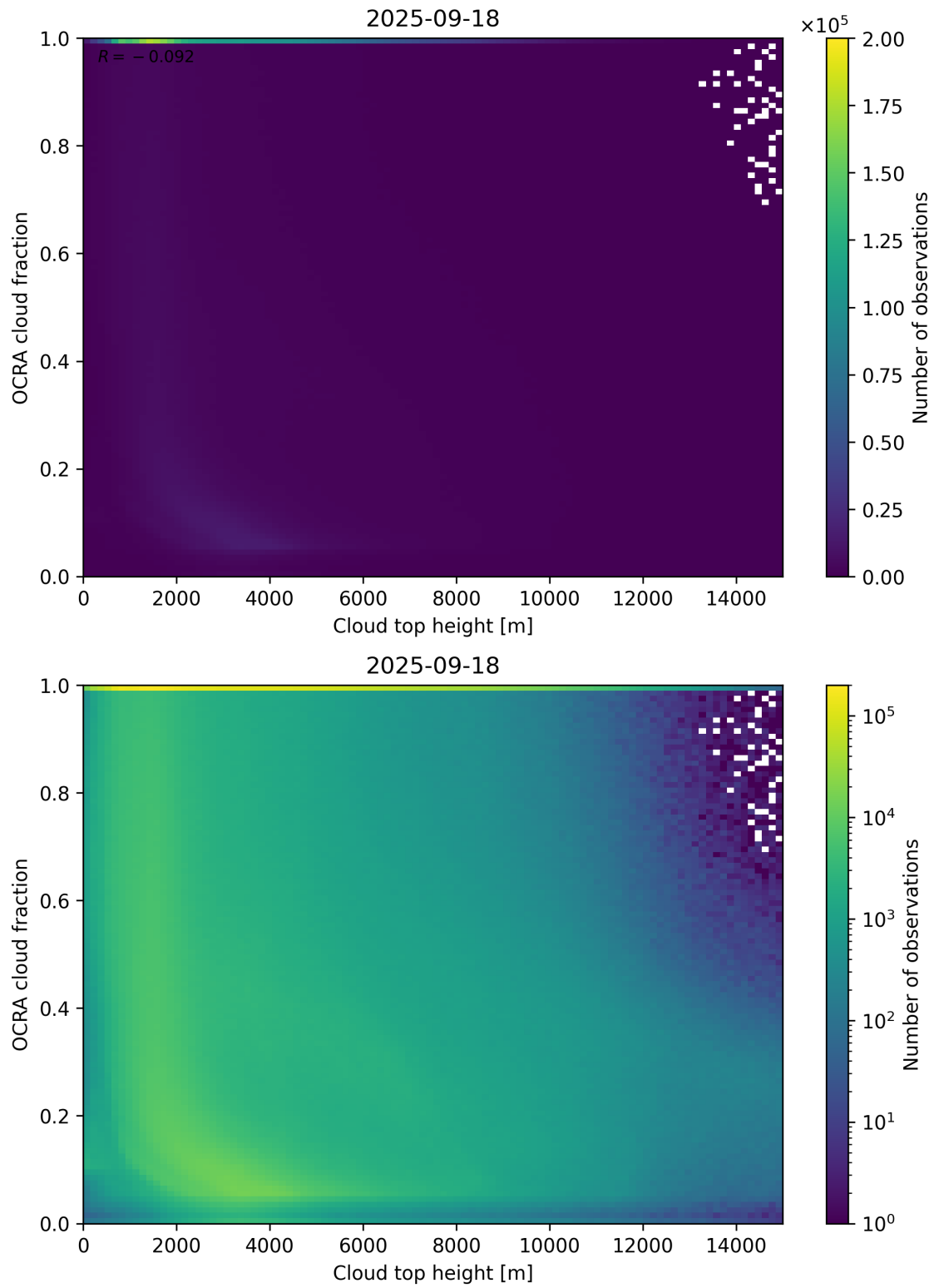
Figure 87: Scatter density plot of “Cloud top height” against “OCRA cloud fraction” for 2025-09-17 to 2025-09-19.
