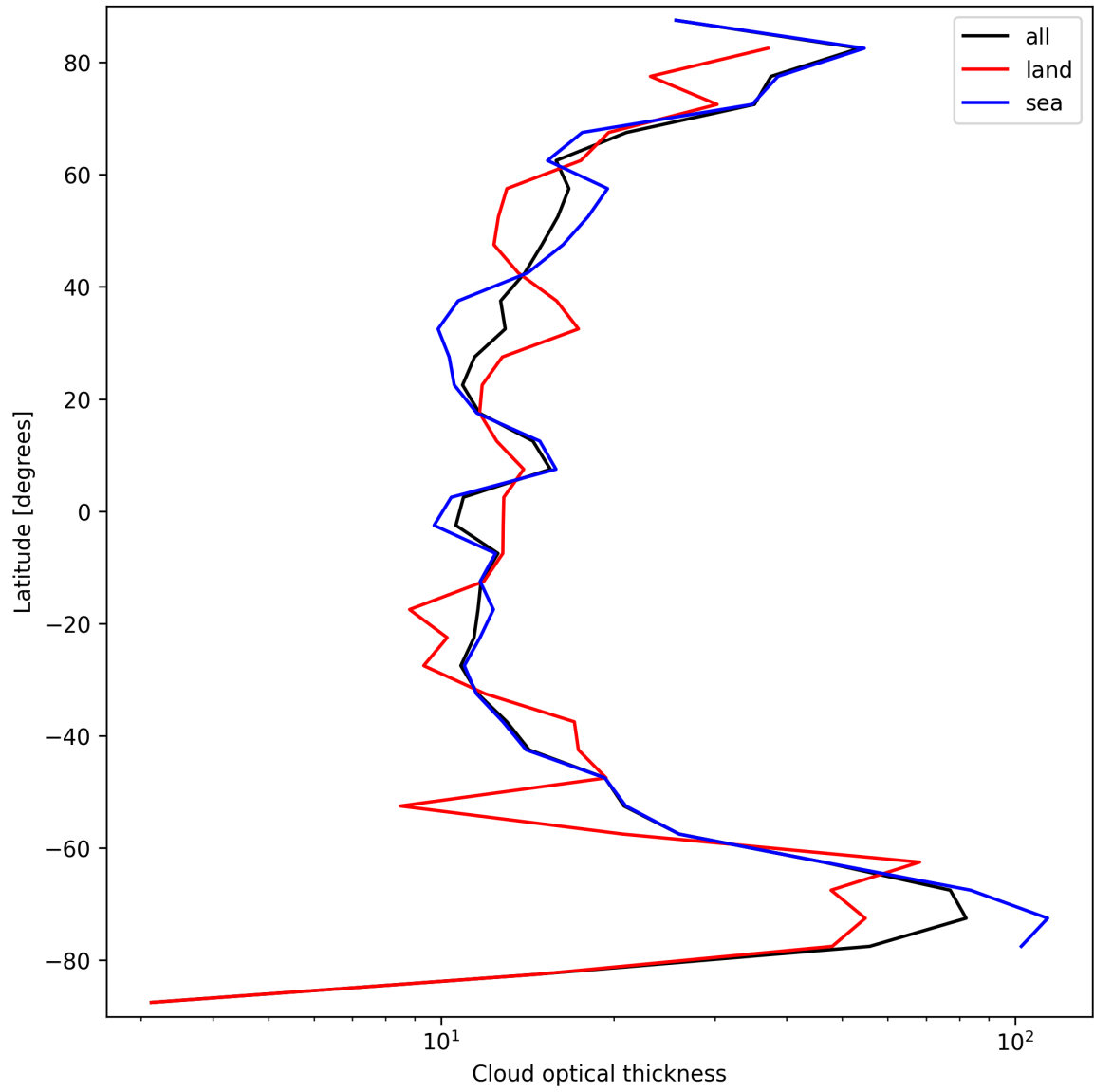
Figure 25: Zonal average of “Cloud optical thickness” for 2025-09-17 to 2025-09-19.
