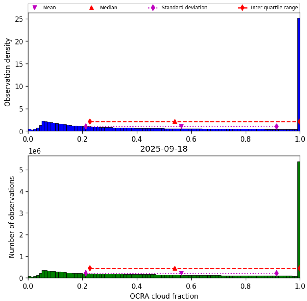
Figure 50: Histogram of “OCRA cloud fraction” for 2025-09-17 to 2025-09-19
