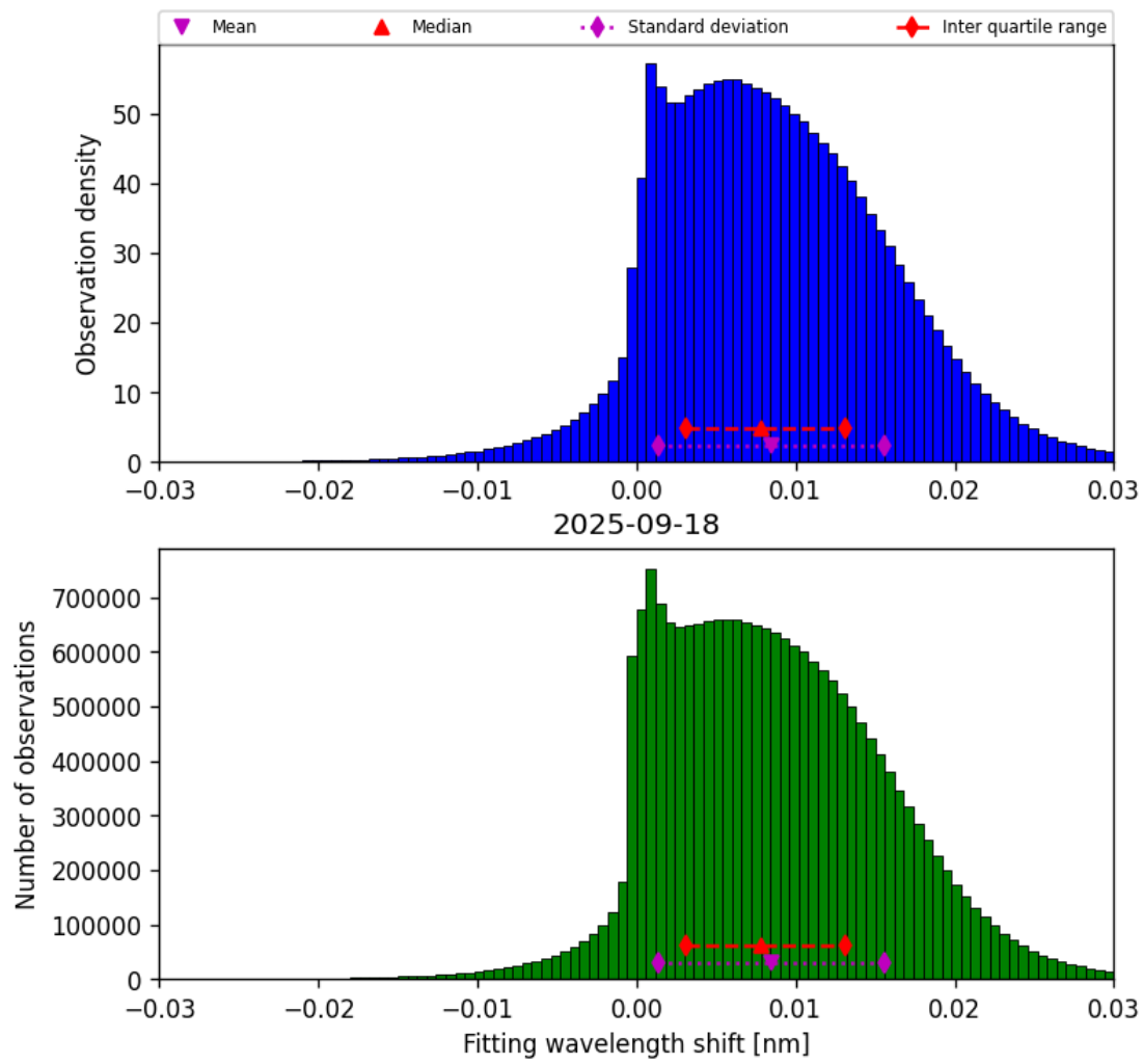
Figure 49: Histogram of “Fitting wavelength shift” for 2025-09-17 to 2025-09-19
