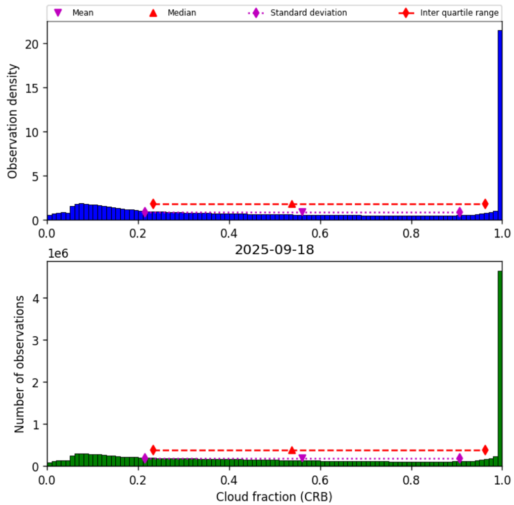
Figure 42: Histogram of “Cloud fraction (CRB)” for 2025-09-17 to 2025-09-19
