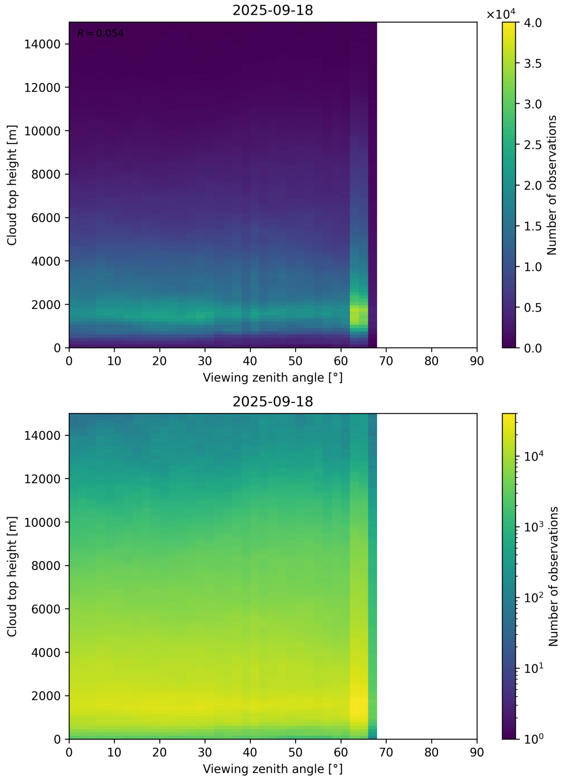
Figure 112: Scatter density plot of “Viewing zenith angle” against “Cloud top height” for 2025-09-17 to 2025-09-19.
