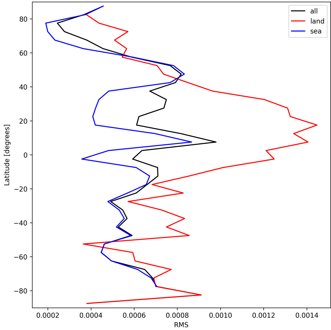
Figure 31: Zonal average of “RMS” for 2025-09-17 to 2025-09-19.
