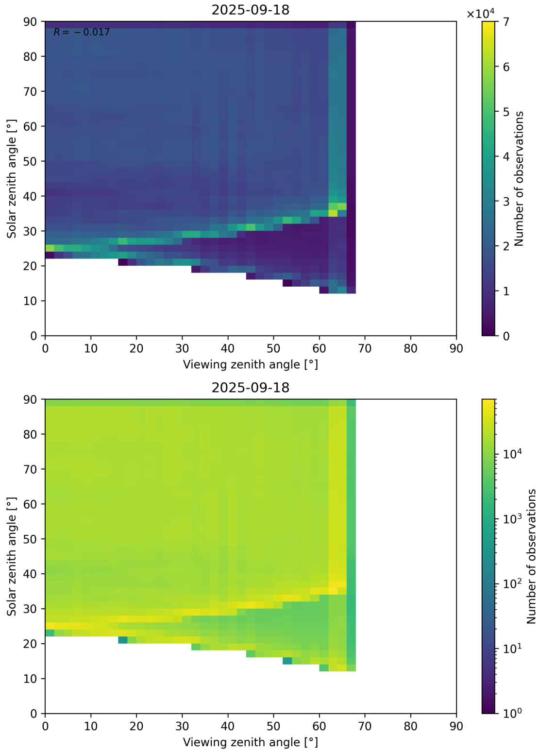
Figure 114: Scatter density plot of “Viewing zenith angle” against “Solar zenith angle” for 2025-09-17 to 2025-09-19.
