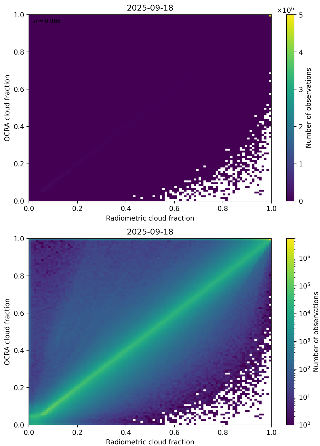
Figure 72: Scatter density plot of “Radiometric cloud fraction” against “OCRA cloud fraction” for 2025-09-17 to 2025-09-19.
