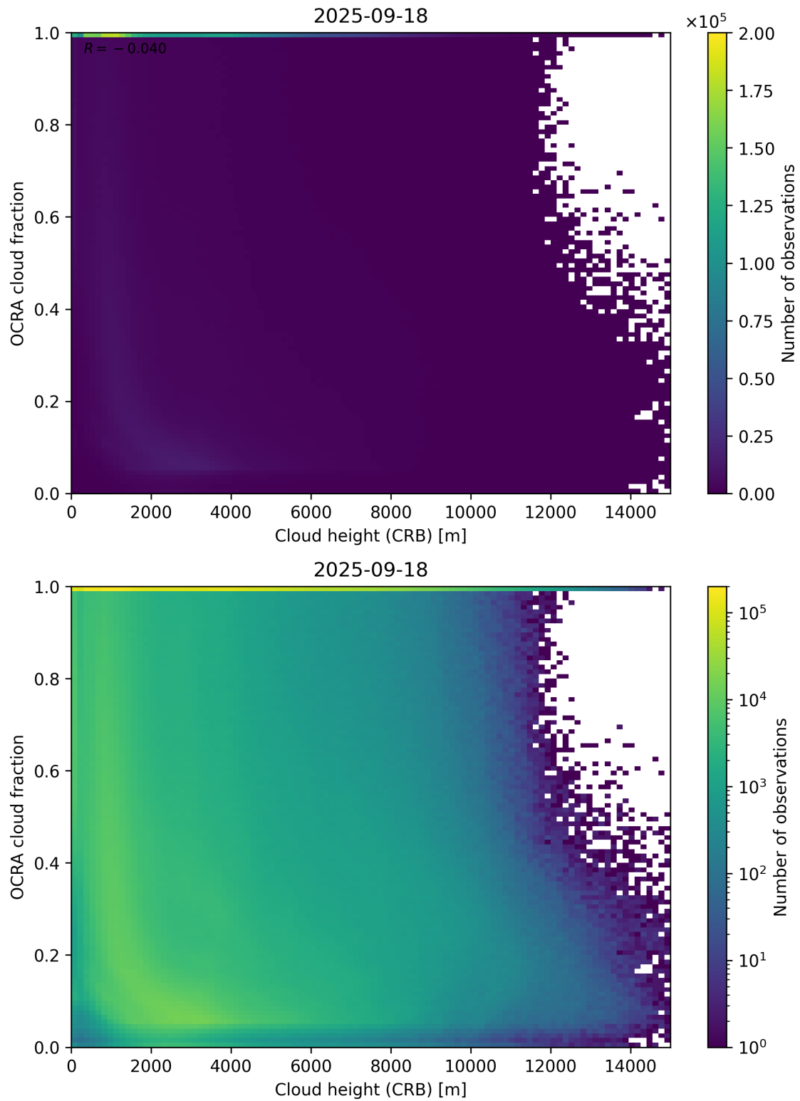
Figure 81: Scatter density plot of “Cloud height (CRB)” against “OCRA cloud fraction” for 2025-09-17 to 2025-09-19.
