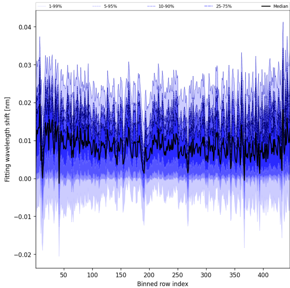
Figure 65: Along track statistics of “Fitting wavelength shift” for 2025-09-17 to 2025-09-19
