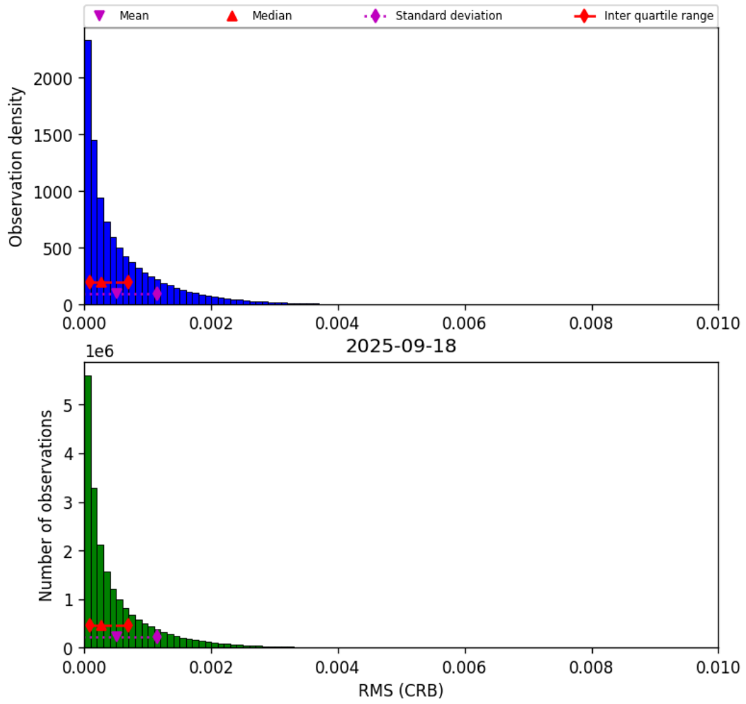
Figure 48: Histogram of “RMS (CRB)” for 2025-09-17 to 2025-09-19
