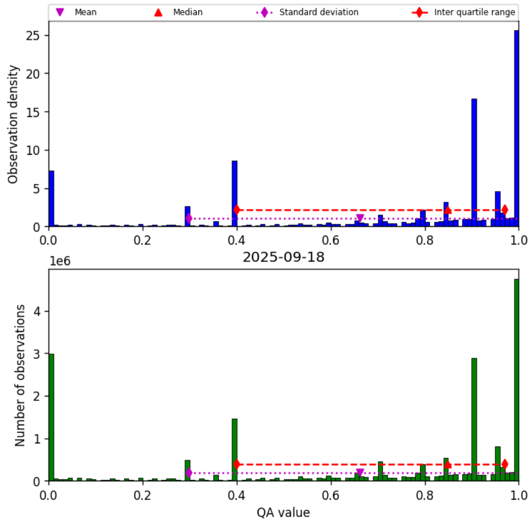
Figure 38: Histogram of “QA value” for 2025-09-17 to 2025-09-19
