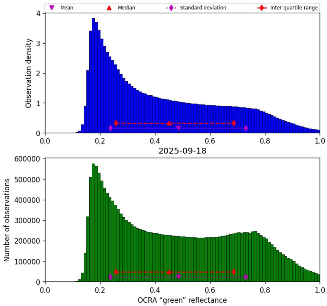
Figure 52: Histogram of “OCRA “green” reflectance” for 2025-09-17 to 2025-09-19
