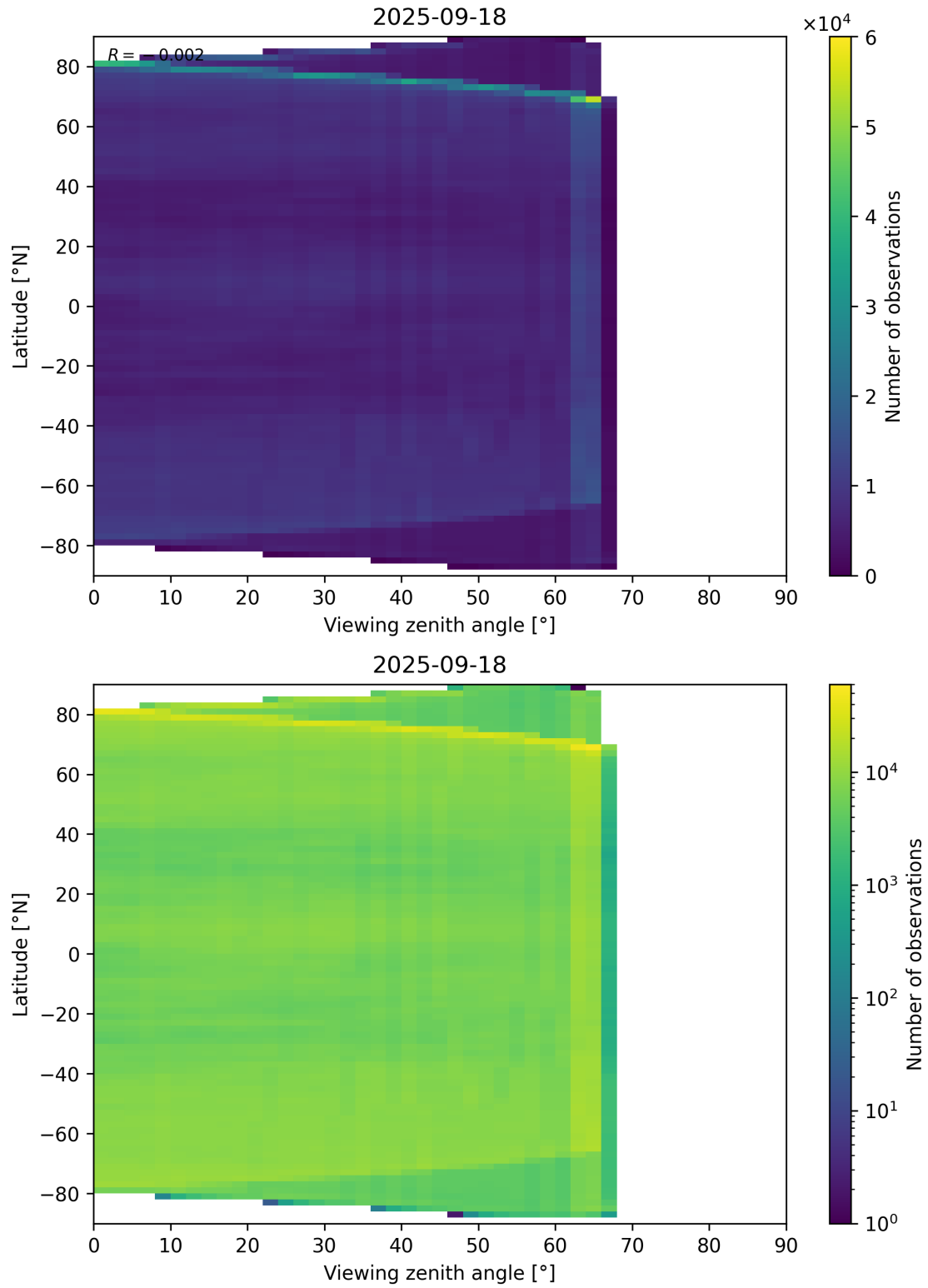
Figure 113: Scatter density plot of “Viewing zenith angle” against “Latitude” for 2025-09-17 to 2025-09-19.
