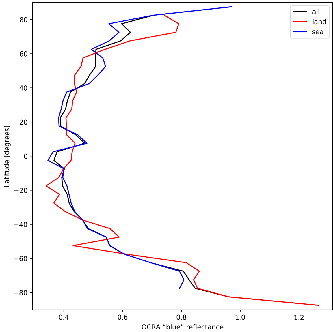
Figure 35: Zonal average of “OCRA “blue” reflectance” for 2025-09-17 to 2025-09-19.
