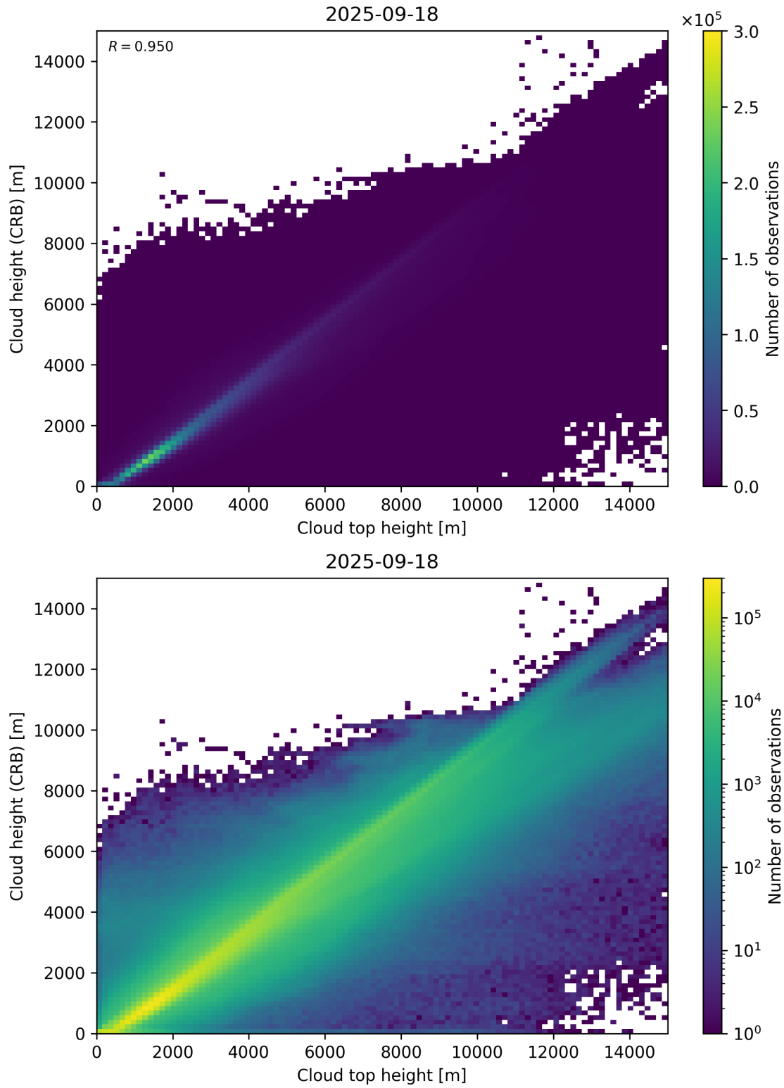
Figure 89: Scatter density plot of “Cloud top height” against “Cloud height (CRB)” for 2025-09-17 to 2025-09-19.
