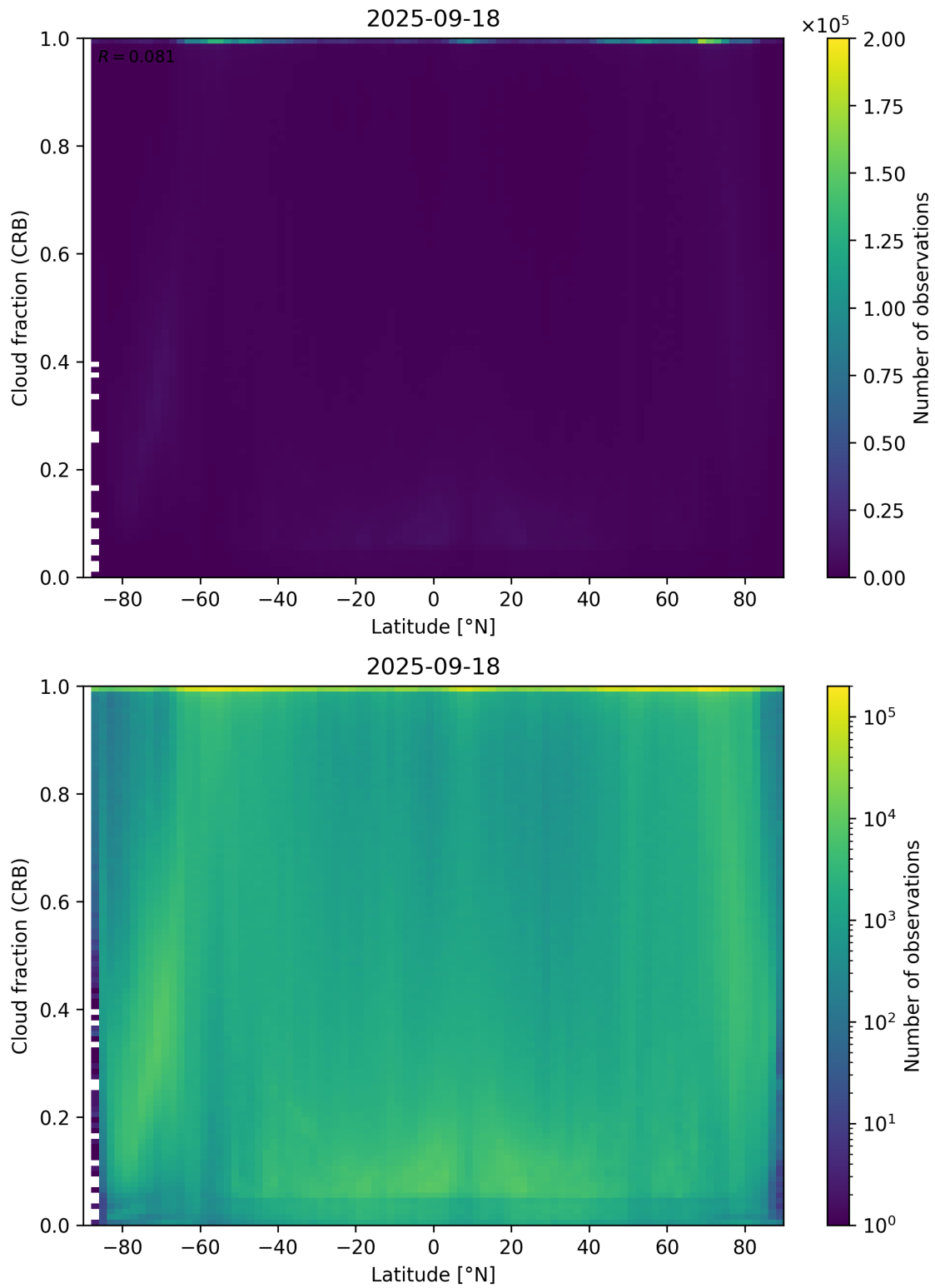
Figure 94: Scatter density plot of “Latitude” against “Cloud fraction (CRB)” for 2025-09-17 to 2025-09-19.
