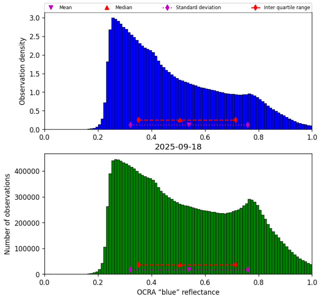
Figure 51: Histogram of “OCRA “blue” reflectance” for 2025-09-17 to 2025-09-19
