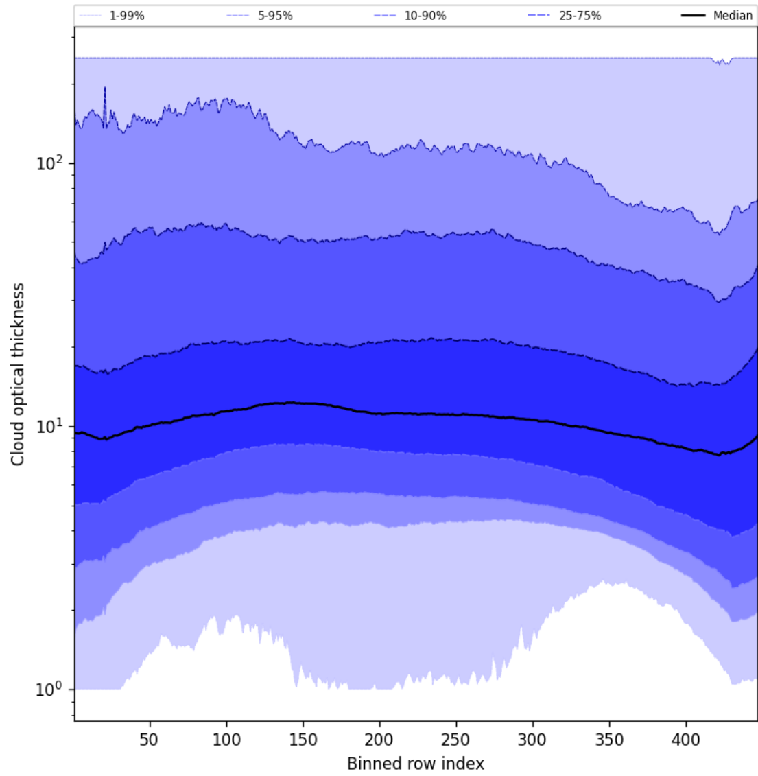
Figure 57: Along track statistics of “Cloud optical thickness” for 2025-09-17 to 2025-09-19
