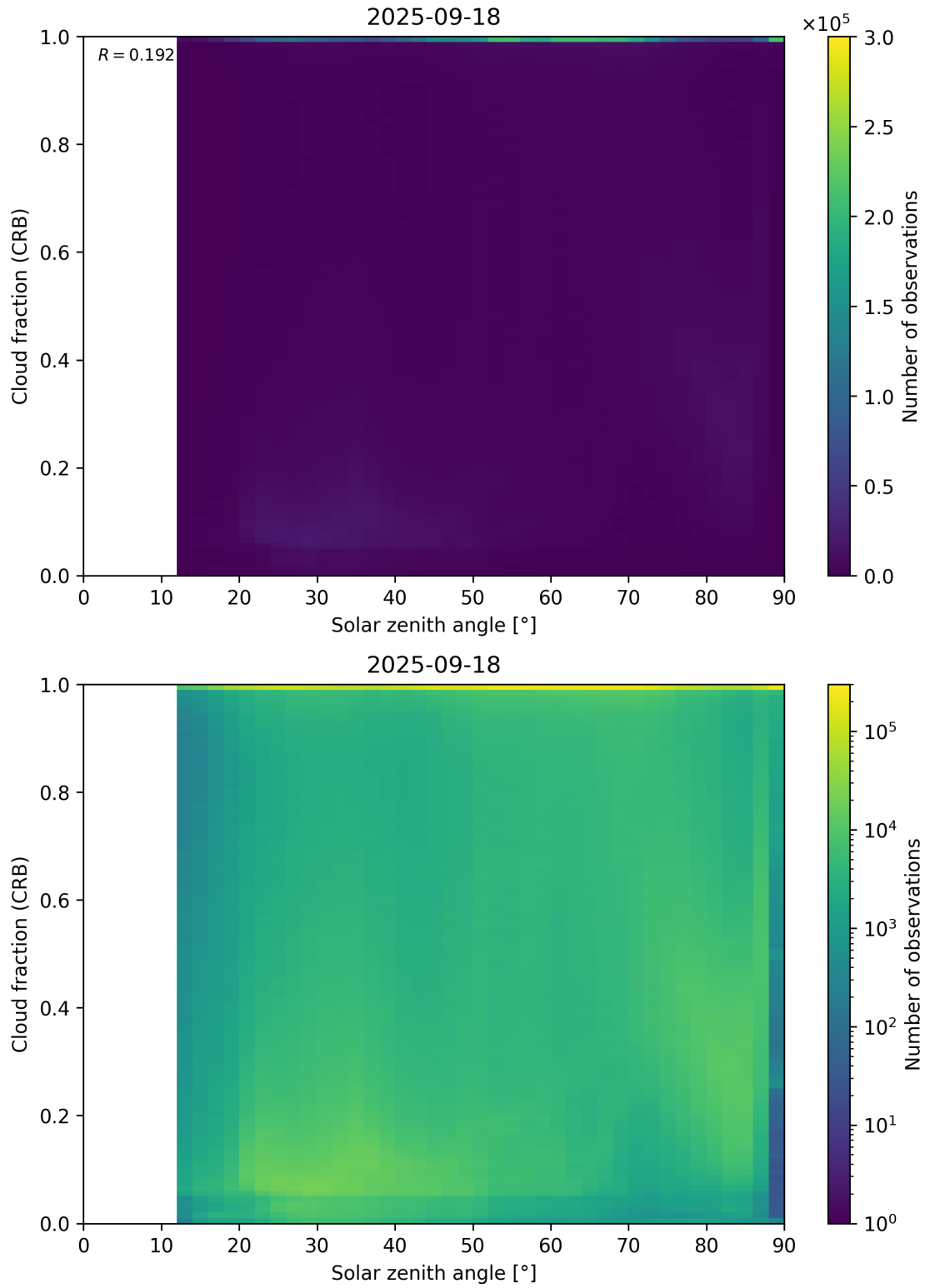
Figure 101: Scatter density plot of “Solar zenith angle” against “Cloud fraction (CRB)” for 2025-09-17 to 2025-09-19.
