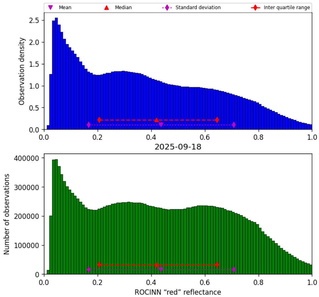
Figure 53: Histogram of “ROCINN “red” reflectance” for 2025-09-17 to 2025-09-19
