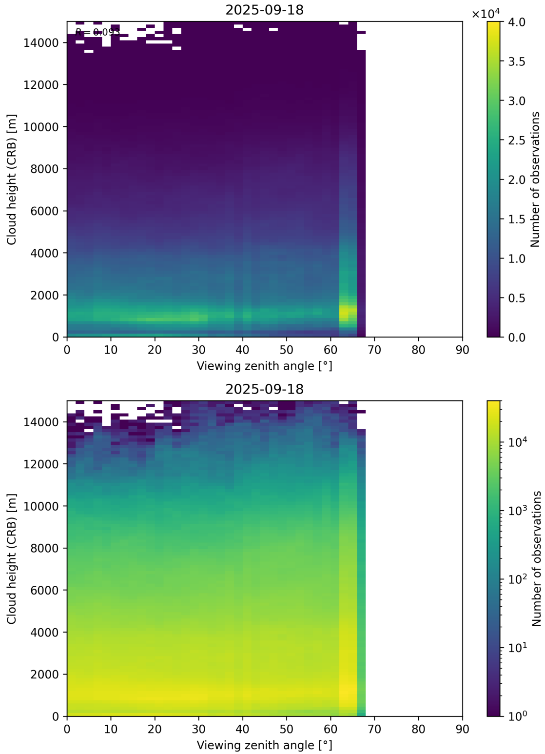
Figure 110: Scatter density plot of “Viewing zenith angle” against “Cloud height (CRB)” for 2025-09-17 to 2025-09-19.
