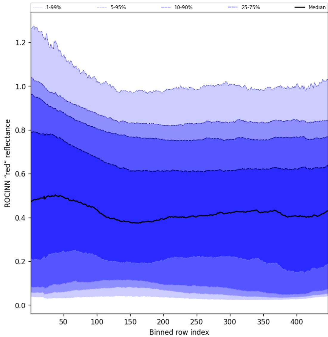
Figure 69: Along track statistics of “ROCINN “red” reflectance” for 2025-09-17 to 2025-09-19
