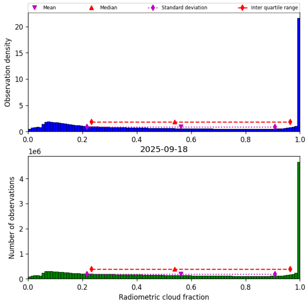
Figure 39: Histogram of “Radiometric cloud fraction” for 2025-09-17 to 2025-09-19
