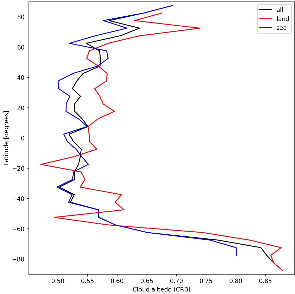
Figure 28: Zonal average of “Cloud albedo (CRB)” for 2025-09-17 to 2025-09-19.
