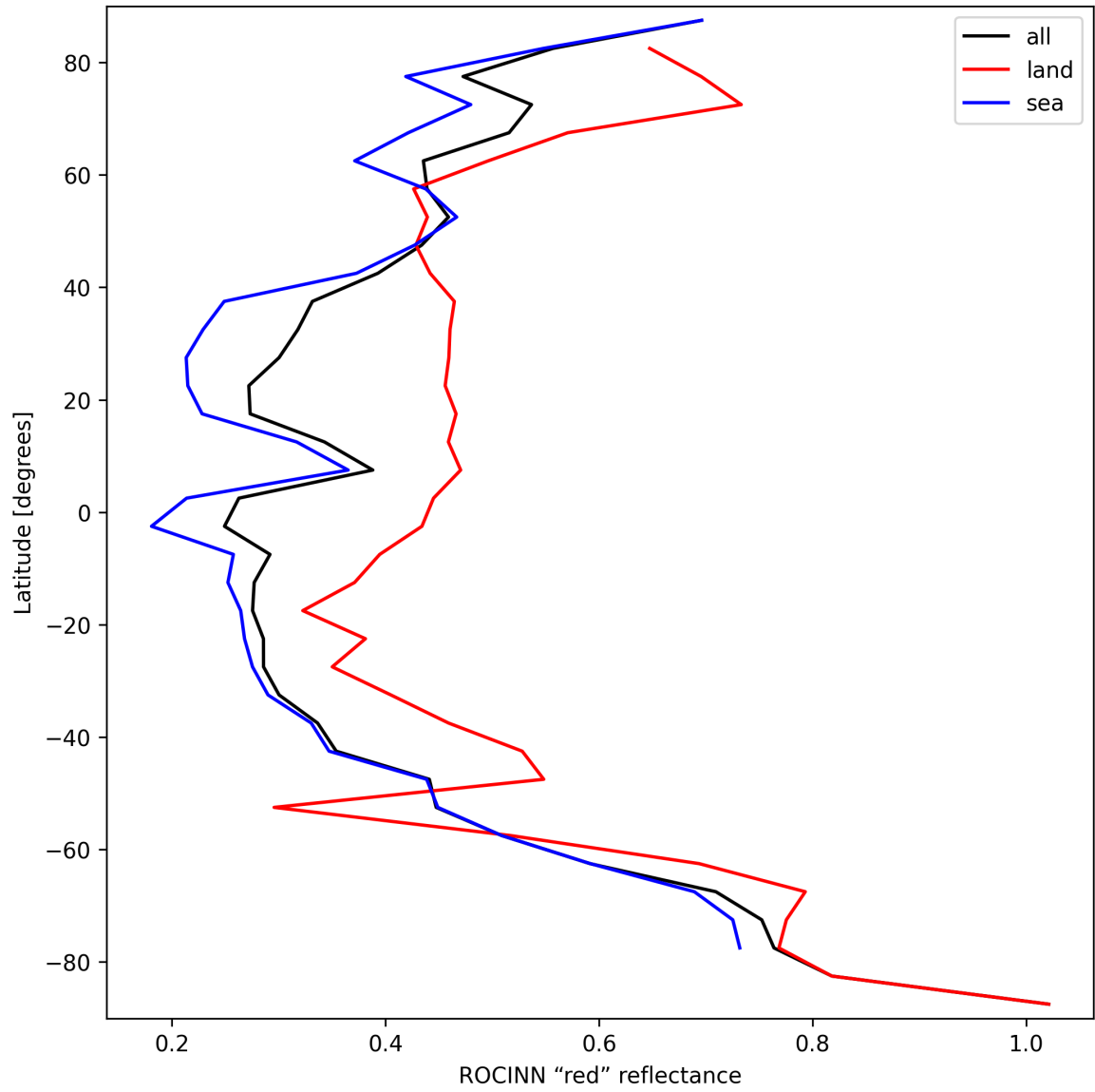
Figure 37: Zonal average of “ROCINN “red” reflectance” for 2025-09-17 to 2025-09-19.
