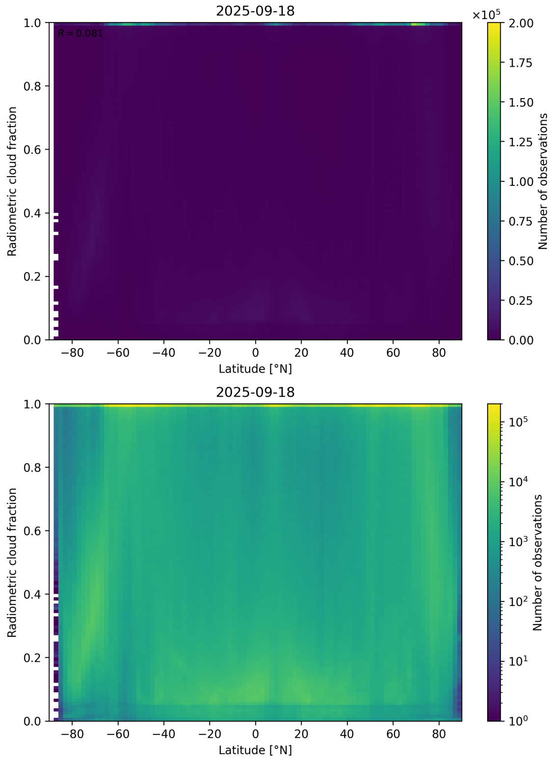
Figure 92: Scatter density plot of “Latitude” against “Radiometric cloud fraction” for 2025-09-17 to 2025-09-19.
