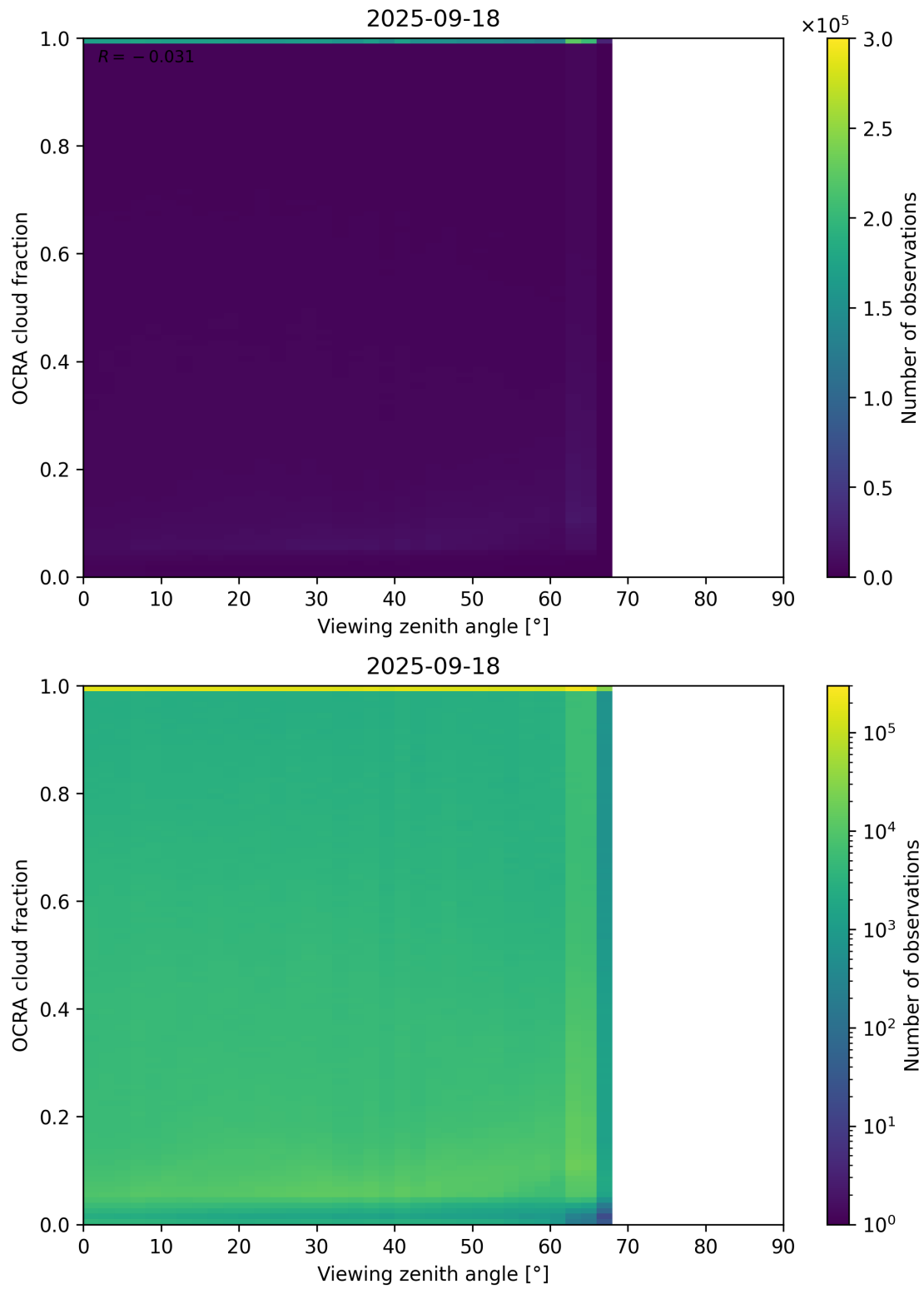
Figure 108: Scatter density plot of “Viewing zenith angle” against “OCRA cloud fraction” for 2025-09-17 to 2025-09-19.
