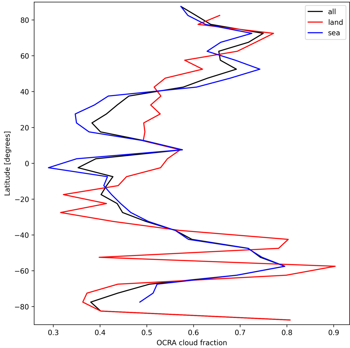
Figure 34: Zonal average of “OCRA cloud fraction” for 2025-09-17 to 2025-09-19.
