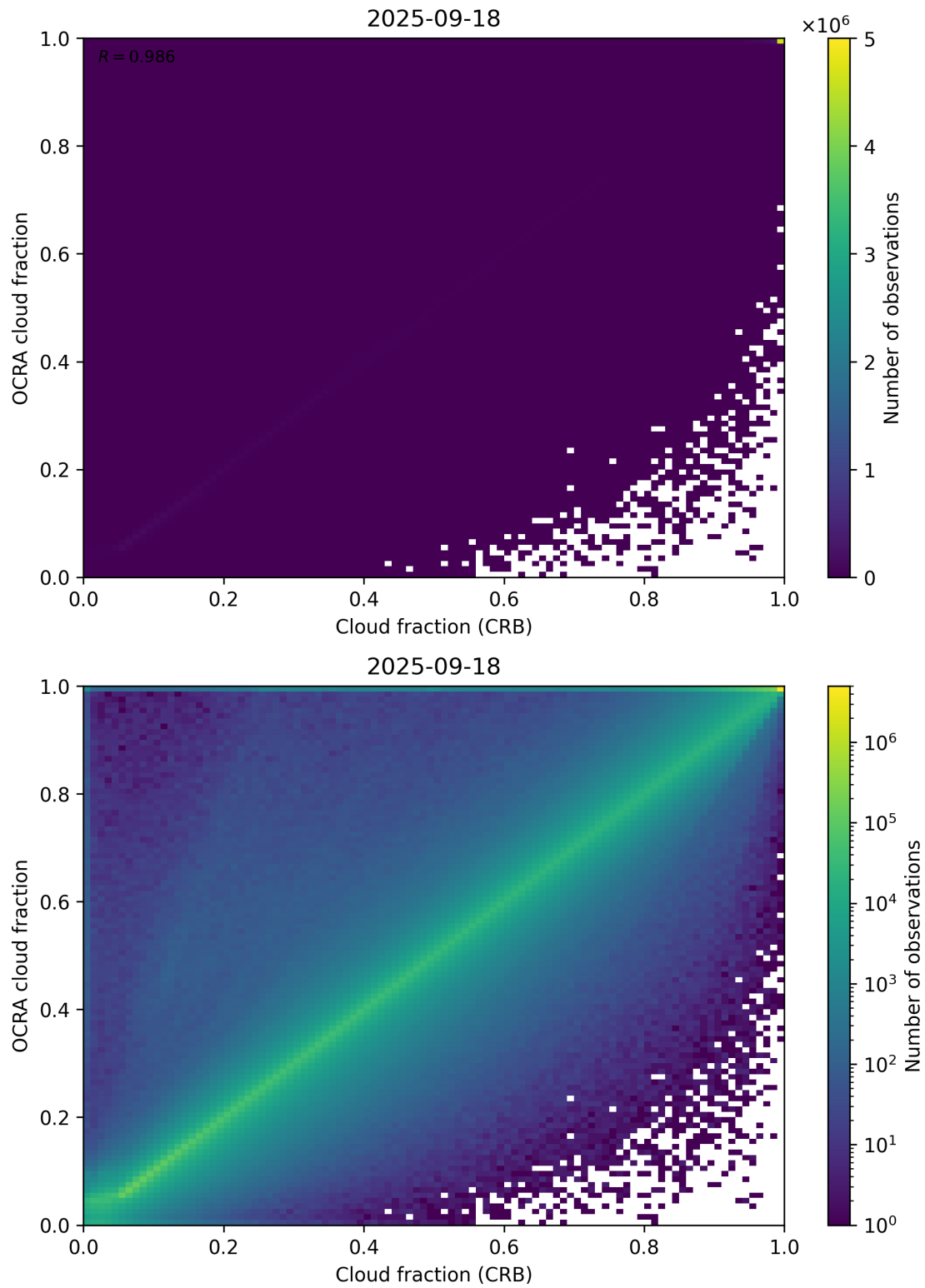
Figure 78: Scatter density plot of “Cloud fraction (CRB)” against “OCRA cloud fraction” for 2025-09-17 to 2025-09-19.
