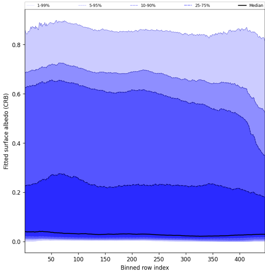
Figure 62: Along track statistics of “Fitted surface albedo (CRB)” for 2025-09-17 to 2025-09-19
