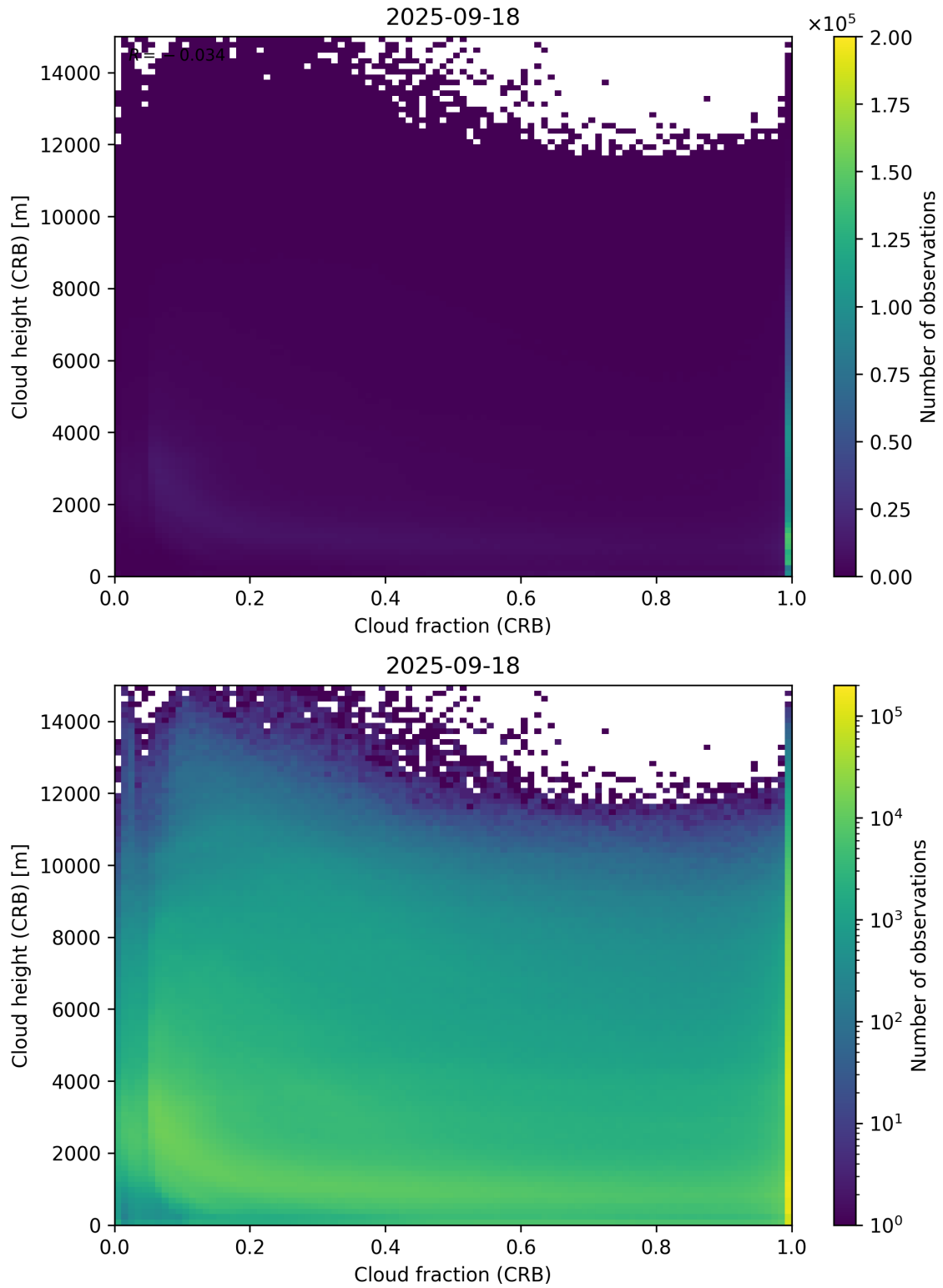
Figure 79: Scatter density plot of “Cloud fraction (CRB)” against “Cloud height (CRB)” for 2025-09-17 to 2025-09-19.
