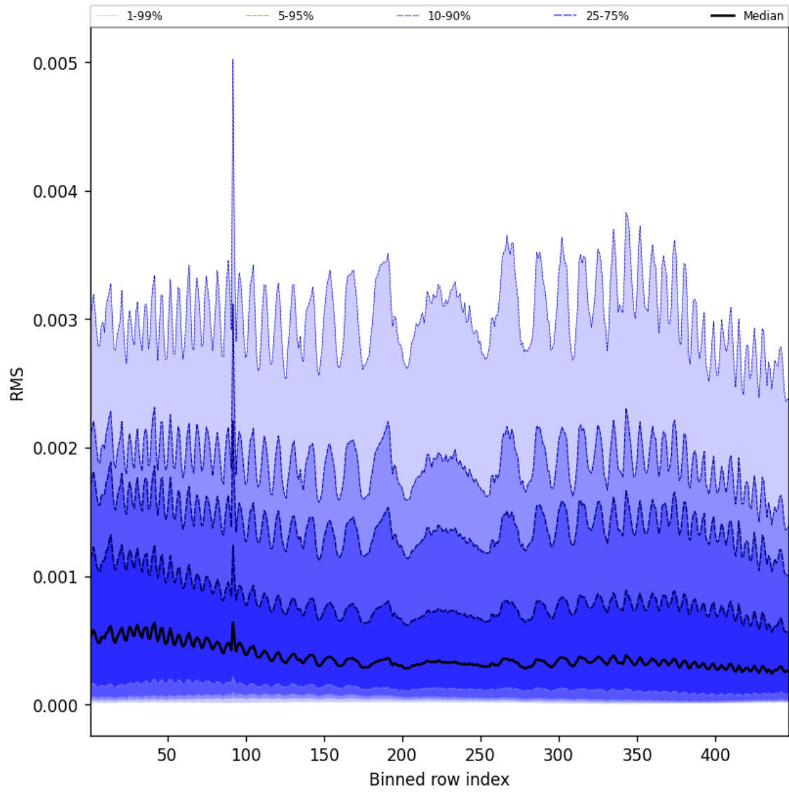
Figure 63: Along track statistics of “RMS” for 2025-09-17 to 2025-09-19
