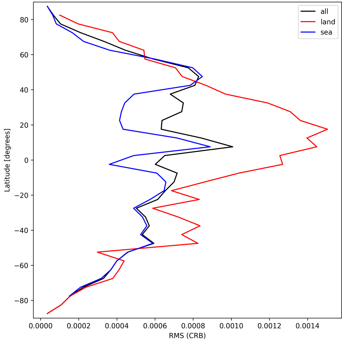
Figure 32: Zonal average of “RMS (CRB)” for 2025-09-17 to 2025-09-19.
