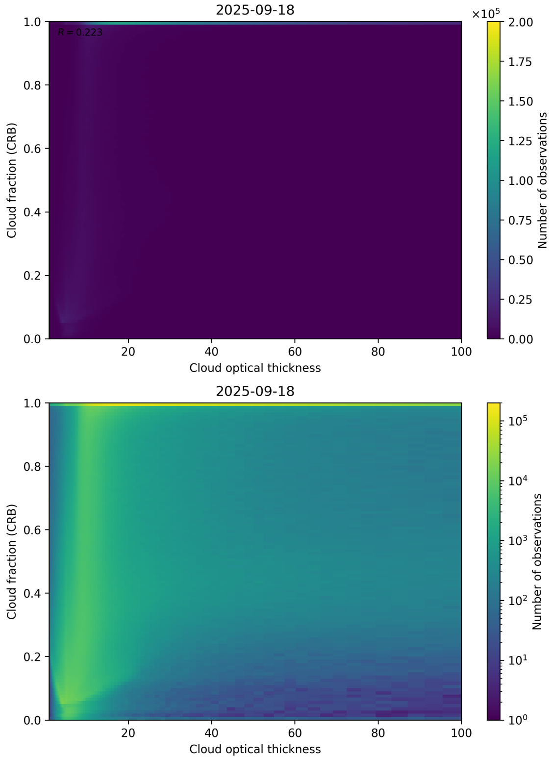
Figure 84: Scatter density plot of “Cloud optical thickness” against “Cloud fraction (CRB)” for 2025-09-17 to 2025-09-19.
