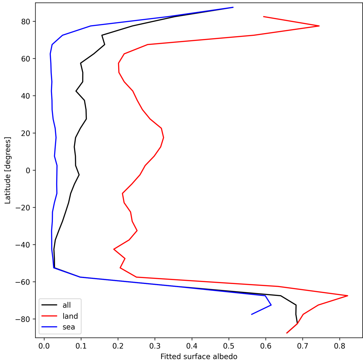
Figure 29: Zonal average of “Fitted surface albedo” for 2025-09-17 to 2025-09-19.
