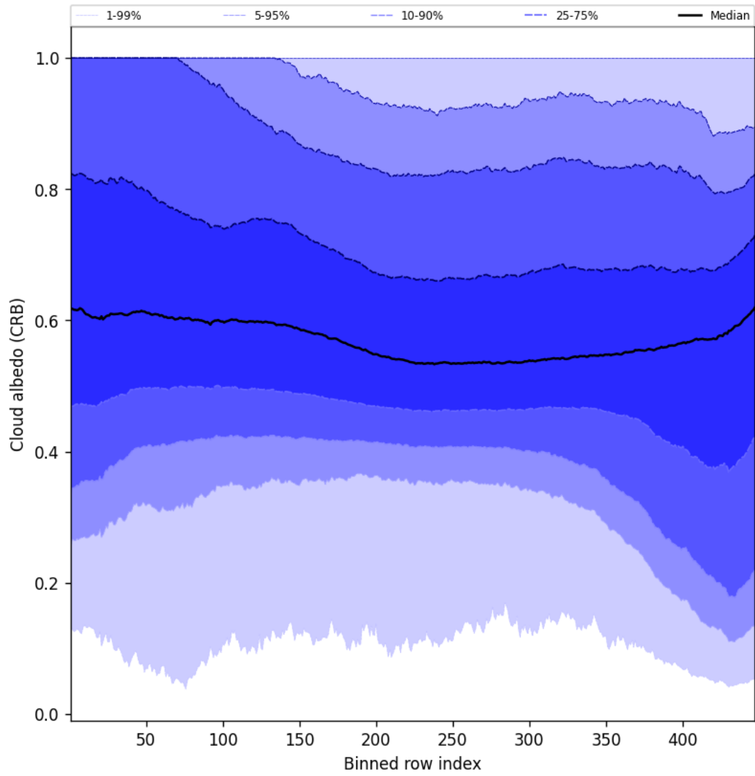
Figure 60: Along track statistics of “Cloud albedo (CRB)” for 2025-09-17 to 2025-09-19
