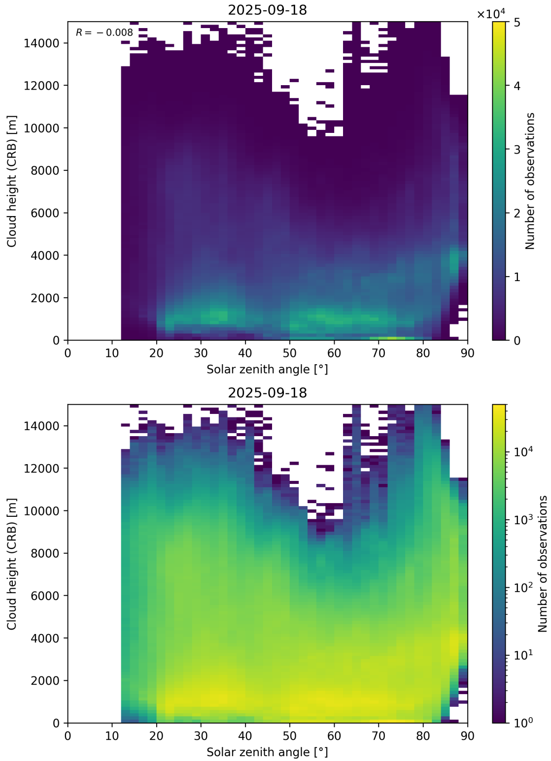
Figure 102: Scatter density plot of “Solar zenith angle” against “Cloud height (CRB)” for 2025-09-17 to 2025-09-19.
