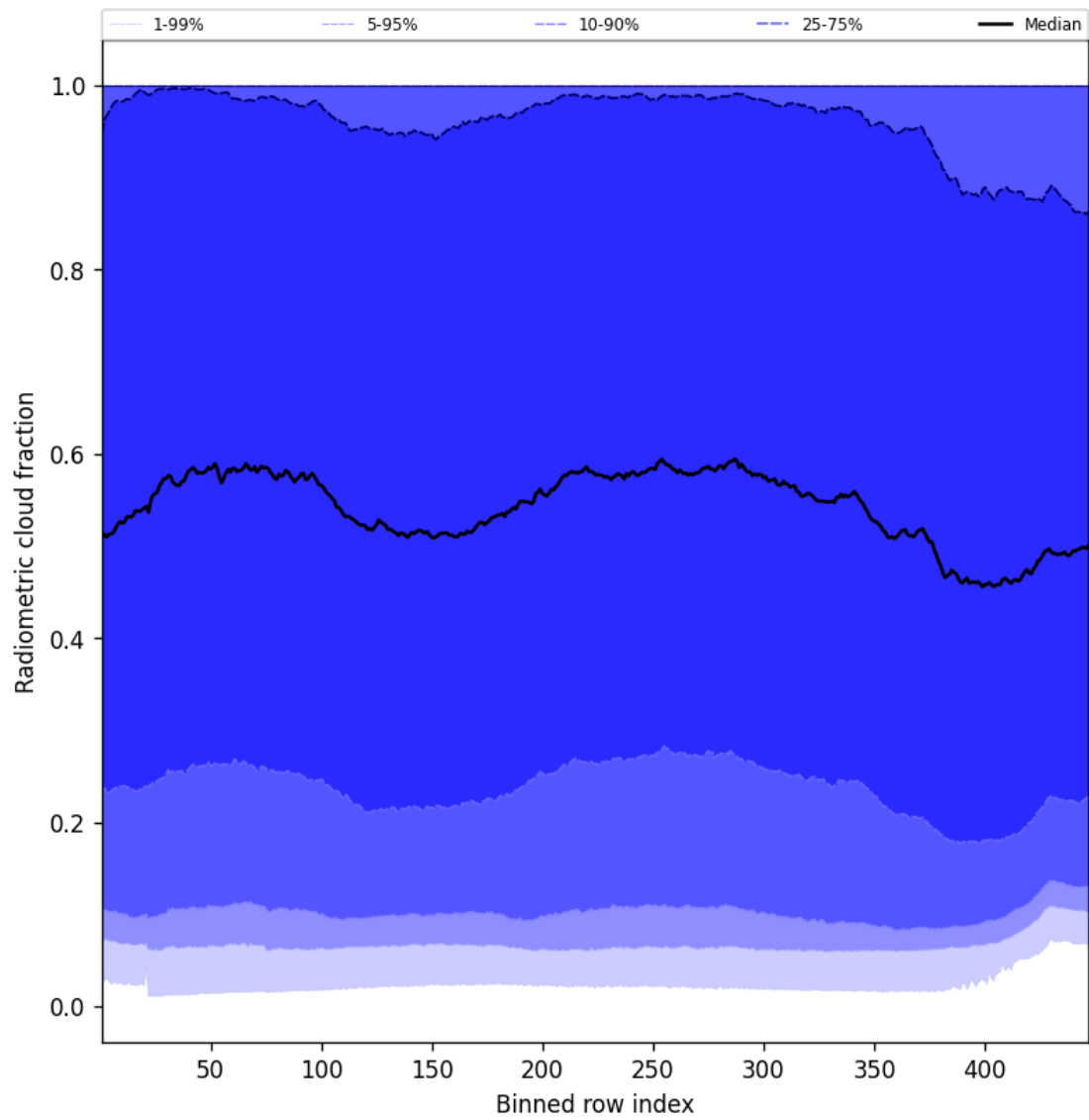
Figure 55: Along track statistics of “Radiometric cloud fraction” for 2025-09-17 to 2025-09-19
