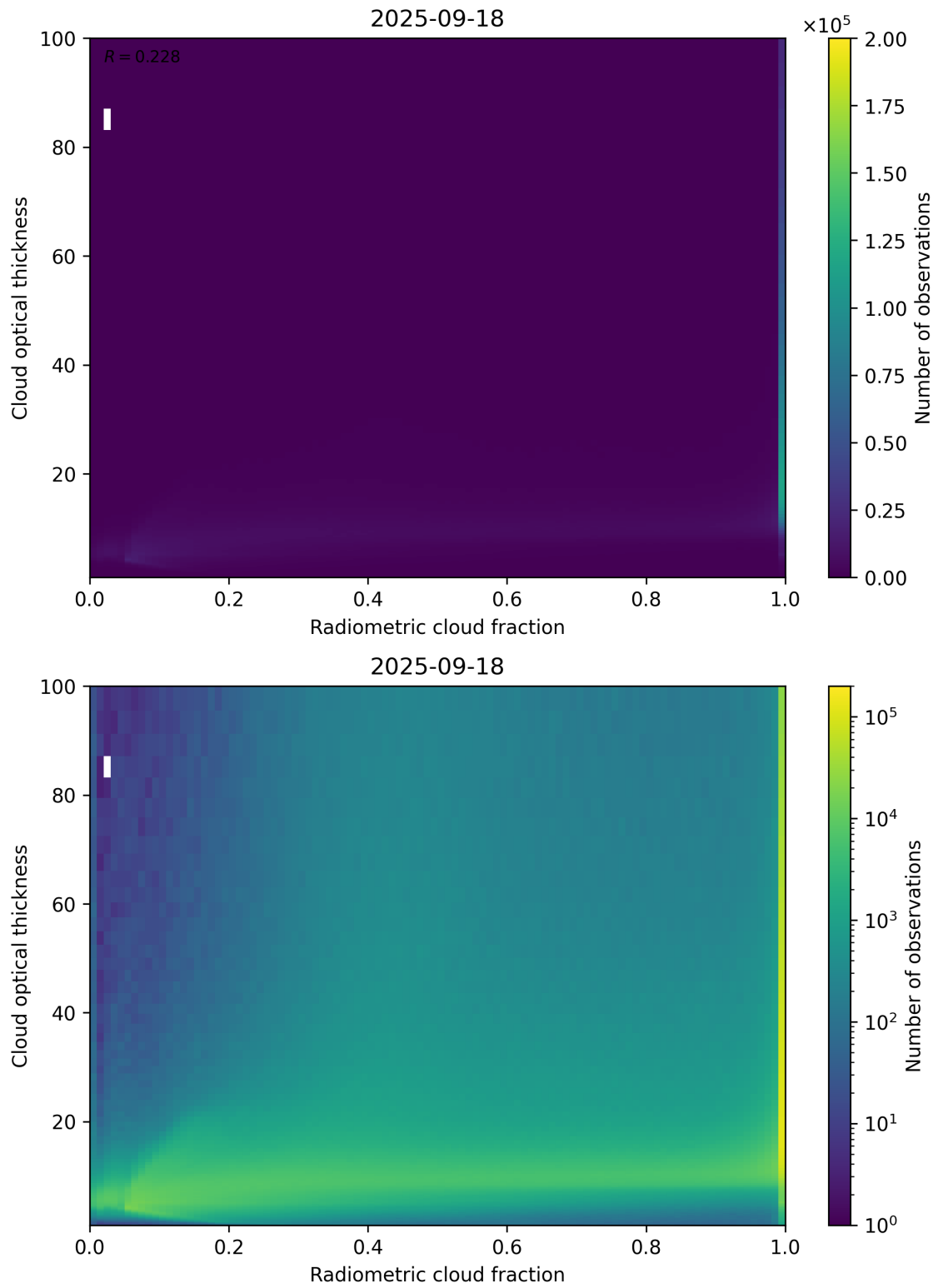
Figure 75: Scatter density plot of “Radiometric cloud fraction” against “Cloud optical thickness” for 2025-09-17 to 2025-09-19.
