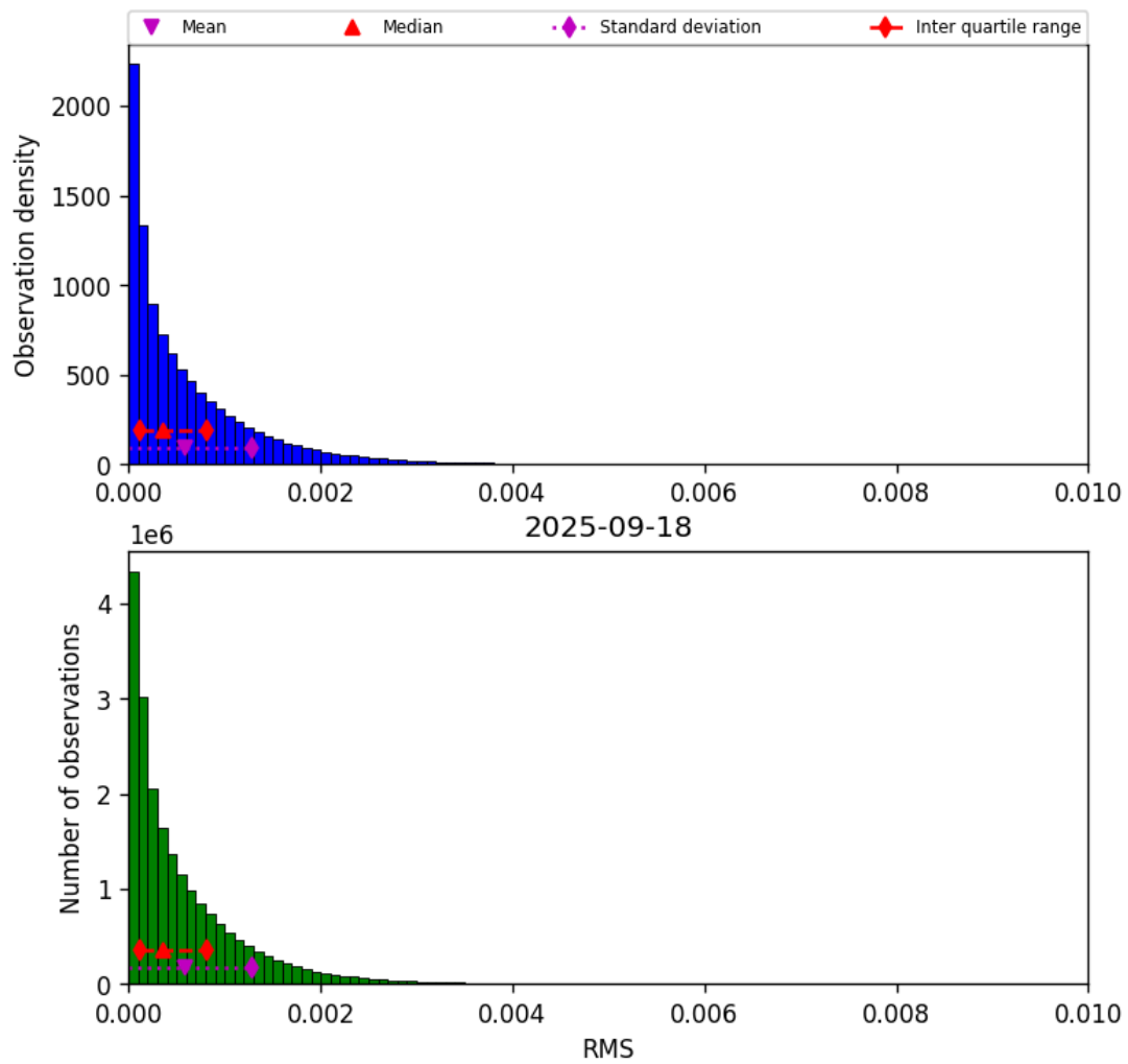
Figure 47: Histogram of “RMS” for 2025-09-17 to 2025-09-19
