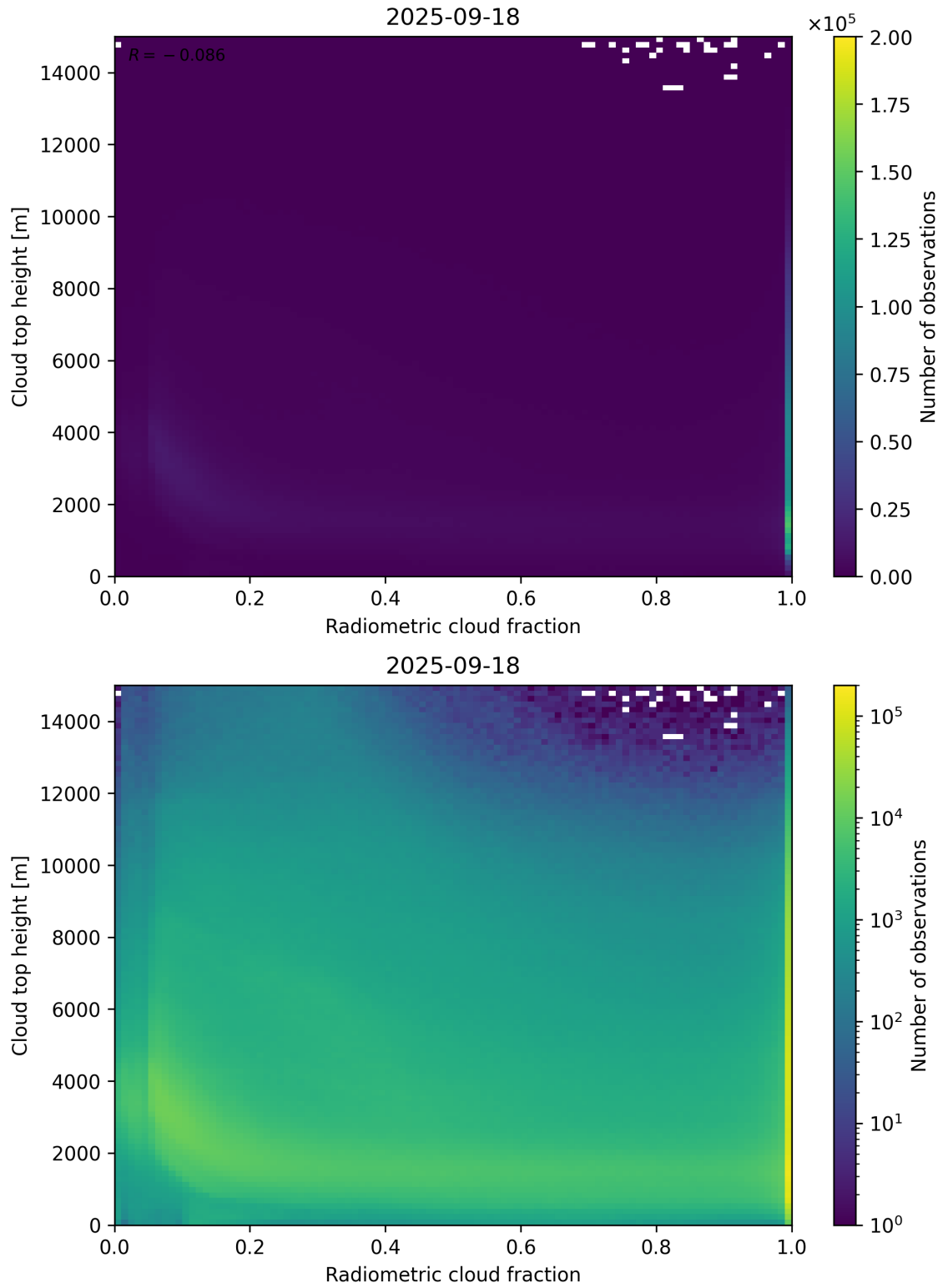
Figure 76: Scatter density plot of “Radiometric cloud fraction” against “Cloud top height” for 2025-09-17 to 2025-09-19.
