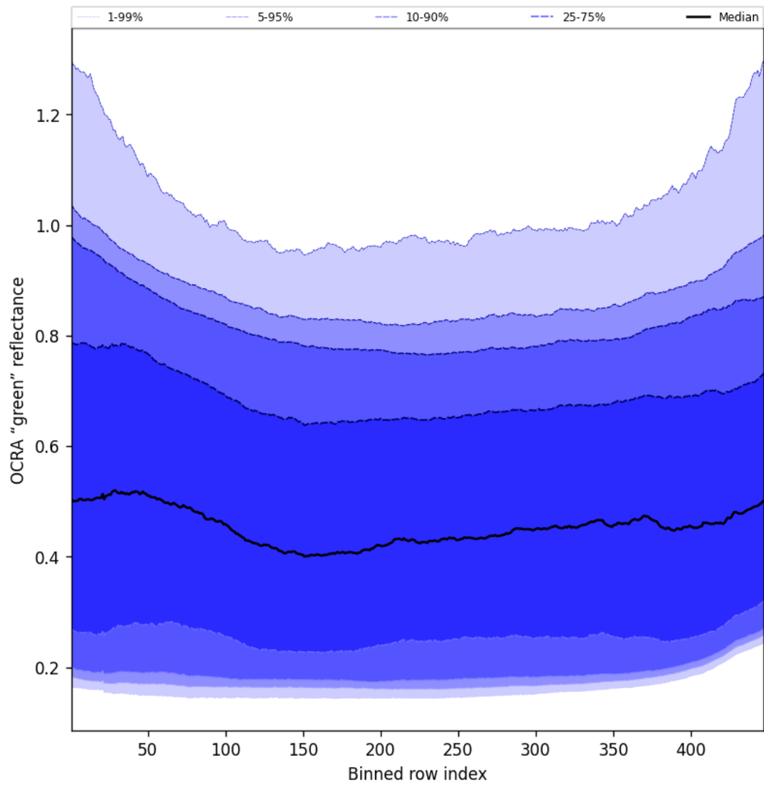
Figure 68: Along track statistics of “OCRA “green” reflectance” for 2025-09-17 to 2025-09-19
