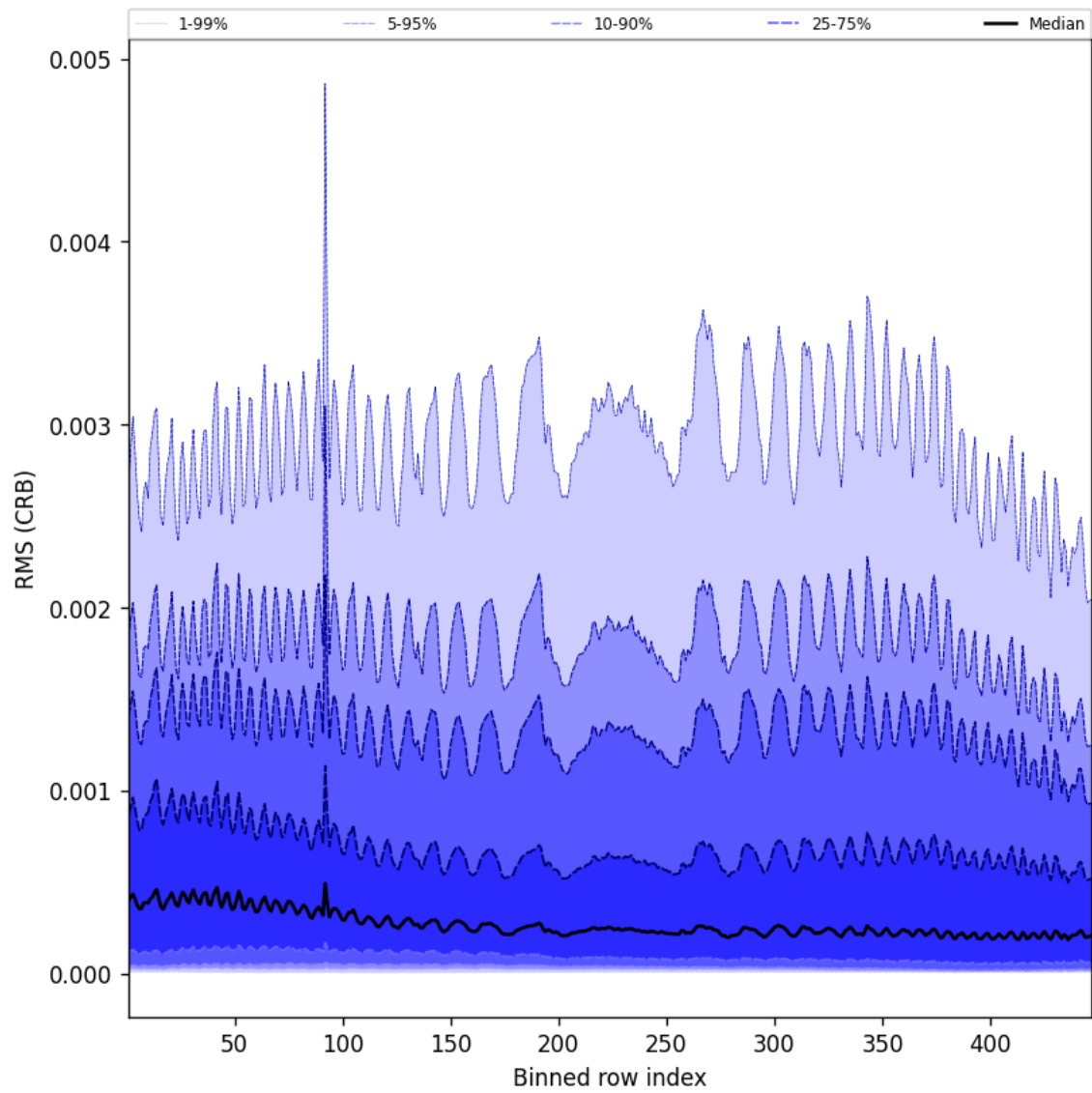
Figure 64: Along track statistics of “RMS (CRB)” for 2025-09-17 to 2025-09-19
