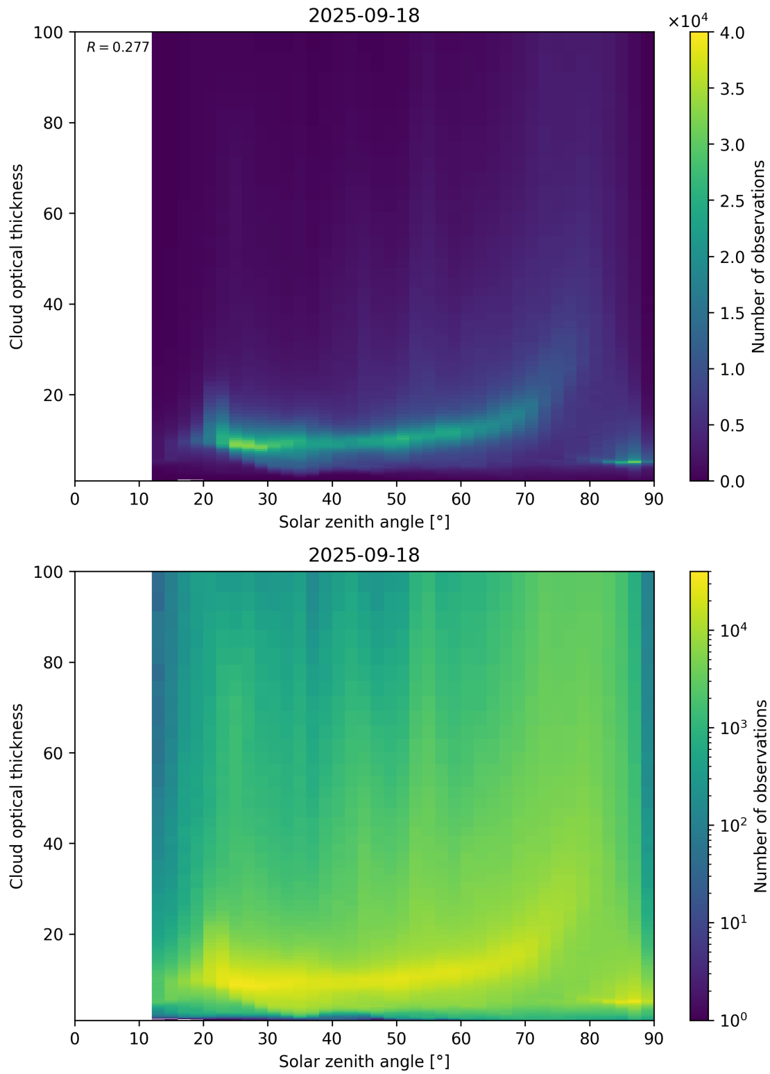
Figure 103: Scatter density plot of “Solar zenith angle” against “Cloud optical thickness” for 2025-09-17 to 2025-09-19.
