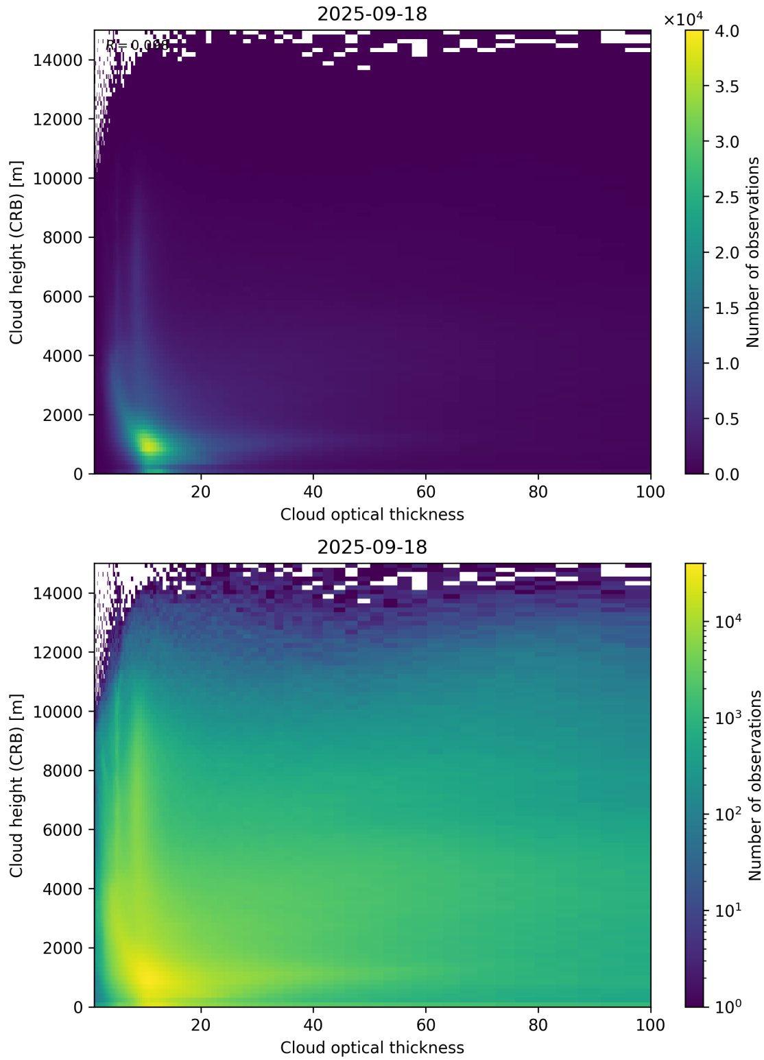
Figure 85: Scatter density plot of “Cloud optical thickness” against “Cloud height (CRB)” for 2025-09-17 to 2025-09-19.
