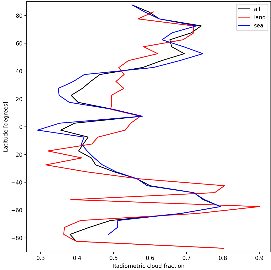
Figure 23: Zonal average of “Radiometric cloud fraction” for 2025-09-17 to 2025-09-19.
