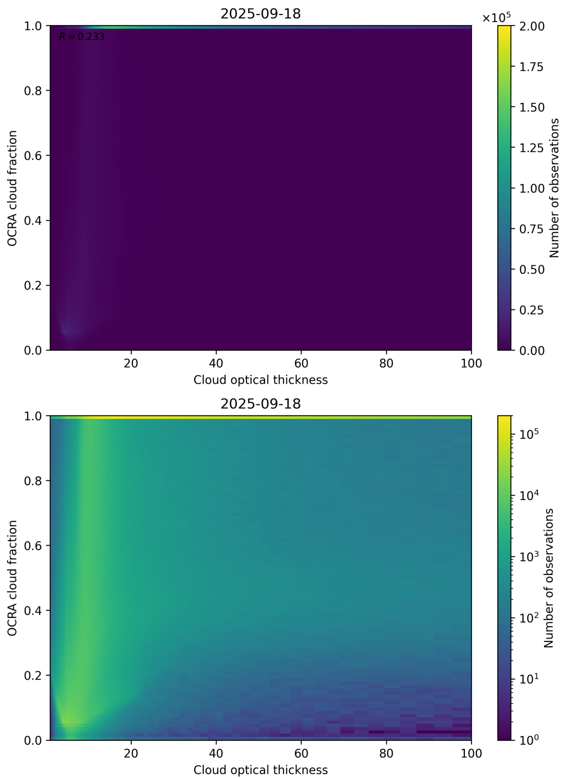
Figure 83: Scatter density plot of “Cloud optical thickness” against “OCRA cloud fraction” for 2025-09-17 to 2025-09-19.
