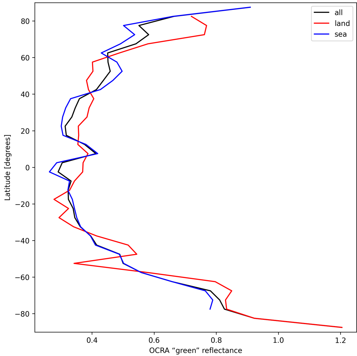
Figure 36: Zonal average of “OCRA “green” reflectance” for 2025-09-17 to 2025-09-19.
