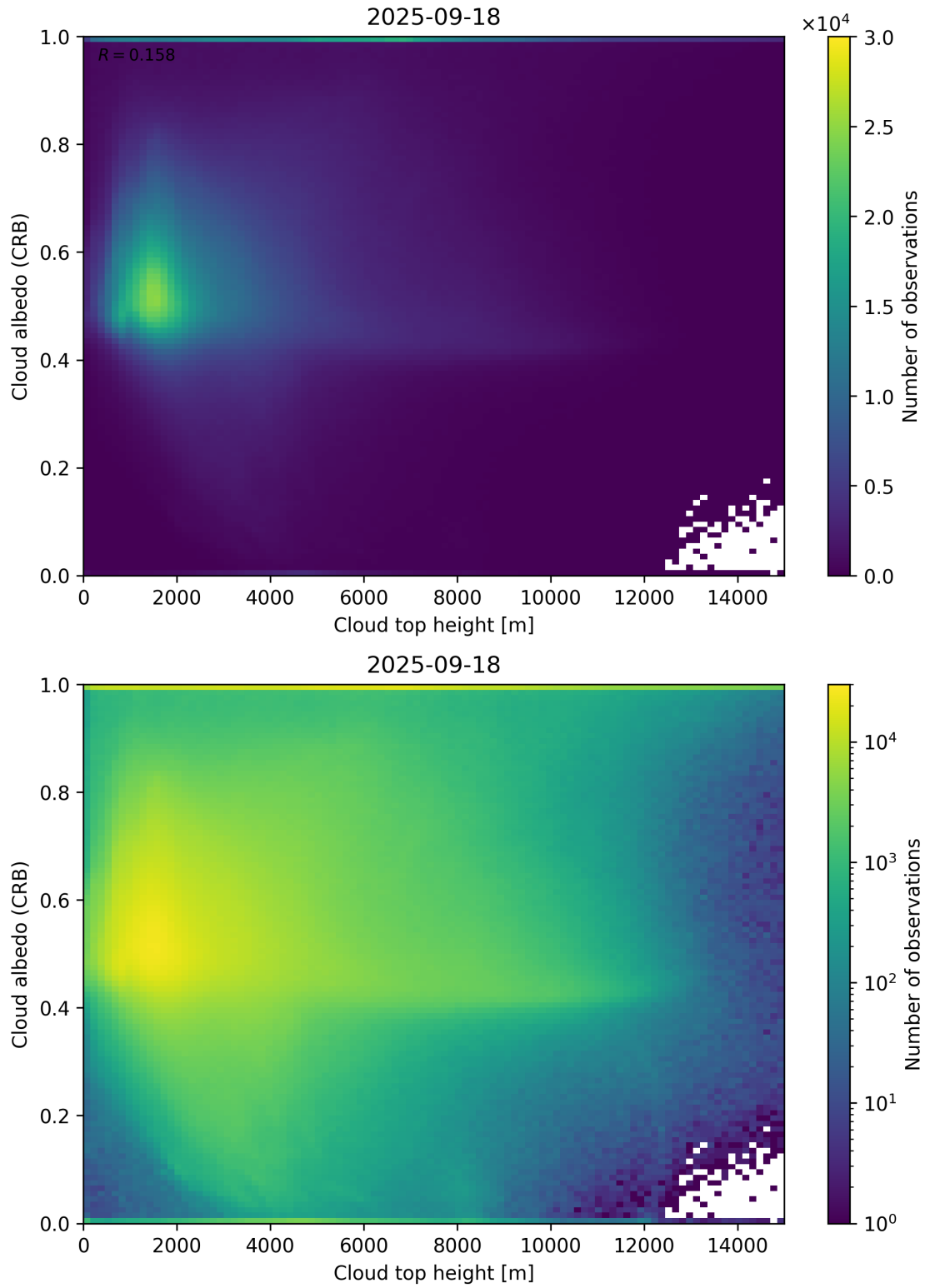
Figure 86: Scatter density plot of “Cloud top height” against “Cloud albedo (CRB)” for 2025-09-17 to 2025-09-19.
