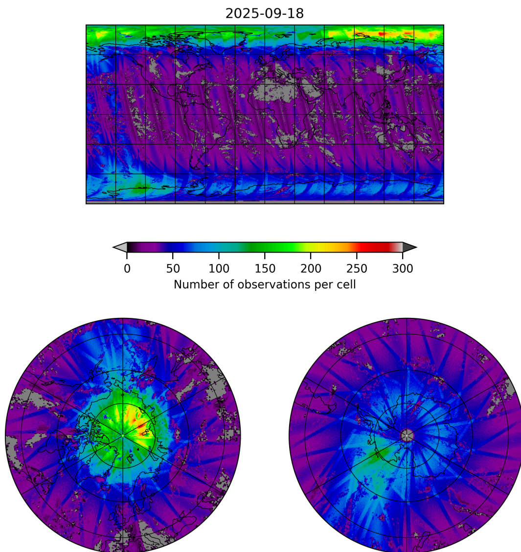
Figure 21: Map of the number of observations for 2025-09-17 to 2025-09-19
