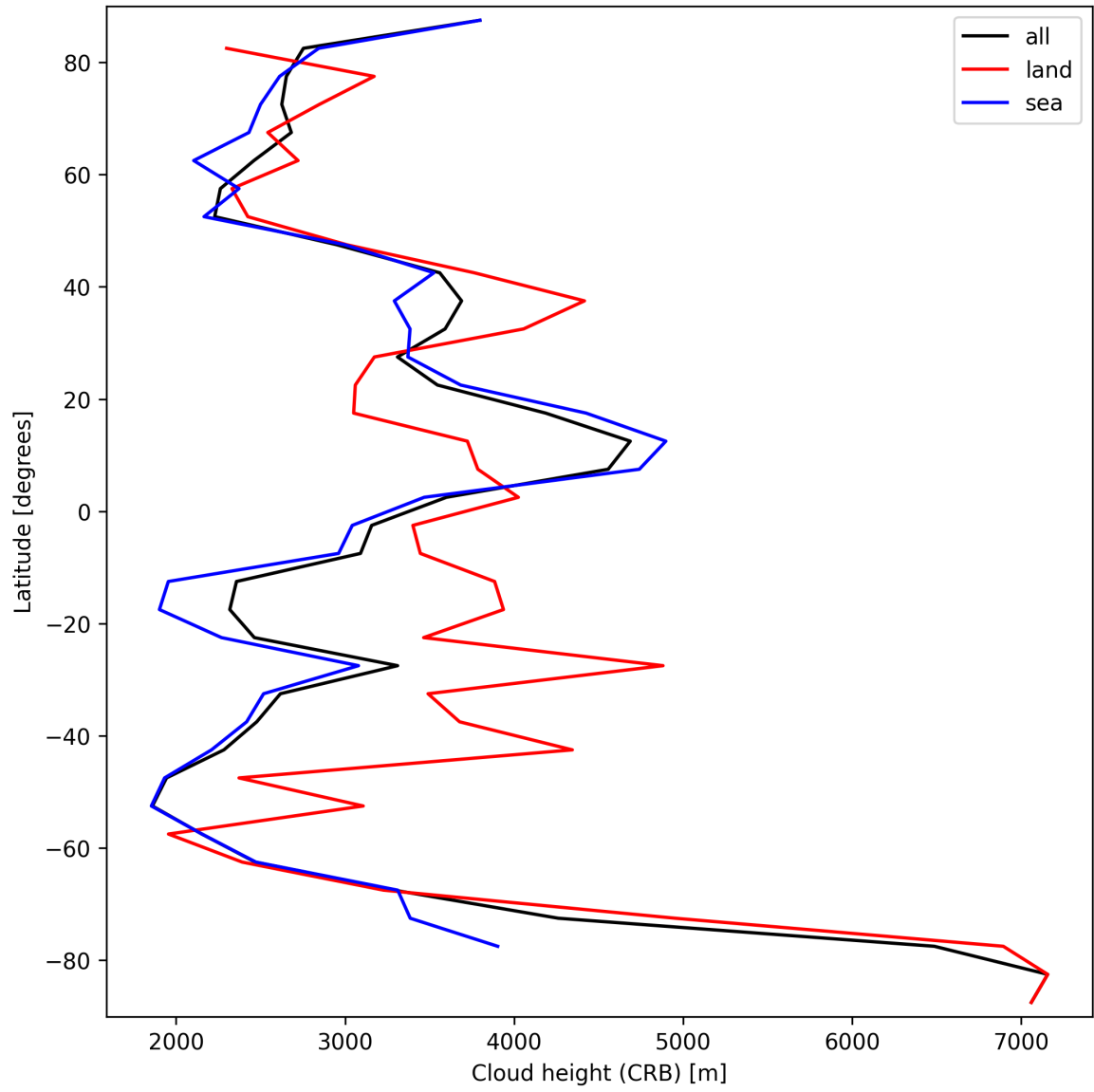
Figure 27: Zonal average of “Cloud height (CRB)” for 2025-09-17 to 2025-09-19.
