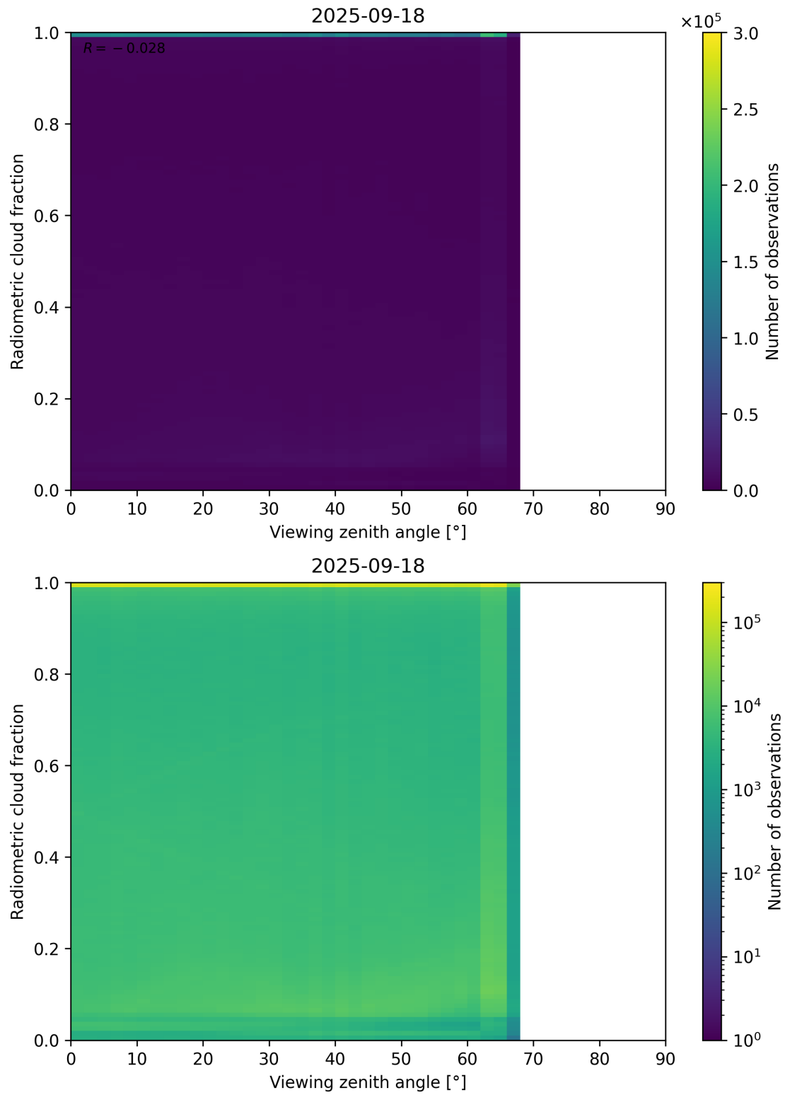
Figure 107: Scatter density plot of “Viewing zenith angle” against “Radiometric cloud fraction” for 2025-09-17 to 2025-09-19.
