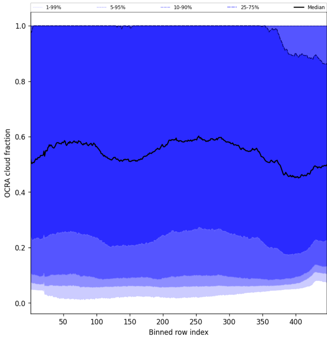
Figure 66: Along track statistics of “OCRA cloud fraction” for 2025-09-17 to 2025-09-19
