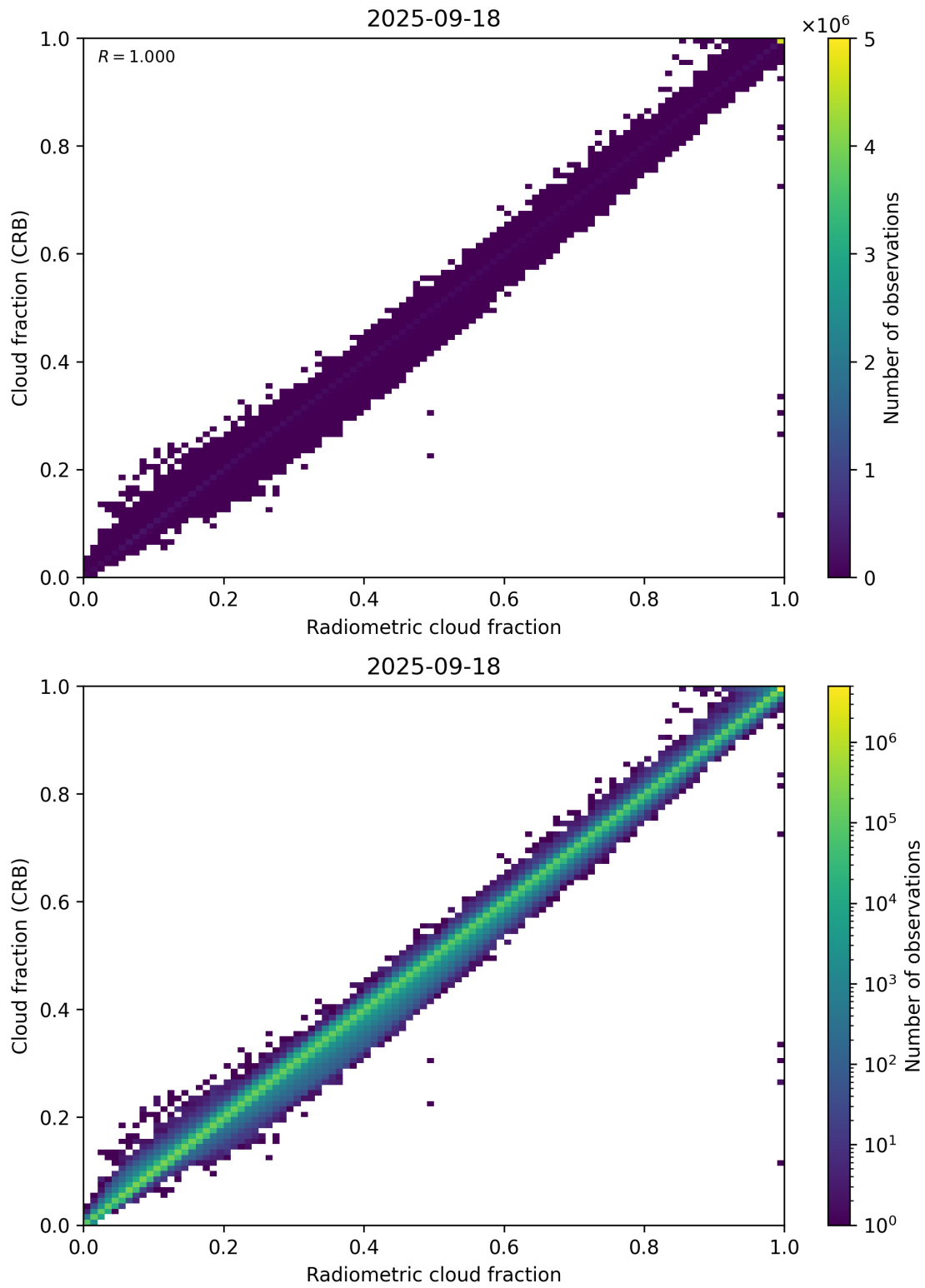
Figure 73: Scatter density plot of “Radiometric cloud fraction” against “Cloud fraction (CRB)” for 2025-09-17 to 2025-09-19.
