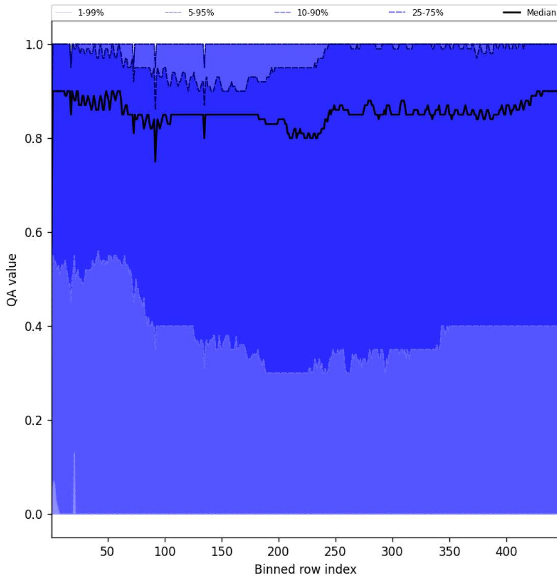
Figure 54: Along track statistics of “QA value” for 2025-09-17 to 2025-09-19
