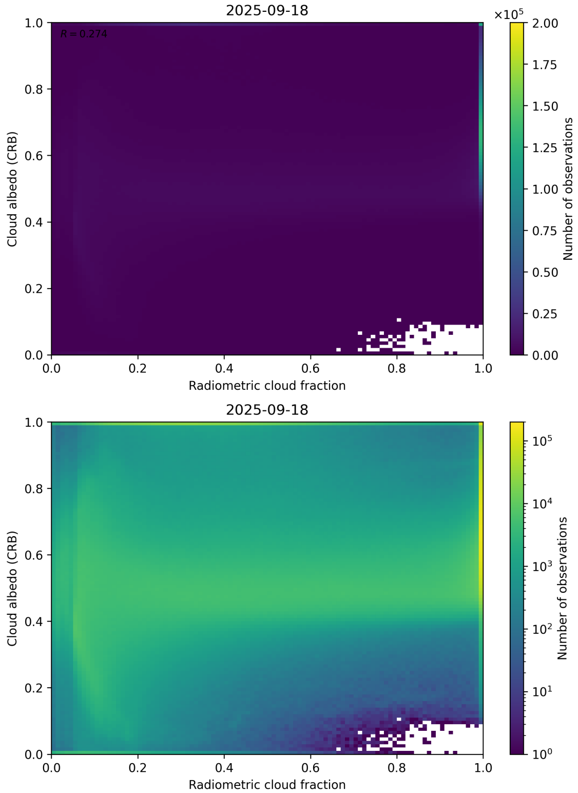
Figure 71: Scatter density plot of “Radiometric cloud fraction” against “Cloud albedo (CRB)” for 2025-09-17 to 2025-09-19.
