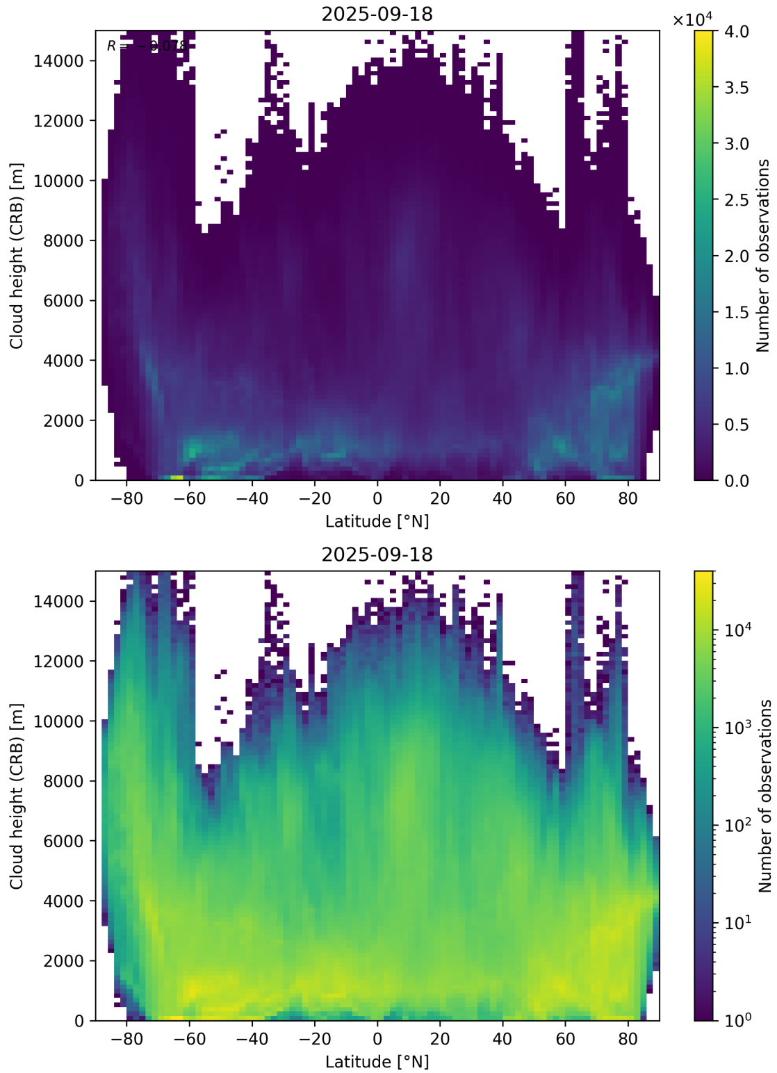
Figure 95: Scatter density plot of “Latitude” against “Cloud height (CRB)” for 2025-09-17 to 2025-09-19.
