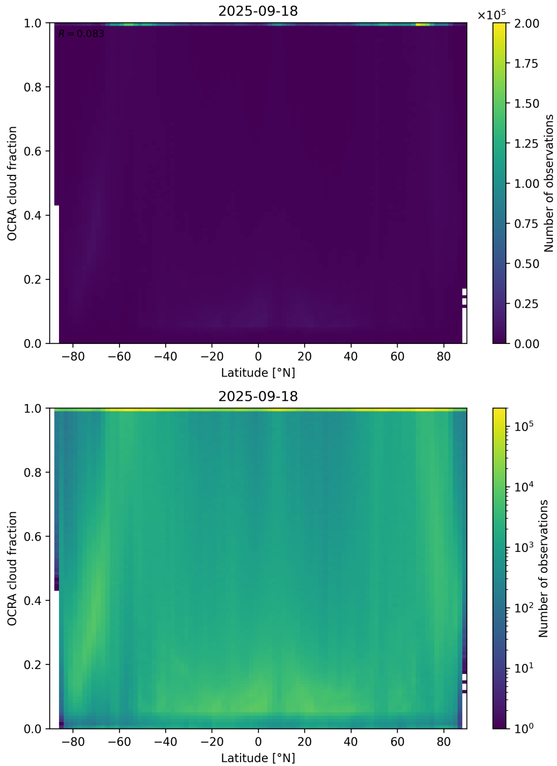
Figure 93: Scatter density plot of “Latitude” against “OCRA cloud fraction” for 2025-09-17 to 2025-09-19.
