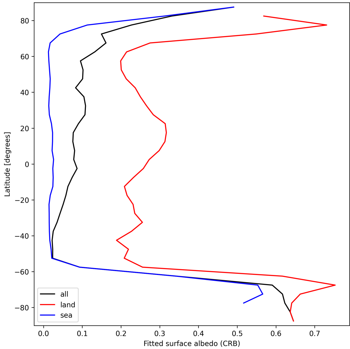
Figure 30: Zonal average of “Fitted surface albedo (CRB)” for 2025-09-17 to 2025-09-19.
