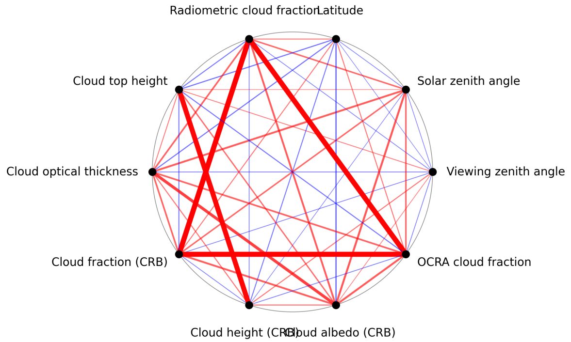
Figure 1: Map of correlation graph for 2025-09-17 to 2025-09-19.
