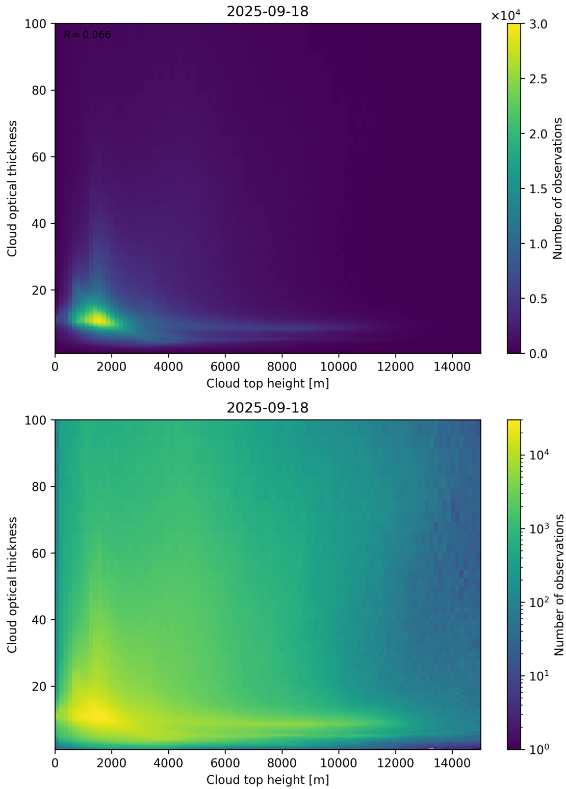
Figure 90: Scatter density plot of “Cloud top height” against “Cloud optical thickness” for 2025-09-17 to 2025-09-19.
