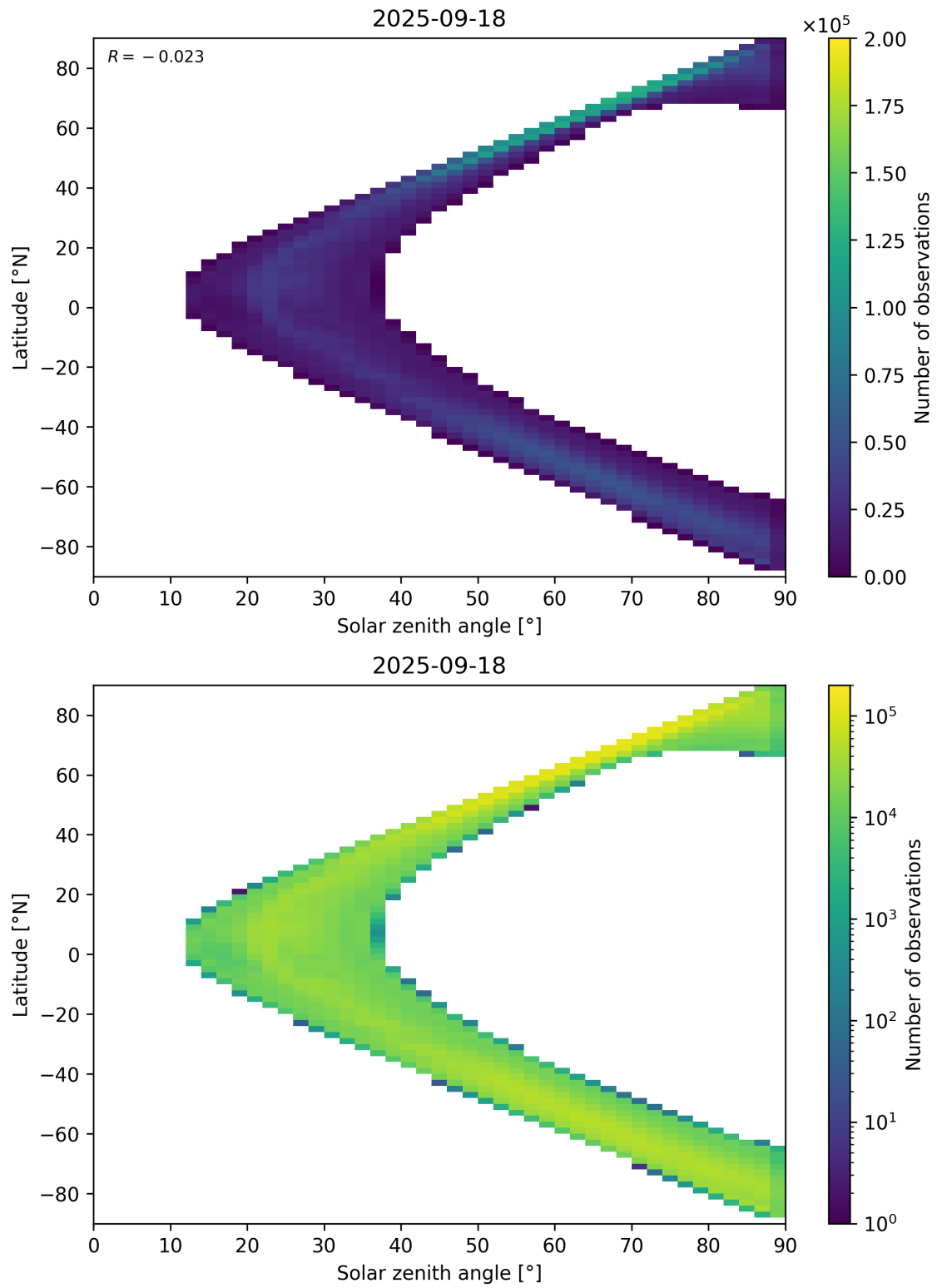
Figure 105: Scatter density plot of “Solar zenith angle” against “Latitude” for 2025-09-17 to 2025-09-19.
