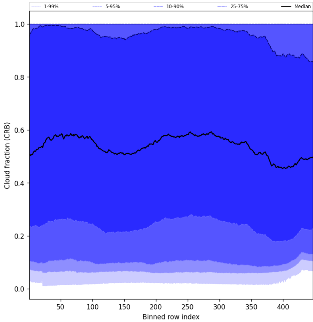
Figure 58: Along track statistics of “Cloud fraction (CRB)” for 2025-09-17 to 2025-09-19
