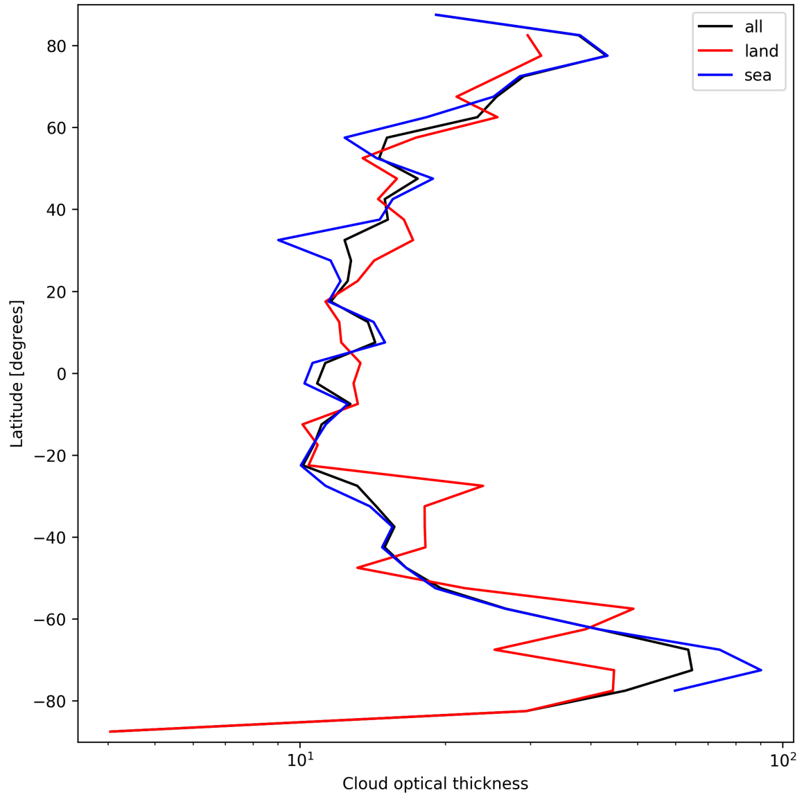
Figure 25: Zonal average of “Cloud optical thickness” for 2025-09-20 to 2025-09-22.
