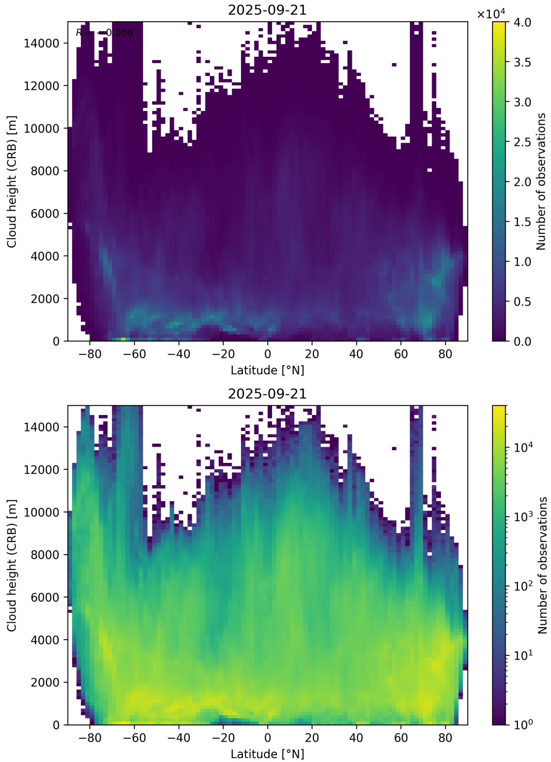
Figure 95: Scatter density plot of “Latitude” against “Cloud height (CRB)” for 2025-09-20 to 2025-09-22.
