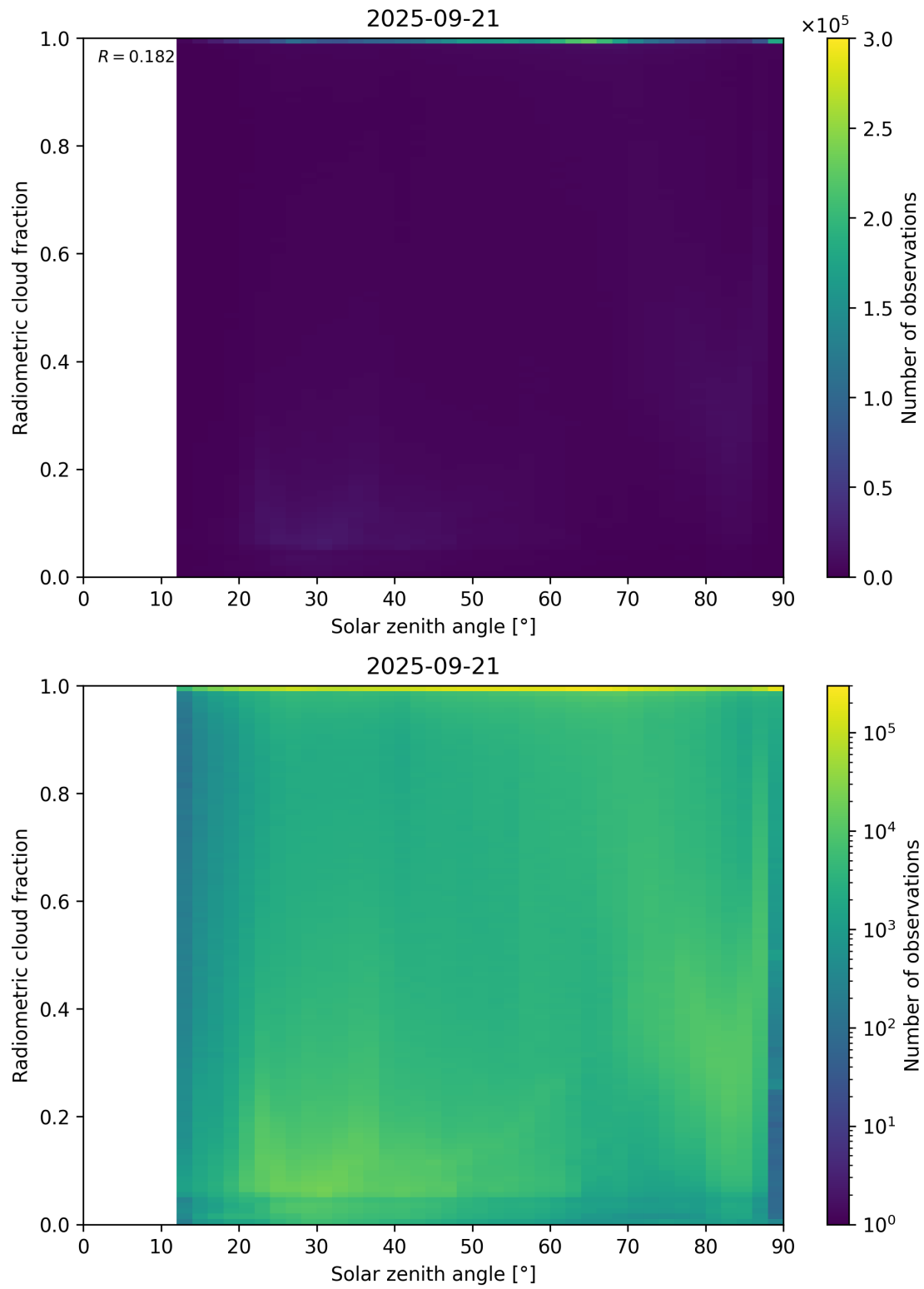
Figure 99: Scatter density plot of “Solar zenith angle” against “Radiometric cloud fraction” for 2025-09-20 to 2025-09-22.
