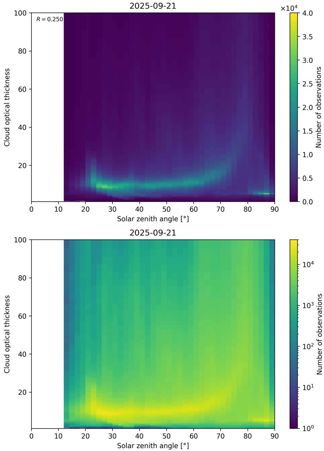
Figure 103: Scatter density plot of “Solar zenith angle” against “Cloud optical thickness” for 2025-09-20 to 2025-09-22.
