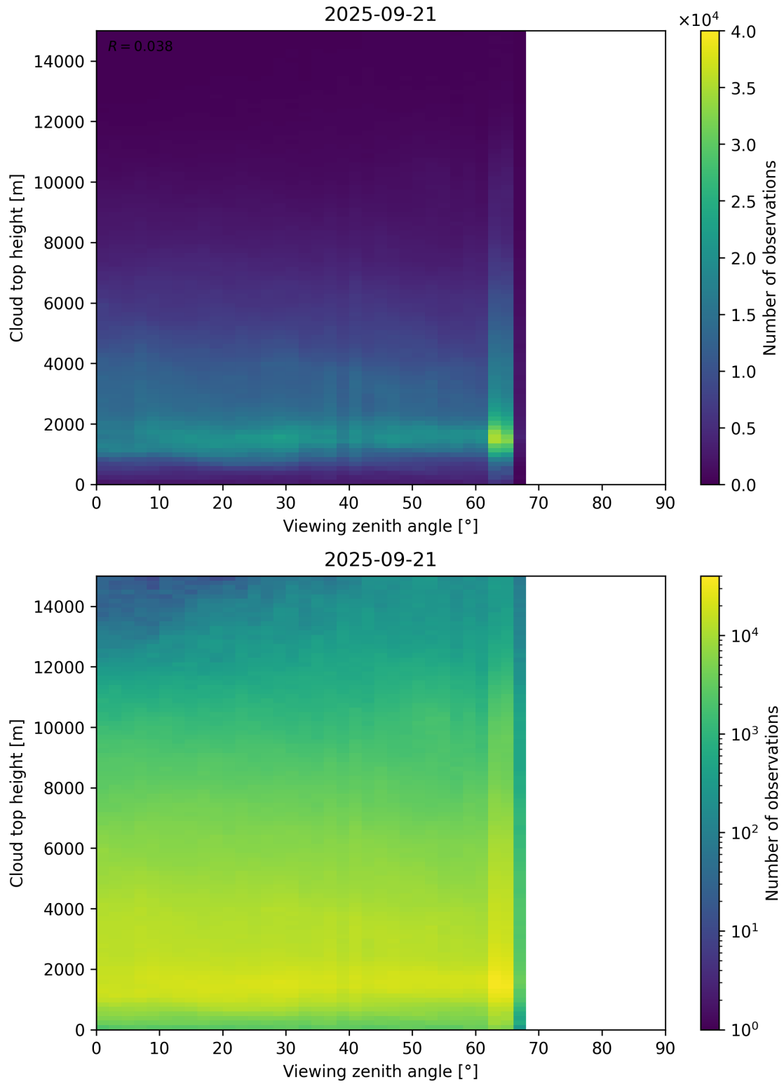
Figure 112: Scatter density plot of “Viewing zenith angle” against “Cloud top height” for 2025-09-20 to 2025-09-22.
