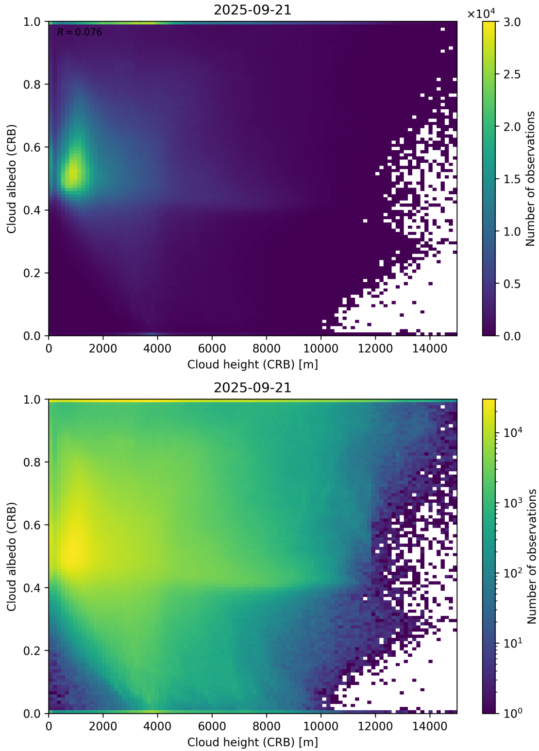
Figure 80: Scatter density plot of “Cloud height (CRB)” against “Cloud albedo (CRB)” for 2025-09-20 to 2025-09-22.
