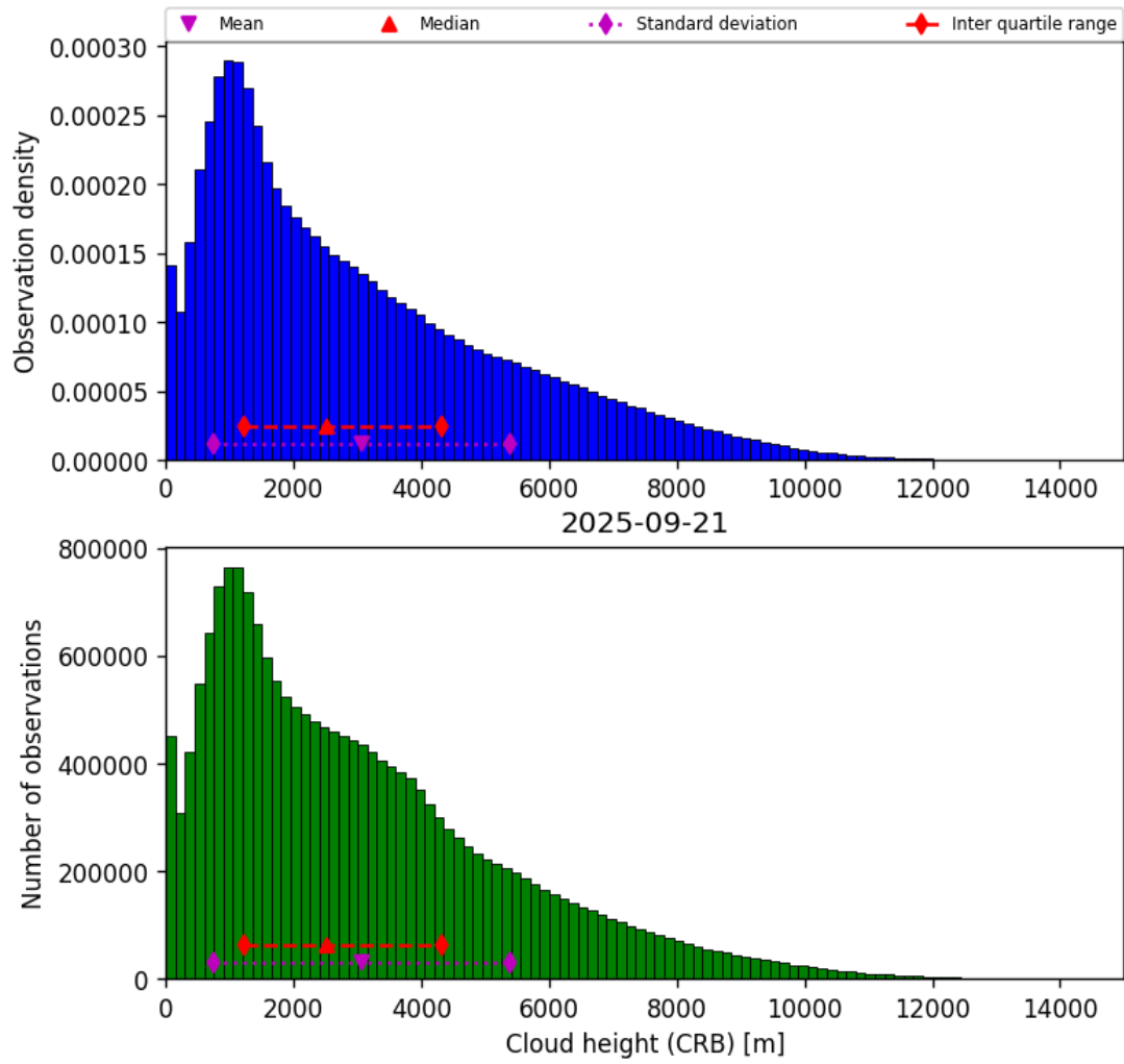
Figure 43: Histogram of “Cloud height (CRB)” for 2025-09-20 to 2025-09-22
