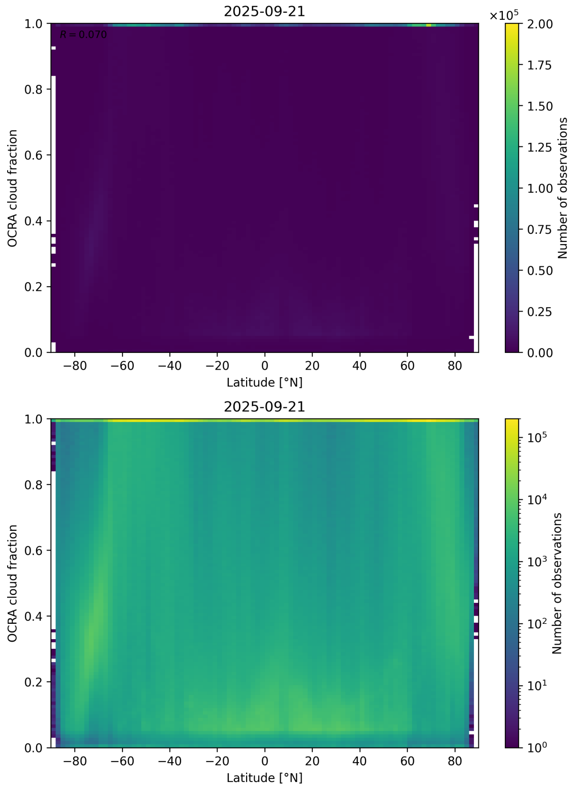
Figure 93: Scatter density plot of “Latitude” against “OCRA cloud fraction” for 2025-09-20 to 2025-09-22.
