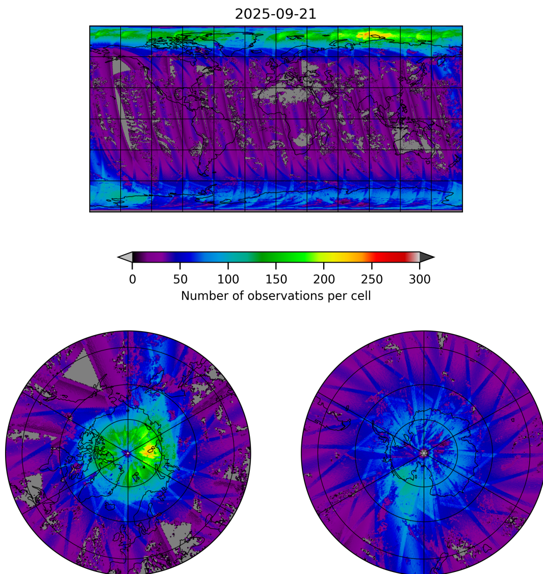
Figure 21: Map of the number of observations for 2025-09-20 to 2025-09-22
