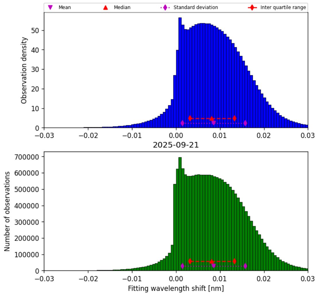
Figure 49: Histogram of “Fitting wavelength shift” for 2025-09-20 to 2025-09-22
