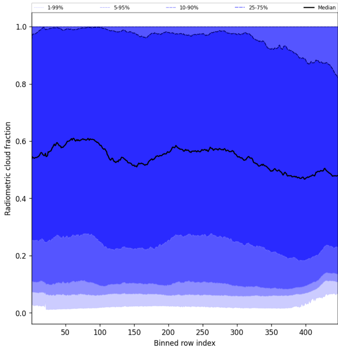
Figure 55: Along track statistics of “Radiometric cloud fraction” for 2025-09-20 to 2025-09-22
