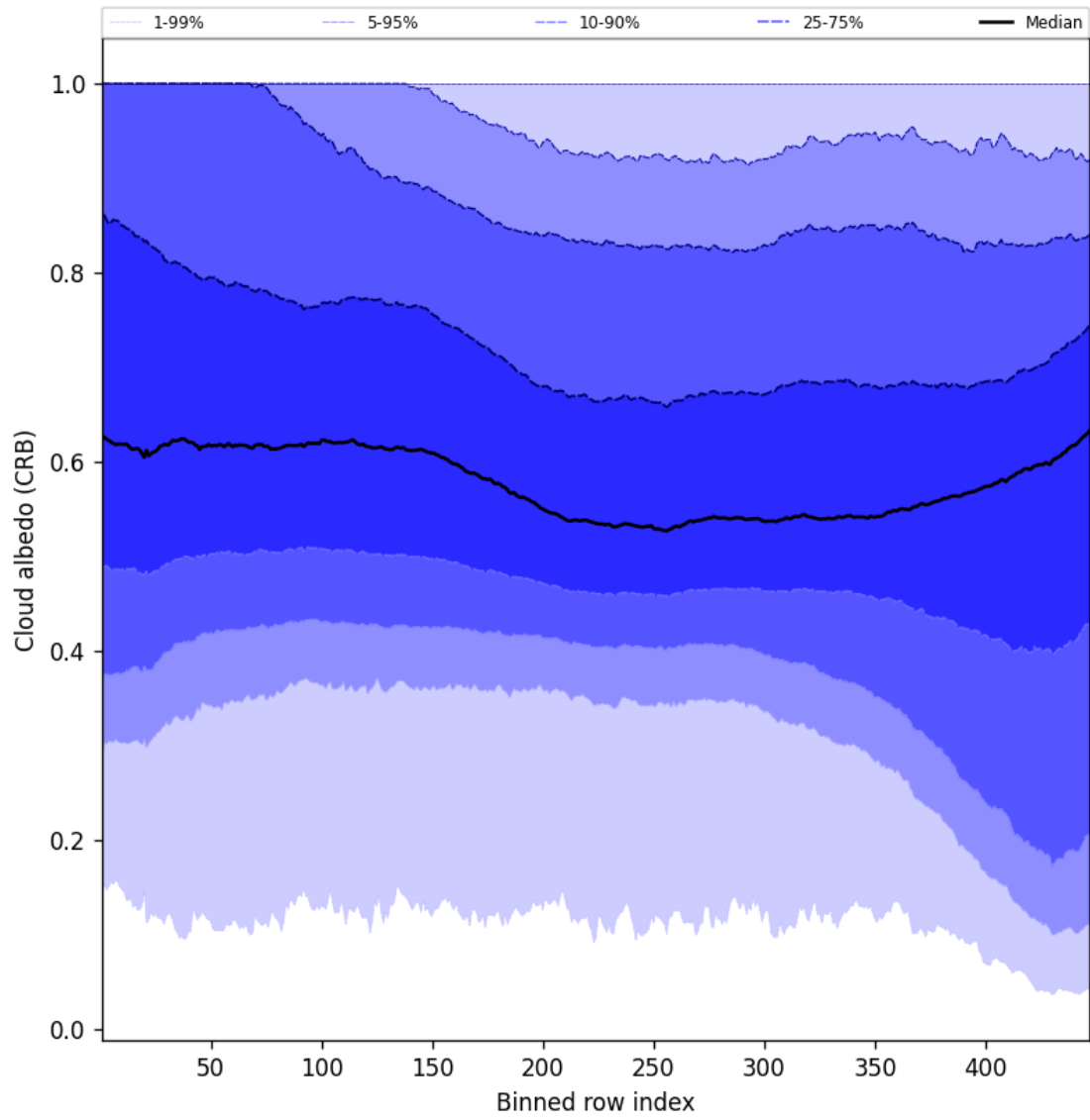
Figure 60: Along track statistics of “Cloud albedo (CRB)” for 2025-09-20 to 2025-09-22
