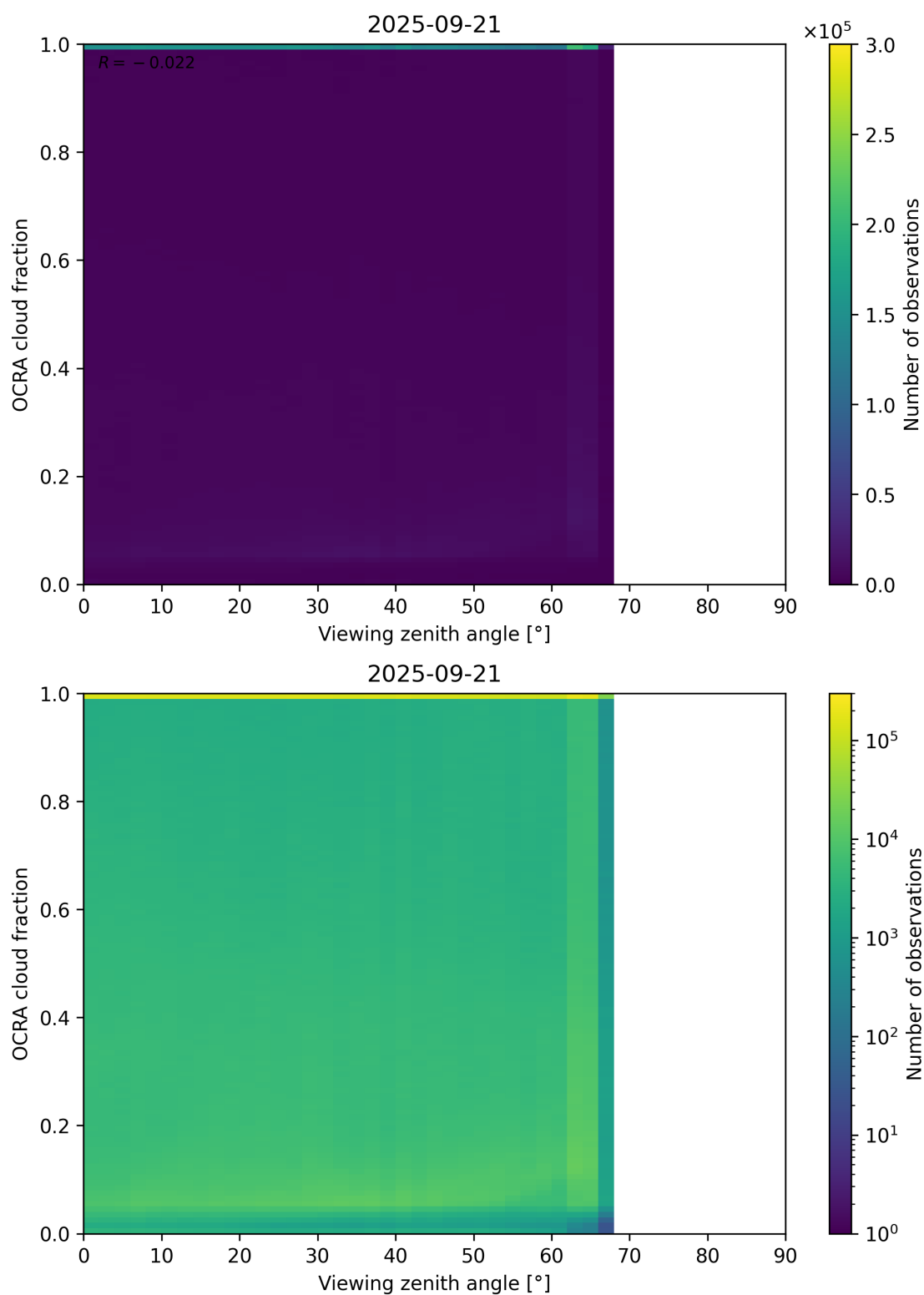
Figure 108: Scatter density plot of “Viewing zenith angle” against “OCRA cloud fraction” for 2025-09-20 to 2025-09-22.
