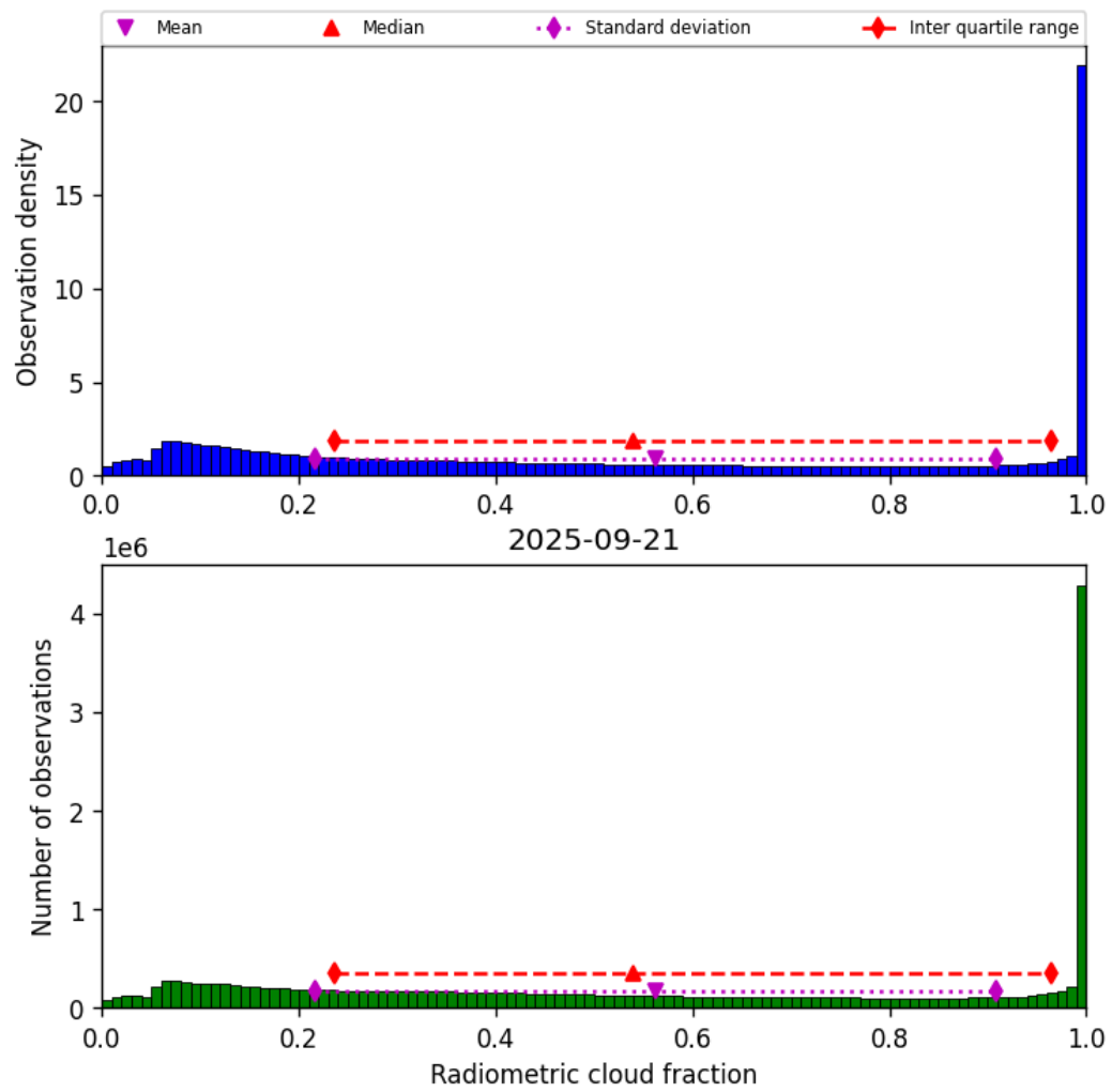
Figure 39: Histogram of “Radiometric cloud fraction” for 2025-09-20 to 2025-09-22
