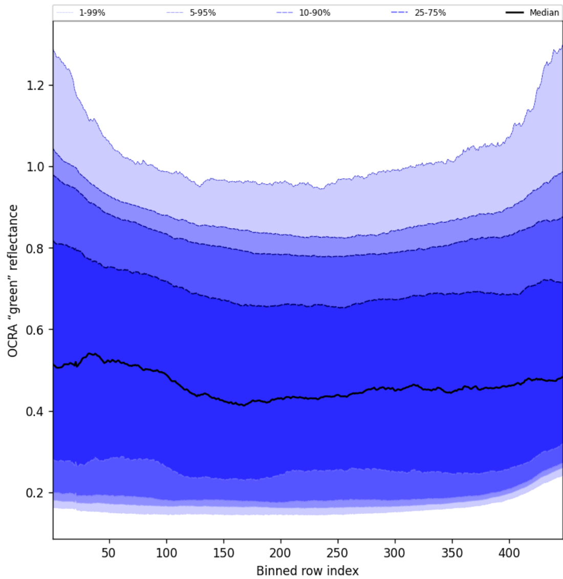
Figure 68: Along track statistics of “OCRA “green” reflectance” for 2025-09-20 to 2025-09-22
