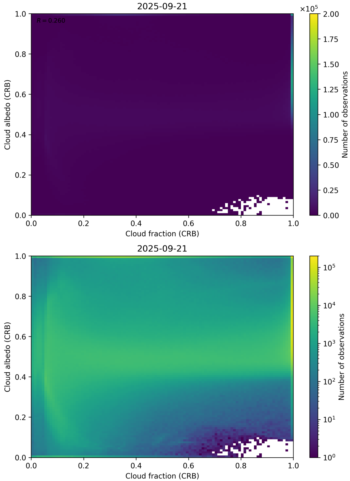
Figure 77: Scatter density plot of “Cloud fraction (CRB)” against “Cloud albedo (CRB)” for 2025-09-20 to 2025-09-22.
