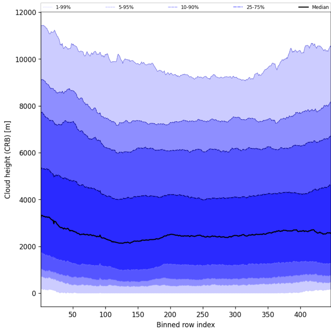
Figure 59: Along track statistics of “Cloud height (CRB)” for 2025-09-20 to 2025-09-22
