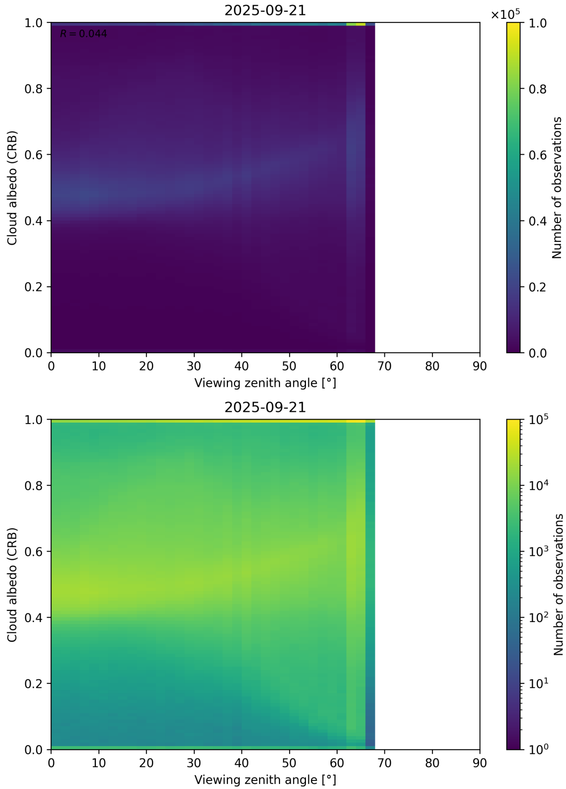
Figure 106: Scatter density plot of “Viewing zenith angle” against “Cloud albedo (CRB)” for 2025-09-20 to 2025-09-22.
