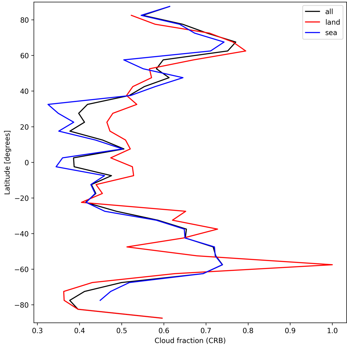
Figure 26: Zonal average of “Cloud fraction (CRB)” for 2025-09-20 to 2025-09-22.
