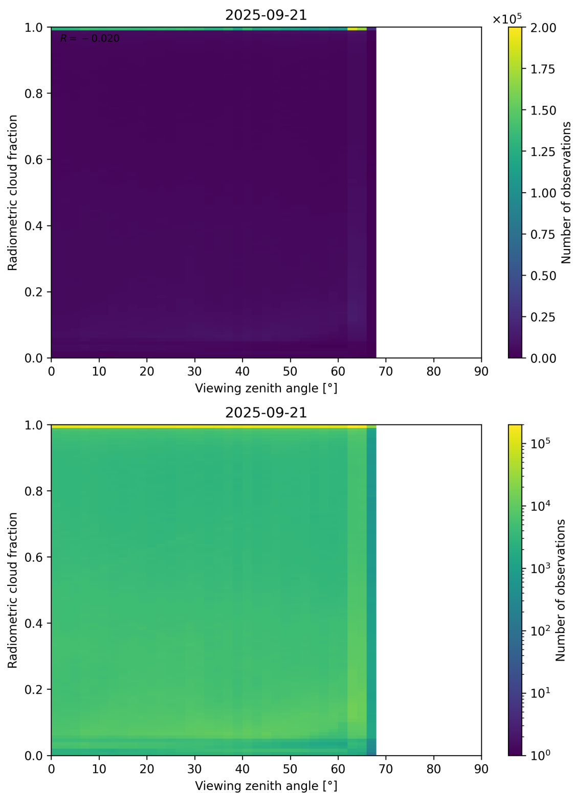
Figure 107: Scatter density plot of “Viewing zenith angle” against “Radiometric cloud fraction” for 2025-09-20 to 2025-09-22.
