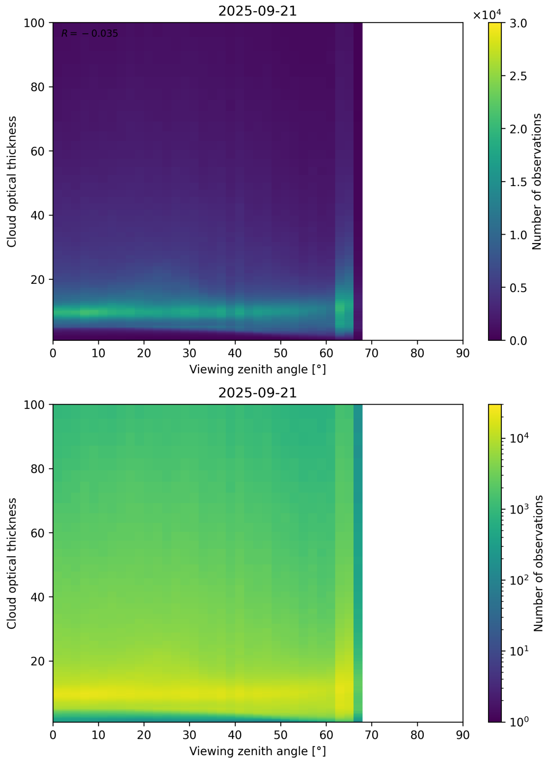
Figure 111: Scatter density plot of “Viewing zenith angle” against “Cloud optical thickness” for 2025-09-20 to 2025-09-22.
