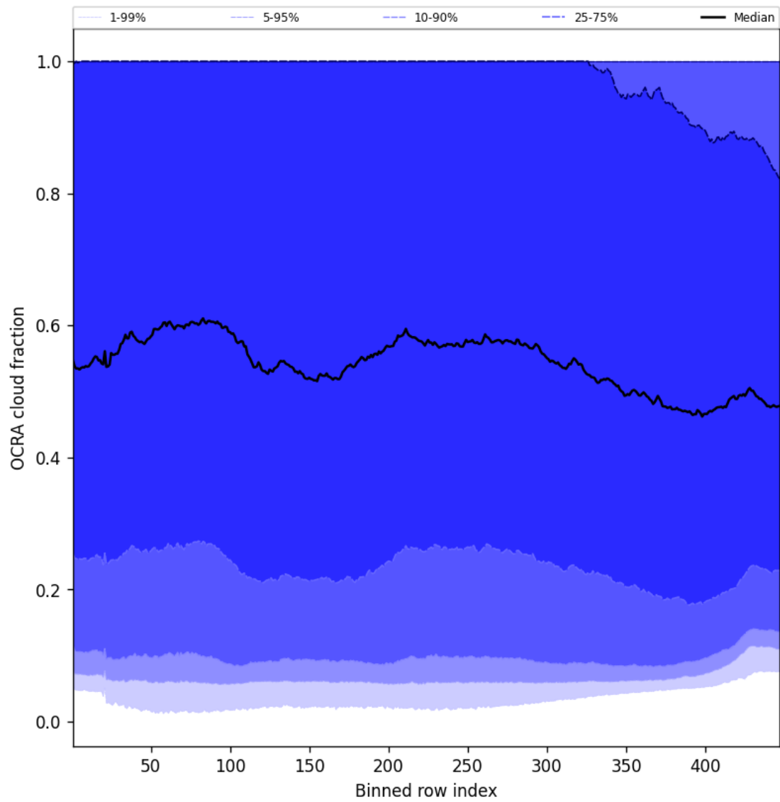
Figure 66: Along track statistics of “OCRA cloud fraction” for 2025-09-20 to 2025-09-22
