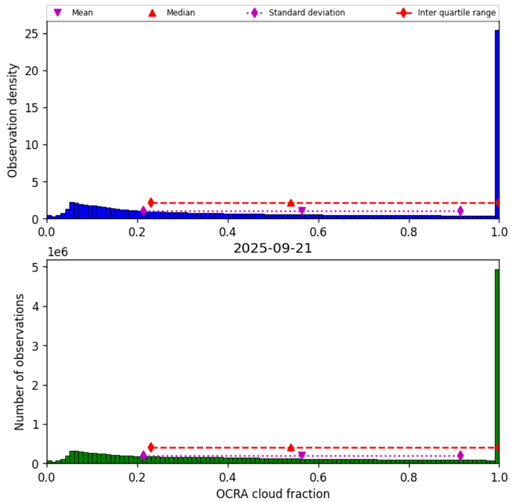
Figure 50: Histogram of “OCRA cloud fraction” for 2025-09-20 to 2025-09-22
