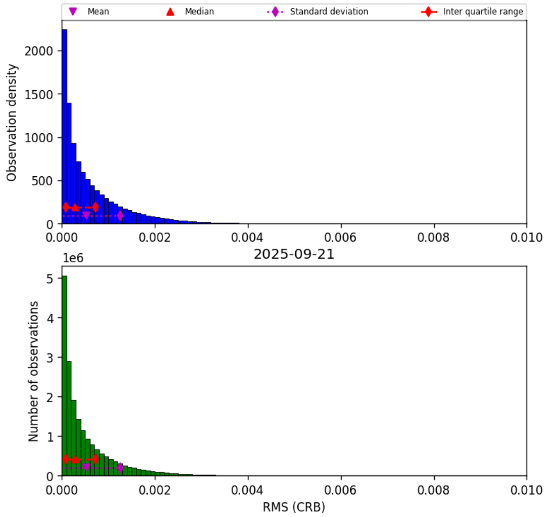
Figure 48: Histogram of “RMS (CRB)” for 2025-09-20 to 2025-09-22
