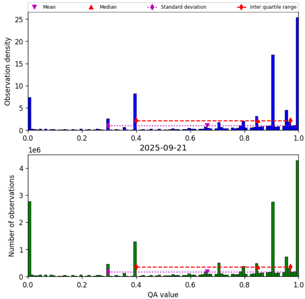
Figure 38: Histogram of “QA value” for 2025-09-20 to 2025-09-22
