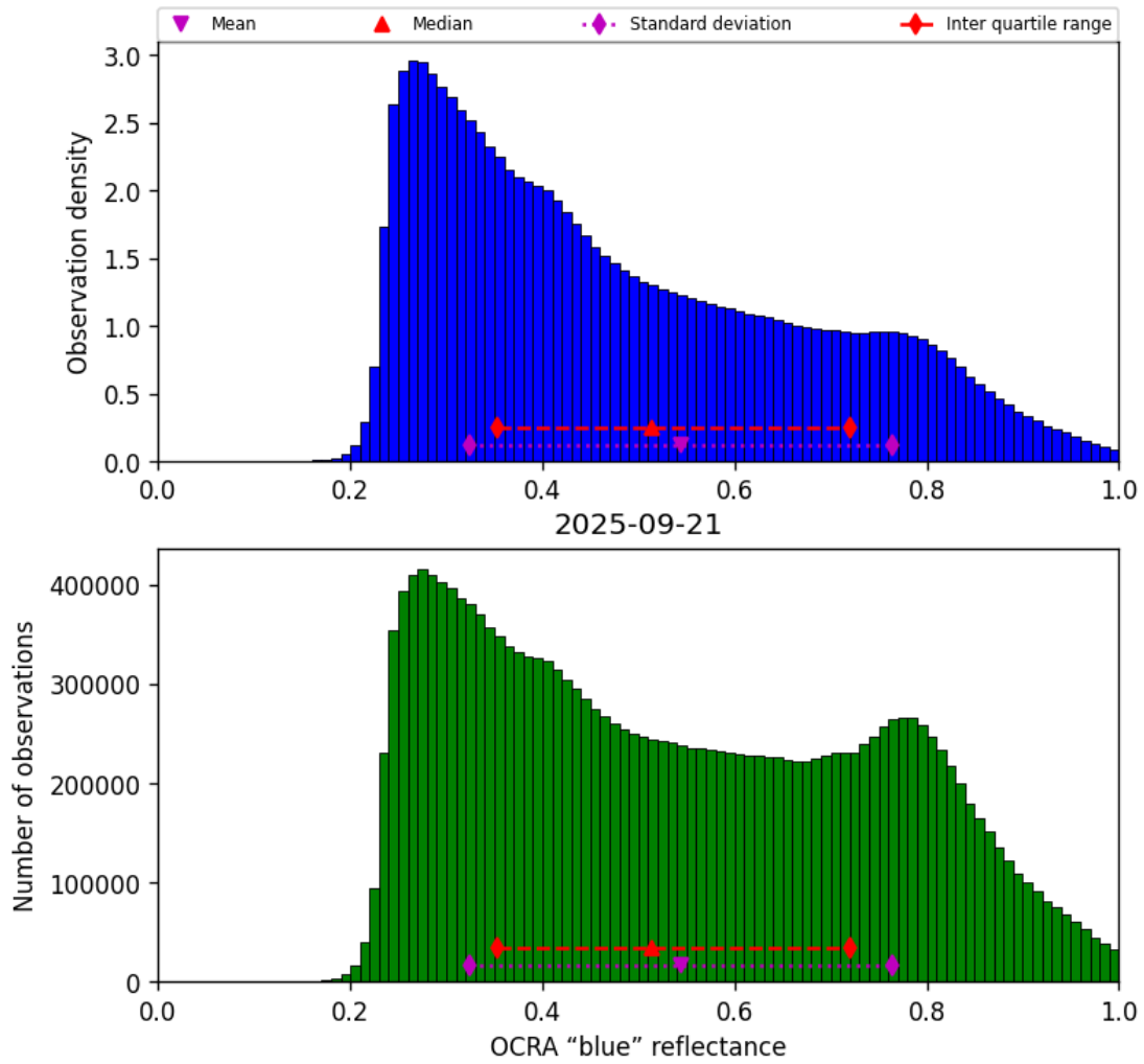
Figure 51: Histogram of “OCRA “blue” reflectance” for 2025-09-20 to 2025-09-22
