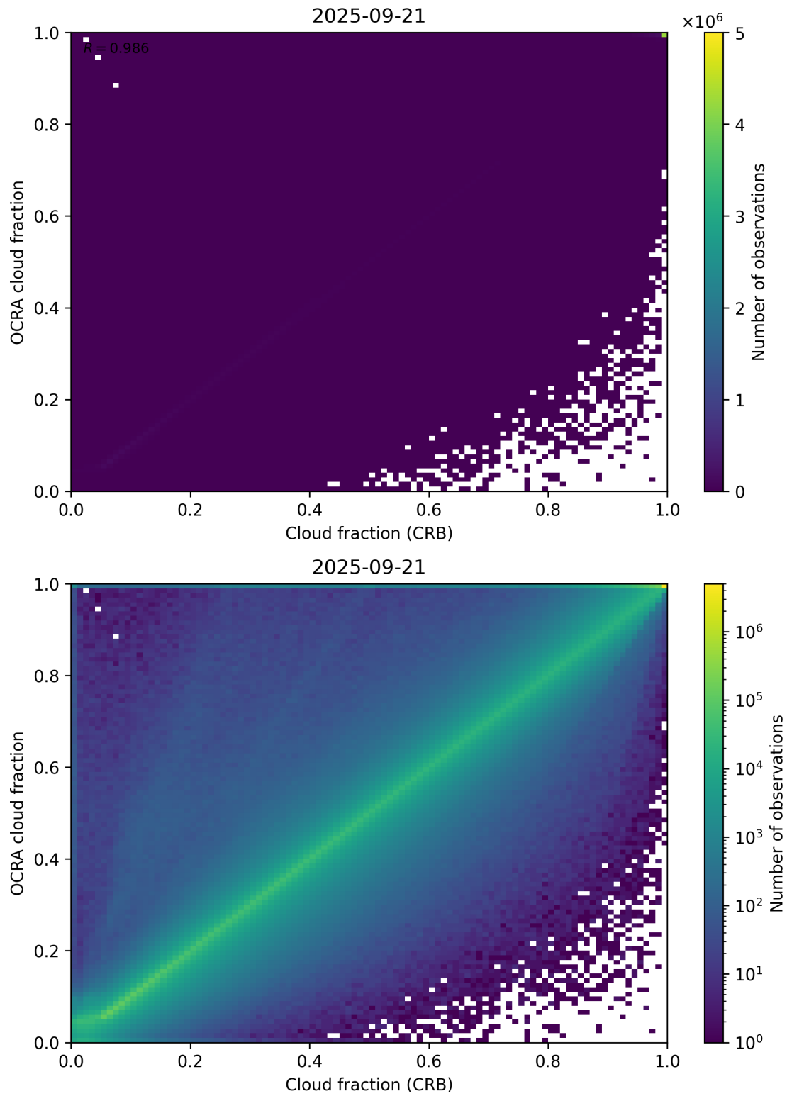
Figure 78: Scatter density plot of “Cloud fraction (CRB)” against “OCRA cloud fraction” for 2025-09-20 to 2025-09-22.
