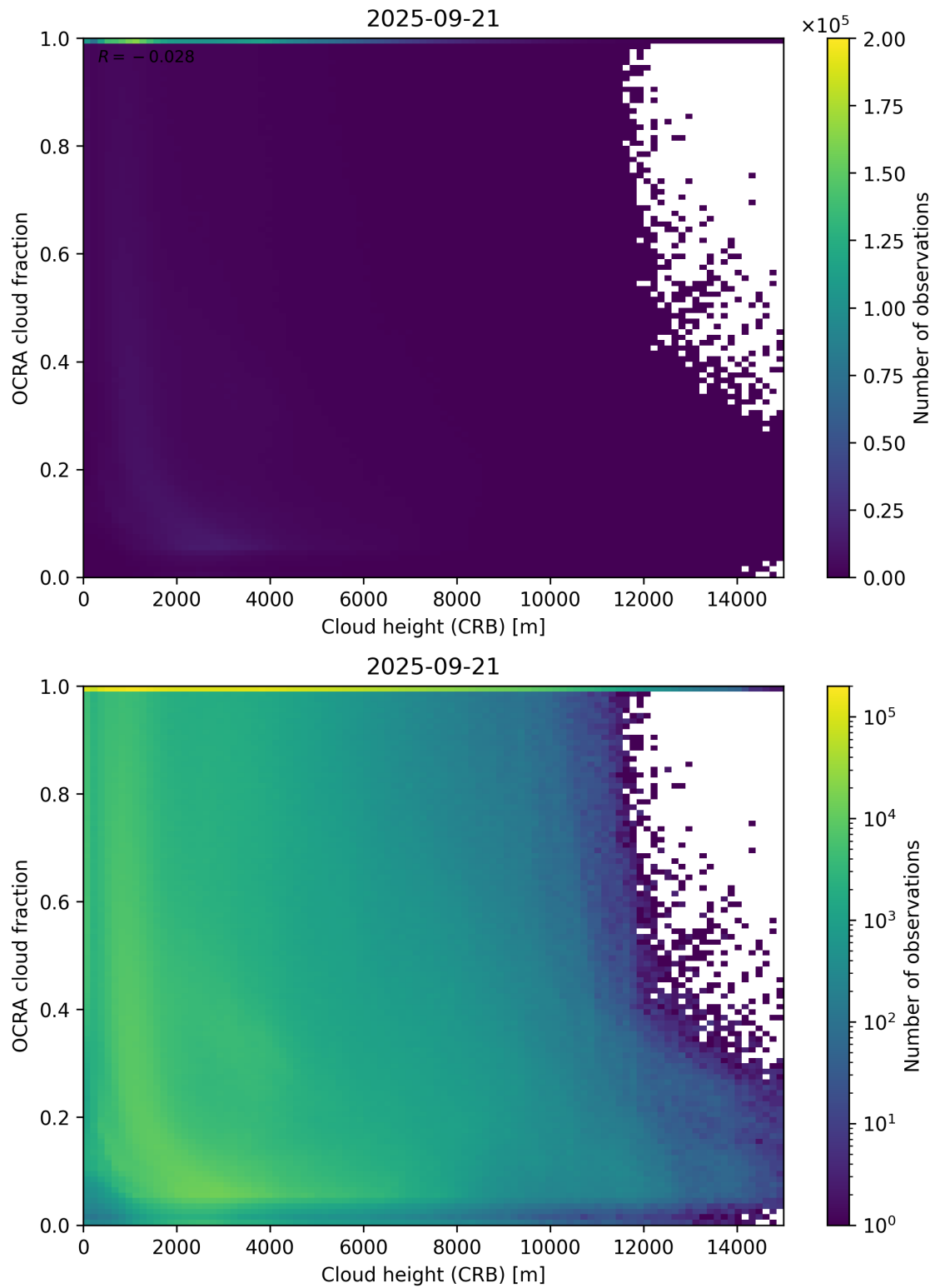
Figure 81: Scatter density plot of “Cloud height (CRB)” against “OCRA cloud fraction” for 2025-09-20 to 2025-09-22.
