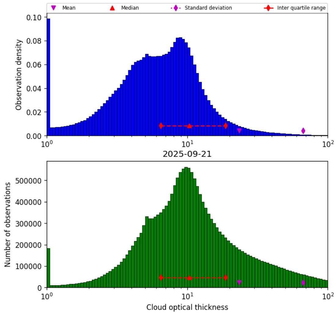
Figure 41: Histogram of “Cloud optical thickness” for 2025-09-20 to 2025-09-22
