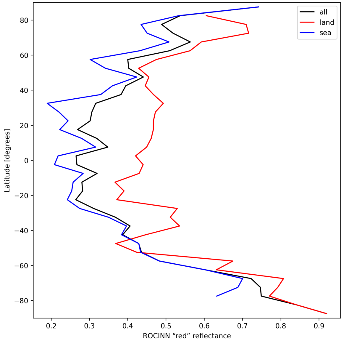
Figure 37: Zonal average of "ROCINN "red" reflectance" for 2025-09-20 to 2025-09-22.
