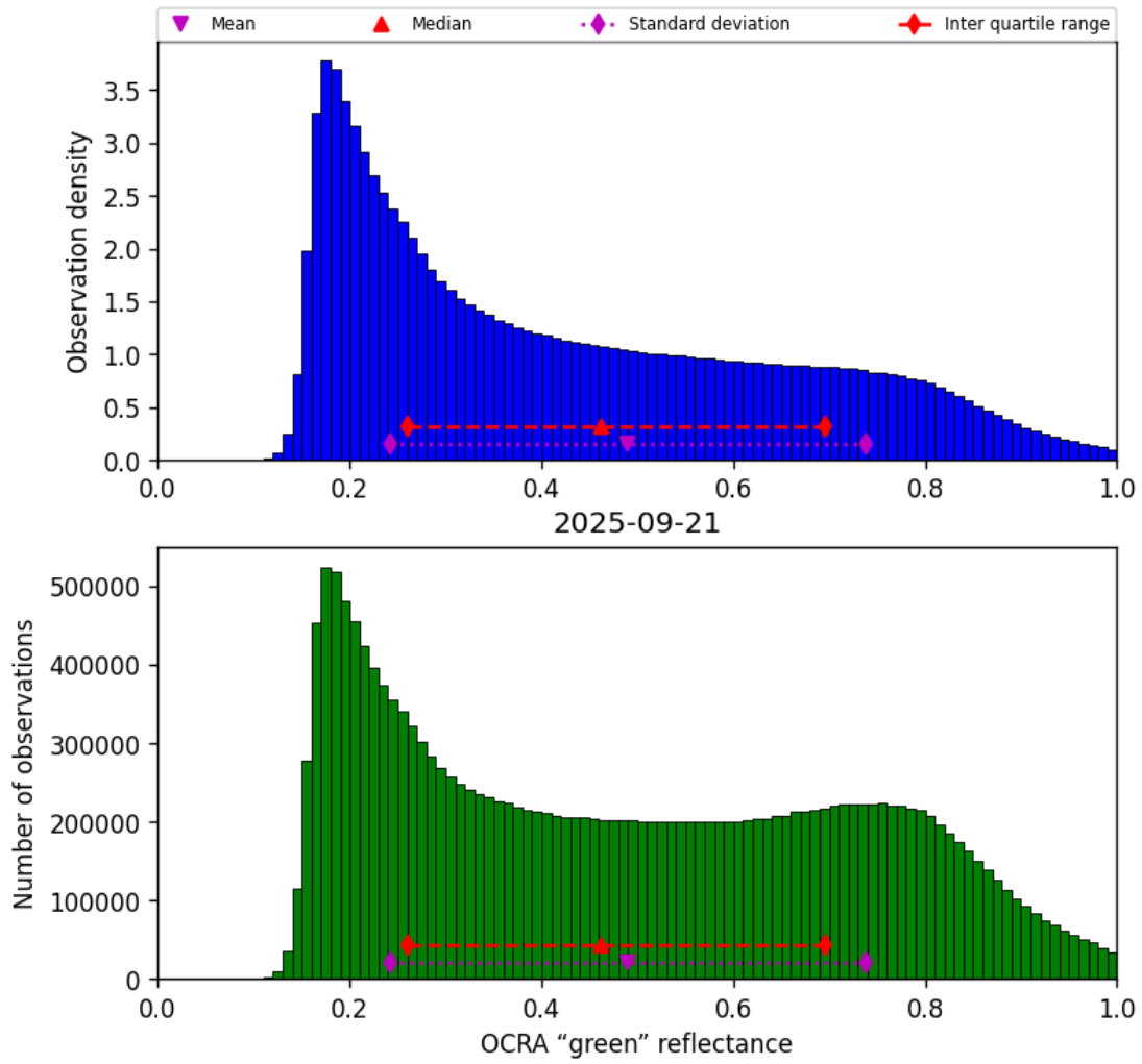
Figure 52: Histogram of “OCRA “green” reflectance” for 2025-09-20 to 2025-09-22
