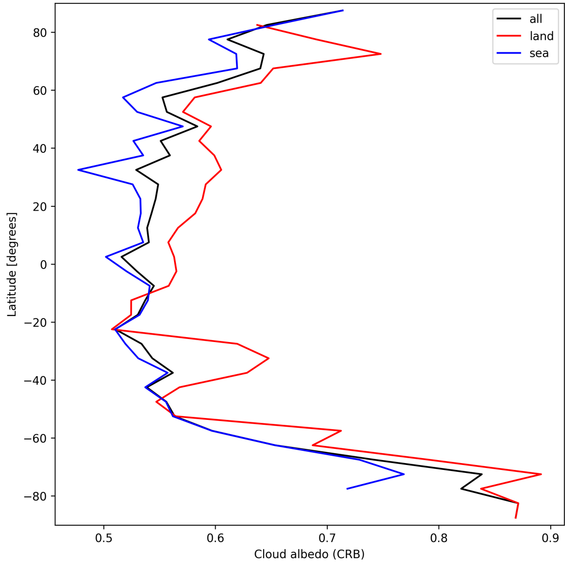
Figure 28: Zonal average of “Cloud albedo (CRB)” for 2025-09-20 to 2025-09-22.
