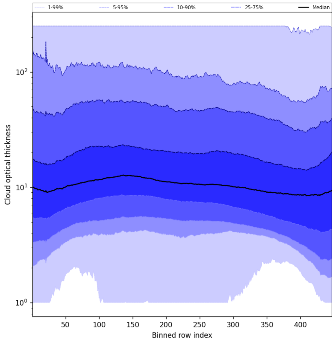
Figure 57: Along track statistics of “Cloud optical thickness” for 2025-09-20 to 2025-09-22
