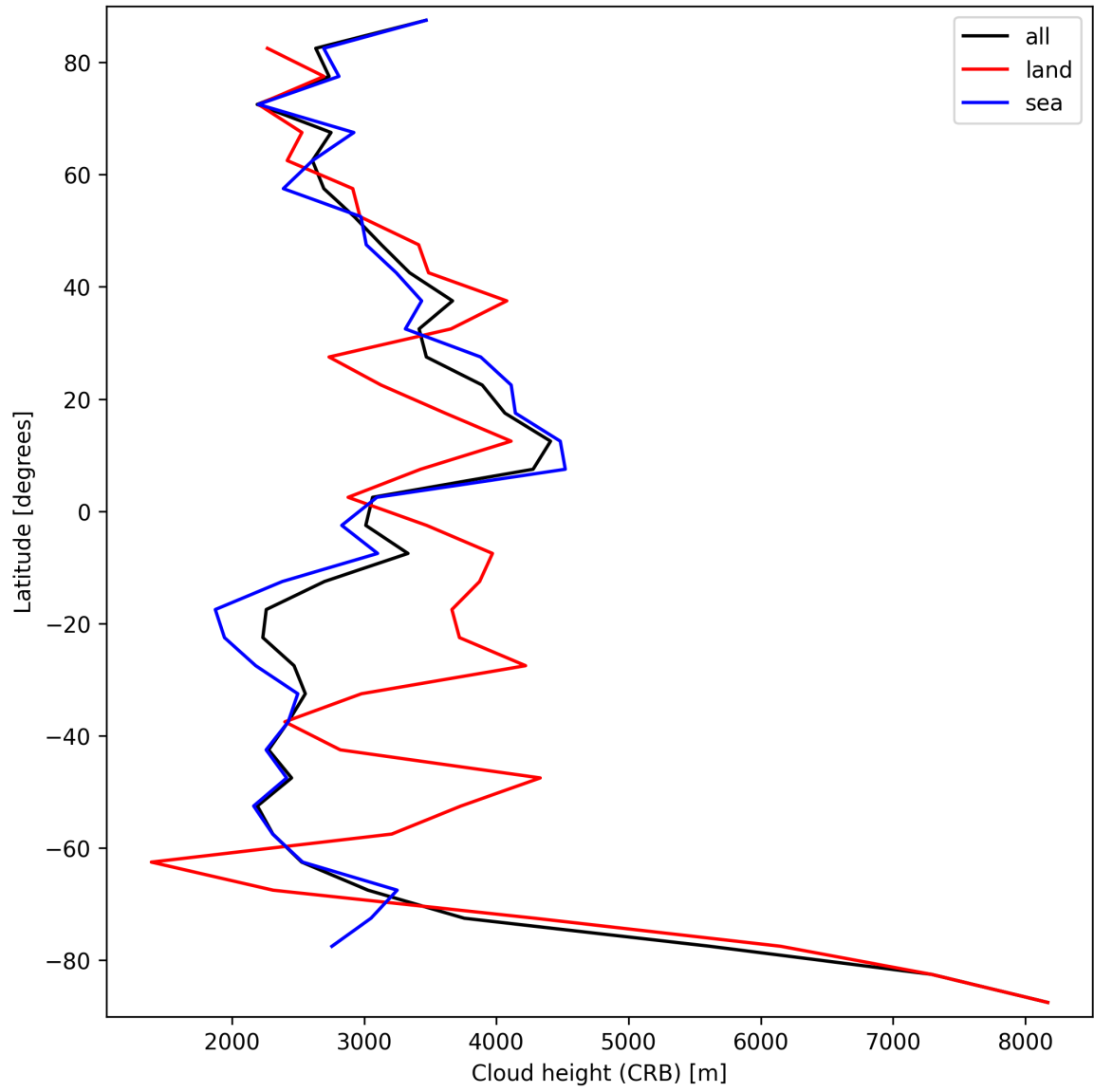
Figure 27: Zonal average of “Cloud height (CRB)” for 2025-09-20 to 2025-09-22.
