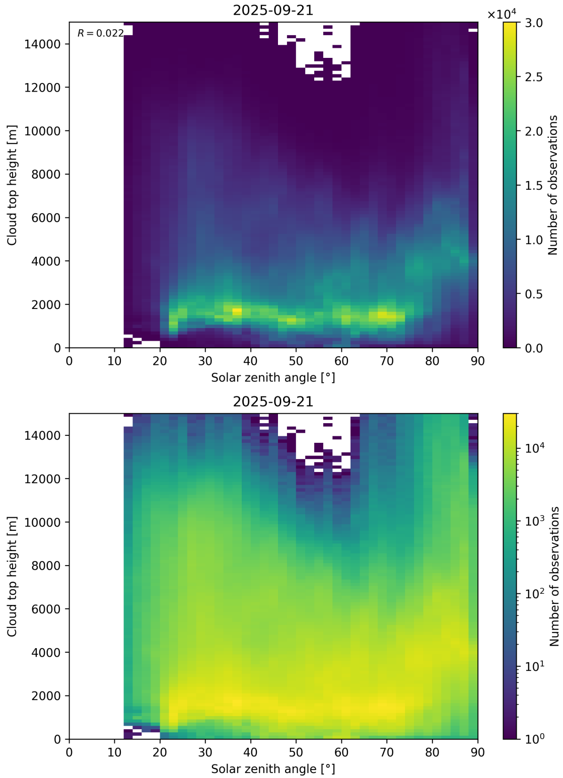
Figure 104: Scatter density plot of “Solar zenith angle” against “Cloud top height” for 2025-09-20 to 2025-09-22.
