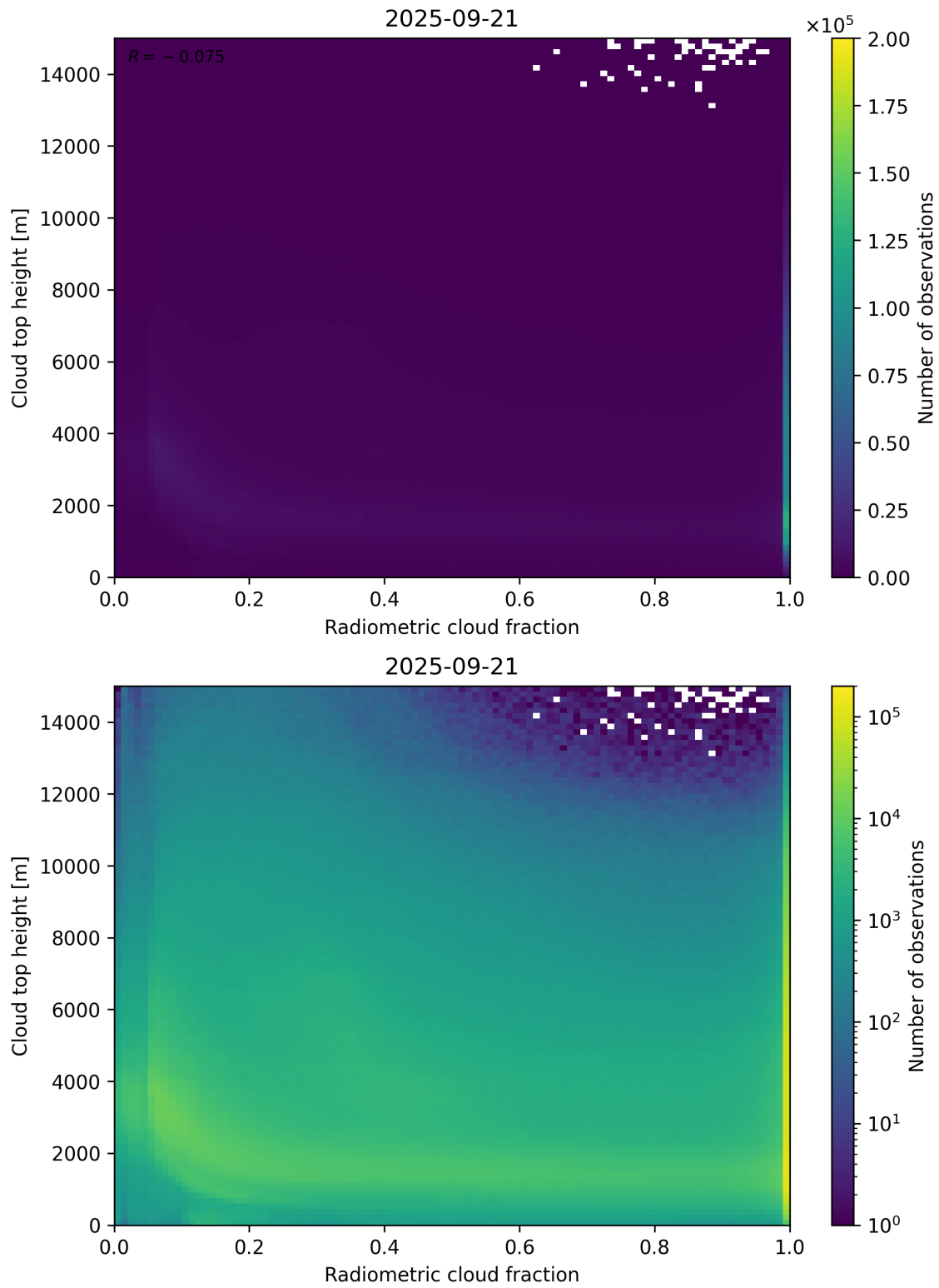
Figure 76: Scatter density plot of “Radiometric cloud fraction” against “Cloud top height” for 2025-09-20 to 2025-09-22.
