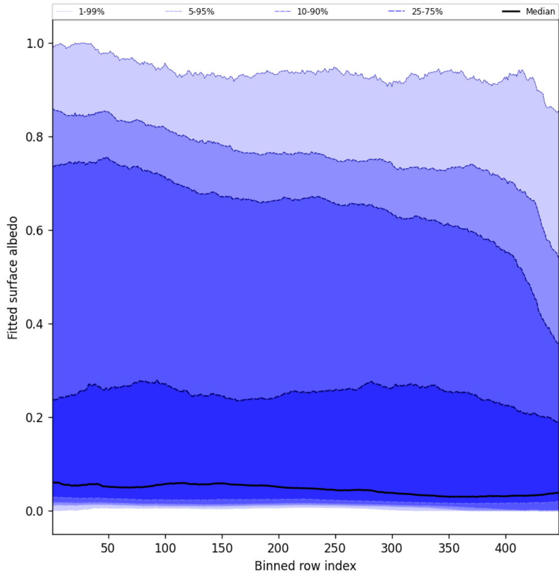
Figure 61: Along track statistics of “Fitted surface albedo” for 2025-09-20 to 2025-09-22
