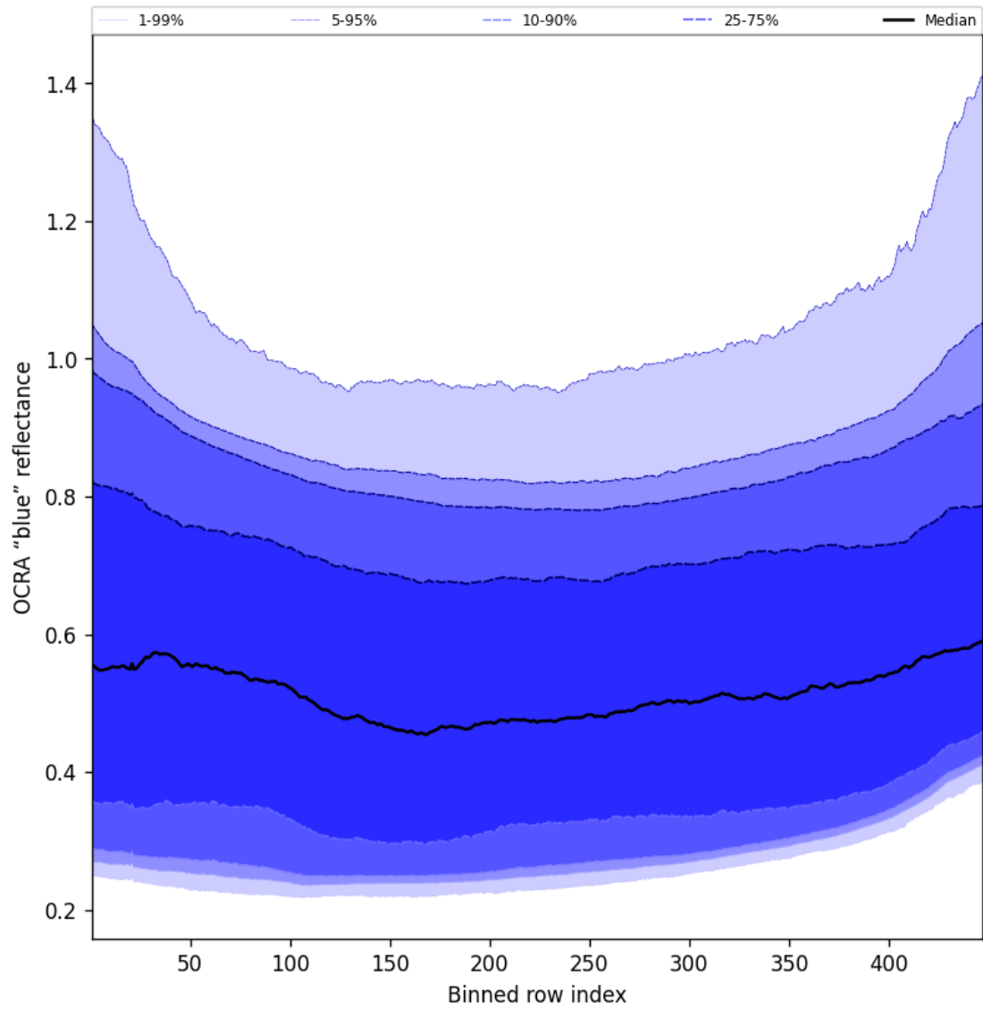
Figure 67: Along track statistics of “OCRA “blue” reflectance” for 2025-09-20 to 2025-09-22
