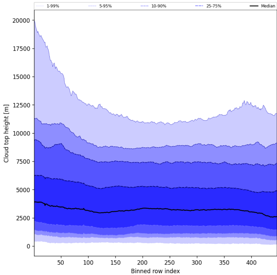
Figure 56: Along track statistics of “Cloud top height” for 2025-09-20 to 2025-09-22
