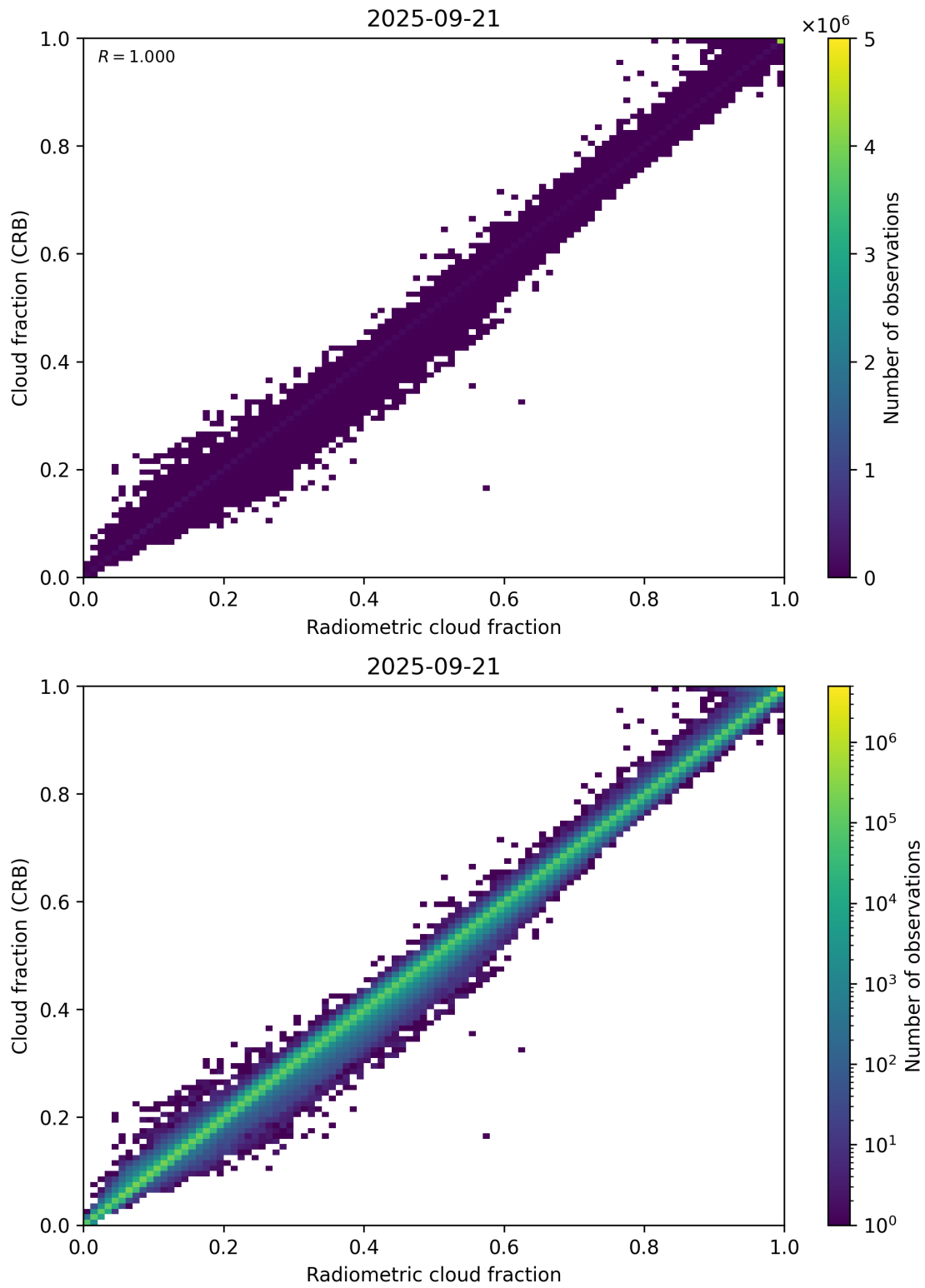
Figure 73: Scatter density plot of “Radiometric cloud fraction” against “Cloud fraction (CRB)” for 2025-09-20 to 2025-09-22.
