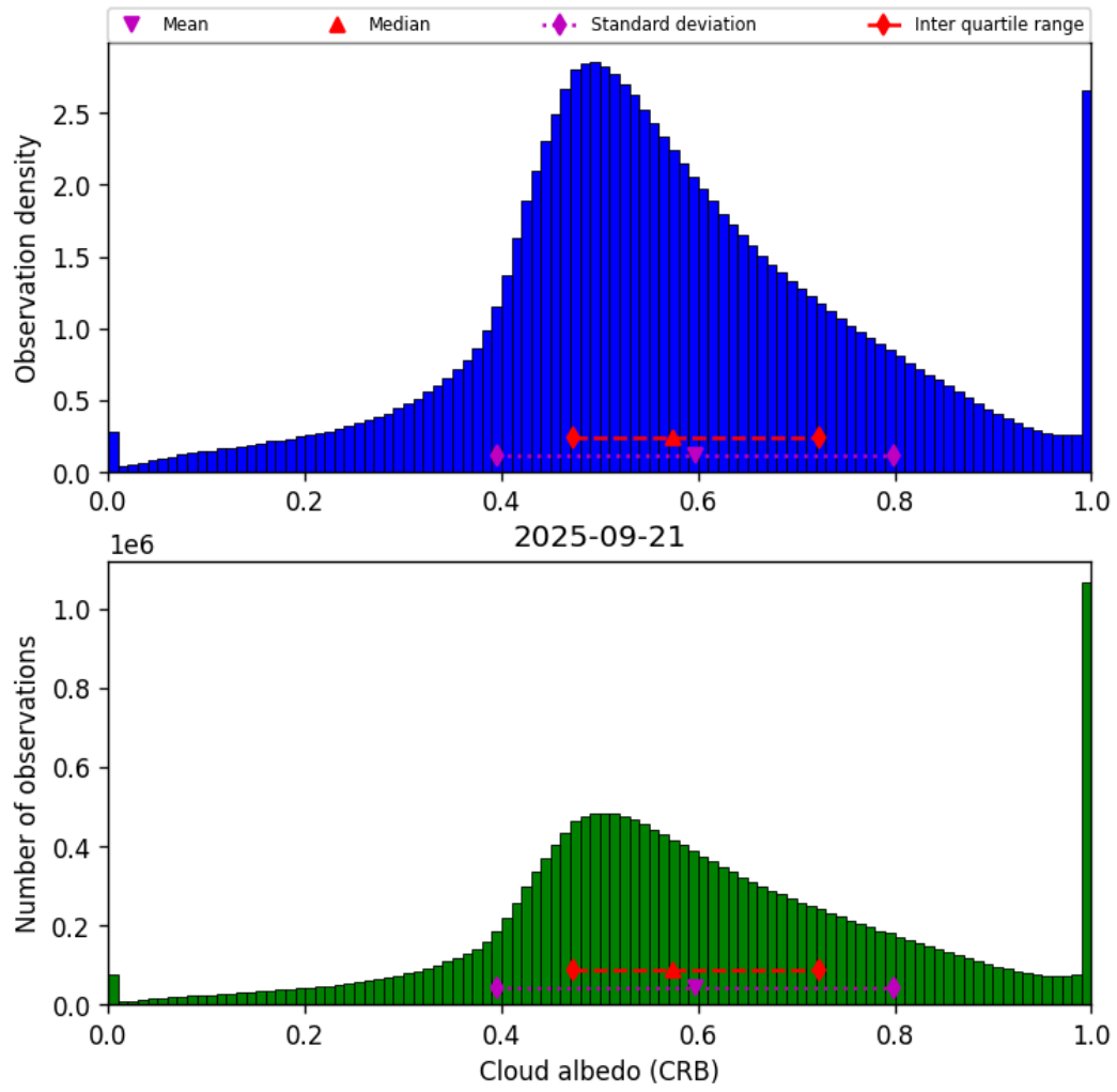
Figure 44: Histogram of “Cloud albedo (CRB)” for 2025-09-20 to 2025-09-22
