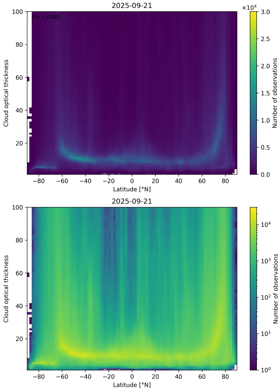
Figure 96: Scatter density plot of “Latitude” against “Cloud optical thickness” for 2025-09-20 to 2025-09-22.
