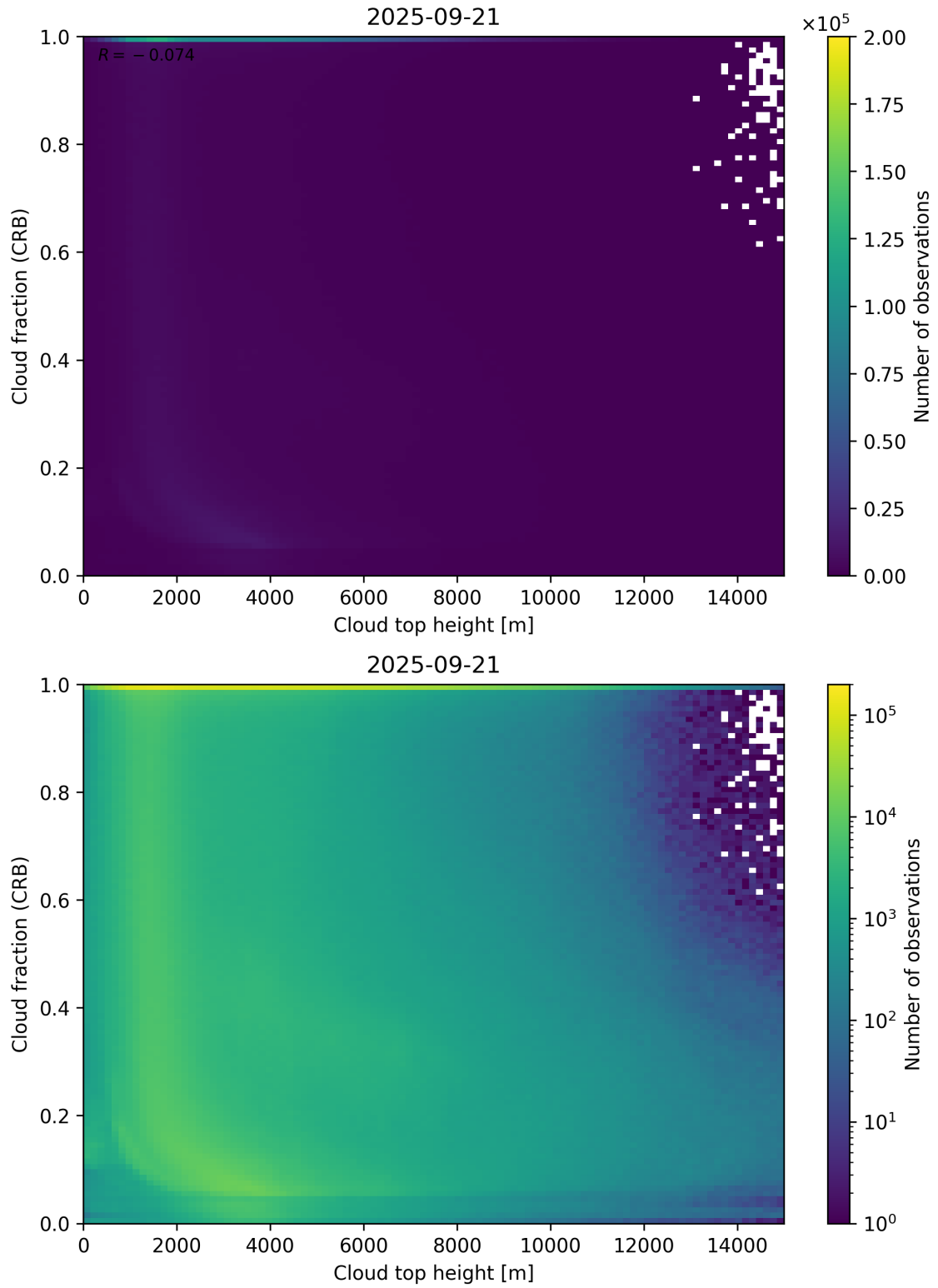
Figure 88: Scatter density plot of “Cloud top height” against “Cloud fraction (CRB)” for 2025-09-20 to 2025-09-22.
