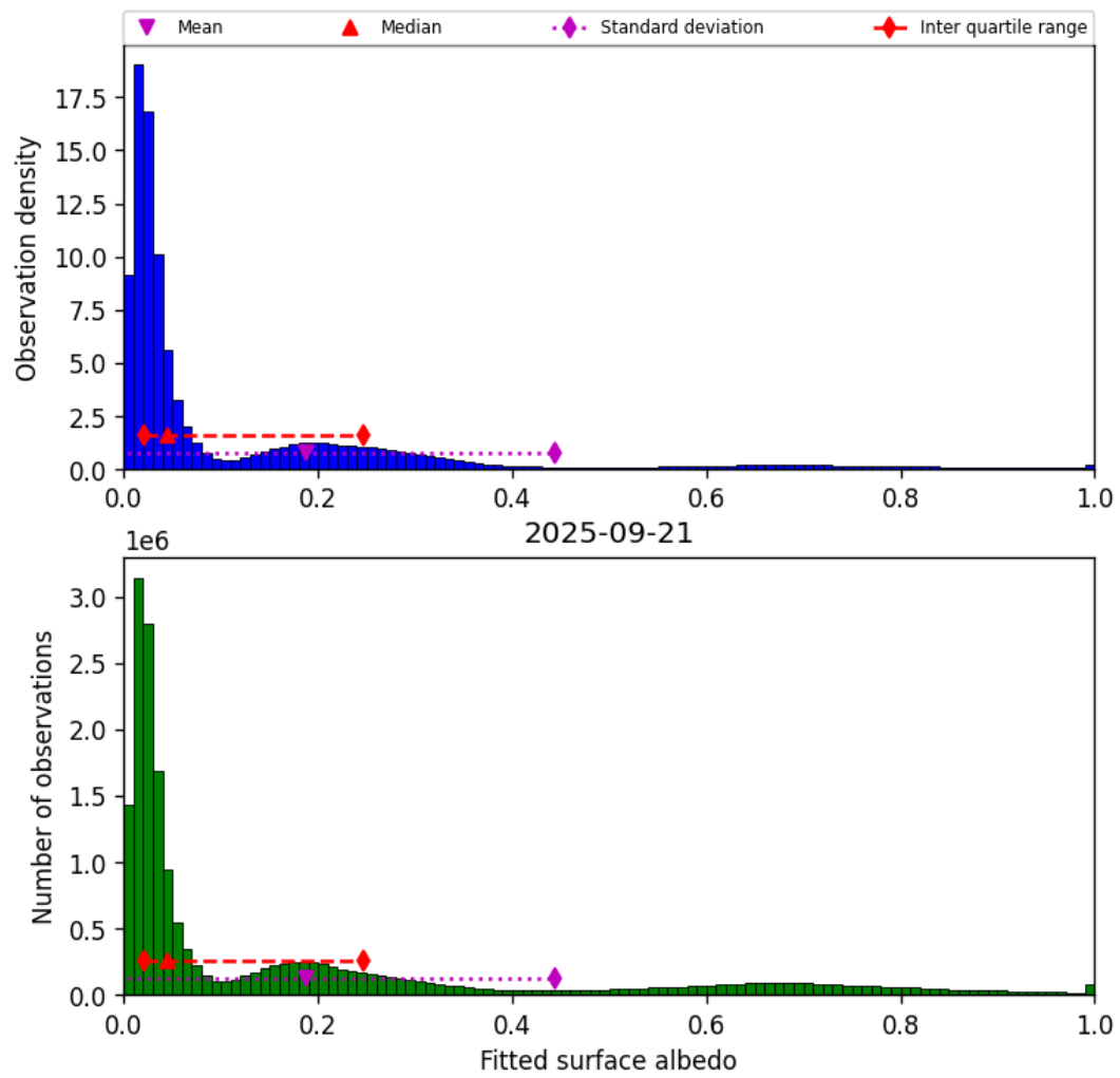
Figure 45: Histogram of “Fitted surface albedo” for 2025-09-20 to 2025-09-22
