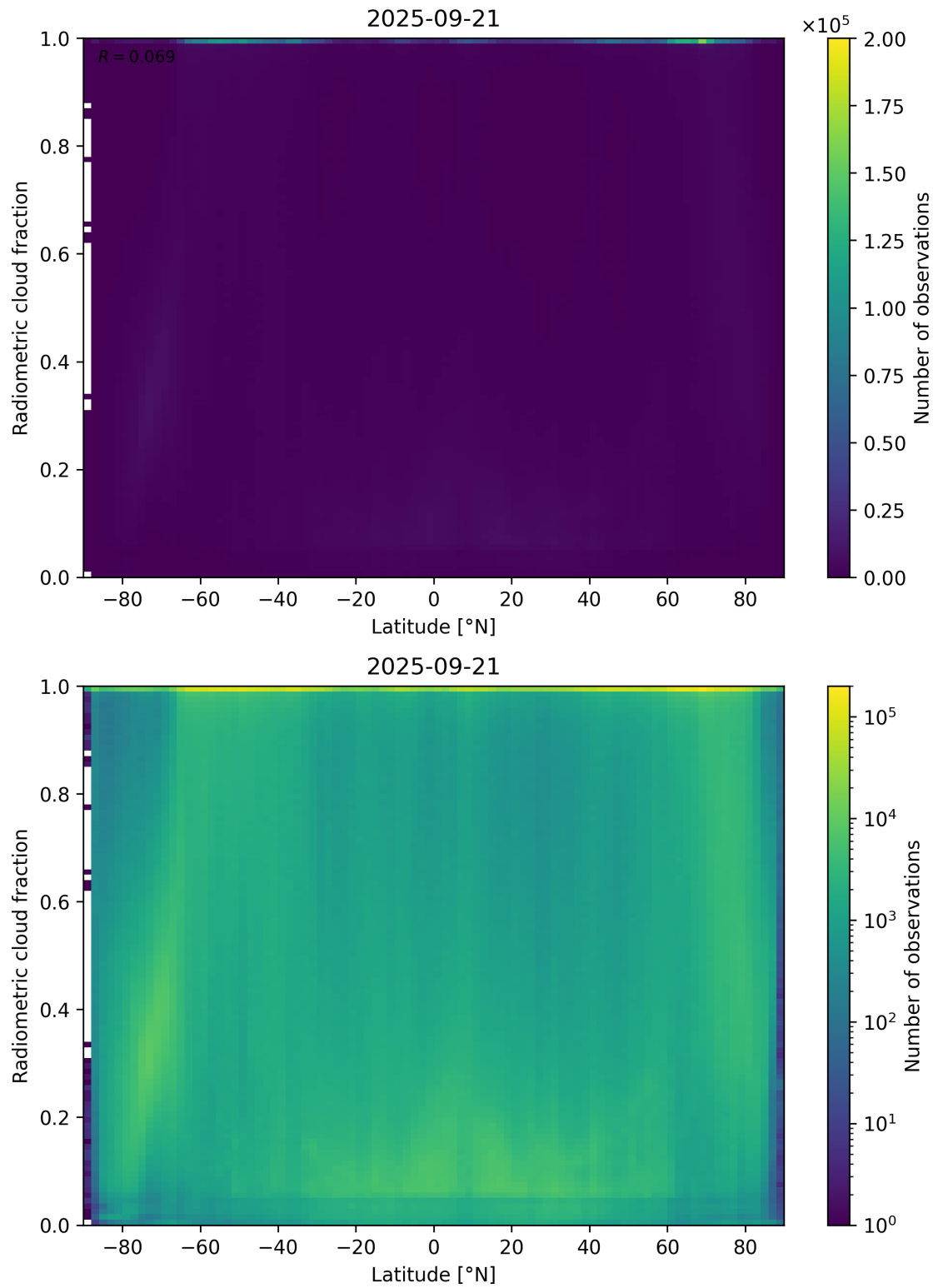
Figure 92: Scatter density plot of “Latitude” against “Radiometric cloud fraction” for 2025-09-20 to 2025-09-22.
