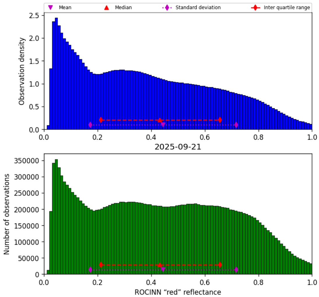
Figure 53: Histogram of “ROCINN “red” reflectance” for 2025-09-20 to 2025-09-22
