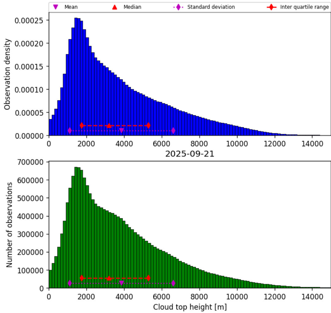
Figure 40: Histogram of “Cloud top height” for 2025-09-20 to 2025-09-22
