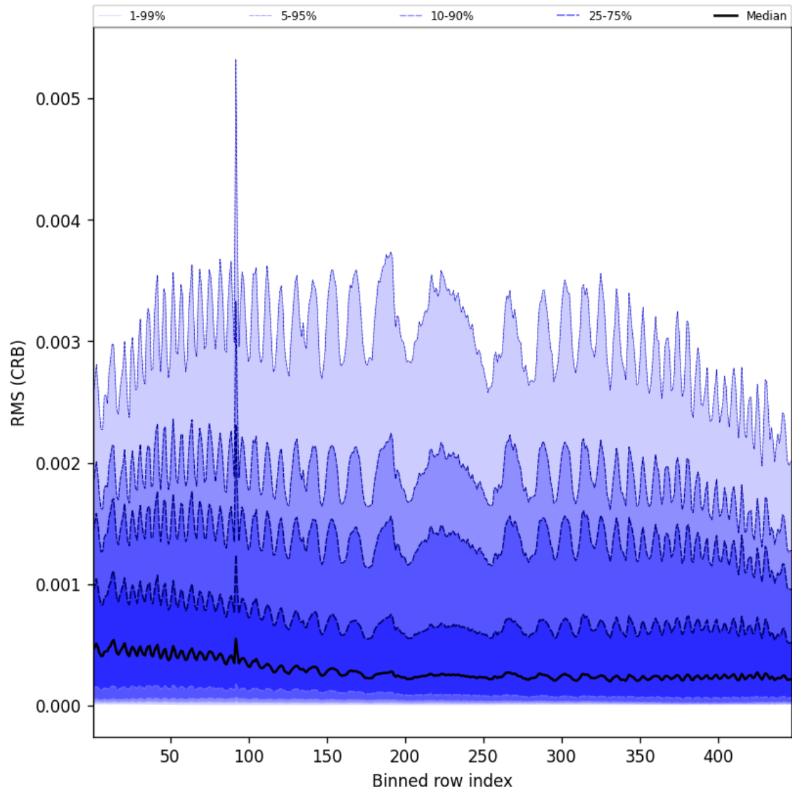
Figure 64: Along track statistics of “RMS (CRB)” for 2025-09-20 to 2025-09-22
