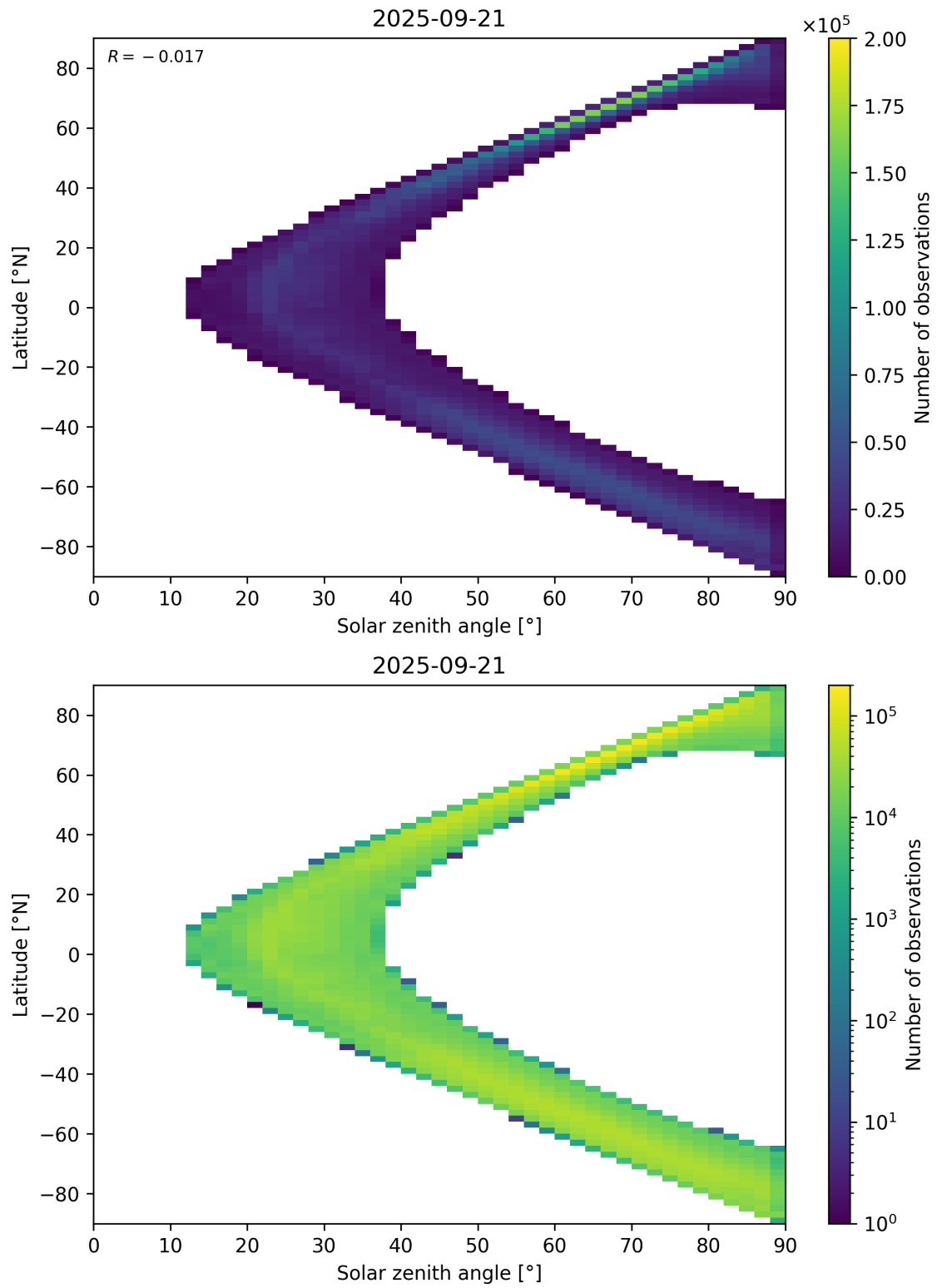
Figure 105: Scatter density plot of “Solar zenith angle” against “Latitude” for 2025-09-20 to 2025-09-22.
