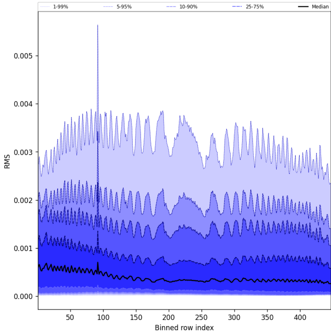
Figure 63: Along track statistics of “RMS” for 2025-09-20 to 2025-09-22
