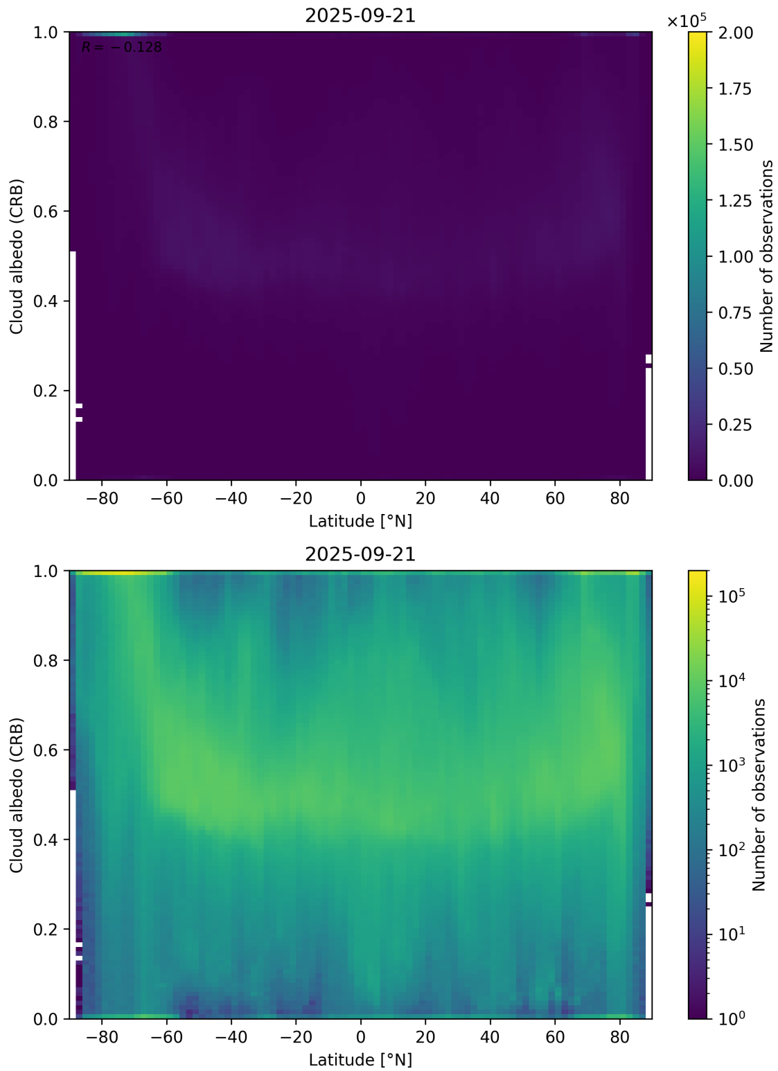
Figure 91: Scatter density plot of “Latitude” against “Cloud albedo (CRB)” for 2025-09-20 to 2025-09-22.
