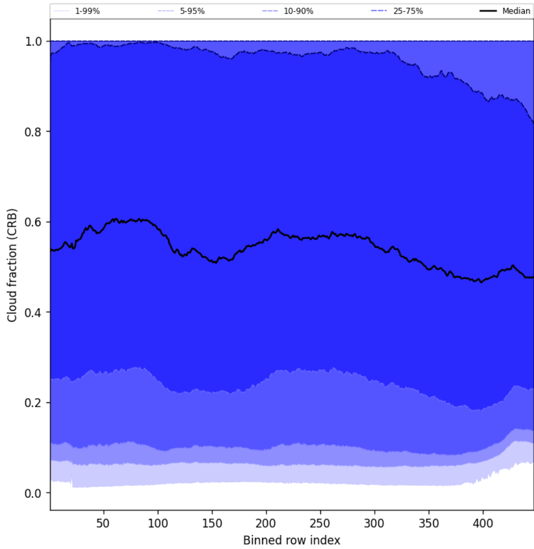
Figure 58: Along track statistics of “Cloud fraction (CRB)” for 2025-09-20 to 2025-09-22
