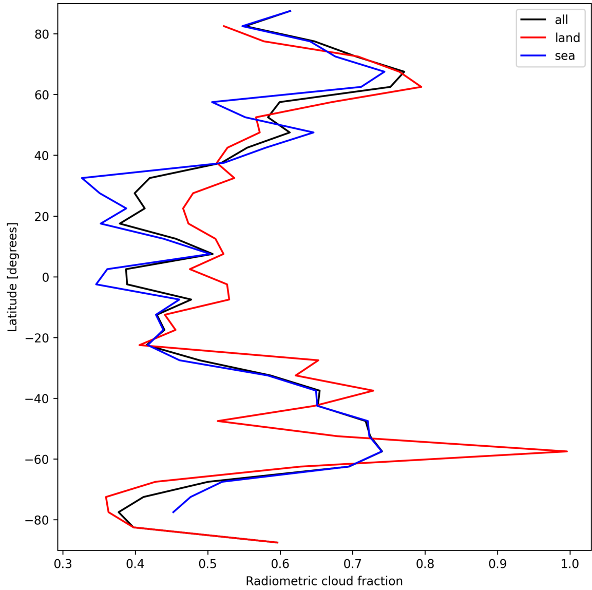
Figure 23: Zonal average of “Radiometric cloud fraction” for 2025-09-20 to 2025-09-22.
