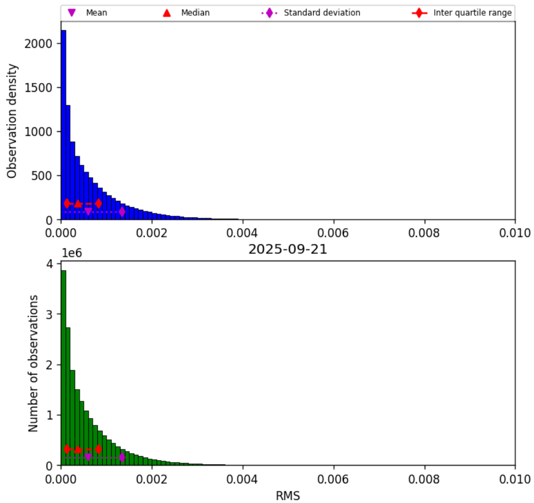
Figure 47: Histogram of “RMS” for 2025-09-20 to 2025-09-22
