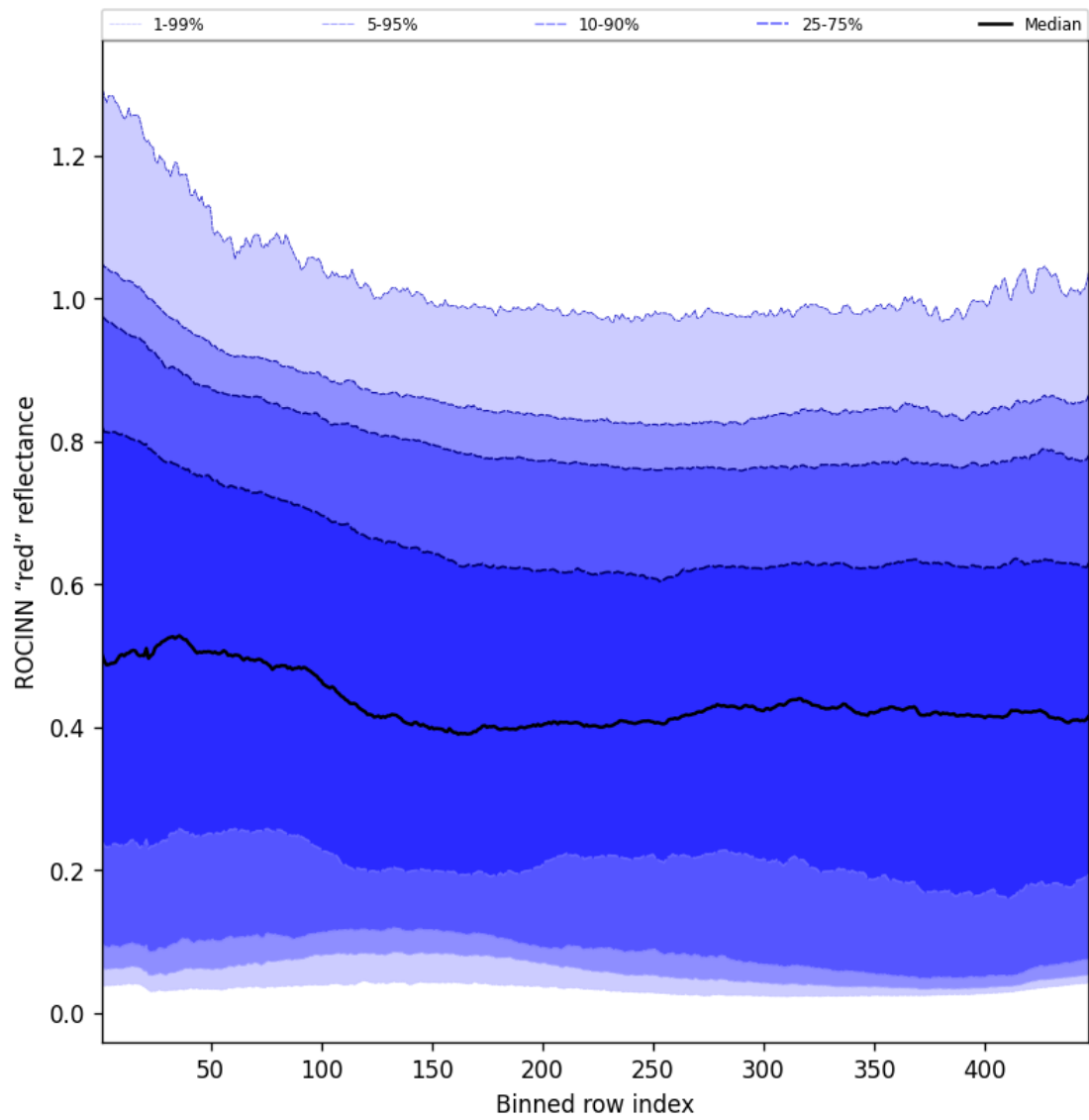
Figure 69: Along track statistics of “ROCINN “red” reflectance” for 2025-09-20 to 2025-09-22
