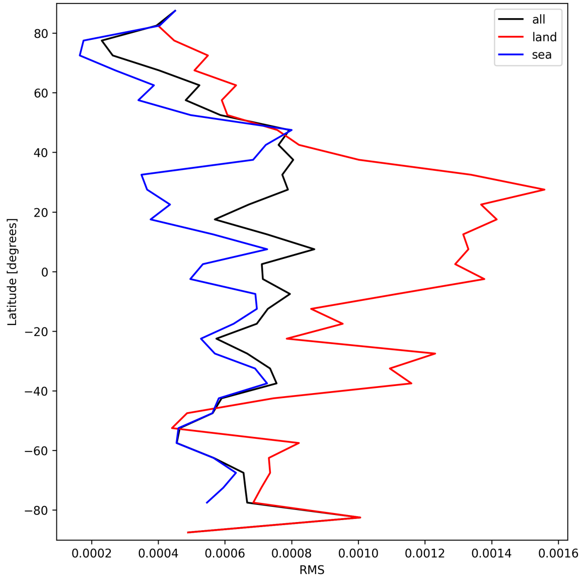
Figure 31: Zonal average of “RMS” for 2025-09-20 to 2025-09-22.
