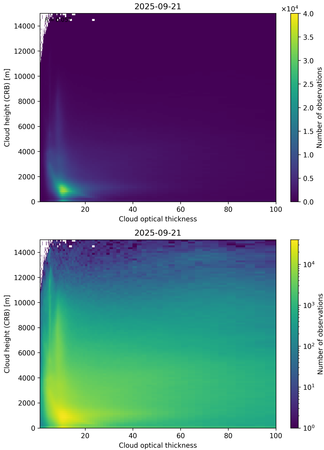
Figure 85: Scatter density plot of “Cloud optical thickness” against “Cloud height (CRB)” for 2025-09-20 to 2025-09-22.
