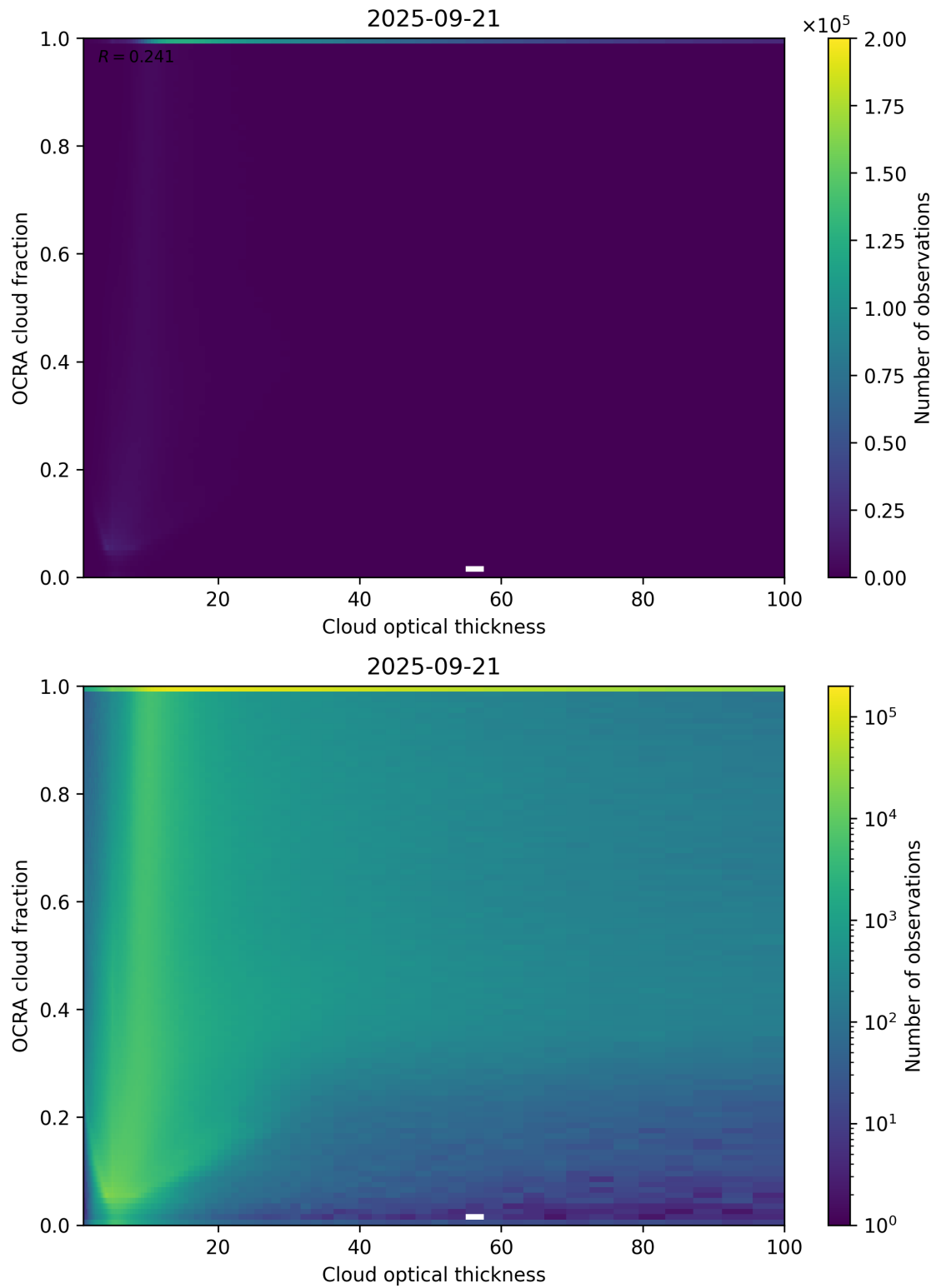
Figure 83: Scatter density plot of “Cloud optical thickness” against “OCRA cloud fraction” for 2025-09-20 to 2025-09-22.
