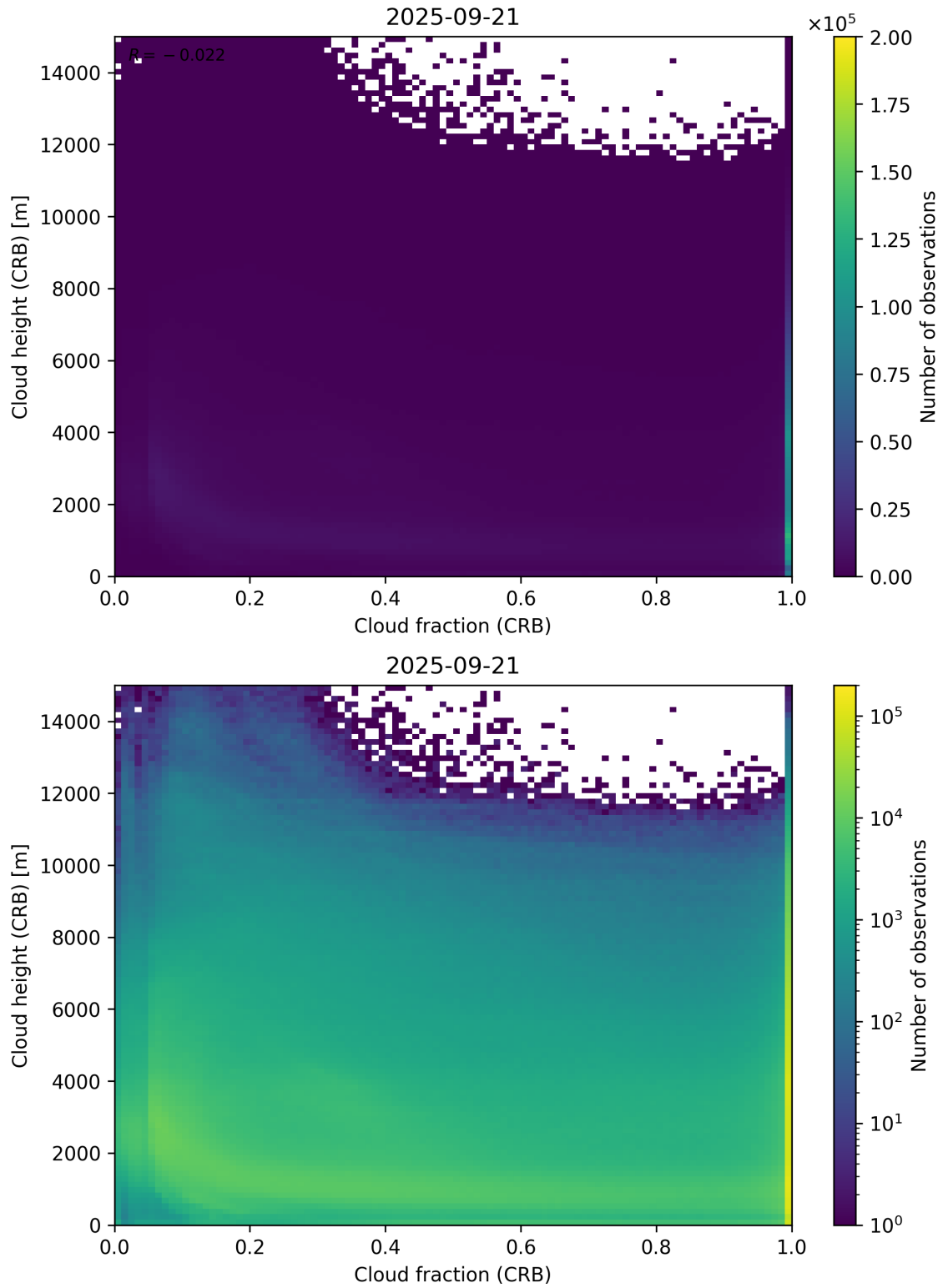
Figure 79: Scatter density plot of “Cloud fraction (CRB)” against “Cloud height (CRB)” for 2025-09-20 to 2025-09-22.
