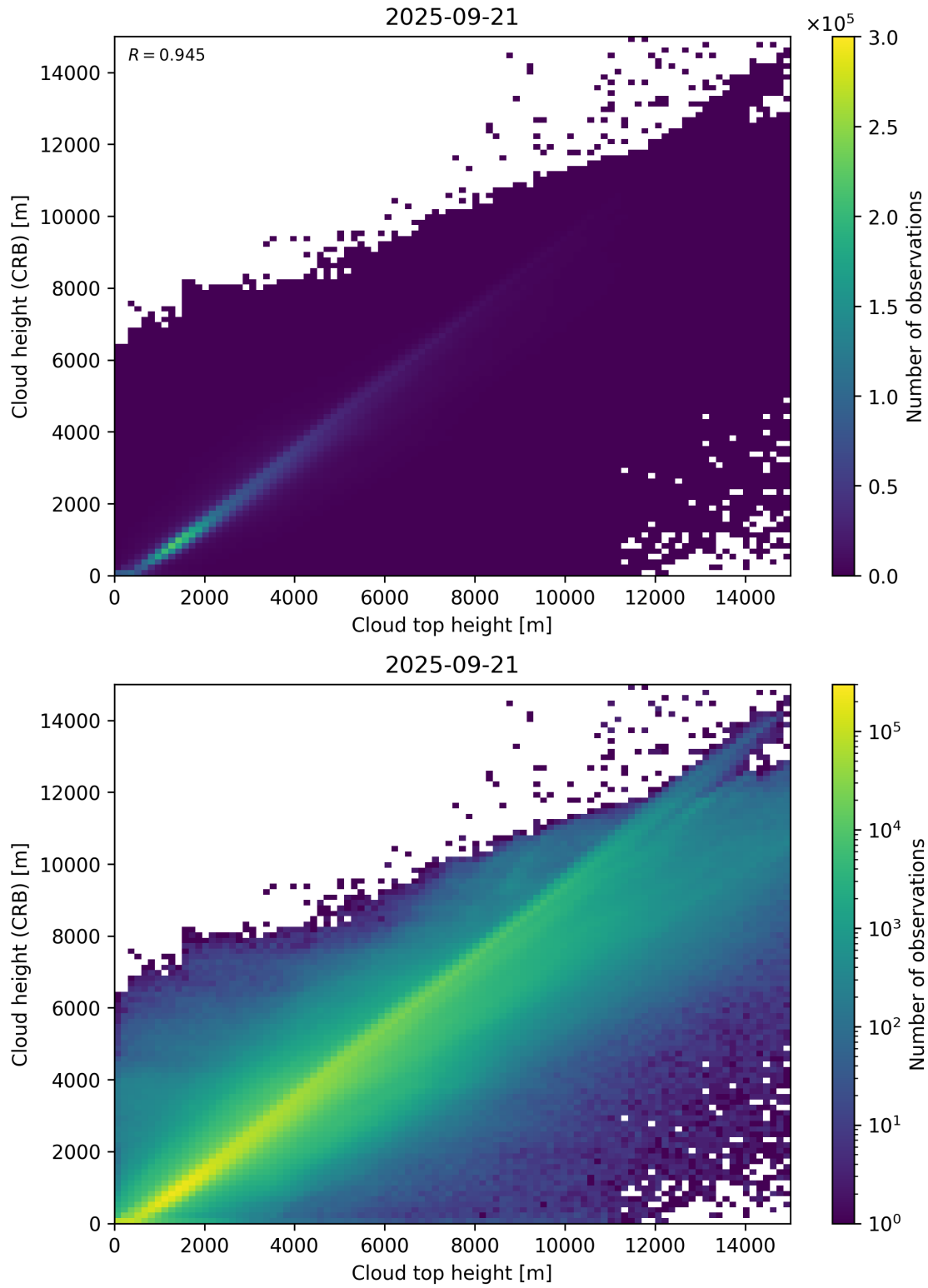
Figure 89: Scatter density plot of “Cloud top height” against “Cloud height (CRB)” for 2025-09-20 to 2025-09-22.
