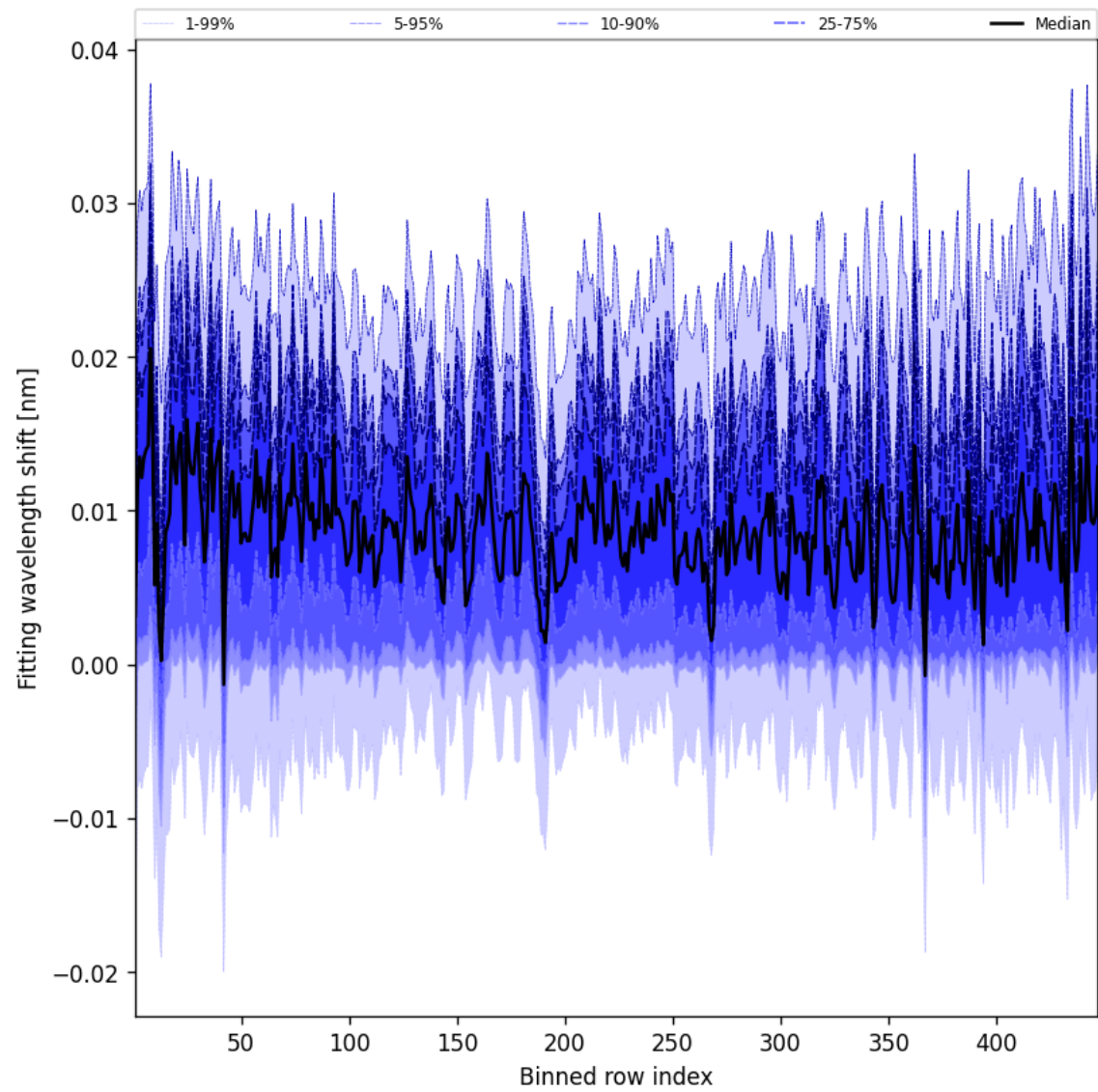
Figure 65: Along track statistics of “Fitting wavelength shift” for 2025-09-20 to 2025-09-22
