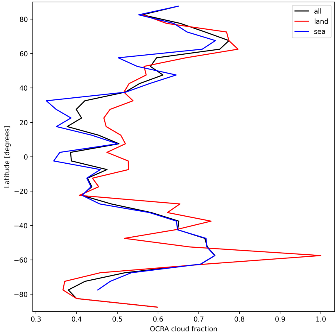
Figure 34: Zonal average of “OCRA cloud fraction” for 2025-09-20 to 2025-09-22.
