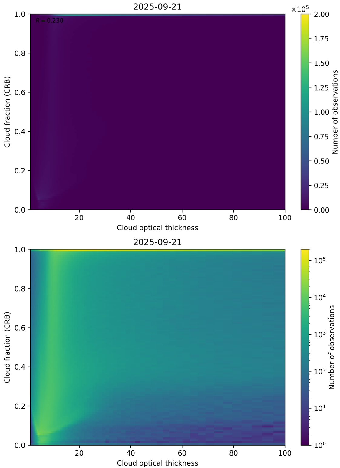
Figure 84: Scatter density plot of “Cloud optical thickness” against “Cloud fraction (CRB)” for 2025-09-20 to 2025-09-22.
