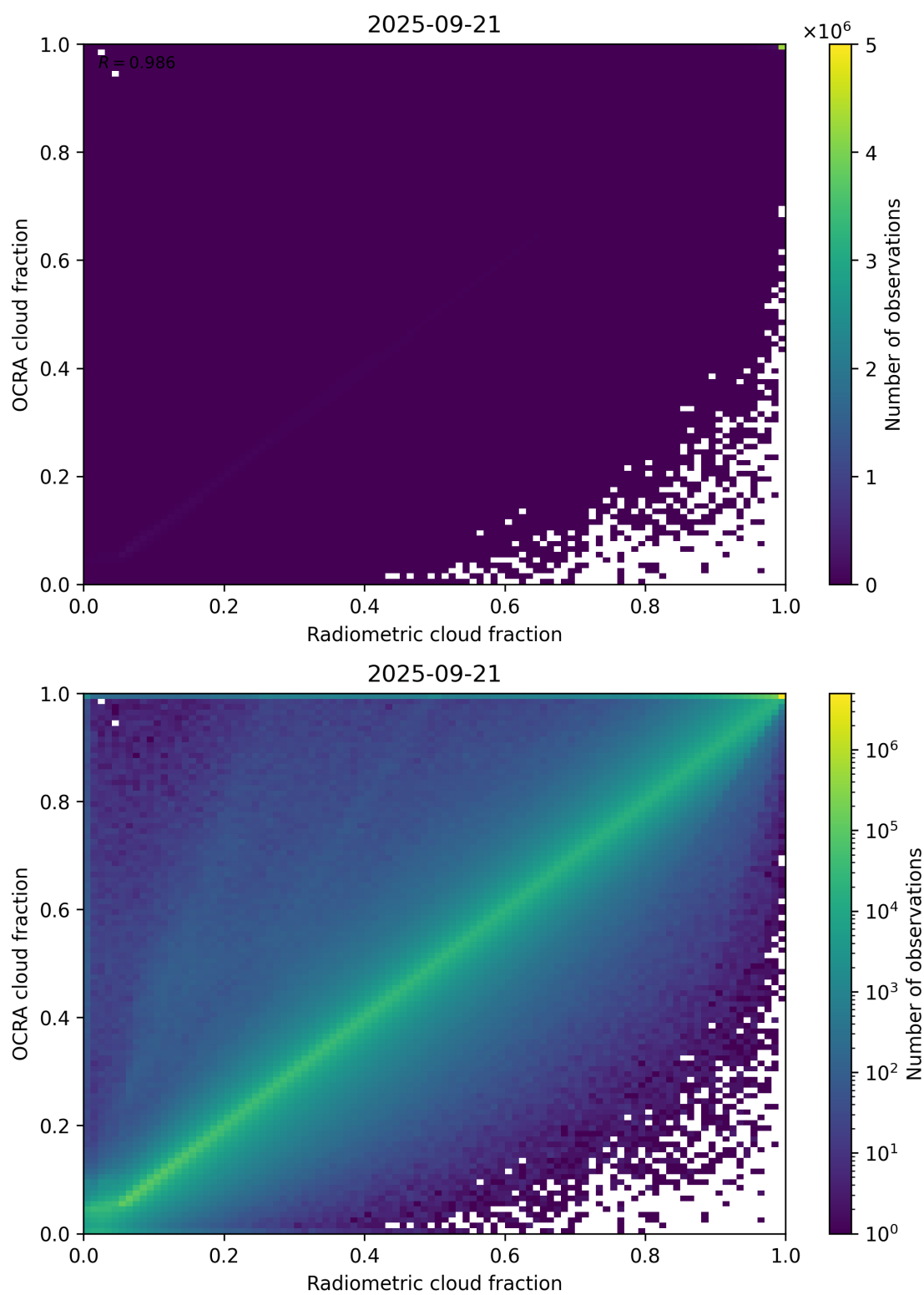
Figure 72: Scatter density plot of “Radiometric cloud fraction” against “OCRA cloud fraction” for 2025-09-20 to 2025-09-22.
