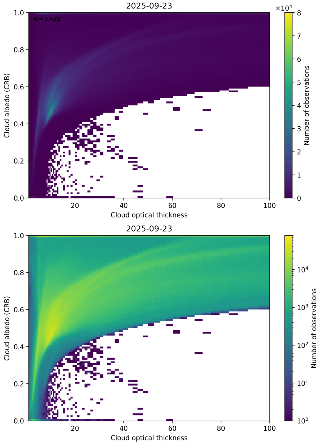
Figure 82: Scatter density plot of “Cloud optical thickness” against “Cloud albedo (CRB)” for 2025-09-22 to 2025-09-24.
