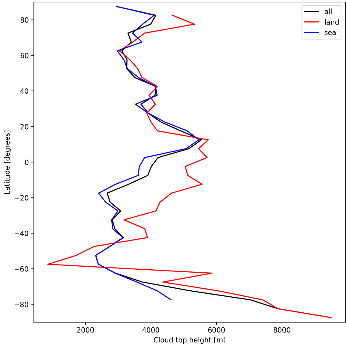
Figure 24: Zonal average of “Cloud top height” for 2025-09-22 to 2025-09-24.
