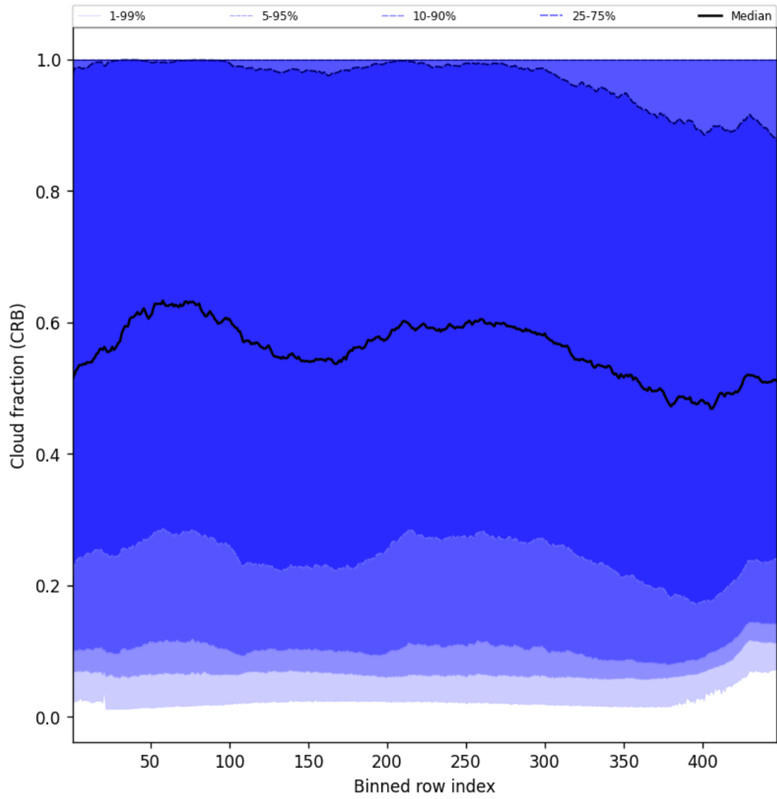
Figure 58: Along track statistics of “Cloud fraction (CRB)” for 2025-09-22 to 2025-09-24
