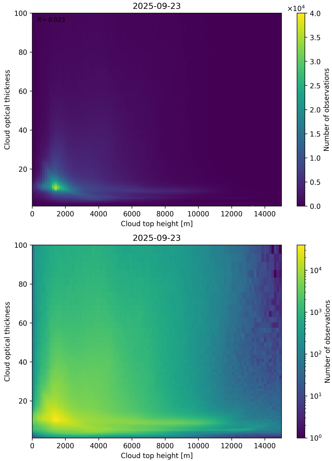
Figure 90: Scatter density plot of “Cloud top height” against “Cloud optical thickness” for 2025-09-22 to 2025-09-24.
