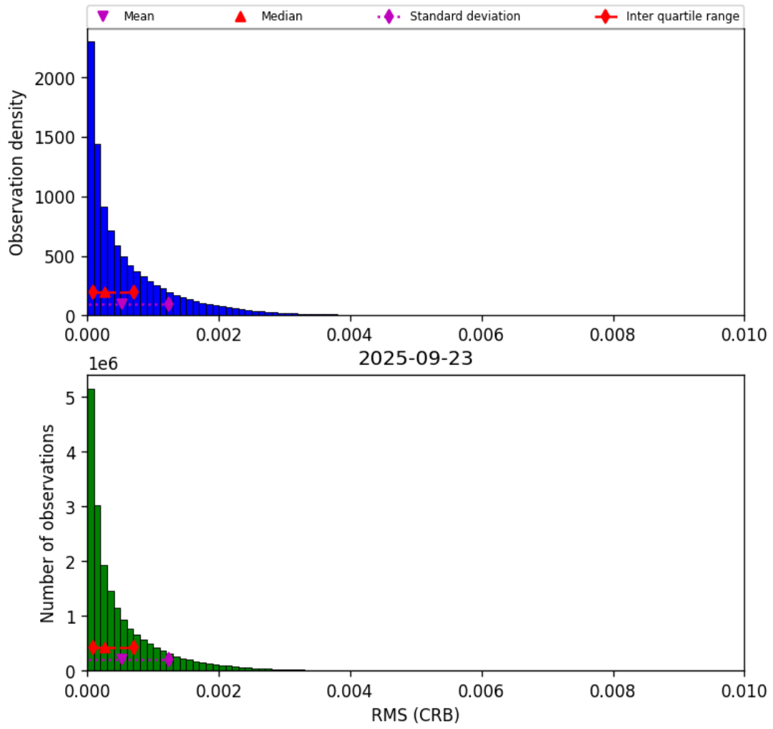
Figure 48: Histogram of “RMS (CRB)” for 2025-09-22 to 2025-09-24
