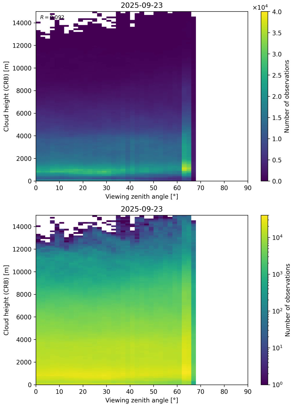
Figure 110: Scatter density plot of “Viewing zenith angle” against “Cloud height (CRB)” for 2025-09-22 to 2025-09-24.
