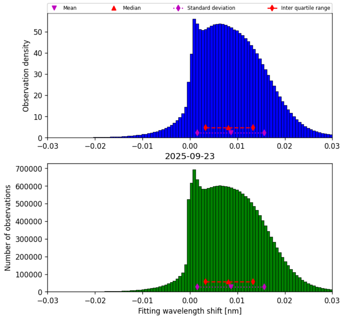
Figure 49: Histogram of “Fitting wavelength shift” for 2025-09-22 to 2025-09-24
