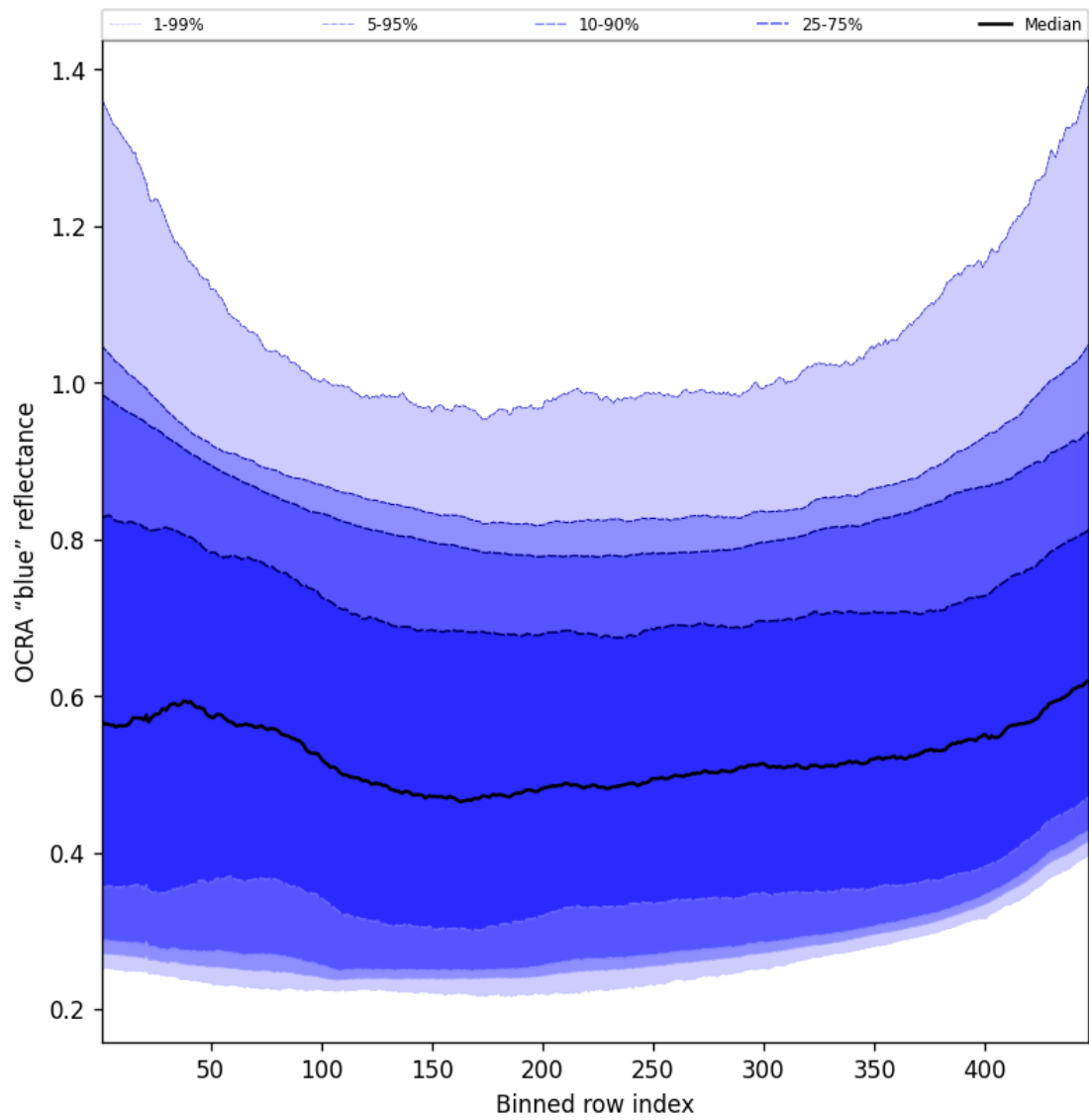
Figure 67: Along track statistics of “OCRA “blue” reflectance” for 2025-09-22 to 2025-09-24
