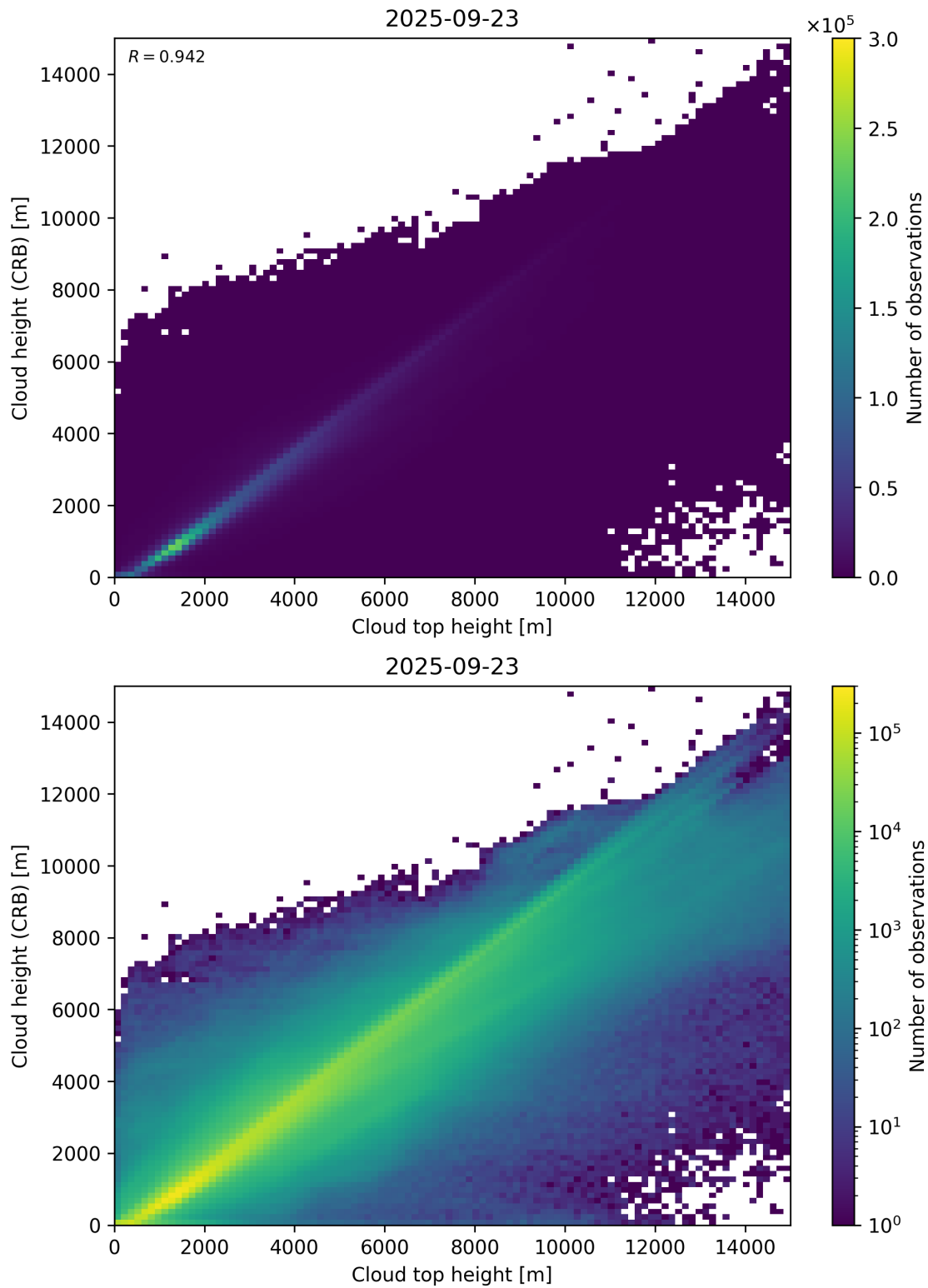
Figure 89: Scatter density plot of “Cloud top height” against “Cloud height (CRB)” for 2025-09-22 to 2025-09-24.
