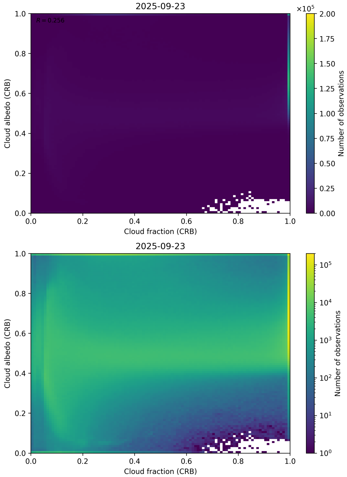
Figure 77: Scatter density plot of “Cloud fraction (CRB)” against “Cloud albedo (CRB)” for 2025-09-22 to 2025-09-24.
