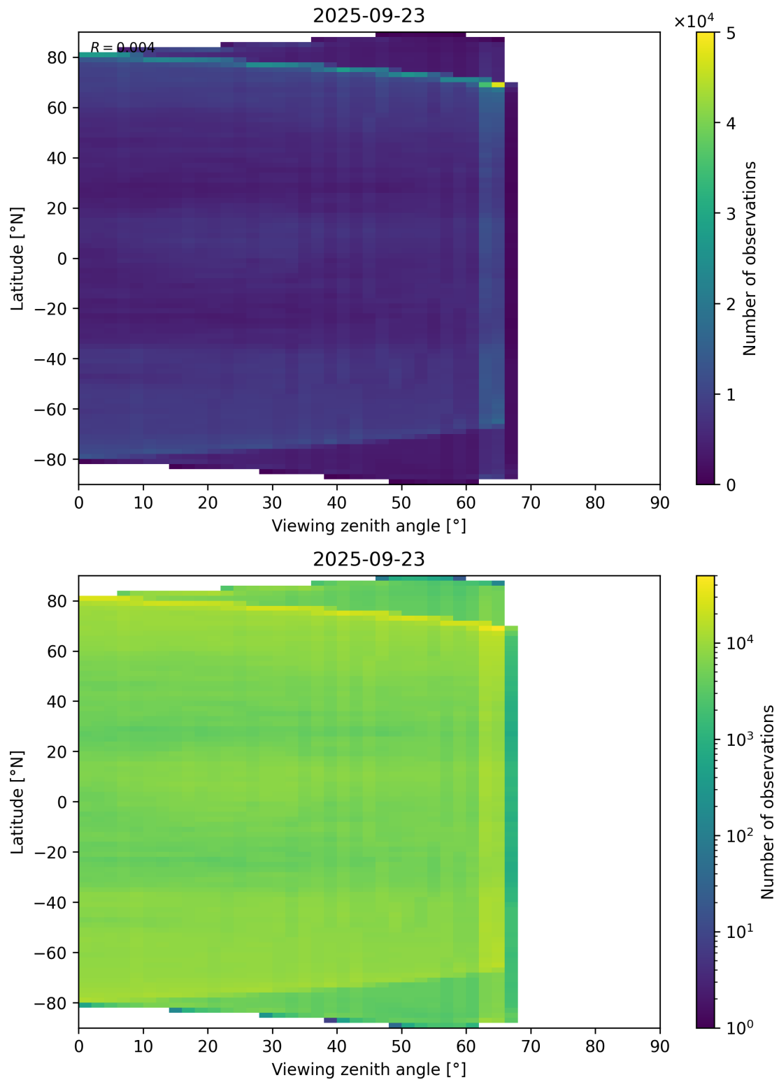
Figure 113: Scatter density plot of “Viewing zenith angle” against “Latitude” for 2025-09-22 to 2025-09-24.
