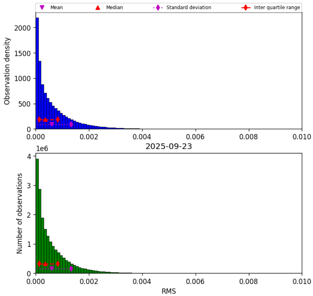
Figure 47: Histogram of “RMS” for 2025-09-22 to 2025-09-24
