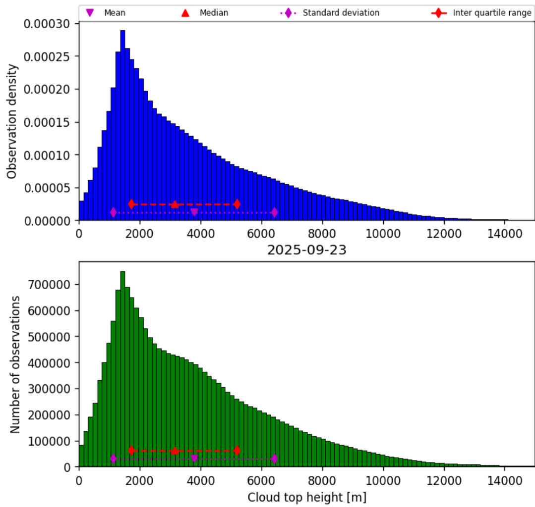
Figure 40: Histogram of “Cloud top height” for 2025-09-22 to 2025-09-24
