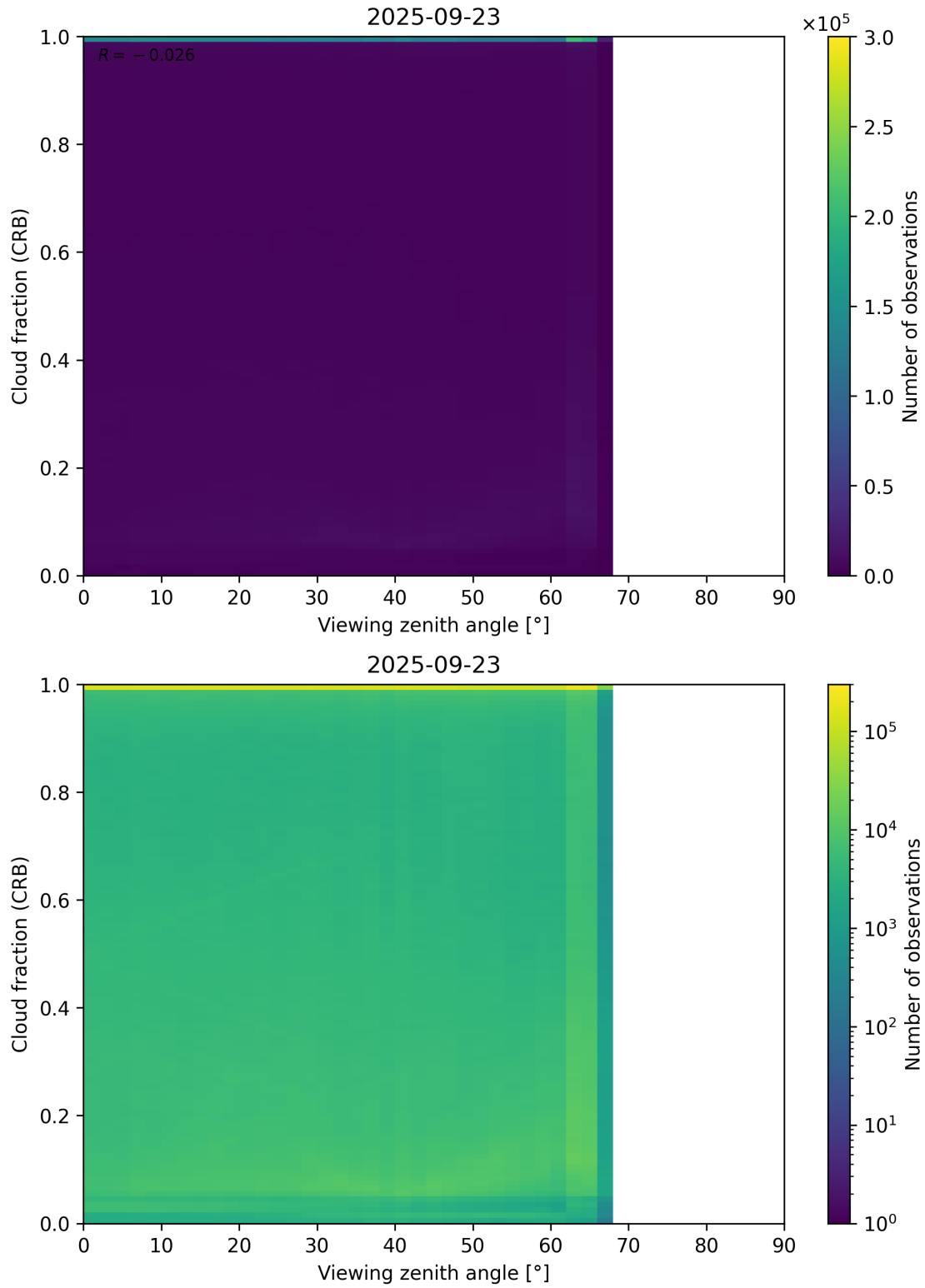
Figure 109: Scatter density plot of “Viewing zenith angle” against “Cloud fraction (CRB)” for 2025-09-22 to 2025-09-24.
