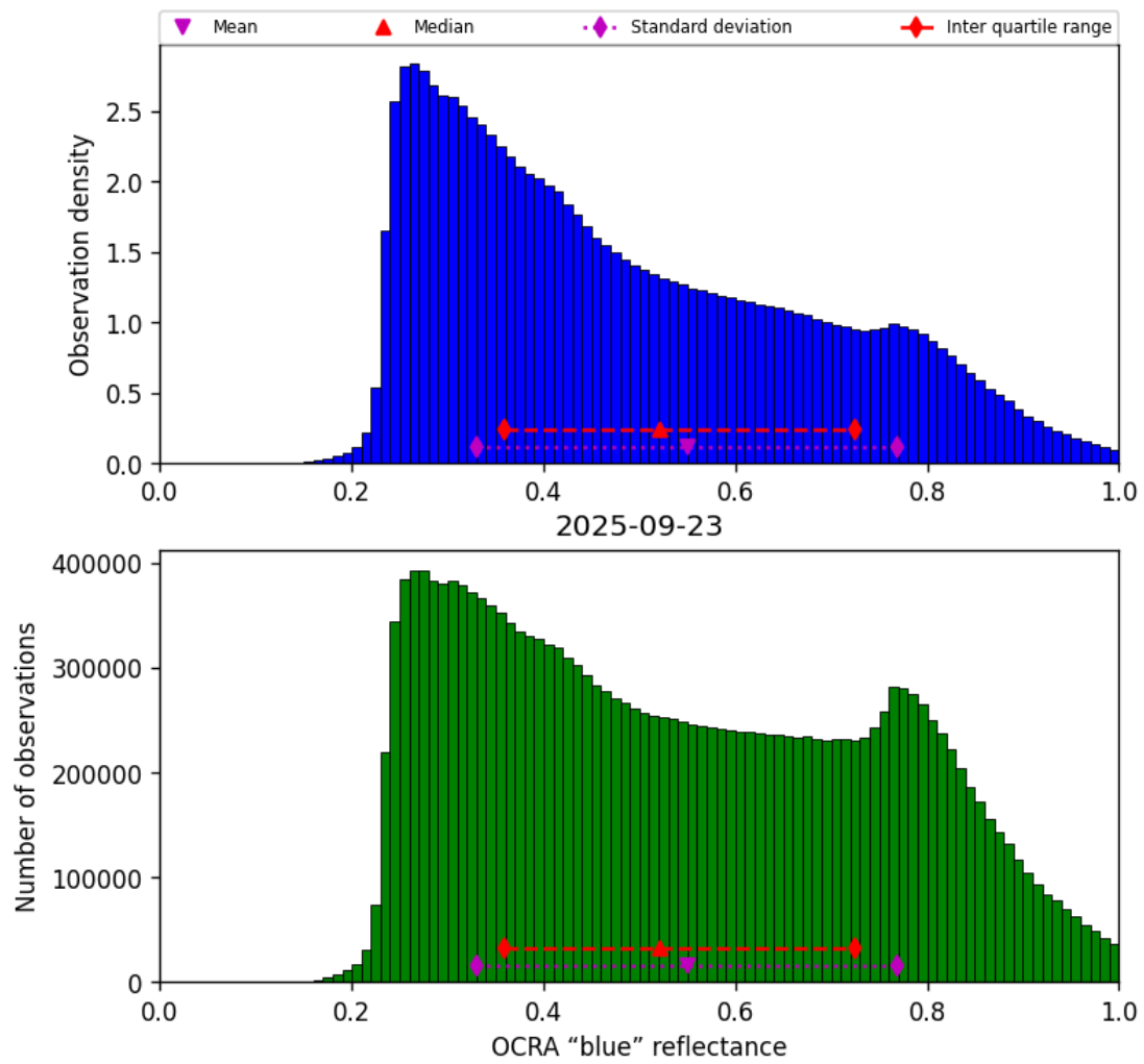
Figure 51: Histogram of “OCRA “blue” reflectance” for 2025-09-22 to 2025-09-24
