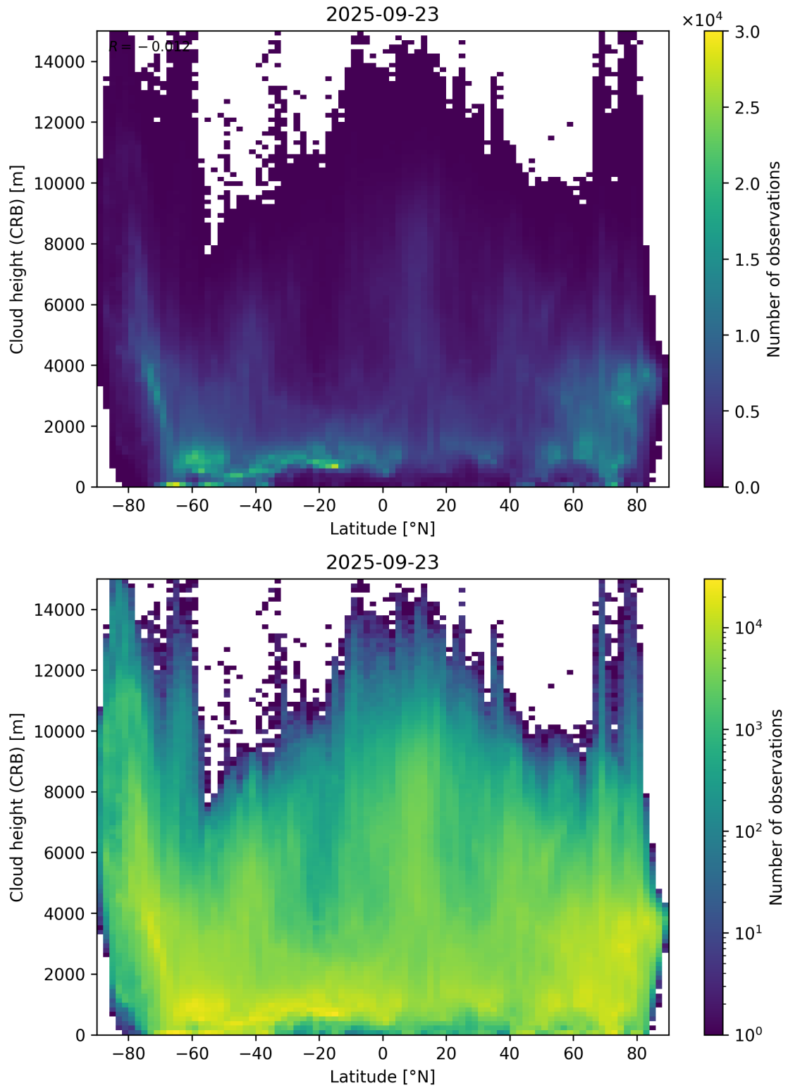
Figure 95: Scatter density plot of “Latitude” against “Cloud height (CRB)” for 2025-09-22 to 2025-09-24.
