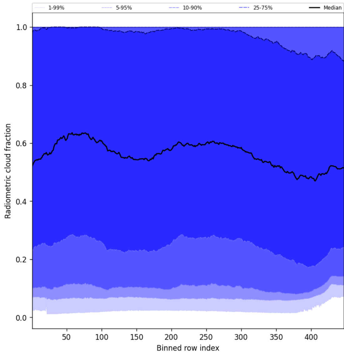
Figure 55: Along track statistics of “Radiometric cloud fraction” for 2025-09-22 to 2025-09-24
