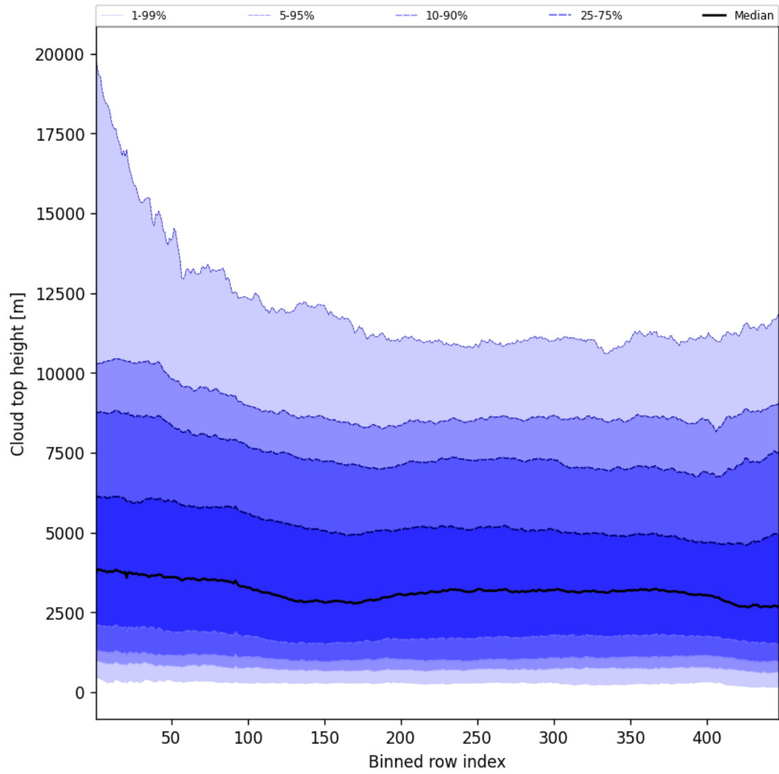
Figure 56: Along track statistics of “Cloud top height” for 2025-09-22 to 2025-09-24
