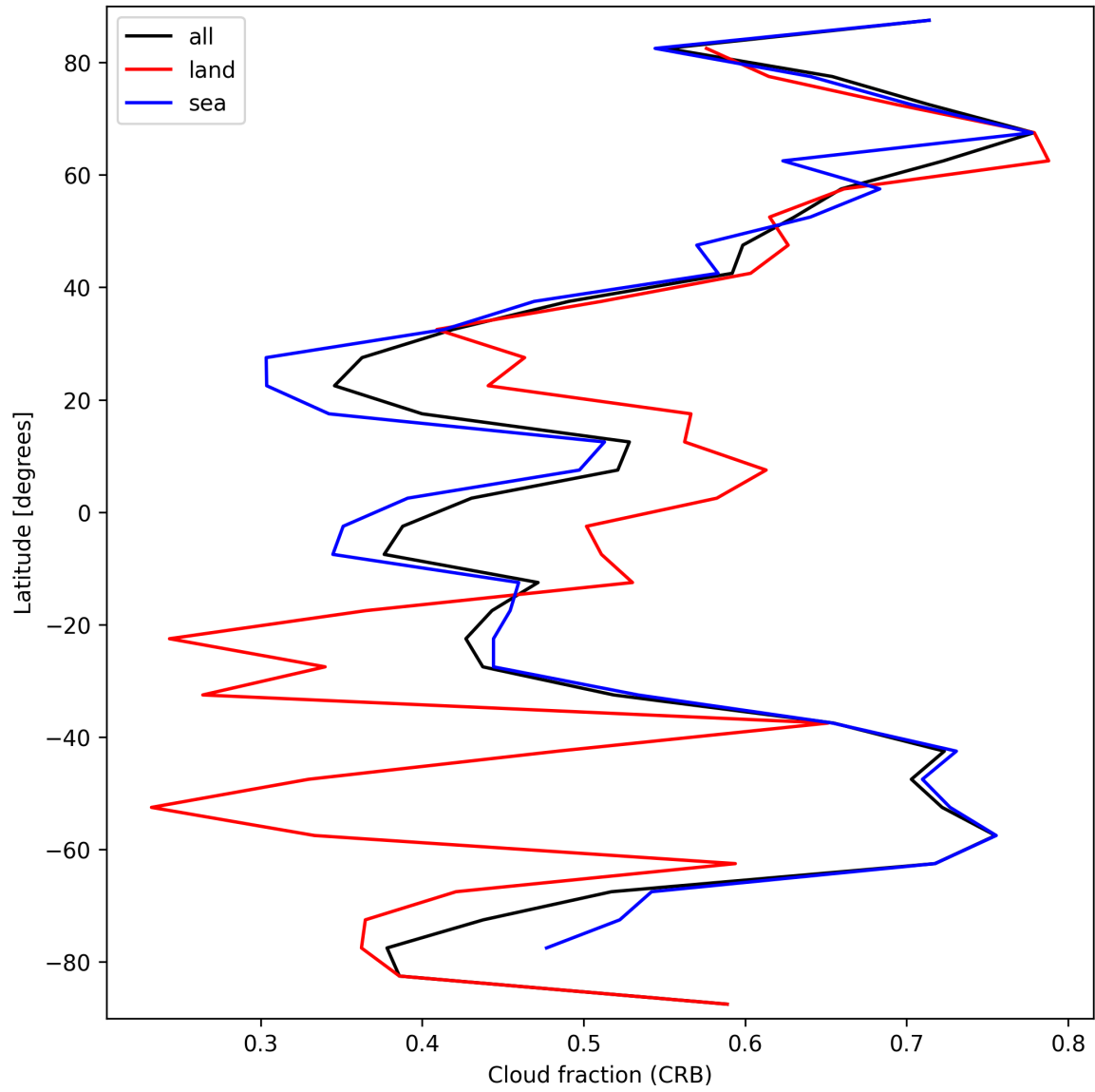
Figure 26: Zonal average of “Cloud fraction (CRB)” for 2025-09-22 to 2025-09-24.
