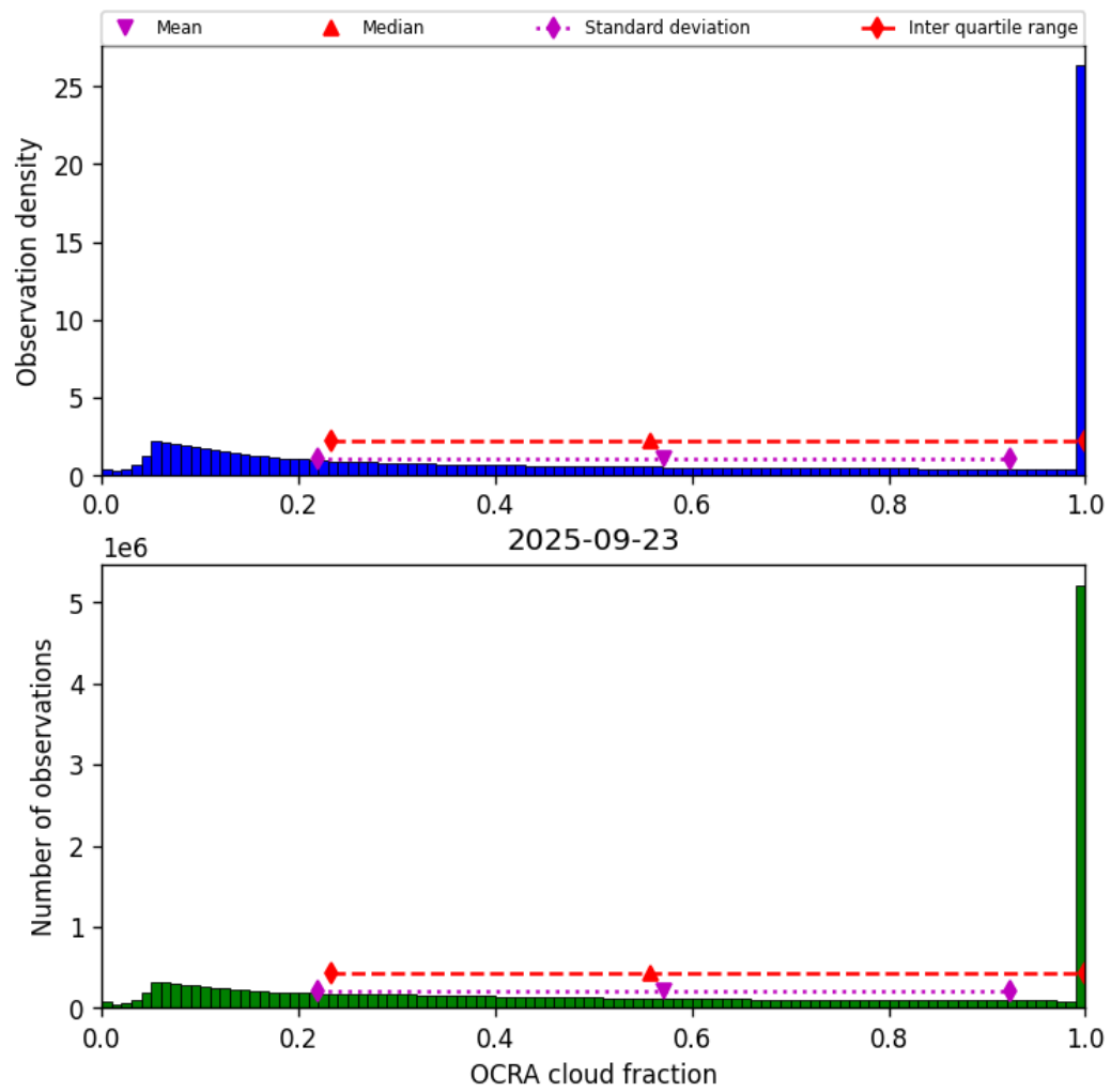
Figure 50: Histogram of “OCRA cloud fraction” for 2025-09-22 to 2025-09-24
