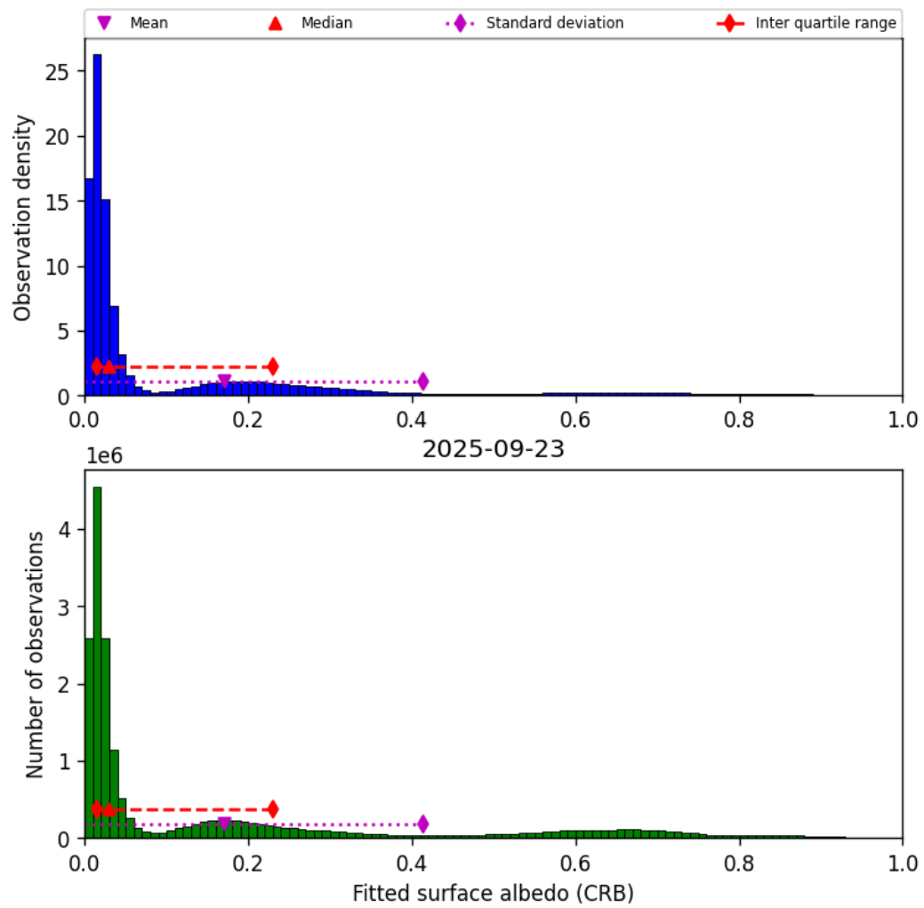
Figure 46: Histogram of “Fitted surface albedo (CRB)” for 2025-09-22 to 2025-09-24
