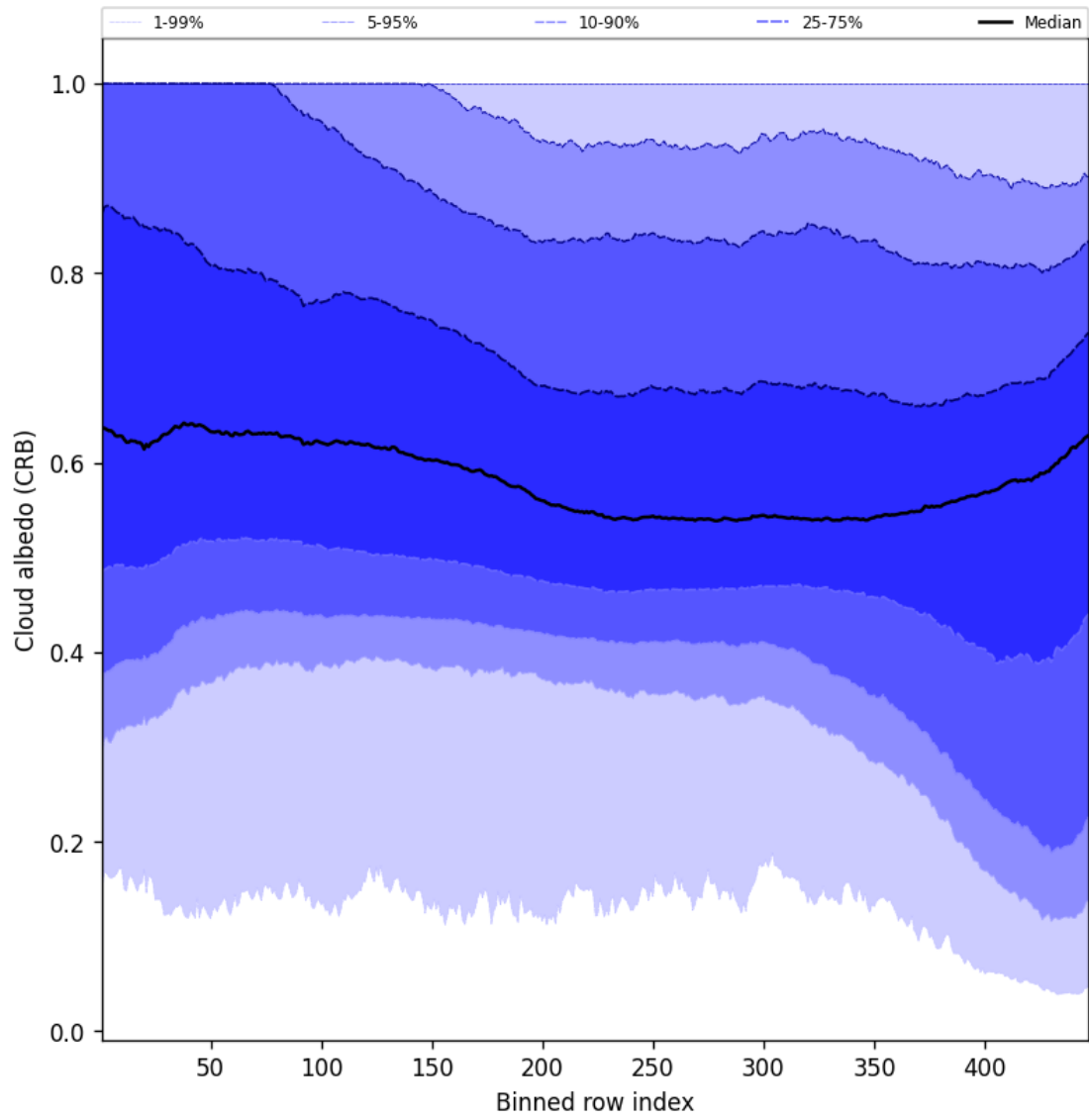
Figure 60: Along track statistics of “Cloud albedo (CRB)” for 2025-09-22 to 2025-09-24
