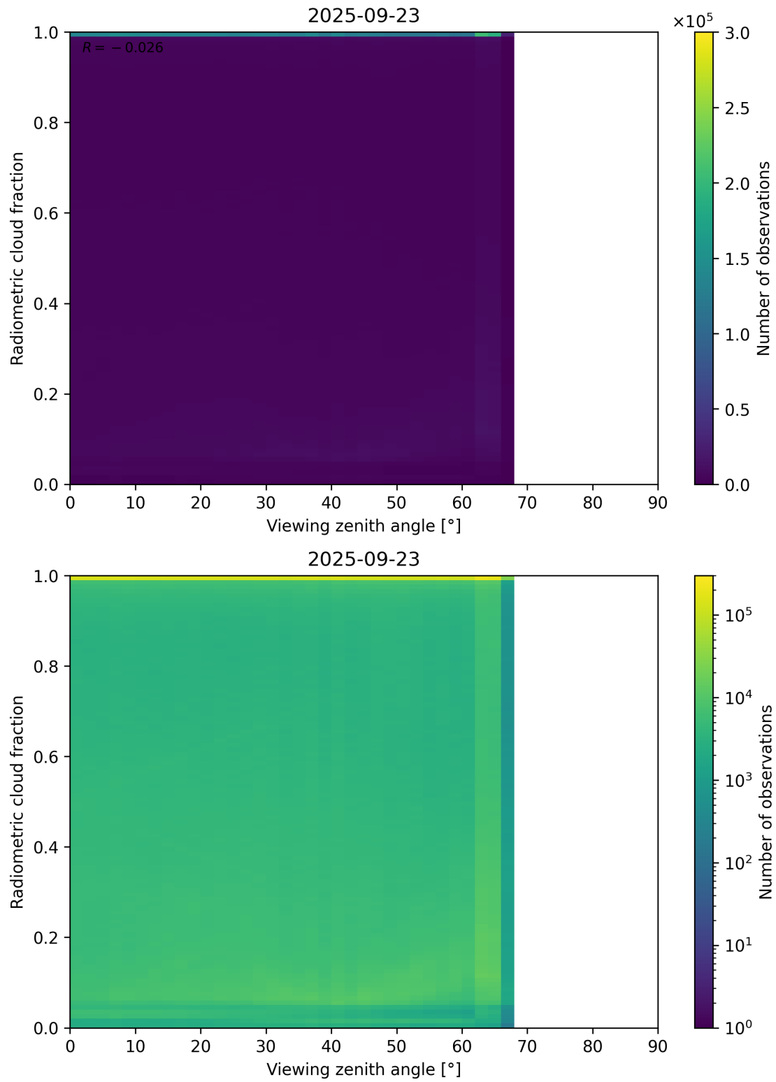
Figure 107: Scatter density plot of “Viewing zenith angle” against “Radiometric cloud fraction” for 2025-09-22 to 2025-09-24.
