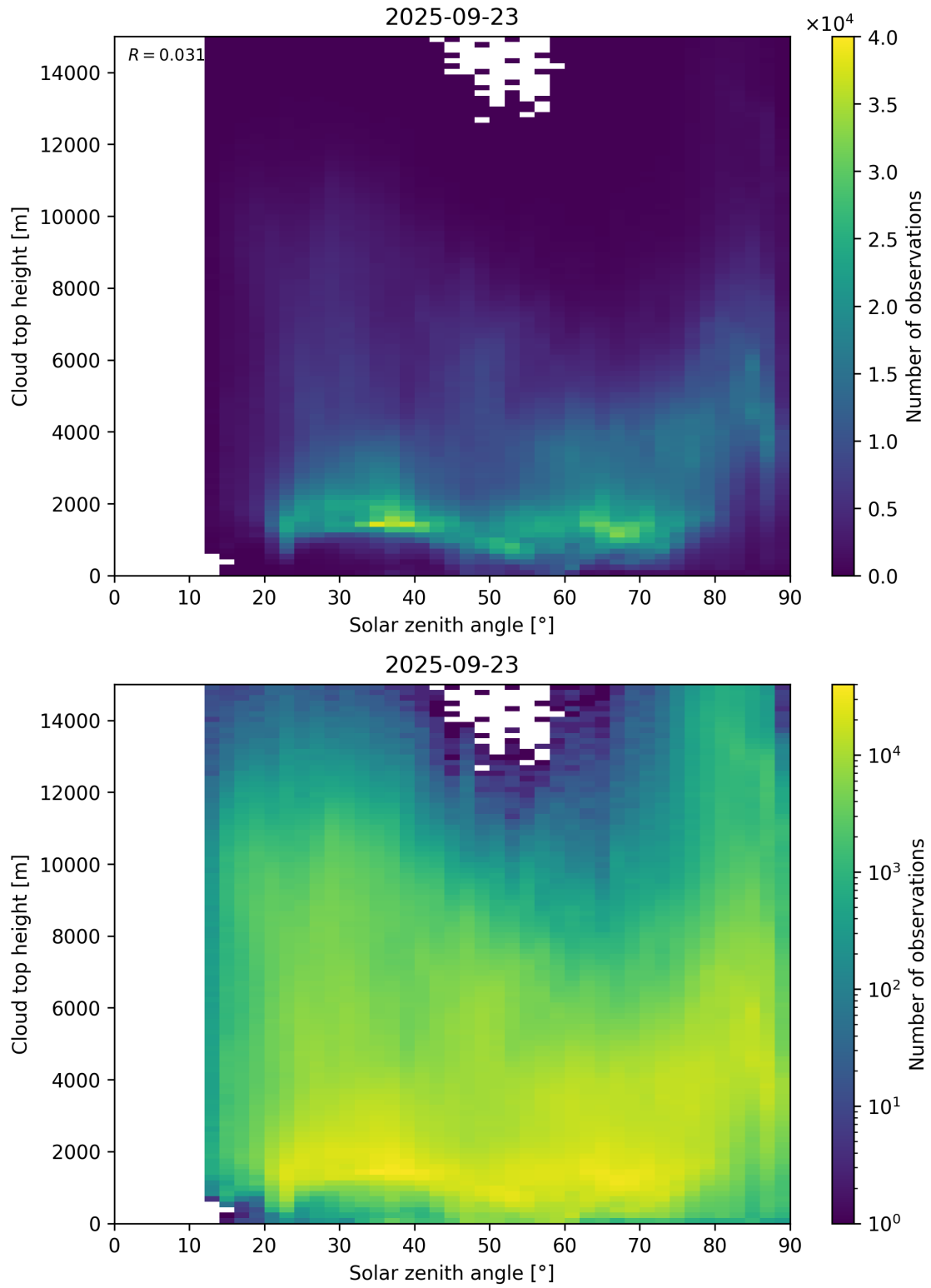
Figure 104: Scatter density plot of “Solar zenith angle” against “Cloud top height” for 2025-09-22 to 2025-09-24.
