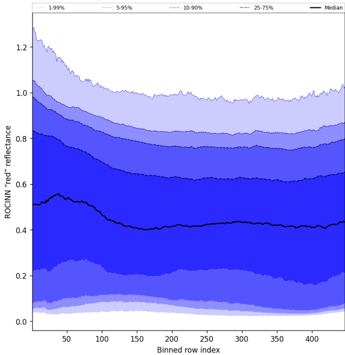
Figure 69: Along track statistics of “ROCINN “red” reflectance” for 2025-09-22 to 2025-09-24
