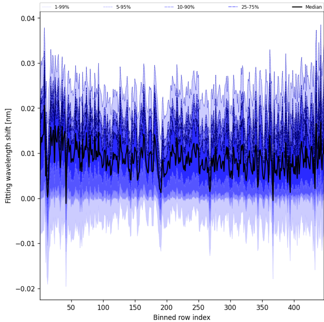
Figure 65: Along track statistics of “Fitting wavelength shift” for 2025-09-22 to 2025-09-24
