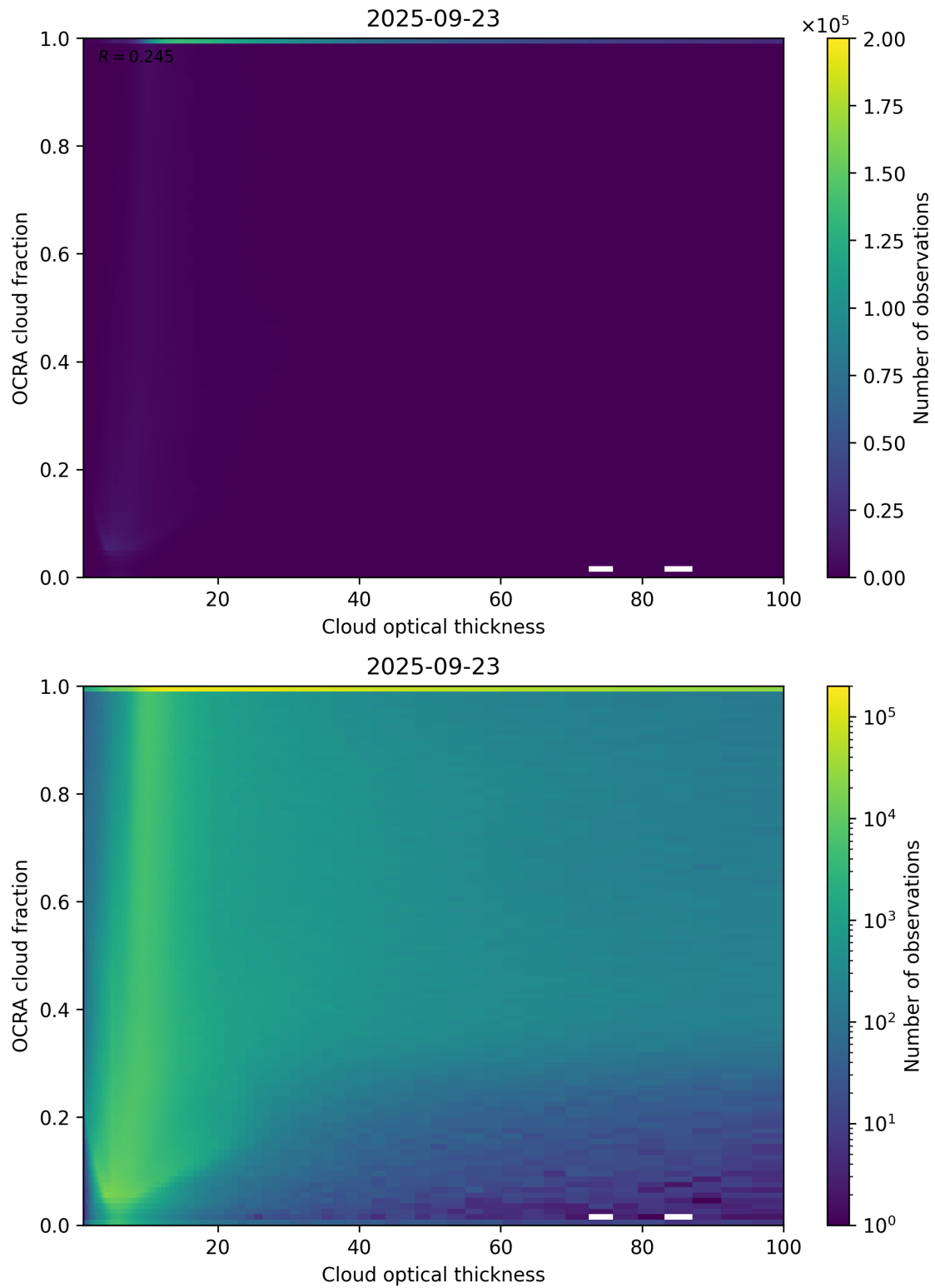
Figure 83: Scatter density plot of “Cloud optical thickness” against “OCRA cloud fraction” for 2025-09-22 to 2025-09-24.
