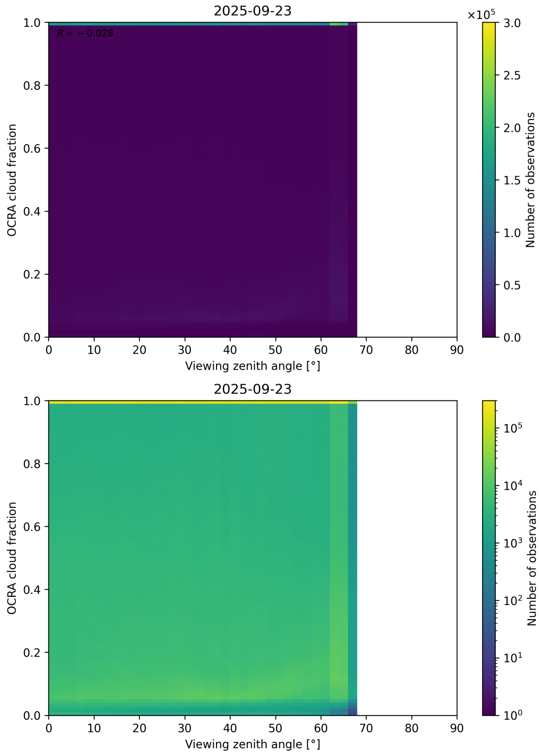
Figure 108: Scatter density plot of “Viewing zenith angle” against “OCRA cloud fraction” for 2025-09-22 to 2025-09-24.
