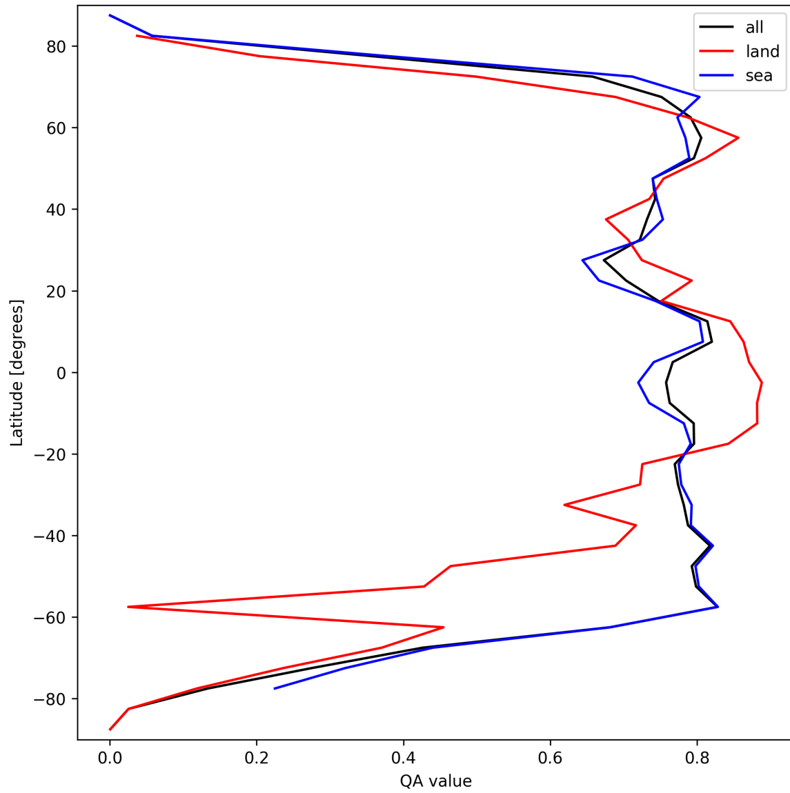
Figure 22: Zonal average of “QA value” for 2025-09-22 to 2025-09-24.
