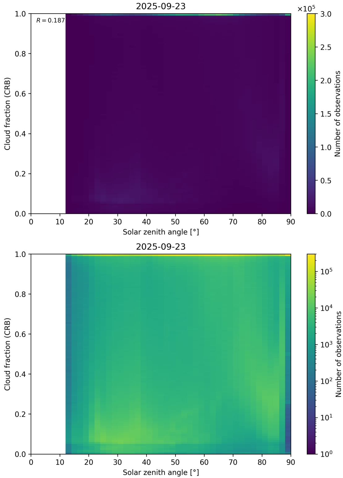
Figure 101: Scatter density plot of “Solar zenith angle” against “Cloud fraction (CRB)” for 2025-09-22 to 2025-09-24.
