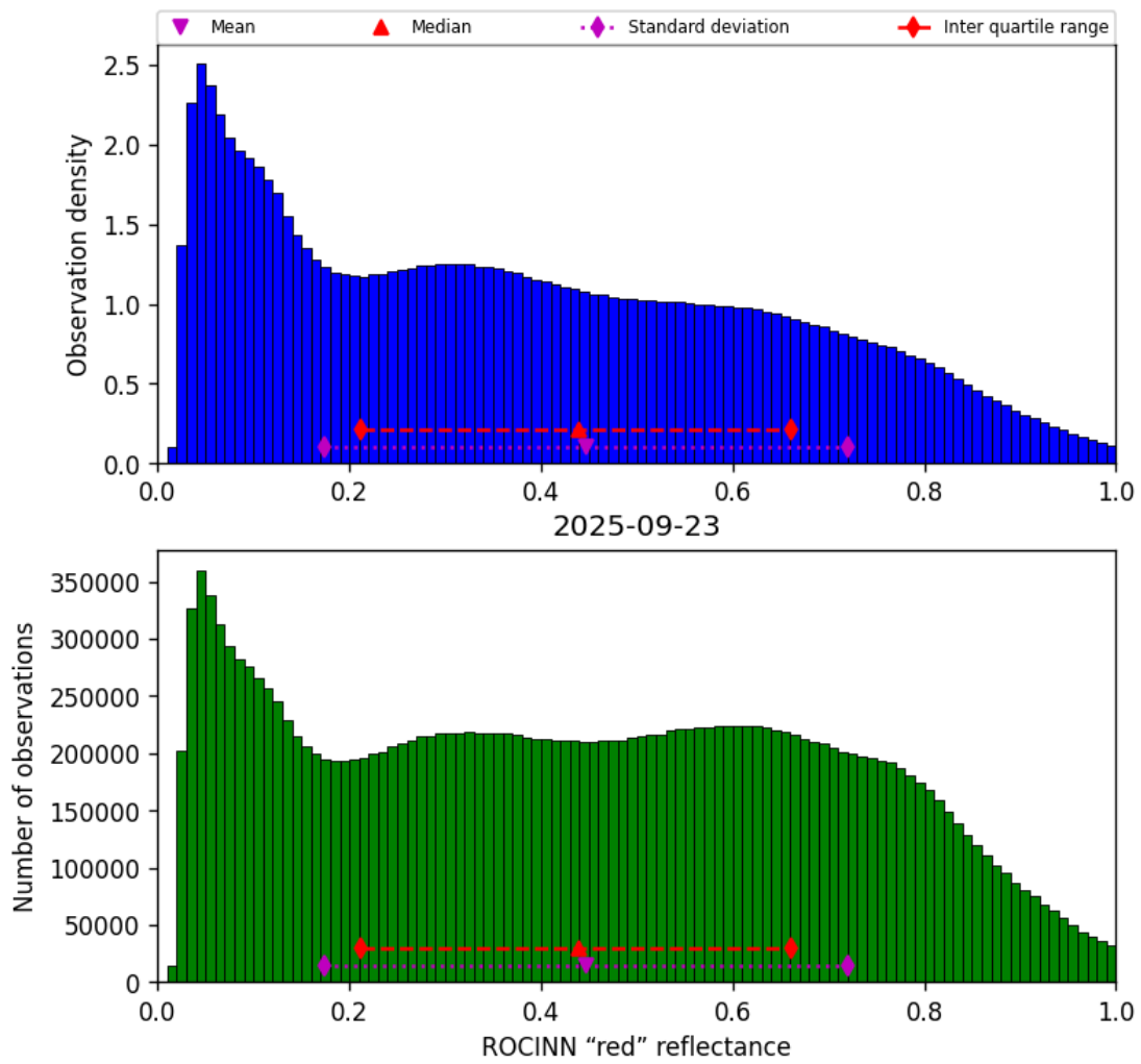
Figure 53: Histogram of “ROCINN “red” reflectance” for 2025-09-22 to 2025-09-24
