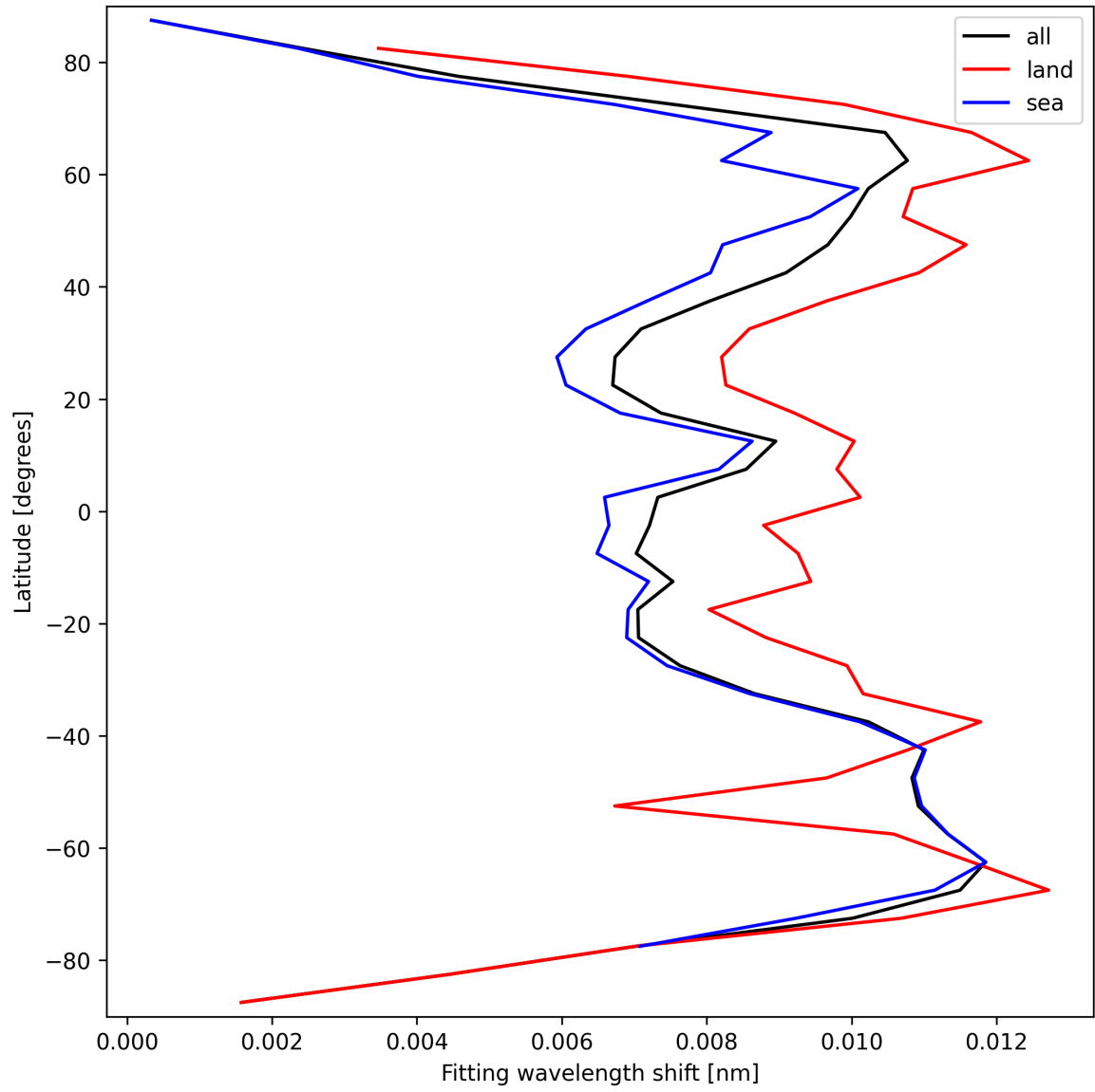
Figure 33: Zonal average of “Fitting wavelength shift” for 2025-09-22 to 2025-09-24.
