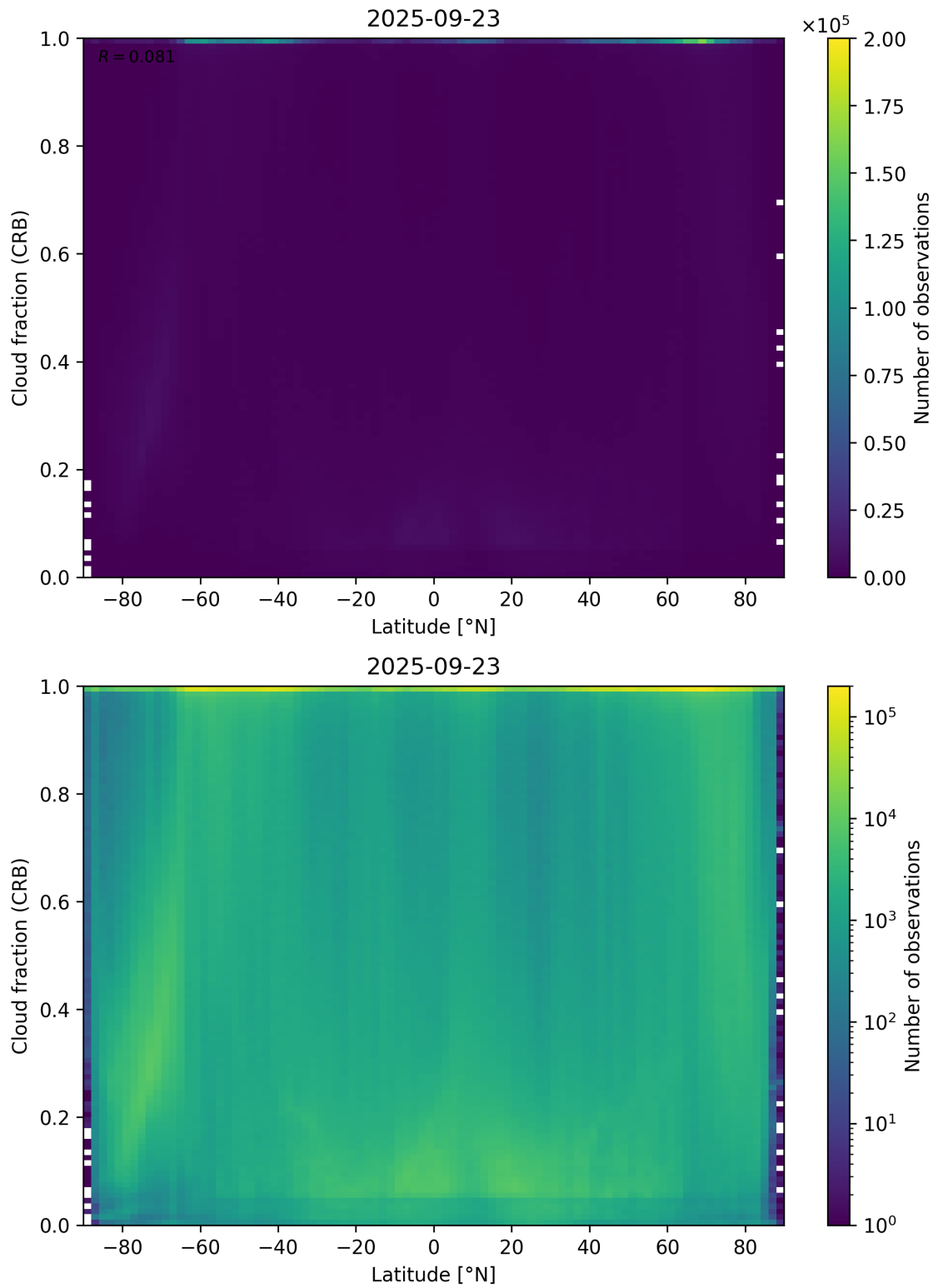
Figure 94: Scatter density plot of “Latitude” against “Cloud fraction (CRB)” for 2025-09-22 to 2025-09-24.
