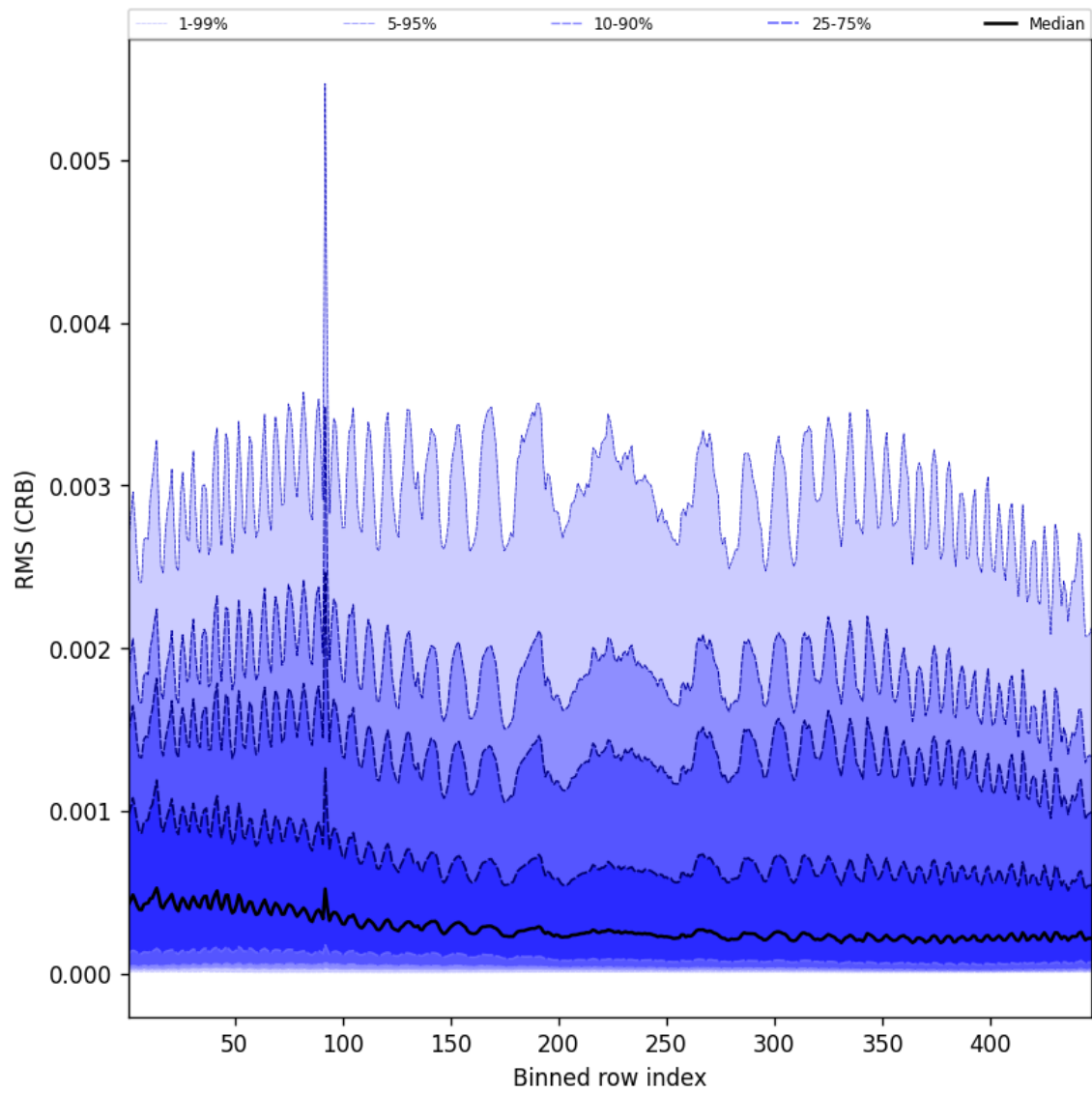
Figure 64: Along track statistics of “RMS (CRB)” for 2025-09-22 to 2025-09-24
