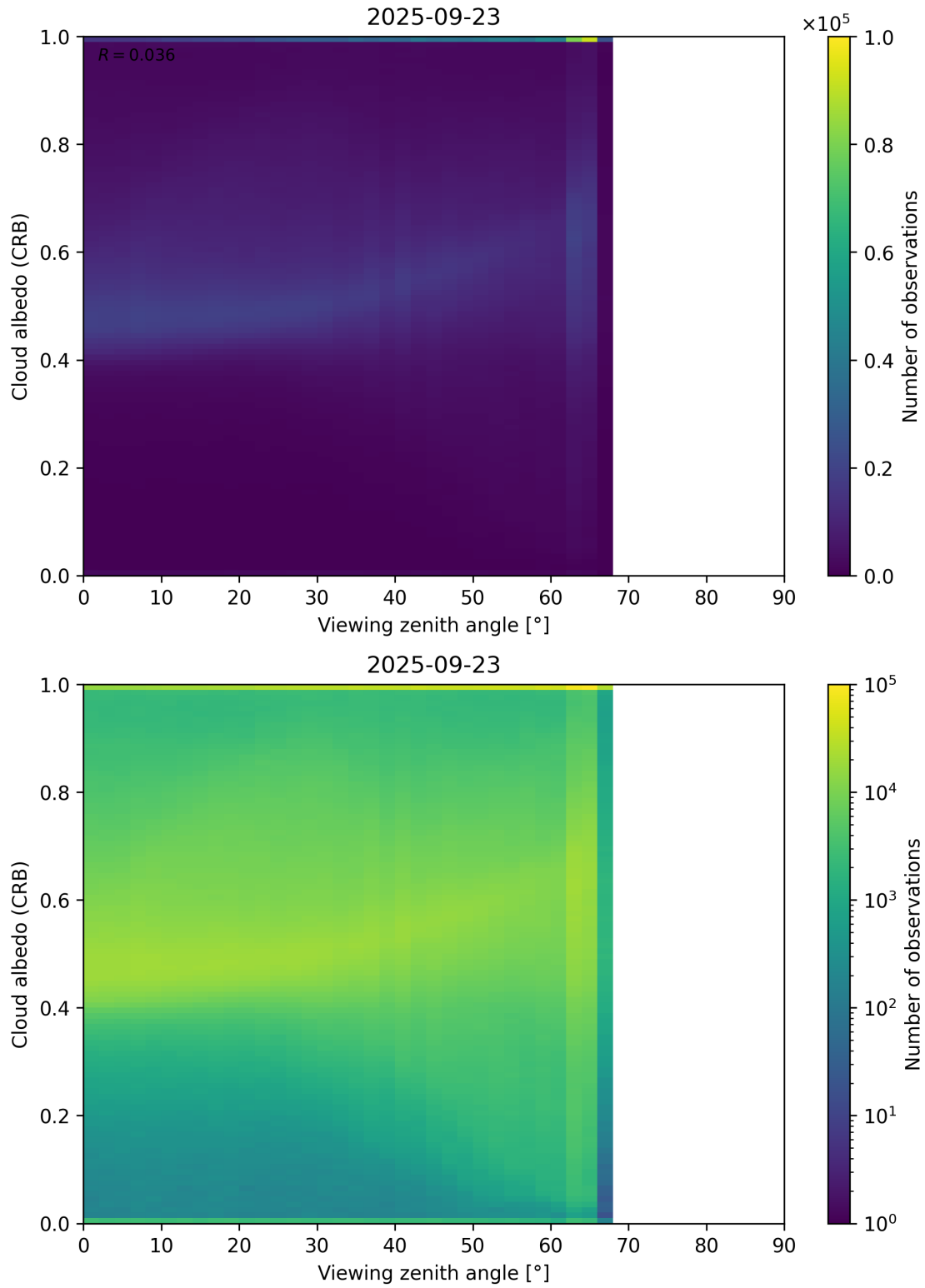
Figure 106: Scatter density plot of “Viewing zenith angle” against “Cloud albedo (CRB)” for 2025-09-22 to 2025-09-24.
