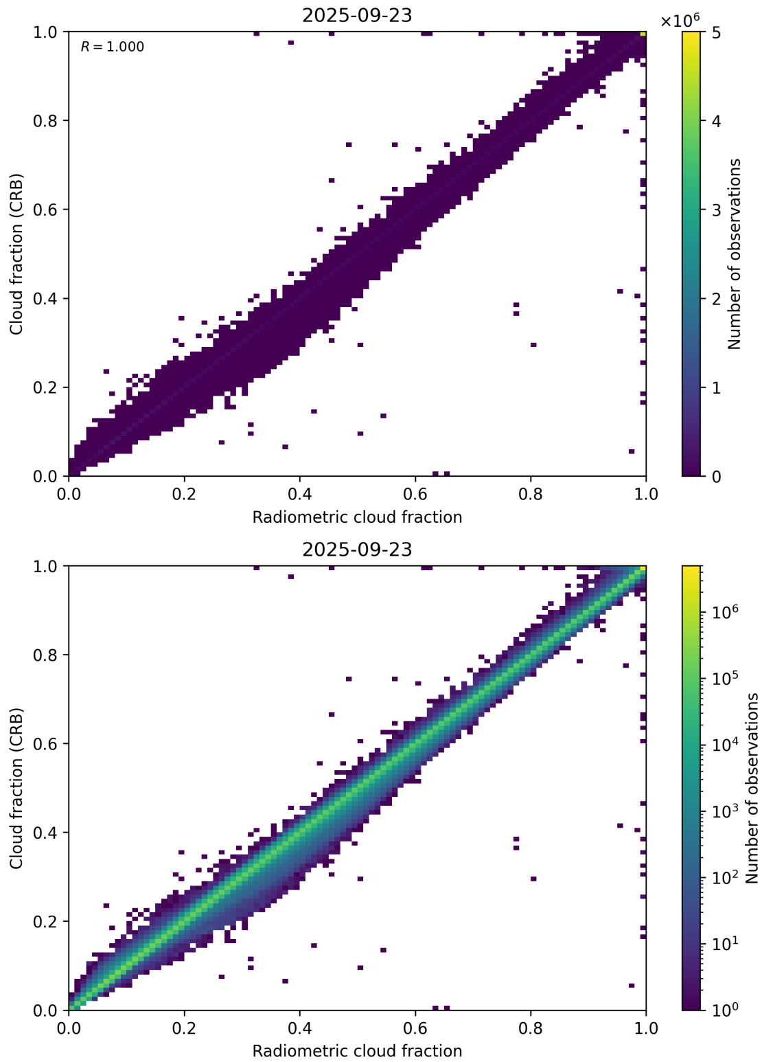
Figure 73: Scatter density plot of “Radiometric cloud fraction” against “Cloud fraction (CRB)” for 2025-09-22 to 2025-09-24.
