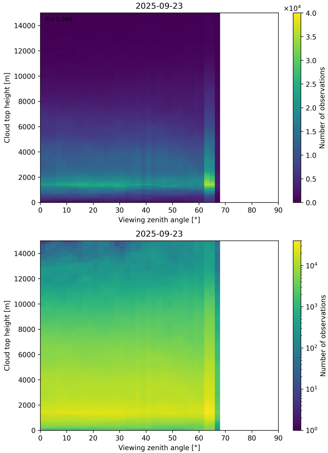
Figure 112: Scatter density plot of “Viewing zenith angle” against “Cloud top height” for 2025-09-22 to 2025-09-24.
