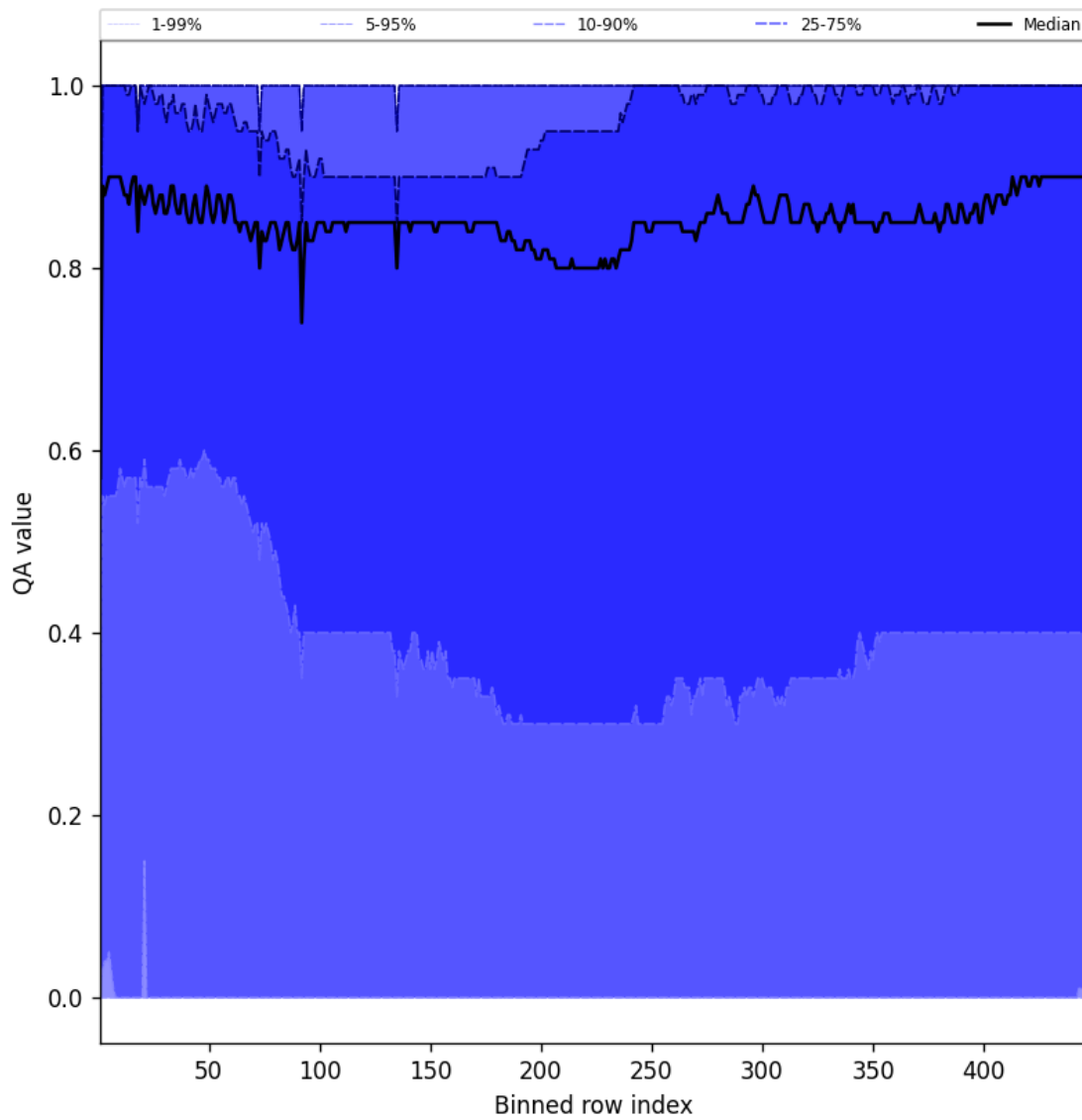
Figure 54: Along track statistics of “QA value” for 2025-09-22 to 2025-09-24
