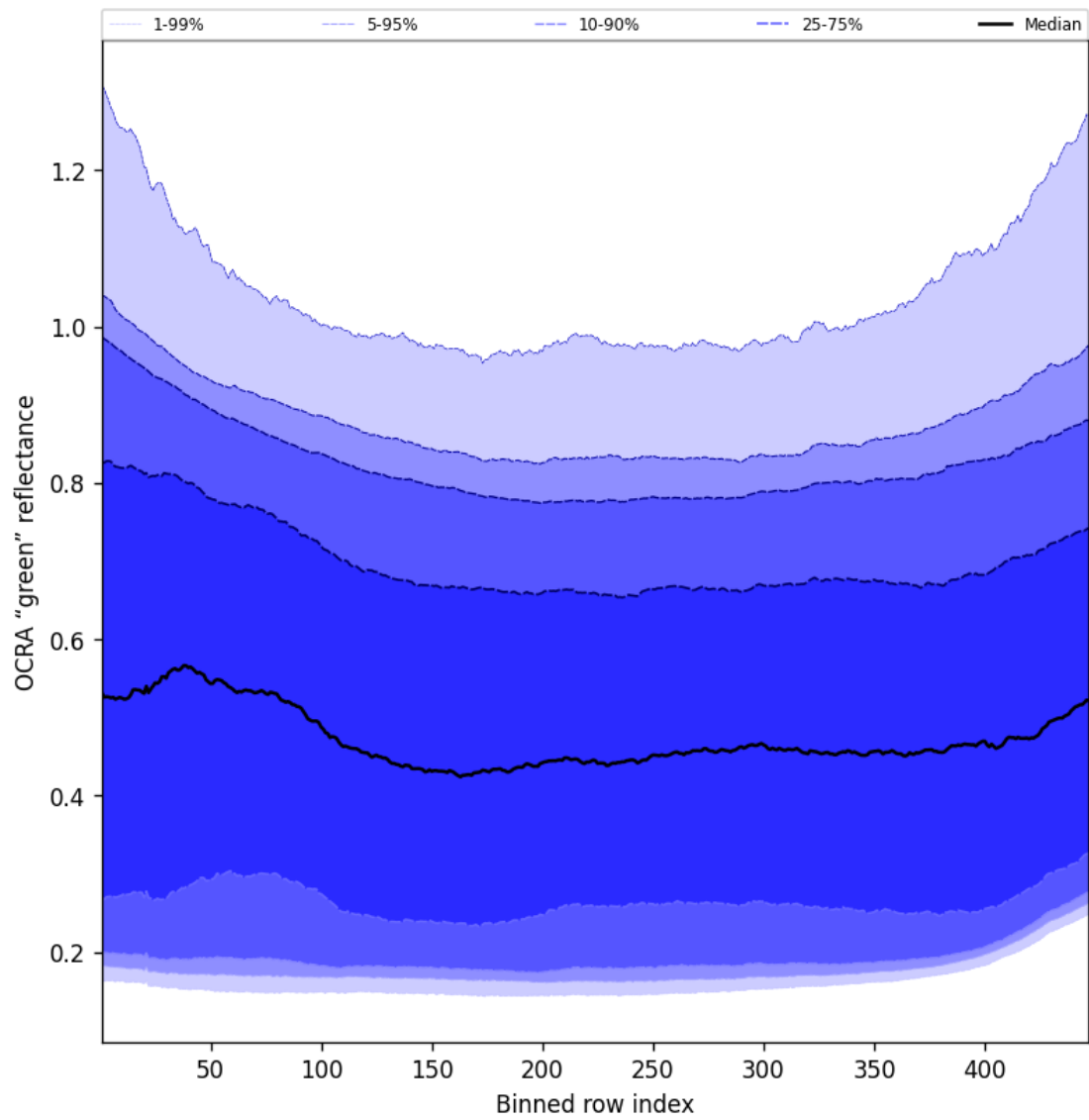
Figure 68: Along track statistics of "OCRA "green" reflectance" for 2025-09-22 to 2025-09-24
