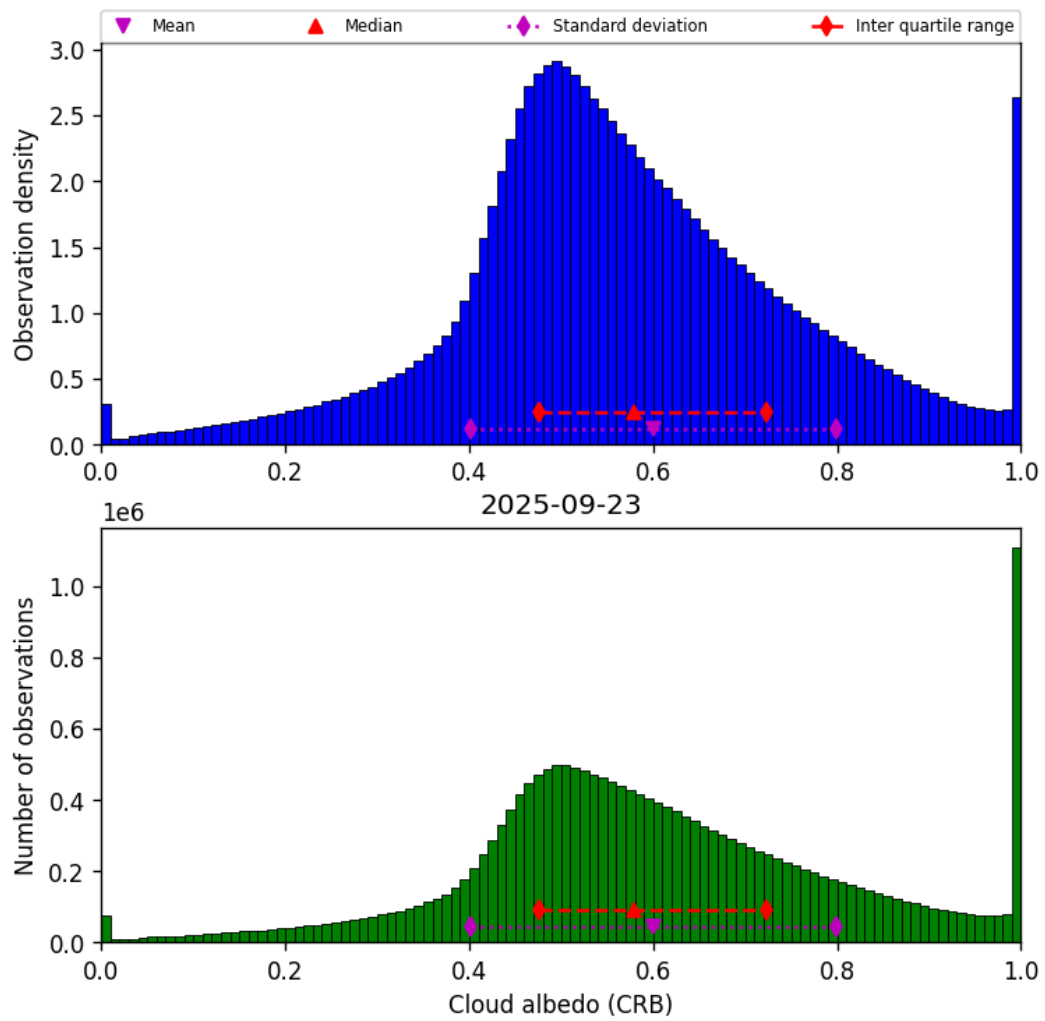
Figure 44: Histogram of “Cloud albedo (CRB)” for 2025-09-22 to 2025-09-24
