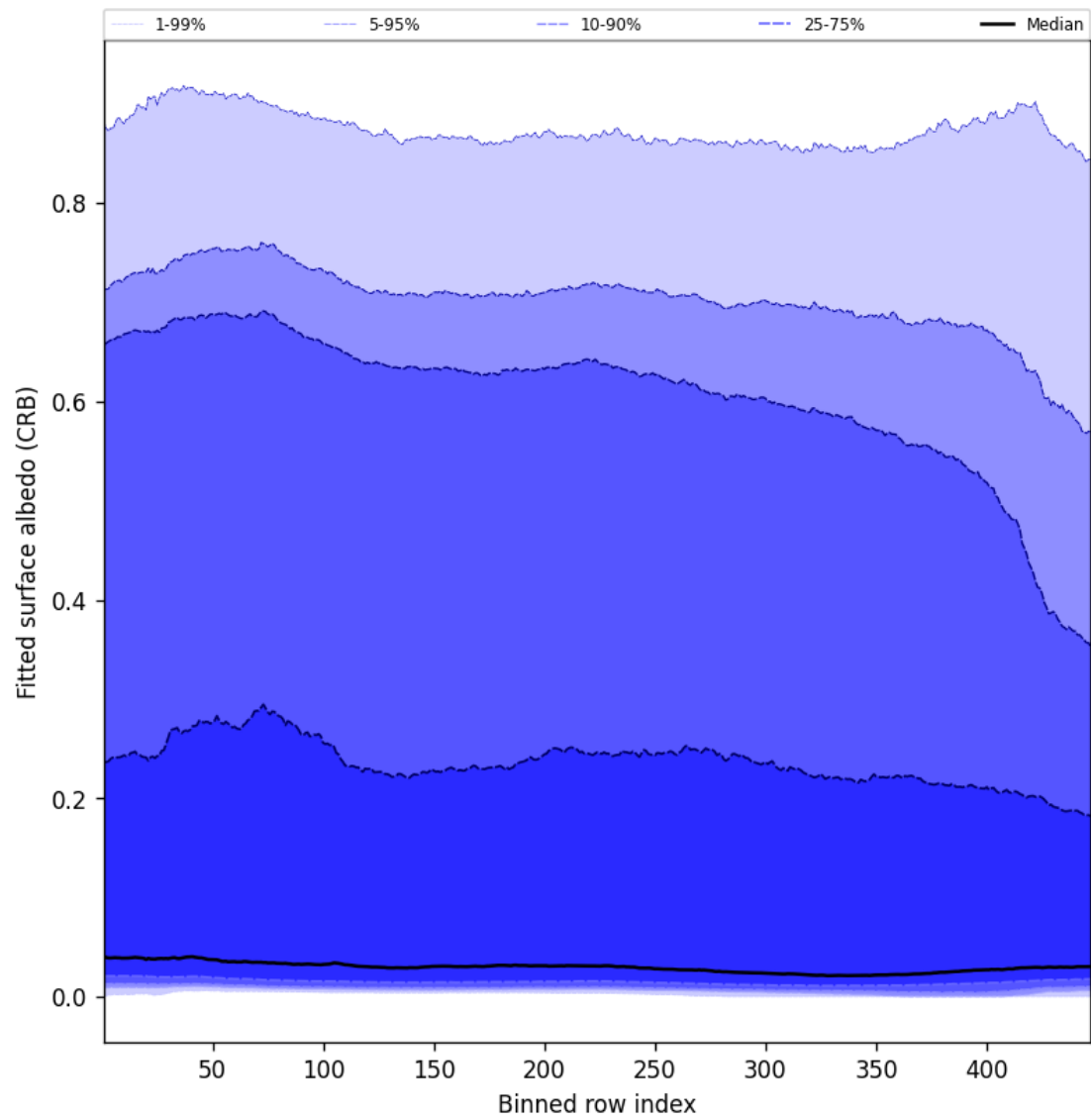
Figure 62: Along track statistics of “Fitted surface albedo (CRB)” for 2025-09-22 to 2025-09-24
