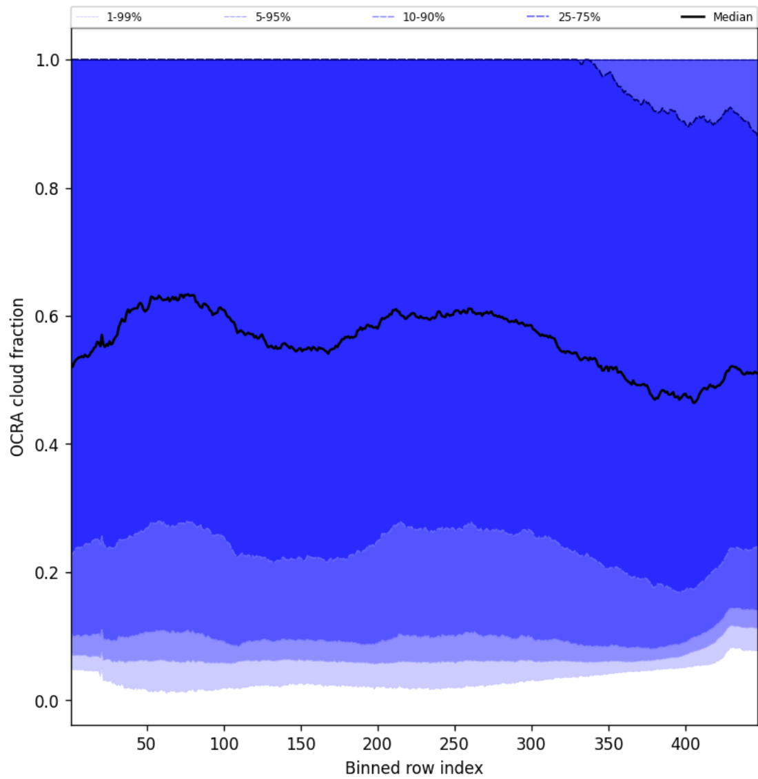
Figure 66: Along track statistics of “OCRA cloud fraction” for 2025-09-22 to 2025-09-24
