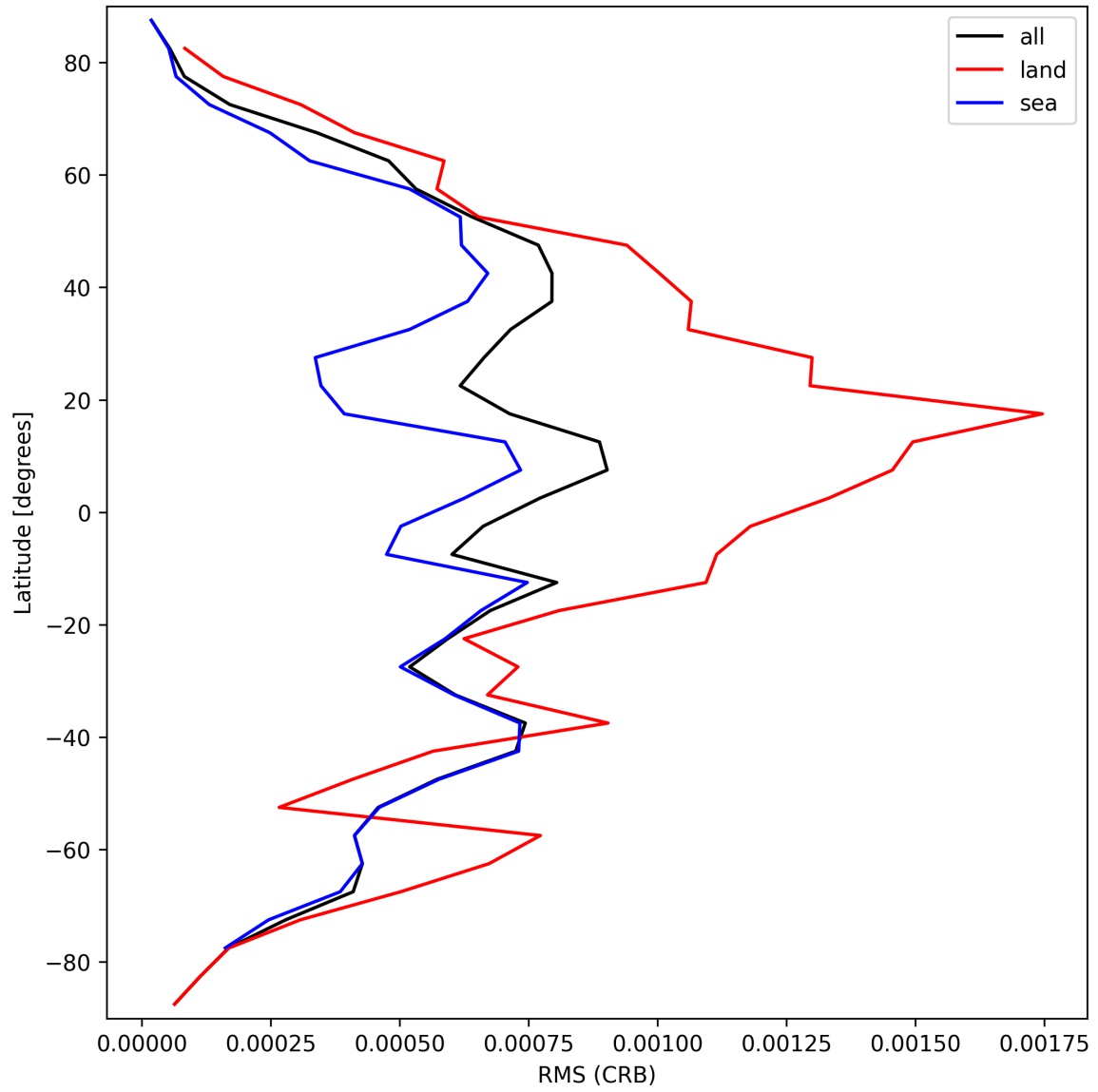
Figure 32: Zonal average of “RMS (CRB)” for 2025-09-22 to 2025-09-24.
