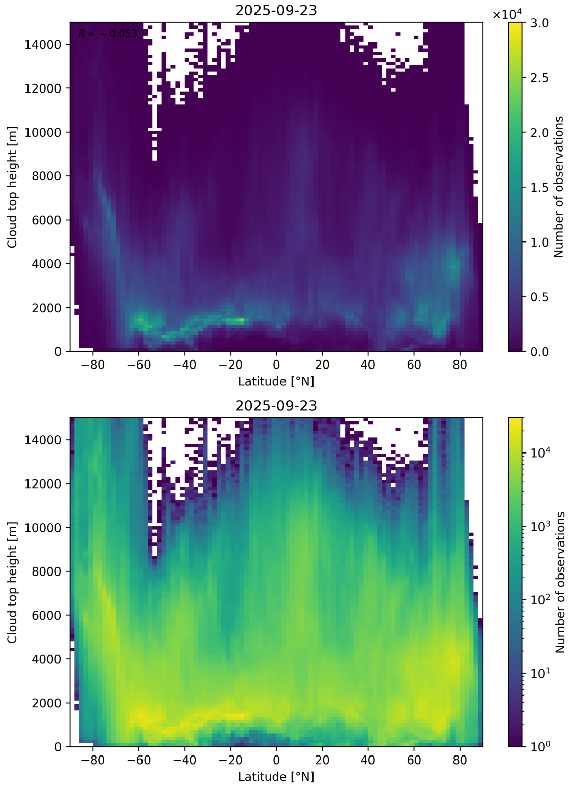
Figure 97: Scatter density plot of “Latitude” against “Cloud top height” for 2025-09-22 to 2025-09-24.
