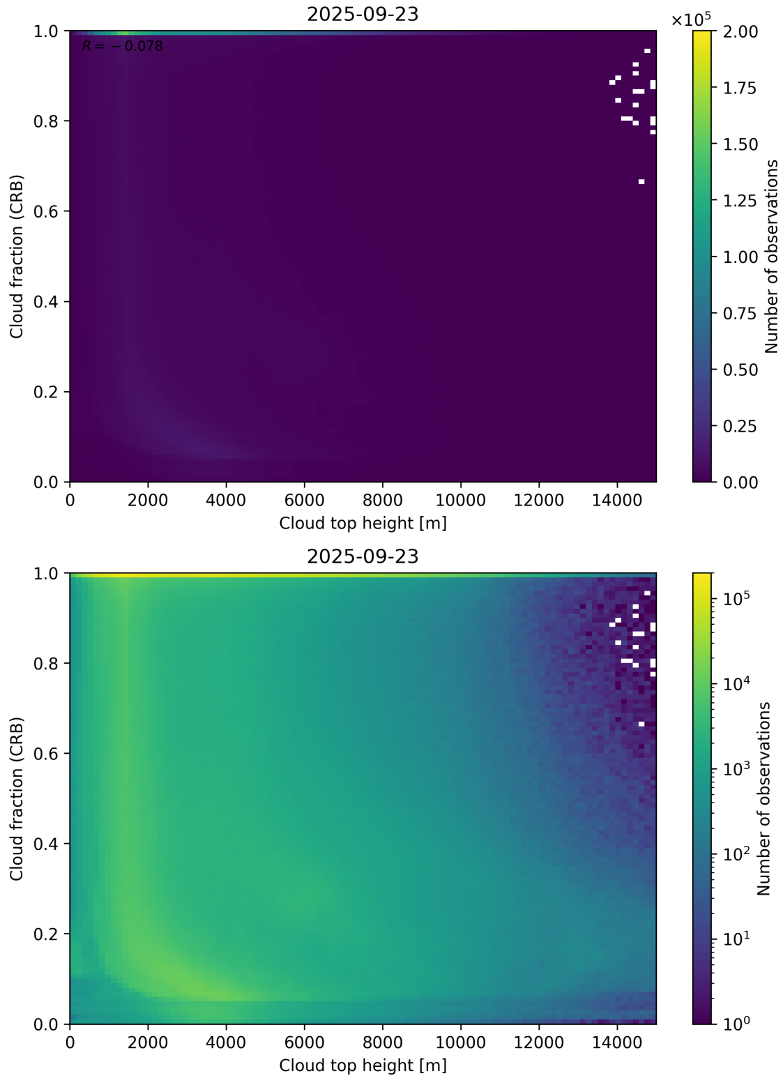
Figure 88: Scatter density plot of “Cloud top height” against “Cloud fraction (CRB)” for 2025-09-22 to 2025-09-24.
