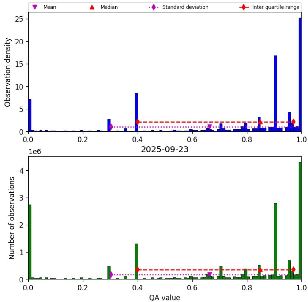
Figure 38: Histogram of “QA value” for 2025-09-22 to 2025-09-24
