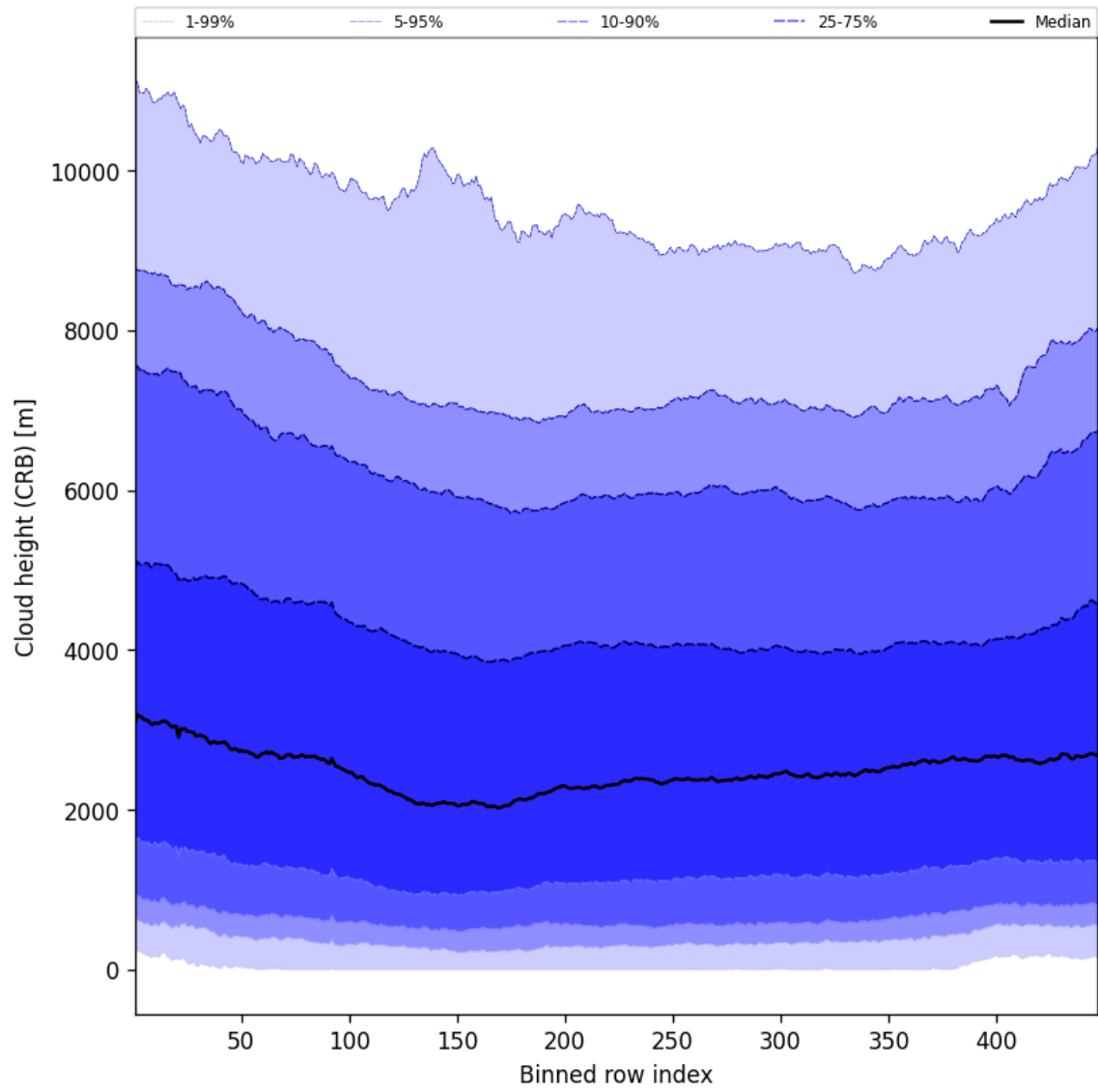
Figure 59: Along track statistics of “Cloud height (CRB)” for 2025-09-22 to 2025-09-24
