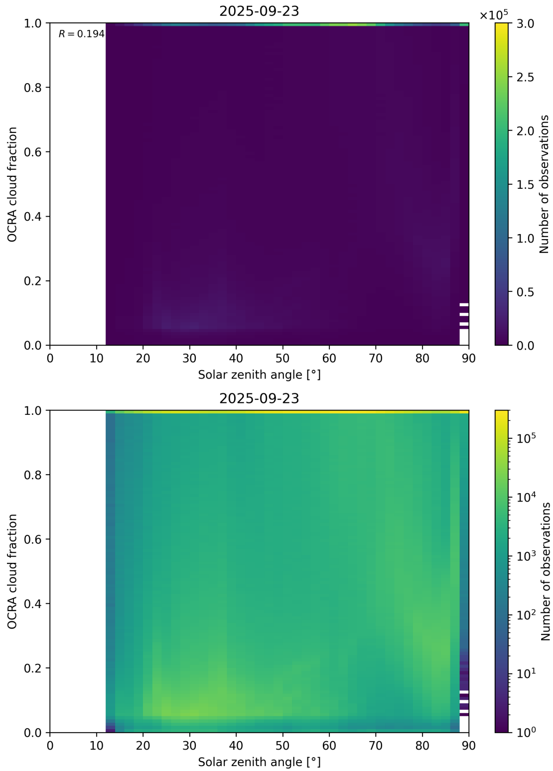
Figure 100: Scatter density plot of “Solar zenith angle” against “OCRA cloud fraction” for 2025-09-22 to 2025-09-24.
