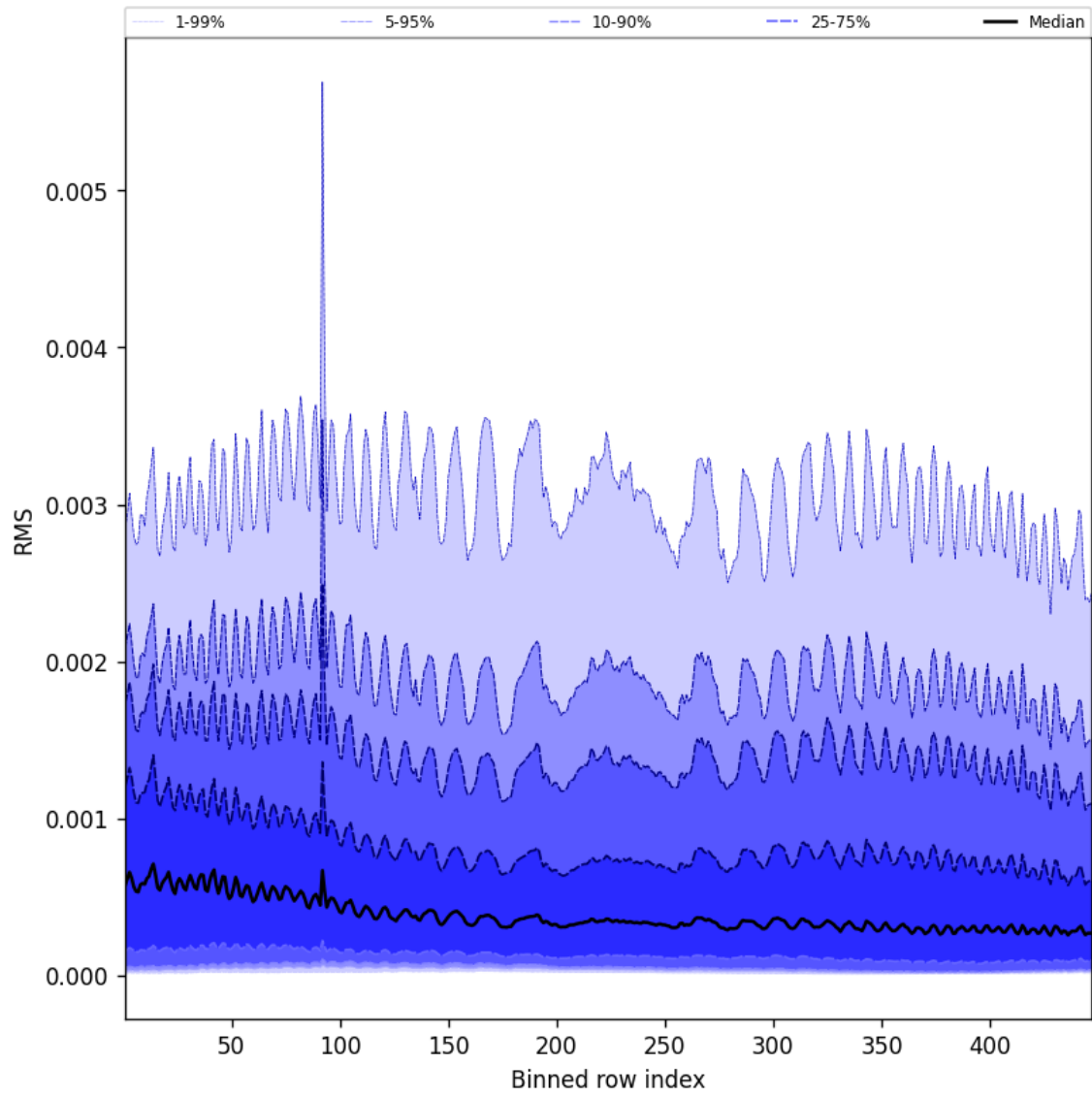
Figure 63: Along track statistics of “RMS” for 2025-09-22 to 2025-09-24
