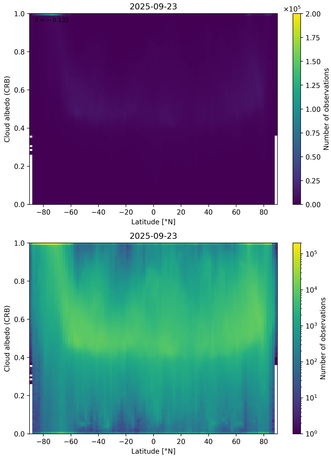
Figure 91: Scatter density plot of “Latitude” against “Cloud albedo (CRB)” for 2025-09-22 to 2025-09-24.
