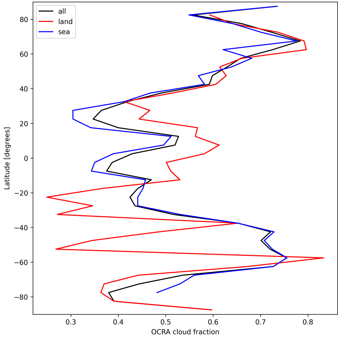
Figure 34: Zonal average of “OCRA cloud fraction” for 2025-09-22 to 2025-09-24.
