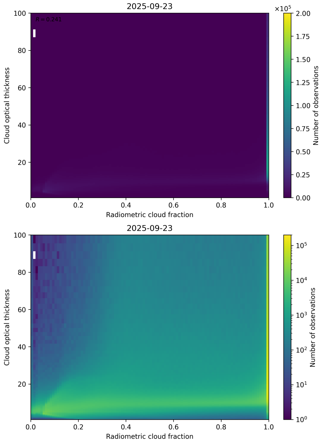
Figure 75: Scatter density plot of “Radiometric cloud fraction” against “Cloud optical thickness” for 2025-09-22 to 2025-09-24.
