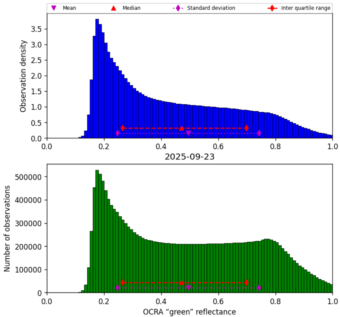
Figure 52: Histogram of “OCRA “green” reflectance” for 2025-09-22 to 2025-09-24
