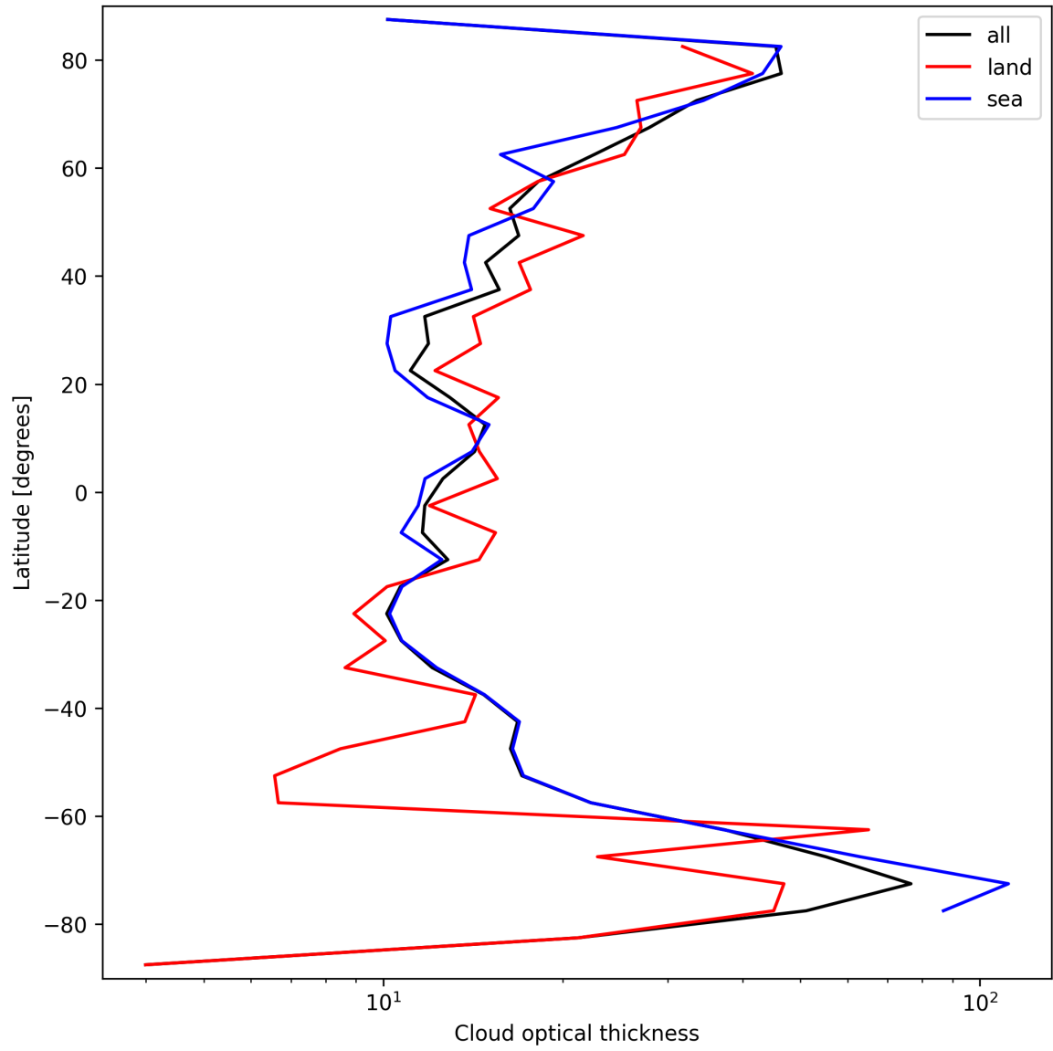
Figure 25: Zonal average of “Cloud optical thickness” for 2025-09-22 to 2025-09-24.
