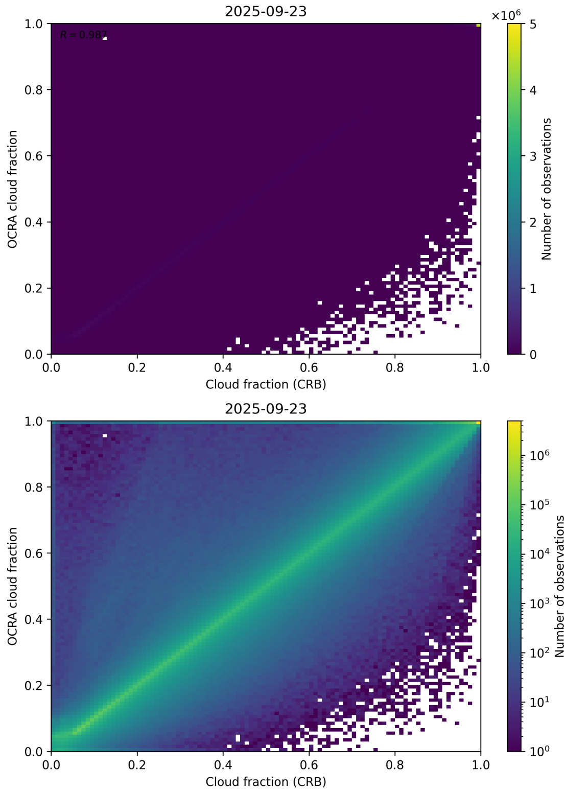
Figure 78: Scatter density plot of “Cloud fraction (CRB)” against “OCRA cloud fraction” for 2025-09-22 to 2025-09-24.
