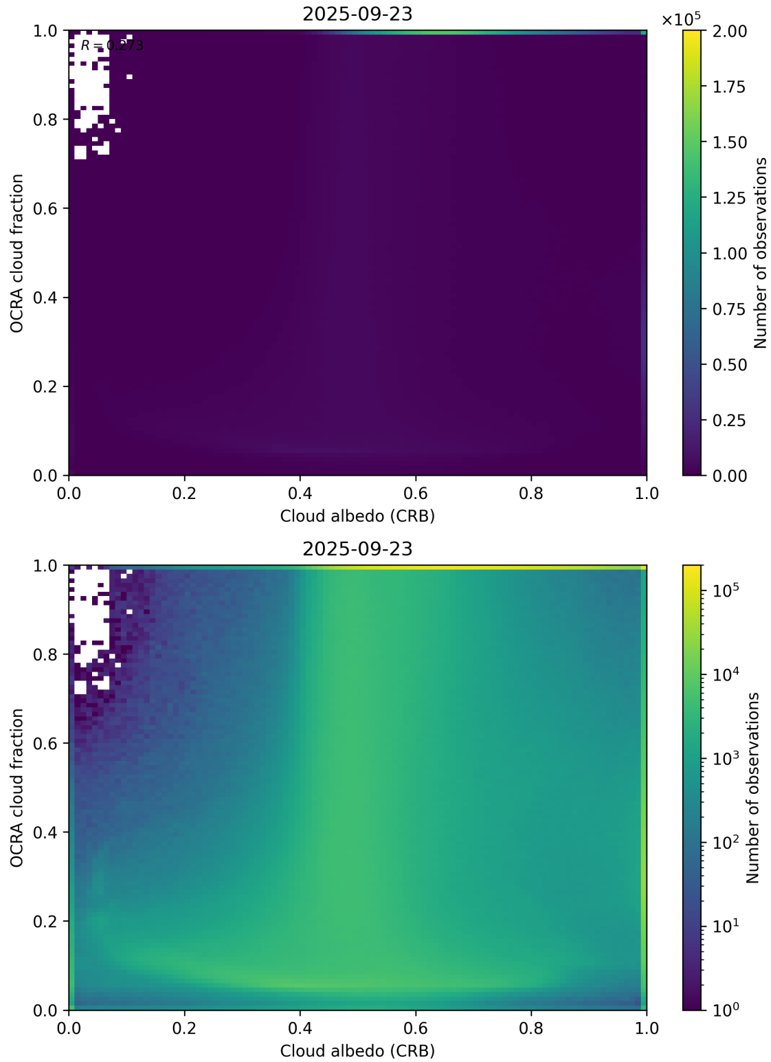
Figure 70: Scatter density plot of “Cloud albedo (CRB)” against “OCRA cloud fraction” for 2025-09-22 to 2025-09-24.
