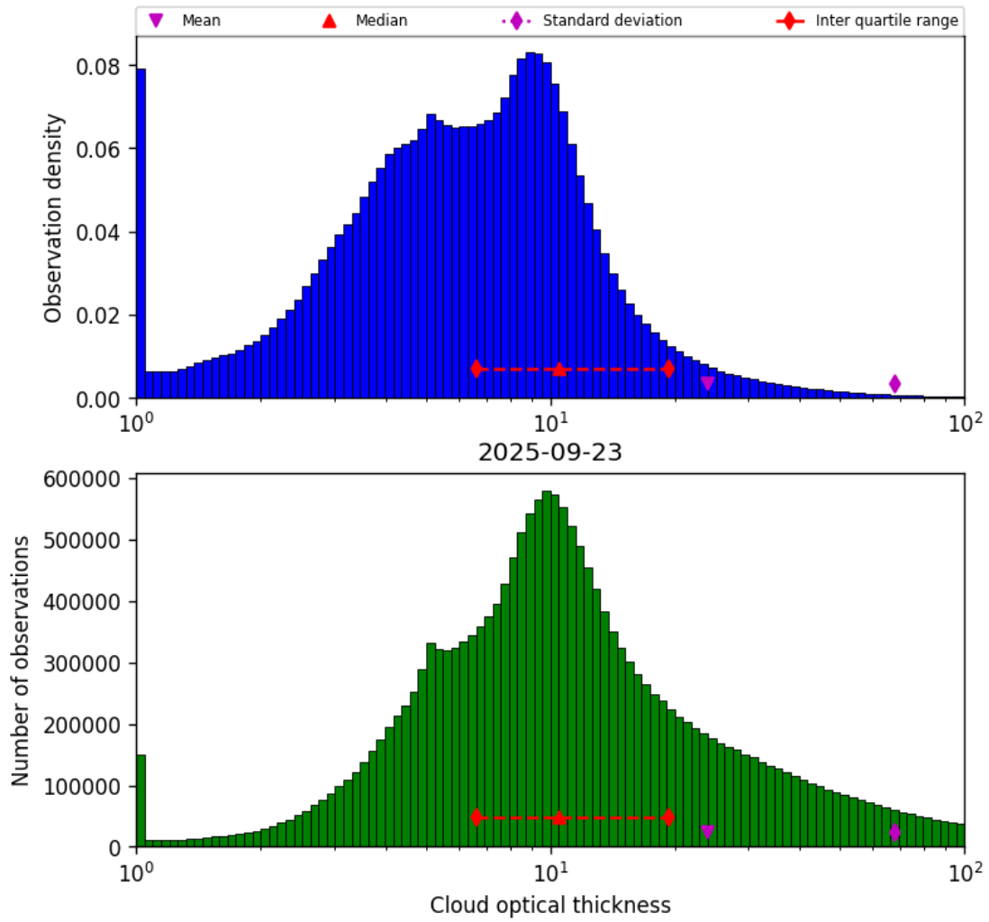
Figure 41: Histogram of “Cloud optical thickness” for 2025-09-22 to 2025-09-24
