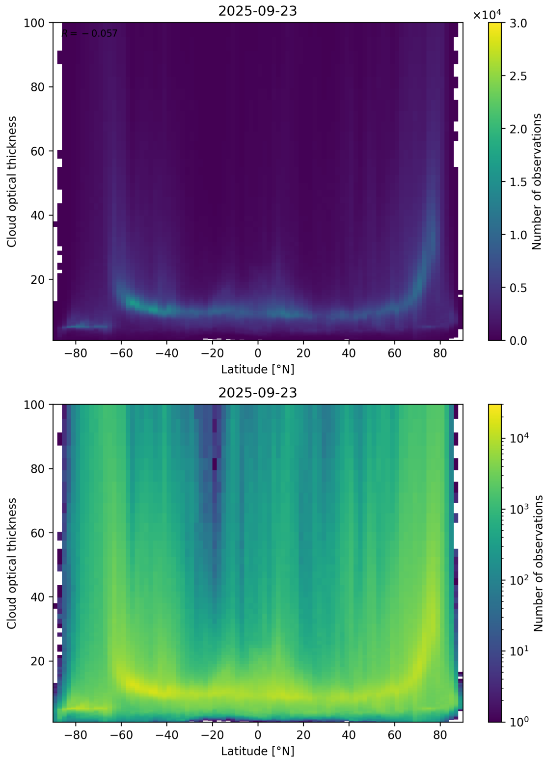
Figure 96: Scatter density plot of “Latitude” against “Cloud optical thickness” for 2025-09-22 to 2025-09-24.
