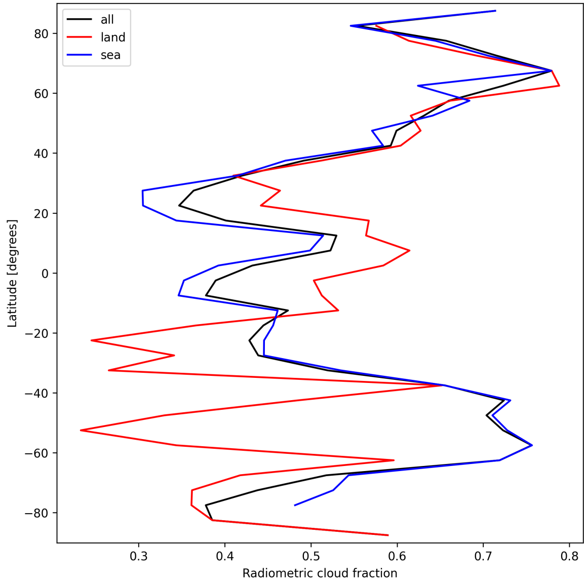
Figure 23: Zonal average of “Radiometric cloud fraction” for 2025-09-22 to 2025-09-24.
