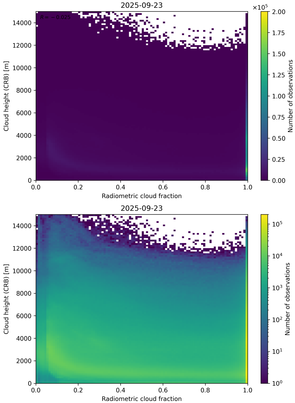
Figure 74: Scatter density plot of “Radiometric cloud fraction” against “Cloud height (CRB)” for 2025-09-22 to 2025-09-24.
