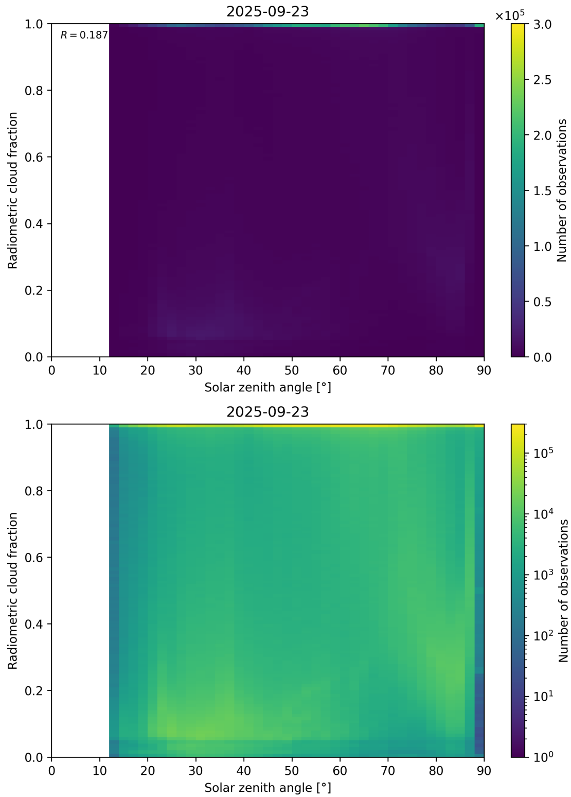
Figure 99: Scatter density plot of “Solar zenith angle” against “Radiometric cloud fraction” for 2025-09-22 to 2025-09-24.
