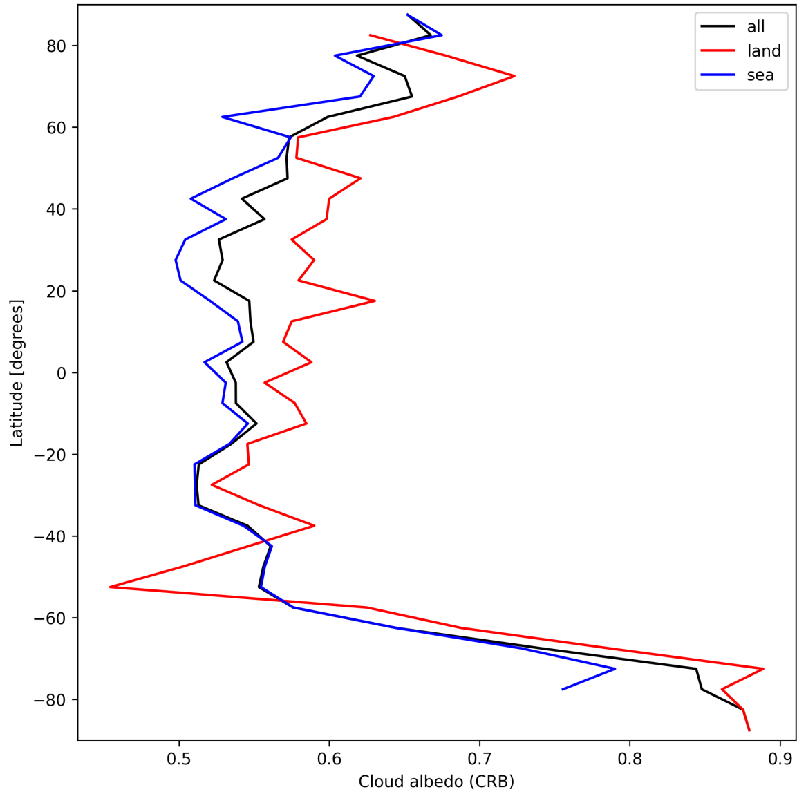
Figure 28: Zonal average of “Cloud albedo (CRB)” for 2025-09-22 to 2025-09-24.
