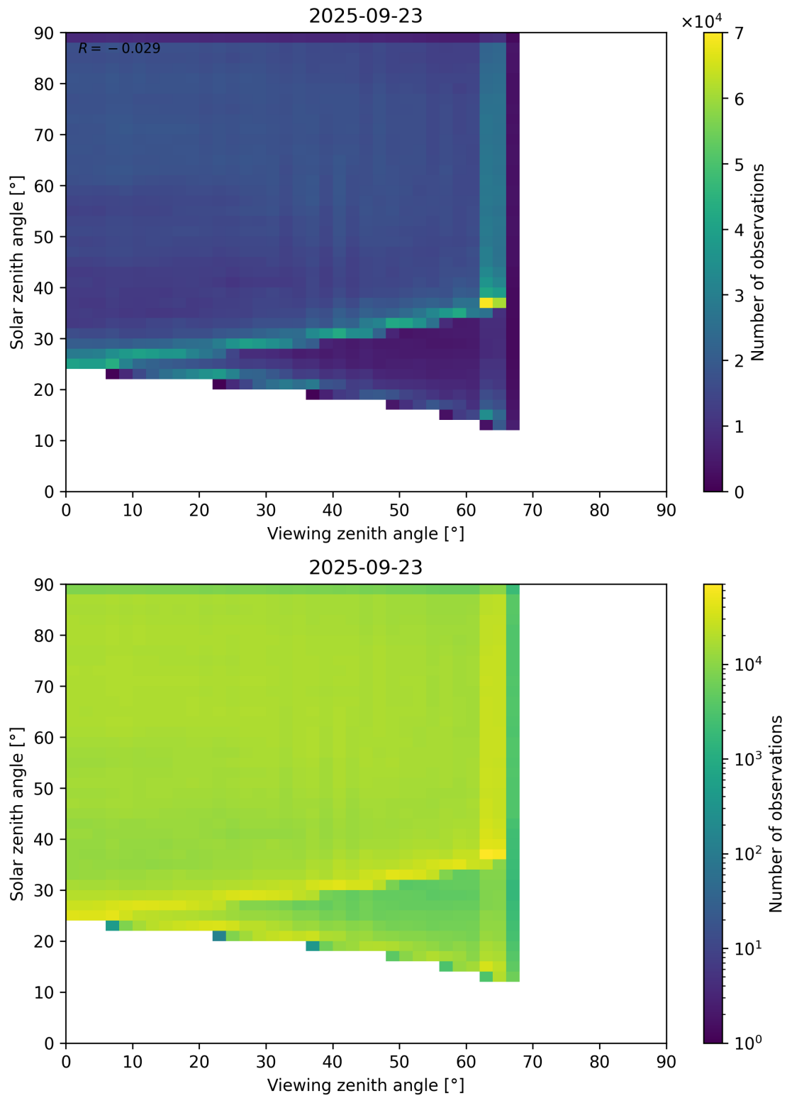
Figure 114: Scatter density plot of “Viewing zenith angle” against “Solar zenith angle” for 2025-09-22 to 2025-09-24.
