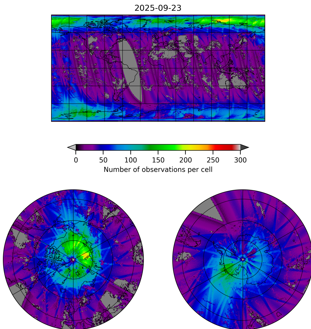
Figure 21: Map of the number of observations for 2025-09-22 to 2025-09-24
