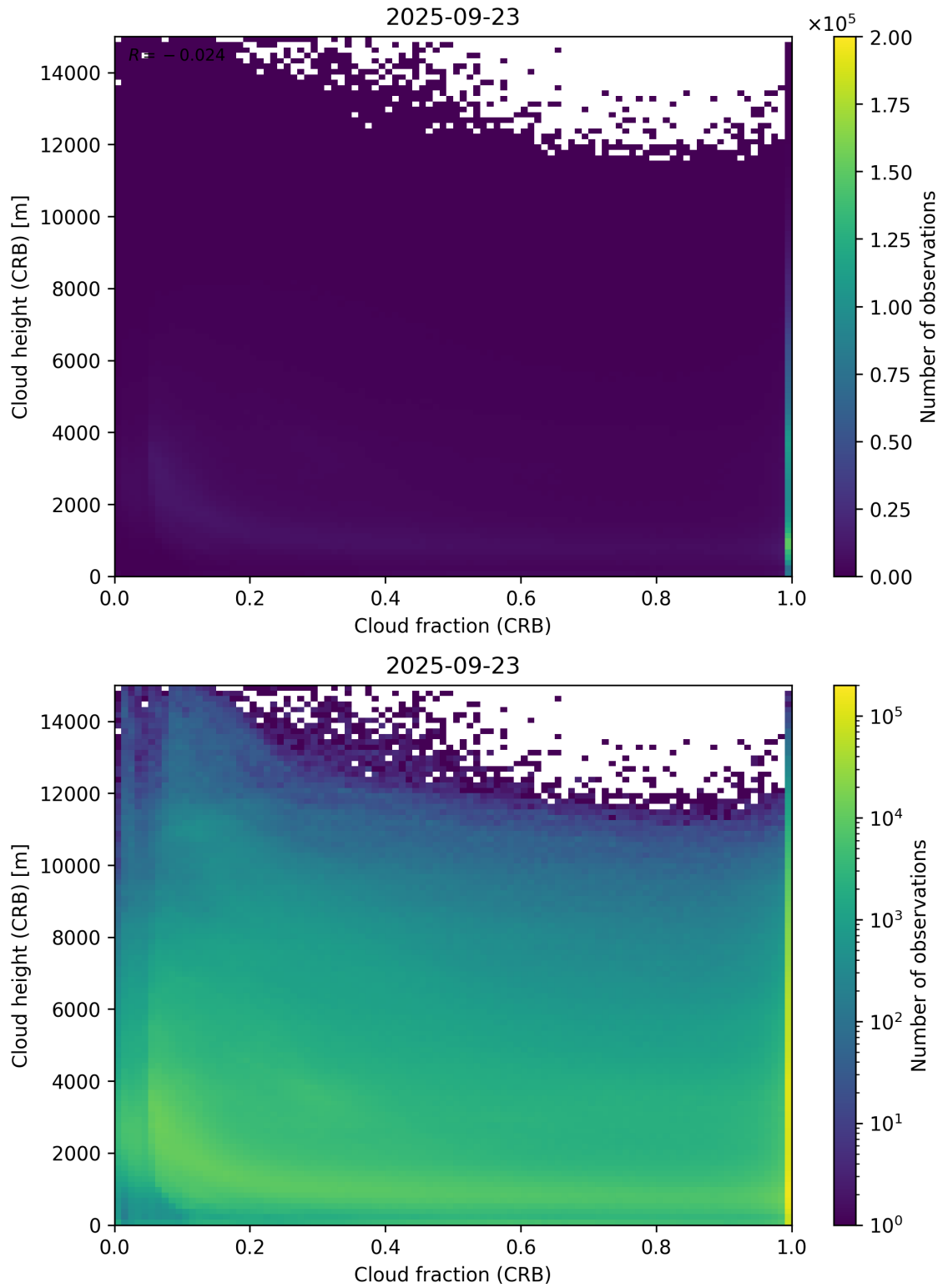
Figure 79: Scatter density plot of “Cloud fraction (CRB)” against “Cloud height (CRB)” for 2025-09-22 to 2025-09-24.
