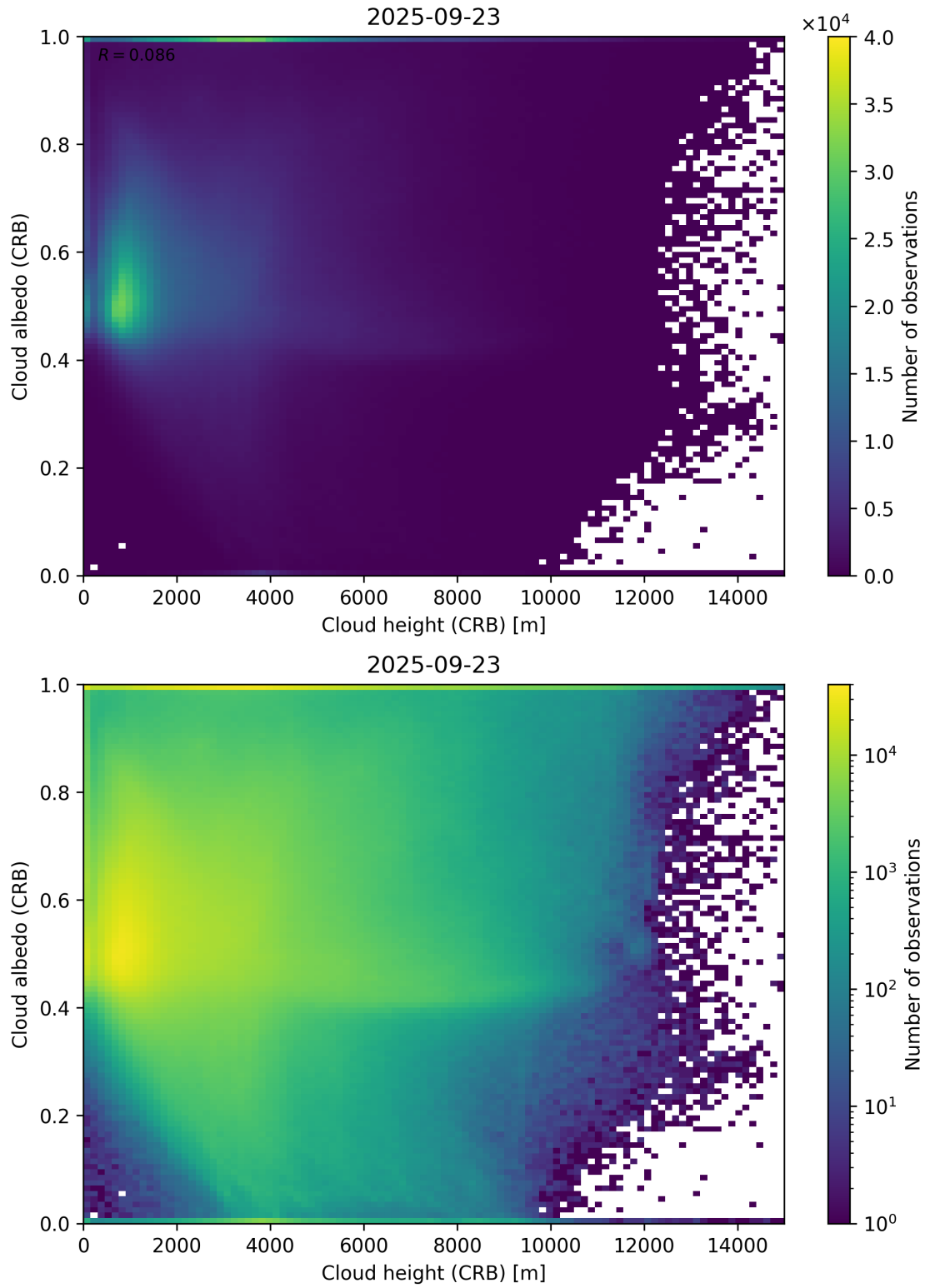
Figure 80: Scatter density plot of “Cloud height (CRB)” against “Cloud albedo (CRB)” for 2025-09-22 to 2025-09-24.
