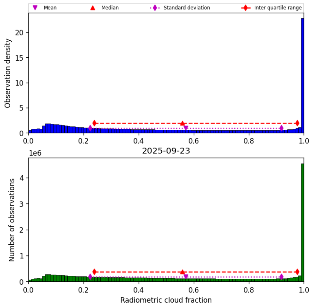
Figure 39: Histogram of “Radiometric cloud fraction” for 2025-09-22 to 2025-09-24
