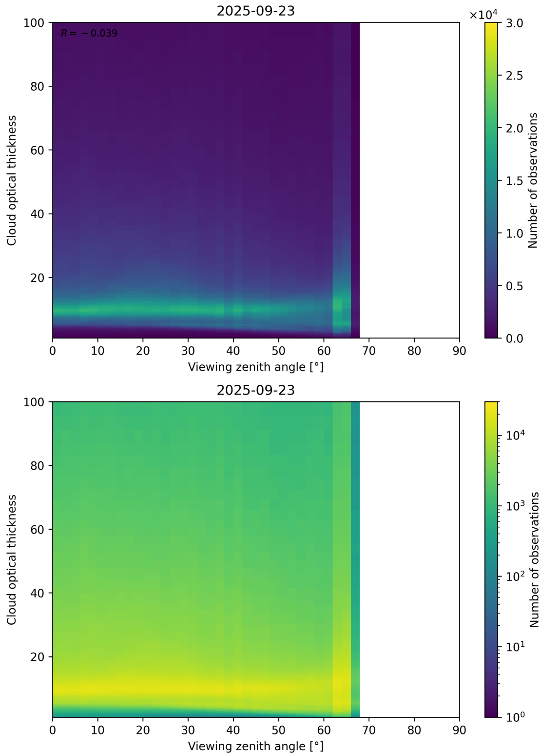
Figure 111: Scatter density plot of “Viewing zenith angle” against “Cloud optical thickness” for 2025-09-22 to 2025-09-24.
