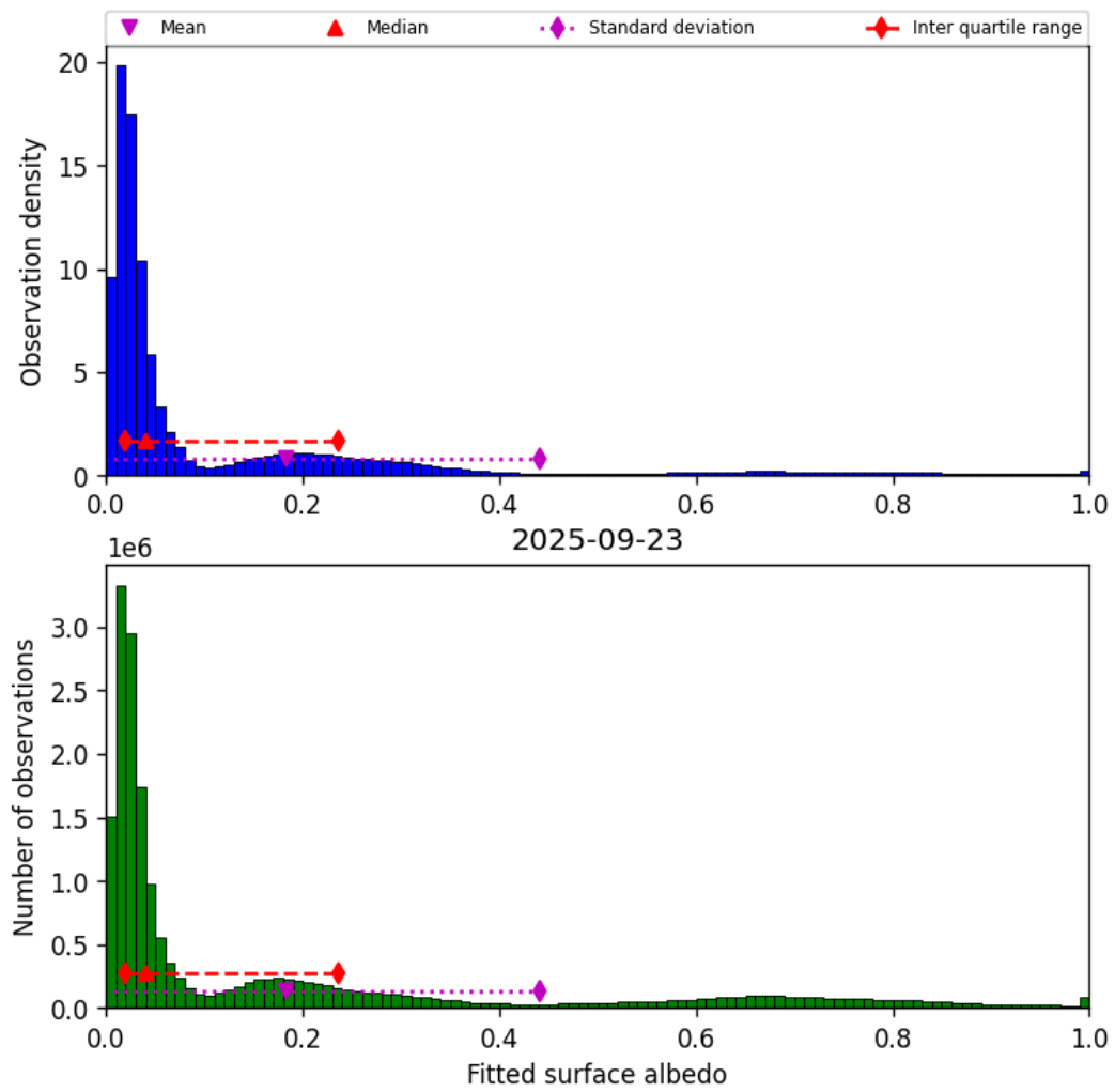
Figure 45: Histogram of “Fitted surface albedo” for 2025-09-22 to 2025-09-24
