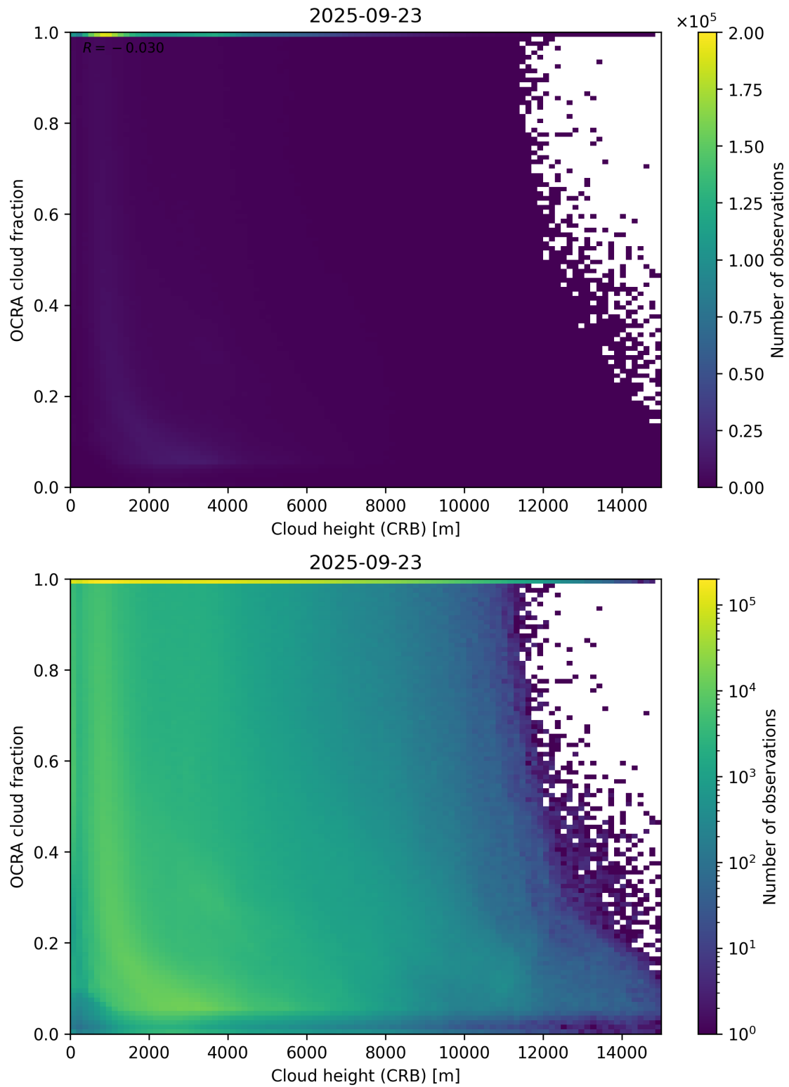
Figure 81: Scatter density plot of “Cloud height (CRB)” against “OCRA cloud fraction” for 2025-09-22 to 2025-09-24.
