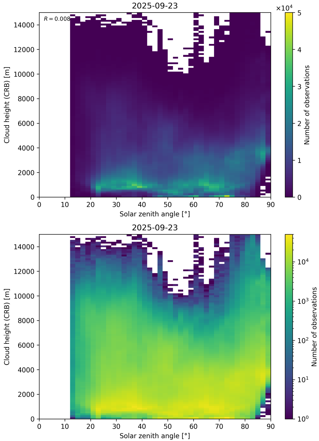
Figure 102: Scatter density plot of “Solar zenith angle” against “Cloud height (CRB)” for 2025-09-22 to 2025-09-24.
