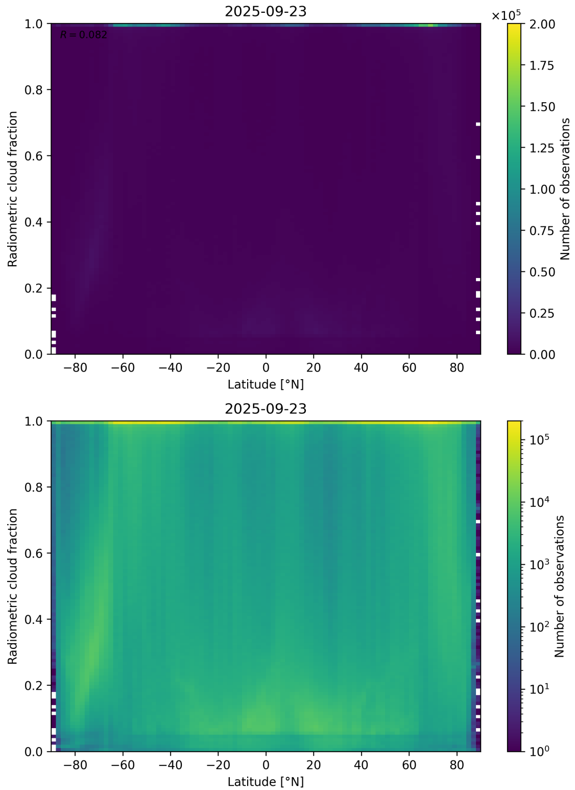
Figure 92: Scatter density plot of “Latitude” against “Radiometric cloud fraction” for 2025-09-22 to 2025-09-24.
