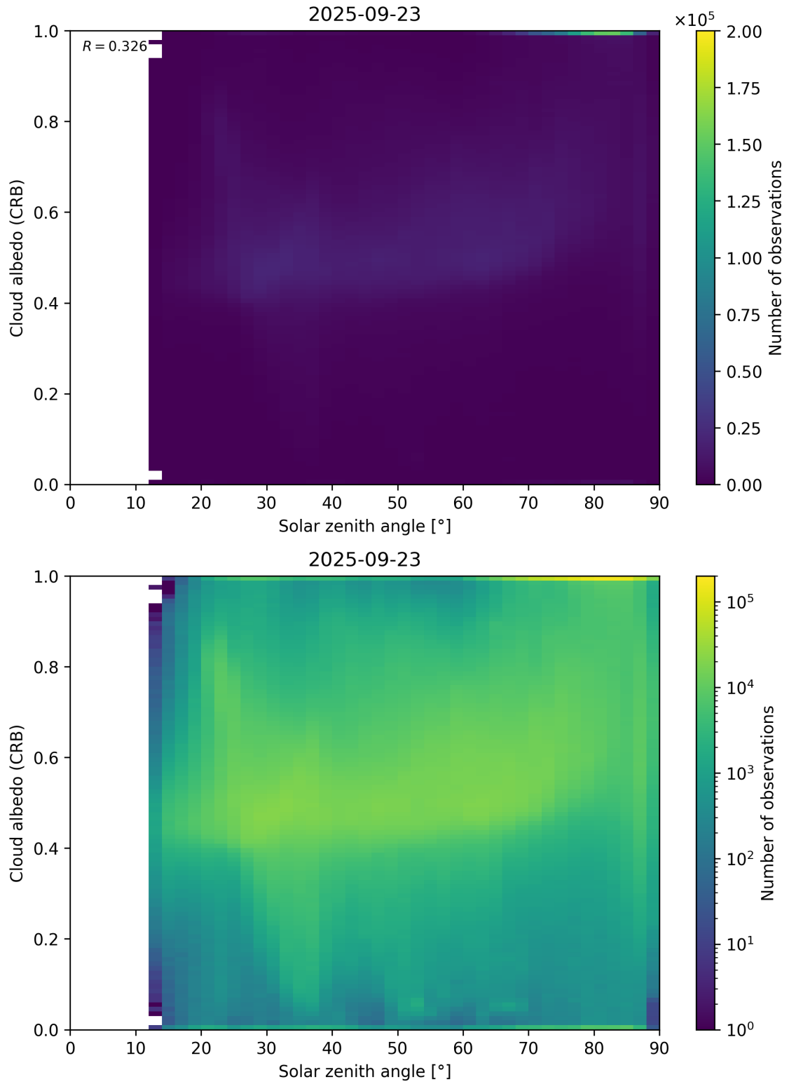
Figure 98: Scatter density plot of “Solar zenith angle” against “Cloud albedo (CRB)” for 2025-09-22 to 2025-09-24.
