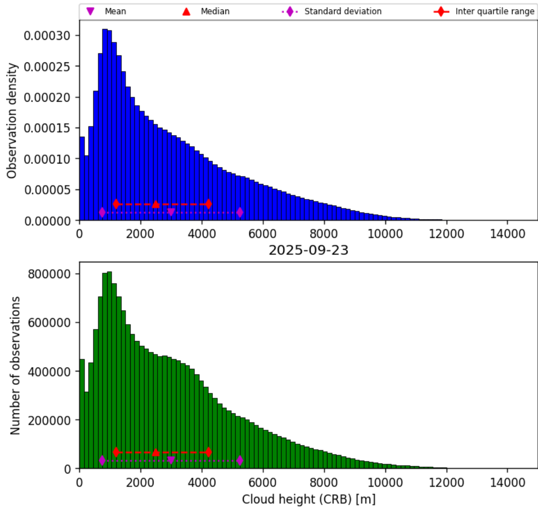
Figure 43: Histogram of “Cloud height (CRB)” for 2025-09-22 to 2025-09-24
