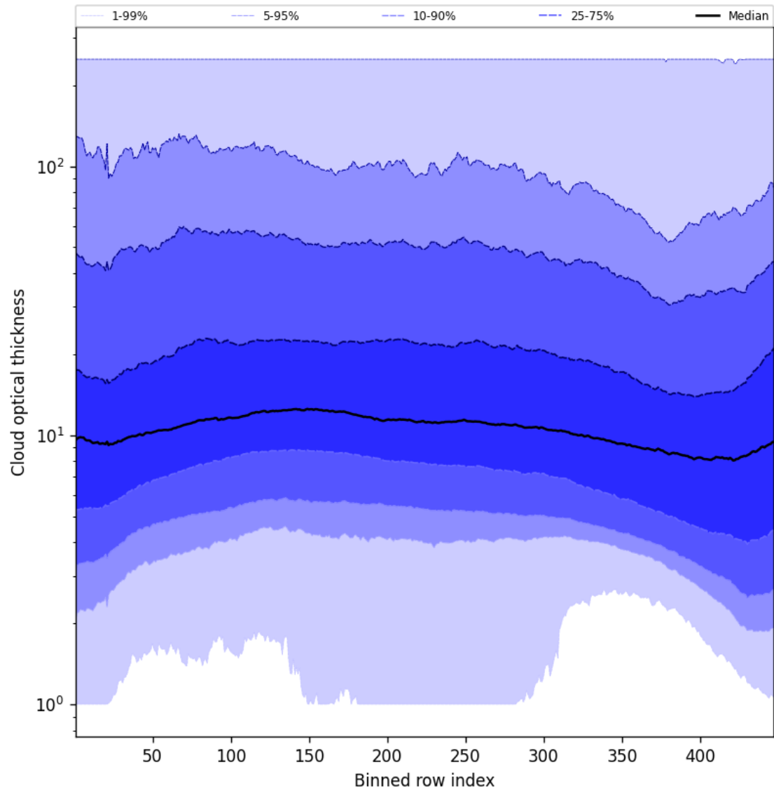
Figure 57: Along track statistics of “Cloud optical thickness” for 2025-09-22 to 2025-09-24
