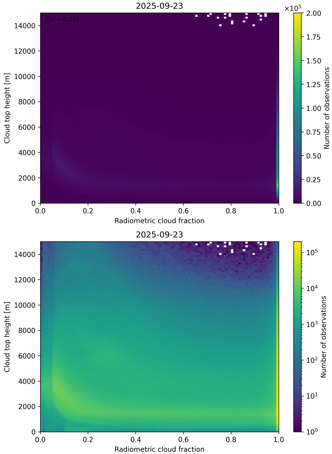
Figure 76: Scatter density plot of “Radiometric cloud fraction” against “Cloud top height” for 2025-09-22 to 2025-09-24.
