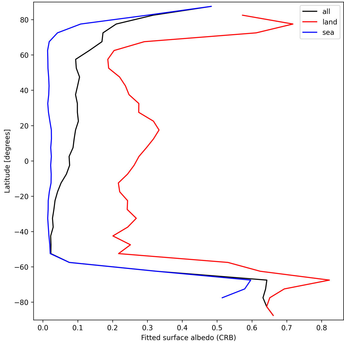
Figure 30: Zonal average of “Fitted surface albedo (CRB)” for 2025-09-22 to 2025-09-24.
