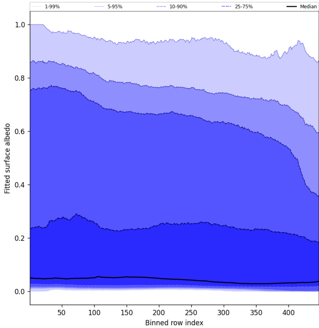
Figure 61: Along track statistics of “Fitted surface albedo” for 2025-09-22 to 2025-09-24
