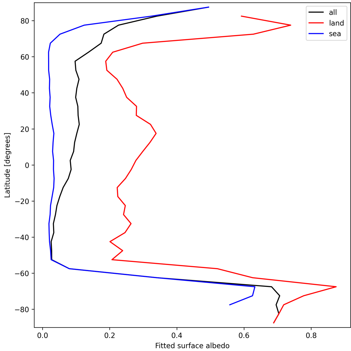
Figure 29: Zonal average of “Fitted surface albedo” for 2025-09-22 to 2025-09-24.
