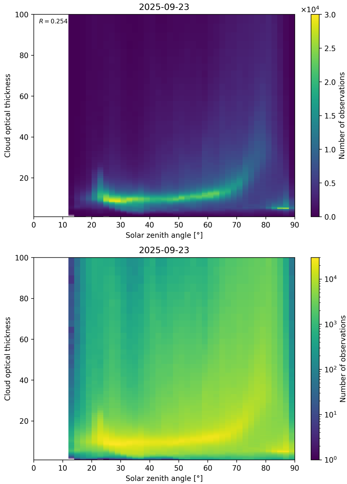
Figure 103: Scatter density plot of “Solar zenith angle” against “Cloud optical thickness” for 2025-09-22 to 2025-09-24.
