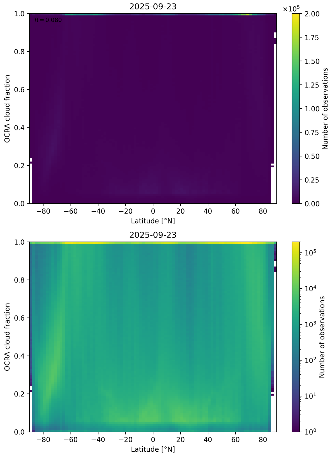
Figure 93: Scatter density plot of “Latitude” against “OCRA cloud fraction” for 2025-09-22 to 2025-09-24.
