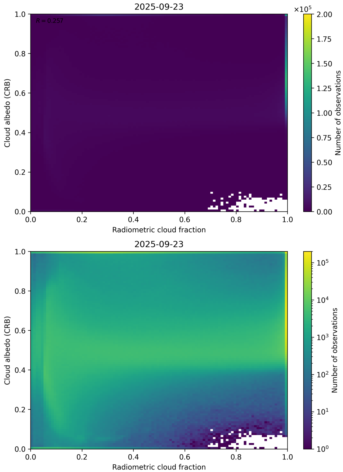
Figure 71: Scatter density plot of “Radiometric cloud fraction” against “Cloud albedo (CRB)” for 2025-09-22 to 2025-09-24.
