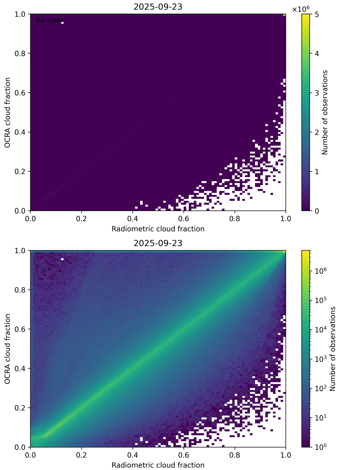
Figure 72: Scatter density plot of “Radiometric cloud fraction” against “OCRA cloud fraction” for 2025-09-22 to 2025-09-24.
