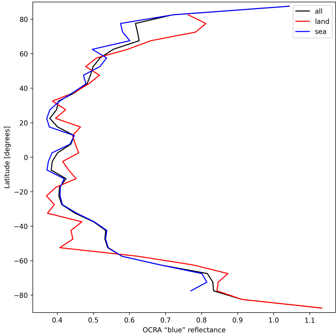
Figure 35: Zonal average of “OCRA “blue” reflectance” for 2025-09-22 to 2025-09-24.
