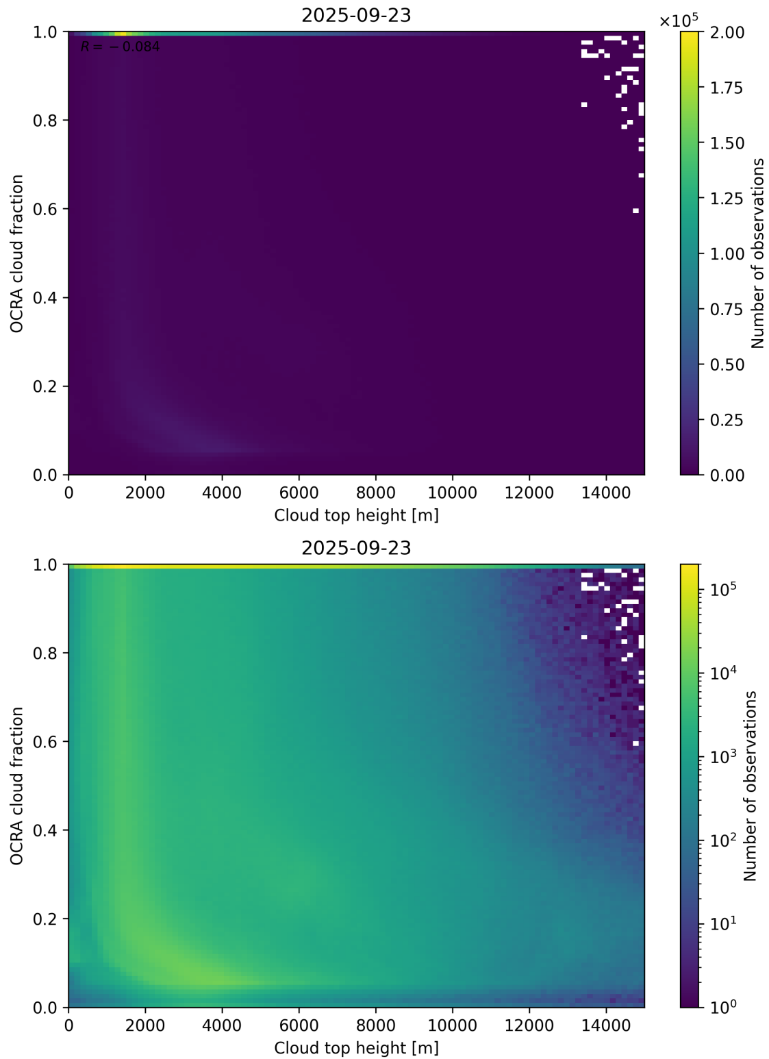
Figure 87: Scatter density plot of “Cloud top height” against “OCRA cloud fraction” for 2025-09-22 to 2025-09-24.
