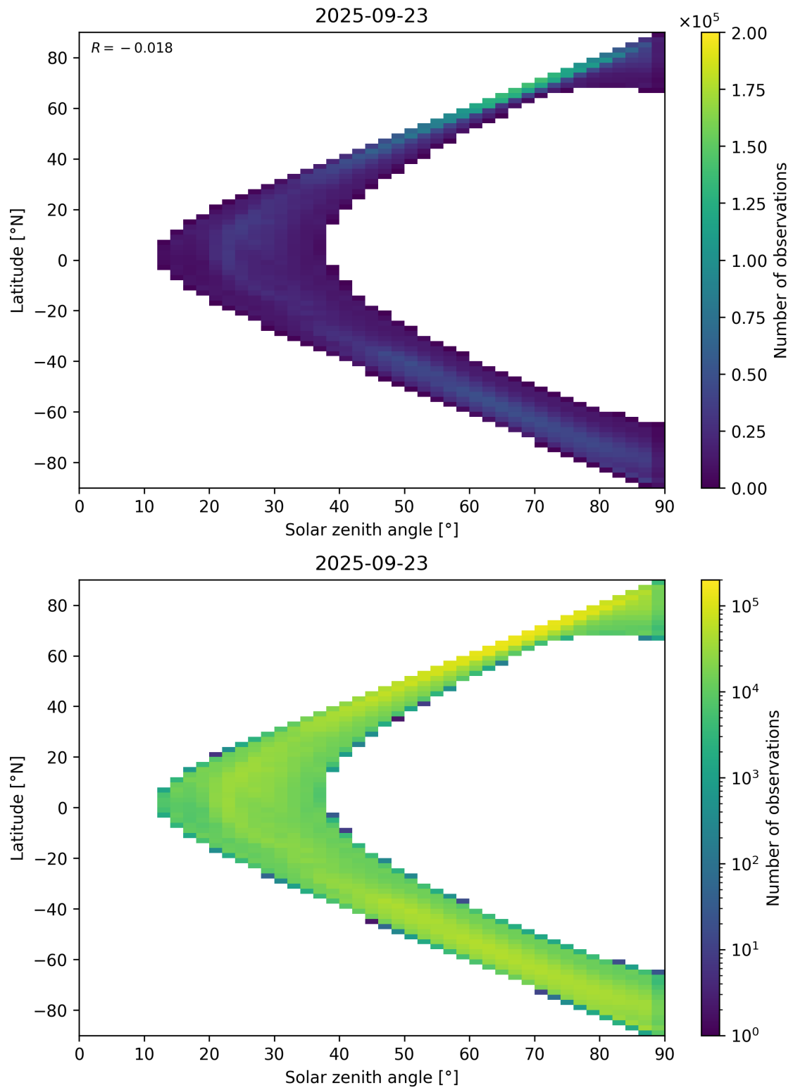
Figure 105: Scatter density plot of “Solar zenith angle” against “Latitude” for 2025-09-22 to 2025-09-24.
