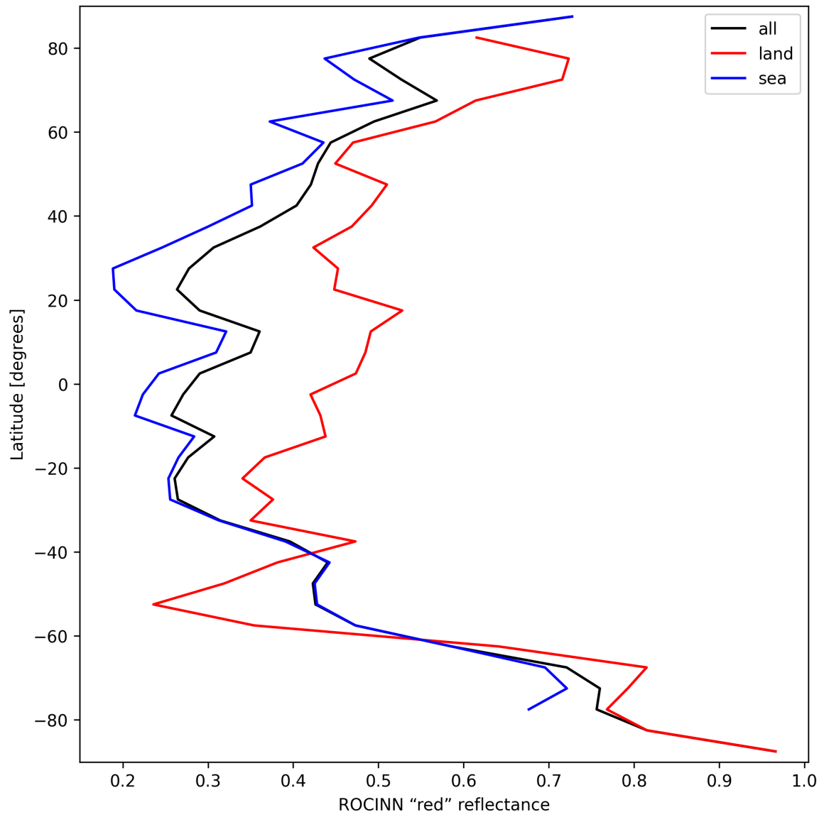
Figure 37: Zonal average of “ROCINN “red” reflectance” for 2025-09-22 to 2025-09-24.
