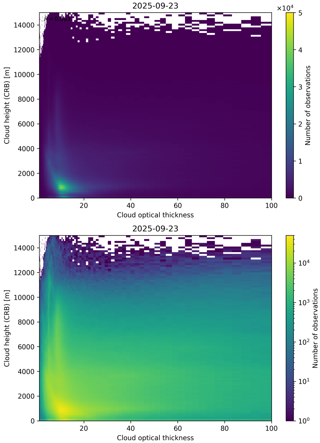
Figure 85: Scatter density plot of “Cloud optical thickness” against “Cloud height (CRB)” for 2025-09-22 to 2025-09-24.
