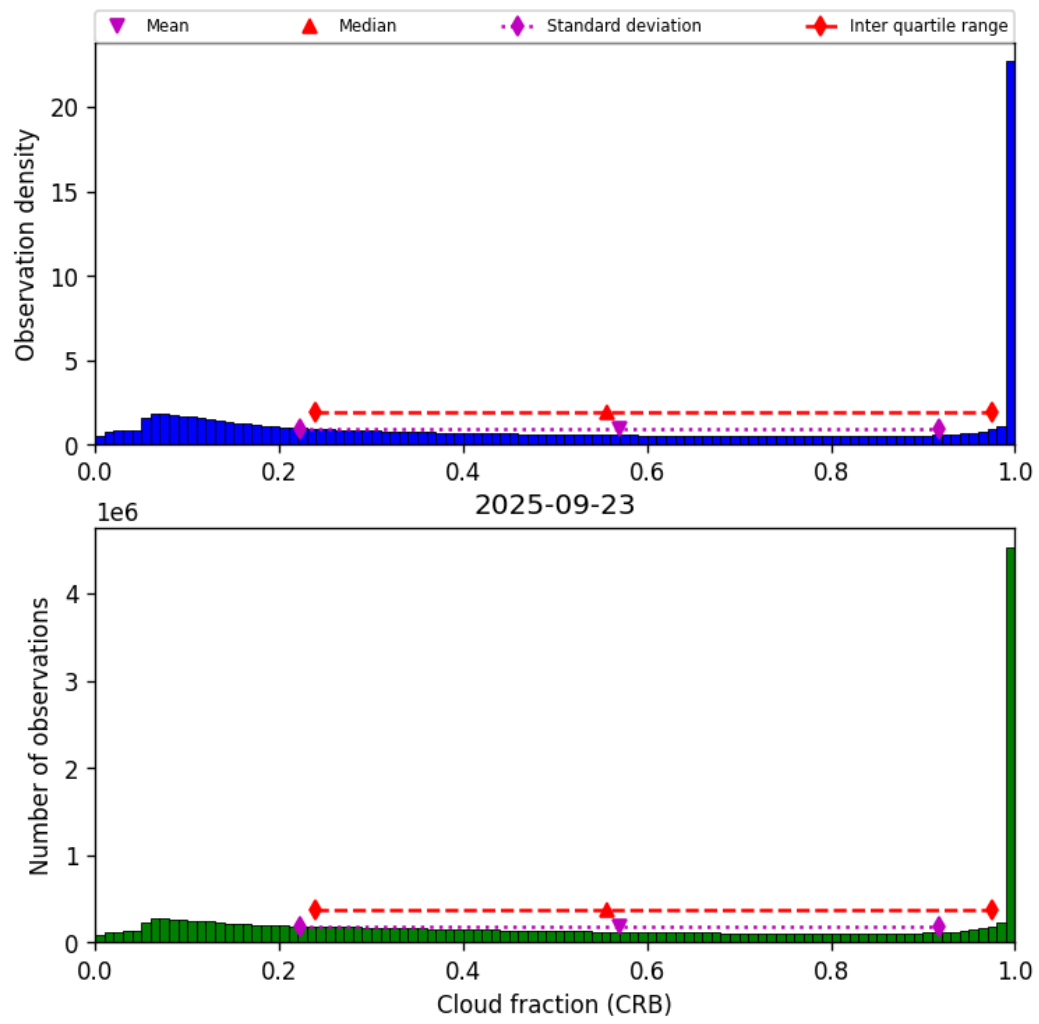
Figure 42: Histogram of “Cloud fraction (CRB)” for 2025-09-22 to 2025-09-24
