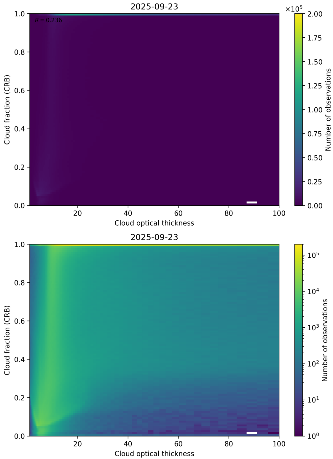
Figure 84: Scatter density plot of “Cloud optical thickness” against “Cloud fraction (CRB)” for 2025-09-22 to 2025-09-24.
