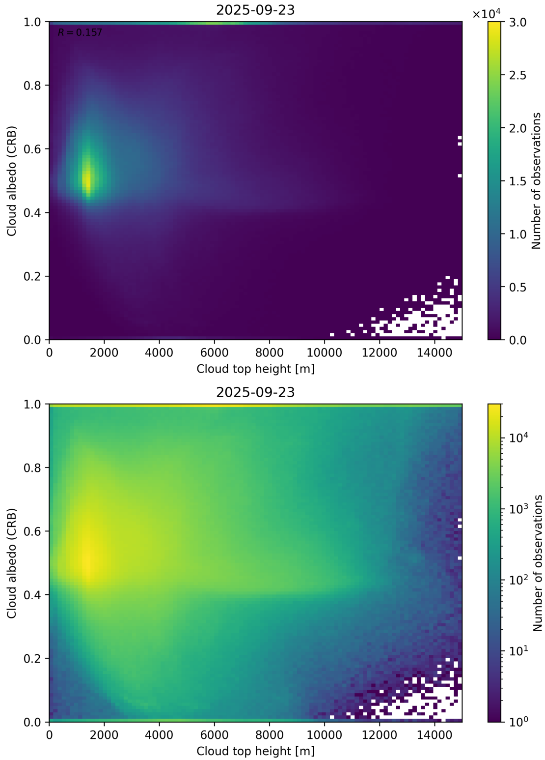
Figure 86: Scatter density plot of “Cloud top height” against “Cloud albedo (CRB)” for 2025-09-22 to 2025-09-24.
