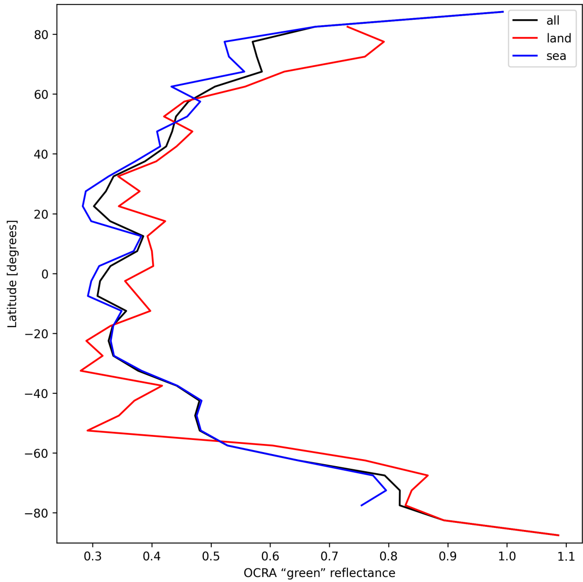
Figure 36: Zonal average of “OCRA “green” reflectance” for 2025-09-22 to 2025-09-24.
