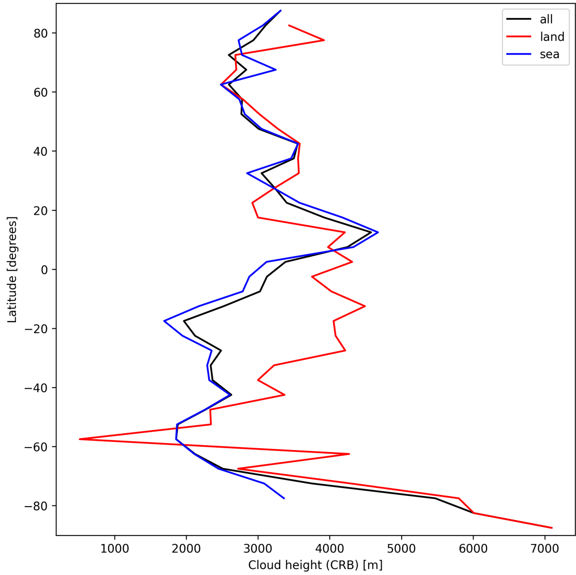
Figure 27: Zonal average of “Cloud height (CRB)” for 2025-09-22 to 2025-09-24.
