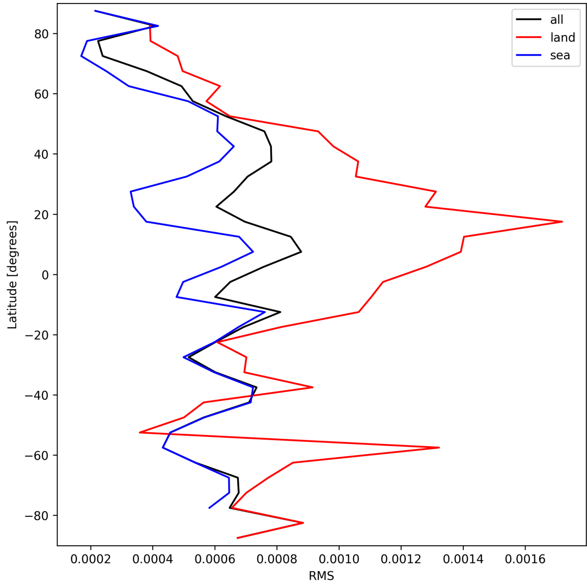
Figure 31: Zonal average of “RMS” for 2025-09-22 to 2025-09-24.
