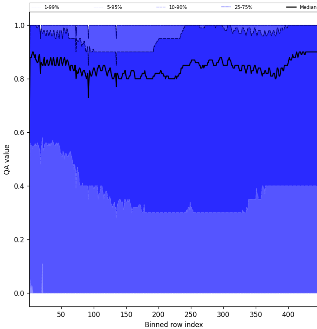
Figure 54: Along track statistics of “QA value” for 2025-09-23 to 2025-09-25
