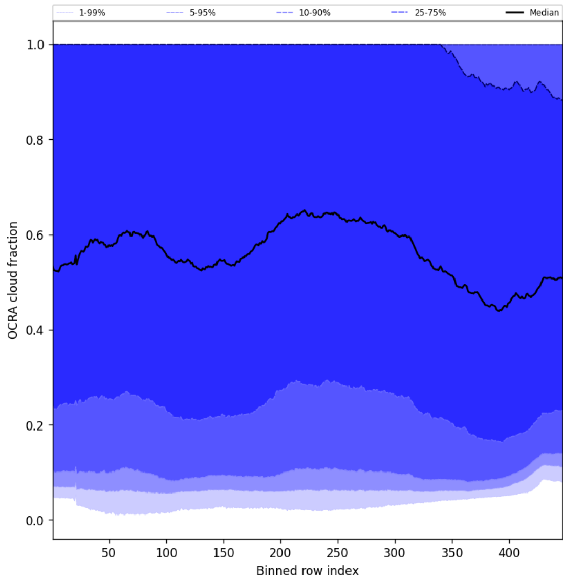
Figure 66: Along track statistics of “OCRA cloud fraction” for 2025-09-23 to 2025-09-25
