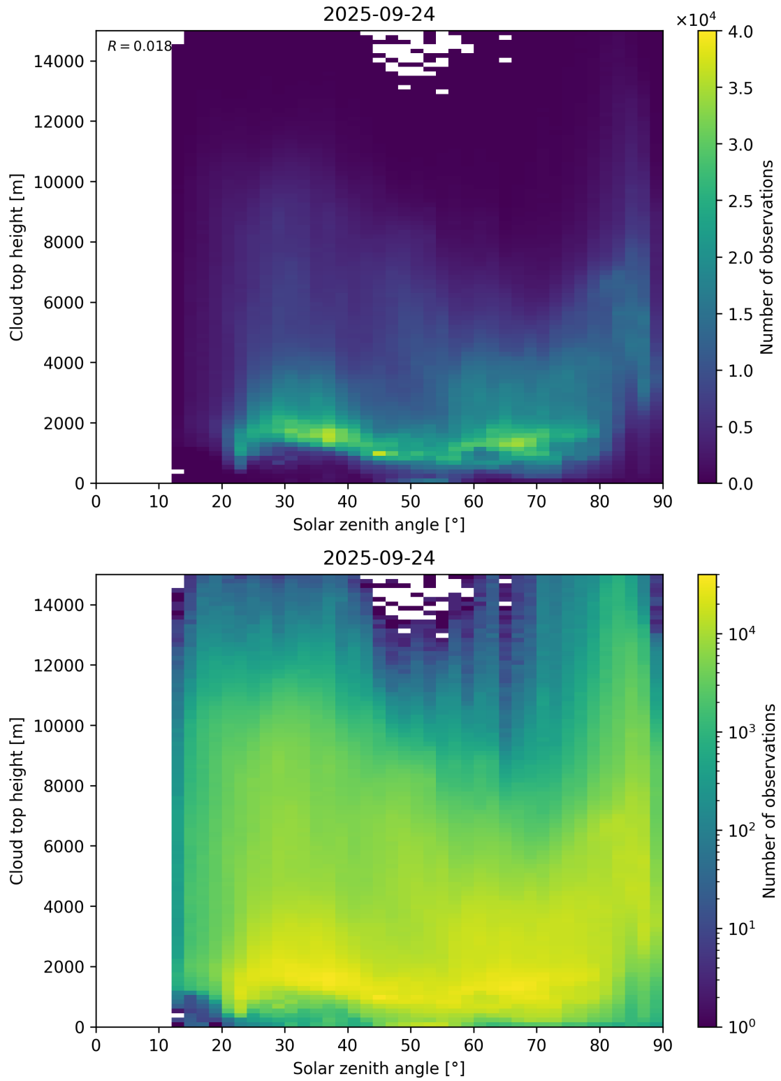
Figure 104: Scatter density plot of “Solar zenith angle” against “Cloud top height” for 2025-09-23 to 2025-09-25.
