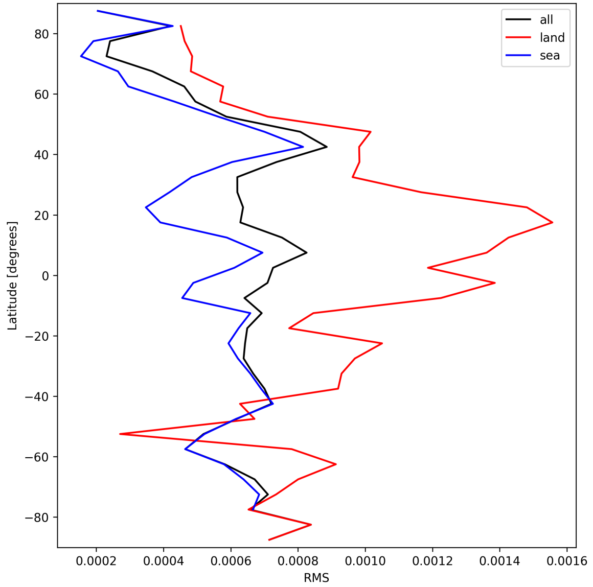
Figure 31: Zonal average of “RMS” for 2025-09-23 to 2025-09-25.
