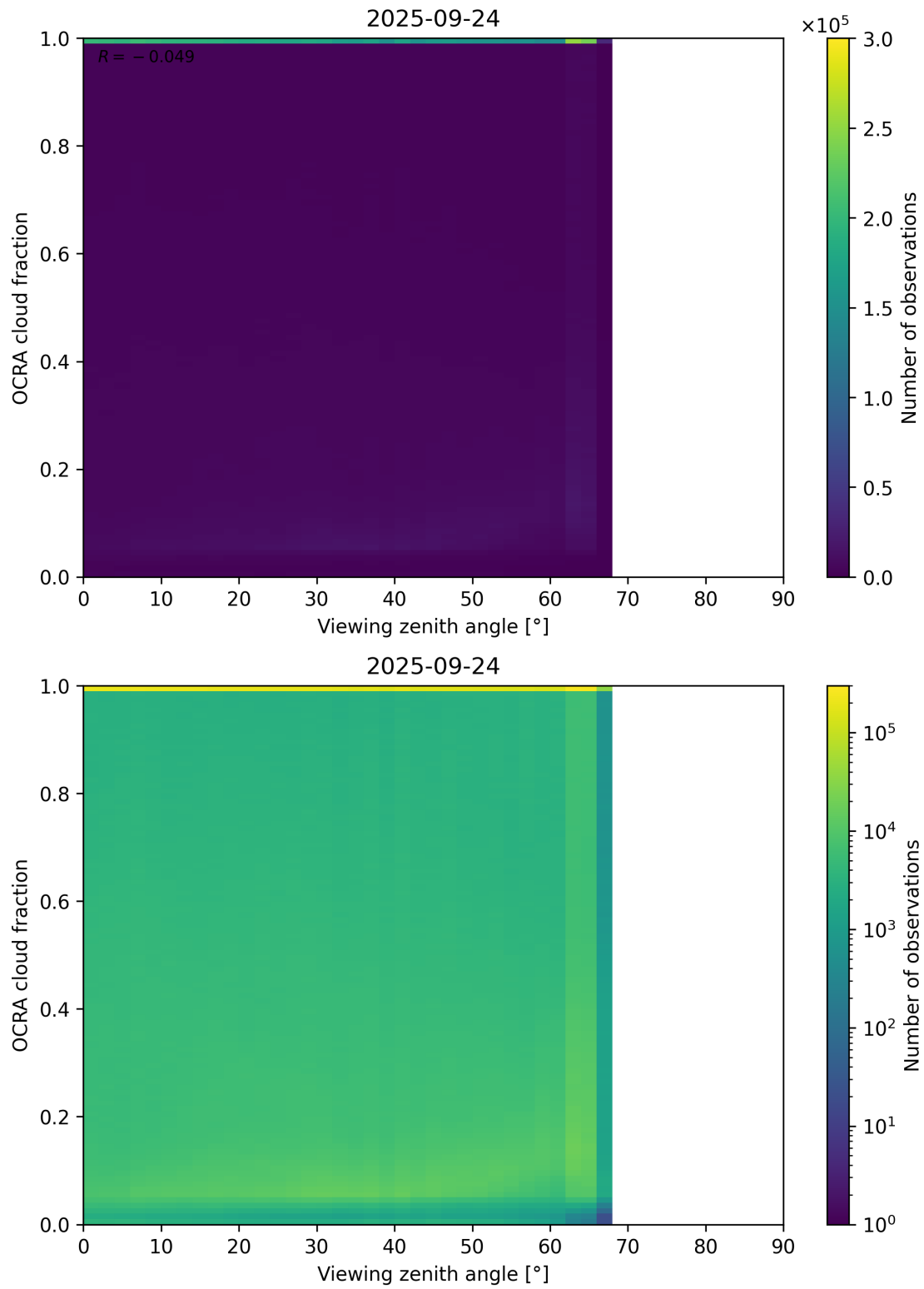
Figure 108: Scatter density plot of “Viewing zenith angle” against “OCRA cloud fraction” for 2025-09-23 to 2025-09-25.
