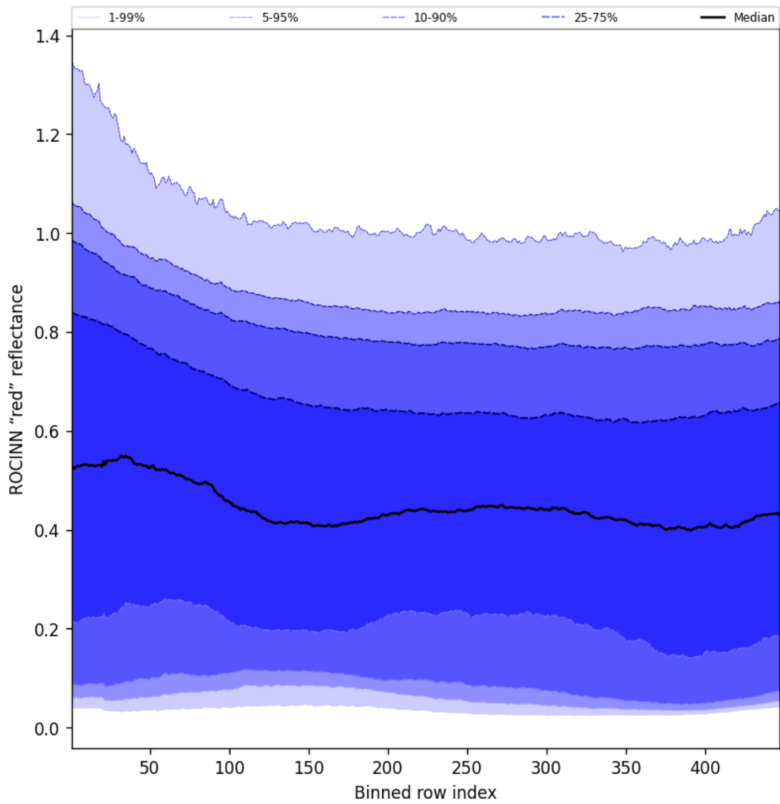
Figure 69: Along track statistics of "ROCINN "red" reflectance" for 2025-09-23 to 2025-09-25
