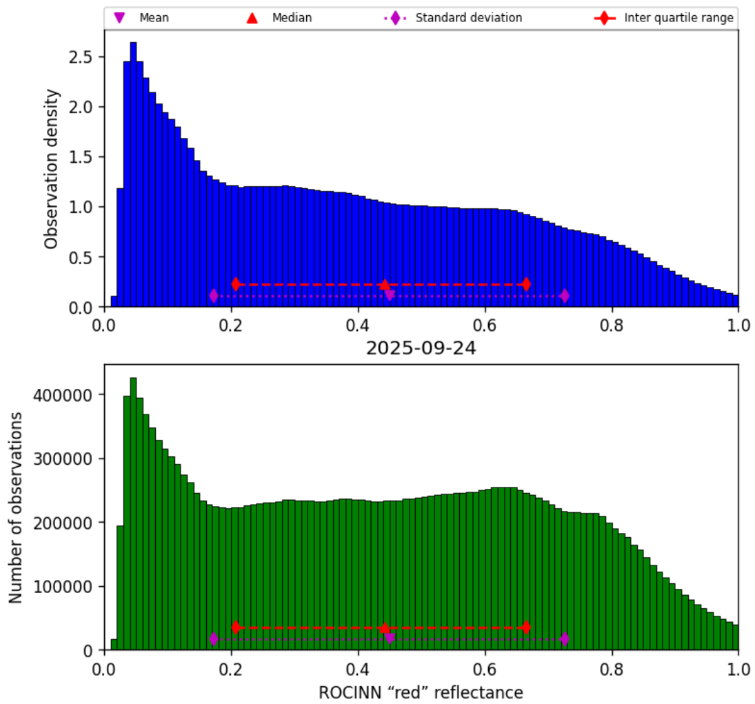
Figure 53: Histogram of “ROCINN “red” reflectance” for 2025-09-23 to 2025-09-25
