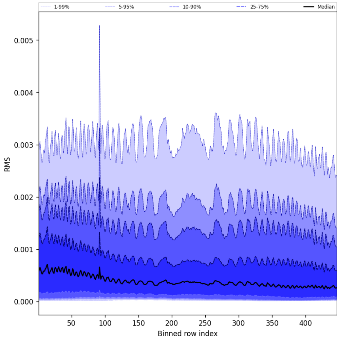
Figure 63: Along track statistics of “RMS” for 2025-09-23 to 2025-09-25
