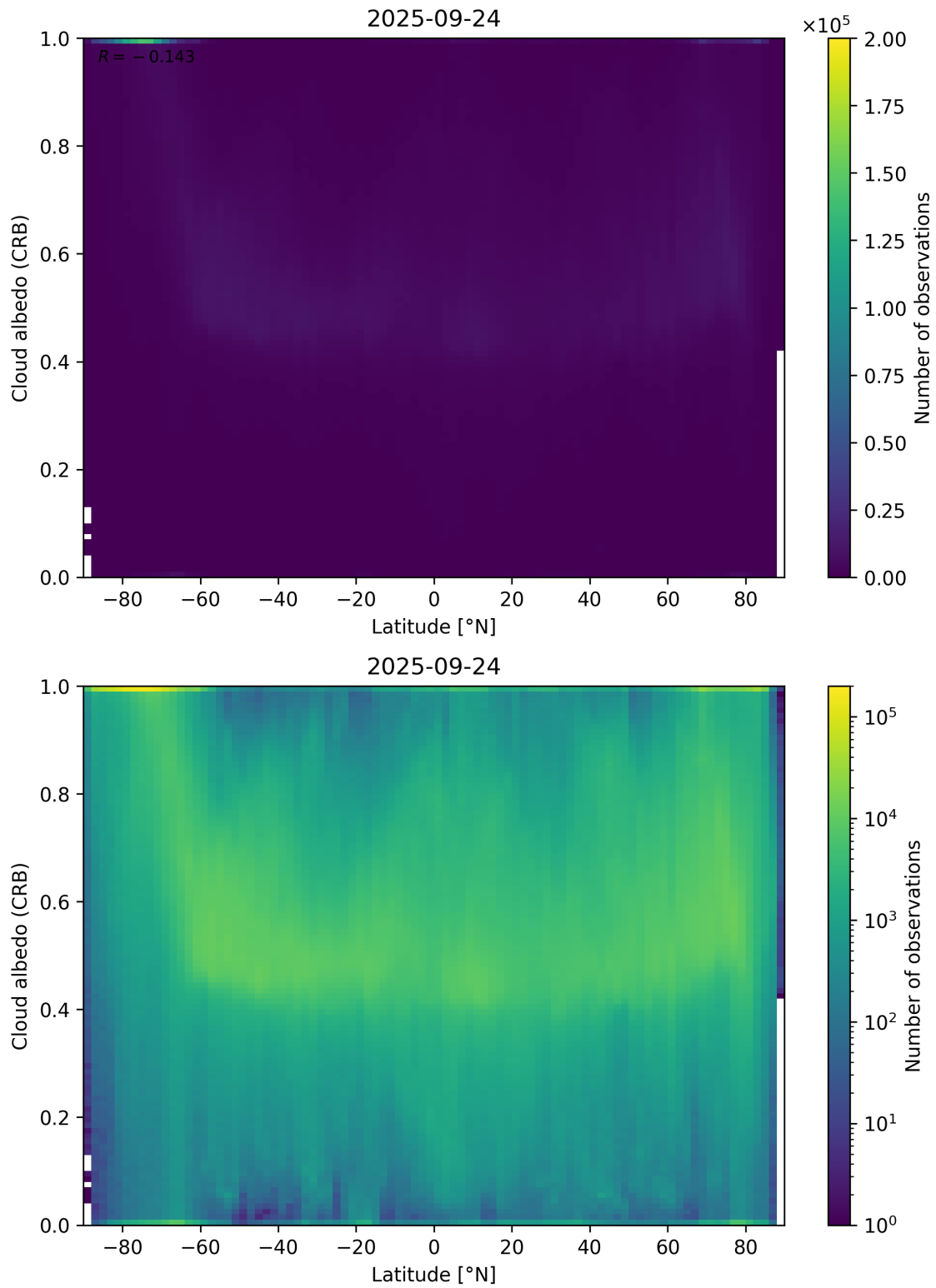
Figure 91: Scatter density plot of “Latitude” against “Cloud albedo (CRB)” for 2025-09-23 to 2025-09-25.
