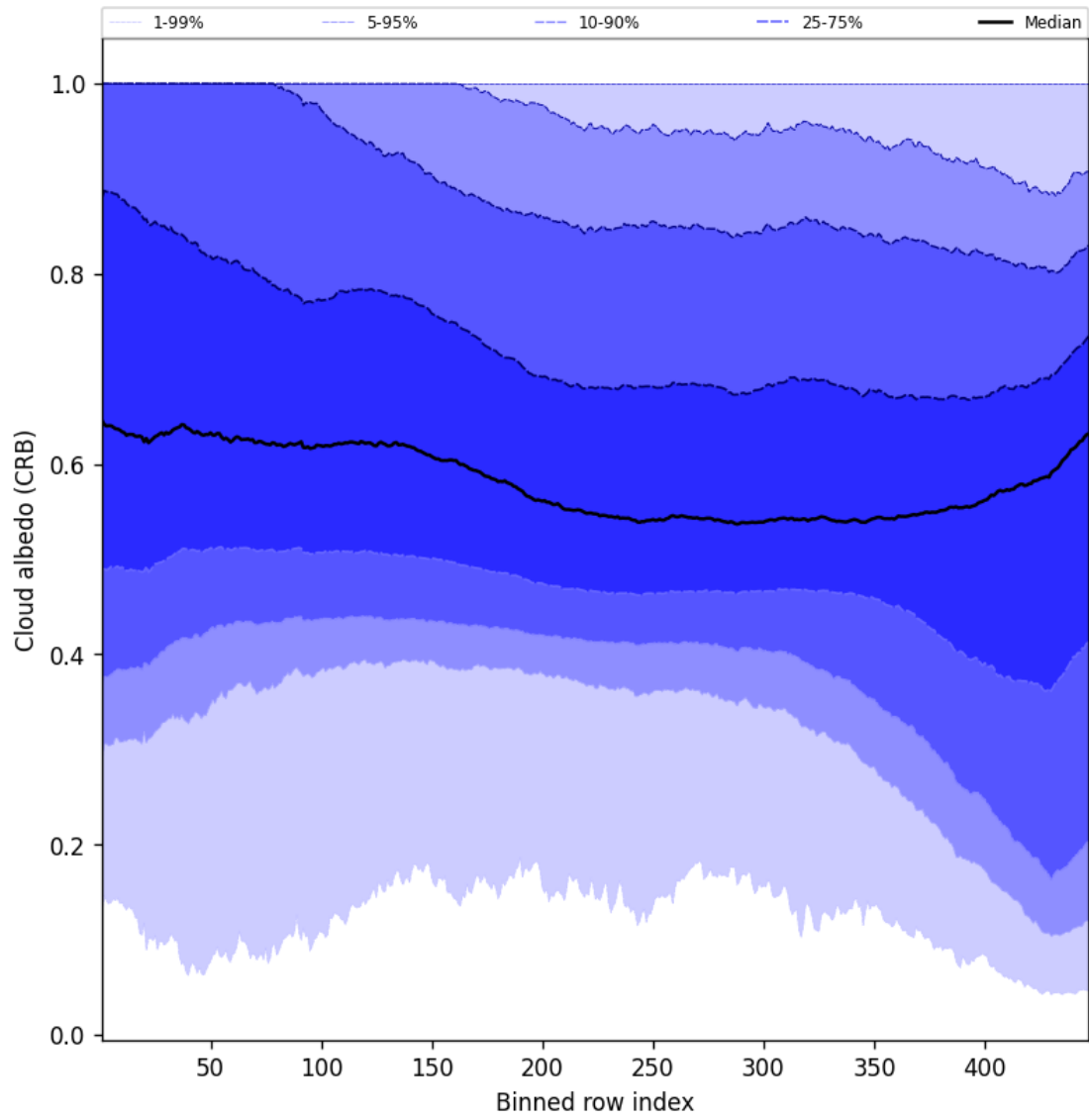
Figure 60: Along track statistics of “Cloud albedo (CRB)” for 2025-09-23 to 2025-09-25
