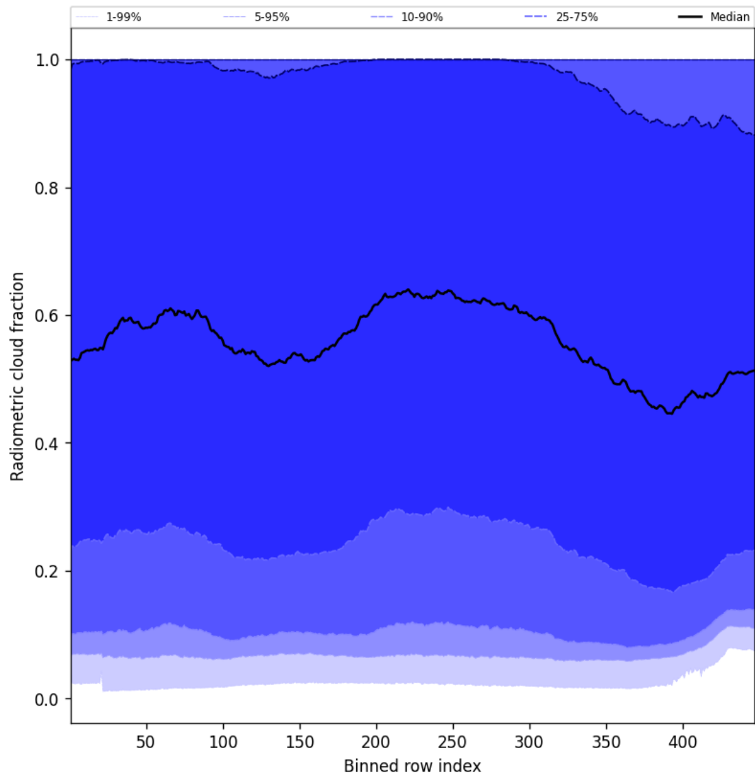
Figure 55: Along track statistics of “Radiometric cloud fraction” for 2025-09-23 to 2025-09-25
