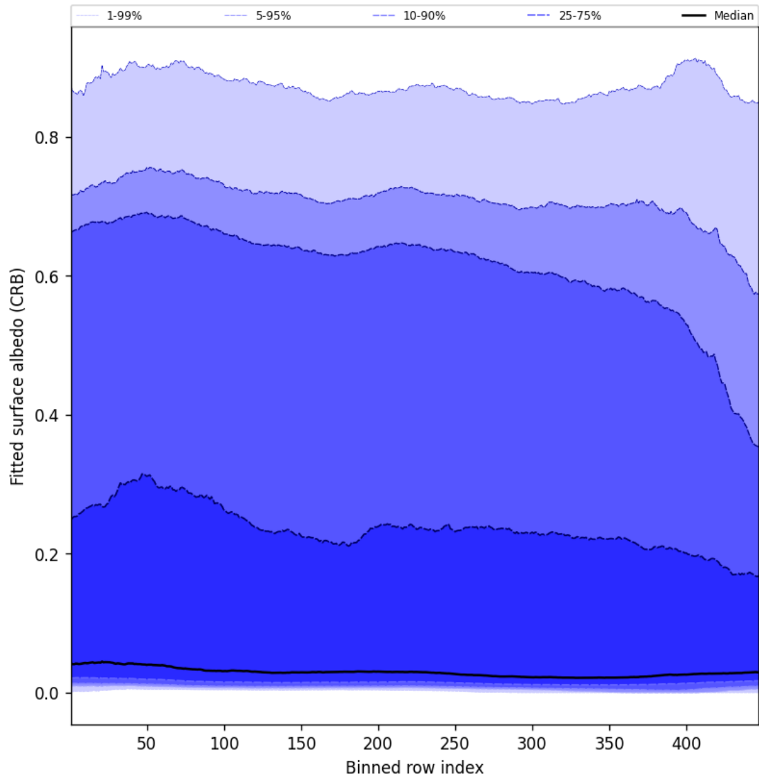
Figure 62: Along track statistics of “Fitted surface albedo (CRB)” for 2025-09-23 to 2025-09-25
