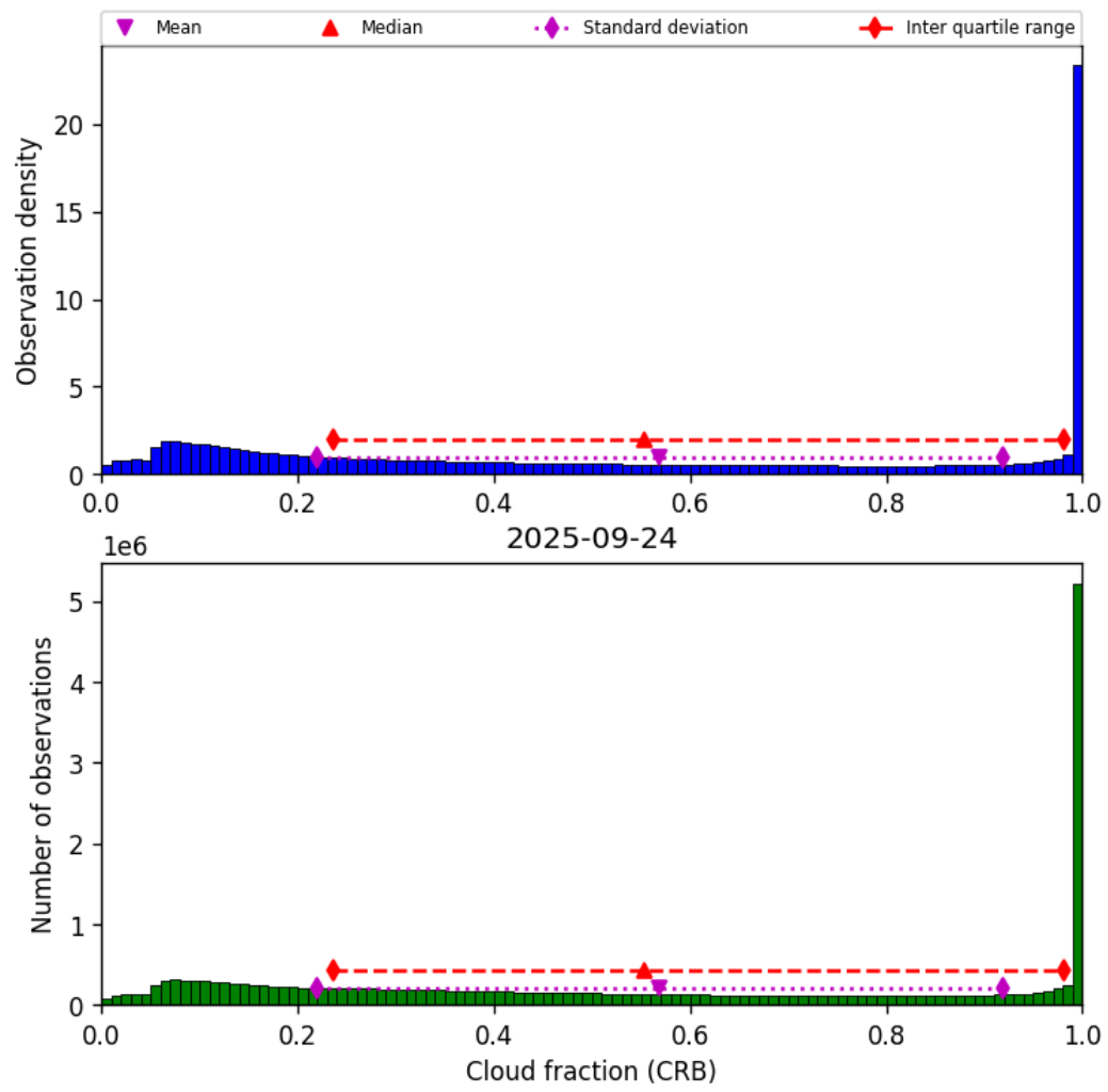
Figure 42: Histogram of “Cloud fraction (CRB)” for 2025-09-23 to 2025-09-25
