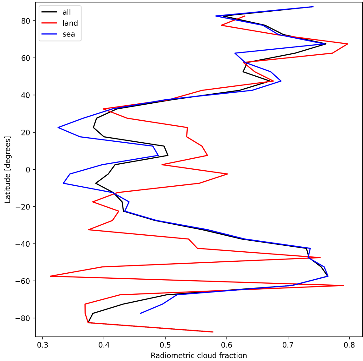
Figure 23: Zonal average of “Radiometric cloud fraction” for 2025-09-23 to 2025-09-25.
