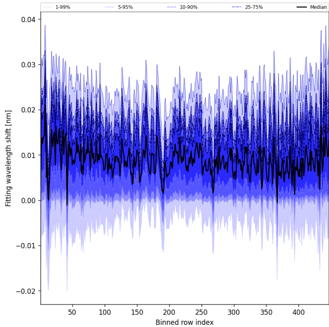
Figure 65: Along track statistics of “Fitting wavelength shift” for 2025-09-23 to 2025-09-25
