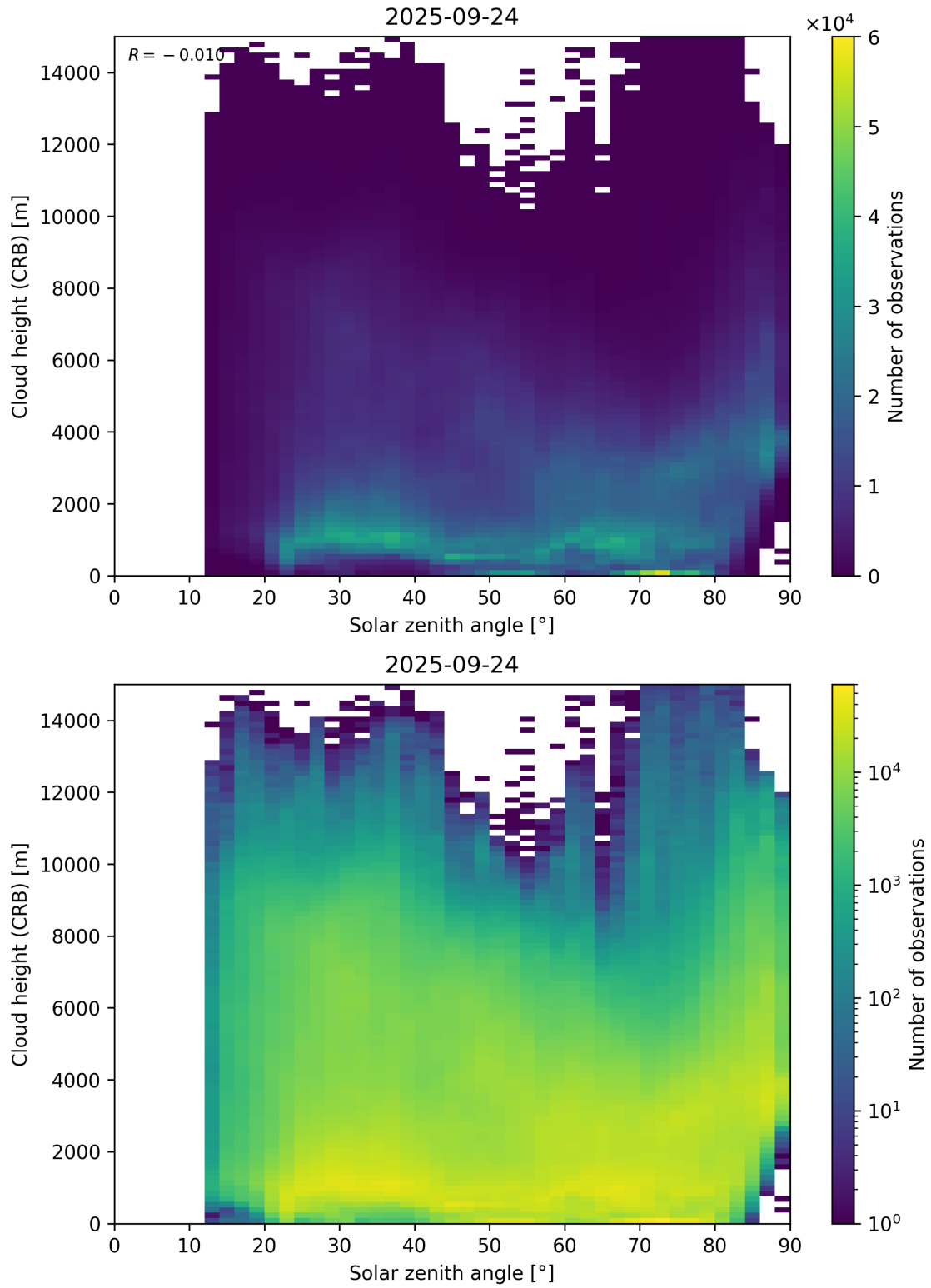
Figure 102: Scatter density plot of “Solar zenith angle” against “Cloud height (CRB)” for 2025-09-23 to 2025-09-25.
