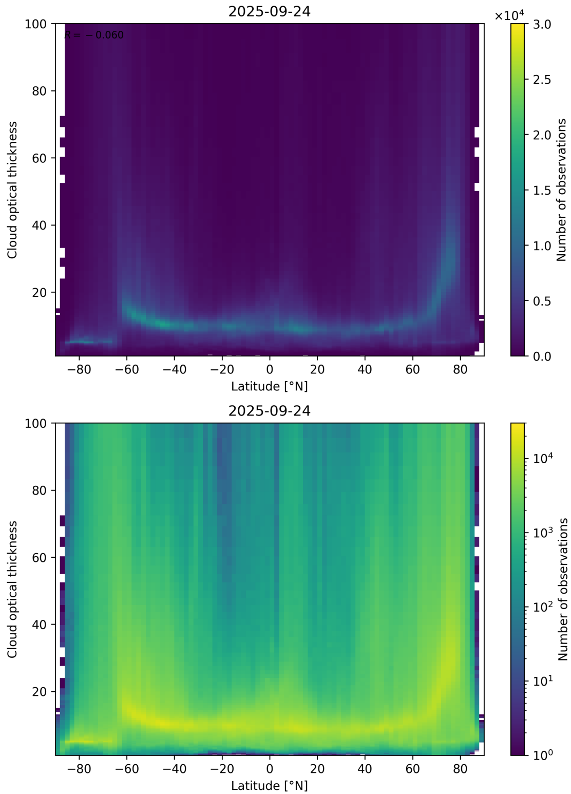
Figure 96: Scatter density plot of “Latitude” against “Cloud optical thickness” for 2025-09-23 to 2025-09-25.
