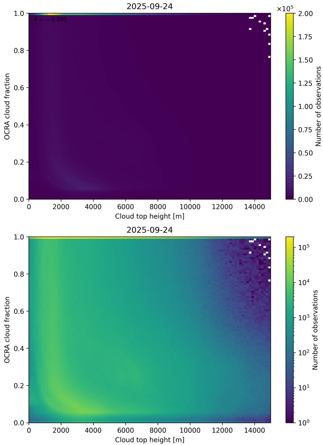
Figure 87: Scatter density plot of “Cloud top height” against “OCRA cloud fraction” for 2025-09-23 to 2025-09-25.
