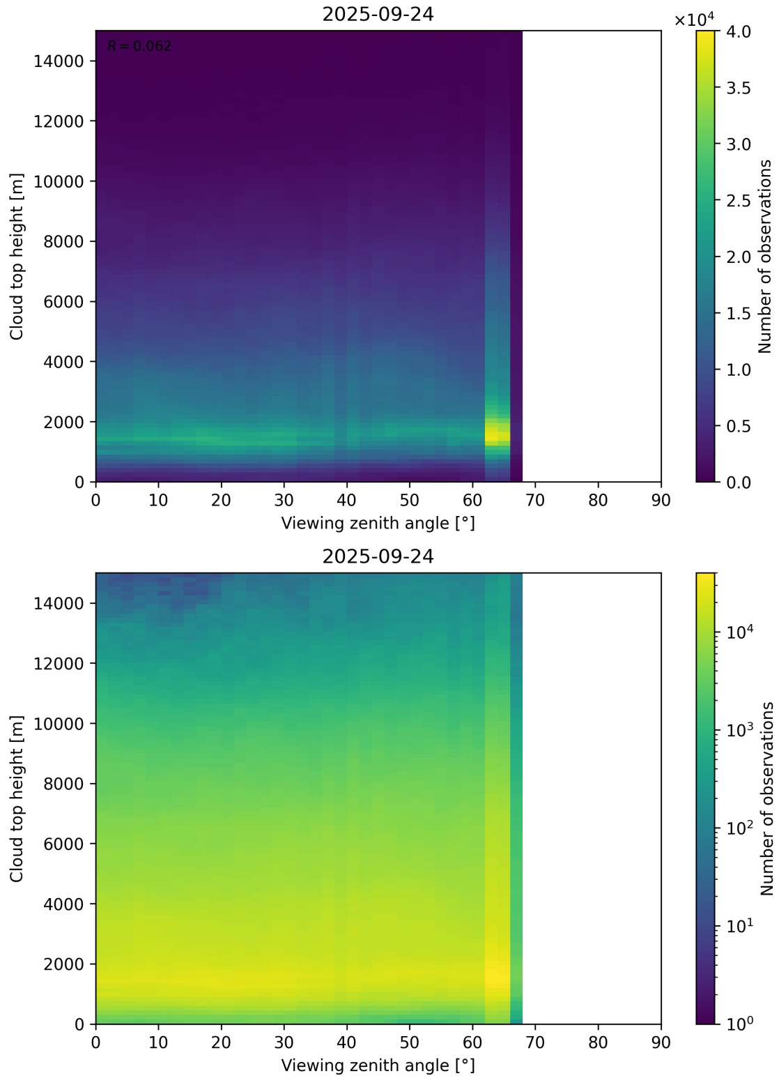
Figure 112: Scatter density plot of “Viewing zenith angle” against “Cloud top height” for 2025-09-23 to 2025-09-25.
