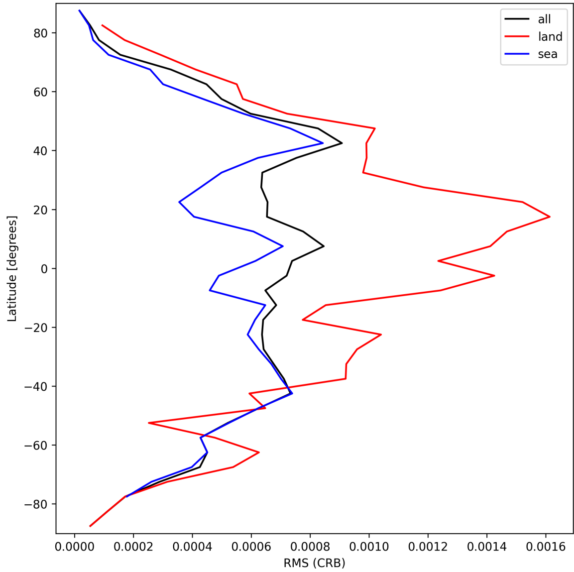
Figure 32: Zonal average of “RMS (CRB)” for 2025-09-23 to 2025-09-25.
