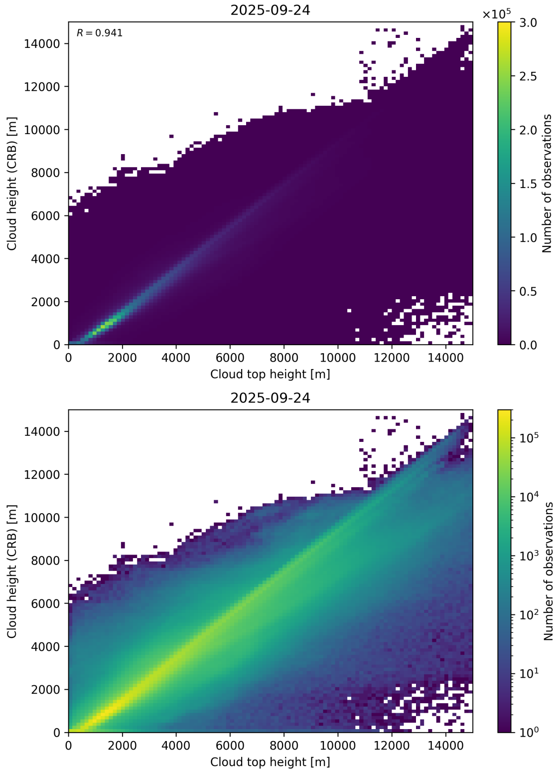
Figure 89: Scatter density plot of “Cloud top height” against “Cloud height (CRB)” for 2025-09-23 to 2025-09-25.
