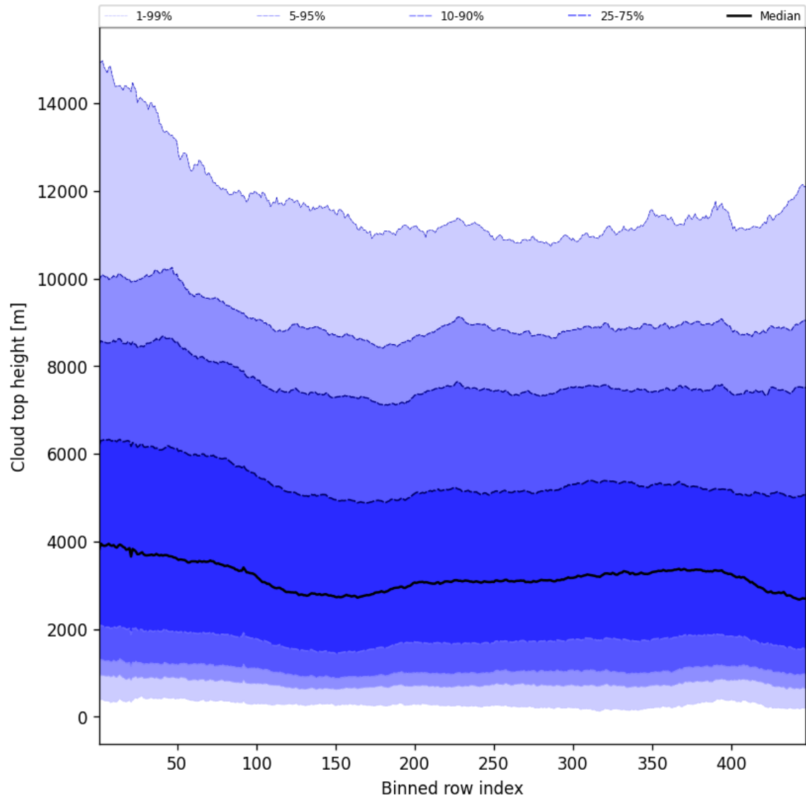
Figure 56: Along track statistics of “Cloud top height” for 2025-09-23 to 2025-09-25
