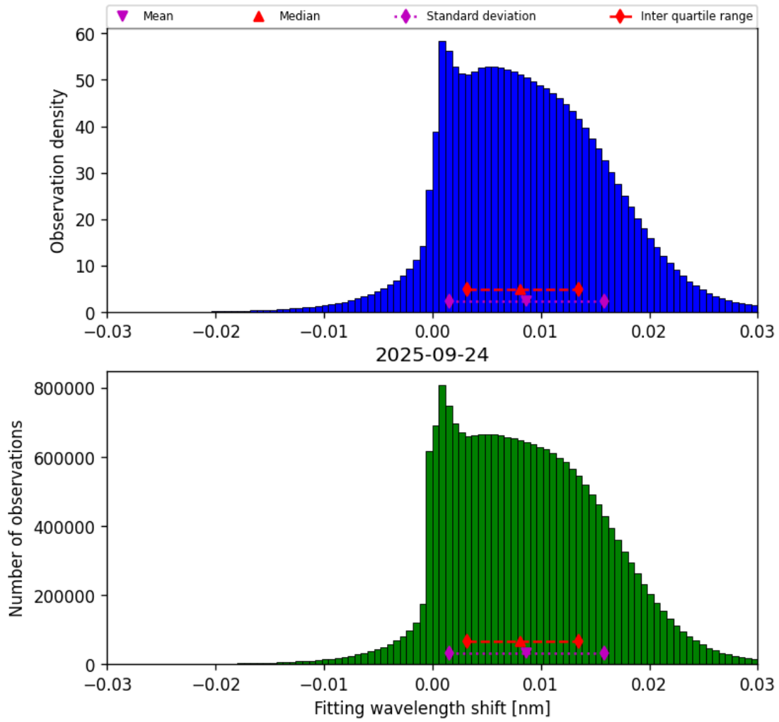
Figure 49: Histogram of “Fitting wavelength shift” for 2025-09-23 to 2025-09-25
