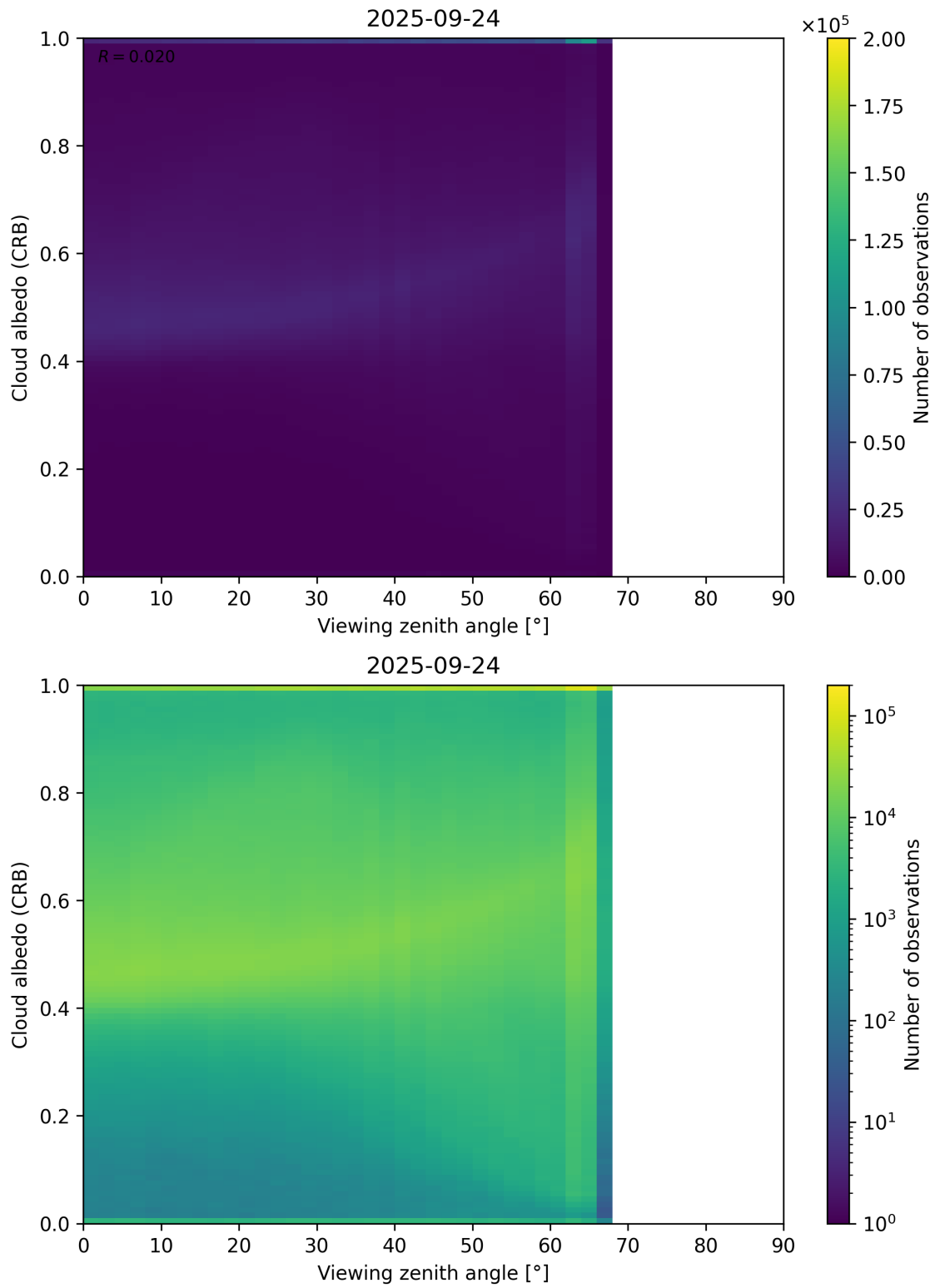
Figure 106: Scatter density plot of “Viewing zenith angle” against “Cloud albedo (CRB)” for 2025-09-23 to 2025-09-25.
