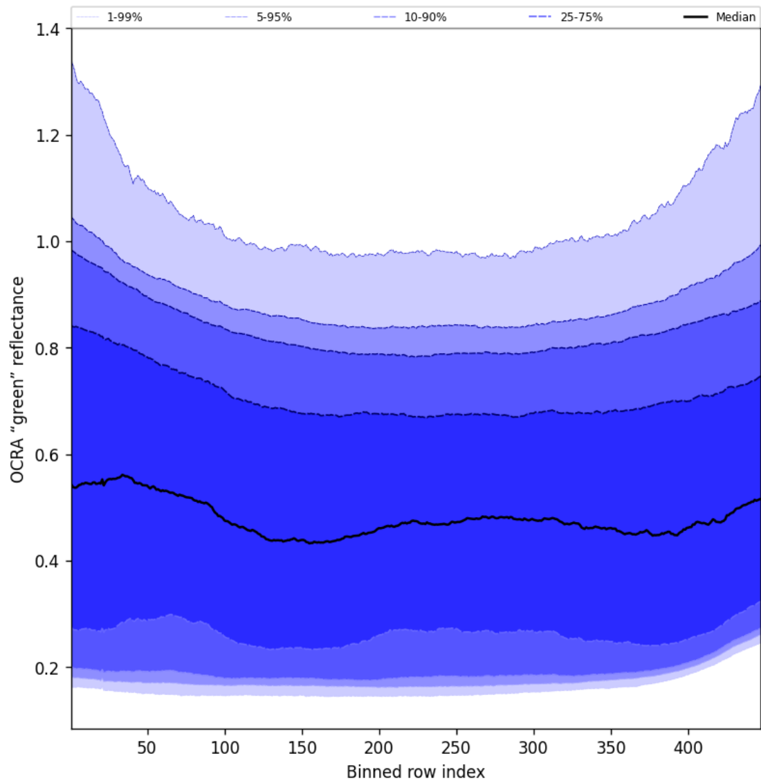
Figure 68: Along track statistics of “OCRA “green” reflectance” for 2025-09-23 to 2025-09-25
