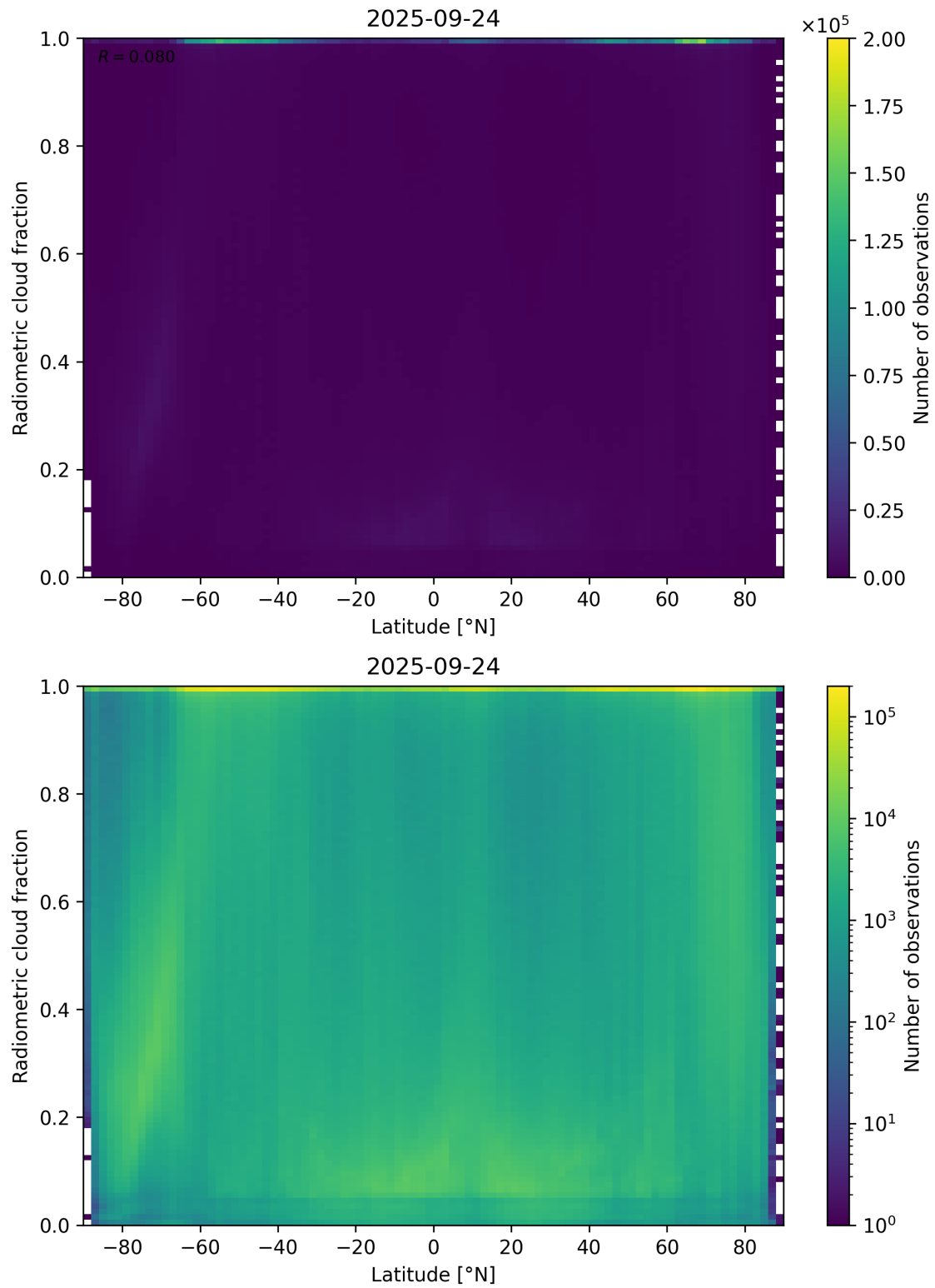
Figure 92: Scatter density plot of “Latitude” against “Radiometric cloud fraction” for 2025-09-23 to 2025-09-25.
