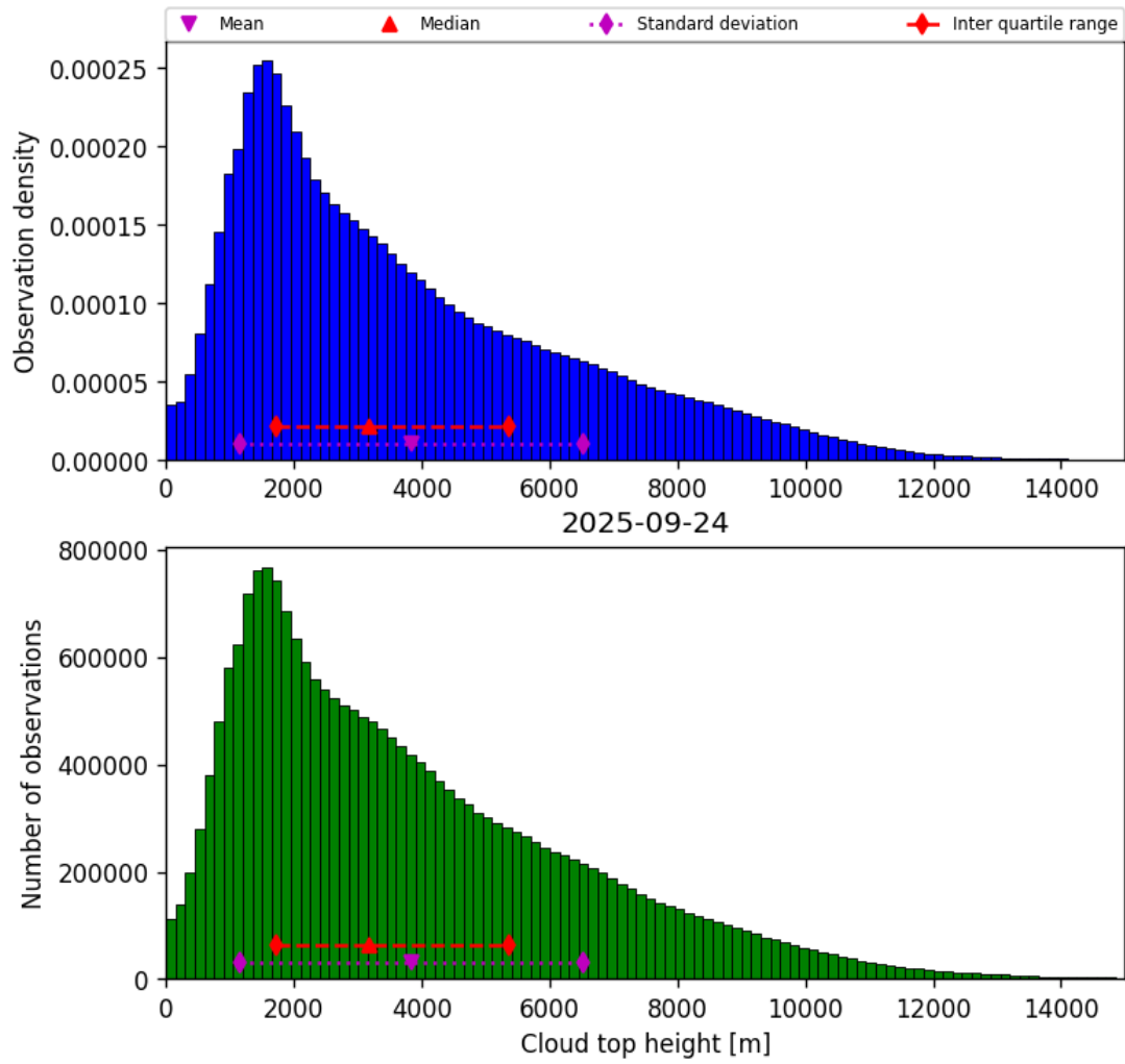
Figure 40: Histogram of “Cloud top height” for 2025-09-23 to 2025-09-25
