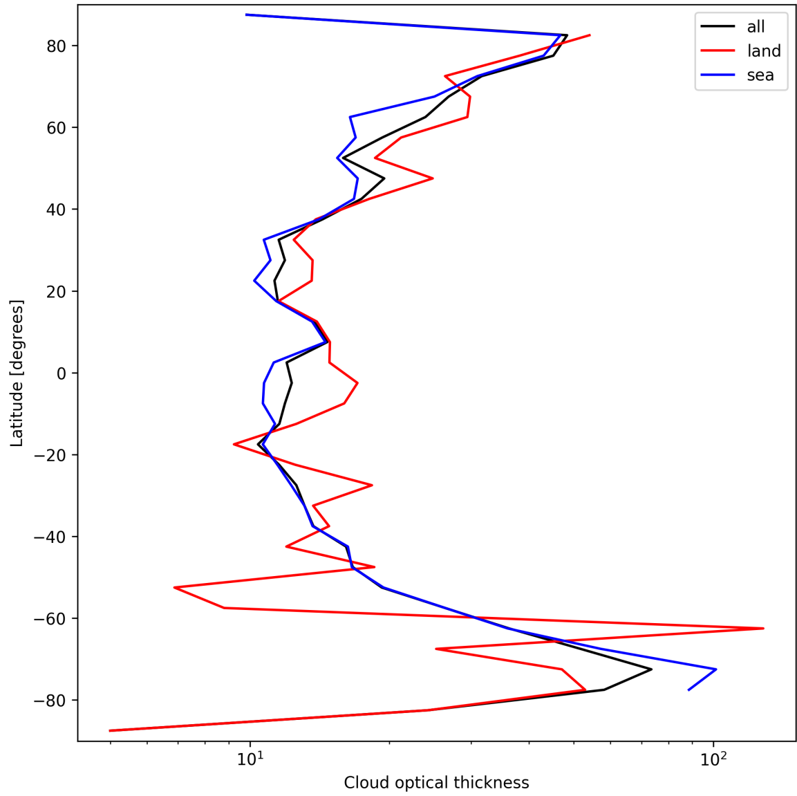
Figure 25: Zonal average of “Cloud optical thickness” for 2025-09-23 to 2025-09-25.
