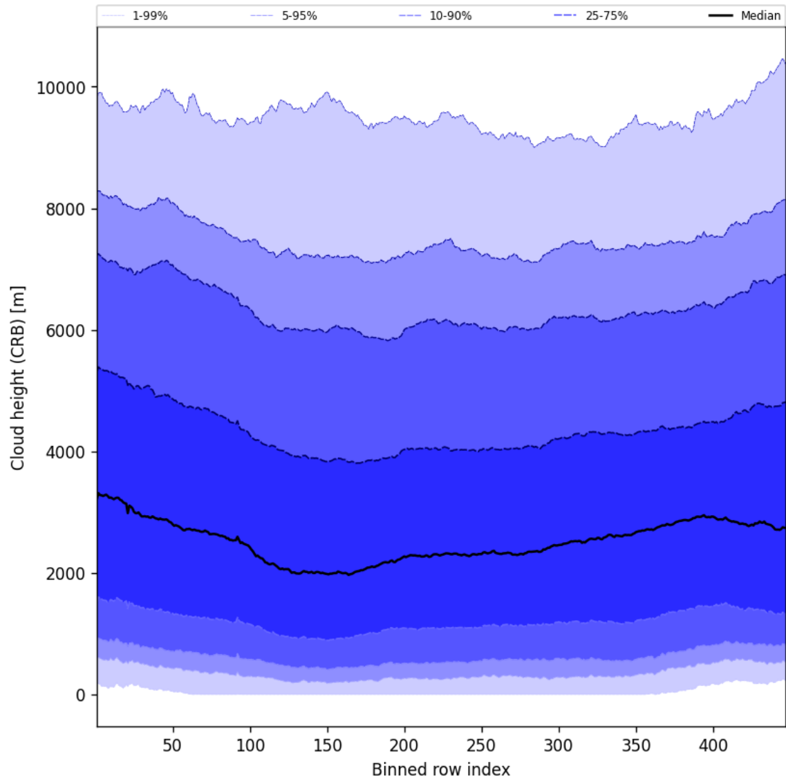
Figure 59: Along track statistics of “Cloud height (CRB)” for 2025-09-23 to 2025-09-25
