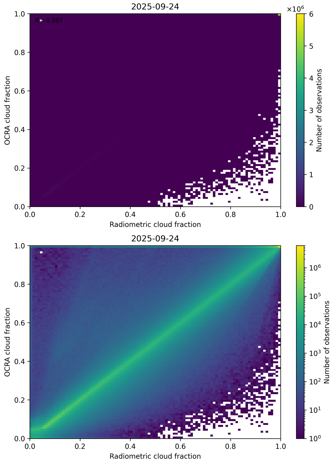
Figure 72: Scatter density plot of “Radiometric cloud fraction” against “OCRA cloud fraction” for 2025-09-23 to 2025-09-25.
