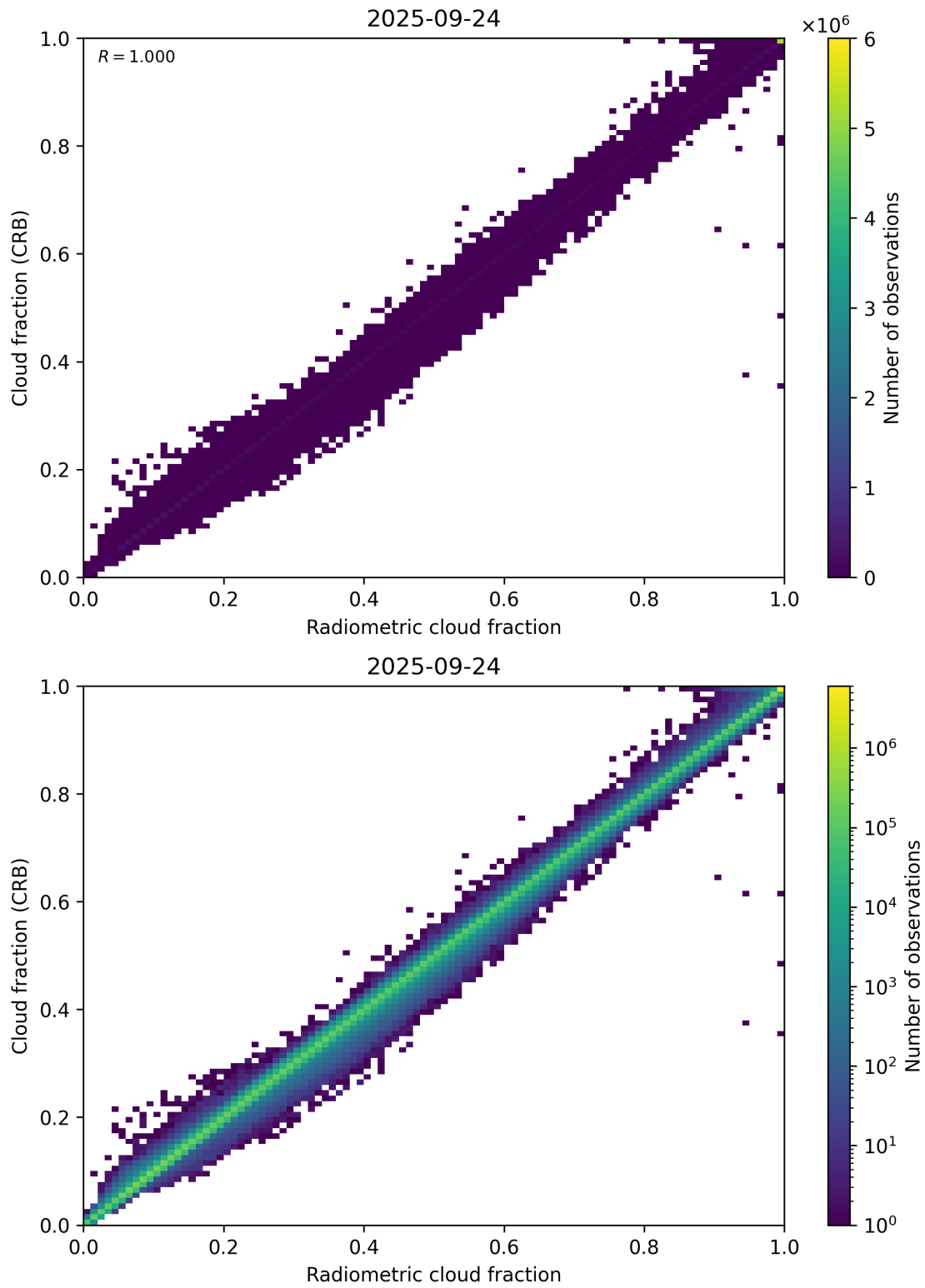
Figure 73: Scatter density plot of “Radiometric cloud fraction” against “Cloud fraction (CRB)” for 2025-09-23 to 2025-09-25.
