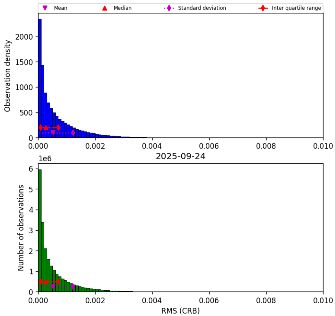
Figure 48: Histogram of “RMS (CRB)” for 2025-09-23 to 2025-09-25
