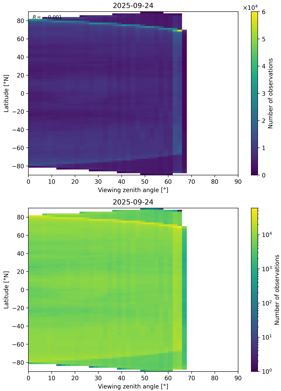
Figure 113: Scatter density plot of “Viewing zenith angle” against “Latitude” for 2025-09-23 to 2025-09-25.
