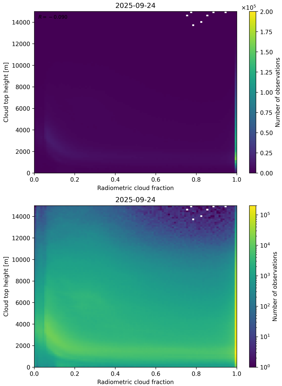
Figure 76: Scatter density plot of “Radiometric cloud fraction” against “Cloud top height” for 2025-09-23 to 2025-09-25.
