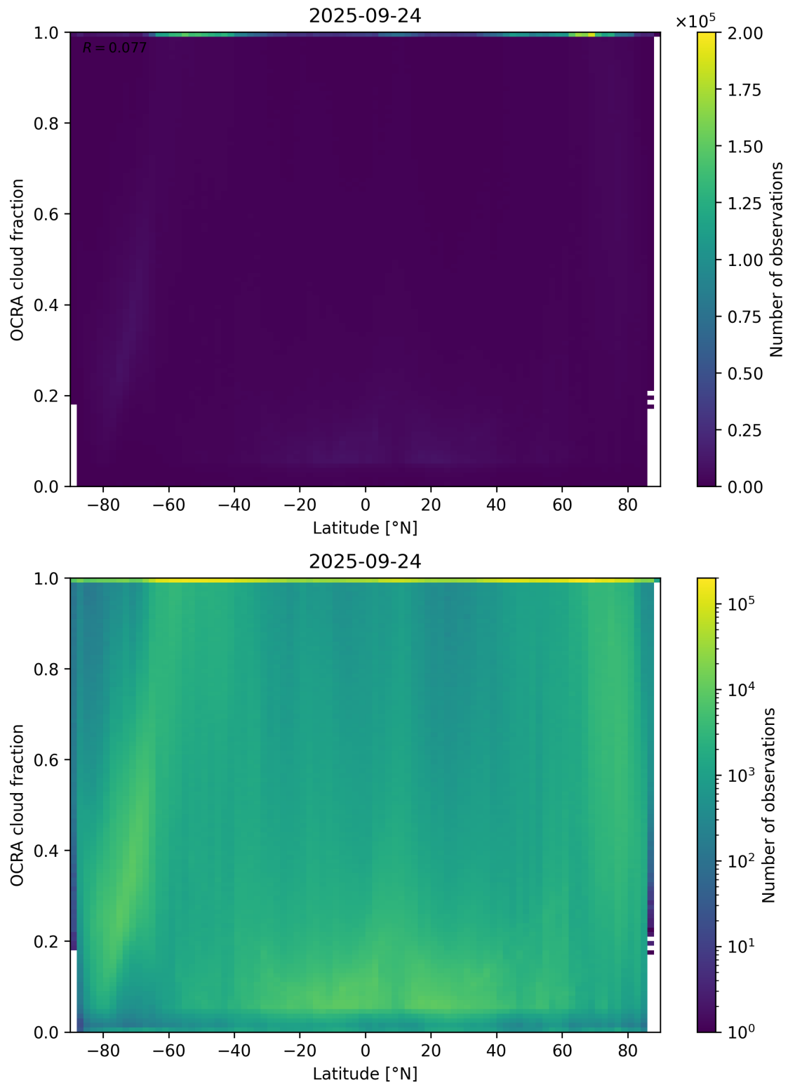
Figure 93: Scatter density plot of “Latitude” against “OCRA cloud fraction” for 2025-09-23 to 2025-09-25.
