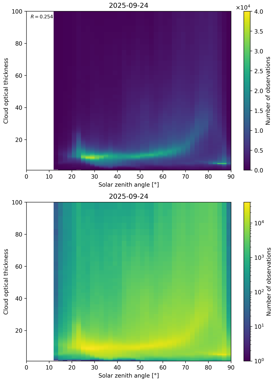
Figure 103: Scatter density plot of “Solar zenith angle” against “Cloud optical thickness” for 2025-09-23 to 2025-09-25.
