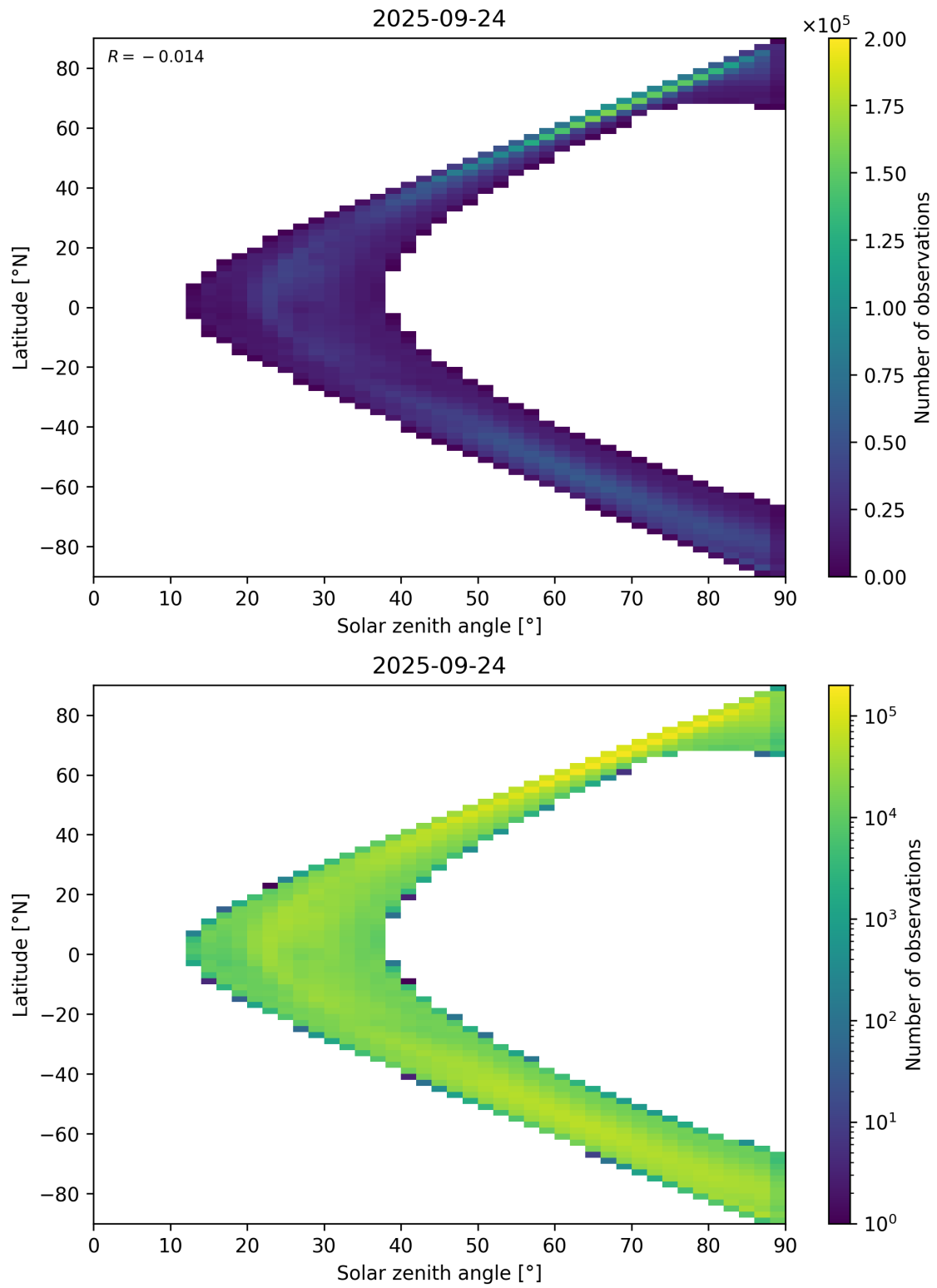
Figure 105: Scatter density plot of “Solar zenith angle” against “Latitude” for 2025-09-23 to 2025-09-25.
