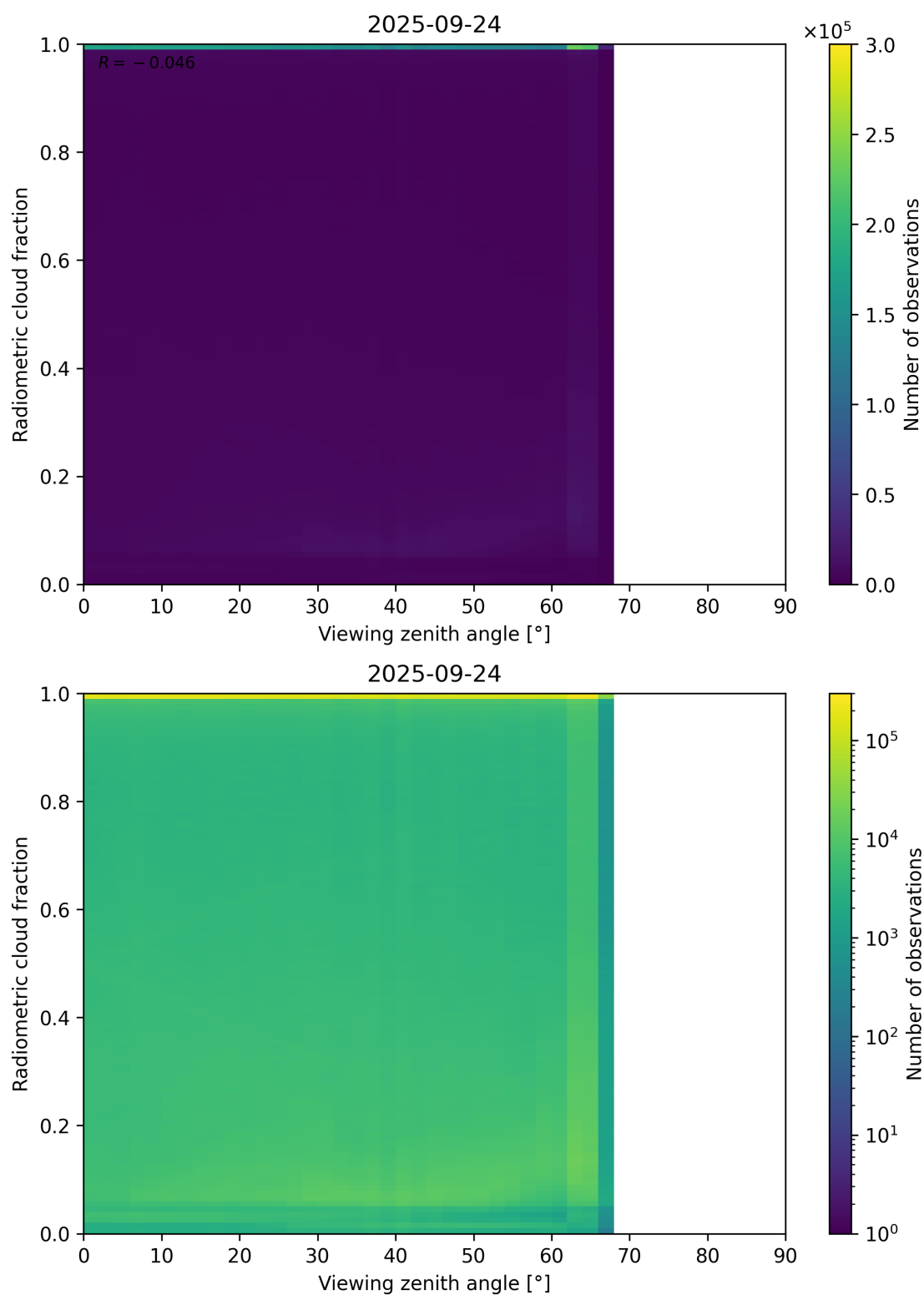
Figure 107: Scatter density plot of “Viewing zenith angle” against “Radiometric cloud fraction” for 2025-09-23 to 2025-09-25.
