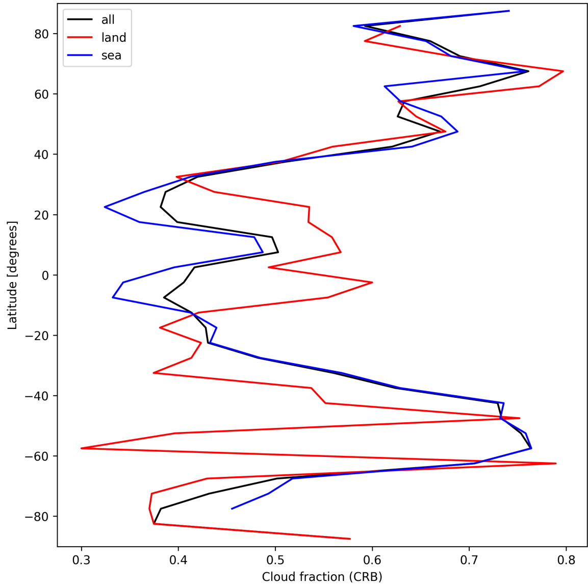
Figure 26: Zonal average of “Cloud fraction (CRB)” for 2025-09-23 to 2025-09-25.
