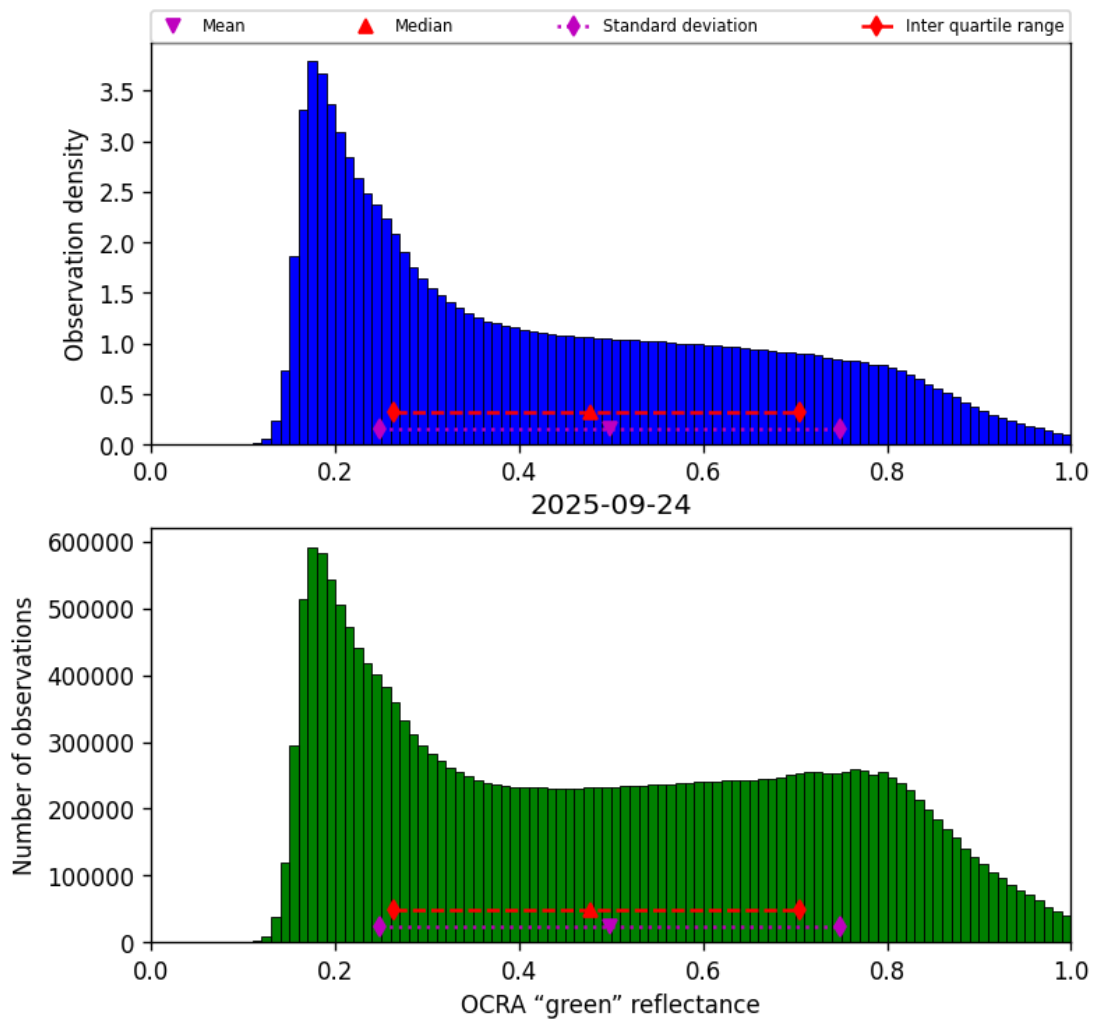
Figure 52: Histogram of “OCRA “green” reflectance” for 2025-09-23 to 2025-09-25
