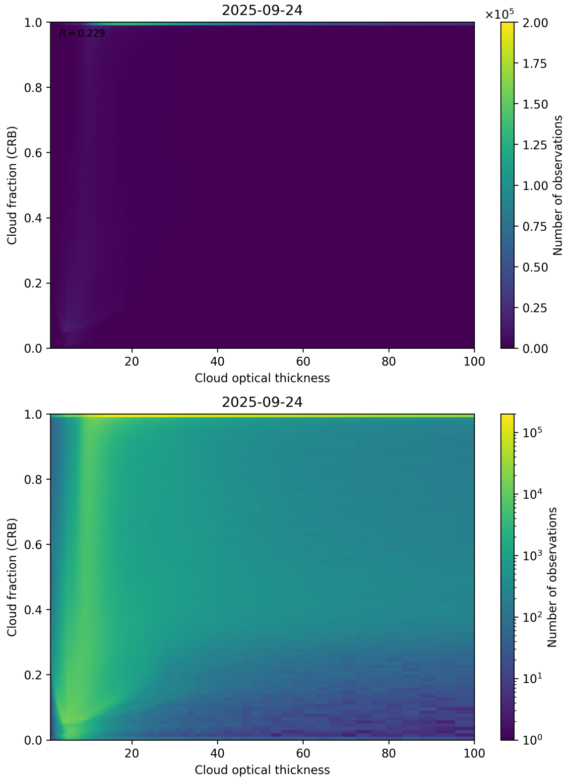
Figure 84: Scatter density plot of “Cloud optical thickness” against “Cloud fraction (CRB)” for 2025-09-23 to 2025-09-25.
