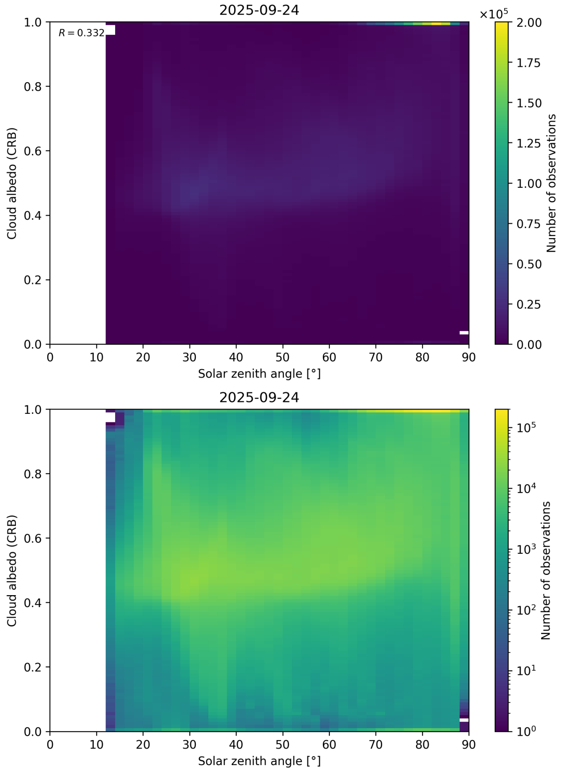
Figure 98: Scatter density plot of “Solar zenith angle” against “Cloud albedo (CRB)” for 2025-09-23 to 2025-09-25.
