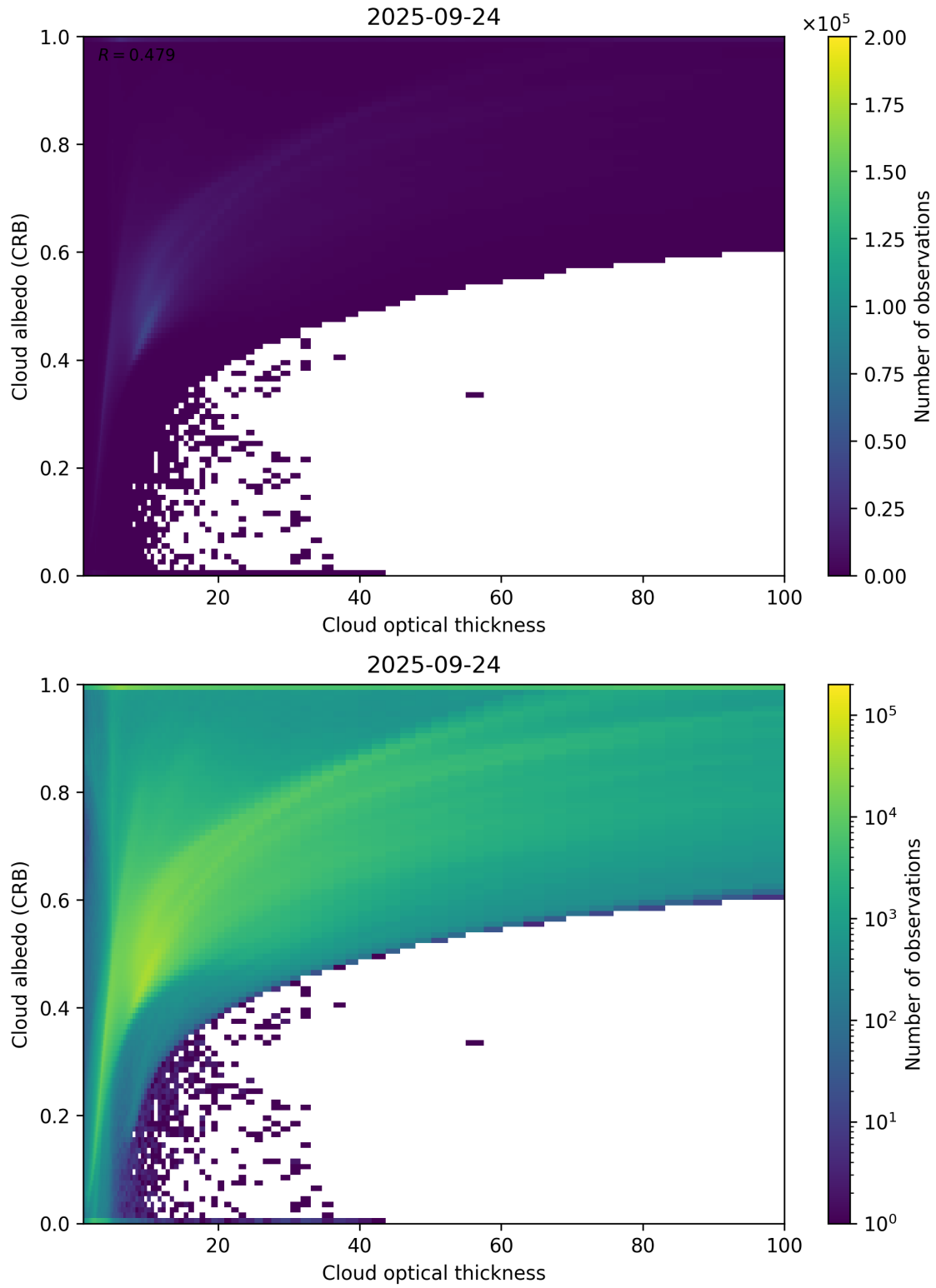
Figure 82: Scatter density plot of “Cloud optical thickness” against “Cloud albedo (CRB)” for 2025-09-23 to 2025-09-25.
