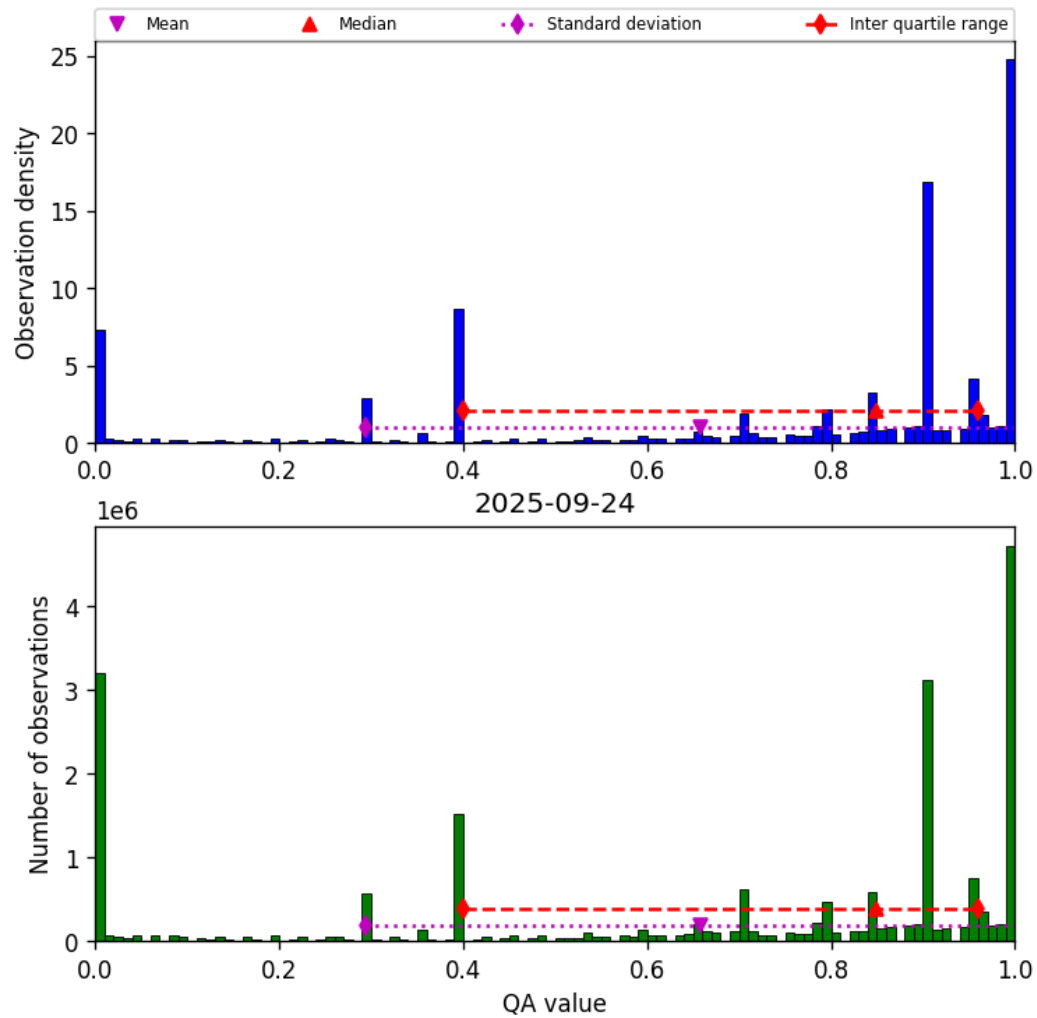
Figure 38: Histogram of “QA value” for 2025-09-23 to 2025-09-25
