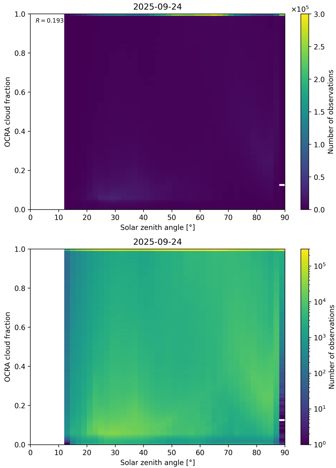
Figure 100: Scatter density plot of “Solar zenith angle” against “OCRA cloud fraction” for 2025-09-23 to 2025-09-25.
