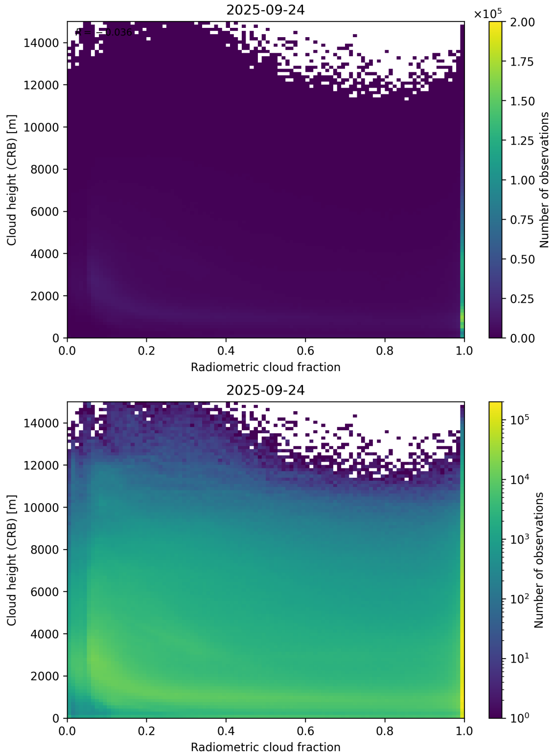
Figure 74: Scatter density plot of “Radiometric cloud fraction” against “Cloud height (CRB)” for 2025-09-23 to 2025-09-25.
