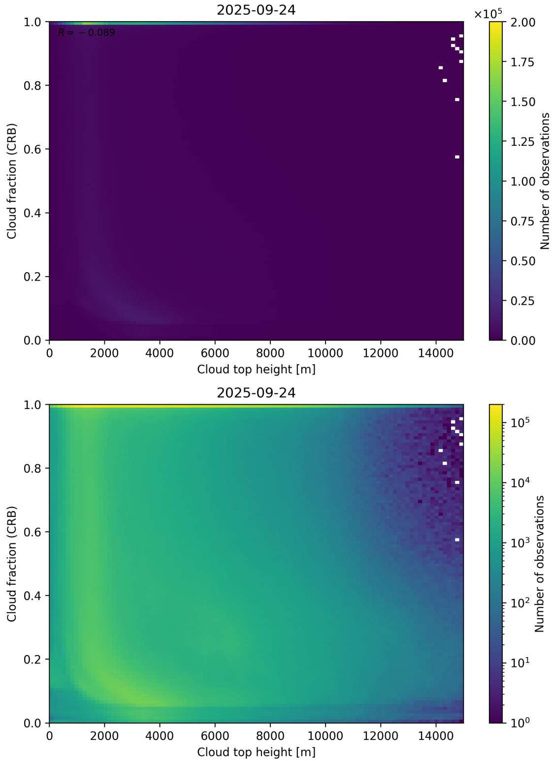
Figure 88: Scatter density plot of “Cloud top height” against “Cloud fraction (CRB)” for 2025-09-23 to 2025-09-25.
