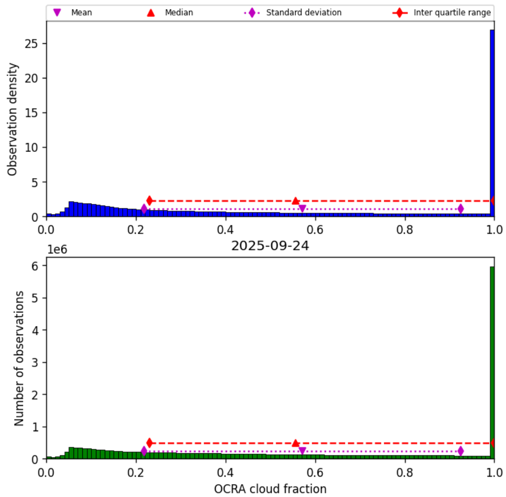
Figure 50: Histogram of “OCRA cloud fraction” for 2025-09-23 to 2025-09-25
