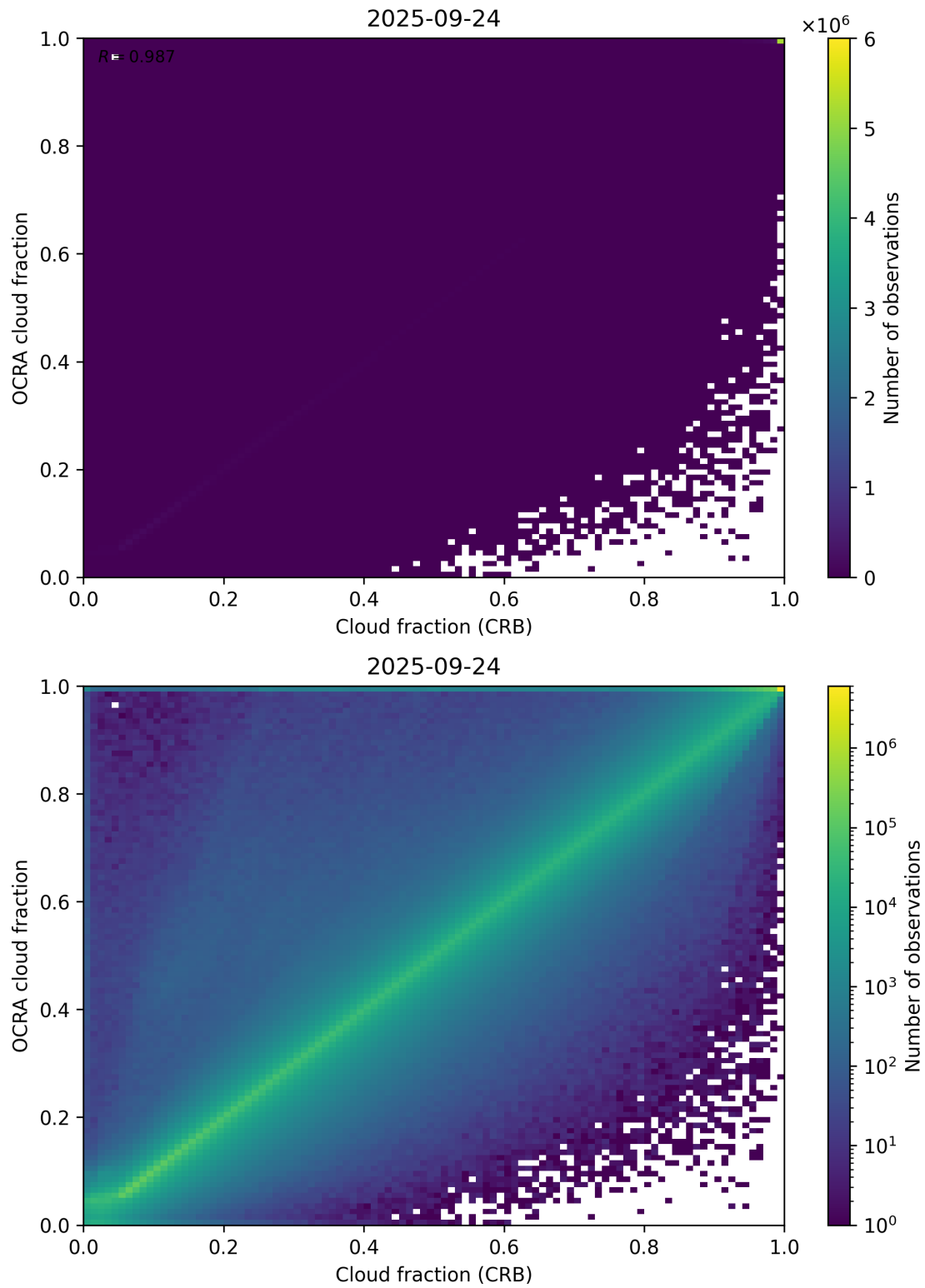
Figure 78: Scatter density plot of “Cloud fraction (CRB)” against “OCRA cloud fraction” for 2025-09-23 to 2025-09-25.
