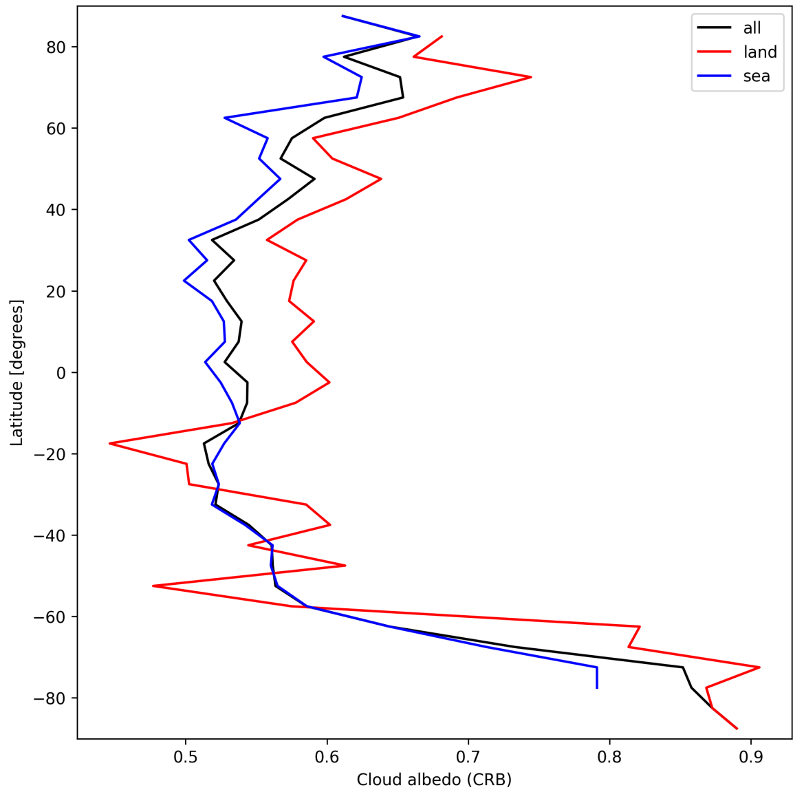
Figure 28: Zonal average of “Cloud albedo (CRB)” for 2025-09-23 to 2025-09-25.
