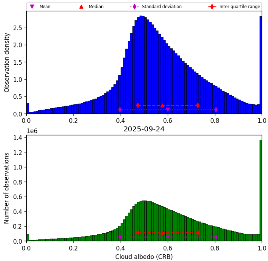
Figure 44: Histogram of “Cloud albedo (CRB)” for 2025-09-23 to 2025-09-25
