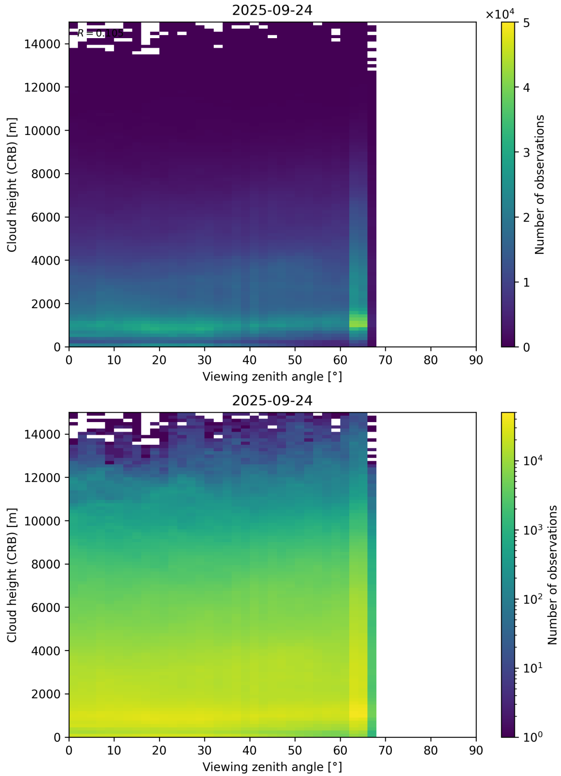
Figure 110: Scatter density plot of “Viewing zenith angle” against “Cloud height (CRB)” for 2025-09-23 to 2025-09-25.
