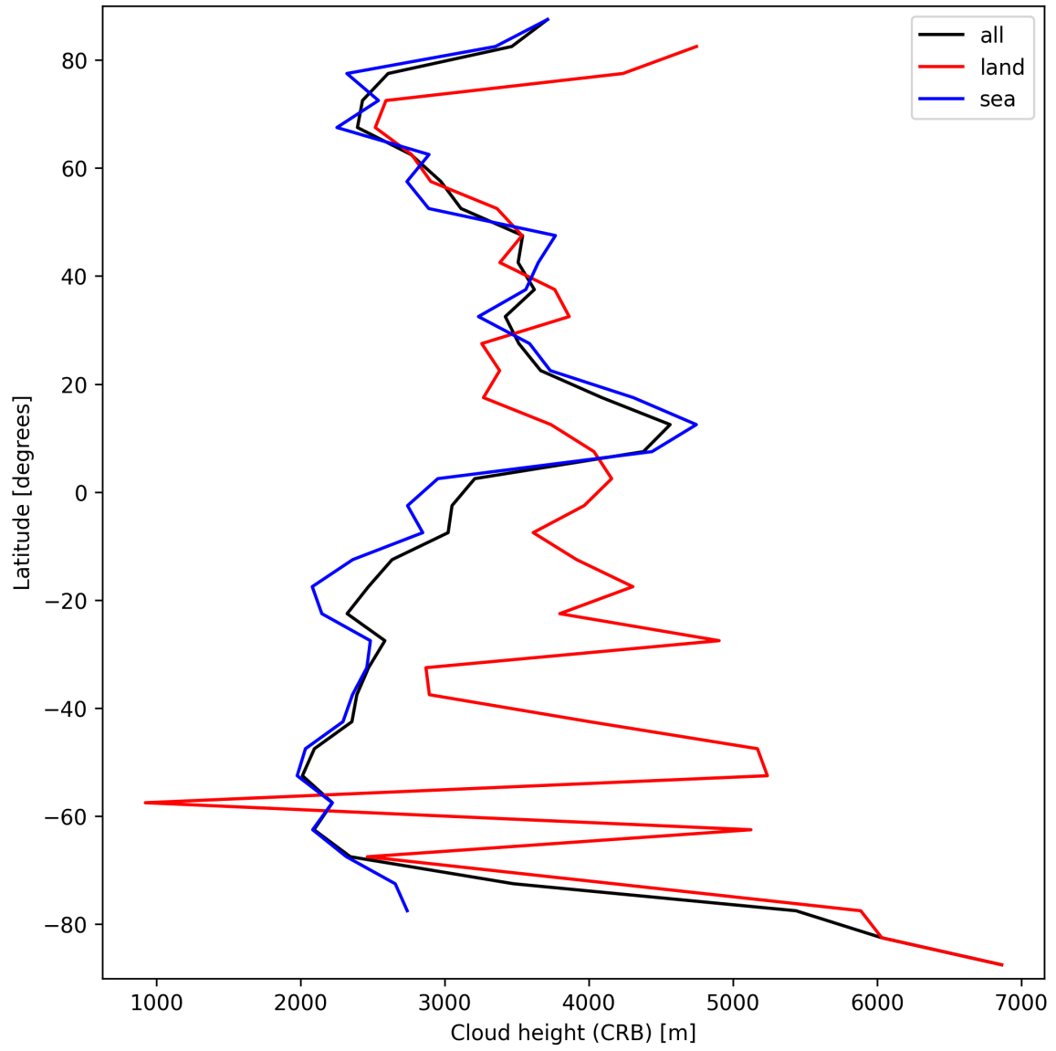
Figure 27: Zonal average of “Cloud height (CRB)” for 2025-09-23 to 2025-09-25.
