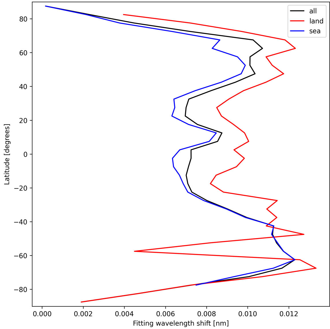
Figure 33: Zonal average of “Fitting wavelength shift” for 2025-09-23 to 2025-09-25.
