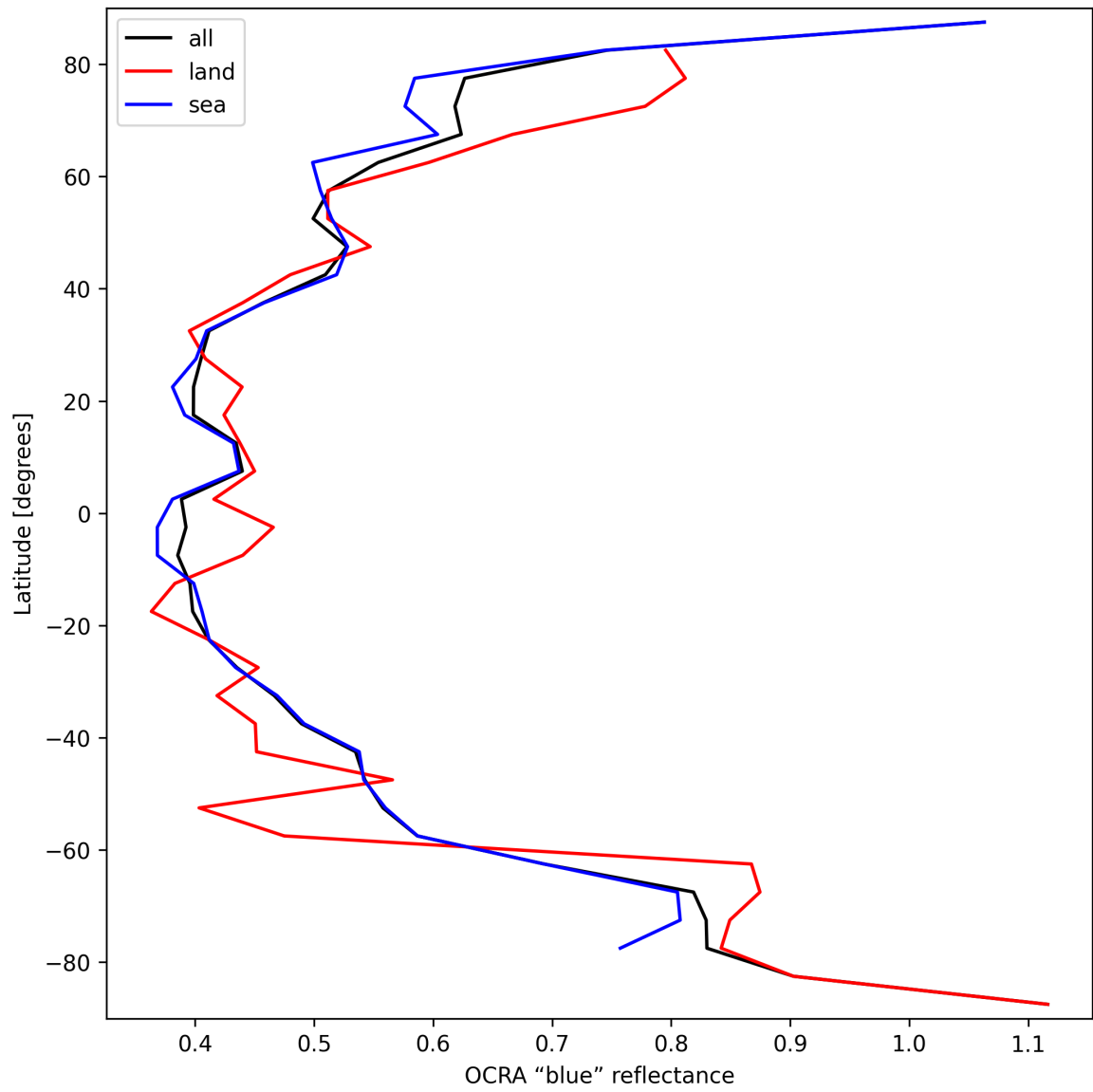
Figure 35: Zonal average of “OCRA “blue” reflectance” for 2025-09-23 to 2025-09-25.
