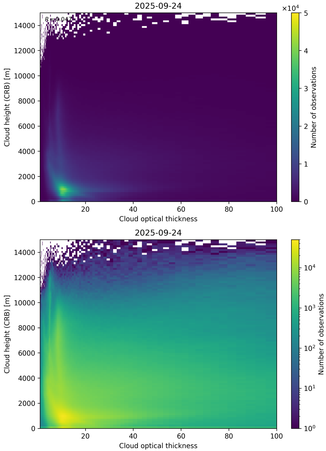
Figure 85: Scatter density plot of “Cloud optical thickness” against “Cloud height (CRB)” for 2025-09-23 to 2025-09-25.
