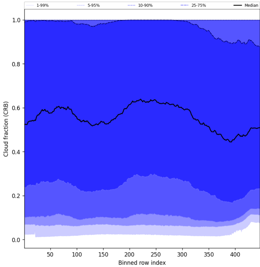
Figure 58: Along track statistics of “Cloud fraction (CRB)” for 2025-09-23 to 2025-09-25
