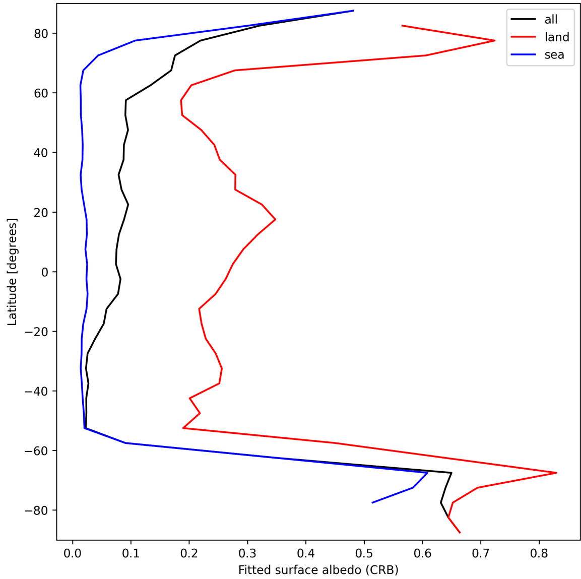
Figure 30: Zonal average of “Fitted surface albedo (CRB)” for 2025-09-23 to 2025-09-25.
