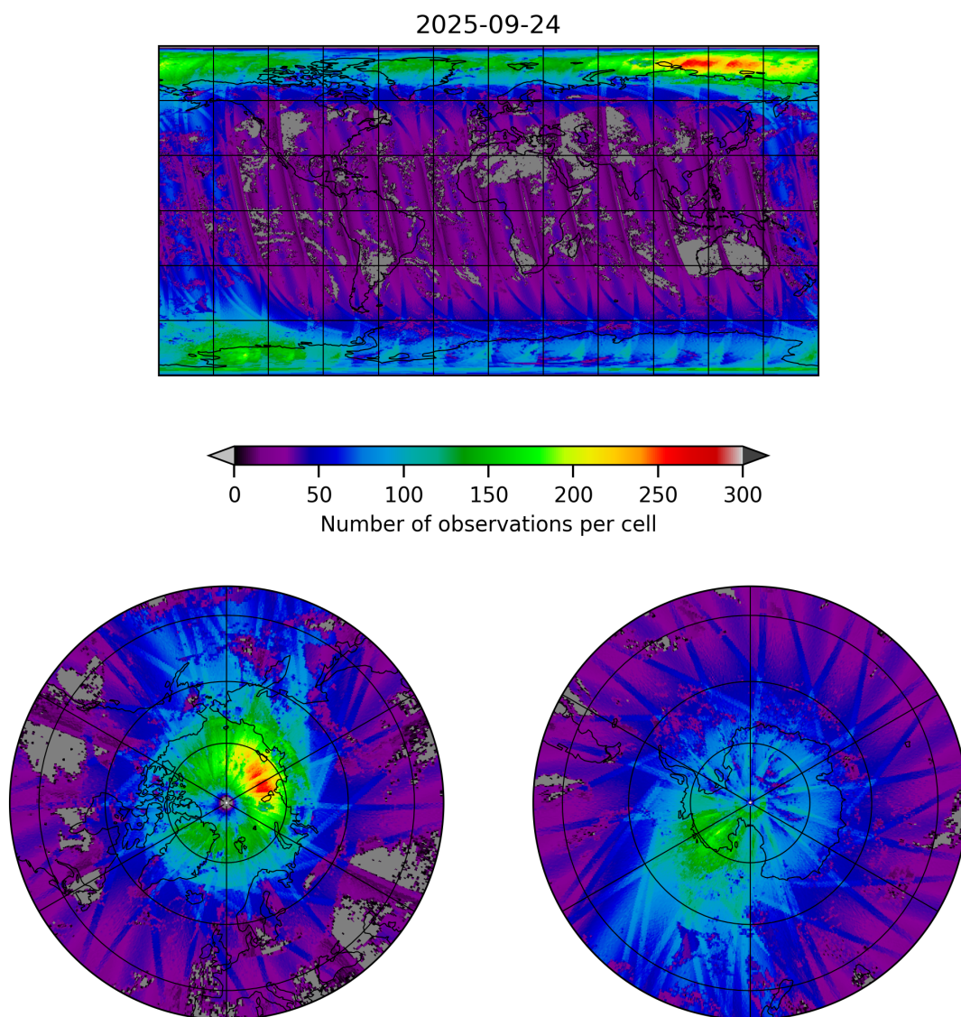
Figure 21: Map of the number of observations for 2025-09-23 to 2025-09-25
