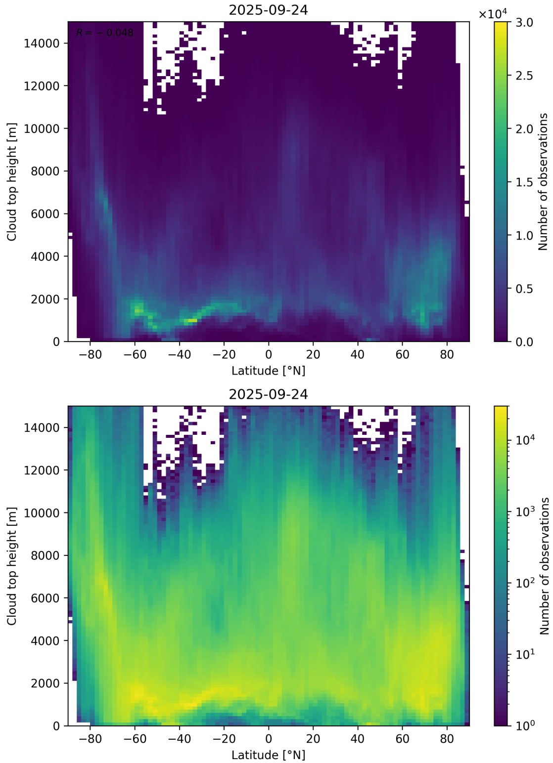
Figure 97: Scatter density plot of “Latitude” against “Cloud top height” for 2025-09-23 to 2025-09-25.
