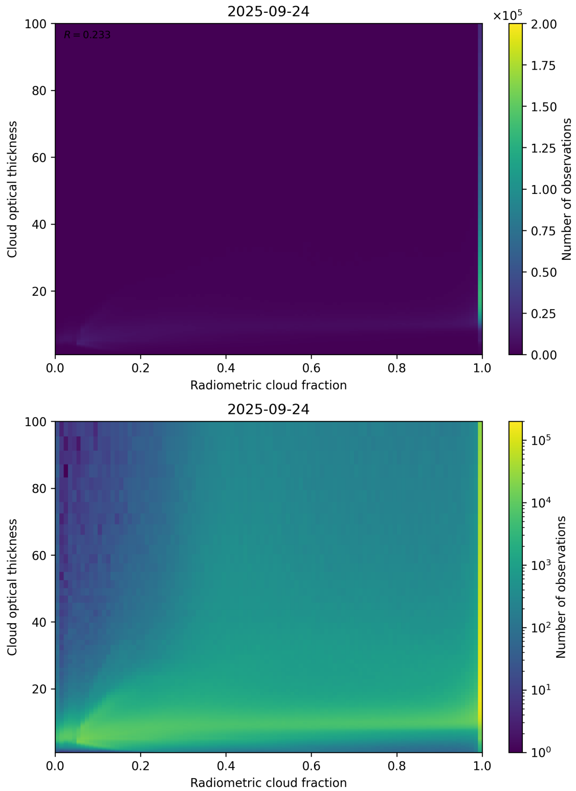
Figure 75: Scatter density plot of “Radiometric cloud fraction” against “Cloud optical thickness” for 2025-09-23 to 2025-09-25.
