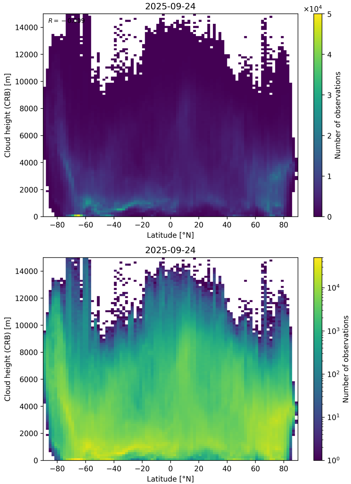
Figure 95: Scatter density plot of “Latitude” against “Cloud height (CRB)” for 2025-09-23 to 2025-09-25.
