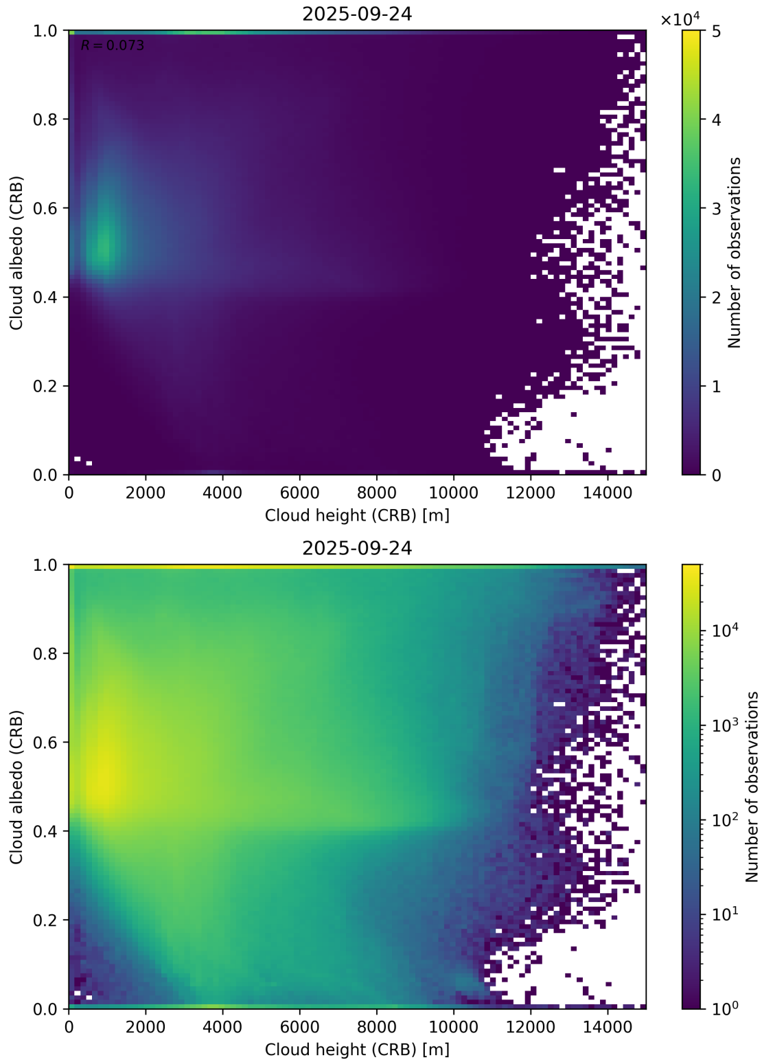
Figure 80: Scatter density plot of “Cloud height (CRB)” against “Cloud albedo (CRB)” for 2025-09-23 to 2025-09-25.
