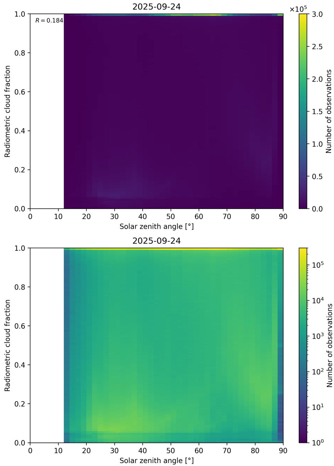
Figure 99: Scatter density plot of “Solar zenith angle” against “Radiometric cloud fraction” for 2025-09-23 to 2025-09-25.
