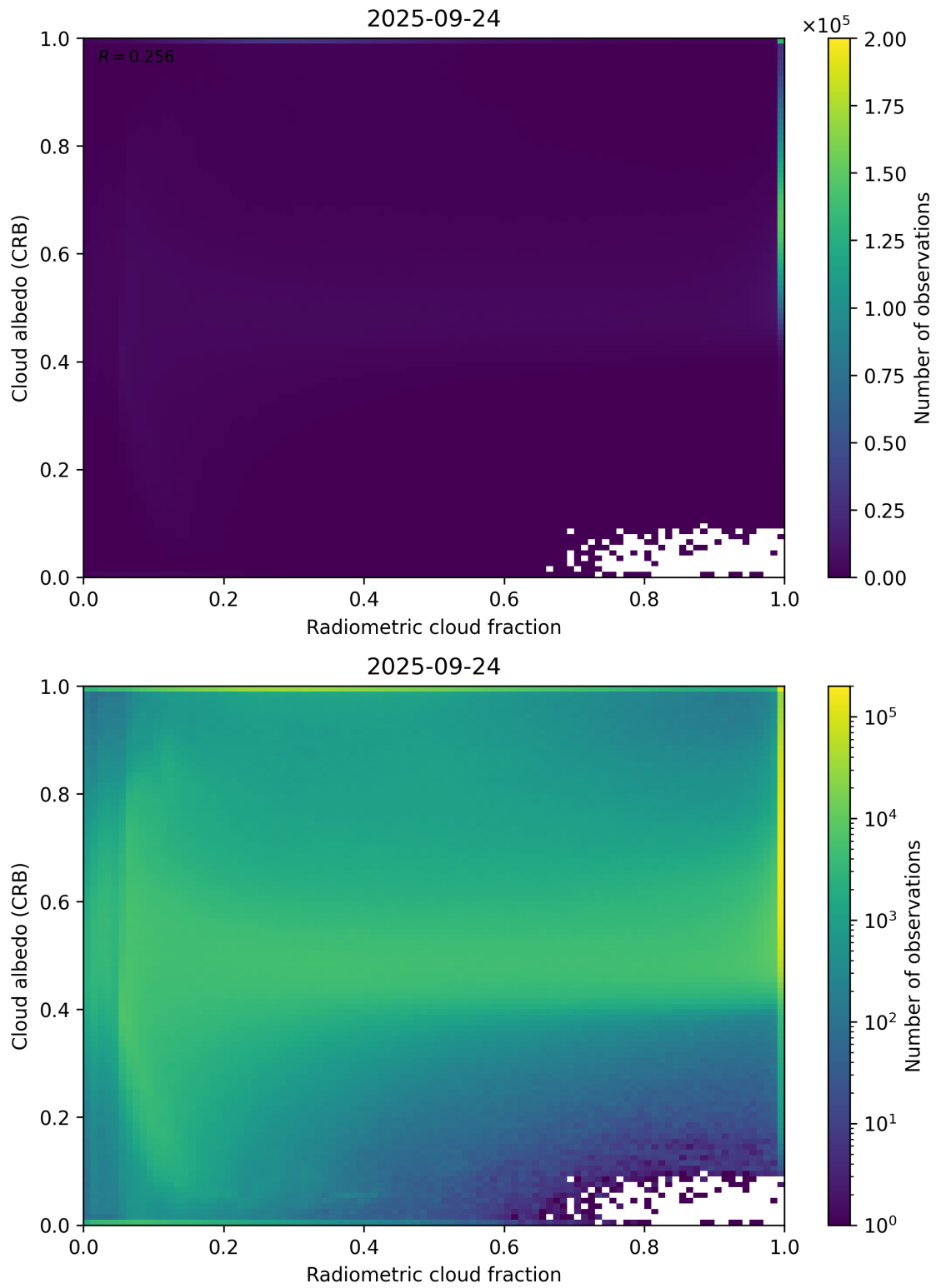
Figure 71: Scatter density plot of “Radiometric cloud fraction” against “Cloud albedo (CRB)” for 2025-09-23 to 2025-09-25.
