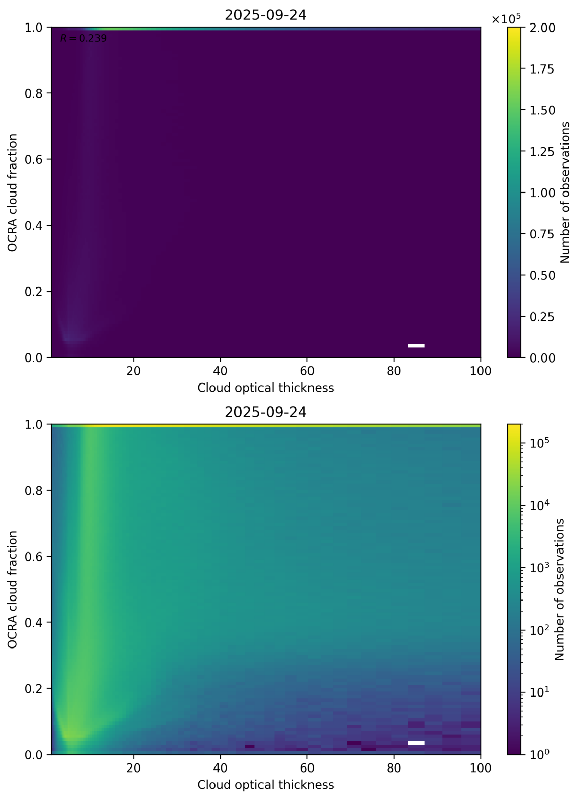
Figure 83: Scatter density plot of “Cloud optical thickness” against “OCRA cloud fraction” for 2025-09-23 to 2025-09-25.
