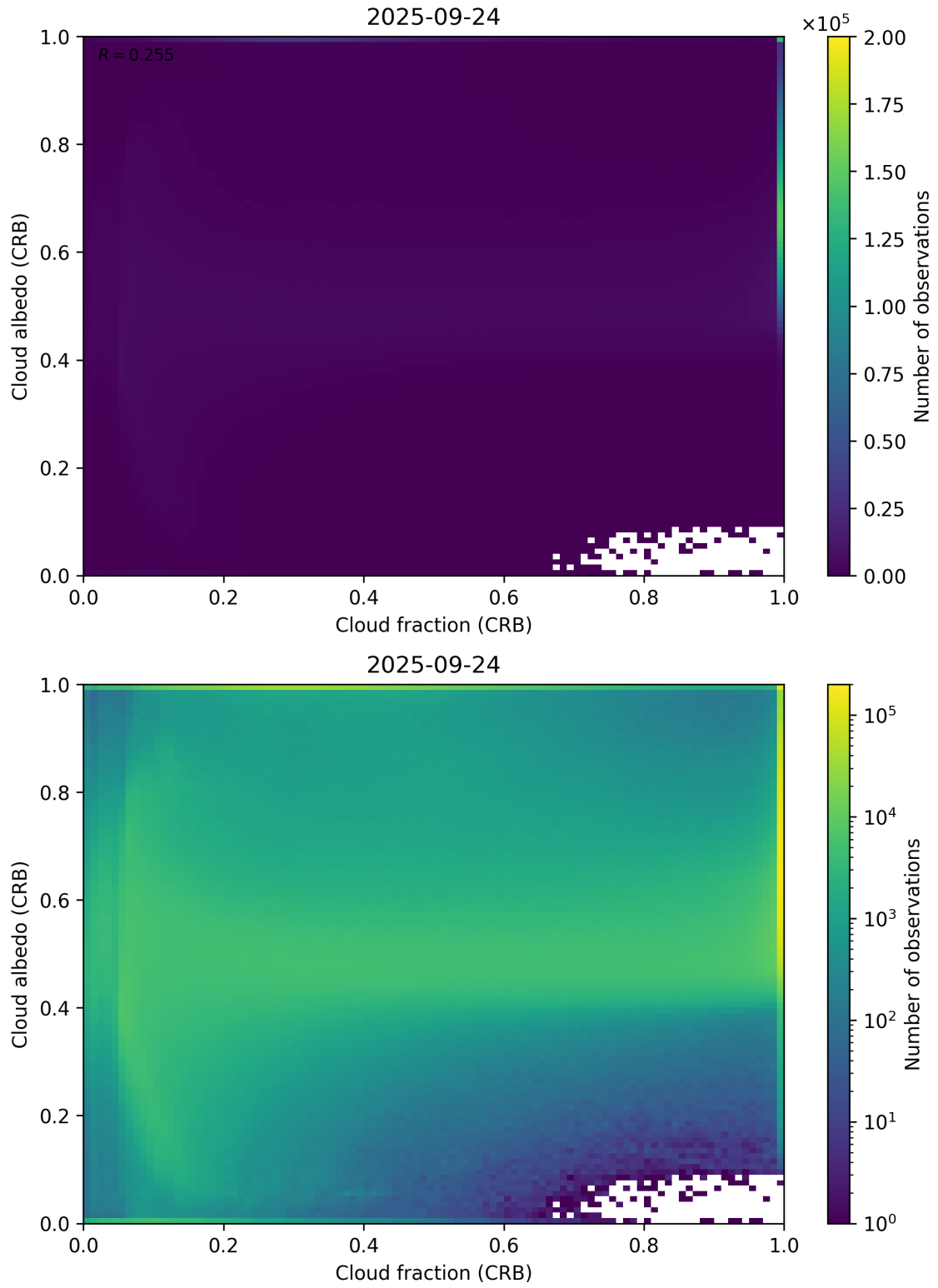
Figure 77: Scatter density plot of “Cloud fraction (CRB)” against “Cloud albedo (CRB)” for 2025-09-23 to 2025-09-25.
