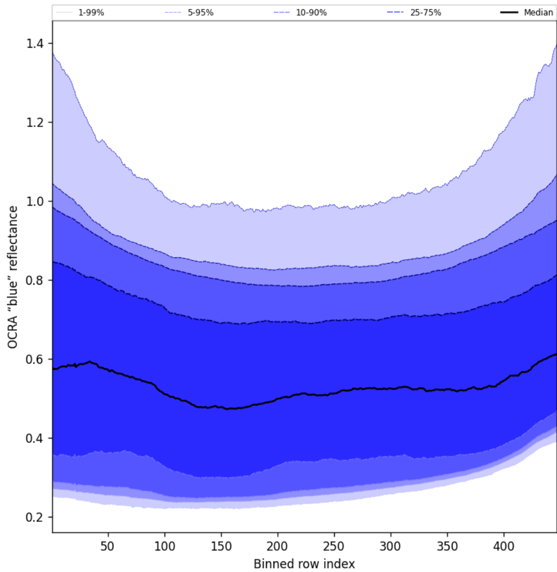
Figure 67: Along track statistics of “OCRA “blue” reflectance” for 2025-09-23 to 2025-09-25
