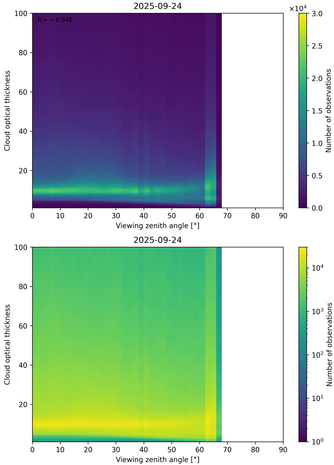
Figure 111: Scatter density plot of “Viewing zenith angle” against “Cloud optical thickness” for 2025-09-23 to 2025-09-25.
