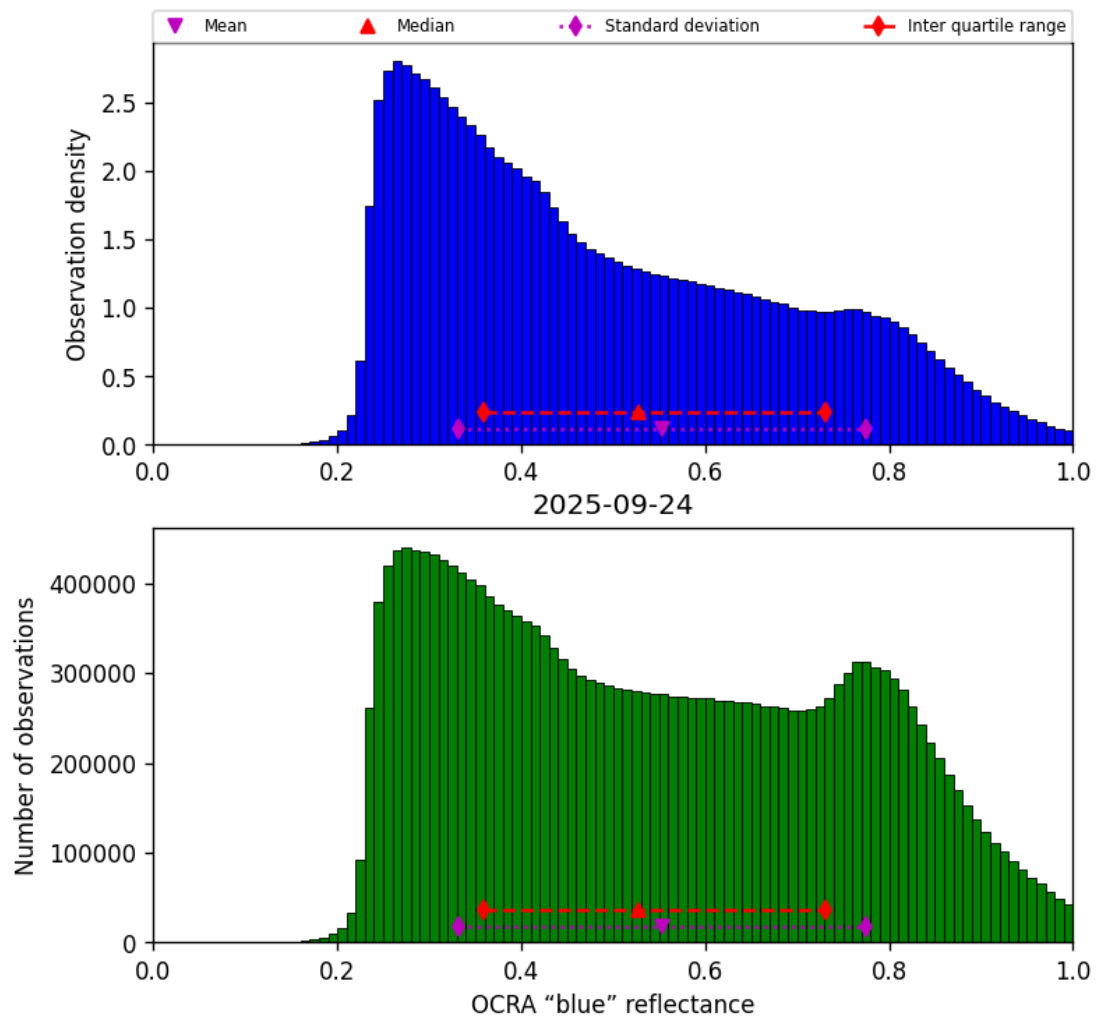
Figure 51: Histogram of “OCRA “blue” reflectance” for 2025-09-23 to 2025-09-25
