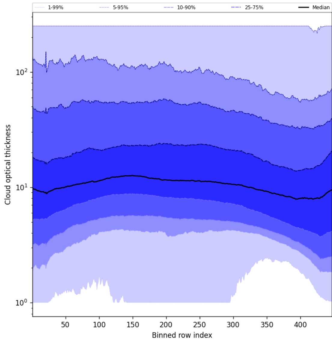
Figure 57: Along track statistics of “Cloud optical thickness” for 2025-09-23 to 2025-09-25
