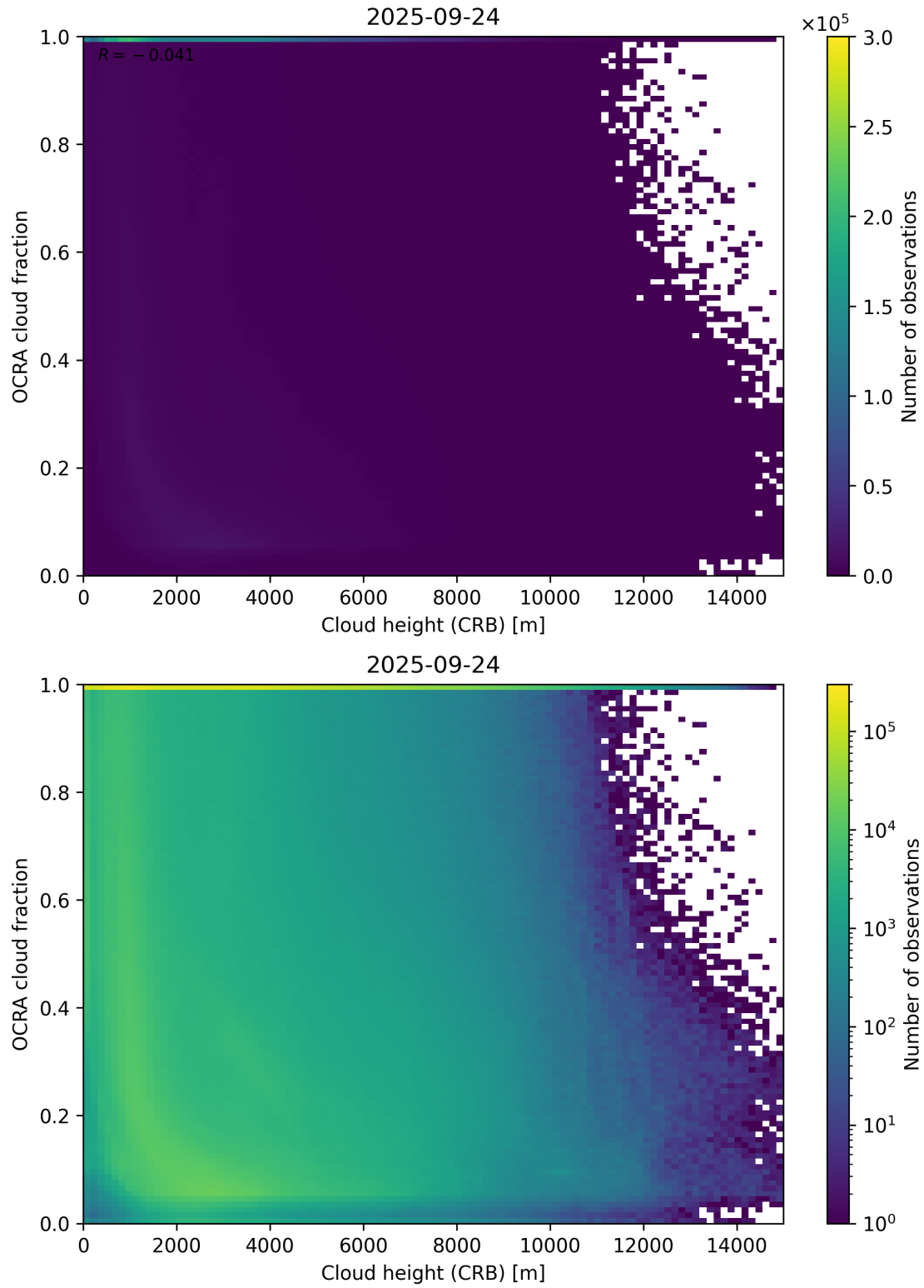
Figure 81: Scatter density plot of “Cloud height (CRB)” against “OCRA cloud fraction” for 2025-09-23 to 2025-09-25.
