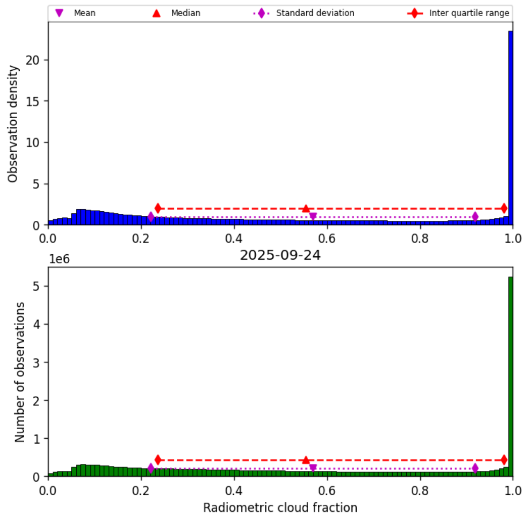
Figure 39: Histogram of “Radiometric cloud fraction” for 2025-09-23 to 2025-09-25
