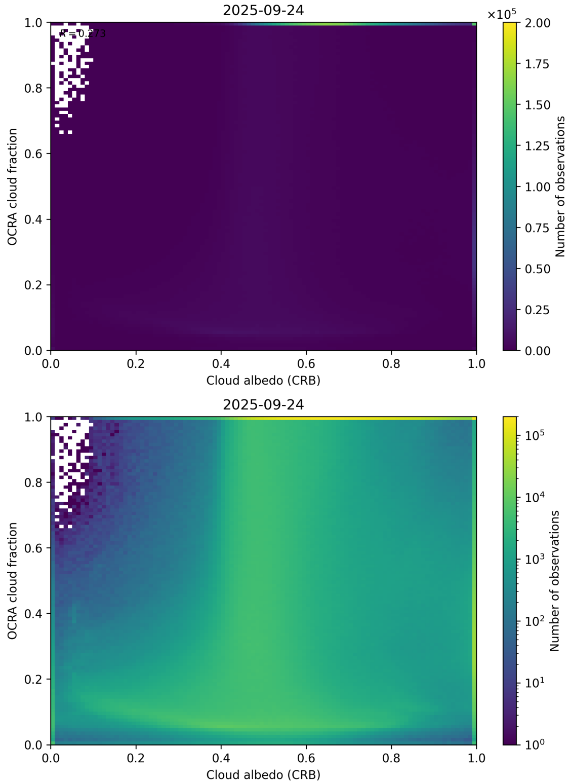
Figure 70: Scatter density plot of “Cloud albedo (CRB)” against “OCRA cloud fraction” for 2025-09-23 to 2025-09-25.
