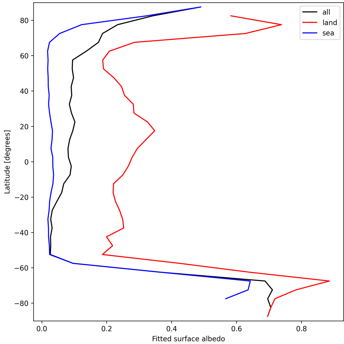
Figure 29: Zonal average of “Fitted surface albedo” for 2025-09-23 to 2025-09-25.
