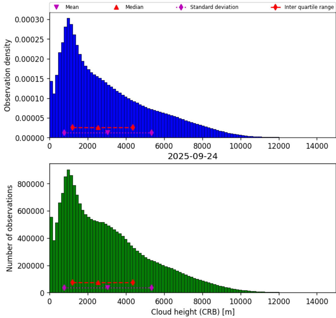
Figure 43: Histogram of “Cloud height (CRB)” for 2025-09-23 to 2025-09-25
