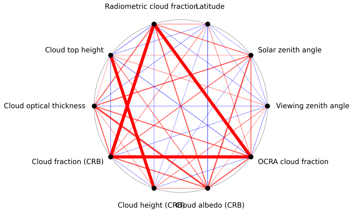
Figure 1: Map of correlation graph for 2025-09-23 to 2025-09-25.
