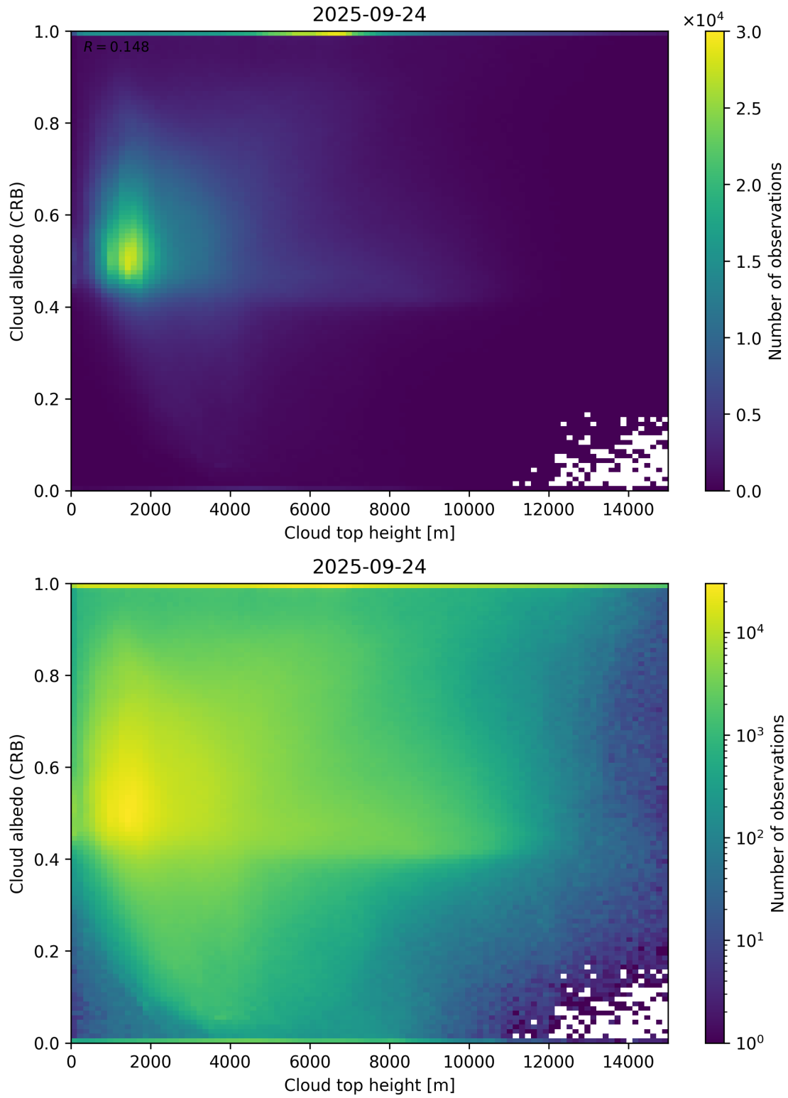
Figure 86: Scatter density plot of “Cloud top height” against “Cloud albedo (CRB)” for 2025-09-23 to 2025-09-25.
