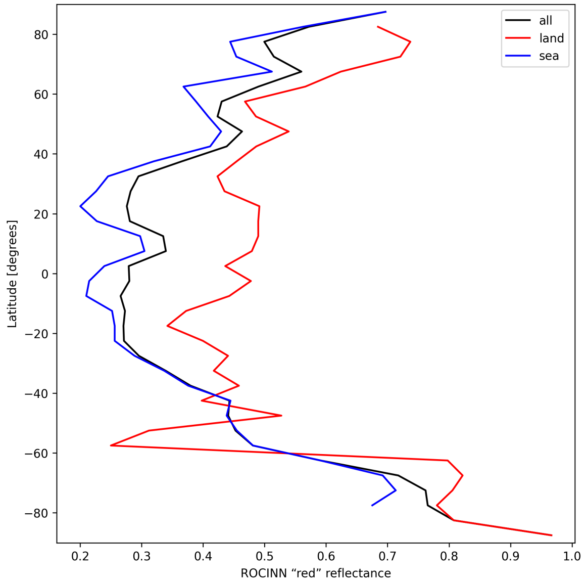
Figure 37: Zonal average of “ROCINN “red” reflectance” for 2025-09-23 to 2025-09-25.
