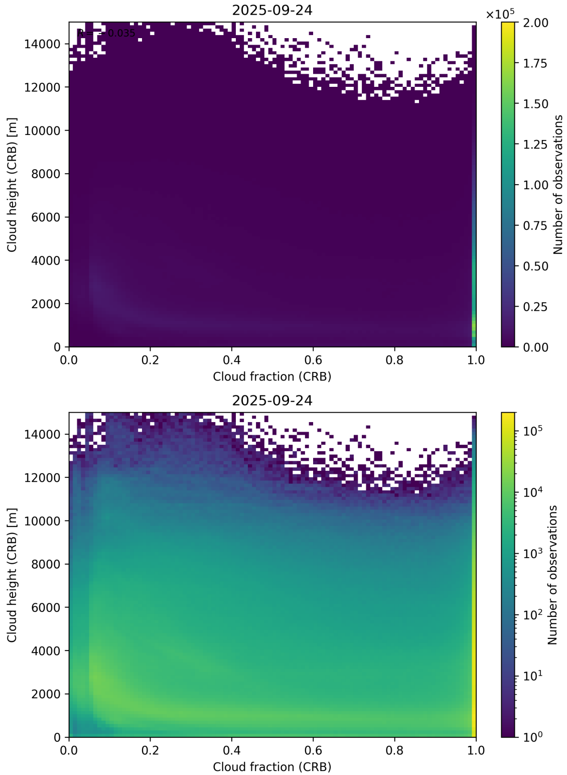
Figure 79: Scatter density plot of “Cloud fraction (CRB)” against “Cloud height (CRB)” for 2025-09-23 to 2025-09-25.
