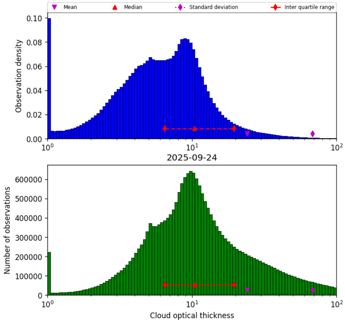
Figure 41: Histogram of “Cloud optical thickness” for 2025-09-23 to 2025-09-25
