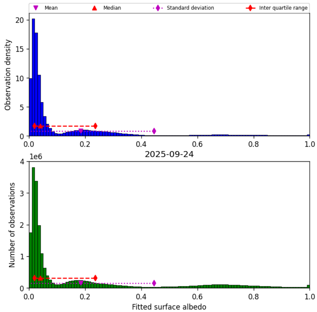
Figure 45: Histogram of “Fitted surface albedo” for 2025-09-23 to 2025-09-25
