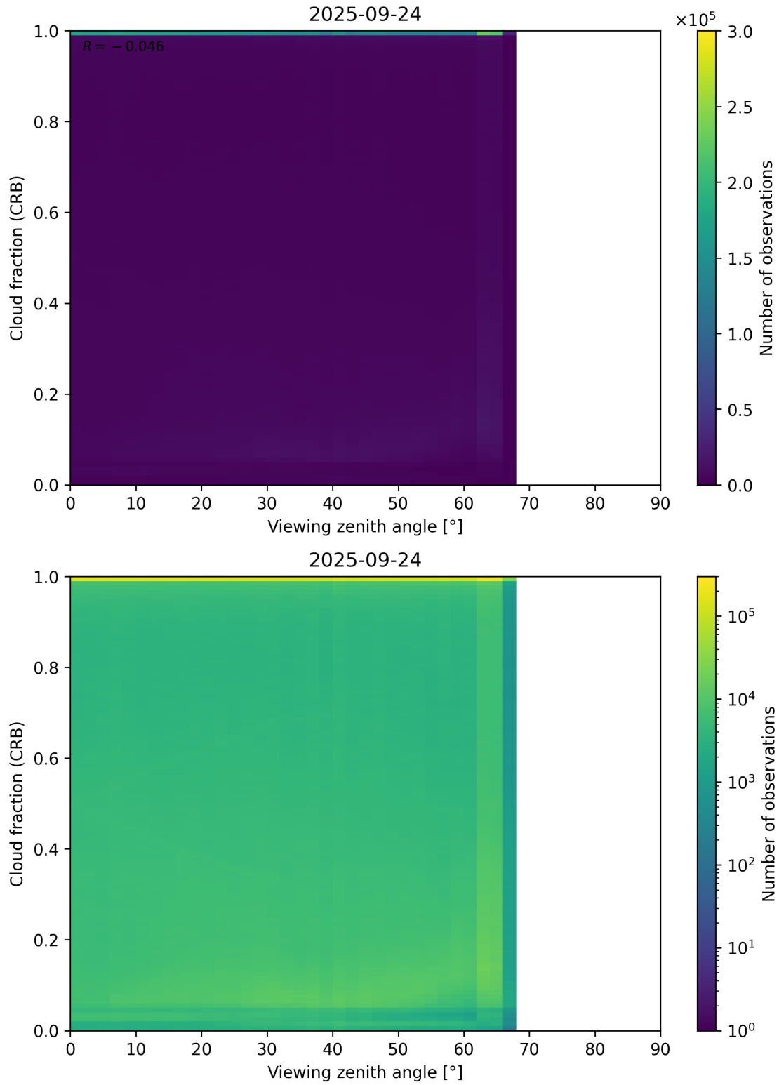
Figure 109: Scatter density plot of “Viewing zenith angle” against “Cloud fraction (CRB)” for 2025-09-23 to 2025-09-25.
