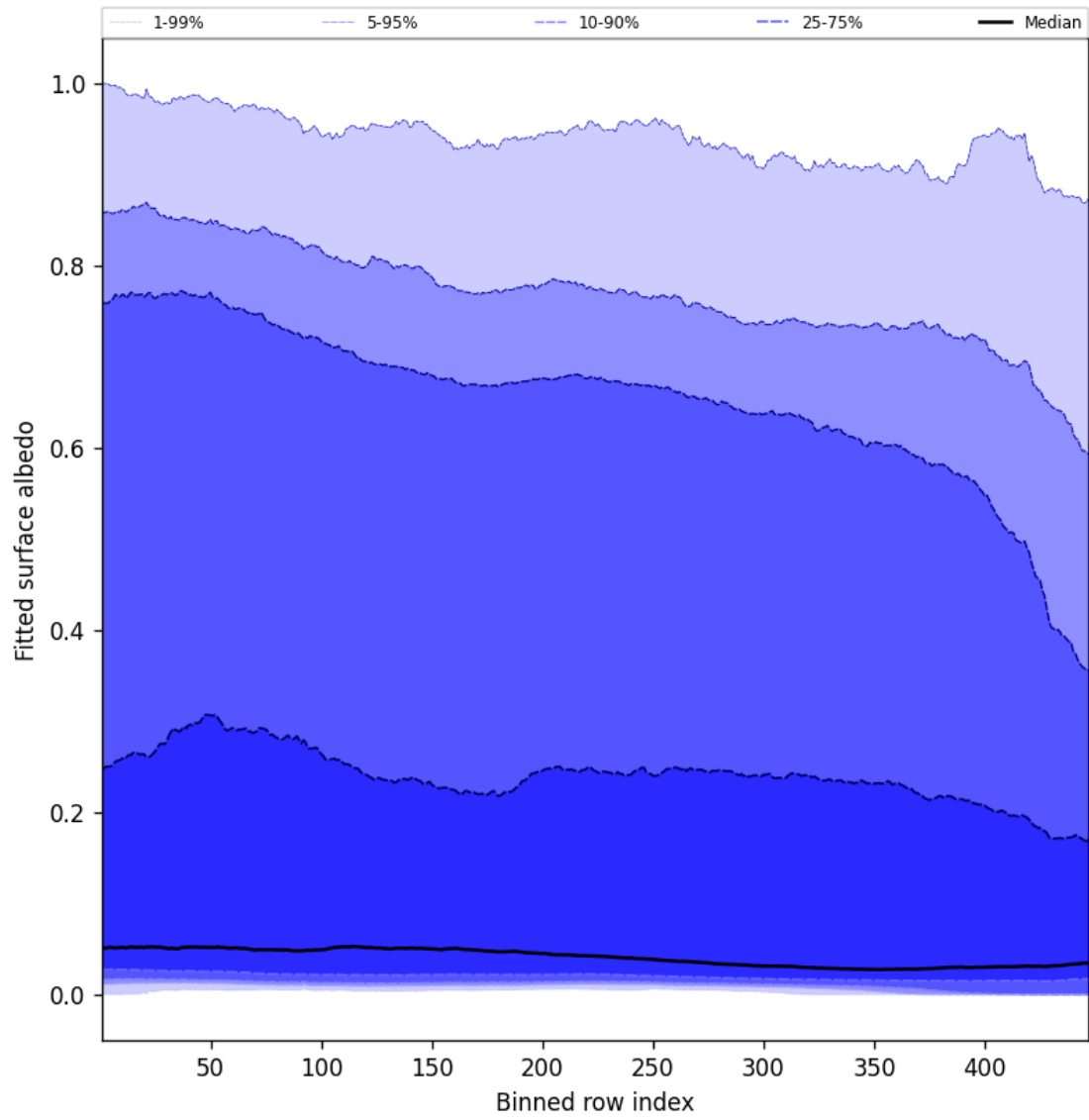
Figure 61: Along track statistics of “Fitted surface albedo” for 2025-09-23 to 2025-09-25
