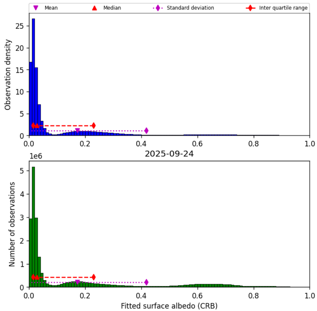
Figure 46: Histogram of “Fitted surface albedo (CRB)” for 2025-09-23 to 2025-09-25
