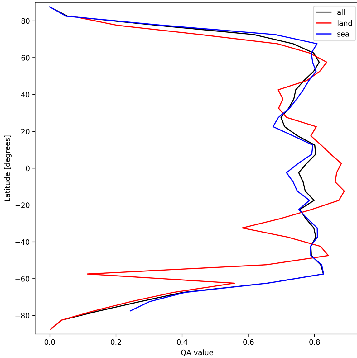
Figure 22: Zonal average of “QA value” for 2025-09-23 to 2025-09-25.
