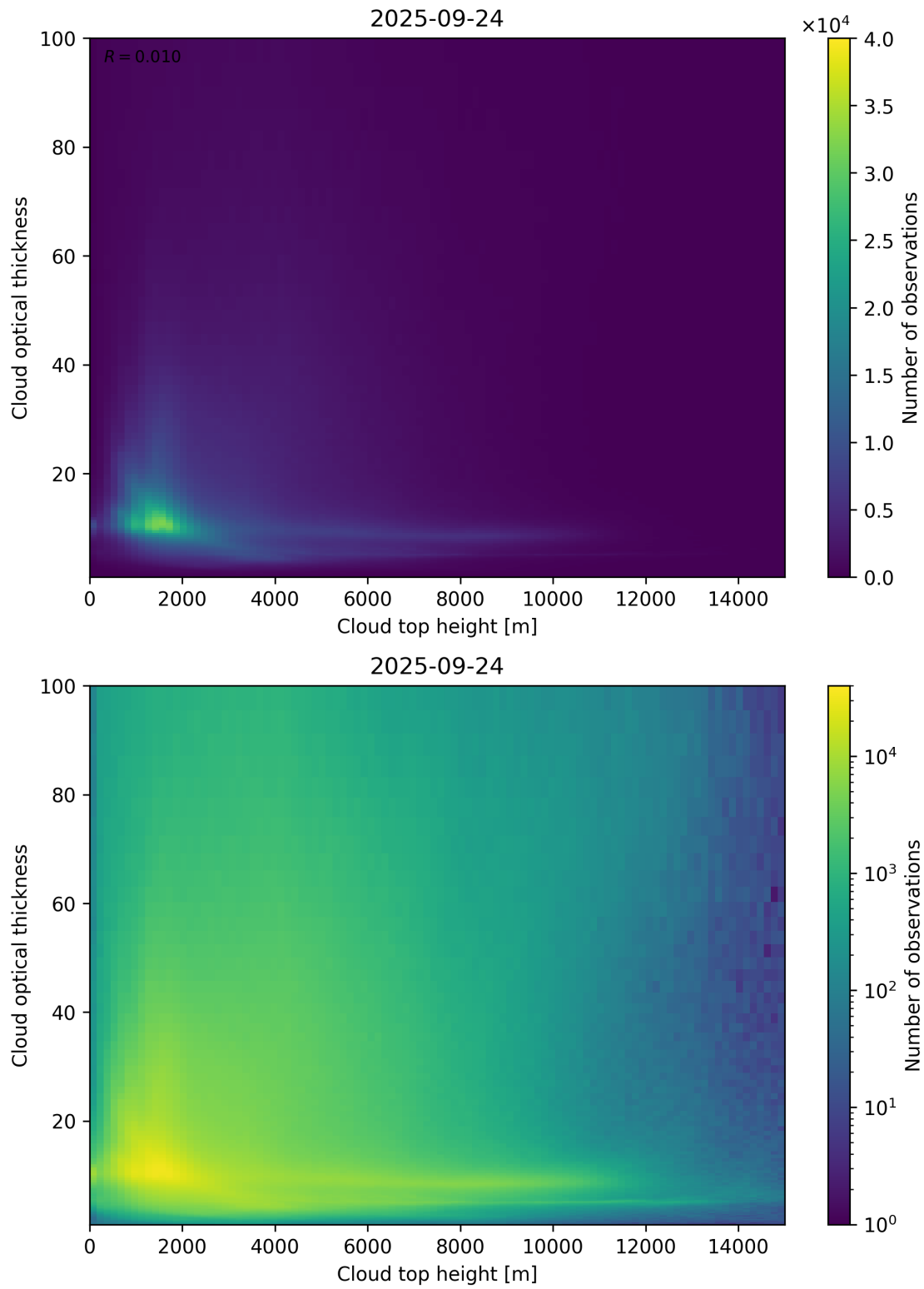
Figure 90: Scatter density plot of “Cloud top height” against “Cloud optical thickness” for 2025-09-23 to 2025-09-25.
