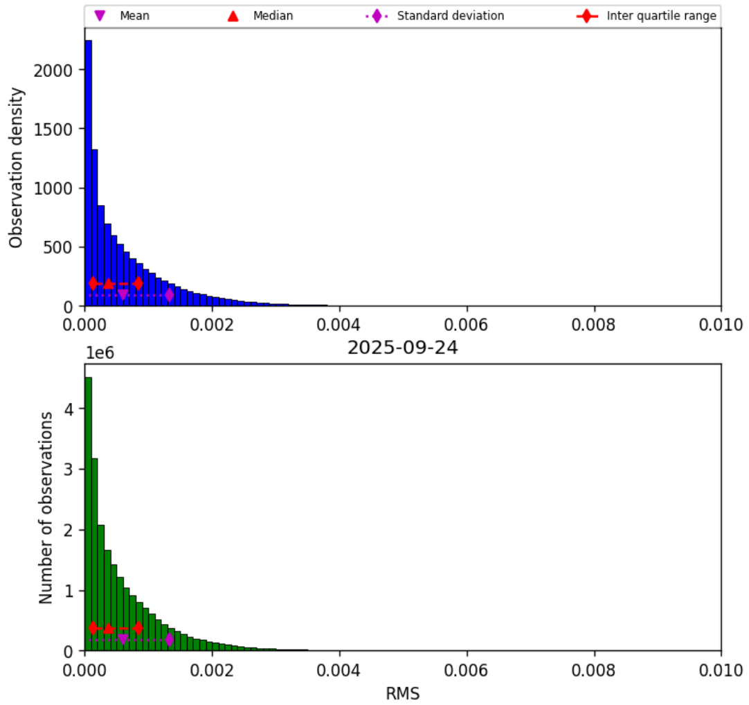
Figure 47: Histogram of “RMS” for 2025-09-23 to 2025-09-25
