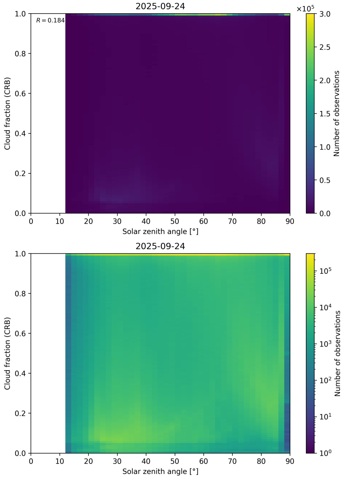
Figure 101: Scatter density plot of “Solar zenith angle” against “Cloud fraction (CRB)” for 2025-09-23 to 2025-09-25.
