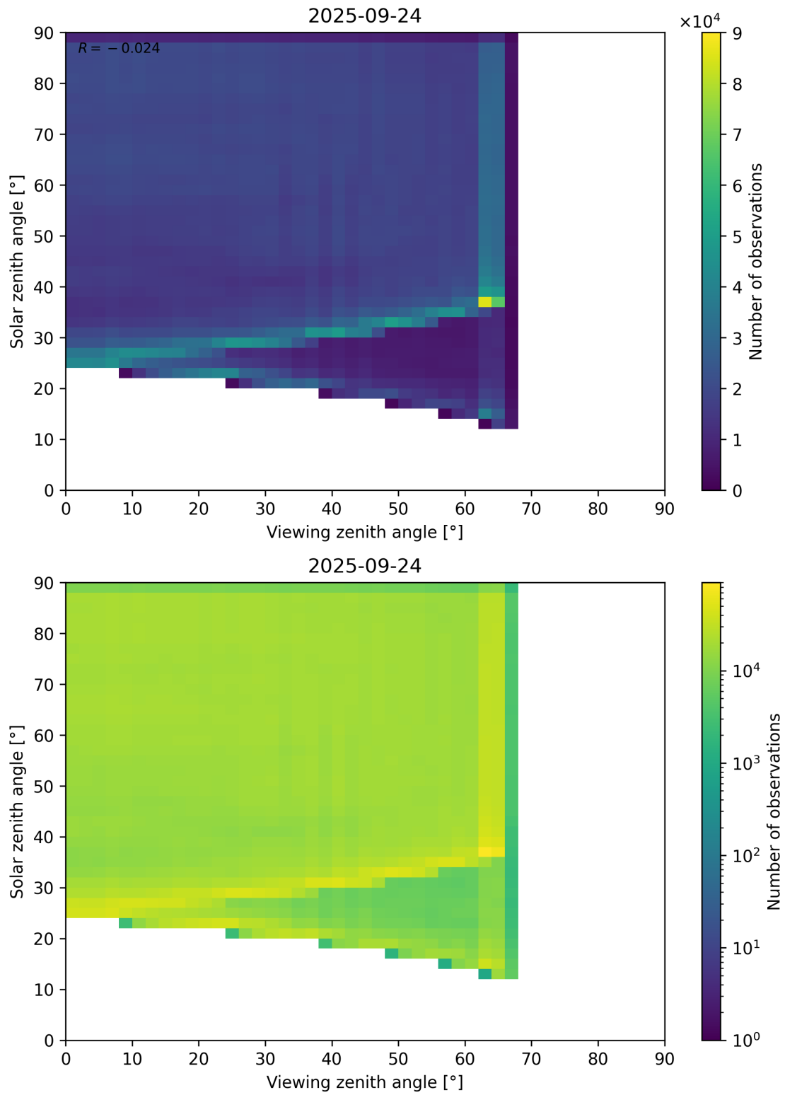
Figure 114: Scatter density plot of “Viewing zenith angle” against “Solar zenith angle” for 2025-09-23 to 2025-09-25.
