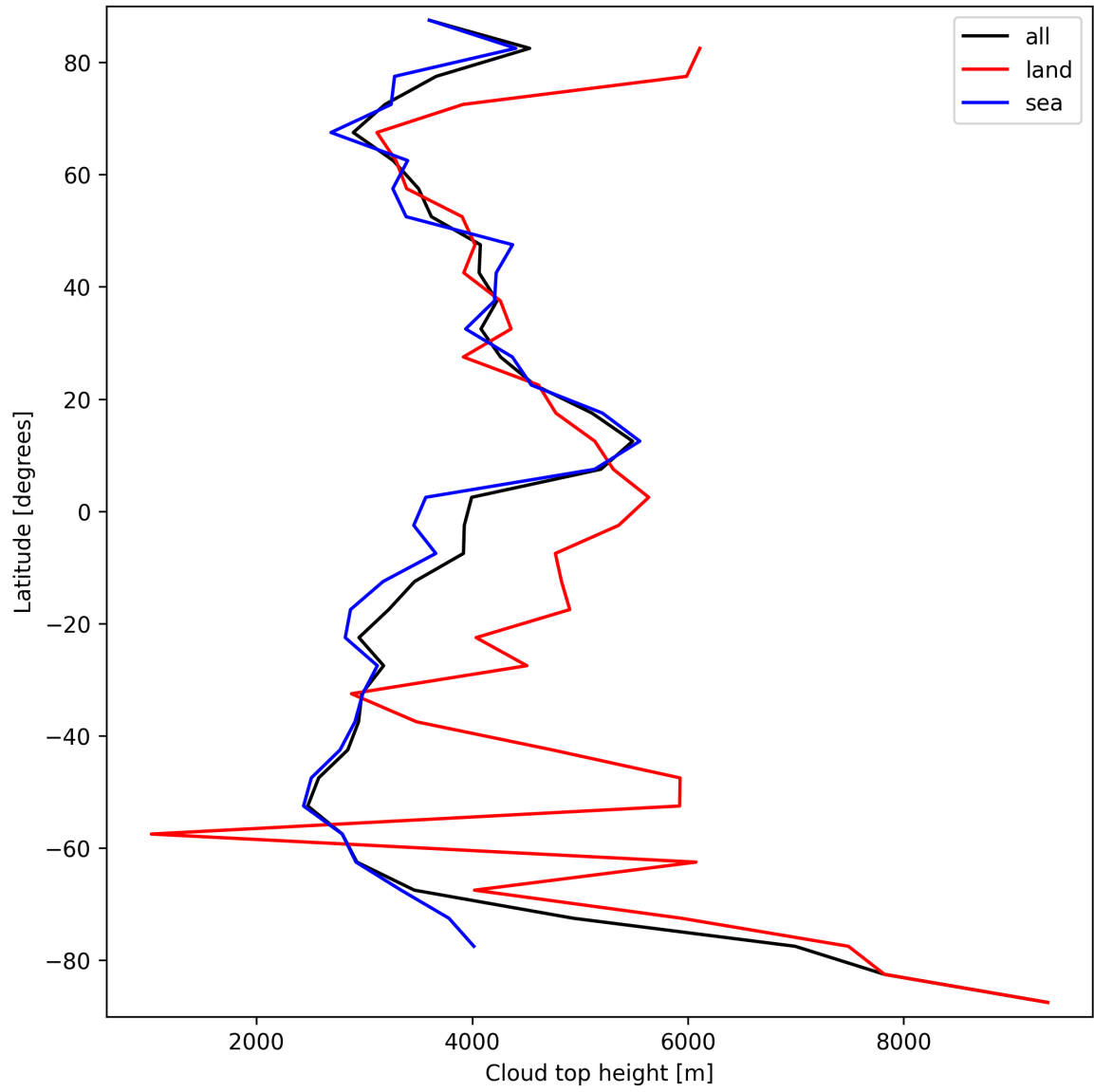
Figure 24: Zonal average of “Cloud top height” for 2025-09-23 to 2025-09-25.
