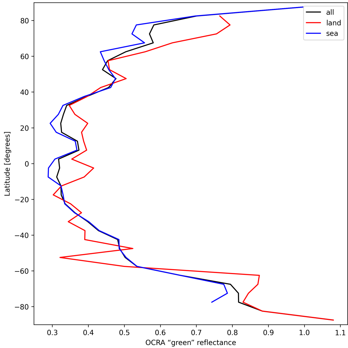
Figure 36: Zonal average of “OCRA “green” reflectance” for 2025-09-23 to 2025-09-25.
