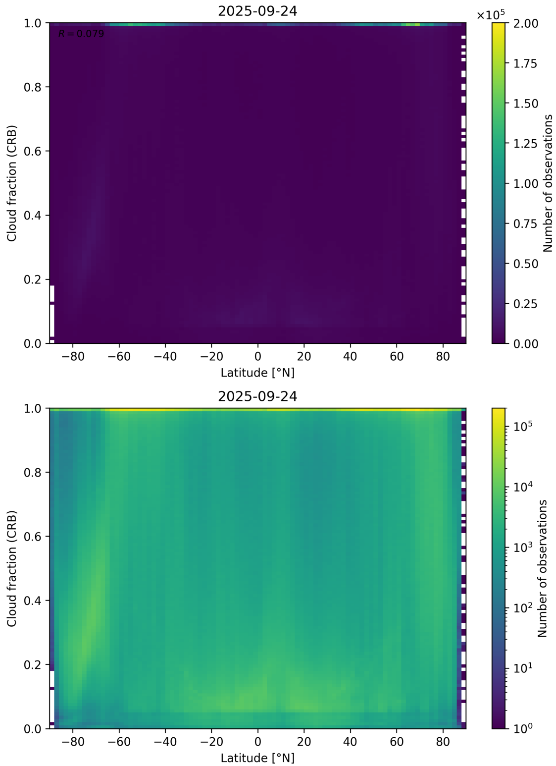
Figure 94: Scatter density plot of “Latitude” against “Cloud fraction (CRB)” for 2025-09-23 to 2025-09-25.
