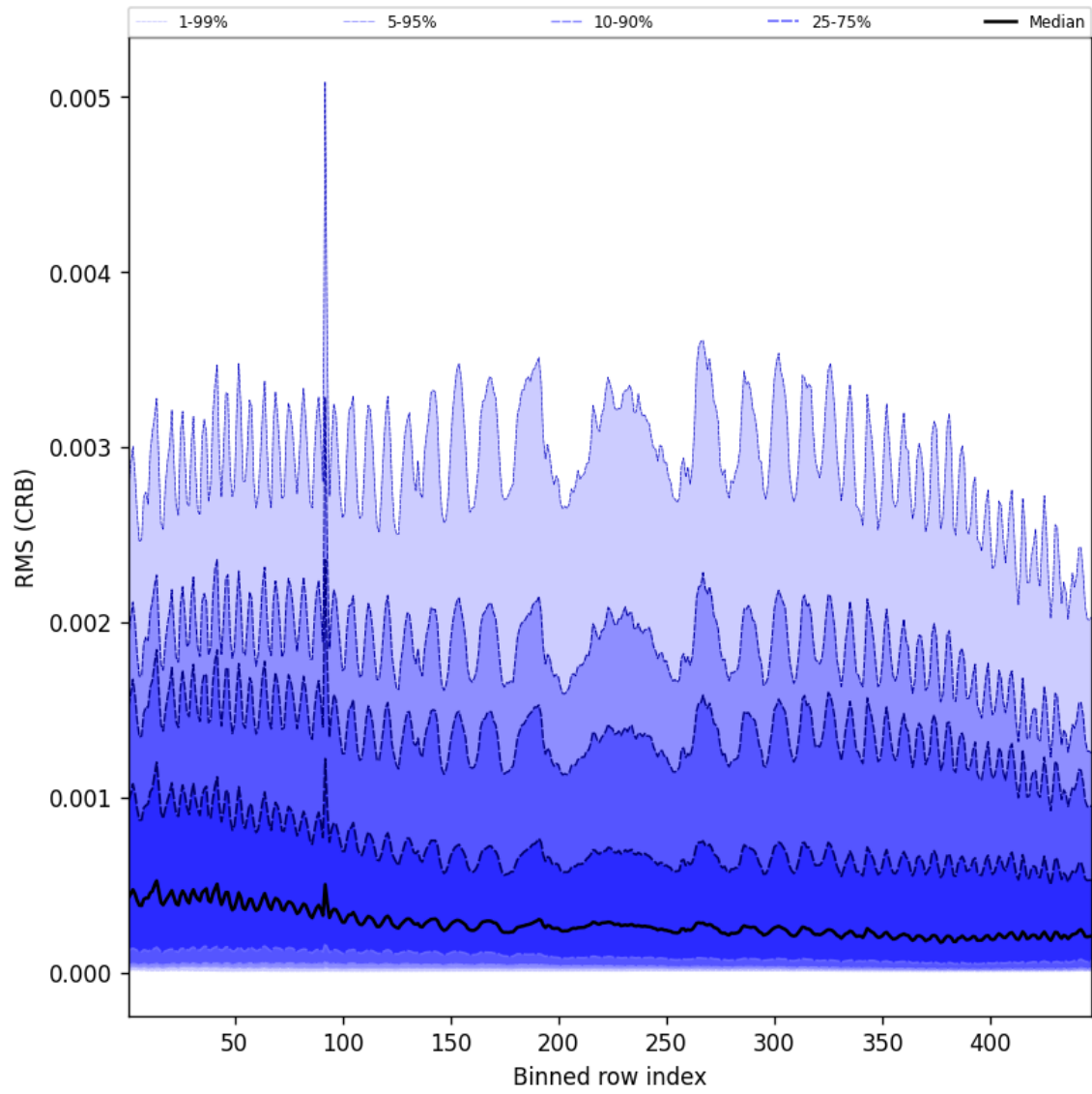
Figure 64: Along track statistics of “RMS (CRB)” for 2025-09-23 to 2025-09-25
