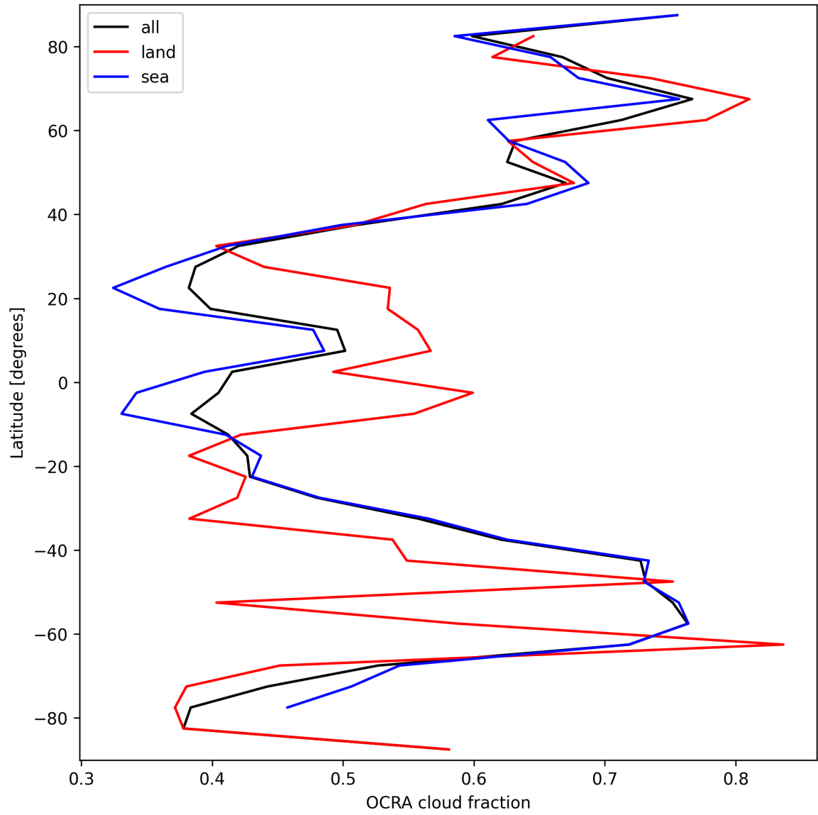
Figure 34: Zonal average of “OCRA cloud fraction” for 2025-09-23 to 2025-09-25.
