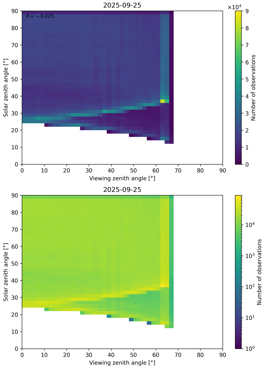
Figure 114: Scatter density plot of “Viewing zenith angle” against “Solar zenith angle” for 2025-09-25 to 2025-09-26.
