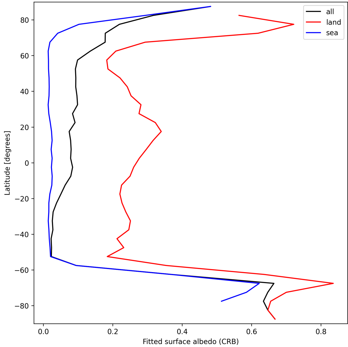
Figure 30: Zonal average of “Fitted surface albedo (CRB)” for 2025-09-25 to 2025-09-26.
