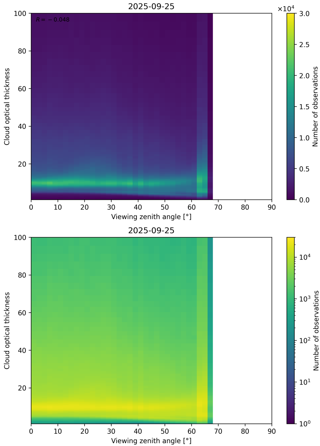
Figure 111: Scatter density plot of “Viewing zenith angle” against “Cloud optical thickness” for 2025-09-25 to 2025-09-26.
