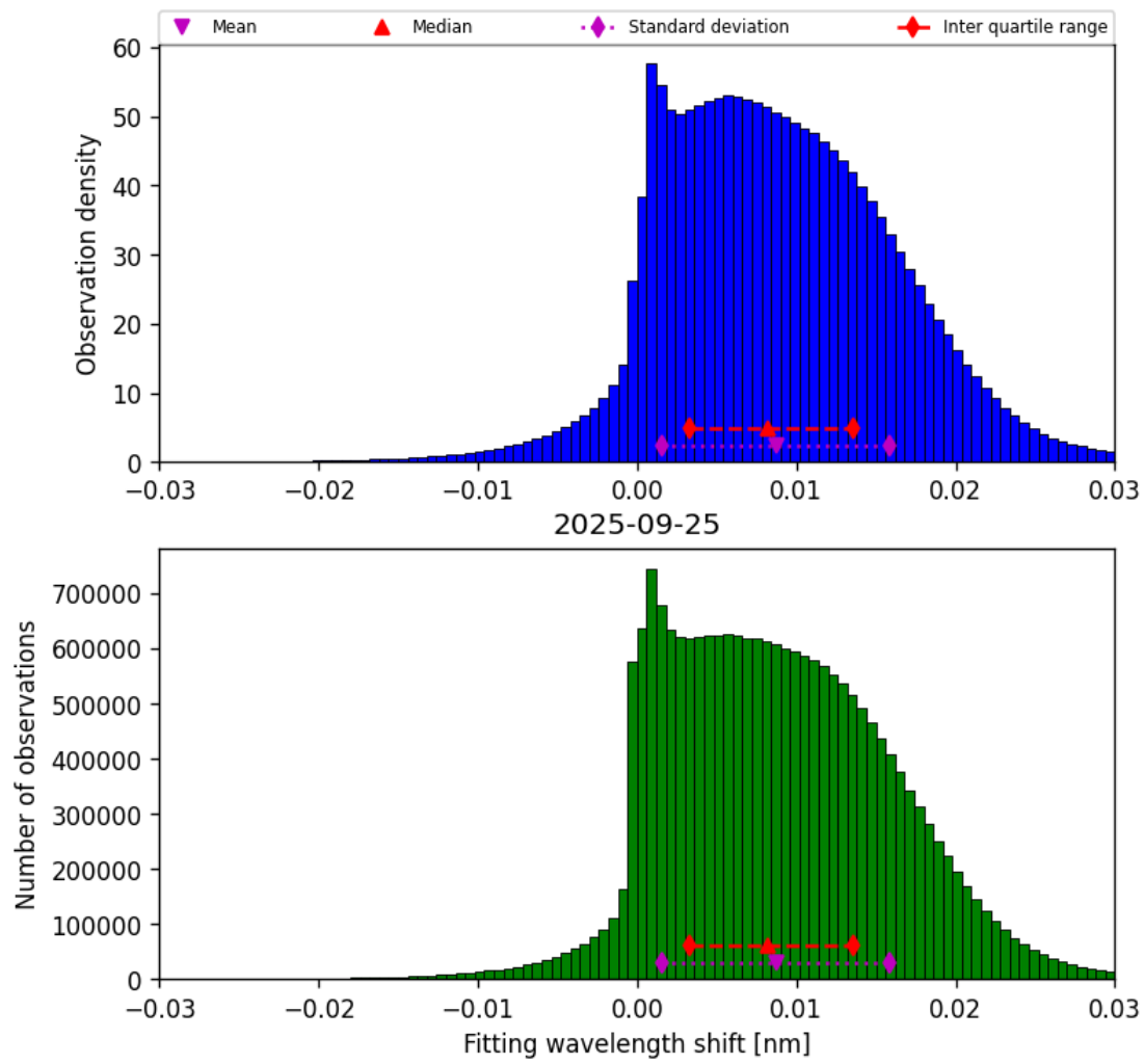
Figure 49: Histogram of “Fitting wavelength shift” for 2025-09-25 to 2025-09-26
