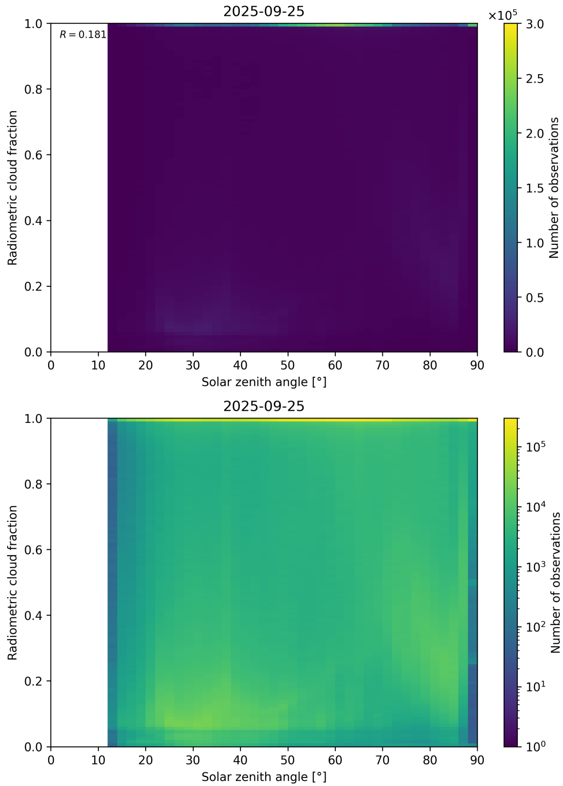
Figure 99: Scatter density plot of “Solar zenith angle” against “Radiometric cloud fraction” for 2025-09-25 to 2025-09-26.
