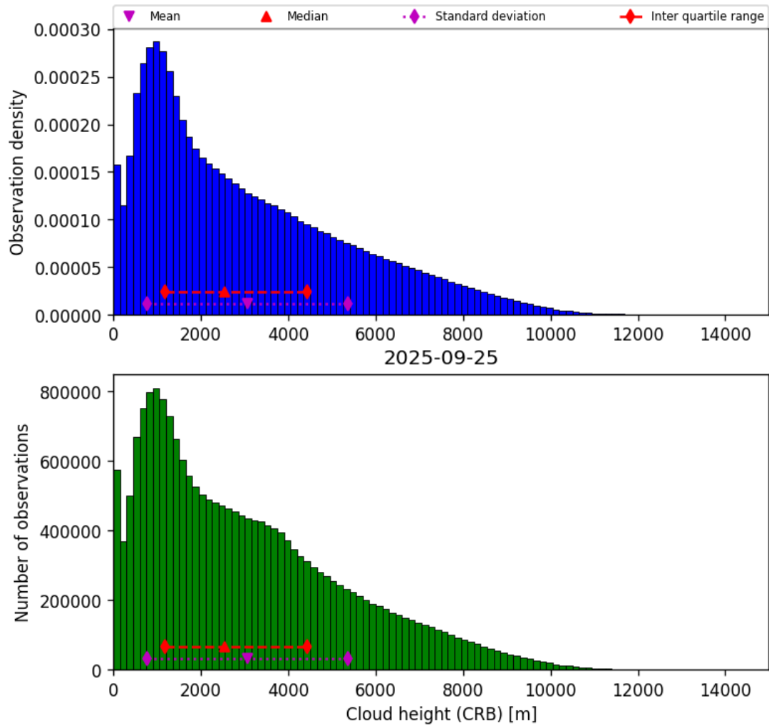
Figure 43: Histogram of “Cloud height (CRB)” for 2025-09-25 to 2025-09-26
