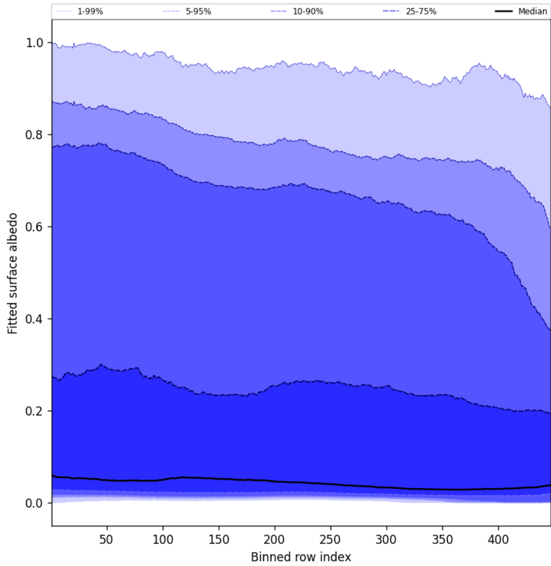
Figure 61: Along track statistics of “Fitted surface albedo” for 2025-09-25 to 2025-09-26
