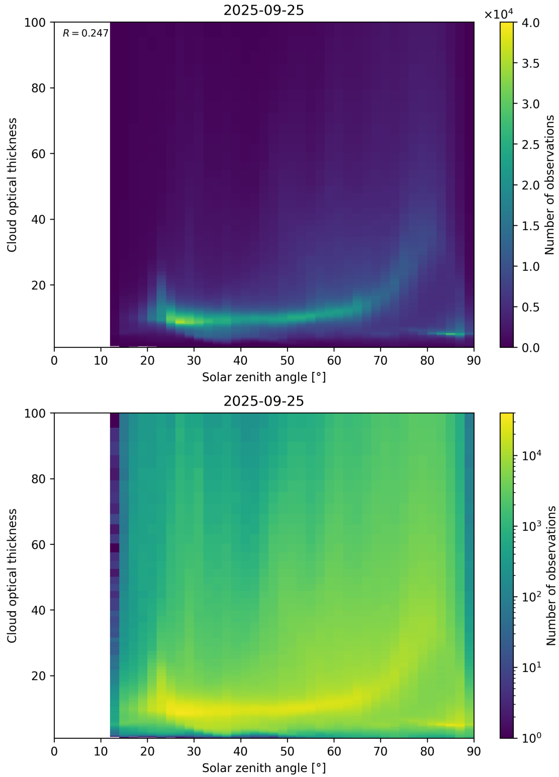
Figure 103: Scatter density plot of “Solar zenith angle” against “Cloud optical thickness” for 2025-09-25 to 2025-09-26.
