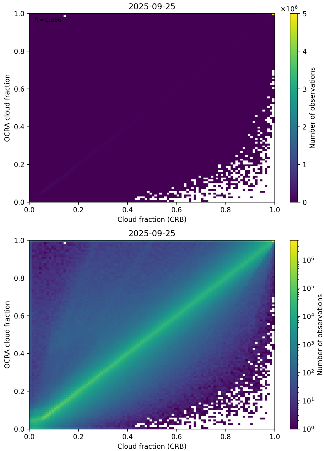
Figure 78: Scatter density plot of “Cloud fraction (CRB)” against “OCRA cloud fraction” for 2025-09-25 to 2025-09-26.
