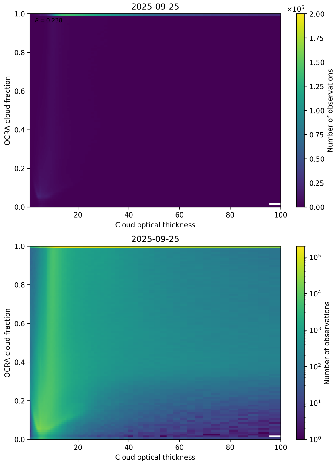
Figure 83: Scatter density plot of “Cloud optical thickness” against “OCRA cloud fraction” for 2025-09-25 to 2025-09-26.
