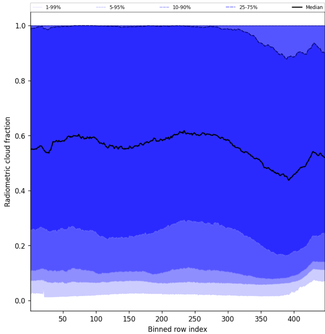
Figure 55: Along track statistics of “Radiometric cloud fraction” for 2025-09-25 to 2025-09-26
