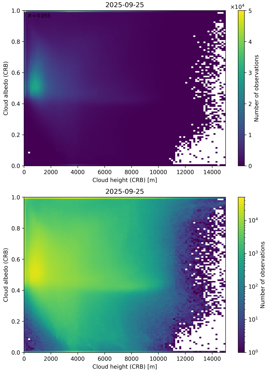
Figure 80: Scatter density plot of “Cloud height (CRB)” against “Cloud albedo (CRB)” for 2025-09-25 to 2025-09-26.
