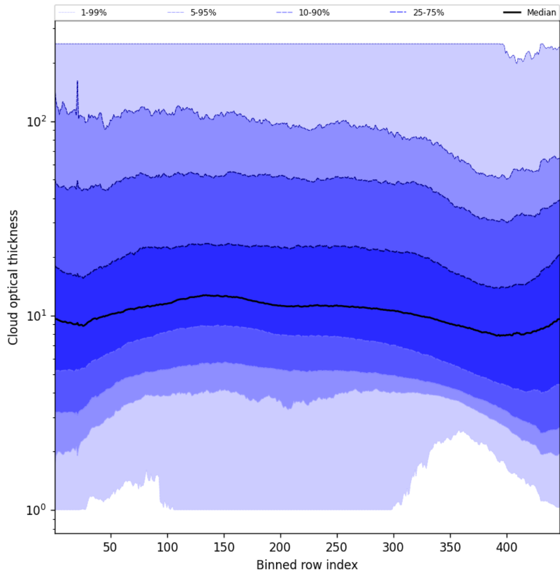
Figure 57: Along track statistics of “Cloud optical thickness” for 2025-09-25 to 2025-09-26
