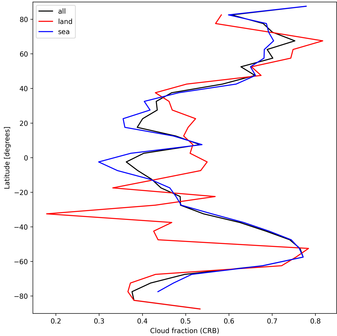
Figure 26: Zonal average of “Cloud fraction (CRB)” for 2025-09-25 to 2025-09-26.
