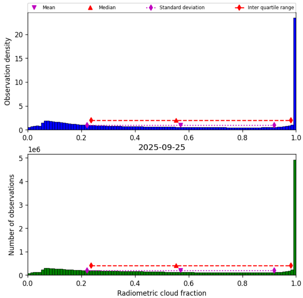
Figure 39: Histogram of “Radiometric cloud fraction” for 2025-09-25 to 2025-09-26
