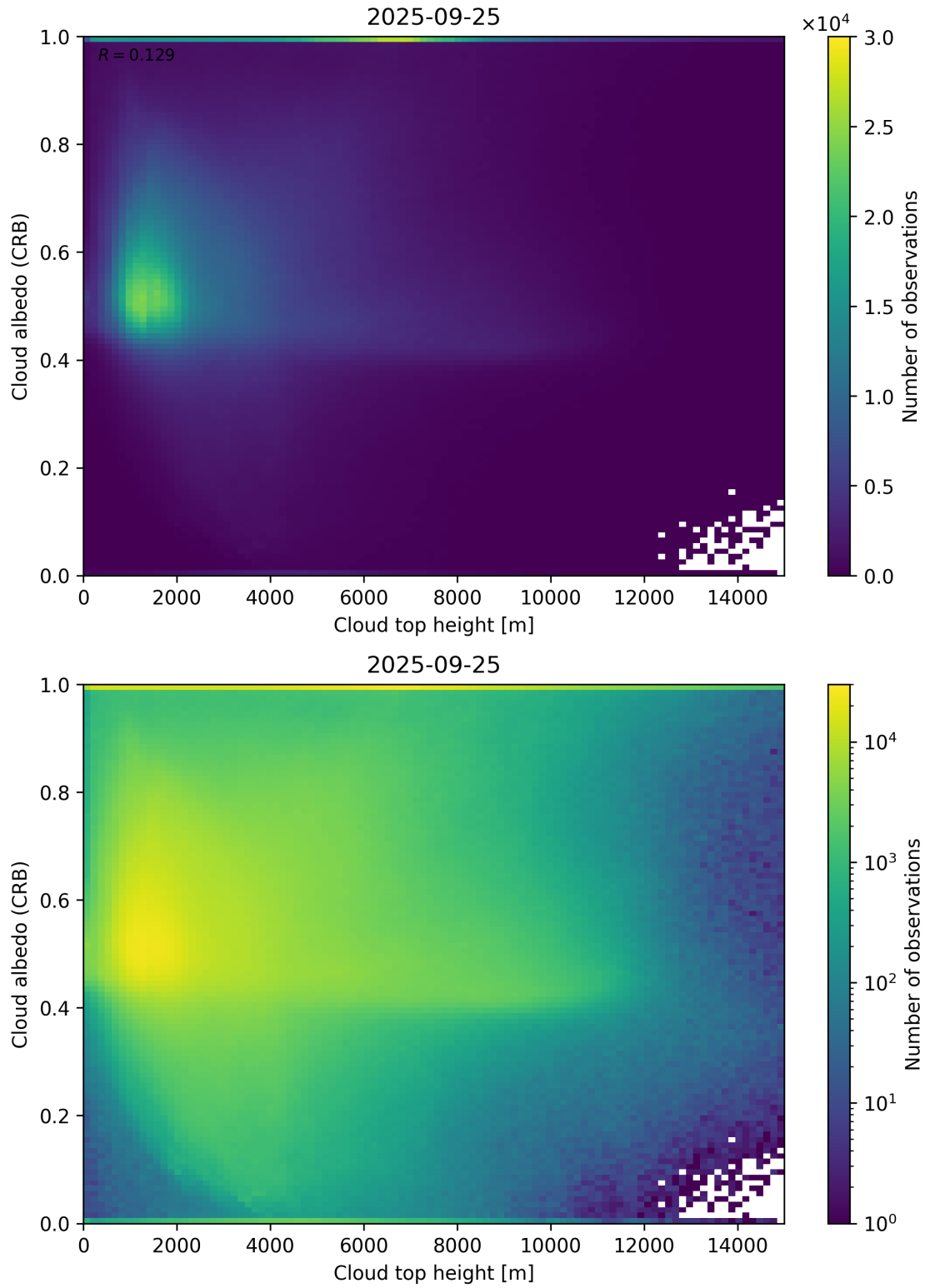
Figure 86: Scatter density plot of “Cloud top height” against “Cloud albedo (CRB)” for 2025-09-25 to 2025-09-26.
