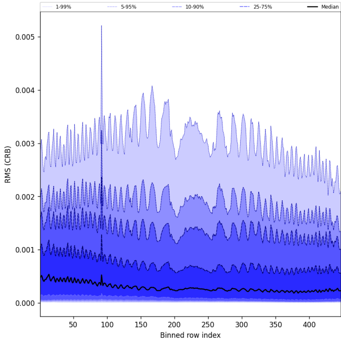
Figure 64: Along track statistics of “RMS (CRB)” for 2025-09-25 to 2025-09-26
