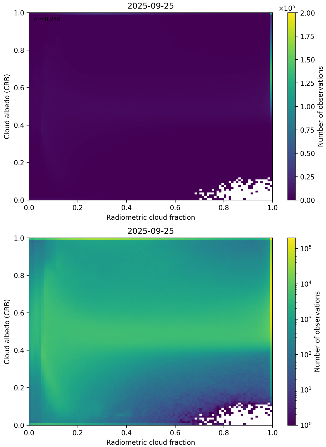
Figure 71: Scatter density plot of “Radiometric cloud fraction” against “Cloud albedo (CRB)” for 2025-09-25 to 2025-09-26.
