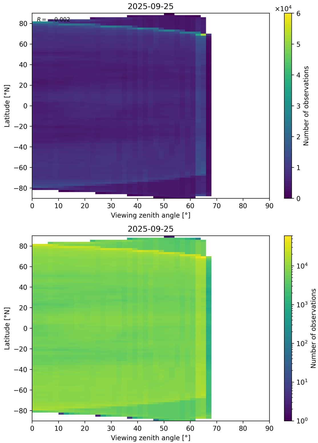
Figure 113: Scatter density plot of “Viewing zenith angle” against “Latitude” for 2025-09-25 to 2025-09-26.
