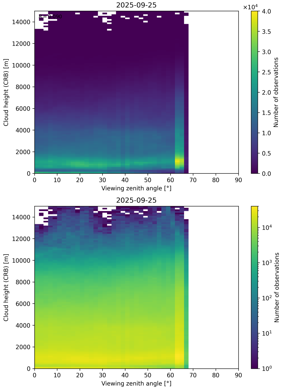
Figure 110: Scatter density plot of “Viewing zenith angle” against “Cloud height (CRB)” for 2025-09-25 to 2025-09-26.
