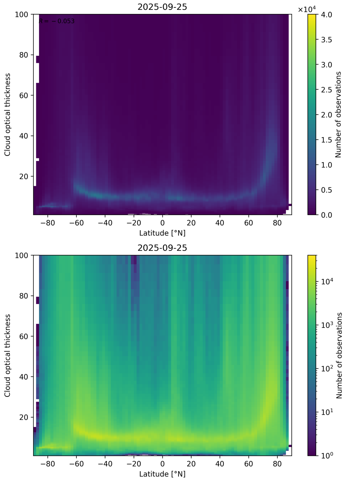
Figure 96: Scatter density plot of “Latitude” against “Cloud optical thickness” for 2025-09-25 to 2025-09-26.
