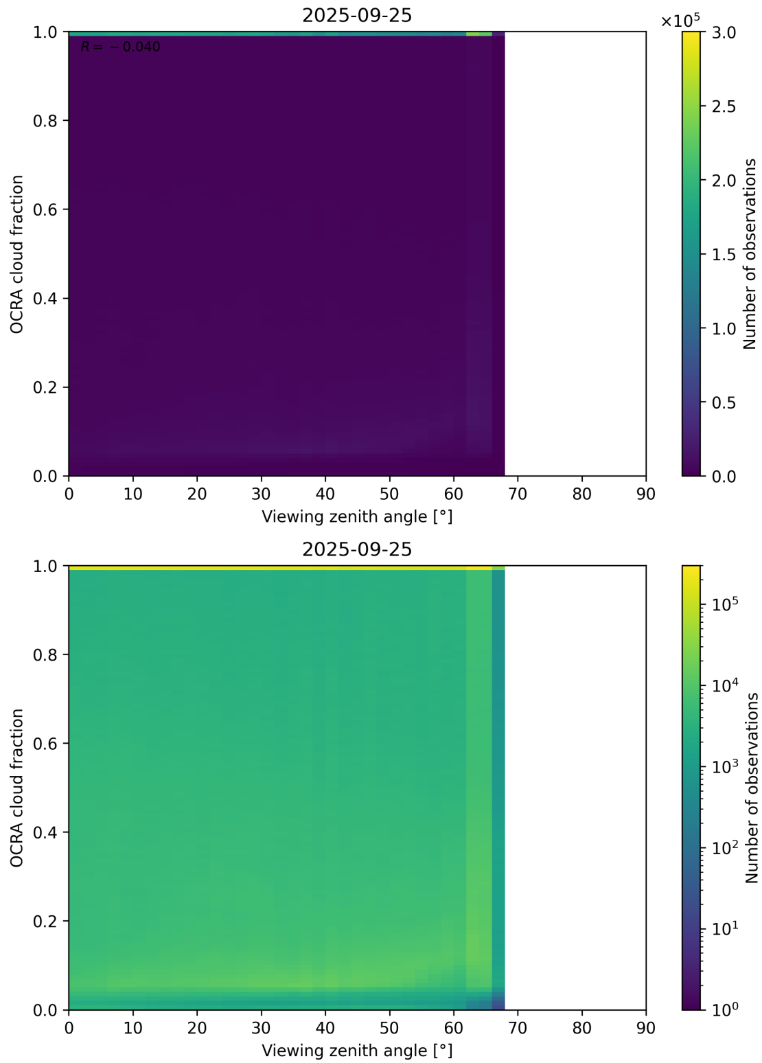
Figure 108: Scatter density plot of “Viewing zenith angle” against “OCRA cloud fraction” for 2025-09-25 to 2025-09-26.
