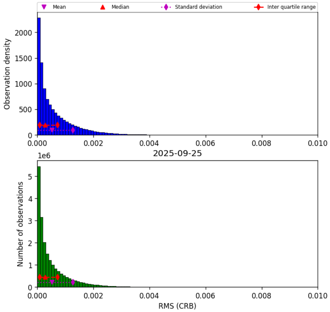
Figure 48: Histogram of “RMS (CRB)” for 2025-09-25 to 2025-09-26
