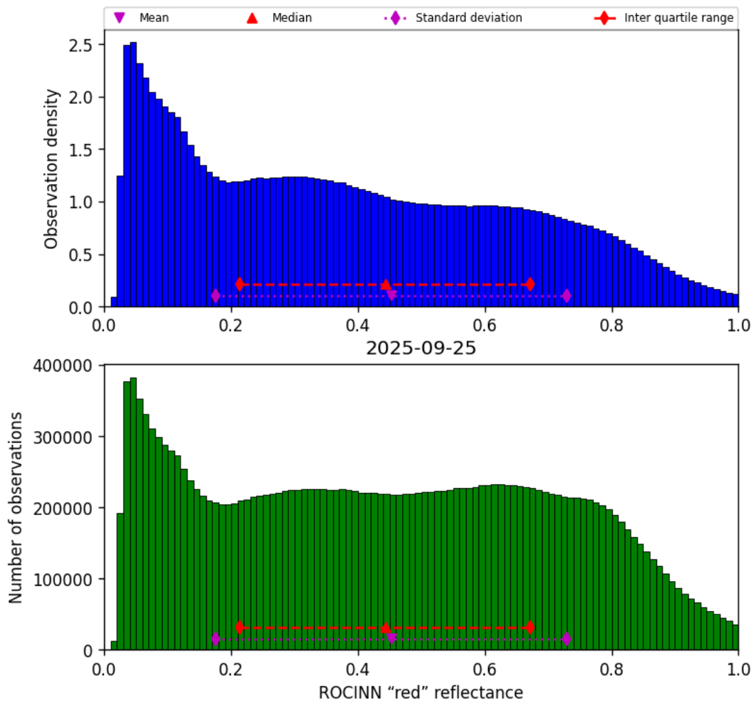
Figure 53: Histogram of “ROCINN “red” reflectance” for 2025-09-25 to 2025-09-26
