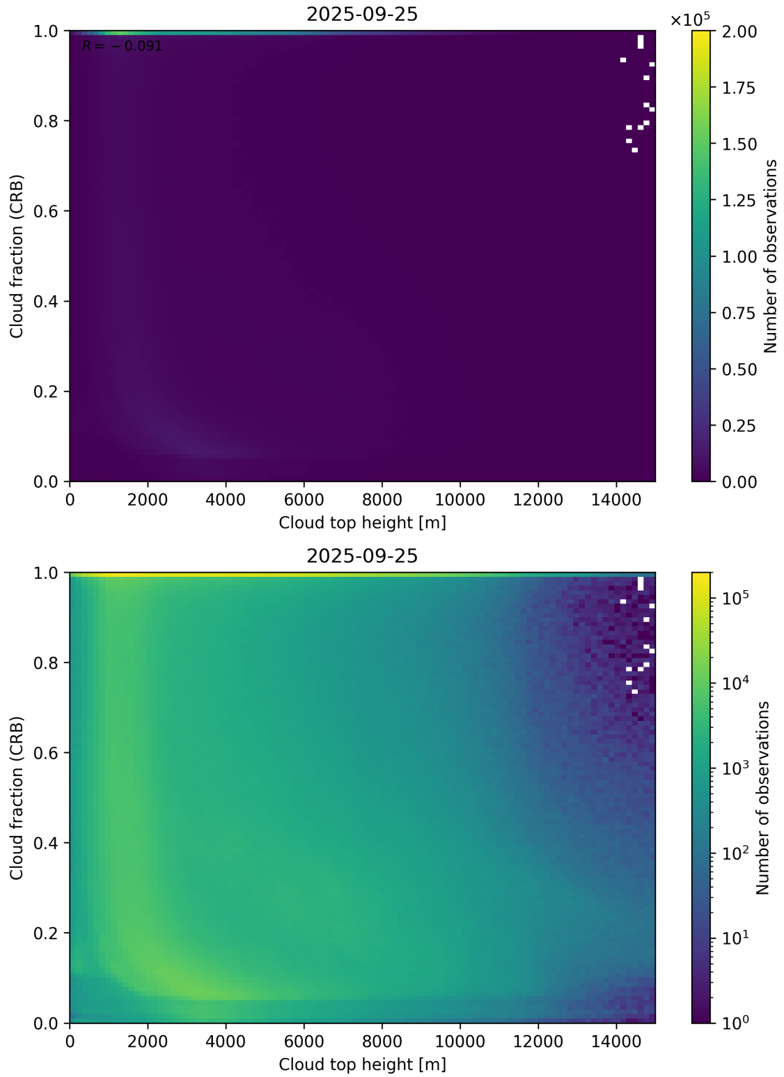
Figure 88: Scatter density plot of “Cloud top height” against “Cloud fraction (CRB)” for 2025-09-25 to 2025-09-26.
