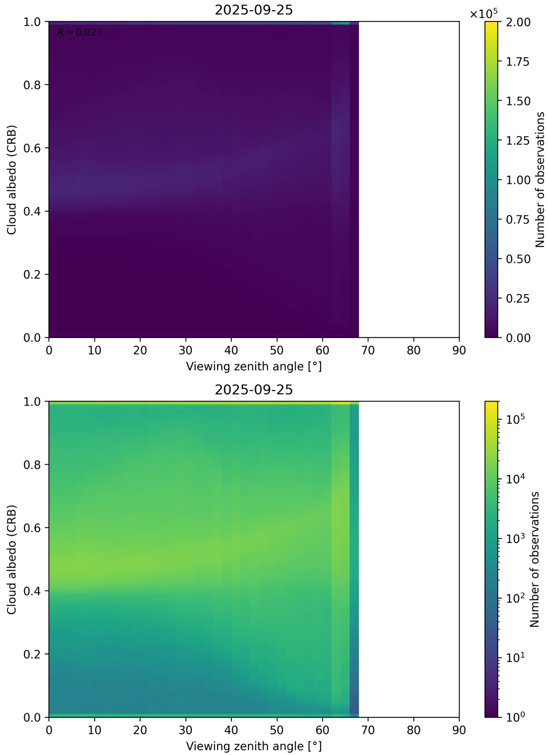
Figure 106: Scatter density plot of “Viewing zenith angle” against “Cloud albedo (CRB)” for 2025-09-25 to 2025-09-26.
