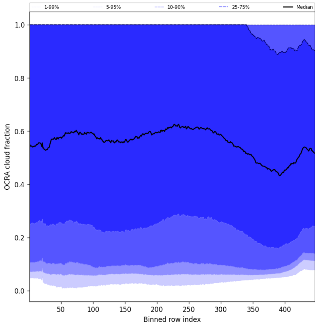
Figure 66: Along track statistics of “OCRA cloud fraction” for 2025-09-25 to 2025-09-26
