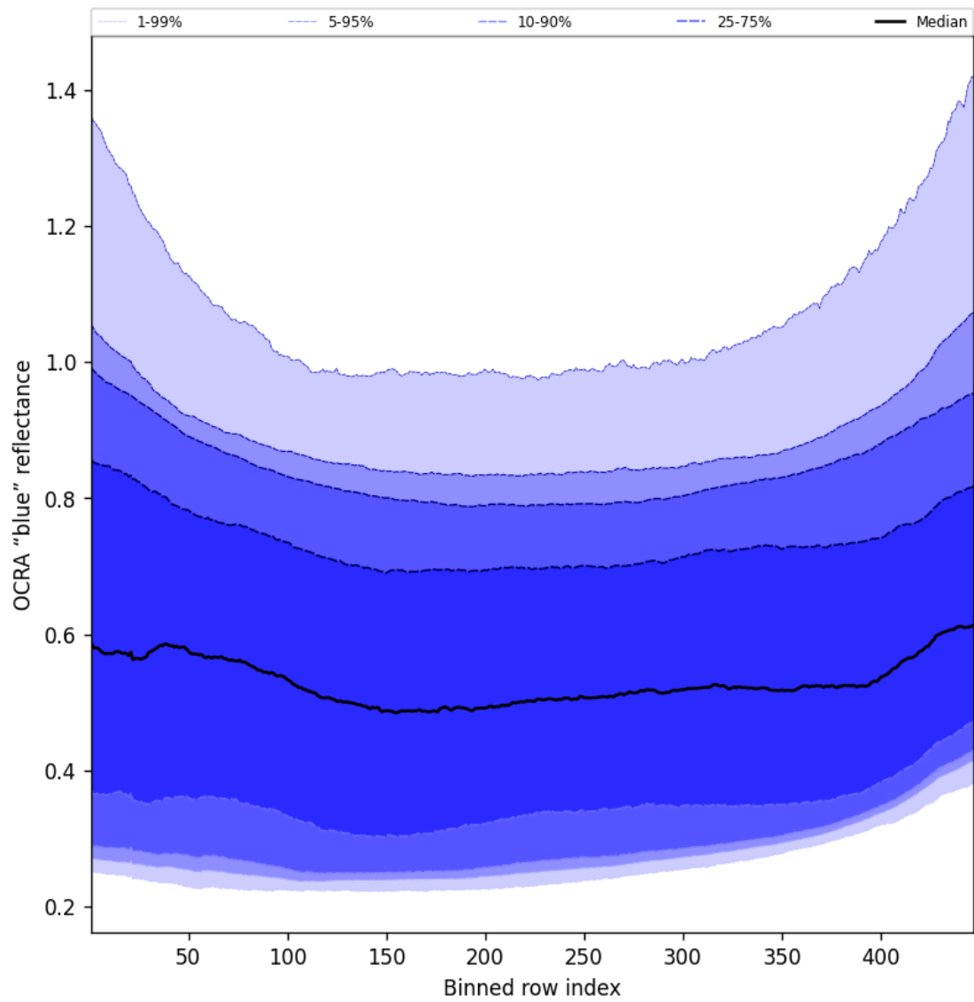
Figure 67: Along track statistics of “OCRA “blue” reflectance” for 2025-09-25 to 2025-09-26
