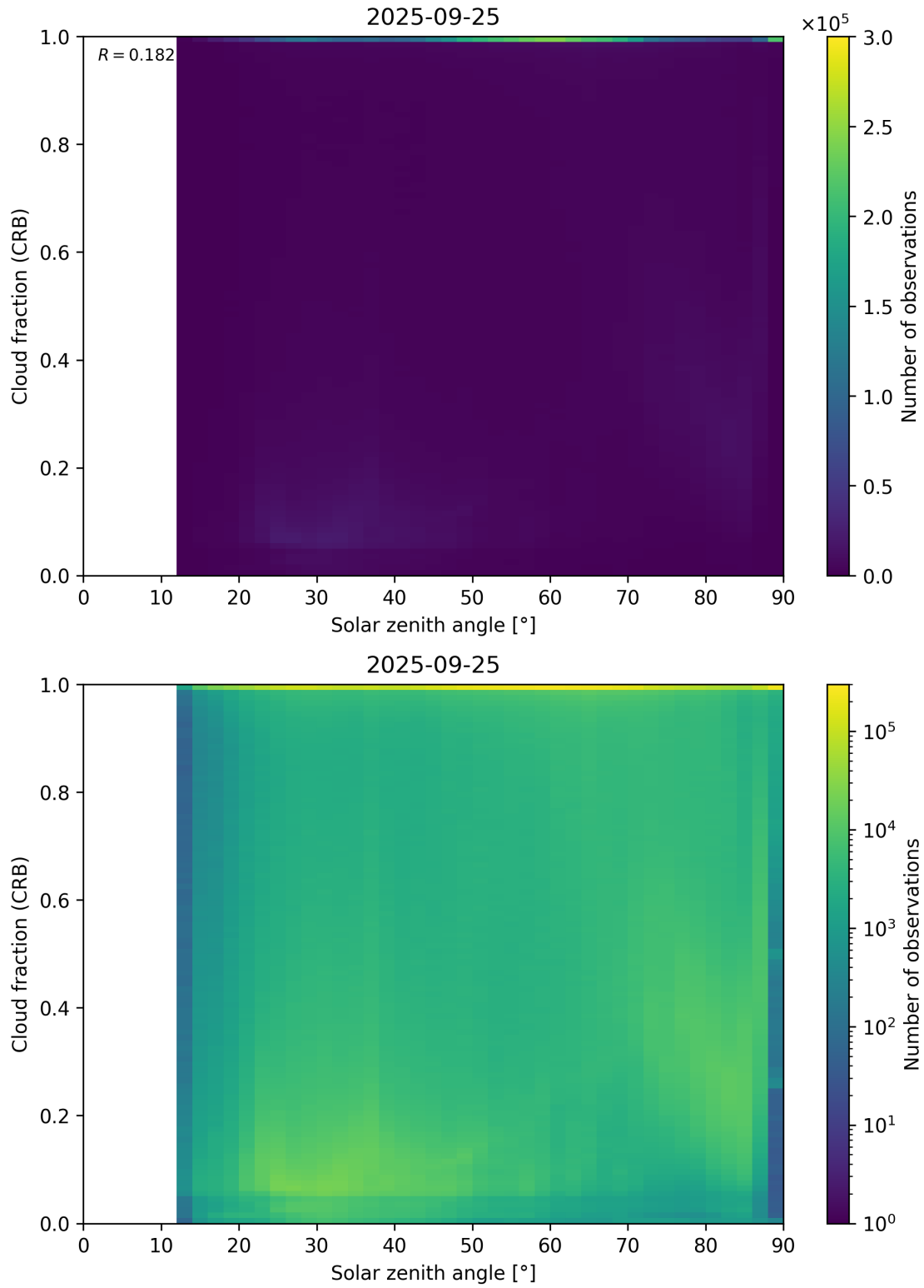
Figure 101: Scatter density plot of “Solar zenith angle” against “Cloud fraction (CRB)” for 2025-09-25 to 2025-09-26.
