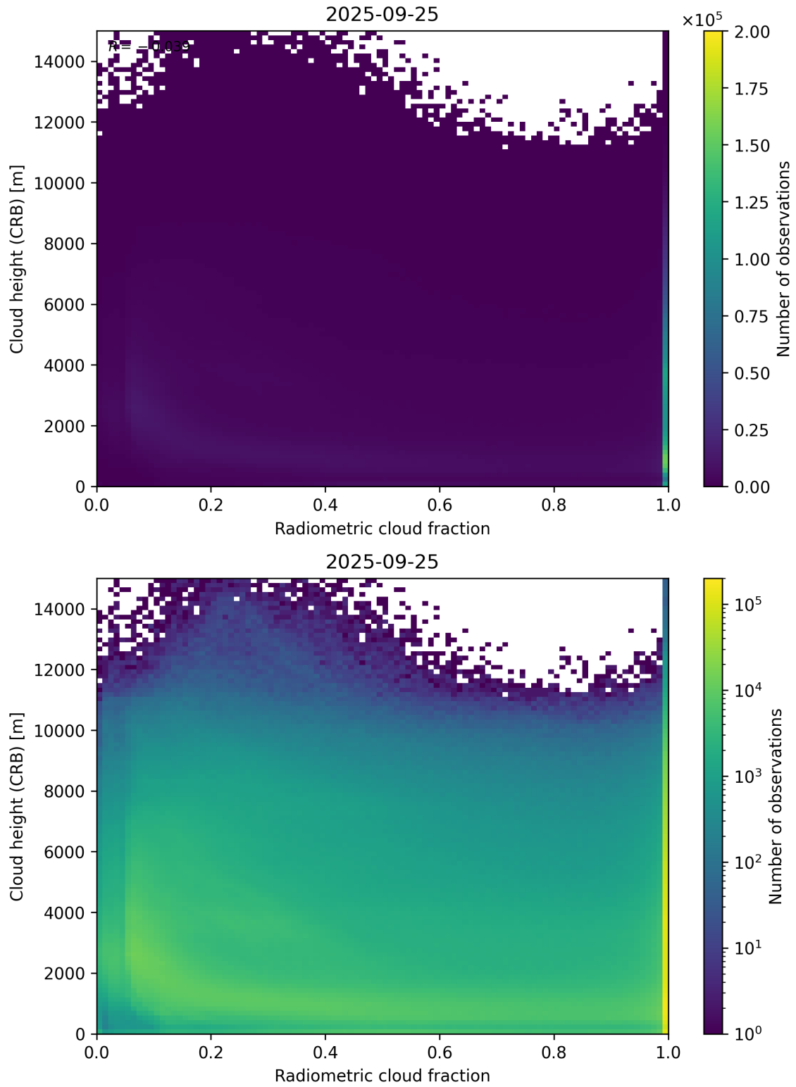
Figure 74: Scatter density plot of “Radiometric cloud fraction” against “Cloud height (CRB)” for 2025-09-25 to 2025-09-26.
