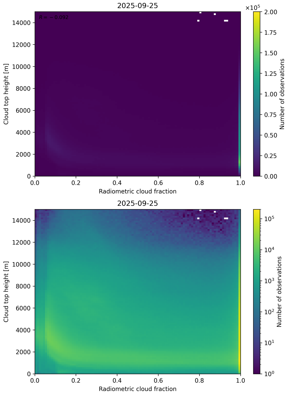
Figure 76: Scatter density plot of “Radiometric cloud fraction” against “Cloud top height” for 2025-09-25 to 2025-09-26.
