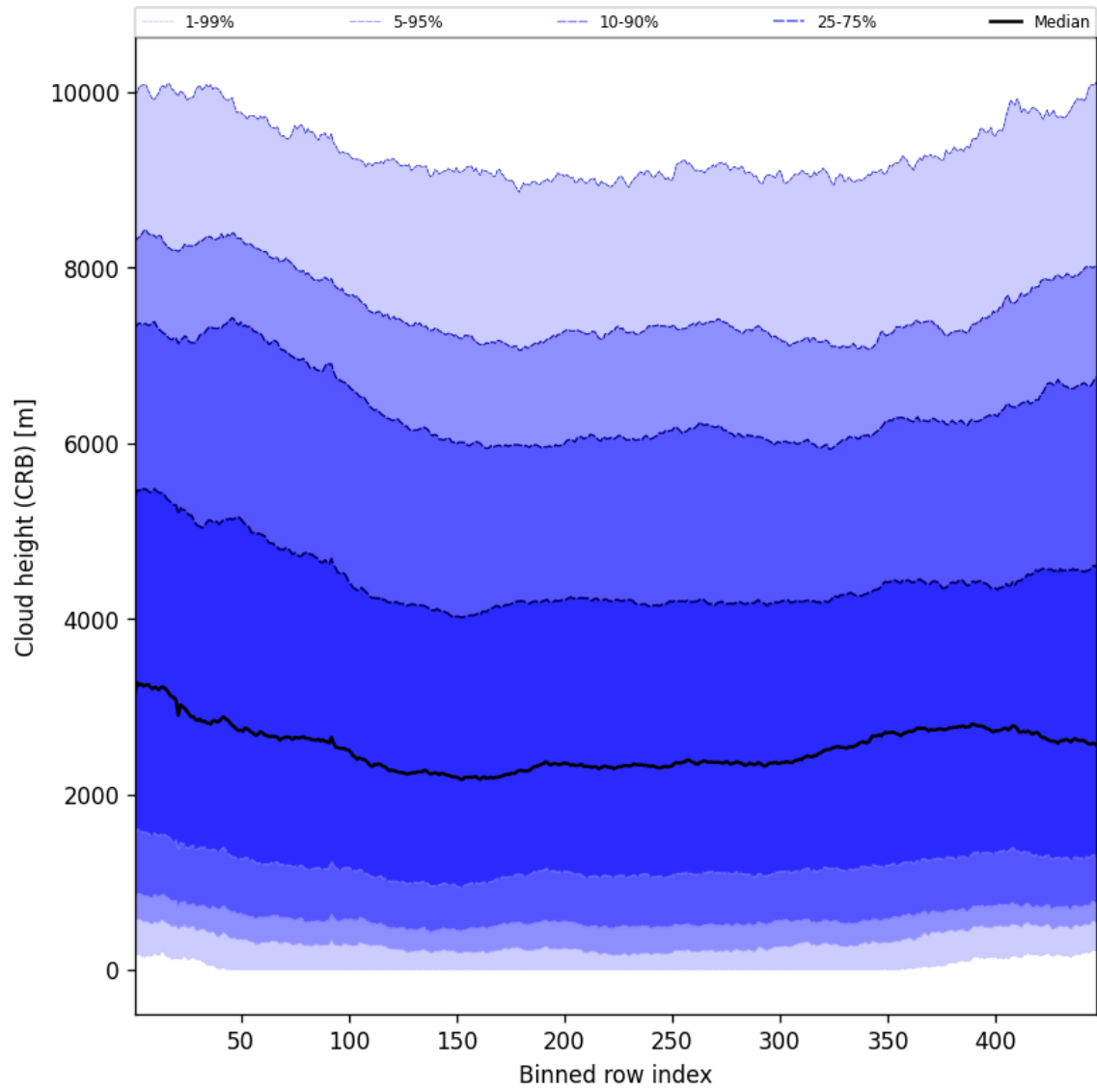
Figure 59: Along track statistics of “Cloud height (CRB)” for 2025-09-25 to 2025-09-26
