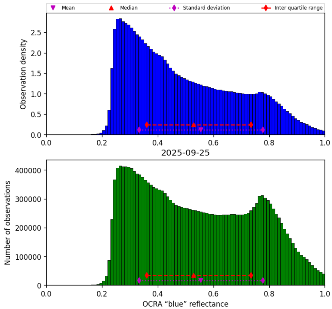
Figure 51: Histogram of “OCRA “blue” reflectance” for 2025-09-25 to 2025-09-26
