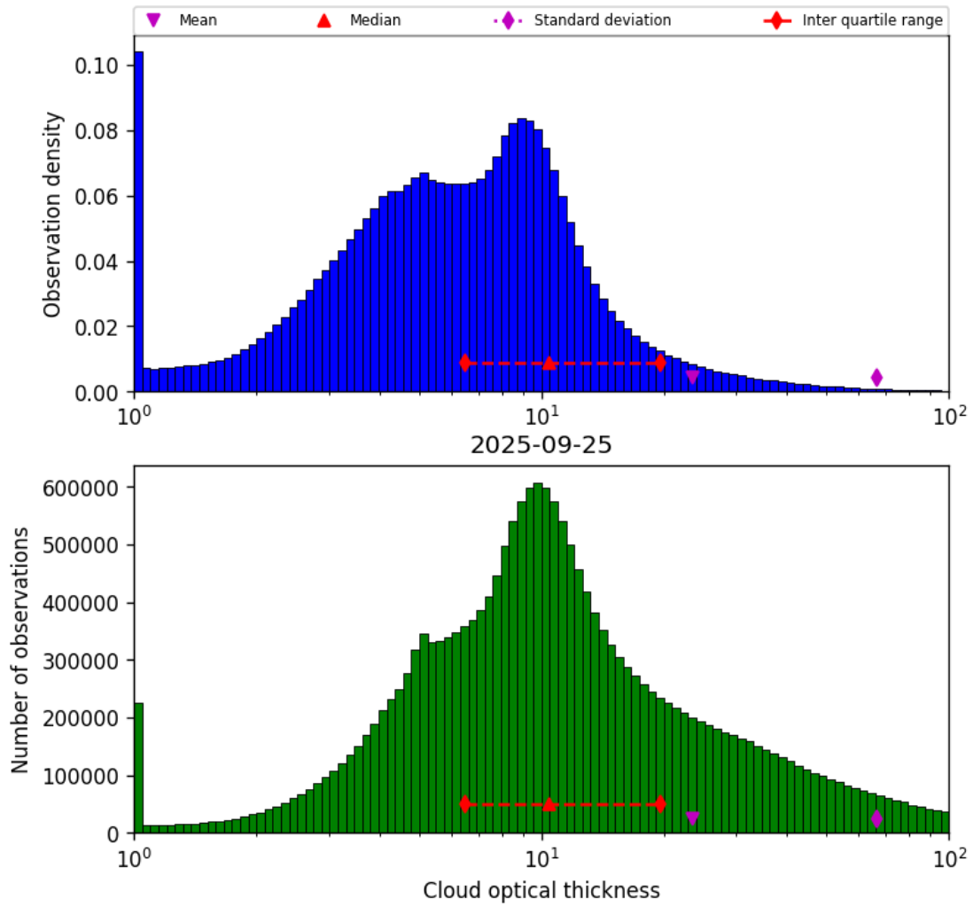
Figure 41: Histogram of “Cloud optical thickness” for 2025-09-25 to 2025-09-26
