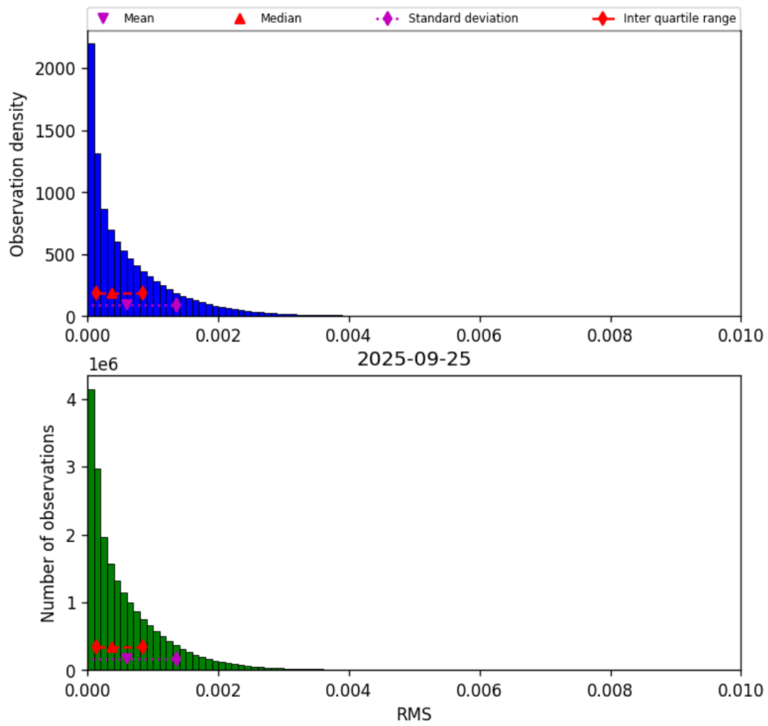
Figure 47: Histogram of “RMS” for 2025-09-25 to 2025-09-26
