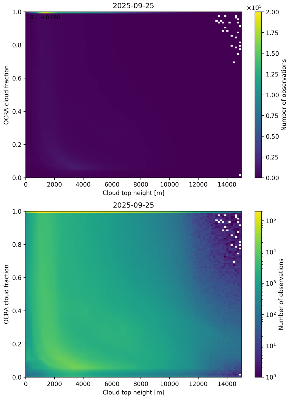
Figure 87: Scatter density plot of “Cloud top height” against “OCRA cloud fraction” for 2025-09-25 to 2025-09-26.
