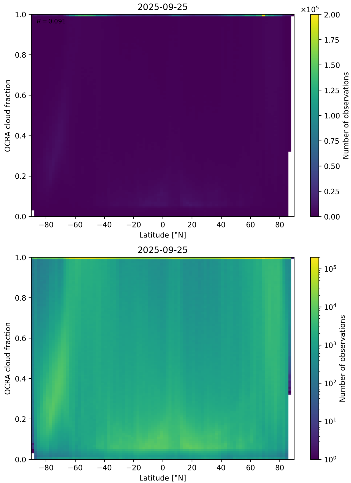
Figure 93: Scatter density plot of “Latitude” against “OCRA cloud fraction” for 2025-09-25 to 2025-09-26.
