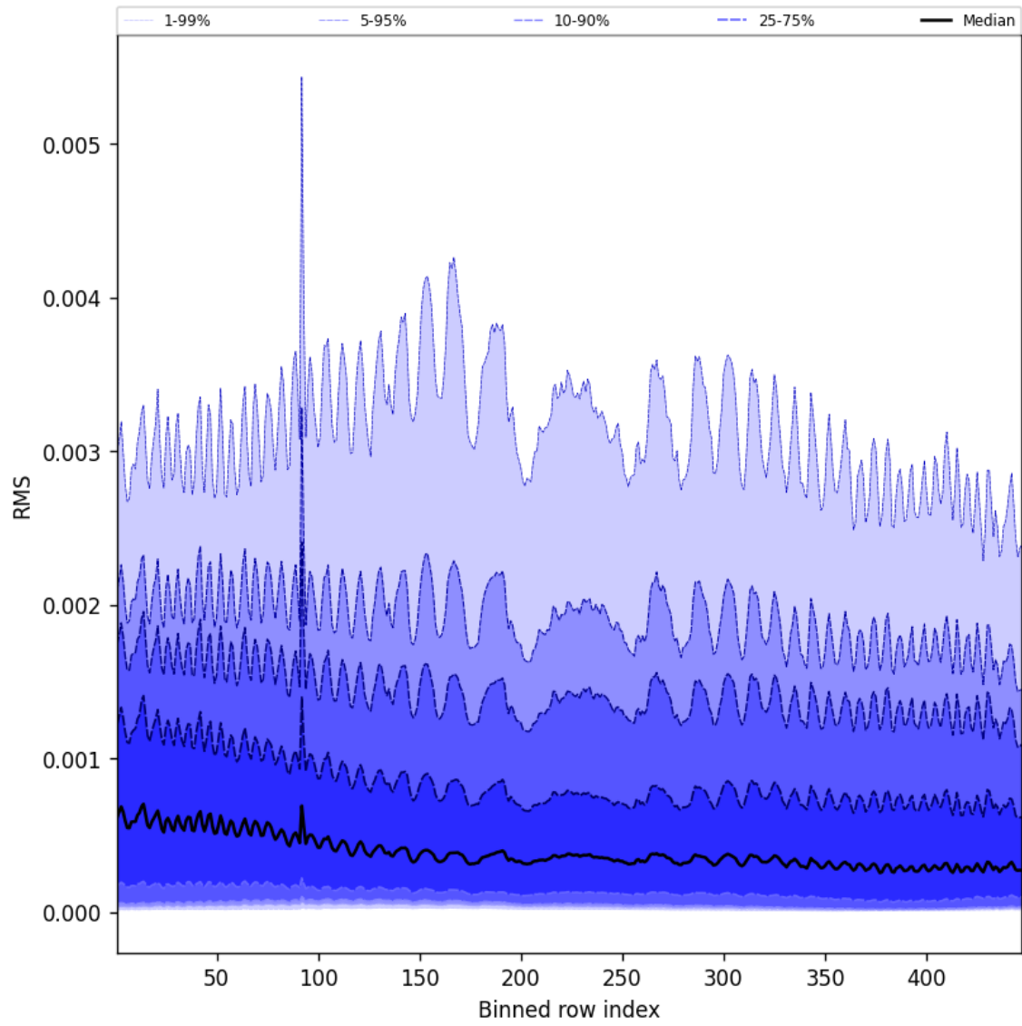
Figure 63: Along track statistics of “RMS” for 2025-09-25 to 2025-09-26
