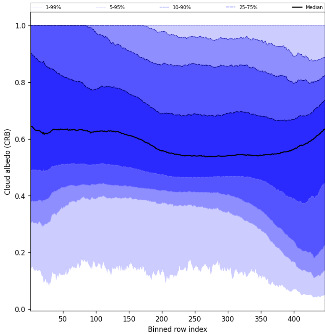
Figure 60: Along track statistics of “Cloud albedo (CRB)” for 2025-09-25 to 2025-09-26
