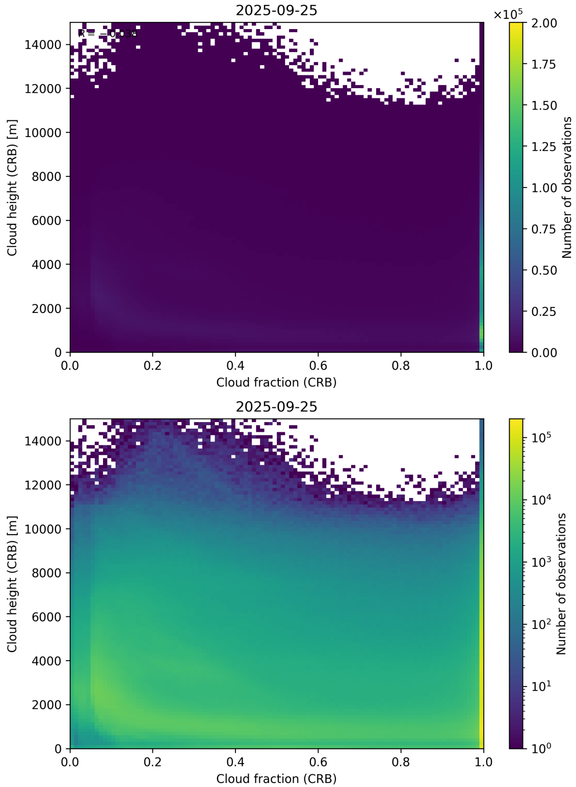
Figure 79: Scatter density plot of “Cloud fraction (CRB)” against “Cloud height (CRB)” for 2025-09-25 to 2025-09-26.
