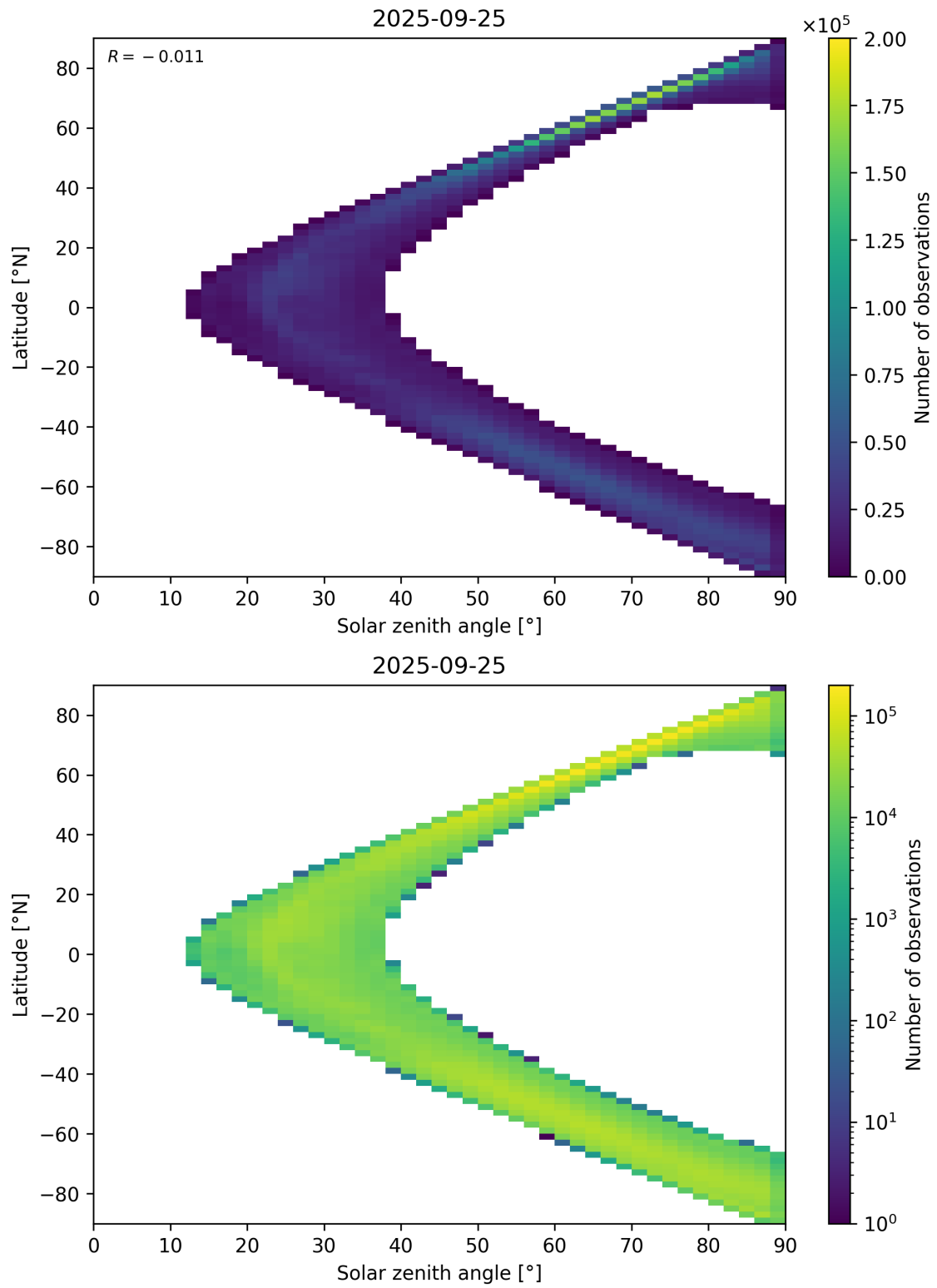
Figure 105: Scatter density plot of “Solar zenith angle” against “Latitude” for 2025-09-25 to 2025-09-26.
