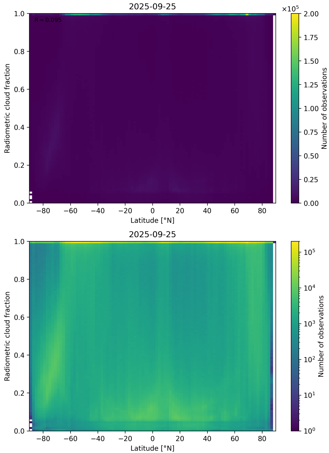
Figure 92: Scatter density plot of “Latitude” against “Radiometric cloud fraction” for 2025-09-25 to 2025-09-26.
