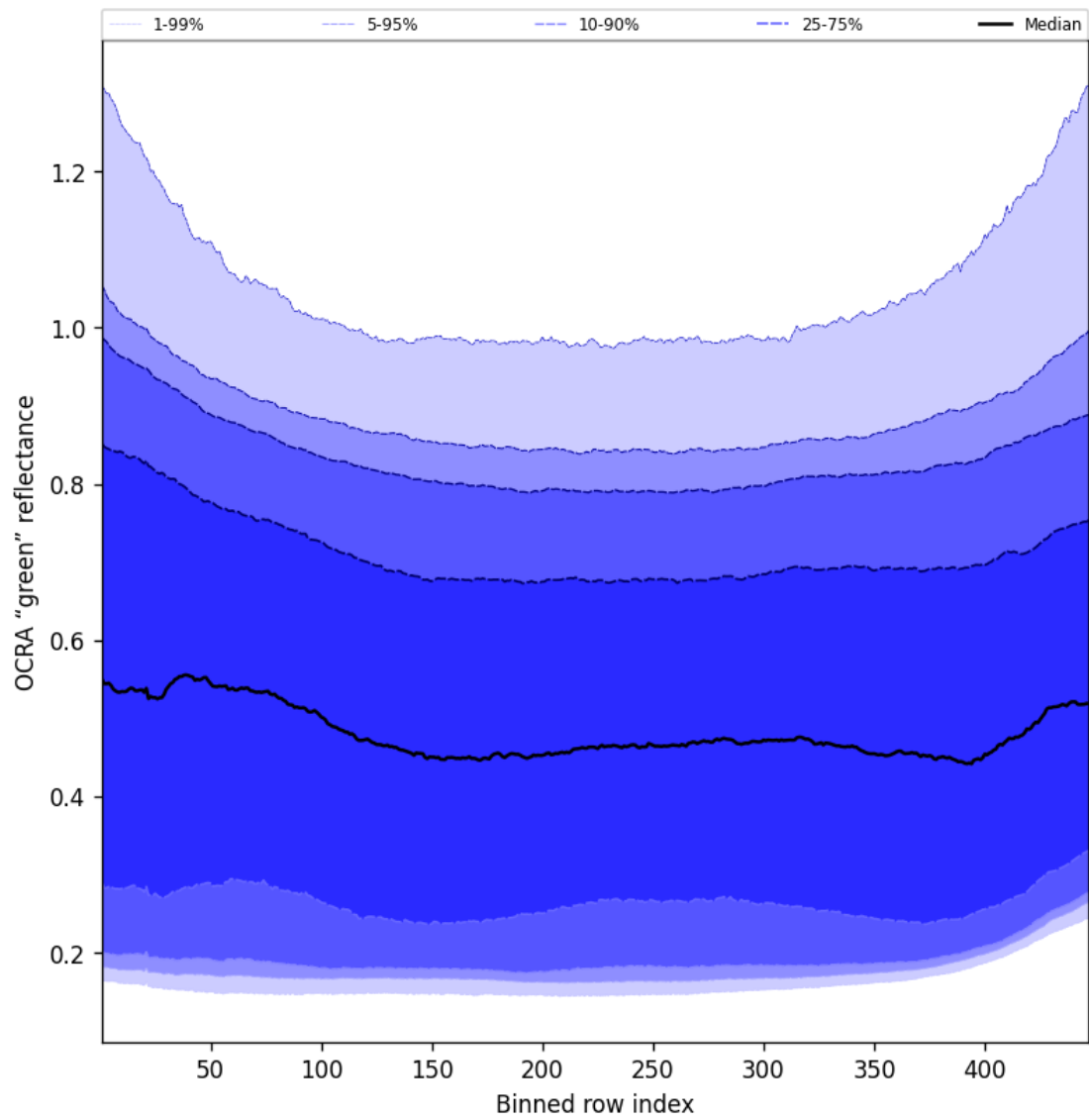
Figure 68: Along track statistics of “OCRA “green” reflectance” for 2025-09-25 to 2025-09-26
