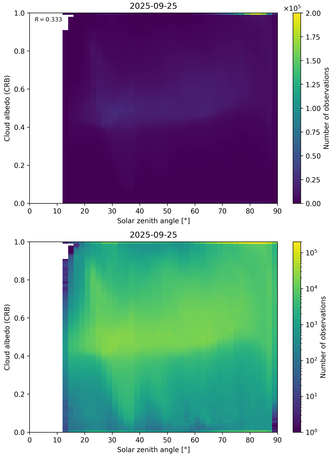
Figure 98: Scatter density plot of “Solar zenith angle” against “Cloud albedo (CRB)” for 2025-09-25 to 2025-09-26.
