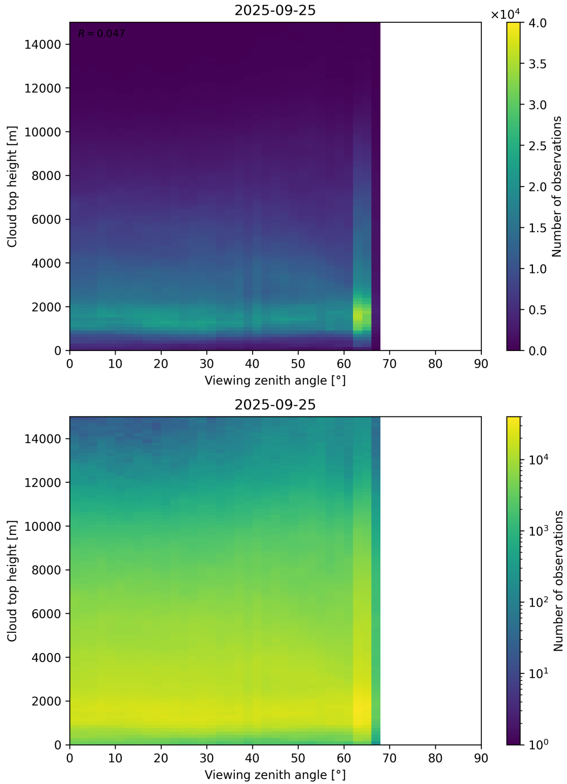
Figure 112: Scatter density plot of “Viewing zenith angle” against “Cloud top height” for 2025-09-25 to 2025-09-26.
