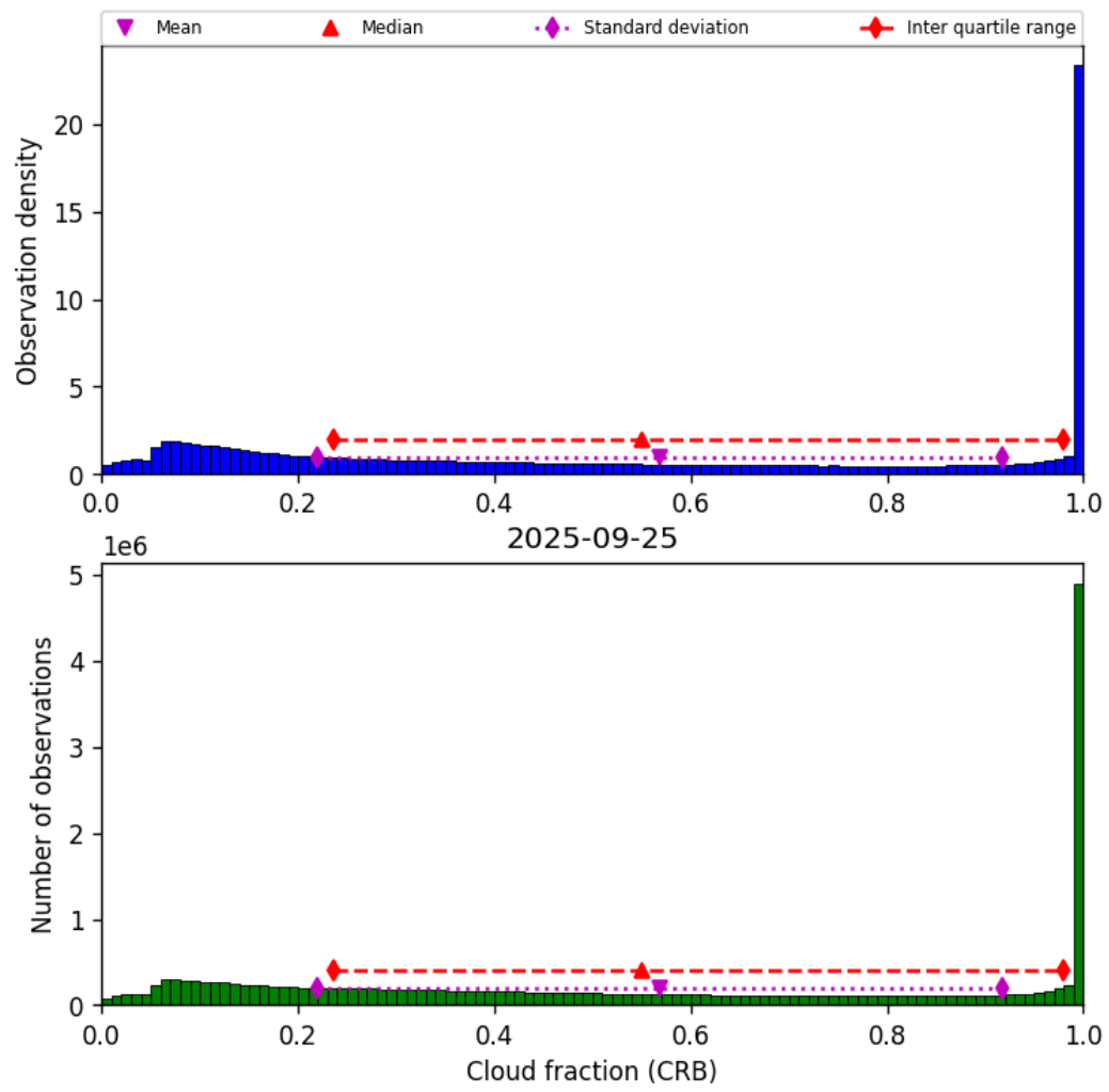
Figure 42: Histogram of "Cloud fraction (CRB)" for 2025-09-25 to 2025-09-26
