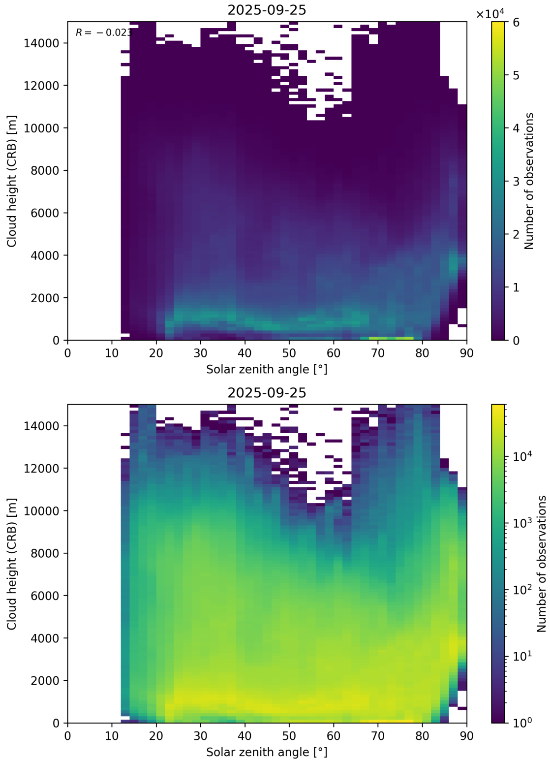
Figure 102: Scatter density plot of “Solar zenith angle” against “Cloud height (CRB)” for 2025-09-25 to 2025-09-26.
