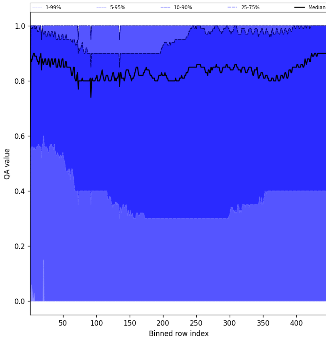
Figure 54: Along track statistics of “QA value” for 2025-09-25 to 2025-09-26
