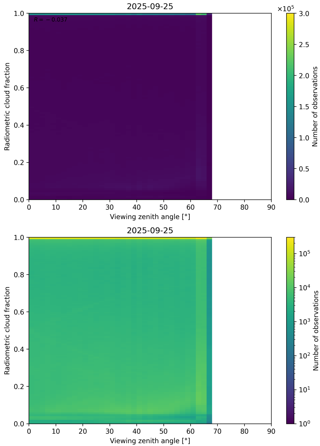
Figure 107: Scatter density plot of “Viewing zenith angle” against “Radiometric cloud fraction” for 2025-09-25 to 2025-09-26.
