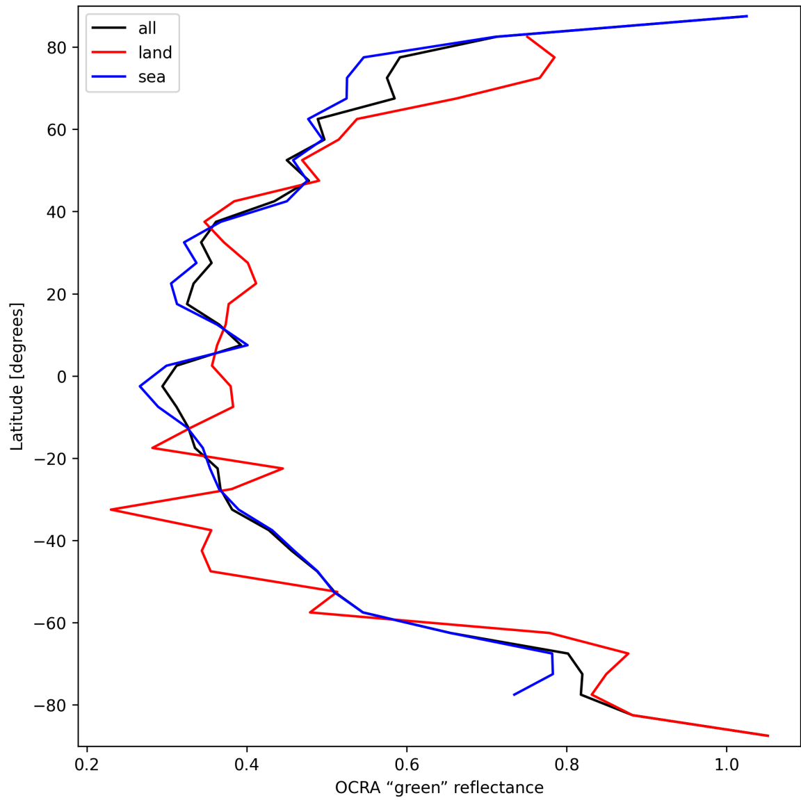
Figure 36: Zonal average of “OCRA “green” reflectance” for 2025-09-25 to 2025-09-26.
