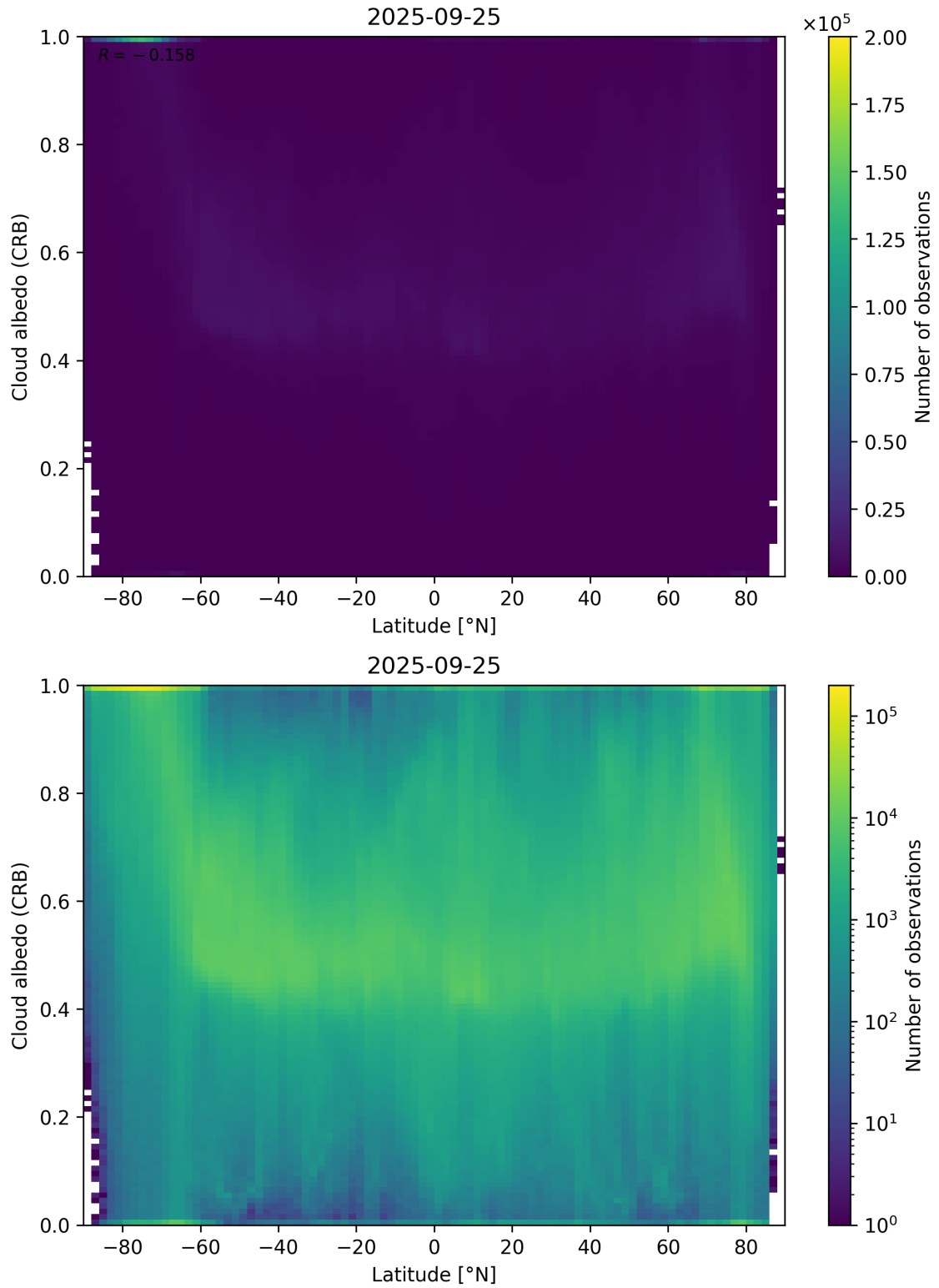
Figure 91: Scatter density plot of “Latitude” against “Cloud albedo (CRB)” for 2025-09-25 to 2025-09-26.
