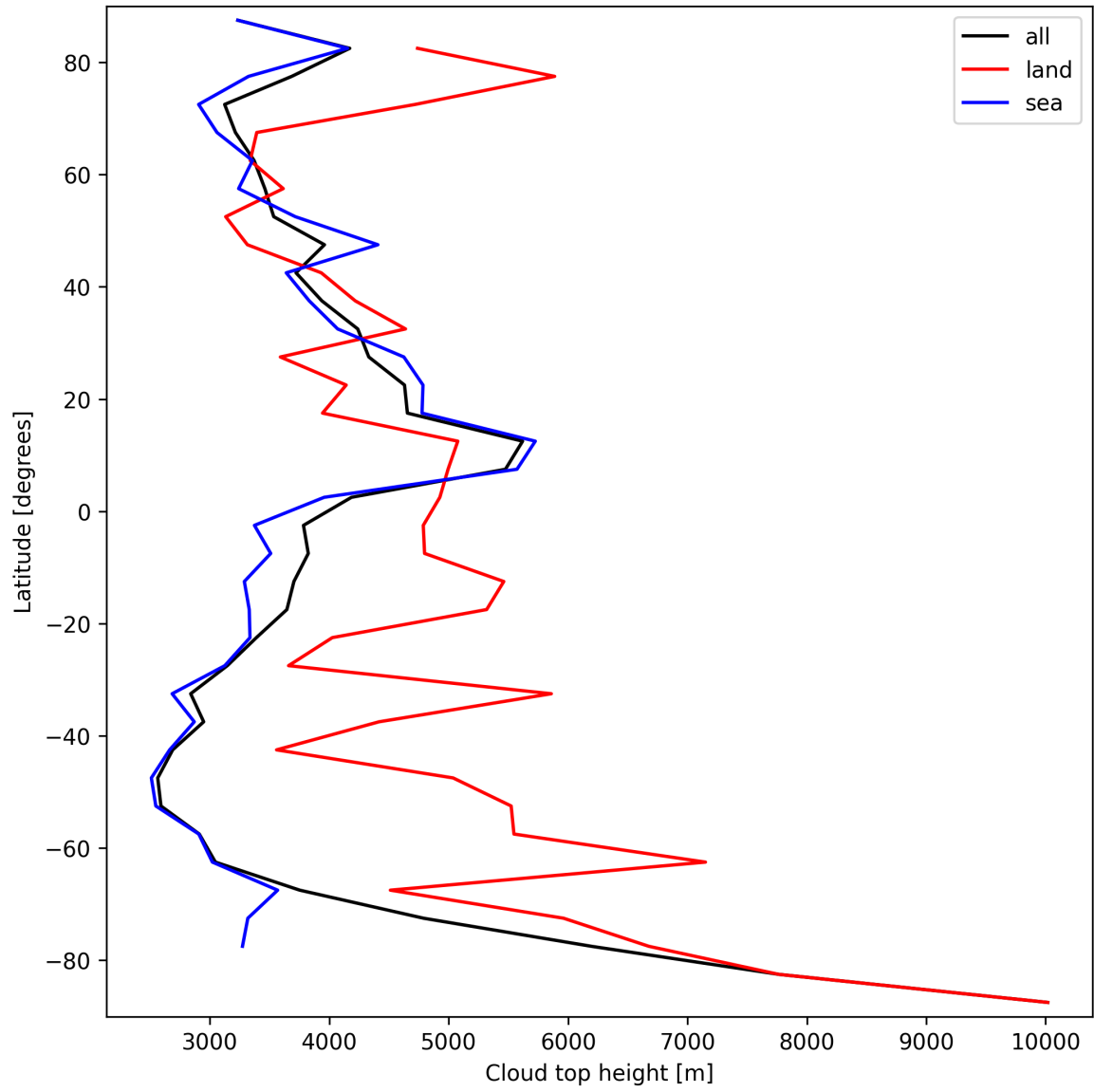
Figure 24: Zonal average of “Cloud top height” for 2025-09-25 to 2025-09-26.
