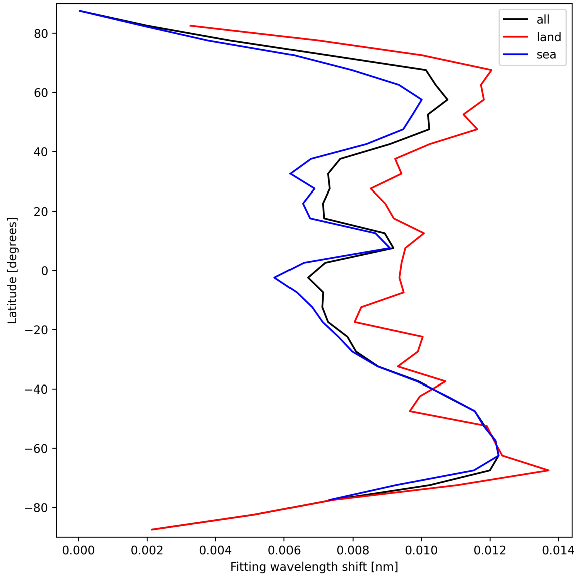
Figure 33: Zonal average of “Fitting wavelength shift” for 2025-09-25 to 2025-09-26.
