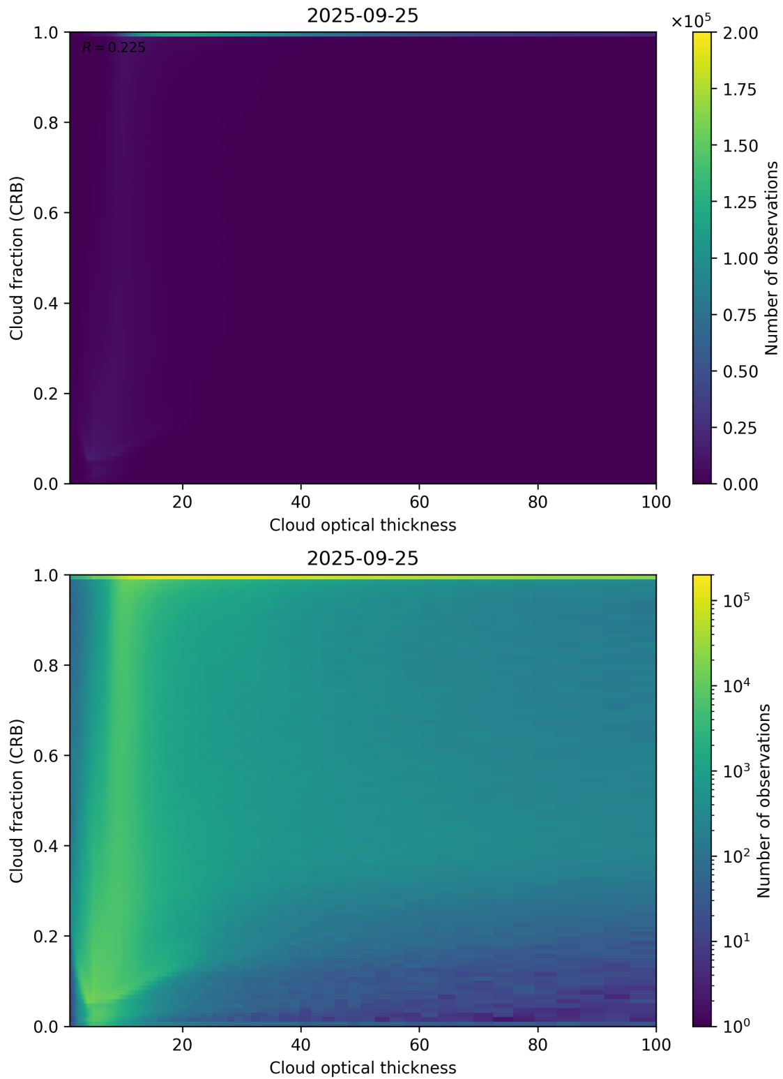
Figure 84: Scatter density plot of “Cloud optical thickness” against “Cloud fraction (CRB)” for 2025-09-25 to 2025-09-26.
