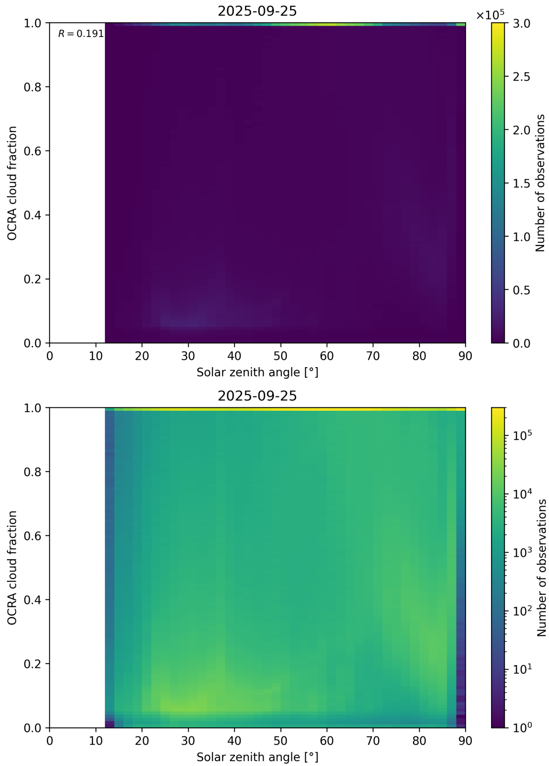
Figure 100: Scatter density plot of “Solar zenith angle” against “OCRA cloud fraction” for 2025-09-25 to 2025-09-26.
