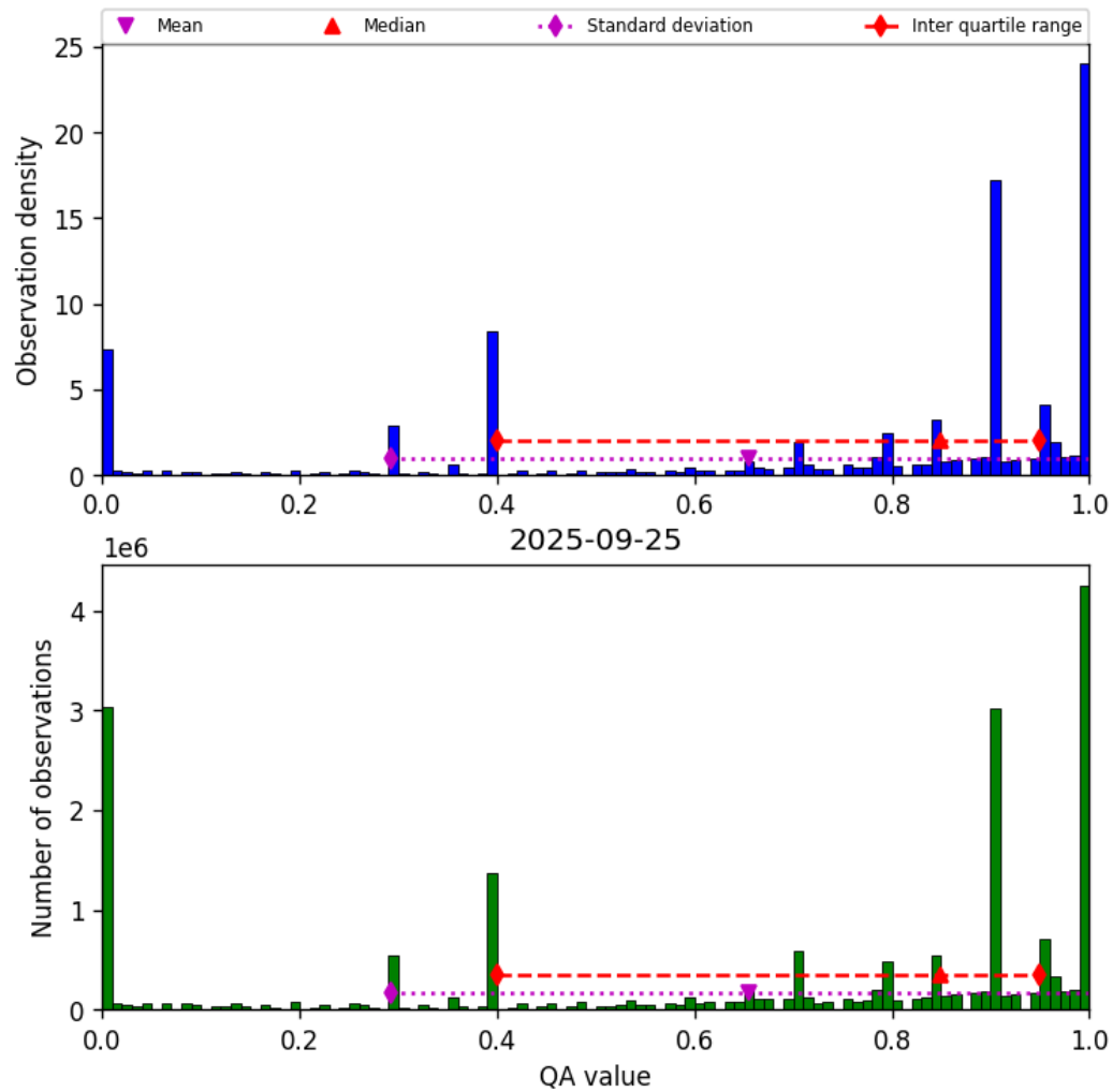
Figure 38: Histogram of “QA value” for 2025-09-25 to 2025-09-26
