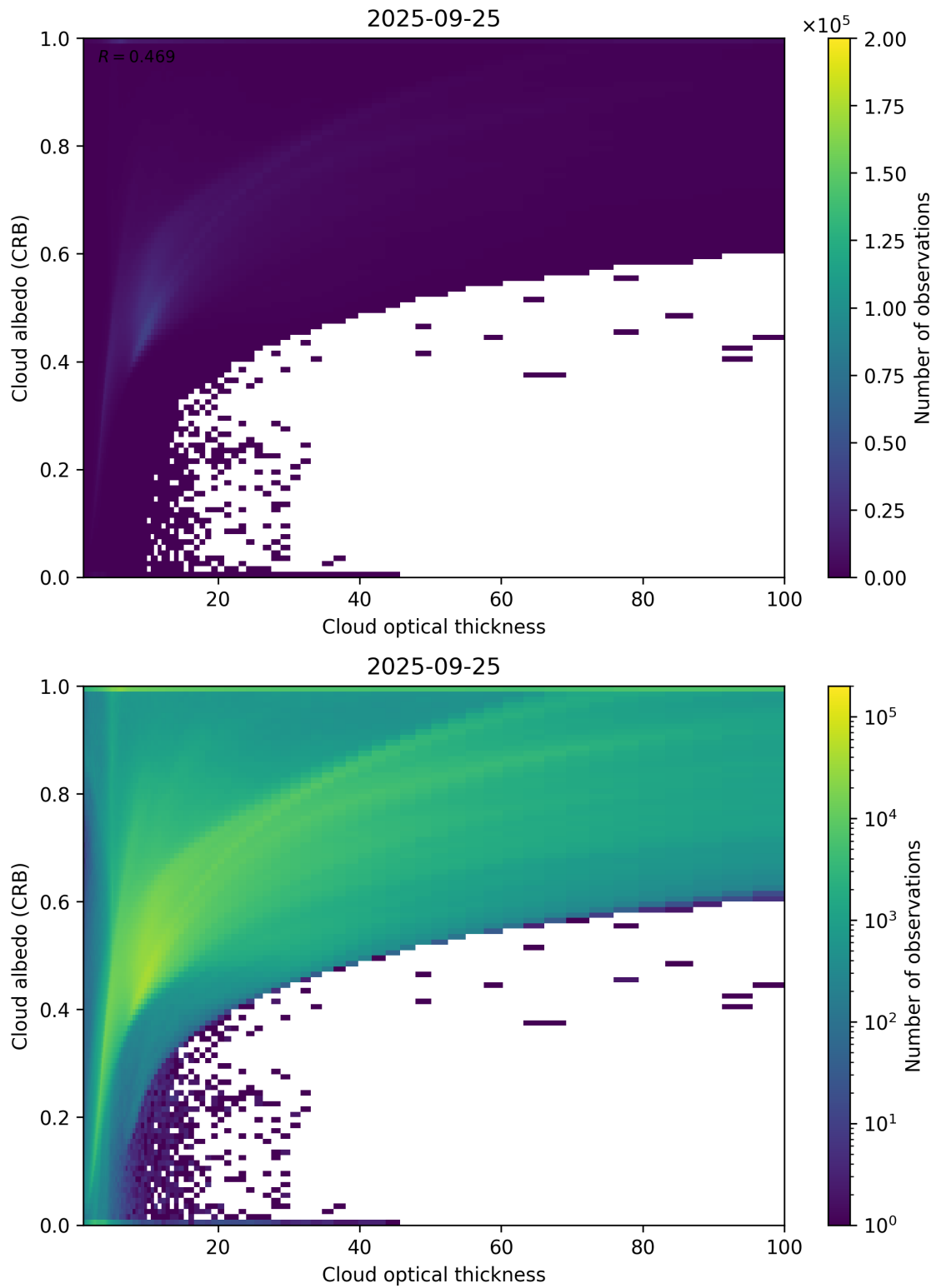
Figure 82: Scatter density plot of “Cloud optical thickness” against “Cloud albedo (CRB)” for 2025-09-25 to 2025-09-26.
