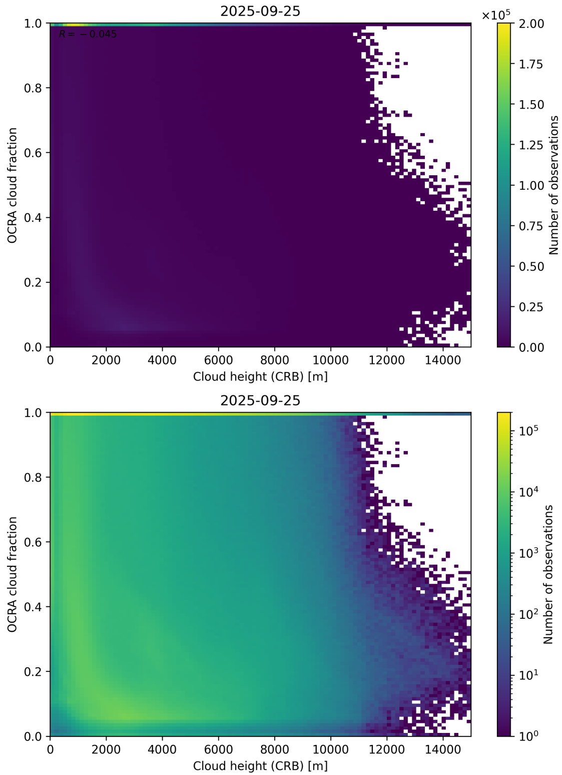
Figure 81: Scatter density plot of “Cloud height (CRB)” against “OCRA cloud fraction” for 2025-09-25 to 2025-09-26.
