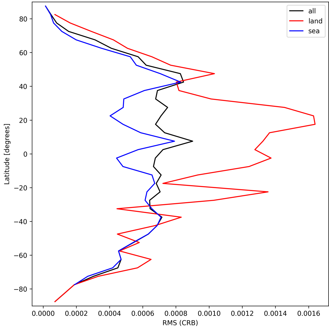
Figure 32: Zonal average of “RMS (CRB)” for 2025-09-25 to 2025-09-26.
