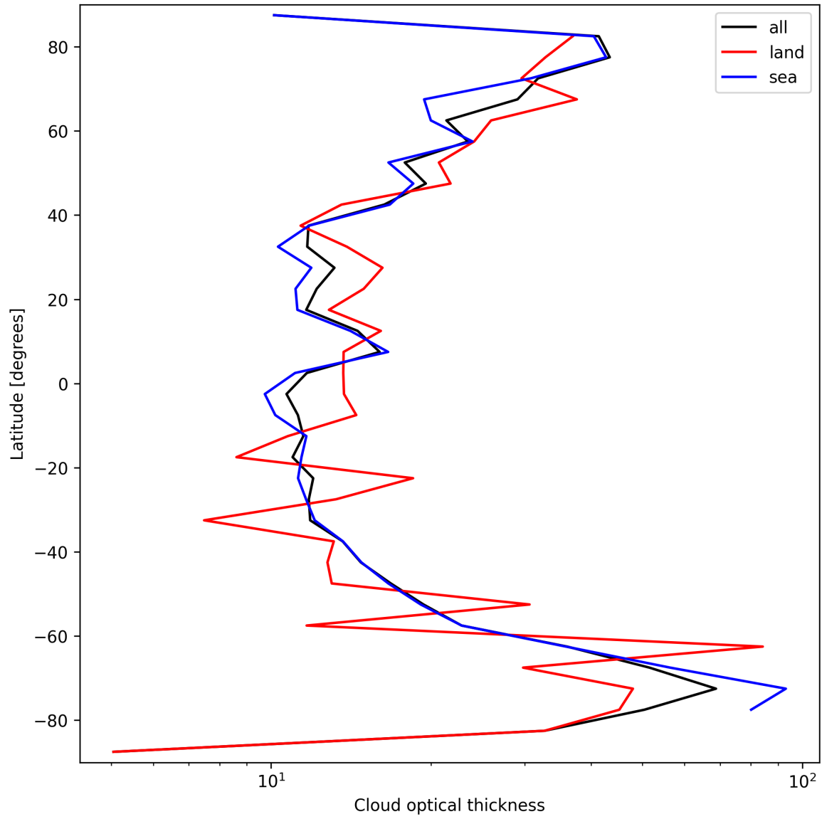
Figure 25: Zonal average of “Cloud optical thickness” for 2025-09-25 to 2025-09-26.
