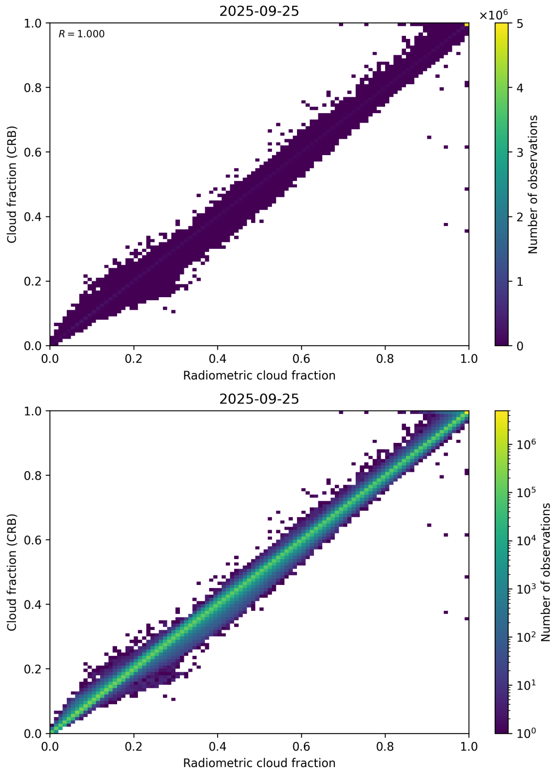
Figure 73: Scatter density plot of “Radiometric cloud fraction” against “Cloud fraction (CRB)” for 2025-09-25 to 2025-09-26.
