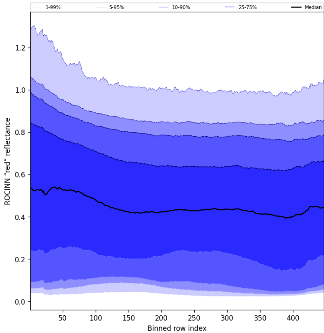
Figure 69: Along track statistics of "ROCINN "red" reflectance" for 2025-09-25 to 2025-09-26
