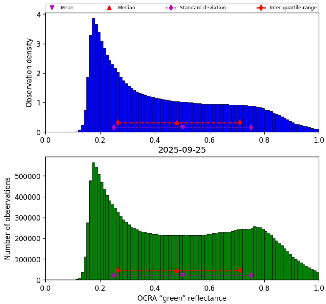
Figure 52: Histogram of “OCRA “green” reflectance” for 2025-09-25 to 2025-09-26
