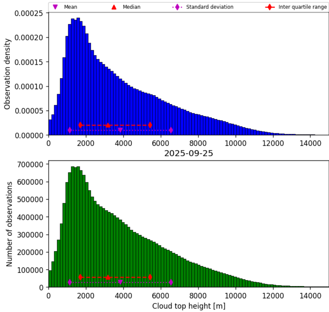
Figure 40: Histogram of “Cloud top height” for 2025-09-25 to 2025-09-26
