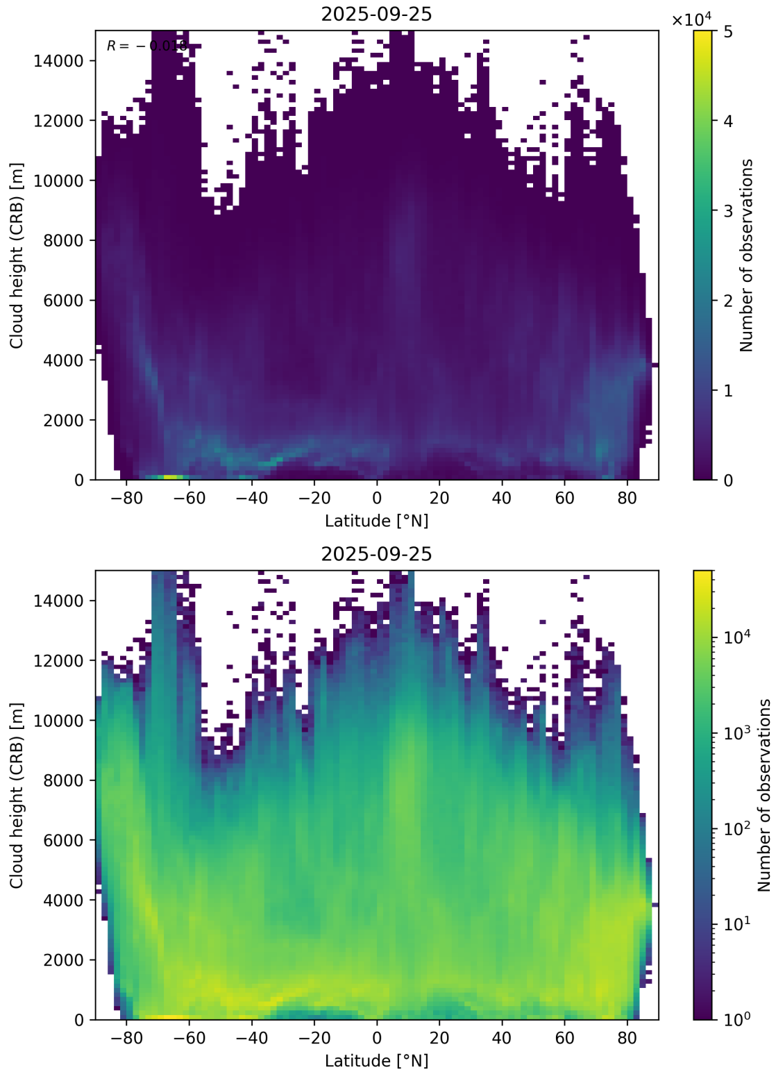
Figure 95: Scatter density plot of “Latitude” against “Cloud height (CRB)” for 2025-09-25 to 2025-09-26.
