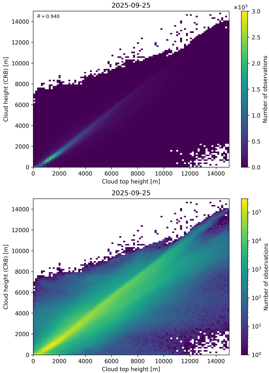
Figure 89: Scatter density plot of “Cloud top height” against “Cloud height (CRB)” for 2025-09-25 to 2025-09-26.
