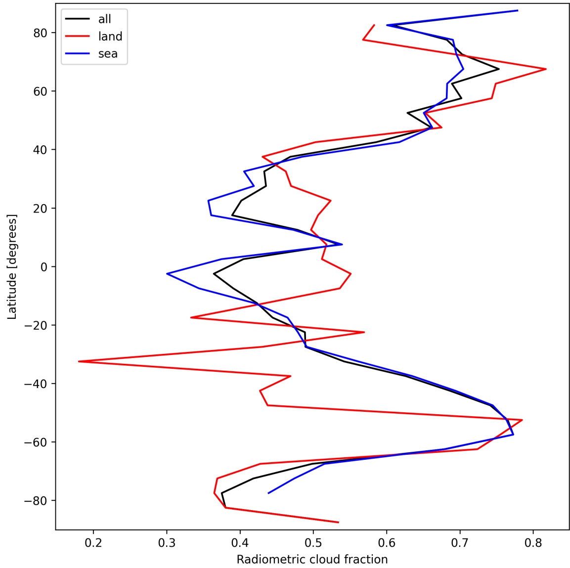
Figure 23: Zonal average of “Radiometric cloud fraction” for 2025-09-25 to 2025-09-26.
