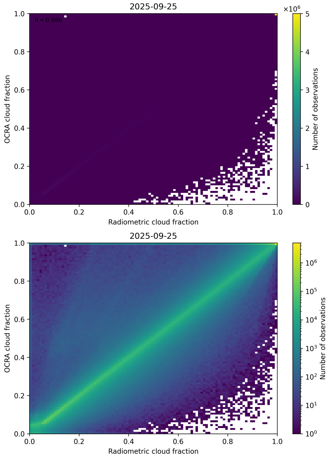
Figure 72: Scatter density plot of “Radiometric cloud fraction” against “OCRA cloud fraction” for 2025-09-25 to 2025-09-26.
