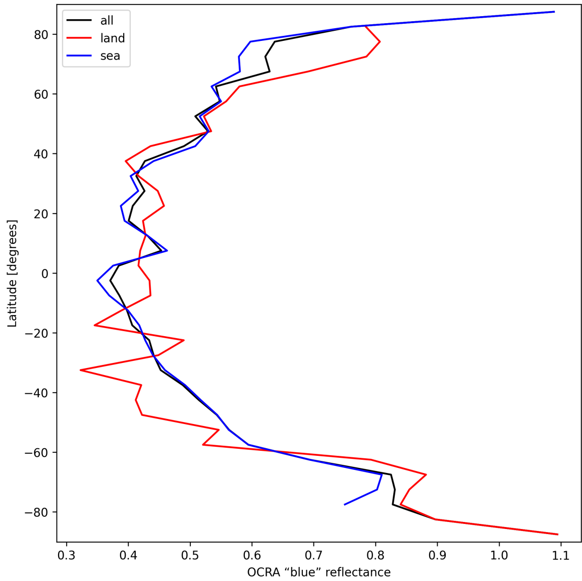
Figure 35: Zonal average of "OCRA "blue" reflectance" for 2025-09-25 to 2025-09-26.
