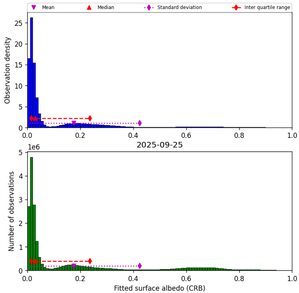
Figure 46: Histogram of “Fitted surface albedo (CRB)” for 2025-09-25 to 2025-09-26
