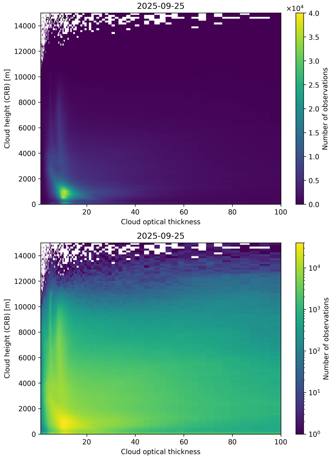
Figure 85: Scatter density plot of “Cloud optical thickness” against “Cloud height (CRB)” for 2025-09-25 to 2025-09-26.
