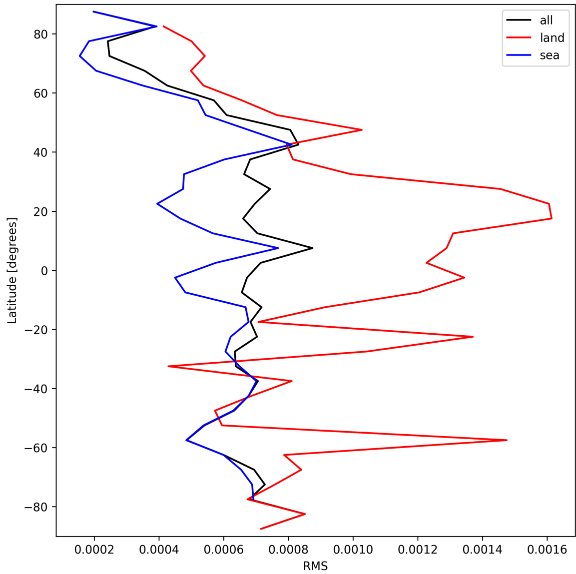
Figure 31: Zonal average of “RMS” for 2025-09-25 to 2025-09-26.
