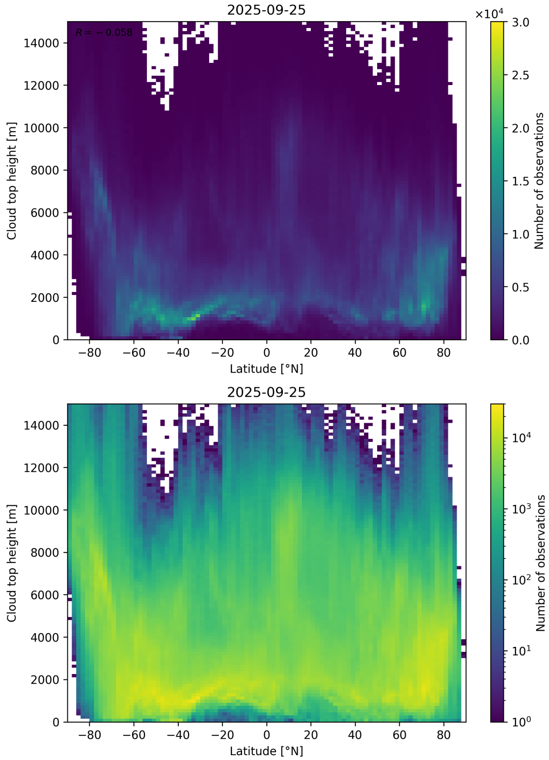
Figure 97: Scatter density plot of “Latitude” against “Cloud top height” for 2025-09-25 to 2025-09-26.
