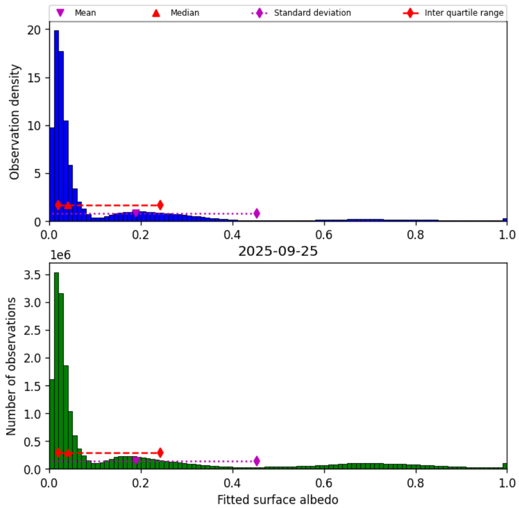
Figure 45: Histogram of “Fitted surface albedo” for 2025-09-25 to 2025-09-26
