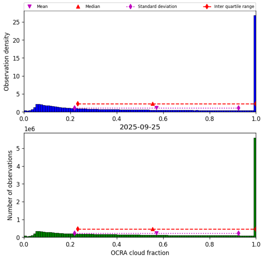
Figure 50: Histogram of “OCRA cloud fraction” for 2025-09-25 to 2025-09-26
