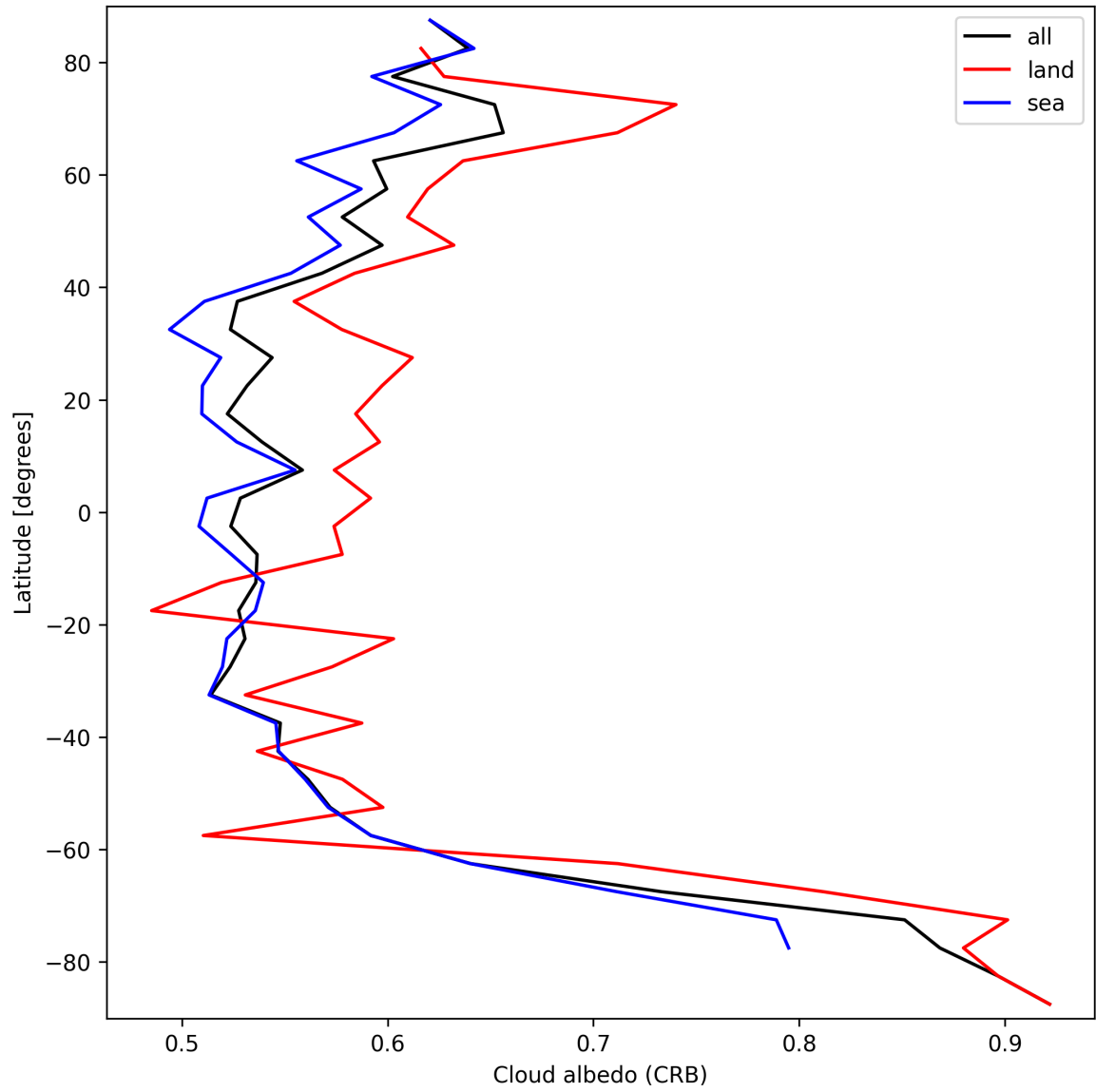
Figure 28: Zonal average of “Cloud albedo (CRB)” for 2025-09-25 to 2025-09-26.
