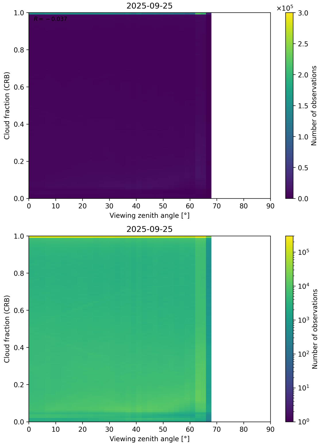
Figure 109: Scatter density plot of “Viewing zenith angle” against “Cloud fraction (CRB)” for 2025-09-25 to 2025-09-26.
