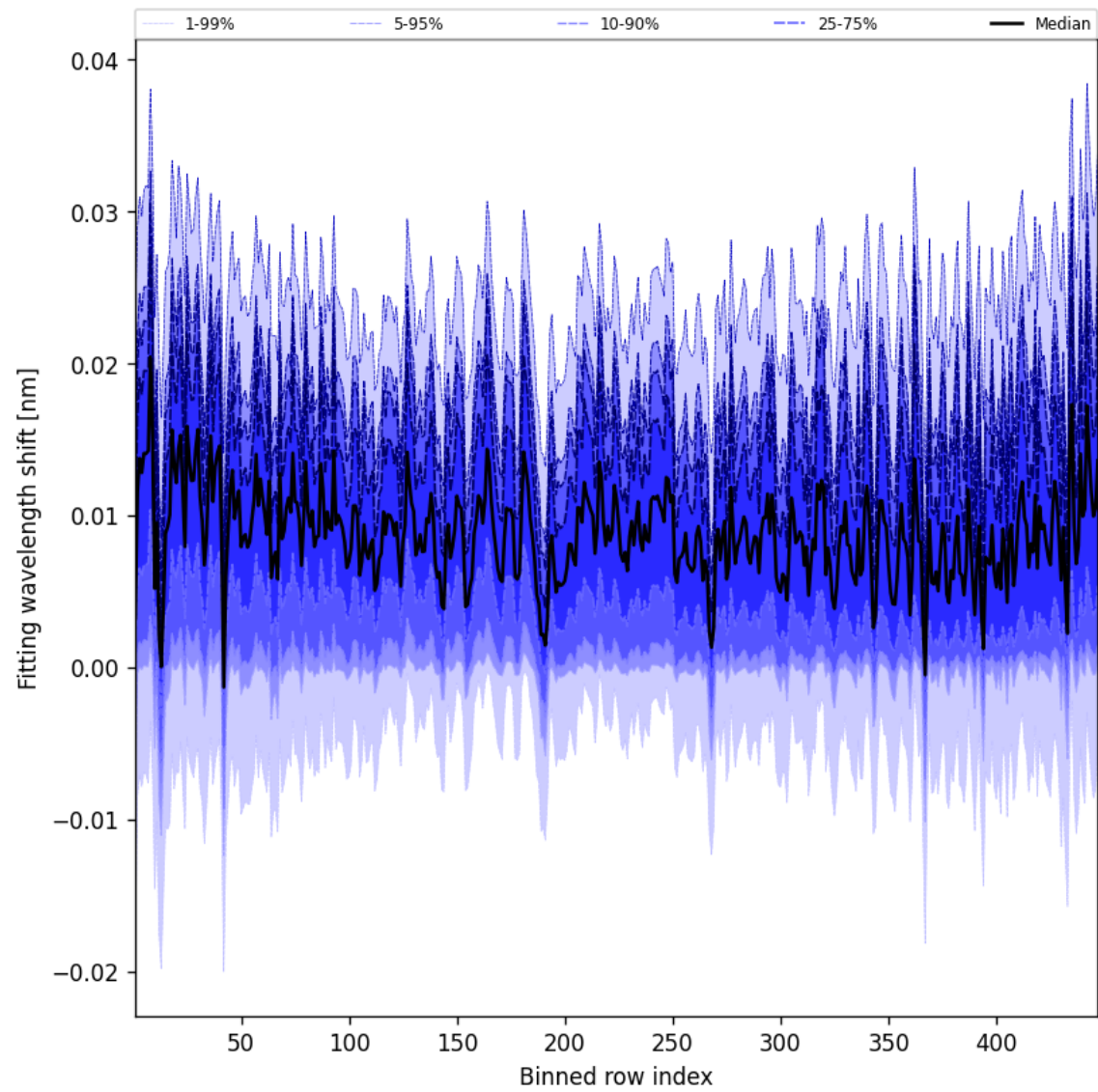
Figure 65: Along track statistics of “Fitting wavelength shift” for 2025-09-25 to 2025-09-26
