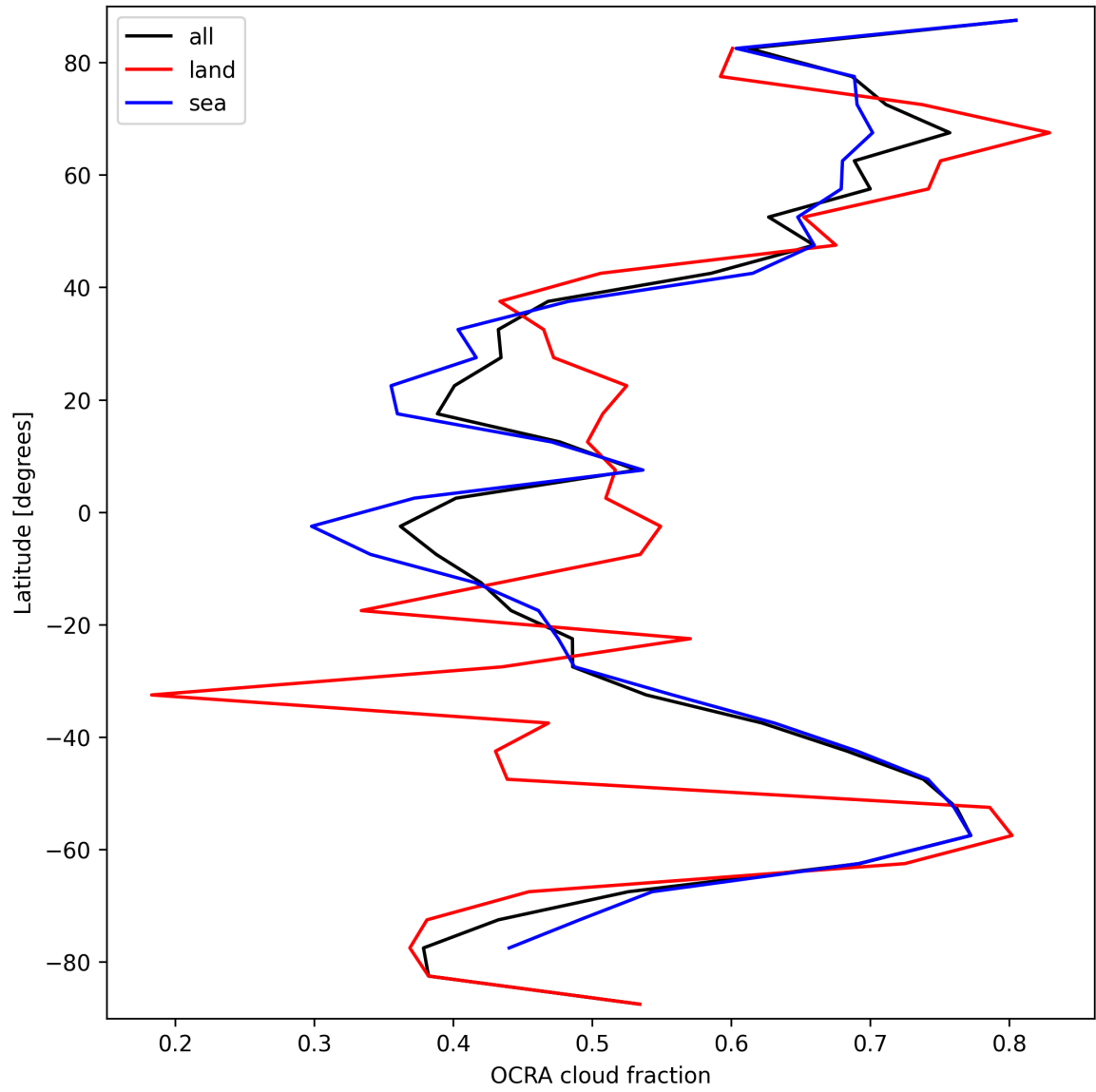
Figure 34: Zonal average of “OCRA cloud fraction” for 2025-09-25 to 2025-09-26.
