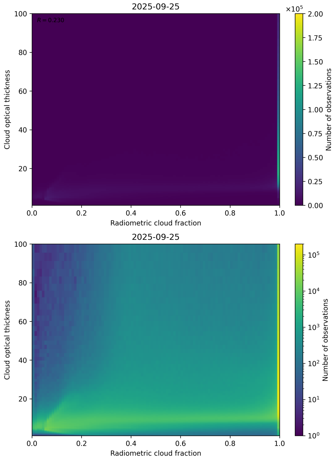
Figure 75: Scatter density plot of “Radiometric cloud fraction” against “Cloud optical thickness” for 2025-09-25 to 2025-09-26.
