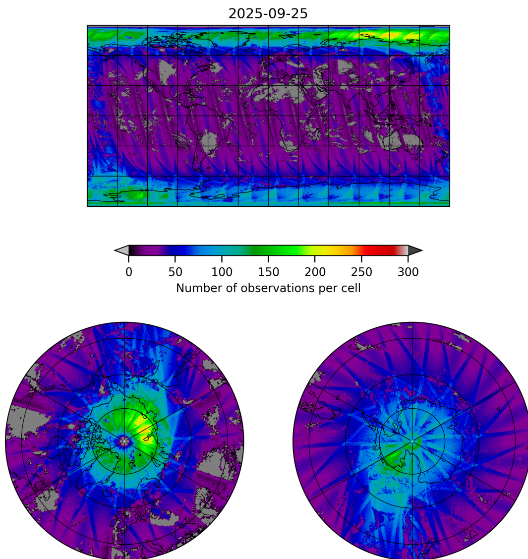
Figure 21: Map of the number of observations for 2025-09-25 to 2025-09-26
