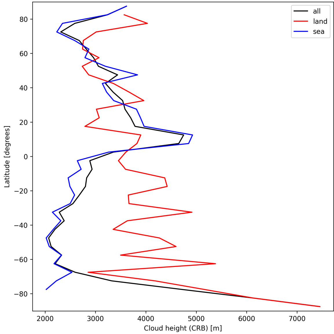
Figure 27: Zonal average of “Cloud height (CRB)” for 2025-09-25 to 2025-09-26.
