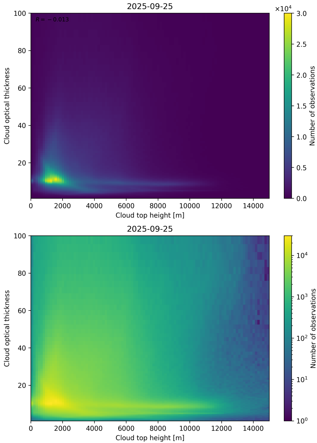
Figure 90: Scatter density plot of “Cloud top height” against “Cloud optical thickness” for 2025-09-25 to 2025-09-26.
