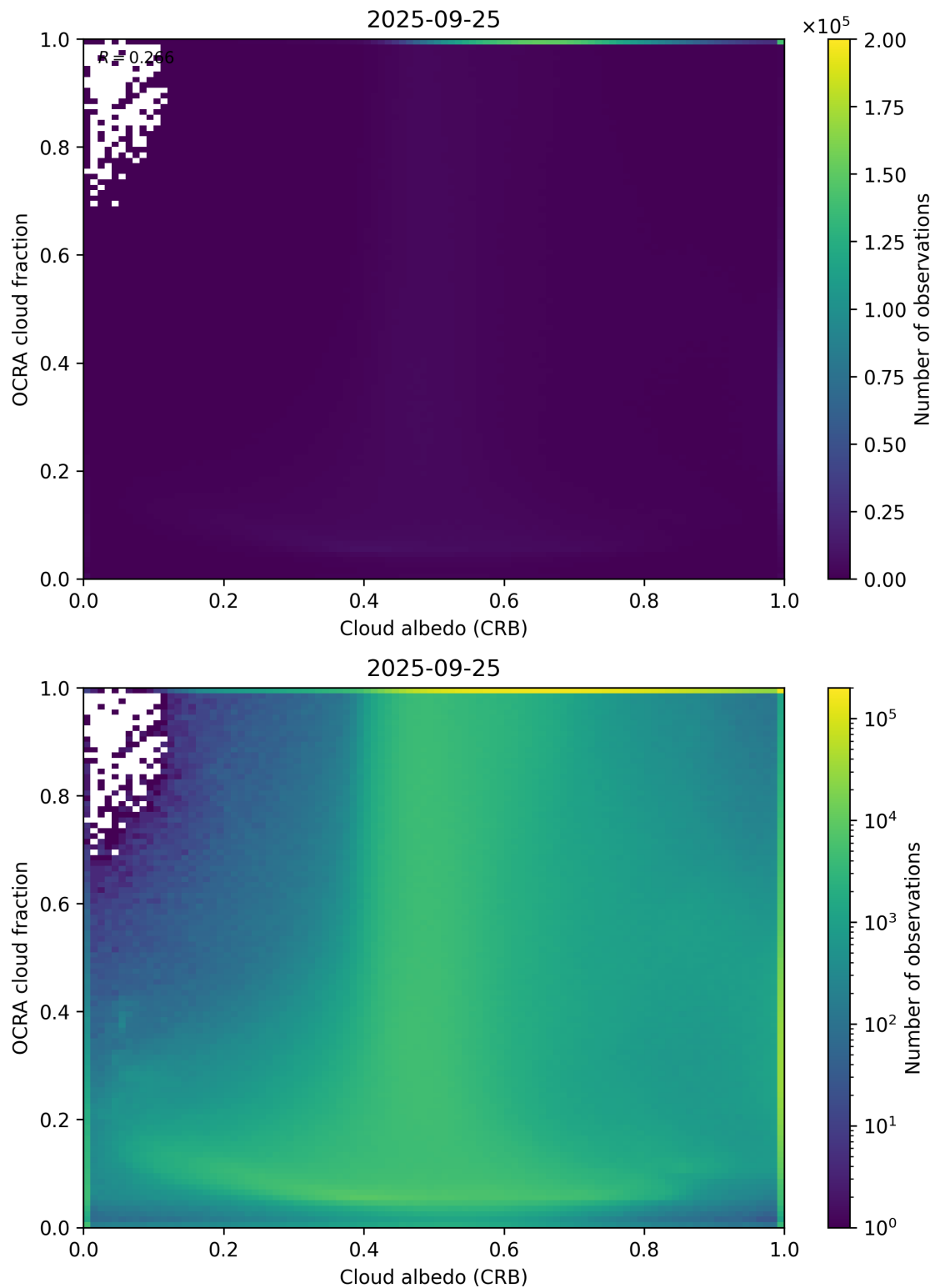
Figure 70: Scatter density plot of “Cloud albedo (CRB)” against “OCRA cloud fraction” for 2025-09-25 to 2025-09-26.
