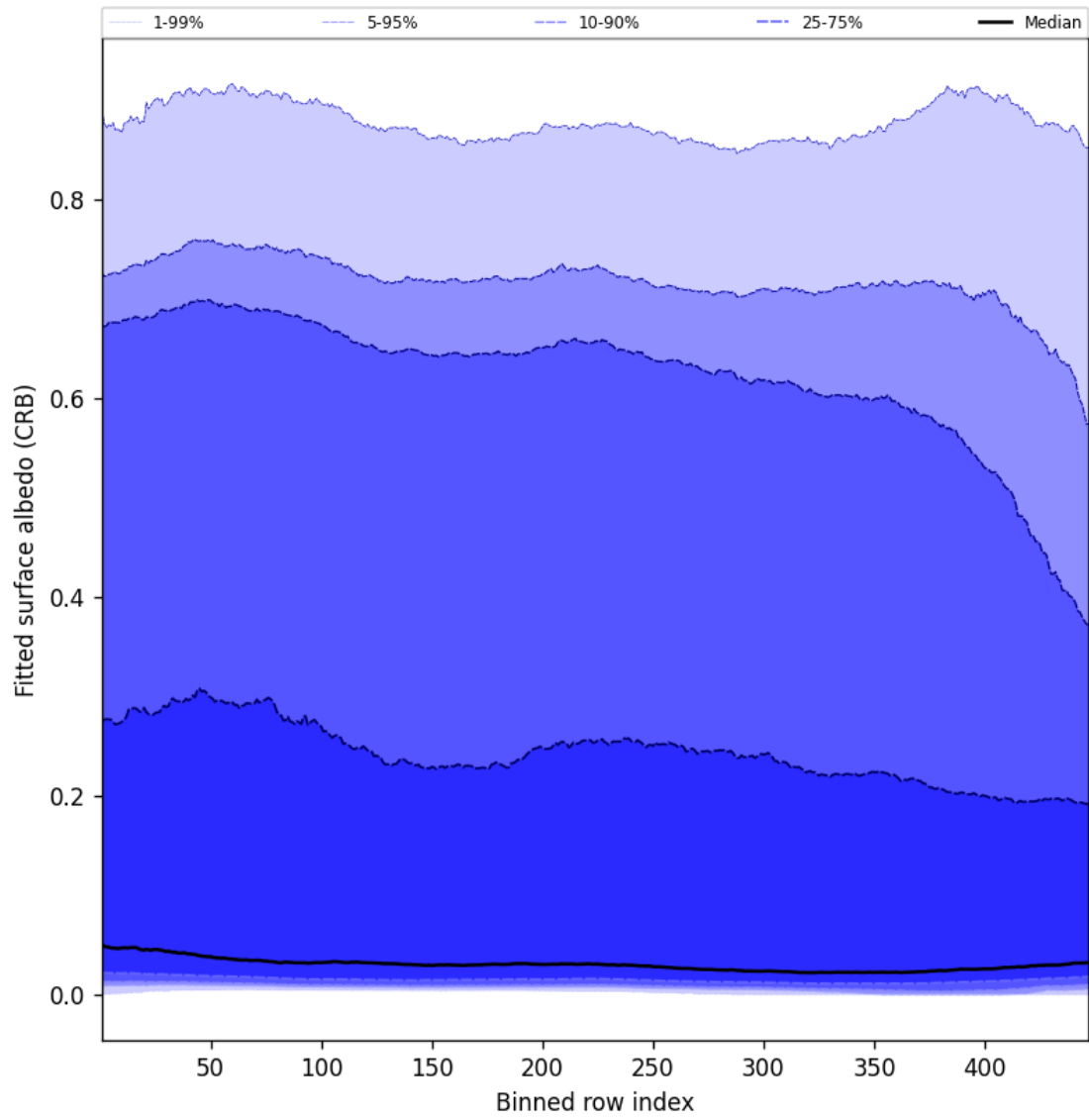
Figure 62: Along track statistics of “Fitted surface albedo (CRB)” for 2025-09-25 to 2025-09-26
