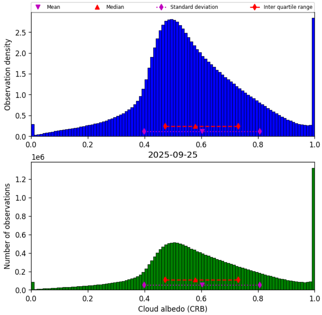
Figure 44: Histogram of “Cloud albedo (CRB)” for 2025-09-25 to 2025-09-26
