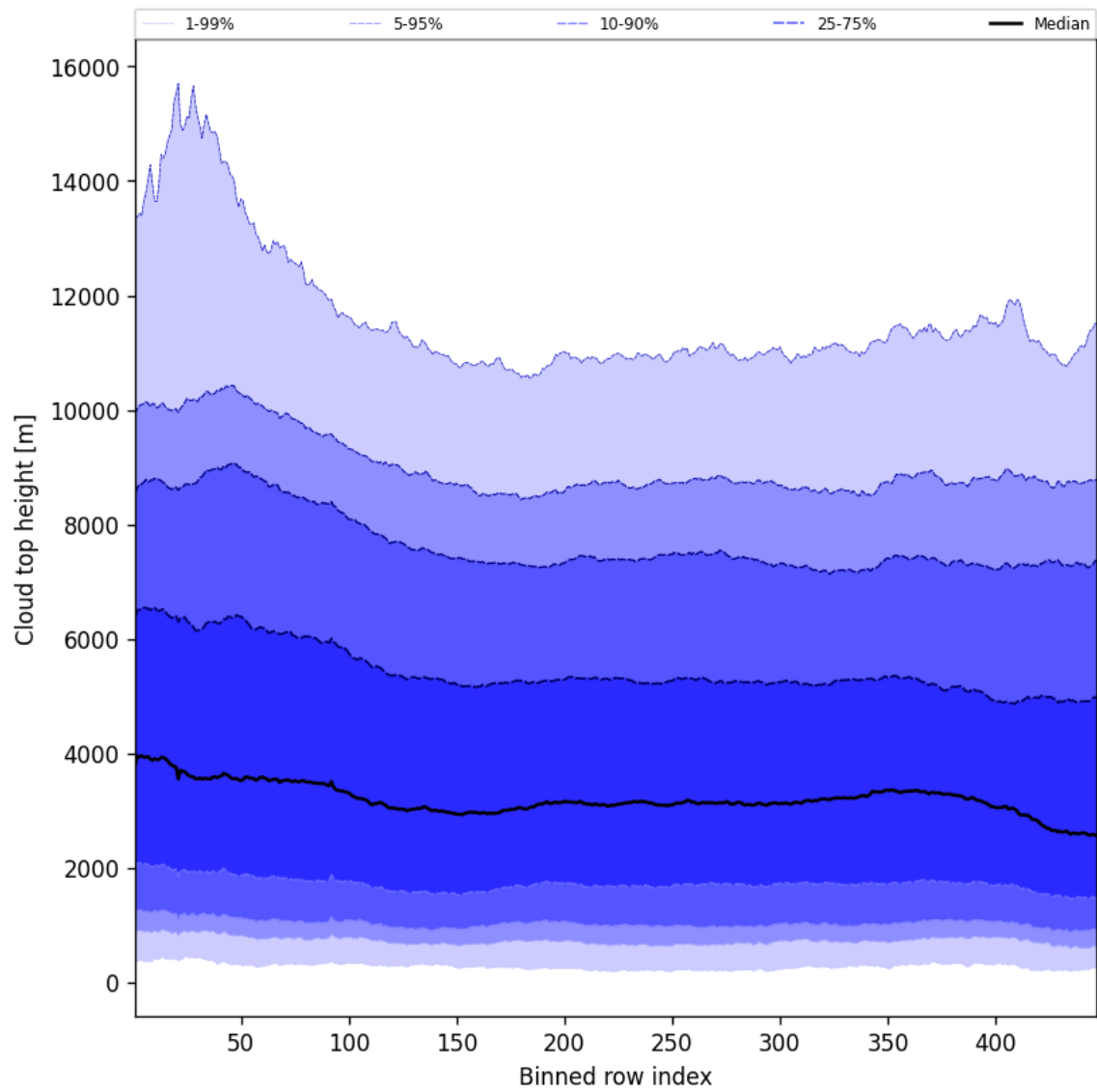
Figure 56: Along track statistics of “Cloud top height” for 2025-09-25 to 2025-09-26
