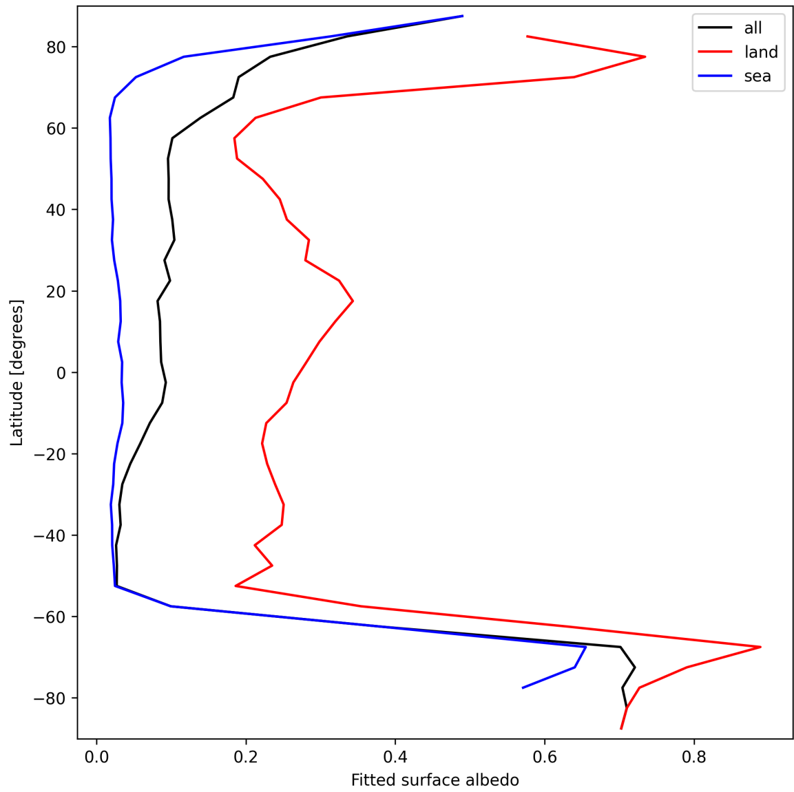
Figure 29: Zonal average of “Fitted surface albedo” for 2025-09-25 to 2025-09-26.
