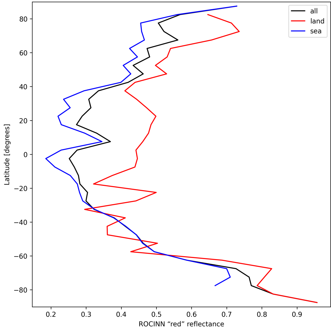
Figure 37: Zonal average of “ROCINN “red” reflectance” for 2025-09-25 to 2025-09-26.
