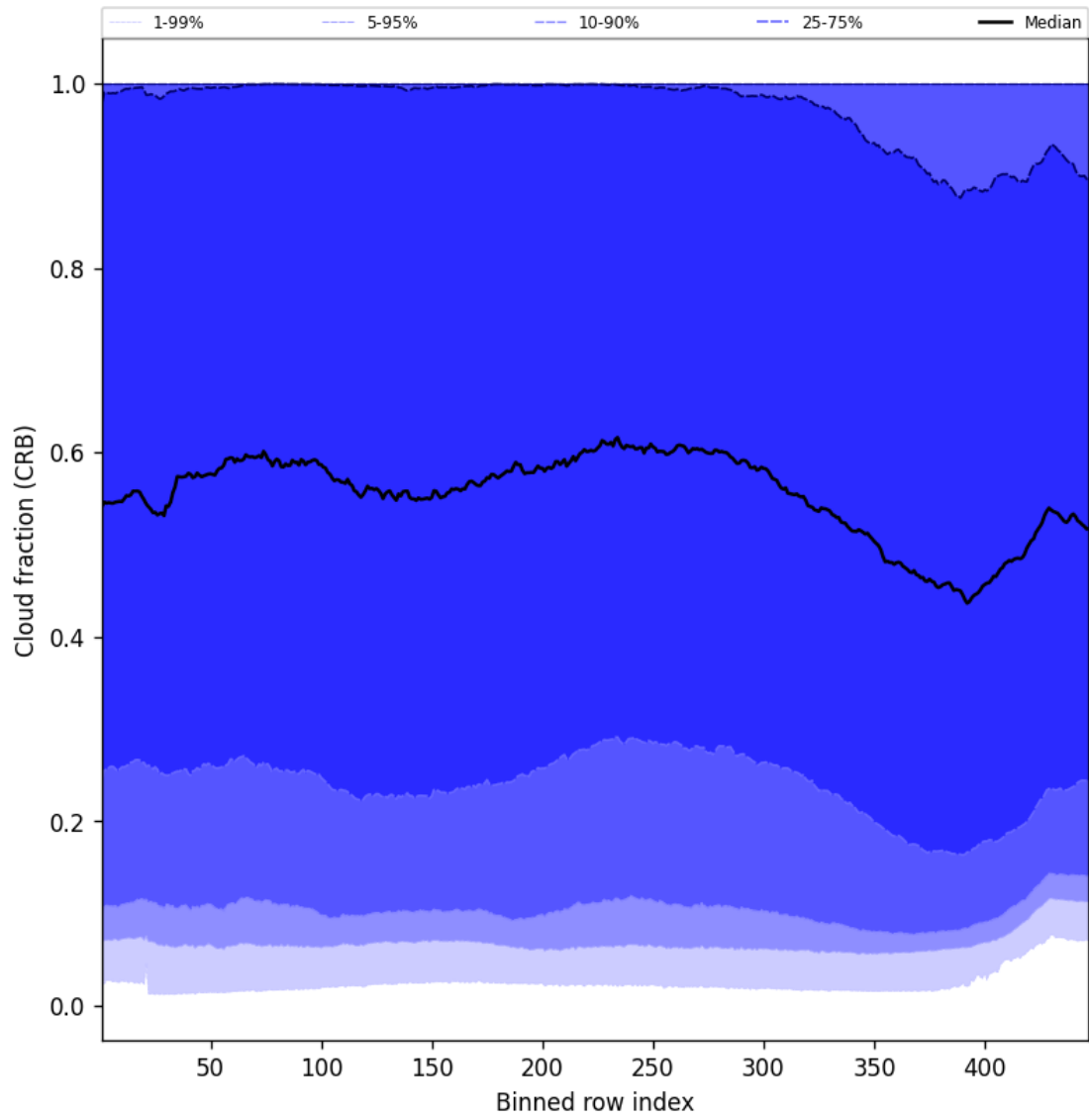
Figure 58: Along track statistics of “Cloud fraction (CRB)” for 2025-09-25 to 2025-09-26
