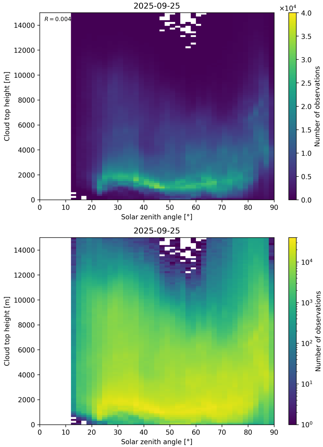
Figure 104: Scatter density plot of “Solar zenith angle” against “Cloud top height” for 2025-09-25 to 2025-09-26.
