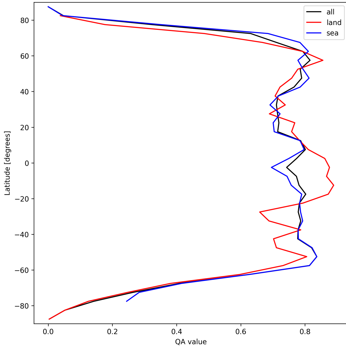
Figure 22: Zonal average of “QA value” for 2025-09-25 to 2025-09-26.
