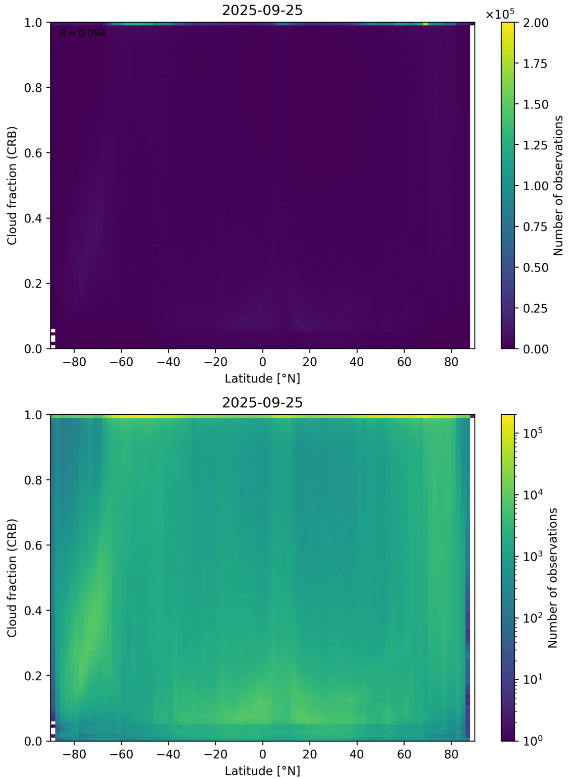
Figure 94: Scatter density plot of “Latitude” against “Cloud fraction (CRB)” for 2025-09-25 to 2025-09-26.
