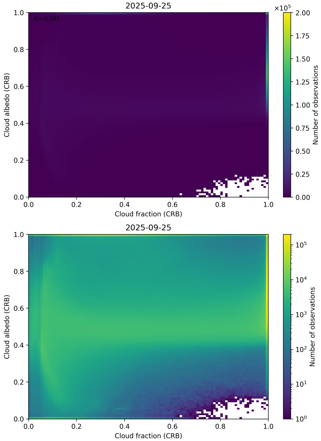
Figure 77: Scatter density plot of “Cloud fraction (CRB)” against “Cloud albedo (CRB)” for 2025-09-25 to 2025-09-26.
