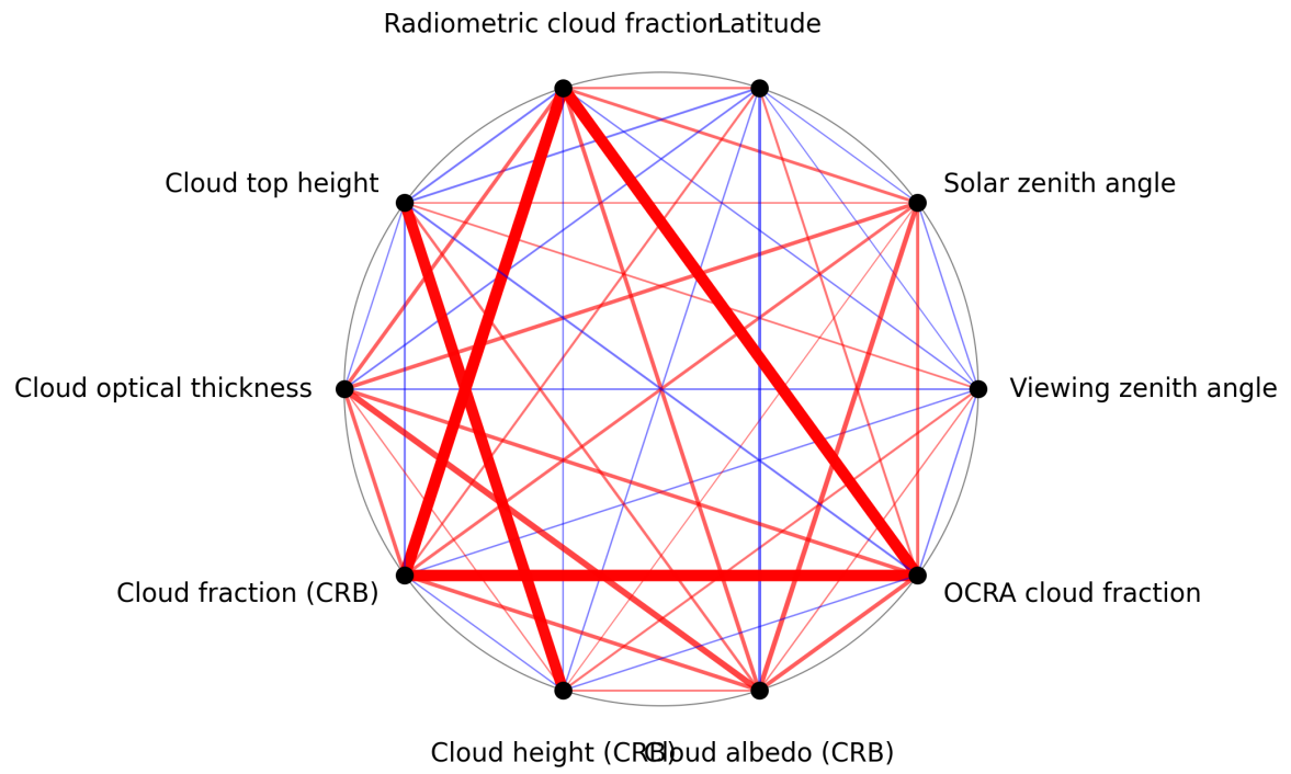
Figure 1: Map of correlation graph for 2025-09-26 to 2025-09-27.
