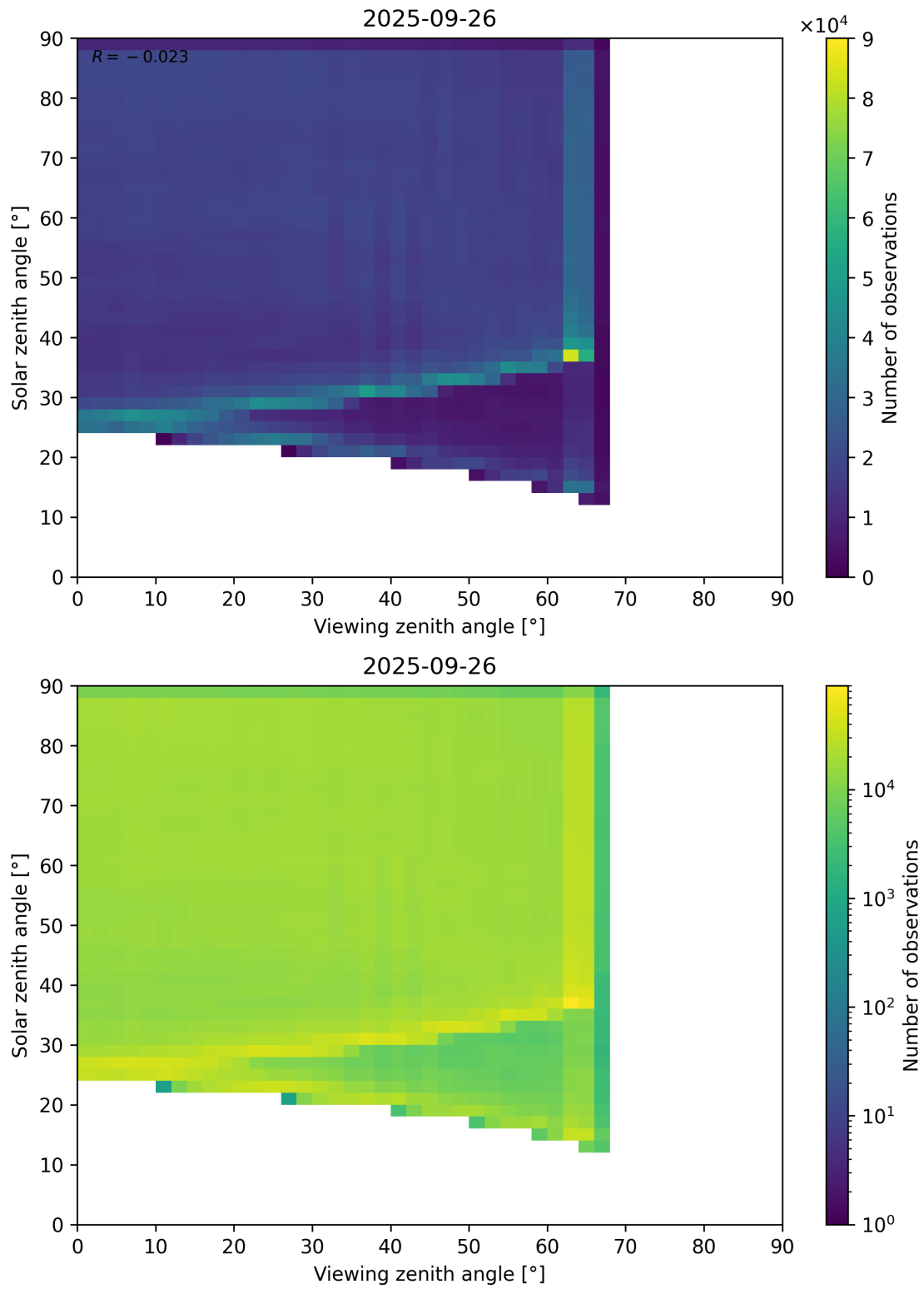
Figure 114: Scatter density plot of “Viewing zenith angle” against “Solar zenith angle” for 2025-09-26 to 2025-09-27.
