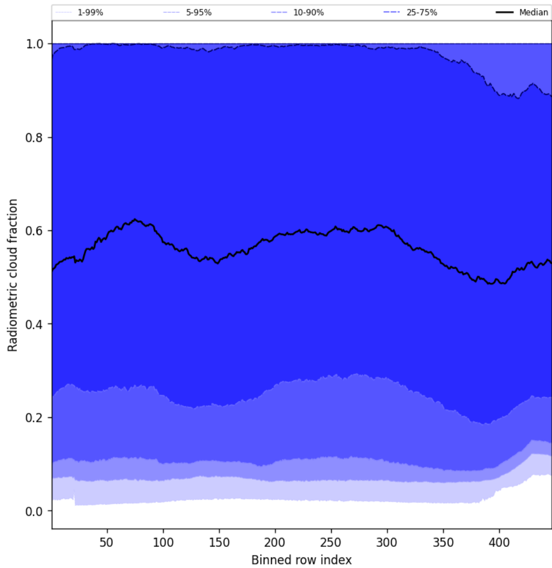
Figure 55: Along track statistics of “Radiometric cloud fraction” for 2025-09-26 to 2025-09-27
