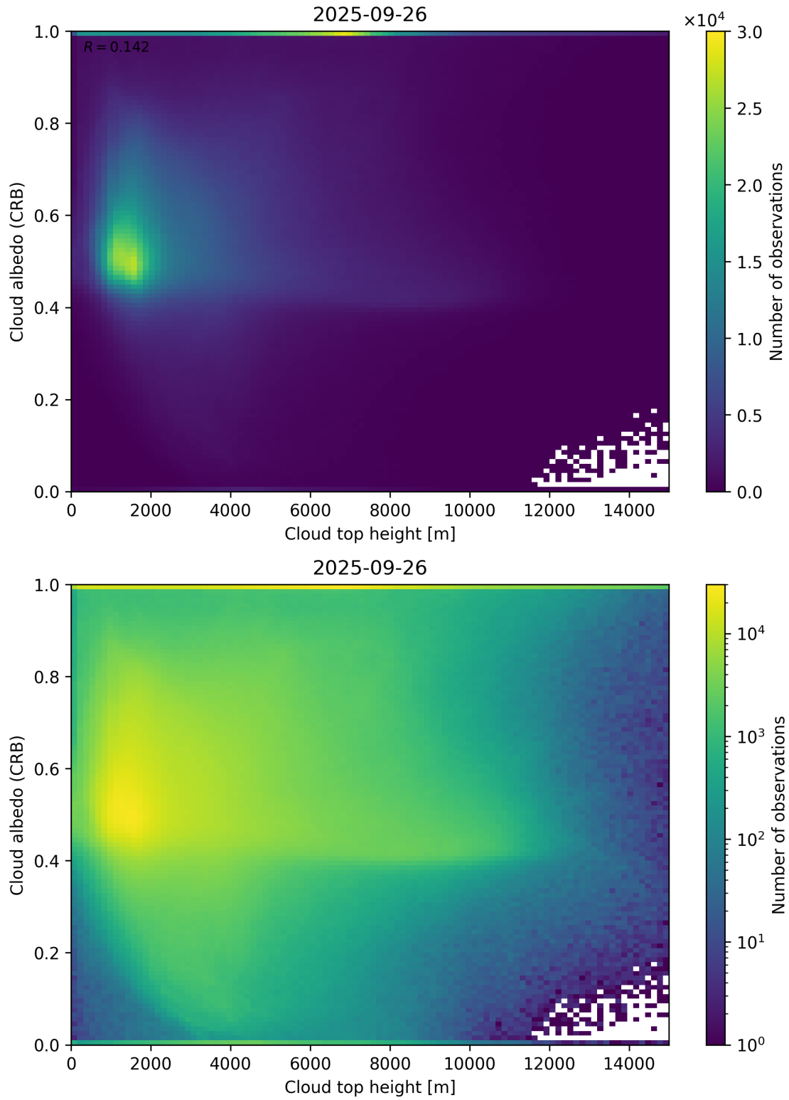
Figure 86: Scatter density plot of “Cloud top height” against “Cloud albedo (CRB)” for 2025-09-26 to 2025-09-27.
