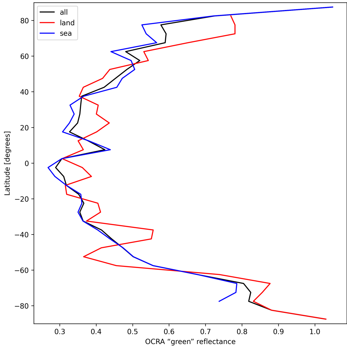
Figure 36: Zonal average of “OCRA “green” reflectance” for 2025-09-26 to 2025-09-27.
