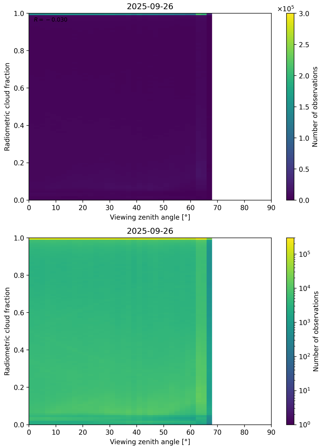
Figure 107: Scatter density plot of “Viewing zenith angle” against “Radiometric cloud fraction” for 2025-09-26 to 2025-09-27.
