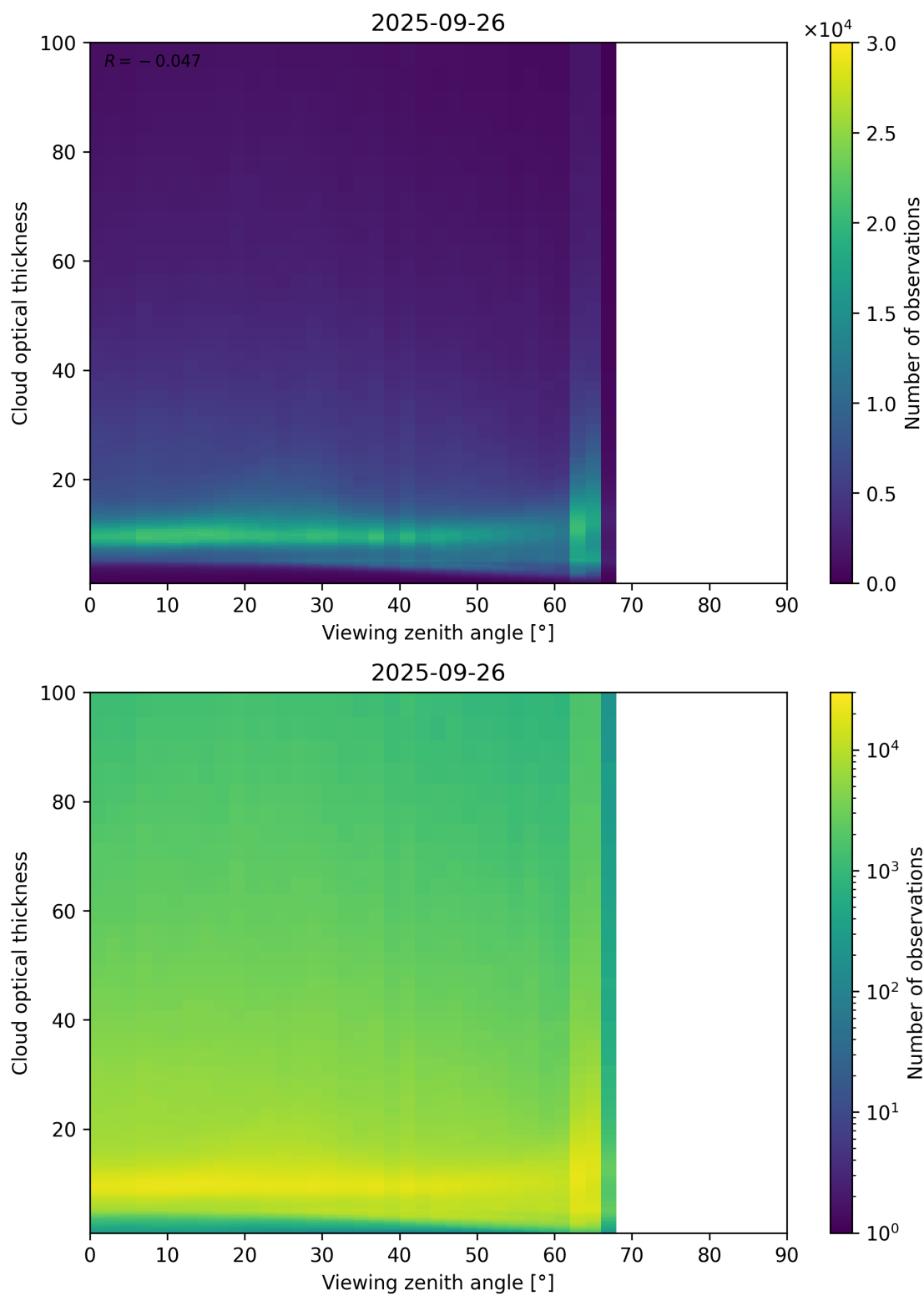
Figure 111: Scatter density plot of “Viewing zenith angle” against “Cloud optical thickness” for 2025-09-26 to 2025-09-27.
