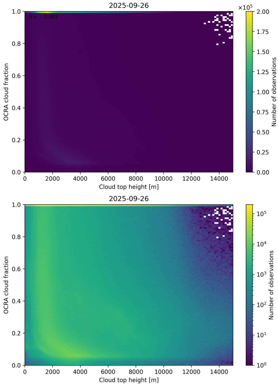
Figure 87: Scatter density plot of “Cloud top height” against “OCRA cloud fraction” for 2025-09-26 to 2025-09-27.
