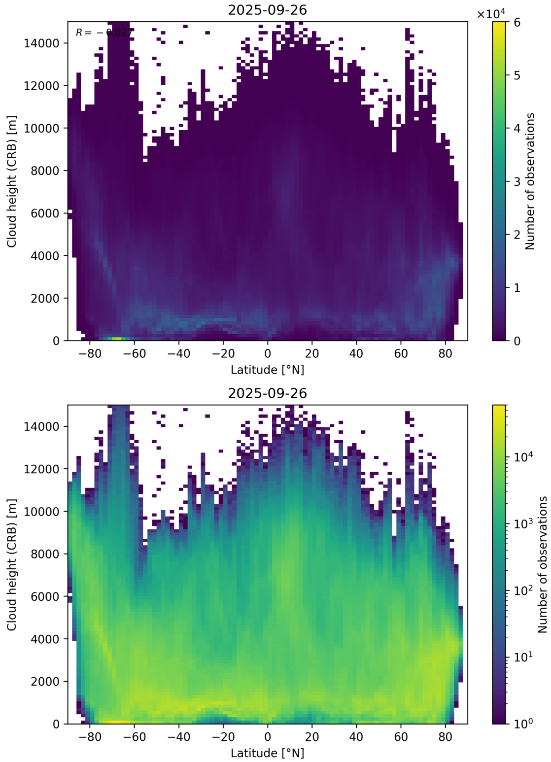
Figure 95: Scatter density plot of “Latitude” against “Cloud height (CRB)” for 2025-09-26 to 2025-09-27.
