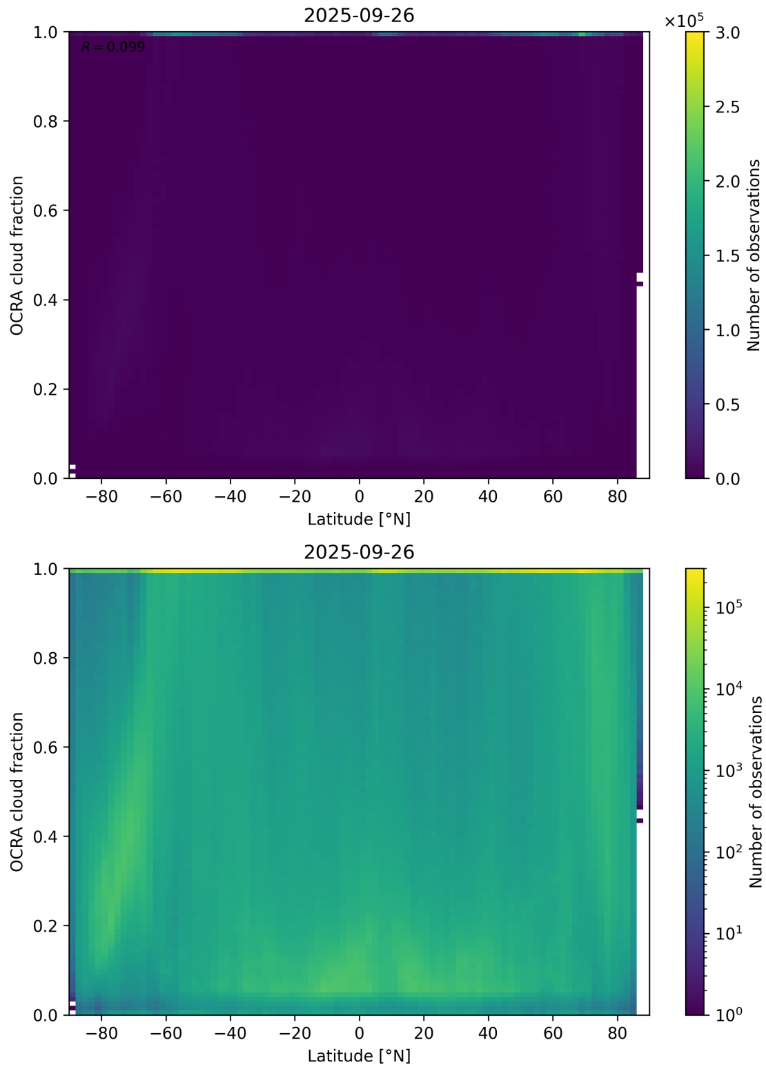
Figure 93: Scatter density plot of “Latitude” against “OCRA cloud fraction” for 2025-09-26 to 2025-09-27.
