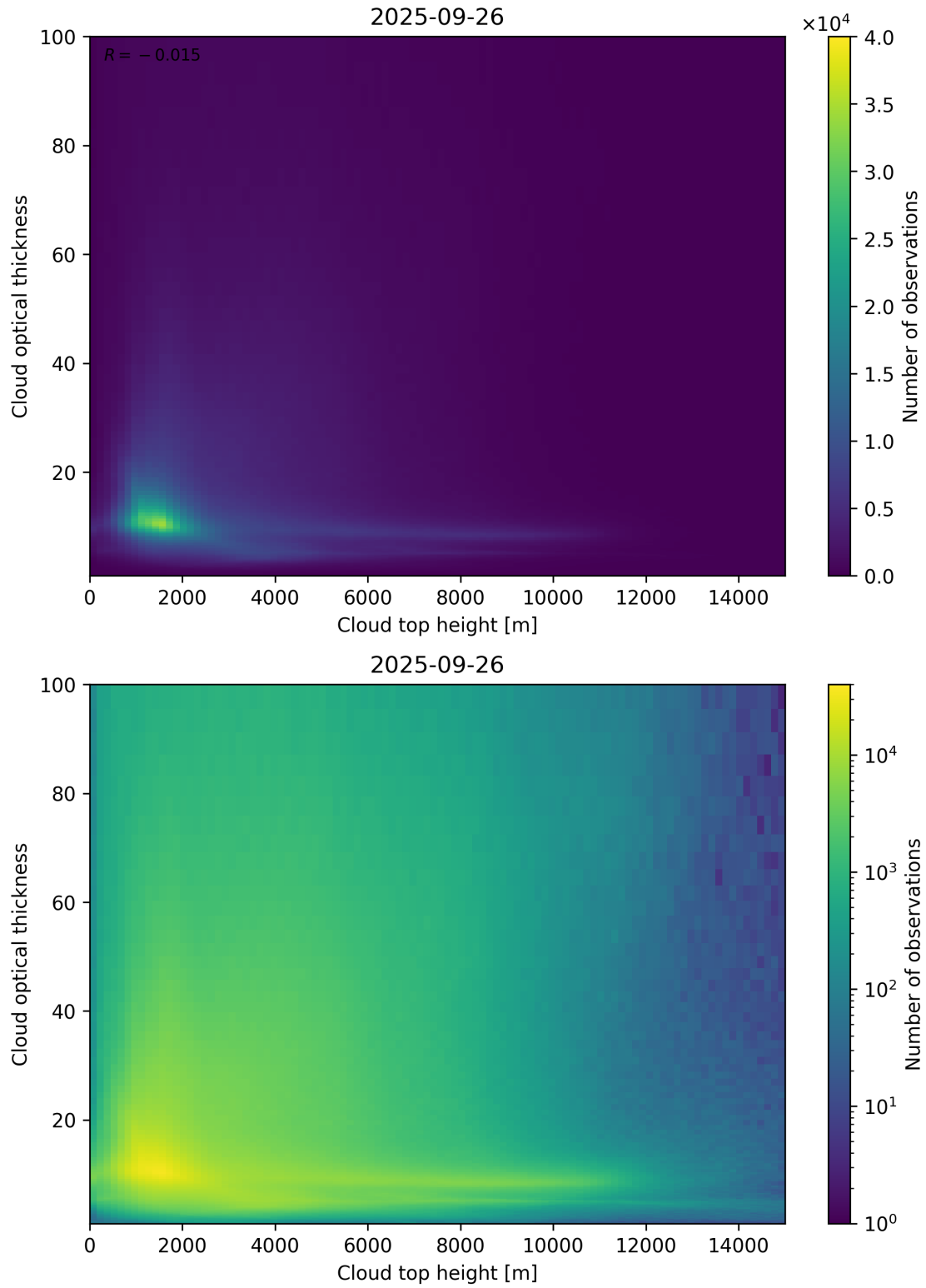
Figure 90: Scatter density plot of “Cloud top height” against “Cloud optical thickness” for 2025-09-26 to 2025-09-27.
