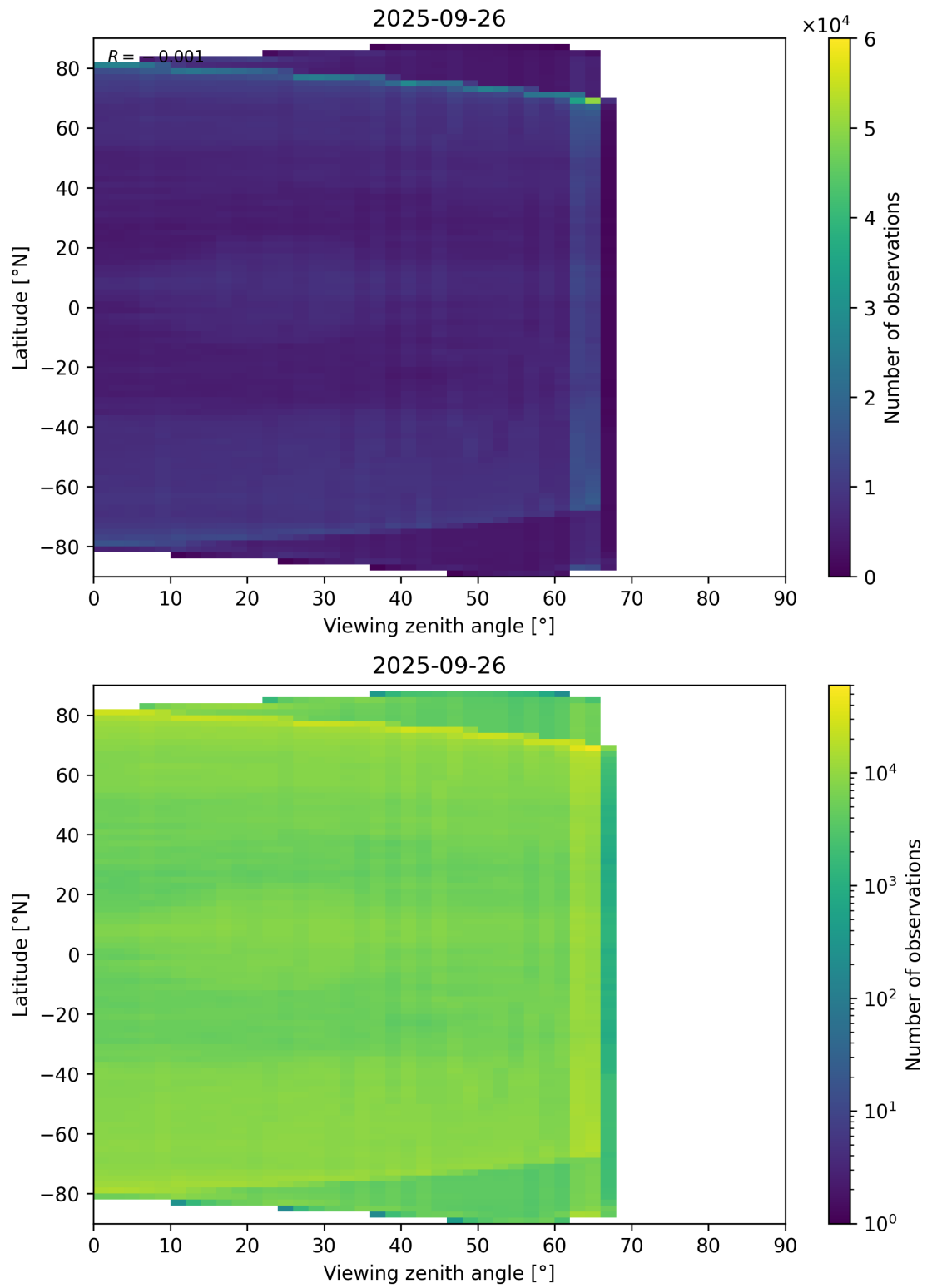
Figure 113: Scatter density plot of “Viewing zenith angle” against “Latitude” for 2025-09-26 to 2025-09-27.
