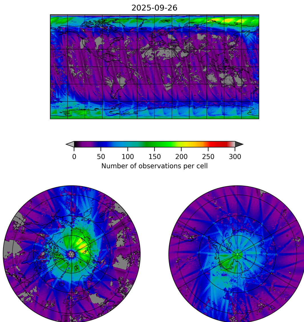
Figure 21: Map of the number of observations for 2025-09-26 to 2025-09-27
