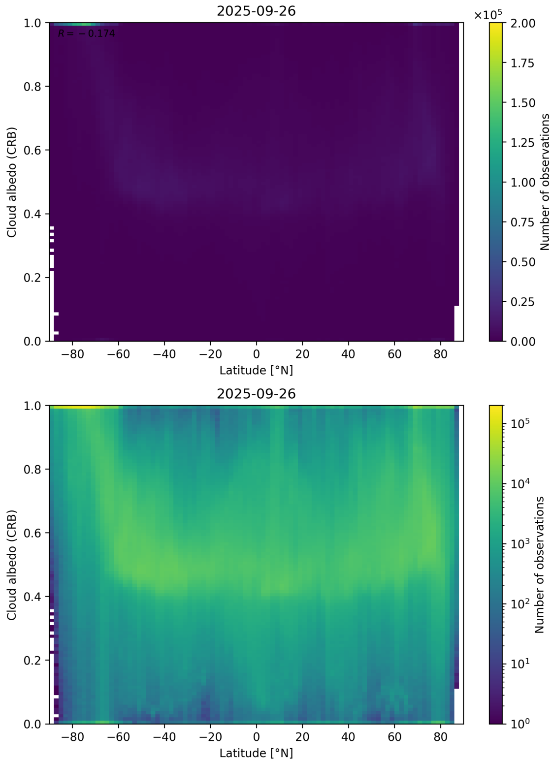
Figure 91: Scatter density plot of “Latitude” against “Cloud albedo (CRB)” for 2025-09-26 to 2025-09-27.
