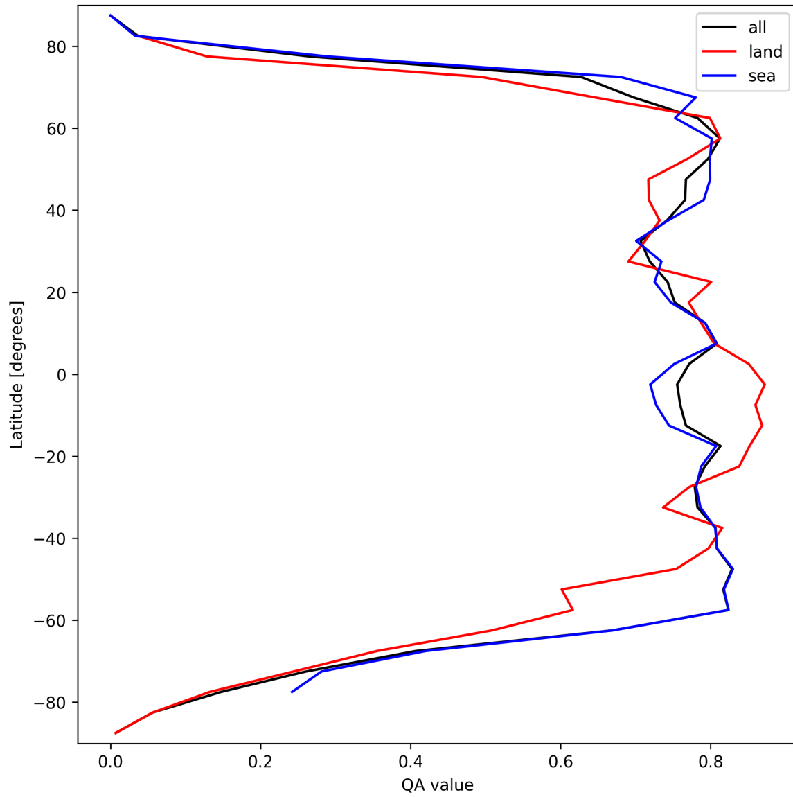
Figure 22: Zonal average of “QA value” for 2025-09-26 to 2025-09-27.
