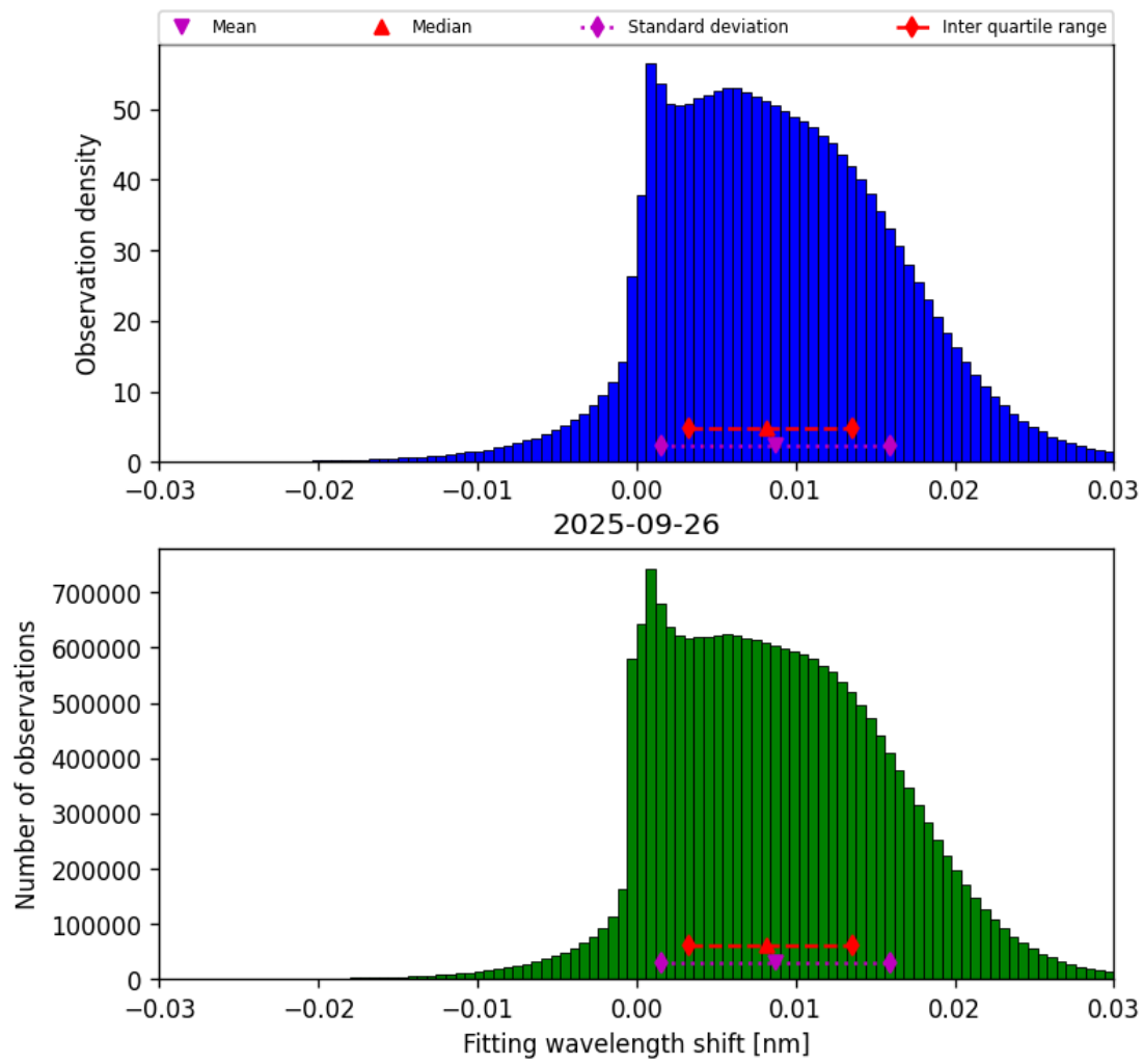
Figure 49: Histogram of “Fitting wavelength shift” for 2025-09-26 to 2025-09-27
