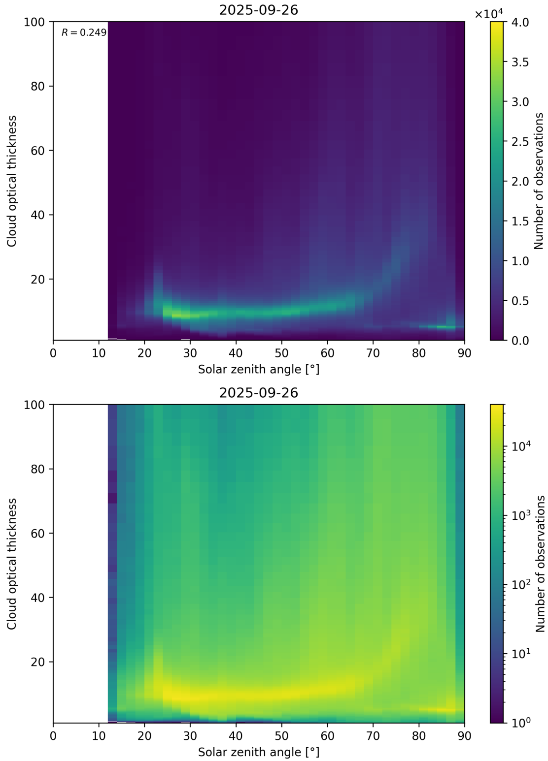
Figure 103: Scatter density plot of “Solar zenith angle” against “Cloud optical thickness” for 2025-09-26 to 2025-09-27.
