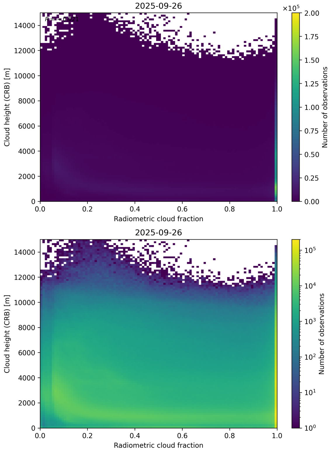
Figure 74: Scatter density plot of “Radiometric cloud fraction” against “Cloud height (CRB)” for 2025-09-26 to 2025-09-27.
