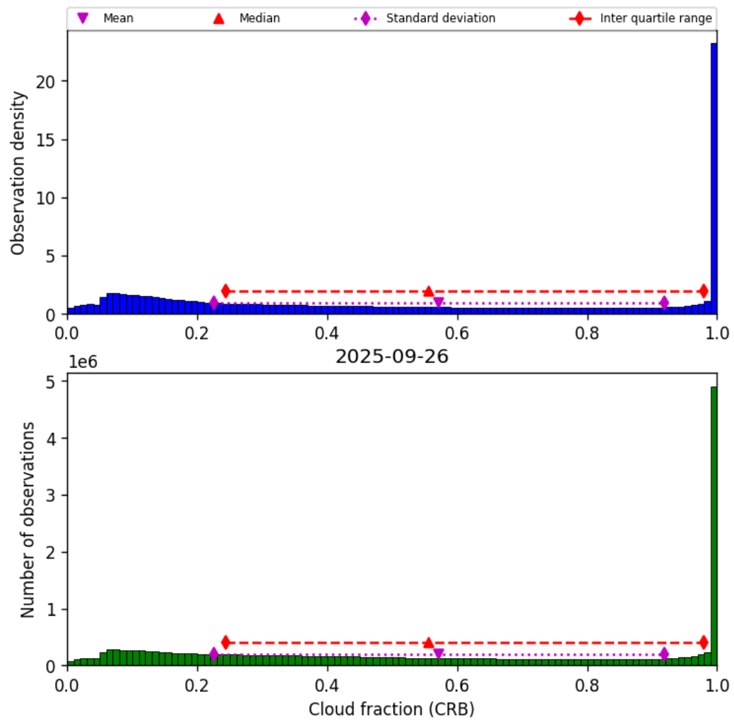
Figure 42: Histogram of “Cloud fraction (CRB)” for 2025-09-26 to 2025-09-27
