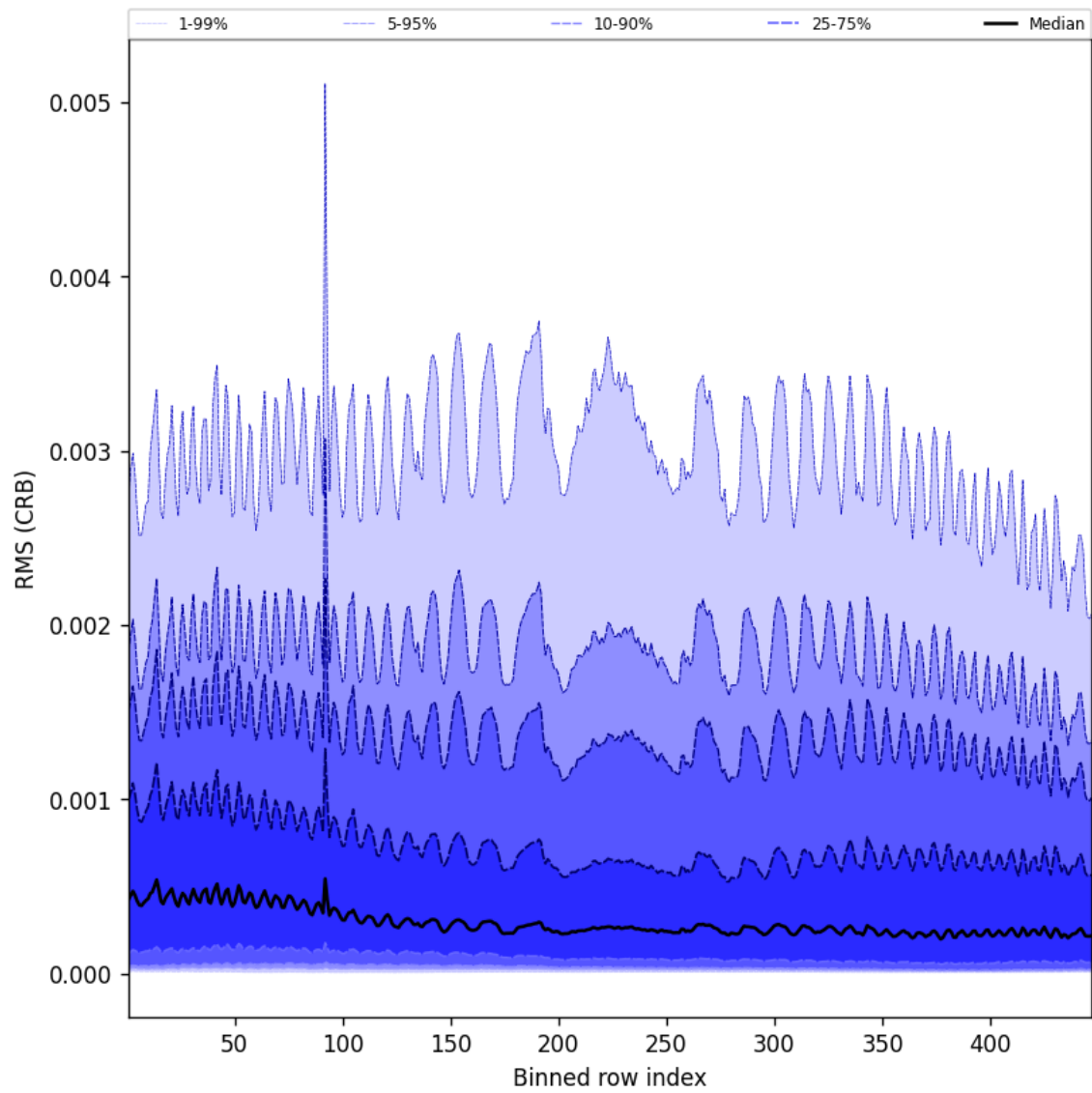
Figure 64: Along track statistics of “RMS (CRB)” for 2025-09-26 to 2025-09-27
