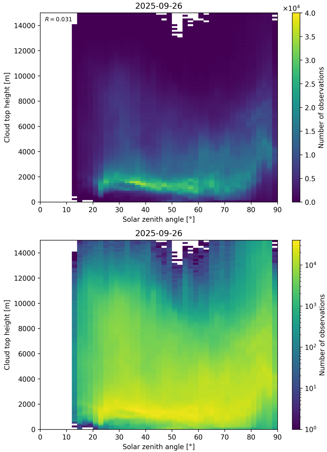
Figure 104: Scatter density plot of “Solar zenith angle” against “Cloud top height” for 2025-09-26 to 2025-09-27.
