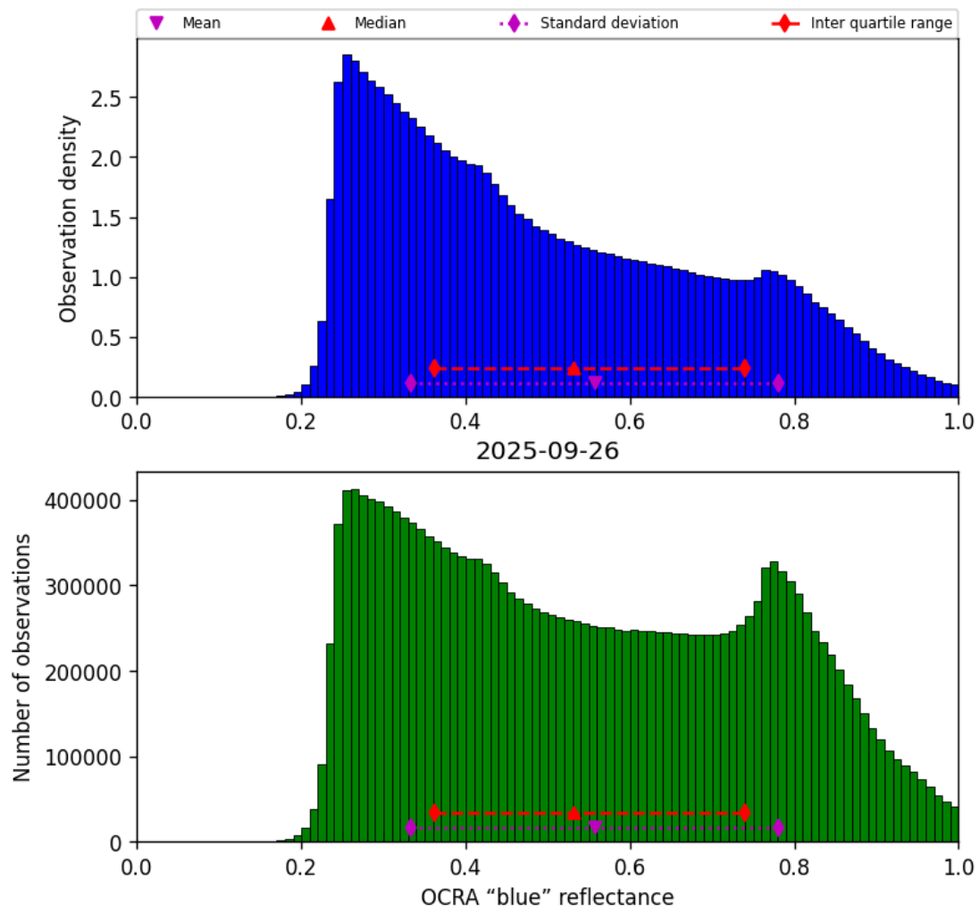
Figure 51: Histogram of “OCRA “blue” reflectance” for 2025-09-26 to 2025-09-27
