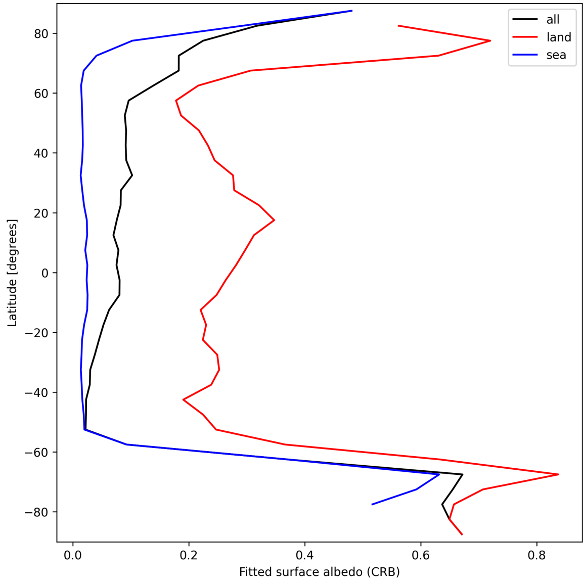
Figure 30: Zonal average of “Fitted surface albedo (CRB)” for 2025-09-26 to 2025-09-27.
