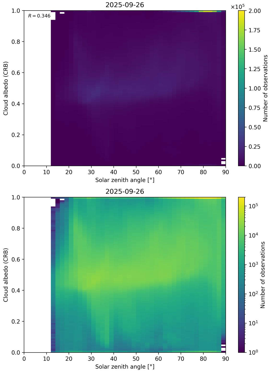
Figure 98: Scatter density plot of “Solar zenith angle” against “Cloud albedo (CRB)” for 2025-09-26 to 2025-09-27.
