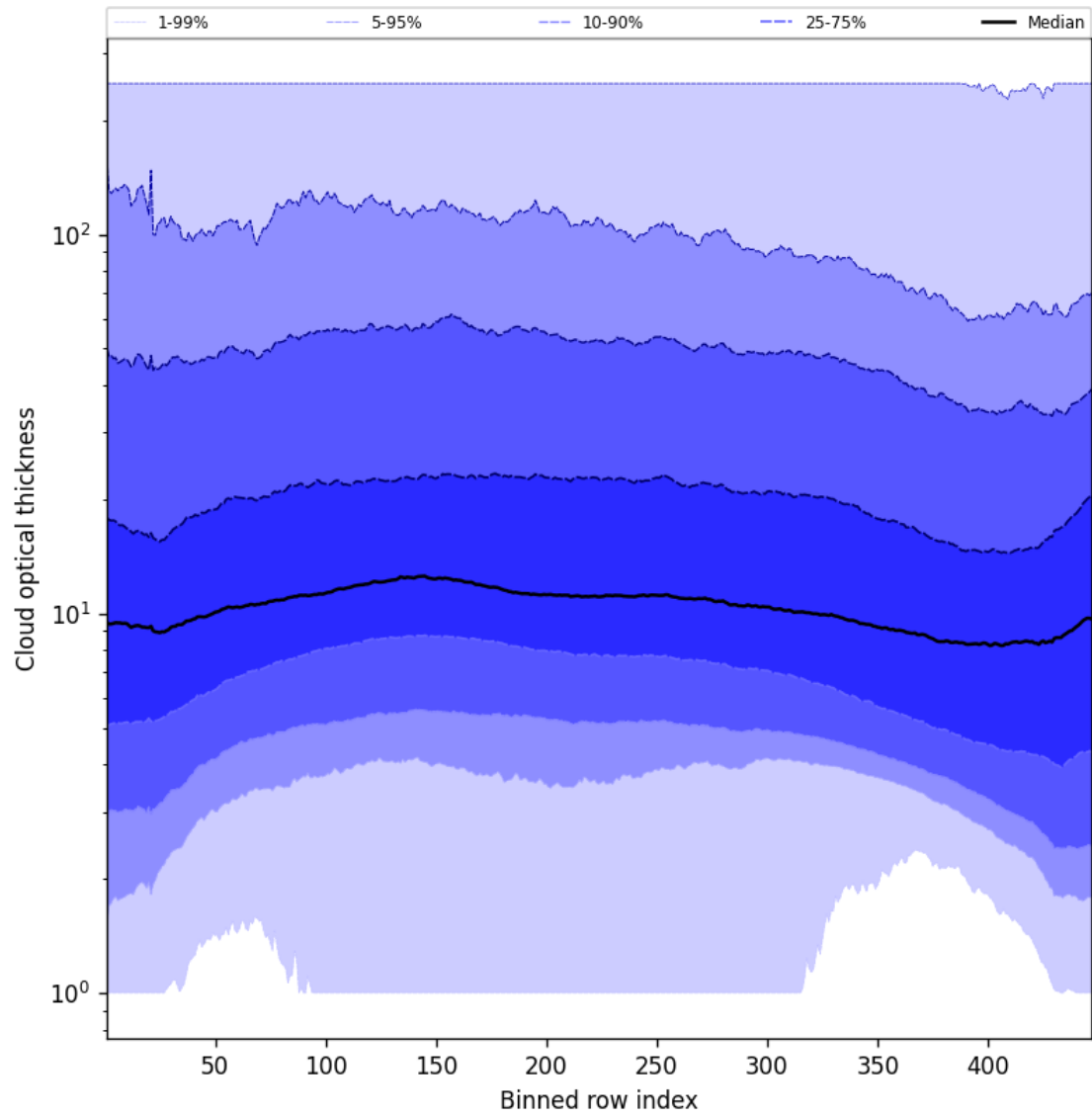
Figure 57: Along track statistics of “Cloud optical thickness” for 2025-09-26 to 2025-09-27
