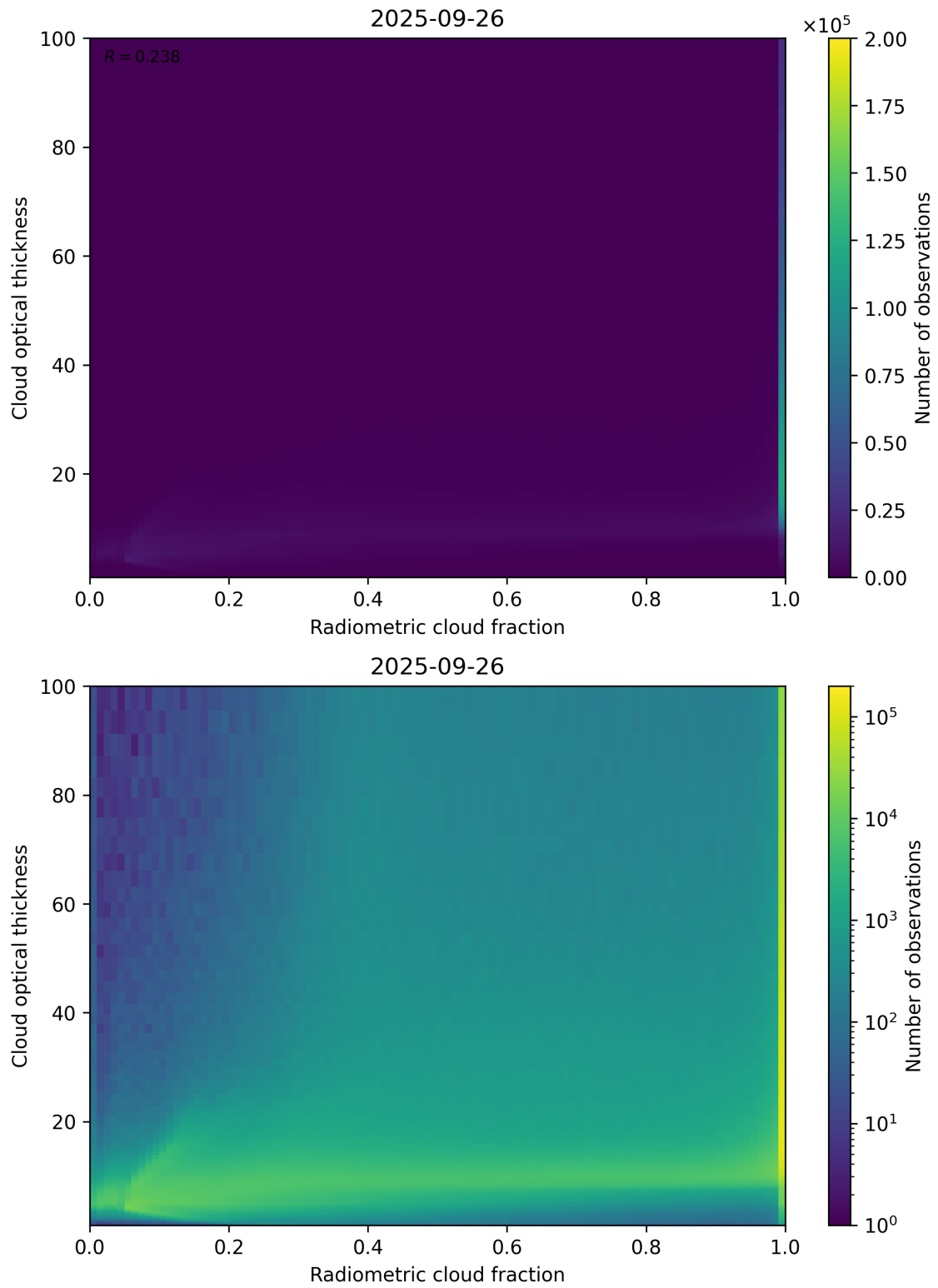
Figure 75: Scatter density plot of “Radiometric cloud fraction” against “Cloud optical thickness” for 2025-09-26 to 2025-09-27.
