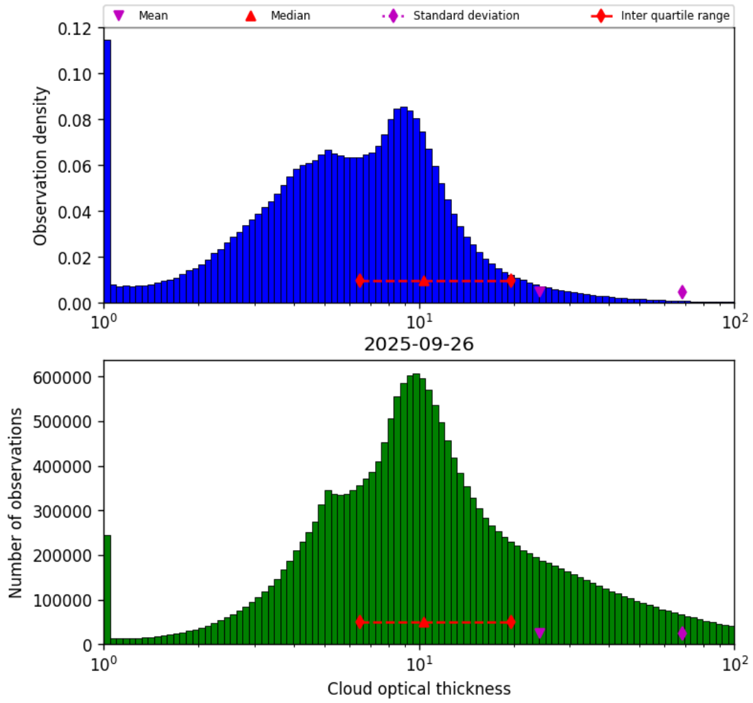
Figure 41: Histogram of “Cloud optical thickness” for 2025-09-26 to 2025-09-27
