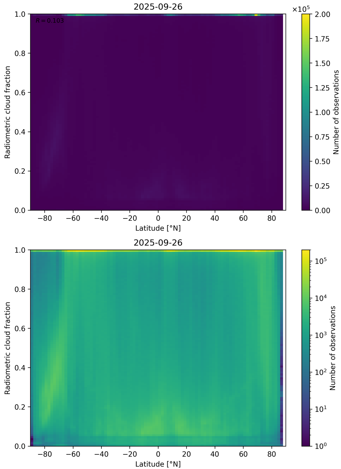
Figure 92: Scatter density plot of “Latitude” against “Radiometric cloud fraction” for 2025-09-26 to 2025-09-27.
