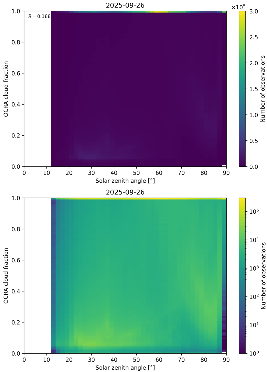
Figure 100: Scatter density plot of “Solar zenith angle” against “OCRA cloud fraction” for 2025-09-26 to 2025-09-27.
