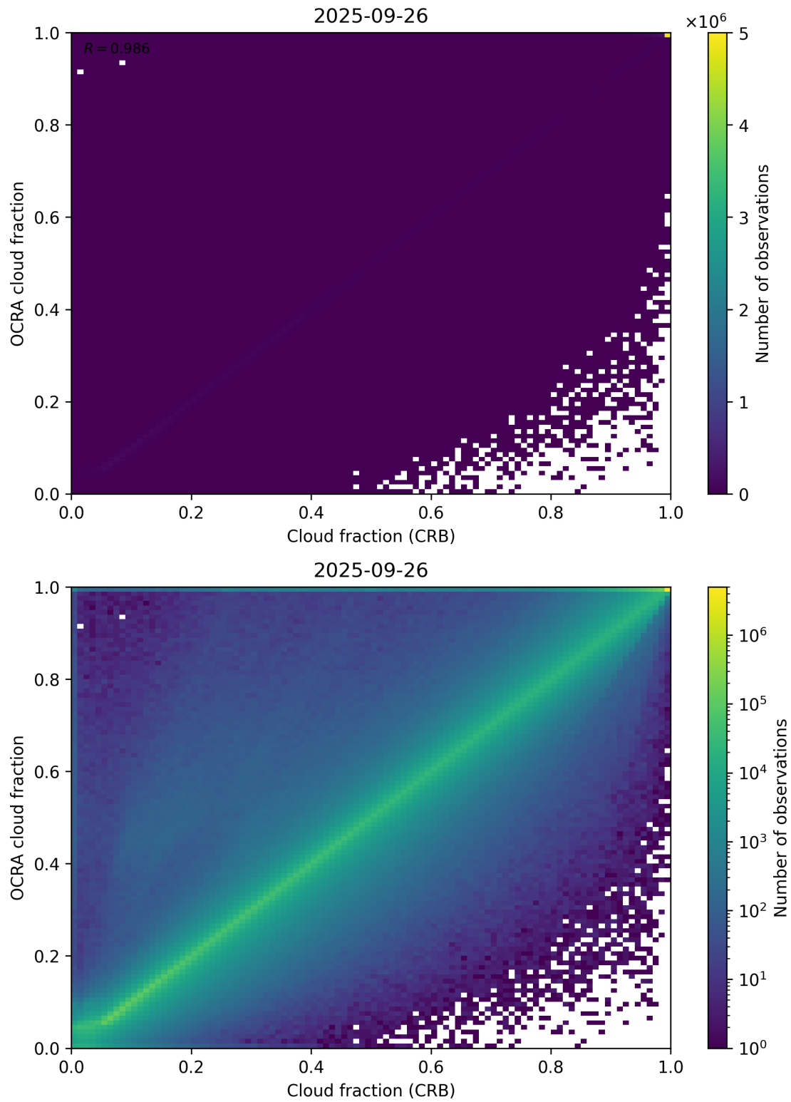
Figure 78: Scatter density plot of “Cloud fraction (CRB)” against “OCRA cloud fraction” for 2025-09-26 to 2025-09-27.
