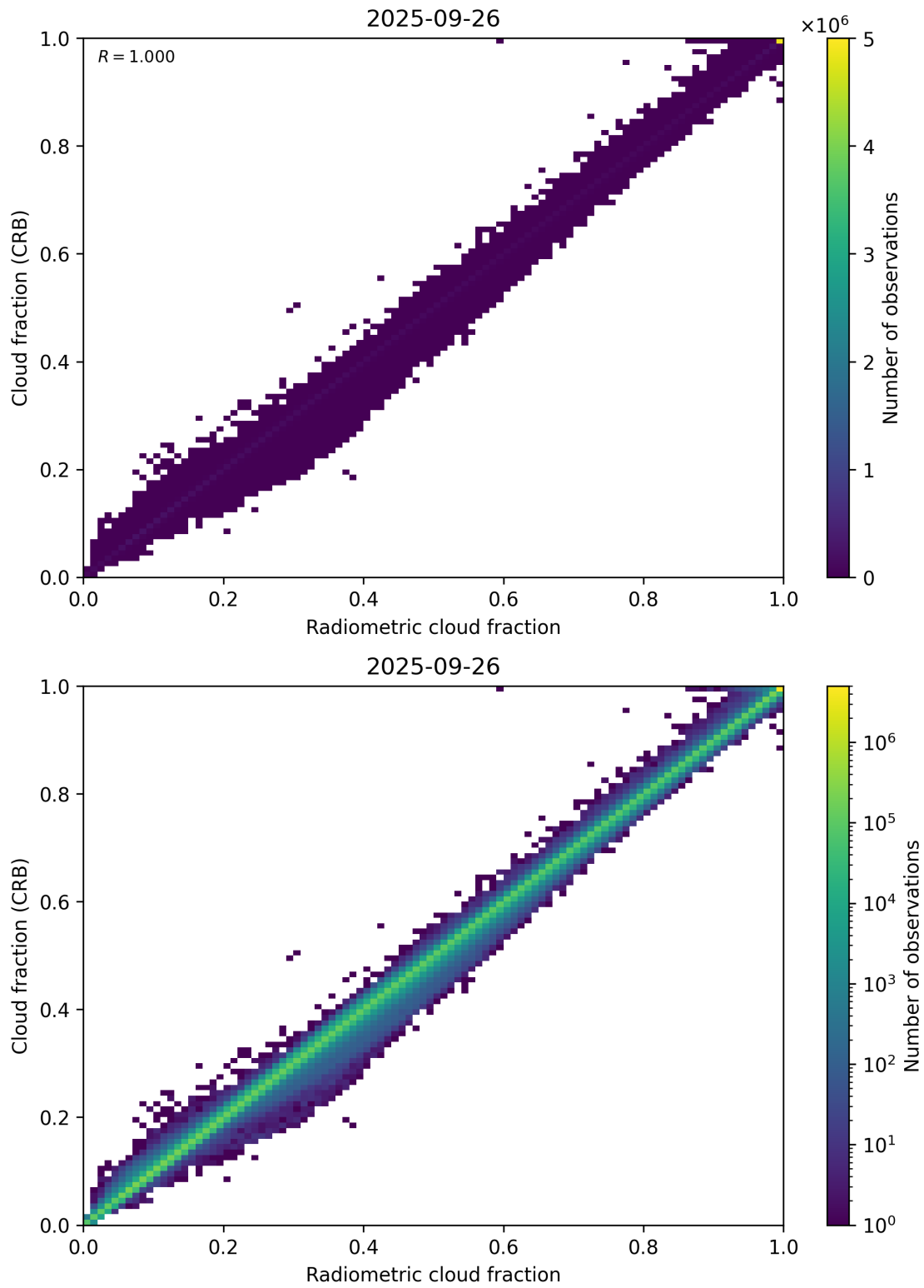
Figure 73: Scatter density plot of “Radiometric cloud fraction” against “Cloud fraction (CRB)” for 2025-09-26 to 2025-09-27.
