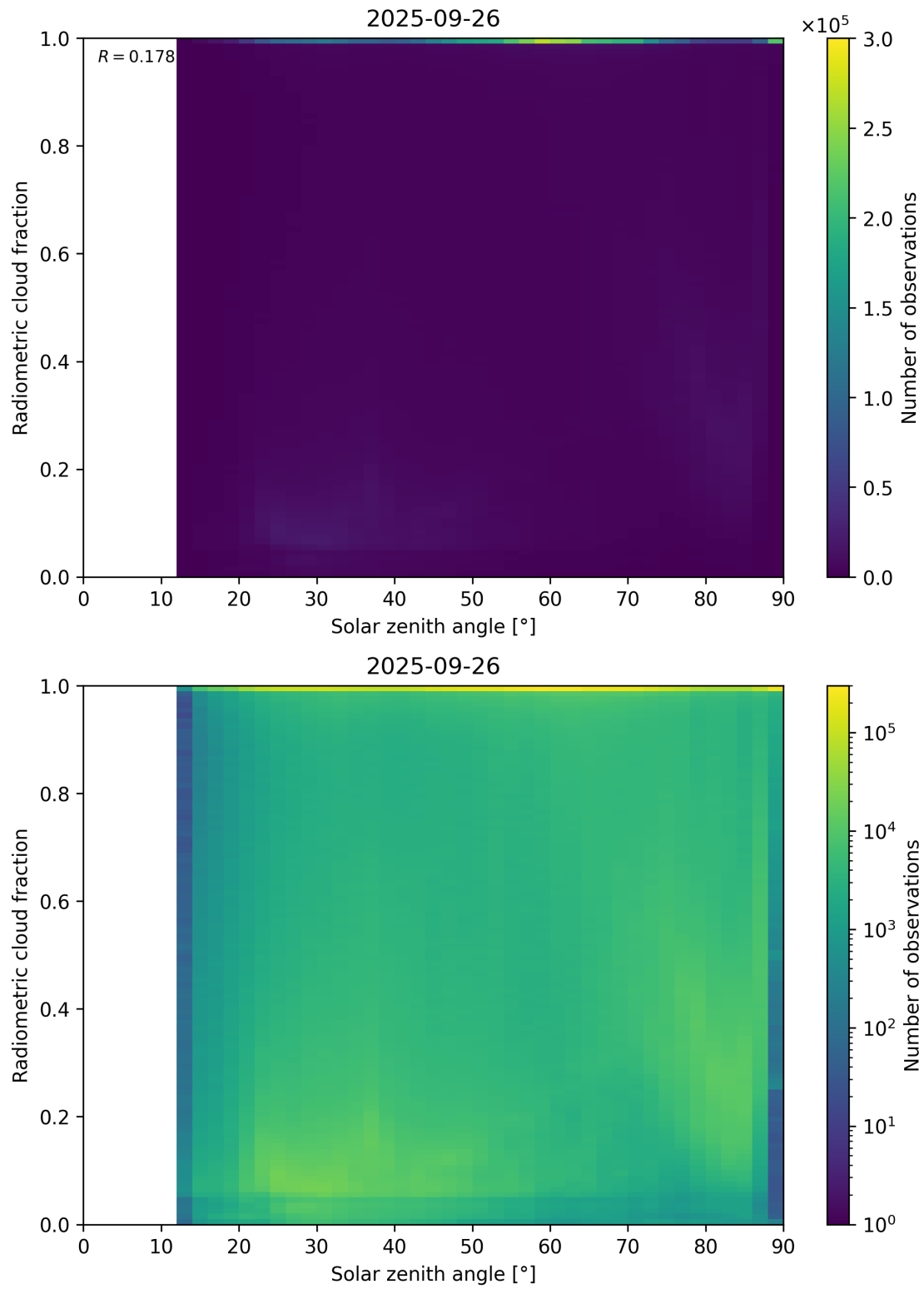
Figure 99: Scatter density plot of “Solar zenith angle” against “Radiometric cloud fraction” for 2025-09-26 to 2025-09-27.
