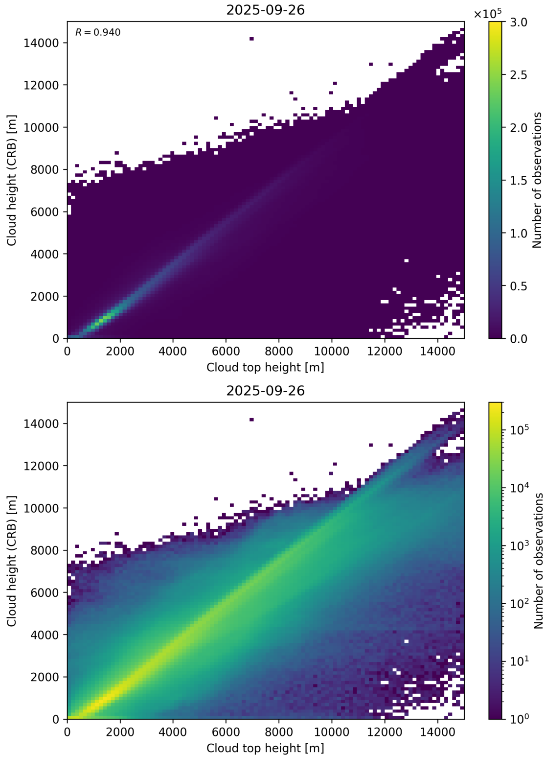
Figure 89: Scatter density plot of “Cloud top height” against “Cloud height (CRB)” for 2025-09-26 to 2025-09-27.
