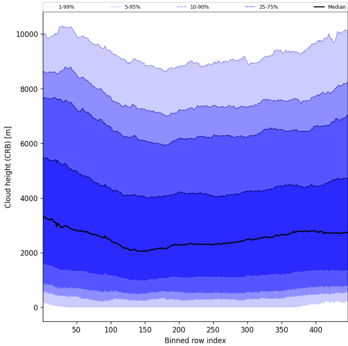
Figure 59: Along track statistics of “Cloud height (CRB)” for 2025-09-26 to 2025-09-27
