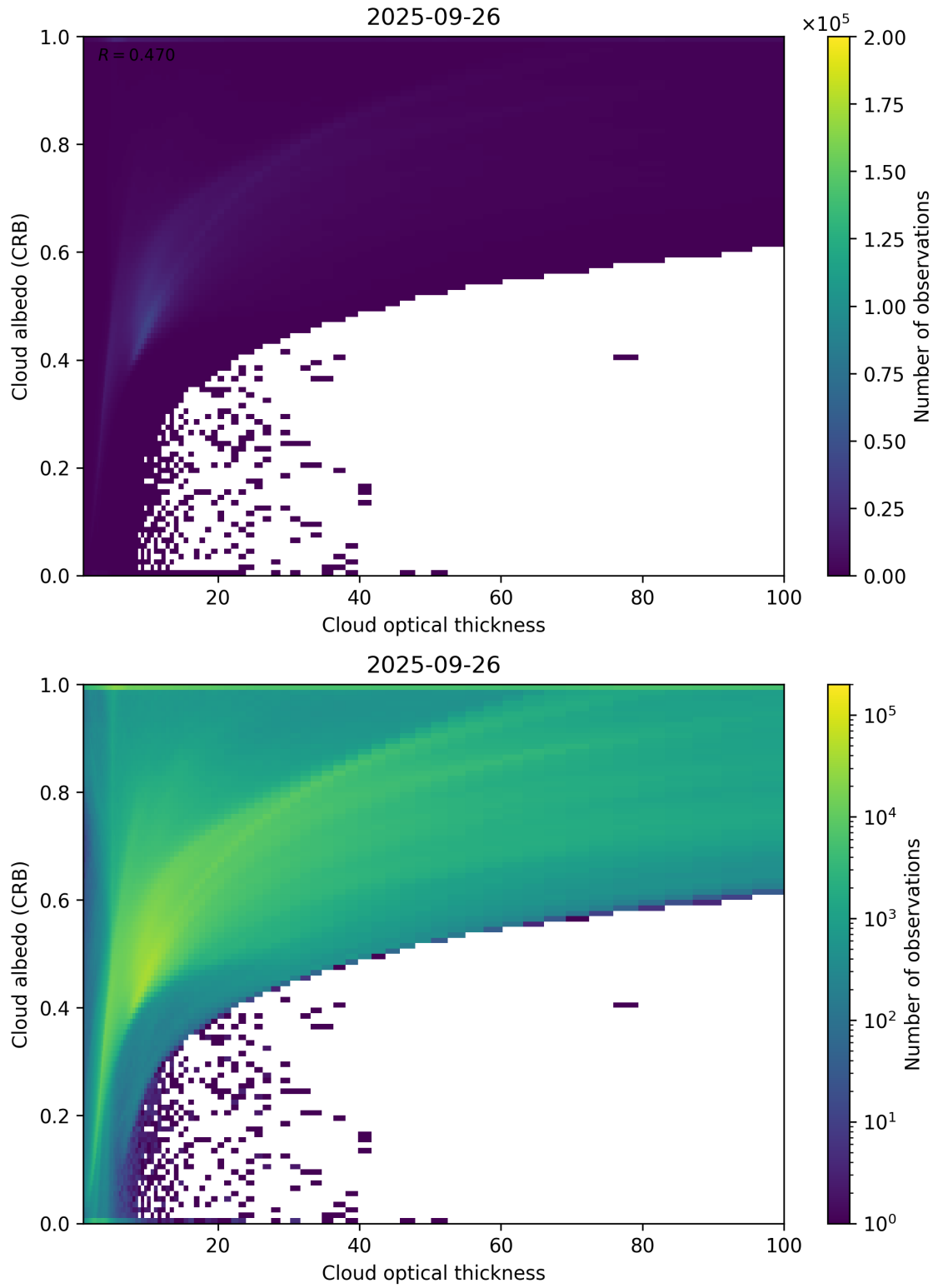
Figure 82: Scatter density plot of “Cloud optical thickness” against “Cloud albedo (CRB)” for 2025-09-26 to 2025-09-27.
