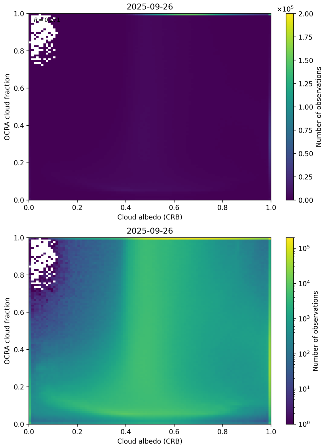
Figure 70: Scatter density plot of “Cloud albedo (CRB)” against “OCRA cloud fraction” for 2025-09-26 to 2025-09-27.
