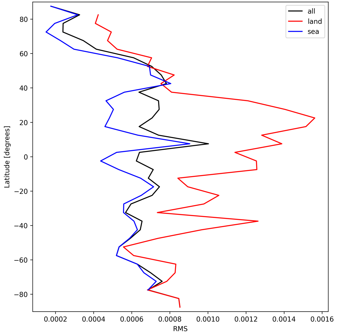
Figure 31: Zonal average of “RMS” for 2025-09-26 to 2025-09-27.
