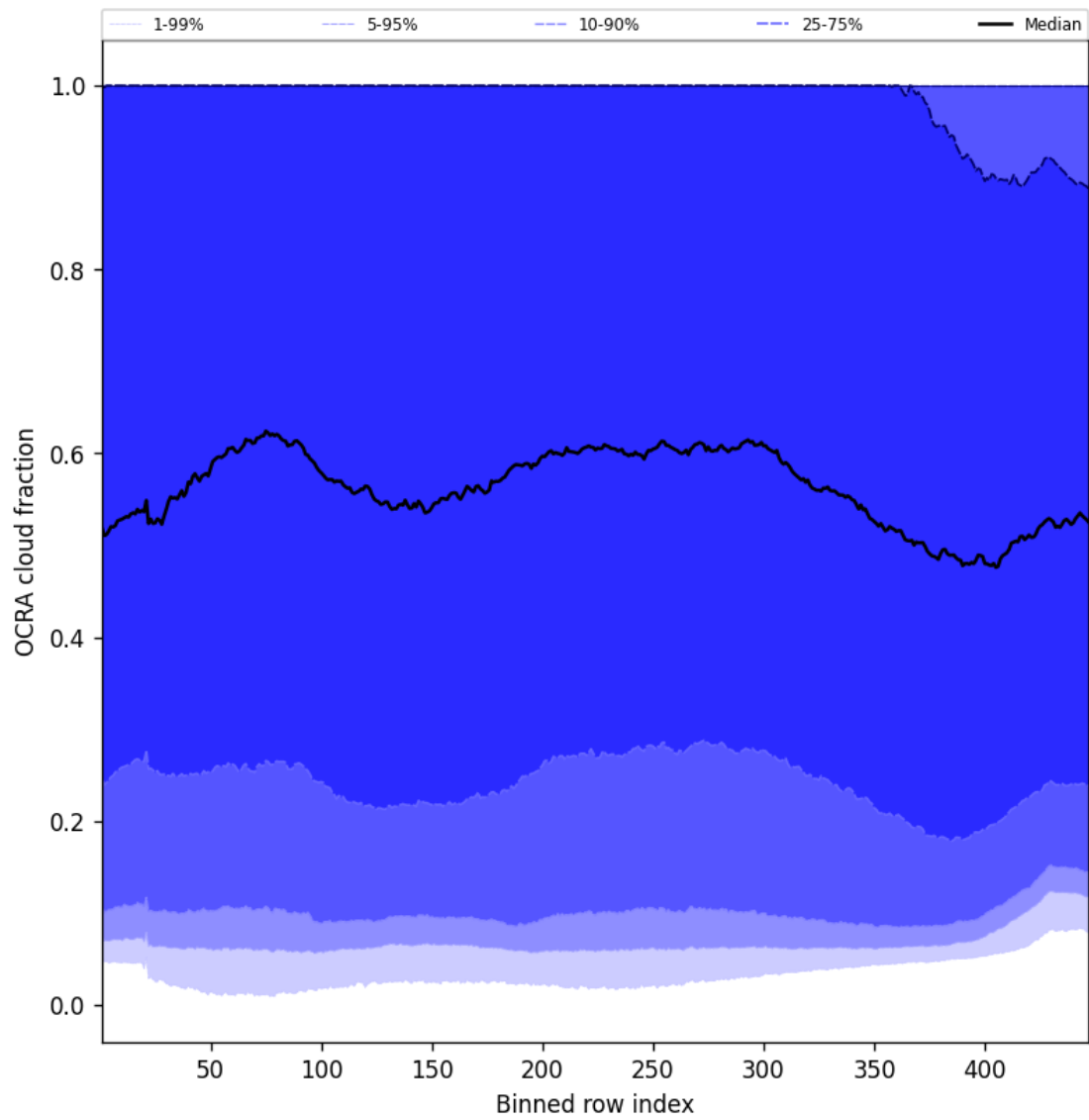
Figure 66: Along track statistics of “OCRA cloud fraction” for 2025-09-26 to 2025-09-27
