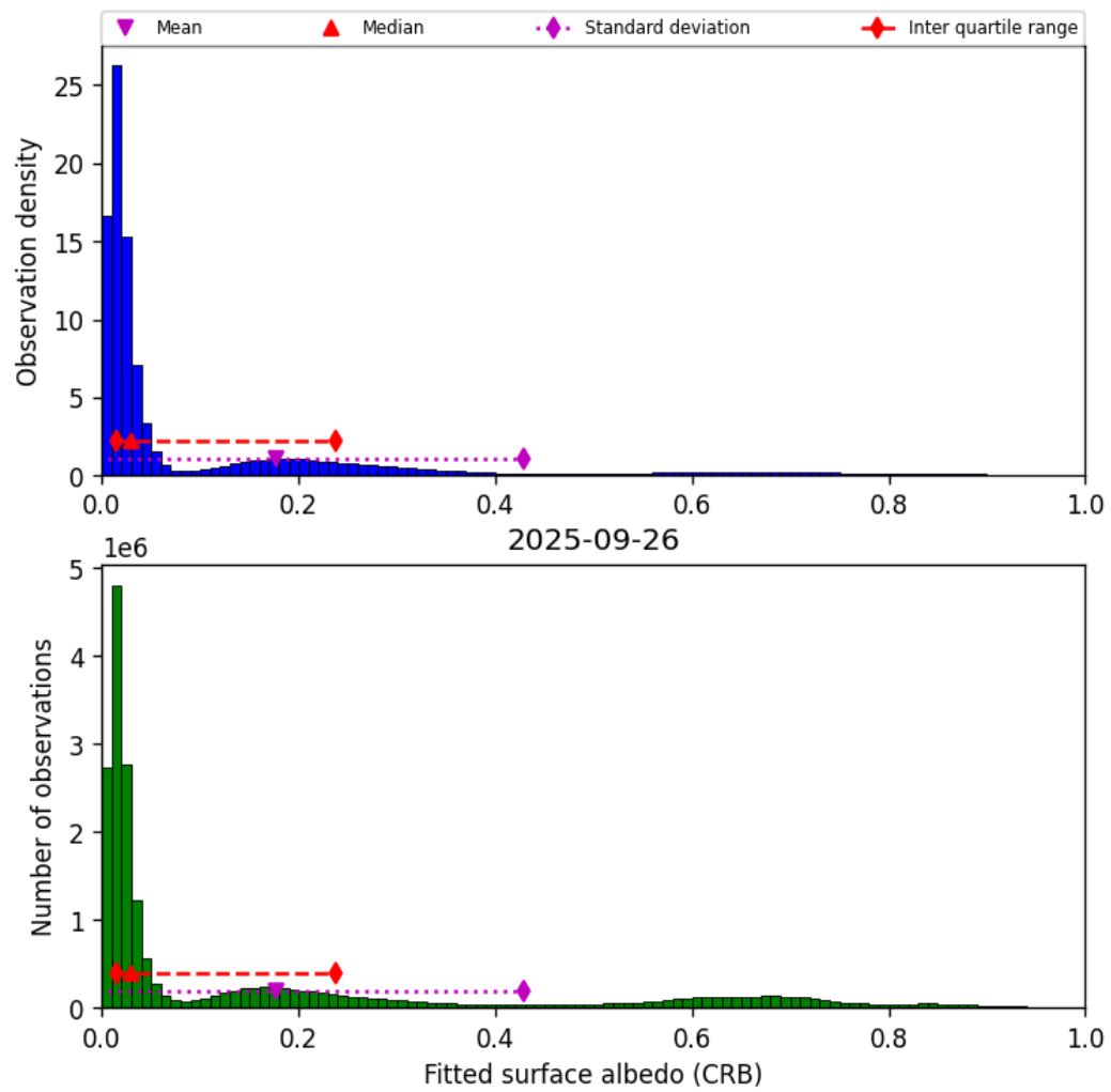
Figure 46: Histogram of “Fitted surface albedo (CRB)” for 2025-09-26 to 2025-09-27
