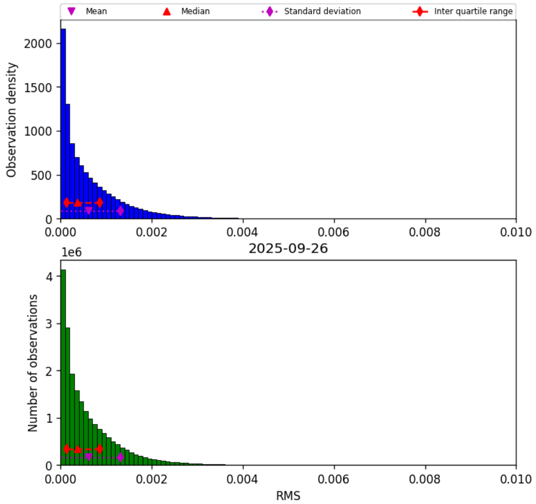
Figure 47: Histogram of “RMS” for 2025-09-26 to 2025-09-27
