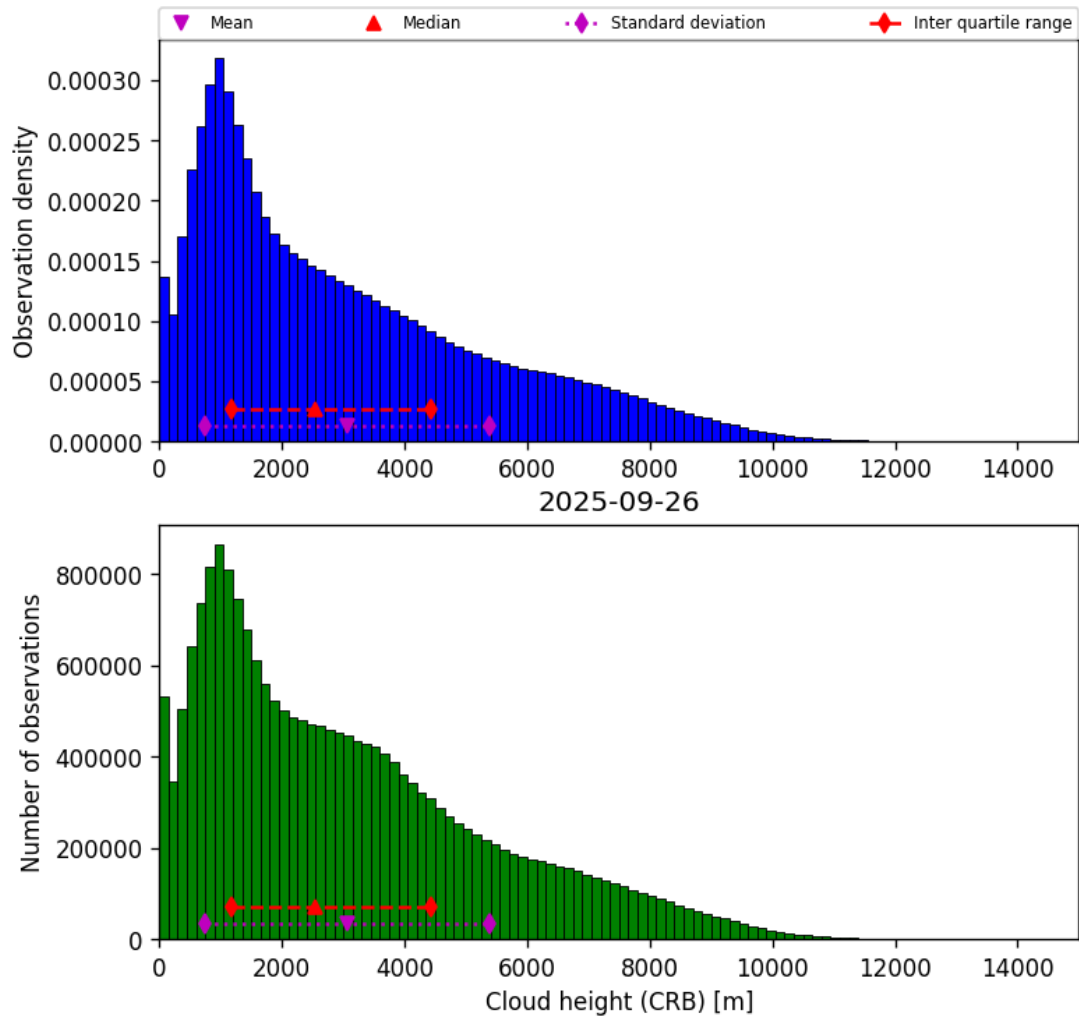
Figure 43: Histogram of “Cloud height (CRB)” for 2025-09-26 to 2025-09-27
