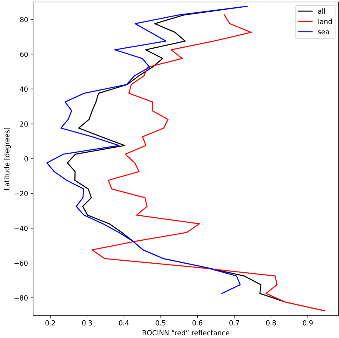
Figure 37: Zonal average of “ROCINN “red” reflectance” for 2025-09-26 to 2025-09-27.
