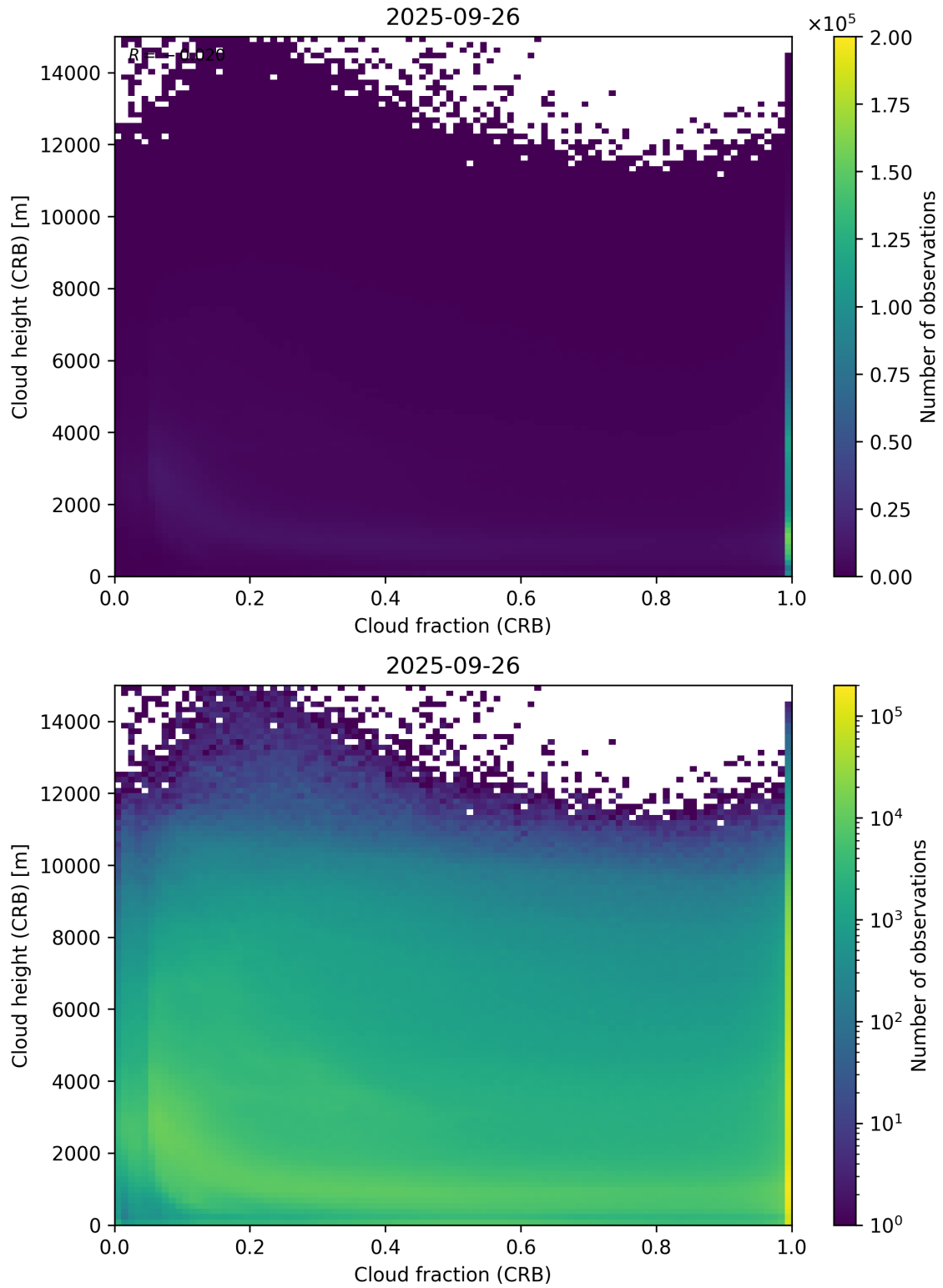
Figure 79: Scatter density plot of “Cloud fraction (CRB)” against “Cloud height (CRB)” for 2025-09-26 to 2025-09-27.
