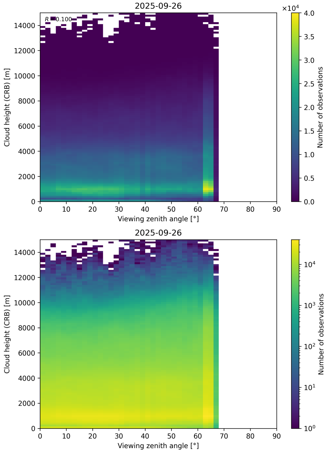
Figure 110: Scatter density plot of “Viewing zenith angle” against “Cloud height (CRB)” for 2025-09-26 to 2025-09-27.
