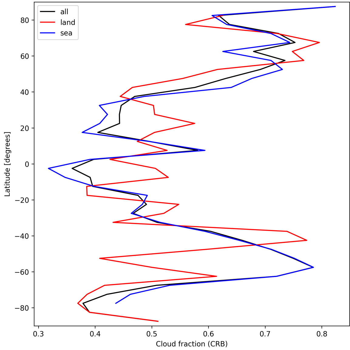
Figure 26: Zonal average of “Cloud fraction (CRB)” for 2025-09-26 to 2025-09-27.
