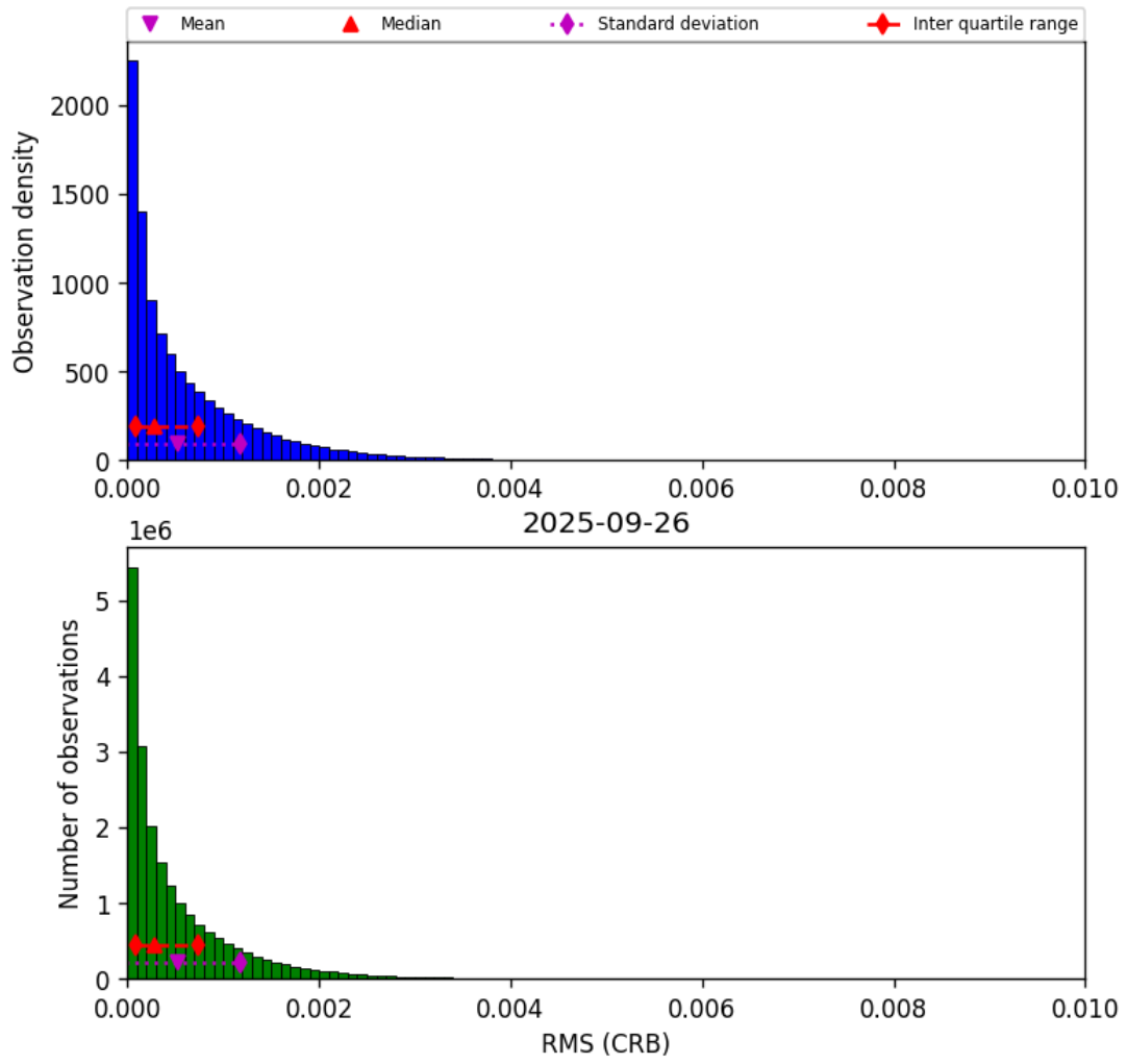
Figure 48: Histogram of “RMS (CRB)” for 2025-09-26 to 2025-09-27
