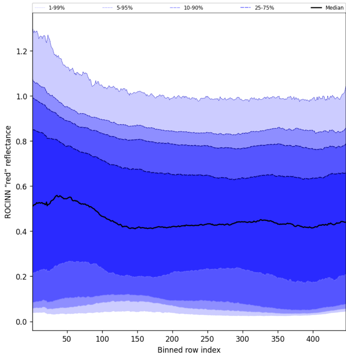
Figure 69: Along track statistics of “ROCINN “red” reflectance” for 2025-09-26 to 2025-09-27
