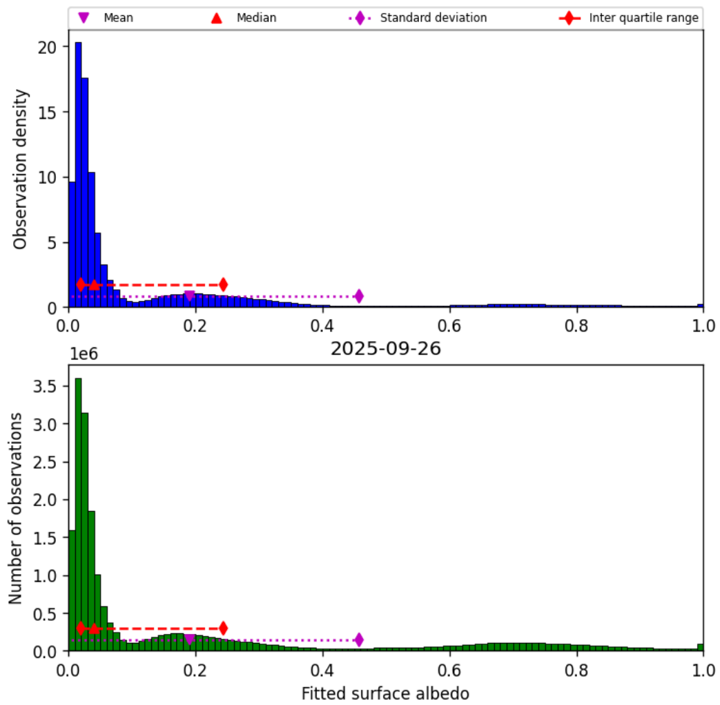
Figure 45: Histogram of “Fitted surface albedo” for 2025-09-26 to 2025-09-27
