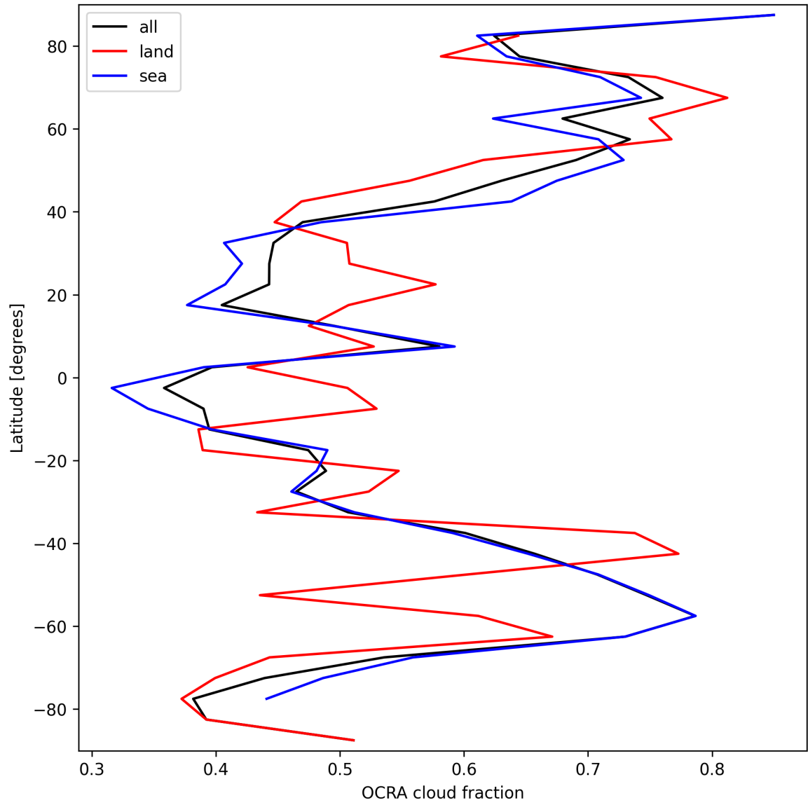
Figure 34: Zonal average of “OCRA cloud fraction” for 2025-09-26 to 2025-09-27.
