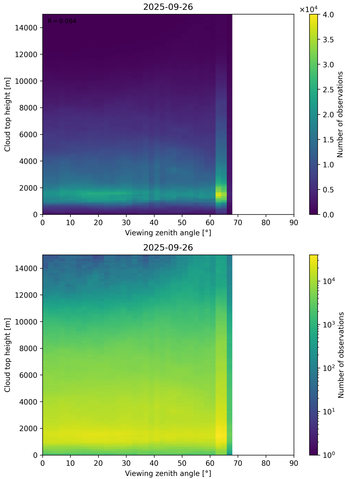
Figure 112: Scatter density plot of “Viewing zenith angle” against “Cloud top height” for 2025-09-26 to 2025-09-27.
