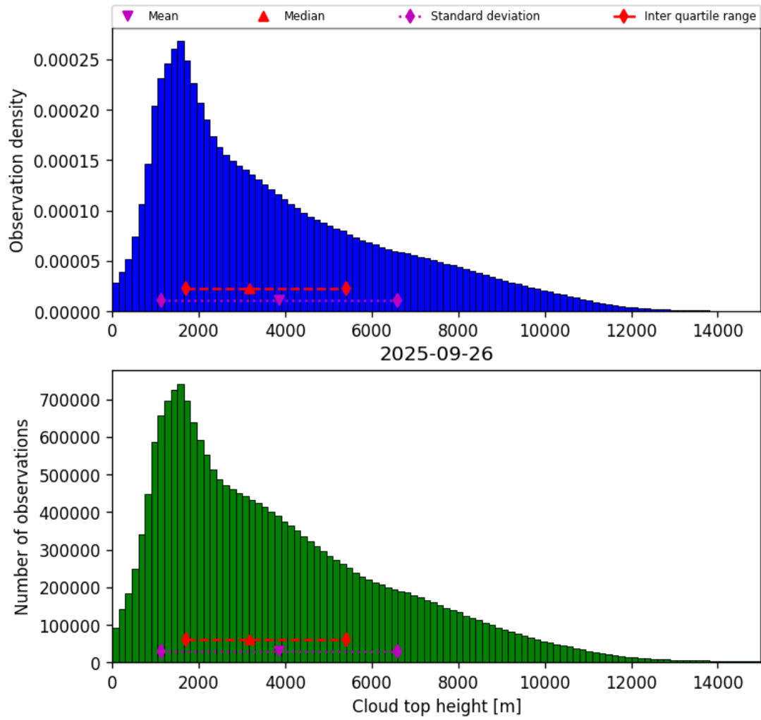
Figure 40: Histogram of “Cloud top height” for 2025-09-26 to 2025-09-27
