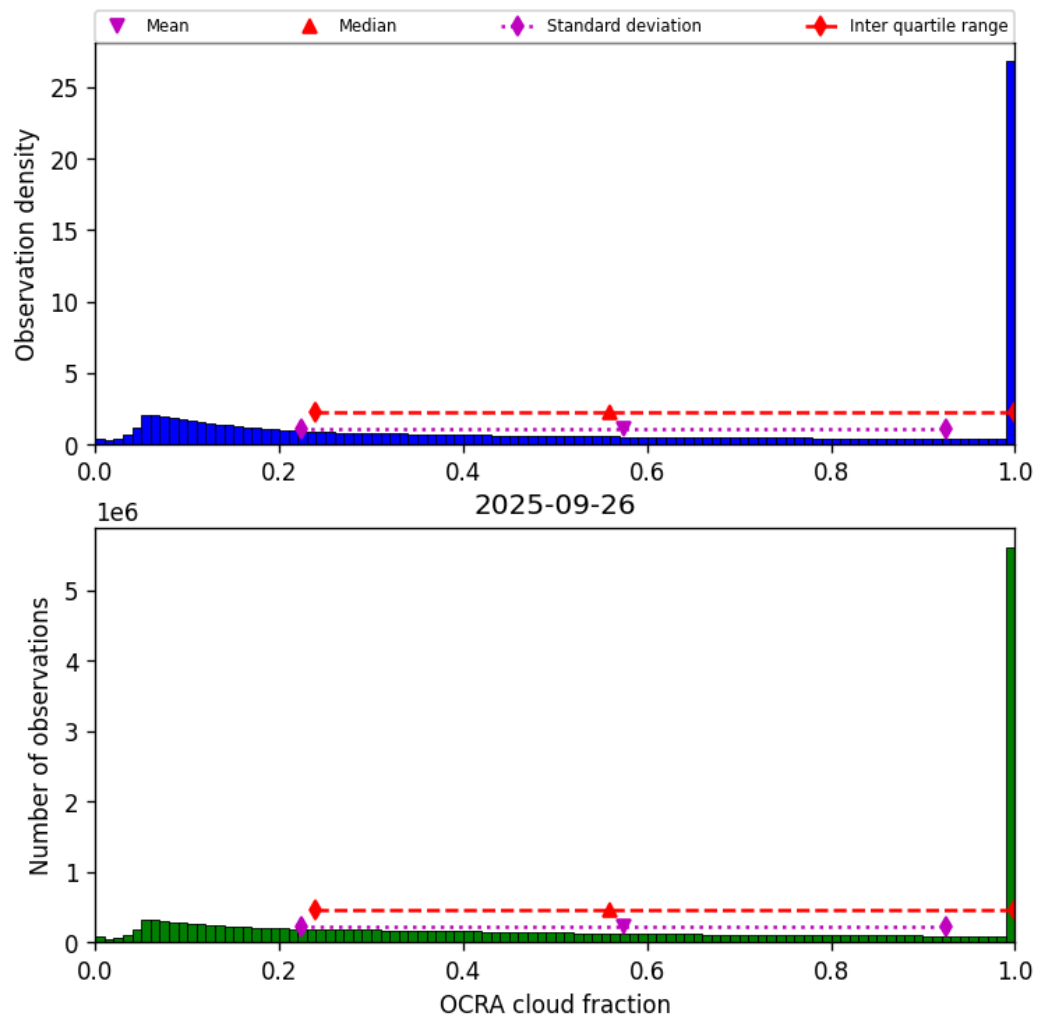
Figure 50: Histogram of “OCRA cloud fraction” for 2025-09-26 to 2025-09-27
