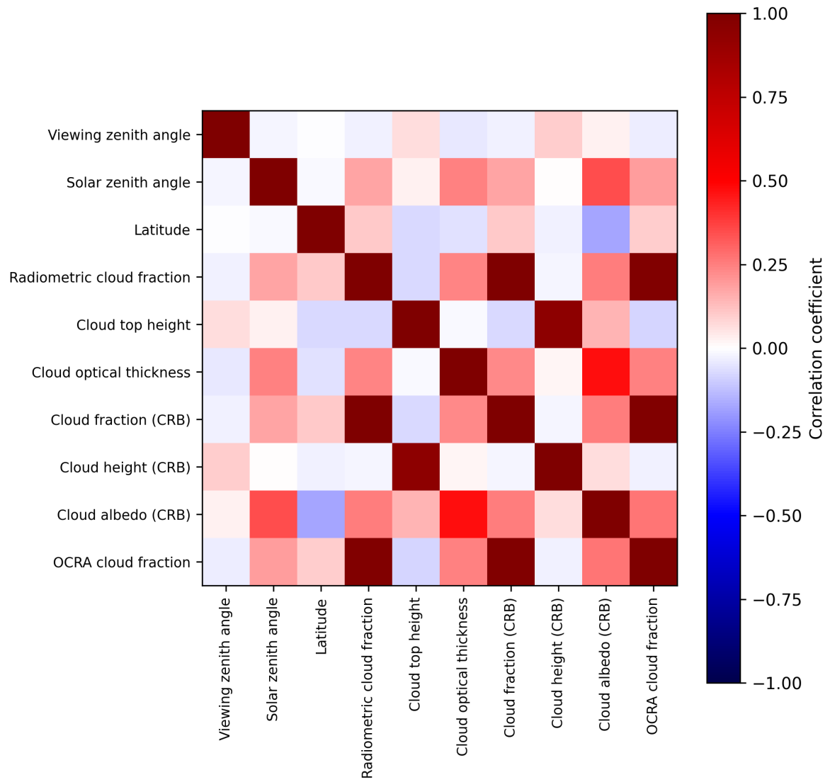
Figure 2: Map of correlation matrix for 2025-09-26 to 2025-09-27.
