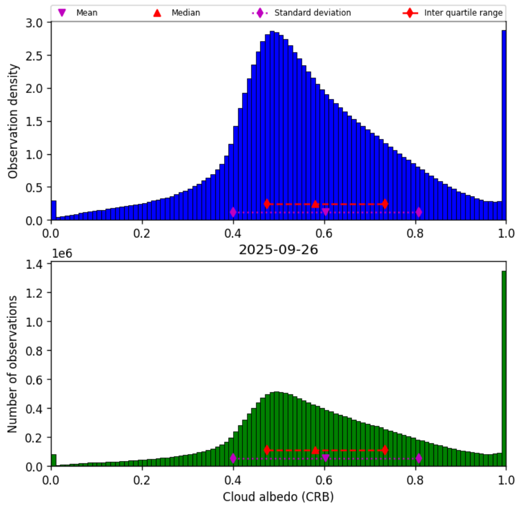
Figure 44: Histogram of “Cloud albedo (CRB)” for 2025-09-26 to 2025-09-27
