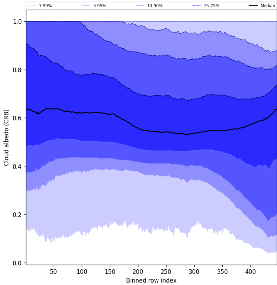
Figure 60: Along track statistics of “Cloud albedo (CRB)” for 2025-09-26 to 2025-09-27
