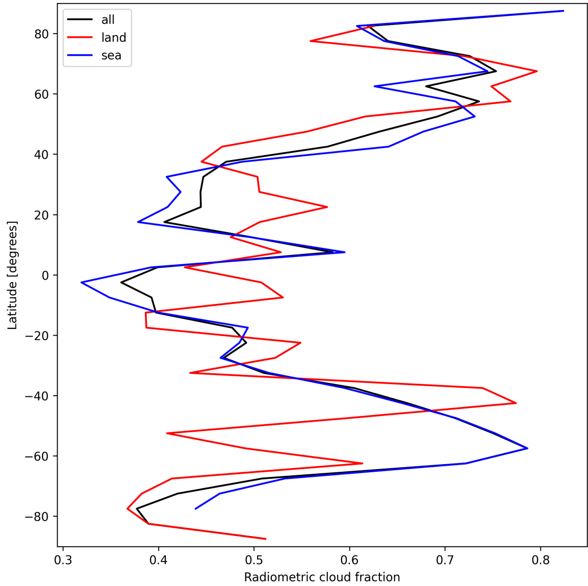
Figure 23: Zonal average of “Radiometric cloud fraction” for 2025-09-26 to 2025-09-27.
