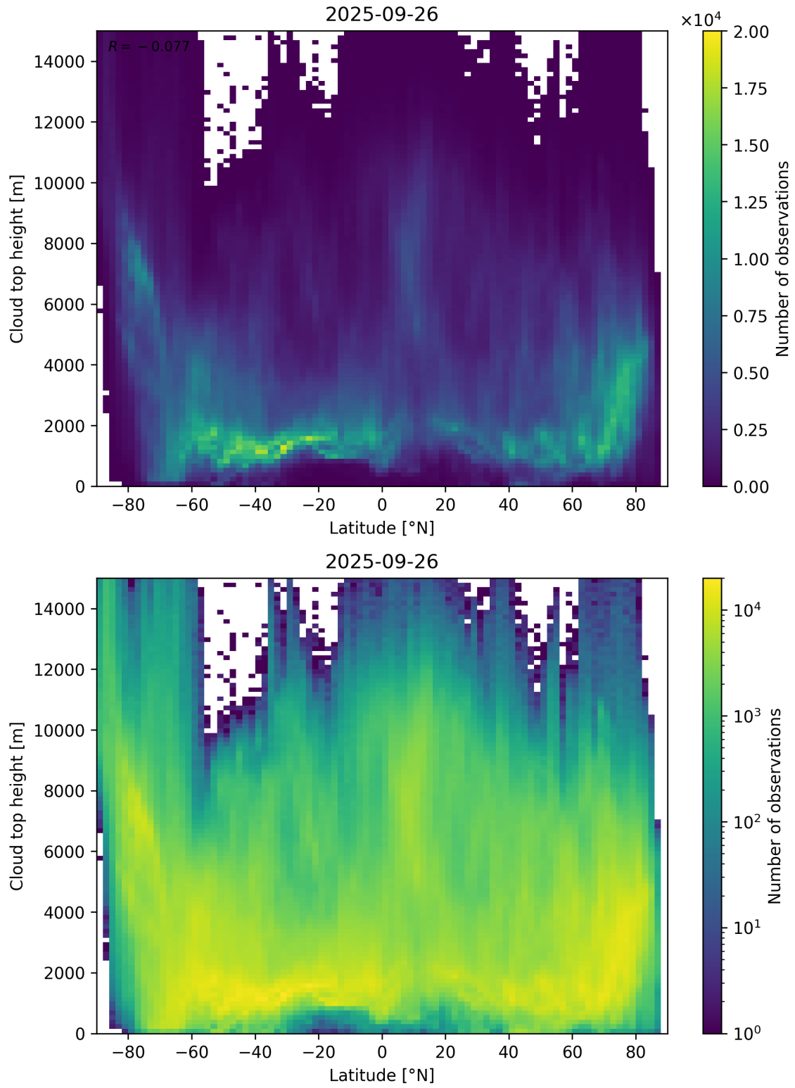
Figure 97: Scatter density plot of “Latitude” against “Cloud top height” for 2025-09-26 to 2025-09-27.
