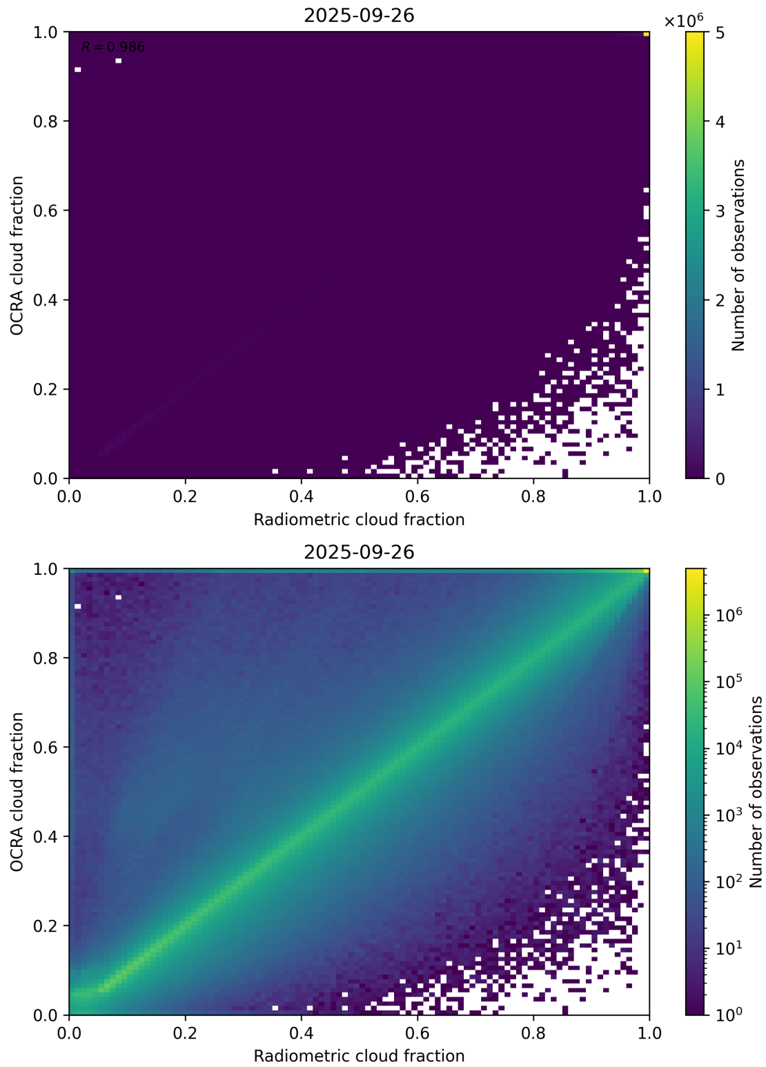
Figure 72: Scatter density plot of “Radiometric cloud fraction” against “OCRA cloud fraction” for 2025-09-26 to 2025-09-27.
