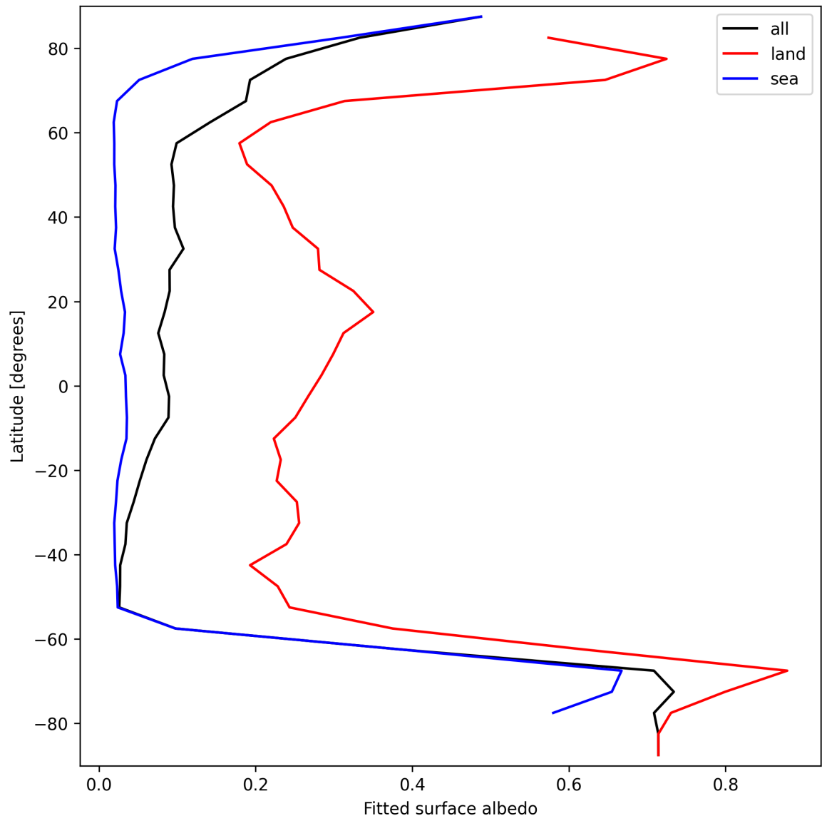
Figure 29: Zonal average of “Fitted surface albedo” for 2025-09-26 to 2025-09-27.
