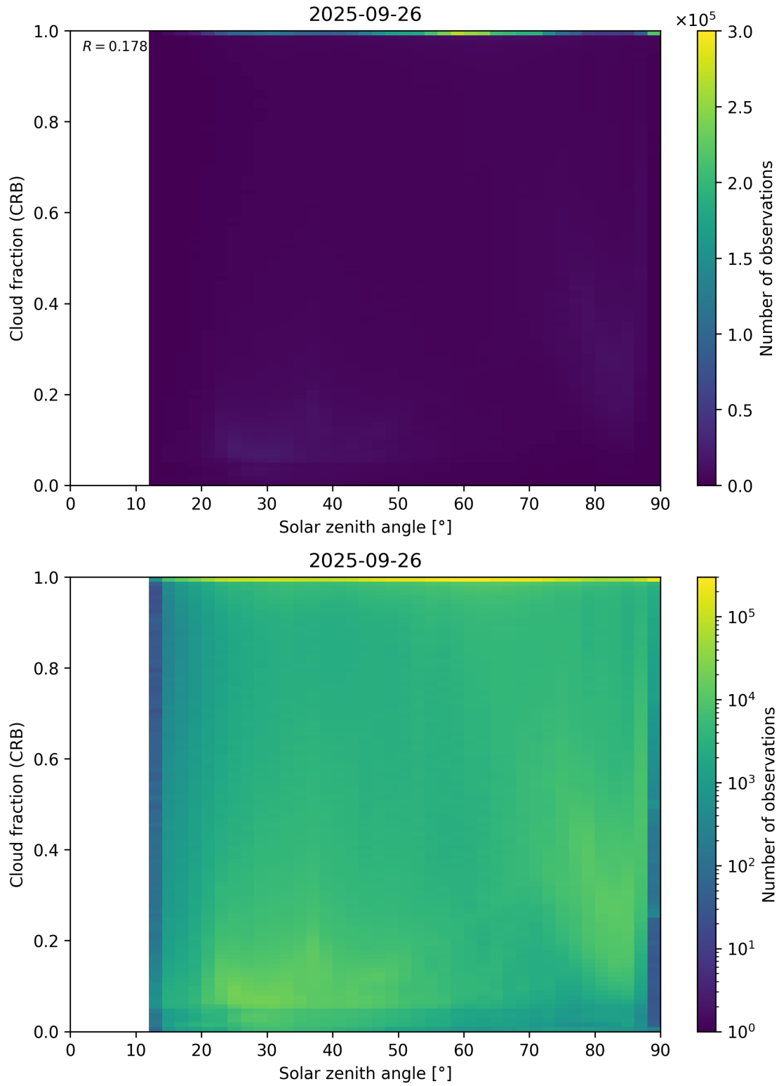
Figure 101: Scatter density plot of “Solar zenith angle” against “Cloud fraction (CRB)” for 2025-09-26 to 2025-09-27.
