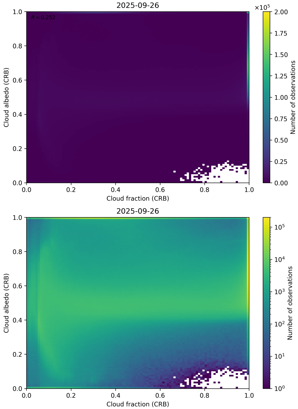
Figure 77: Scatter density plot of “Cloud fraction (CRB)” against “Cloud albedo (CRB)” for 2025-09-26 to 2025-09-27.
