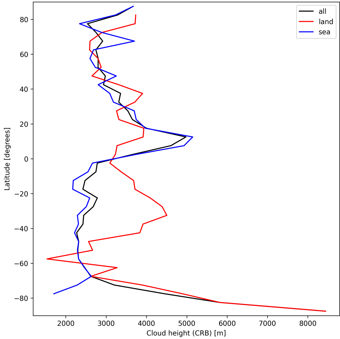
Figure 27: Zonal average of “Cloud height (CRB)” for 2025-09-26 to 2025-09-27.
