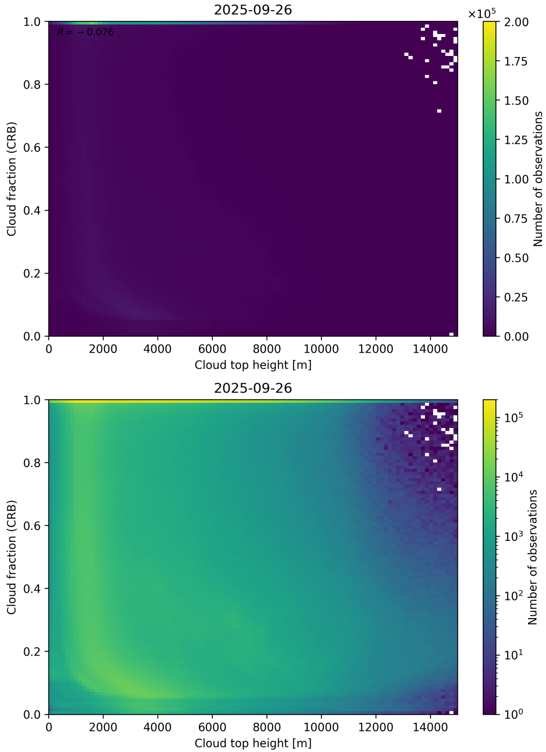
Figure 88: Scatter density plot of “Cloud top height” against “Cloud fraction (CRB)” for 2025-09-26 to 2025-09-27.
