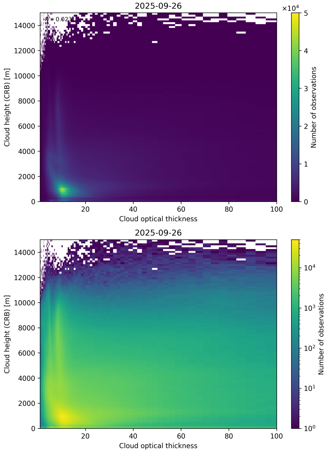
Figure 85: Scatter density plot of “Cloud optical thickness” against “Cloud height (CRB)” for 2025-09-26 to 2025-09-27.
