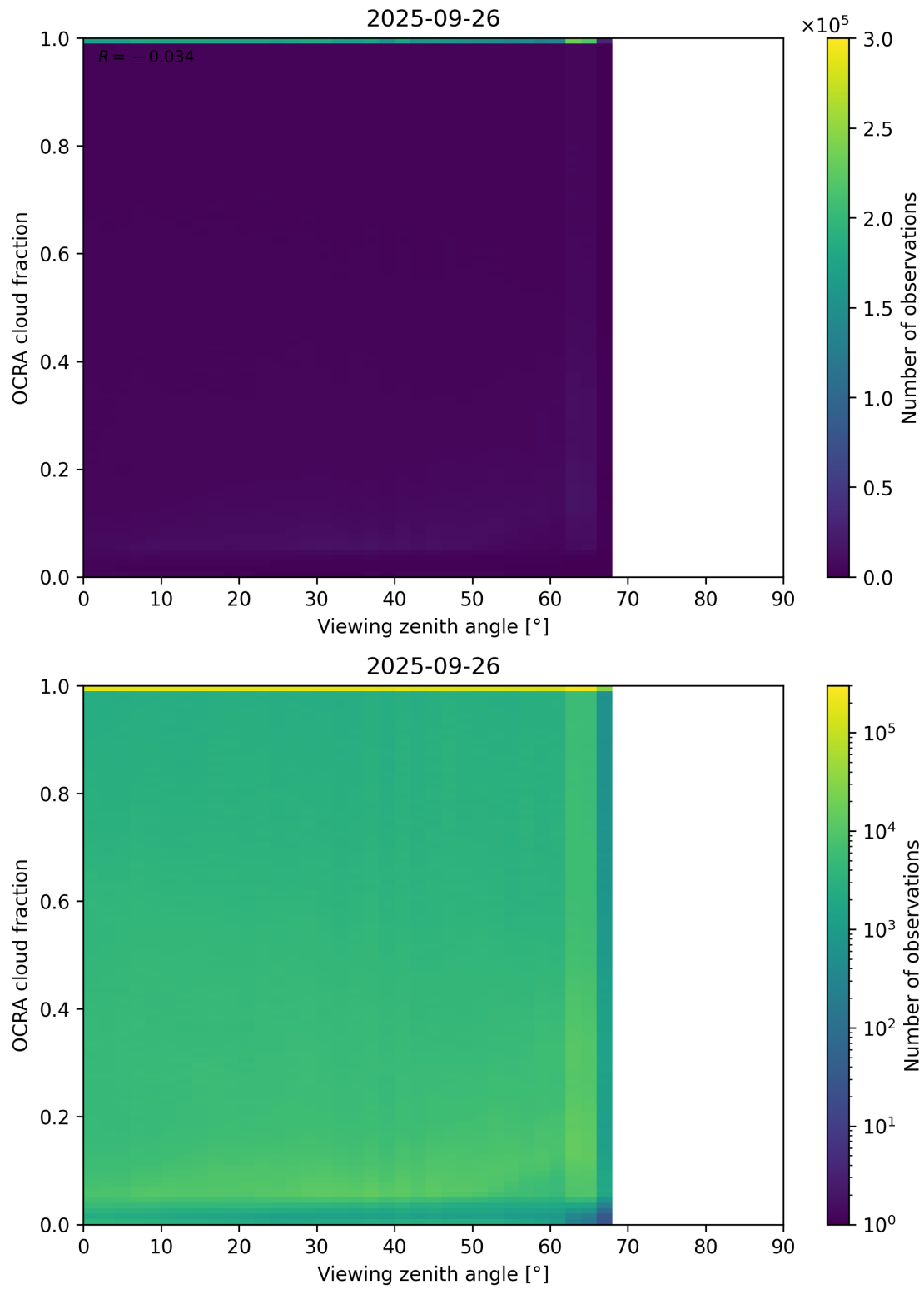
Figure 108: Scatter density plot of “Viewing zenith angle” against “OCRA cloud fraction” for 2025-09-26 to 2025-09-27.
