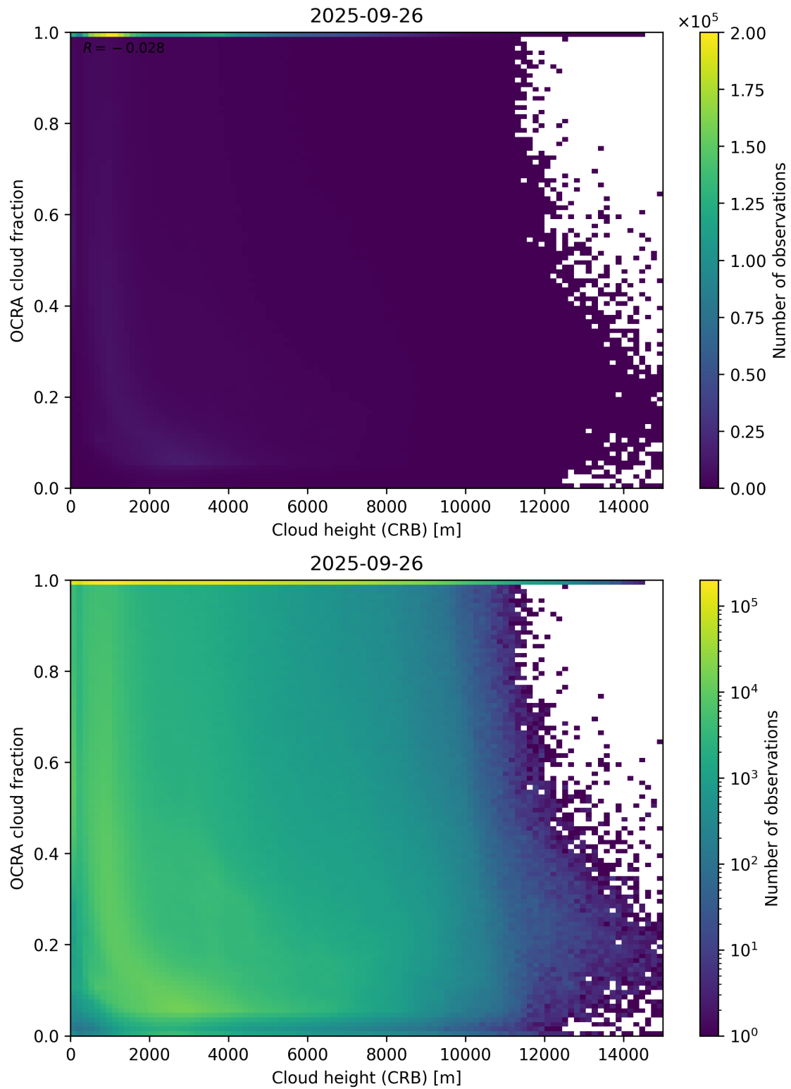
Figure 81: Scatter density plot of “Cloud height (CRB)” against “OCRA cloud fraction” for 2025-09-26 to 2025-09-27.
