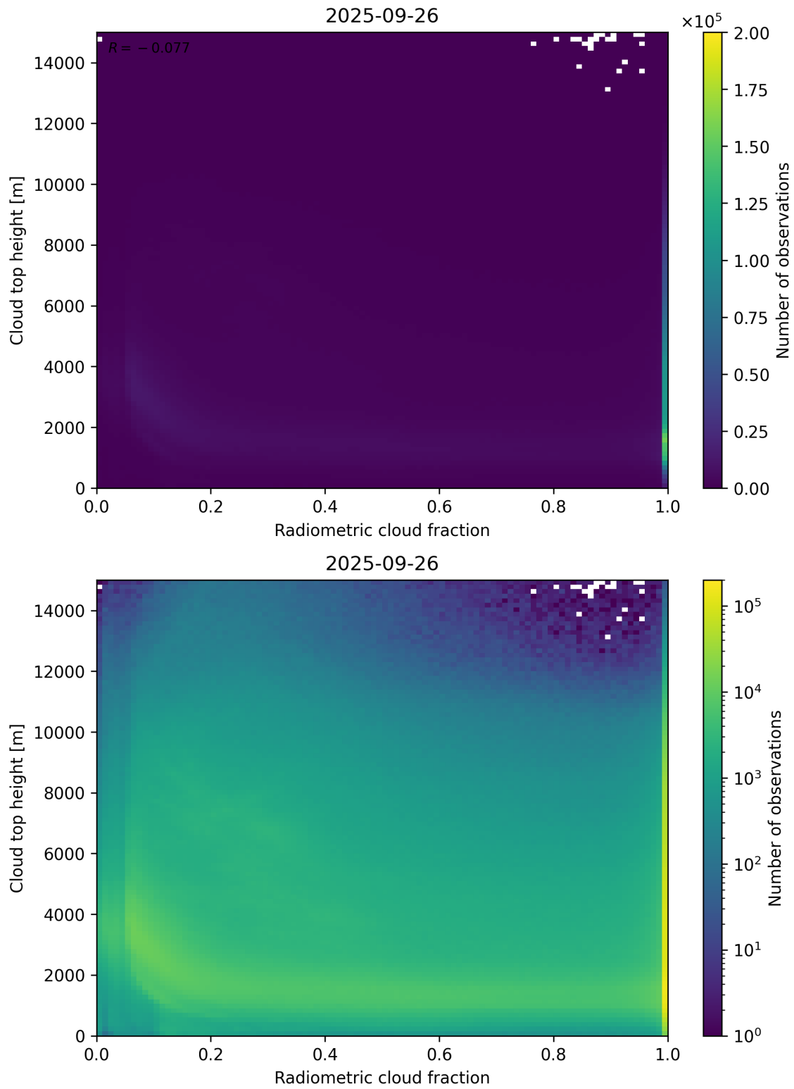
Figure 76: Scatter density plot of “Radiometric cloud fraction” against “Cloud top height” for 2025-09-26 to 2025-09-27.
