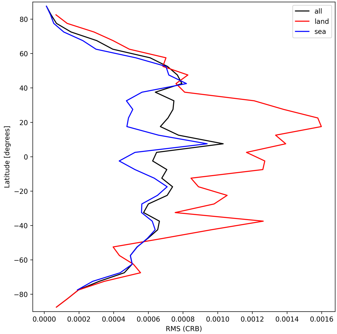
Figure 32: Zonal average of “RMS (CRB)” for 2025-09-26 to 2025-09-27.
