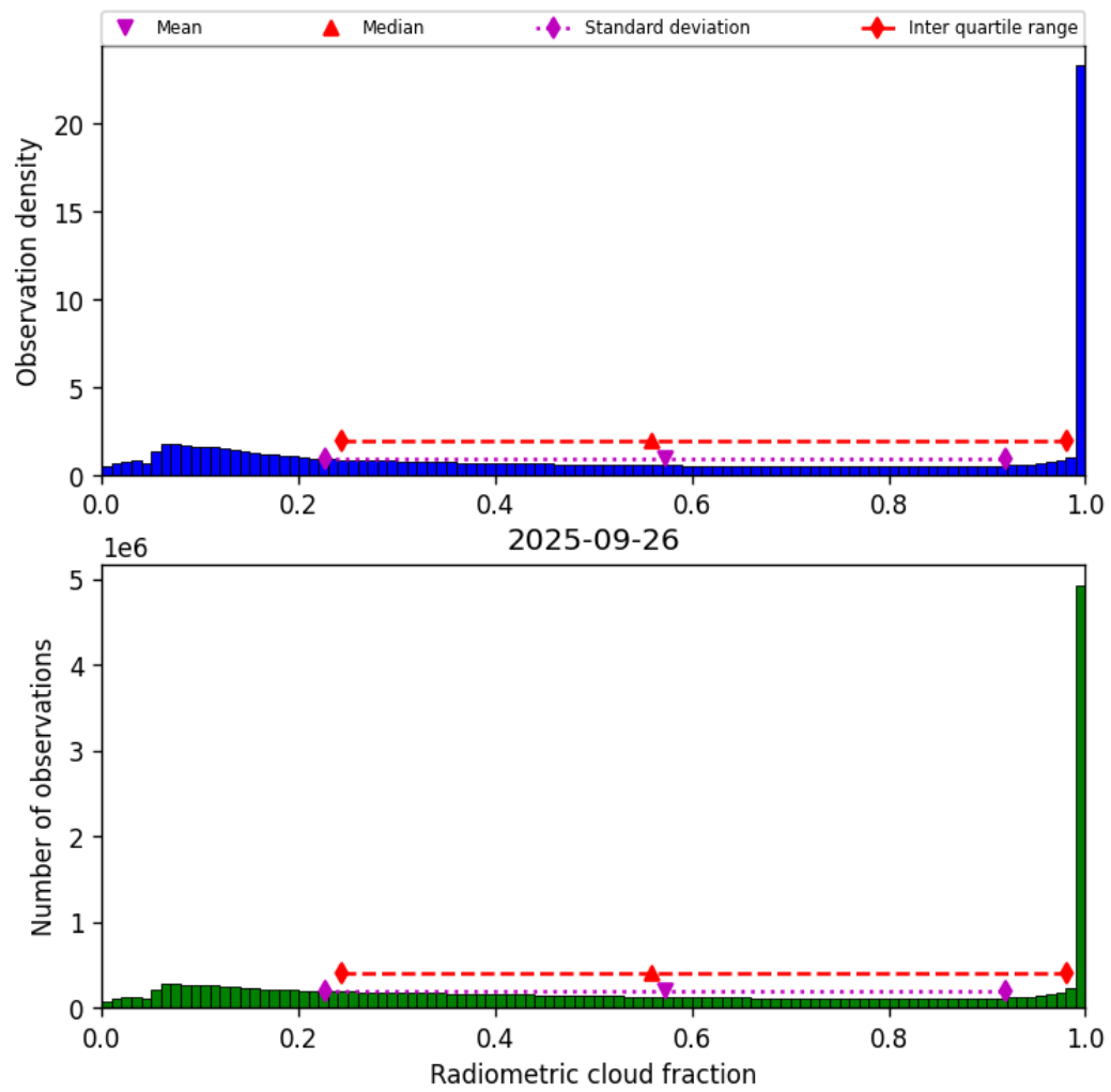
Figure 39: Histogram of “Radiometric cloud fraction” for 2025-09-26 to 2025-09-27
