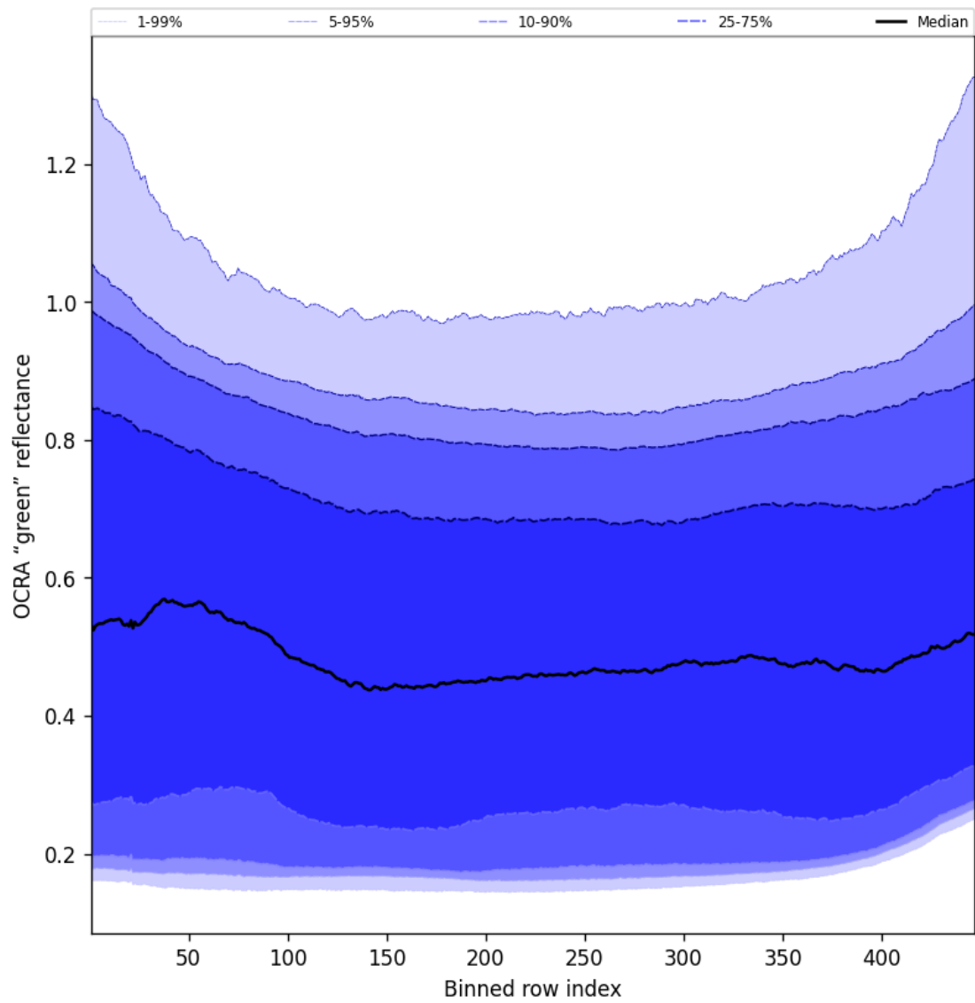
Figure 68: Along track statistics of “OCRA “green” reflectance” for 2025-09-26 to 2025-09-27
