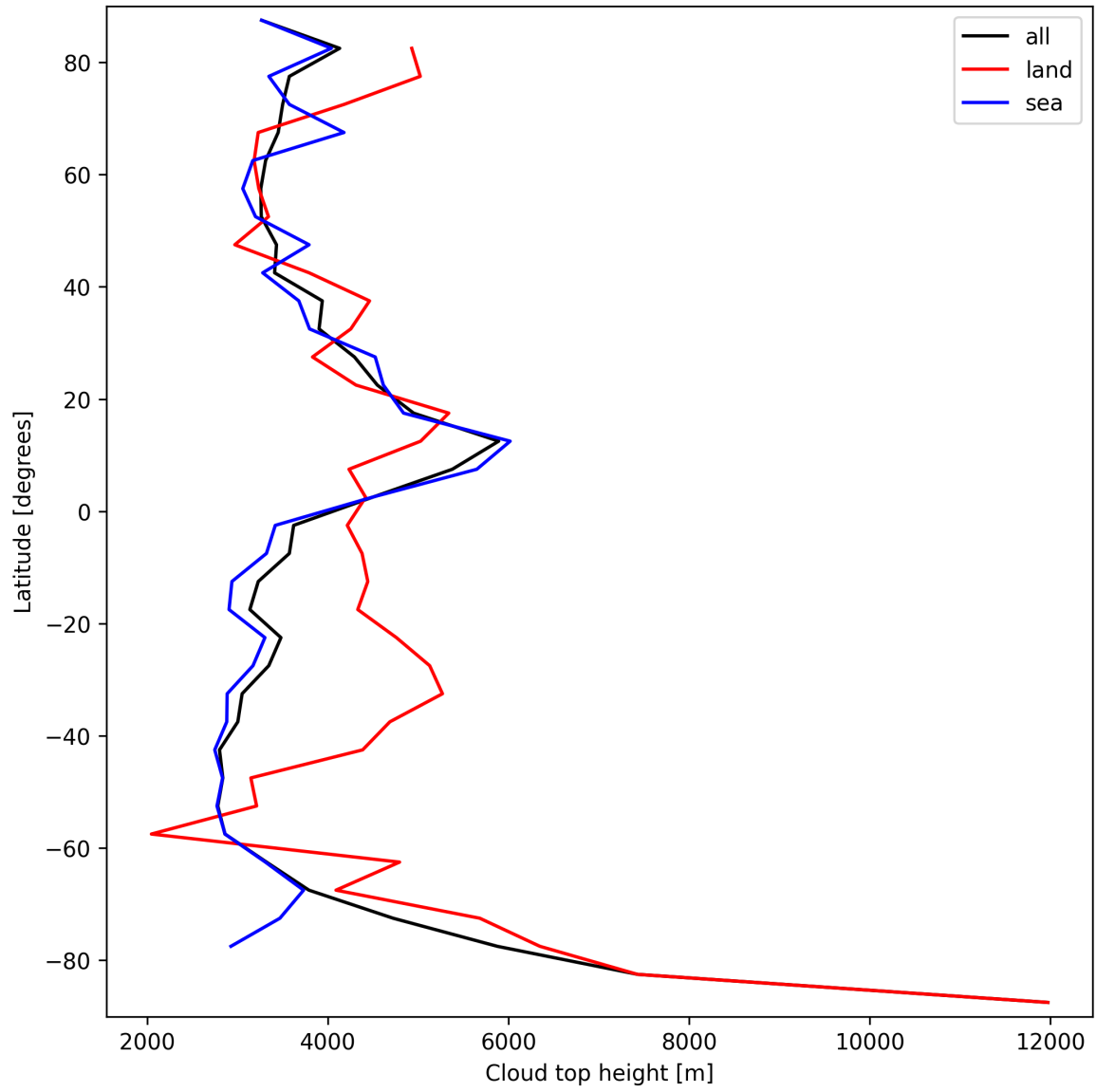
Figure 24: Zonal average of “Cloud top height” for 2025-09-26 to 2025-09-27.
