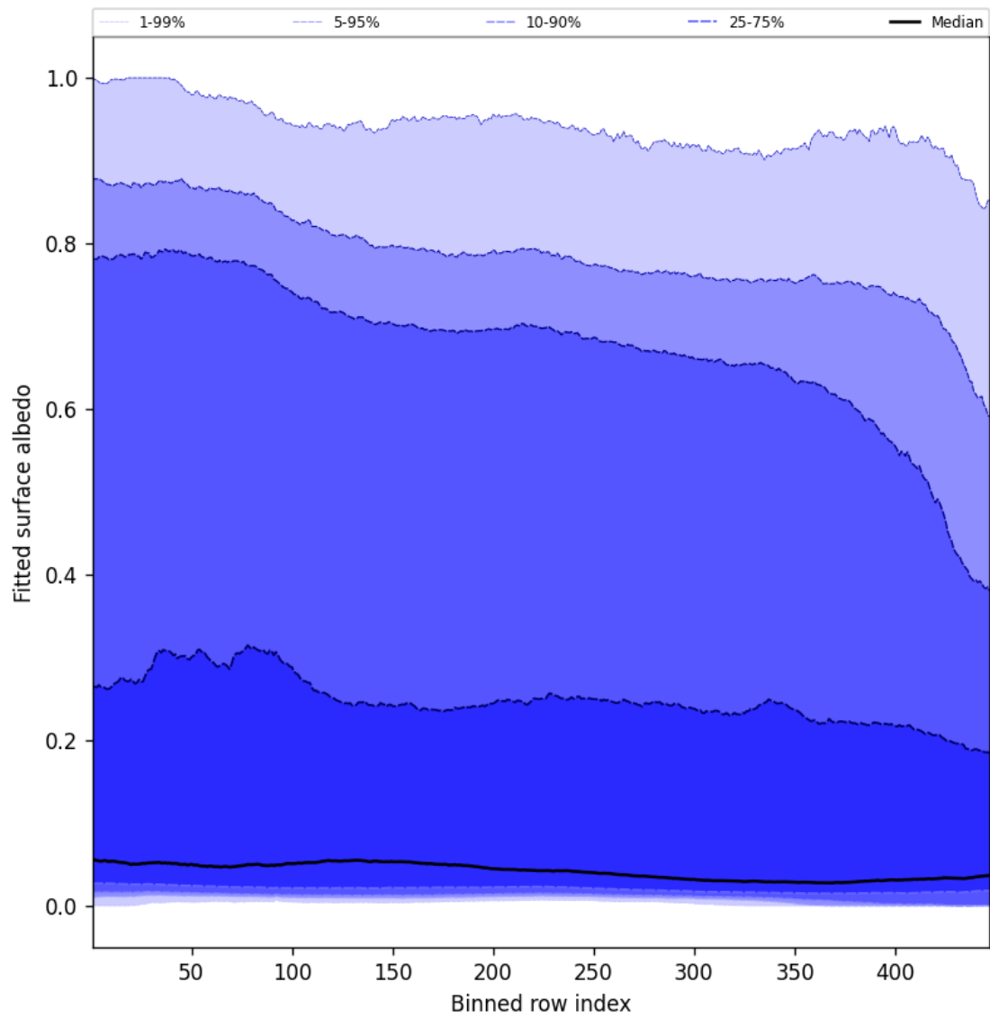
Figure 61: Along track statistics of “Fitted surface albedo” for 2025-09-26 to 2025-09-27
