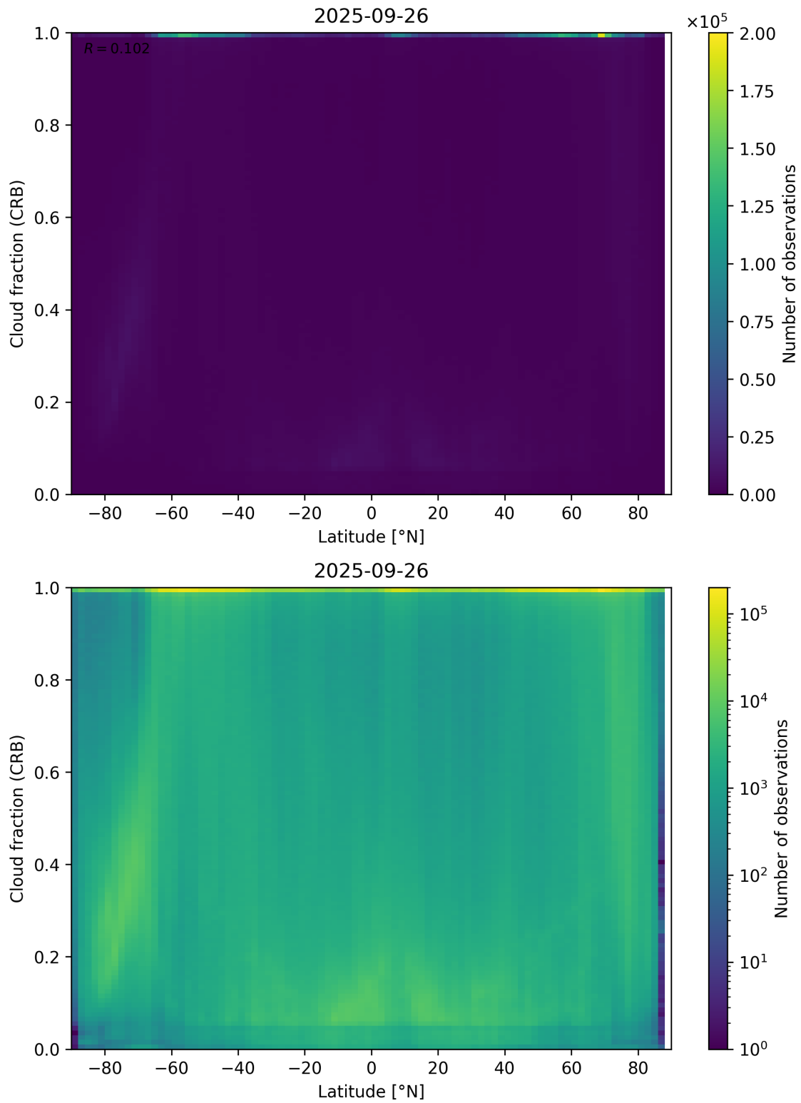
Figure 94: Scatter density plot of “Latitude” against “Cloud fraction (CRB)” for 2025-09-26 to 2025-09-27.
