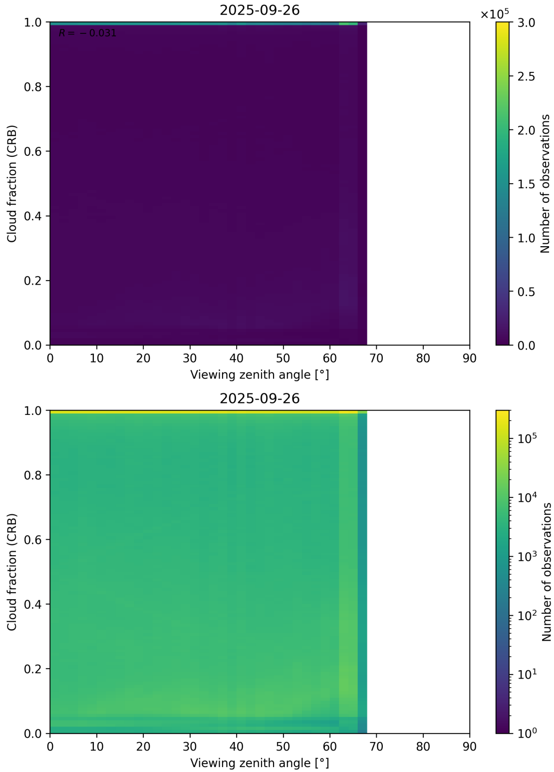
Figure 109: Scatter density plot of “Viewing zenith angle” against “Cloud fraction (CRB)” for 2025-09-26 to 2025-09-27.
