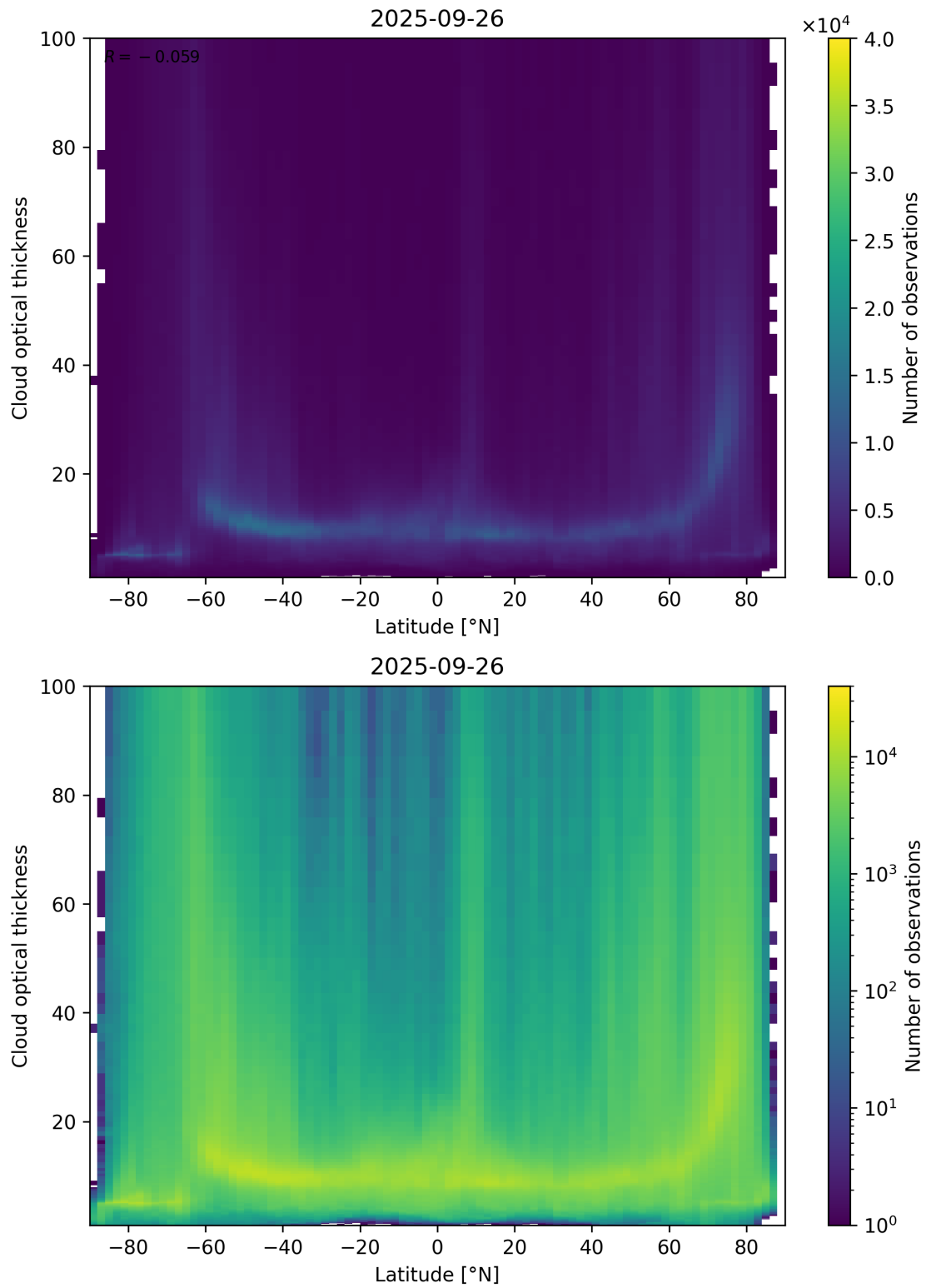
Figure 96: Scatter density plot of “Latitude” against “Cloud optical thickness” for 2025-09-26 to 2025-09-27.
