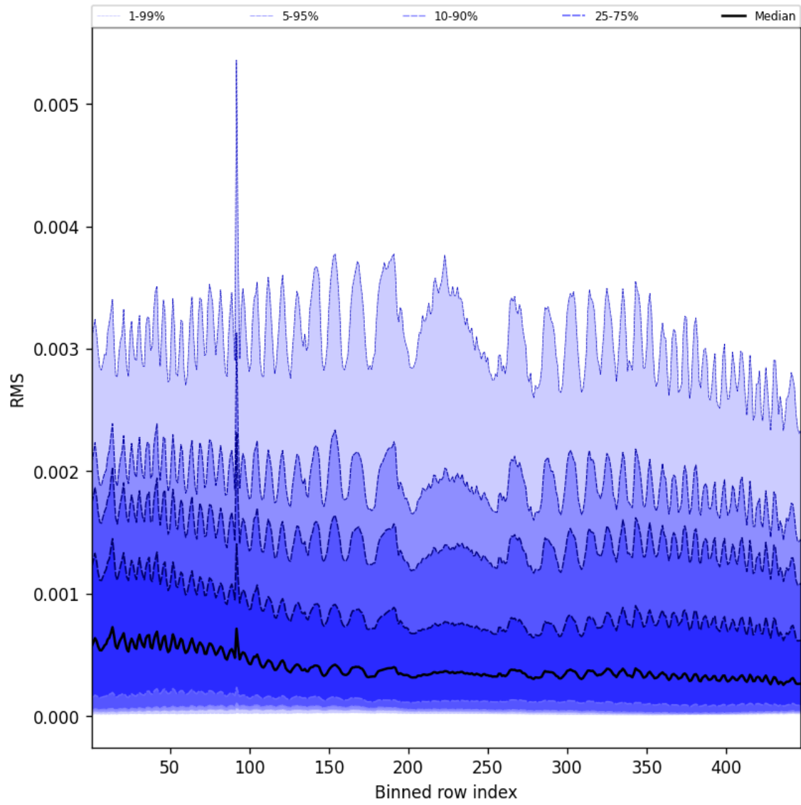
Figure 63: Along track statistics of “RMS” for 2025-09-26 to 2025-09-27
