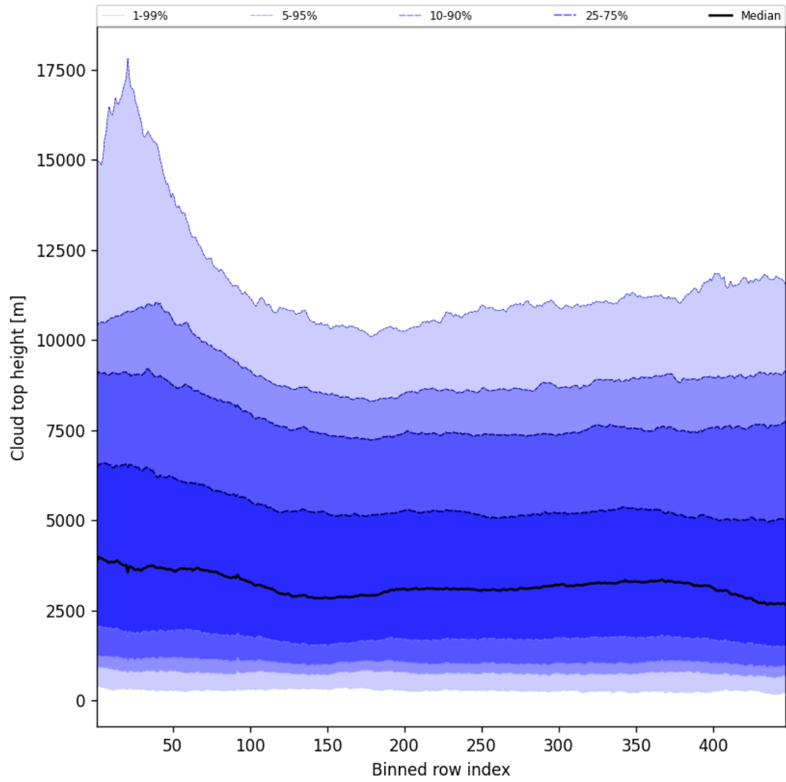
Figure 56: Along track statistics of “Cloud top height” for 2025-09-26 to 2025-09-27
