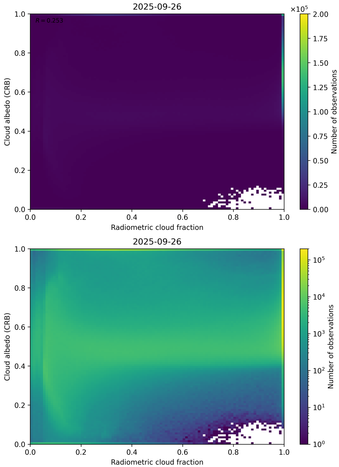
Figure 71: Scatter density plot of “Radiometric cloud fraction” against “Cloud albedo (CRB)” for 2025-09-26 to 2025-09-27.
