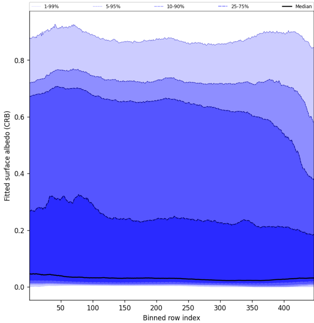
Figure 62: Along track statistics of “Fitted surface albedo (CRB)” for 2025-09-26 to 2025-09-27
