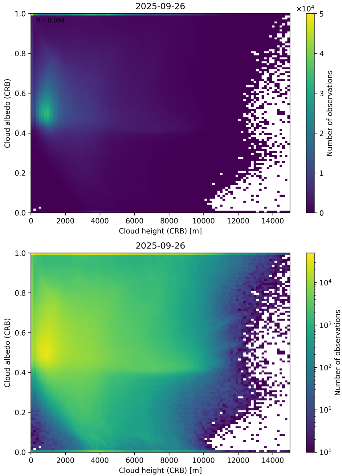
Figure 80: Scatter density plot of “Cloud height (CRB)” against “Cloud albedo (CRB)” for 2025-09-26 to 2025-09-27.
