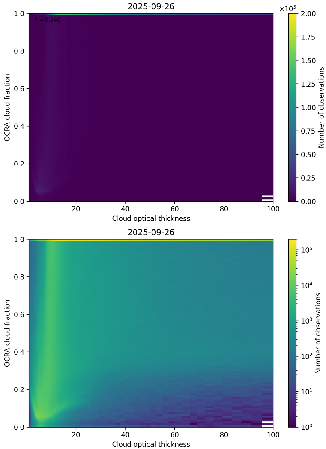
Figure 83: Scatter density plot of “Cloud optical thickness” against “OCRA cloud fraction” for 2025-09-26 to 2025-09-27.
