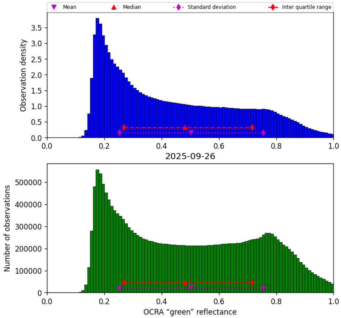
Figure 52: Histogram of “OCRA “green” reflectance” for 2025-09-26 to 2025-09-27
