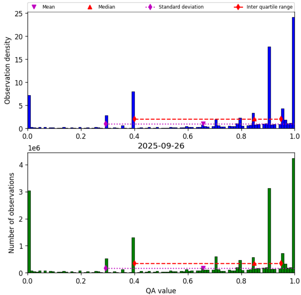
Figure 38: Histogram of “QA value” for 2025-09-26 to 2025-09-27
