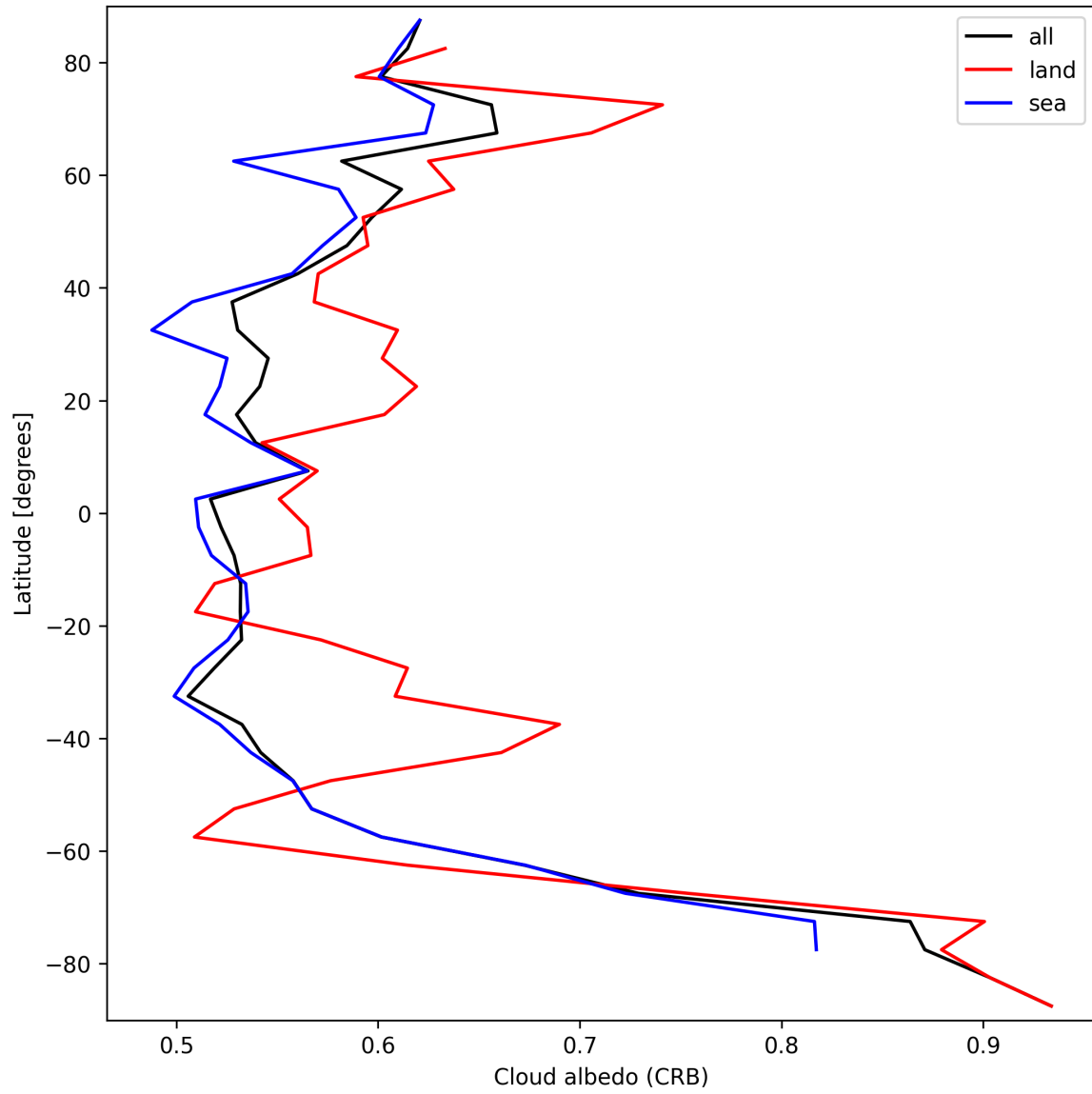
Figure 28: Zonal average of “Cloud albedo (CRB)” for 2025-09-26 to 2025-09-27.
