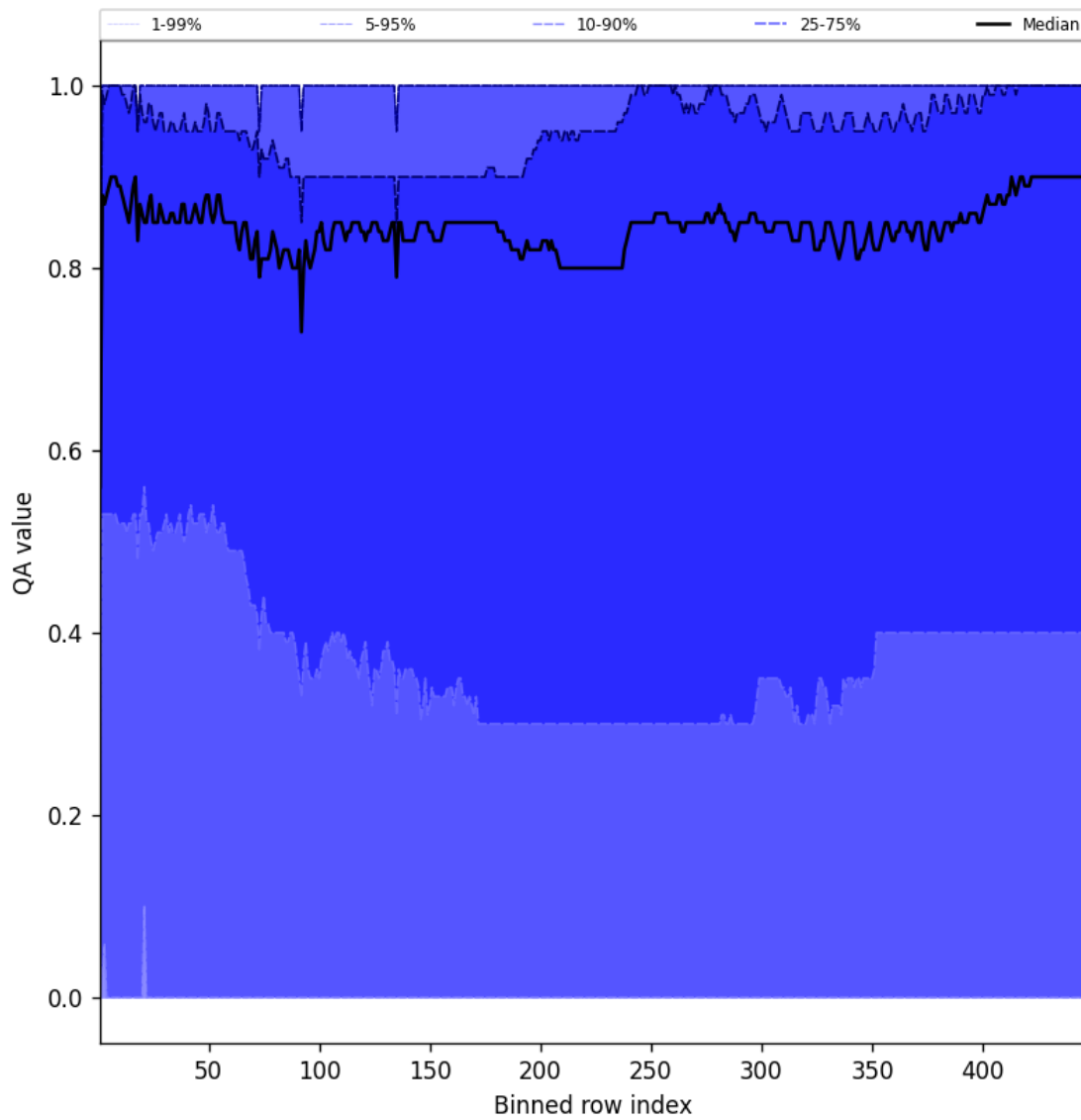
Figure 54: Along track statistics of “QA value” for 2025-09-26 to 2025-09-27
