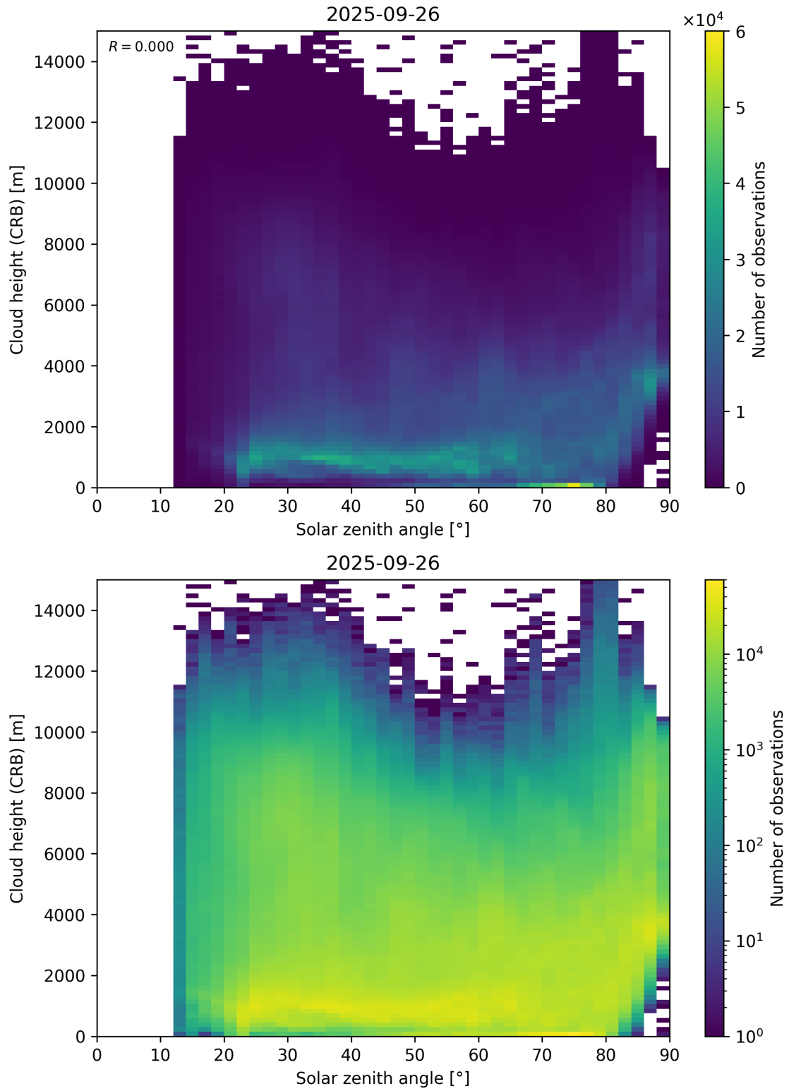
Figure 102: Scatter density plot of “Solar zenith angle” against “Cloud height (CRB)” for 2025-09-26 to 2025-09-27.
