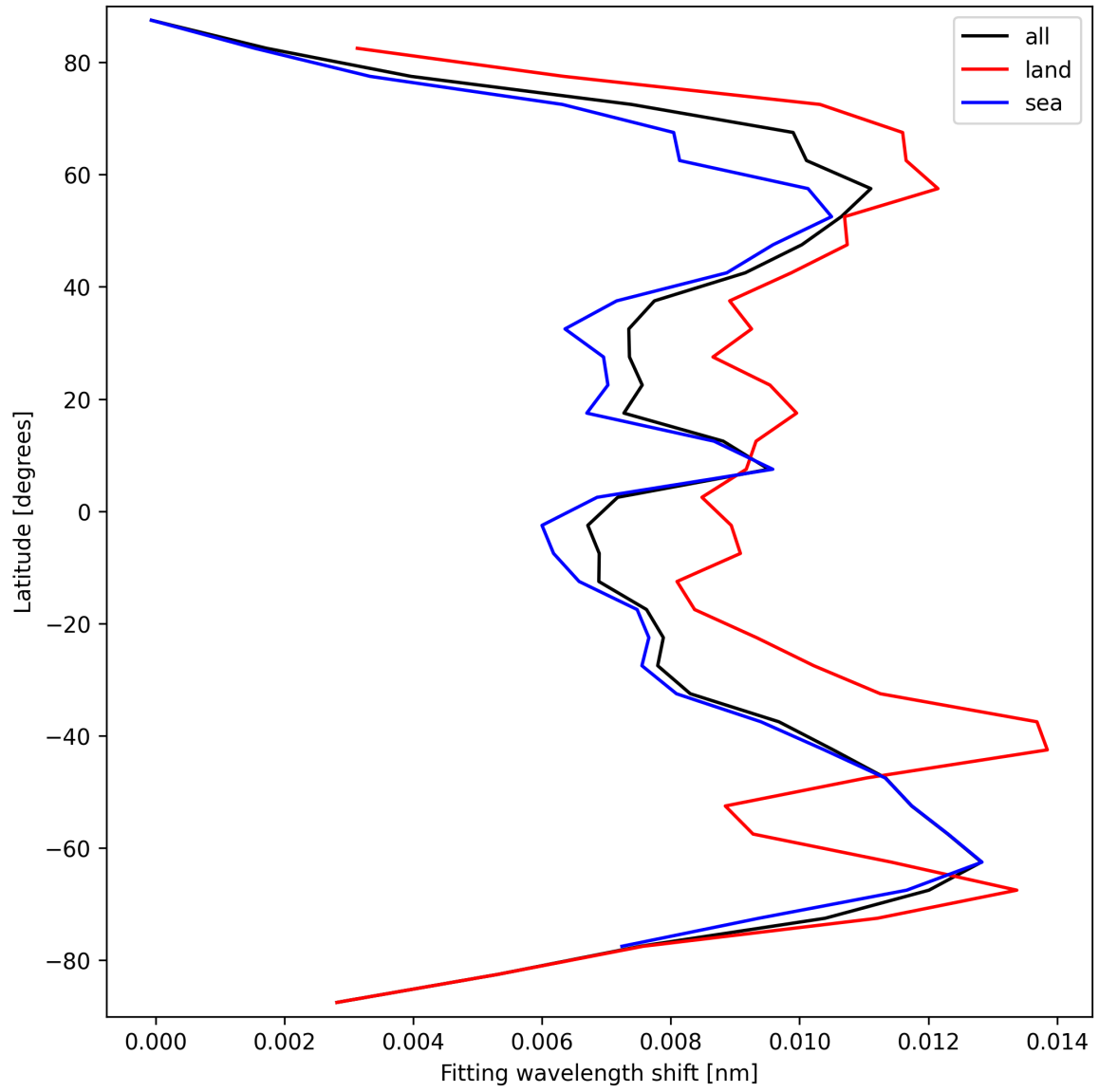
Figure 33: Zonal average of “Fitting wavelength shift” for 2025-09-26 to 2025-09-27.
