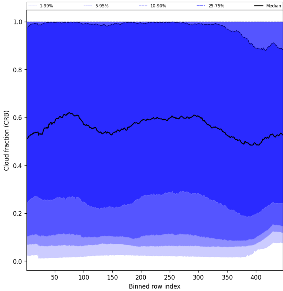
Figure 58: Along track statistics of “Cloud fraction (CRB)” for 2025-09-26 to 2025-09-27
