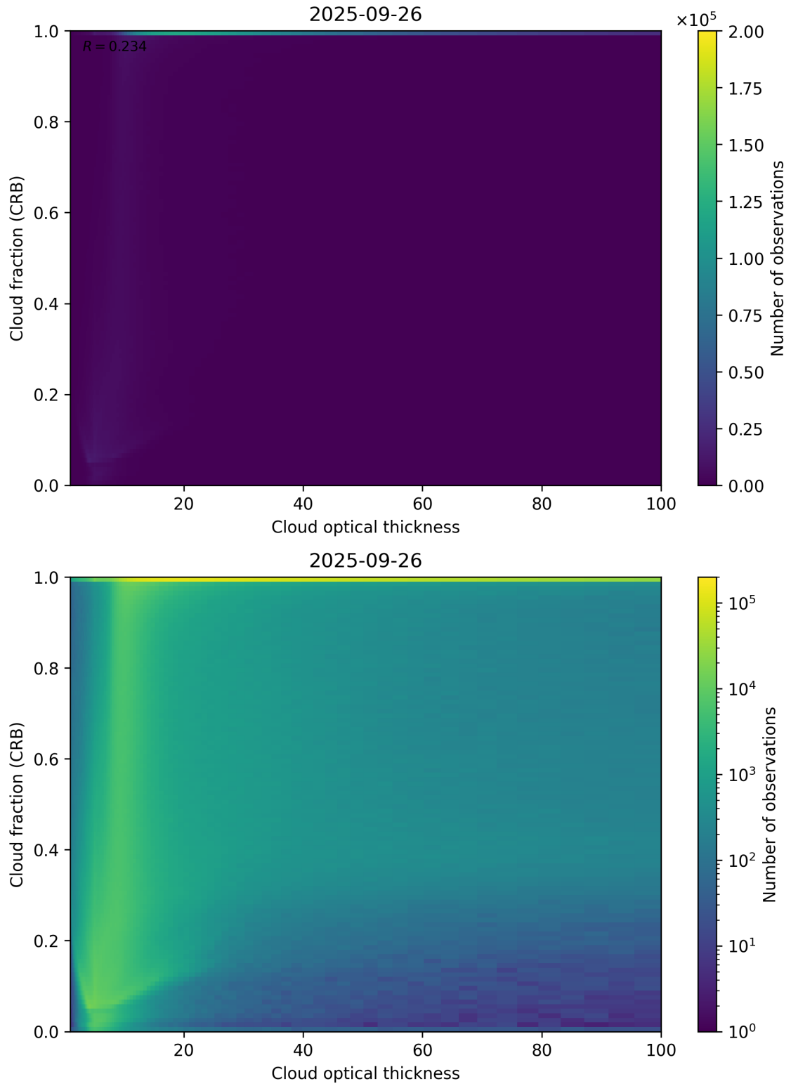
Figure 84: Scatter density plot of “Cloud optical thickness” against “Cloud fraction (CRB)” for 2025-09-26 to 2025-09-27.
