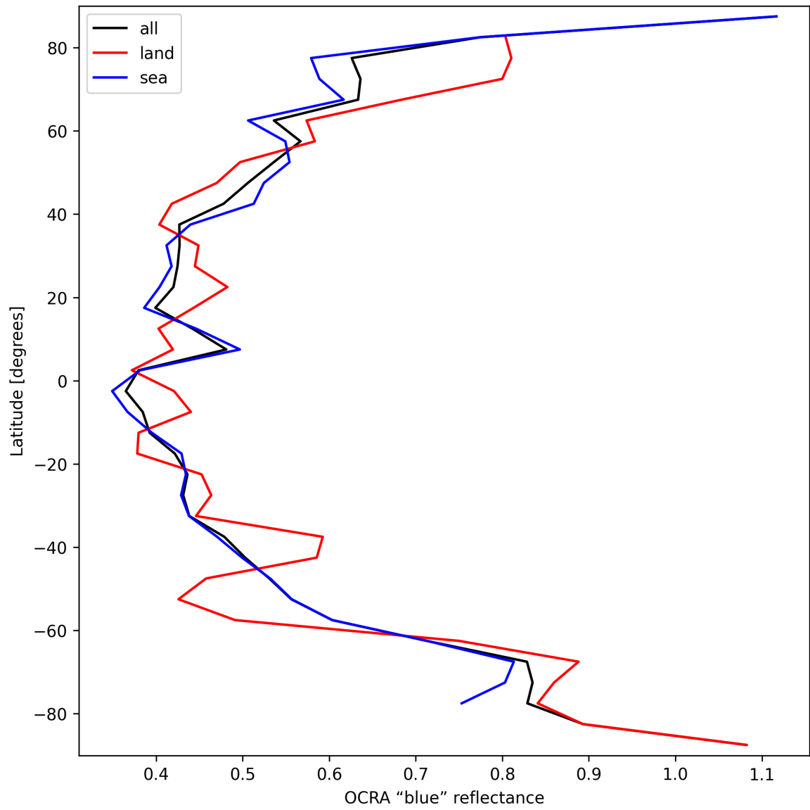
Figure 35: Zonal average of “OCRA “blue” reflectance” for 2025-09-26 to 2025-09-27.
