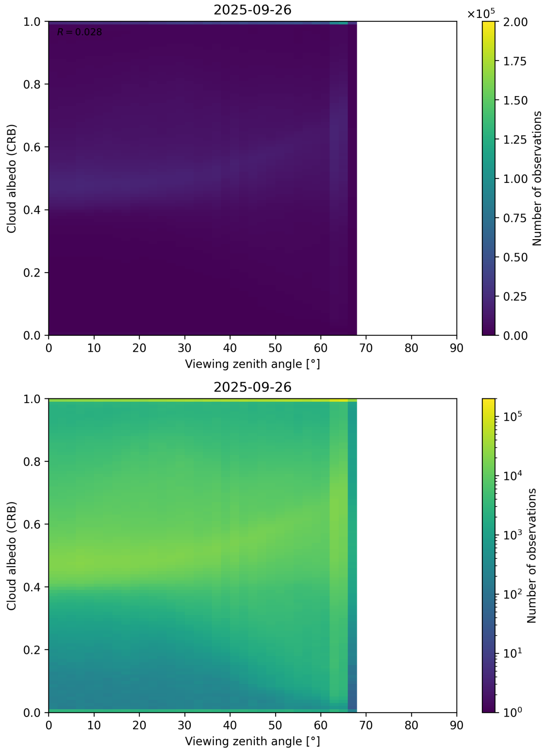
Figure 106: Scatter density plot of “Viewing zenith angle” against “Cloud albedo (CRB)” for 2025-09-26 to 2025-09-27.
