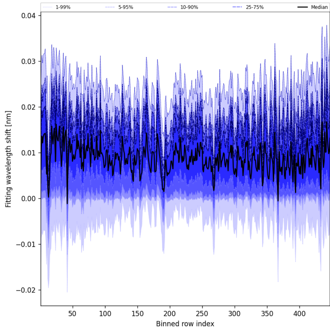
Figure 65: Along track statistics of “Fitting wavelength shift” for 2025-09-26 to 2025-09-27
