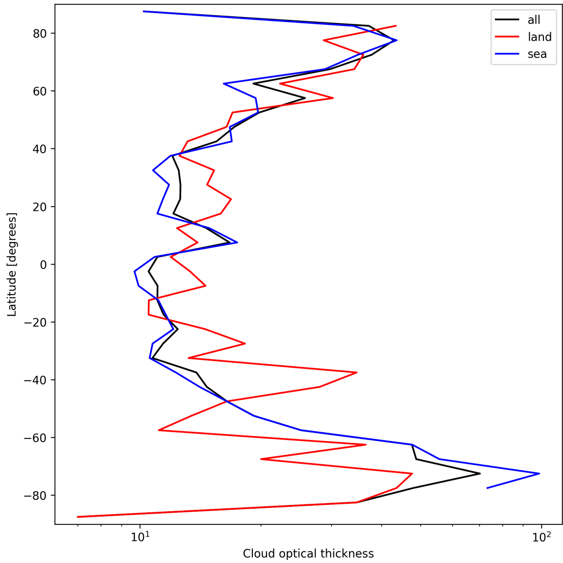
Figure 25: Zonal average of “Cloud optical thickness” for 2025-09-26 to 2025-09-27.
