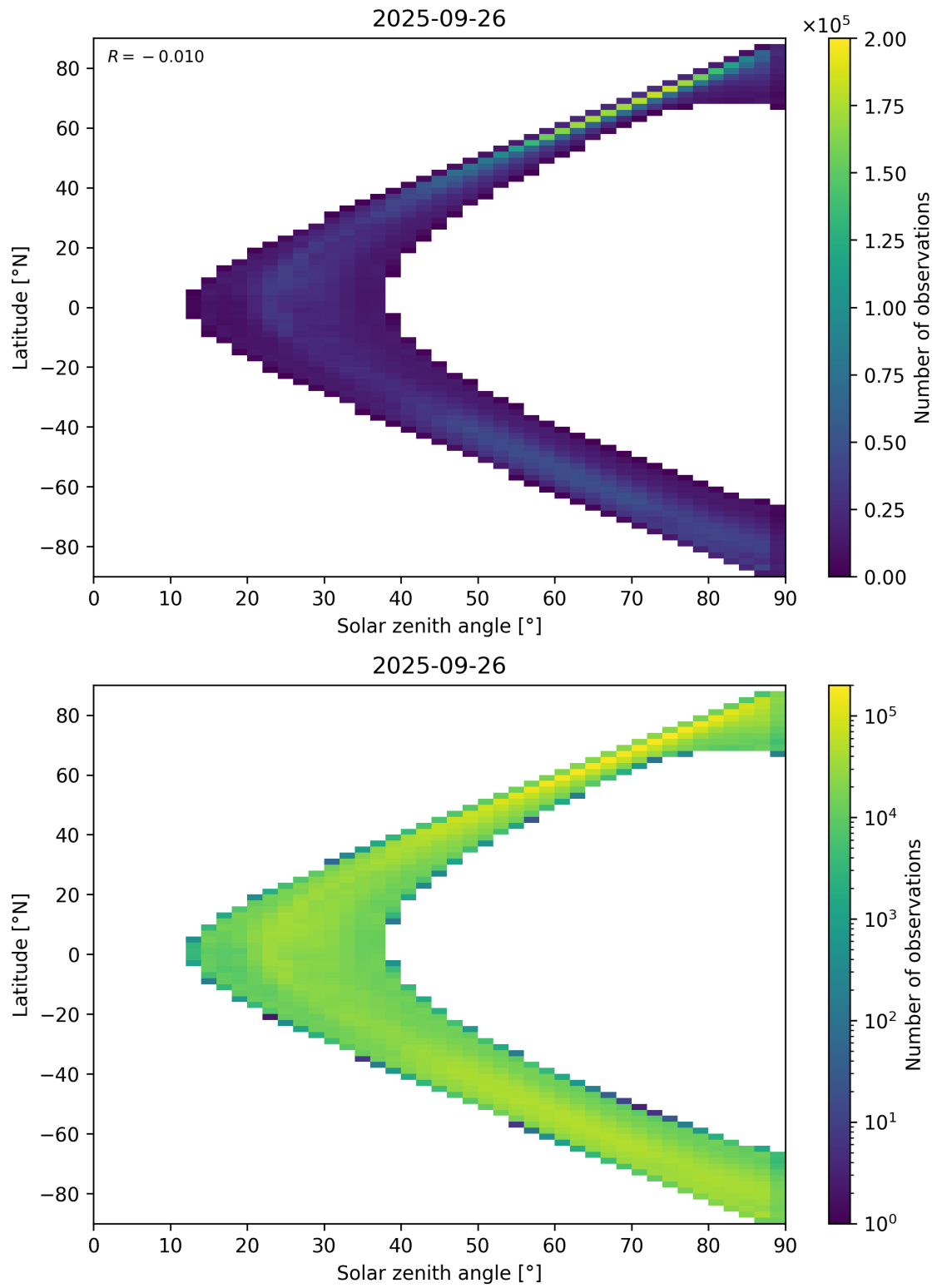
Figure 105: Scatter density plot of “Solar zenith angle” against “Latitude” for 2025-09-26 to 2025-09-27.
