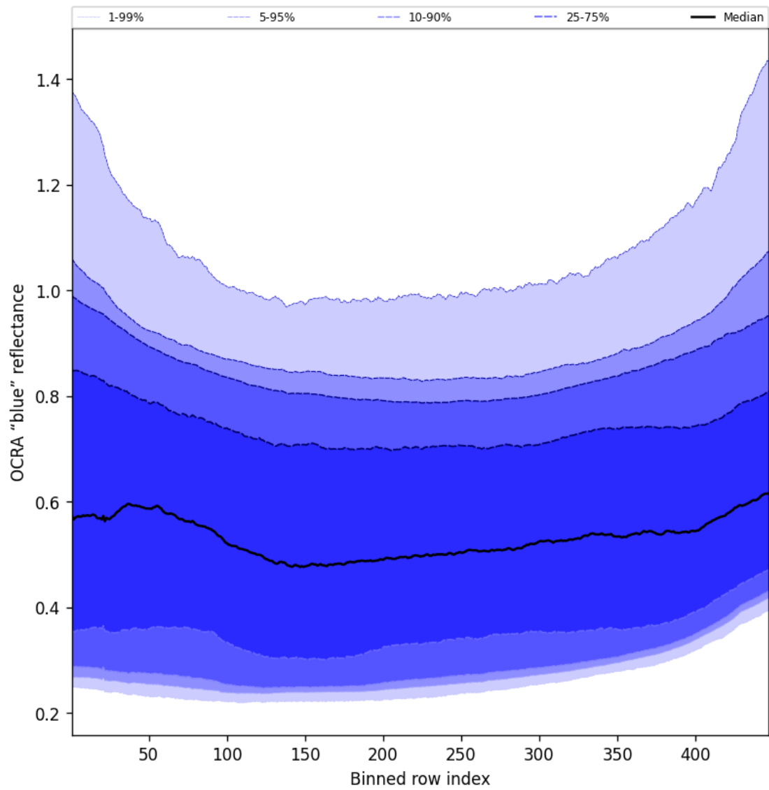
Figure 67: Along track statistics of “OCRA “blue” reflectance” for 2025-09-26 to 2025-09-27
