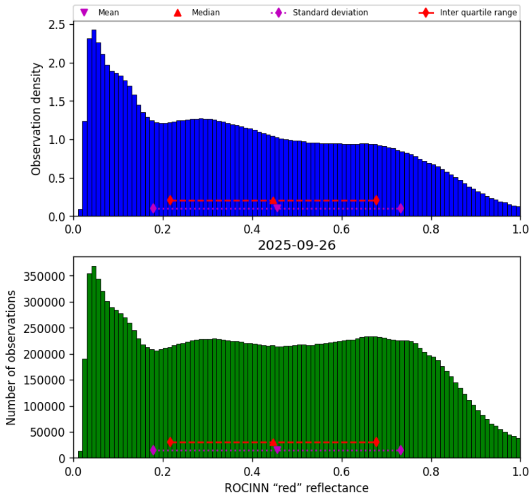
Figure 53: Histogram of “ROCINN “red” reflectance” for 2025-09-26 to 2025-09-27
