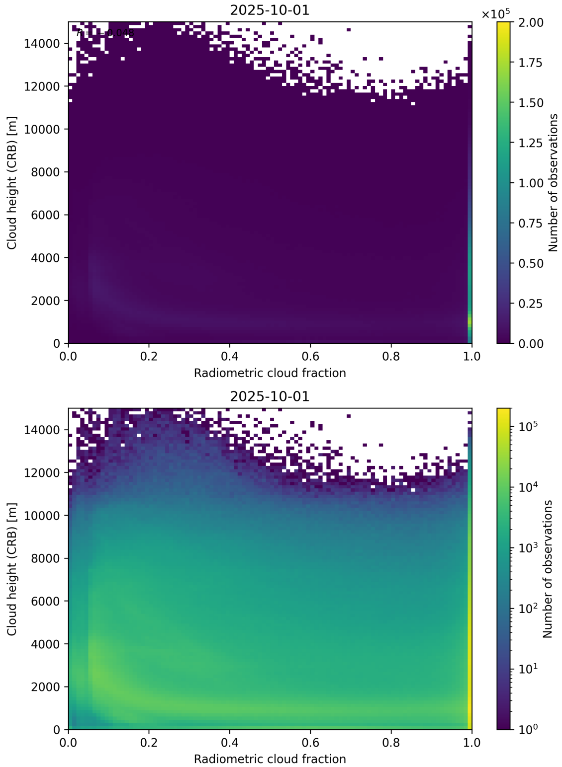
Figure 74: Scatter density plot of “Radiometric cloud fraction” against “Cloud height (CRB)” for 2025-10-01 to 2025-10-02.
