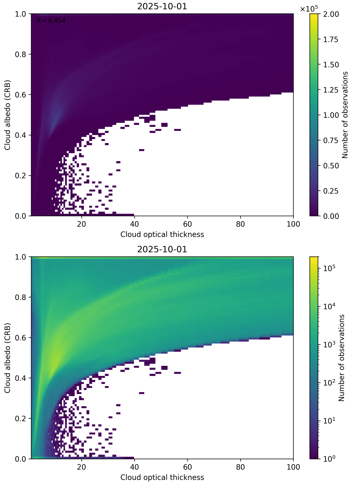
Figure 82: Scatter density plot of “Cloud optical thickness” against “Cloud albedo (CRB)” for 2025-10-01 to 2025-10-02.
