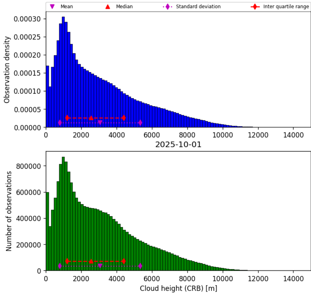
Figure 43: Histogram of “Cloud height (CRB)” for 2025-10-01 to 2025-10-02
