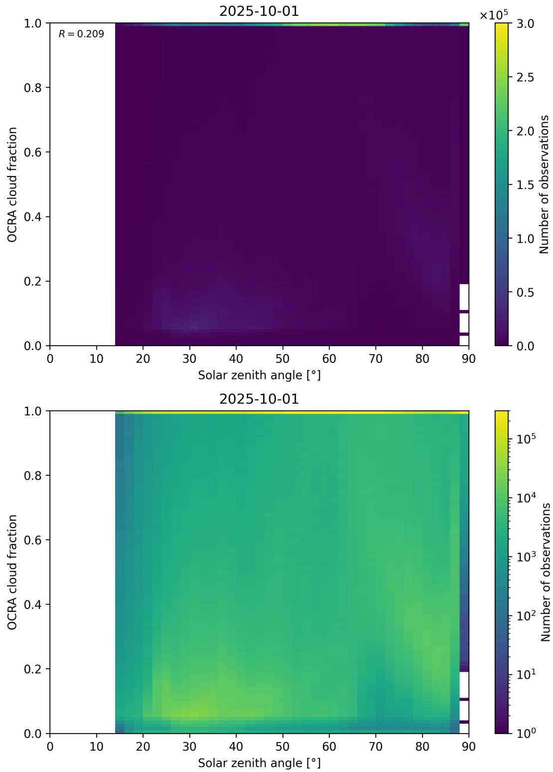
Figure 100: Scatter density plot of “Solar zenith angle” against “OCRA cloud fraction” for 2025-10-01 to 2025-10-02.
