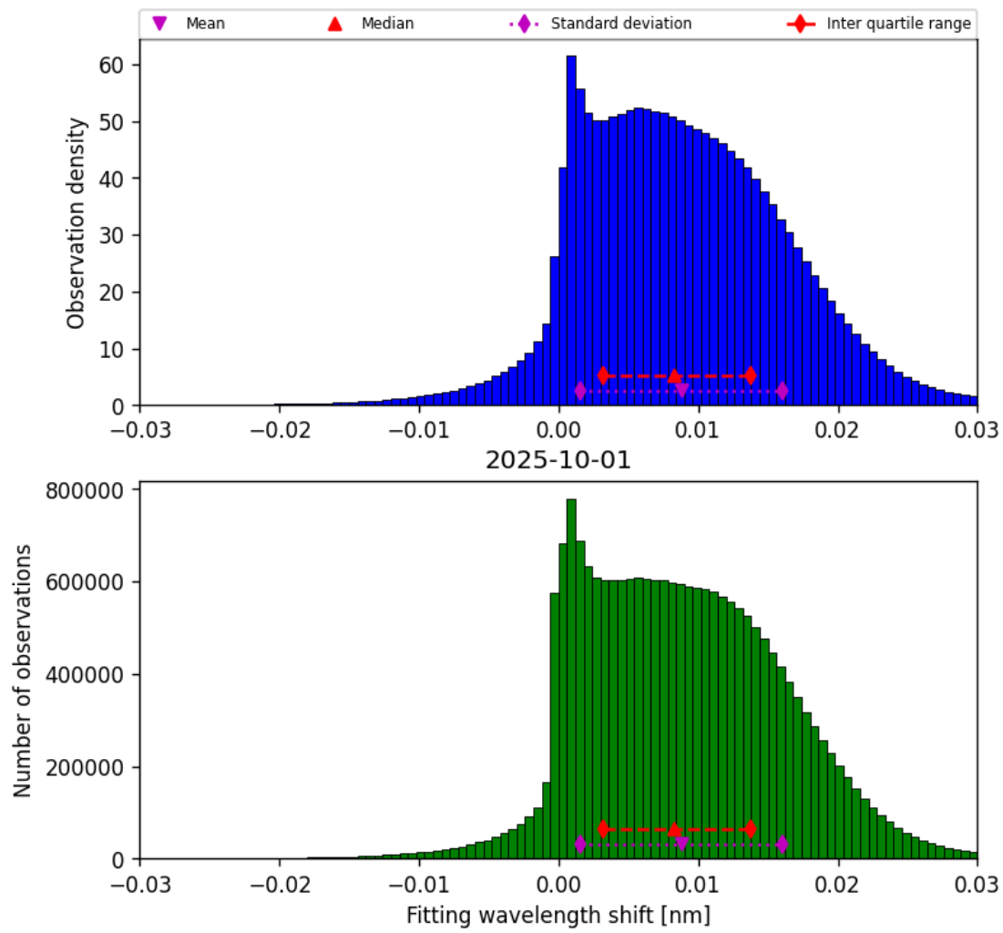
Figure 49: Histogram of “Fitting wavelength shift” for 2025-10-01 to 2025-10-02
