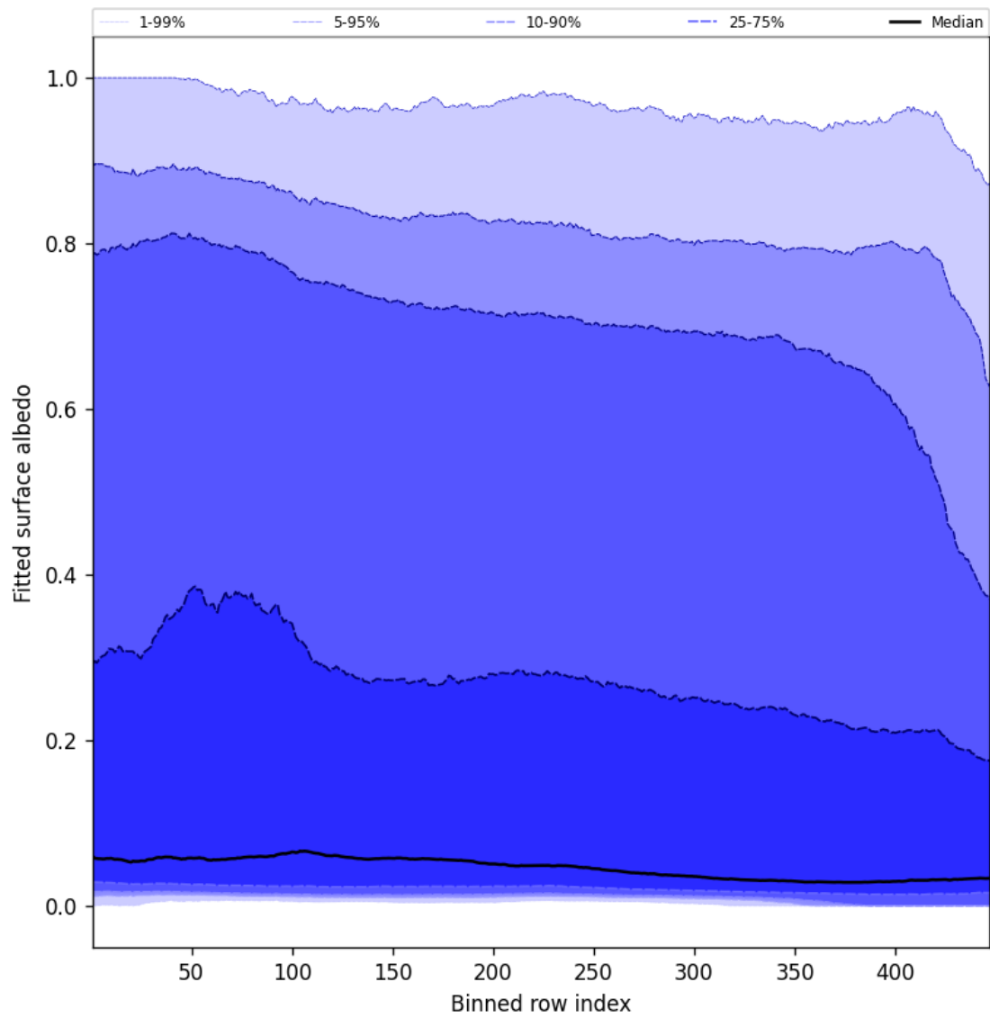
Figure 61: Along track statistics of “Fitted surface albedo” for 2025-10-01 to 2025-10-02
