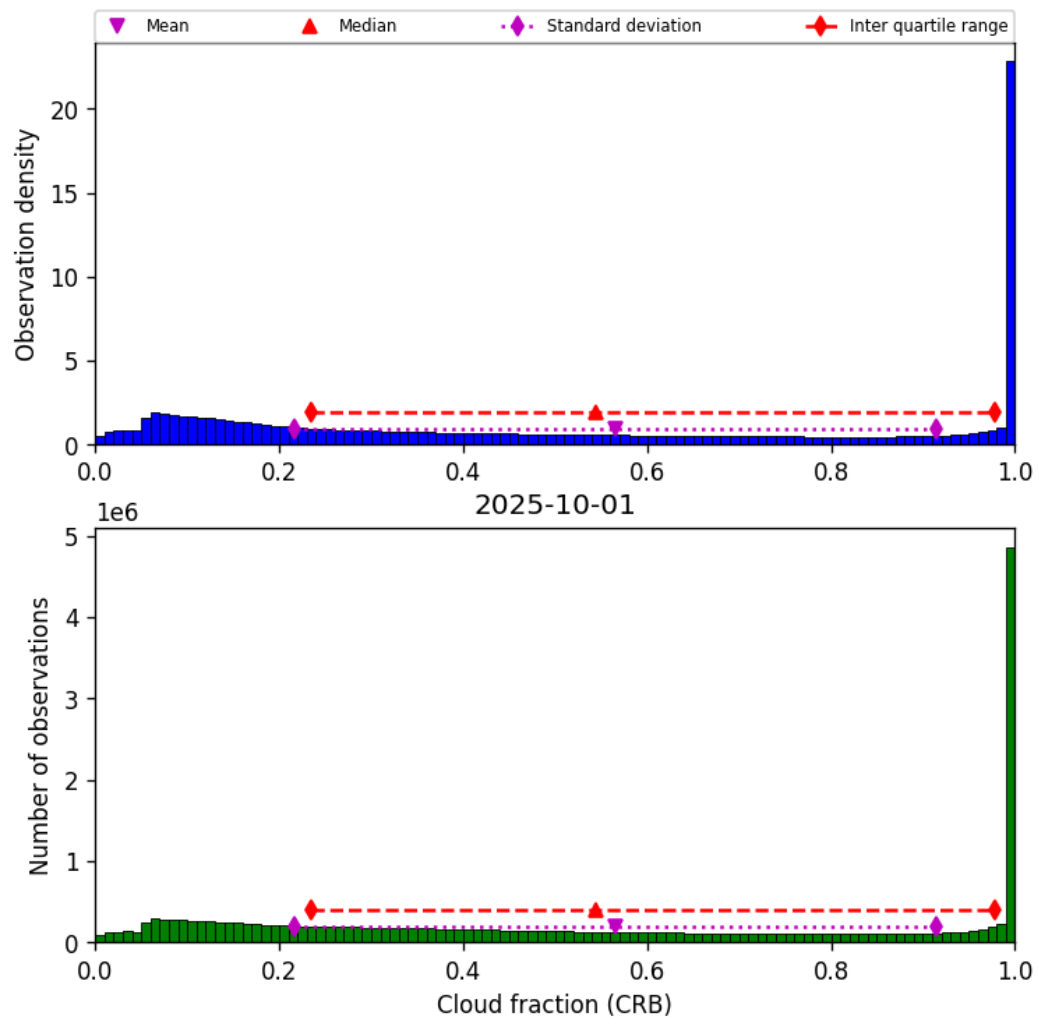
Figure 42: Histogram of “Cloud fraction (CRB)” for 2025-10-01 to 2025-10-02
