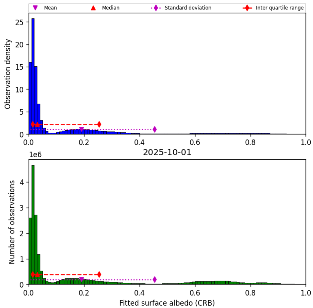
Figure 46: Histogram of “Fitted surface albedo (CRB)” for 2025-10-01 to 2025-10-02
