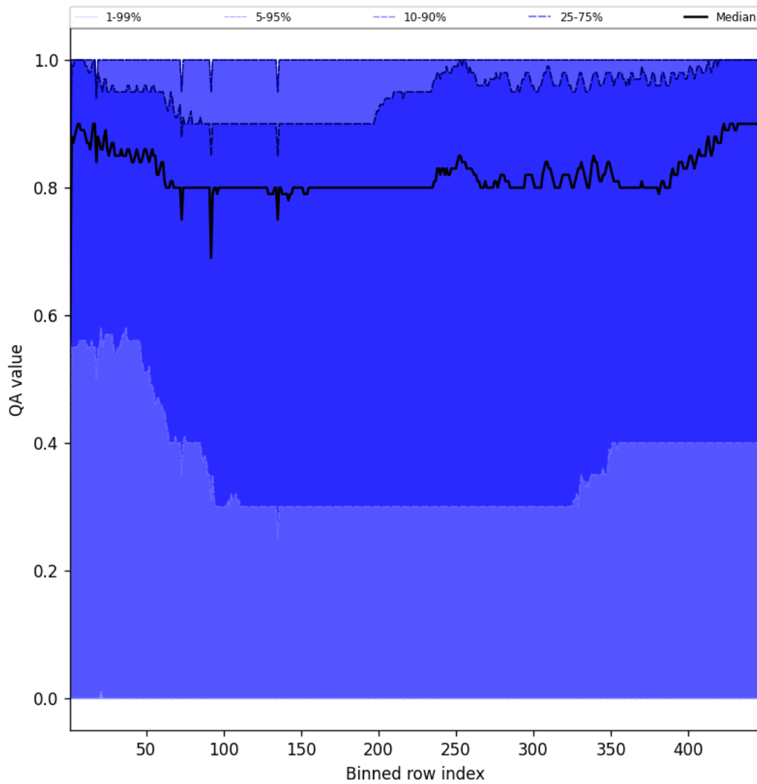
Figure 54: Along track statistics of “QA value” for 2025-10-01 to 2025-10-02
