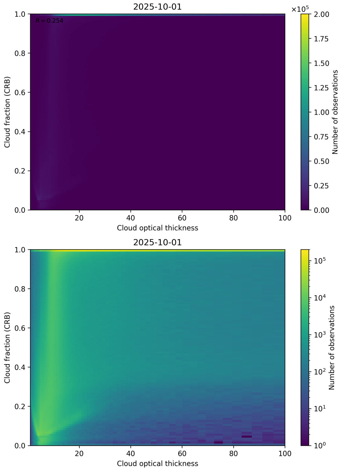
Figure 84: Scatter density plot of “Cloud optical thickness” against “Cloud fraction (CRB)” for 2025-10-01 to 2025-10-02.
