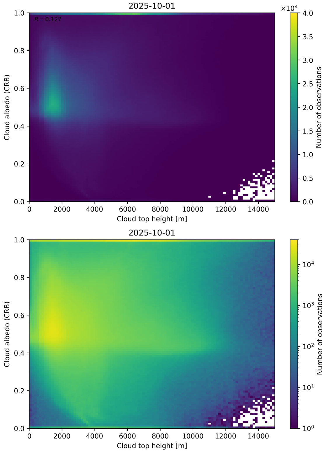
Figure 86: Scatter density plot of “Cloud top height” against “Cloud albedo (CRB)” for 2025-10-01 to 2025-10-02.
