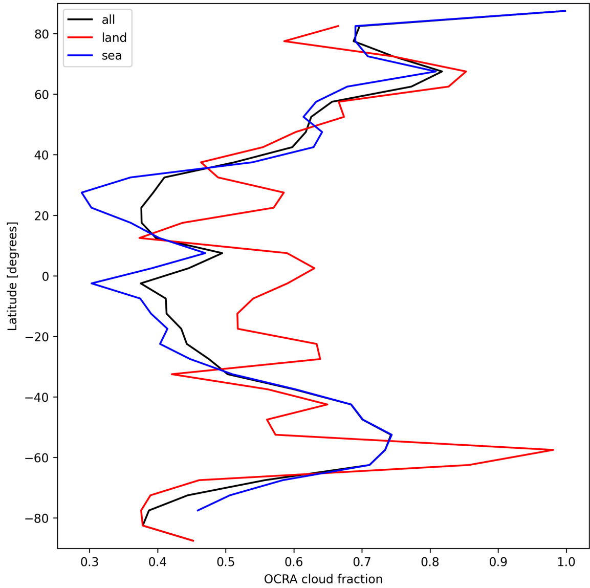
Figure 34: Zonal average of “OCRA cloud fraction” for 2025-10-01 to 2025-10-02.
