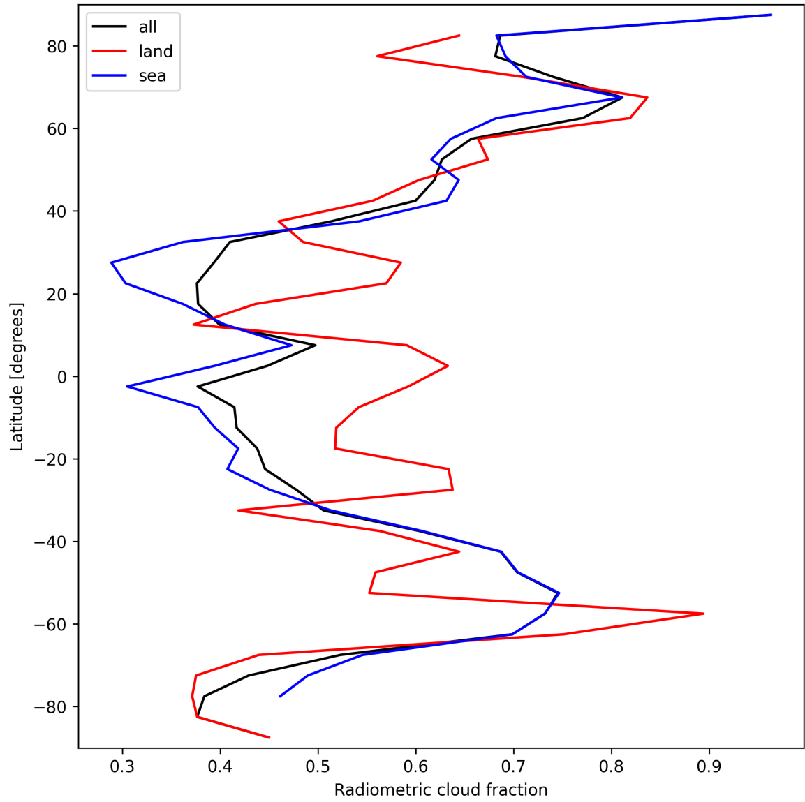
Figure 23: Zonal average of “Radiometric cloud fraction” for 2025-10-01 to 2025-10-02.
