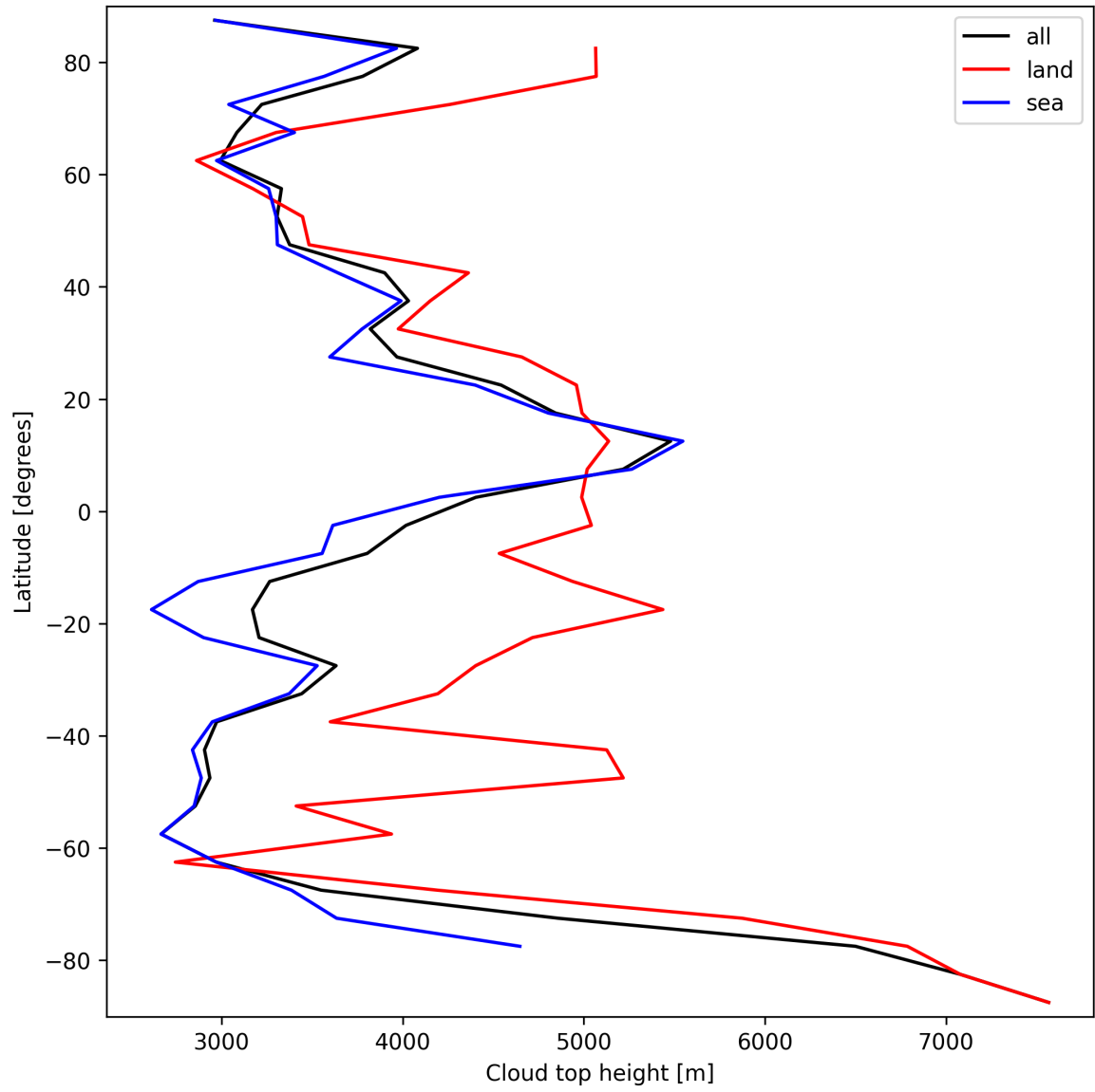
Figure 24: Zonal average of “Cloud top height” for 2025-10-01 to 2025-10-02.
