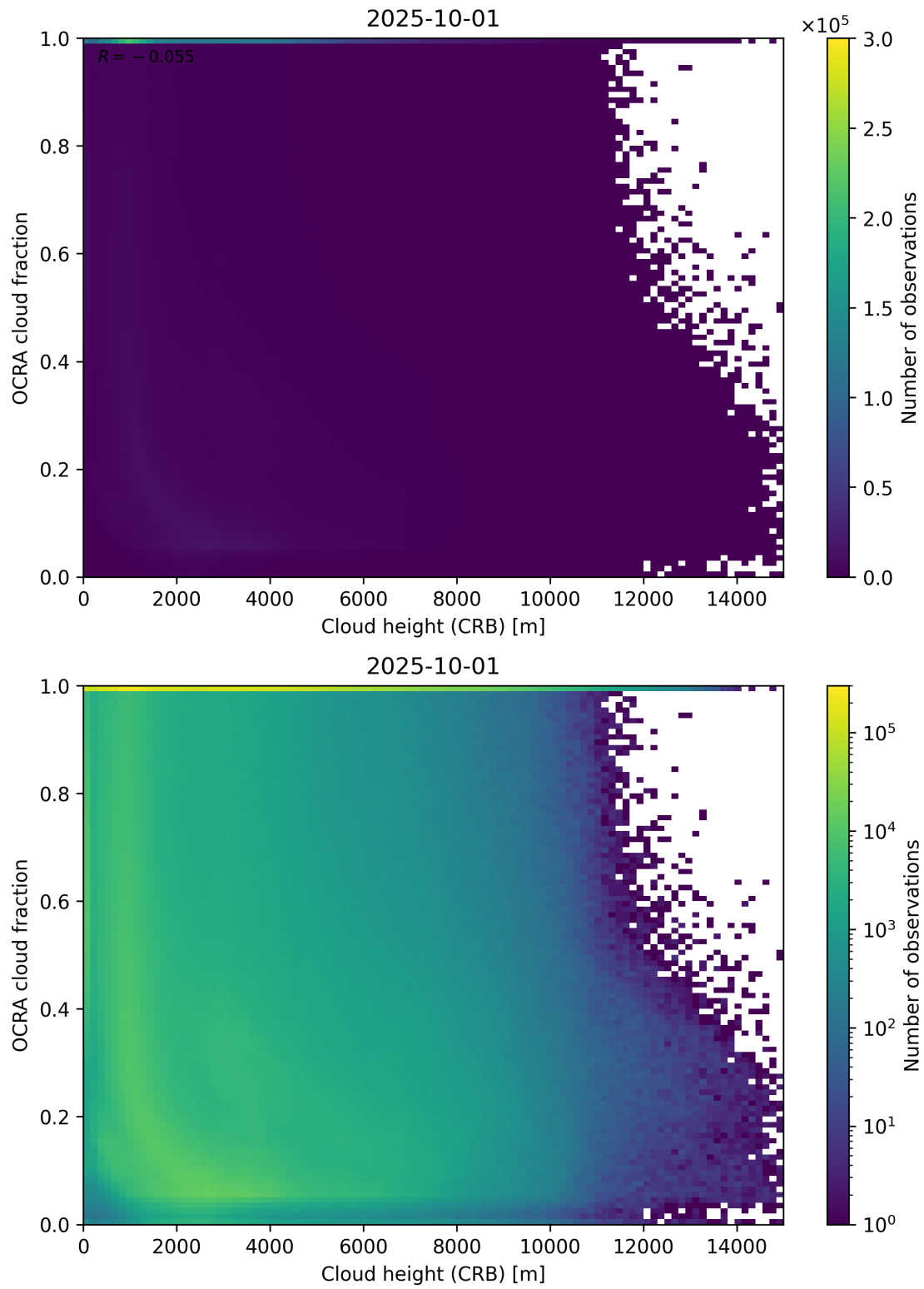
Figure 81: Scatter density plot of “Cloud height (CRB)” against “OCRA cloud fraction” for 2025-10-01 to 2025-10-02.
