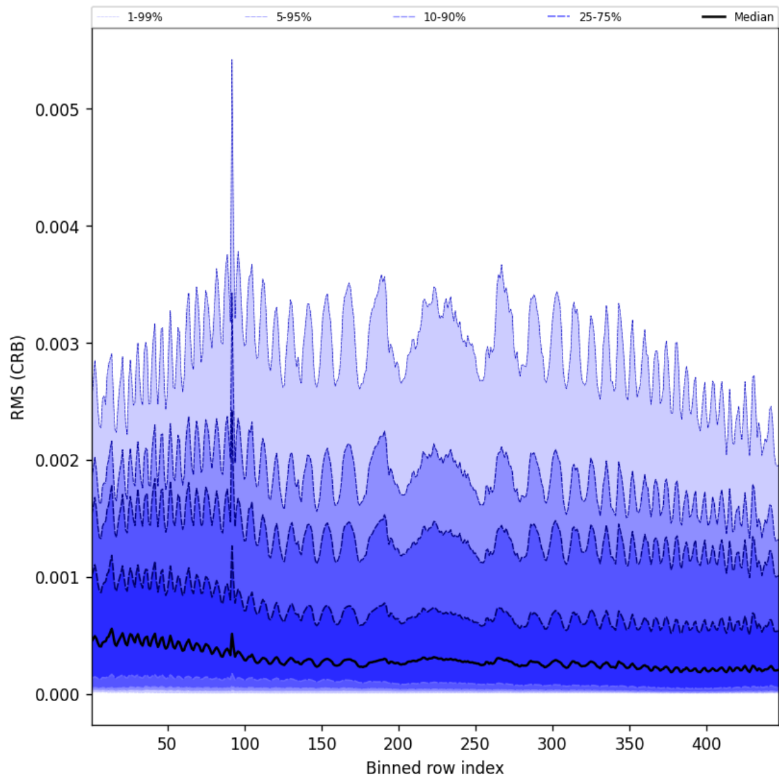
Figure 64: Along track statistics of “RMS (CRB)” for 2025-10-01 to 2025-10-02
