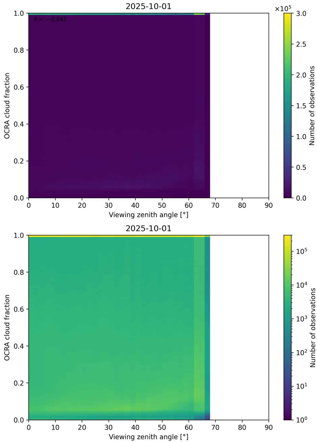
Figure 108: Scatter density plot of “Viewing zenith angle” against “OCRA cloud fraction” for 2025-10-01 to 2025-10-02.
