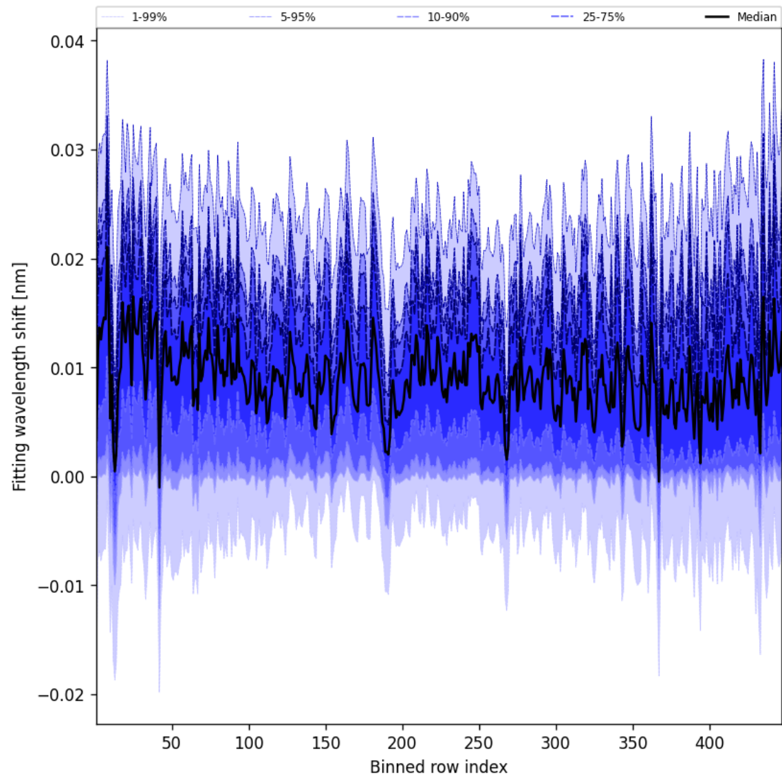
Figure 65: Along track statistics of “Fitting wavelength shift” for 2025-10-01 to 2025-10-02
