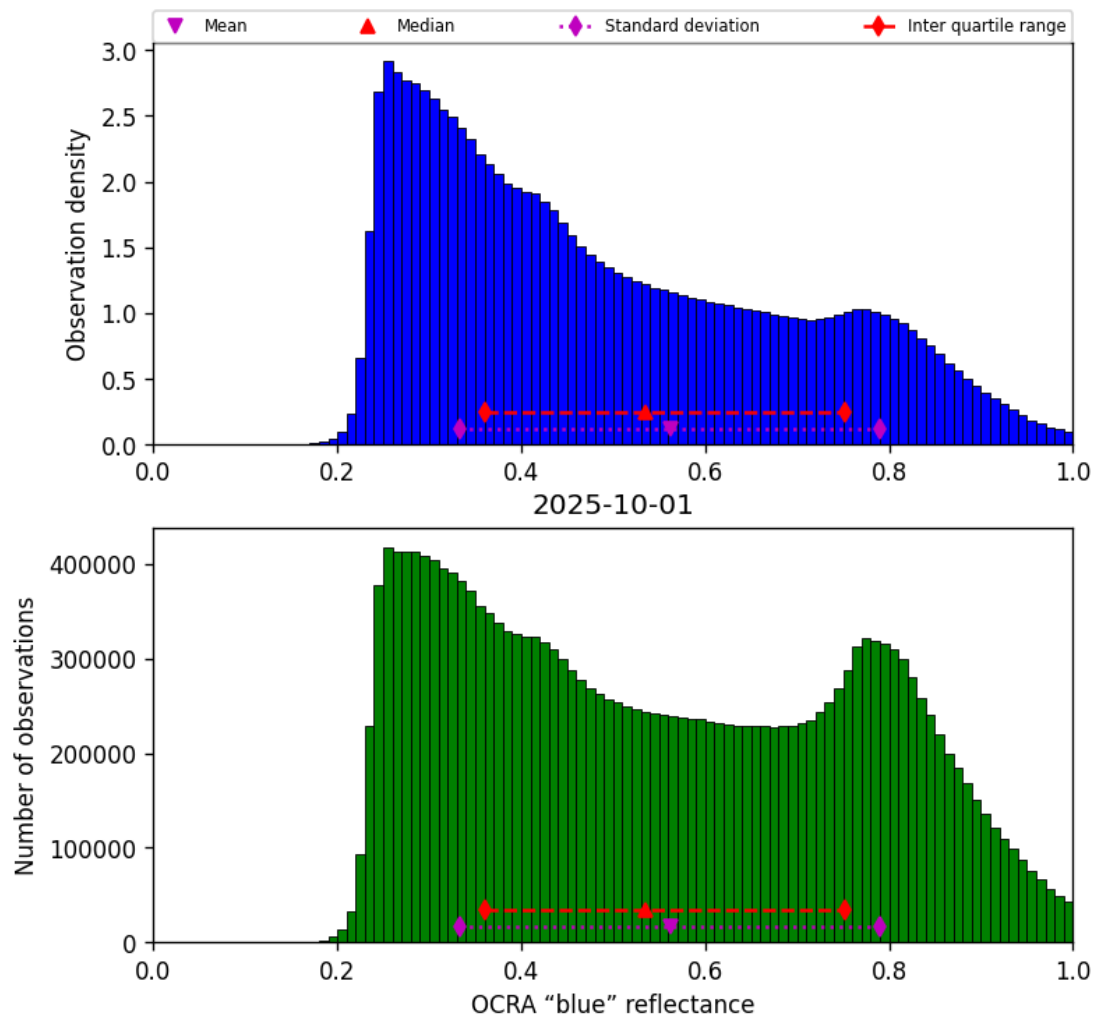
Figure 51: Histogram of “OCRA “blue” reflectance” for 2025-10-01 to 2025-10-02
