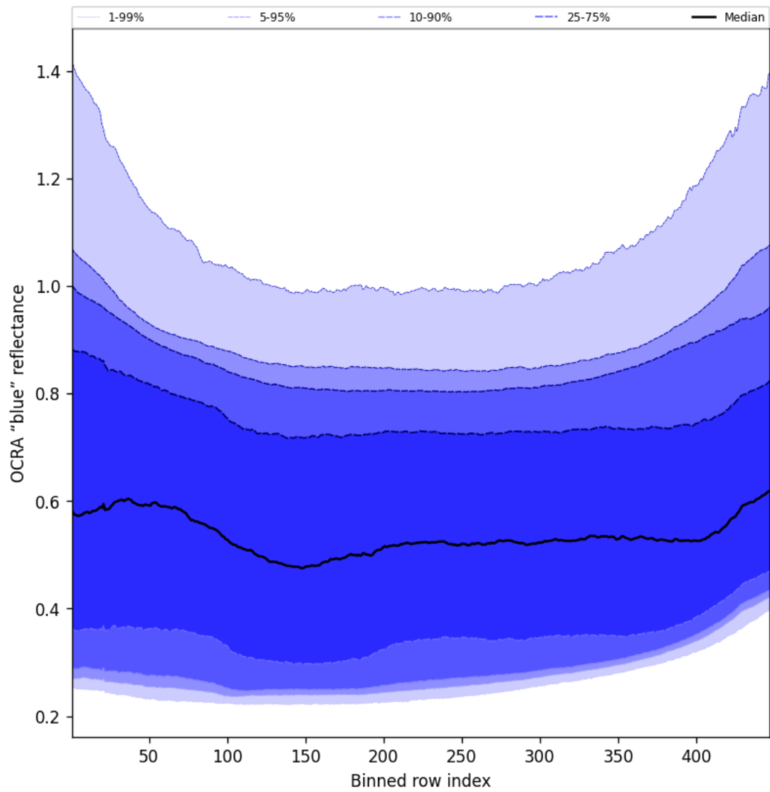
Figure 67: Along track statistics of “OCRA “blue” reflectance” for 2025-10-01 to 2025-10-02
