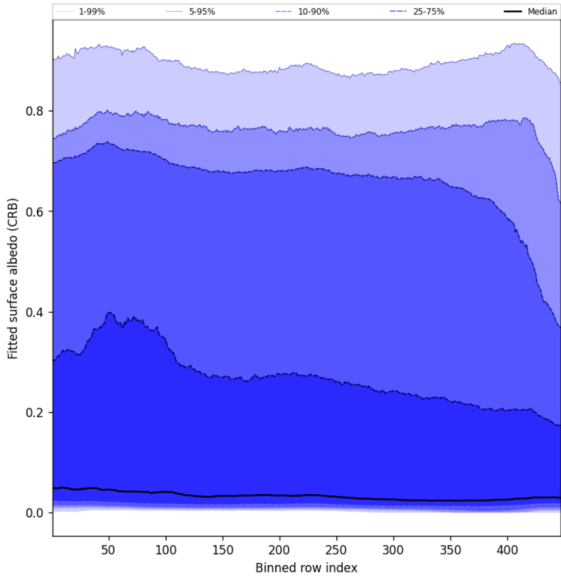
Figure 62: Along track statistics of “Fitted surface albedo (CRB)” for 2025-10-01 to 2025-10-02
