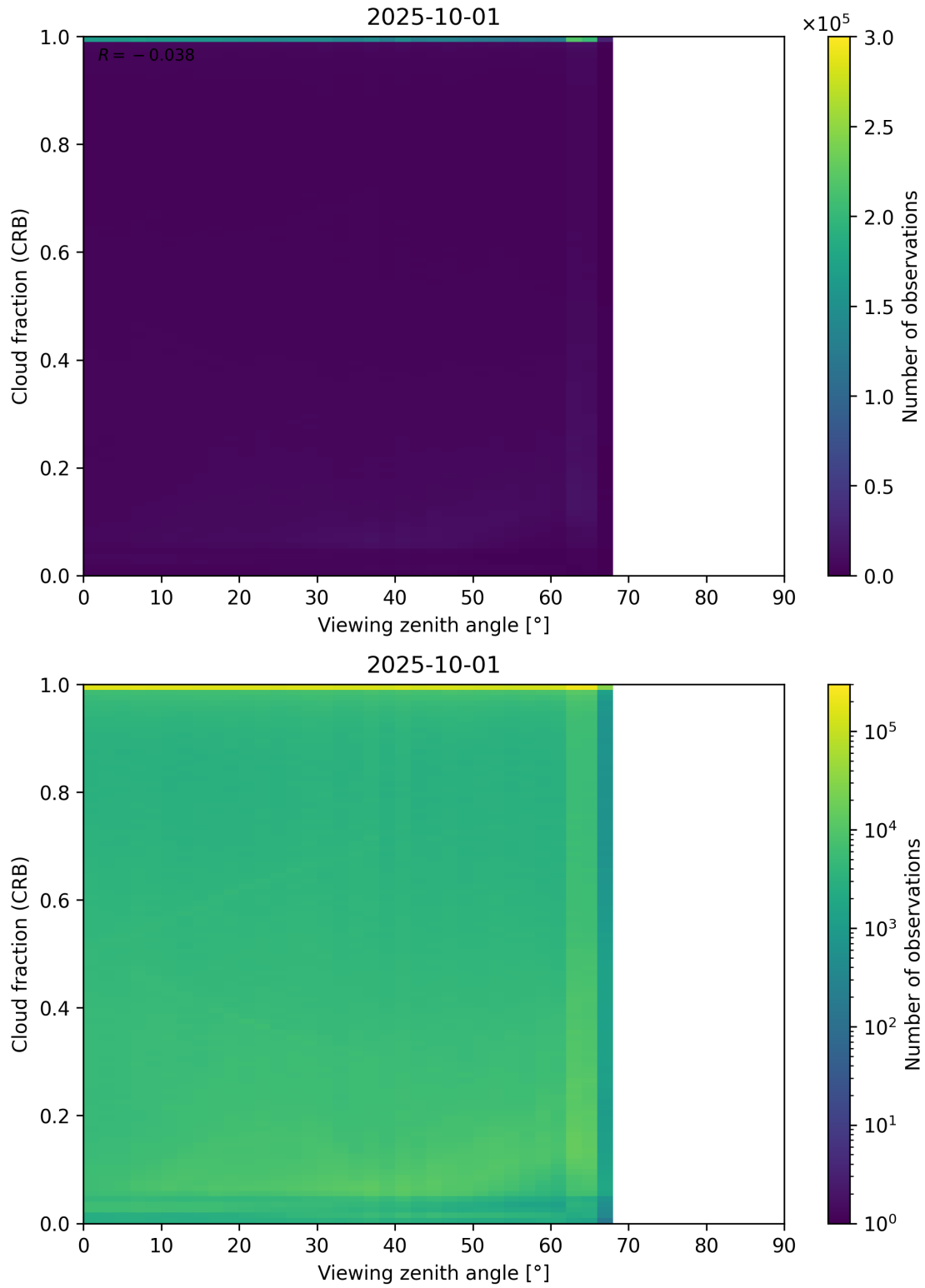
Figure 109: Scatter density plot of “Viewing zenith angle” against “Cloud fraction (CRB)” for 2025-10-01 to 2025-10-02.
