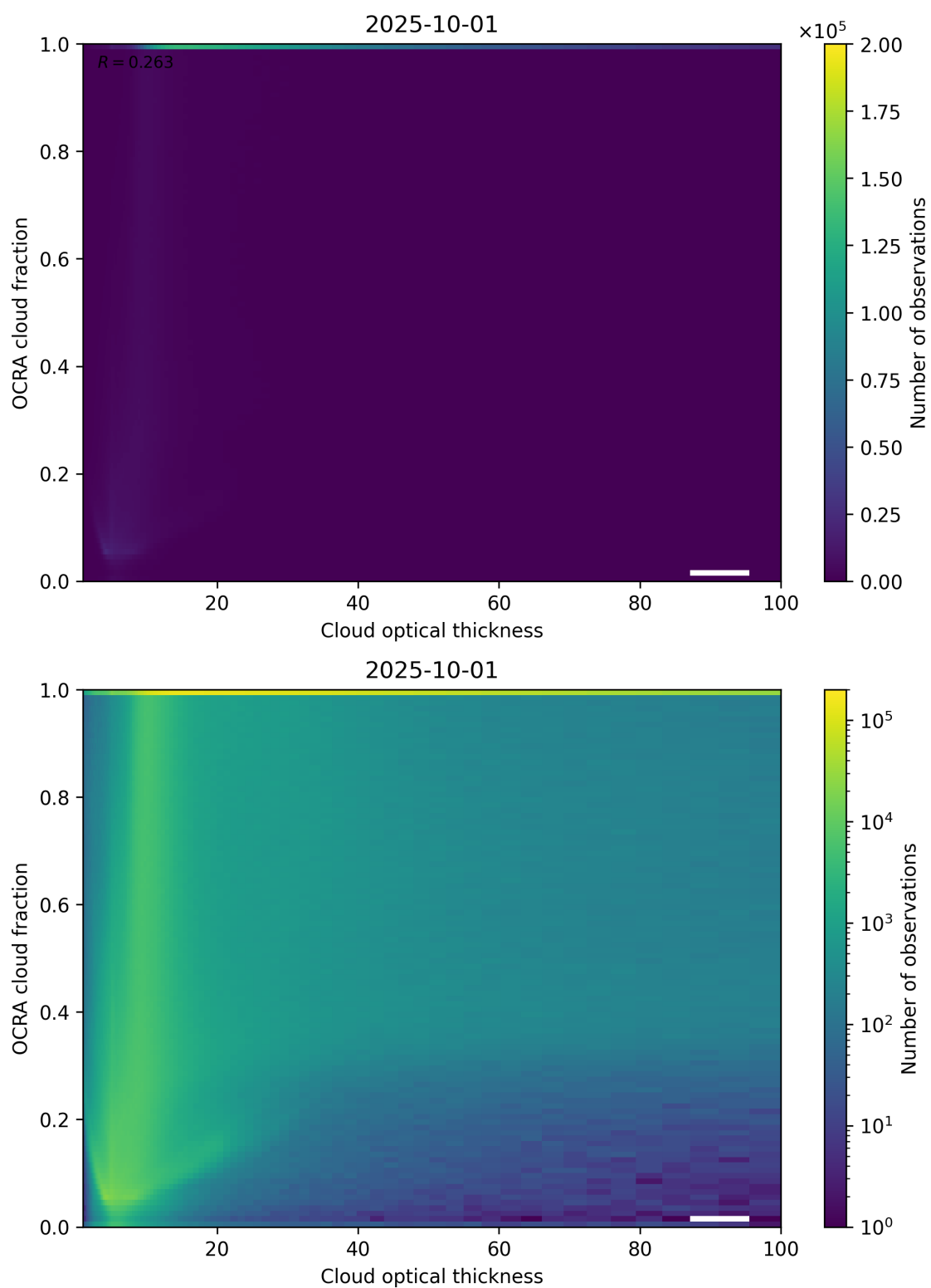
Figure 83: Scatter density plot of “Cloud optical thickness” against “OCRA cloud fraction” for 2025-10-01 to 2025-10-02.
