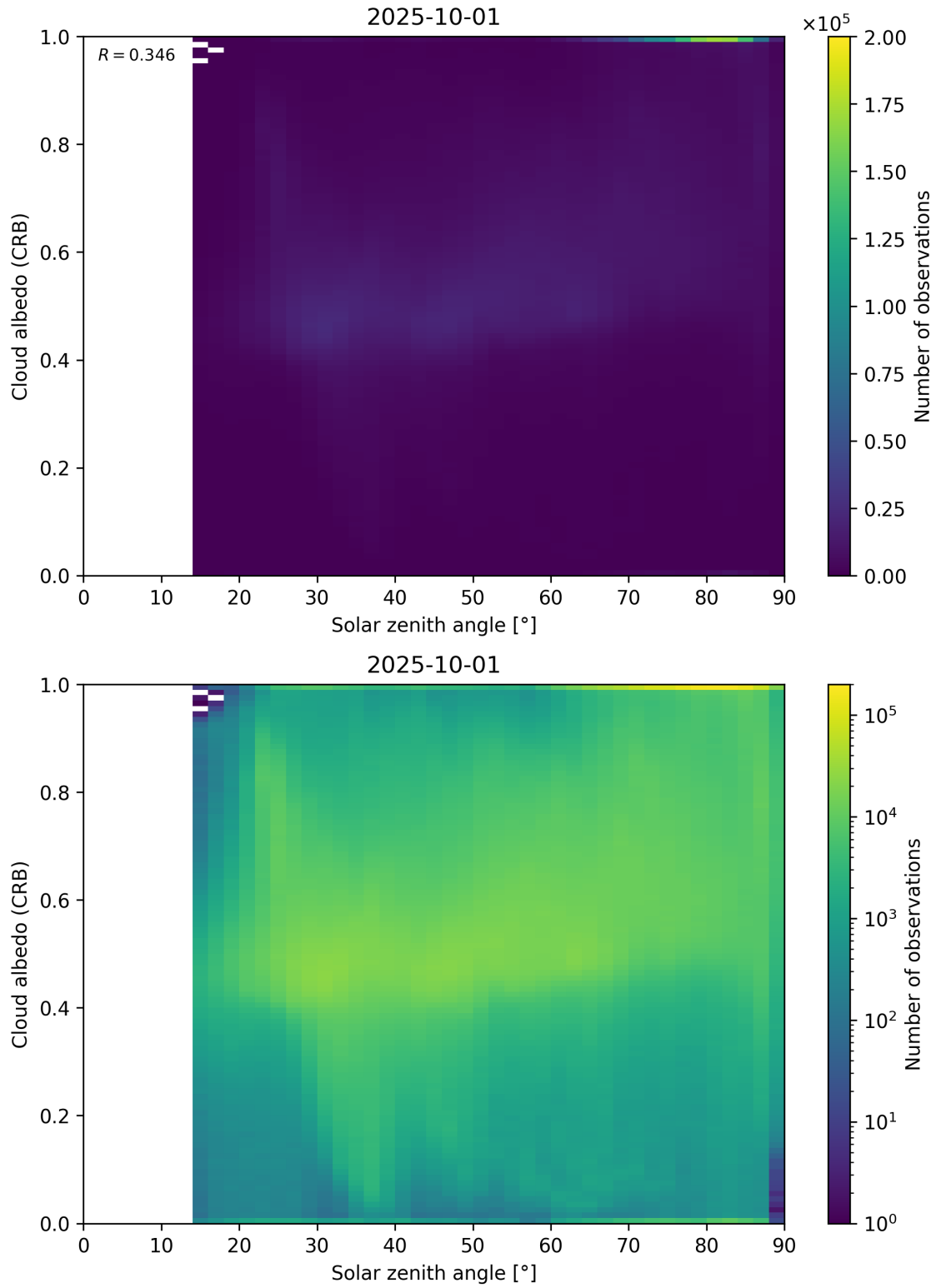
Figure 98: Scatter density plot of “Solar zenith angle” against “Cloud albedo (CRB)” for 2025-10-01 to 2025-10-02.
