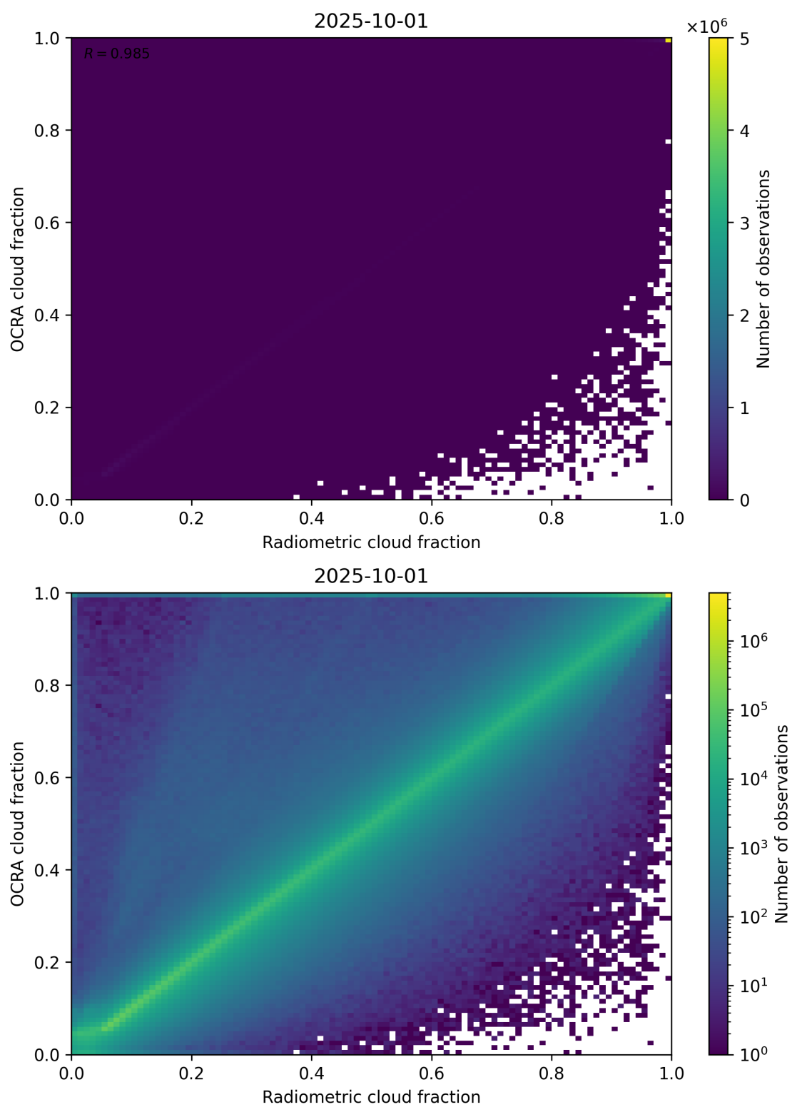
Figure 72: Scatter density plot of “Radiometric cloud fraction” against “OCRA cloud fraction” for 2025-10-01 to 2025-10-02.
