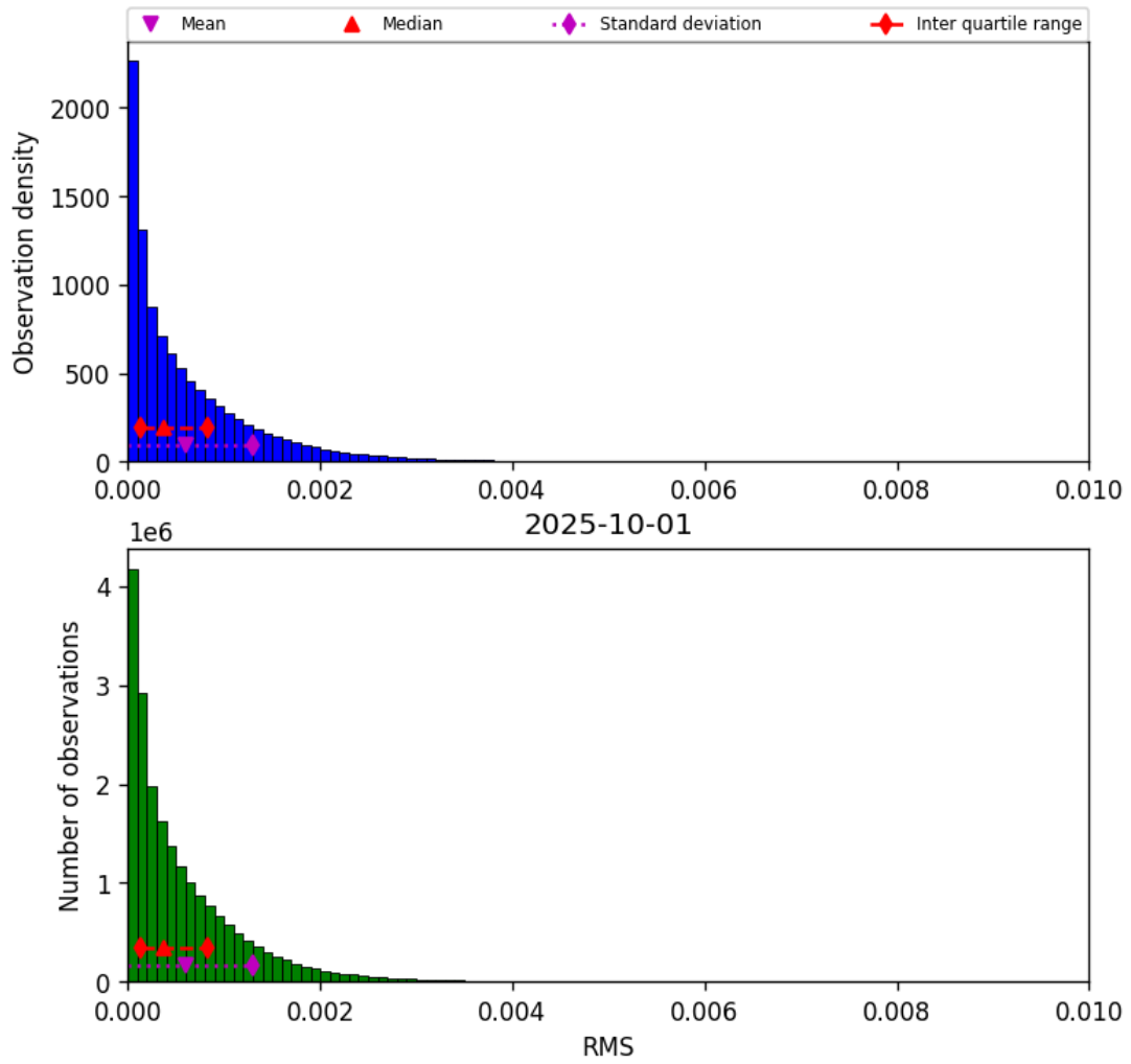
Figure 47: Histogram of “RMS” for 2025-10-01 to 2025-10-02
