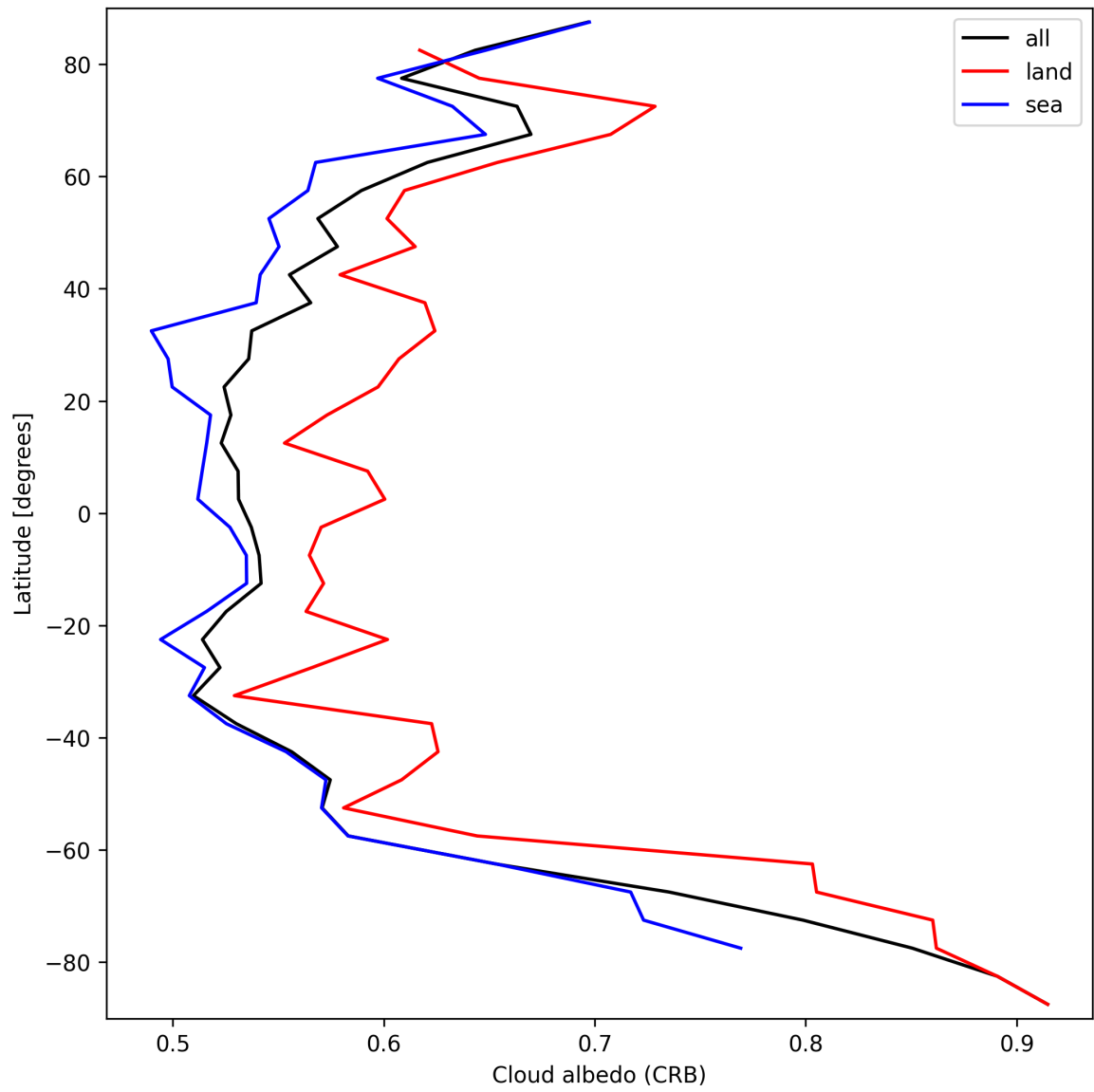
Figure 28: Zonal average of “Cloud albedo (CRB)” for 2025-10-01 to 2025-10-02.
