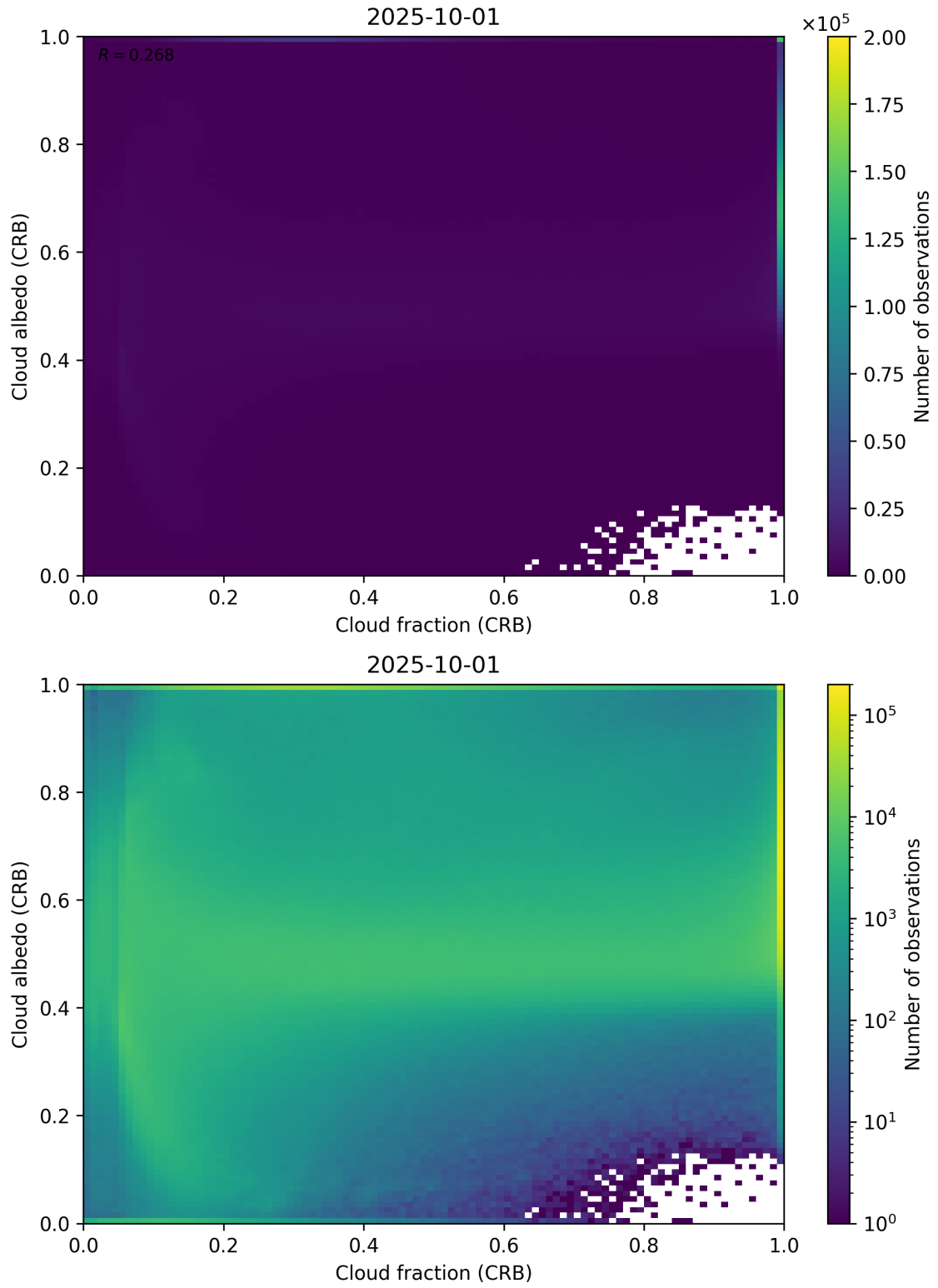
Figure 77: Scatter density plot of “Cloud fraction (CRB)” against “Cloud albedo (CRB)” for 2025-10-01 to 2025-10-02.
