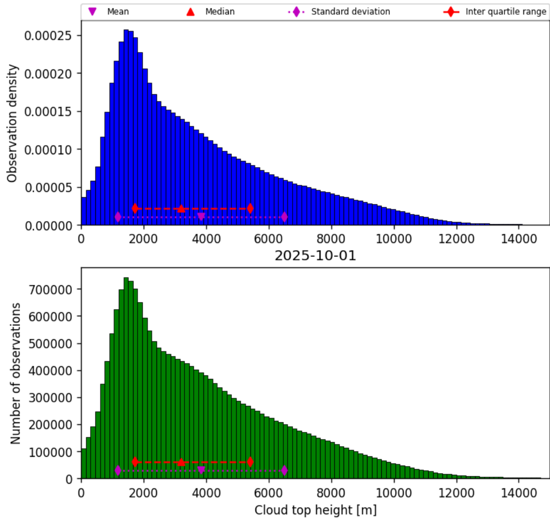
Figure 40: Histogram of “Cloud top height” for 2025-10-01 to 2025-10-02
