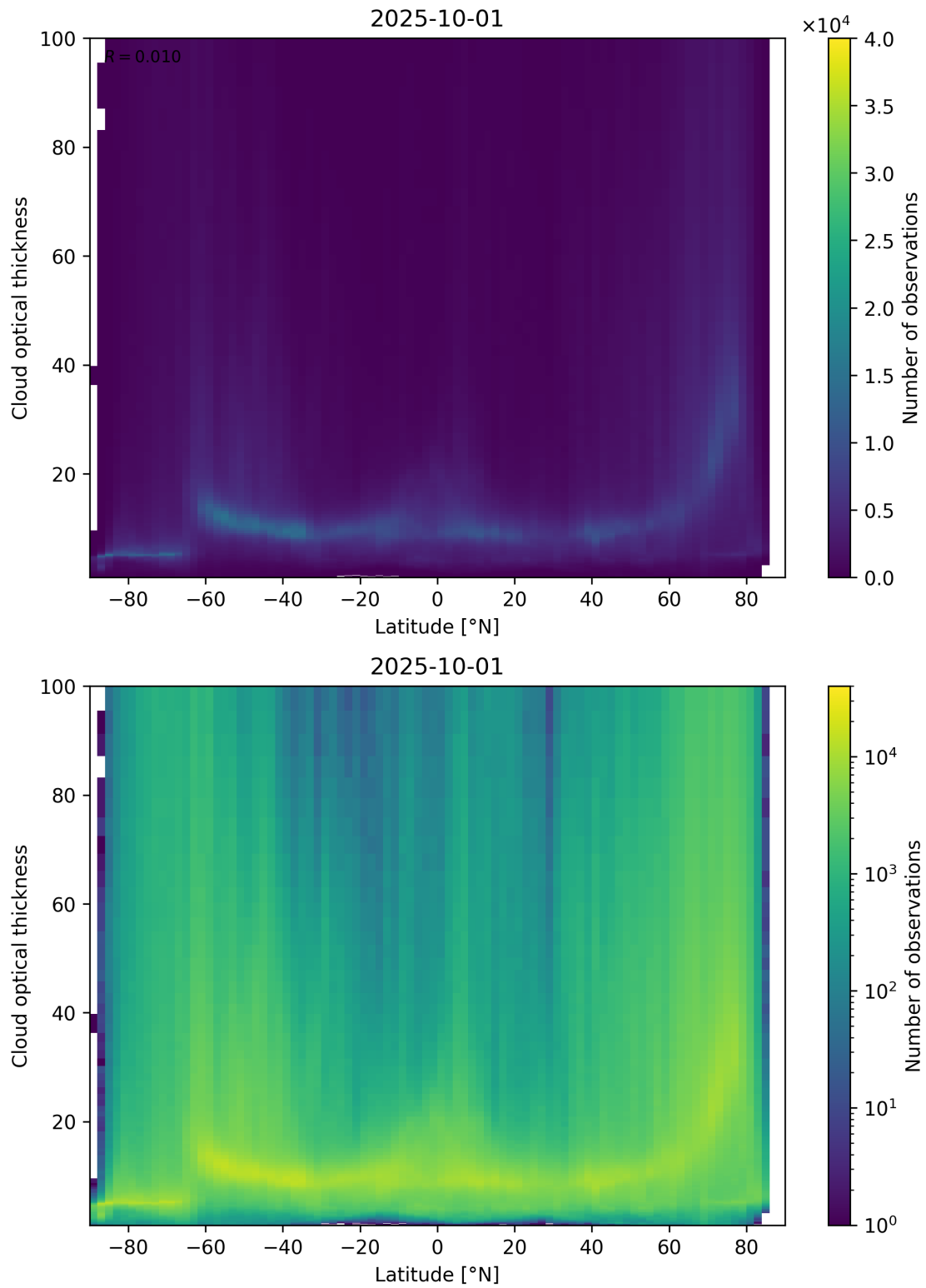
Figure 96: Scatter density plot of “Latitude” against “Cloud optical thickness” for 2025-10-01 to 2025-10-02.
