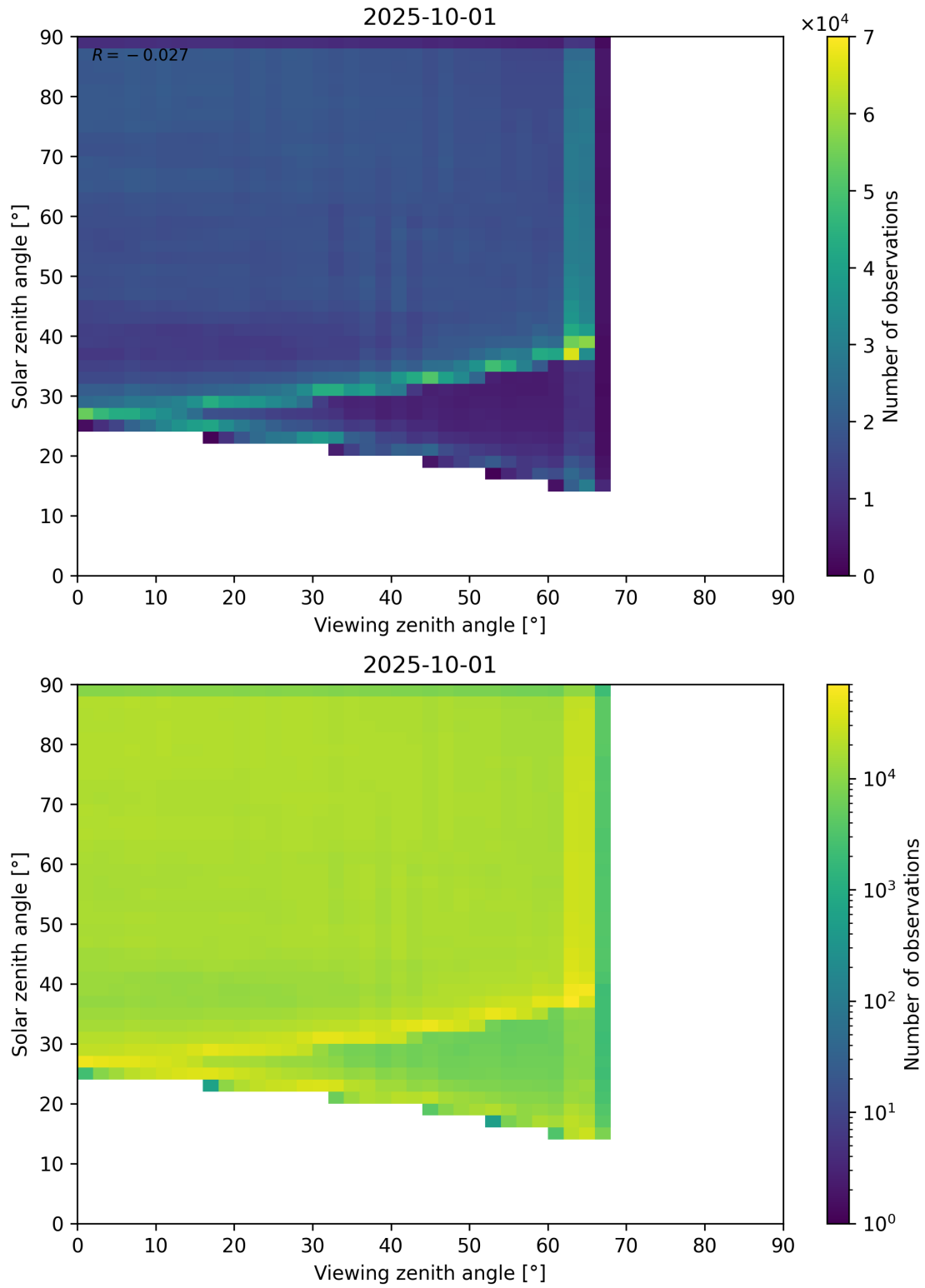
Figure 114: Scatter density plot of “Viewing zenith angle” against “Solar zenith angle” for 2025-10-01 to 2025-10-02.
