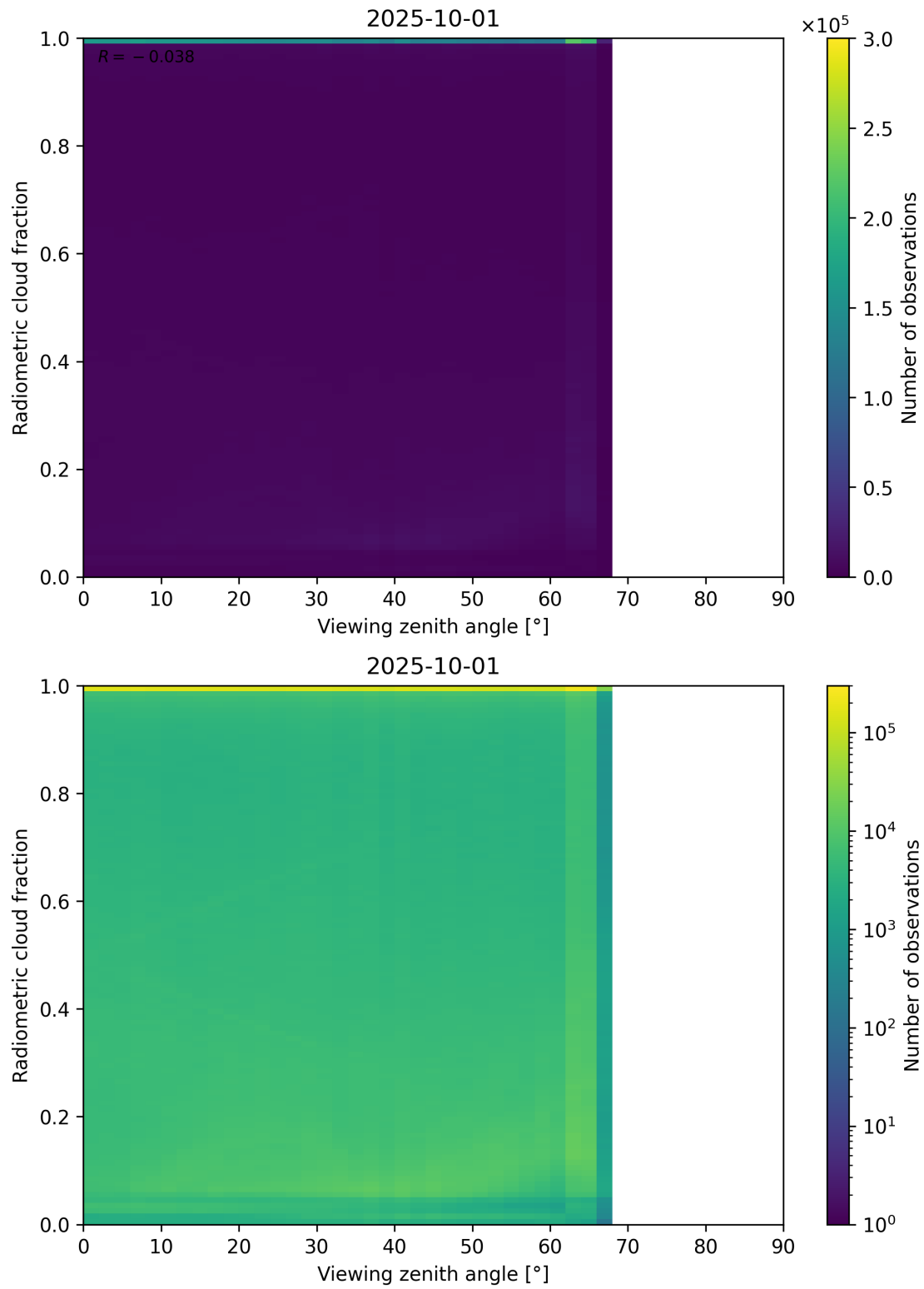
Figure 107: Scatter density plot of “Viewing zenith angle” against “Radiometric cloud fraction” for 2025-10-01 to 2025-10-02.
