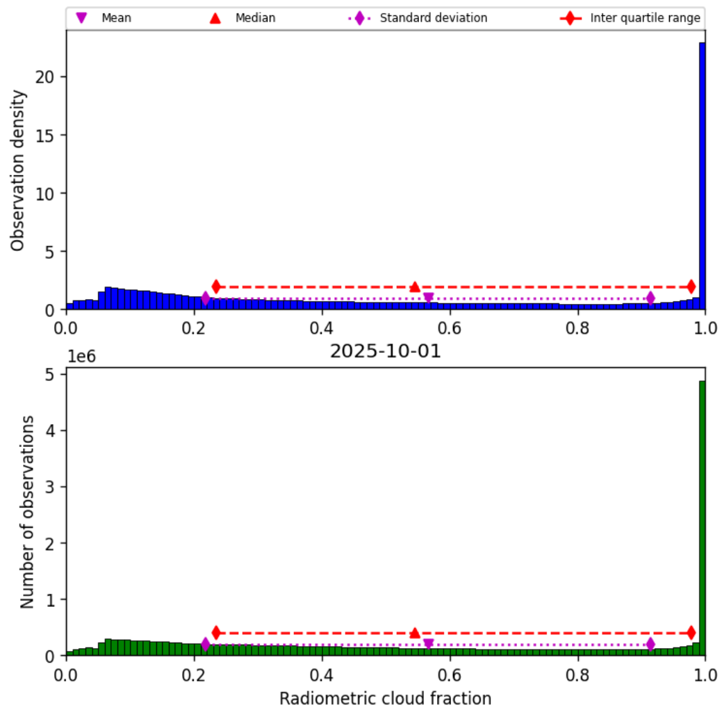
Figure 39: Histogram of “Radiometric cloud fraction” for 2025-10-01 to 2025-10-02
