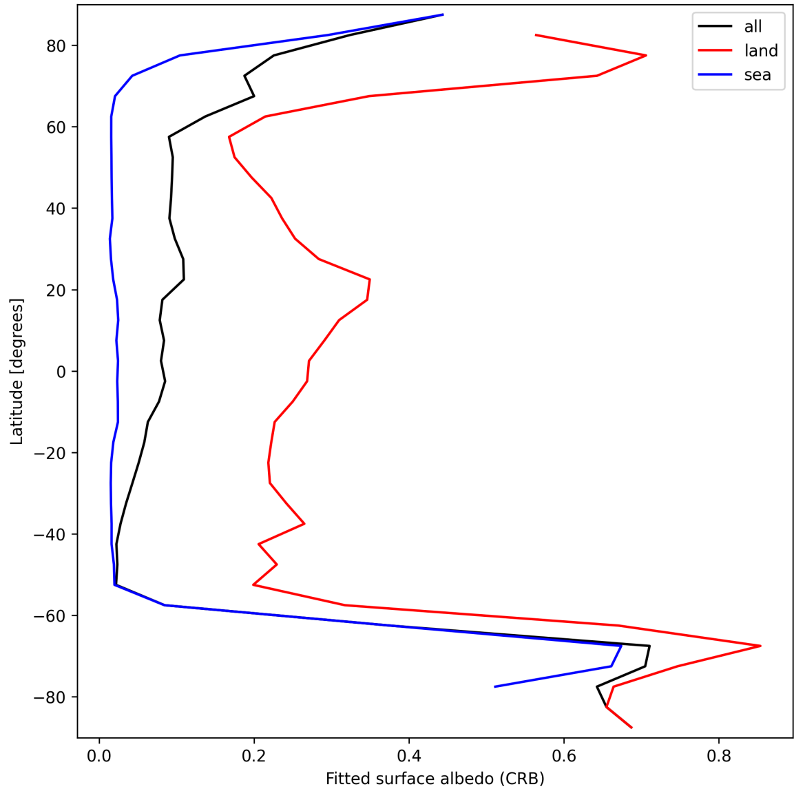
Figure 30: Zonal average of “Fitted surface albedo (CRB)” for 2025-10-01 to 2025-10-02.
