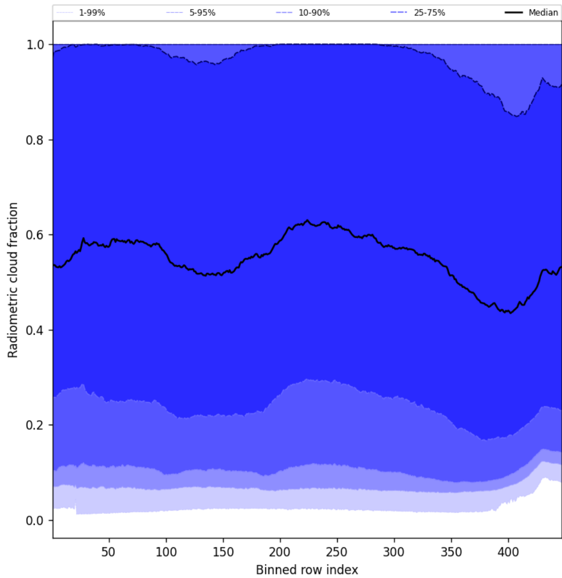
Figure 55: Along track statistics of “Radiometric cloud fraction” for 2025-10-01 to 2025-10-02
