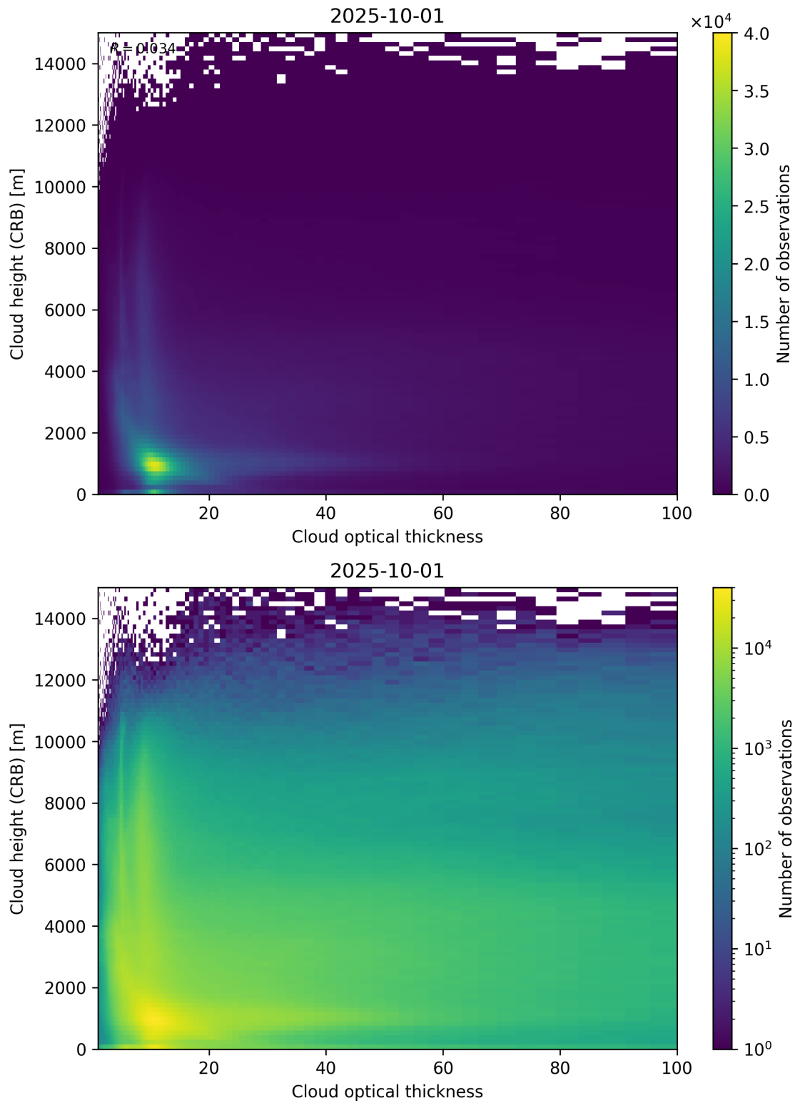
Figure 85: Scatter density plot of “Cloud optical thickness” against “Cloud height (CRB)” for 2025-10-01 to 2025-10-02.
