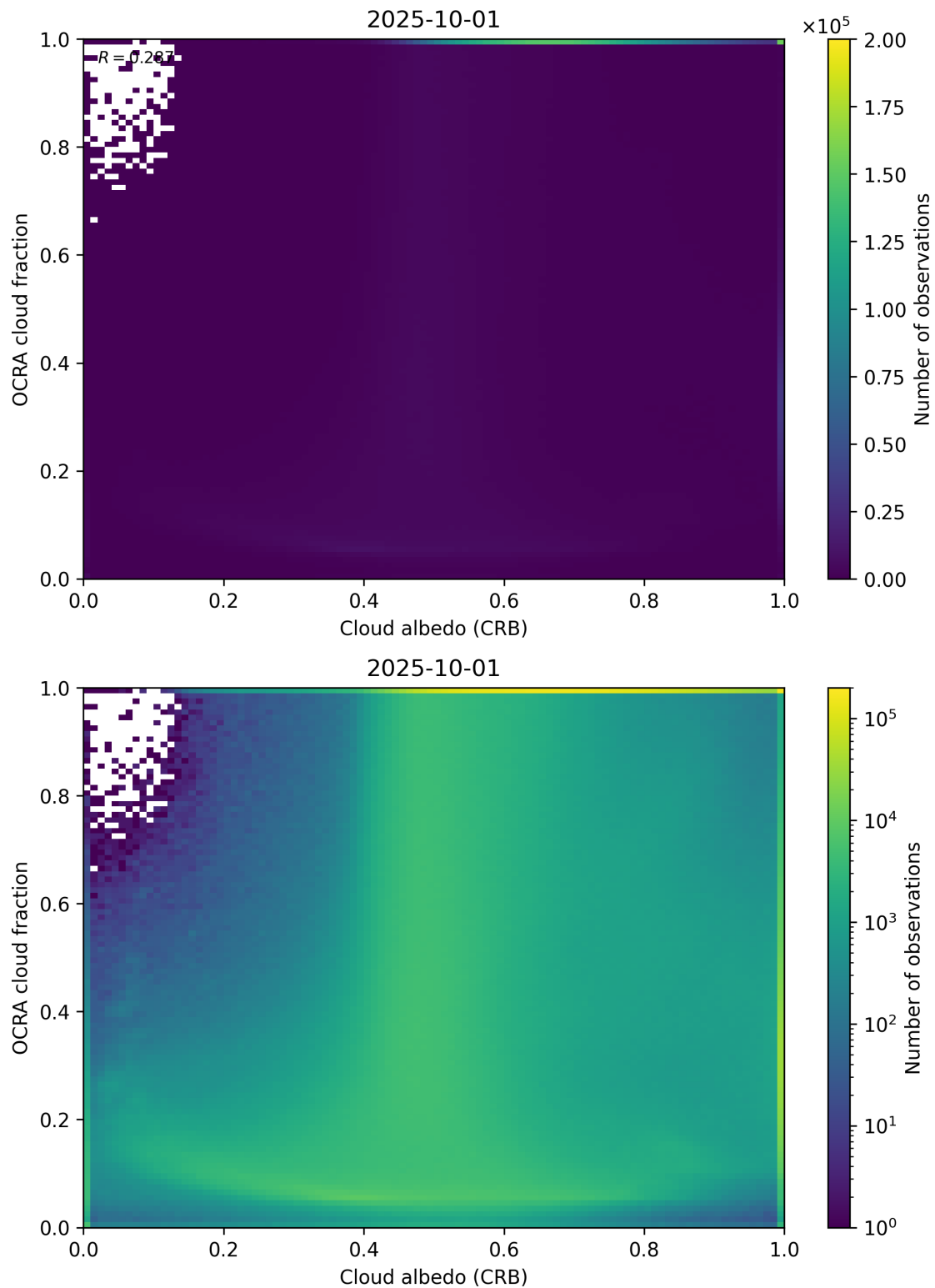
Figure 70: Scatter density plot of “Cloud albedo (CRB)” against “OCRA cloud fraction” for 2025-10-01 to 2025-10-02.
