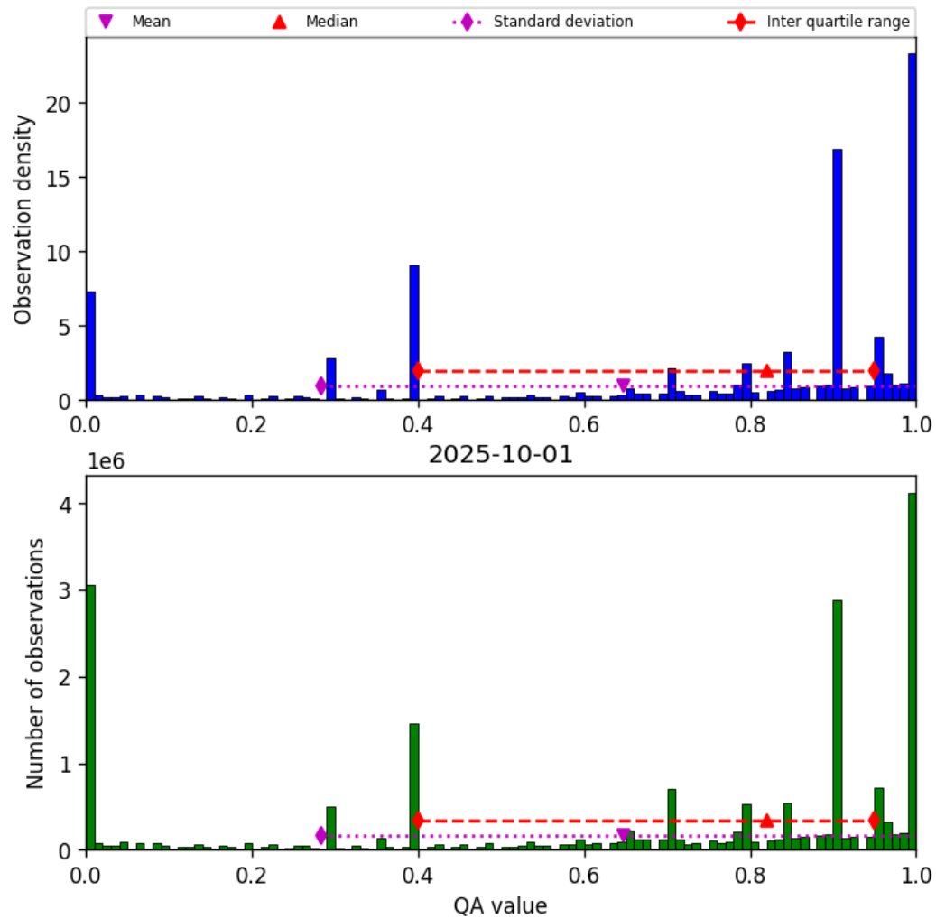
Figure 38: Histogram of “QA value” for 2025-10-01 to 2025-10-02
