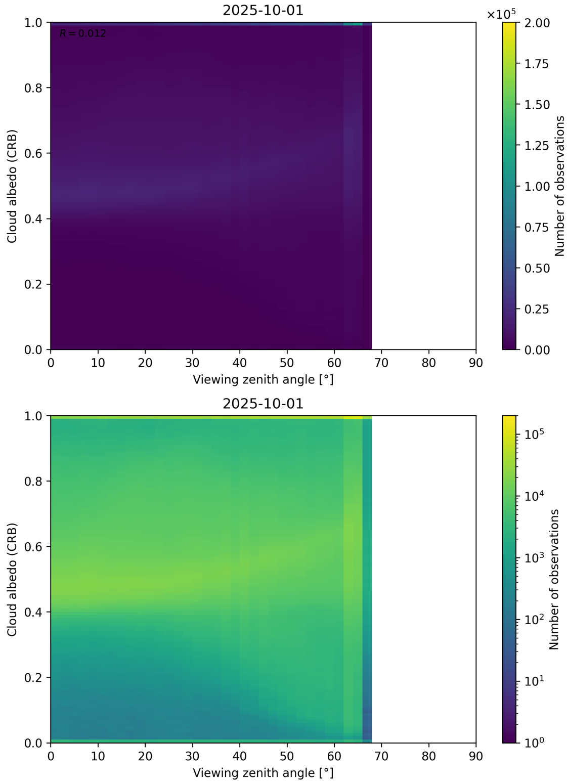
Figure 106: Scatter density plot of “Viewing zenith angle” against “Cloud albedo (CRB)” for 2025-10-01 to 2025-10-02.
