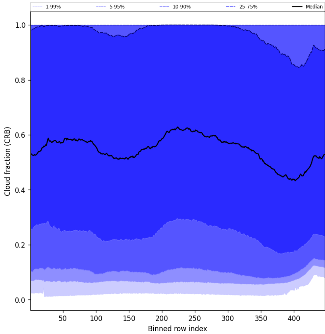
Figure 58: Along track statistics of “Cloud fraction (CRB)” for 2025-10-01 to 2025-10-02
