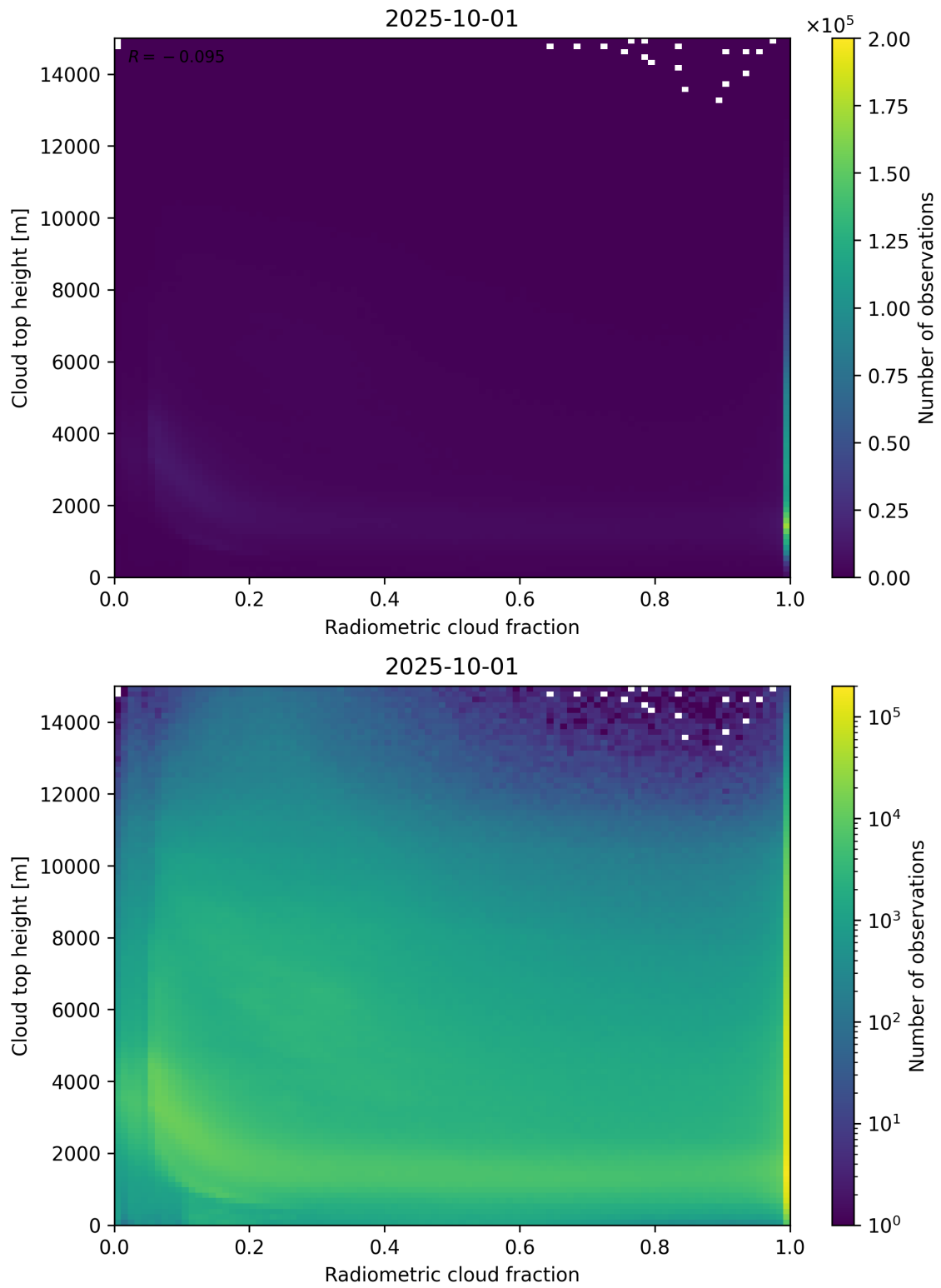
Figure 76: Scatter density plot of “Radiometric cloud fraction” against “Cloud top height” for 2025-10-01 to 2025-10-02.
