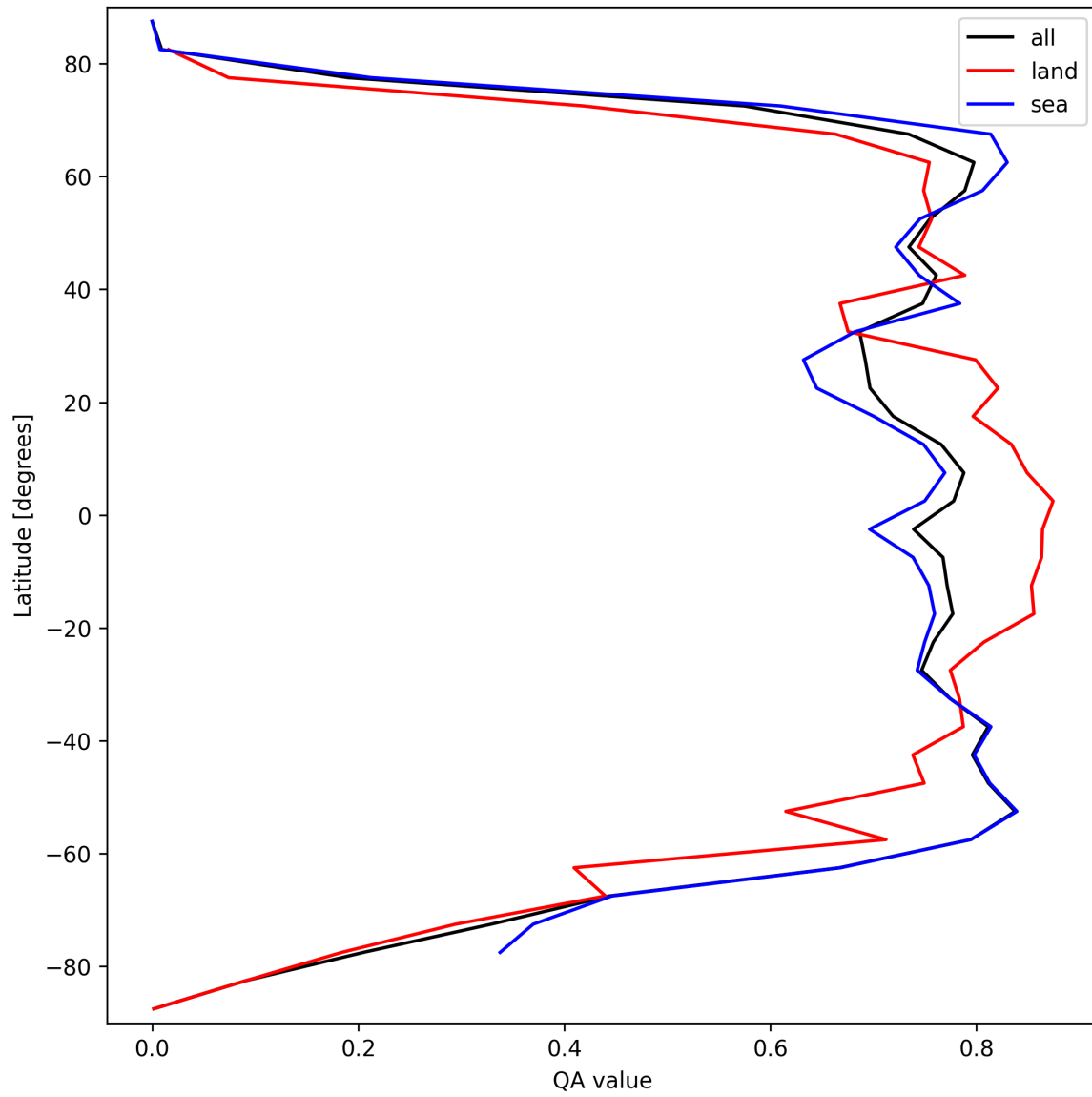
Figure 22: Zonal average of “QA value” for 2025-10-01 to 2025-10-02.
