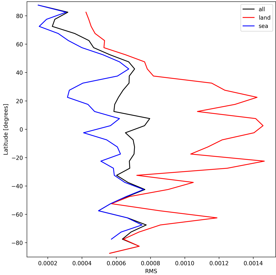
Figure 31: Zonal average of “RMS” for 2025-10-01 to 2025-10-02.
