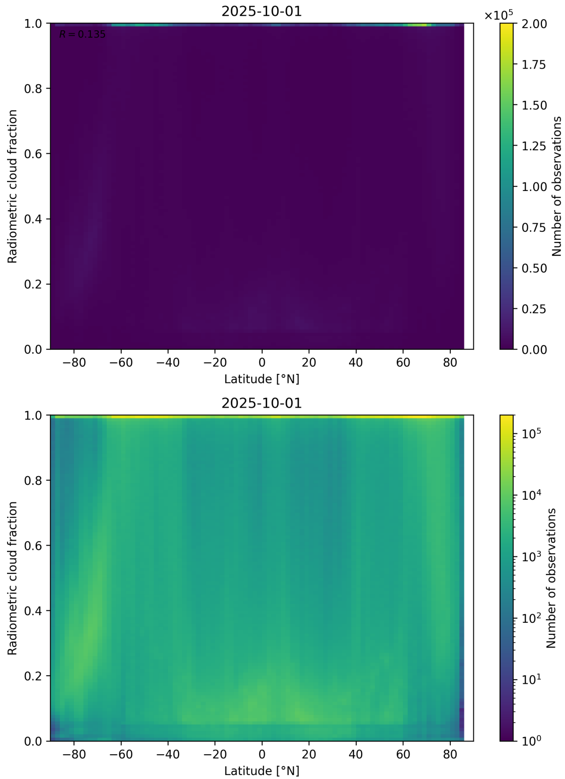
Figure 92: Scatter density plot of “Latitude” against “Radiometric cloud fraction” for 2025-10-01 to 2025-10-02.
