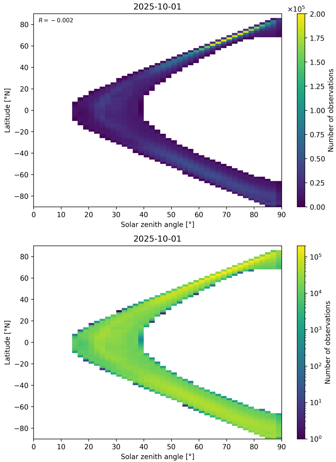
Figure 105: Scatter density plot of “Solar zenith angle” against “Latitude” for 2025-10-01 to 2025-10-02.
