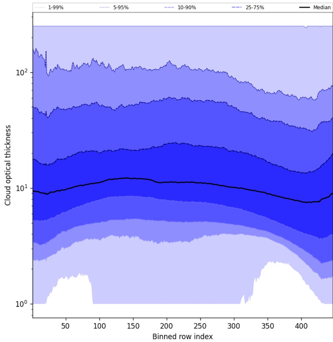
Figure 57: Along track statistics of “Cloud optical thickness” for 2025-10-01 to 2025-10-02
