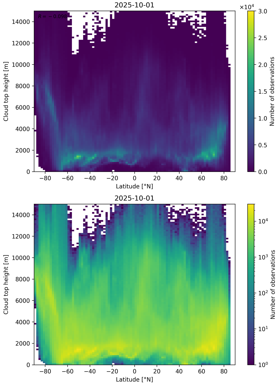
Figure 97: Scatter density plot of “Latitude” against “Cloud top height” for 2025-10-01 to 2025-10-02.
