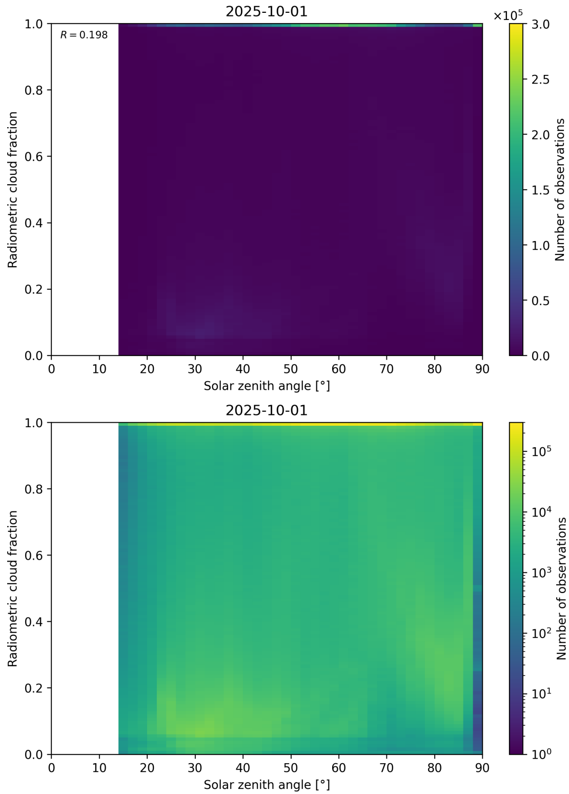
Figure 99: Scatter density plot of “Solar zenith angle” against “Radiometric cloud fraction” for 2025-10-01 to 2025-10-02.
