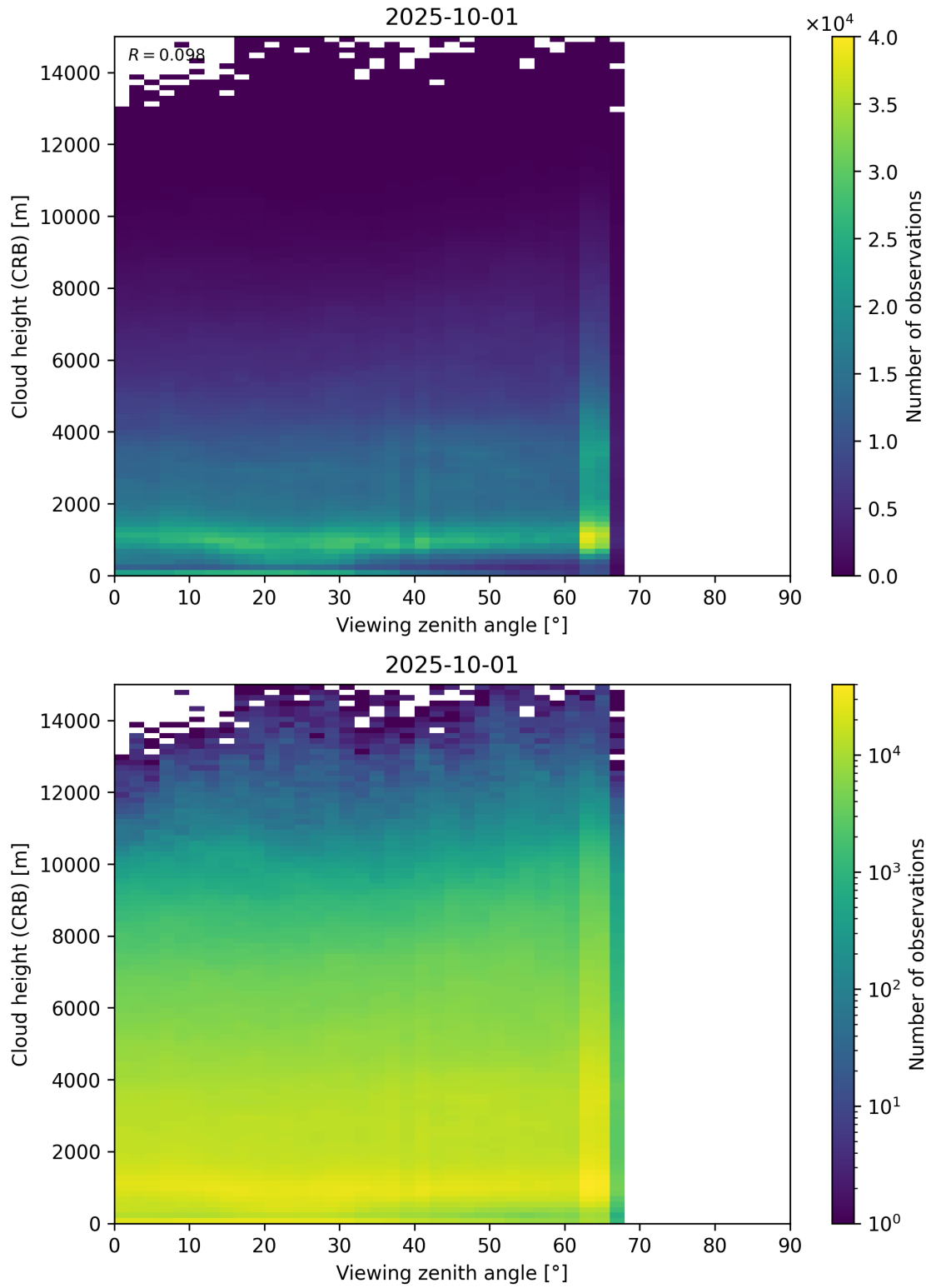
Figure 110: Scatter density plot of “Viewing zenith angle” against “Cloud height (CRB)” for 2025-10-01 to 2025-10-02.
