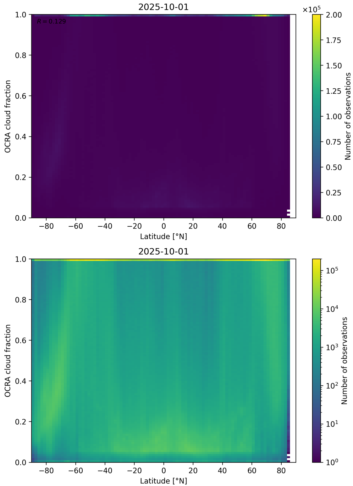
Figure 93: Scatter density plot of “Latitude” against “OCRA cloud fraction” for 2025-10-01 to 2025-10-02.
