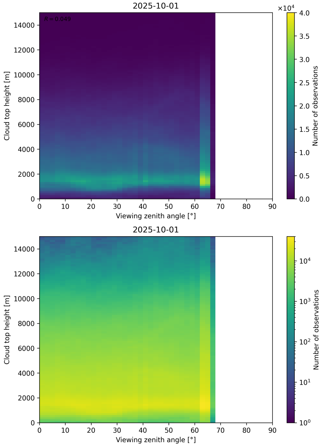
Figure 112: Scatter density plot of “Viewing zenith angle” against “Cloud top height” for 2025-10-01 to 2025-10-02.
