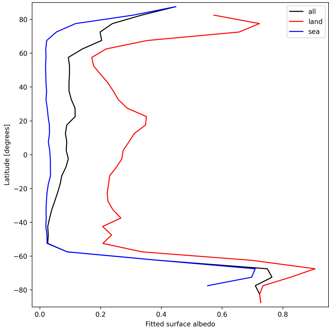
Figure 29: Zonal average of “Fitted surface albedo” for 2025-10-01 to 2025-10-02.
