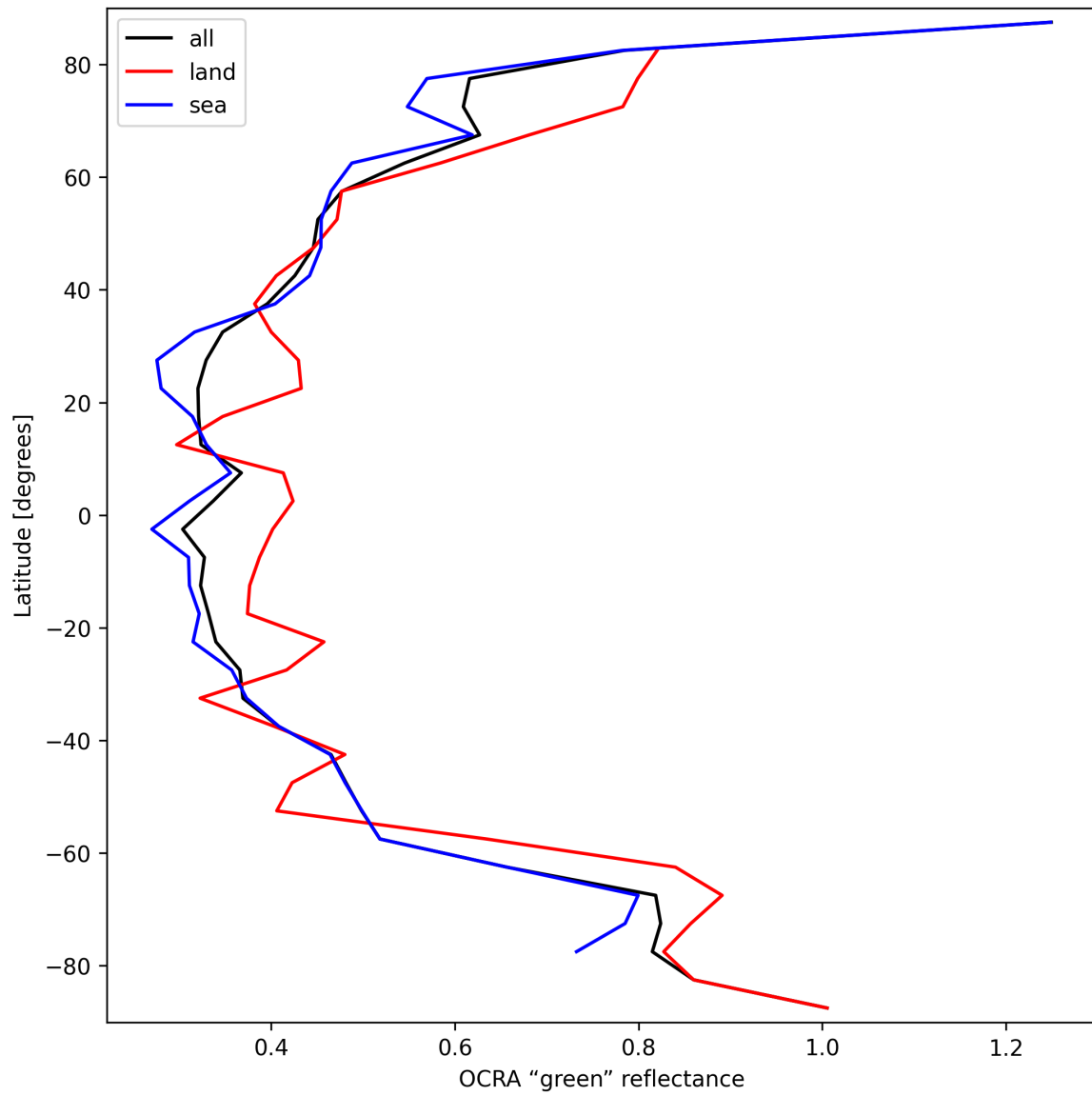
Figure 36: Zonal average of “OCRA “green” reflectance” for 2025-10-01 to 2025-10-02.
