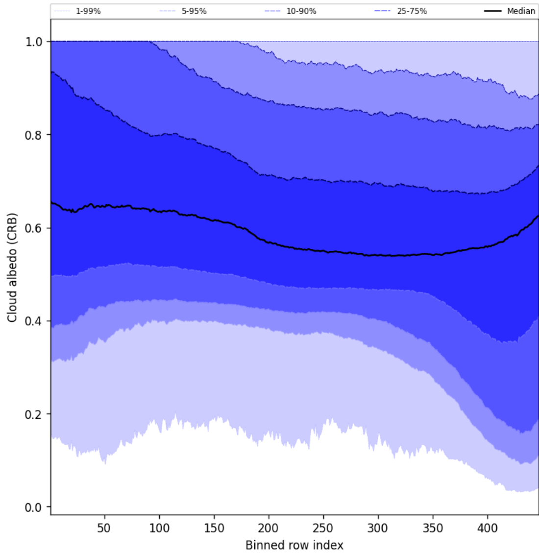
Figure 60: Along track statistics of “Cloud albedo (CRB)” for 2025-10-01 to 2025-10-02
