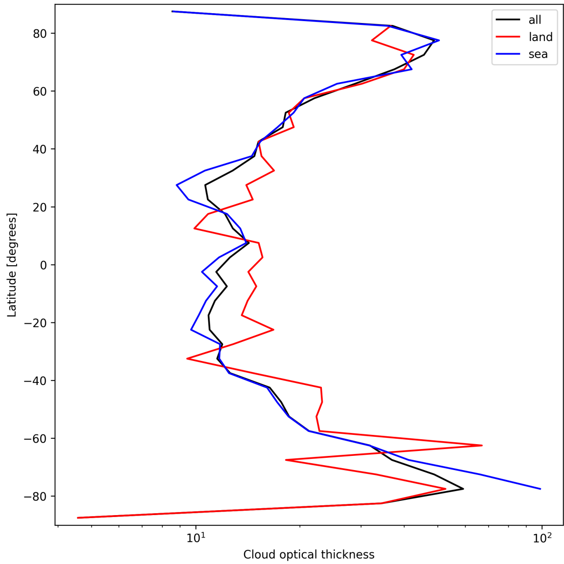
Figure 25: Zonal average of “Cloud optical thickness” for 2025-10-01 to 2025-10-02.
