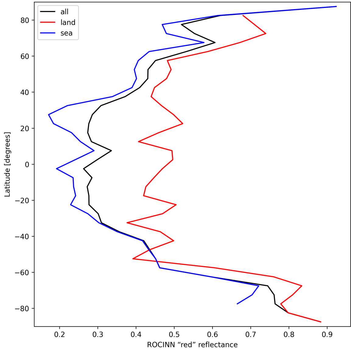
Figure 37: Zonal average of “ROCINN “red” reflectance” for 2025-10-01 to 2025-10-02.
