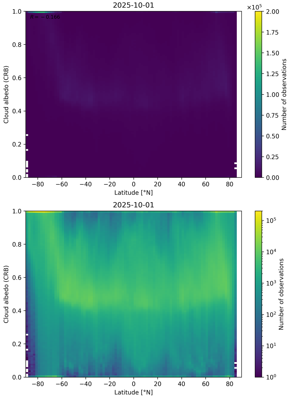
Figure 91: Scatter density plot of “Latitude” against “Cloud albedo (CRB)” for 2025-10-01 to 2025-10-02.
