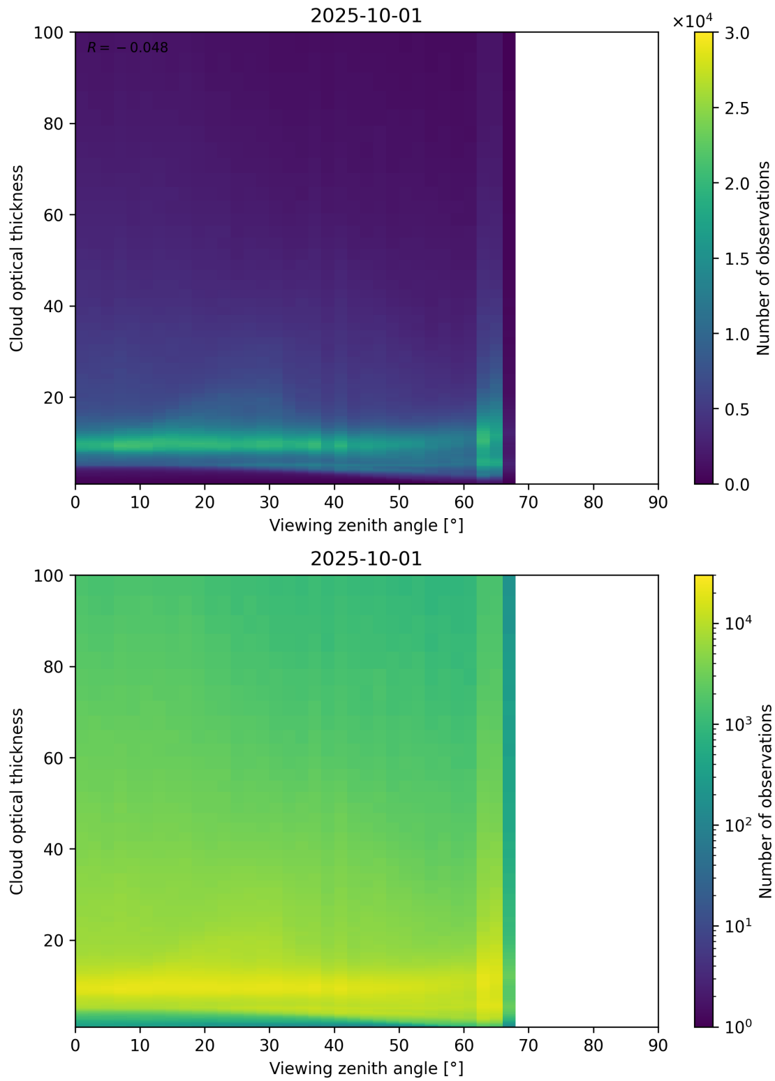
Figure 111: Scatter density plot of “Viewing zenith angle” against “Cloud optical thickness” for 2025-10-01 to 2025-10-02.
