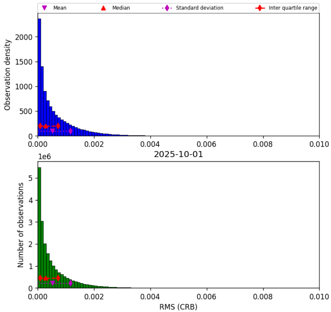
Figure 48: Histogram of "RMS (CRB)" for 2025-10-01 to 2025-10-02
