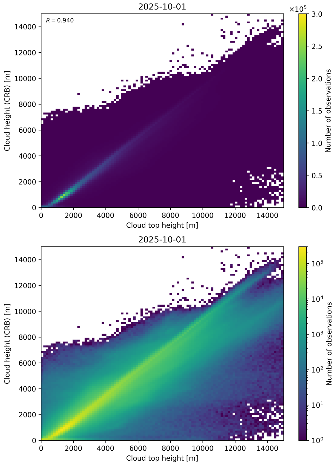
Figure 89: Scatter density plot of “Cloud top height” against “Cloud height (CRB)” for 2025-10-01 to 2025-10-02.
