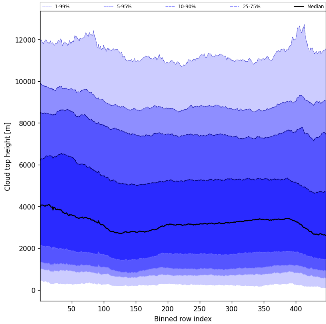
Figure 56: Along track statistics of “Cloud top height” for 2025-10-01 to 2025-10-02
