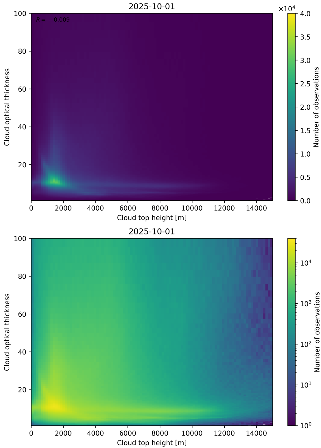
Figure 90: Scatter density plot of “Cloud top height” against “Cloud optical thickness” for 2025-10-01 to 2025-10-02.
