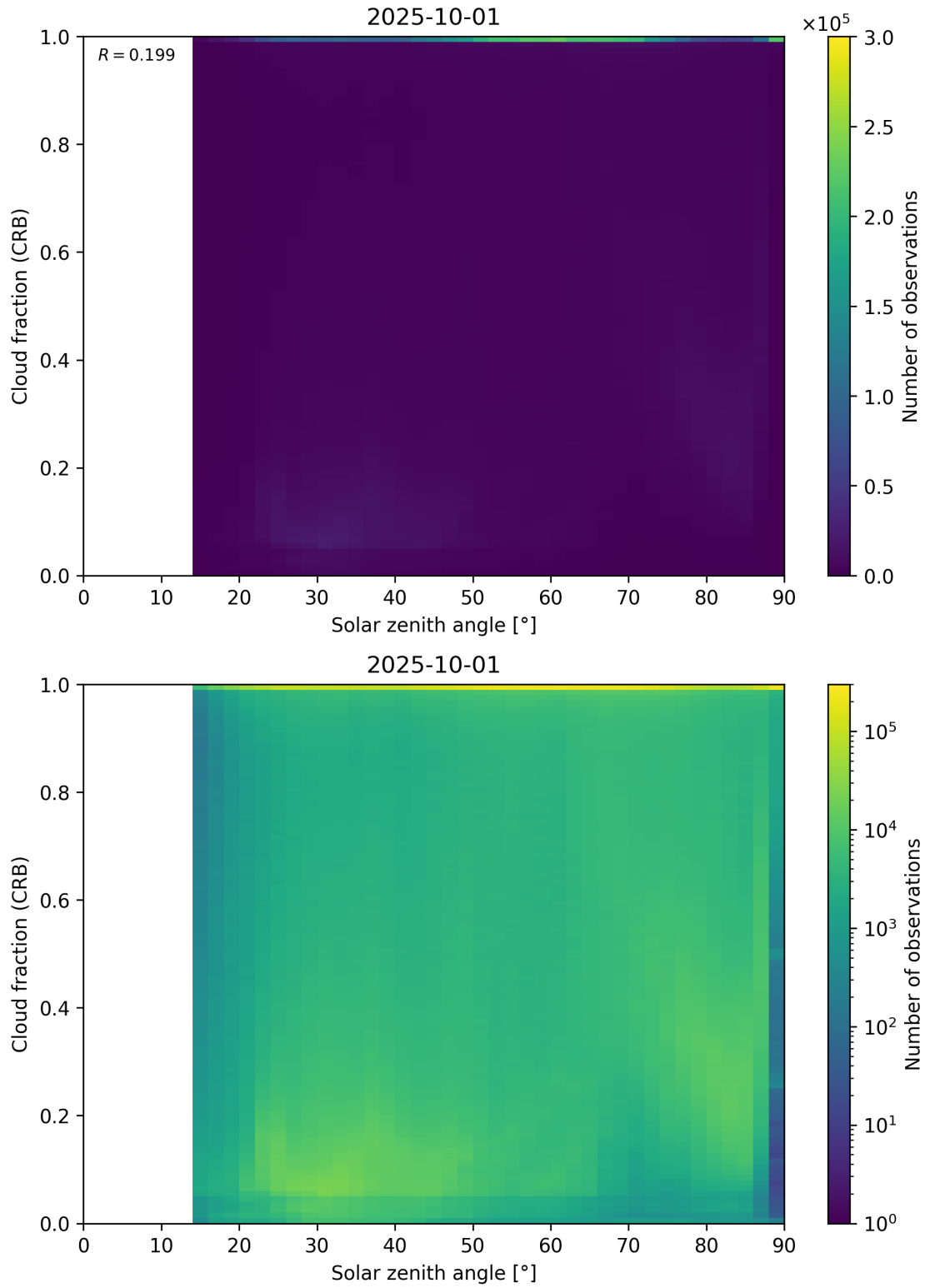
Figure 101: Scatter density plot of “Solar zenith angle” against “Cloud fraction (CRB)” for 2025-10-01 to 2025-10-02.
