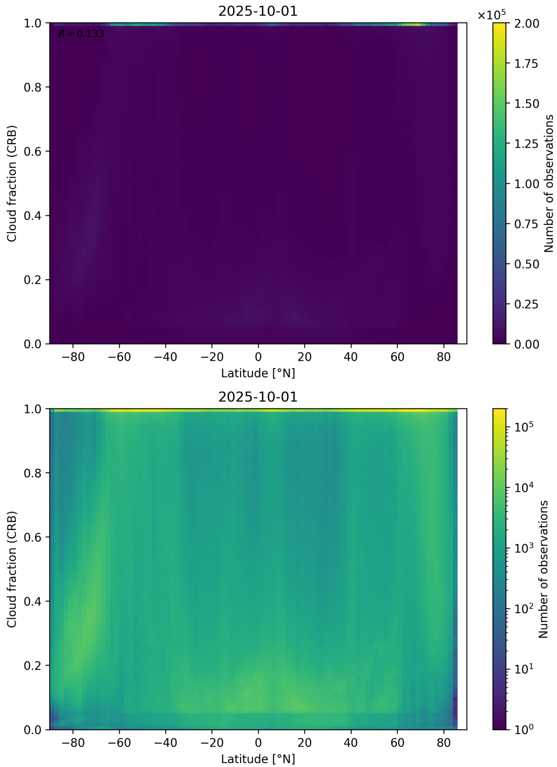
Figure 94: Scatter density plot of “Latitude” against “Cloud fraction (CRB)” for 2025-10-01 to 2025-10-02.
