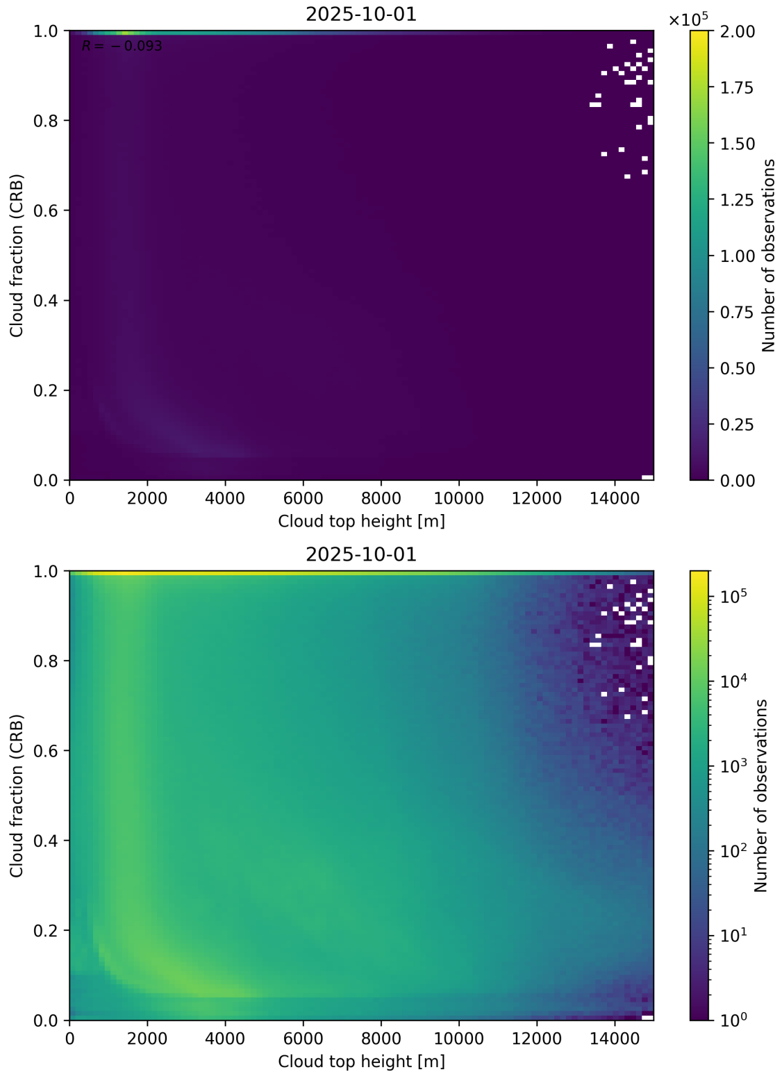
Figure 88: Scatter density plot of “Cloud top height” against “Cloud fraction (CRB)” for 2025-10-01 to 2025-10-02.
