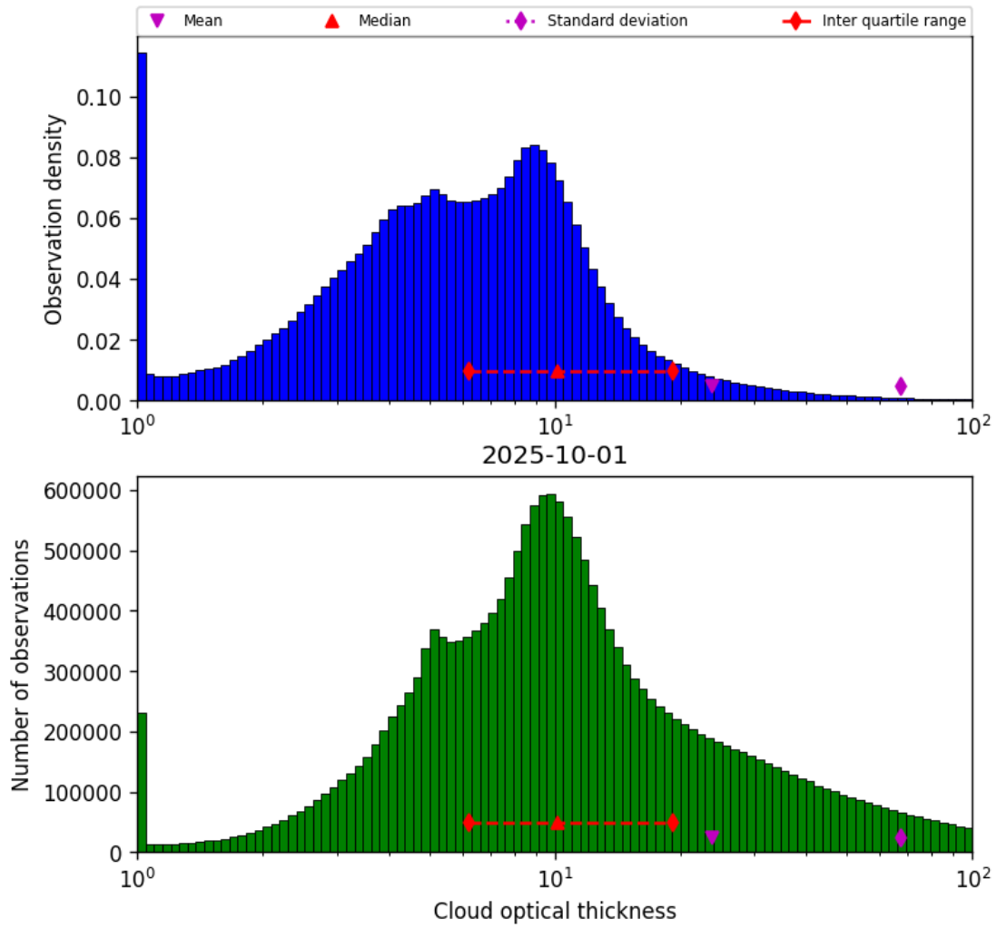
Figure 41: Histogram of “Cloud optical thickness” for 2025-10-01 to 2025-10-02
