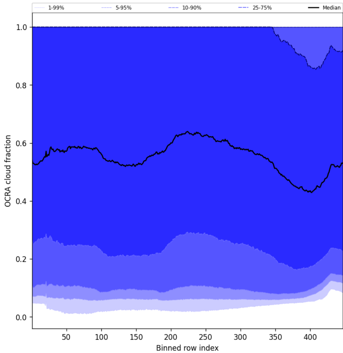
Figure 66: Along track statistics of “OCRA cloud fraction” for 2025-10-01 to 2025-10-02
