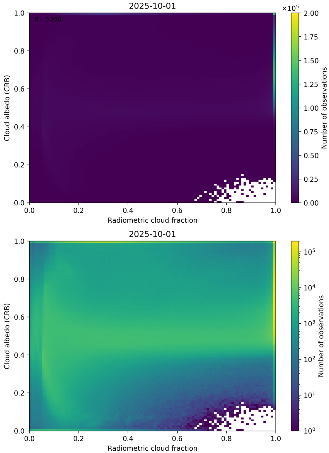
Figure 71: Scatter density plot of “Radiometric cloud fraction” against “Cloud albedo (CRB)” for 2025-10-01 to 2025-10-02.
