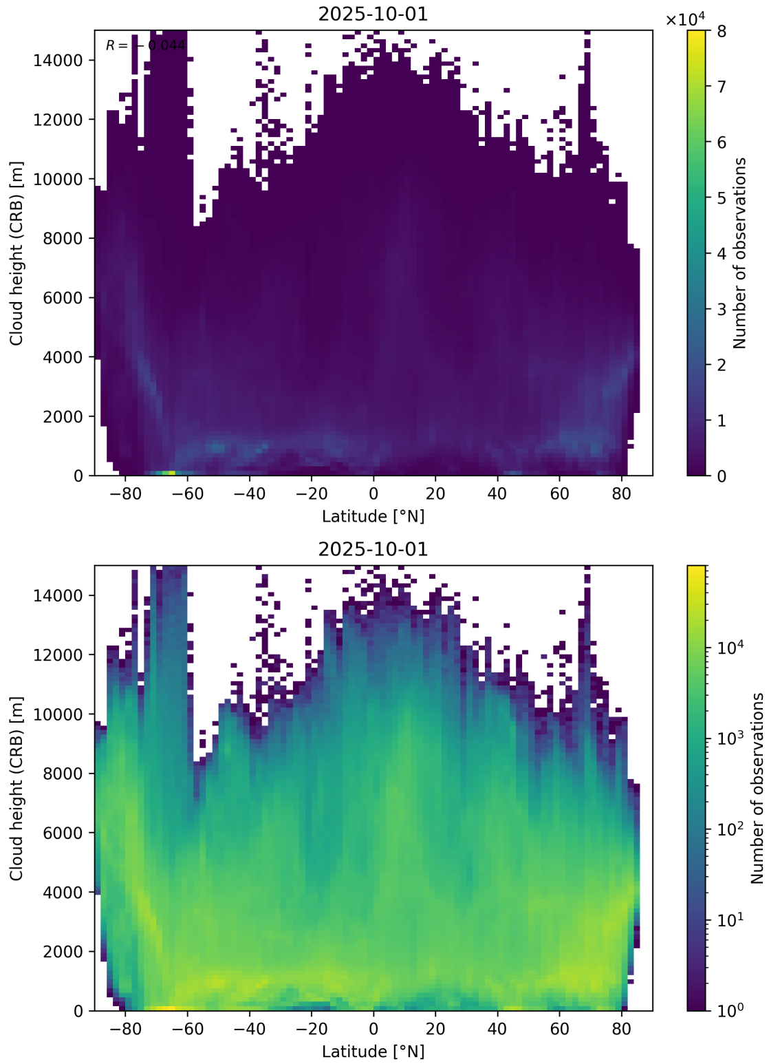
Figure 95: Scatter density plot of “Latitude” against “Cloud height (CRB)” for 2025-10-01 to 2025-10-02.
