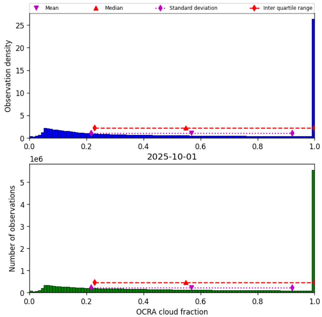
Figure 50: Histogram of “OCRA cloud fraction” for 2025-10-01 to 2025-10-02
