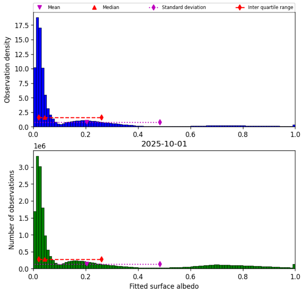
Figure 45: Histogram of “Fitted surface albedo” for 2025-10-01 to 2025-10-02
