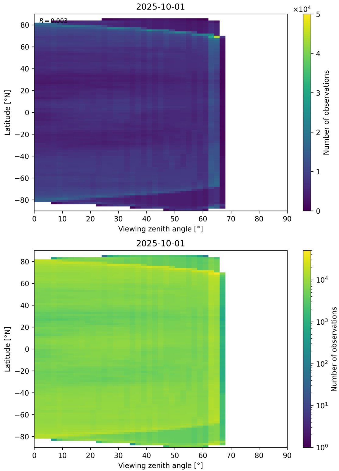
Figure 113: Scatter density plot of “Viewing zenith angle” against “Latitude” for 2025-10-01 to 2025-10-02.
