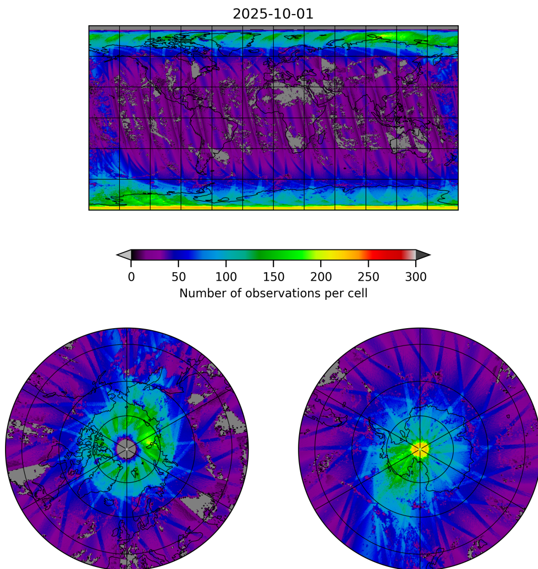
Figure 21: Map of the number of observations for 2025-10-01 to 2025-10-02
