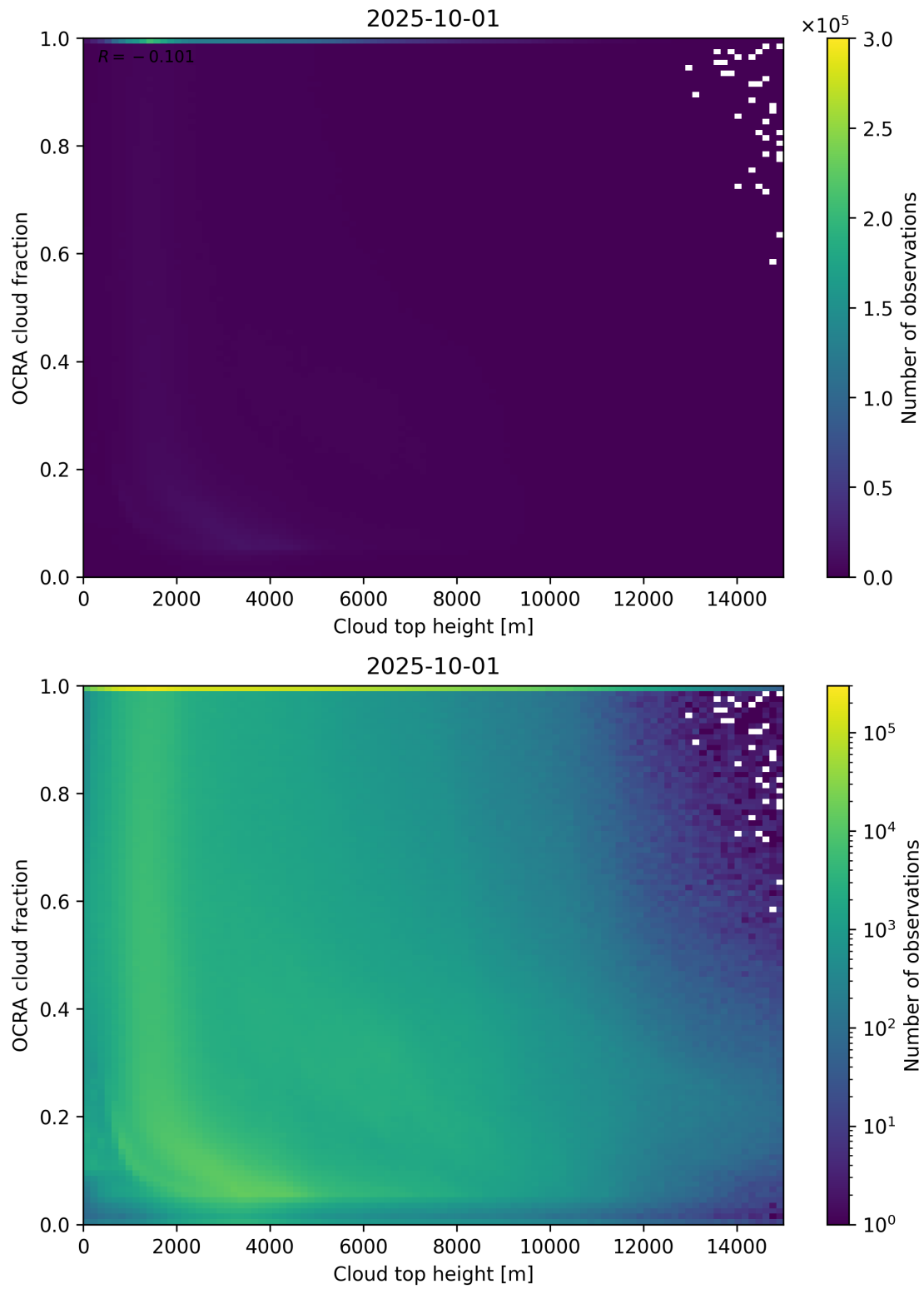
Figure 87: Scatter density plot of “Cloud top height” against “OCRA cloud fraction” for 2025-10-01 to 2025-10-02.
