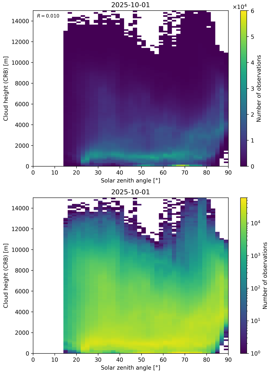
Figure 102: Scatter density plot of “Solar zenith angle” against “Cloud height (CRB)” for 2025-10-01 to 2025-10-02.
