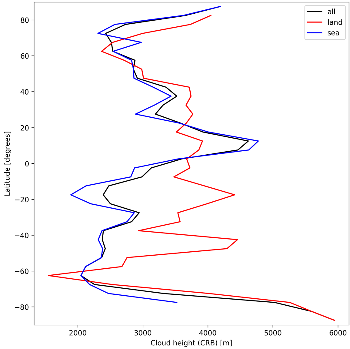
Figure 27: Zonal average of “Cloud height (CRB)” for 2025-10-01 to 2025-10-02.
