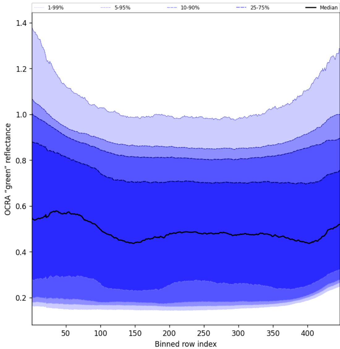
Figure 68: Along track statistics of “OCRA “green” reflectance” for 2025-10-01 to 2025-10-02
