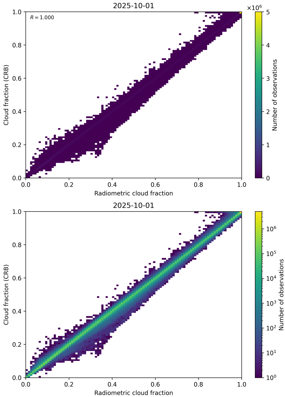
Figure 73: Scatter density plot of “Radiometric cloud fraction” against “Cloud fraction (CRB)” for 2025-10-01 to 2025-10-02.
