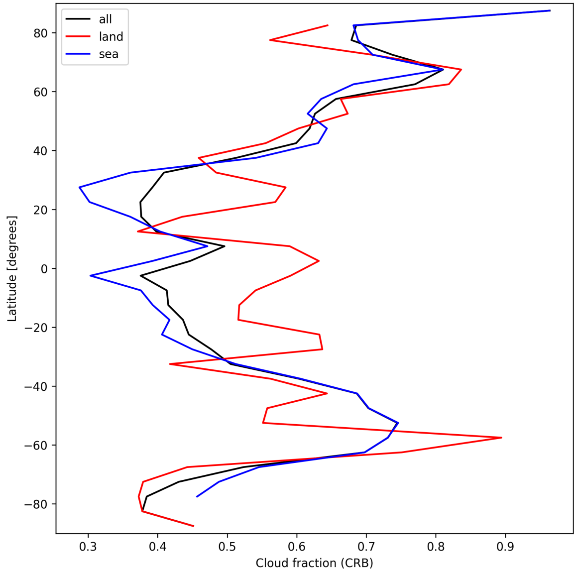
Figure 26: Zonal average of “Cloud fraction (CRB)” for 2025-10-01 to 2025-10-02.
