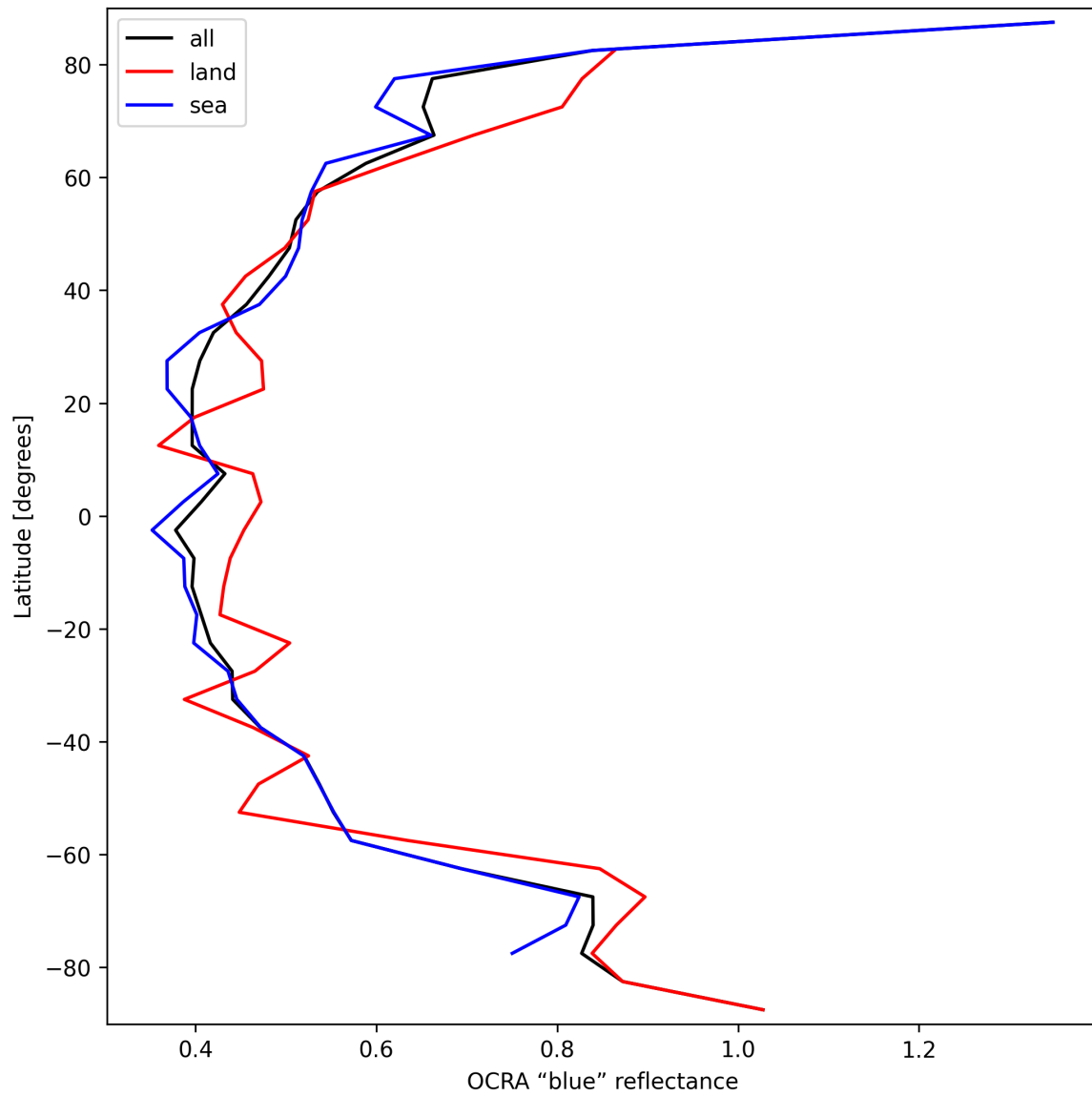
Figure 35: Zonal average of “OCRA “blue” reflectance” for 2025-10-01 to 2025-10-02.
