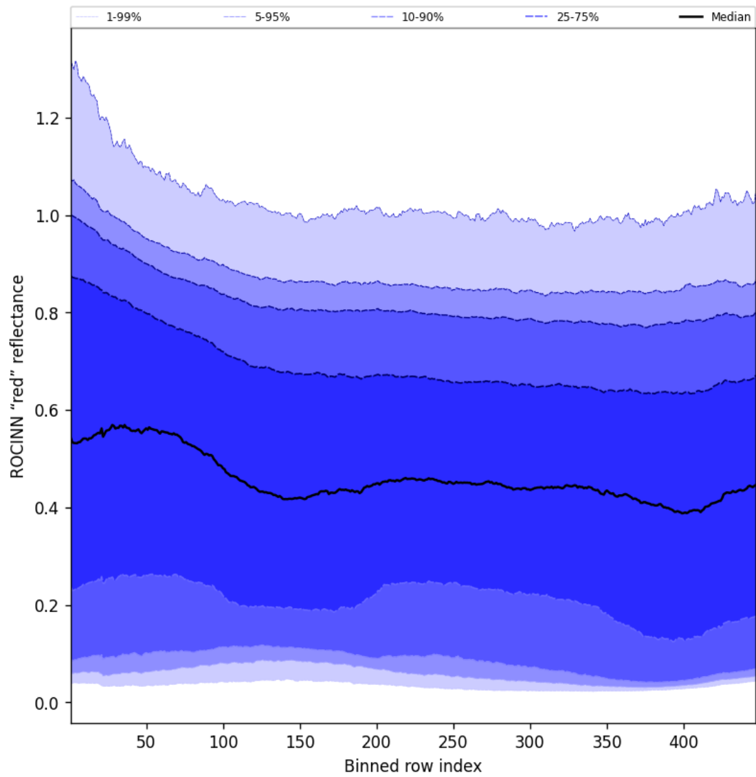
Figure 69: Along track statistics of “ROCINN “red” reflectance” for 2025-10-01 to 2025-10-02
