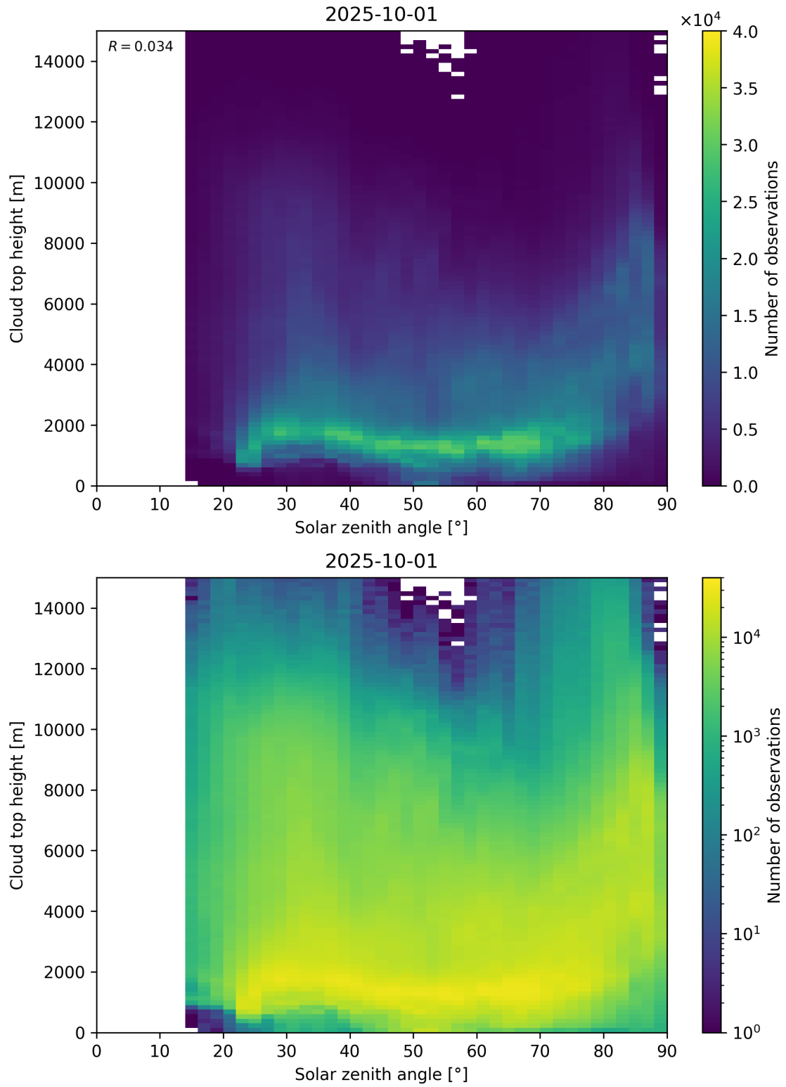
Figure 104: Scatter density plot of “Solar zenith angle” against “Cloud top height” for 2025-10-01 to 2025-10-02.
