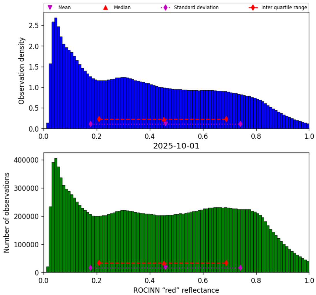
Figure 53: Histogram of “ROCINN “red” reflectance” for 2025-10-01 to 2025-10-02
