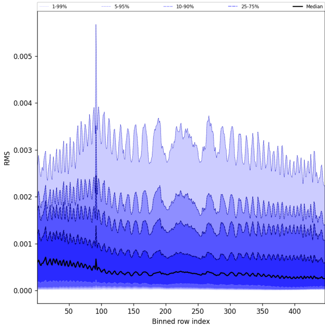
Figure 63: Along track statistics of “RMS” for 2025-10-01 to 2025-10-02
