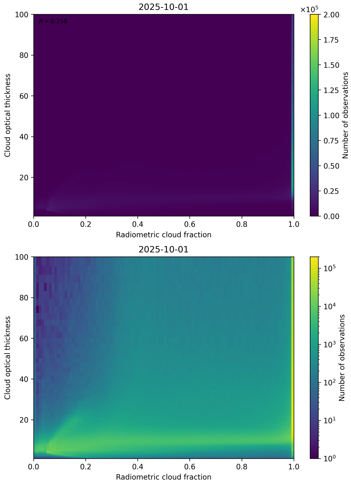
Figure 75: Scatter density plot of “Radiometric cloud fraction” against “Cloud optical thickness” for 2025-10-01 to 2025-10-02.
