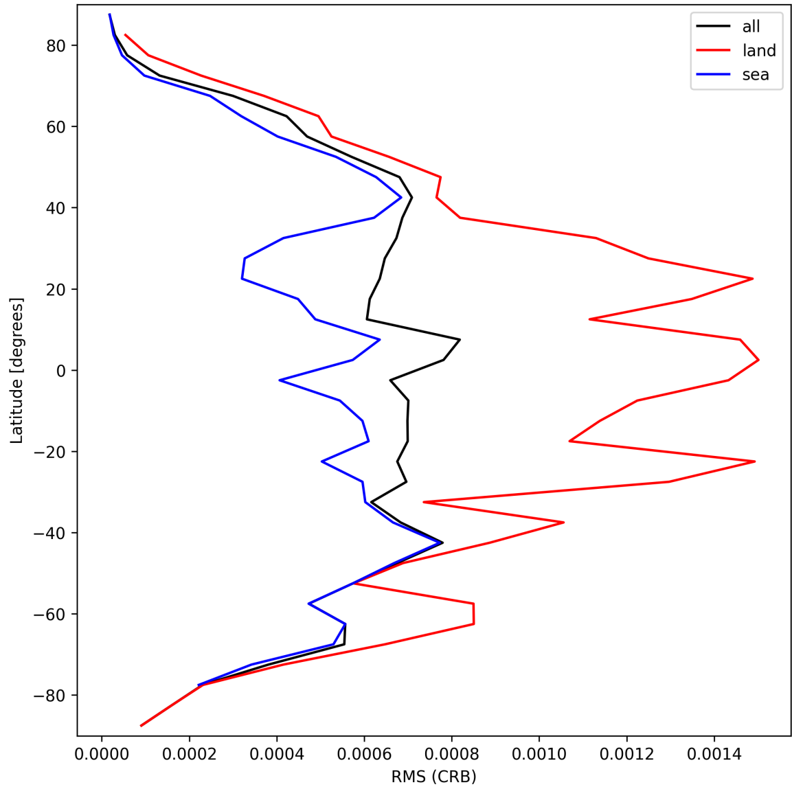
Figure 32: Zonal average of “RMS (CRB)” for 2025-10-01 to 2025-10-02.
