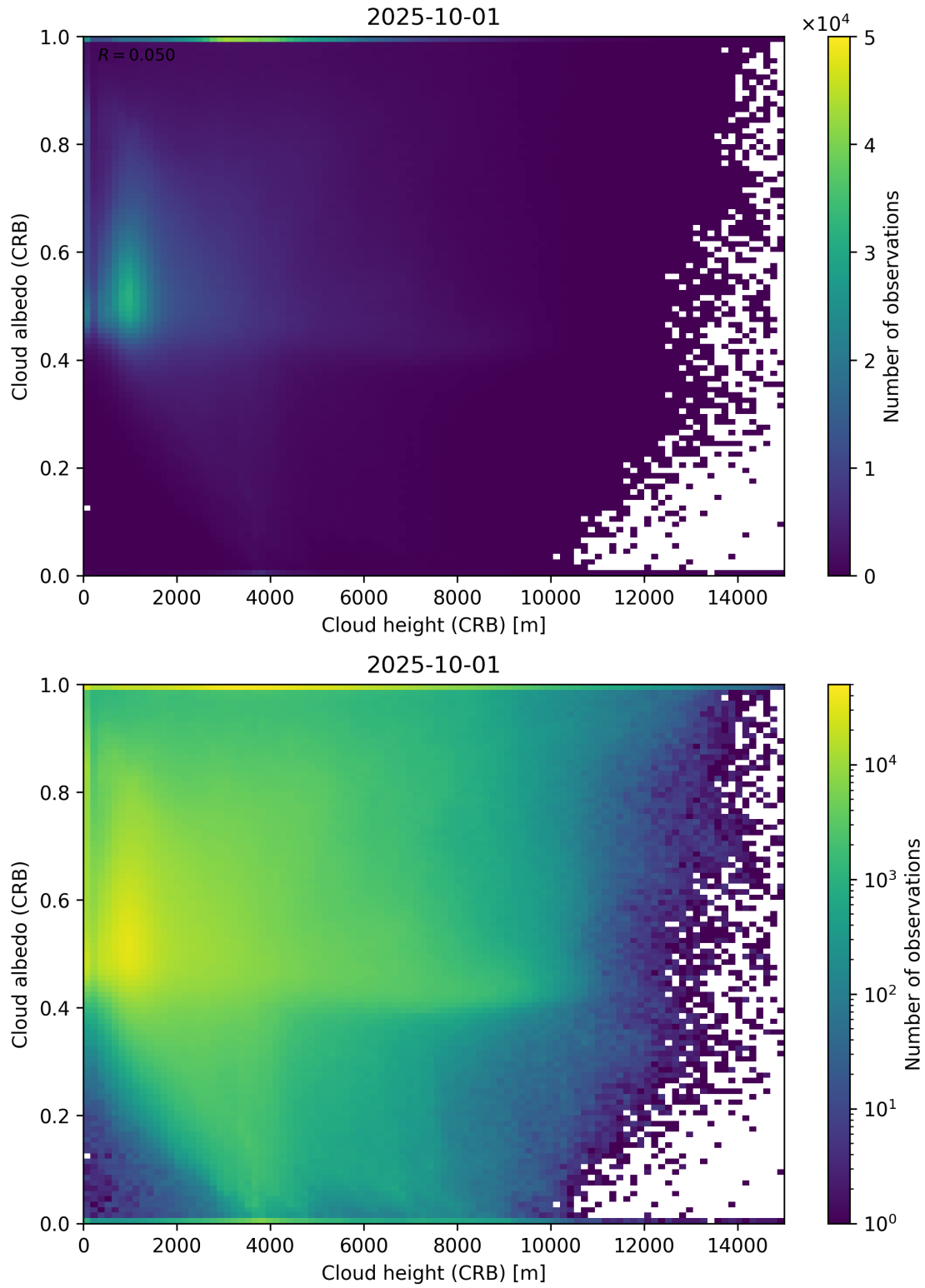
Figure 80: Scatter density plot of “Cloud height (CRB)” against “Cloud albedo (CRB)” for 2025-10-01 to 2025-10-02.
