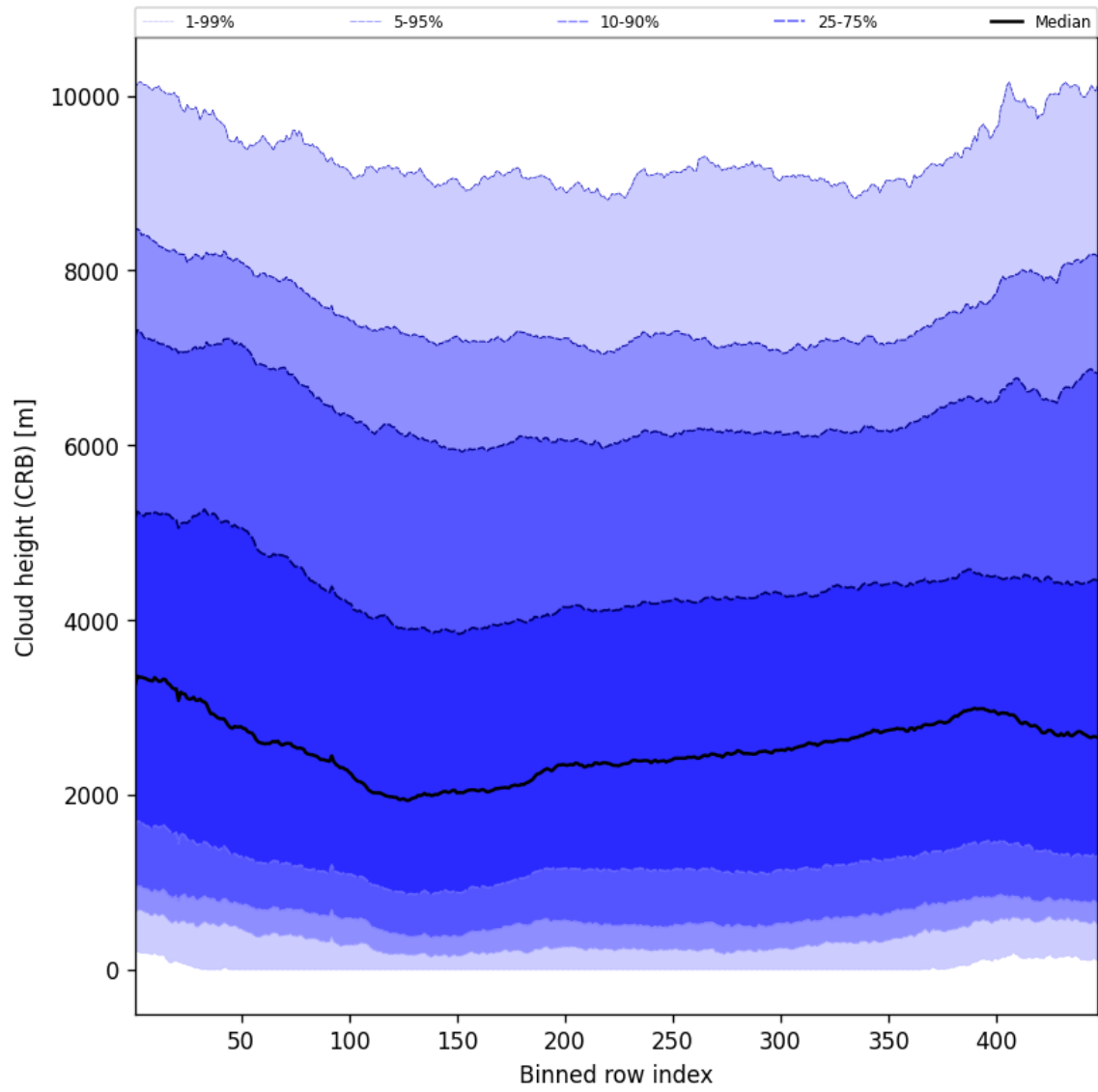
Figure 59: Along track statistics of “Cloud height (CRB)” for 2025-10-01 to 2025-10-02
