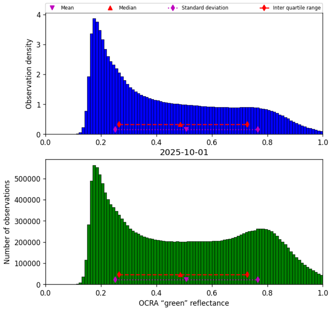
Figure 52: Histogram of “OCRA “green” reflectance” for 2025-10-01 to 2025-10-02
