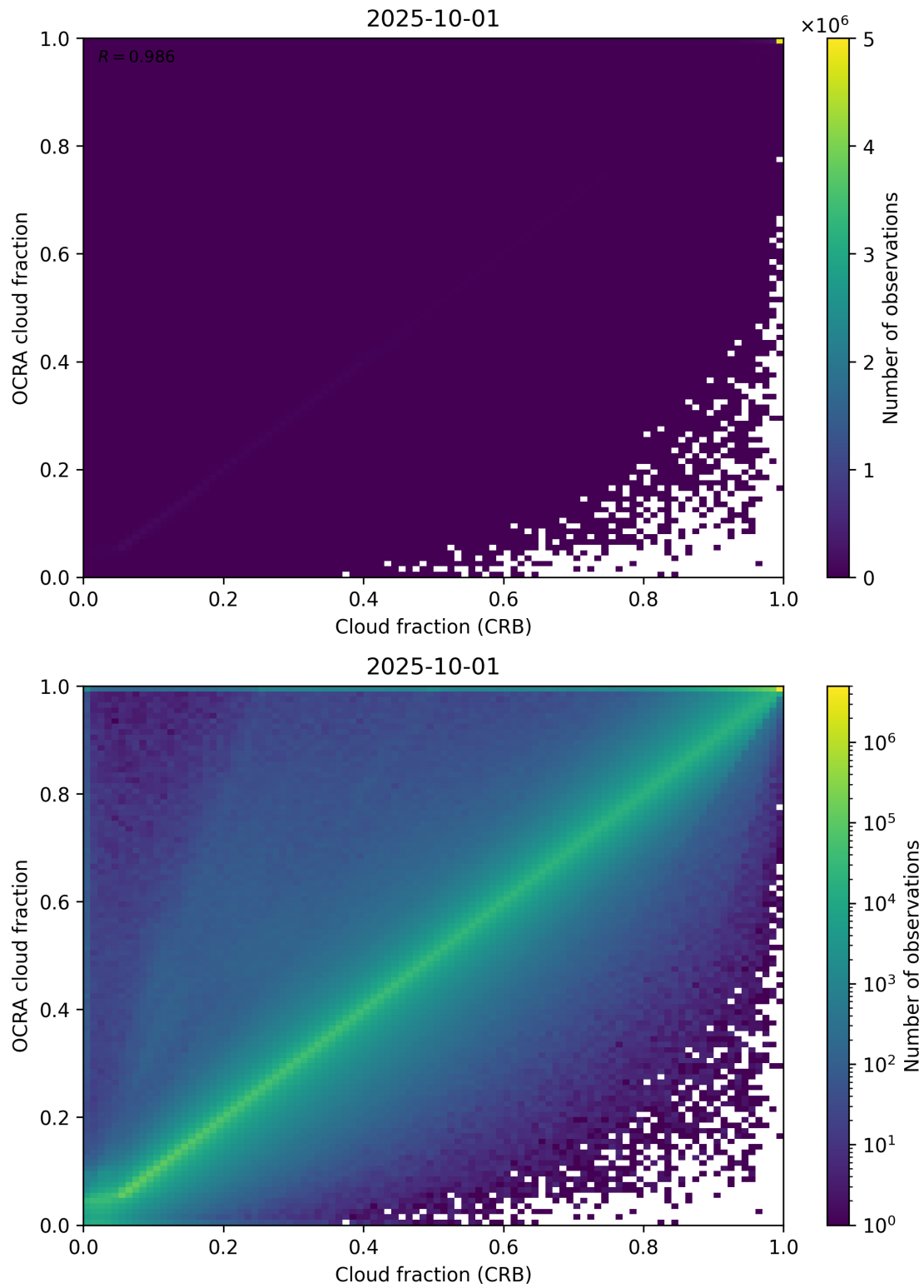
Figure 78: Scatter density plot of “Cloud fraction (CRB)” against “OCRA cloud fraction” for 2025-10-01 to 2025-10-02.
