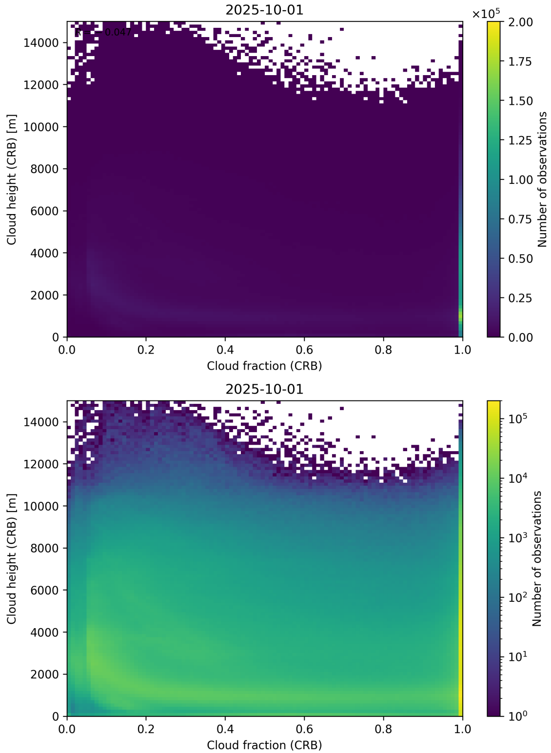
Figure 79: Scatter density plot of “Cloud fraction (CRB)” against “Cloud height (CRB)” for 2025-10-01 to 2025-10-02.
