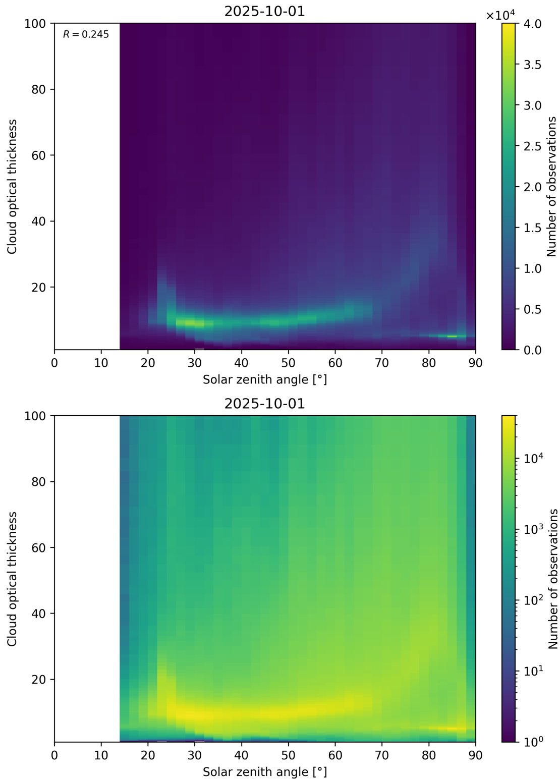
Figure 103: Scatter density plot of “Solar zenith angle” against “Cloud optical thickness” for 2025-10-01 to 2025-10-02.
