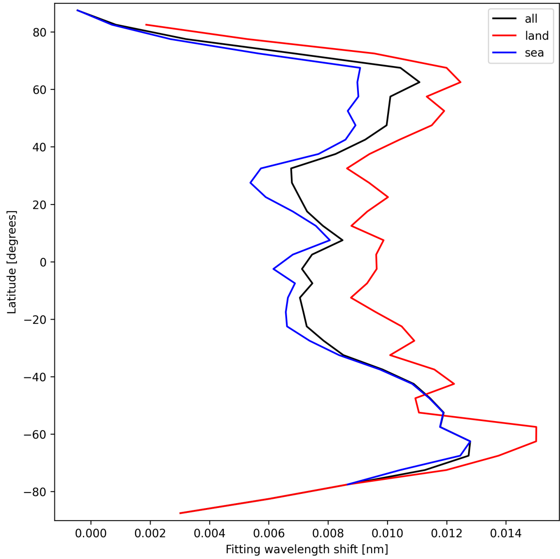
Figure 33: Zonal average of “Fitting wavelength shift” for 2025-10-01 to 2025-10-02.
