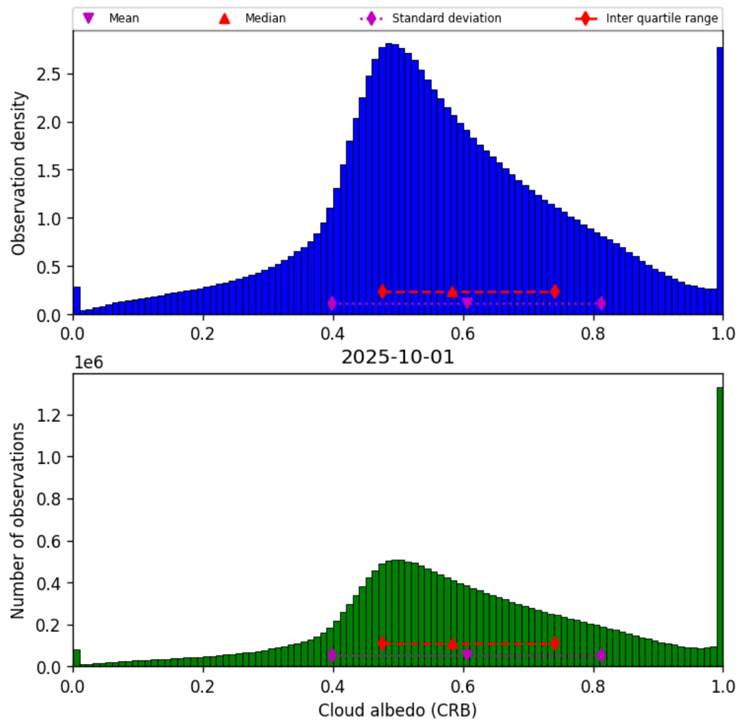
Figure 44: Histogram of “Cloud albedo (CRB)” for 2025-10-01 to 2025-10-02
