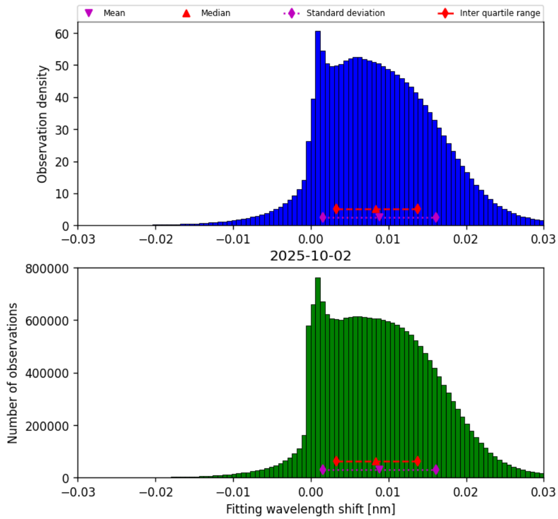
Figure 49: Histogram of “Fitting wavelength shift” for 2025-10-01 to 2025-10-03
