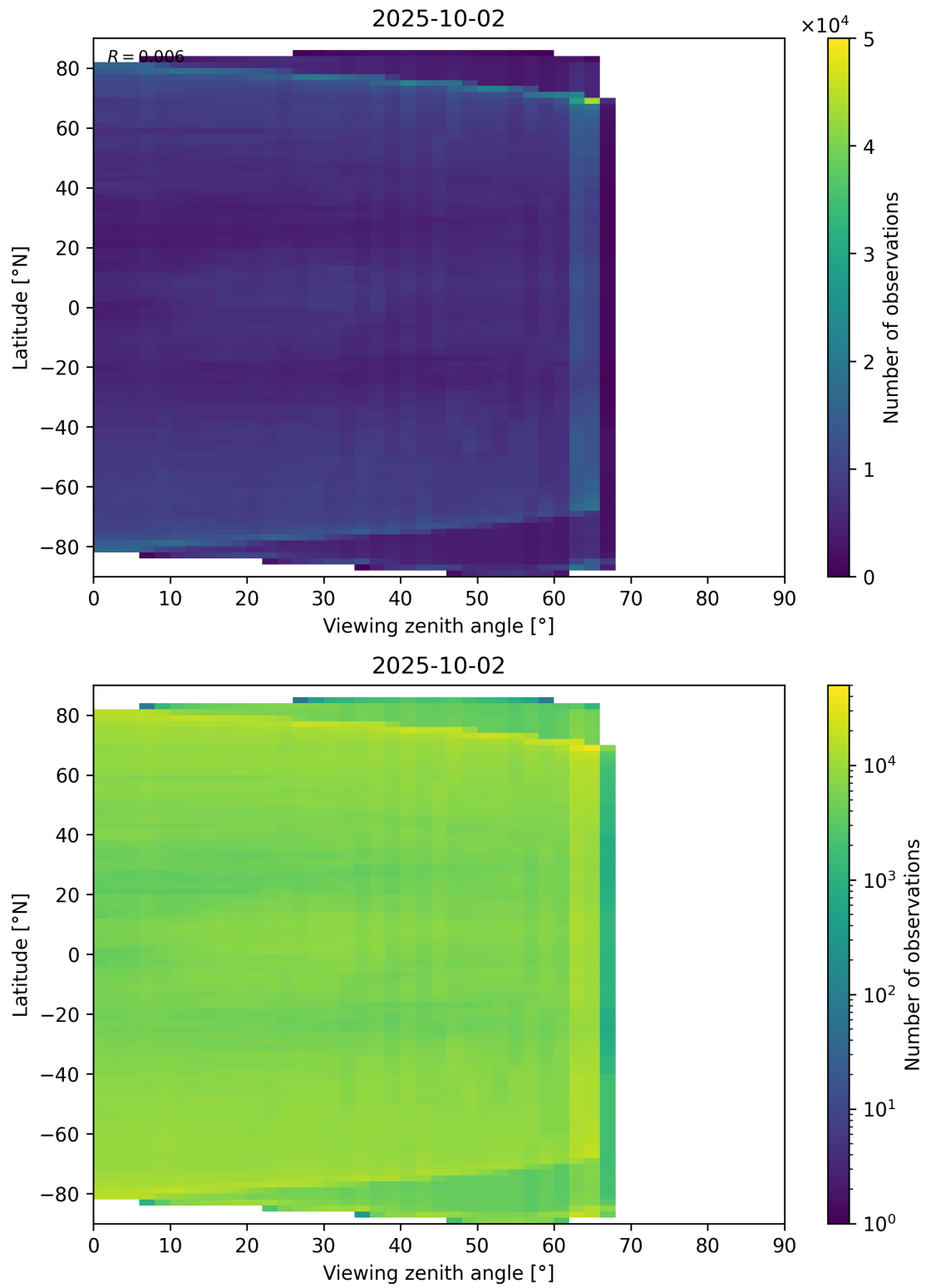
Figure 113: Scatter density plot of “Viewing zenith angle” against “Latitude” for 2025-10-01 to 2025-10-03.
