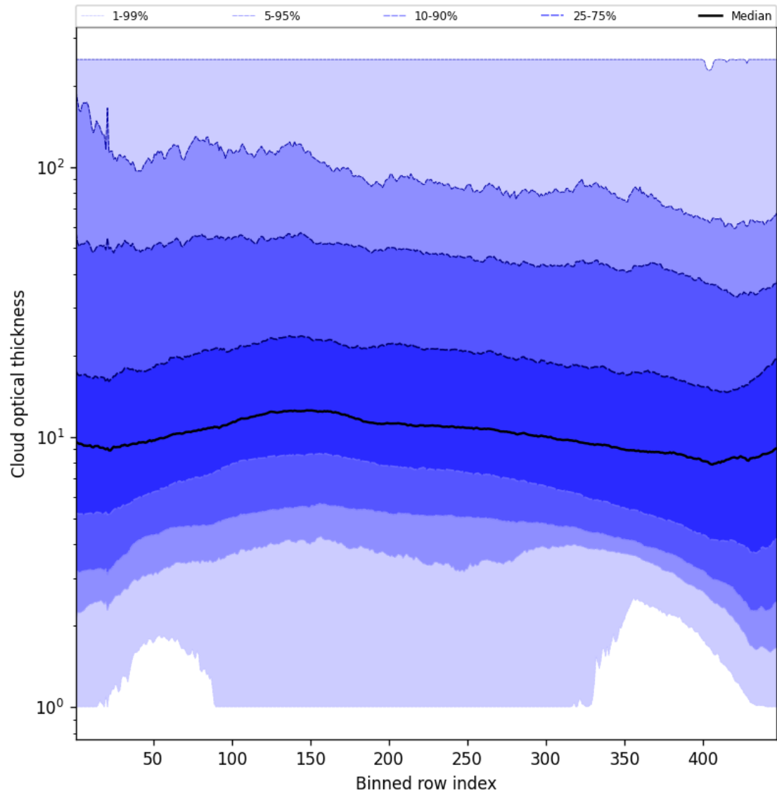
Figure 57: Along track statistics of “Cloud optical thickness” for 2025-10-01 to 2025-10-03
