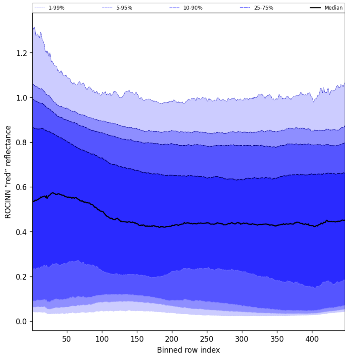
Figure 69: Along track statistics of “ROCINN “red” reflectance” for 2025-10-01 to 2025-10-03
