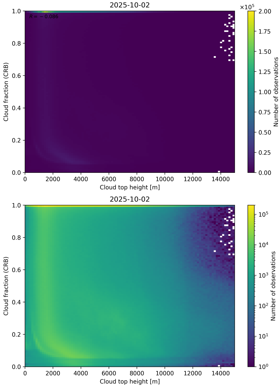
Figure 88: Scatter density plot of “Cloud top height” against “Cloud fraction (CRB)” for 2025-10-01 to 2025-10-03.
