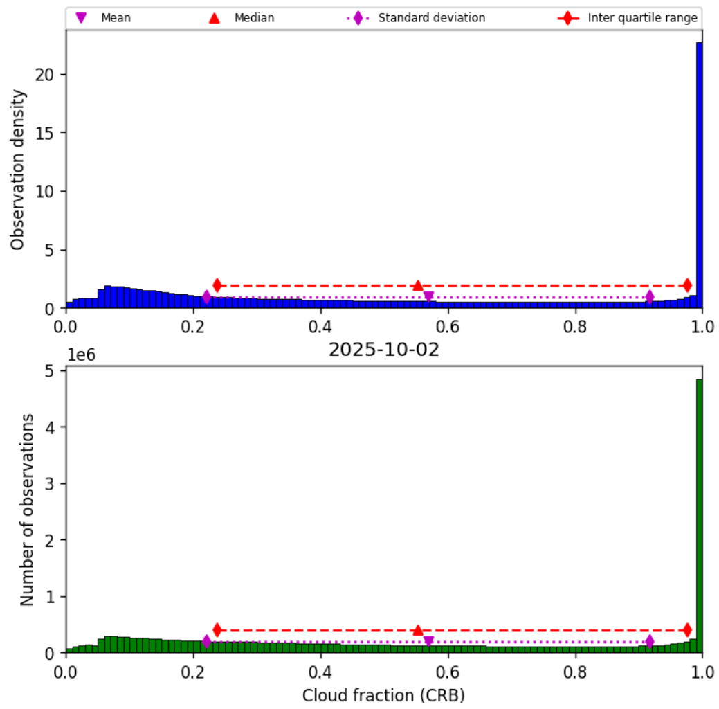
Figure 42: Histogram of “Cloud fraction (CRB)” for 2025-10-01 to 2025-10-03
