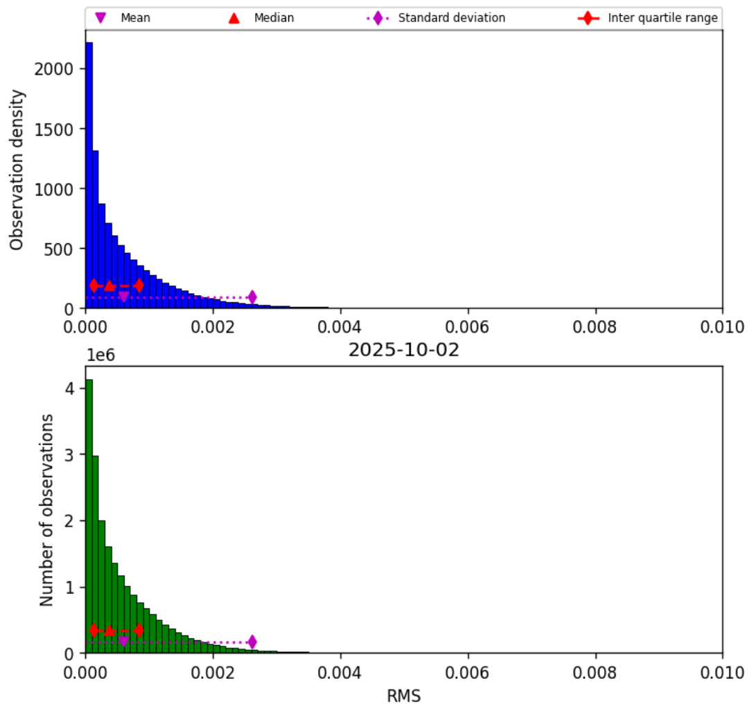
Figure 47: Histogram of “RMS” for 2025-10-01 to 2025-10-03
