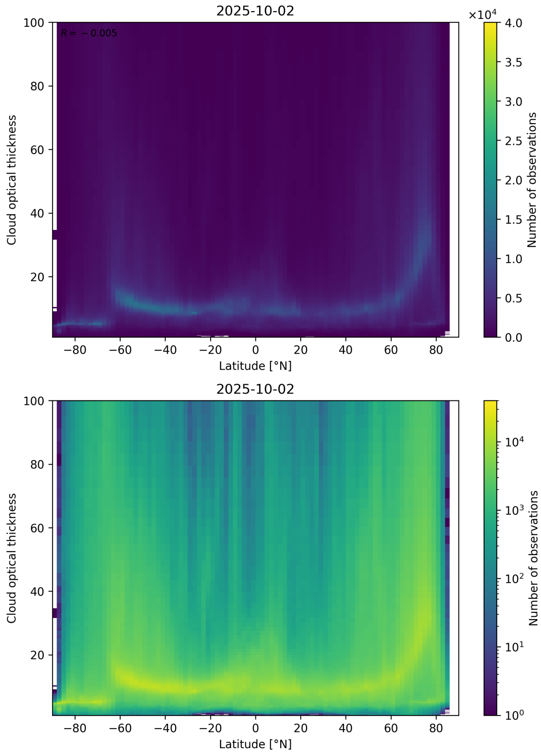
Figure 96: Scatter density plot of “Latitude” against “Cloud optical thickness” for 2025-10-01 to 2025-10-03.
