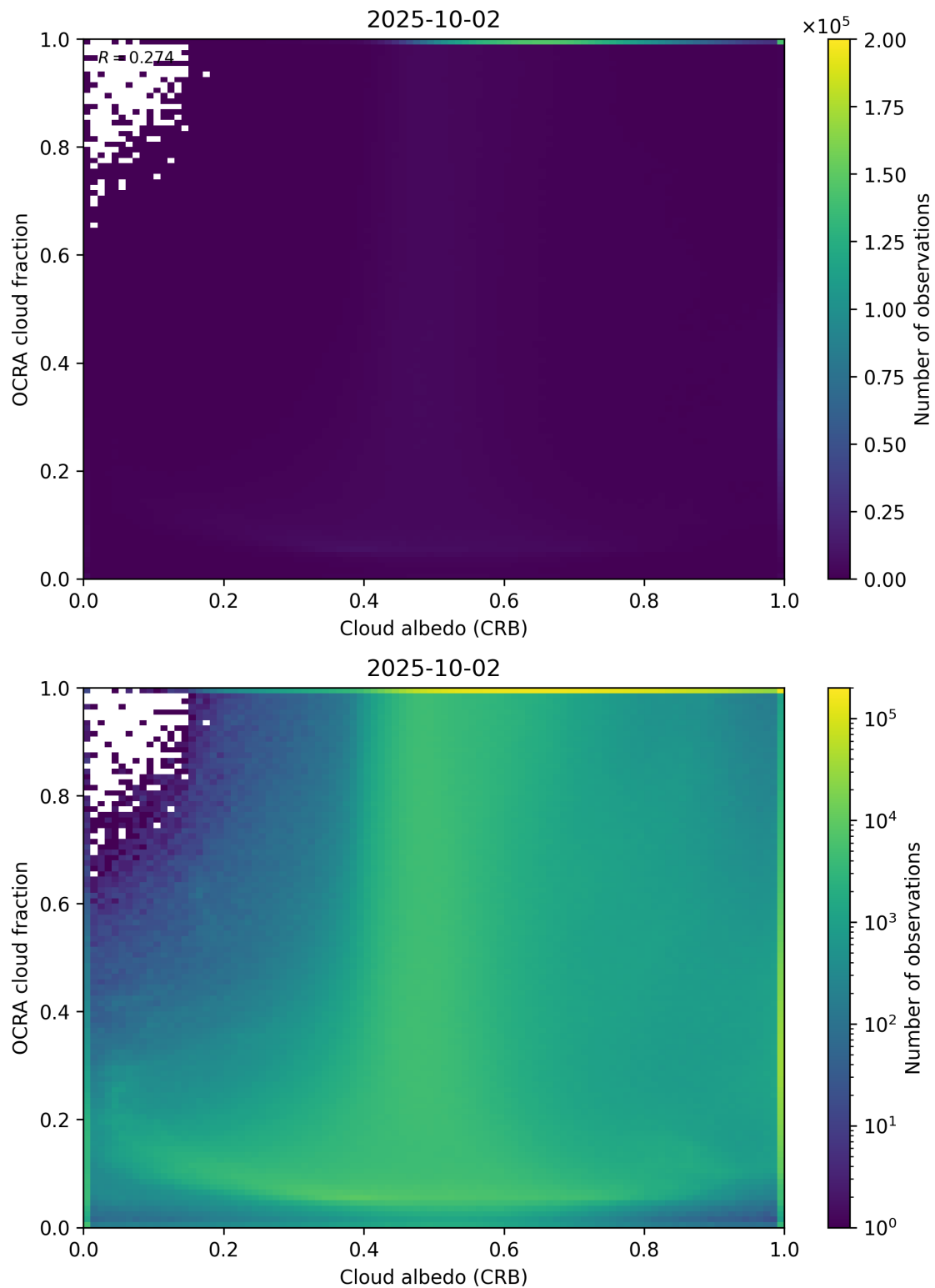
Figure 70: Scatter density plot of “Cloud albedo (CRB)” against “OCRA cloud fraction” for 2025-10-01 to 2025-10-03.
