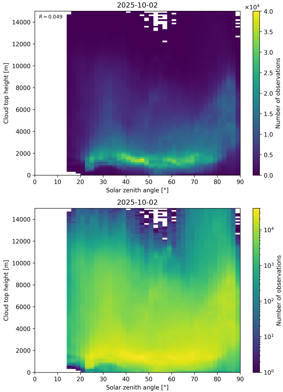
Figure 104: Scatter density plot of “Solar zenith angle” against “Cloud top height” for 2025-10-01 to 2025-10-03.
