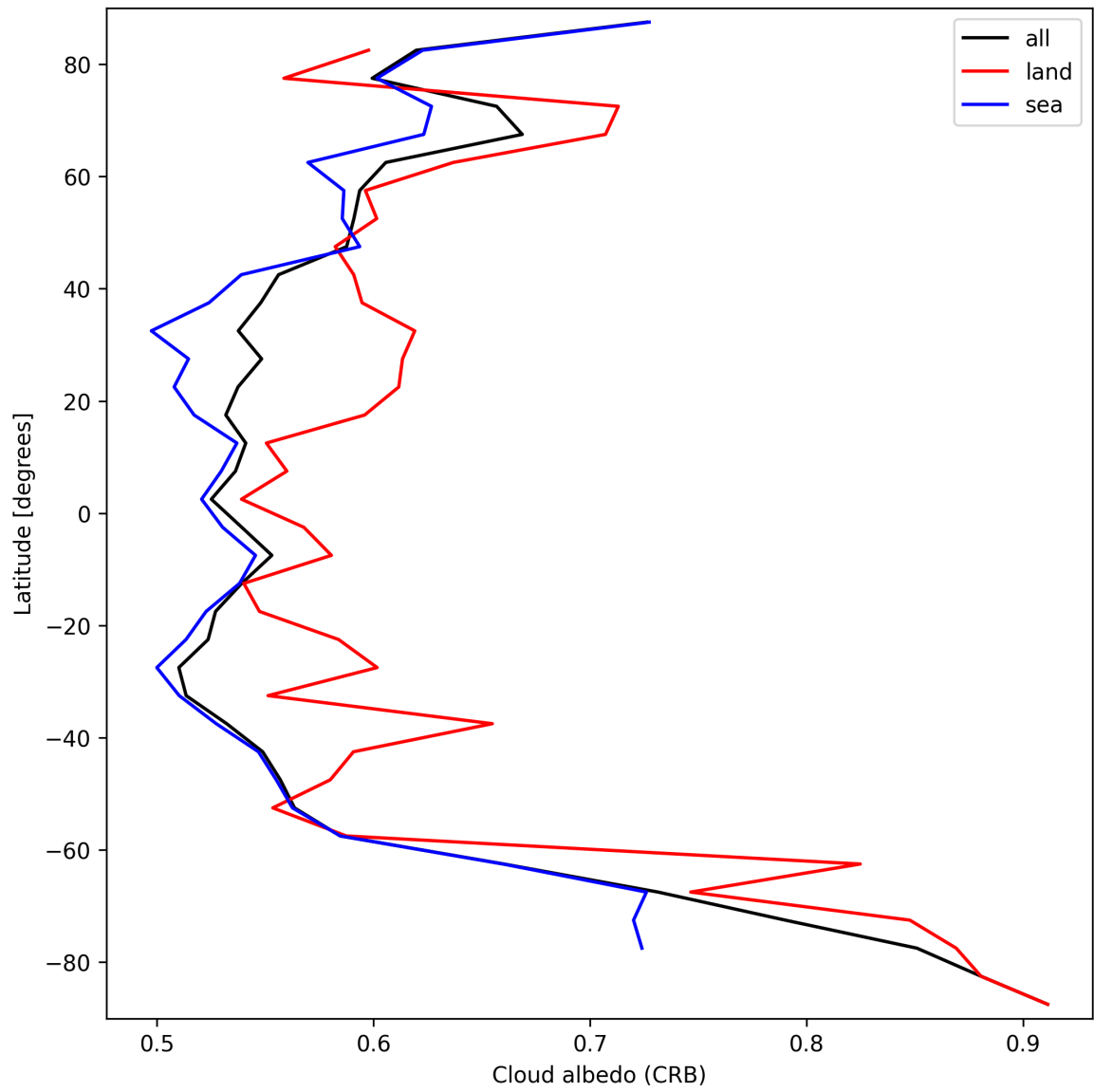
Figure 28: Zonal average of “Cloud albedo (CRB)” for 2025-10-01 to 2025-10-03.
