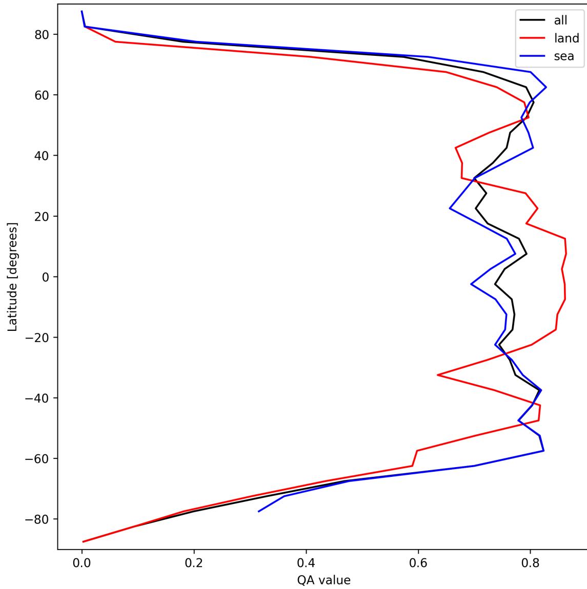
Figure 22: Zonal average of “QA value” for 2025-10-01 to 2025-10-03.
