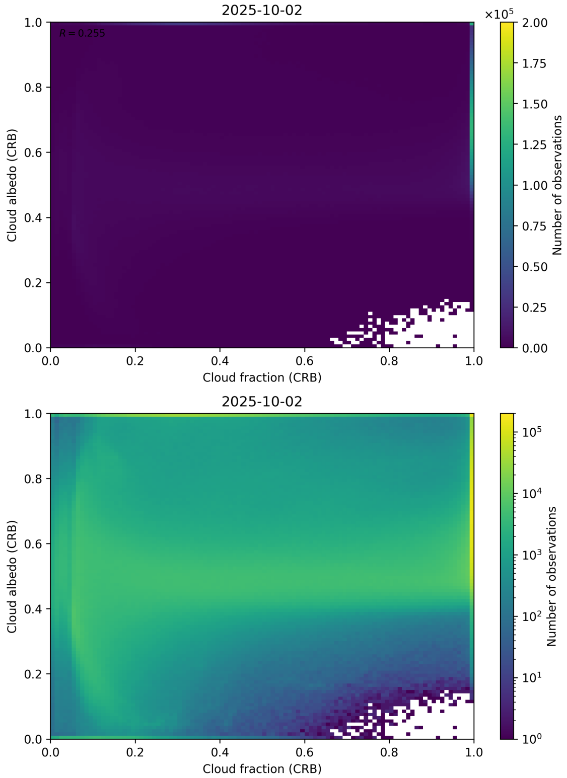
Figure 77: Scatter density plot of “Cloud fraction (CRB)” against “Cloud albedo (CRB)” for 2025-10-01 to 2025-10-03.
