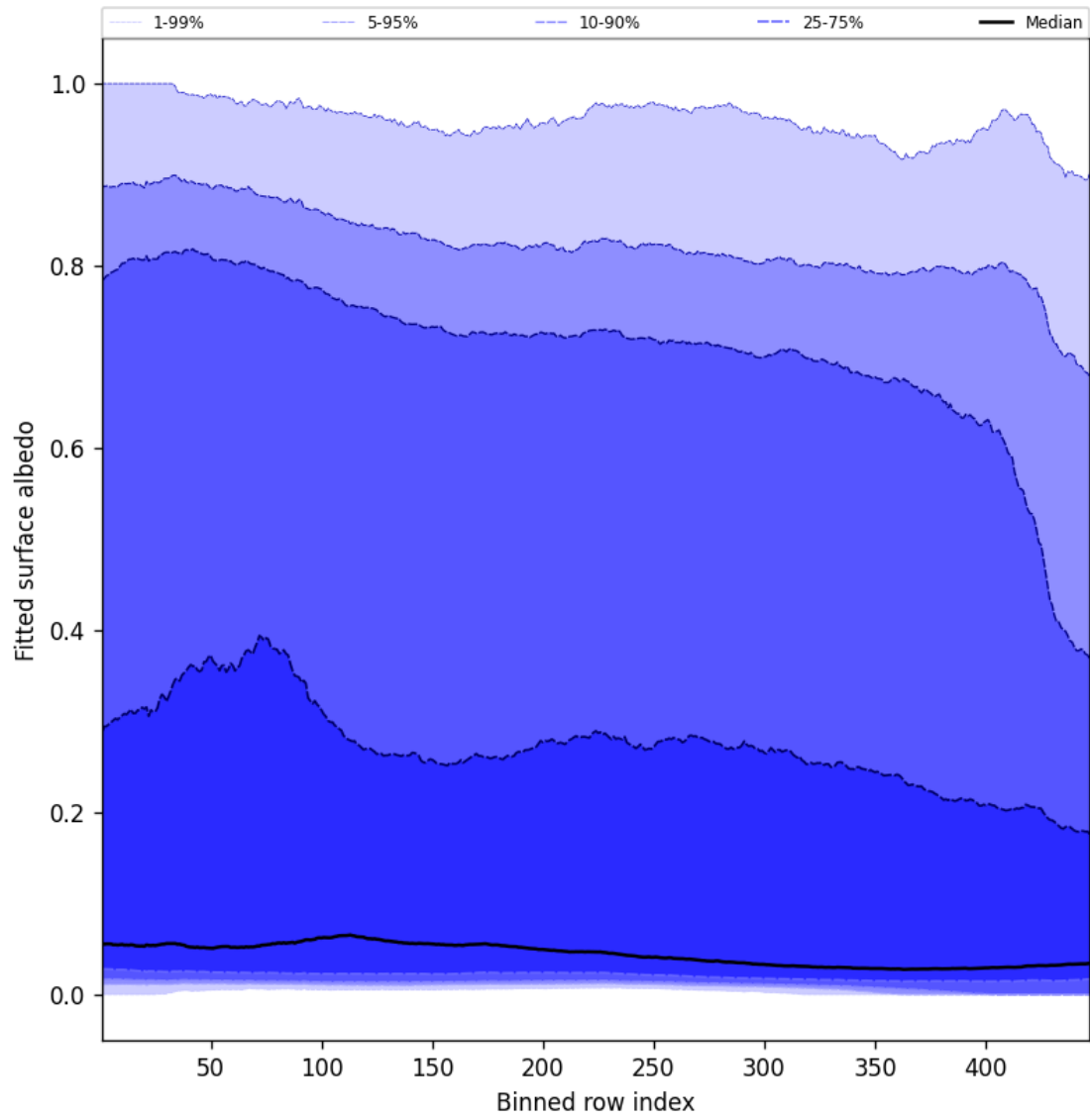
Figure 61: Along track statistics of “Fitted surface albedo” for 2025-10-01 to 2025-10-03
