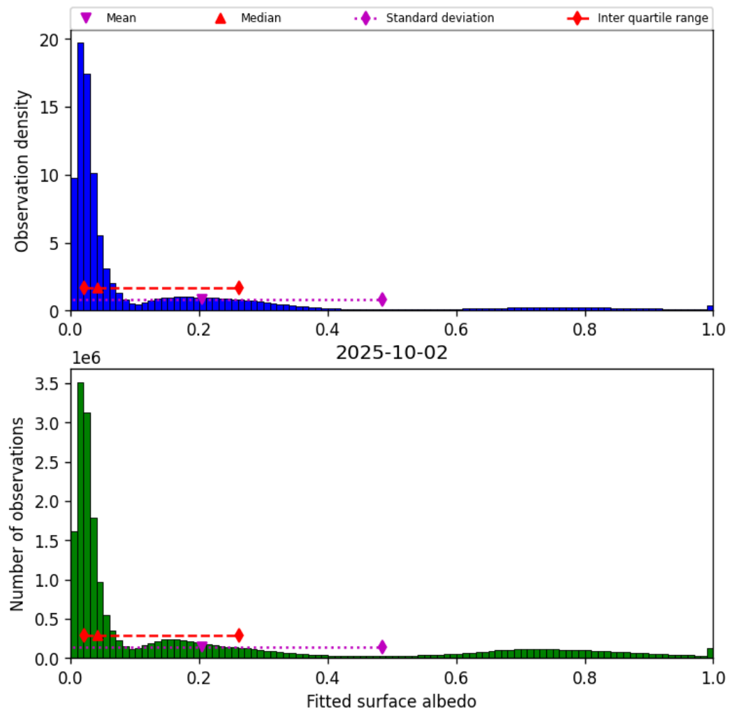
Figure 45: Histogram of “Fitted surface albedo” for 2025-10-01 to 2025-10-03
