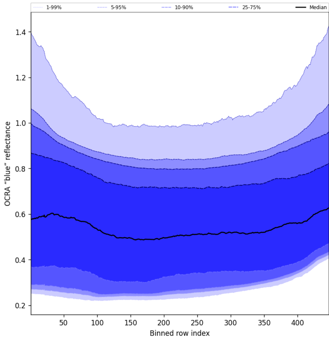
Figure 67: Along track statistics of “OCRA “blue” reflectance” for 2025-10-01 to 2025-10-03
