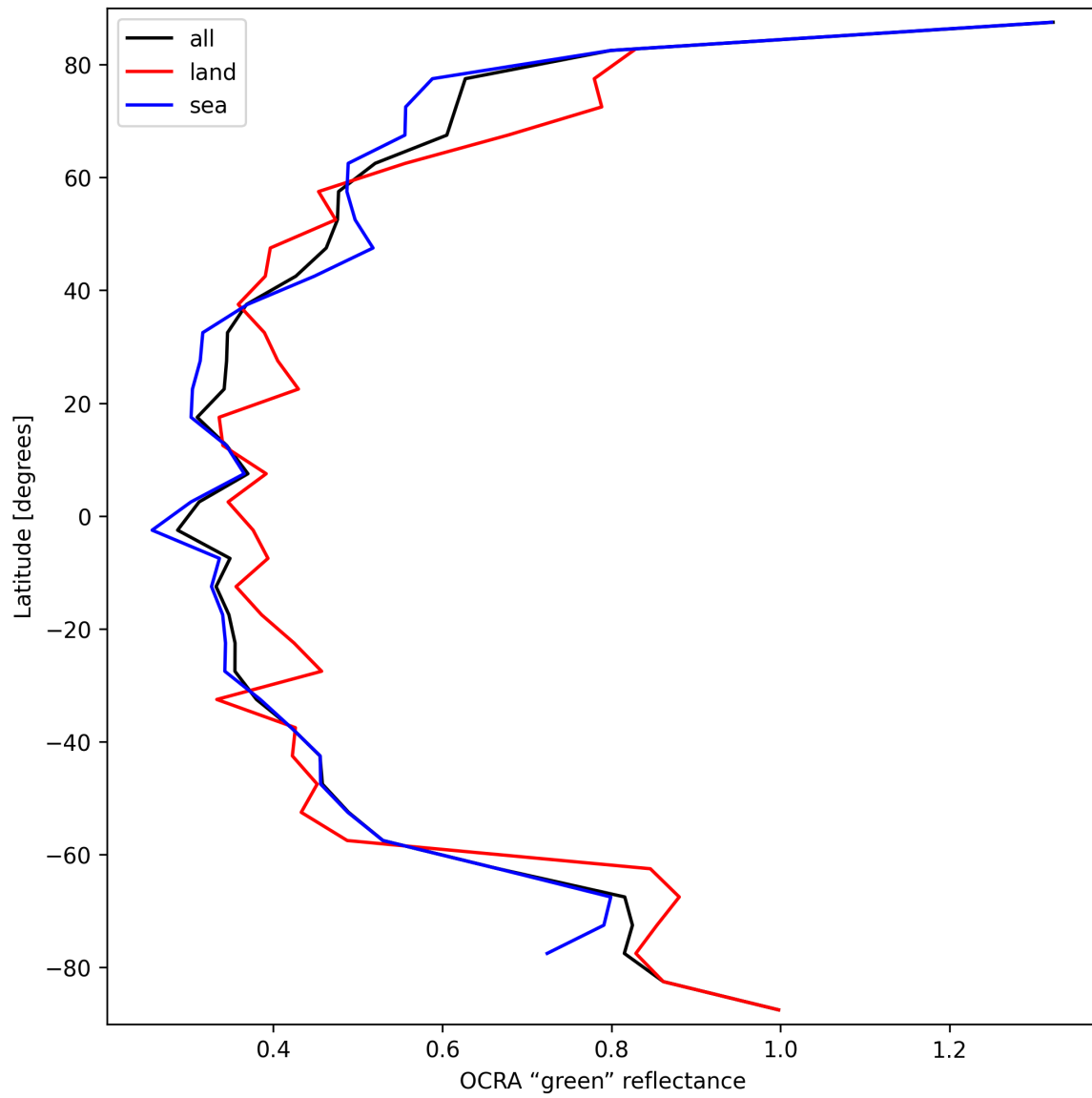
Figure 36: Zonal average of “OCRA “green” reflectance” for 2025-10-01 to 2025-10-03.
