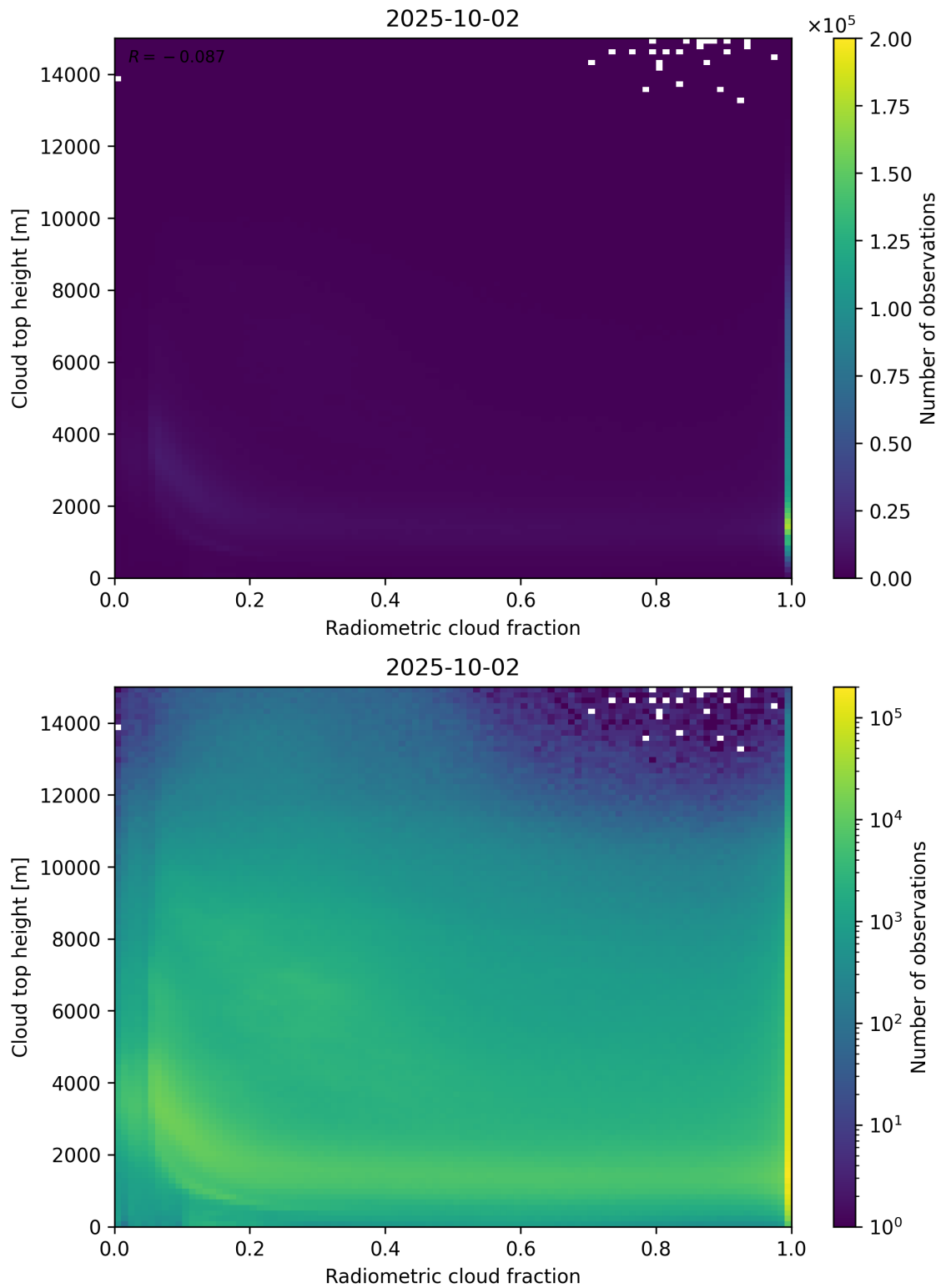
Figure 76: Scatter density plot of “Radiometric cloud fraction” against “Cloud top height” for 2025-10-01 to 2025-10-03.
