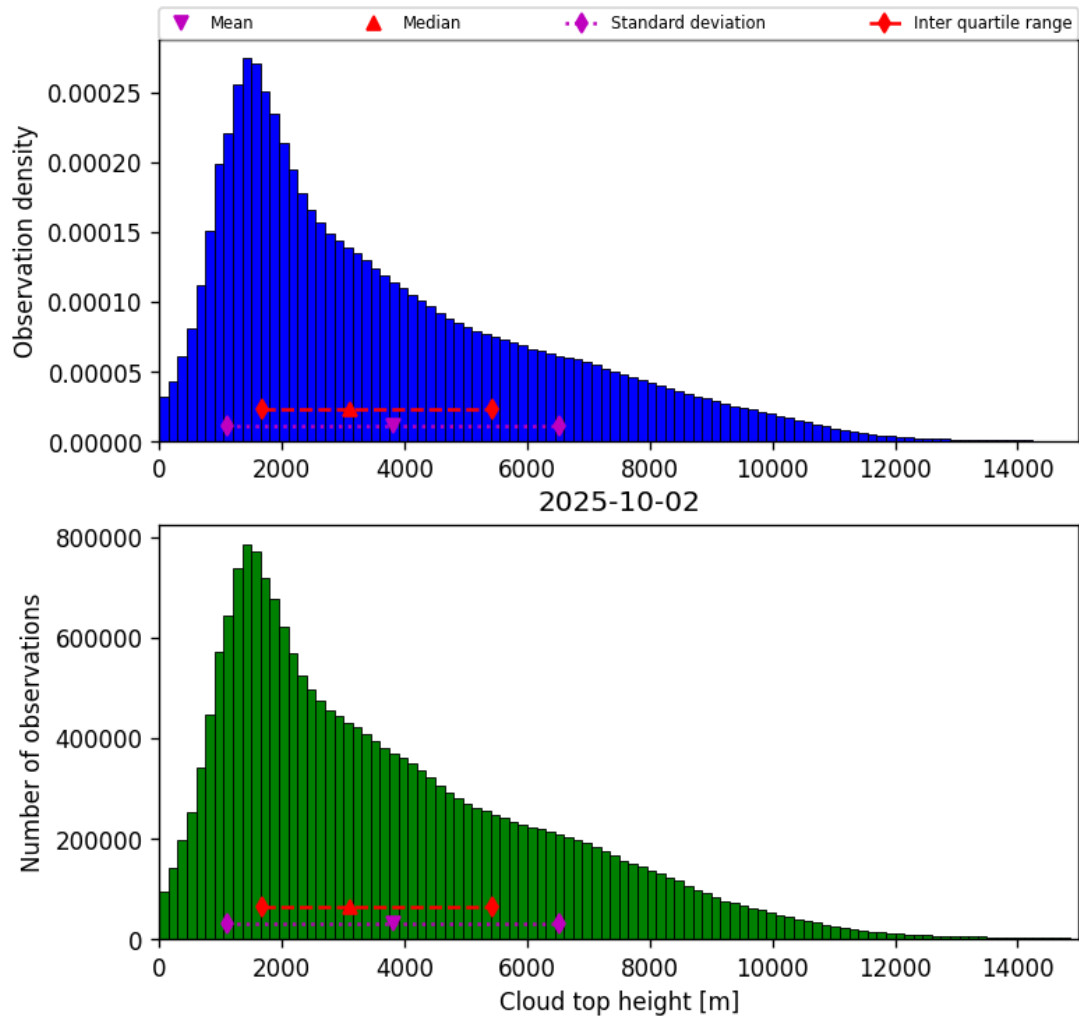
Figure 40: Histogram of “Cloud top height” for 2025-10-01 to 2025-10-03
