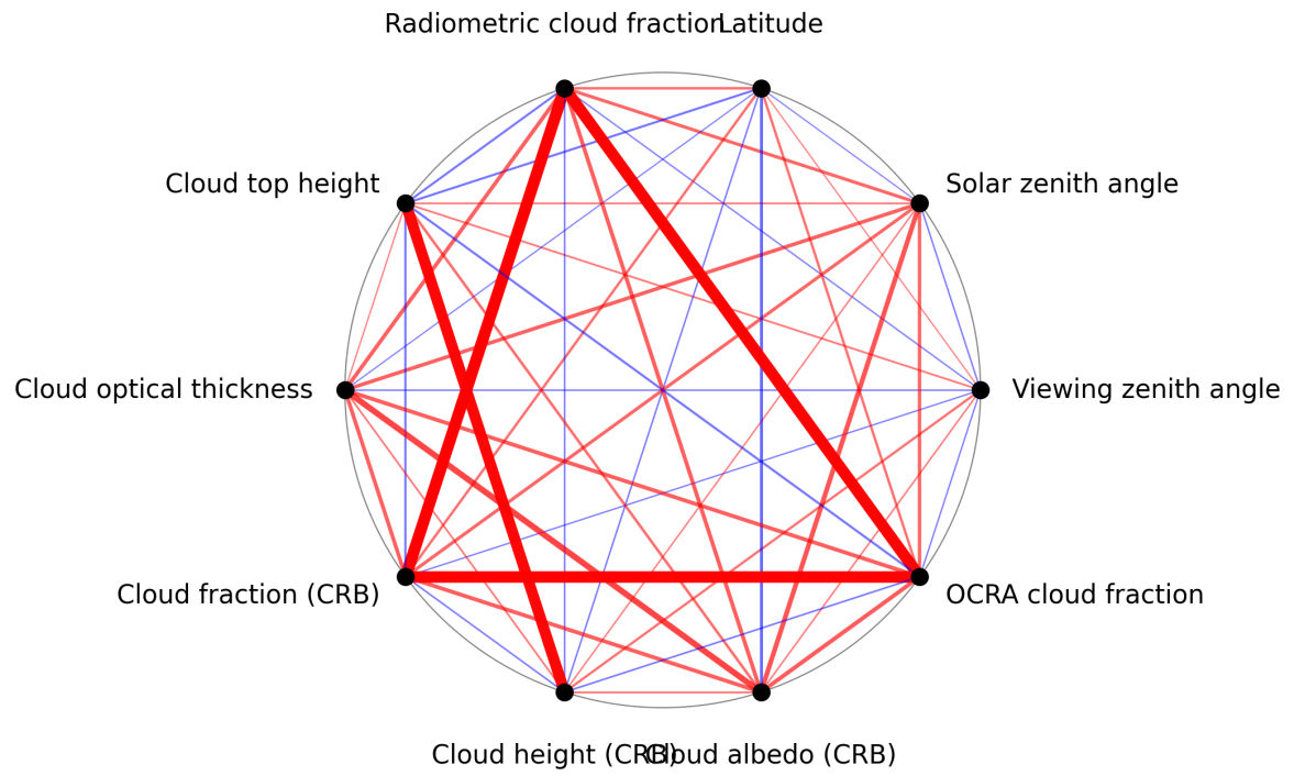
Figure 1: Map of correlation graph for 2025-10-01 to 2025-10-03.
