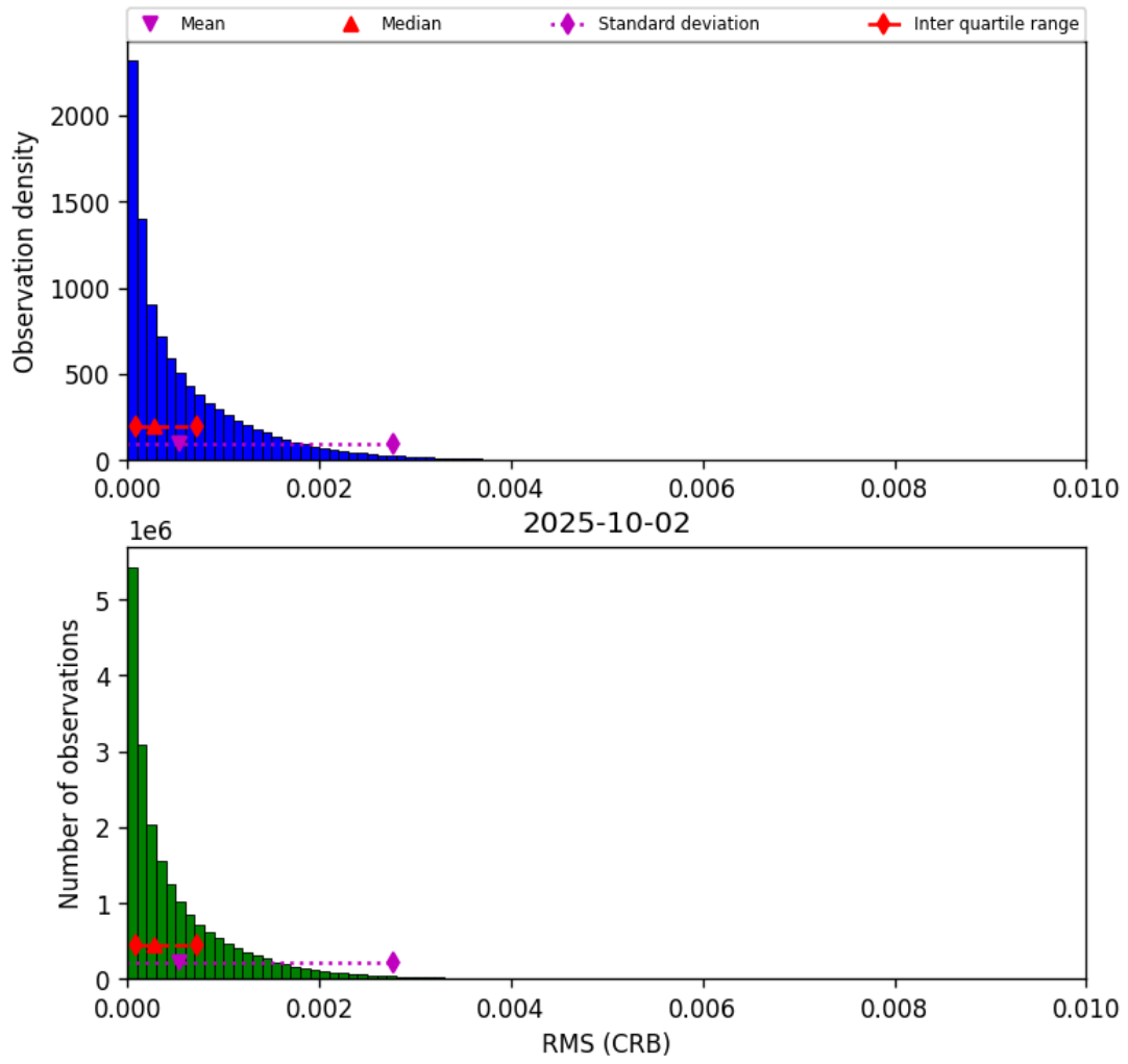
Figure 48: Histogram of “RMS (CRB)” for 2025-10-01 to 2025-10-03
