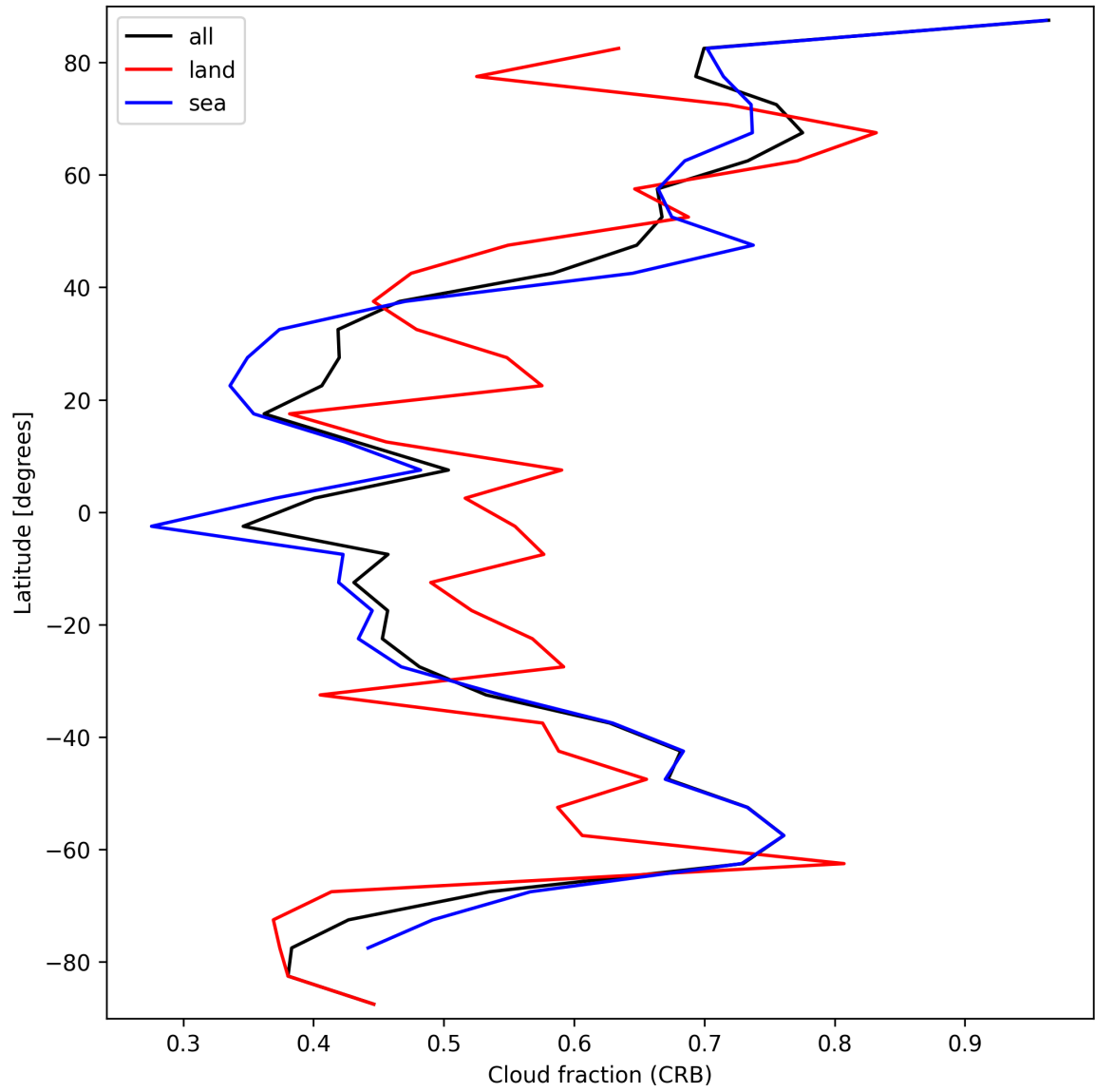
Figure 26: Zonal average of “Cloud fraction (CRB)” for 2025-10-01 to 2025-10-03.
