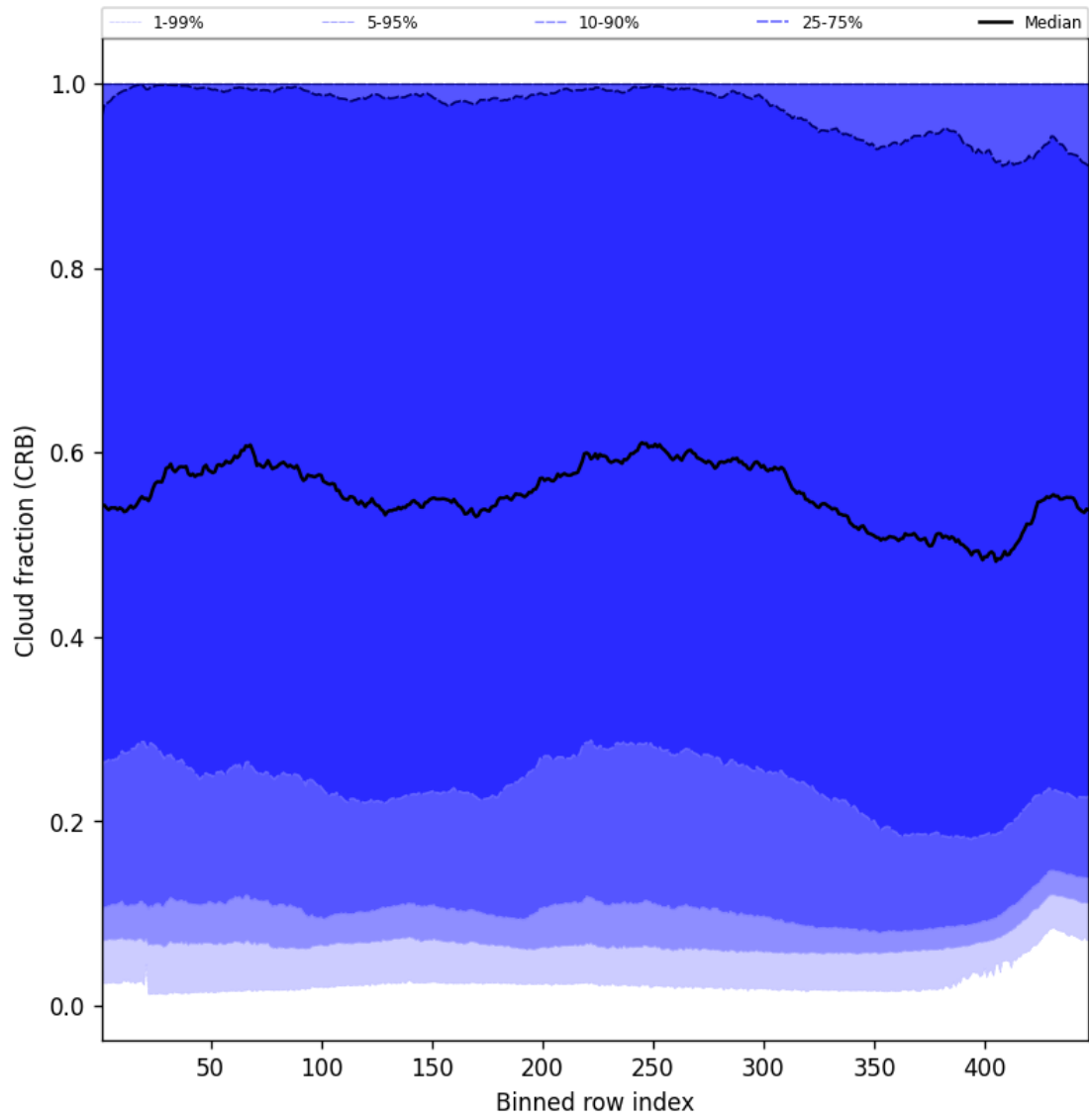
Figure 58: Along track statistics of “Cloud fraction (CRB)” for 2025-10-01 to 2025-10-03
