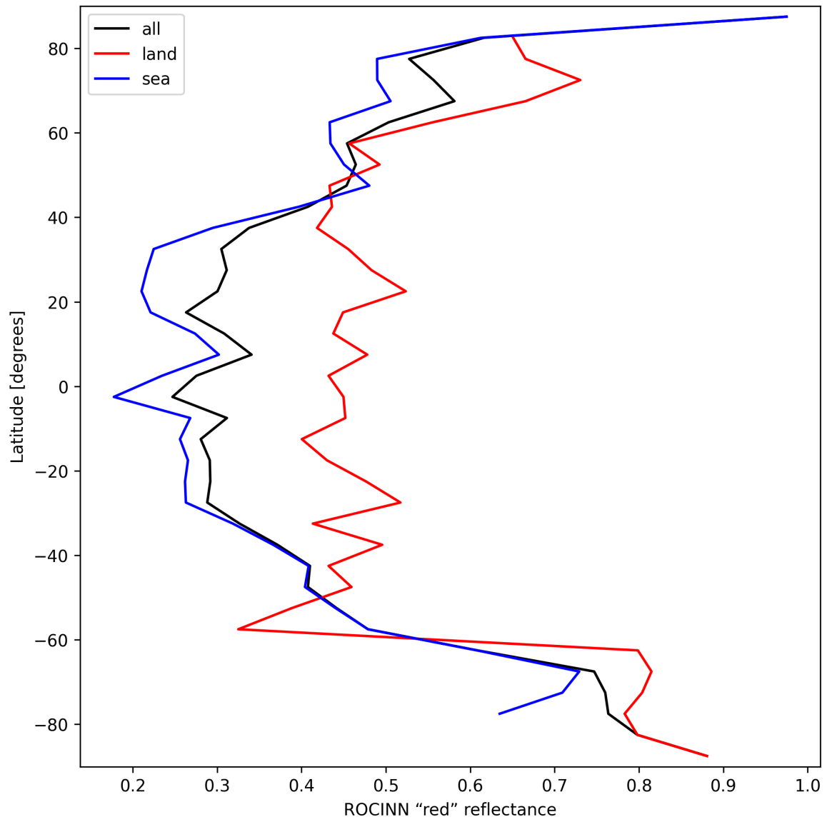
Figure 37: Zonal average of “ROCINN “red” reflectance” for 2025-10-01 to 2025-10-03.
