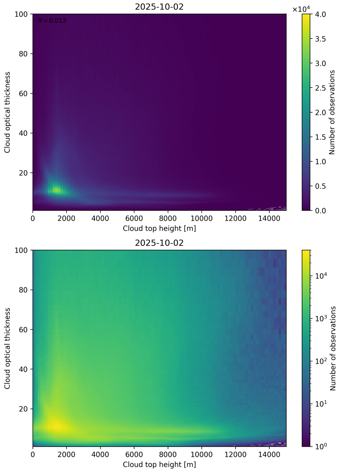
Figure 90: Scatter density plot of “Cloud top height” against “Cloud optical thickness” for 2025-10-01 to 2025-10-03.
