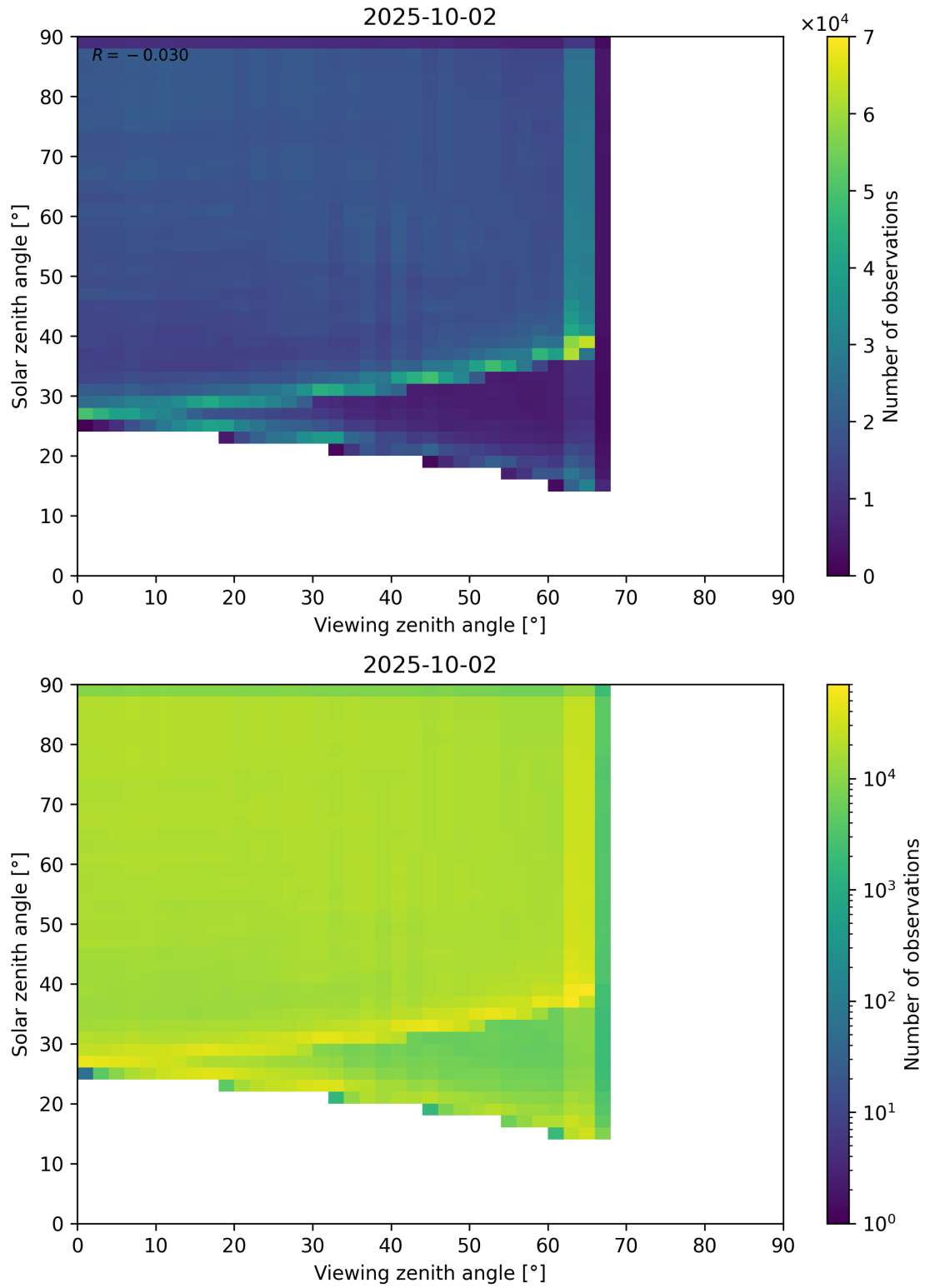
Figure 114: Scatter density plot of “Viewing zenith angle” against “Solar zenith angle” for 2025-10-01 to 2025-10-03.
