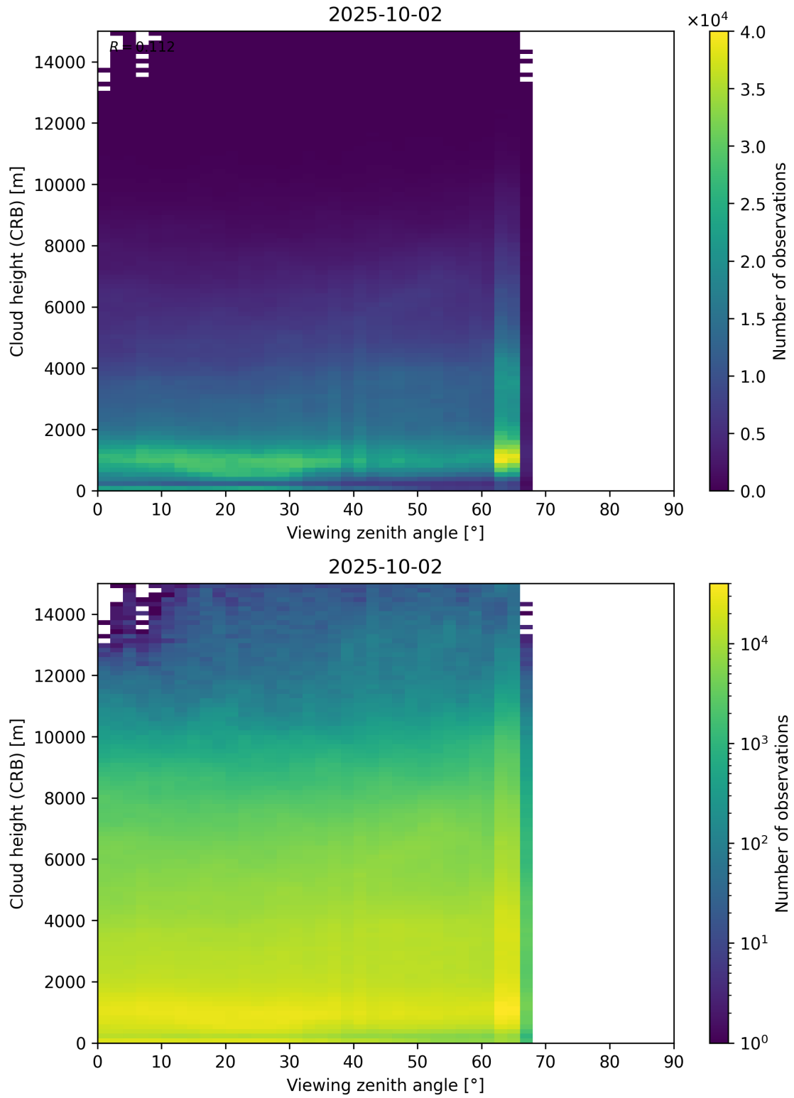
Figure 110: Scatter density plot of “Viewing zenith angle” against “Cloud height (CRB)” for 2025-10-01 to 2025-10-03.
