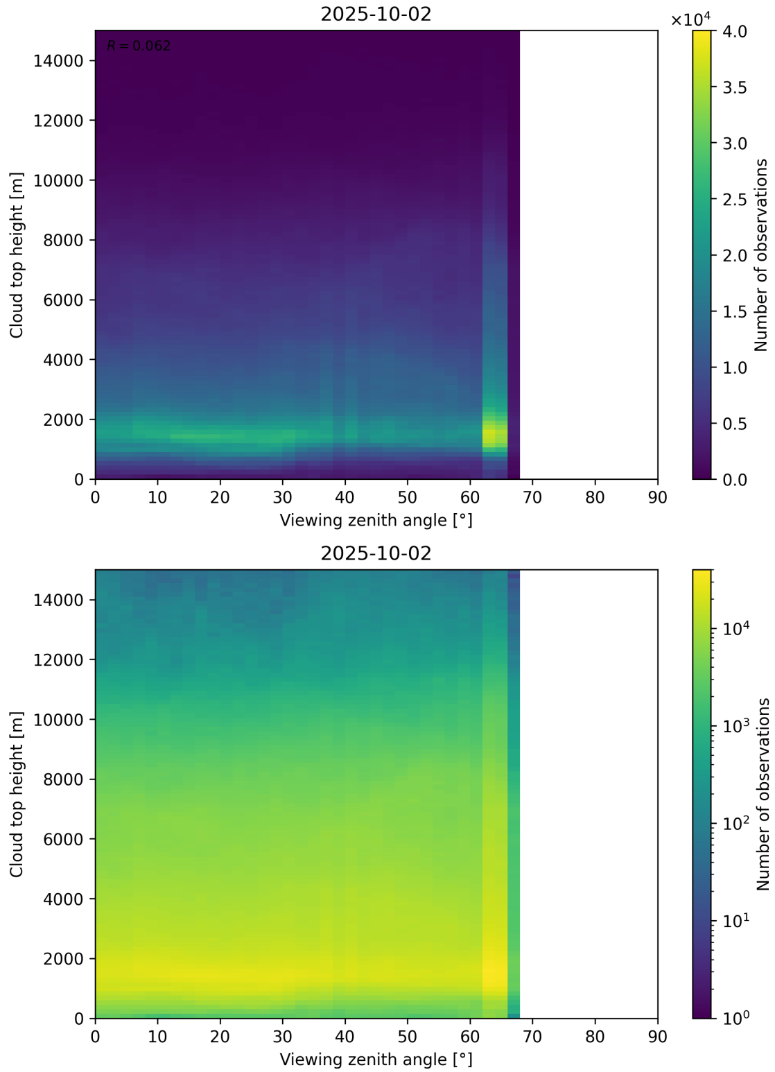
Figure 112: Scatter density plot of “Viewing zenith angle” against “Cloud top height” for 2025-10-01 to 2025-10-03.
