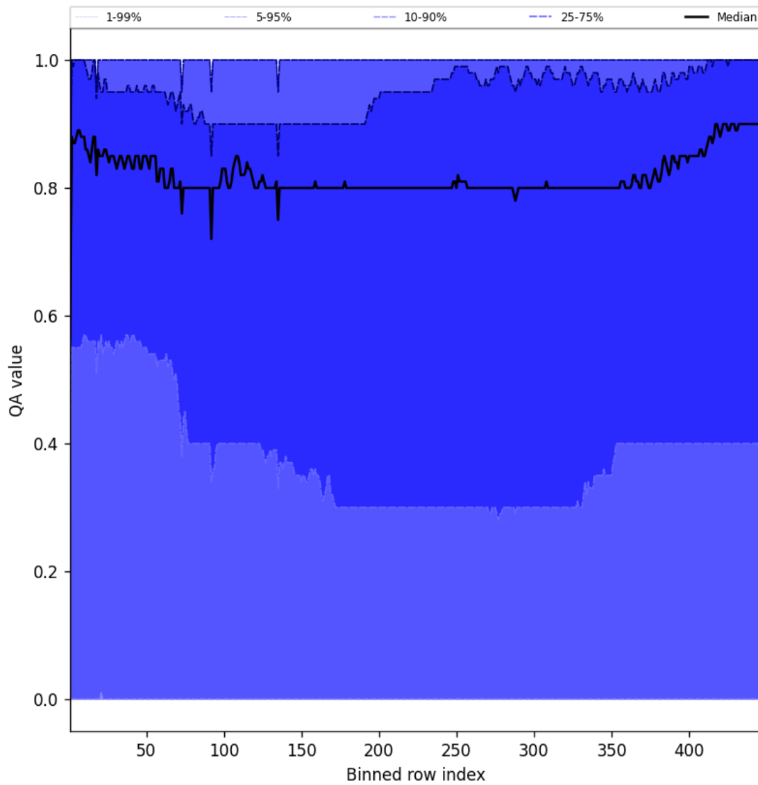
Figure 54: Along track statistics of “QA value” for 2025-10-01 to 2025-10-03
