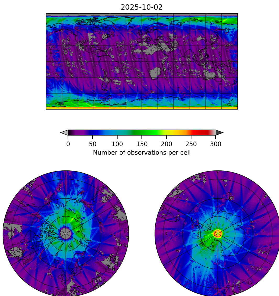
Figure 21: Map of the number of observations for 2025-10-01 to 2025-10-03
