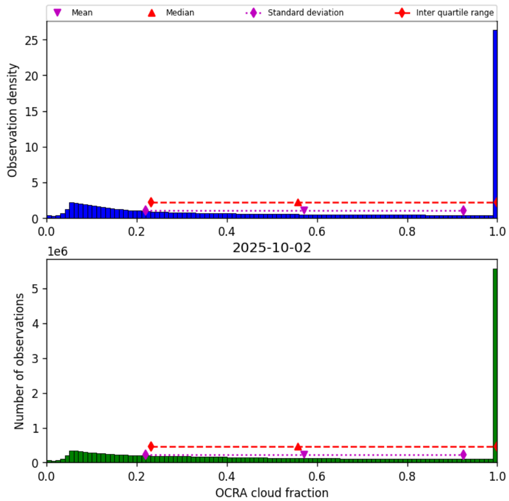
Figure 50: Histogram of “OCRA cloud fraction” for 2025-10-01 to 2025-10-03
