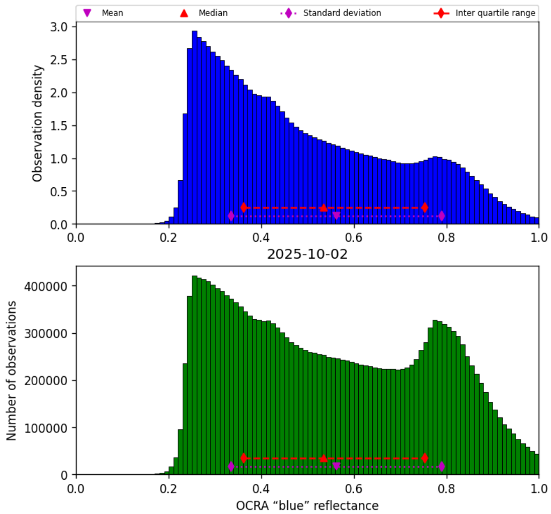
Figure 51: Histogram of “OCRA “blue” reflectance” for 2025-10-01 to 2025-10-03
