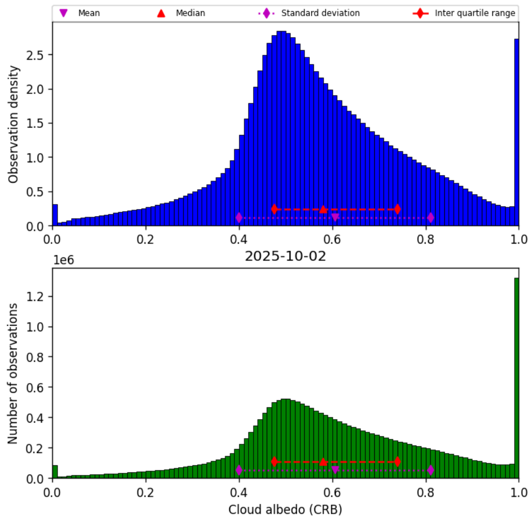
Figure 44: Histogram of “Cloud albedo (CRB)” for 2025-10-01 to 2025-10-03
