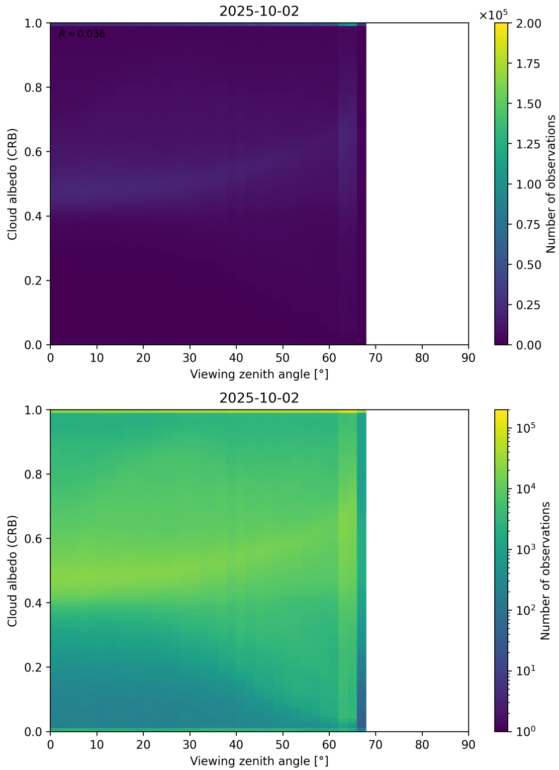
Figure 106: Scatter density plot of “Viewing zenith angle” against “Cloud albedo (CRB)” for 2025-10-01 to 2025-10-03.
