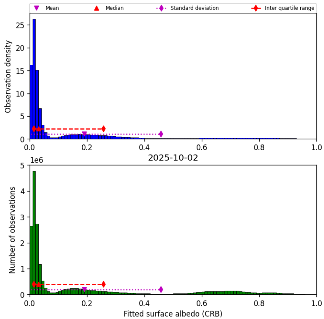
Figure 46: Histogram of “Fitted surface albedo (CRB)” for 2025-10-01 to 2025-10-03
