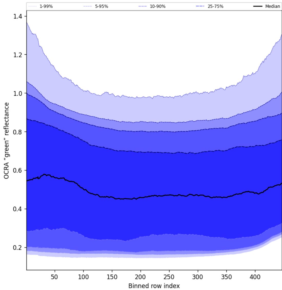
Figure 68: Along track statistics of “OCRA “green” reflectance” for 2025-10-01 to 2025-10-03
