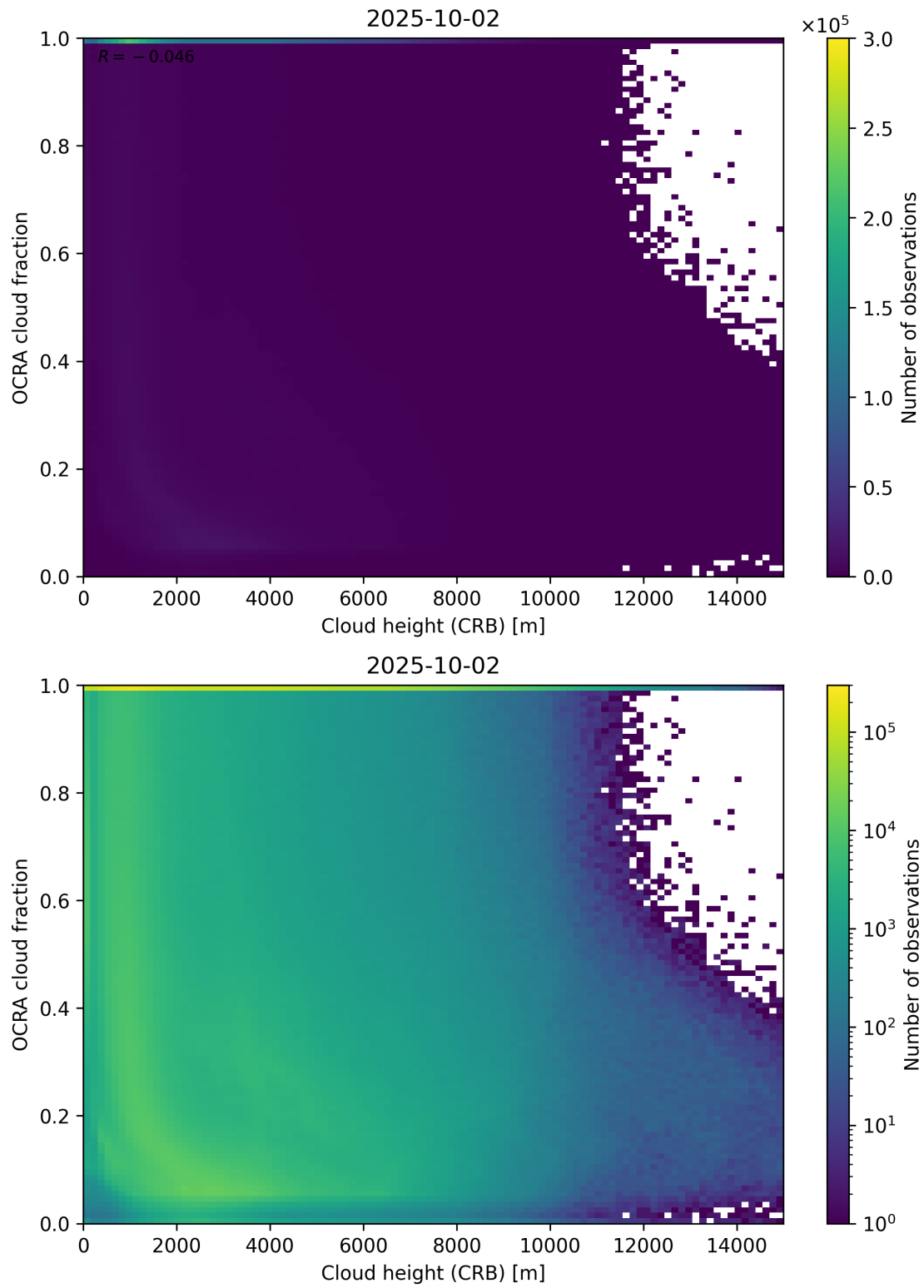
Figure 81: Scatter density plot of “Cloud height (CRB)” against “OCRA cloud fraction” for 2025-10-01 to 2025-10-03.
