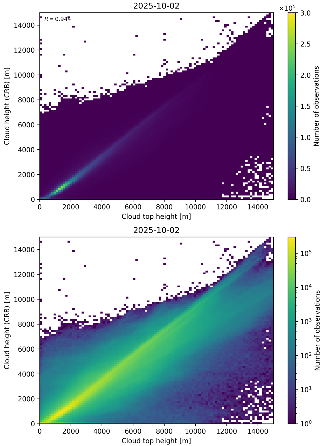
Figure 89: Scatter density plot of “Cloud top height” against “Cloud height (CRB)” for 2025-10-01 to 2025-10-03.
