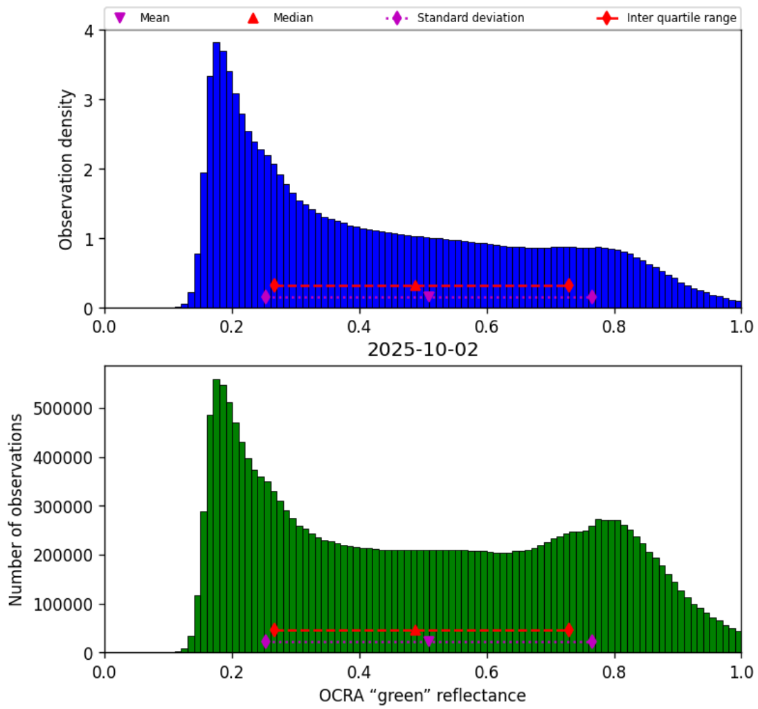
Figure 52: Histogram of “OCRA “green” reflectance” for 2025-10-01 to 2025-10-03
