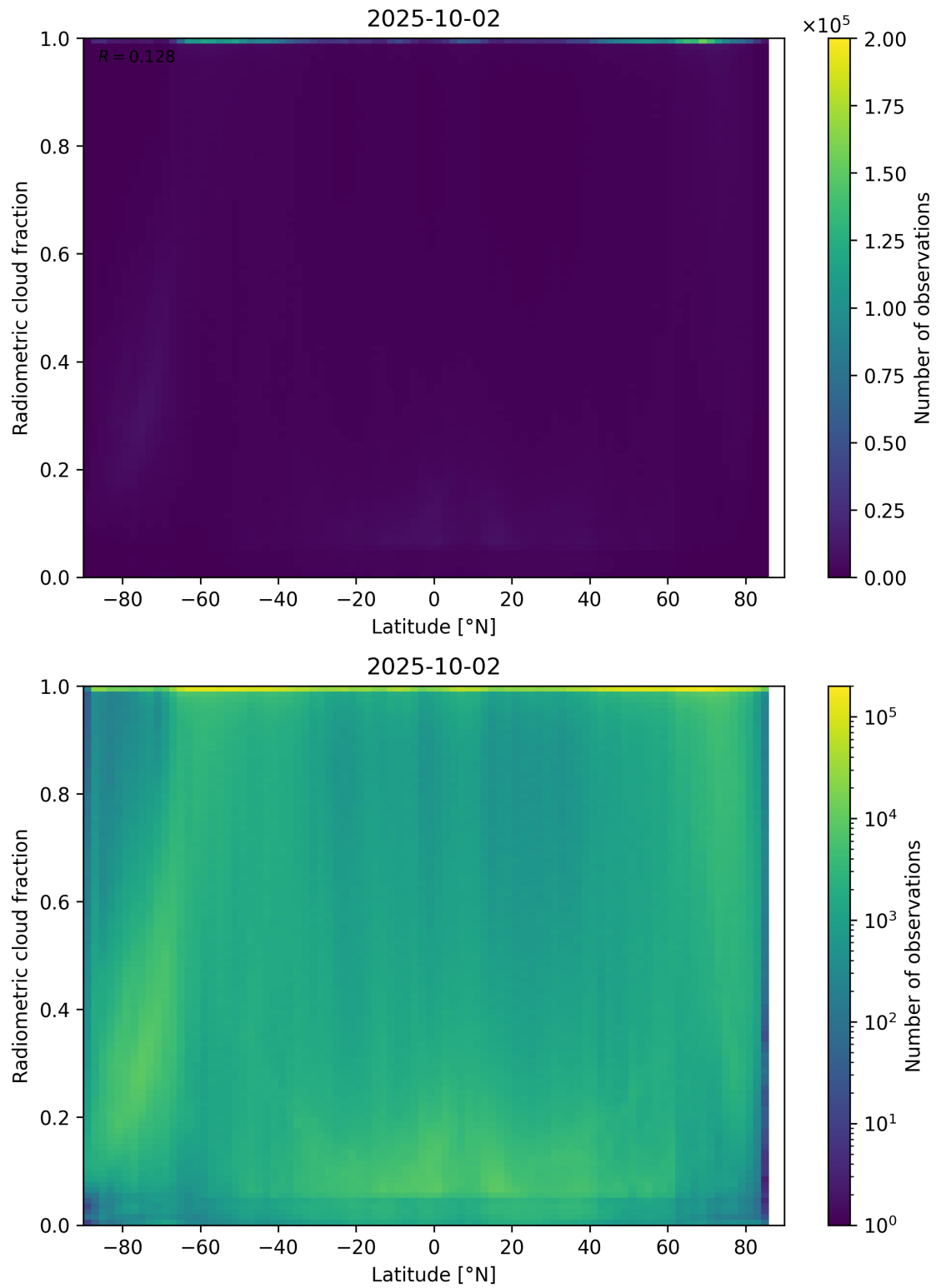
Figure 92: Scatter density plot of “Latitude” against “Radiometric cloud fraction” for 2025-10-01 to 2025-10-03.
