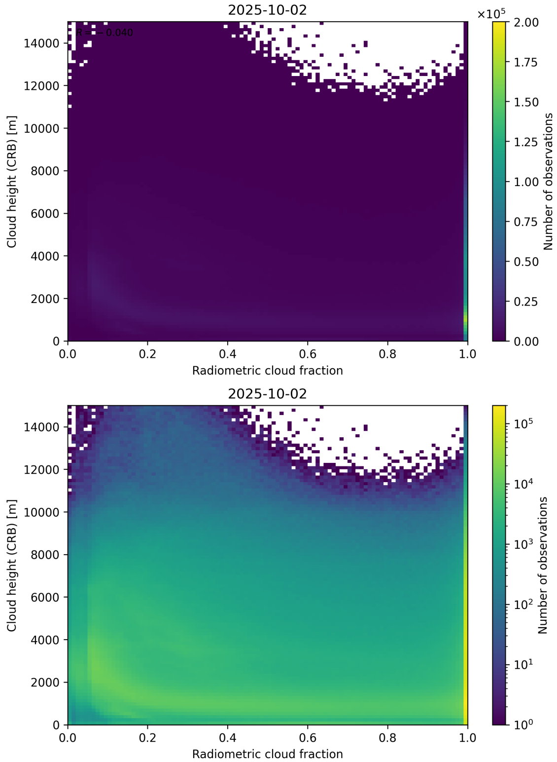
Figure 74: Scatter density plot of “Radiometric cloud fraction” against “Cloud height (CRB)” for 2025-10-01 to 2025-10-03.
