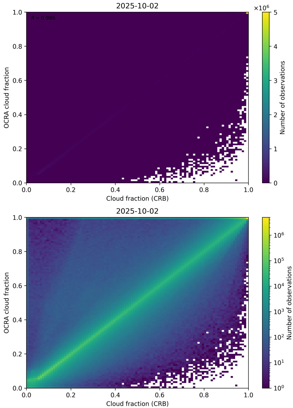
Figure 78: Scatter density plot of “Cloud fraction (CRB)” against “OCRA cloud fraction” for 2025-10-01 to 2025-10-03.
