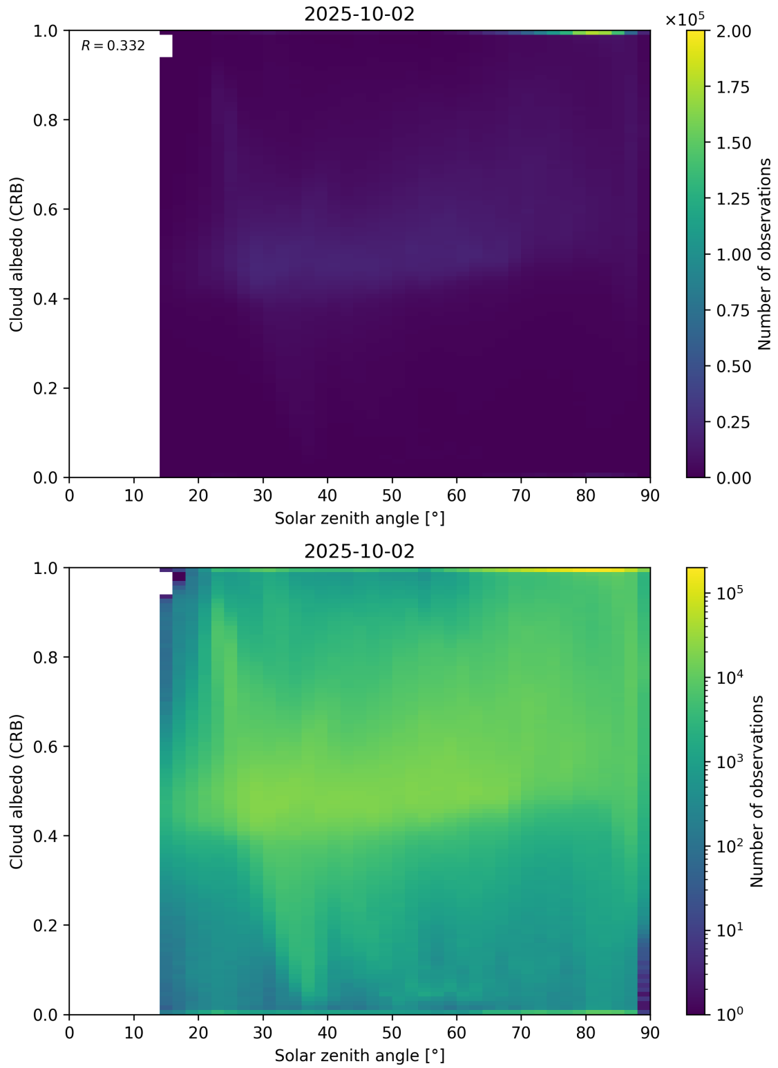
Figure 98: Scatter density plot of “Solar zenith angle” against “Cloud albedo (CRB)” for 2025-10-01 to 2025-10-03.
