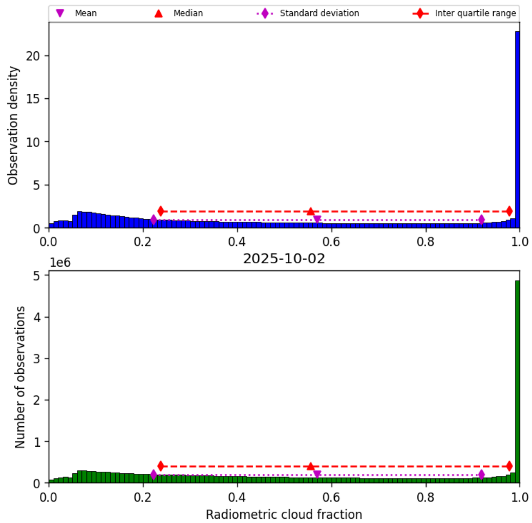
Figure 39: Histogram of “Radiometric cloud fraction” for 2025-10-01 to 2025-10-03
