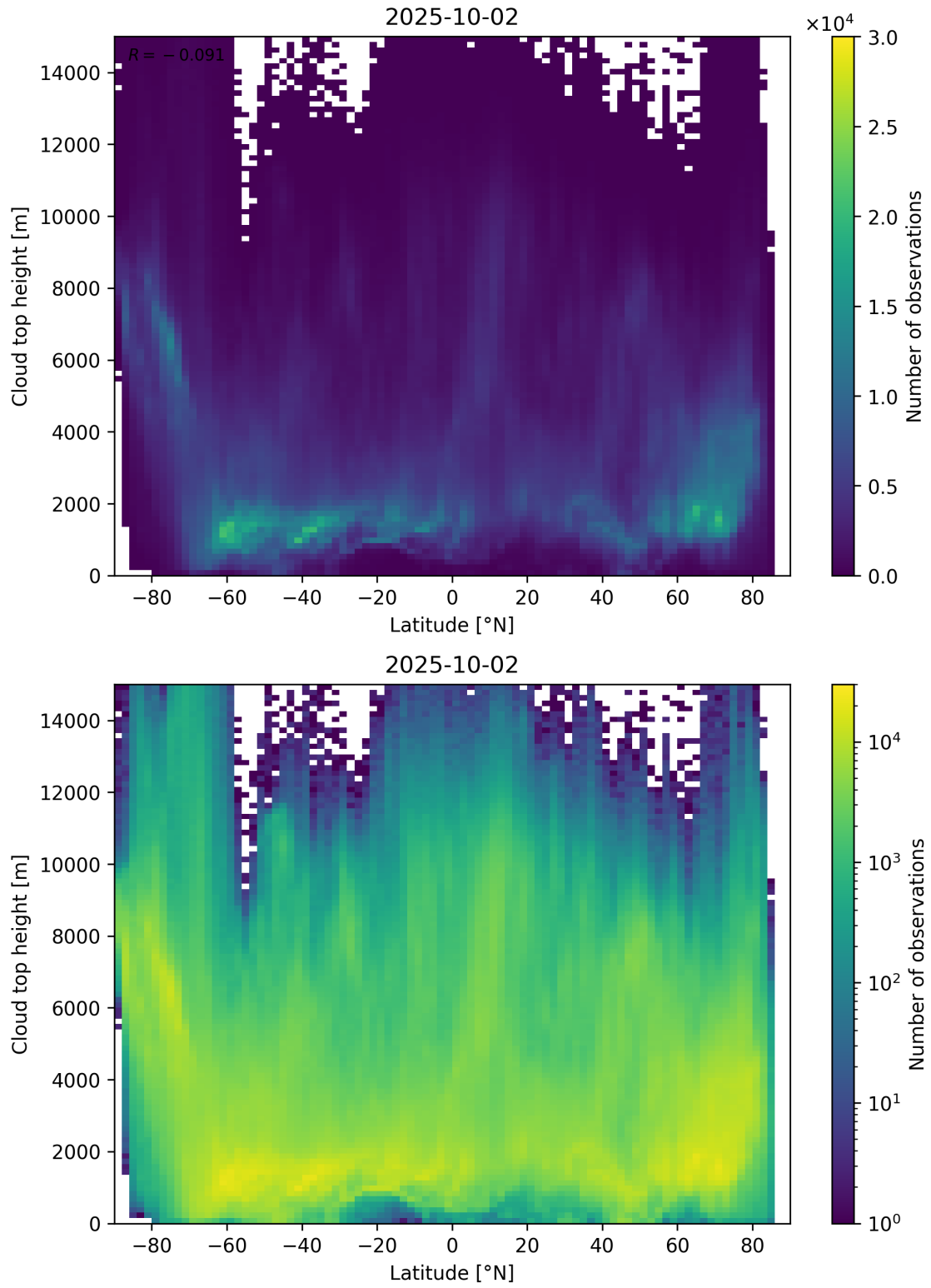
Figure 97: Scatter density plot of “Latitude” against “Cloud top height” for 2025-10-01 to 2025-10-03.
