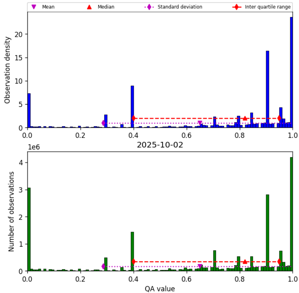
Figure 38: Histogram of “QA value” for 2025-10-01 to 2025-10-03
