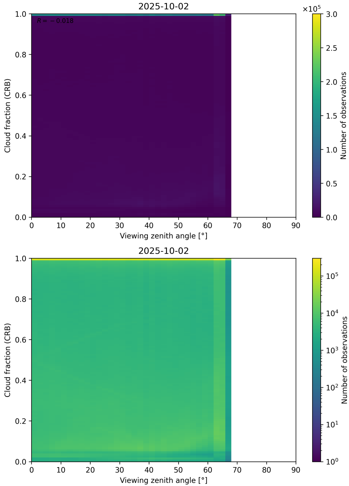
Figure 109: Scatter density plot of “Viewing zenith angle” against “Cloud fraction (CRB)” for 2025-10-01 to 2025-10-03.
