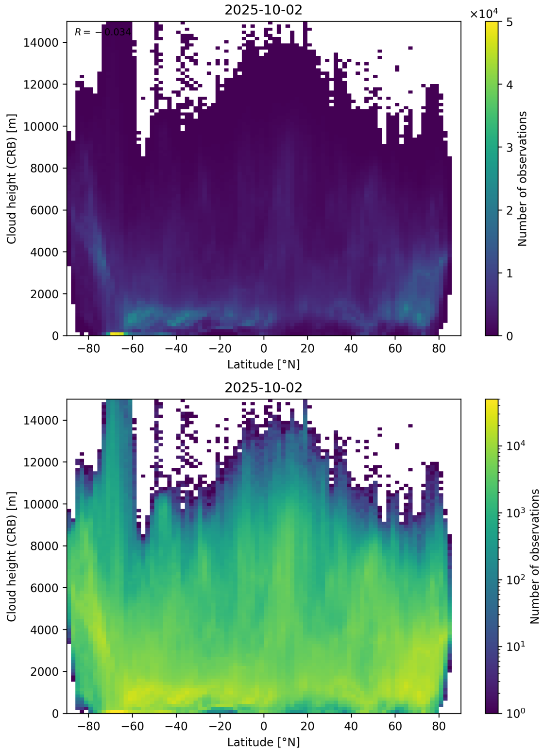
Figure 95: Scatter density plot of “Latitude” against “Cloud height (CRB)” for 2025-10-01 to 2025-10-03.
