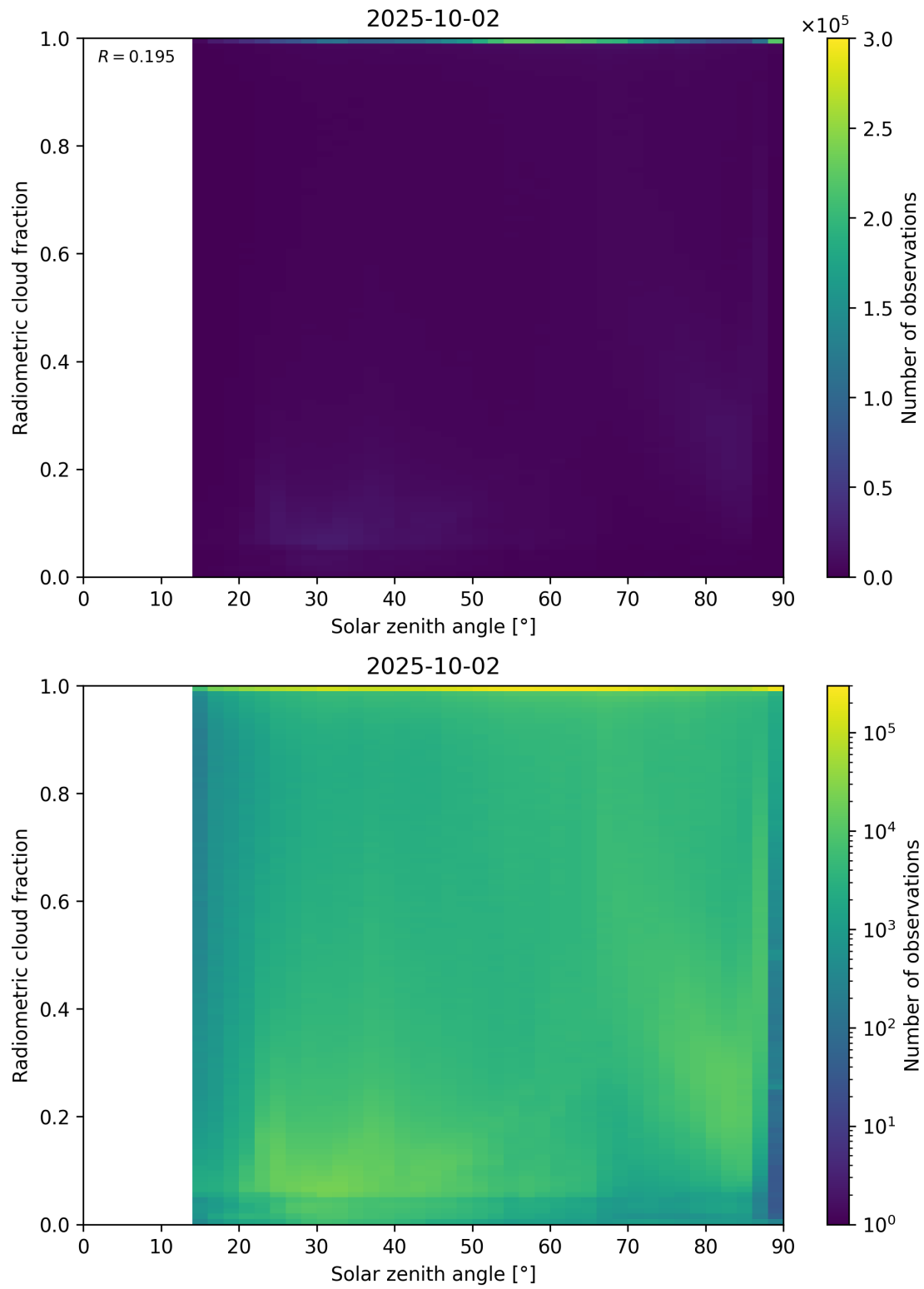
Figure 99: Scatter density plot of “Solar zenith angle” against “Radiometric cloud fraction” for 2025-10-01 to 2025-10-03.
