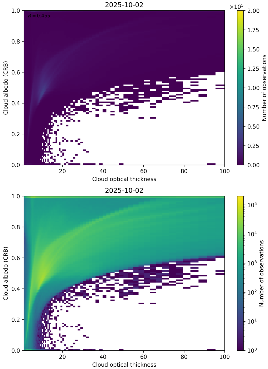
Figure 82: Scatter density plot of “Cloud optical thickness” against “Cloud albedo (CRB)” for 2025-10-01 to 2025-10-03.
