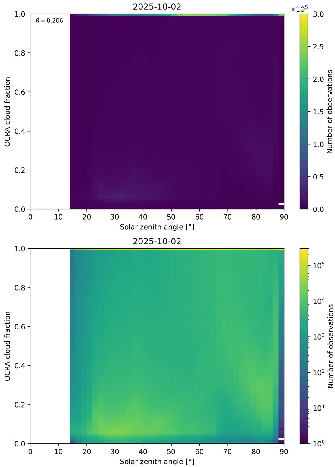
Figure 100: Scatter density plot of “Solar zenith angle” against “OCRA cloud fraction” for 2025-10-01 to 2025-10-03.
