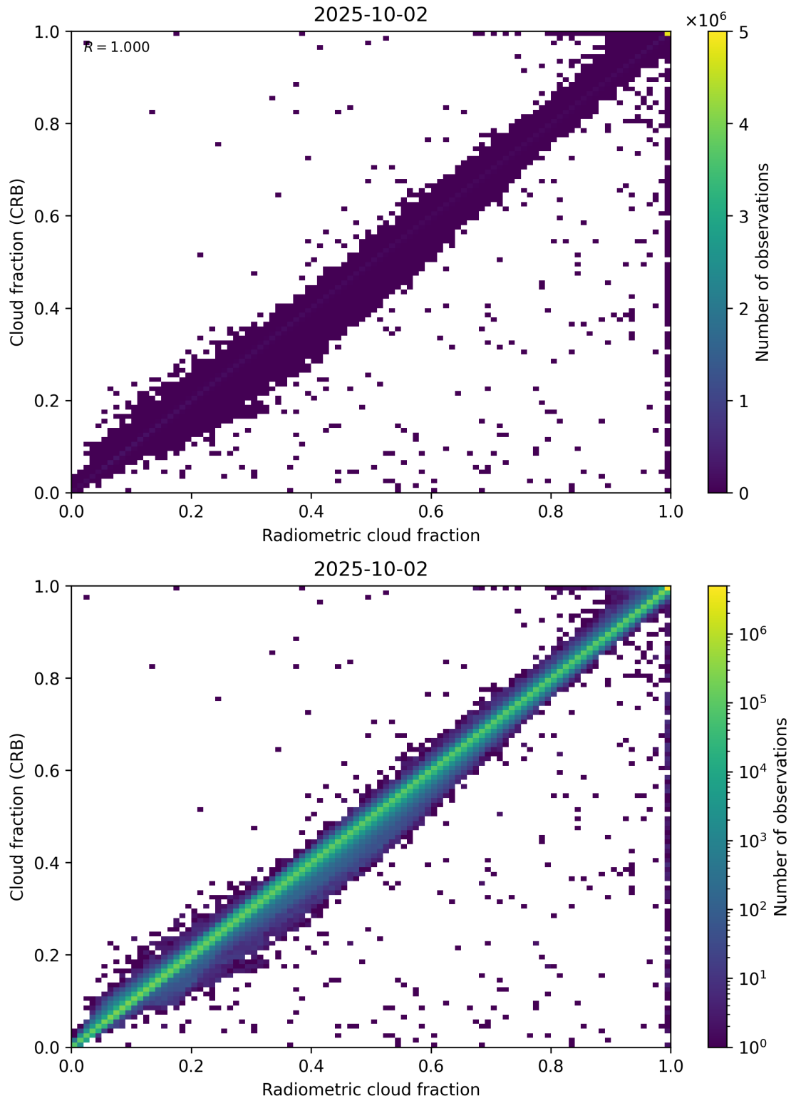
Figure 73: Scatter density plot of “Radiometric cloud fraction” against “Cloud fraction (CRB)” for 2025-10-01 to 2025-10-03.
