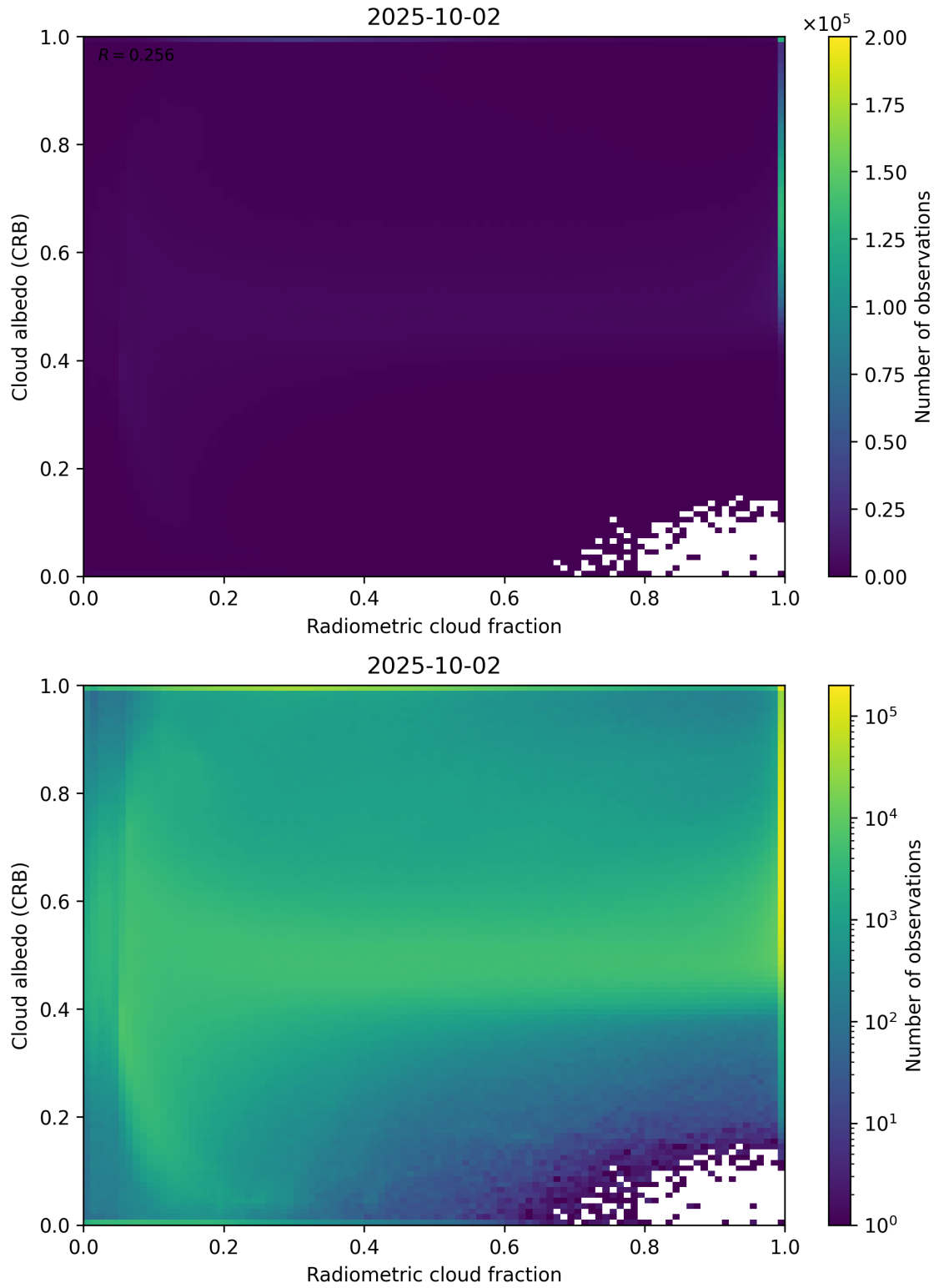
Figure 71: Scatter density plot of “Radiometric cloud fraction” against “Cloud albedo (CRB)” for 2025-10-01 to 2025-10-03.
