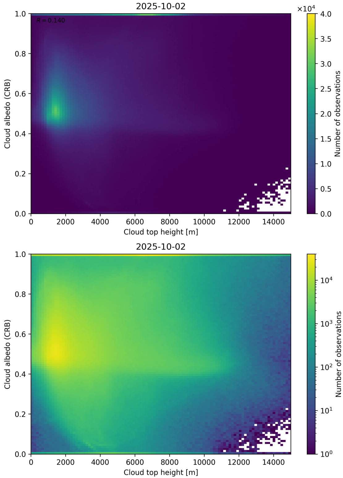
Figure 86: Scatter density plot of “Cloud top height” against “Cloud albedo (CRB)” for 2025-10-01 to 2025-10-03.
