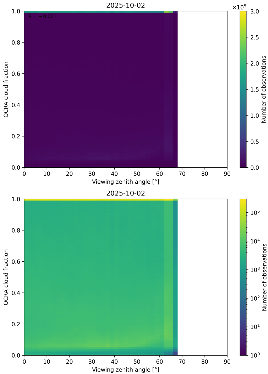
Figure 108: Scatter density plot of “Viewing zenith angle” against “OCRA cloud fraction” for 2025-10-01 to 2025-10-03.
