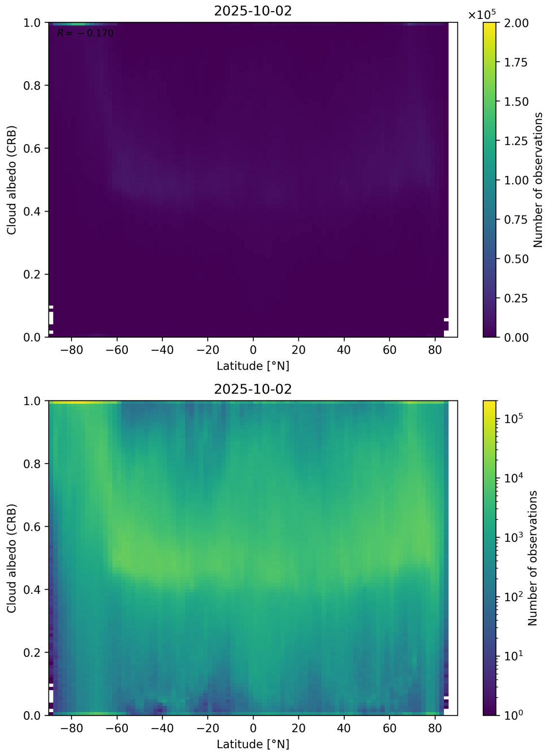
Figure 91: Scatter density plot of “Latitude” against “Cloud albedo (CRB)” for 2025-10-01 to 2025-10-03.
