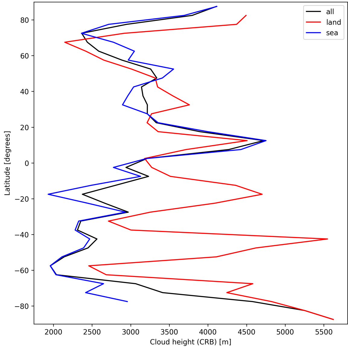
Figure 27: Zonal average of “Cloud height (CRB)” for 2025-10-01 to 2025-10-03.
