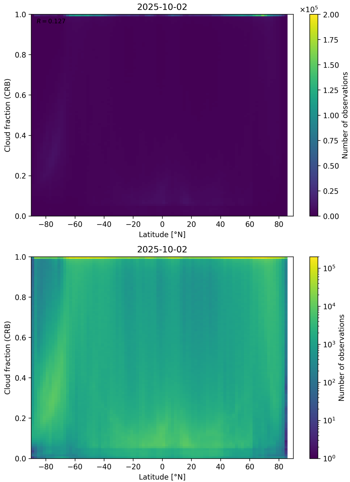
Figure 94: Scatter density plot of “Latitude” against “Cloud fraction (CRB)” for 2025-10-01 to 2025-10-03.
