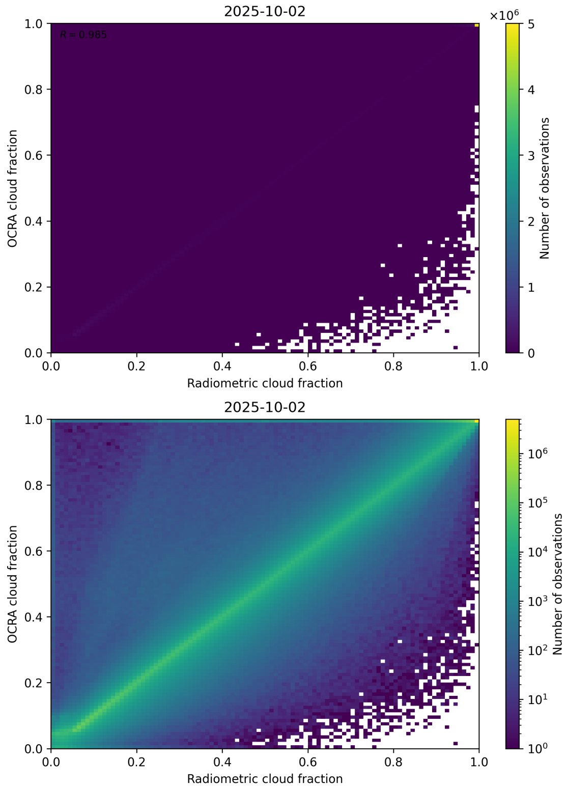
Figure 72: Scatter density plot of “Radiometric cloud fraction” against “OCRA cloud fraction” for 2025-10-01 to 2025-10-03.
