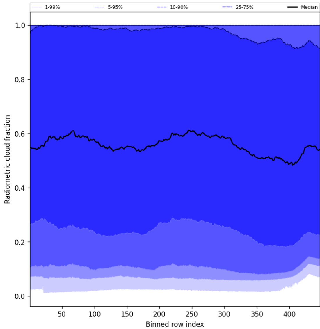
Figure 55: Along track statistics of “Radiometric cloud fraction” for 2025-10-01 to 2025-10-03
