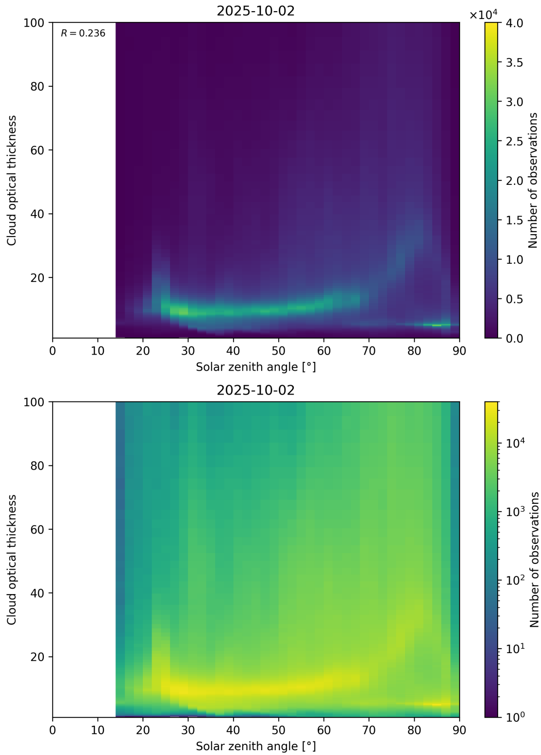
Figure 103: Scatter density plot of “Solar zenith angle” against “Cloud optical thickness” for 2025-10-01 to 2025-10-03.
