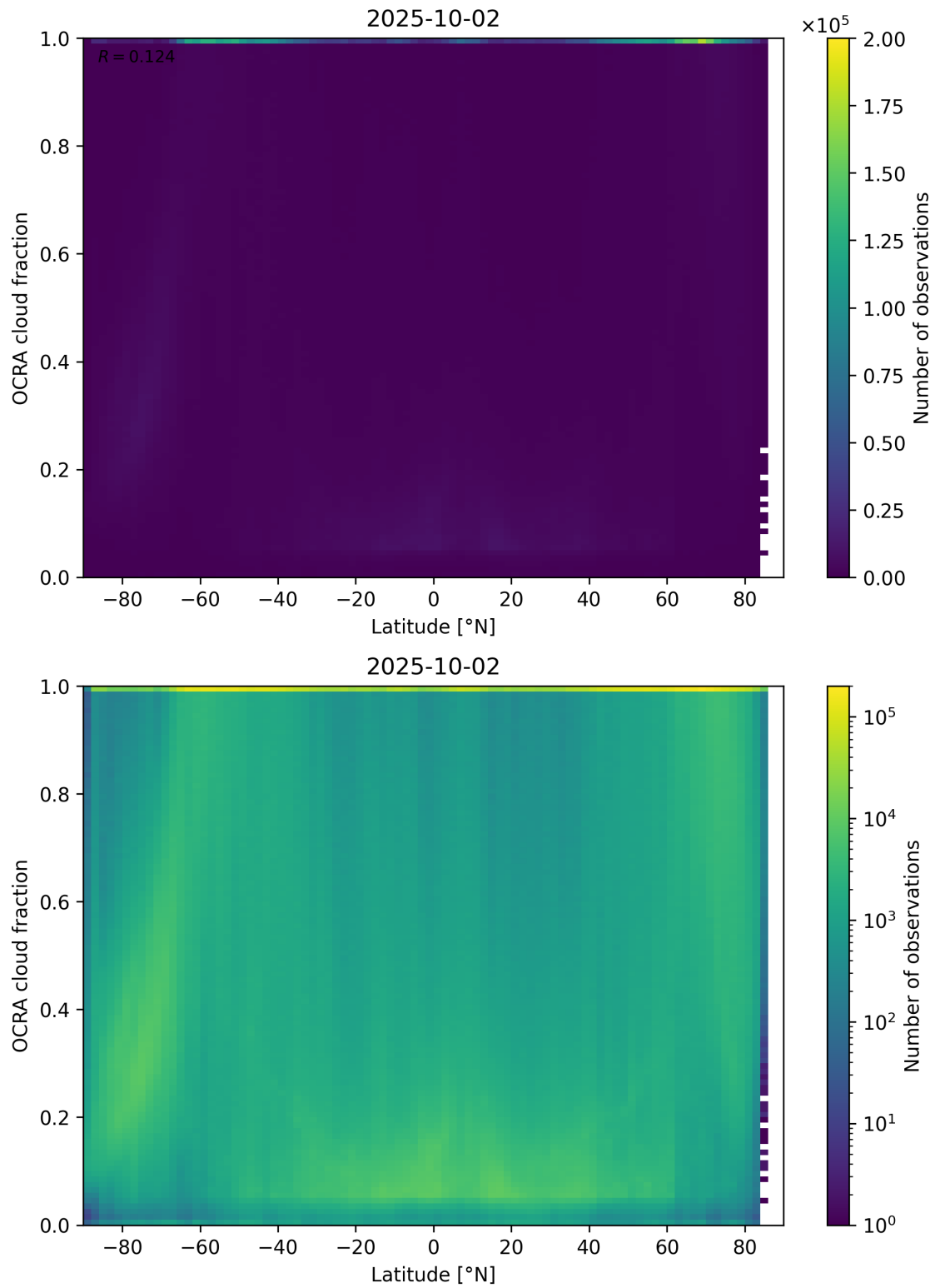
Figure 93: Scatter density plot of “Latitude” against “OCRA cloud fraction” for 2025-10-01 to 2025-10-03.
