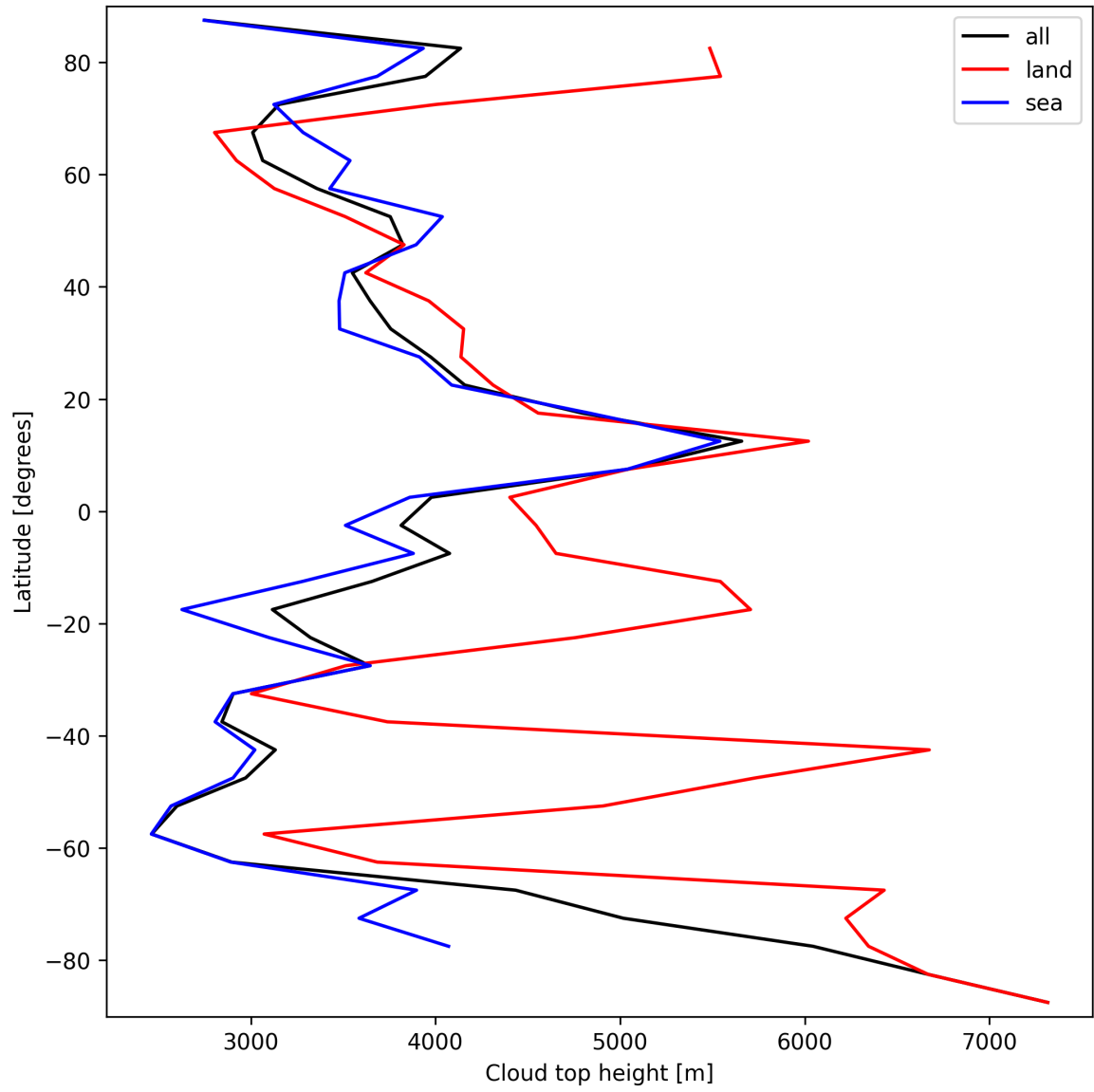
Figure 24: Zonal average of “Cloud top height” for 2025-10-01 to 2025-10-03.
