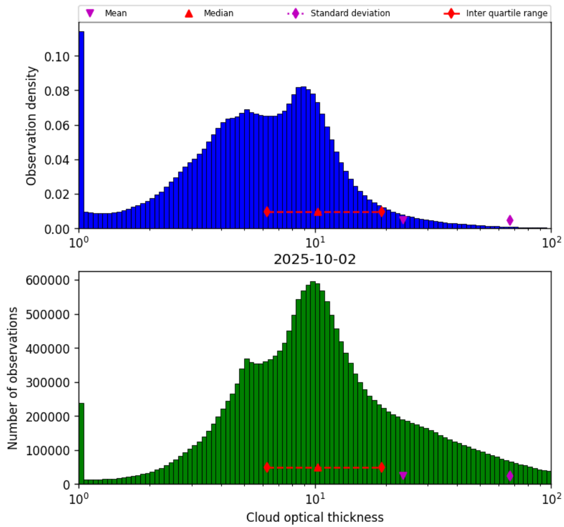
Figure 41: Histogram of “Cloud optical thickness” for 2025-10-01 to 2025-10-03
