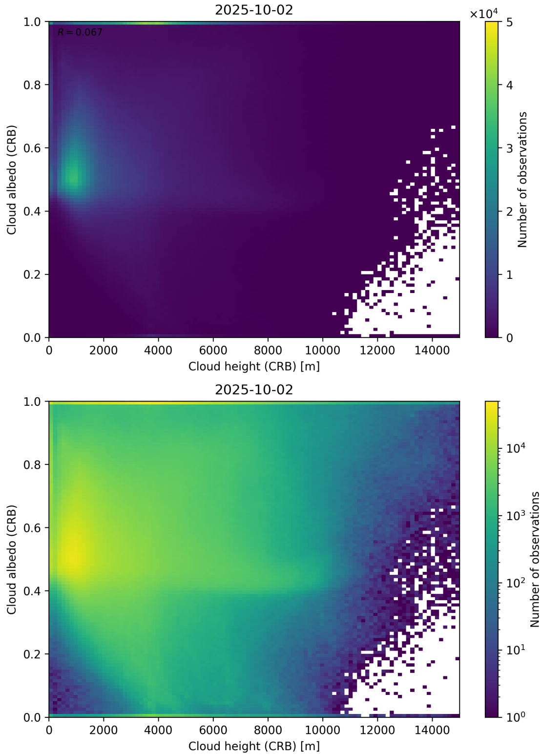
Figure 80: Scatter density plot of “Cloud height (CRB)” against “Cloud albedo (CRB)” for 2025-10-01 to 2025-10-03.
