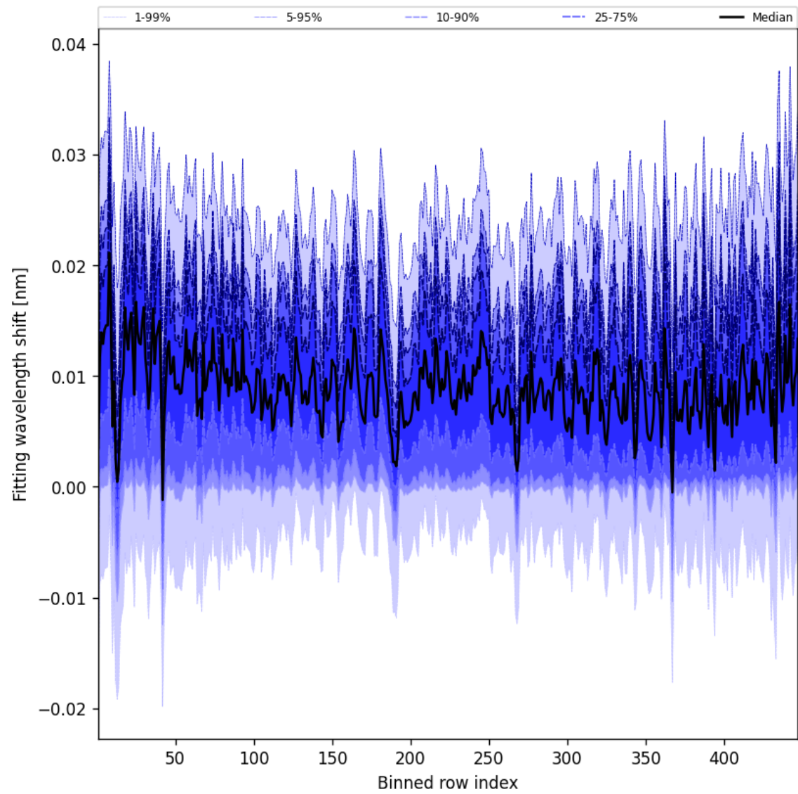
Figure 65: Along track statistics of “Fitting wavelength shift” for 2025-10-01 to 2025-10-03
