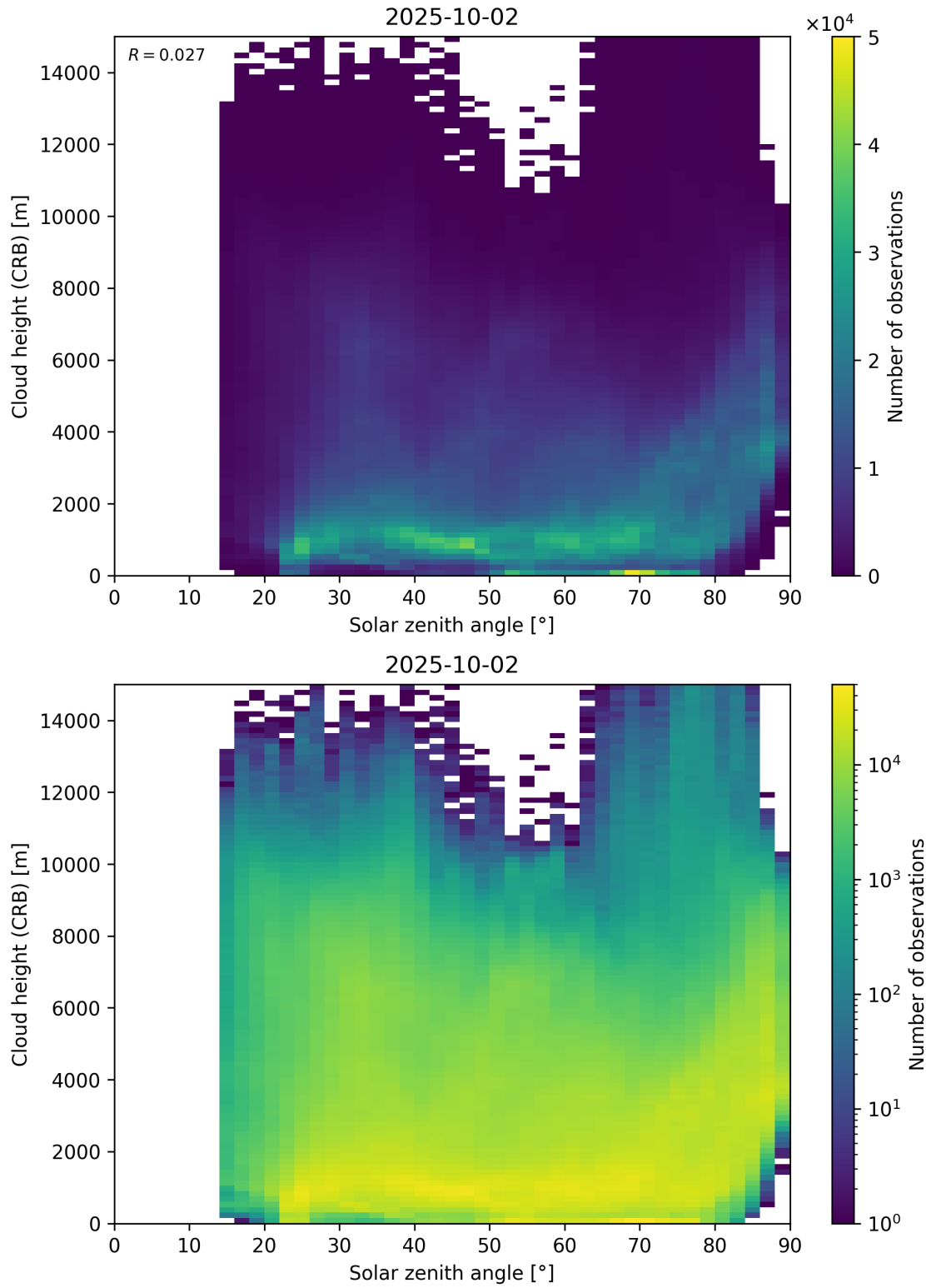
Figure 102: Scatter density plot of “Solar zenith angle” against “Cloud height (CRB)” for 2025-10-01 to 2025-10-03.
