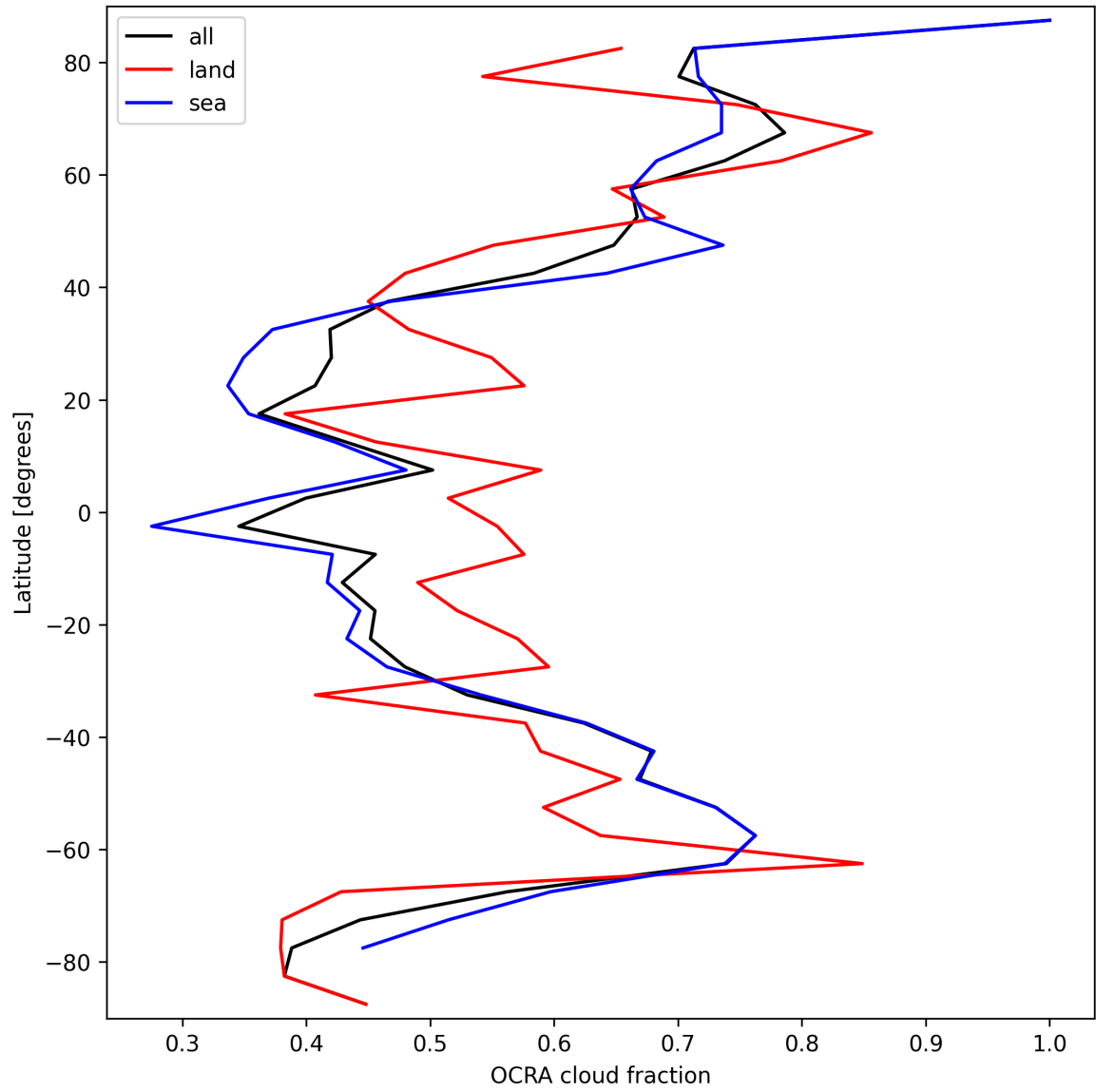
Figure 34: Zonal average of “OCRA cloud fraction” for 2025-10-01 to 2025-10-03.
