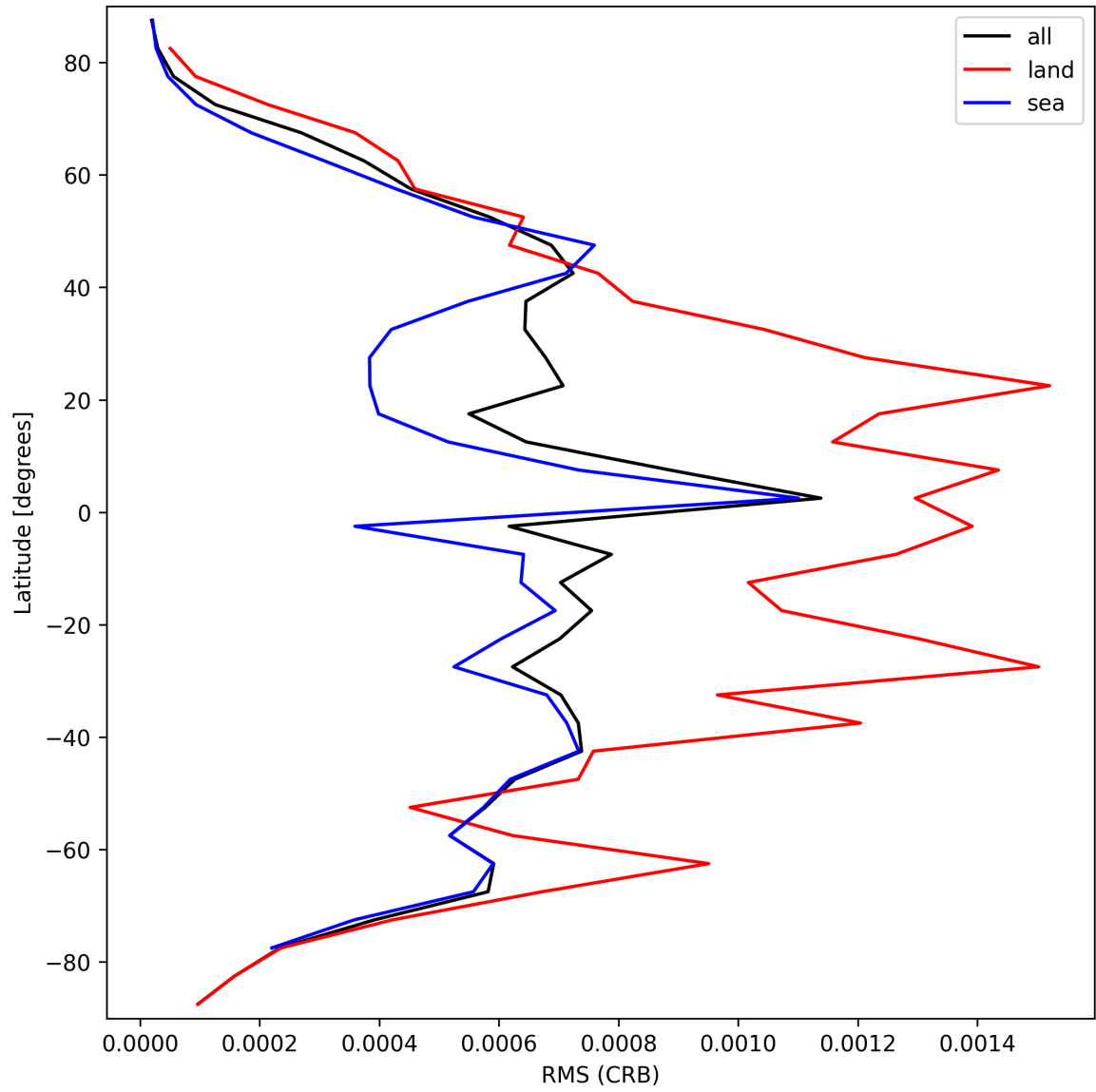
Figure 32: Zonal average of “RMS (CRB)” for 2025-10-01 to 2025-10-03.
