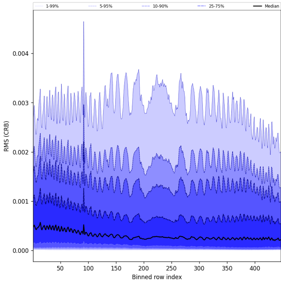
Figure 64: Along track statistics of “RMS (CRB)” for 2025-10-01 to 2025-10-03
