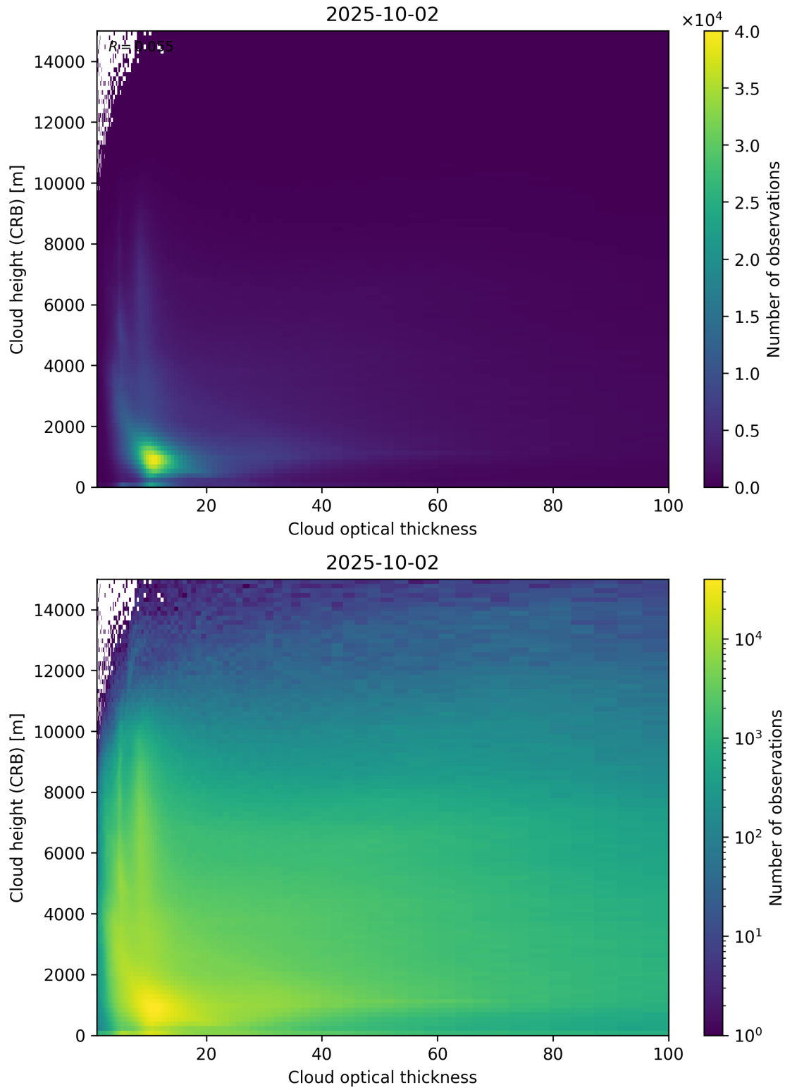
Figure 85: Scatter density plot of “Cloud optical thickness” against “Cloud height (CRB)” for 2025-10-01 to 2025-10-03.
