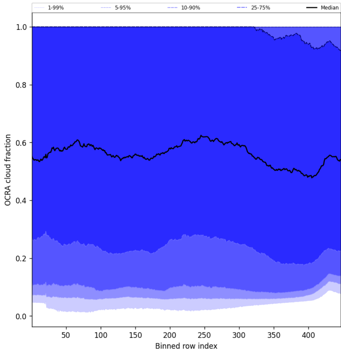
Figure 66: Along track statistics of “OCRA cloud fraction” for 2025-10-01 to 2025-10-03
