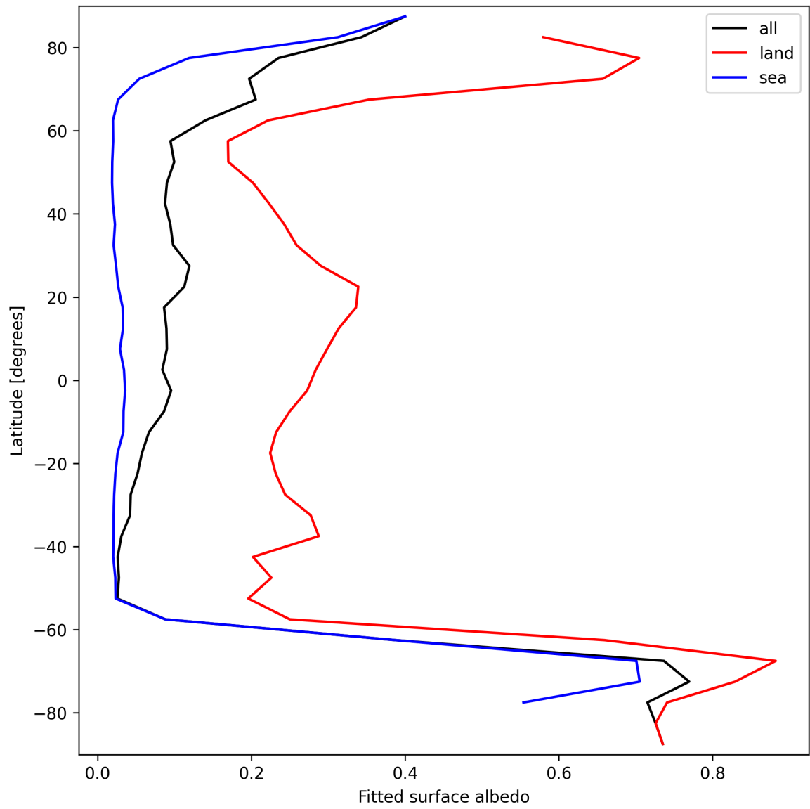
Figure 29: Zonal average of “Fitted surface albedo” for 2025-10-01 to 2025-10-03.
