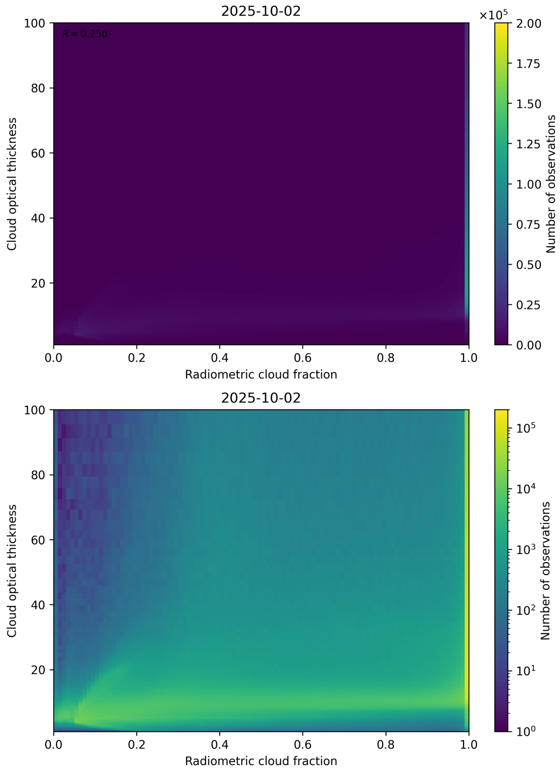
Figure 75: Scatter density plot of “Radiometric cloud fraction” against “Cloud optical thickness” for 2025-10-01 to 2025-10-03.
