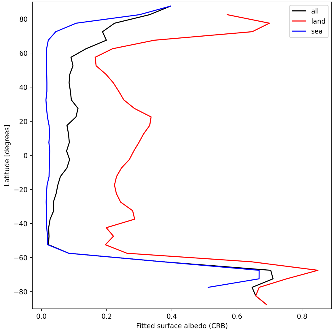
Figure 30: Zonal average of “Fitted surface albedo (CRB)” for 2025-10-01 to 2025-10-03.
