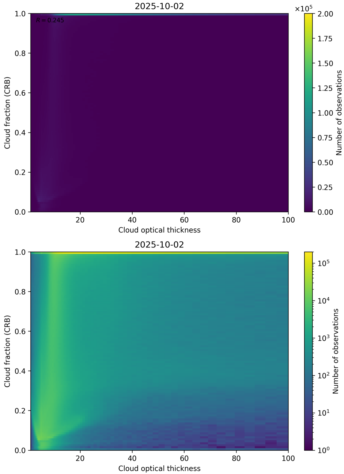
Figure 84: Scatter density plot of “Cloud optical thickness” against “Cloud fraction (CRB)” for 2025-10-01 to 2025-10-03.
