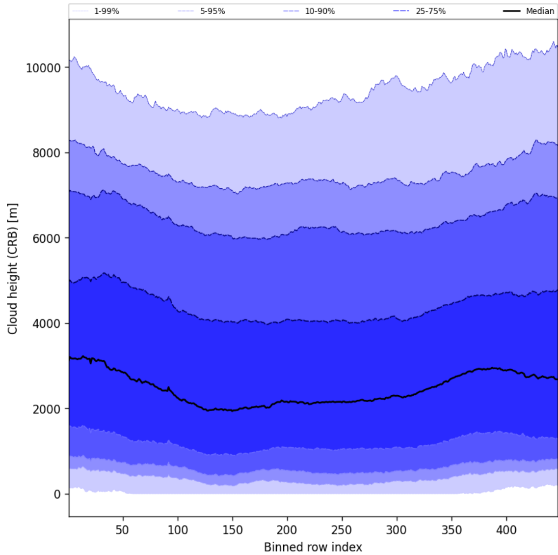
Figure 59: Along track statistics of “Cloud height (CRB)” for 2025-10-01 to 2025-10-03
