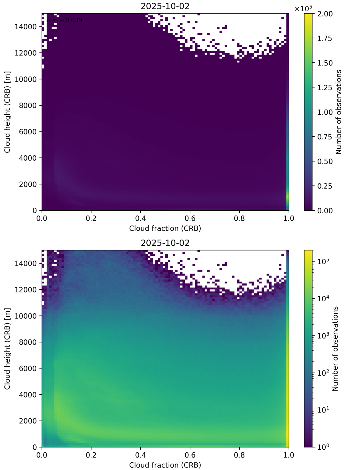
Figure 79: Scatter density plot of “Cloud fraction (CRB)” against “Cloud height (CRB)” for 2025-10-01 to 2025-10-03.
