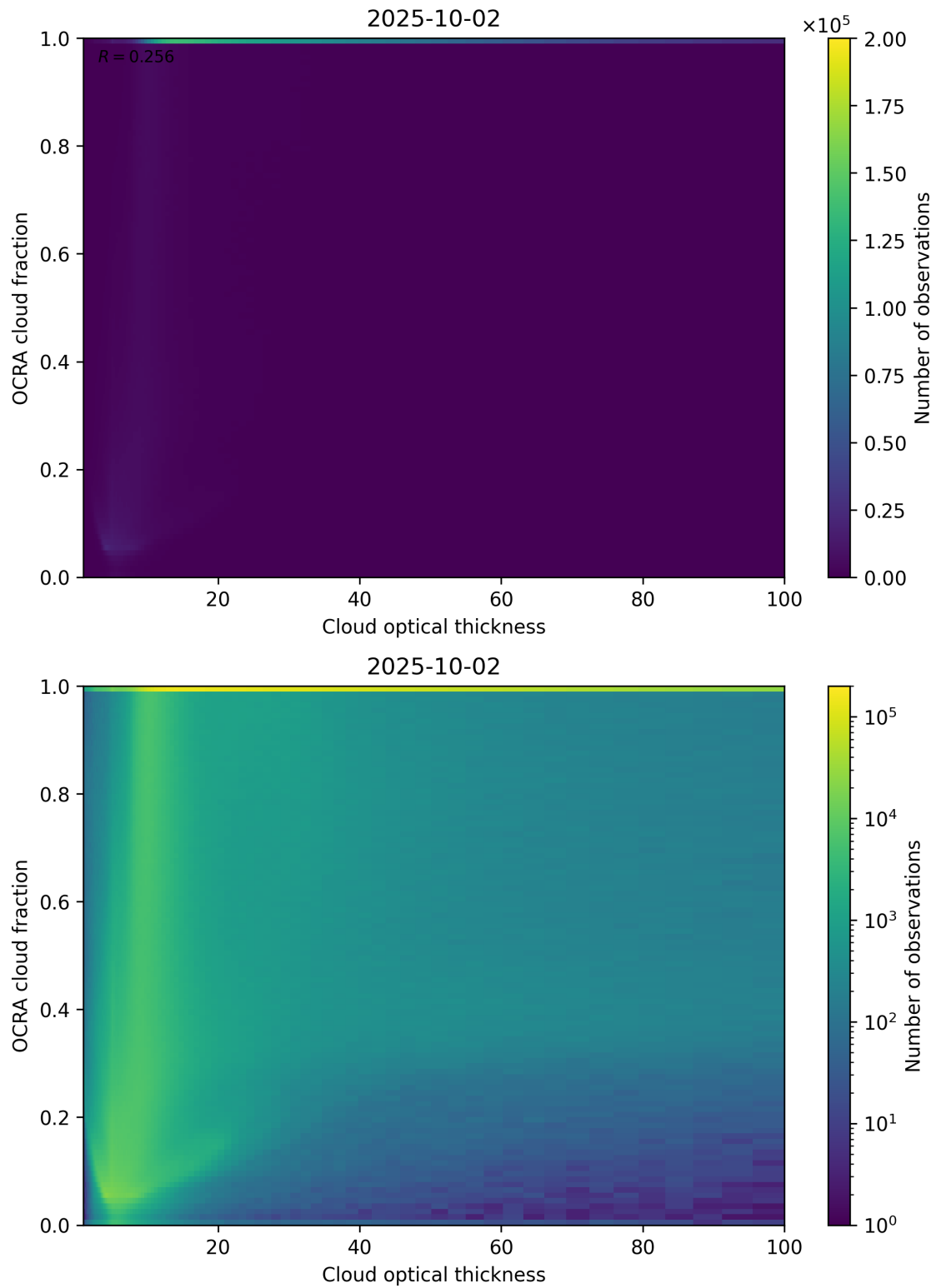
Figure 83: Scatter density plot of “Cloud optical thickness” against “OCRA cloud fraction” for 2025-10-01 to 2025-10-03.
