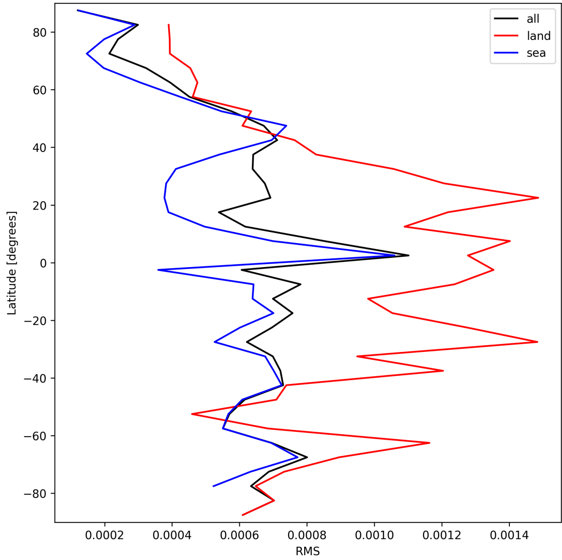
Figure 31: Zonal average of “RMS” for 2025-10-01 to 2025-10-03.
