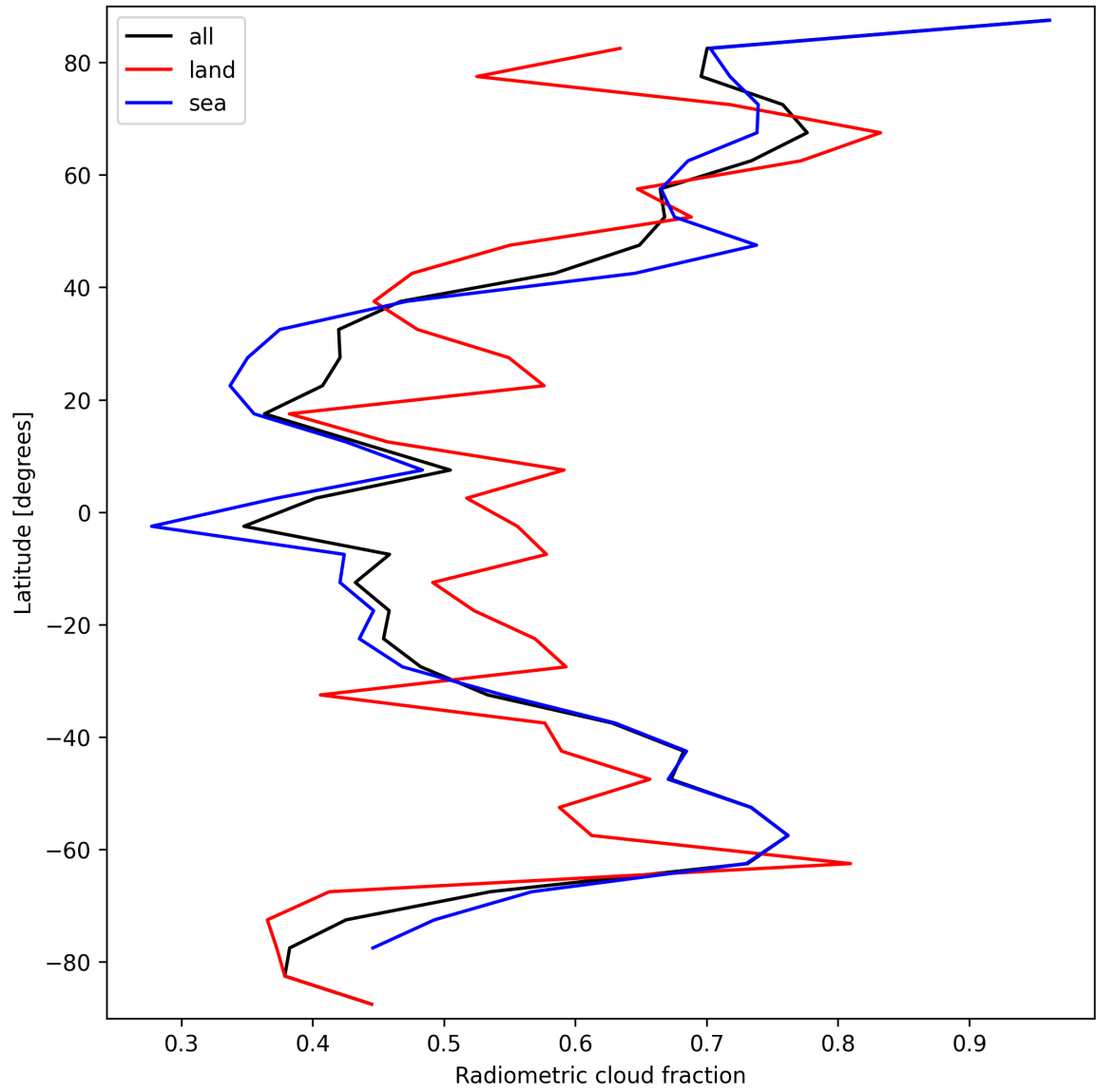
Figure 23: Zonal average of “Radiometric cloud fraction” for 2025-10-01 to 2025-10-03.
