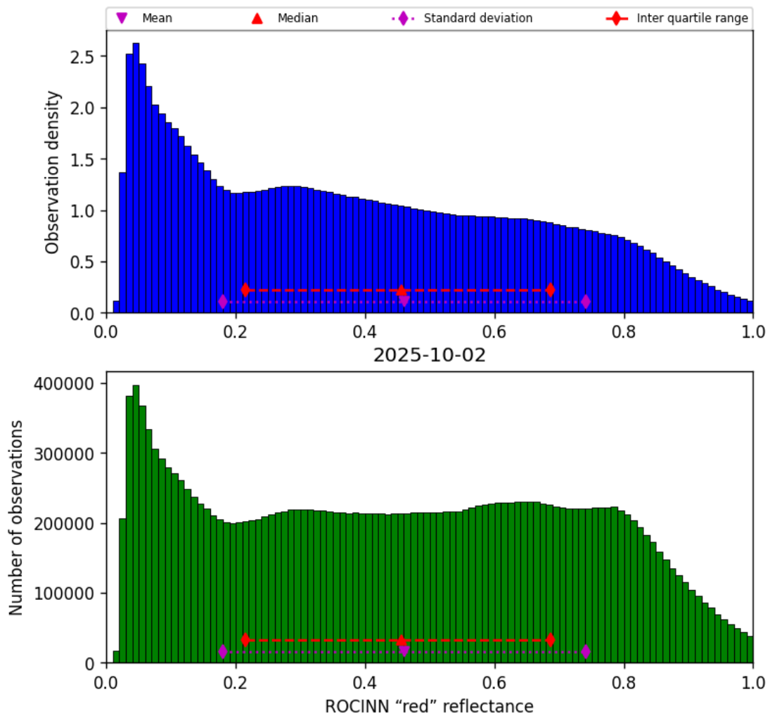
Figure 53: Histogram of “ROCINN “red” reflectance” for 2025-10-01 to 2025-10-03
