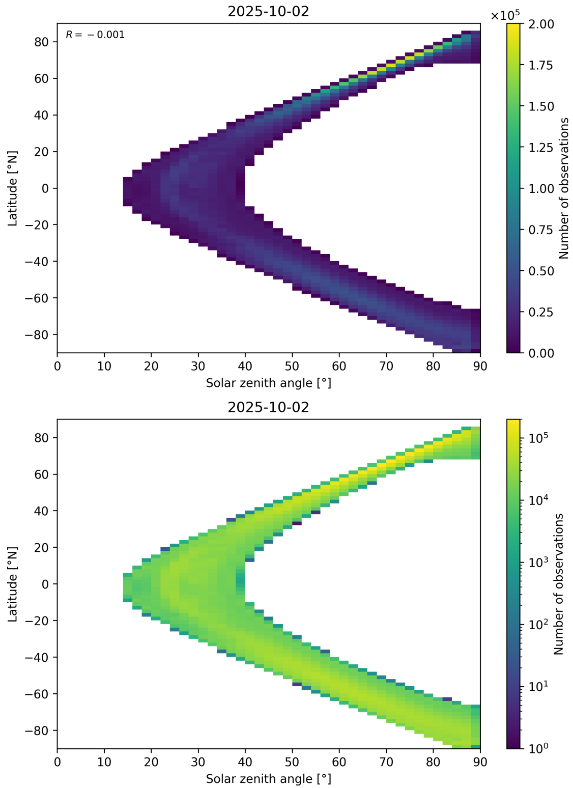
Figure 105: Scatter density plot of “Solar zenith angle” against “Latitude” for 2025-10-01 to 2025-10-03.
