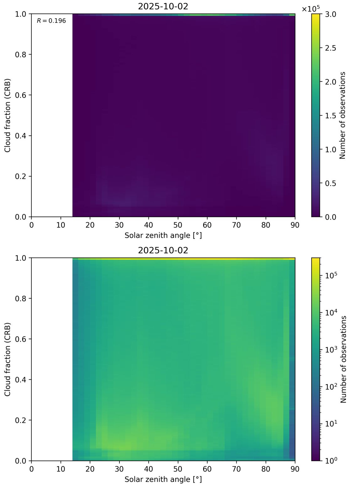
Figure 101: Scatter density plot of “Solar zenith angle” against “Cloud fraction (CRB)” for 2025-10-01 to 2025-10-03.
