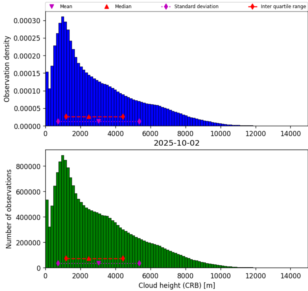
Figure 43: Histogram of “Cloud height (CRB)” for 2025-10-01 to 2025-10-03
