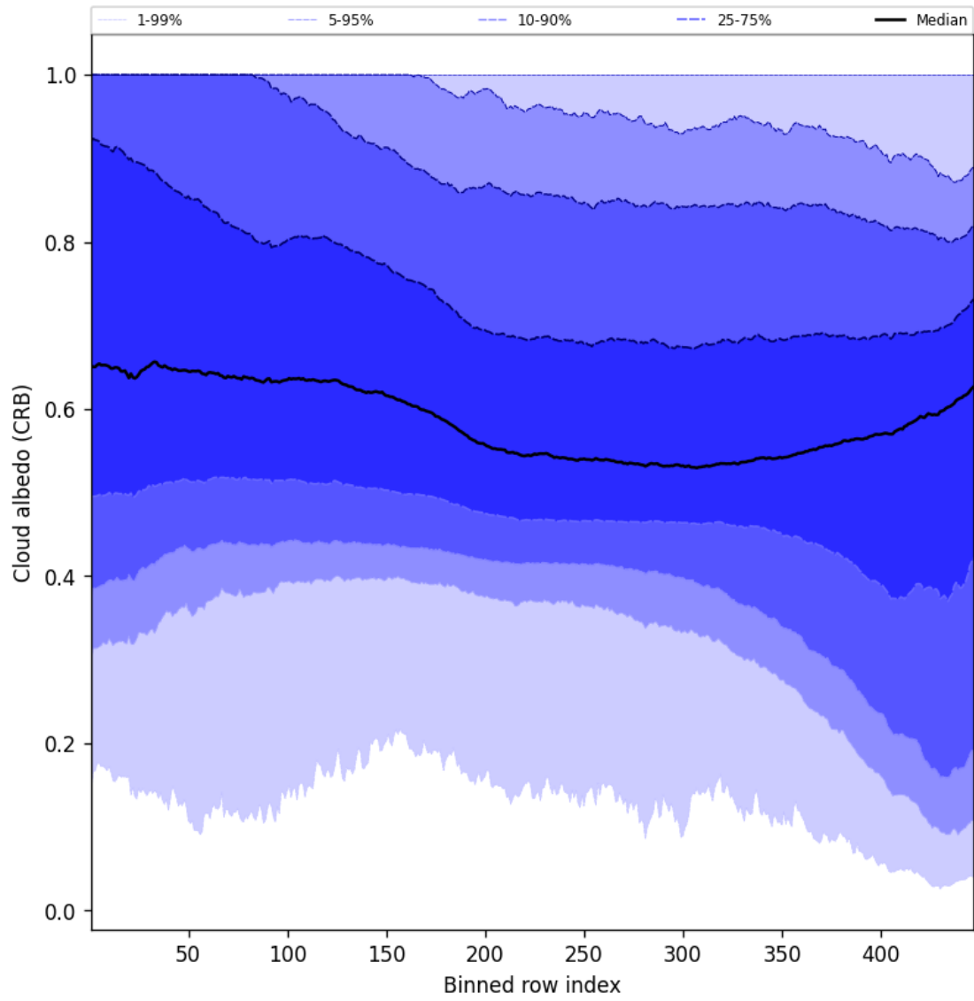
Figure 60: Along track statistics of “Cloud albedo (CRB)” for 2025-10-01 to 2025-10-03
