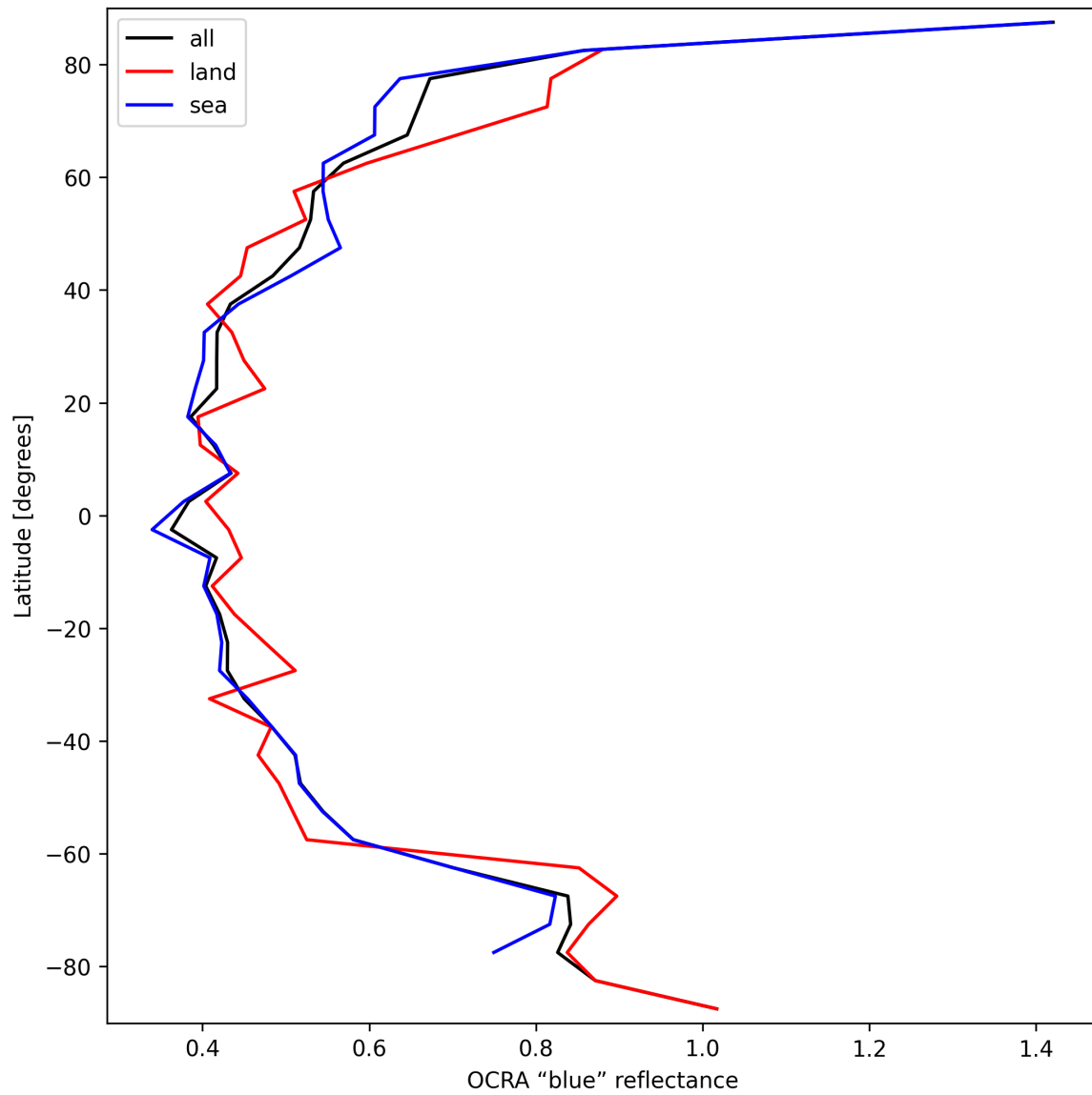
Figure 35: Zonal average of “OCRA “blue” reflectance” for 2025-10-01 to 2025-10-03.
