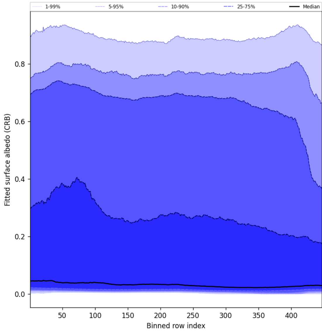
Figure 62: Along track statistics of “Fitted surface albedo (CRB)” for 2025-10-01 to 2025-10-03
