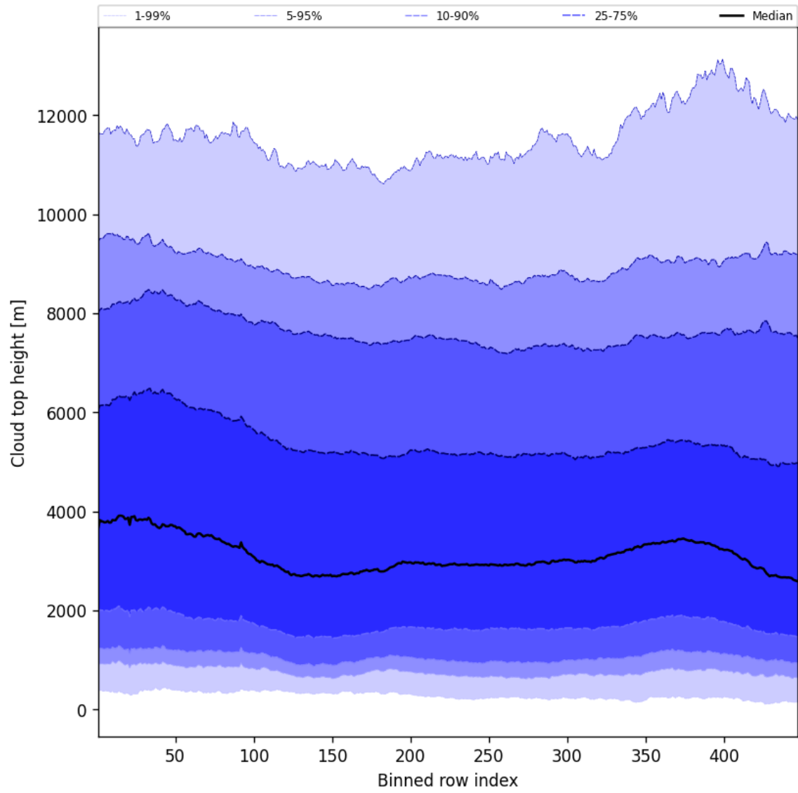
Figure 56: Along track statistics of “Cloud top height” for 2025-10-01 to 2025-10-03
