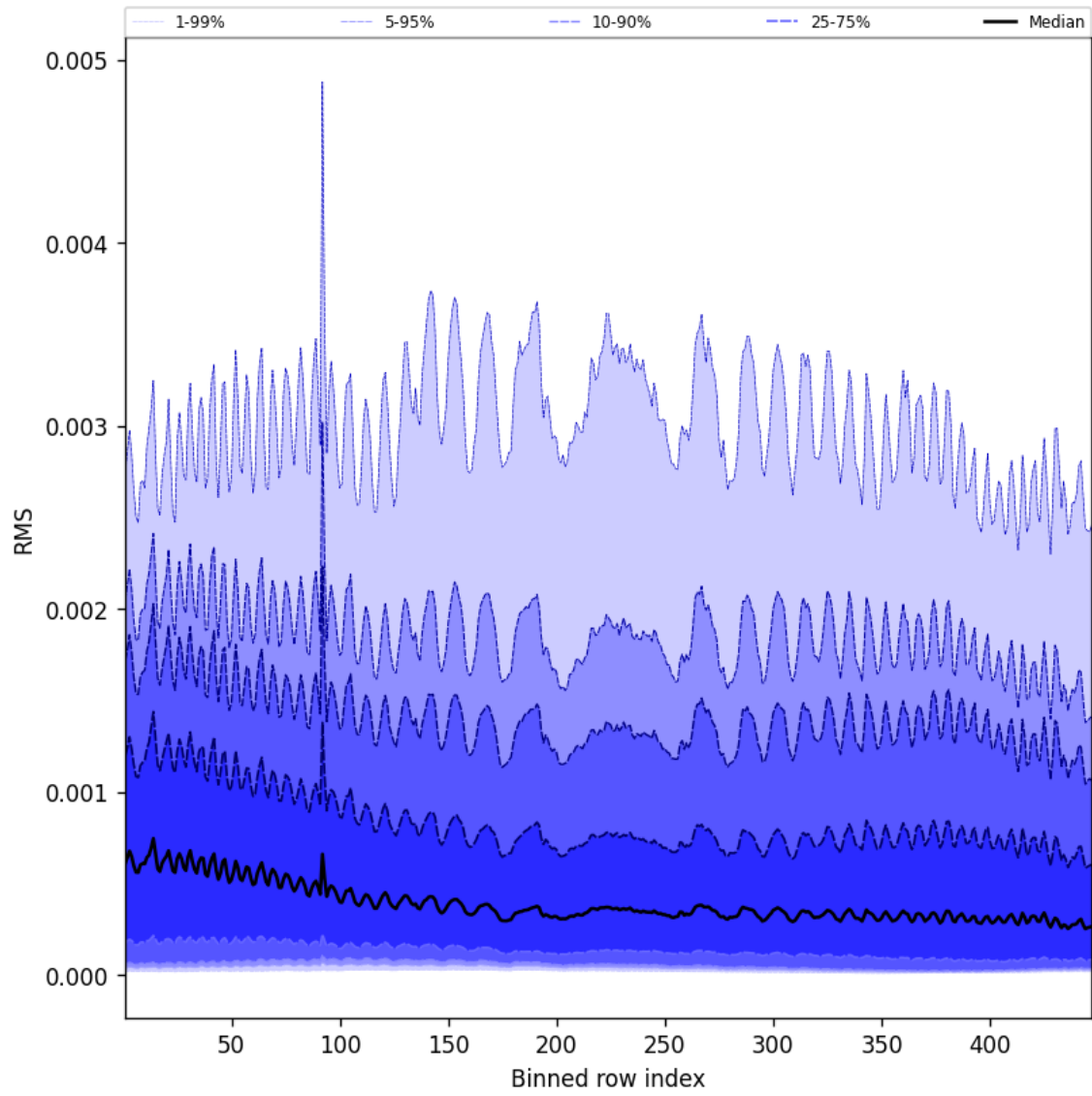
Figure 63: Along track statistics of “RMS” for 2025-10-01 to 2025-10-03
