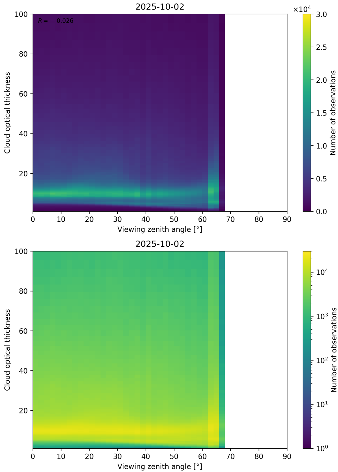
Figure 111: Scatter density plot of “Viewing zenith angle” against “Cloud optical thickness” for 2025-10-01 to 2025-10-03.
