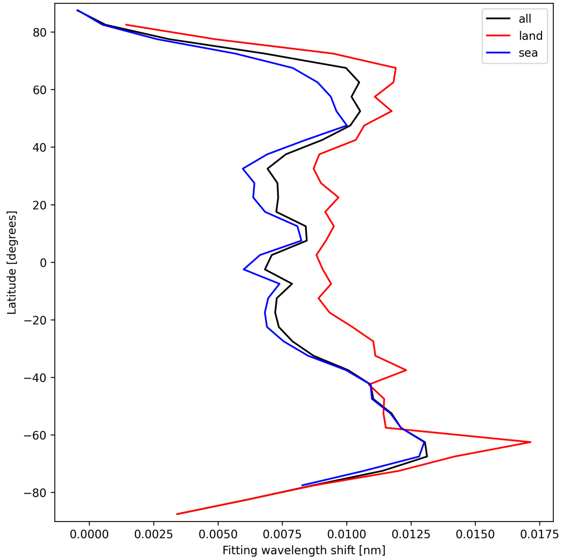
Figure 33: Zonal average of “Fitting wavelength shift” for 2025-10-01 to 2025-10-03.
