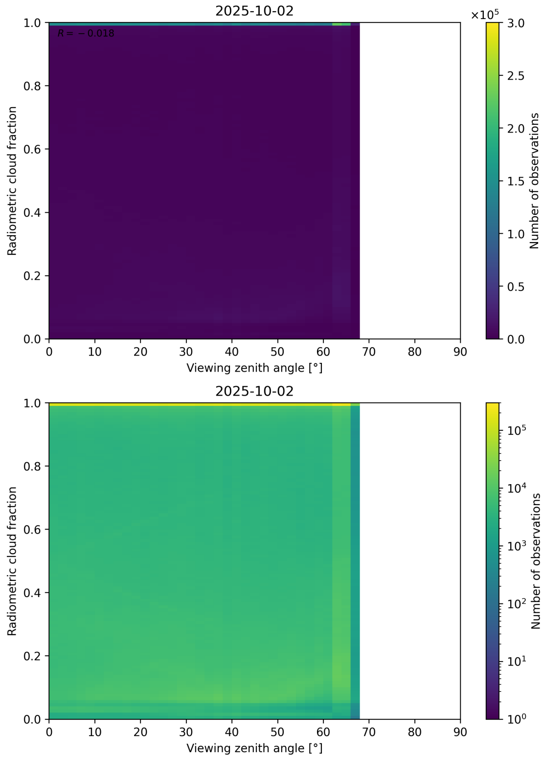
Figure 107: Scatter density plot of “Viewing zenith angle” against “Radiometric cloud fraction” for 2025-10-01 to 2025-10-03.
