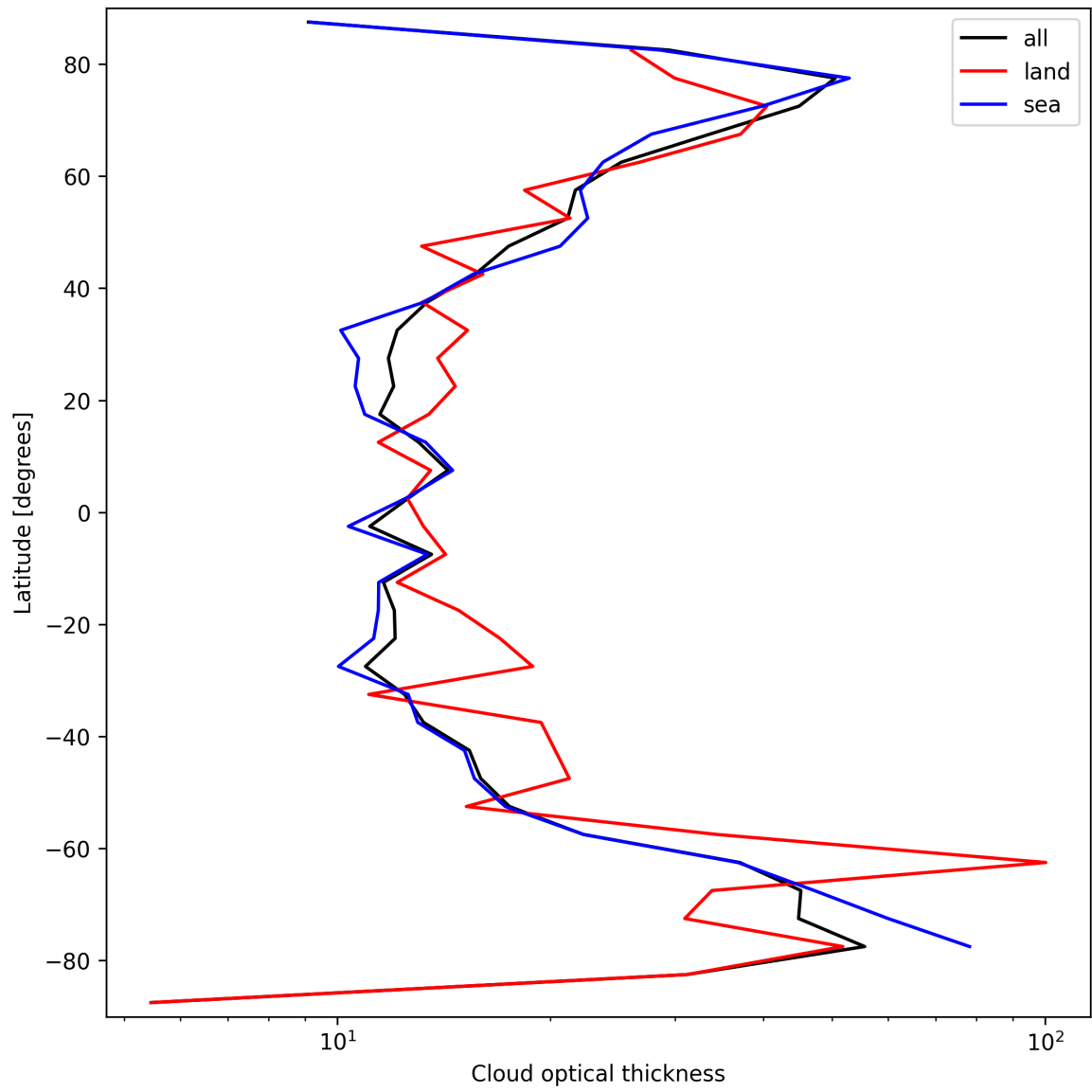
Figure 25: Zonal average of “Cloud optical thickness” for 2025-10-01 to 2025-10-03.
