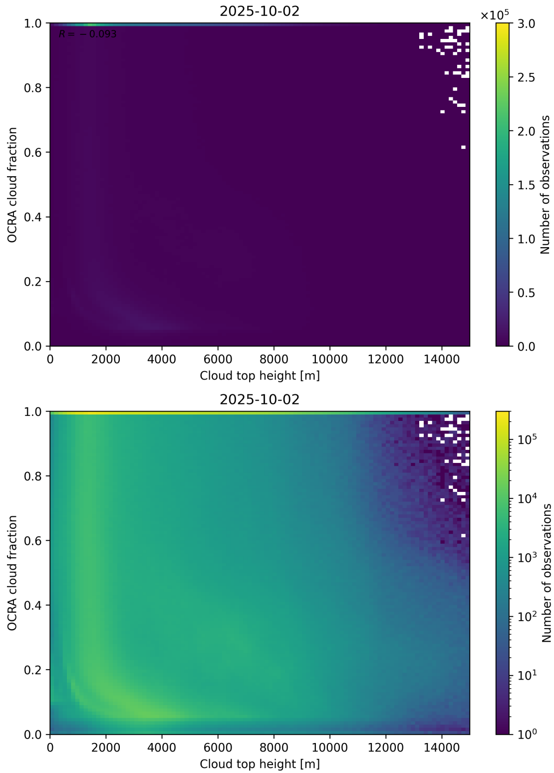
Figure 87: Scatter density plot of “Cloud top height” against “OCRA cloud fraction” for 2025-10-01 to 2025-10-03.
