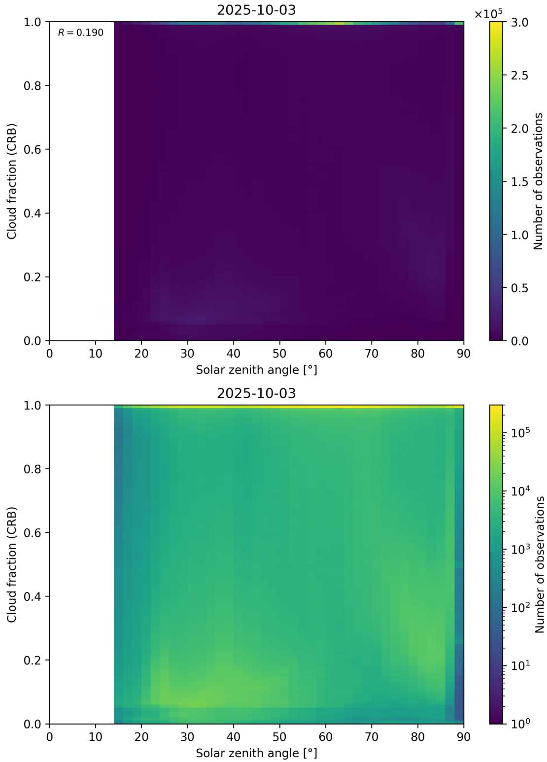
Figure 101: Scatter density plot of “Solar zenith angle” against “Cloud fraction (CRB)” for 2025-10-02 to 2025-10-04.
