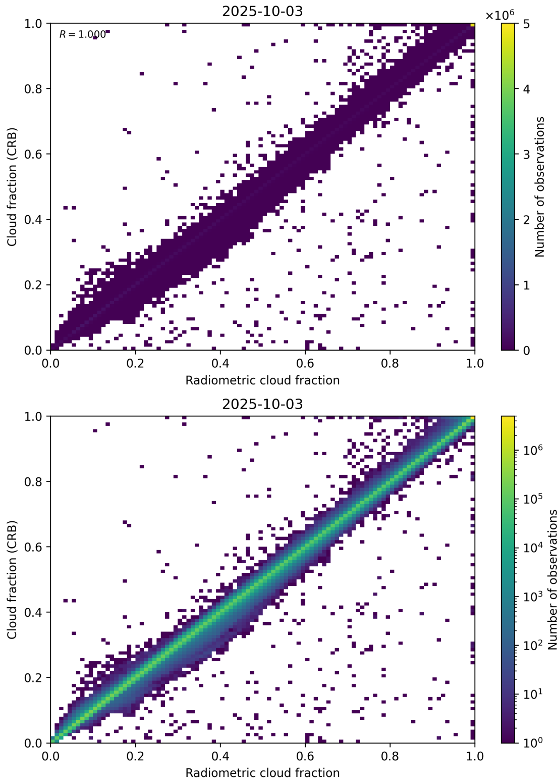
Figure 73: Scatter density plot of “Radiometric cloud fraction” against “Cloud fraction (CRB)” for 2025-10-02 to 2025-10-04.
