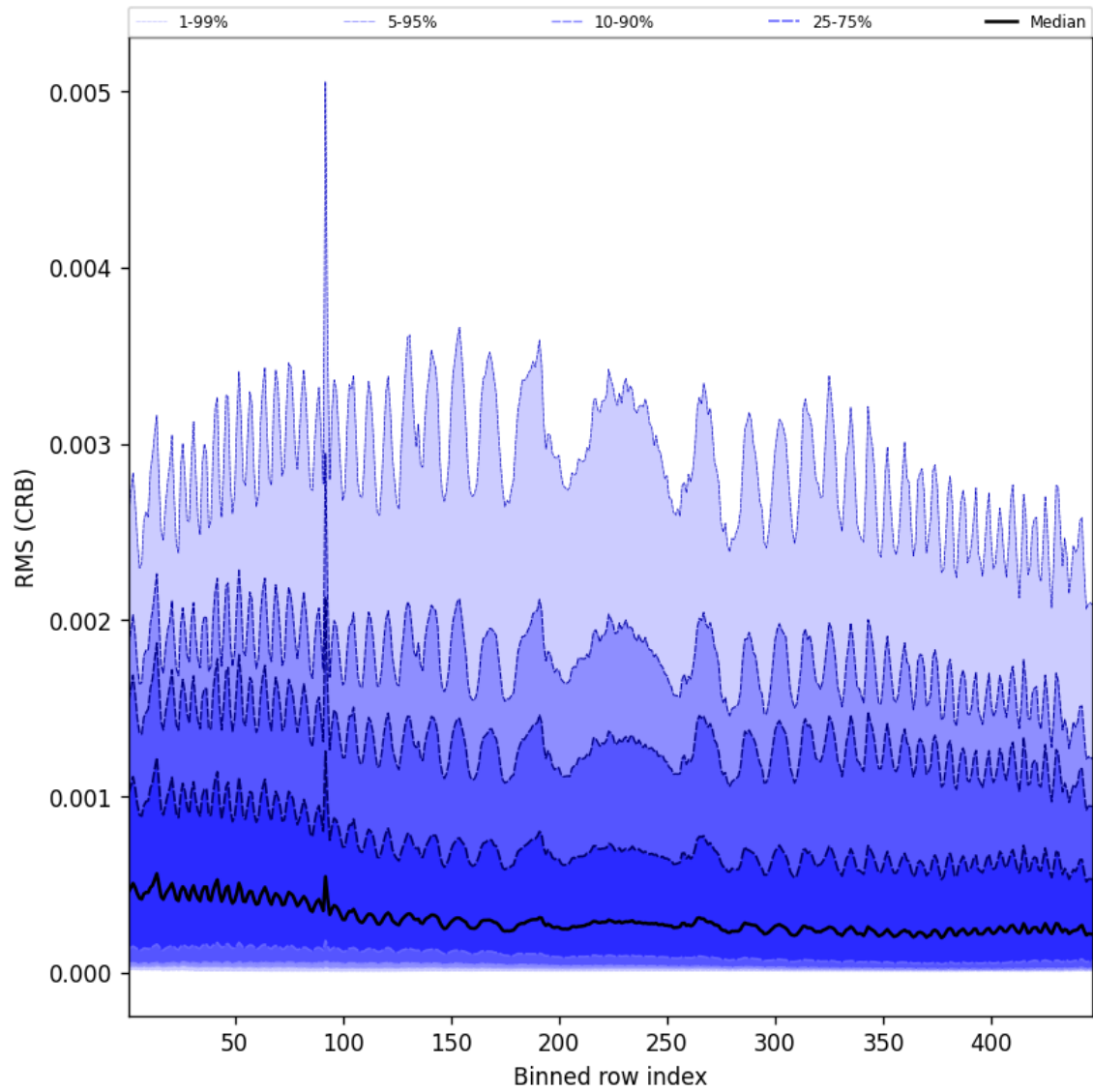
Figure 64: Along track statistics of “RMS (CRB)” for 2025-10-02 to 2025-10-04
