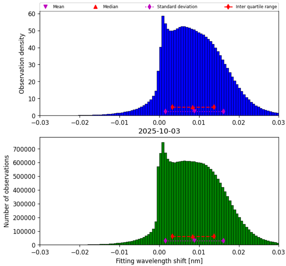
Figure 49: Histogram of “Fitting wavelength shift” for 2025-10-02 to 2025-10-04
