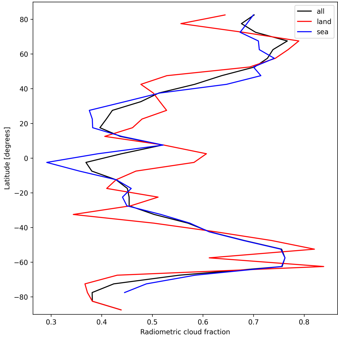
Figure 23: Zonal average of “Radiometric cloud fraction” for 2025-10-02 to 2025-10-04.
