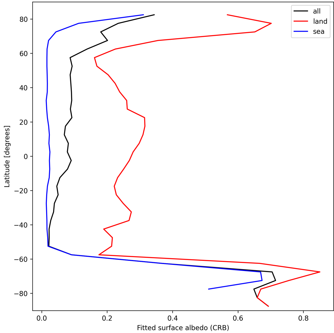
Figure 30: Zonal average of “Fitted surface albedo (CRB)” for 2025-10-02 to 2025-10-04.
