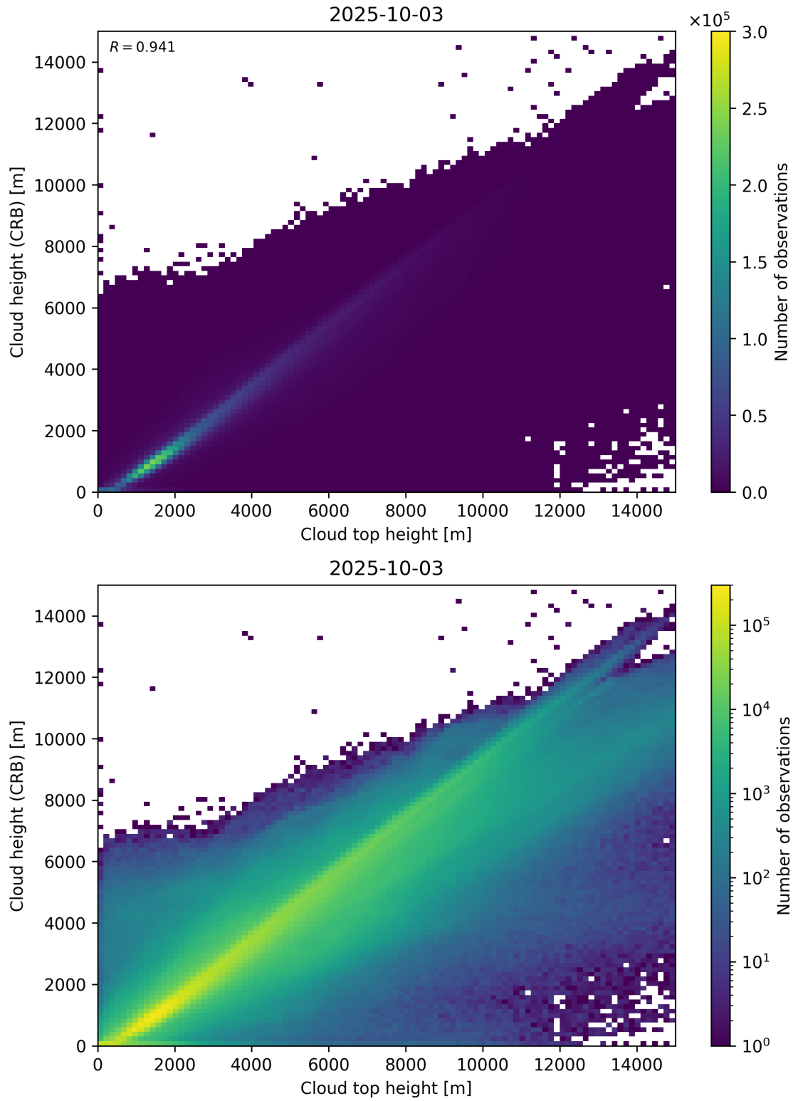
Figure 89: Scatter density plot of “Cloud top height” against “Cloud height (CRB)” for 2025-10-02 to 2025-10-04.
