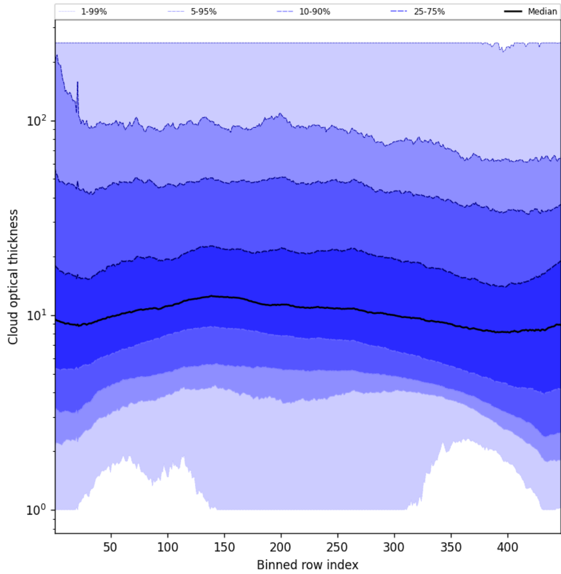
Figure 57: Along track statistics of “Cloud optical thickness” for 2025-10-02 to 2025-10-04
