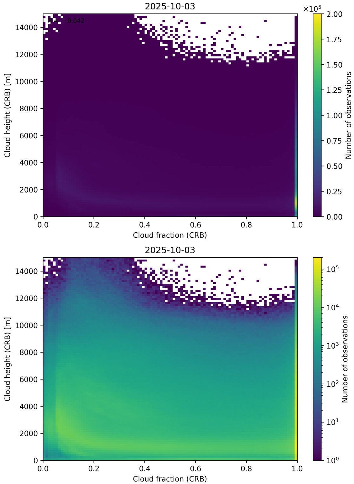
Figure 79: Scatter density plot of “Cloud fraction (CRB)” against “Cloud height (CRB)” for 2025-10-02 to 2025-10-04.
