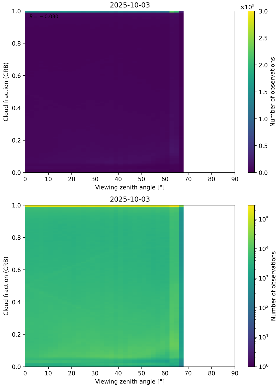
Figure 109: Scatter density plot of “Viewing zenith angle” against “Cloud fraction (CRB)” for 2025-10-02 to 2025-10-04.
