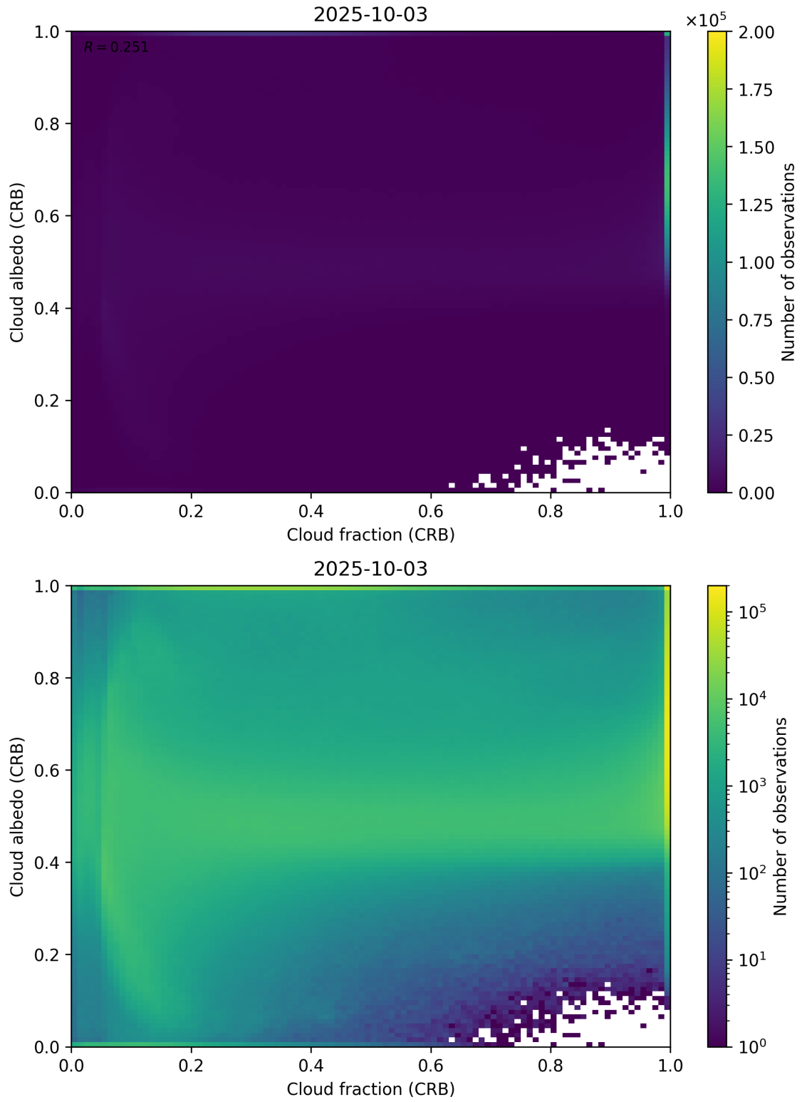
Figure 77: Scatter density plot of “Cloud fraction (CRB)” against “Cloud albedo (CRB)” for 2025-10-02 to 2025-10-04.
