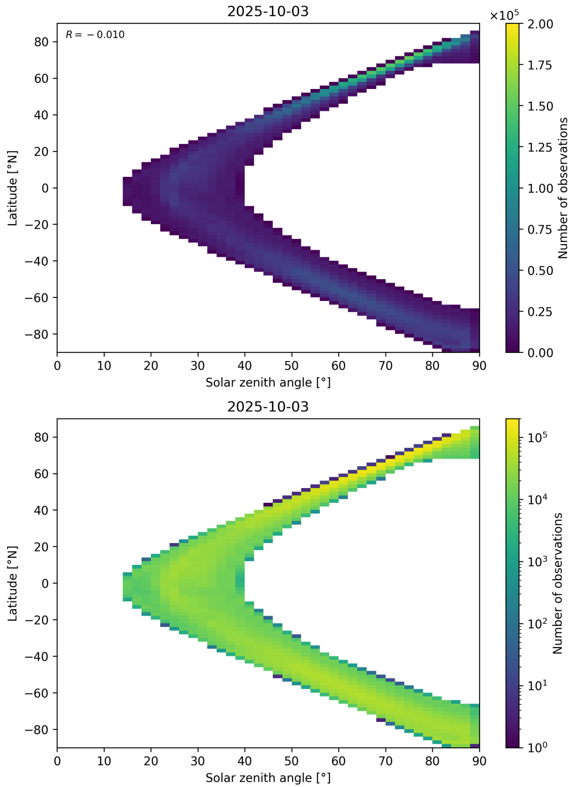
Figure 105: Scatter density plot of “Solar zenith angle” against “Latitude” for 2025-10-02 to 2025-10-04.
