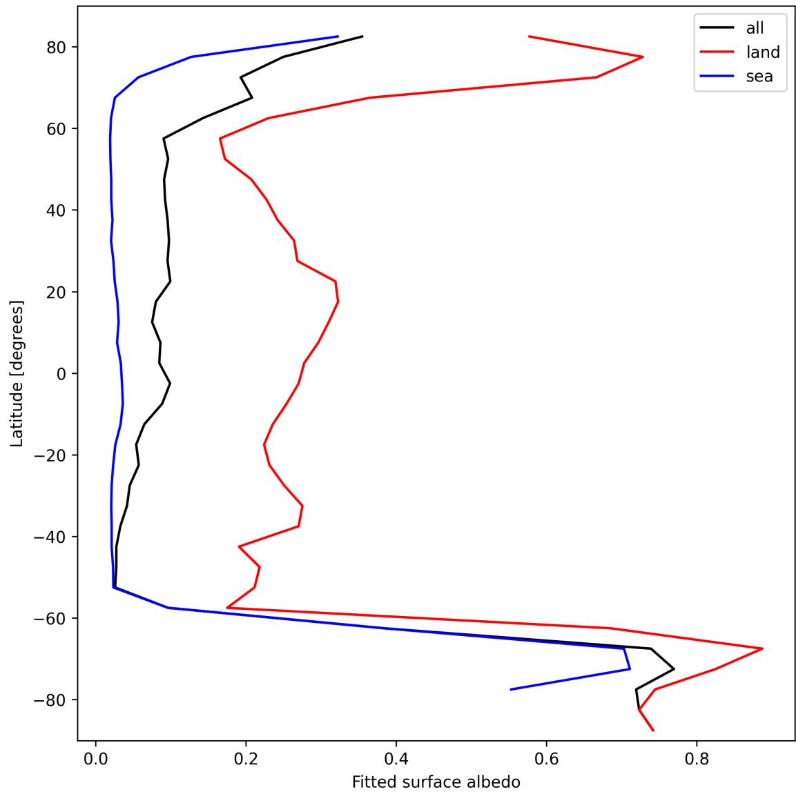
Figure 29: Zonal average of “Fitted surface albedo” for 2025-10-02 to 2025-10-04.
