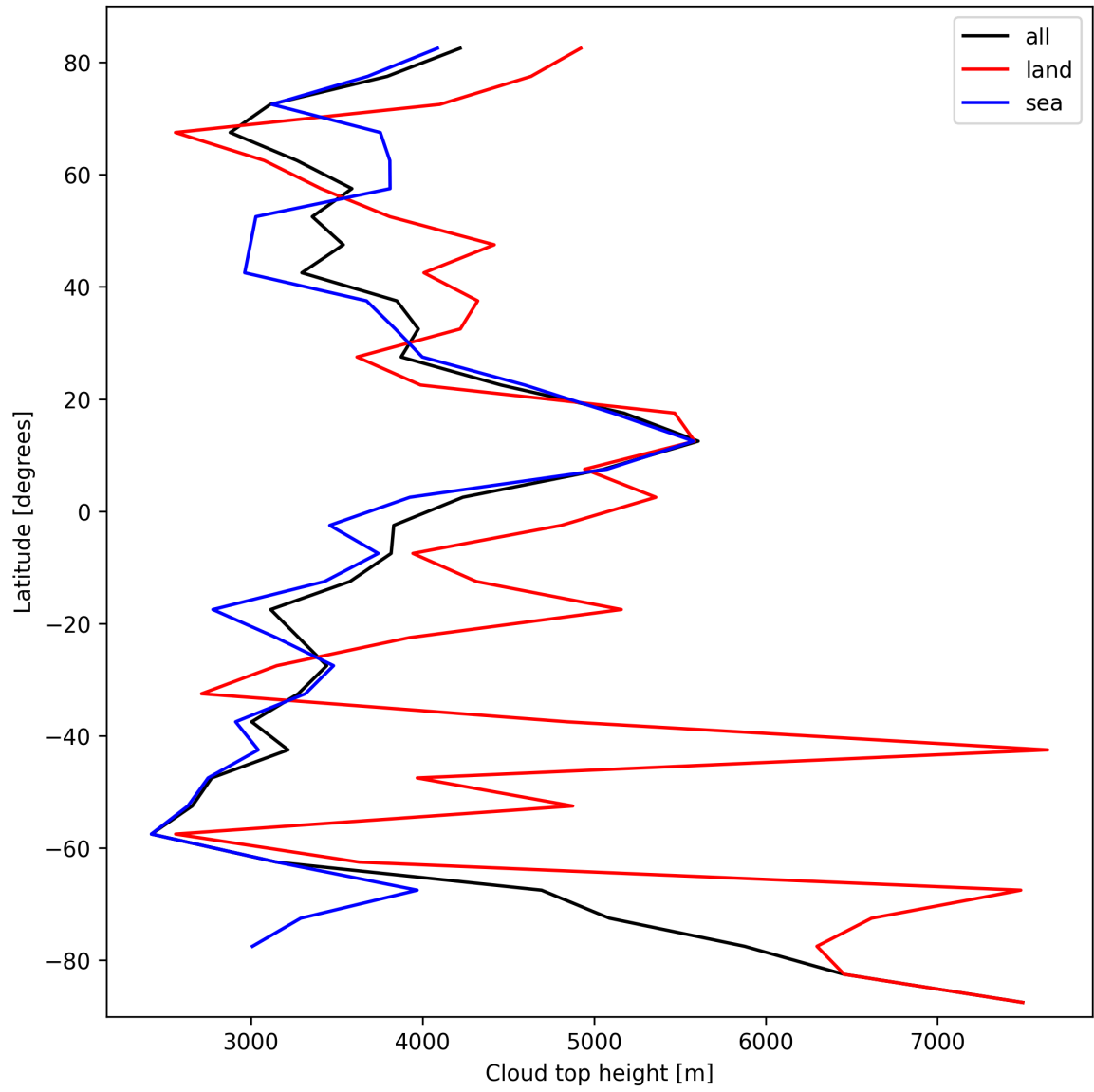
Figure 24: Zonal average of “Cloud top height” for 2025-10-02 to 2025-10-04.
