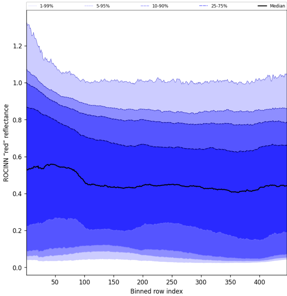
Figure 69: Along track statistics of “ROCINN “red” reflectance” for 2025-10-02 to 2025-10-04
