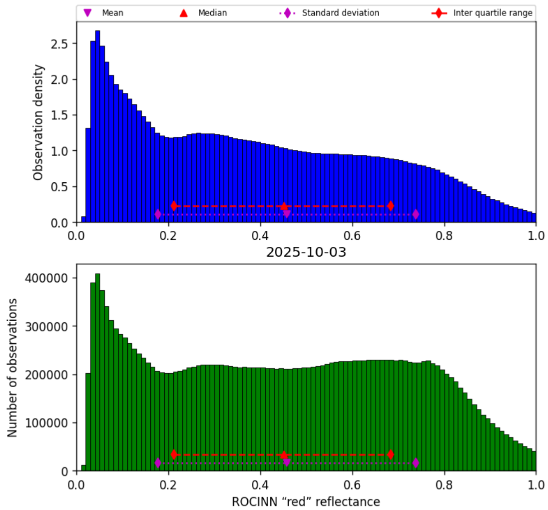
Figure 53: Histogram of “ROCINN “red” reflectance” for 2025-10-02 to 2025-10-04
