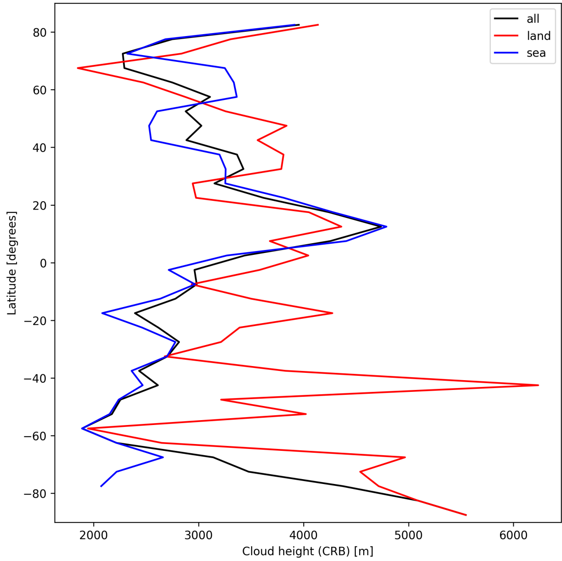
Figure 27: Zonal average of “Cloud height (CRB)” for 2025-10-02 to 2025-10-04.
