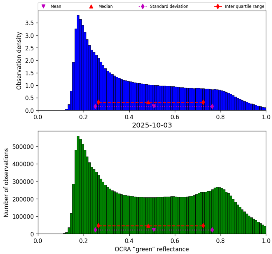
Figure 52: Histogram of “OCRA “green” reflectance” for 2025-10-02 to 2025-10-04
