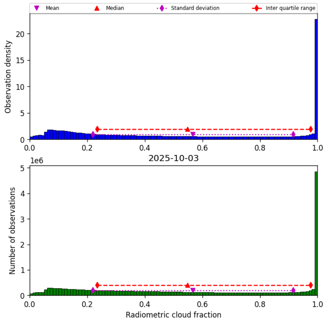
Figure 39: Histogram of "Radiometric cloud fraction" for 2025-10-02 to 2025-10-04
