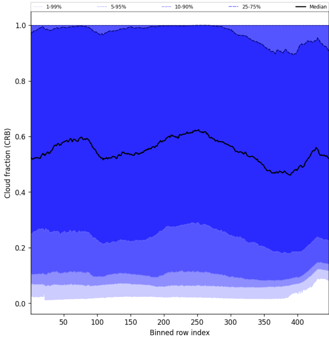
Figure 58: Along track statistics of “Cloud fraction (CRB)” for 2025-10-02 to 2025-10-04
