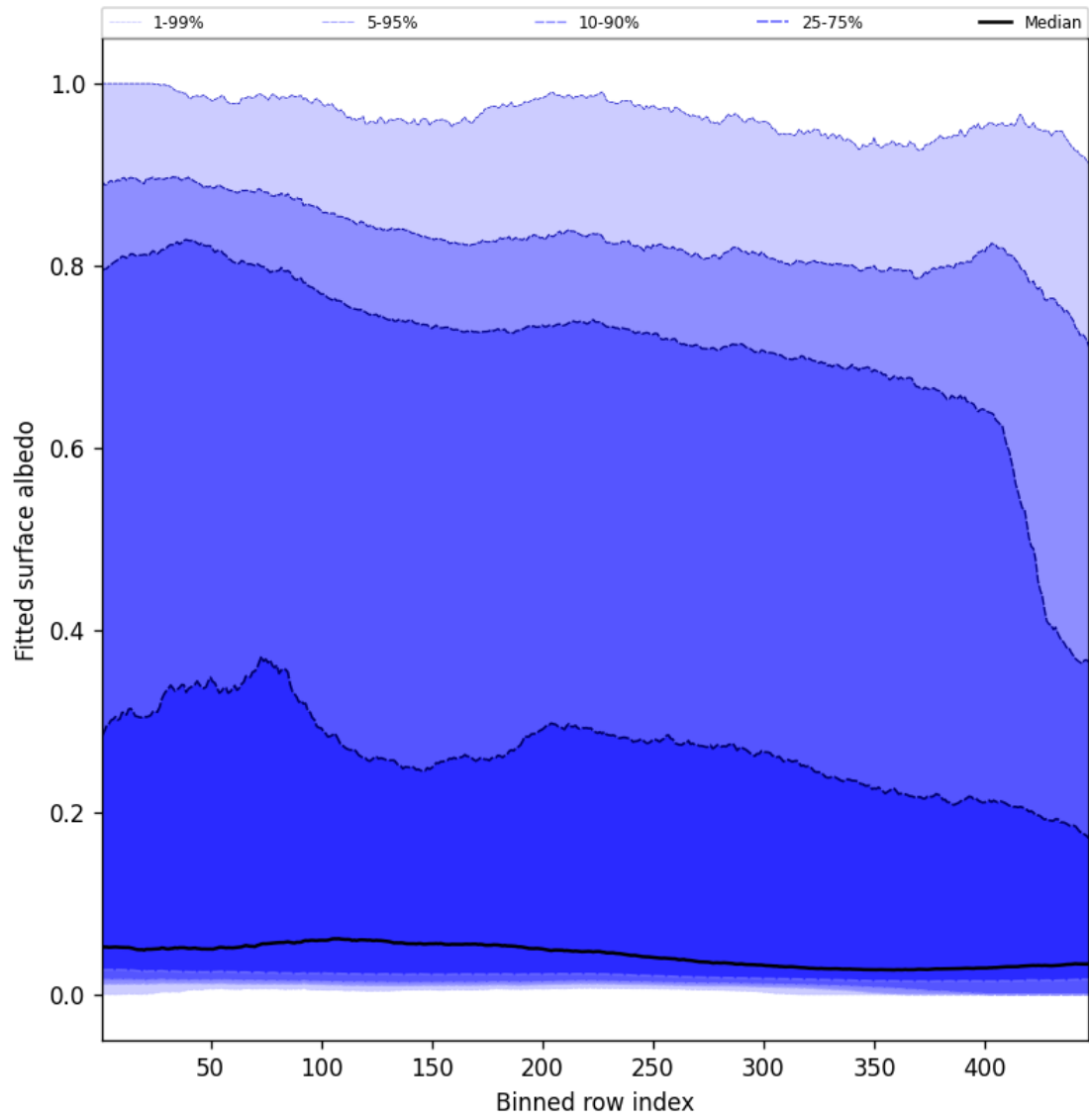
Figure 61: Along track statistics of “Fitted surface albedo” for 2025-10-02 to 2025-10-04
