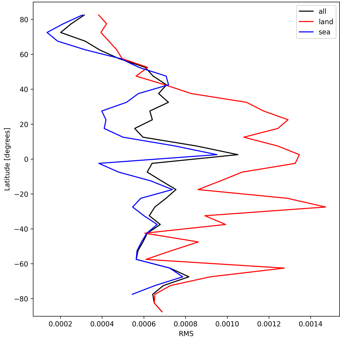
Figure 31: Zonal average of “RMS” for 2025-10-02 to 2025-10-04.
