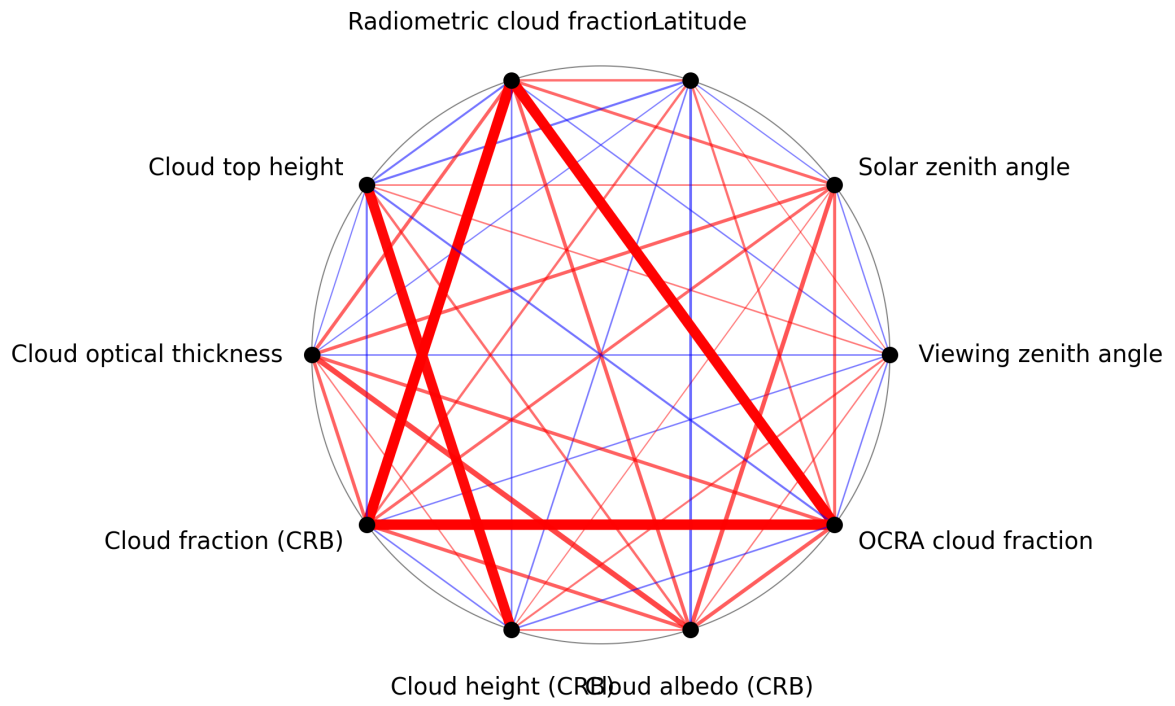
Figure 1: Map of correlation graph for 2025-10-02 to 2025-10-04.
