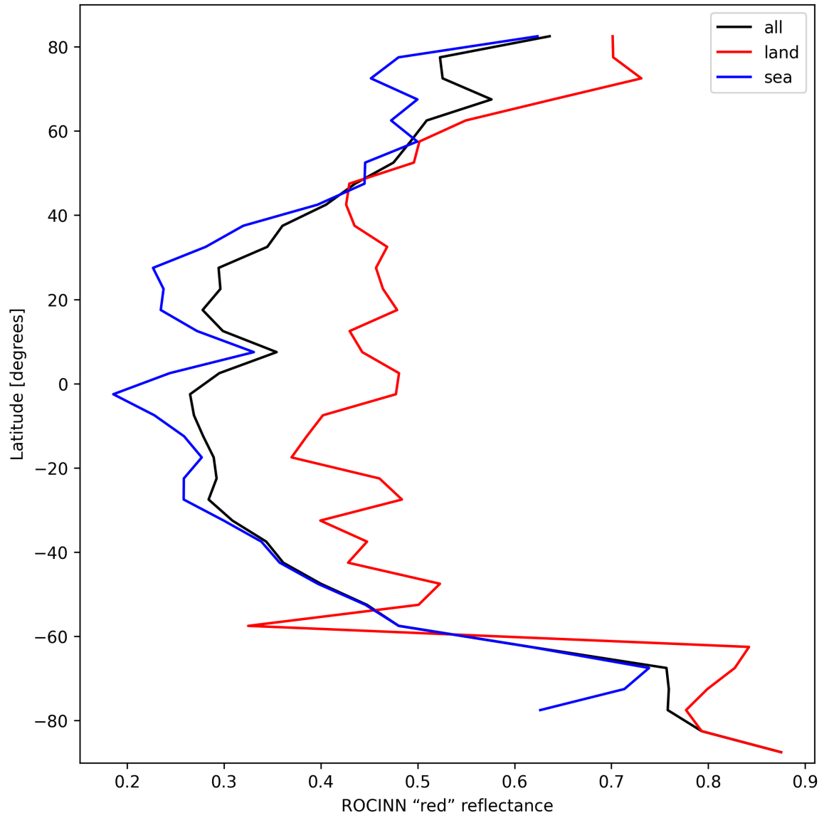
Figure 37: Zonal average of “ROCINN “red” reflectance” for 2025-10-02 to 2025-10-04.
