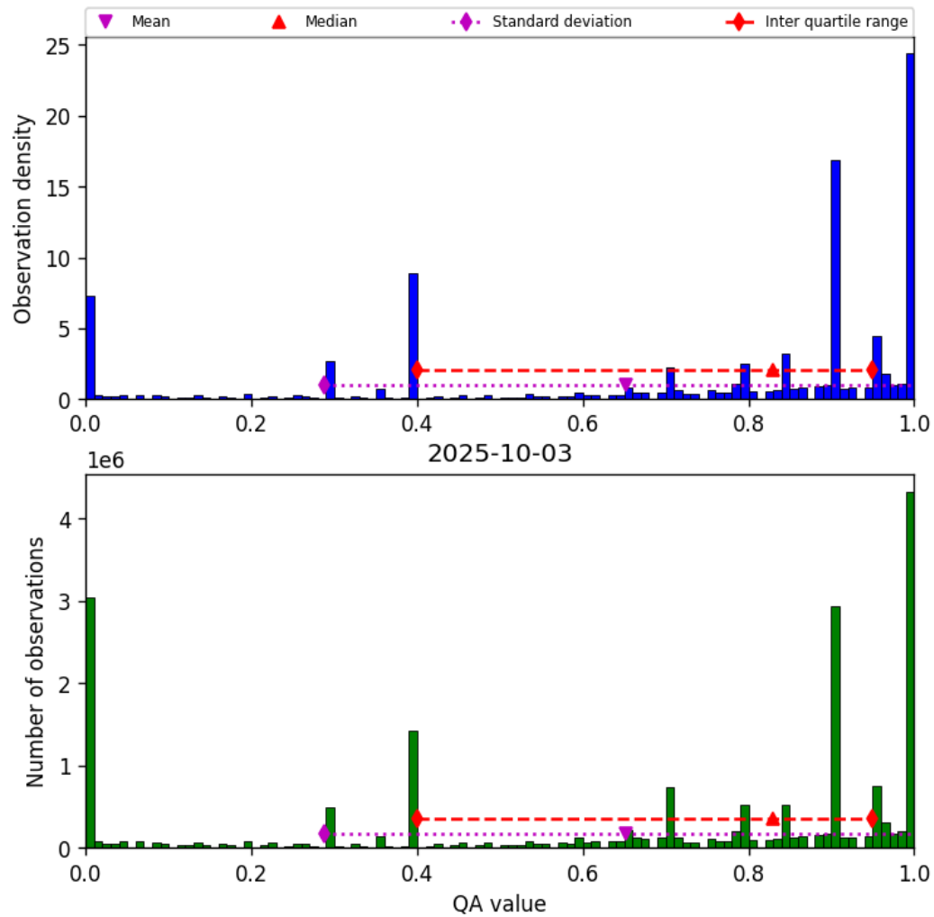
Figure 38: Histogram of “QA value” for 2025-10-02 to 2025-10-04
