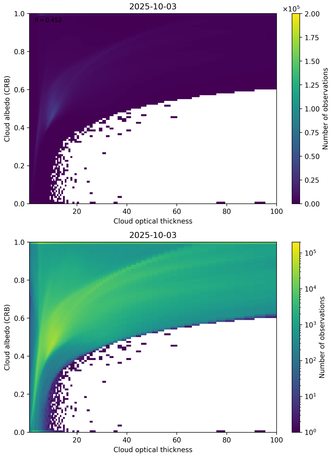
Figure 82: Scatter density plot of “Cloud optical thickness” against “Cloud albedo (CRB)” for 2025-10-02 to 2025-10-04.
