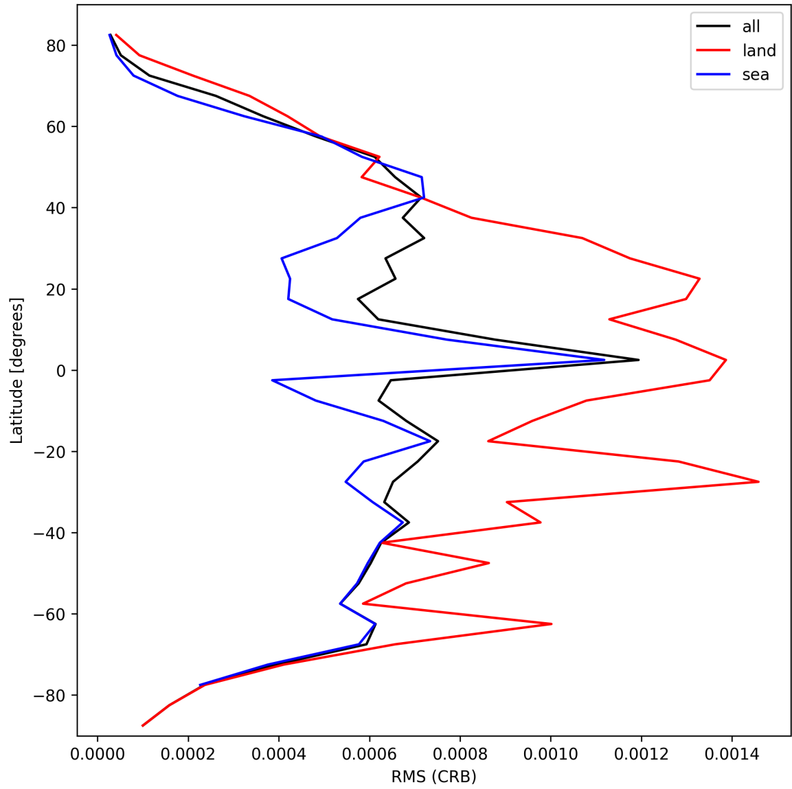
Figure 32: Zonal average of “RMS (CRB)” for 2025-10-02 to 2025-10-04.
