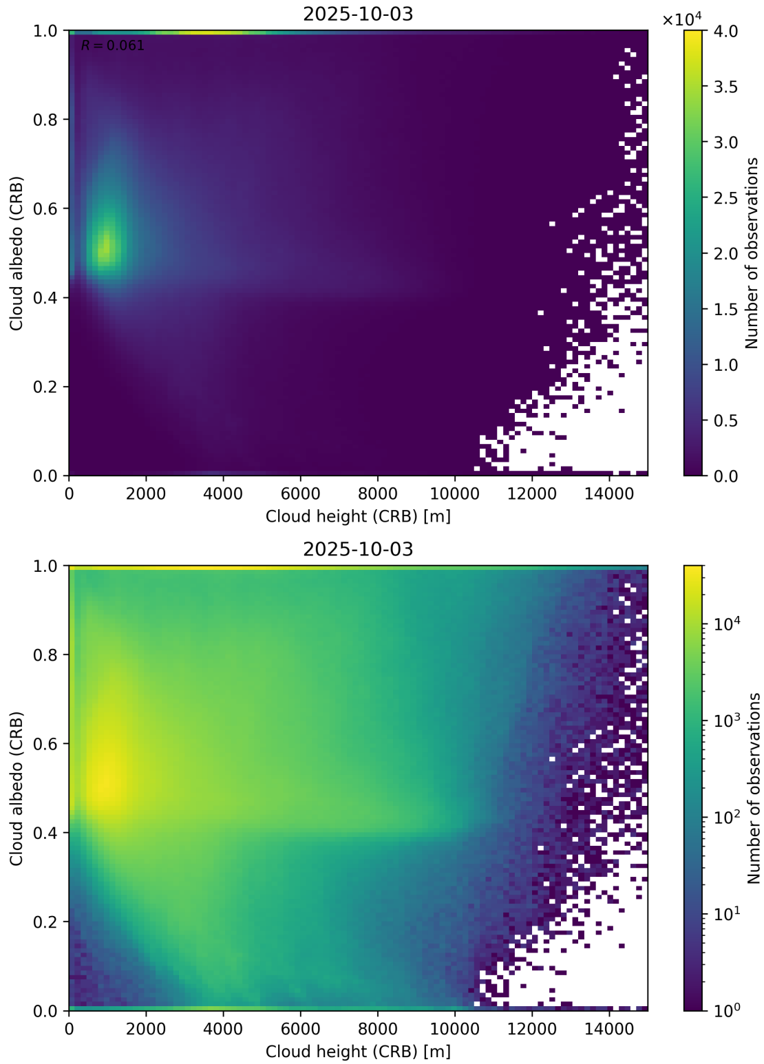
Figure 80: Scatter density plot of “Cloud height (CRB)” against “Cloud albedo (CRB)” for 2025-10-02 to 2025-10-04.
