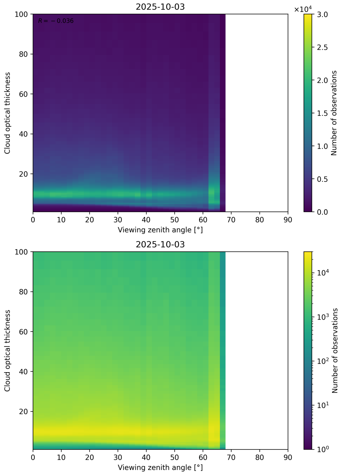
Figure 111: Scatter density plot of “Viewing zenith angle” against “Cloud optical thickness” for 2025-10-02 to 2025-10-04.
