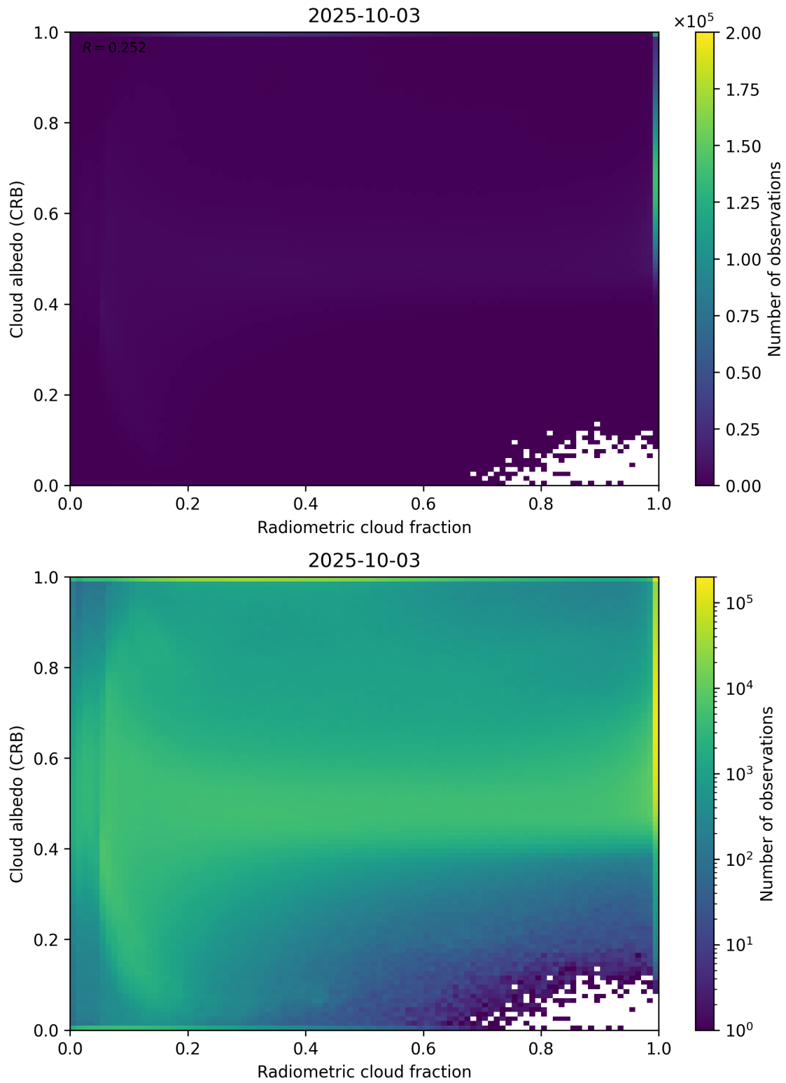
Figure 71: Scatter density plot of “Radiometric cloud fraction” against “Cloud albedo (CRB)” for 2025-10-02 to 2025-10-04.
