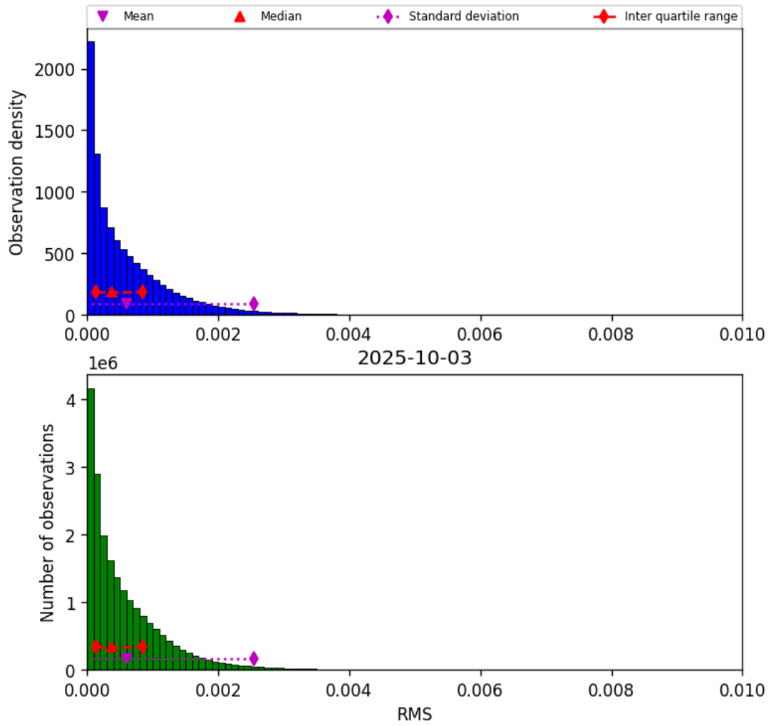
Figure 47: Histogram of “RMS” for 2025-10-02 to 2025-10-04
