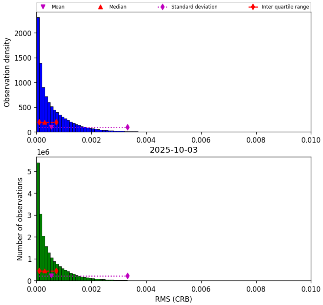
Figure 48: Histogram of “RMS (CRB)” for 2025-10-02 to 2025-10-04
