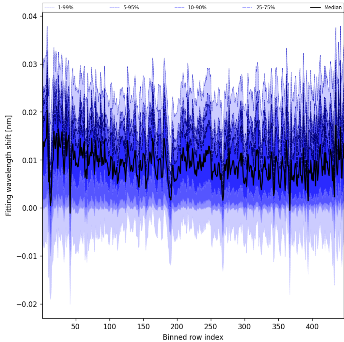
Figure 65: Along track statistics of “Fitting wavelength shift” for 2025-10-02 to 2025-10-04
