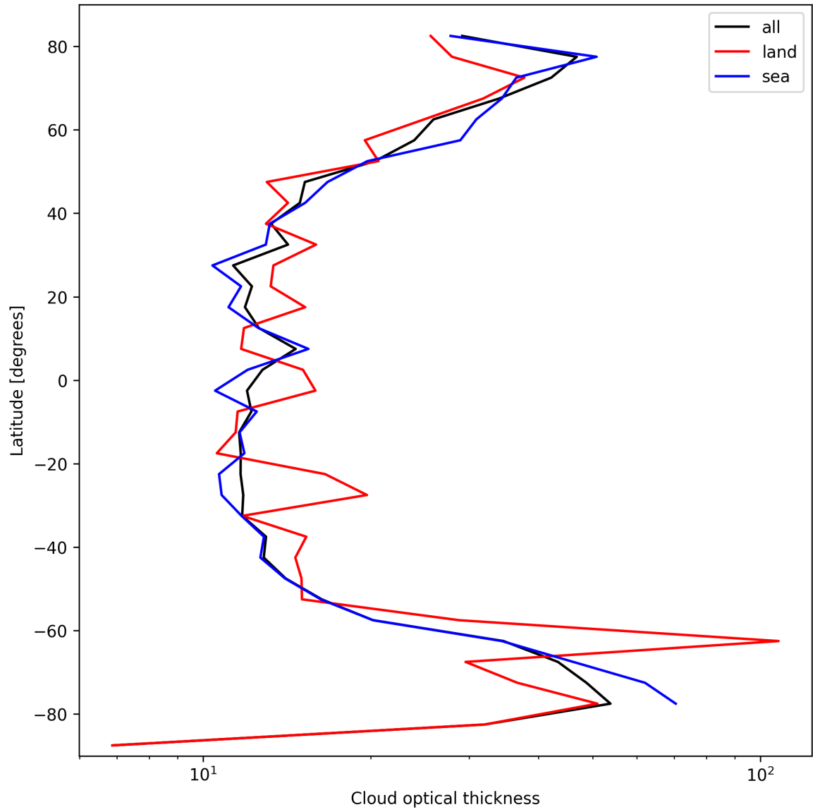
Figure 25: Zonal average of “Cloud optical thickness” for 2025-10-02 to 2025-10-04.
