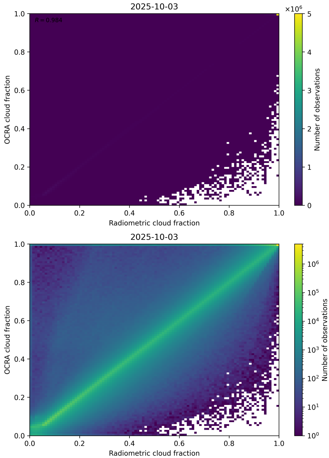
Figure 72: Scatter density plot of “Radiometric cloud fraction” against “OCRA cloud fraction” for 2025-10-02 to 2025-10-04.
