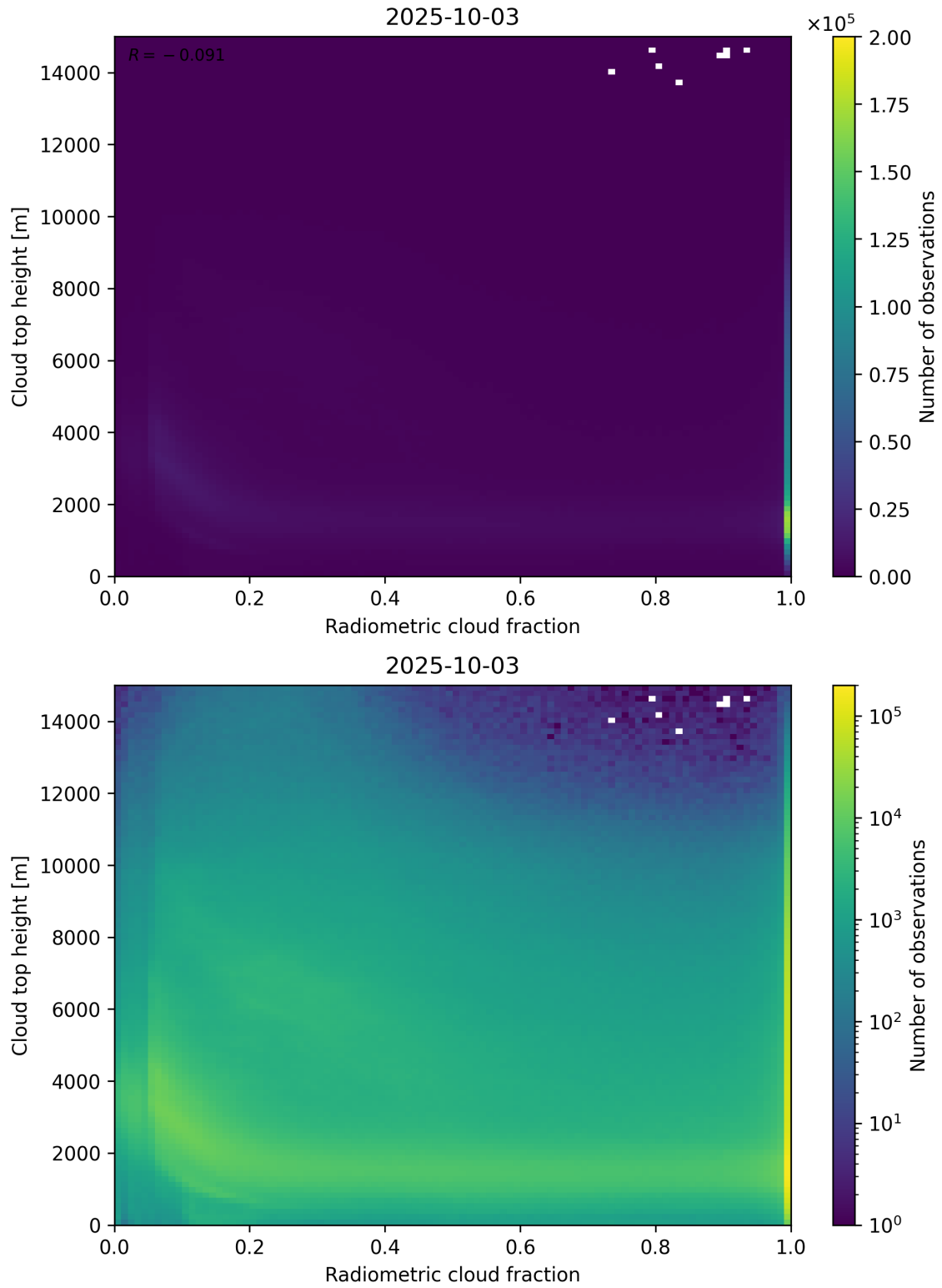
Figure 76: Scatter density plot of “Radiometric cloud fraction” against “Cloud top height” for 2025-10-02 to 2025-10-04.
