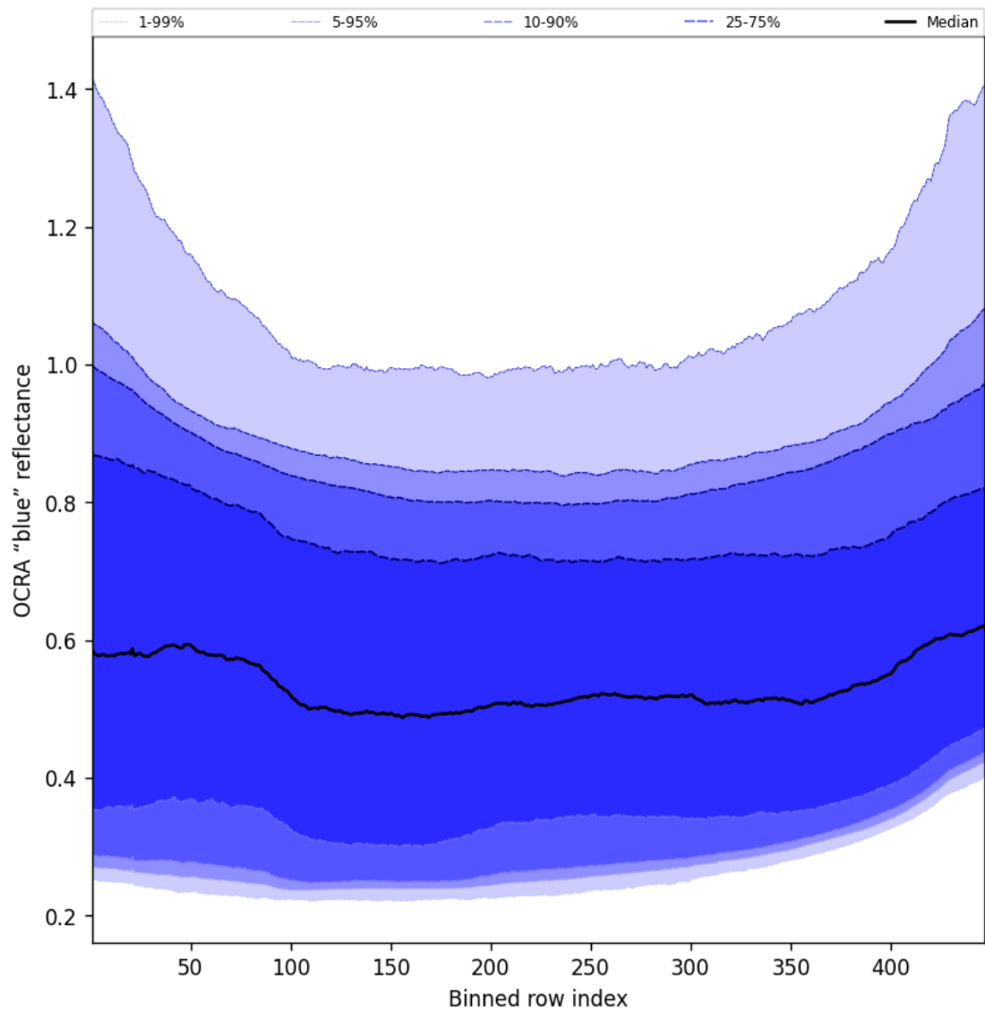
Figure 67: Along track statistics of “OCRA “blue” reflectance” for 2025-10-02 to 2025-10-04
