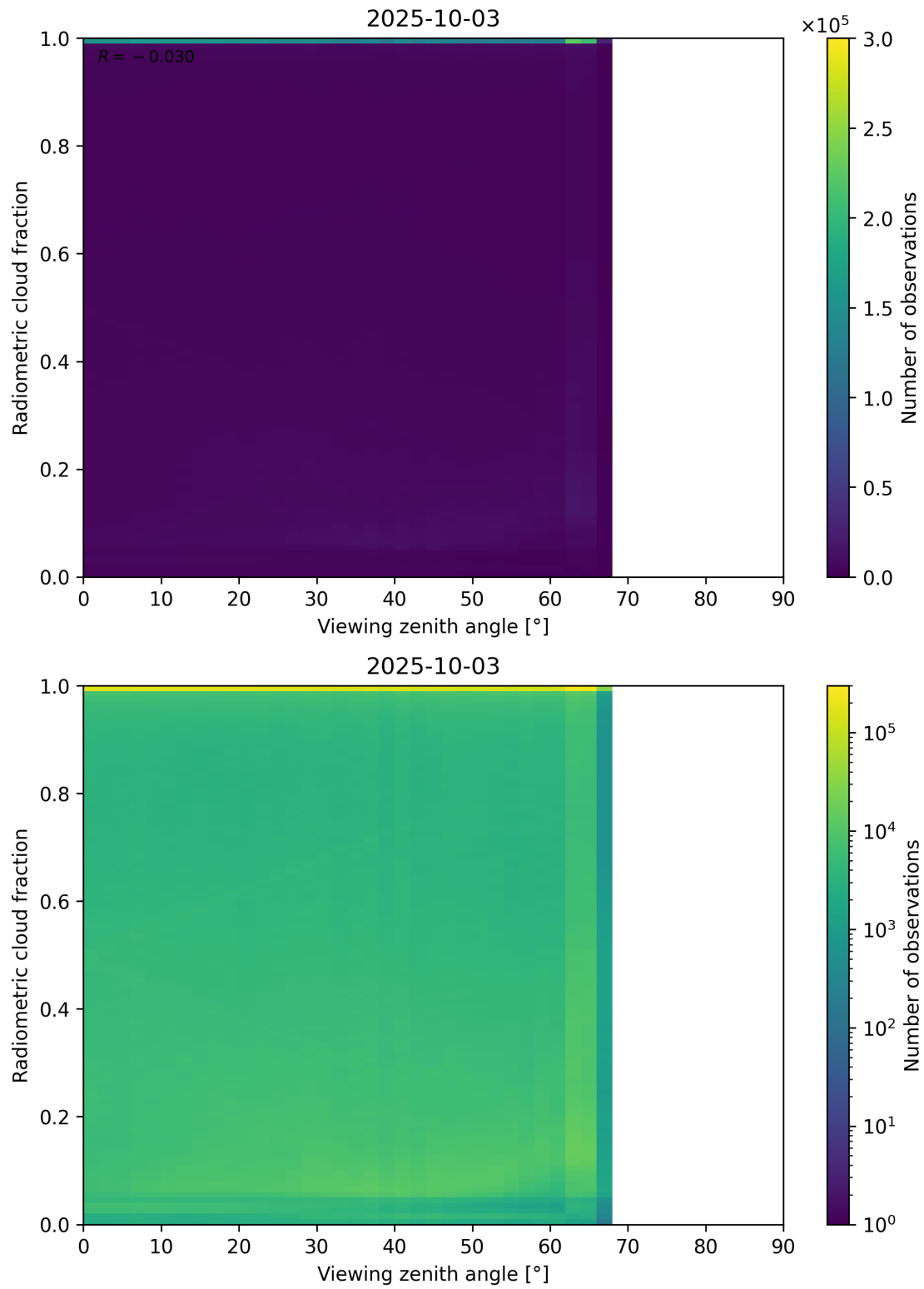
Figure 107: Scatter density plot of “Viewing zenith angle” against “Radiometric cloud fraction” for 2025-10-02 to 2025-10-04.
