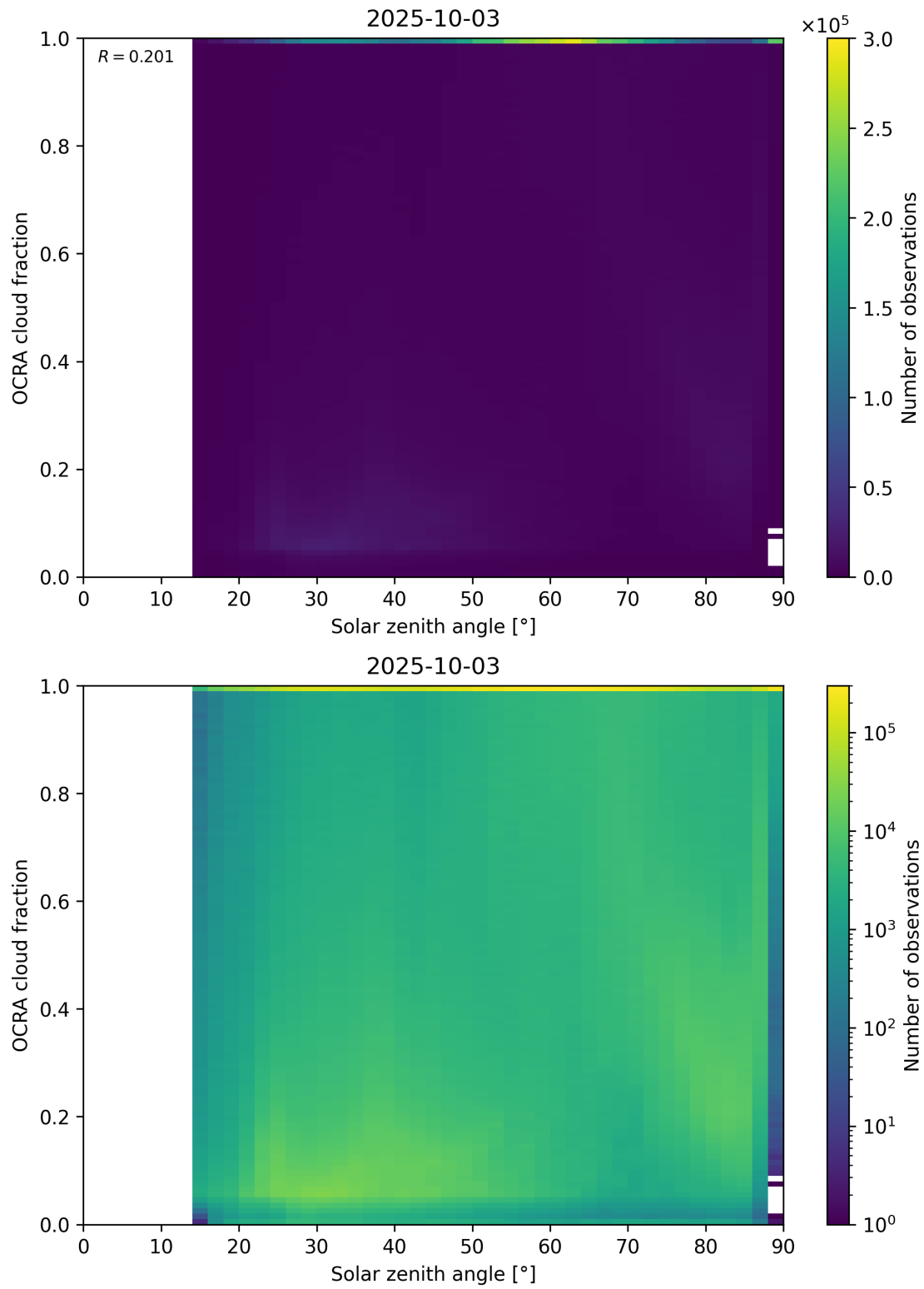
Figure 100: Scatter density plot of “Solar zenith angle” against “OCRA cloud fraction” for 2025-10-02 to 2025-10-04.
