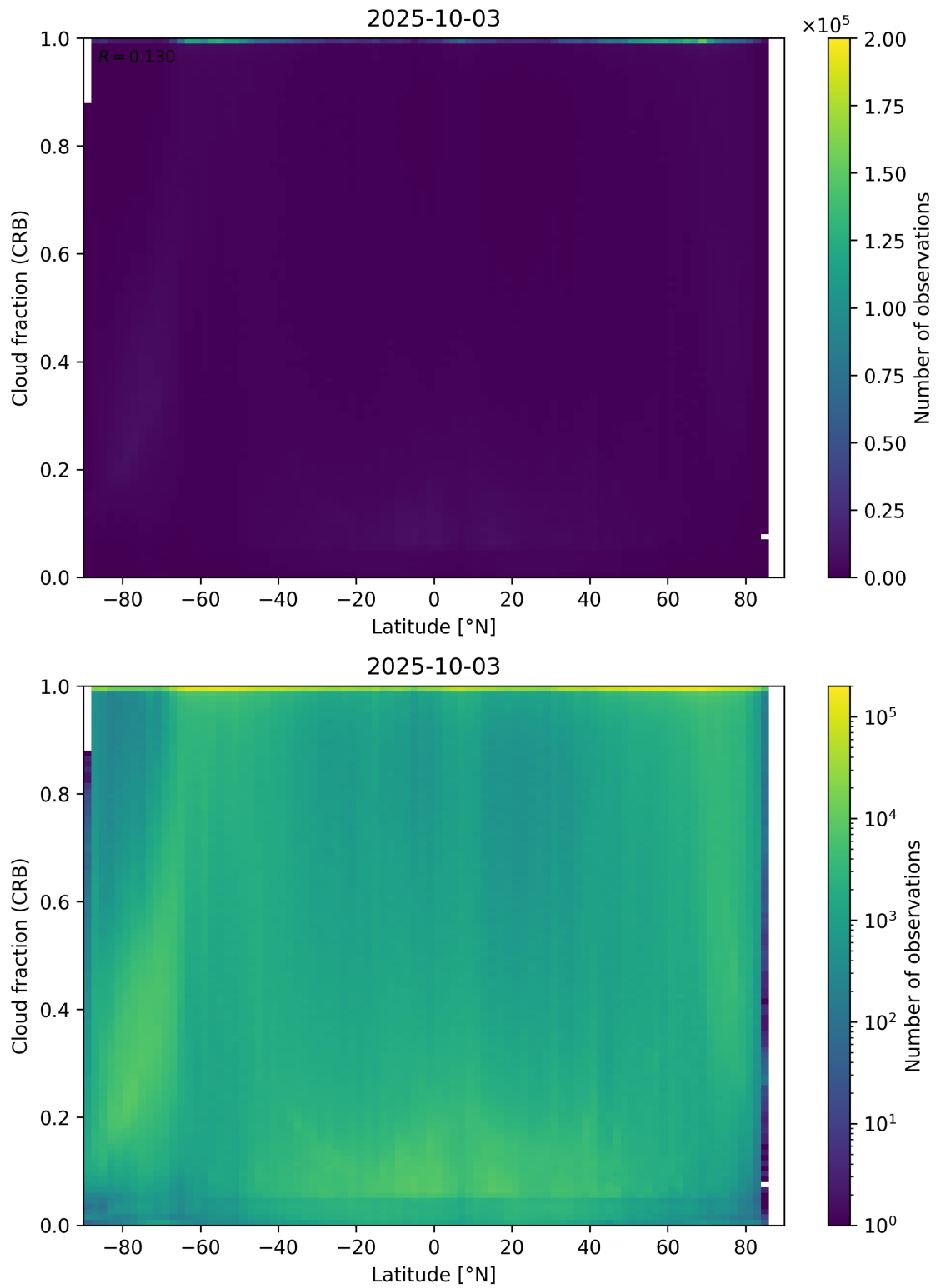
Figure 94: Scatter density plot of “Latitude” against “Cloud fraction (CRB)” for 2025-10-02 to 2025-10-04.
