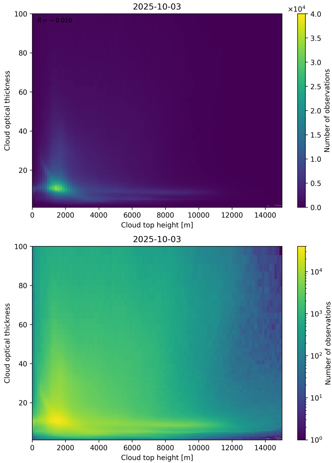
Figure 90: Scatter density plot of “Cloud top height” against “Cloud optical thickness” for 2025-10-02 to 2025-10-04.
