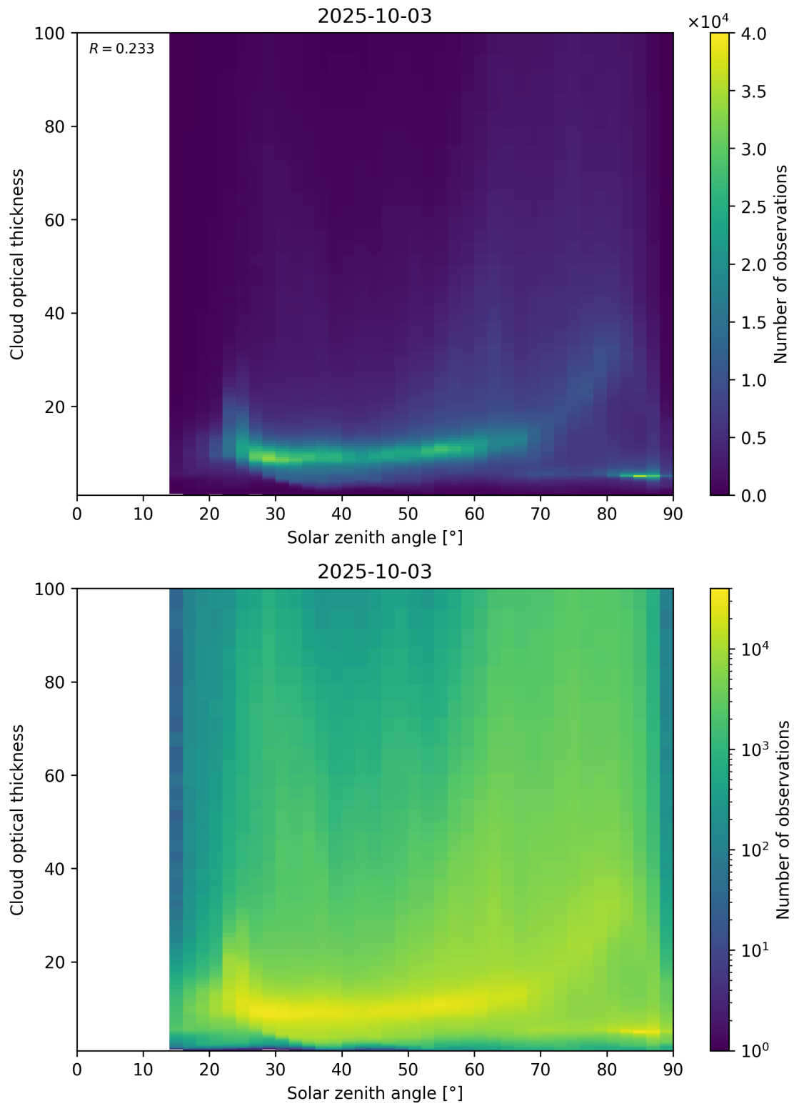
Figure 103: Scatter density plot of “Solar zenith angle” against “Cloud optical thickness” for 2025-10-02 to 2025-10-04.
