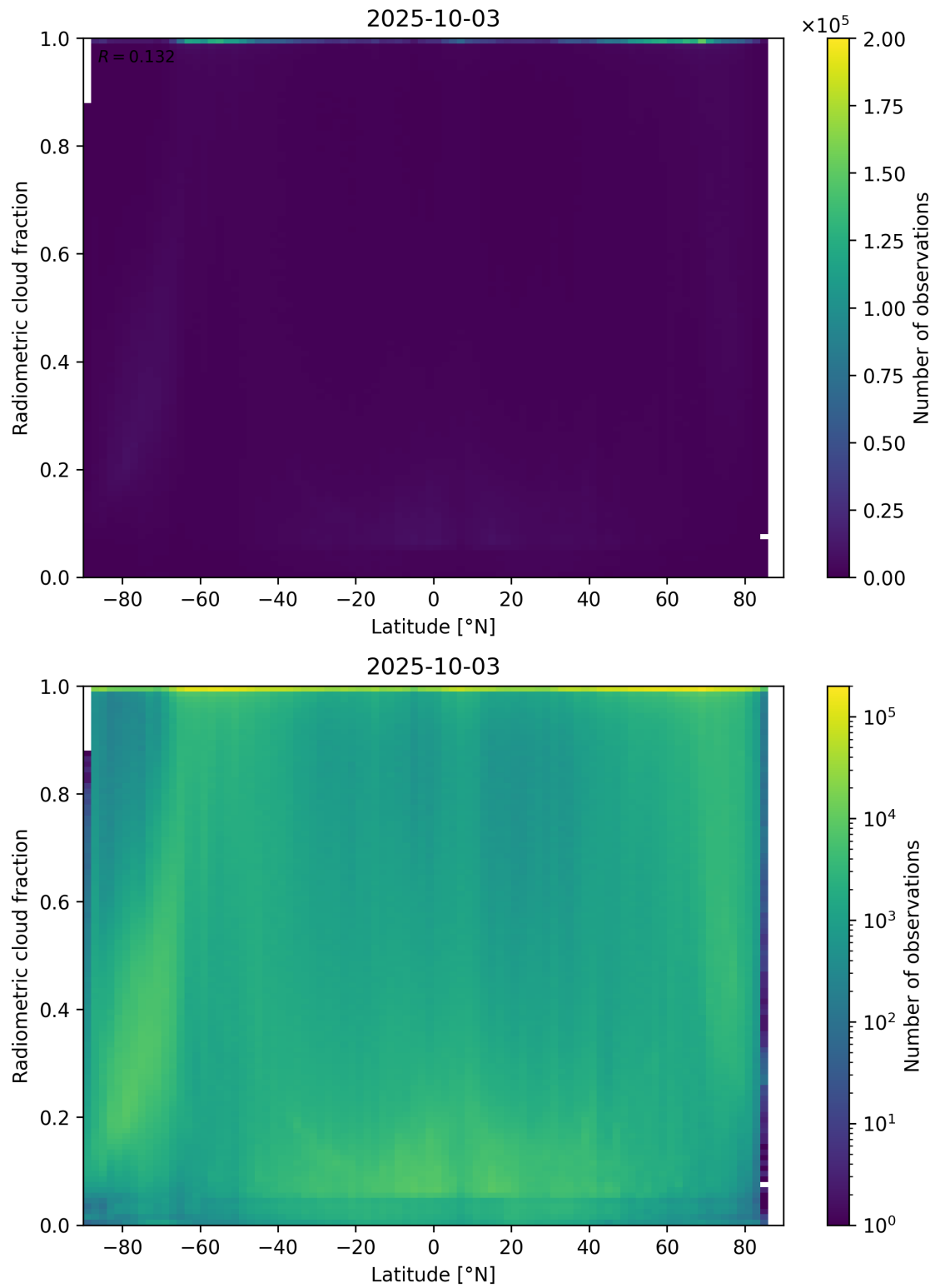
Figure 92: Scatter density plot of “Latitude” against “Radiometric cloud fraction” for 2025-10-02 to 2025-10-04.
