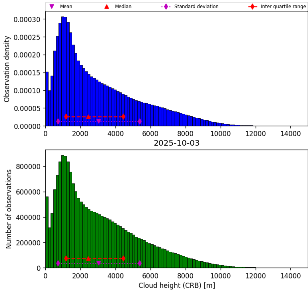
Figure 43: Histogram of “Cloud height (CRB)” for 2025-10-02 to 2025-10-04
