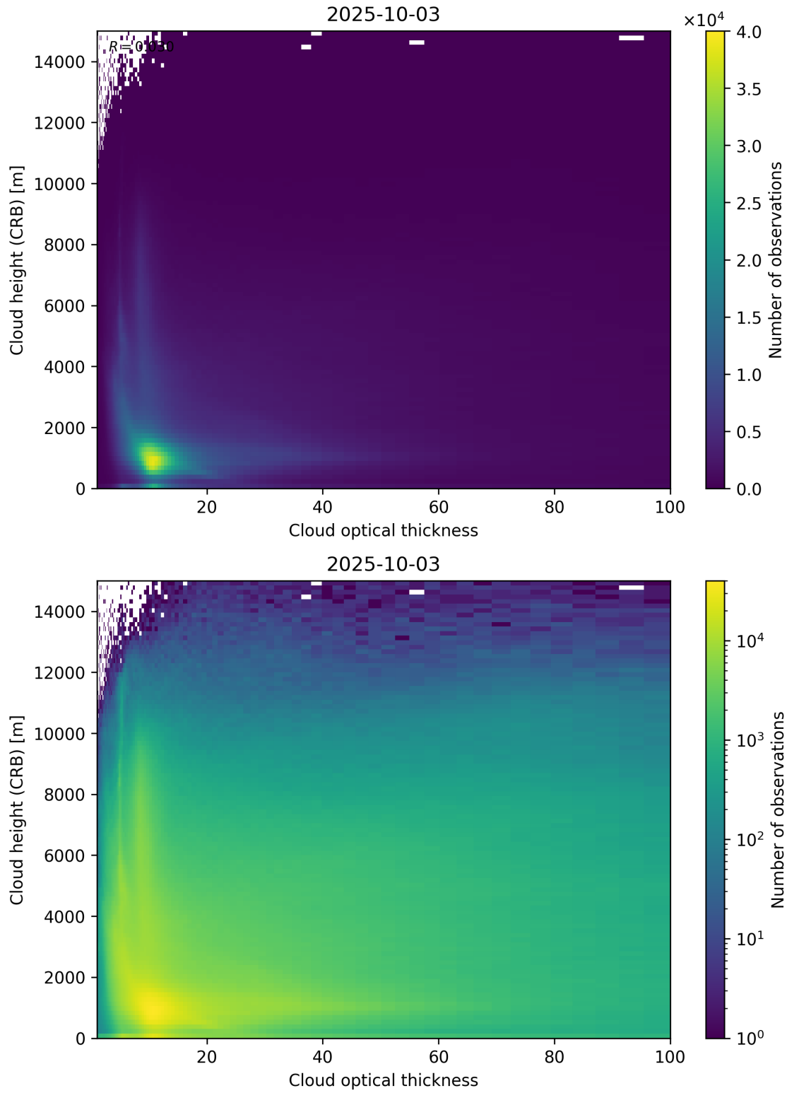
Figure 85: Scatter density plot of “Cloud optical thickness” against “Cloud height (CRB)” for 2025-10-02 to 2025-10-04.
