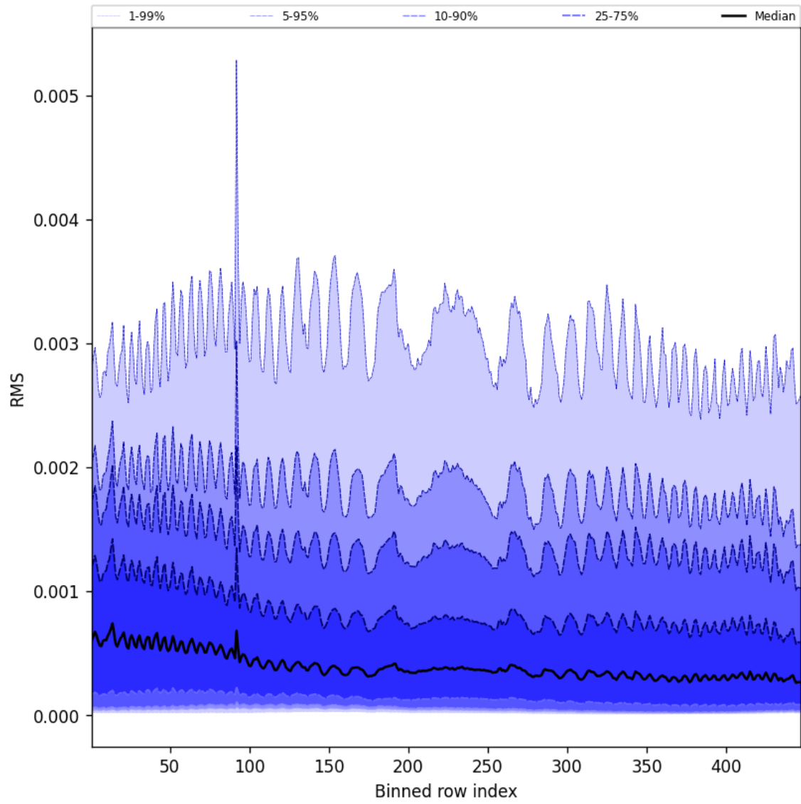
Figure 63: Along track statistics of “RMS” for 2025-10-02 to 2025-10-04
