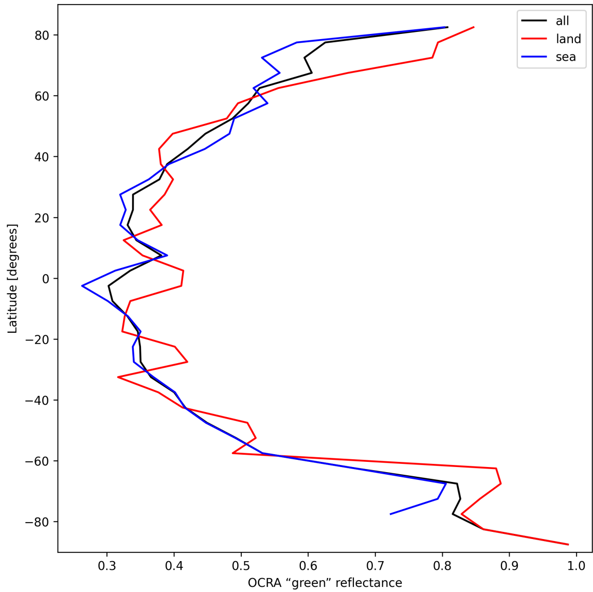
Figure 36: Zonal average of “OCRA “green” reflectance” for 2025-10-02 to 2025-10-04.
