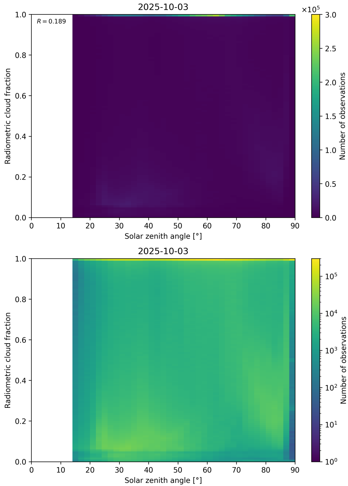
Figure 99: Scatter density plot of “Solar zenith angle” against “Radiometric cloud fraction” for 2025-10-02 to 2025-10-04.
