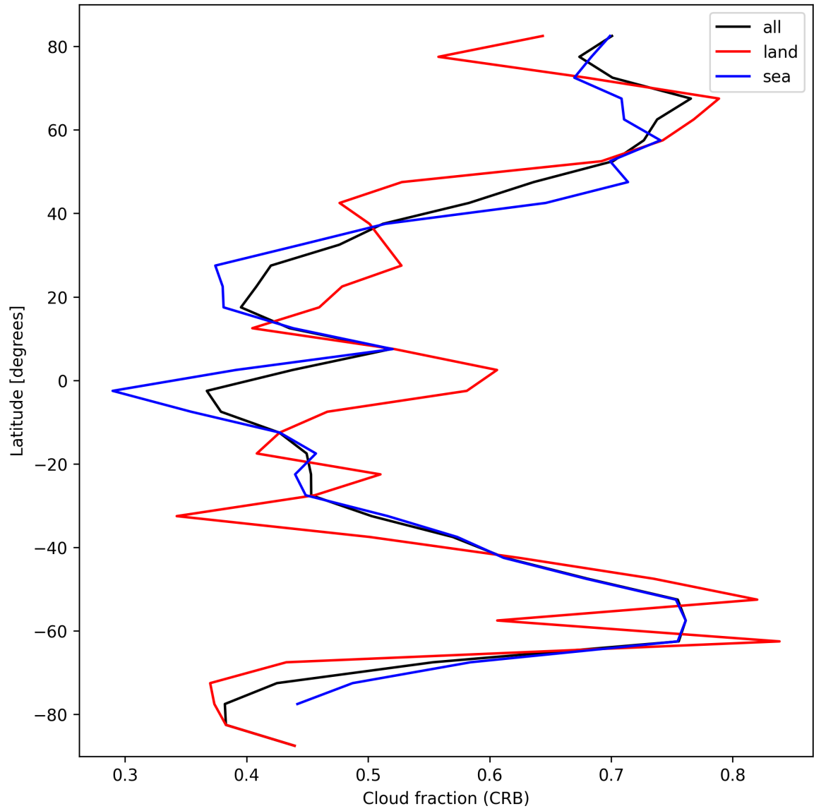
Figure 26: Zonal average of “Cloud fraction (CRB)” for 2025-10-02 to 2025-10-04.
