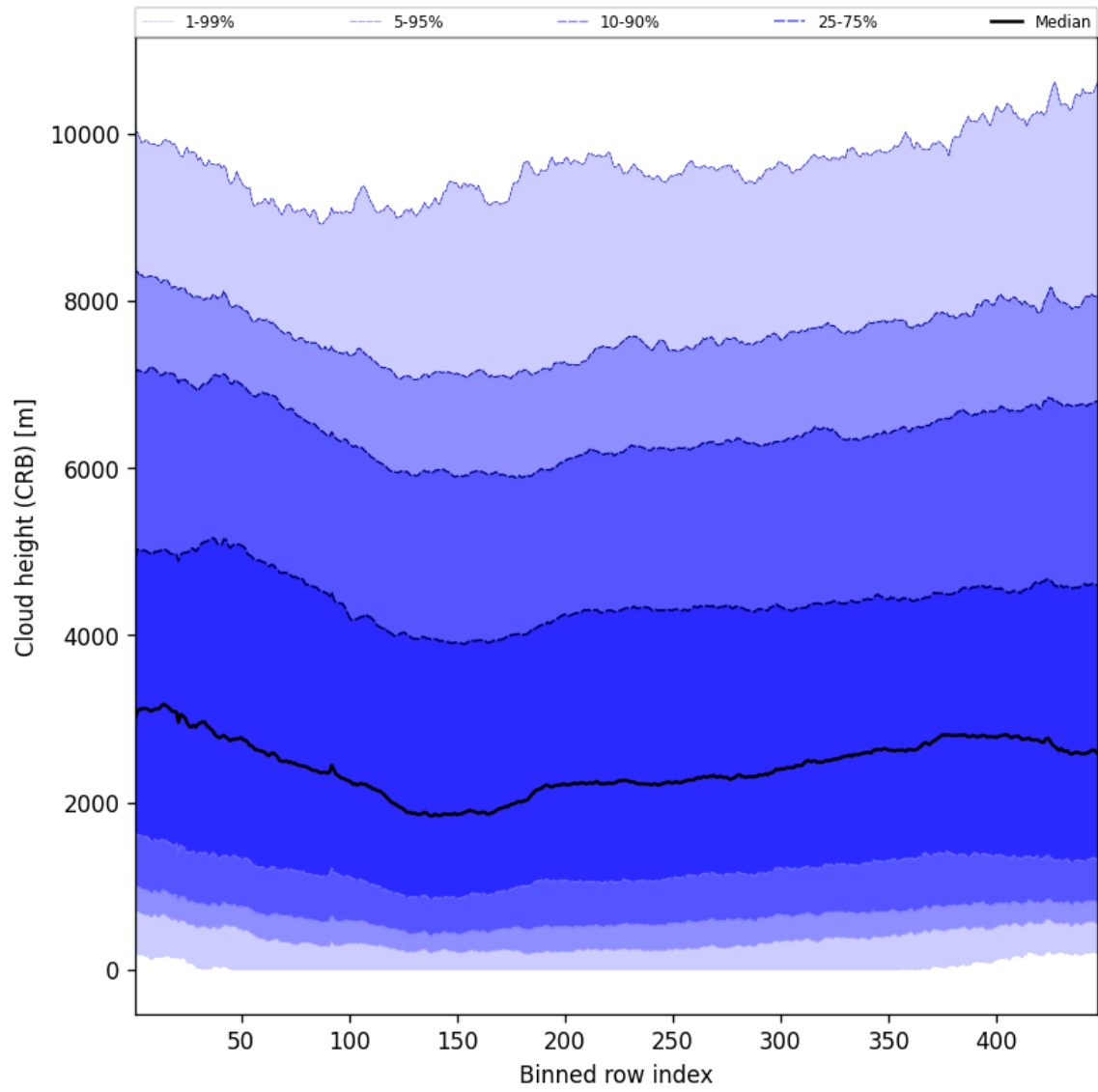
Figure 59: Along track statistics of “Cloud height (CRB)” for 2025-10-02 to 2025-10-04
