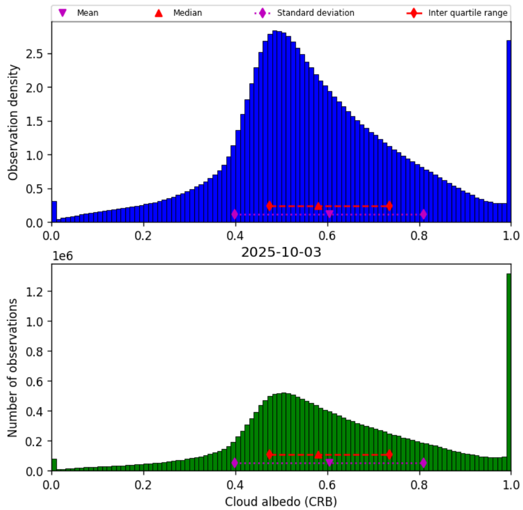
Figure 44: Histogram of “Cloud albedo (CRB)” for 2025-10-02 to 2025-10-04
