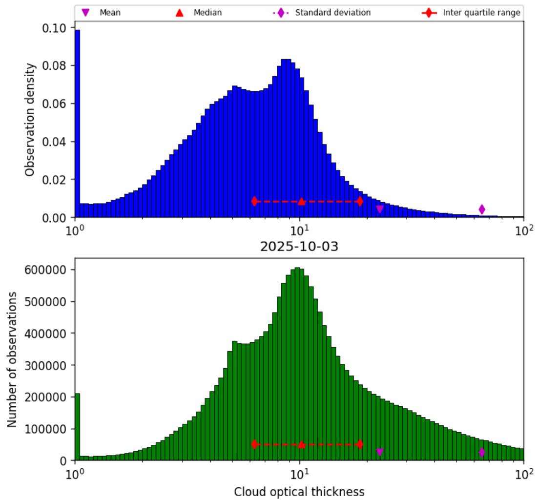
Figure 41: Histogram of “Cloud optical thickness” for 2025-10-02 to 2025-10-04
