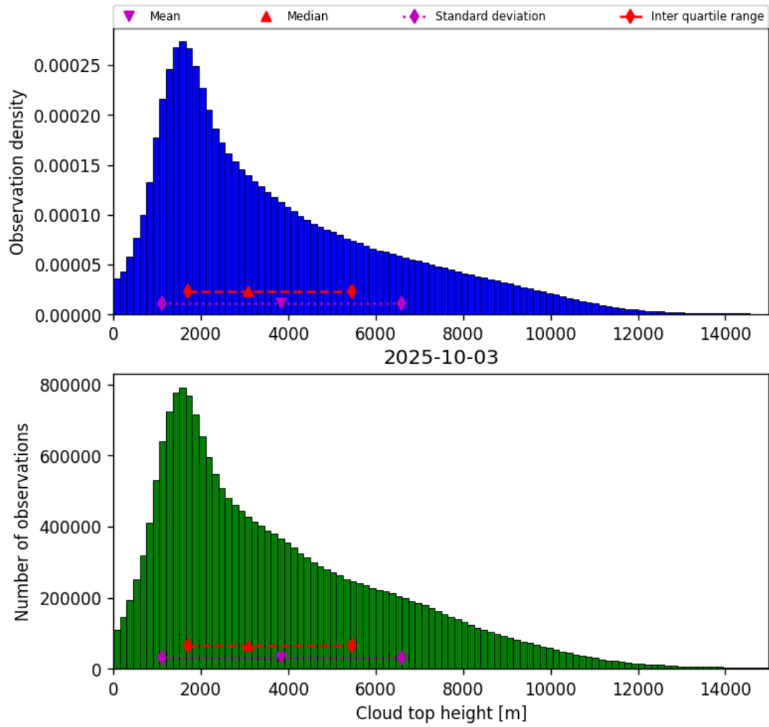
Figure 40: Histogram of “Cloud top height” for 2025-10-02 to 2025-10-04
