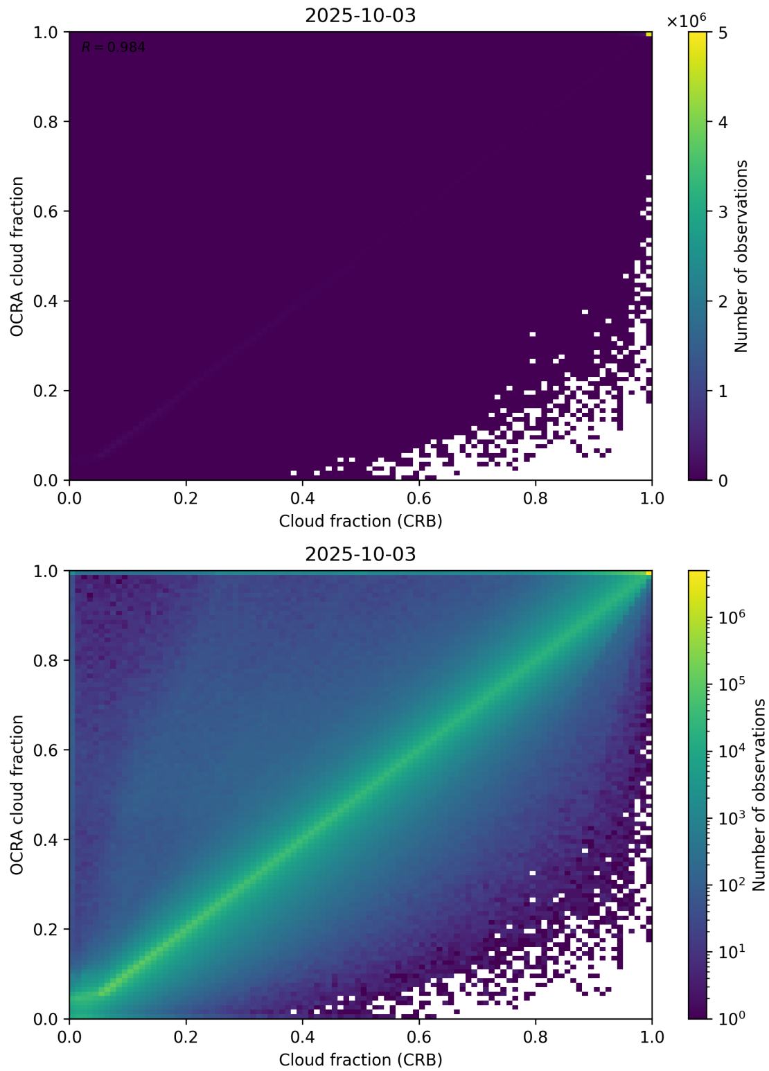
Figure 78: Scatter density plot of “Cloud fraction (CRB)” against “OCRA cloud fraction” for 2025-10-02 to 2025-10-04.
