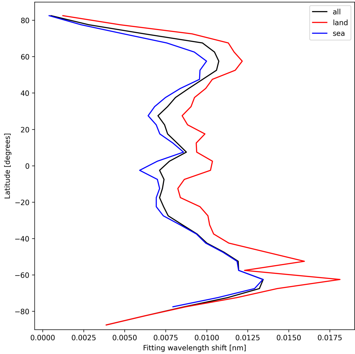
Figure 33: Zonal average of “Fitting wavelength shift” for 2025-10-02 to 2025-10-04.
