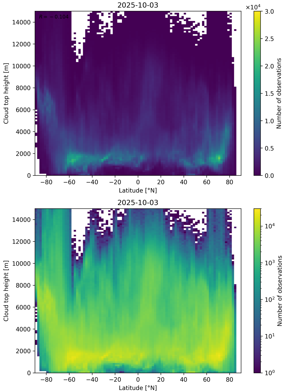
Figure 97: Scatter density plot of “Latitude” against “Cloud top height” for 2025-10-02 to 2025-10-04.
