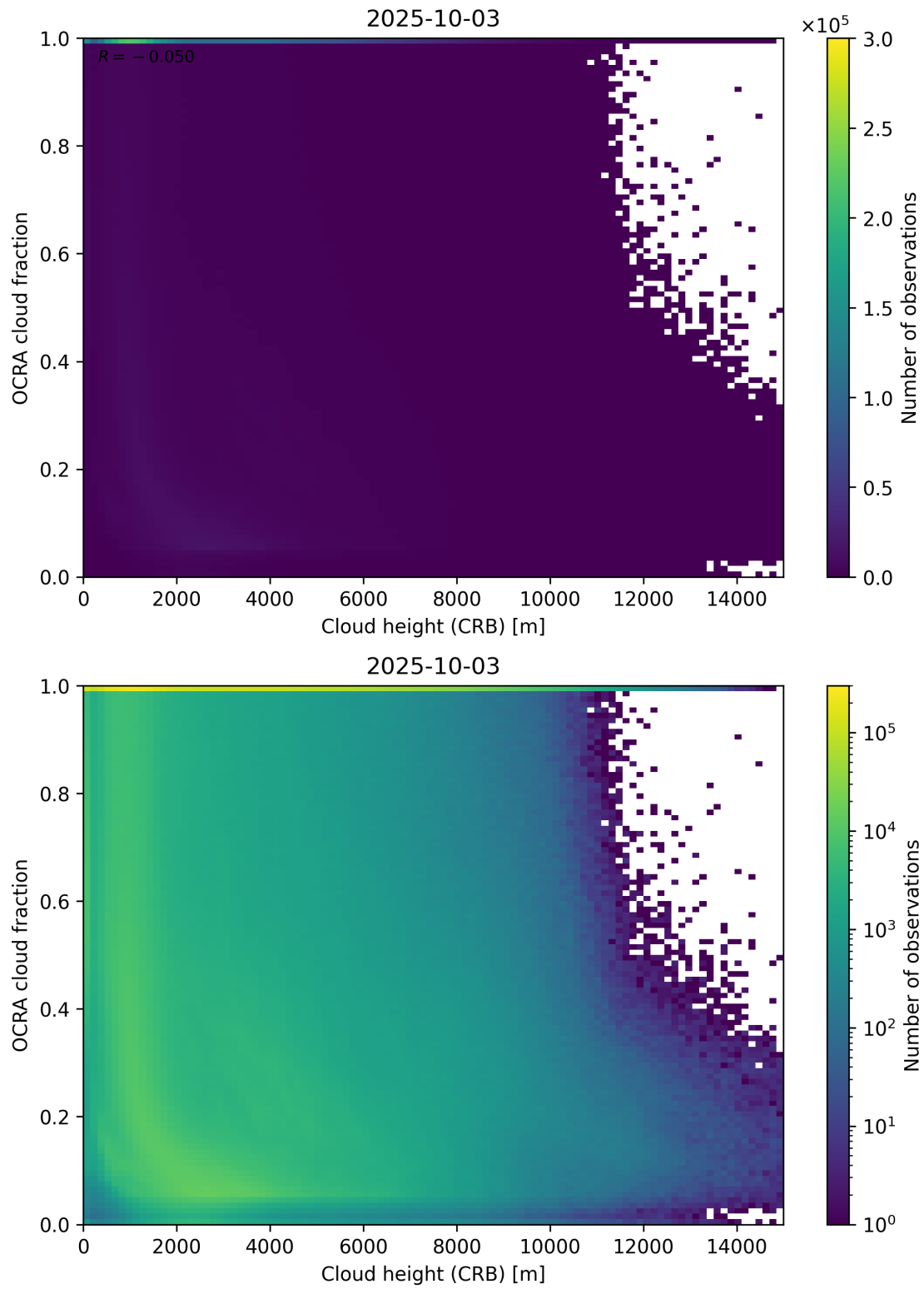
Figure 81: Scatter density plot of “Cloud height (CRB)” against “OCRA cloud fraction” for 2025-10-02 to 2025-10-04.
