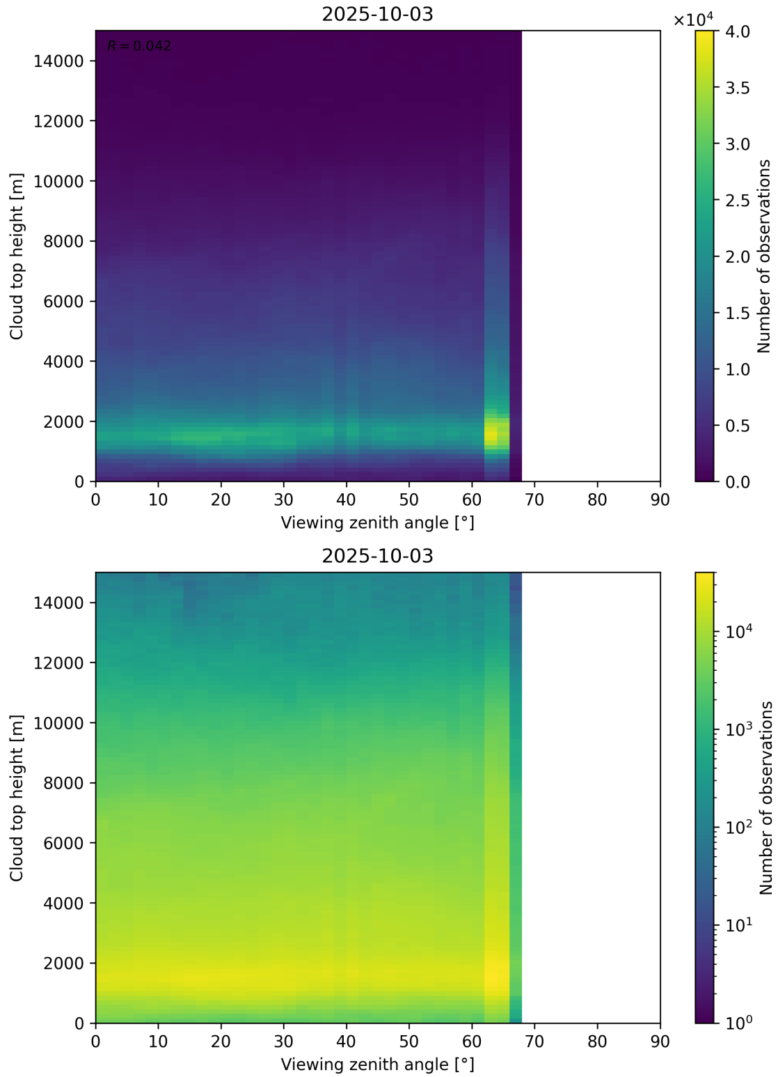
Figure 112: Scatter density plot of “Viewing zenith angle” against “Cloud top height” for 2025-10-02 to 2025-10-04.
