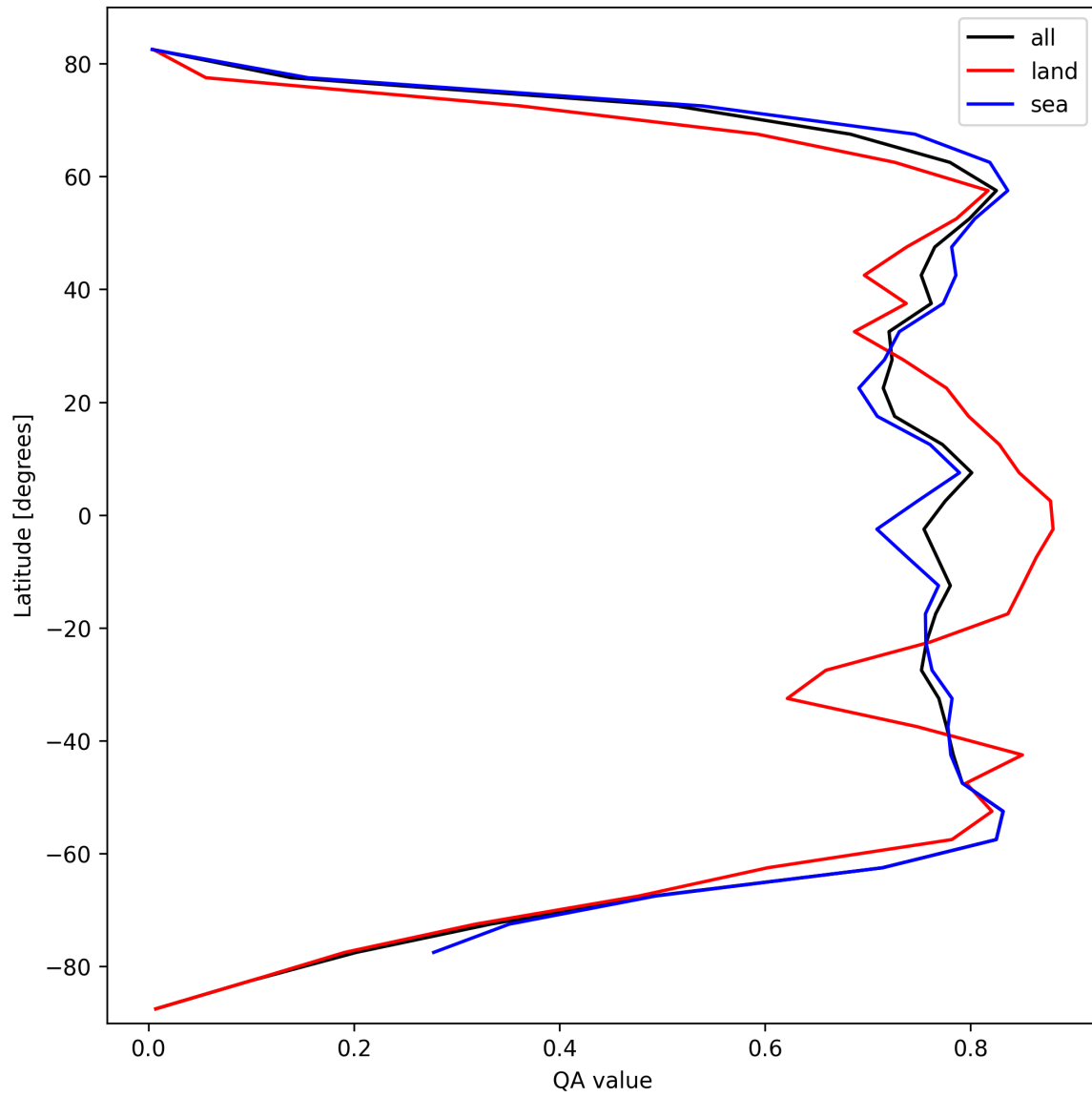
Figure 22: Zonal average of “QA value” for 2025-10-02 to 2025-10-04.
