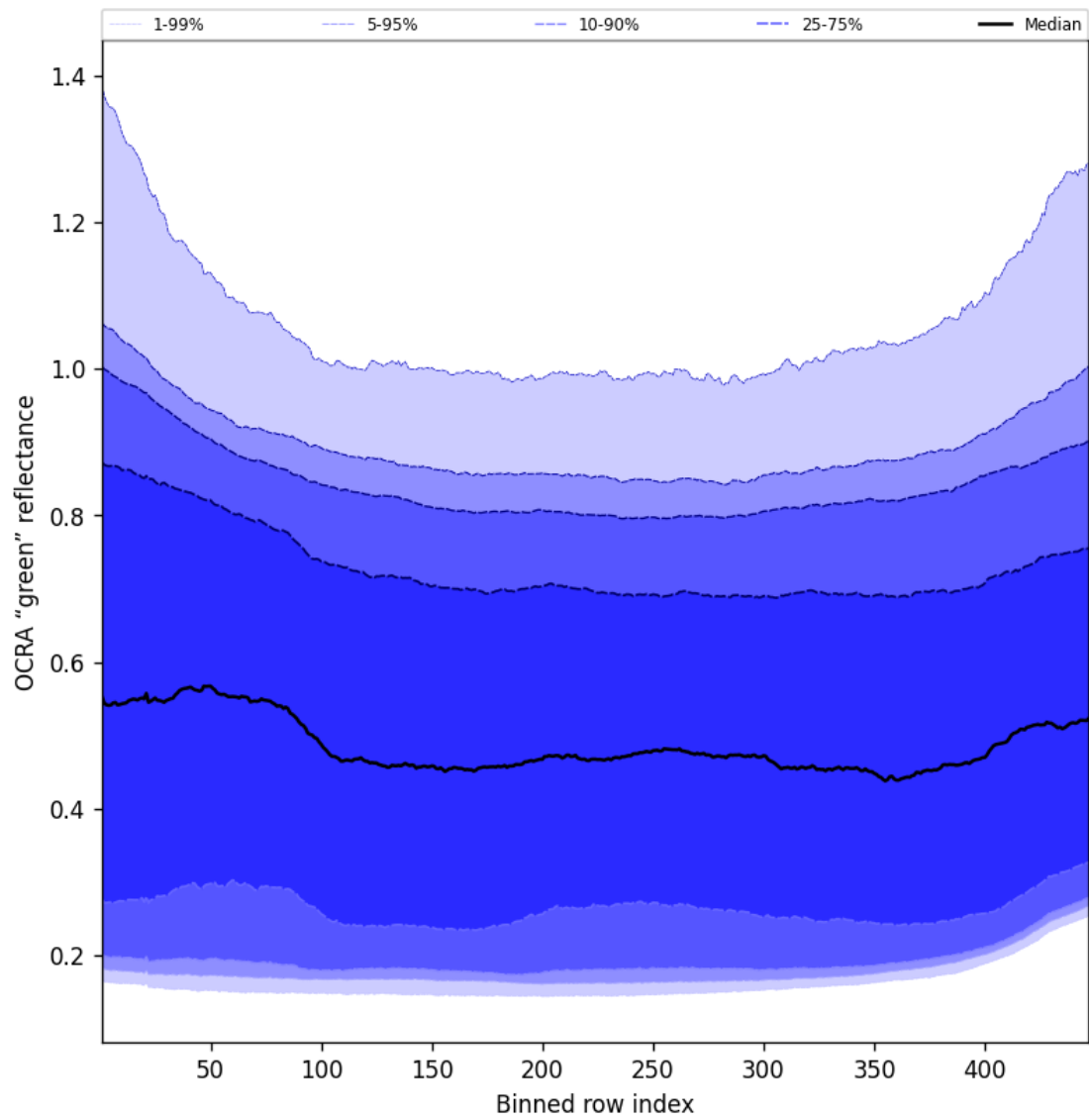
Figure 68: Along track statistics of “OCRA “green” reflectance” for 2025-10-02 to 2025-10-04
