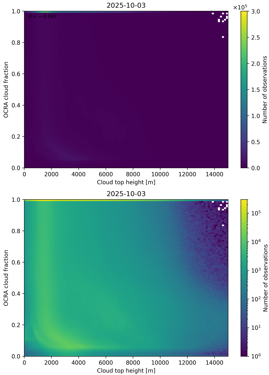
Figure 87: Scatter density plot of “Cloud top height” against “OCRA cloud fraction” for 2025-10-02 to 2025-10-04.
