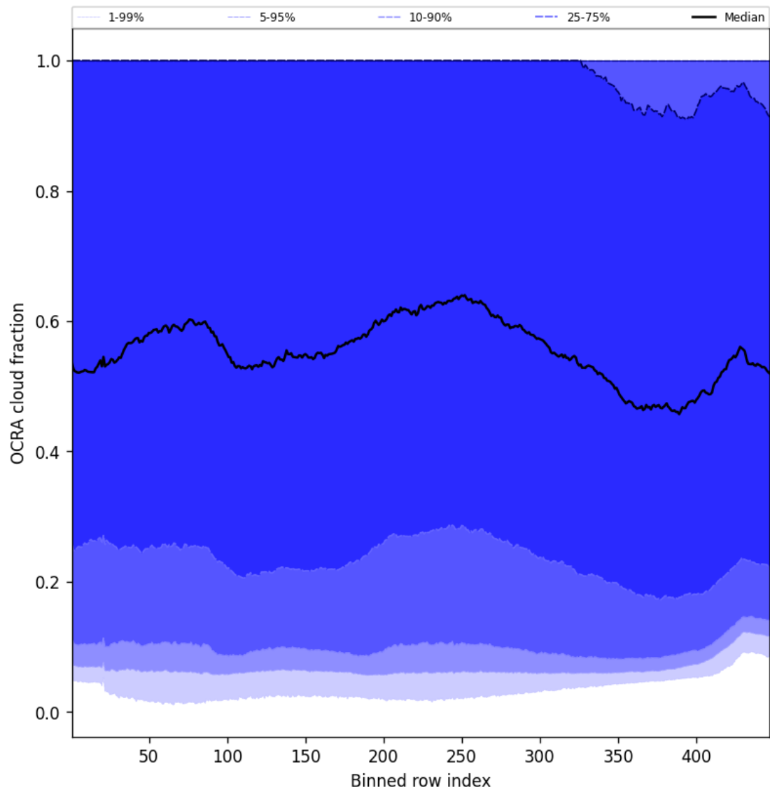
Figure 66: Along track statistics of “OCRA cloud fraction” for 2025-10-02 to 2025-10-04
