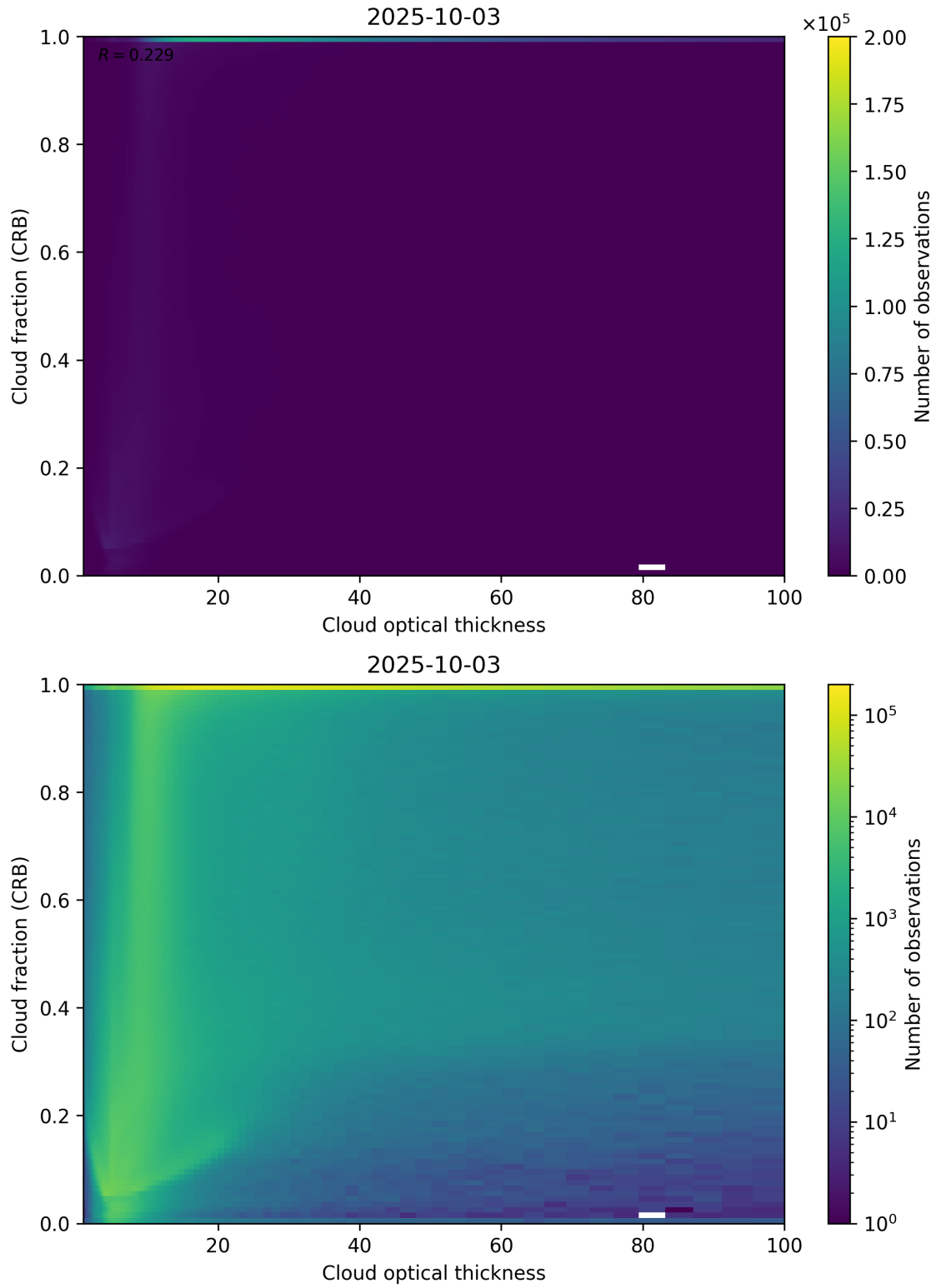
Figure 84: Scatter density plot of “Cloud optical thickness” against “Cloud fraction (CRB)” for 2025-10-02 to 2025-10-04.
