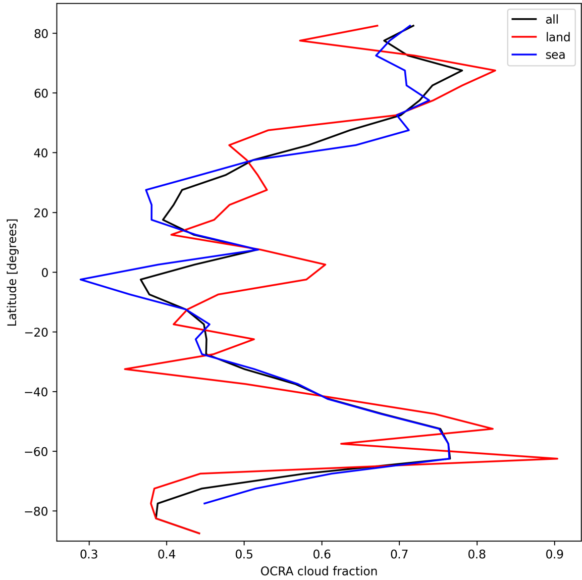
Figure 34: Zonal average of “OCRA cloud fraction” for 2025-10-02 to 2025-10-04.
