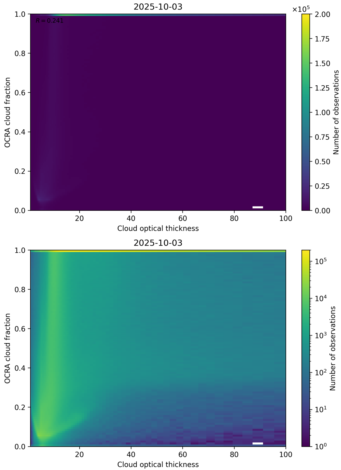
Figure 83: Scatter density plot of “Cloud optical thickness” against “OCRA cloud fraction” for 2025-10-02 to 2025-10-04.
