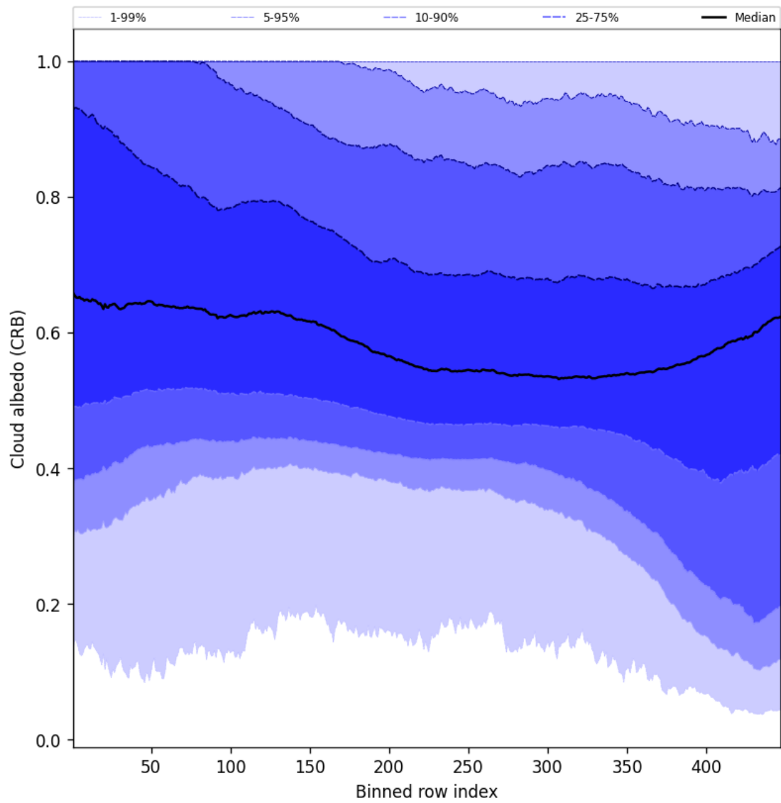
Figure 60: Along track statistics of “Cloud albedo (CRB)” for 2025-10-02 to 2025-10-04
