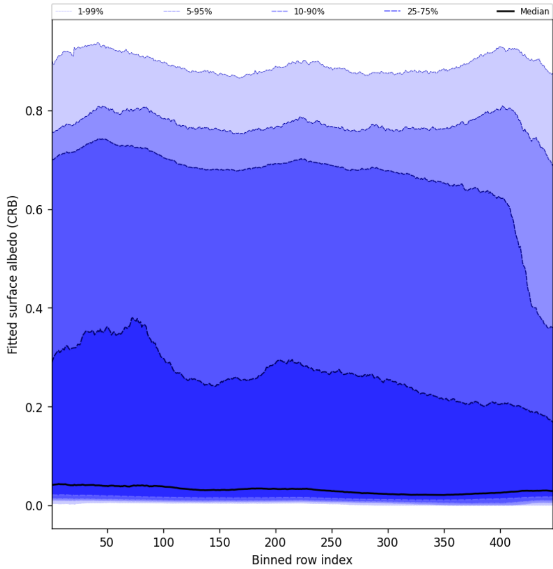
Figure 62: Along track statistics of “Fitted surface albedo (CRB)” for 2025-10-02 to 2025-10-04
