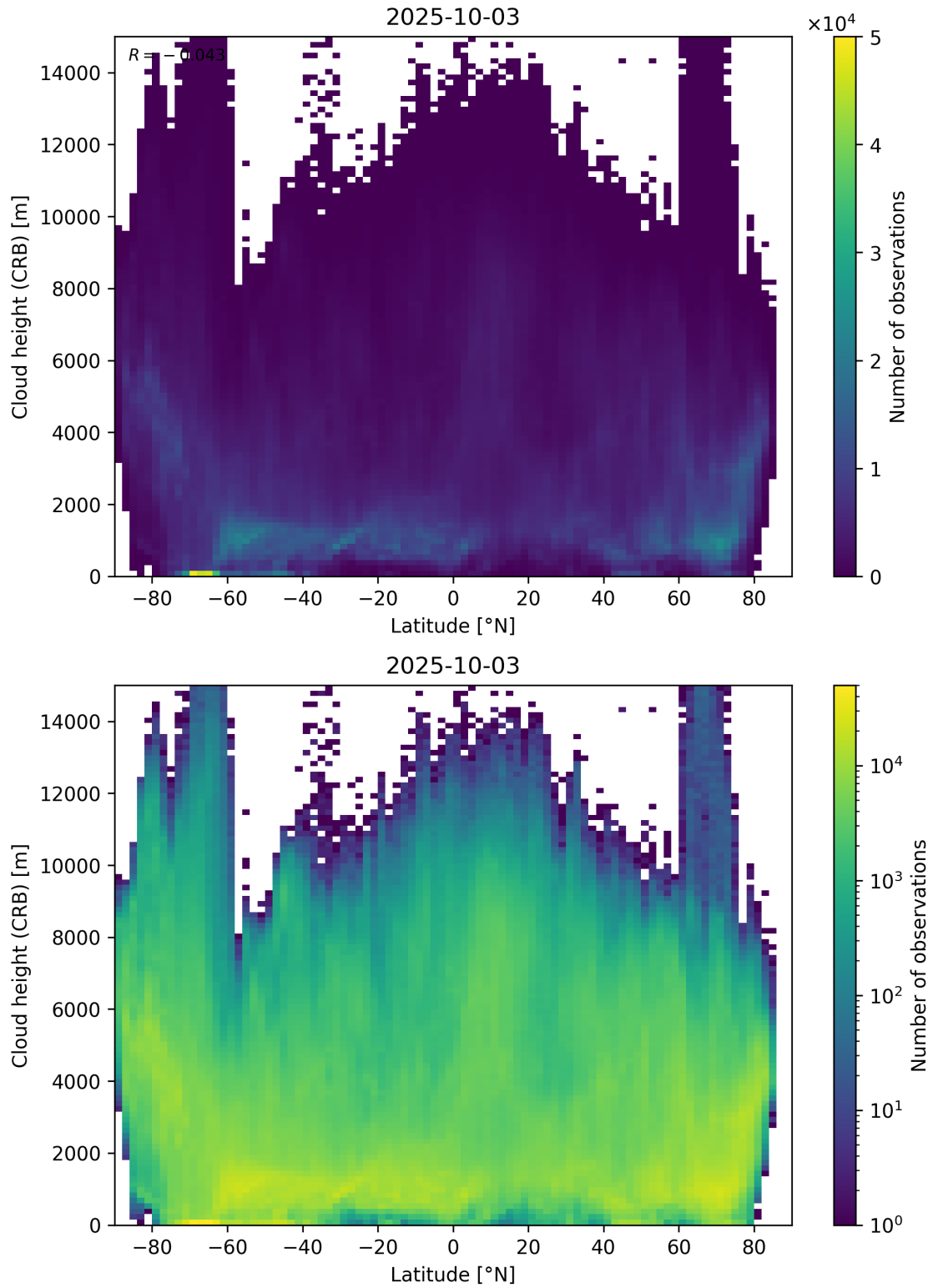
Figure 95: Scatter density plot of “Latitude” against “Cloud height (CRB)” for 2025-10-02 to 2025-10-04.
