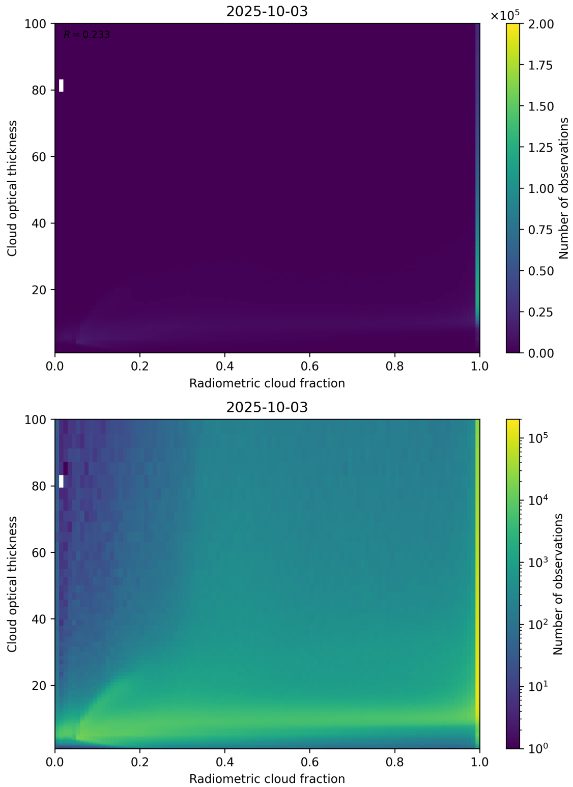
Figure 75: Scatter density plot of “Radiometric cloud fraction” against “Cloud optical thickness” for 2025-10-02 to 2025-10-04.
