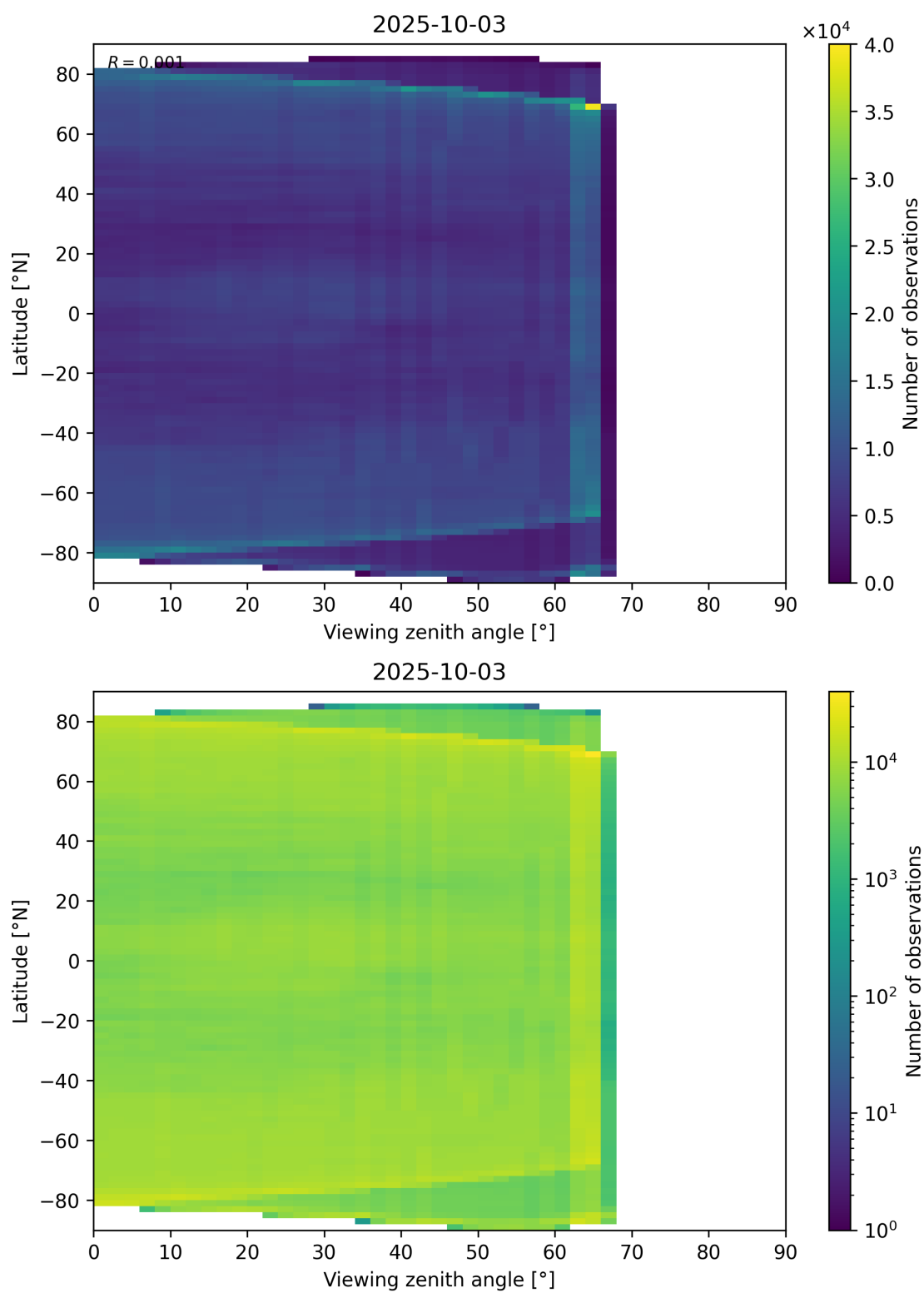
Figure 113: Scatter density plot of “Viewing zenith angle” against “Latitude” for 2025-10-02 to 2025-10-04.
