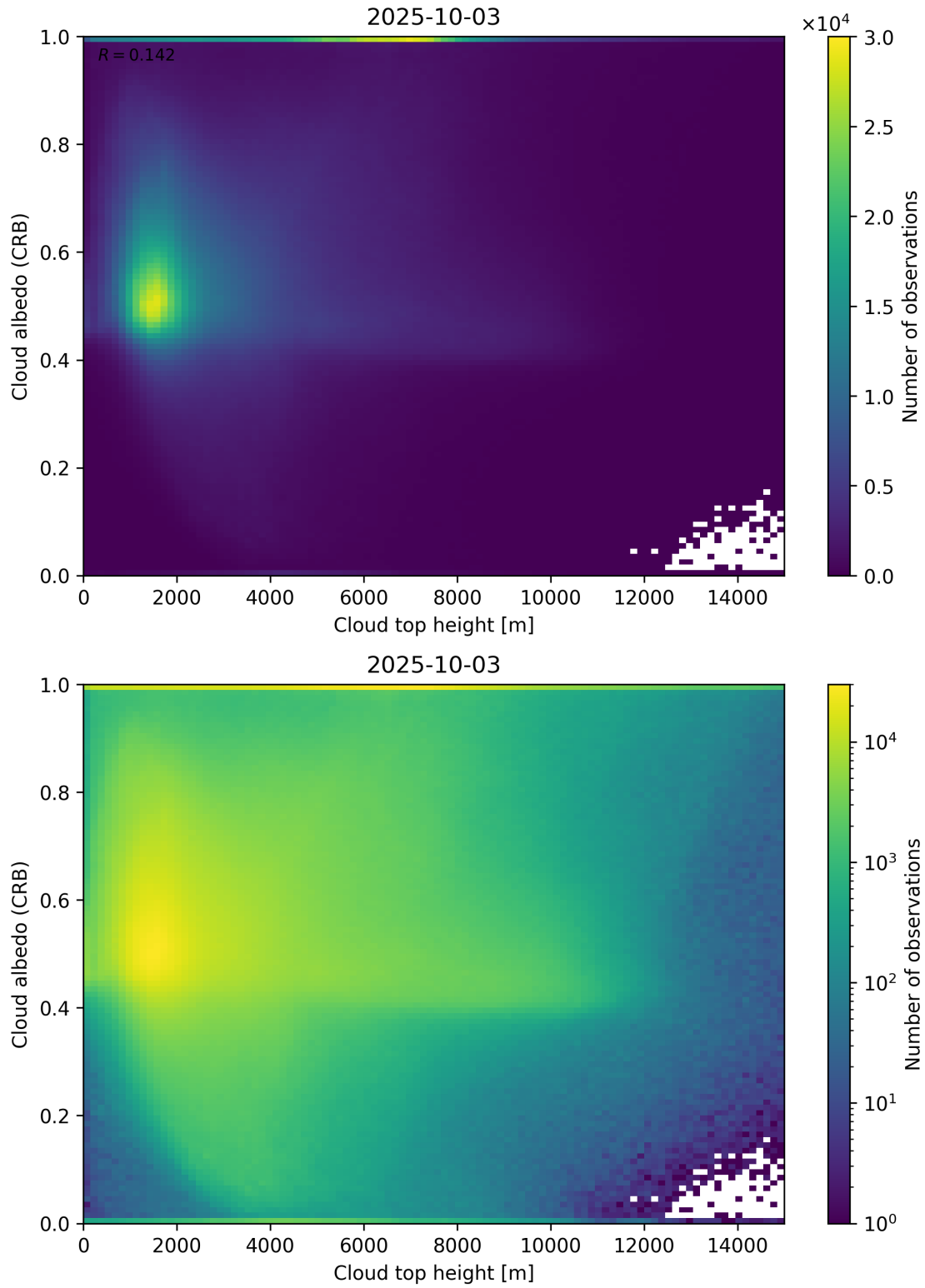
Figure 86: Scatter density plot of “Cloud top height” against “Cloud albedo (CRB)” for 2025-10-02 to 2025-10-04.
