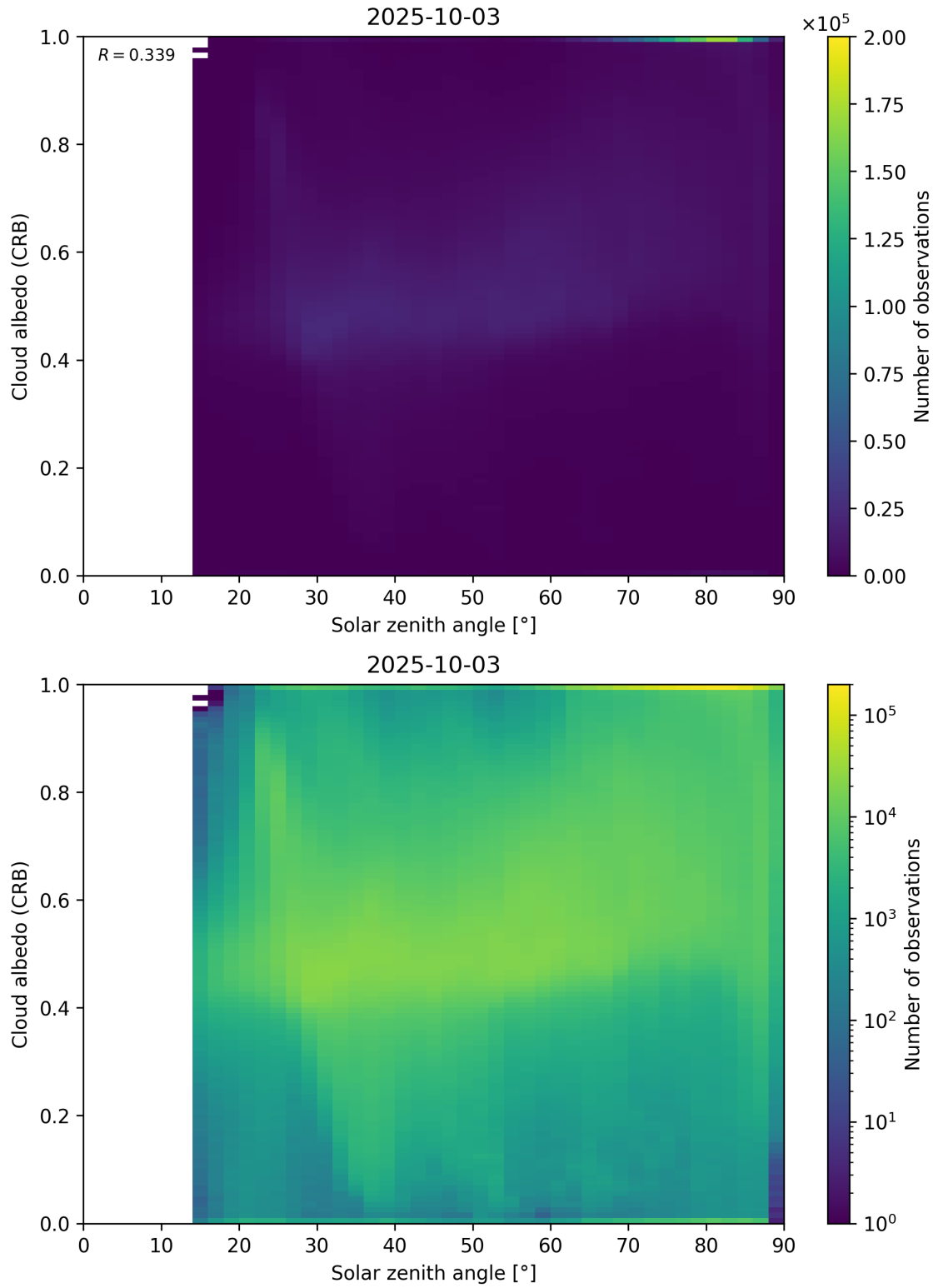
Figure 98: Scatter density plot of “Solar zenith angle” against “Cloud albedo (CRB)” for 2025-10-02 to 2025-10-04.
