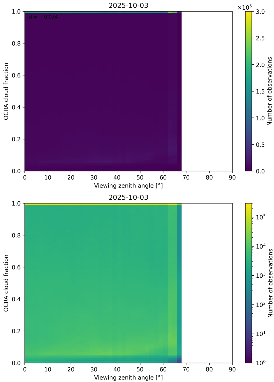
Figure 108: Scatter density plot of “Viewing zenith angle” against “OCRA cloud fraction” for 2025-10-02 to 2025-10-04.
