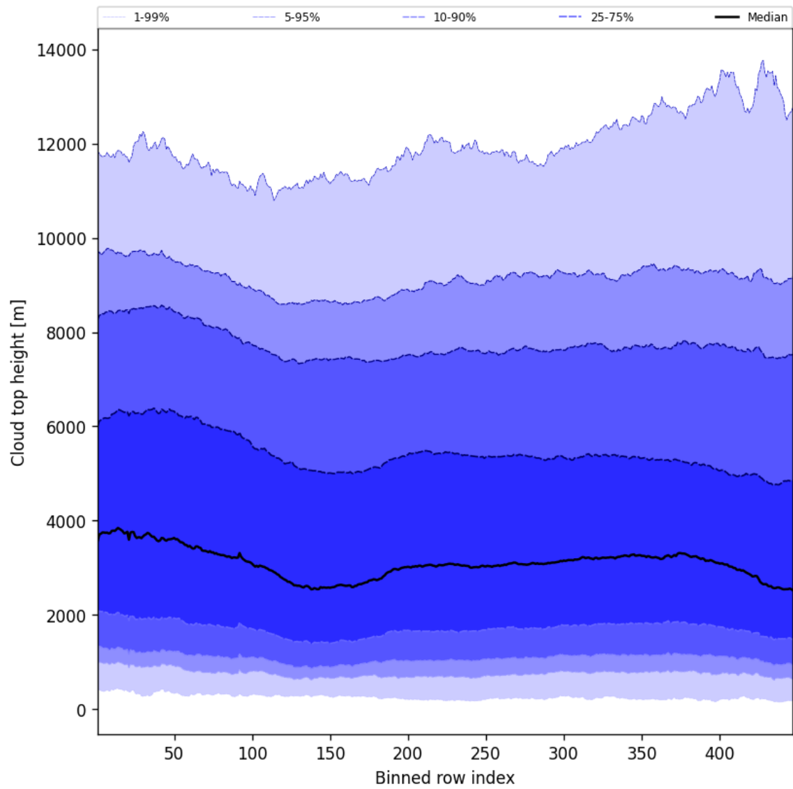
Figure 56: Along track statistics of “Cloud top height” for 2025-10-02 to 2025-10-04
