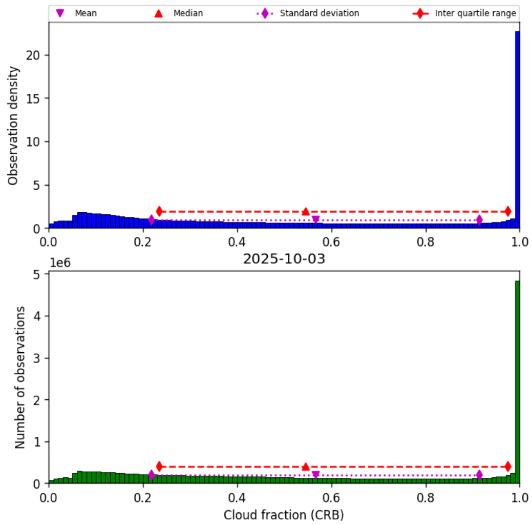
Figure 42: Histogram of “Cloud fraction (CRB)” for 2025-10-02 to 2025-10-04
