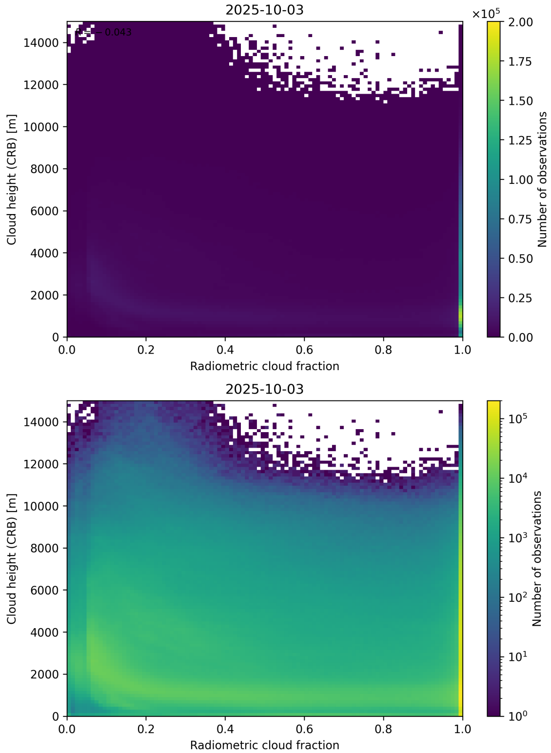
Figure 74: Scatter density plot of “Radiometric cloud fraction” against “Cloud height (CRB)” for 2025-10-02 to 2025-10-04.
