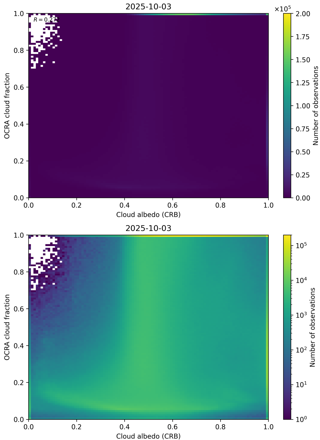
Figure 70: Scatter density plot of “Cloud albedo (CRB)” against “OCRA cloud fraction” for 2025-10-02 to 2025-10-04.
