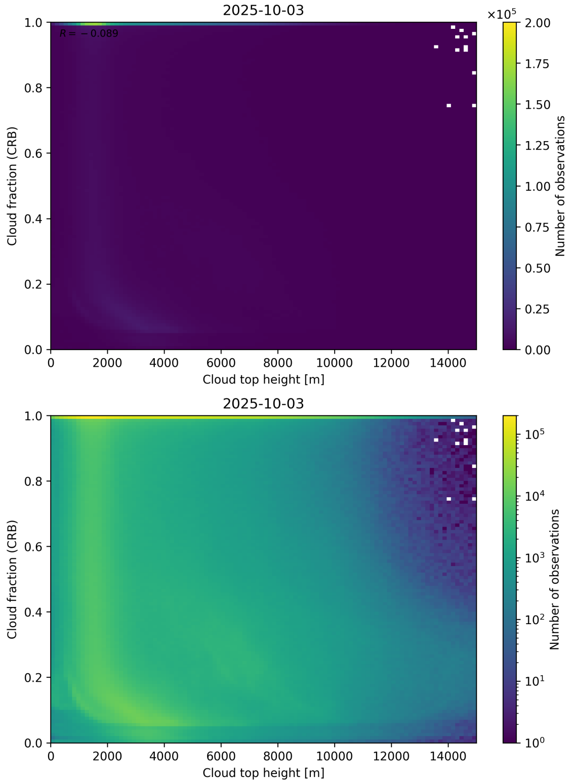
Figure 88: Scatter density plot of “Cloud top height” against “Cloud fraction (CRB)” for 2025-10-02 to 2025-10-04.
