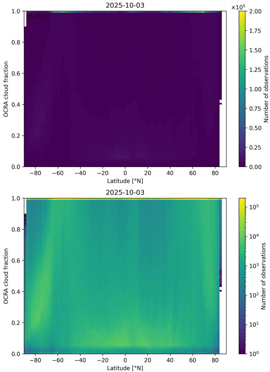
Figure 93: Scatter density plot of “Latitude” against “OCRA cloud fraction” for 2025-10-02 to 2025-10-04.
