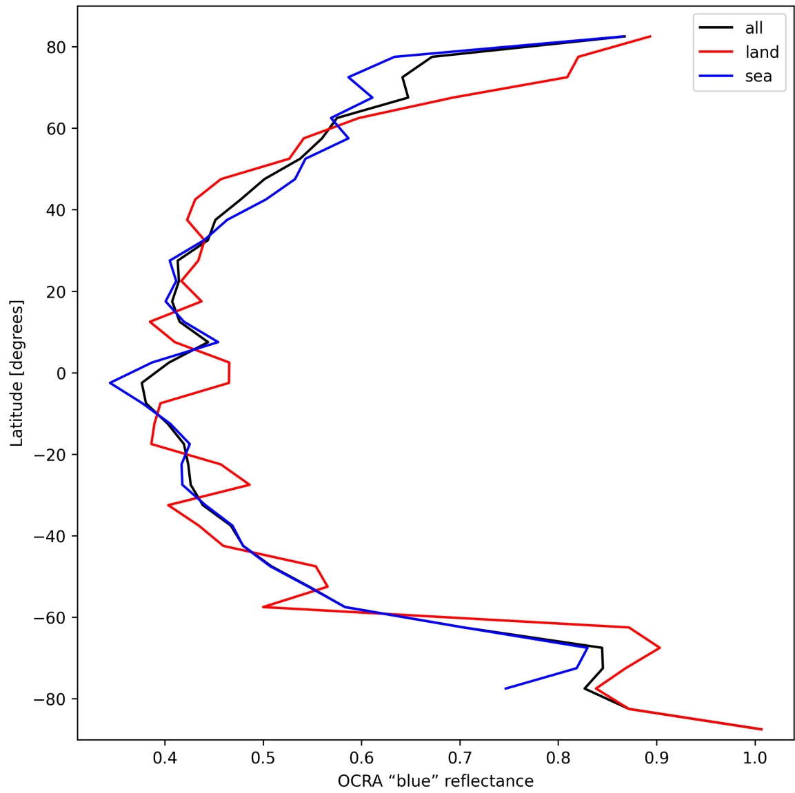
Figure 35: Zonal average of "OCRA "blue" reflectance" for 2025-10-02 to 2025-10-04.
