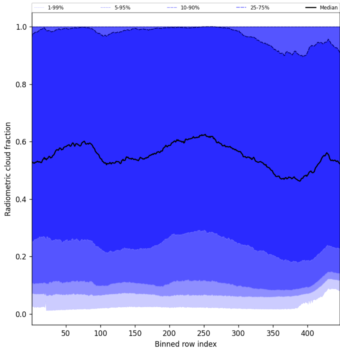
Figure 55: Along track statistics of “Radiometric cloud fraction” for 2025-10-02 to 2025-10-04
