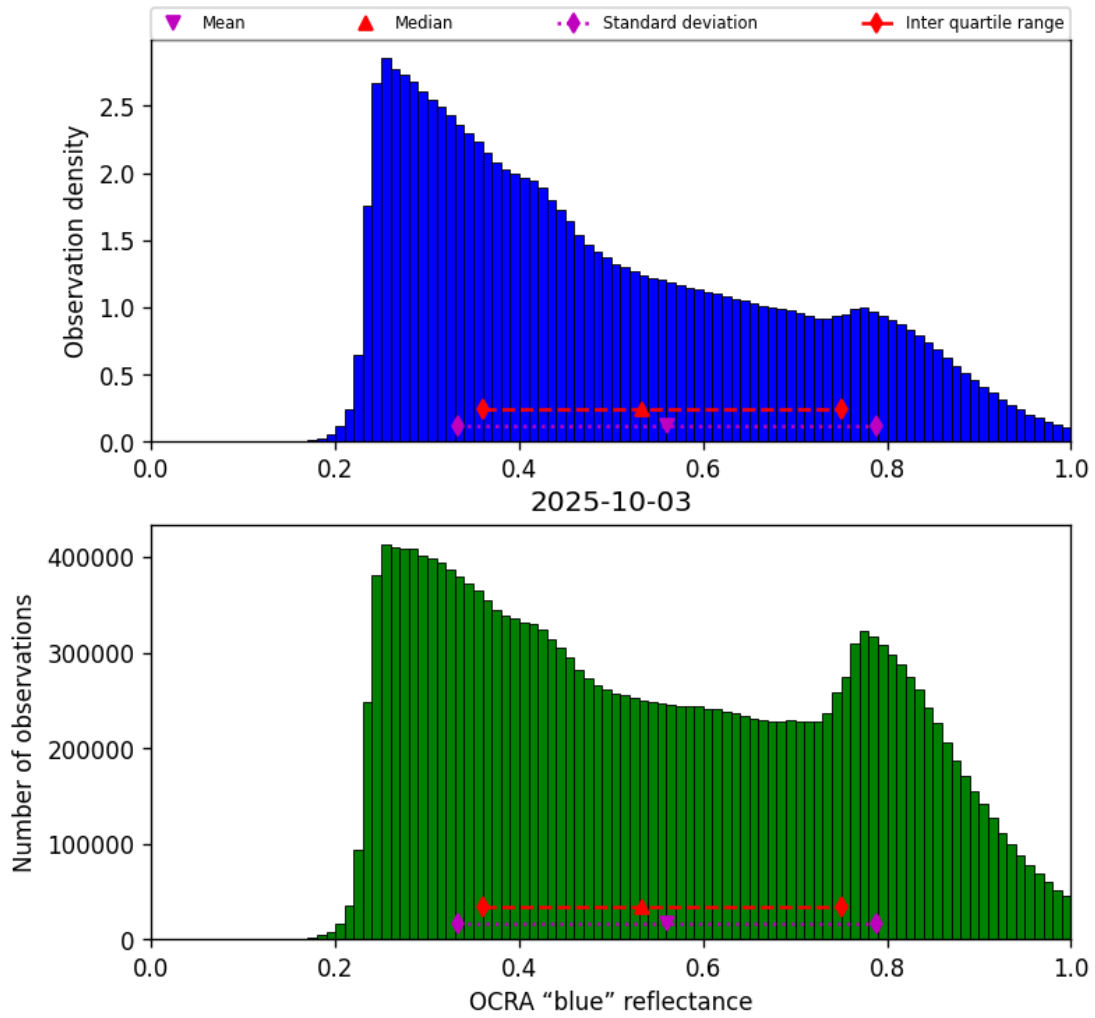
Figure 51: Histogram of “OCRA “blue” reflectance” for 2025-10-02 to 2025-10-04
