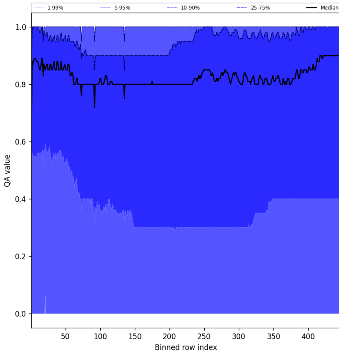
Figure 54: Along track statistics of “QA value” for 2025-10-02 to 2025-10-04
