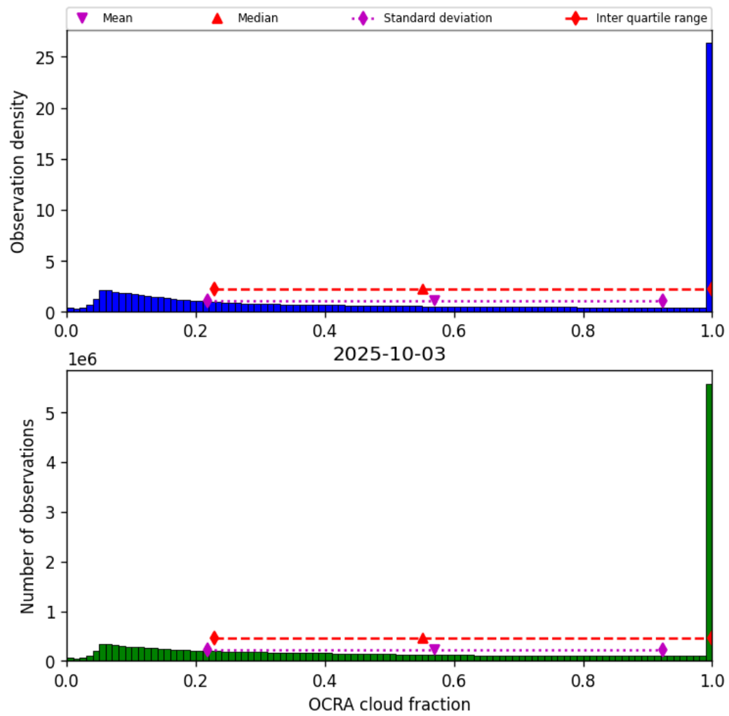
Figure 50: Histogram of “OCRA cloud fraction” for 2025-10-02 to 2025-10-04
