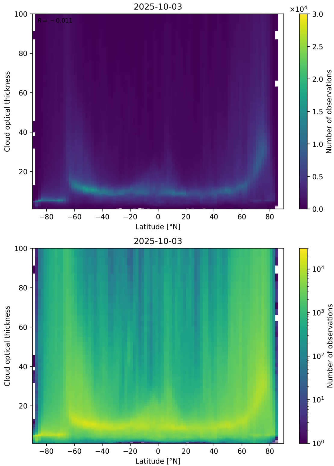
Figure 96: Scatter density plot of “Latitude” against “Cloud optical thickness” for 2025-10-02 to 2025-10-04.
