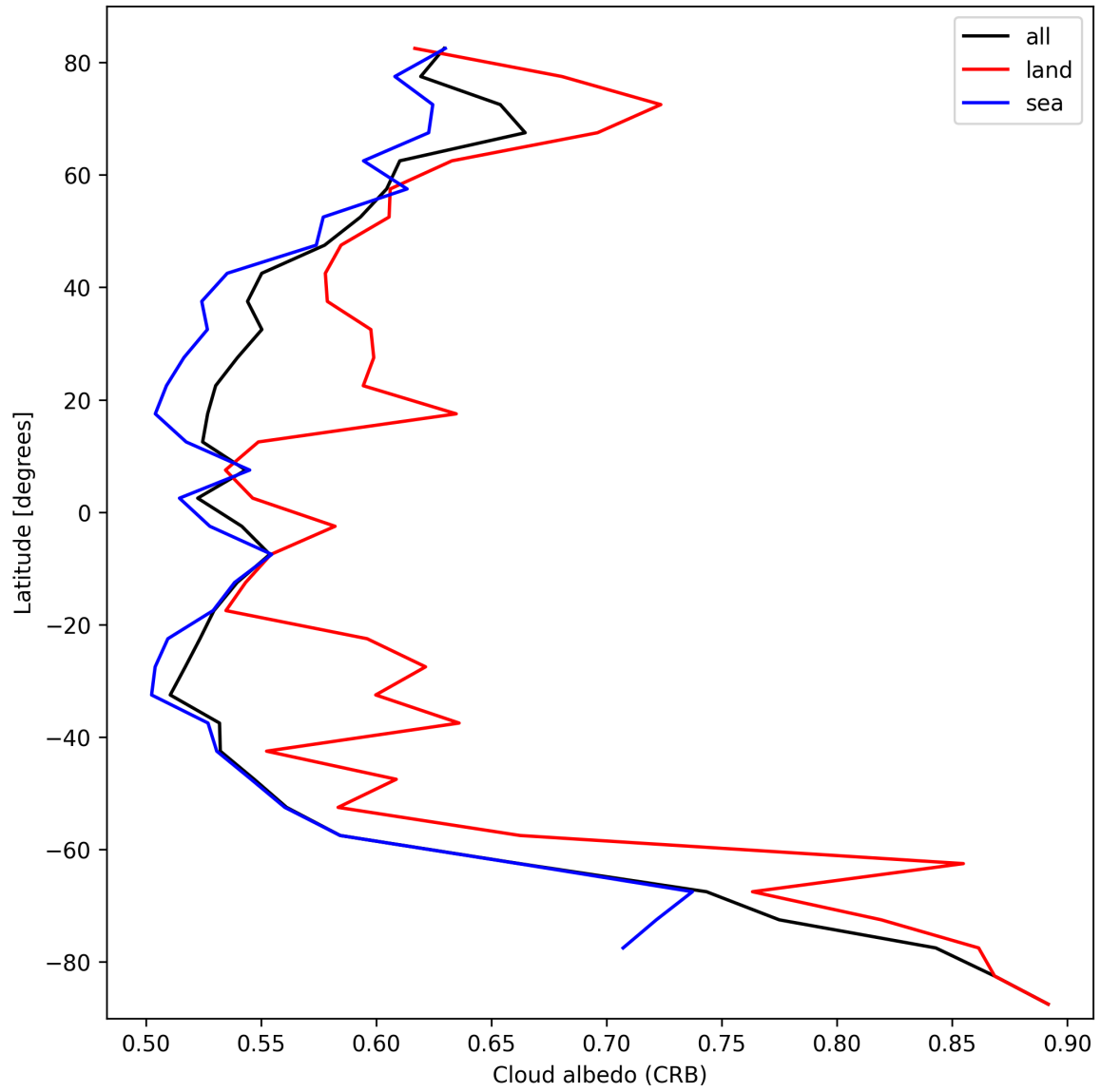
Figure 28: Zonal average of “Cloud albedo (CRB)” for 2025-10-02 to 2025-10-04.
