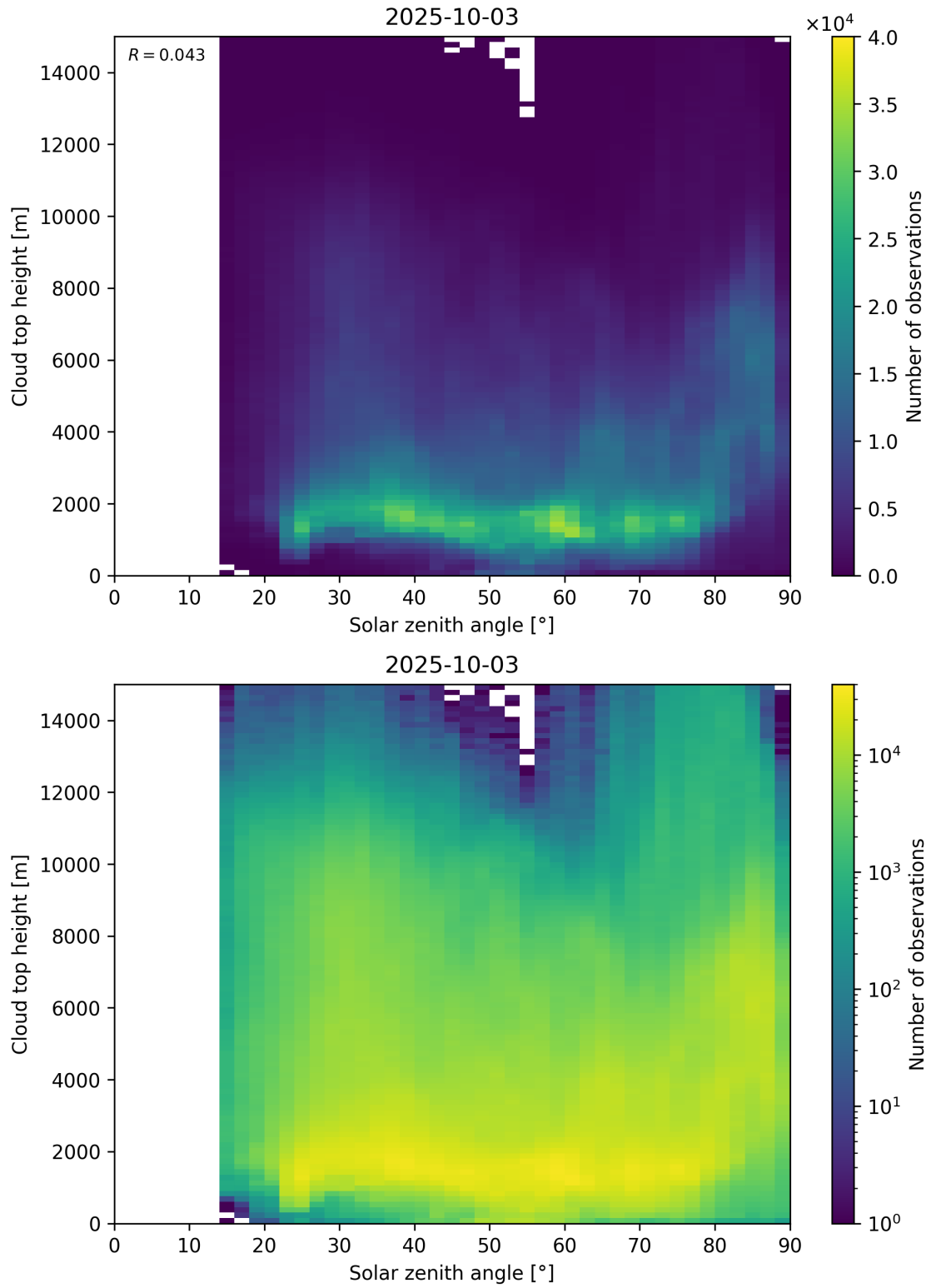
Figure 104: Scatter density plot of “Solar zenith angle” against “Cloud top height” for 2025-10-02 to 2025-10-04.
