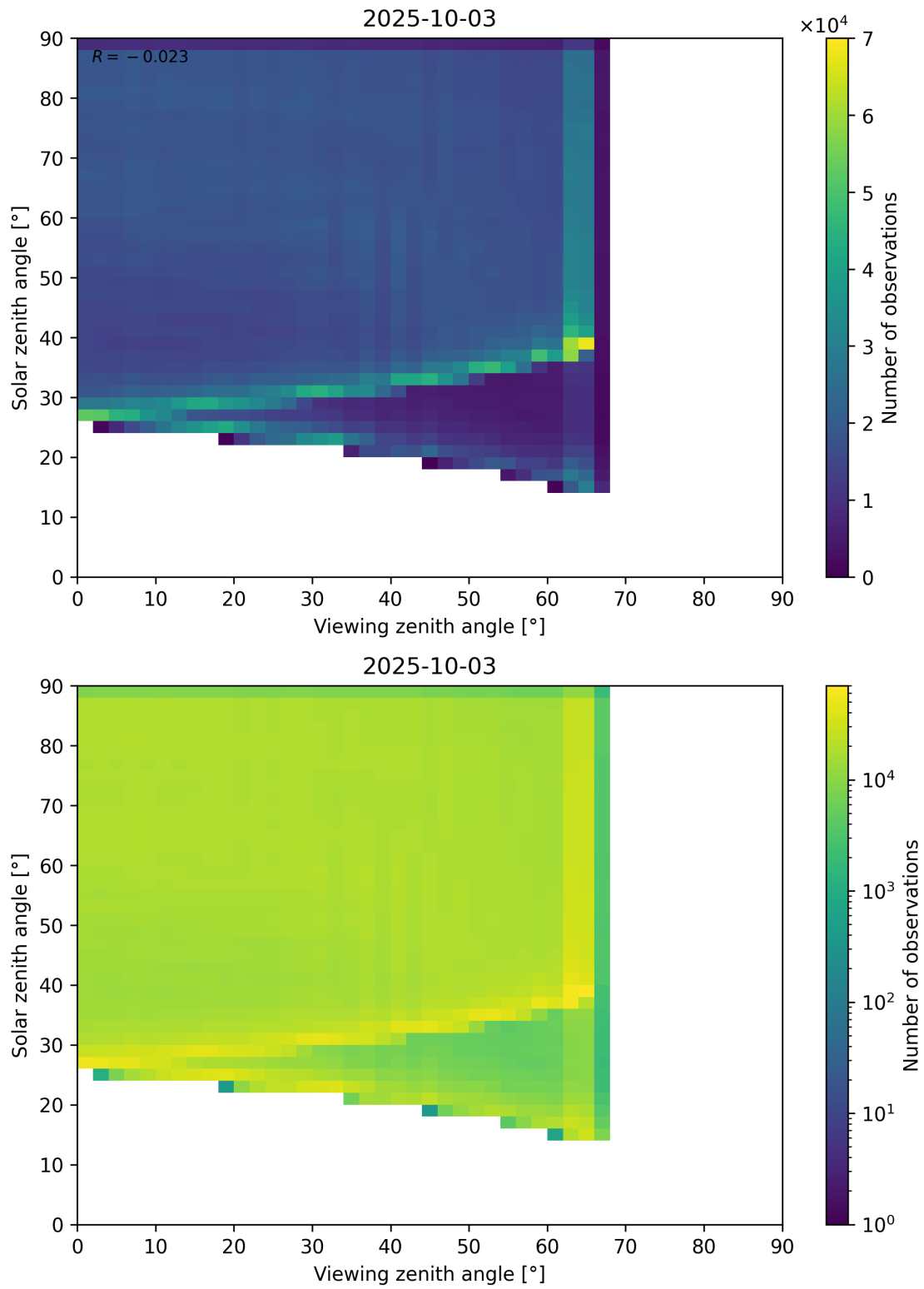
Figure 114: Scatter density plot of “Viewing zenith angle” against “Solar zenith angle” for 2025-10-02 to 2025-10-04.
