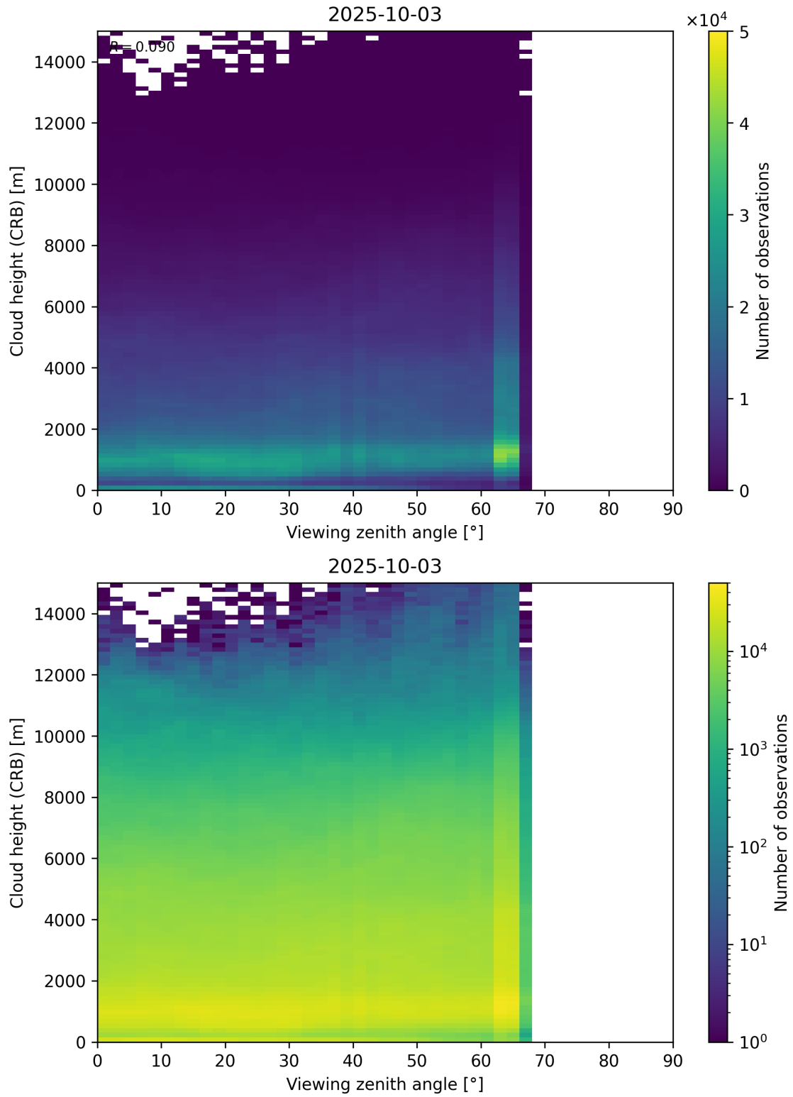
Figure 110: Scatter density plot of “Viewing zenith angle” against “Cloud height (CRB)” for 2025-10-02 to 2025-10-04.
