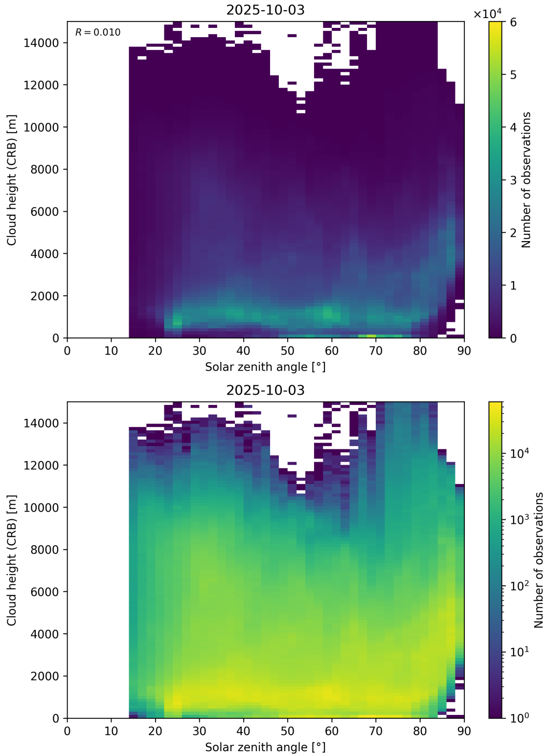
Figure 102: Scatter density plot of “Solar zenith angle” against “Cloud height (CRB)” for 2025-10-02 to 2025-10-04.
