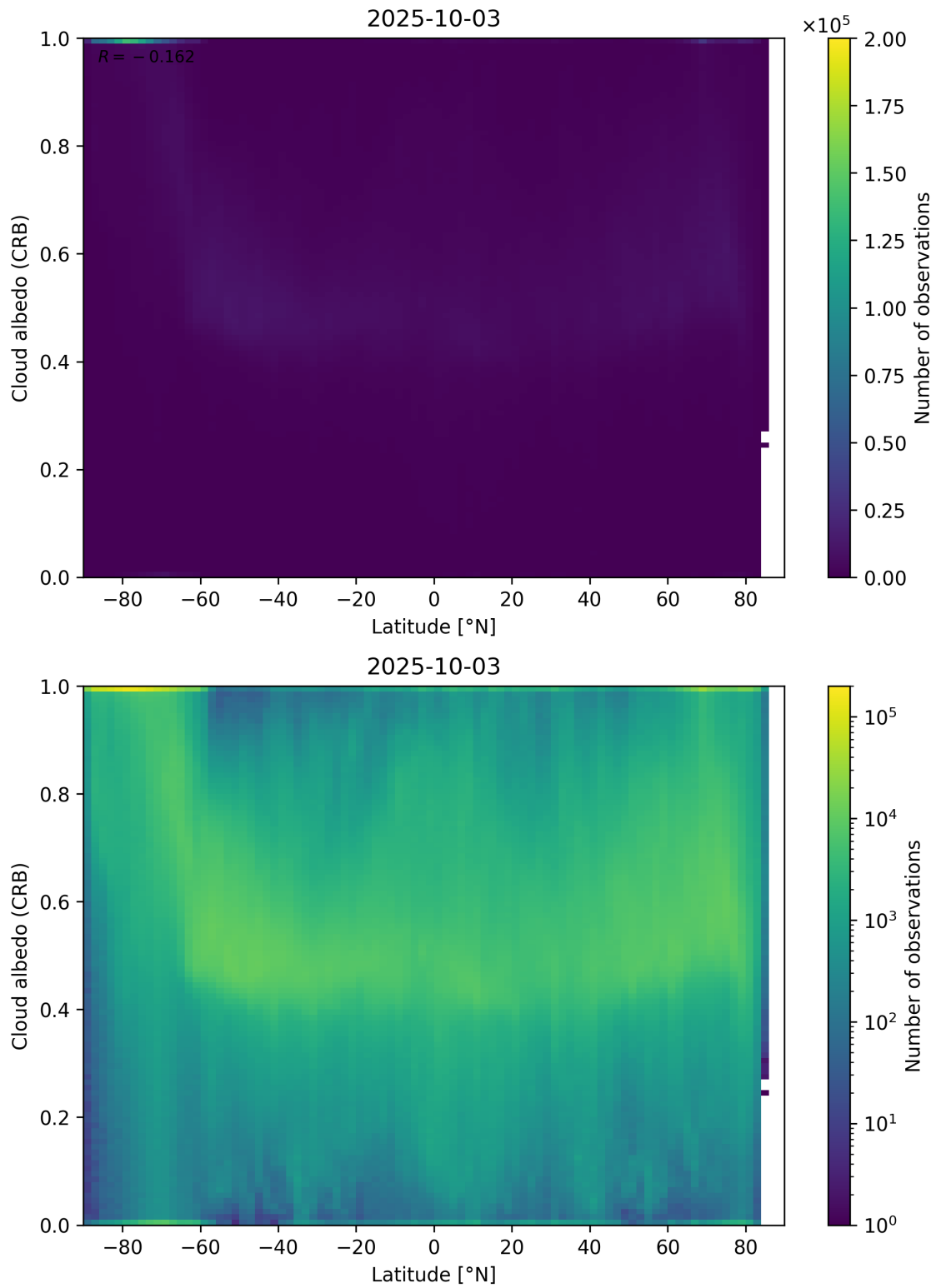
Figure 91: Scatter density plot of “Latitude” against “Cloud albedo (CRB)” for 2025-10-02 to 2025-10-04.
