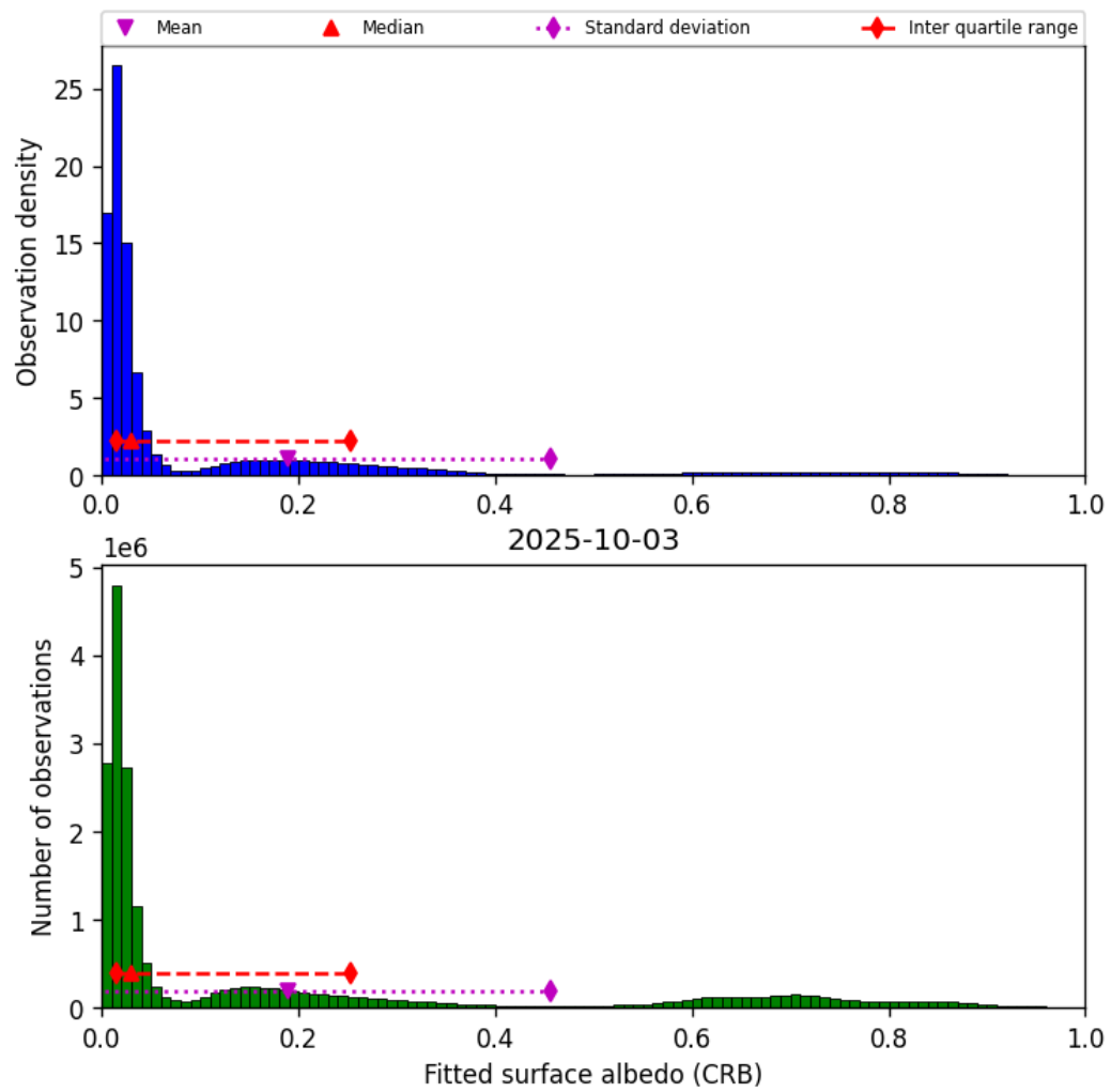
Figure 46: Histogram of “Fitted surface albedo (CRB)” for 2025-10-02 to 2025-10-04
