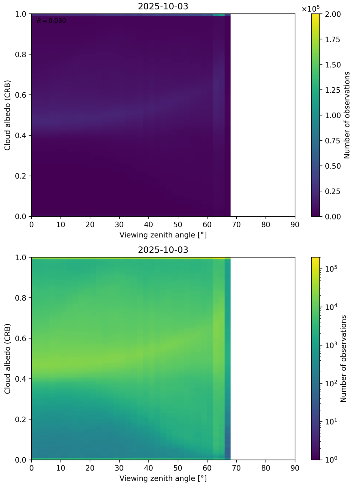
Figure 106: Scatter density plot of “Viewing zenith angle” against “Cloud albedo (CRB)” for 2025-10-02 to 2025-10-04.
