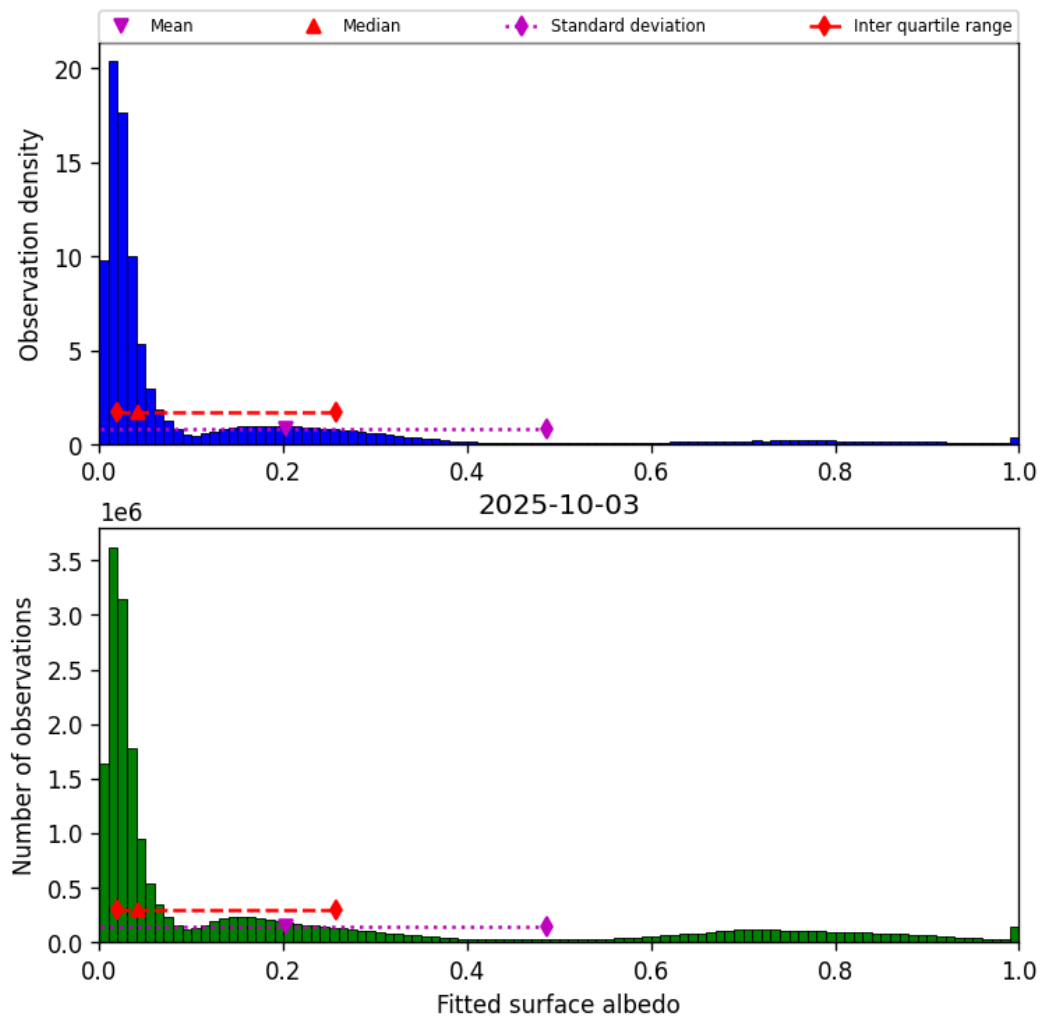
Figure 45: Histogram of “Fitted surface albedo” for 2025-10-02 to 2025-10-04
