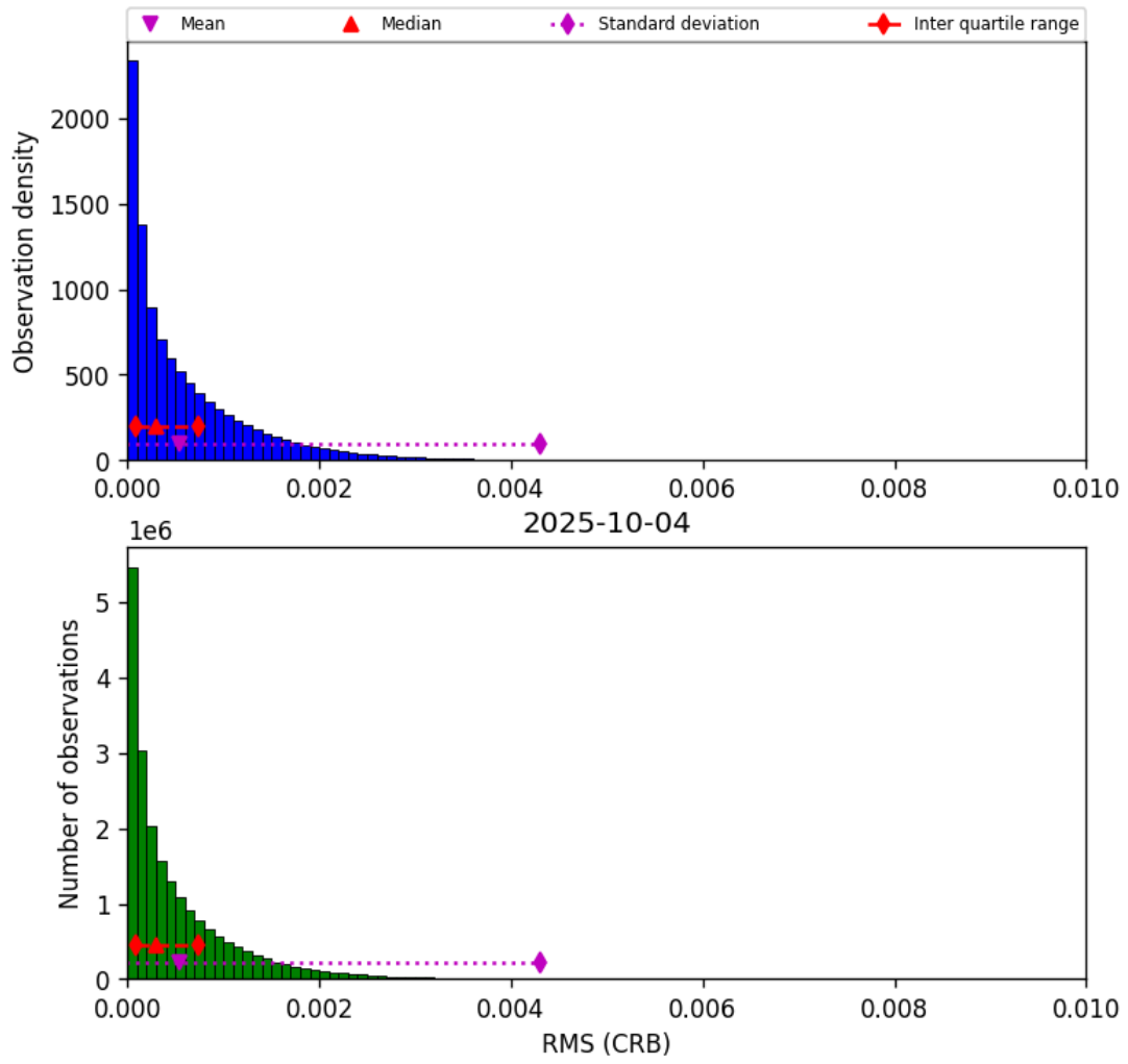
Figure 48: Histogram of “RMS (CRB)” for 2025-10-03 to 2025-10-05
