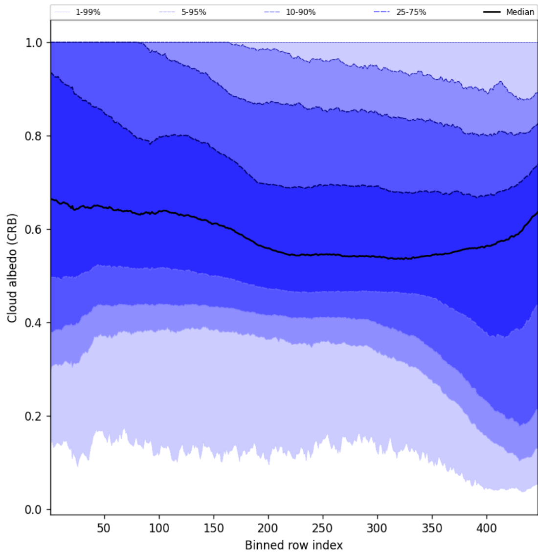
Figure 60: Along track statistics of “Cloud albedo (CRB)” for 2025-10-03 to 2025-10-05
