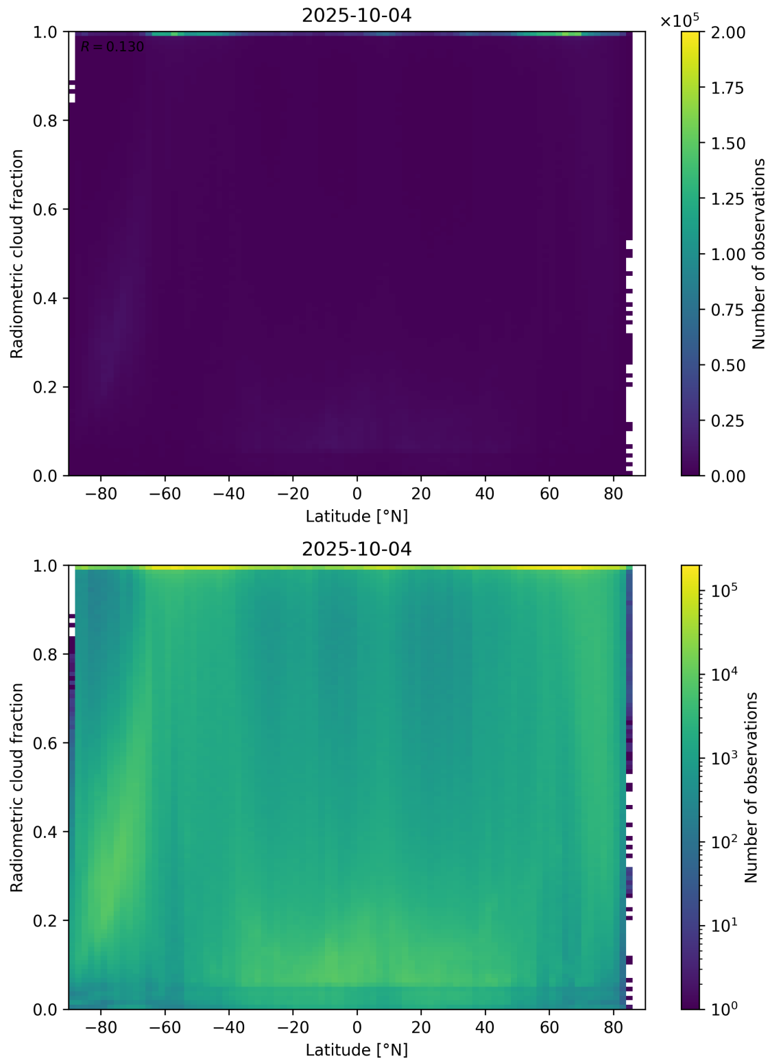
Figure 92: Scatter density plot of “Latitude” against “Radiometric cloud fraction” for 2025-10-03 to 2025-10-05.
