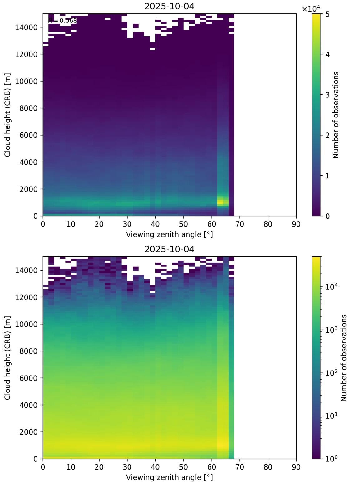
Figure 110: Scatter density plot of “Viewing zenith angle” against “Cloud height (CRB)” for 2025-10-03 to 2025-10-05.
