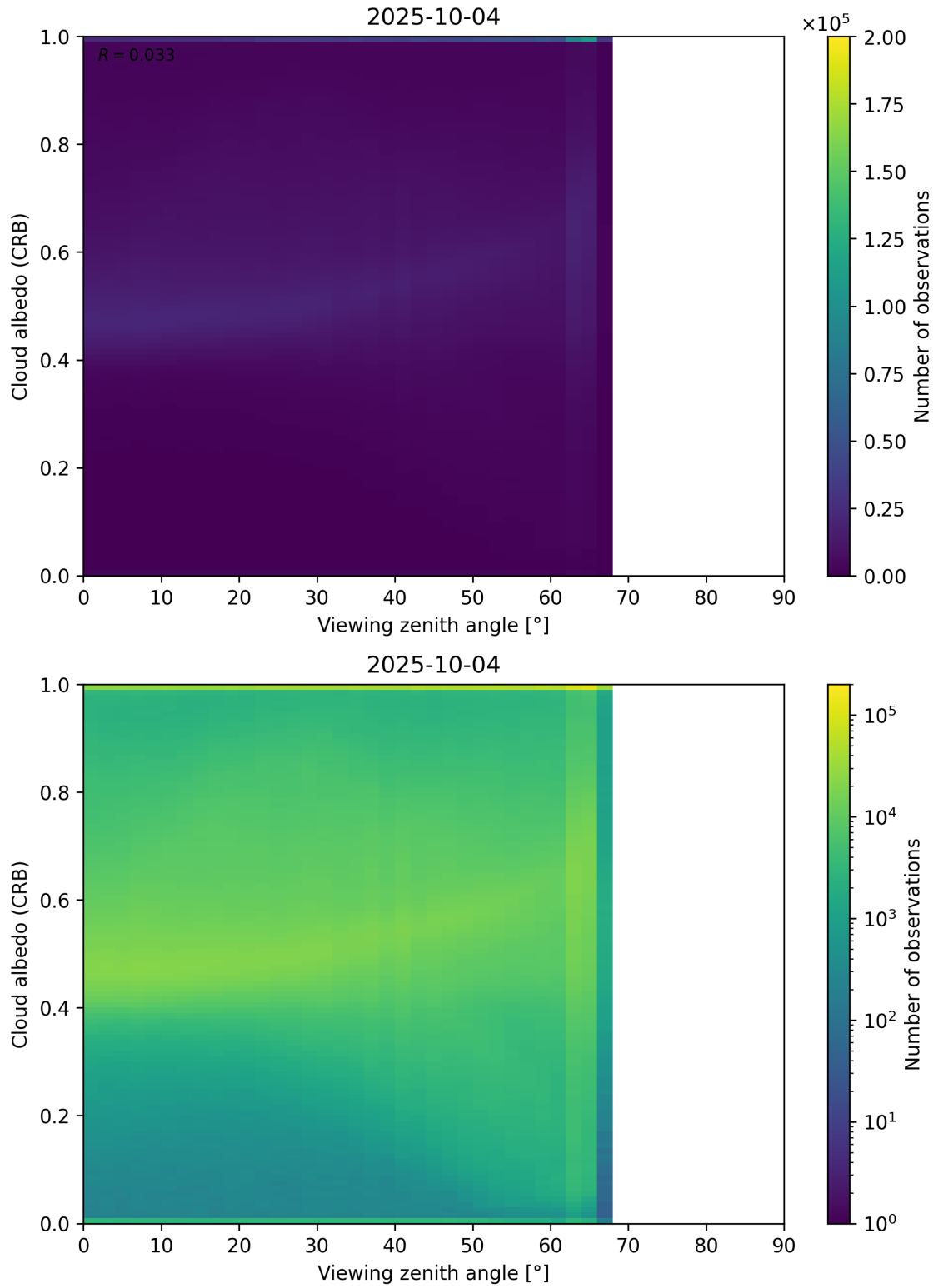
Figure 106: Scatter density plot of “Viewing zenith angle” against “Cloud albedo (CRB)” for 2025-10-03 to 2025-10-05.
