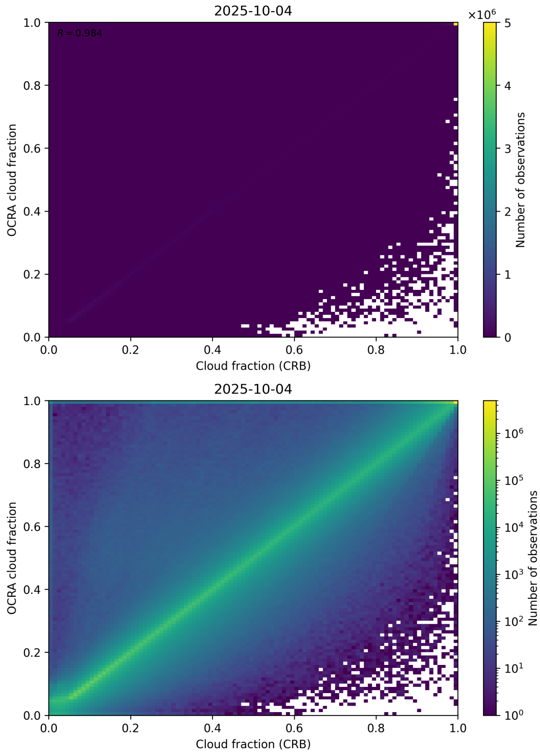
Figure 78: Scatter density plot of “Cloud fraction (CRB)” against “OCRA cloud fraction” for 2025-10-03 to 2025-10-05.
