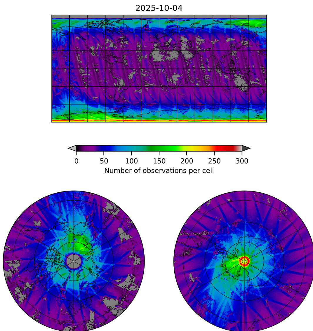
Figure 21: Map of the number of observations for 2025-10-03 to 2025-10-05
