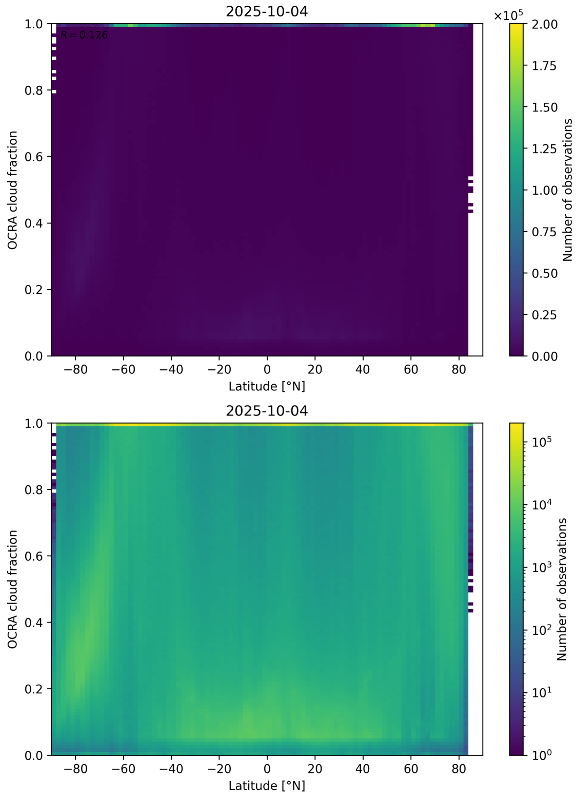
Figure 93: Scatter density plot of “Latitude” against “OCRA cloud fraction” for 2025-10-03 to 2025-10-05.
