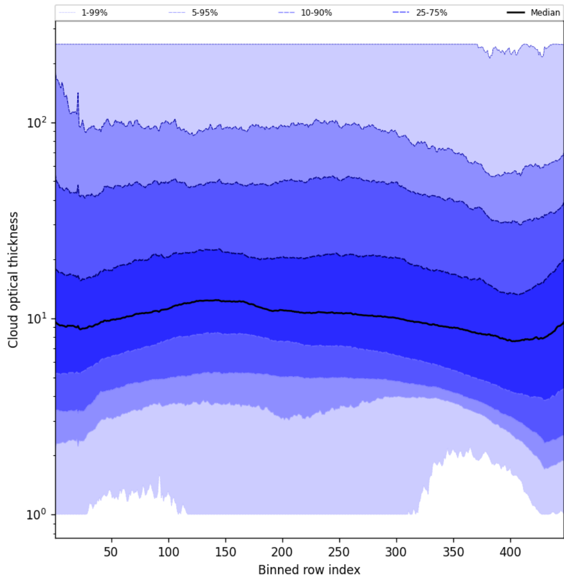
Figure 57: Along track statistics of “Cloud optical thickness” for 2025-10-03 to 2025-10-05
