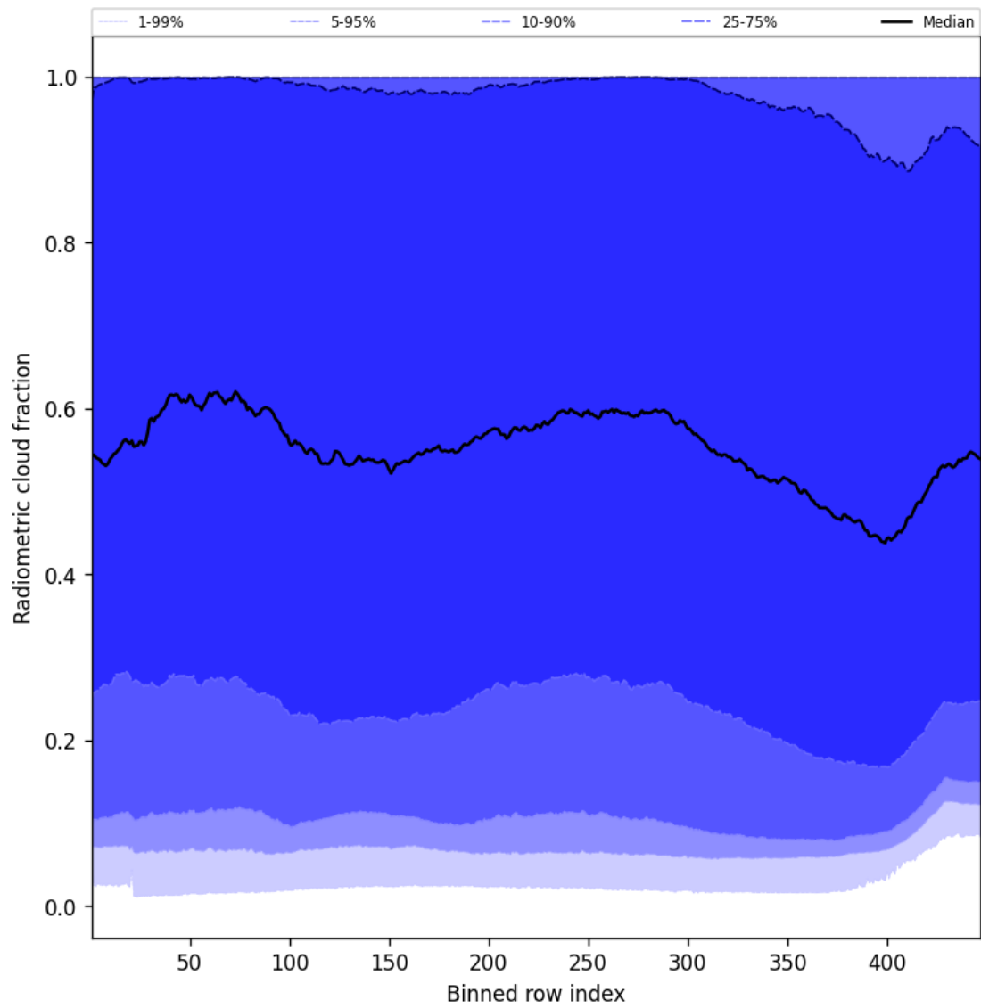
Figure 55: Along track statistics of “Radiometric cloud fraction” for 2025-10-03 to 2025-10-05
