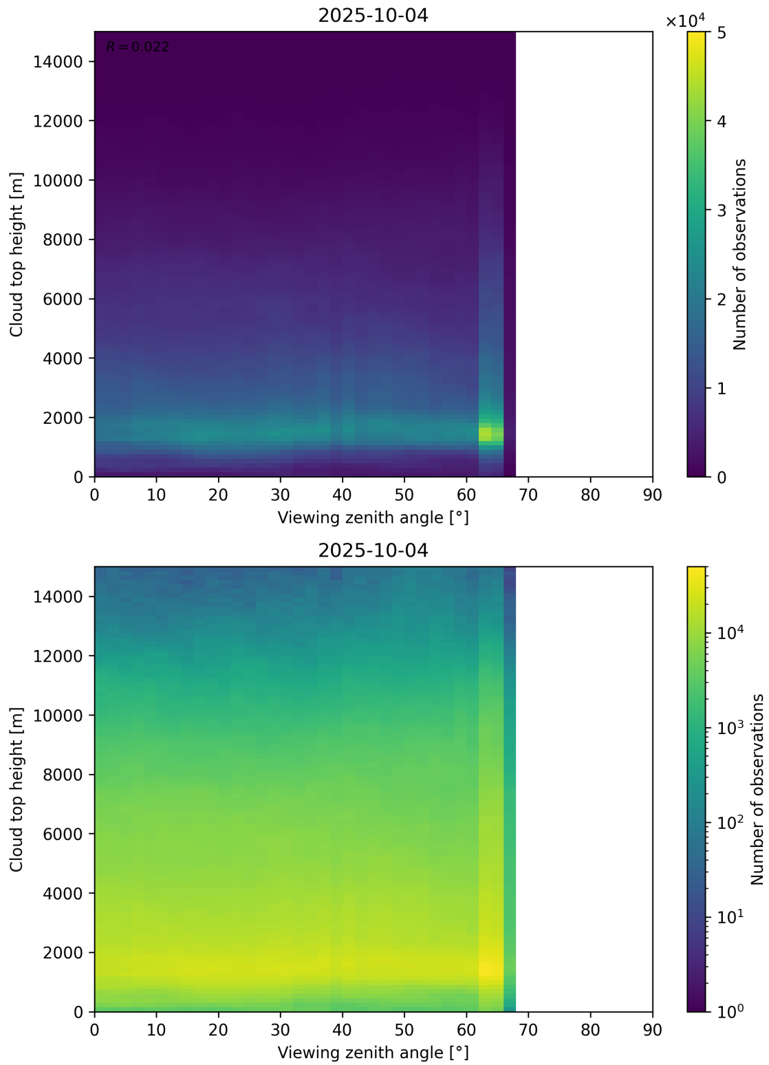
Figure 112: Scatter density plot of “Viewing zenith angle” against “Cloud top height” for 2025-10-03 to 2025-10-05.
