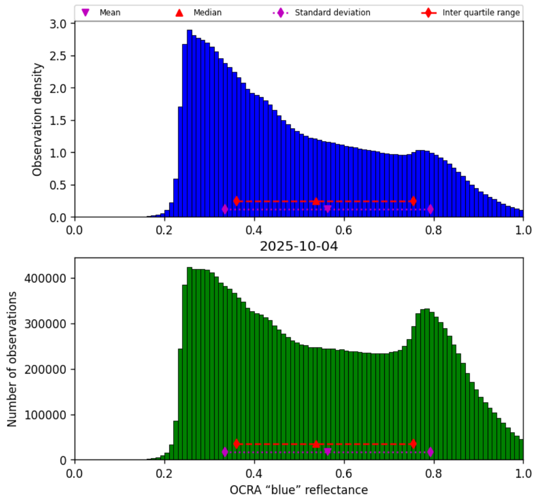
Figure 51: Histogram of “OCRA “blue” reflectance” for 2025-10-03 to 2025-10-05
