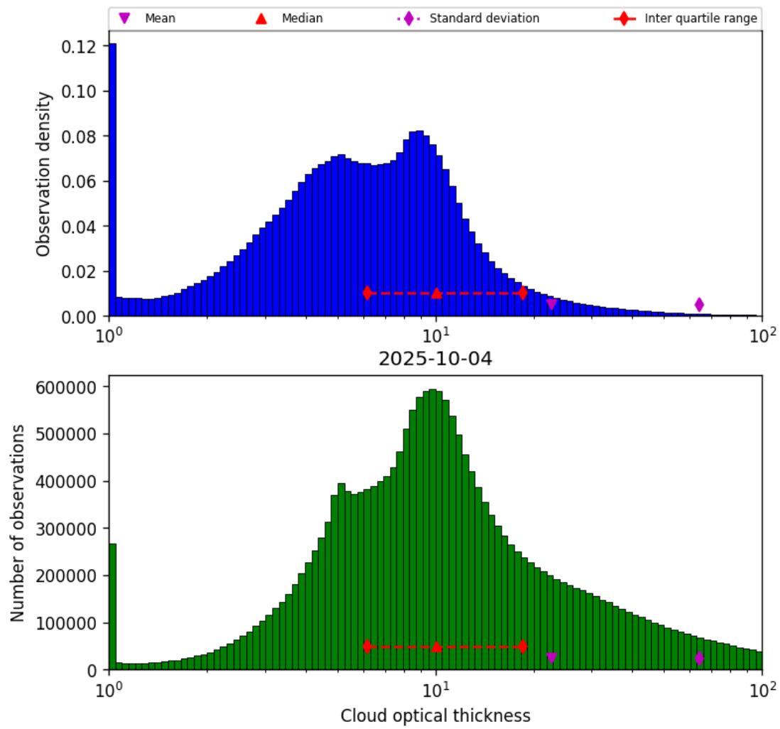
Figure 41: Histogram of “Cloud optical thickness” for 2025-10-03 to 2025-10-05
