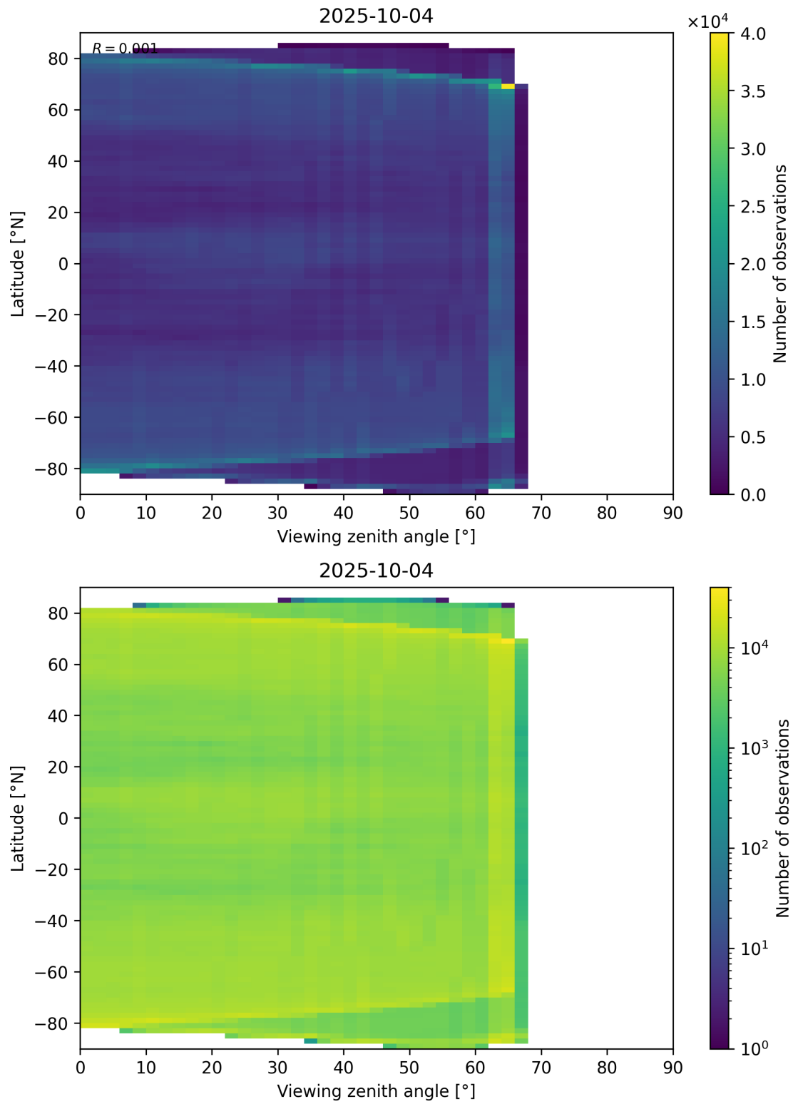
Figure 113: Scatter density plot of “Viewing zenith angle” against “Latitude” for 2025-10-03 to 2025-10-05.
