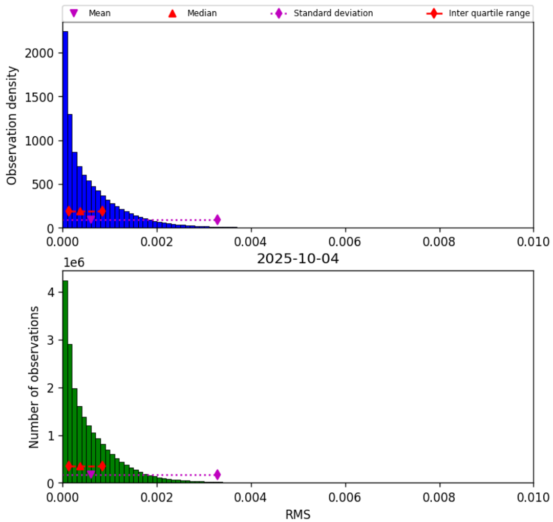
Figure 47: Histogram of “RMS” for 2025-10-03 to 2025-10-05
