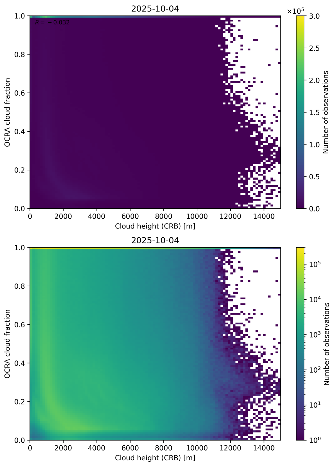
Figure 81: Scatter density plot of “Cloud height (CRB)” against “OCRA cloud fraction” for 2025-10-03 to 2025-10-05.
