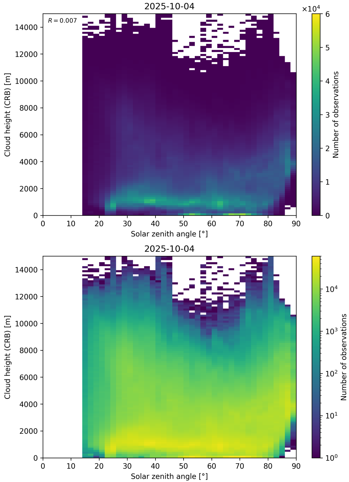
Figure 102: Scatter density plot of “Solar zenith angle” against “Cloud height (CRB)” for 2025-10-03 to 2025-10-05.
