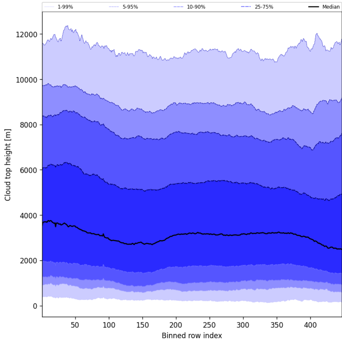
Figure 56: Along track statistics of “Cloud top height” for 2025-10-03 to 2025-10-05
