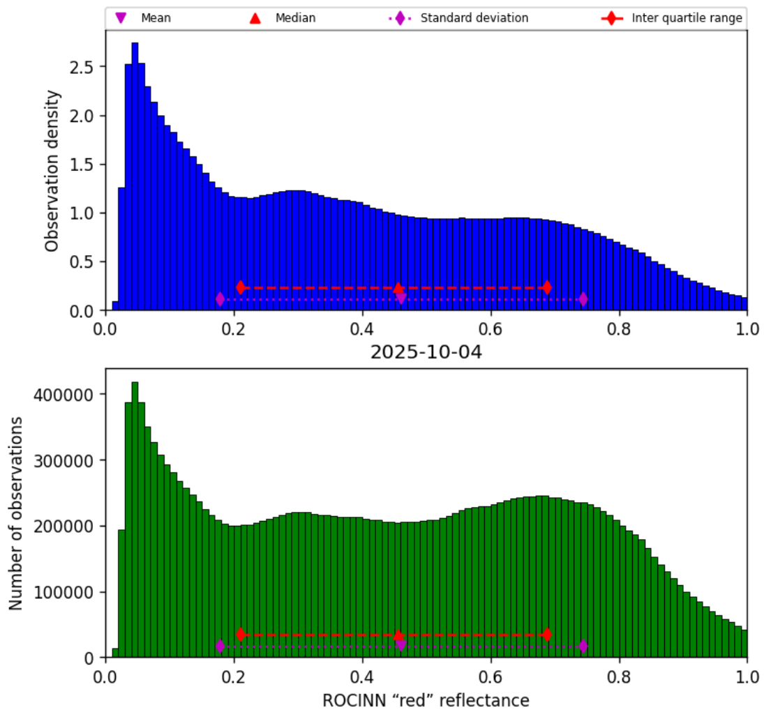
Figure 53: Histogram of “ROCINN “red” reflectance” for 2025-10-03 to 2025-10-05
