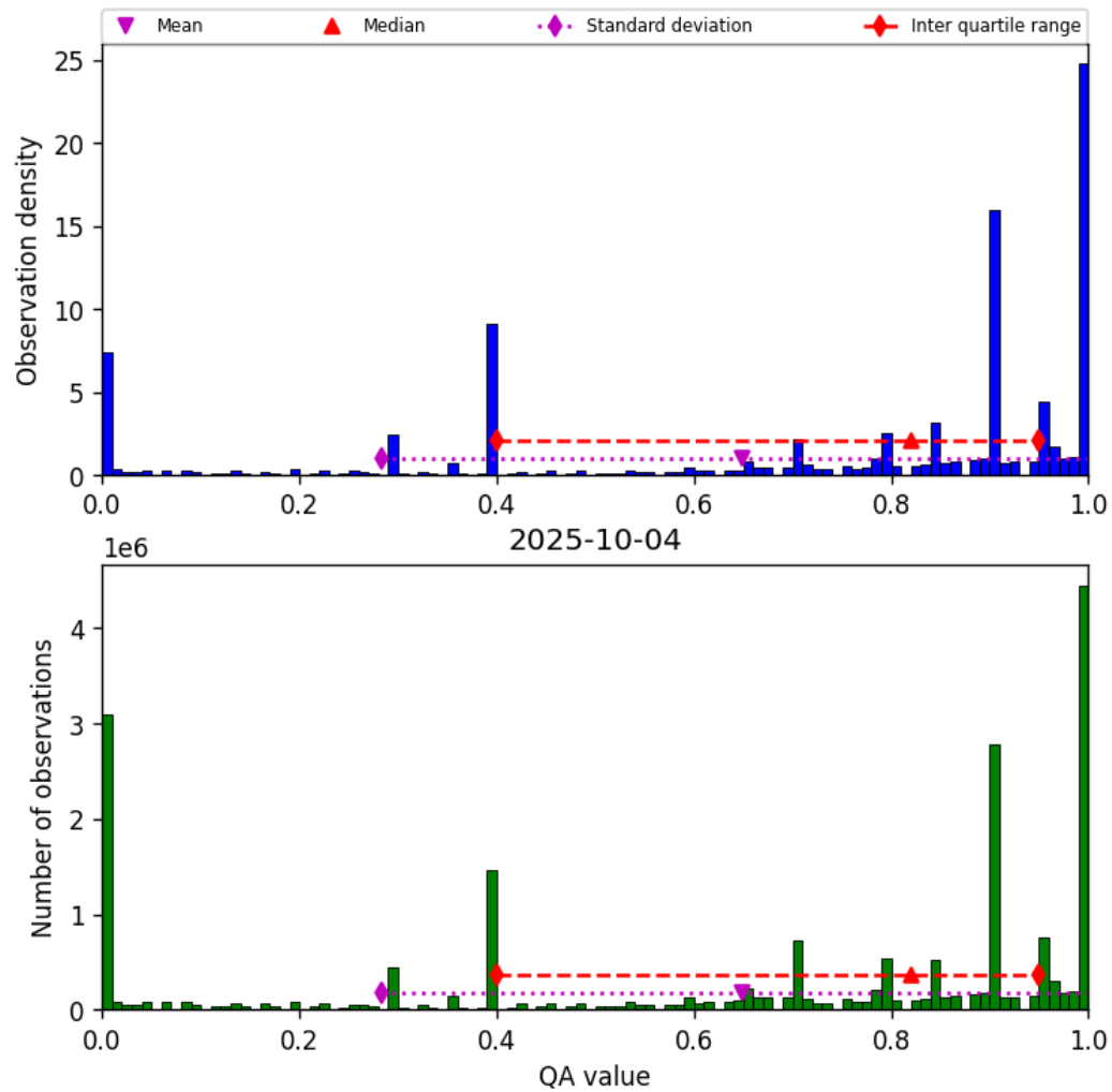
Figure 38: Histogram of “QA value” for 2025-10-03 to 2025-10-05
