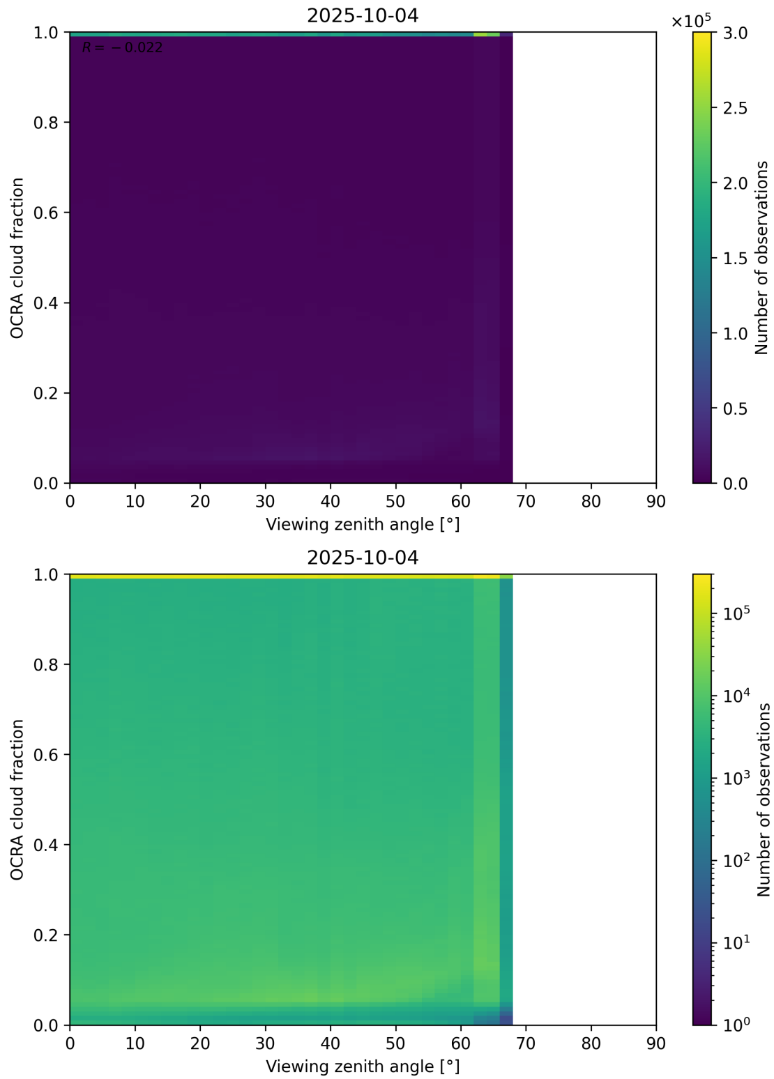
Figure 108: Scatter density plot of “Viewing zenith angle” against “OCRA cloud fraction” for 2025-10-03 to 2025-10-05.
