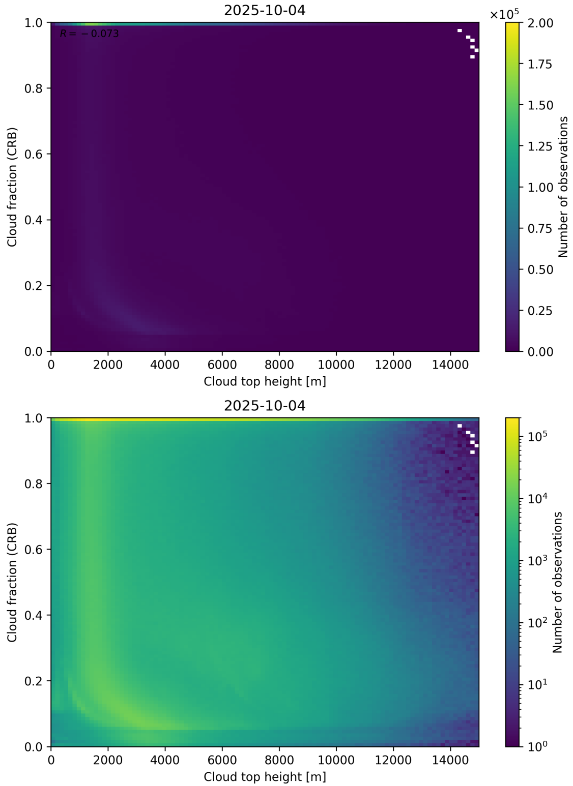
Figure 88: Scatter density plot of “Cloud top height” against “Cloud fraction (CRB)” for 2025-10-03 to 2025-10-05.
