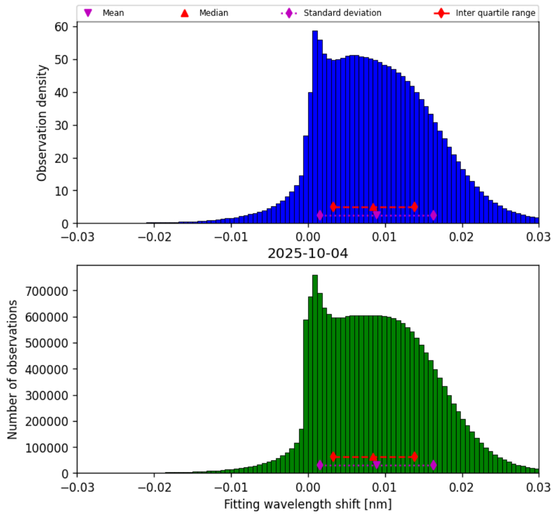
Figure 49: Histogram of “Fitting wavelength shift” for 2025-10-03 to 2025-10-05
