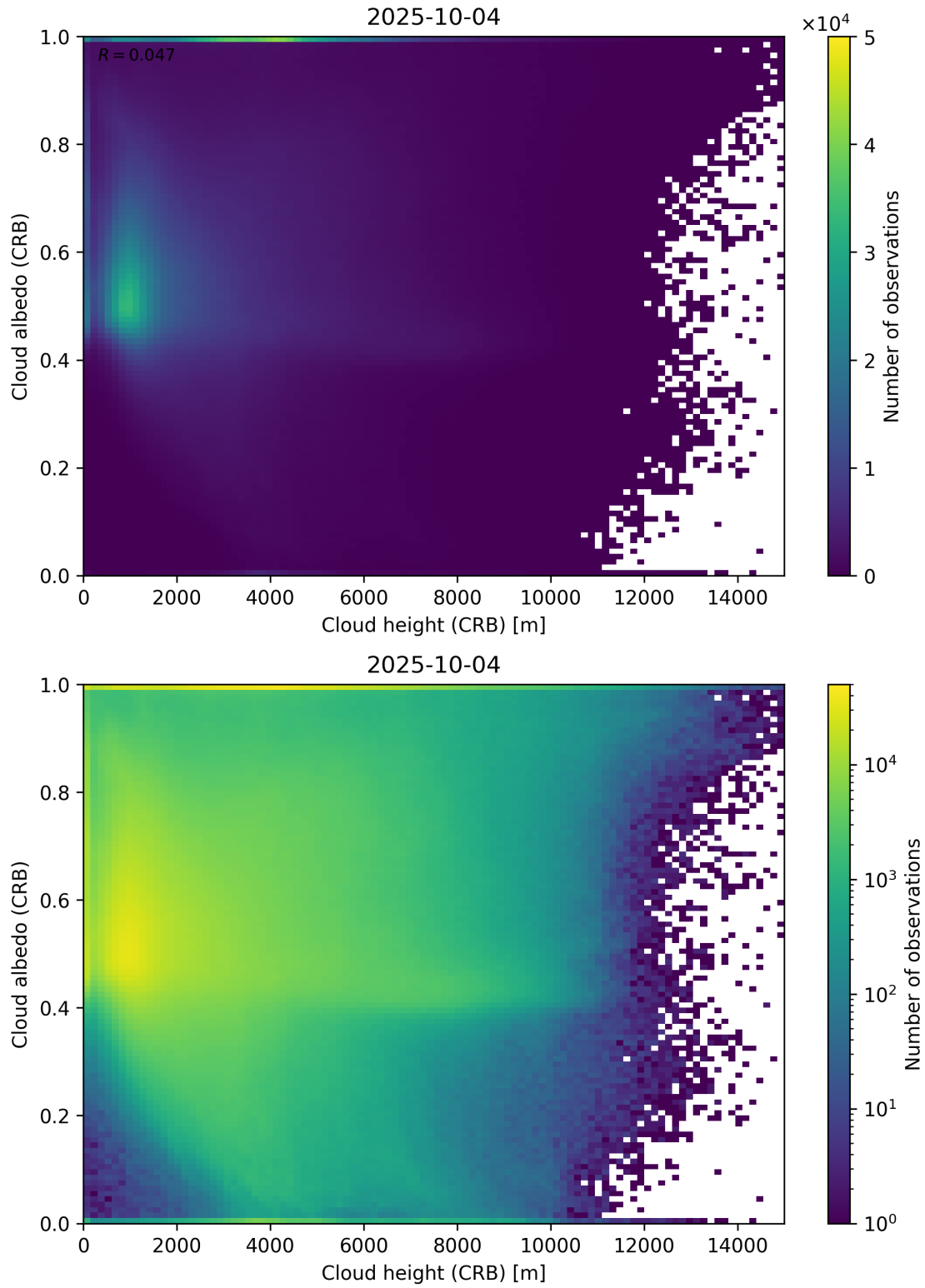
Figure 80: Scatter density plot of “Cloud height (CRB)” against “Cloud albedo (CRB)” for 2025-10-03 to 2025-10-05.
