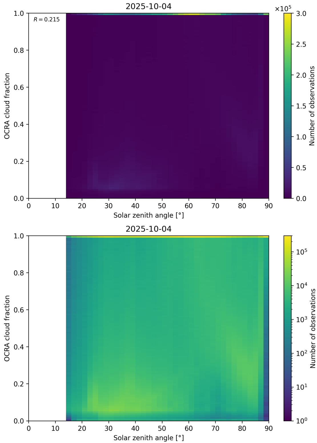
Figure 100: Scatter density plot of “Solar zenith angle” against “OCRA cloud fraction” for 2025-10-03 to 2025-10-05.
