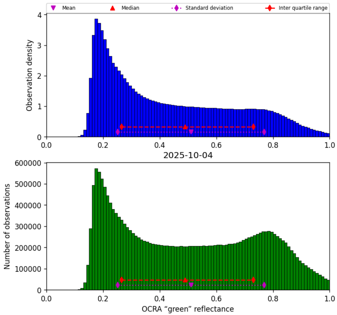
Figure 52: Histogram of “OCRA “green” reflectance” for 2025-10-03 to 2025-10-05
