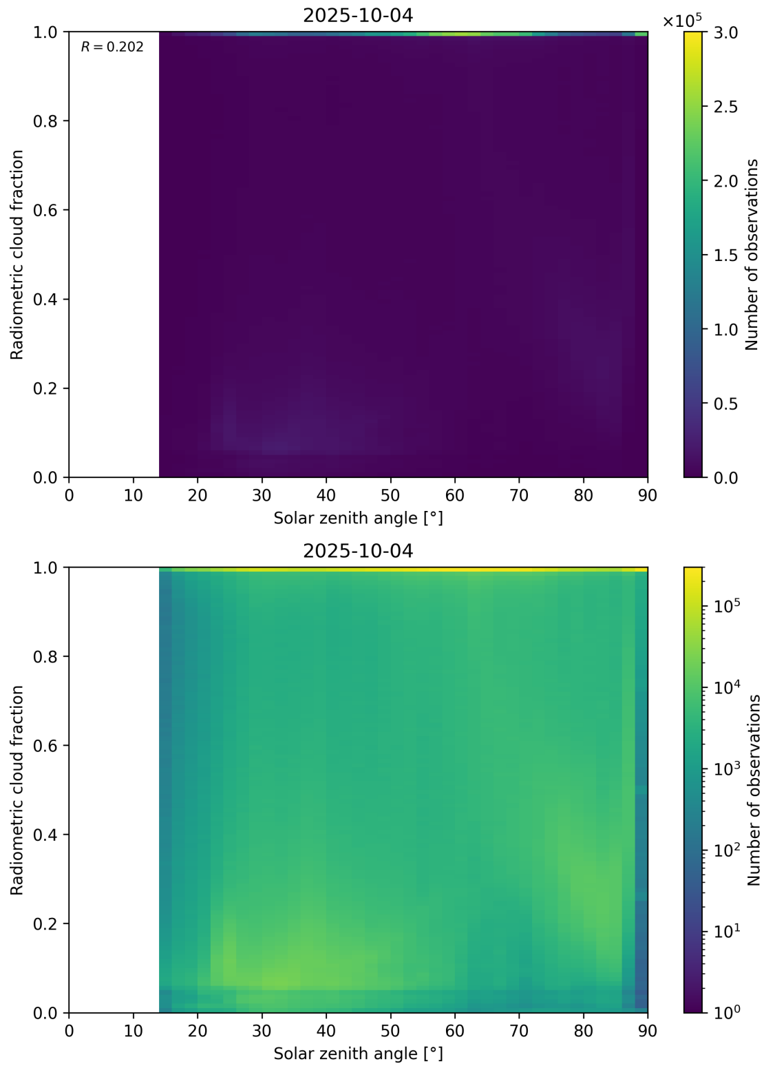
Figure 99: Scatter density plot of “Solar zenith angle” against “Radiometric cloud fraction” for 2025-10-03 to 2025-10-05.
