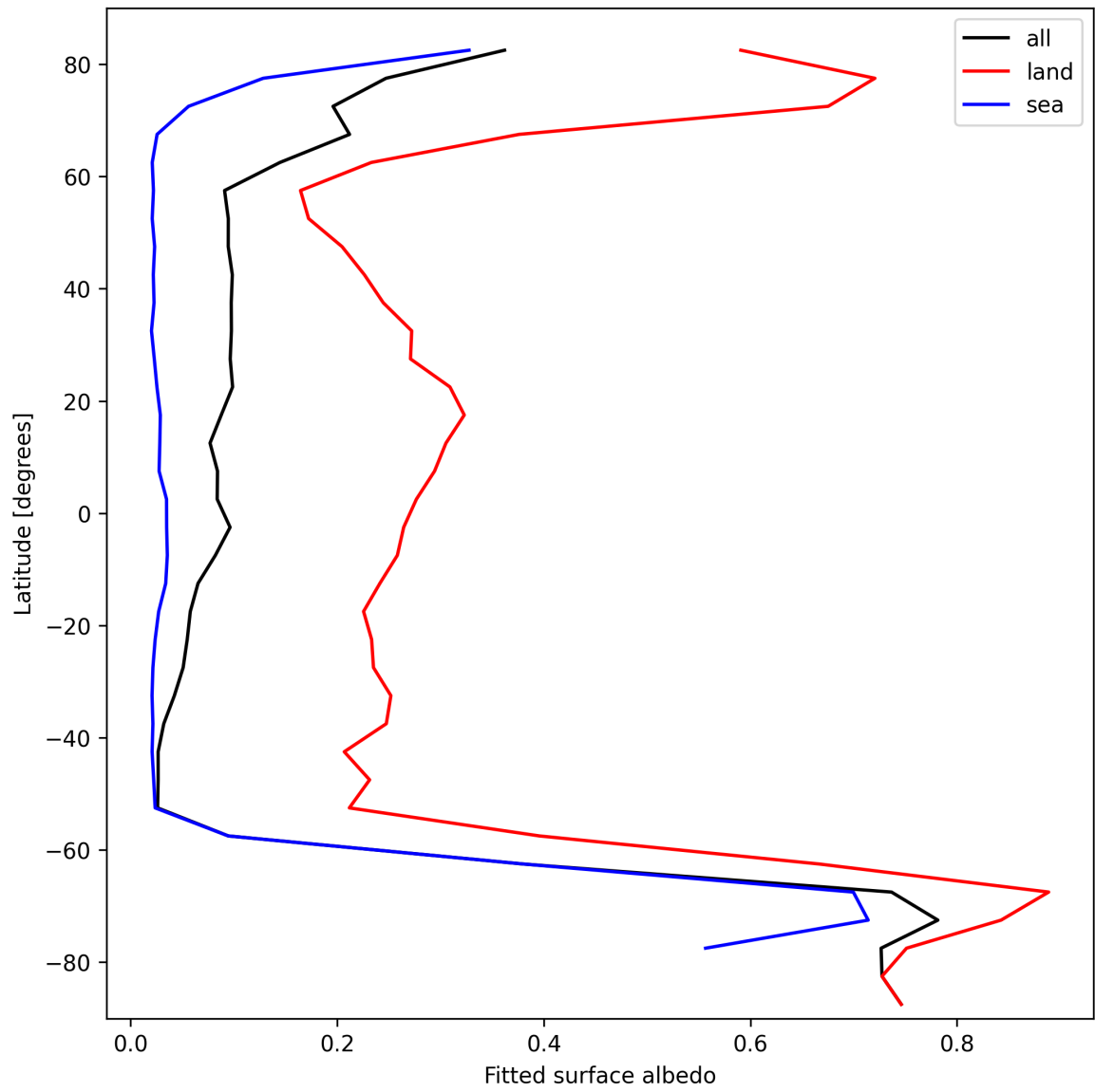
Figure 29: Zonal average of “Fitted surface albedo” for 2025-10-03 to 2025-10-05.
