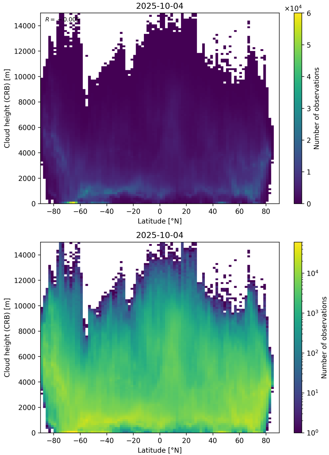
Figure 95: Scatter density plot of “Latitude” against “Cloud height (CRB)” for 2025-10-03 to 2025-10-05.
