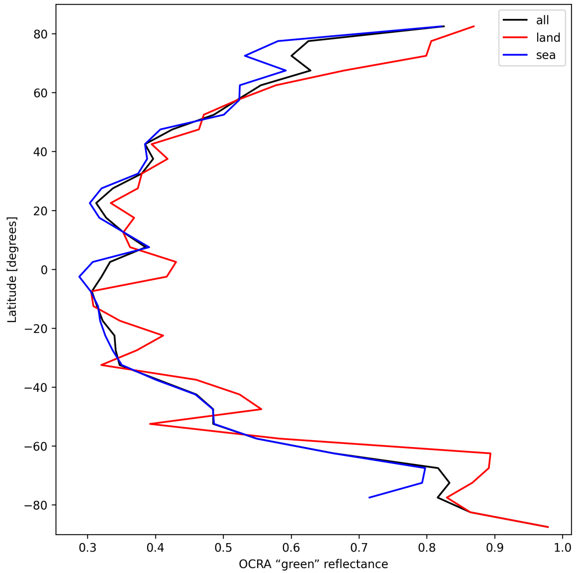
Figure 36: Zonal average of “OCRA “green” reflectance” for 2025-10-03 to 2025-10-05.
