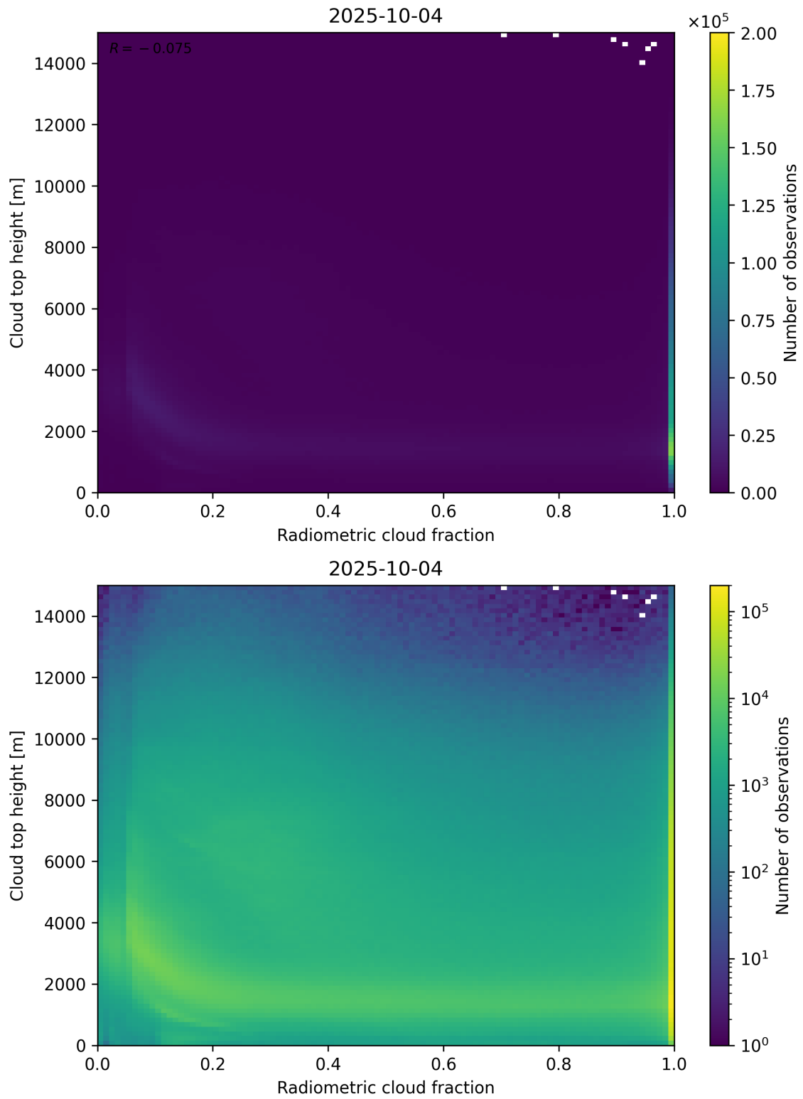
Figure 76: Scatter density plot of “Radiometric cloud fraction” against “Cloud top height” for 2025-10-03 to 2025-10-05.
