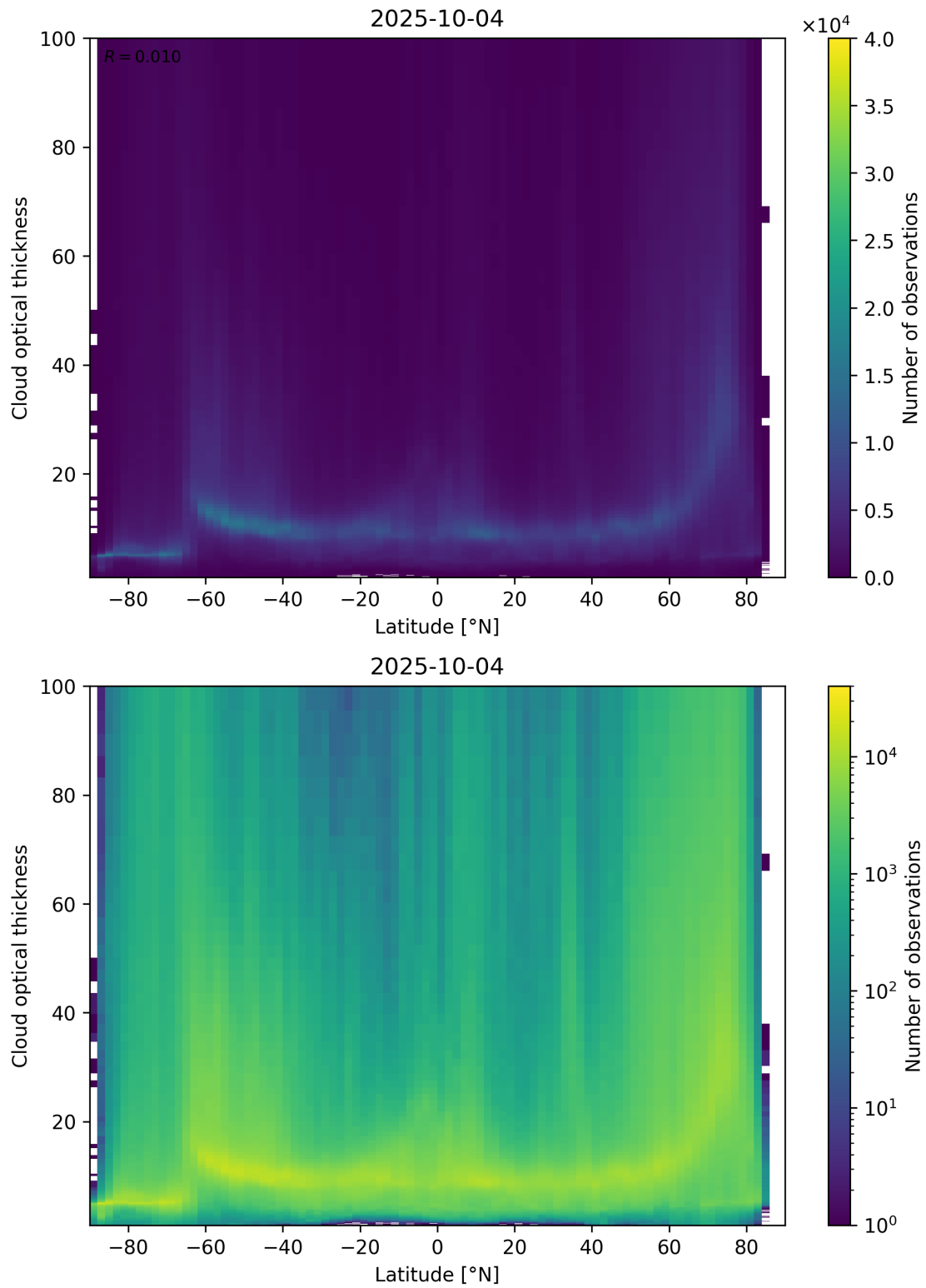
Figure 96: Scatter density plot of “Latitude” against “Cloud optical thickness” for 2025-10-03 to 2025-10-05.
