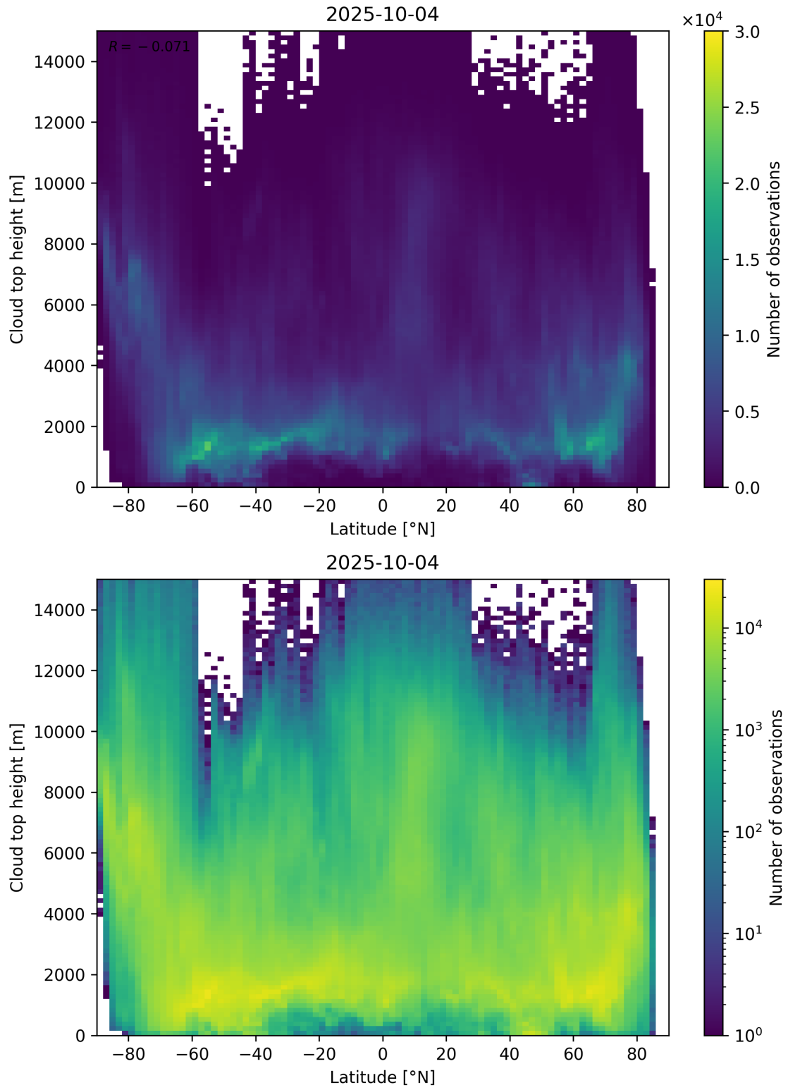
Figure 97: Scatter density plot of “Latitude” against “Cloud top height” for 2025-10-03 to 2025-10-05.
