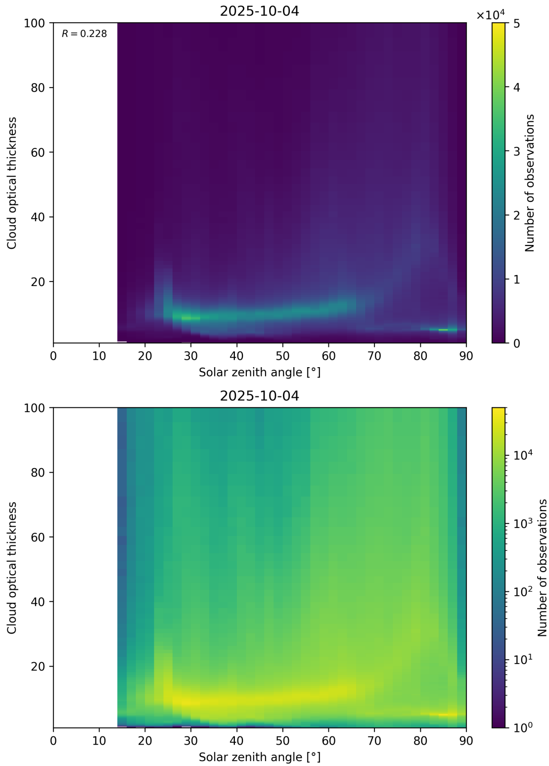
Figure 103: Scatter density plot of “Solar zenith angle” against “Cloud optical thickness” for 2025-10-03 to 2025-10-05.
