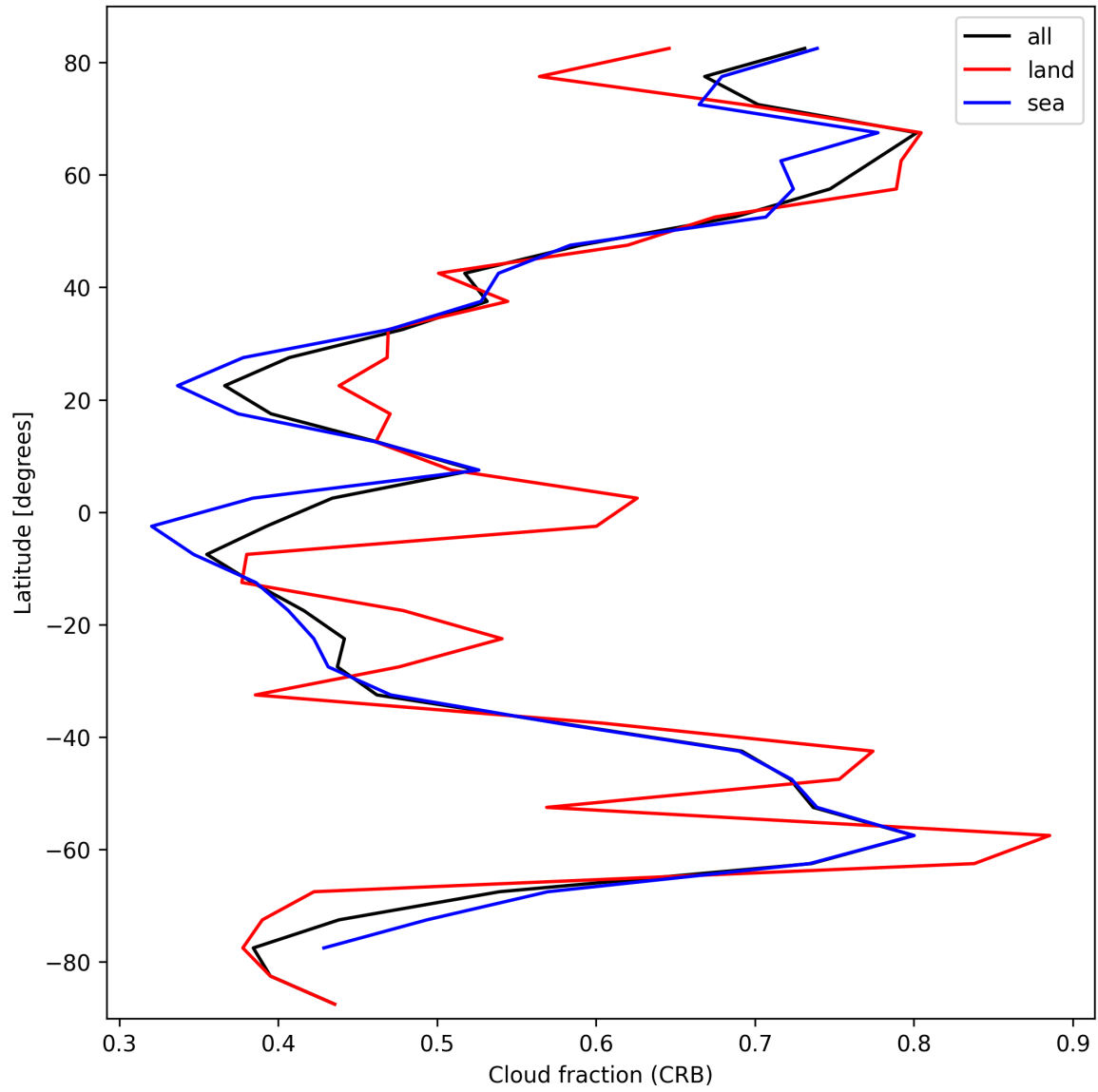
Figure 26: Zonal average of “Cloud fraction (CRB)” for 2025-10-03 to 2025-10-05.
