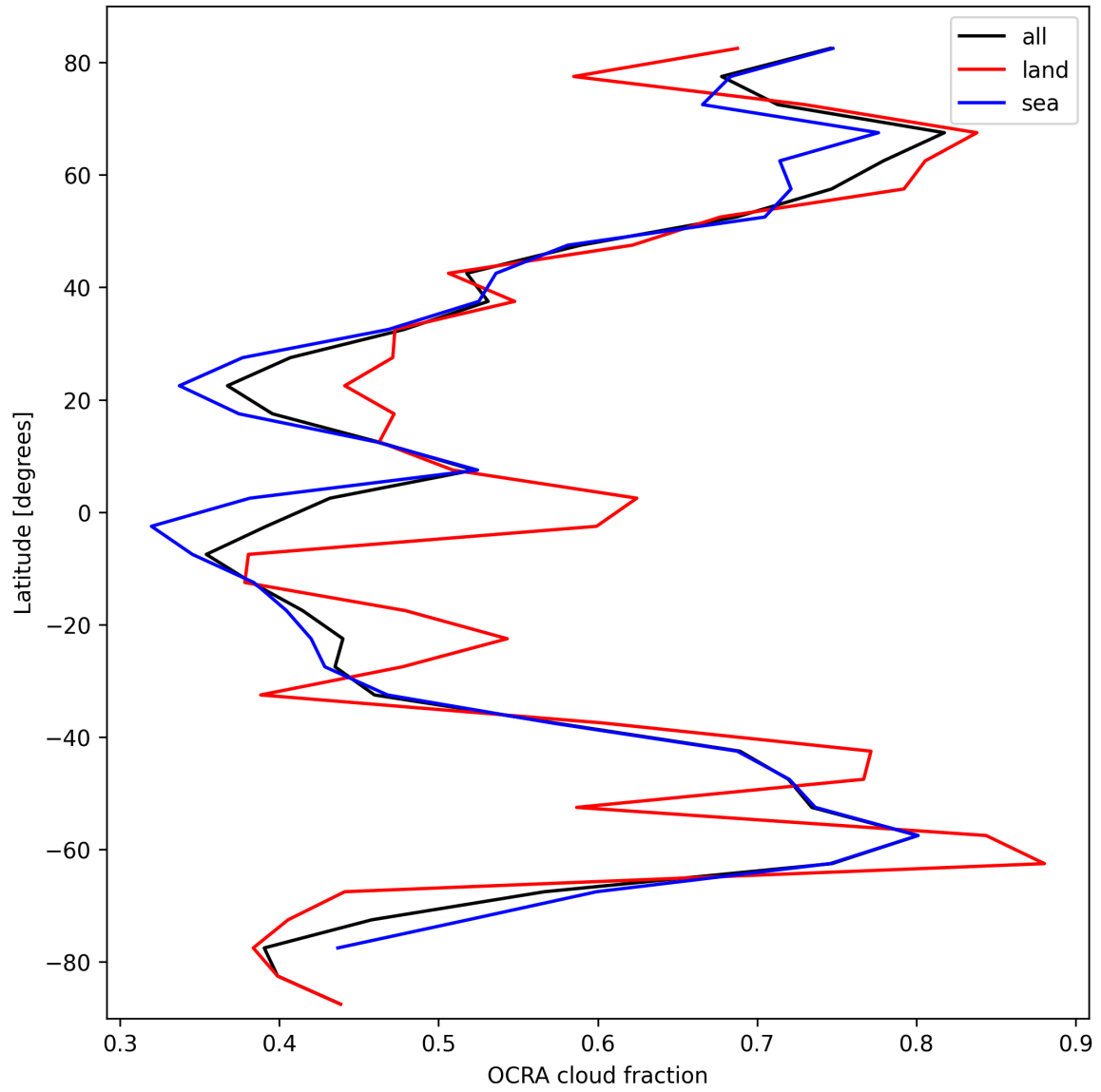
Figure 34: Zonal average of “OCRA cloud fraction” for 2025-10-03 to 2025-10-05.
