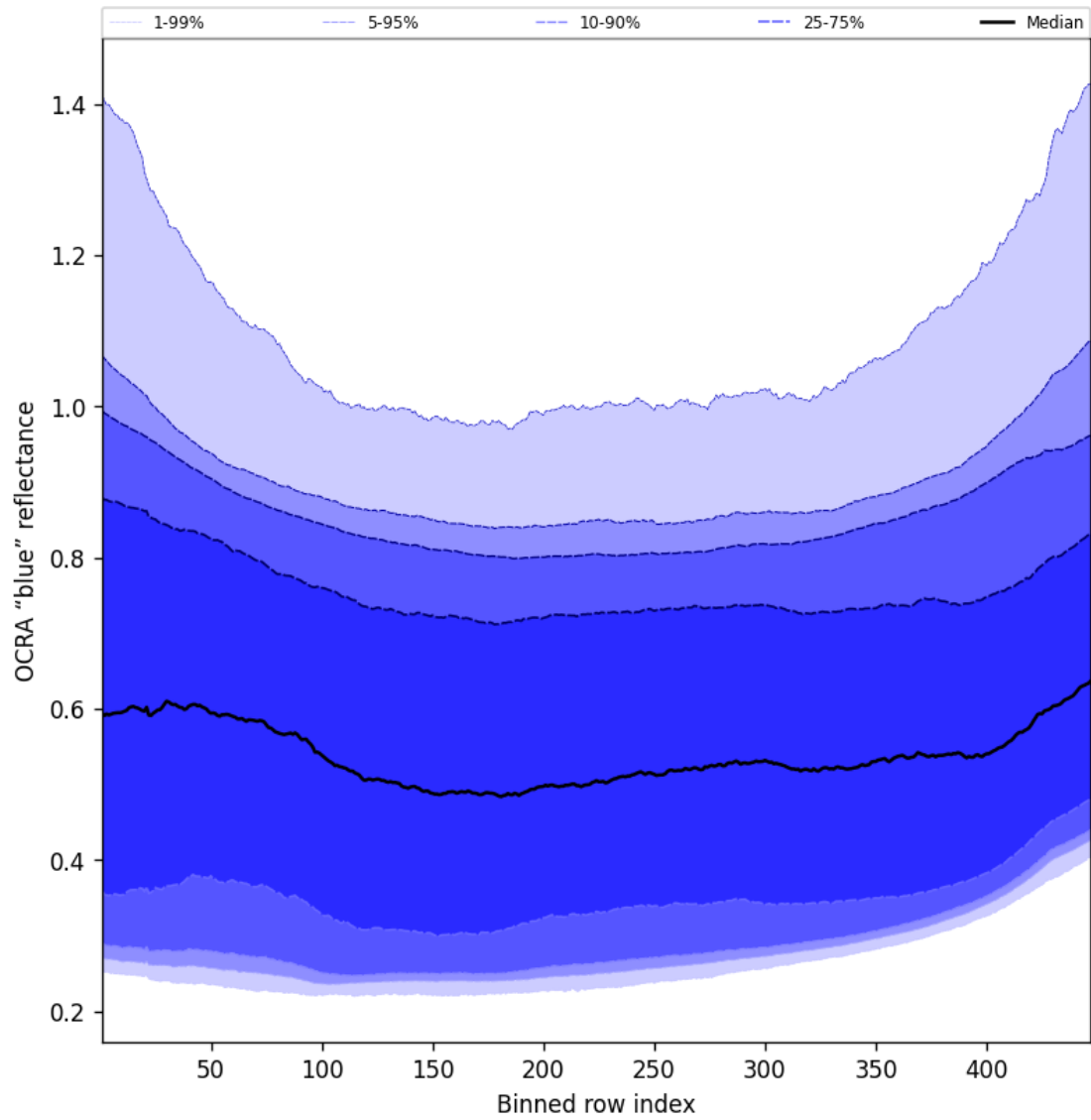
Figure 67: Along track statistics of “OCRA “blue” reflectance” for 2025-10-03 to 2025-10-05
