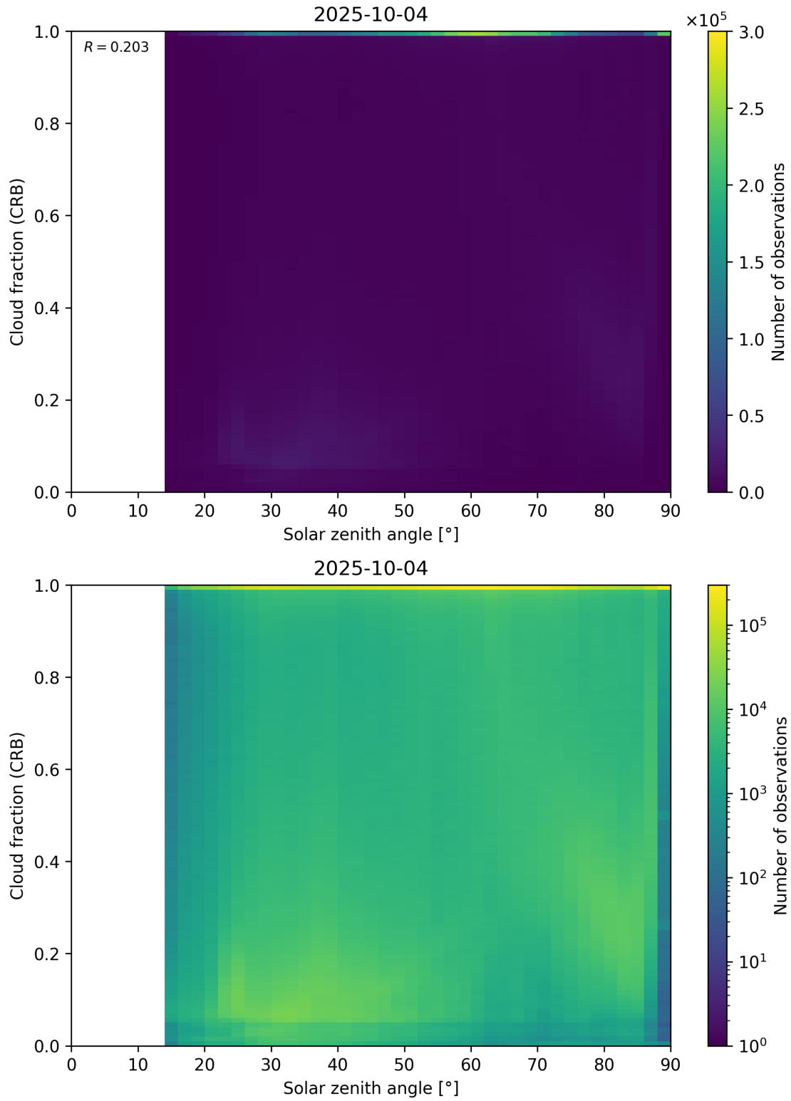
Figure 101: Scatter density plot of “Solar zenith angle” against “Cloud fraction (CRB)” for 2025-10-03 to 2025-10-05.
