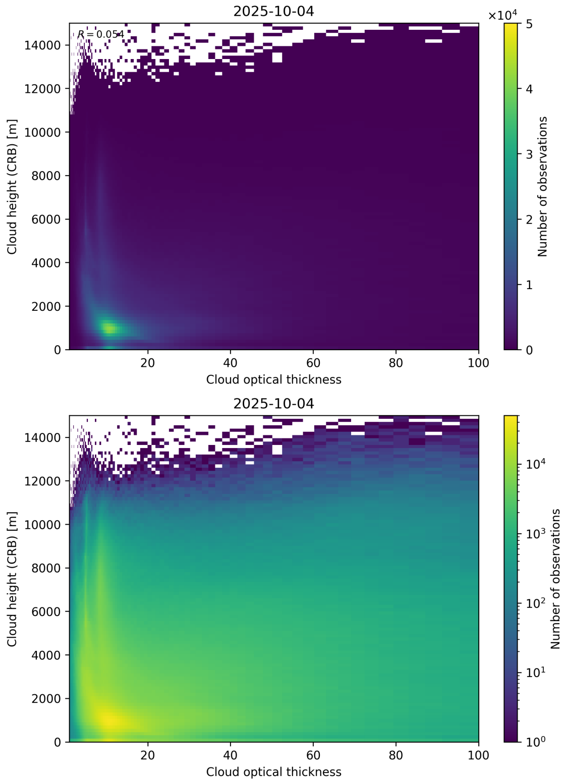
Figure 85: Scatter density plot of “Cloud optical thickness” against “Cloud height (CRB)” for 2025-10-03 to 2025-10-05.
