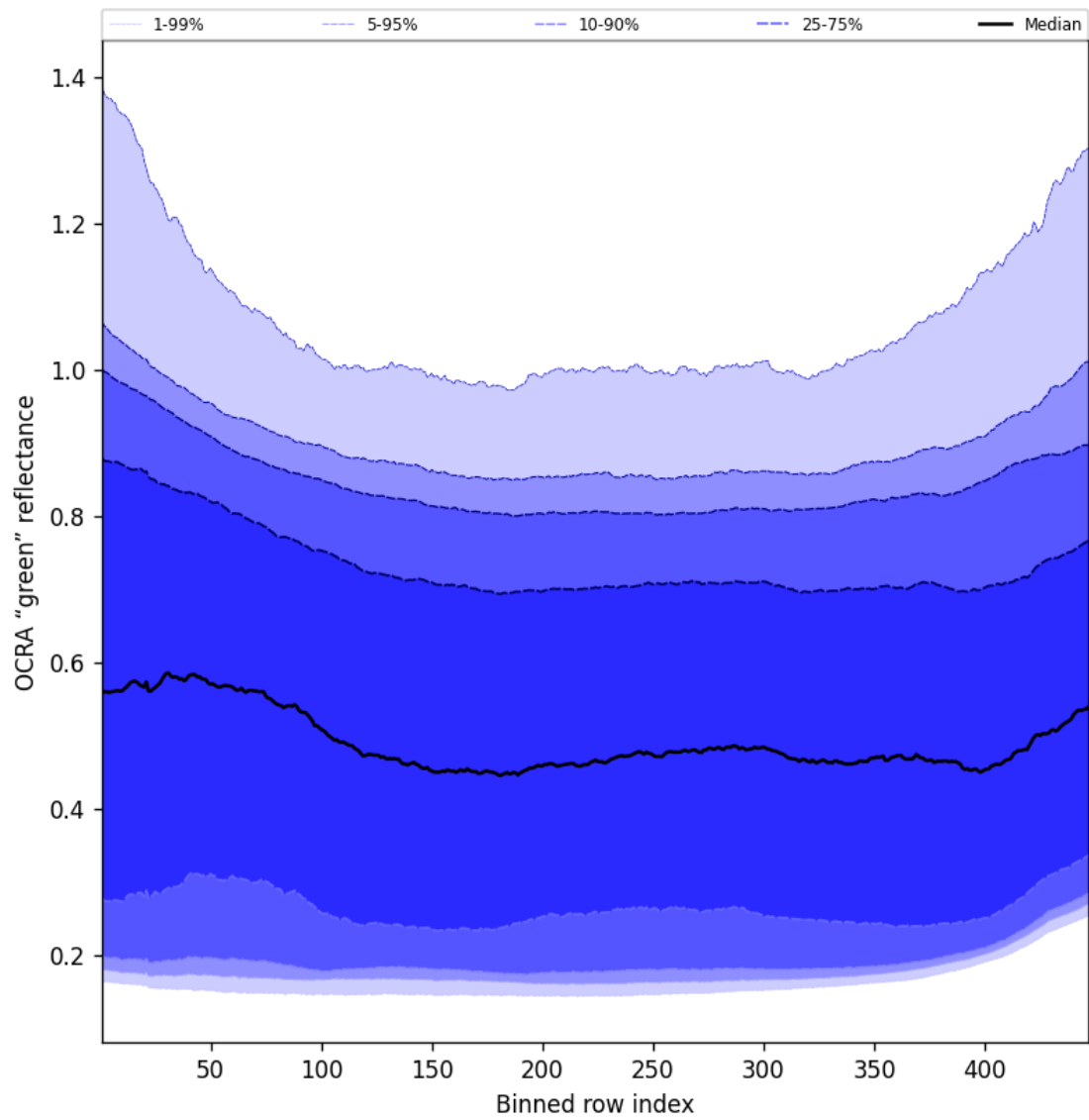
Figure 68: Along track statistics of “OCRA “green” reflectance” for 2025-10-03 to 2025-10-05
