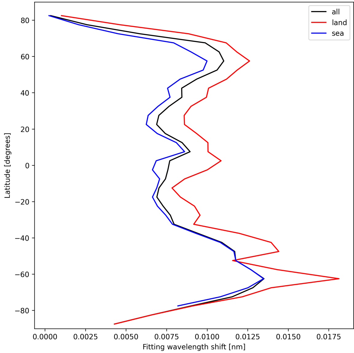
Figure 33: Zonal average of “Fitting wavelength shift” for 2025-10-03 to 2025-10-05.
