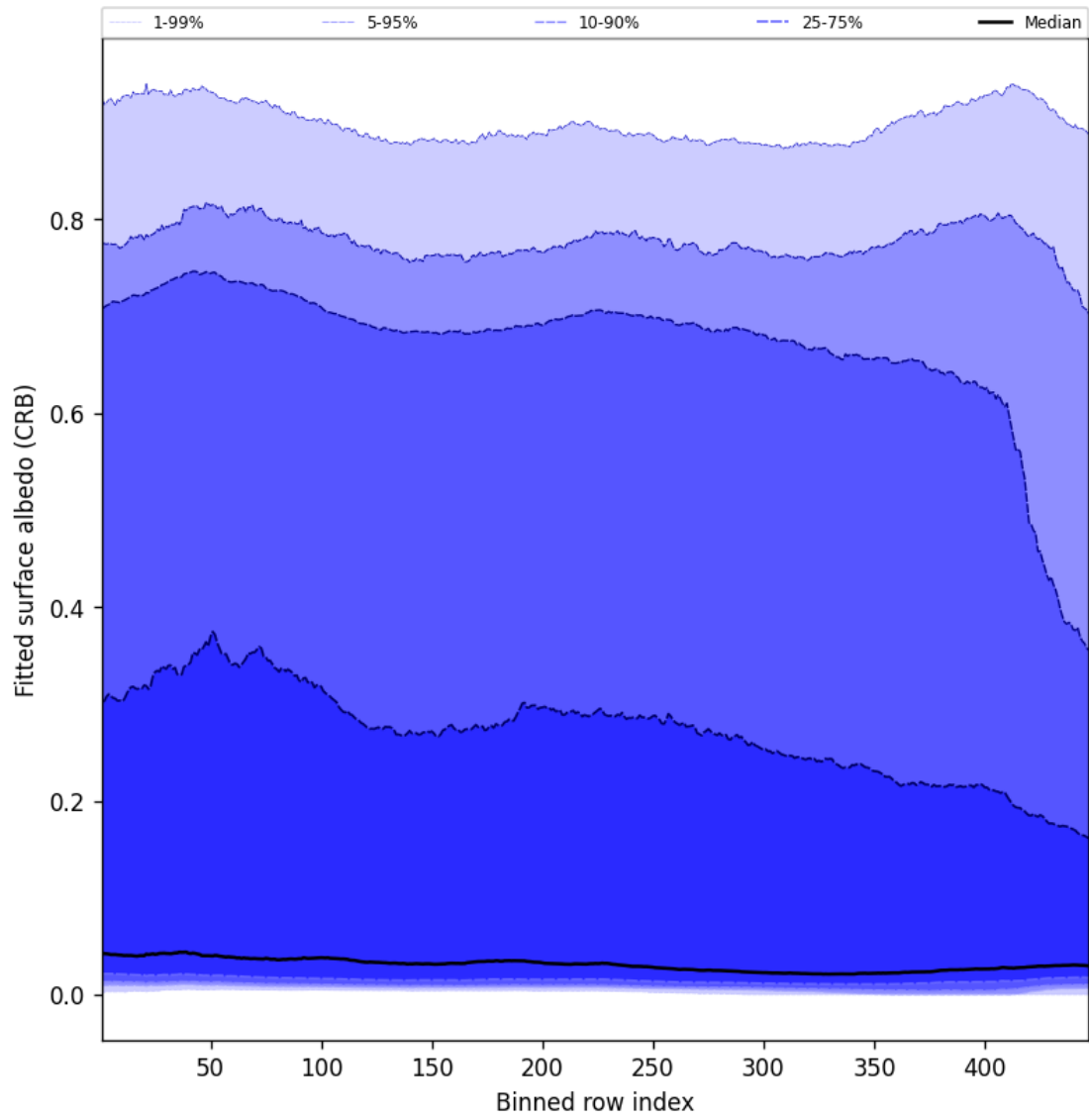
Figure 62: Along track statistics of “Fitted surface albedo (CRB)” for 2025-10-03 to 2025-10-05
