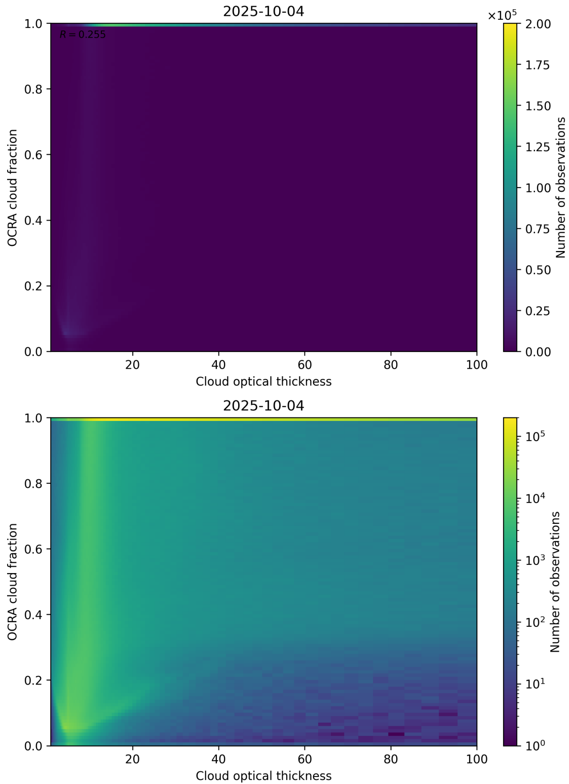
Figure 83: Scatter density plot of “Cloud optical thickness” against “OCRA cloud fraction” for 2025-10-03 to 2025-10-05.
