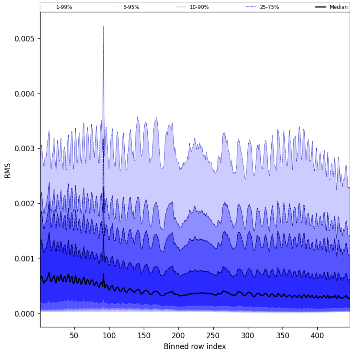
Figure 63: Along track statistics of “RMS” for 2025-10-03 to 2025-10-05
