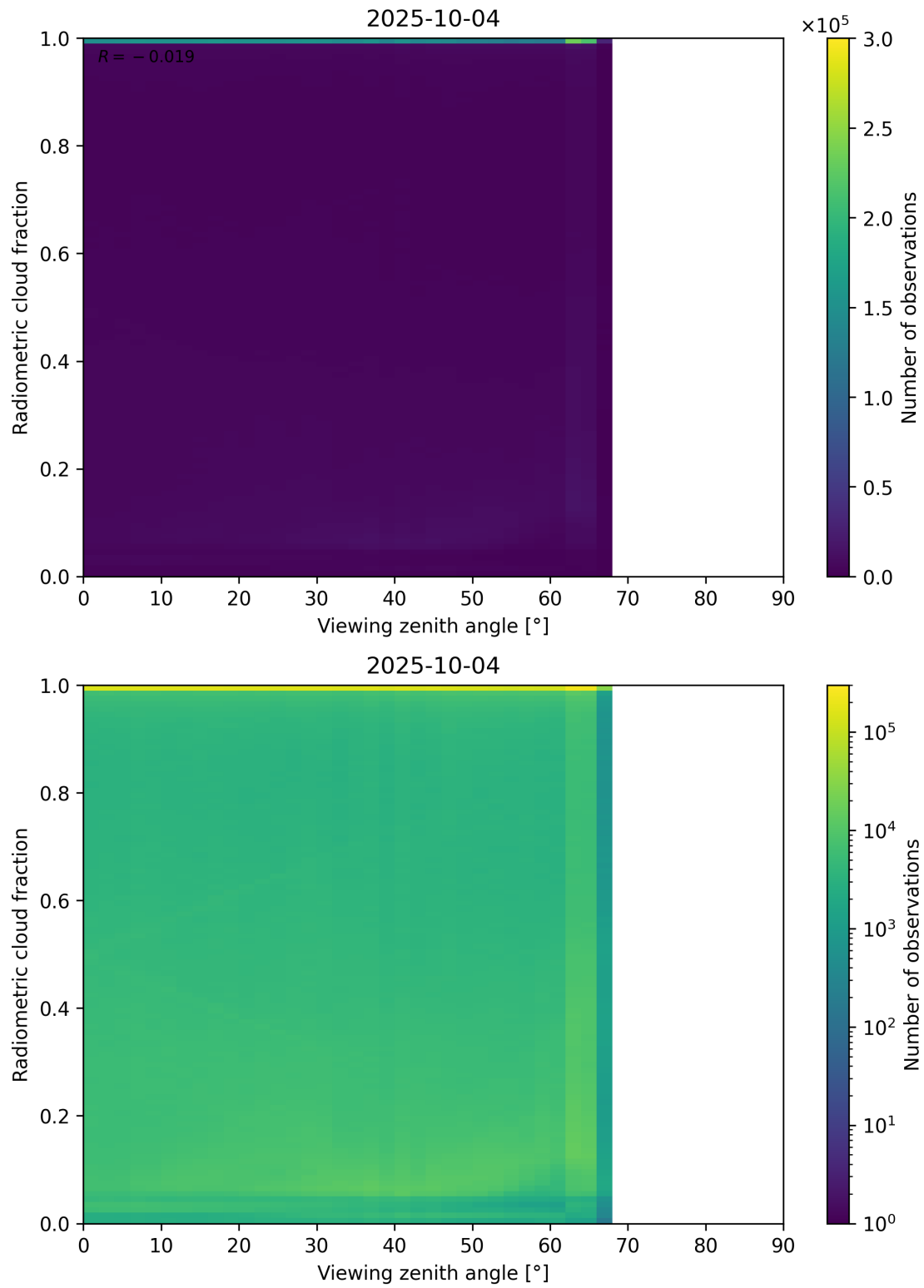
Figure 107: Scatter density plot of “Viewing zenith angle” against “Radiometric cloud fraction” for 2025-10-03 to 2025-10-05.
