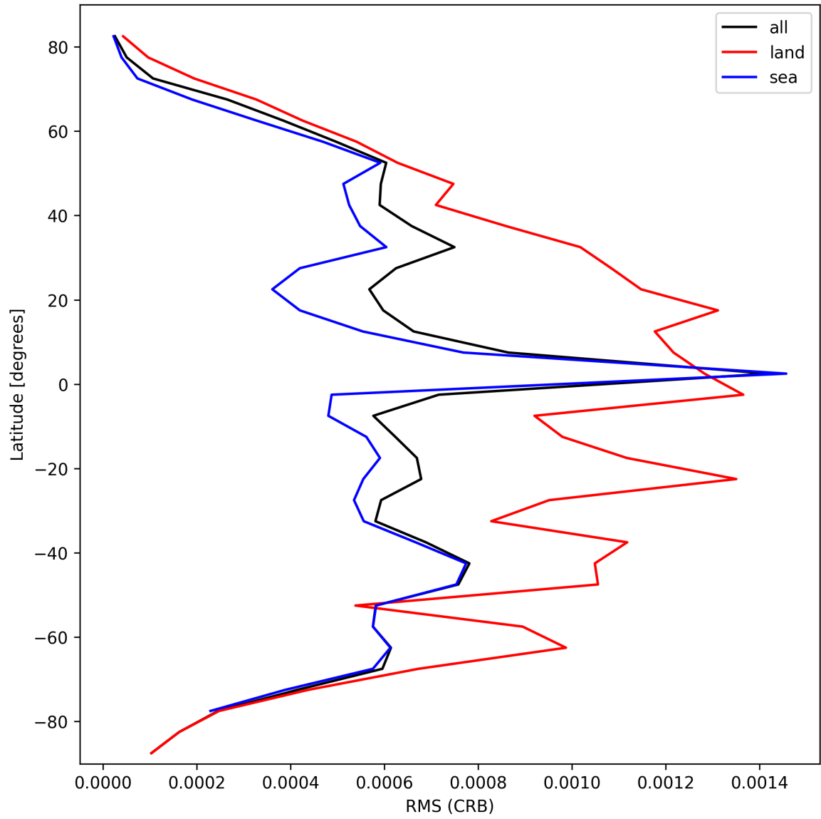
Figure 32: Zonal average of “RMS (CRB)” for 2025-10-03 to 2025-10-05.
