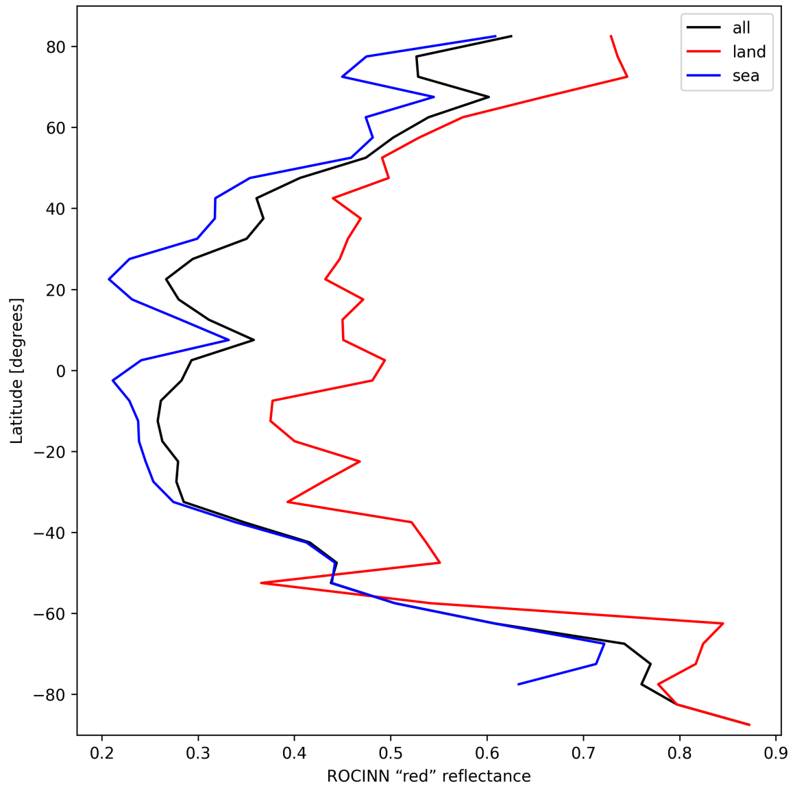
Figure 37: Zonal average of “ROCINN “red” reflectance” for 2025-10-03 to 2025-10-05.
