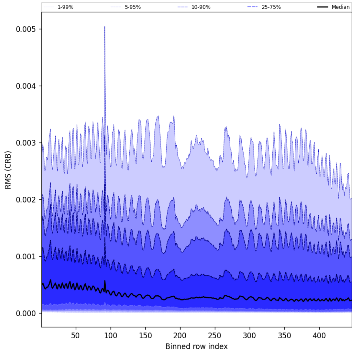
Figure 64: Along track statistics of “RMS (CRB)” for 2025-10-03 to 2025-10-05
