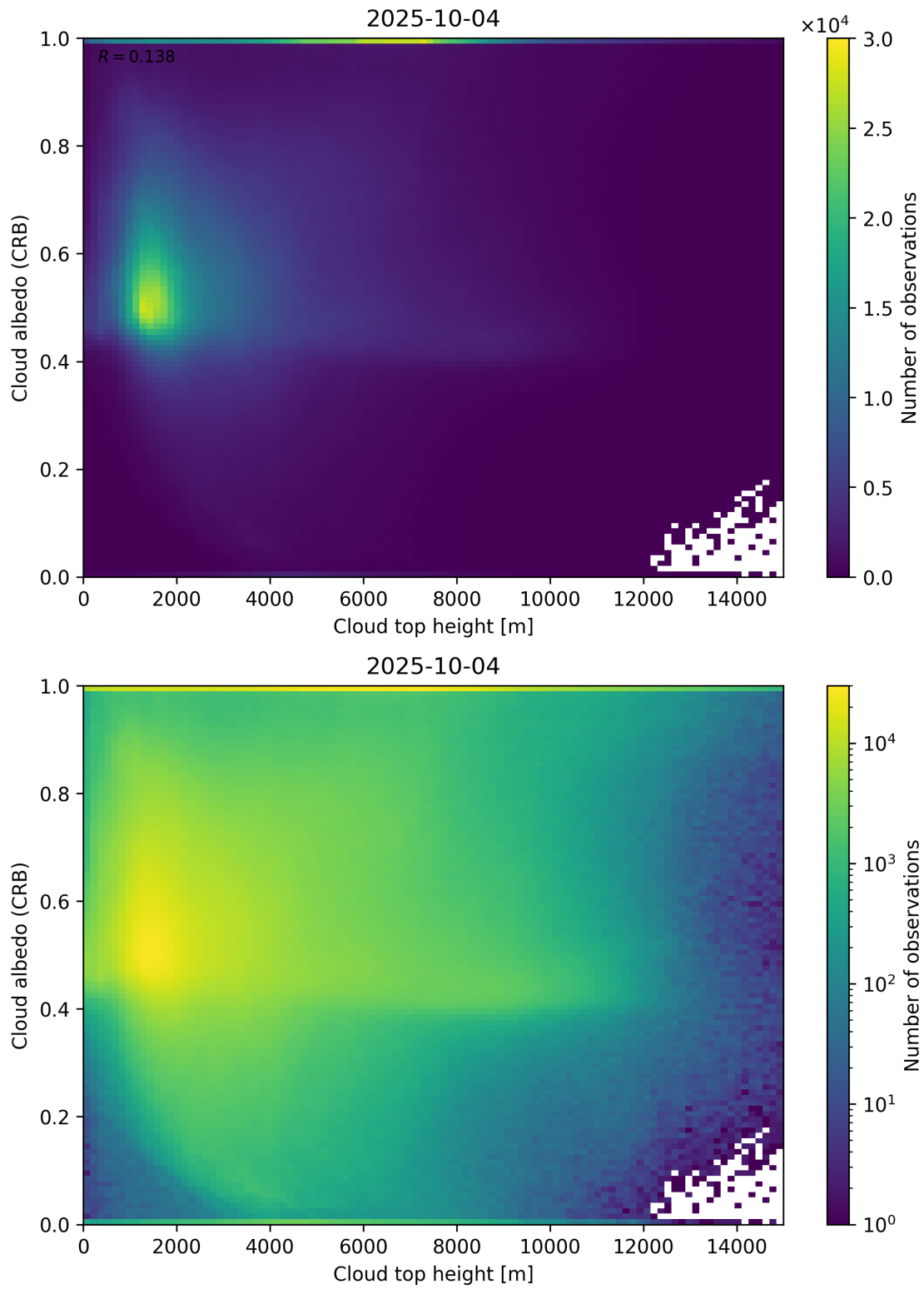
Figure 86: Scatter density plot of “Cloud top height” against “Cloud albedo (CRB)” for 2025-10-03 to 2025-10-05.
