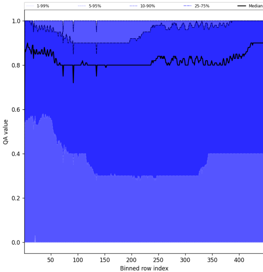
Figure 54: Along track statistics of “QA value” for 2025-10-03 to 2025-10-05
