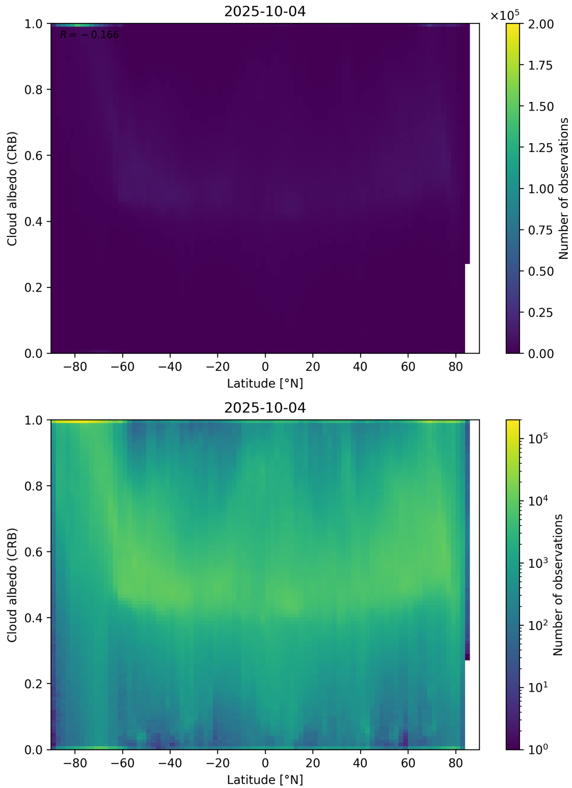
Figure 91: Scatter density plot of “Latitude” against “Cloud albedo (CRB)” for 2025-10-03 to 2025-10-05.
