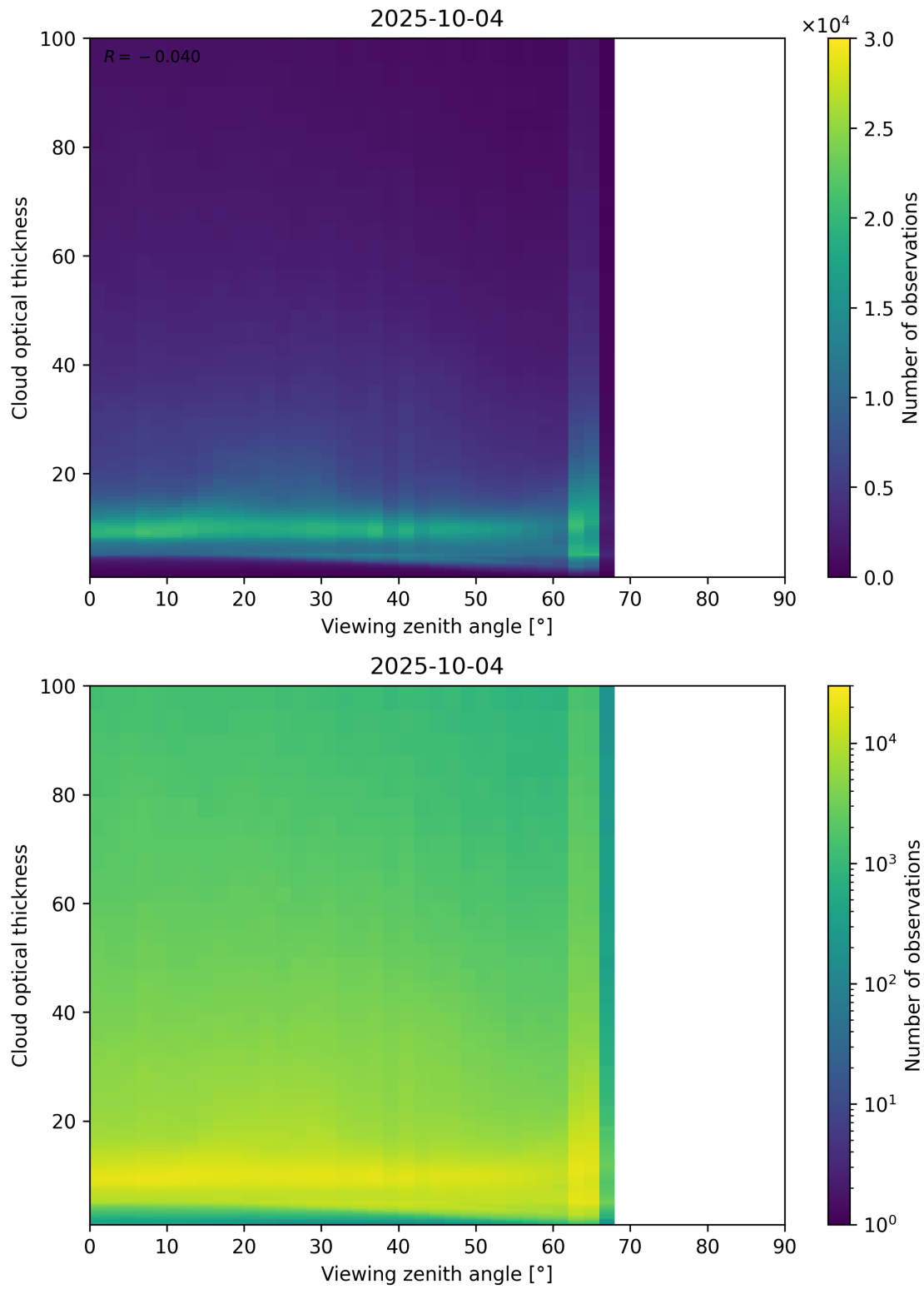
Figure 111: Scatter density plot of “Viewing zenith angle” against “Cloud optical thickness” for 2025-10-03 to 2025-10-05.
