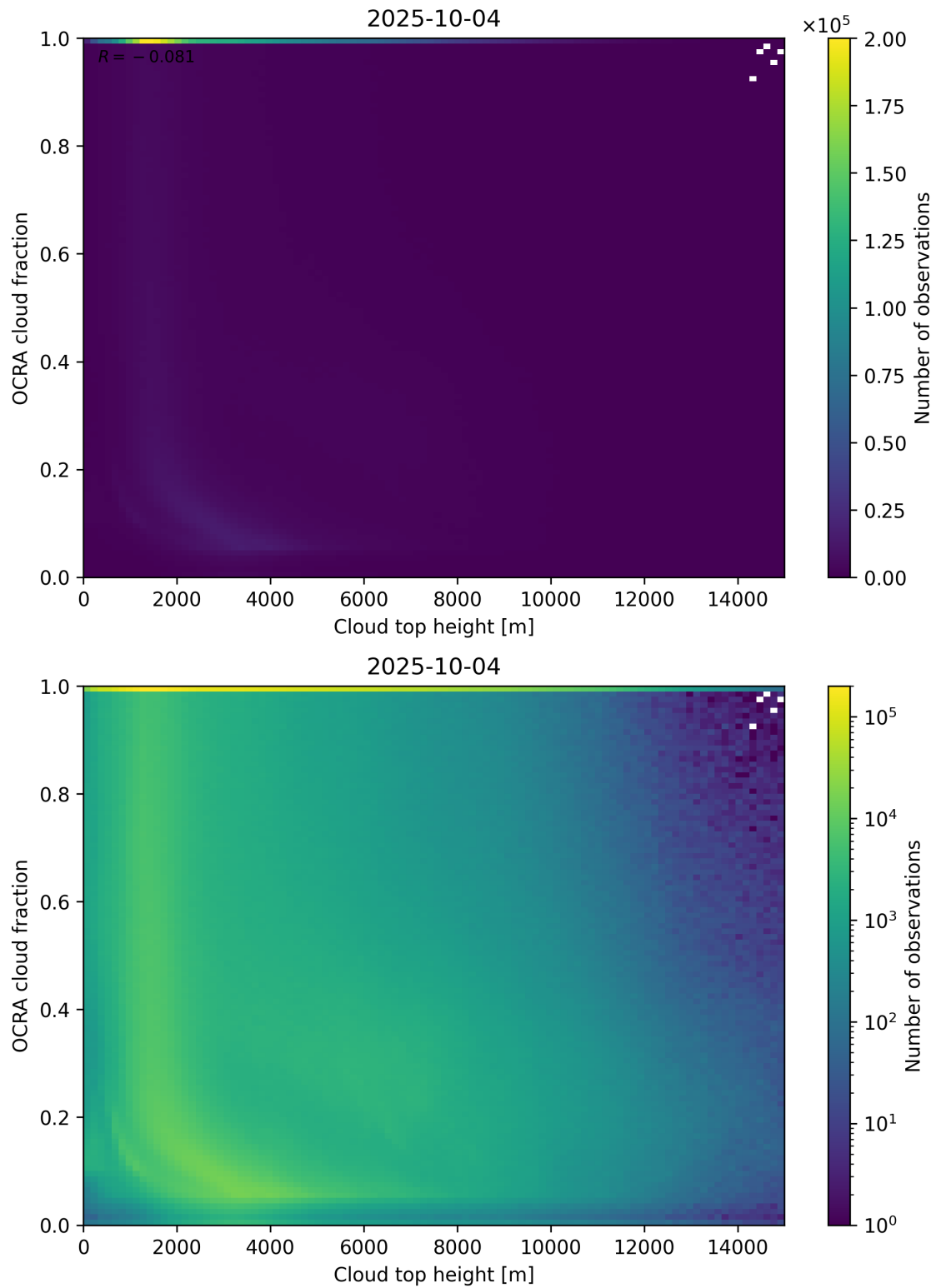
Figure 87: Scatter density plot of “Cloud top height” against “OCRA cloud fraction” for 2025-10-03 to 2025-10-05.
