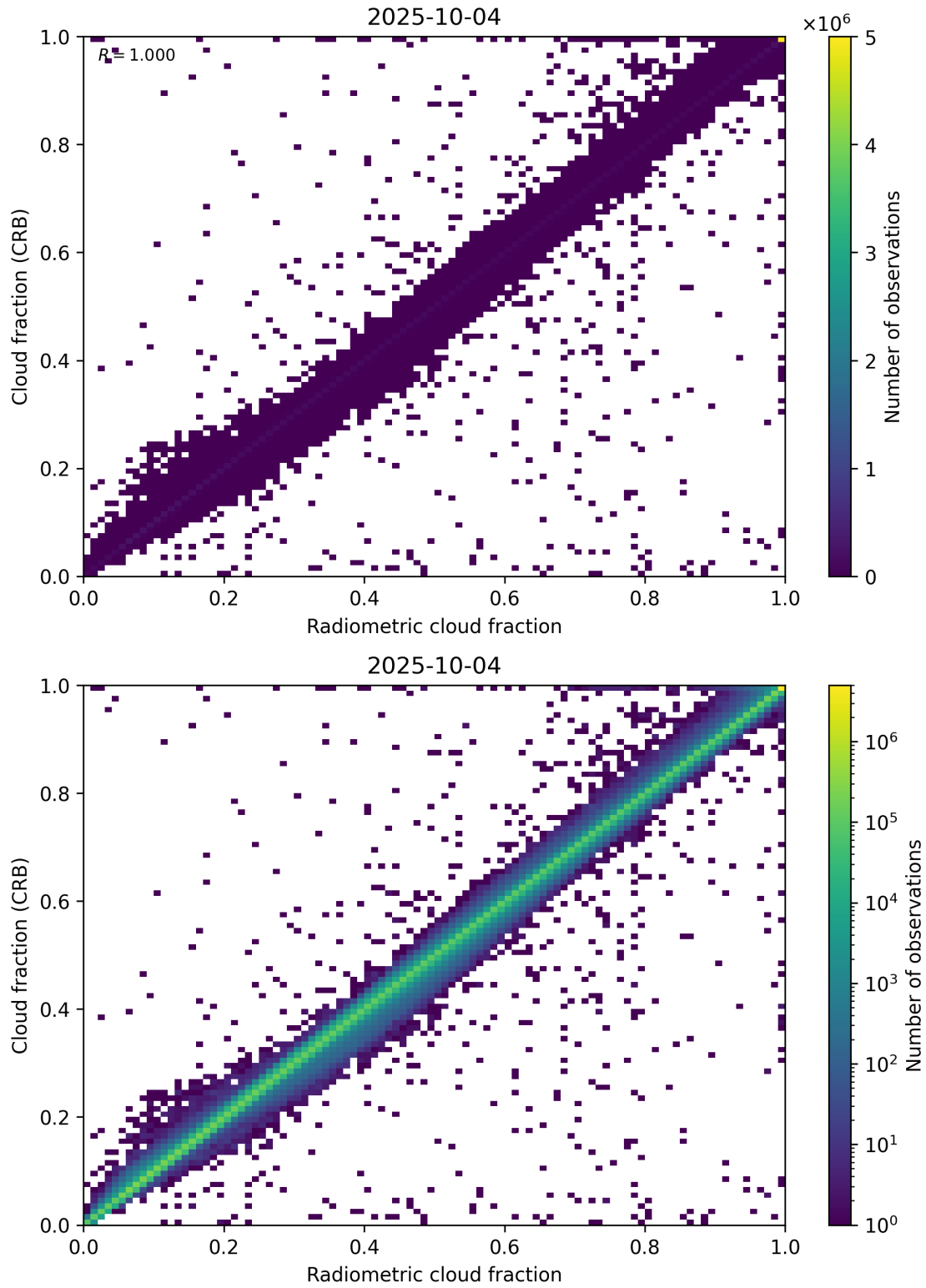
Figure 73: Scatter density plot of “Radiometric cloud fraction” against “Cloud fraction (CRB)” for 2025-10-03 to 2025-10-05.
