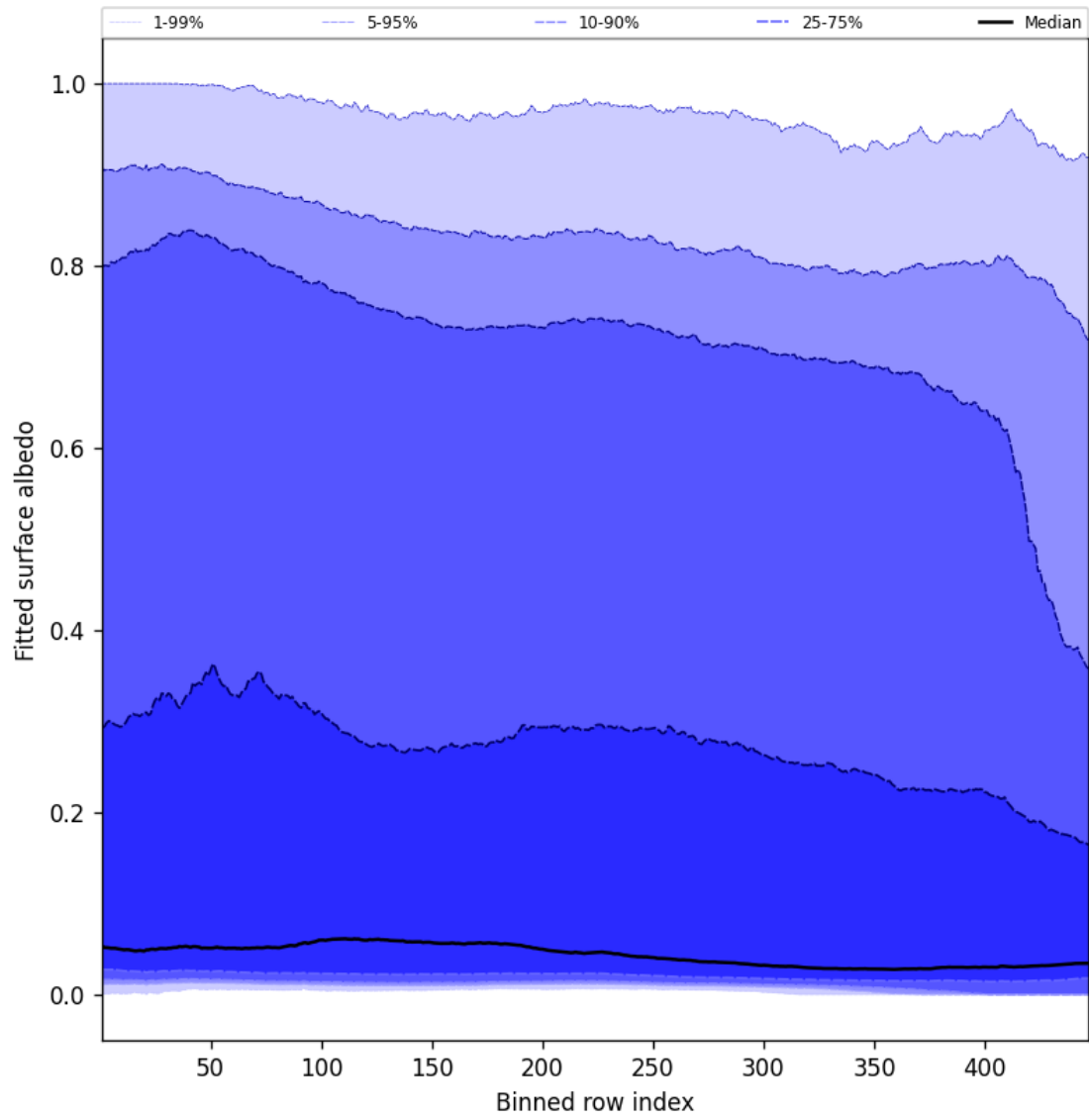
Figure 61: Along track statistics of “Fitted surface albedo” for 2025-10-03 to 2025-10-05
