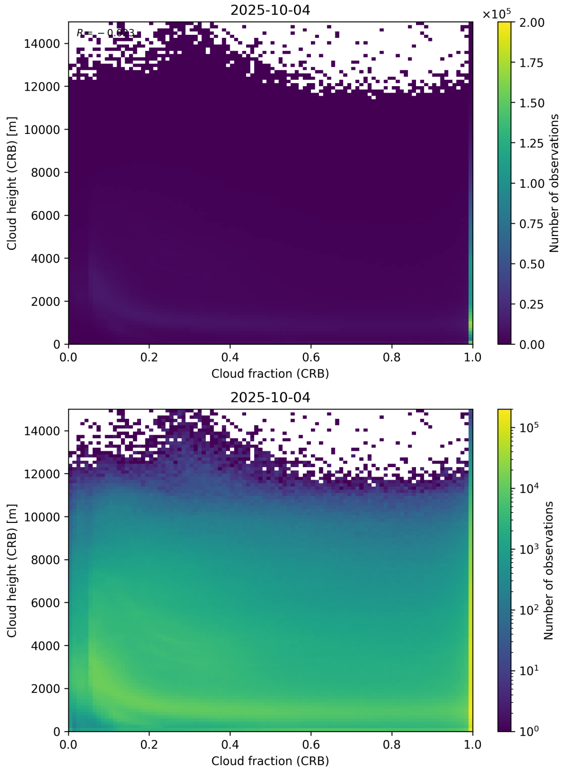
Figure 79: Scatter density plot of “Cloud fraction (CRB)” against “Cloud height (CRB)” for 2025-10-03 to 2025-10-05.
