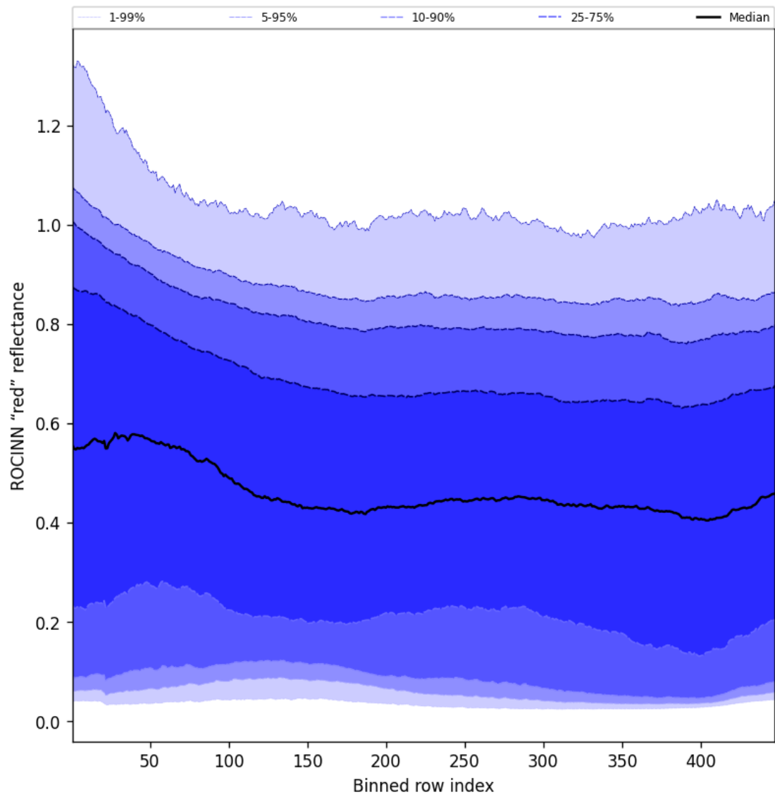
Figure 69: Along track statistics of “ROCINN “red” reflectance” for 2025-10-03 to 2025-10-05
