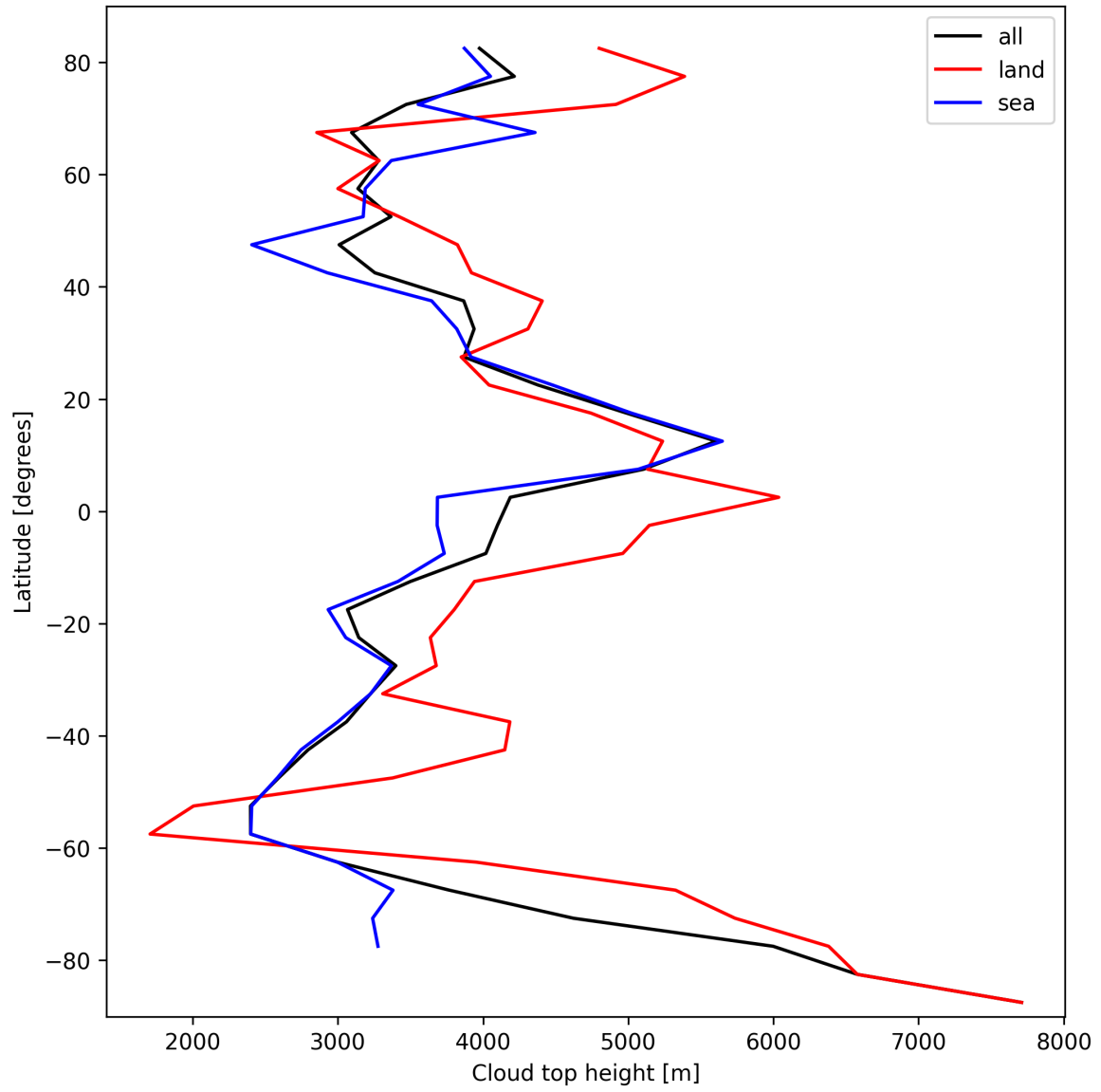
Figure 24: Zonal average of “Cloud top height” for 2025-10-03 to 2025-10-05.
