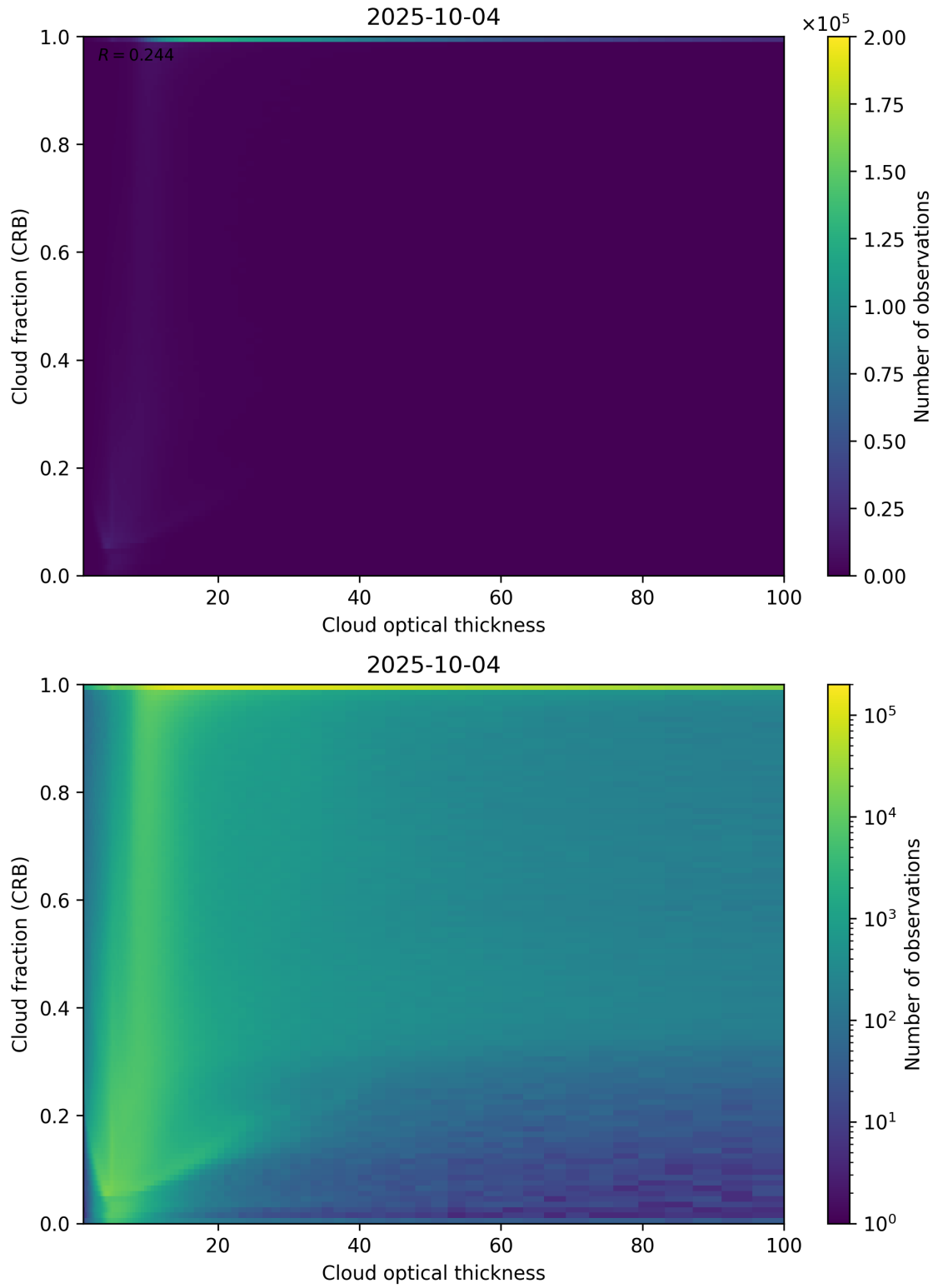
Figure 84: Scatter density plot of “Cloud optical thickness” against “Cloud fraction (CRB)” for 2025-10-03 to 2025-10-05.
