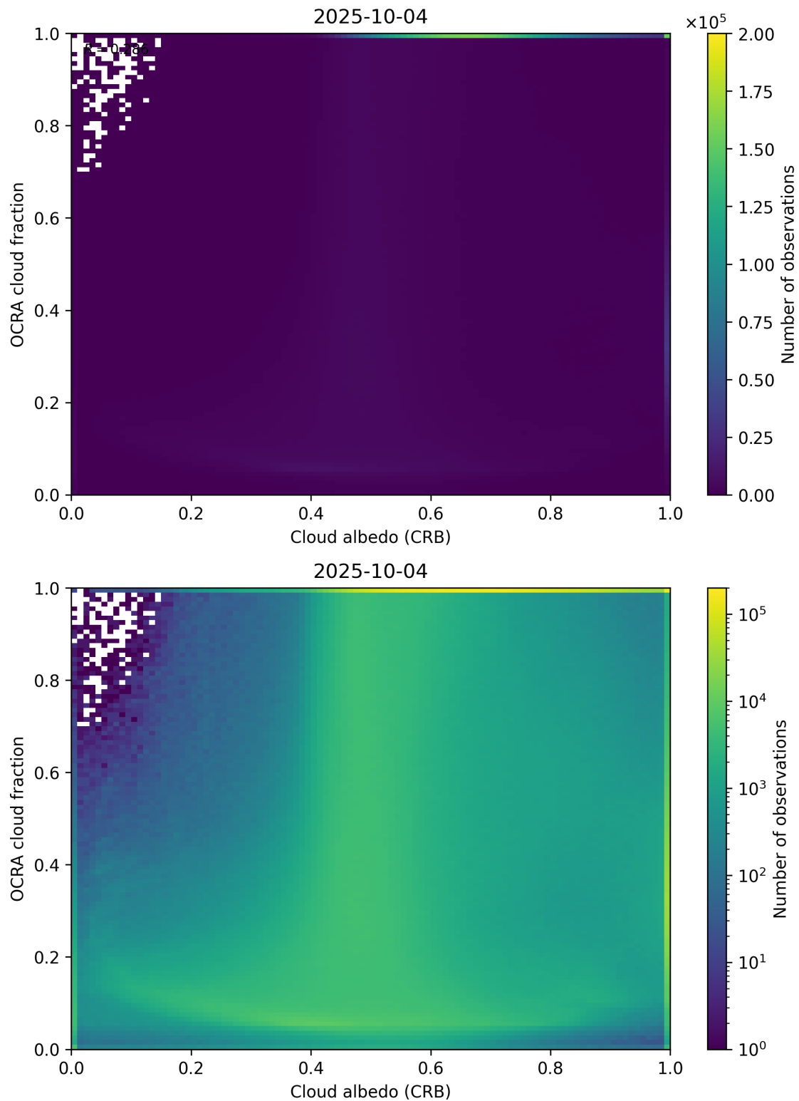
Figure 70: Scatter density plot of “Cloud albedo (CRB)” against “OCRA cloud fraction” for 2025-10-03 to 2025-10-05.
