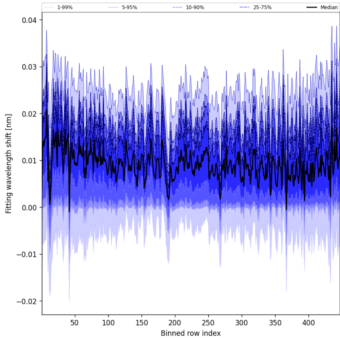
Figure 65: Along track statistics of “Fitting wavelength shift” for 2025-10-03 to 2025-10-05
