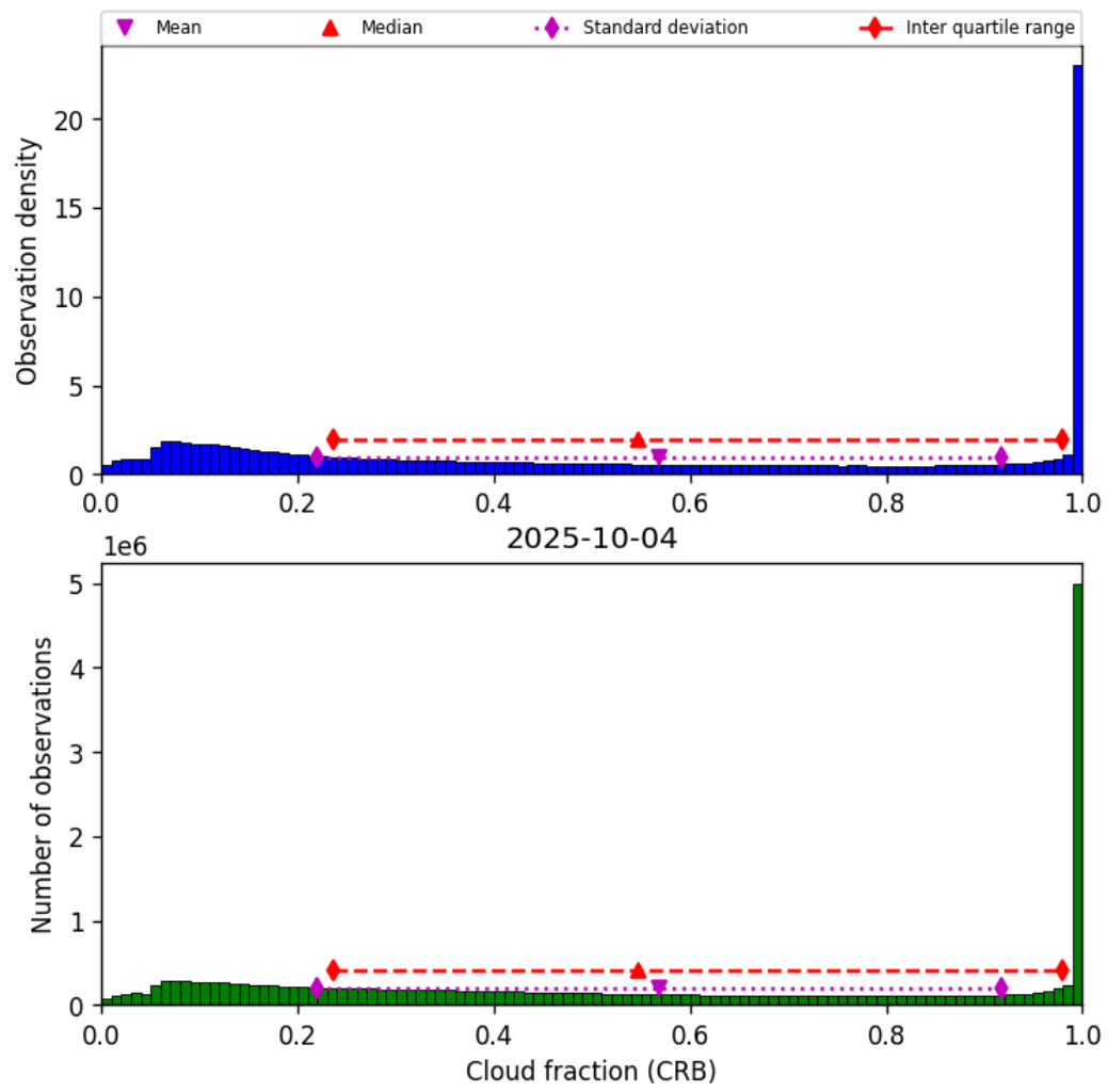
Figure 42: Histogram of "Cloud fraction (CRB)" for 2025-10-03 to 2025-10-05
