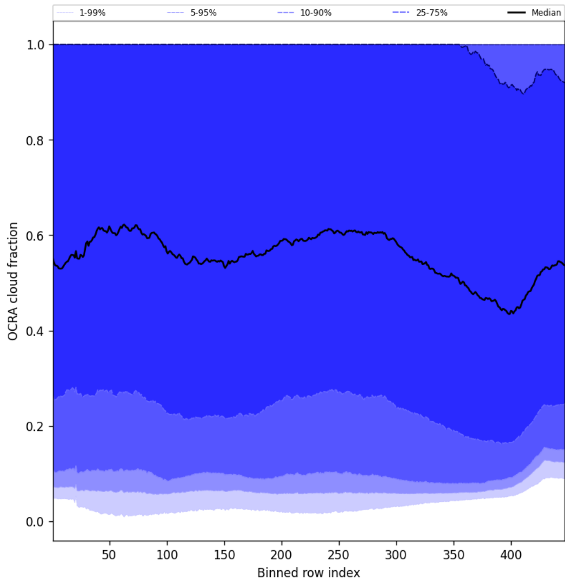
Figure 66: Along track statistics of “OCRA cloud fraction” for 2025-10-03 to 2025-10-05
