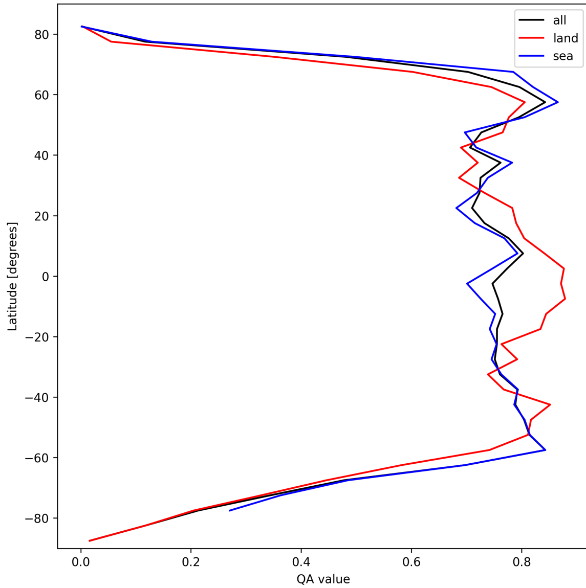
Figure 22: Zonal average of “QA value” for 2025-10-03 to 2025-10-05.
