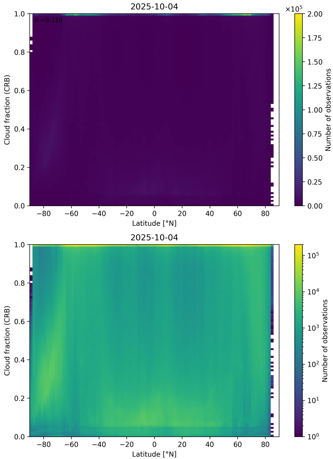
Figure 94: Scatter density plot of “Latitude” against “Cloud fraction (CRB)” for 2025-10-03 to 2025-10-05.
