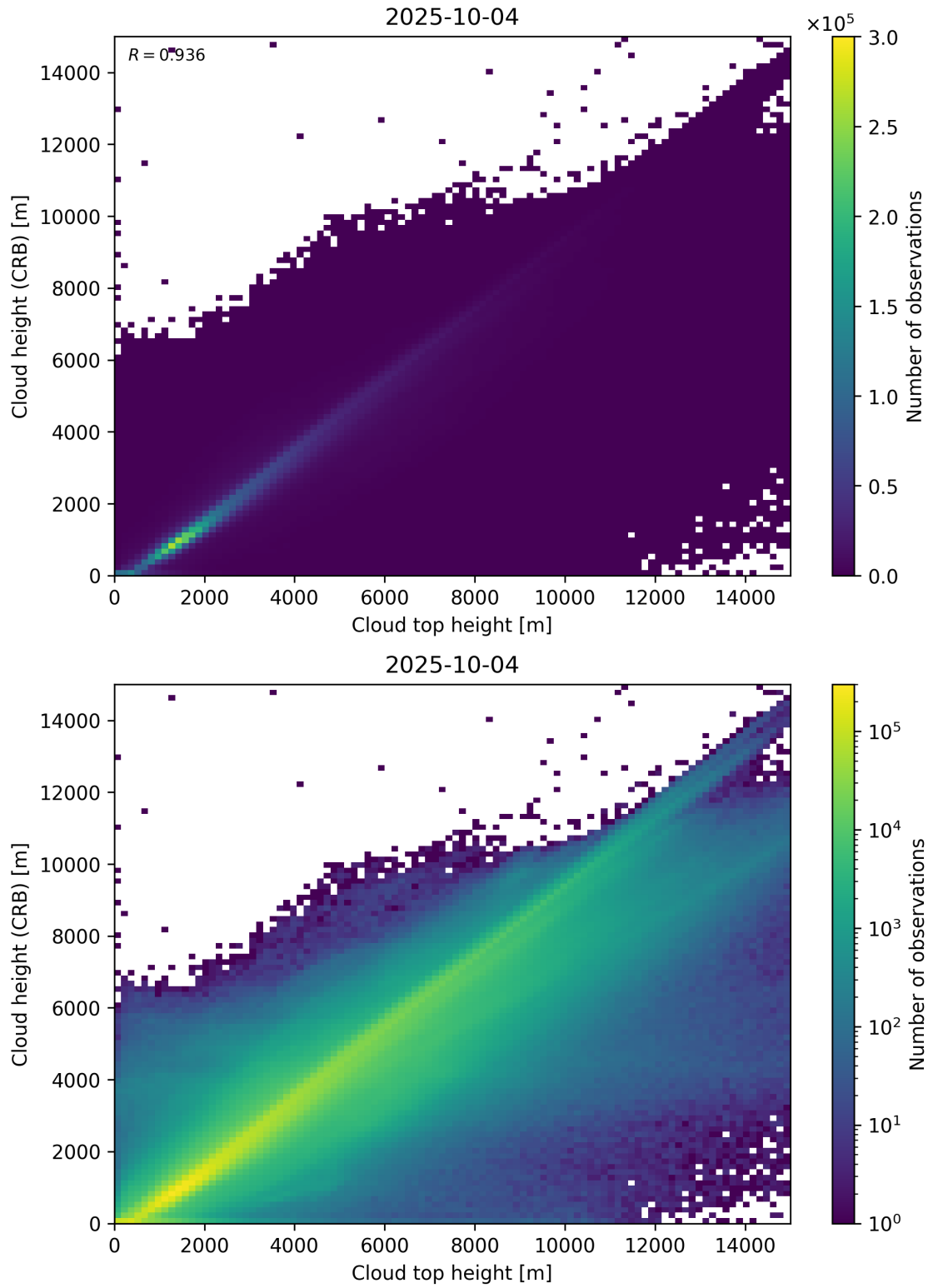
Figure 89: Scatter density plot of “Cloud top height” against “Cloud height (CRB)” for 2025-10-03 to 2025-10-05.
