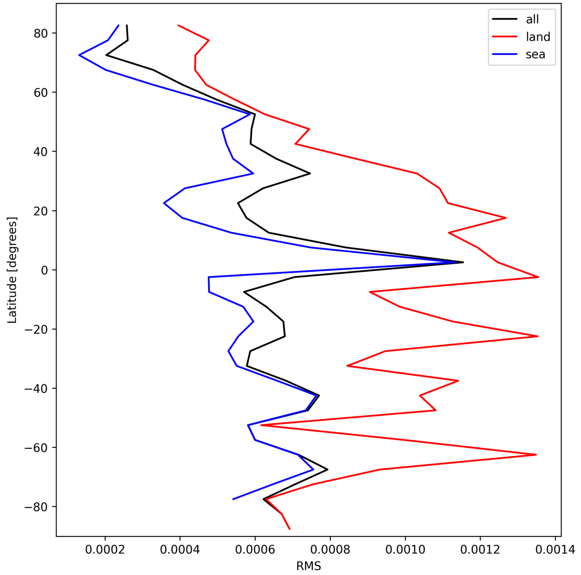
Figure 31: Zonal average of “RMS” for 2025-10-03 to 2025-10-05.
