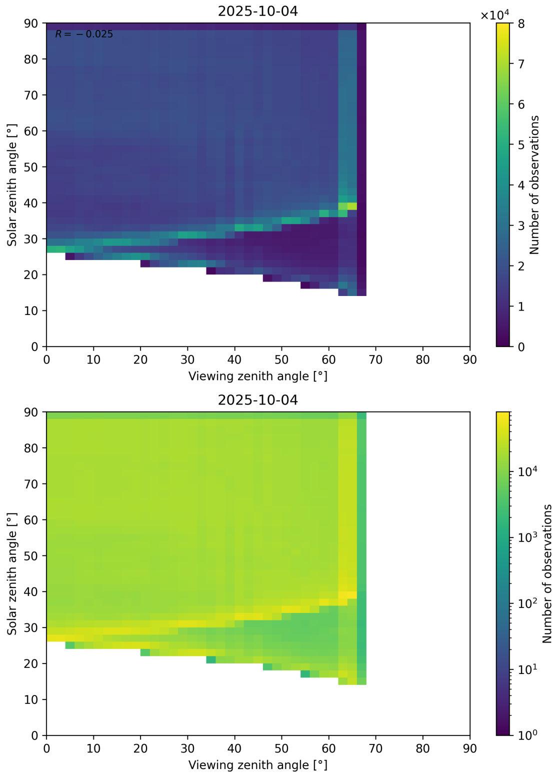
Figure 114: Scatter density plot of “Viewing zenith angle” against “Solar zenith angle” for 2025-10-03 to 2025-10-05.
