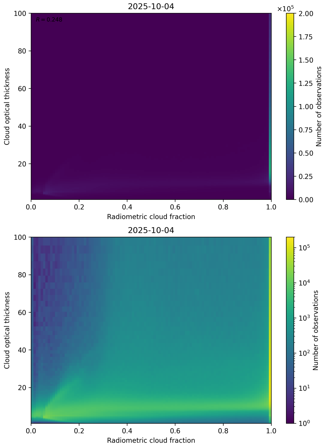
Figure 75: Scatter density plot of “Radiometric cloud fraction” against “Cloud optical thickness” for 2025-10-03 to 2025-10-05.
