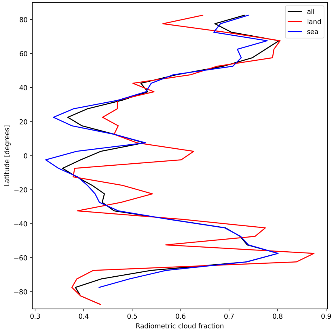
Figure 23: Zonal average of “Radiometric cloud fraction” for 2025-10-03 to 2025-10-05.
