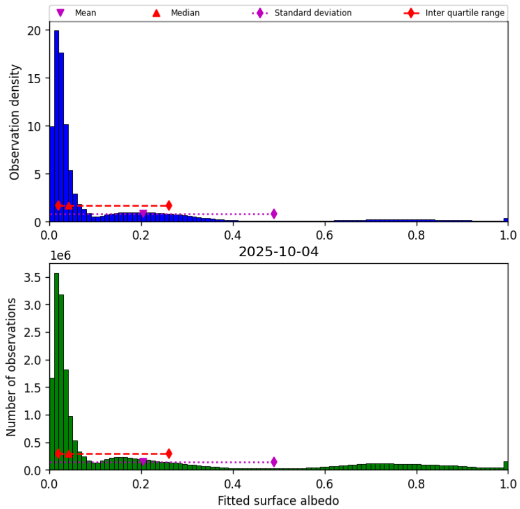
Figure 45: Histogram of “Fitted surface albedo” for 2025-10-03 to 2025-10-05
