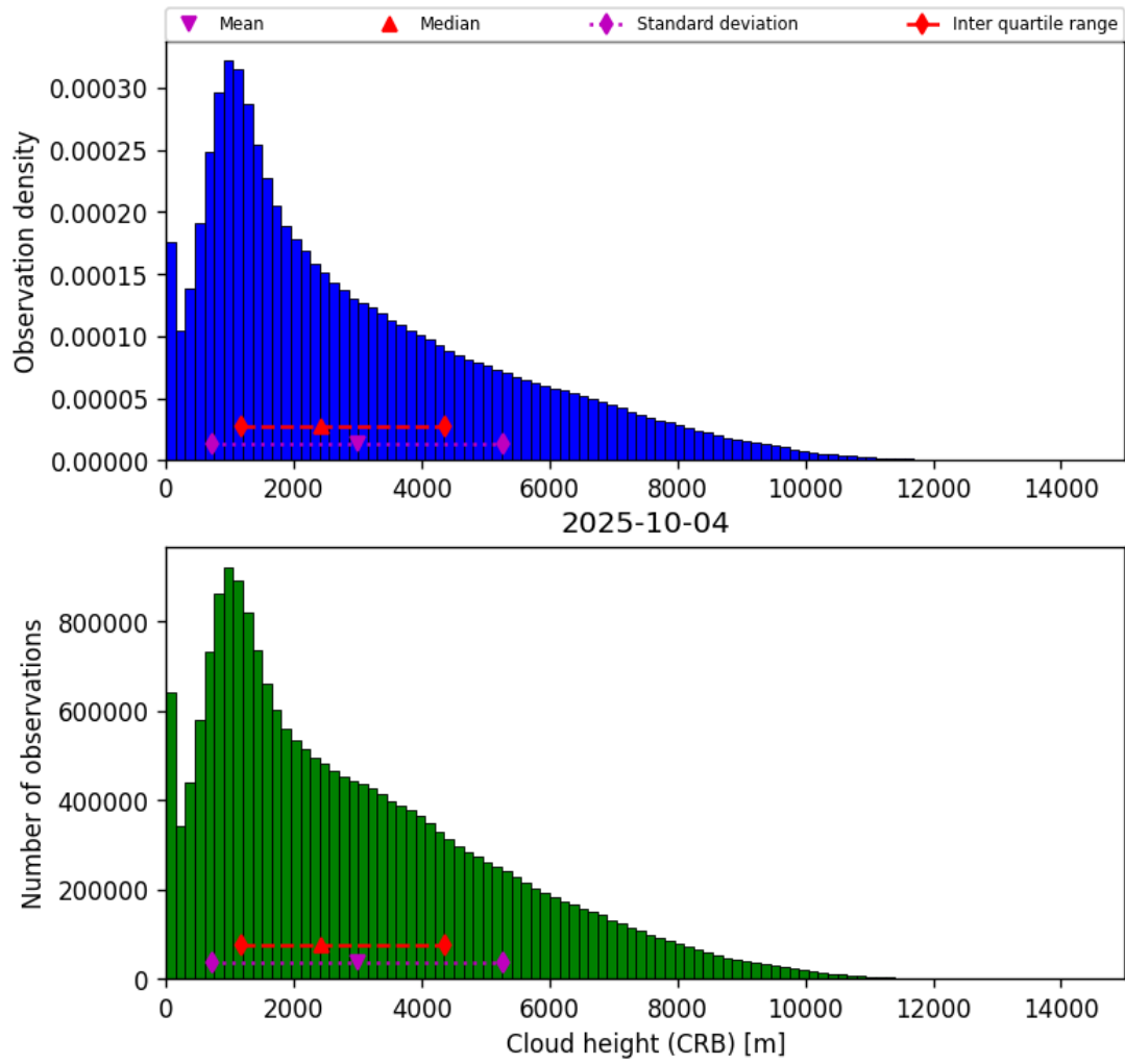
Figure 43: Histogram of “Cloud height (CRB)” for 2025-10-03 to 2025-10-05
