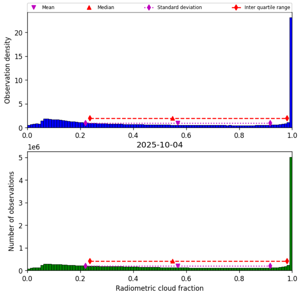
Figure 39: Histogram of “Radiometric cloud fraction” for 2025-10-03 to 2025-10-05
