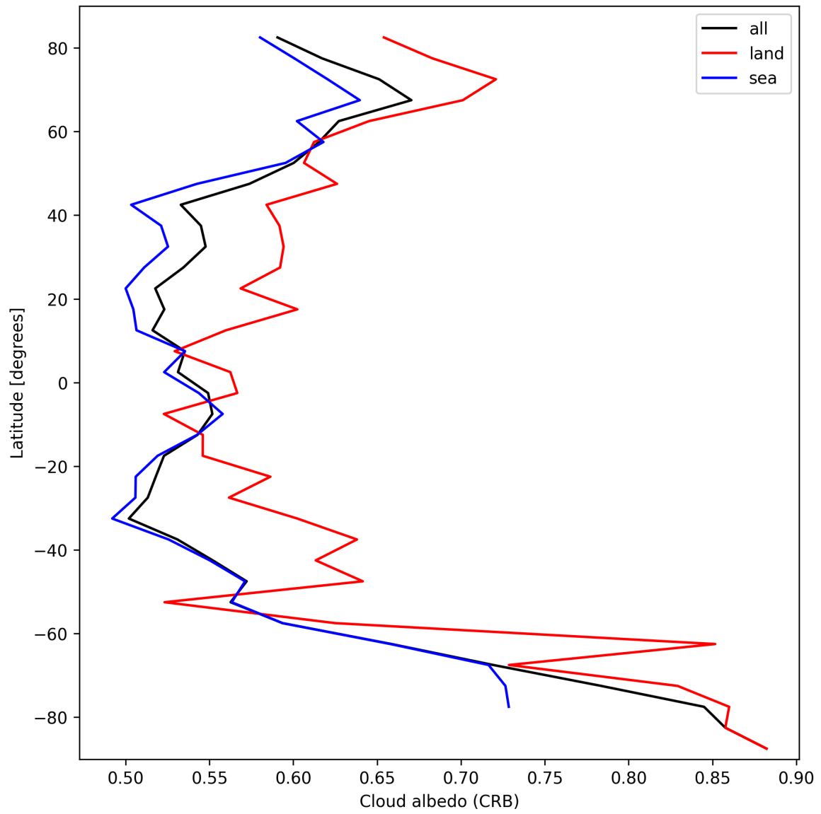
Figure 28: Zonal average of “Cloud albedo (CRB)” for 2025-10-03 to 2025-10-05.
