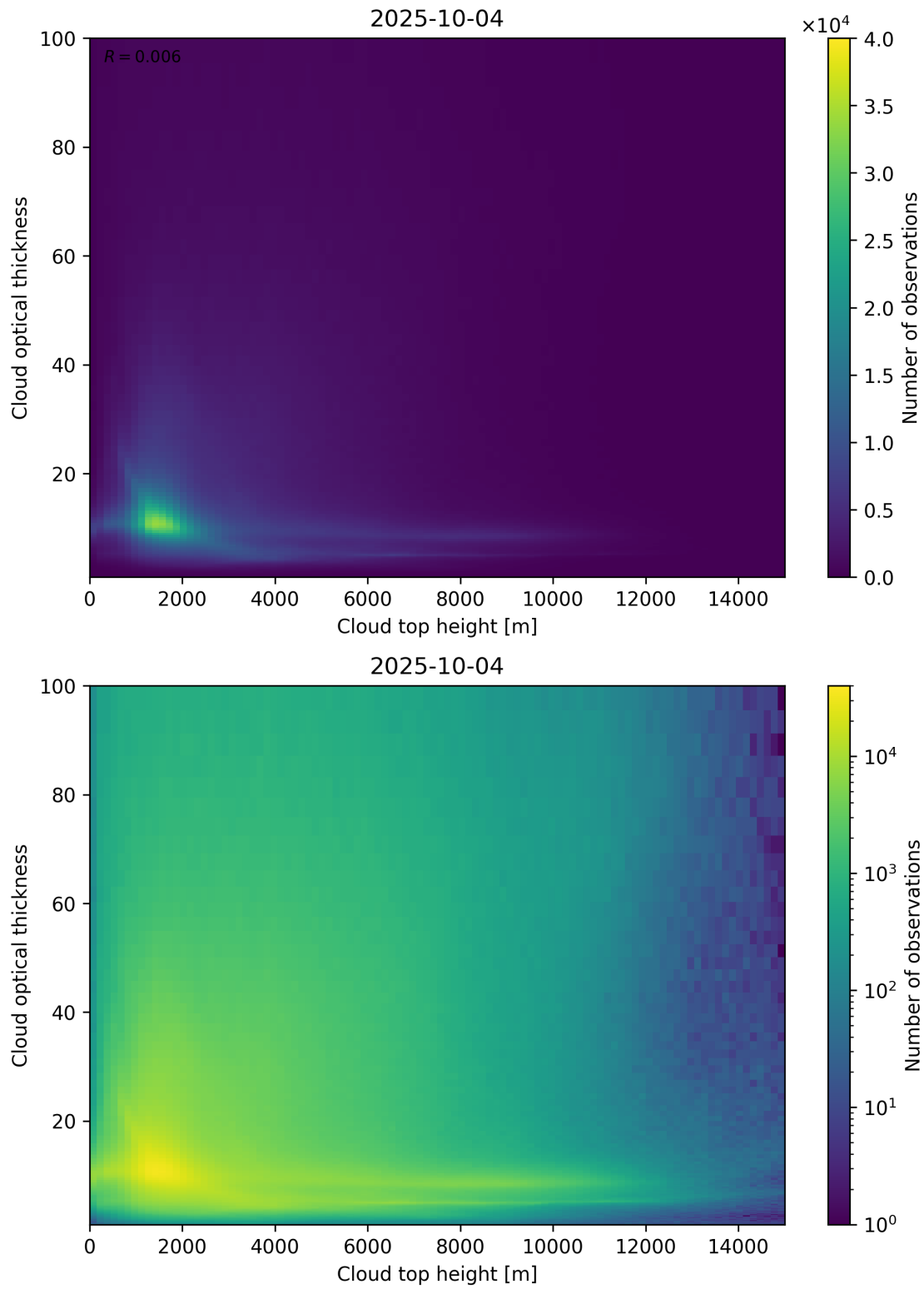
Figure 90: Scatter density plot of “Cloud top height” against “Cloud optical thickness” for 2025-10-03 to 2025-10-05.
