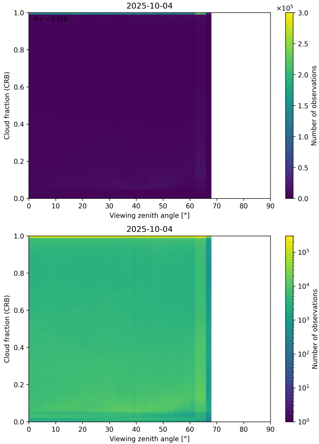
Figure 109: Scatter density plot of “Viewing zenith angle” against “Cloud fraction (CRB)” for 2025-10-03 to 2025-10-05.
