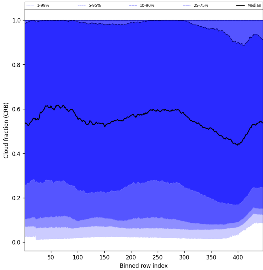
Figure 58: Along track statistics of “Cloud fraction (CRB)” for 2025-10-03 to 2025-10-05
