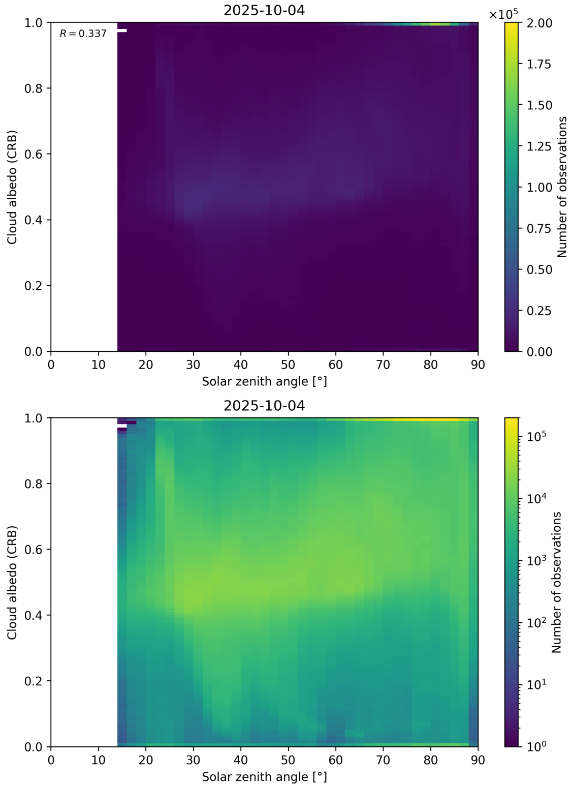
Figure 98: Scatter density plot of “Solar zenith angle” against “Cloud albedo (CRB)” for 2025-10-03 to 2025-10-05.
