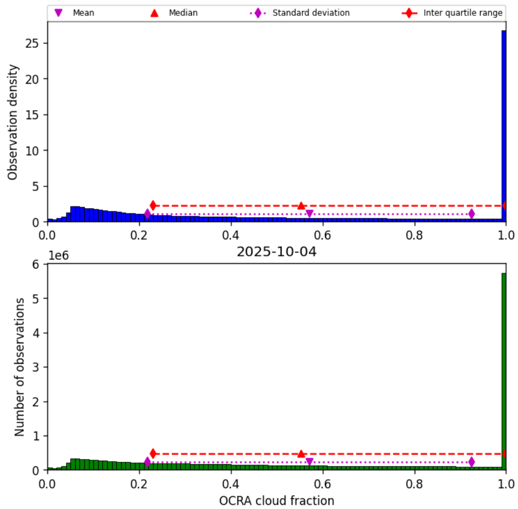
Figure 50: Histogram of “OCRA cloud fraction” for 2025-10-03 to 2025-10-05
