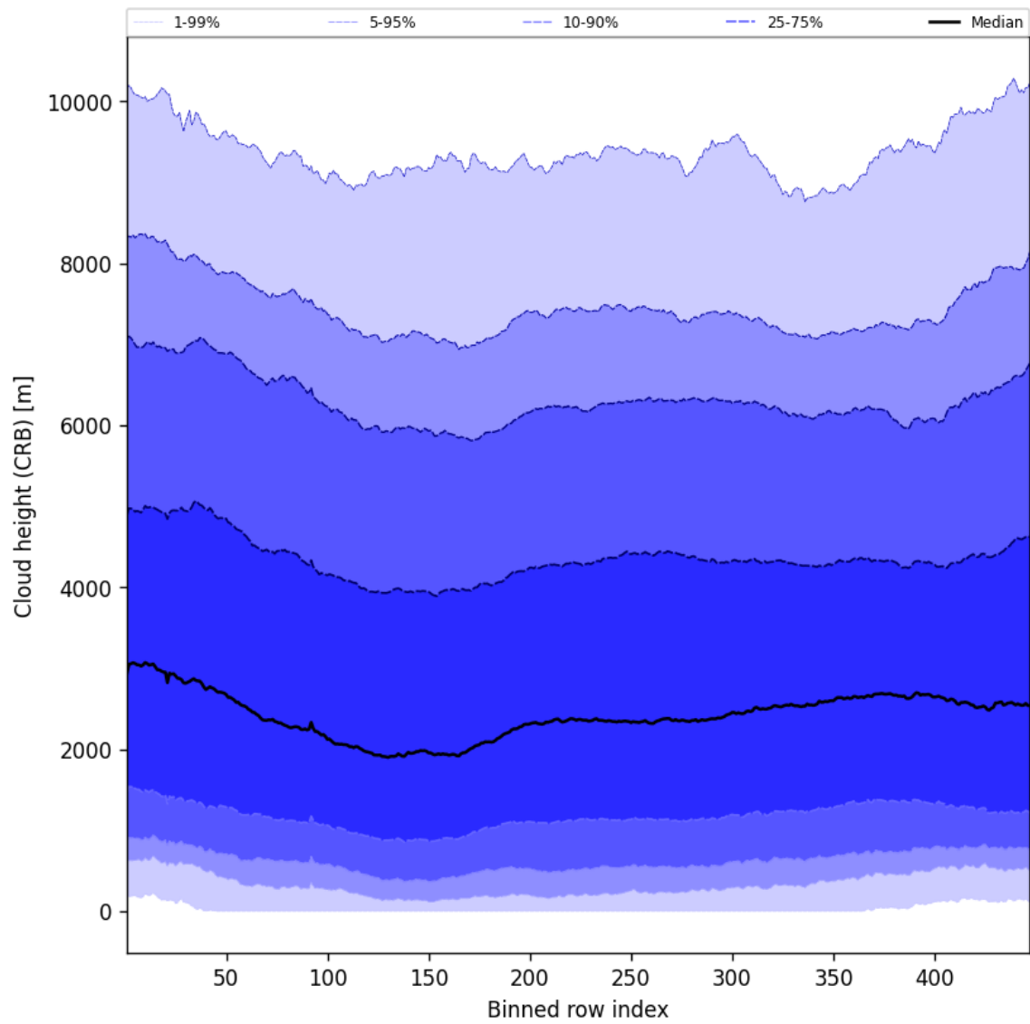
Figure 59: Along track statistics of “Cloud height (CRB)” for 2025-10-03 to 2025-10-05
