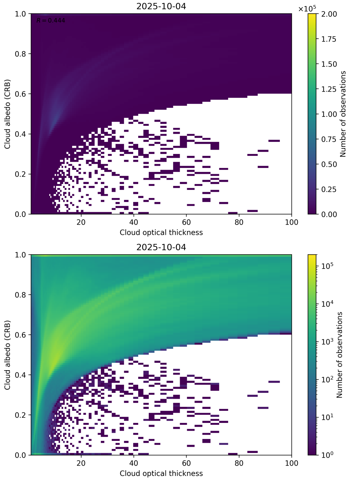
Figure 82: Scatter density plot of “Cloud optical thickness” against “Cloud albedo (CRB)” for 2025-10-03 to 2025-10-05.
