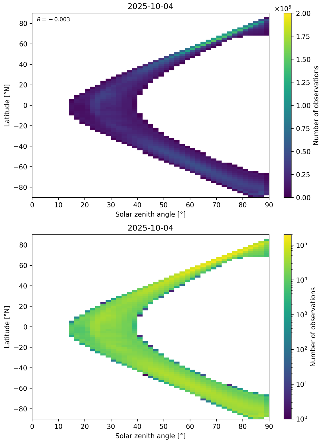
Figure 105: Scatter density plot of “Solar zenith angle” against “Latitude” for 2025-10-03 to 2025-10-05.
