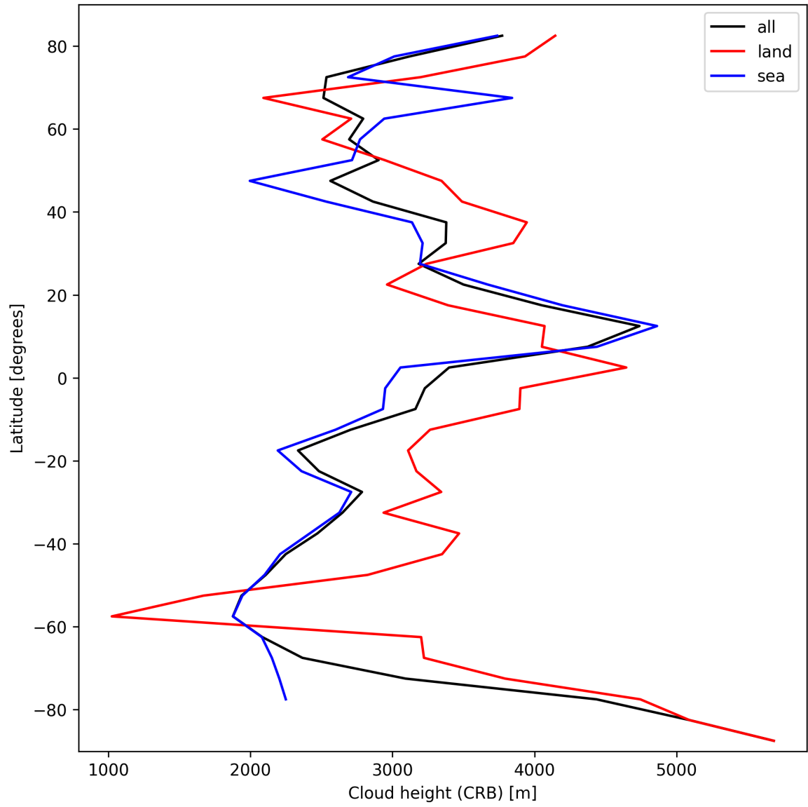
Figure 27: Zonal average of “Cloud height (CRB)” for 2025-10-03 to 2025-10-05.
