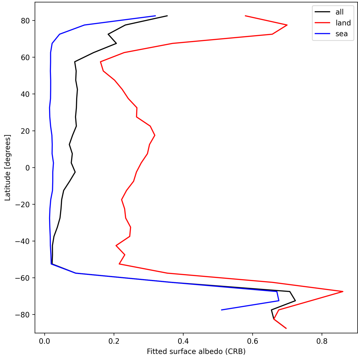
Figure 30: Zonal average of “Fitted surface albedo (CRB)” for 2025-10-03 to 2025-10-05.
