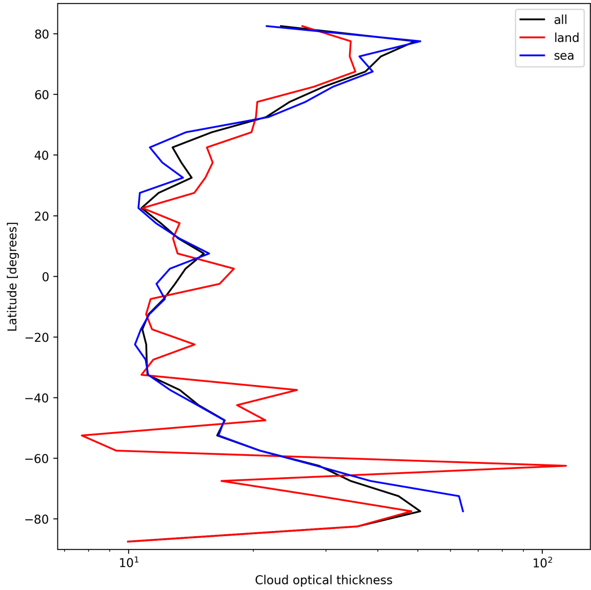
Figure 25: Zonal average of “Cloud optical thickness” for 2025-10-03 to 2025-10-05.
