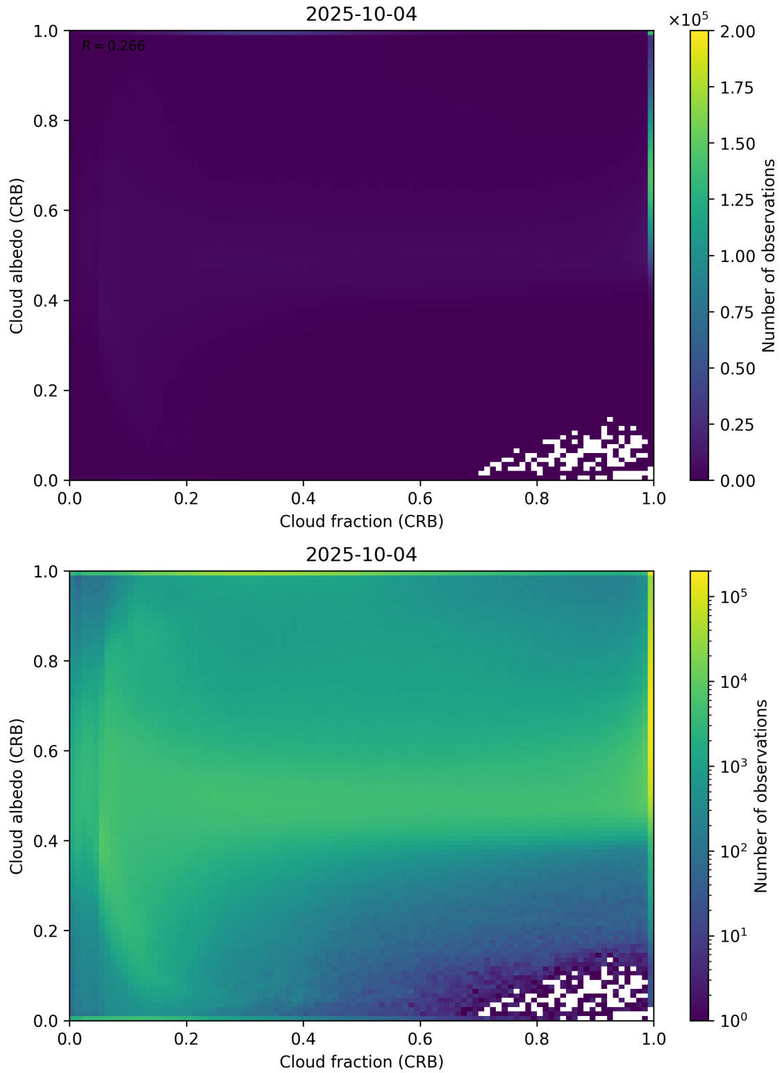
Figure 77: Scatter density plot of “Cloud fraction (CRB)” against “Cloud albedo (CRB)” for 2025-10-03 to 2025-10-05.
