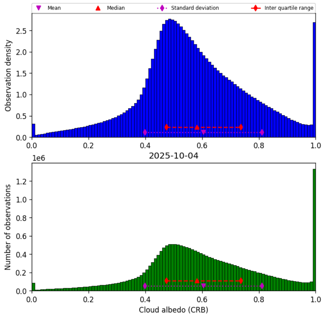
Figure 44: Histogram of “Cloud albedo (CRB)” for 2025-10-03 to 2025-10-05
