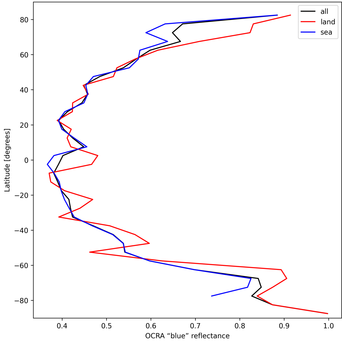
Figure 35: Zonal average of “OCRA “blue” reflectance” for 2025-10-03 to 2025-10-05.
