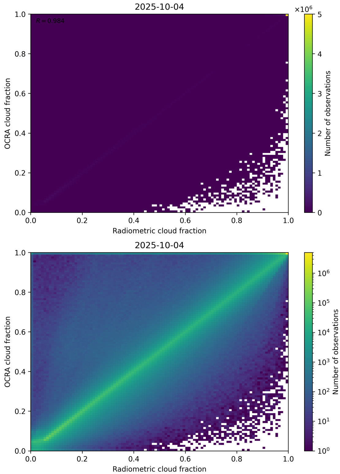
Figure 72: Scatter density plot of “Radiometric cloud fraction” against “OCRA cloud fraction” for 2025-10-03 to 2025-10-05.
