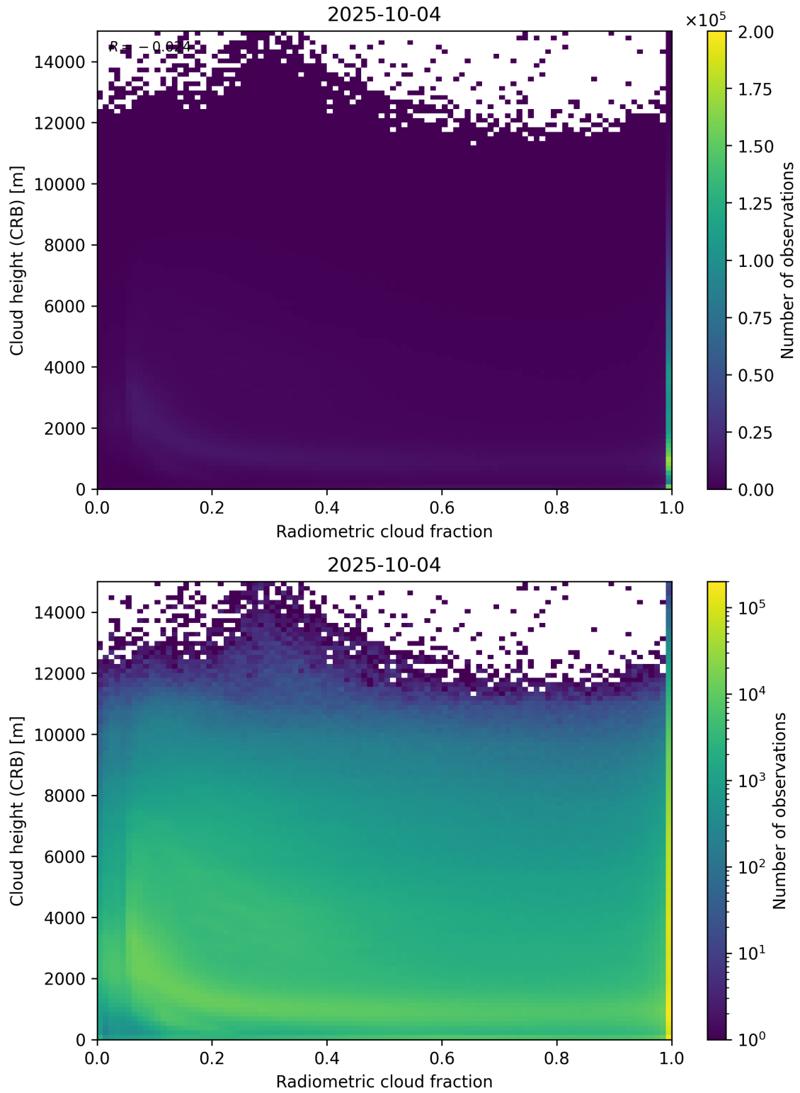
Figure 74: Scatter density plot of “Radiometric cloud fraction” against “Cloud height (CRB)” for 2025-10-03 to 2025-10-05.
