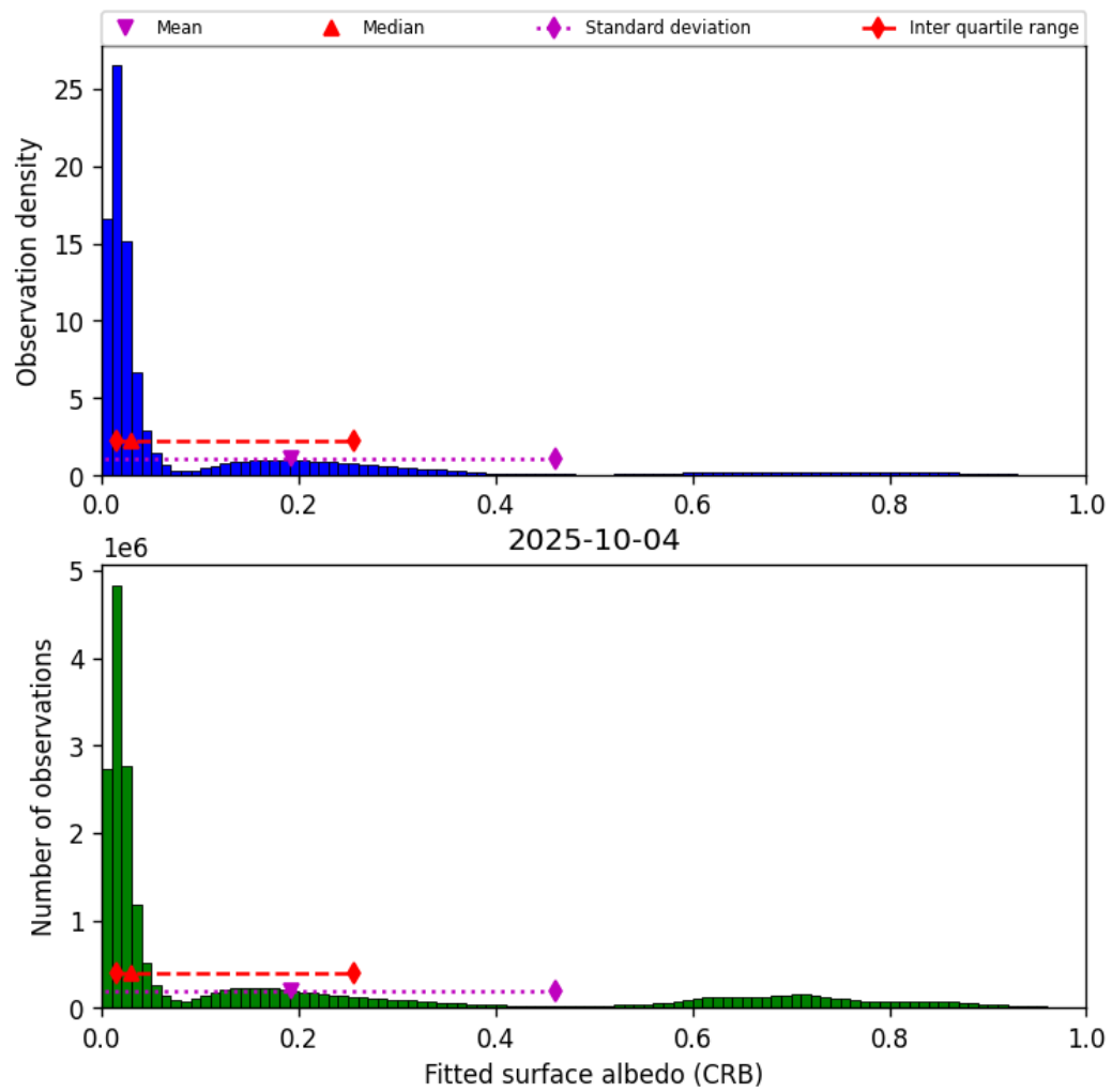
Figure 46: Histogram of “Fitted surface albedo (CRB)” for 2025-10-03 to 2025-10-05
