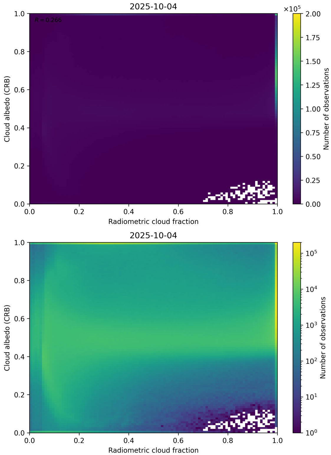
Figure 71: Scatter density plot of “Radiometric cloud fraction” against “Cloud albedo (CRB)” for 2025-10-03 to 2025-10-05.
