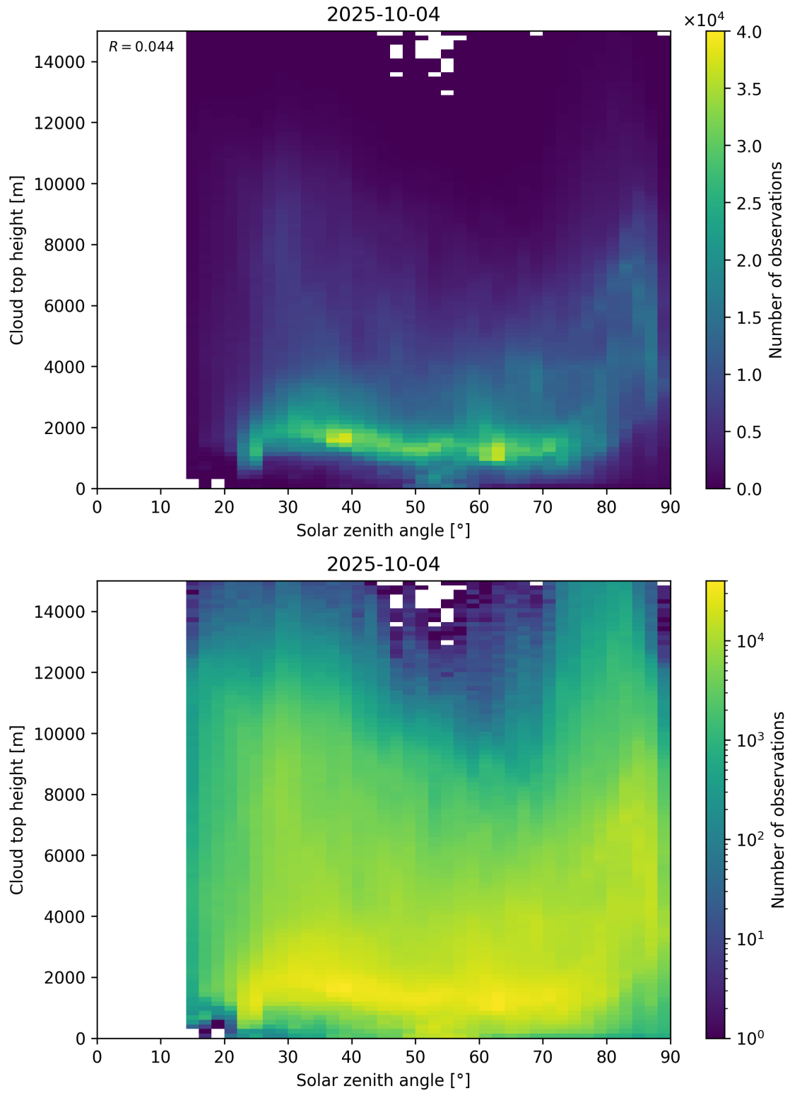
Figure 104: Scatter density plot of “Solar zenith angle” against “Cloud top height” for 2025-10-03 to 2025-10-05.
