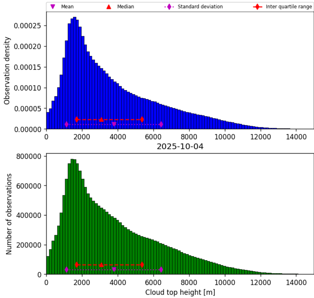
Figure 40: Histogram of “Cloud top height” for 2025-10-03 to 2025-10-05
