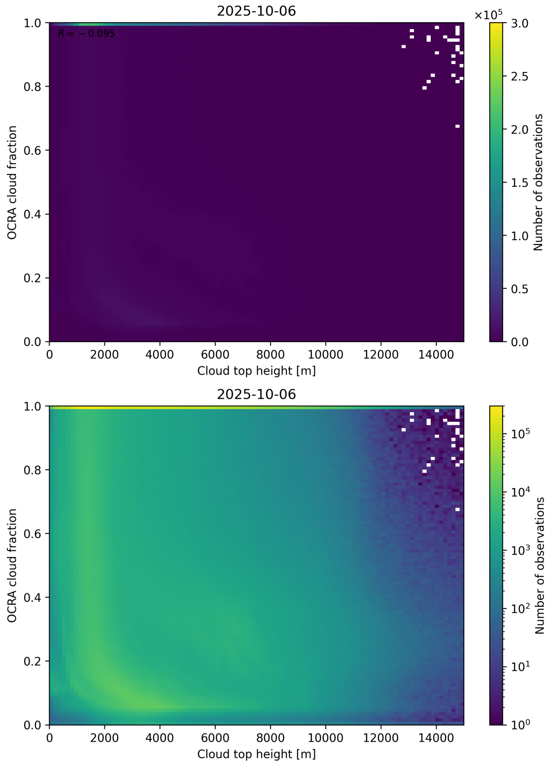
Figure 87: Scatter density plot of “Cloud top height” against “OCRA cloud fraction” for 2025-10-06 to 2025-10-07.
