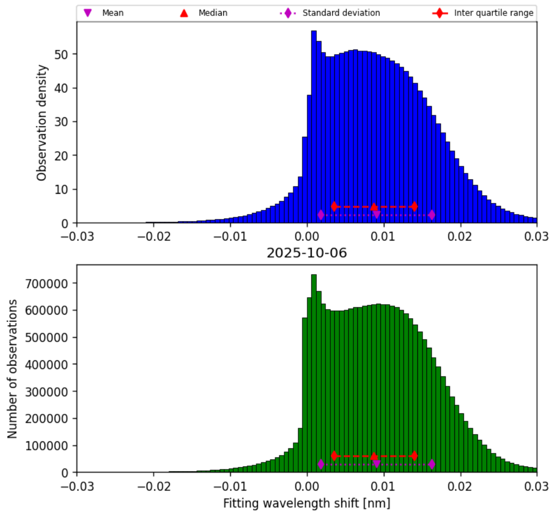
Figure 49: Histogram of “Fitting wavelength shift” for 2025-10-06 to 2025-10-07
