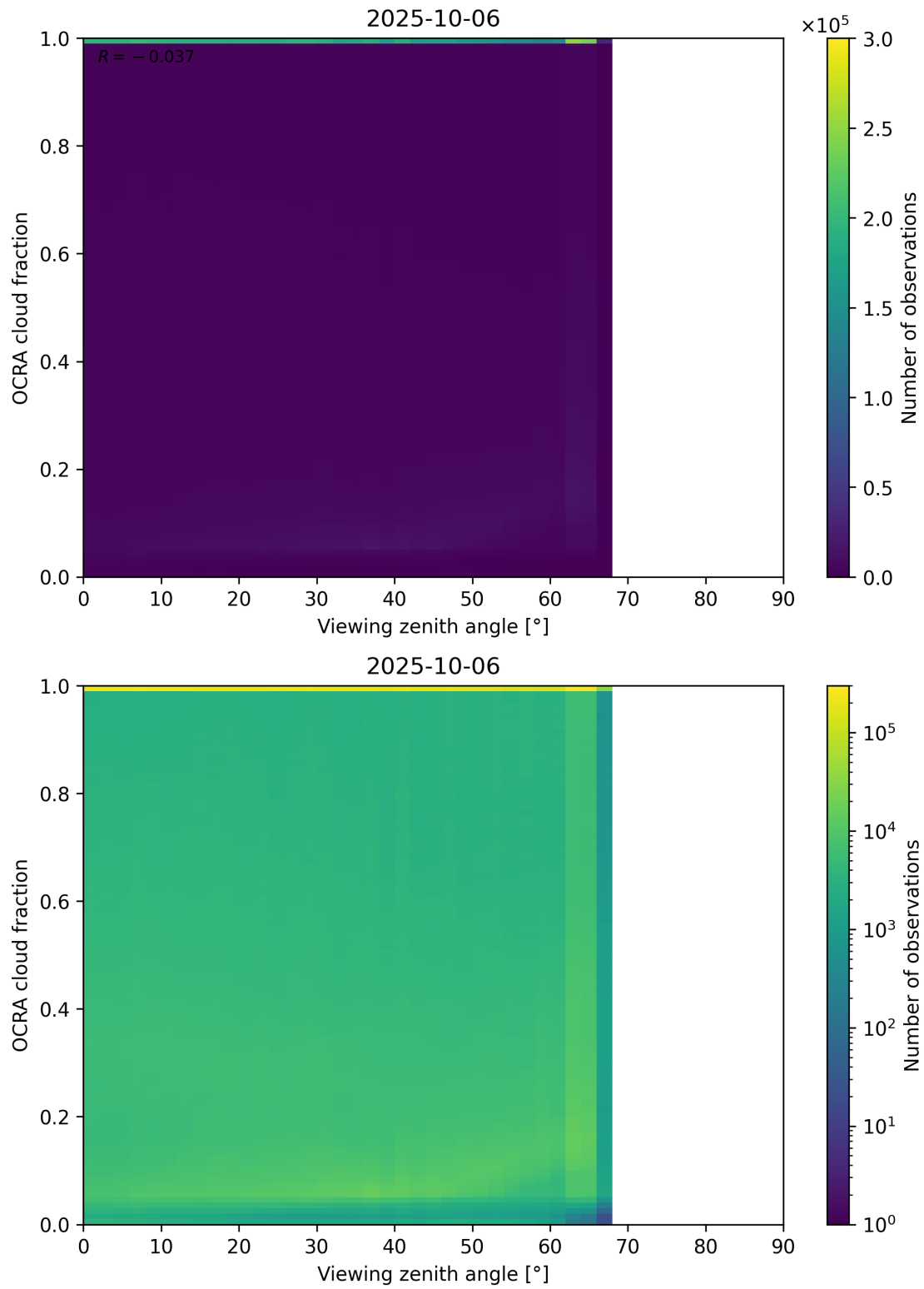
Figure 108: Scatter density plot of “Viewing zenith angle” against “OCRA cloud fraction” for 2025-10-06 to 2025-10-07.
