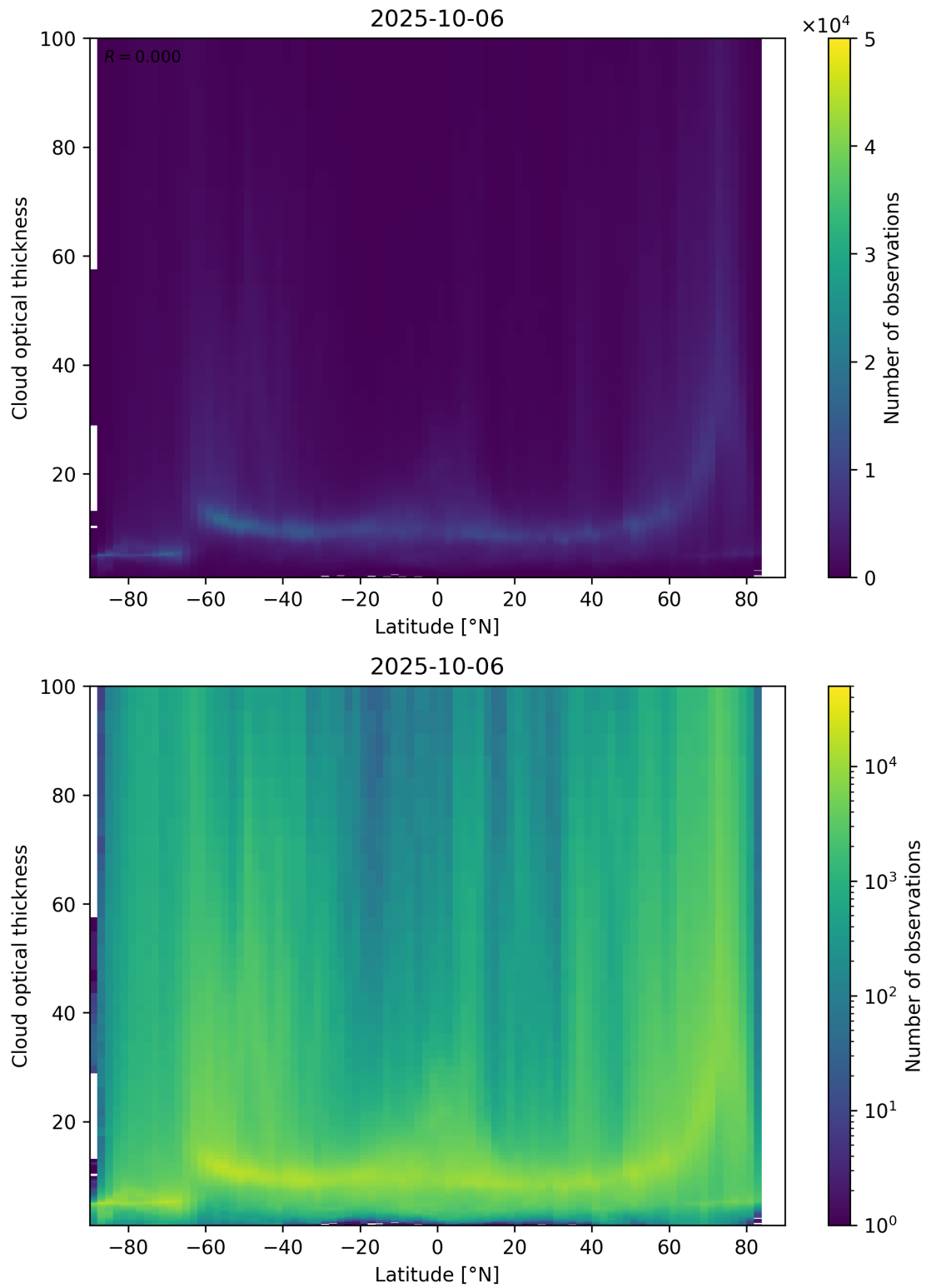
Figure 96: Scatter density plot of “Latitude” against “Cloud optical thickness” for 2025-10-06 to 2025-10-07.
