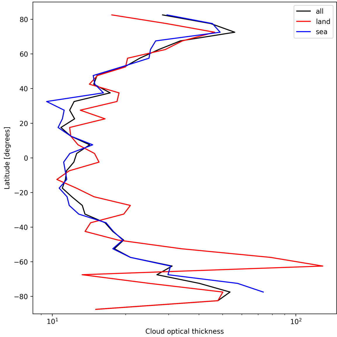
Figure 25: Zonal average of “Cloud optical thickness” for 2025-10-06 to 2025-10-07.
