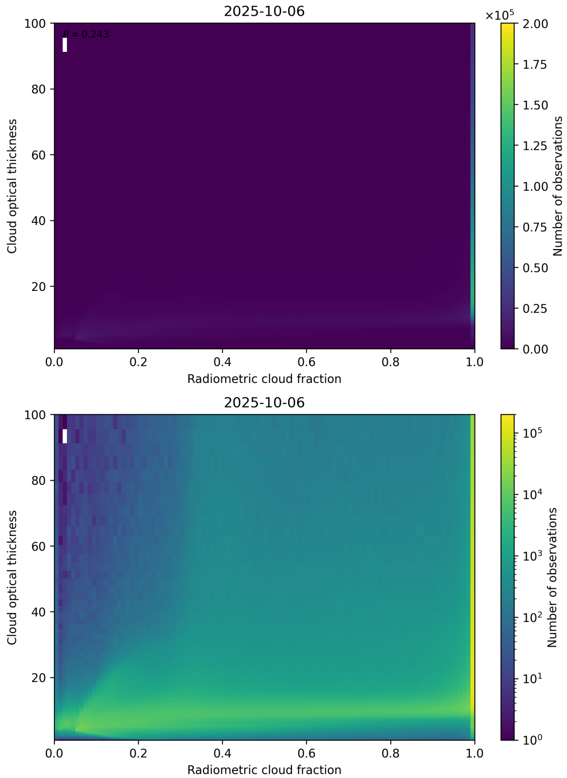
Figure 75: Scatter density plot of “Radiometric cloud fraction” against “Cloud optical thickness” for 2025-10-06 to 2025-10-07.
