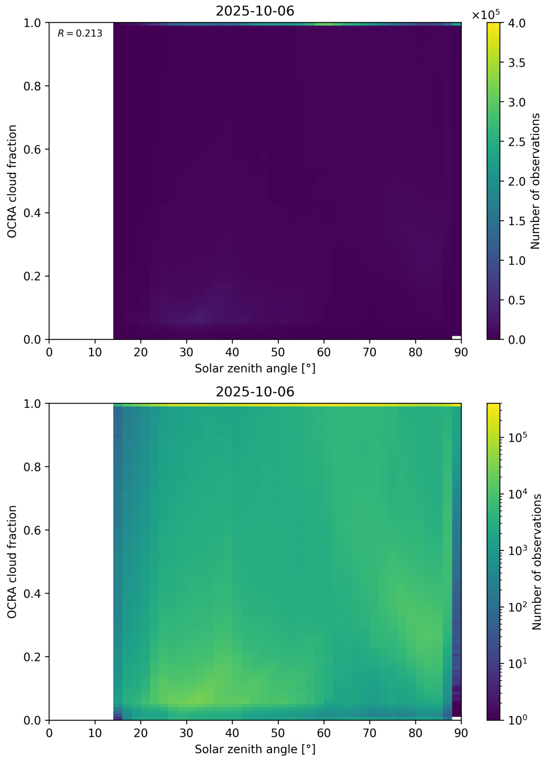
Figure 100: Scatter density plot of “Solar zenith angle” against “OCRA cloud fraction” for 2025-10-06 to 2025-10-07.
