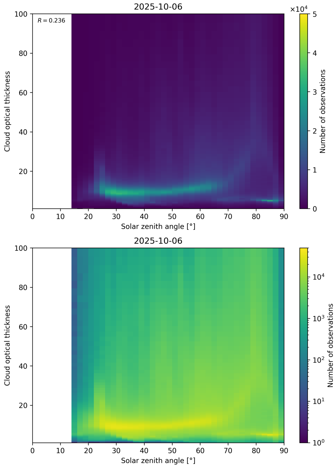
Figure 103: Scatter density plot of “Solar zenith angle” against “Cloud optical thickness” for 2025-10-06 to 2025-10-07.
