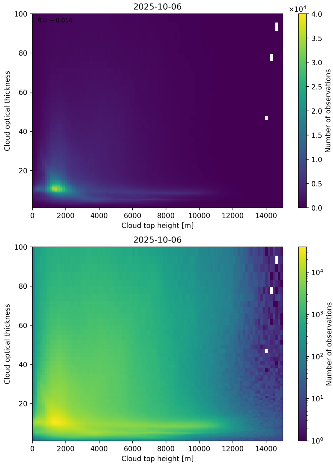
Figure 90: Scatter density plot of “Cloud top height” against “Cloud optical thickness” for 2025-10-06 to 2025-10-07.
