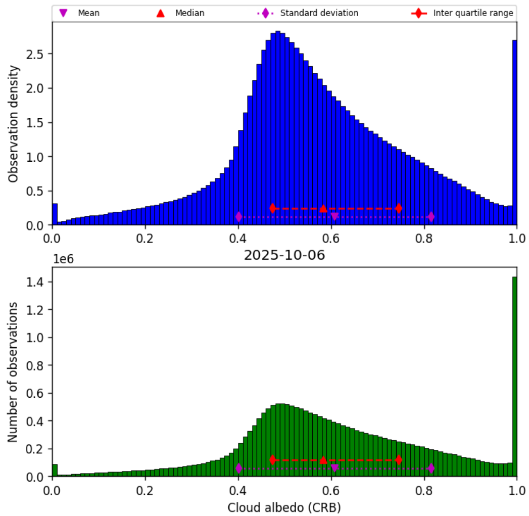
Figure 44: Histogram of “Cloud albedo (CRB)” for 2025-10-06 to 2025-10-07
