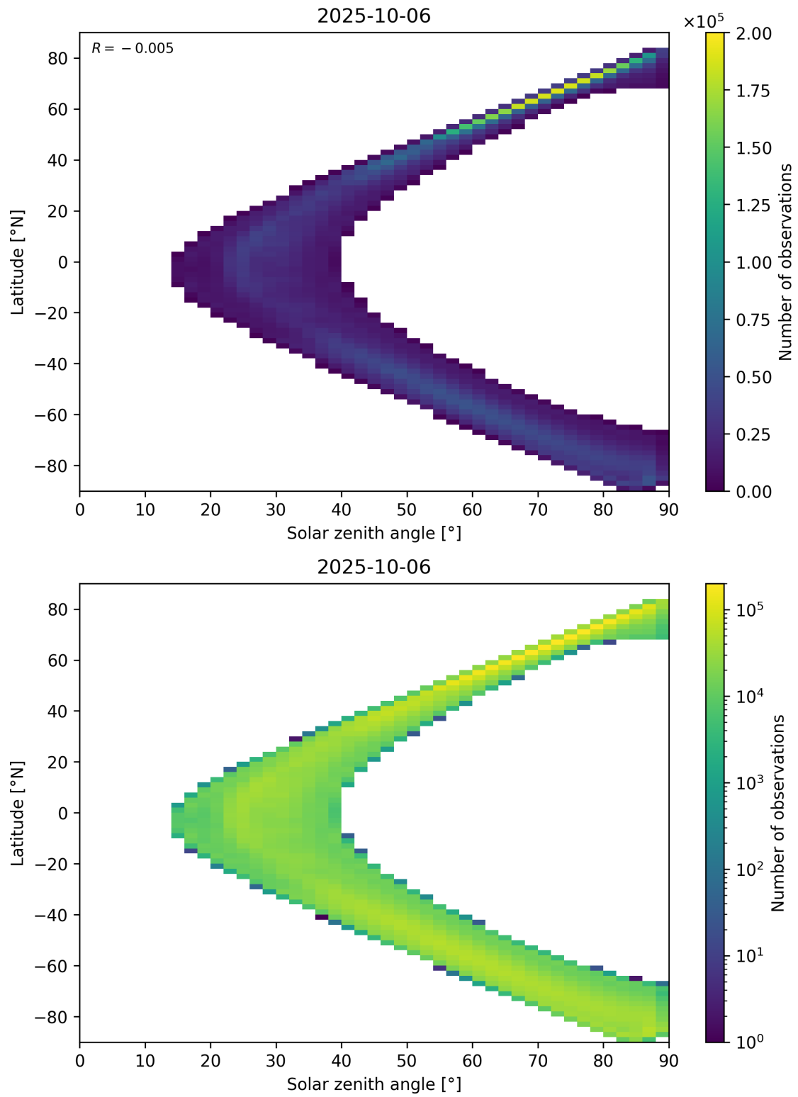
Figure 105: Scatter density plot of “Solar zenith angle” against “Latitude” for 2025-10-06 to 2025-10-07.
