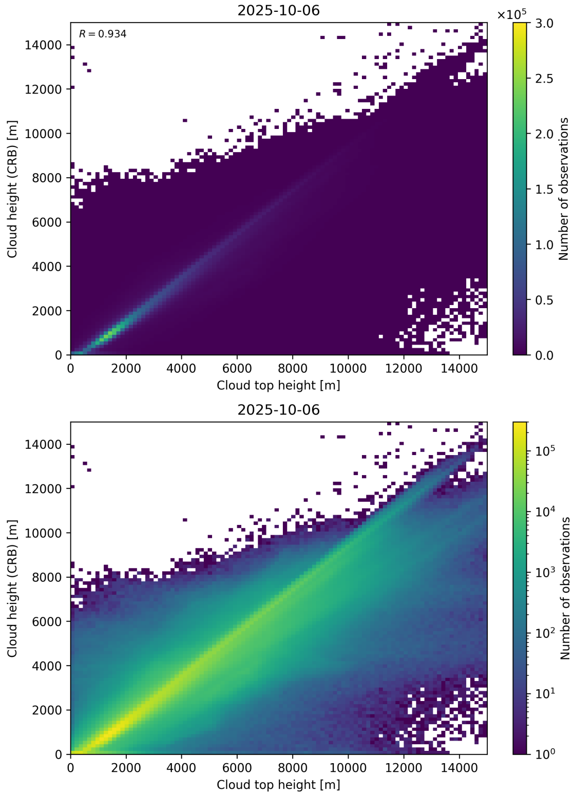
Figure 89: Scatter density plot of “Cloud top height” against “Cloud height (CRB)” for 2025-10-06 to 2025-10-07.
