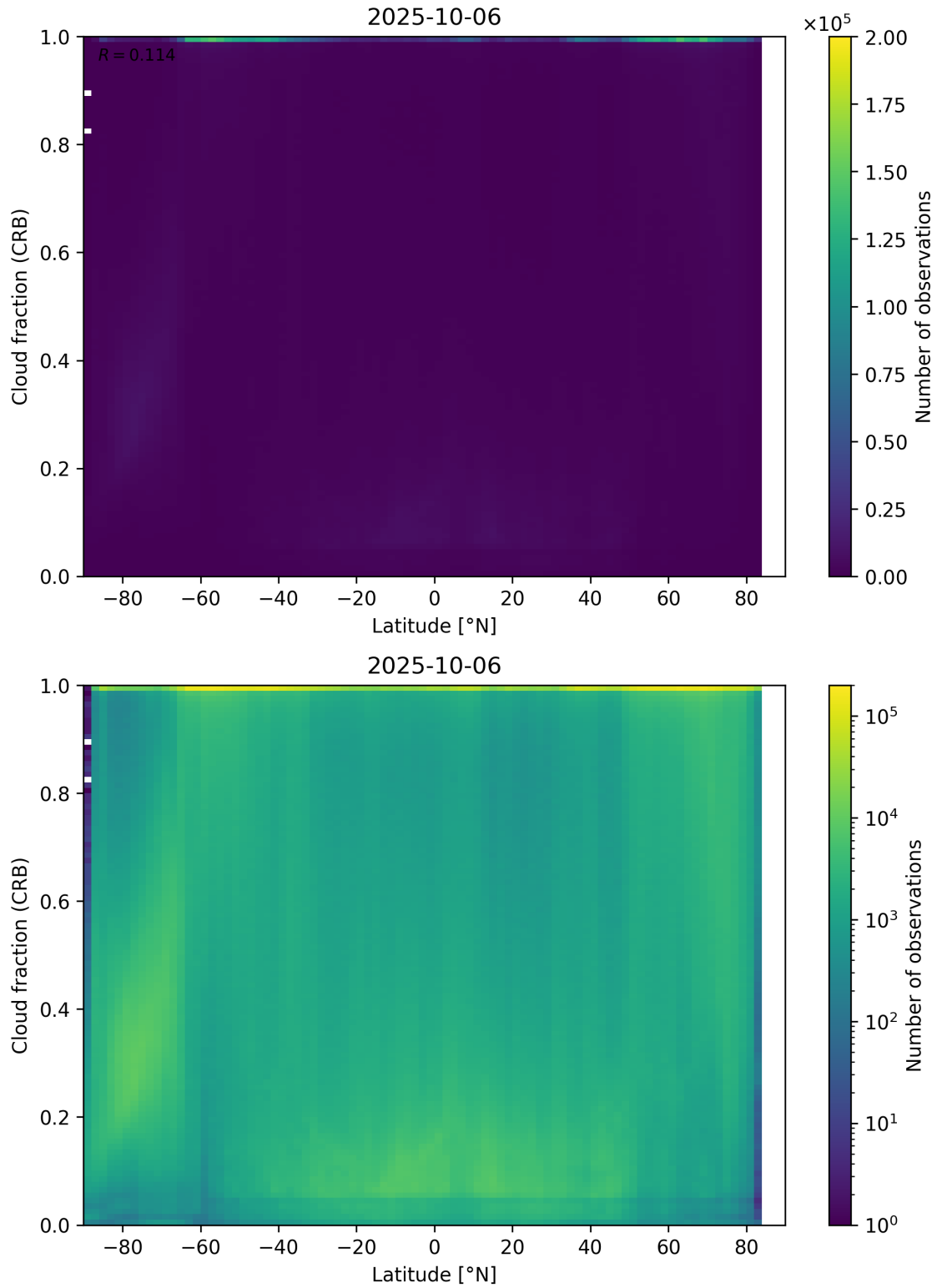
Figure 94: Scatter density plot of “Latitude” against “Cloud fraction (CRB)” for 2025-10-06 to 2025-10-07.
