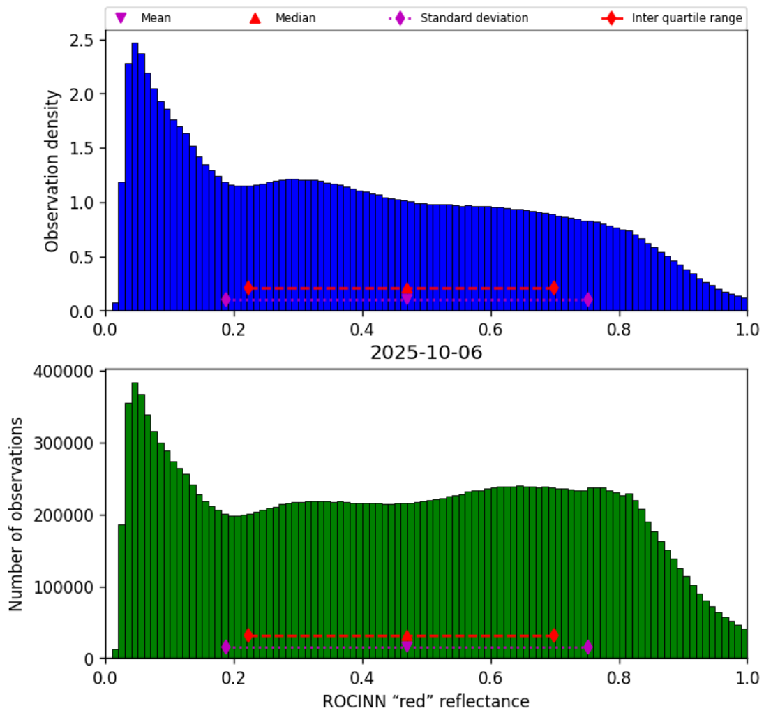
Figure 53: Histogram of “ROCINN “red” reflectance” for 2025-10-06 to 2025-10-07
