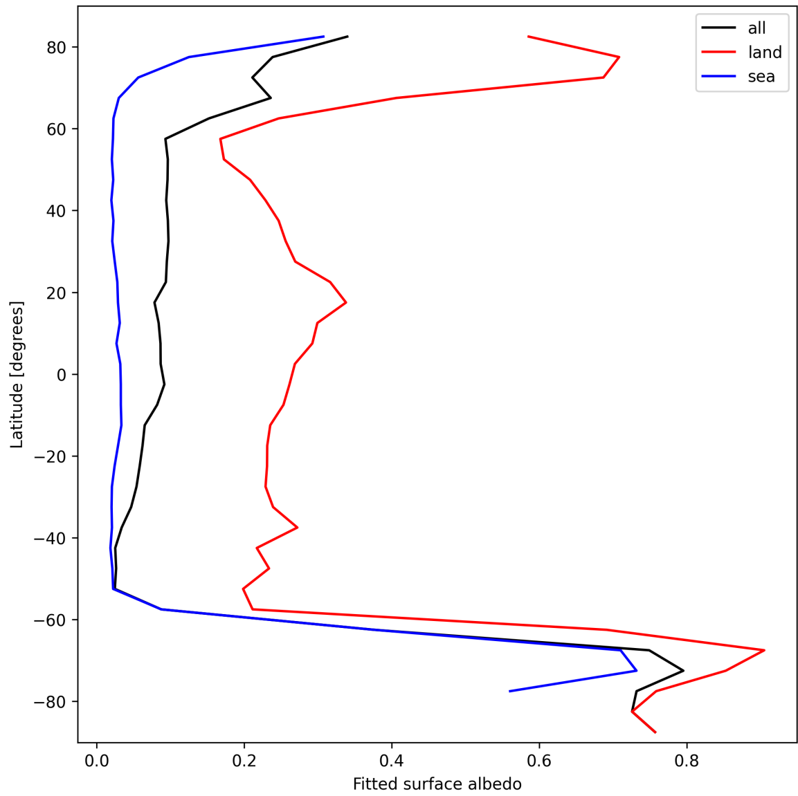
Figure 29: Zonal average of “Fitted surface albedo” for 2025-10-06 to 2025-10-07.
