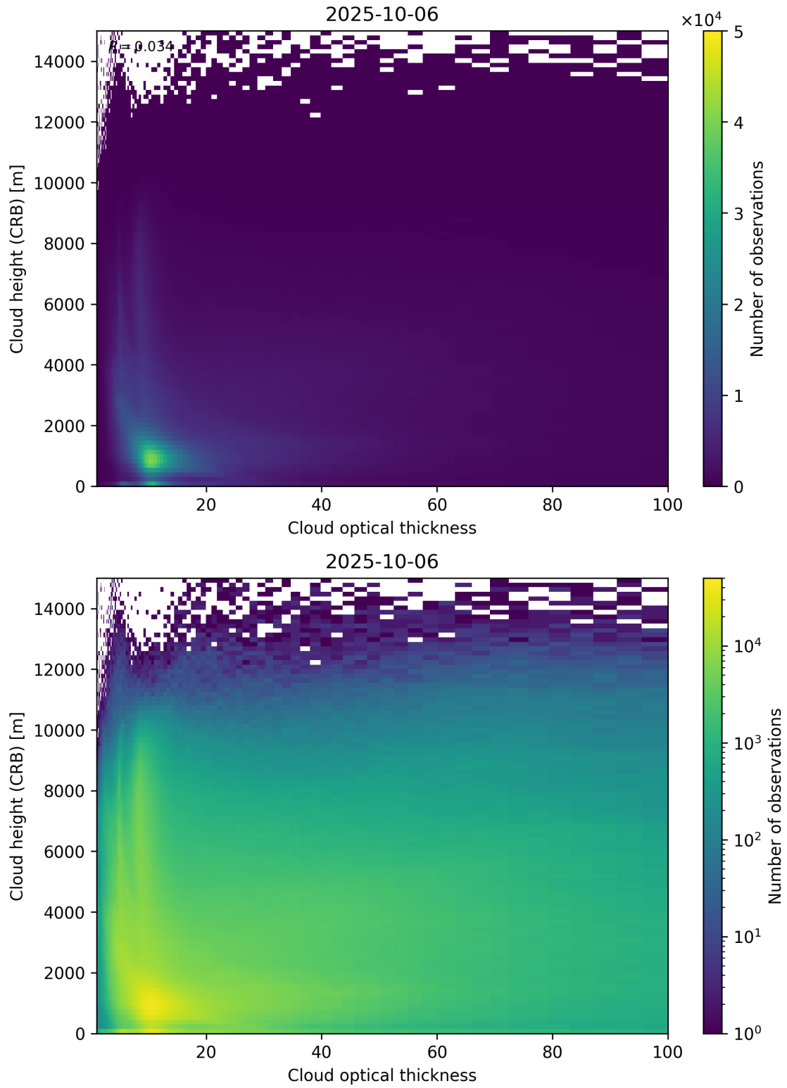
Figure 85: Scatter density plot of “Cloud optical thickness” against “Cloud height (CRB)” for 2025-10-06 to 2025-10-07.
