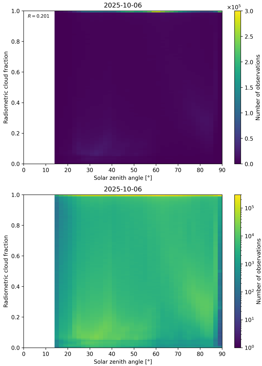
Figure 99: Scatter density plot of “Solar zenith angle” against “Radiometric cloud fraction” for 2025-10-06 to 2025-10-07.
