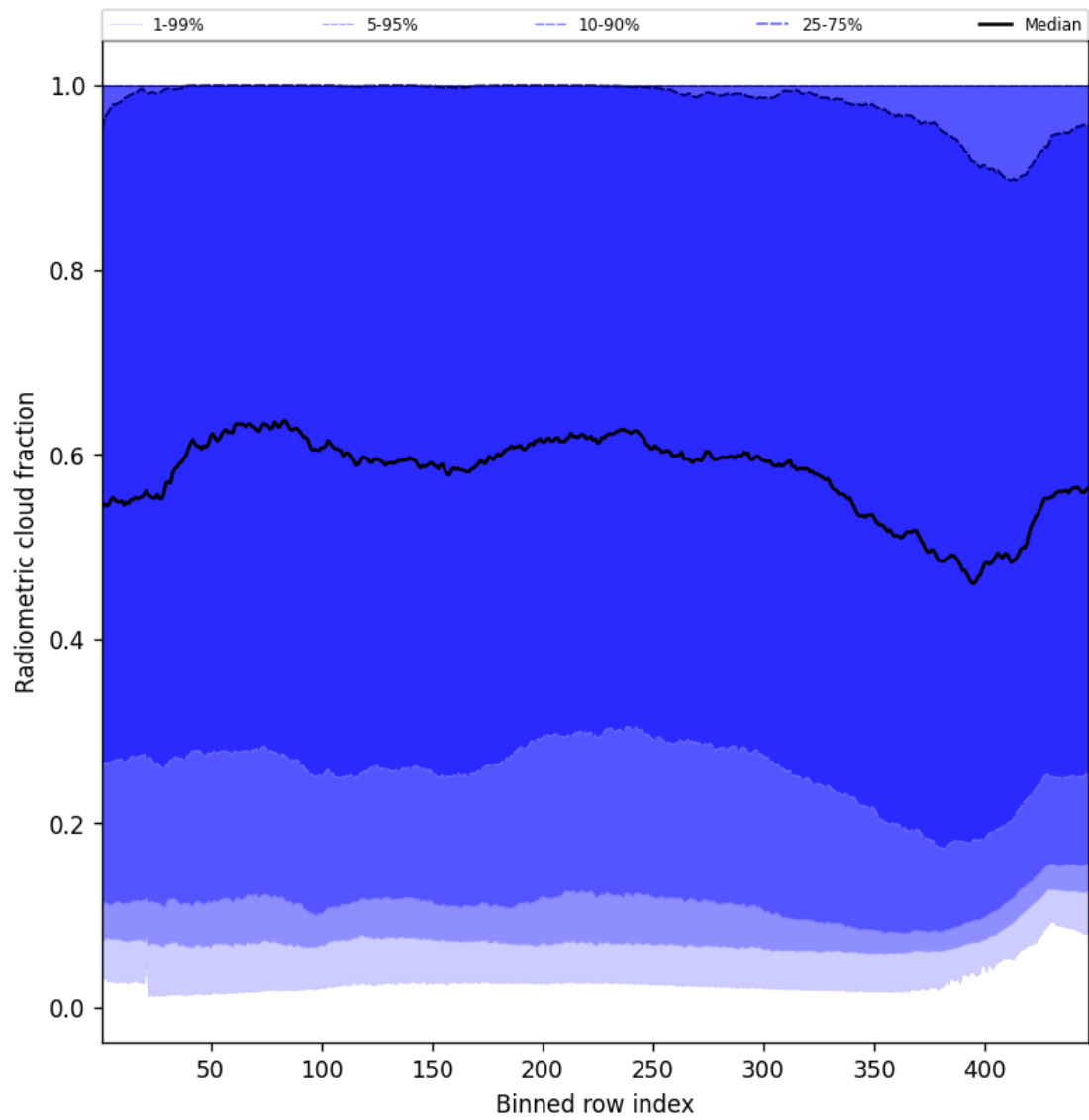
Figure 55: Along track statistics of “Radiometric cloud fraction” for 2025-10-06 to 2025-10-07
