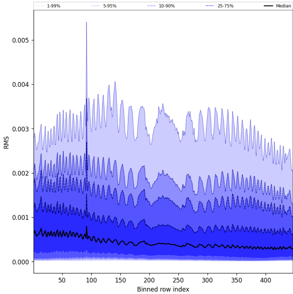
Figure 63: Along track statistics of “RMS” for 2025-10-06 to 2025-10-07
