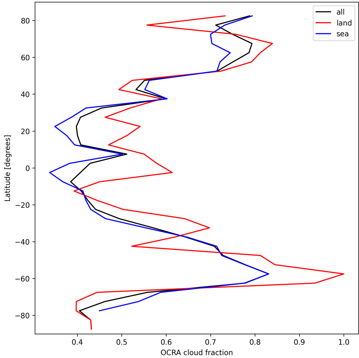
Figure 34: Zonal average of “OCRA cloud fraction” for 2025-10-06 to 2025-10-07.
