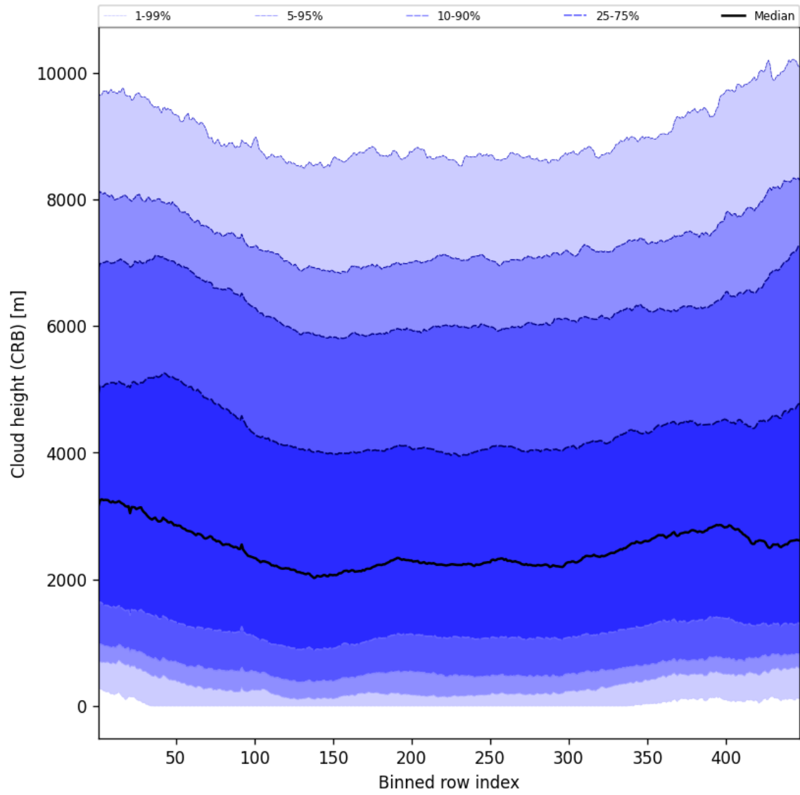
Figure 59: Along track statistics of “Cloud height (CRB)” for 2025-10-06 to 2025-10-07
