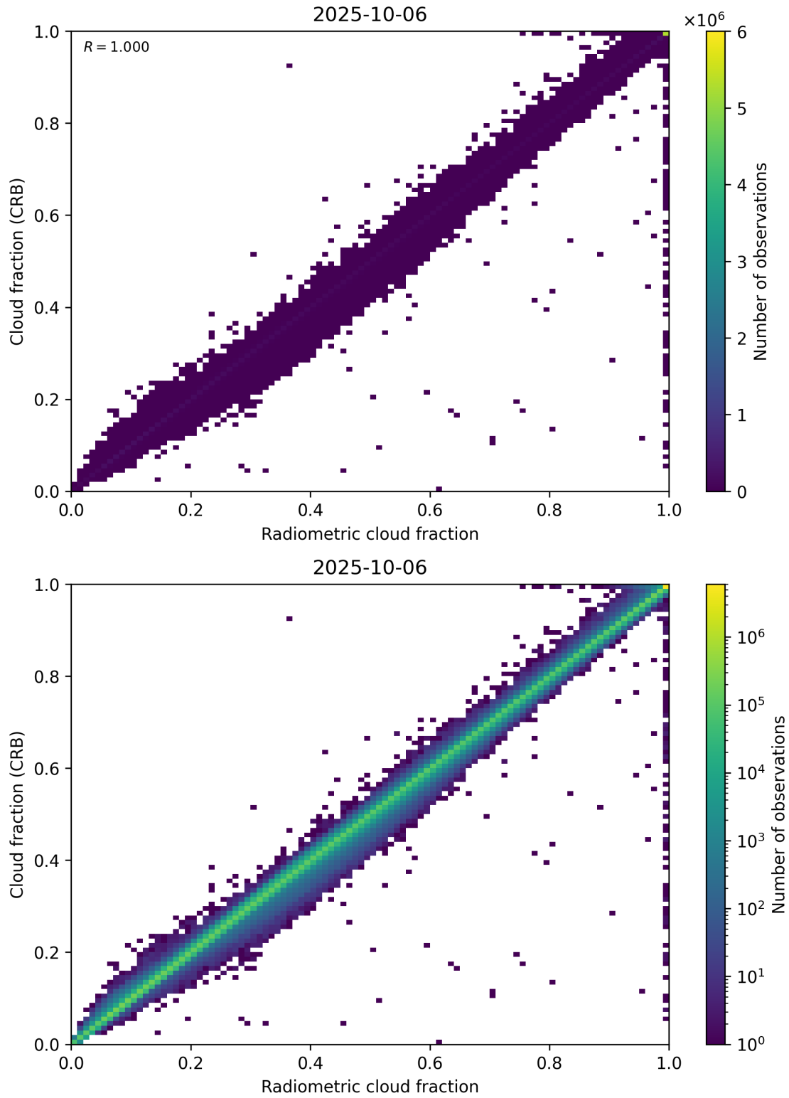
Figure 73: Scatter density plot of “Radiometric cloud fraction” against “Cloud fraction (CRB)” for 2025-10-06 to 2025-10-07.
