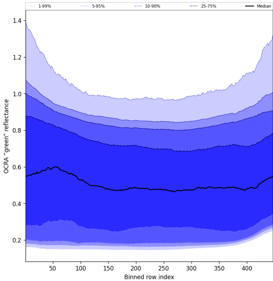
Figure 68: Along track statistics of “OCRA “green” reflectance” for 2025-10-06 to 2025-10-07
