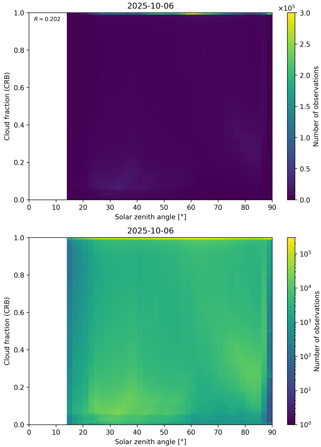
Figure 101: Scatter density plot of “Solar zenith angle” against “Cloud fraction (CRB)” for 2025-10-06 to 2025-10-07.
