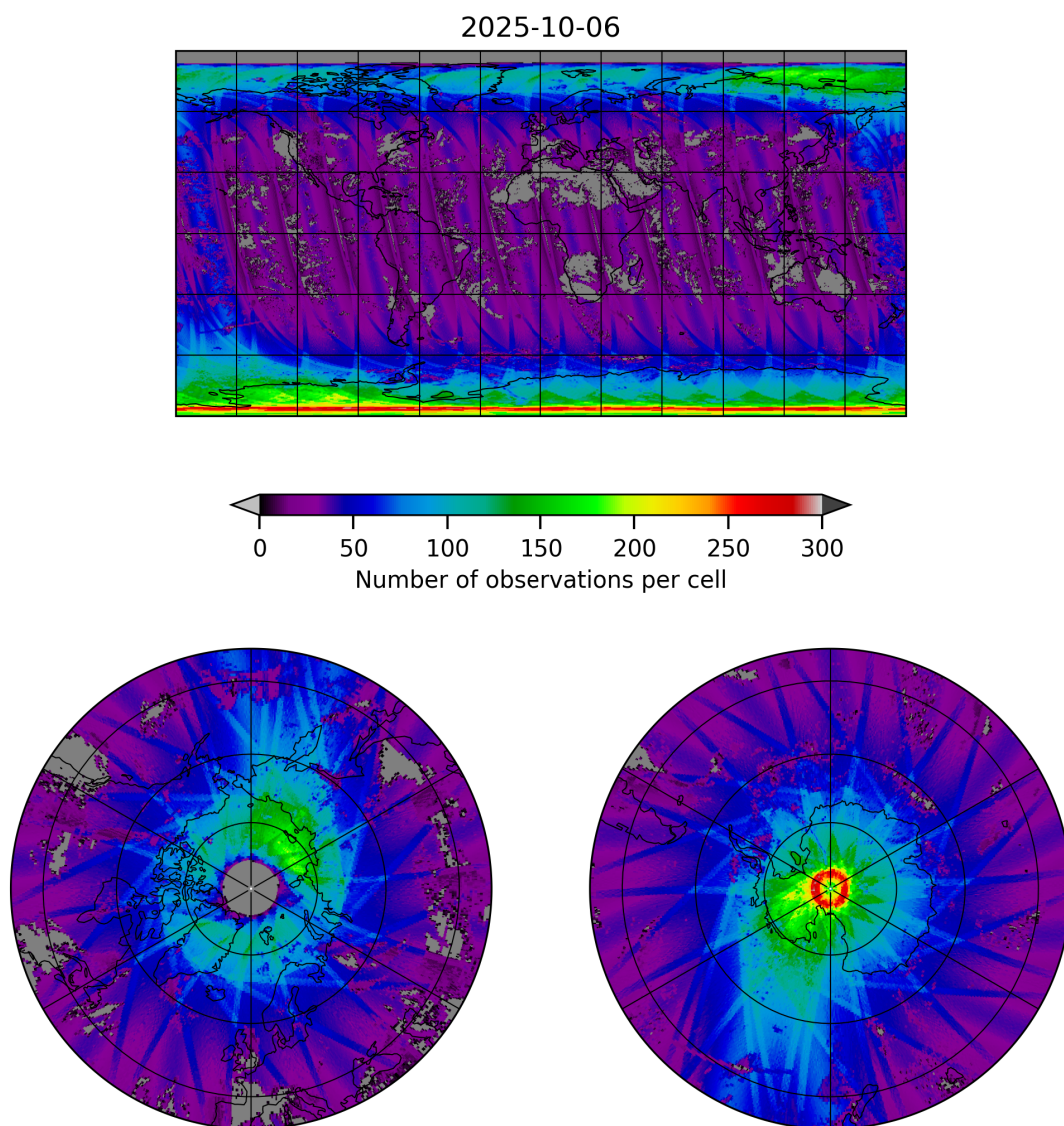
Figure 21: Map of the number of observations for 2025-10-06 to 2025-10-07
