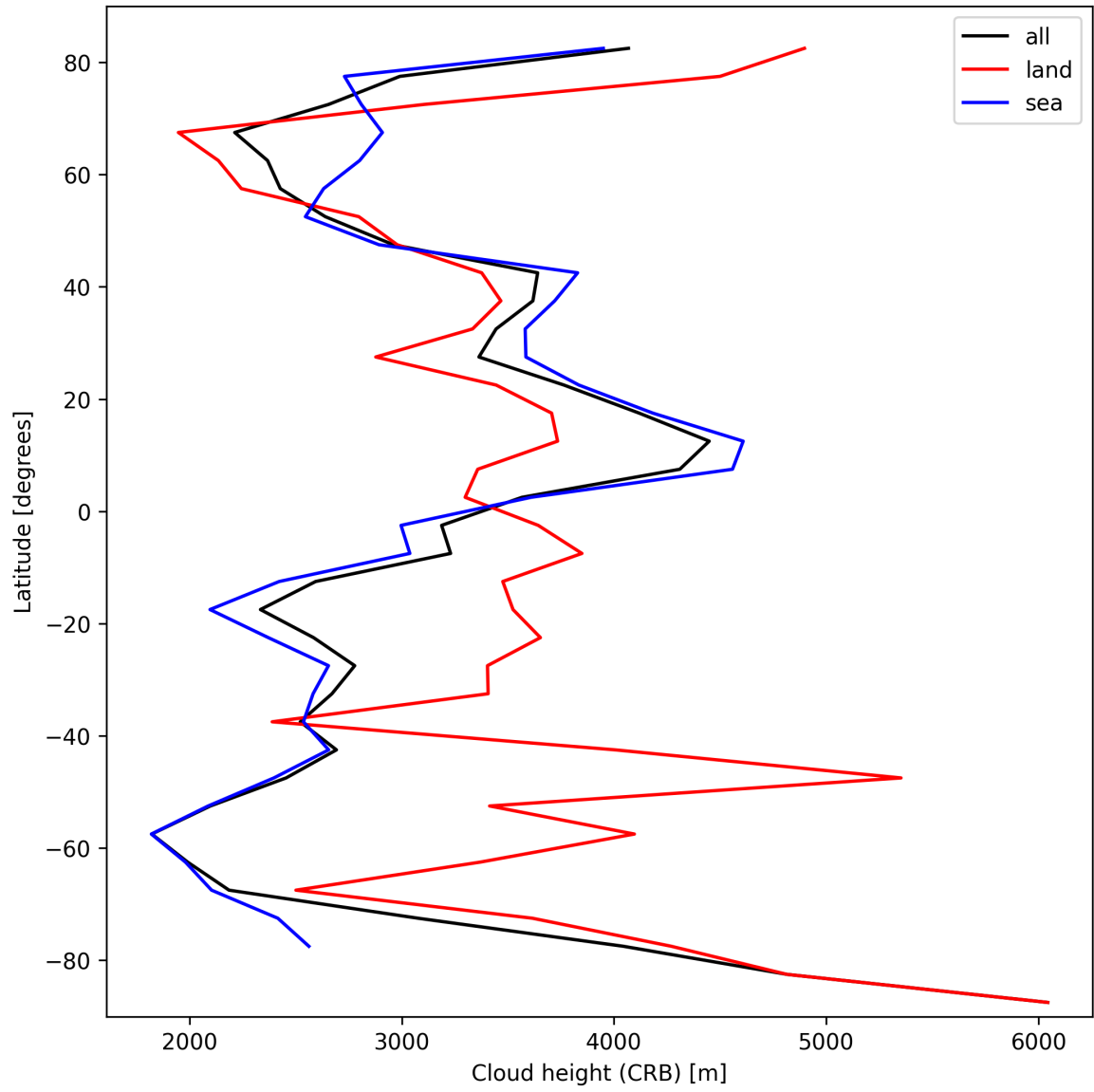
Figure 27: Zonal average of “Cloud height (CRB)” for 2025-10-06 to 2025-10-07.
