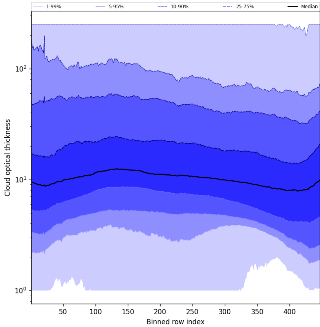
Figure 57: Along track statistics of “Cloud optical thickness” for 2025-10-06 to 2025-10-07
