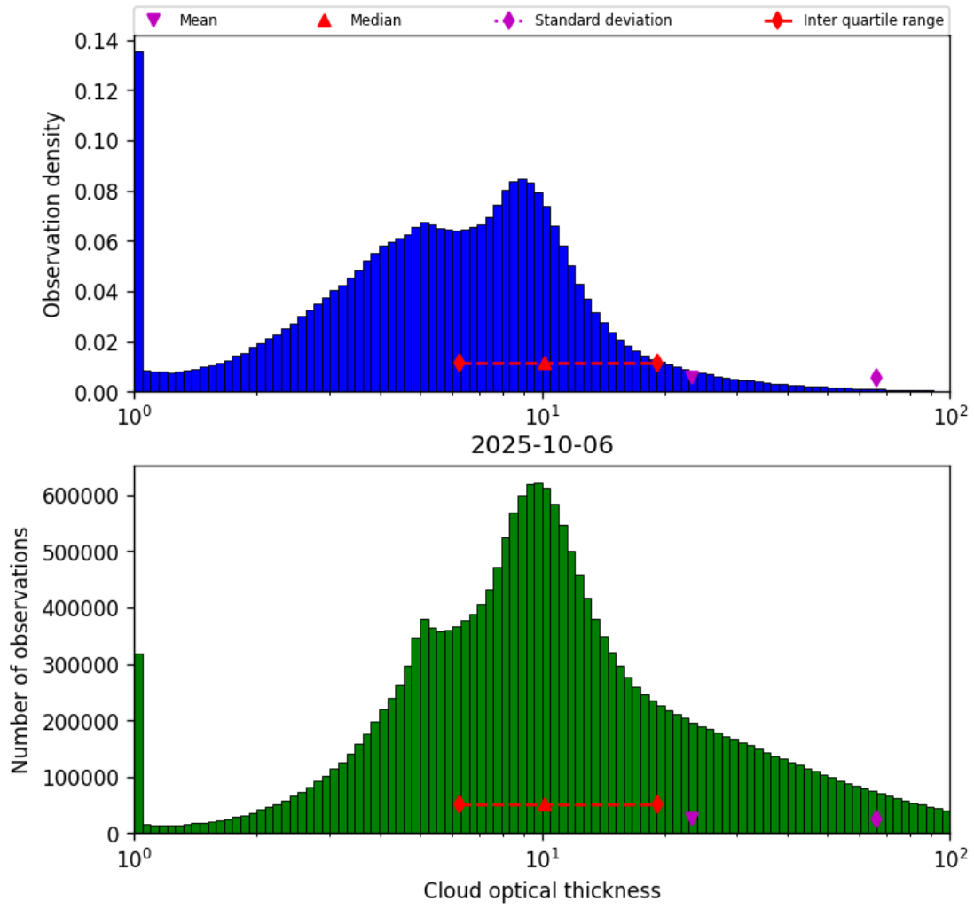
Figure 41: Histogram of “Cloud optical thickness” for 2025-10-06 to 2025-10-07
