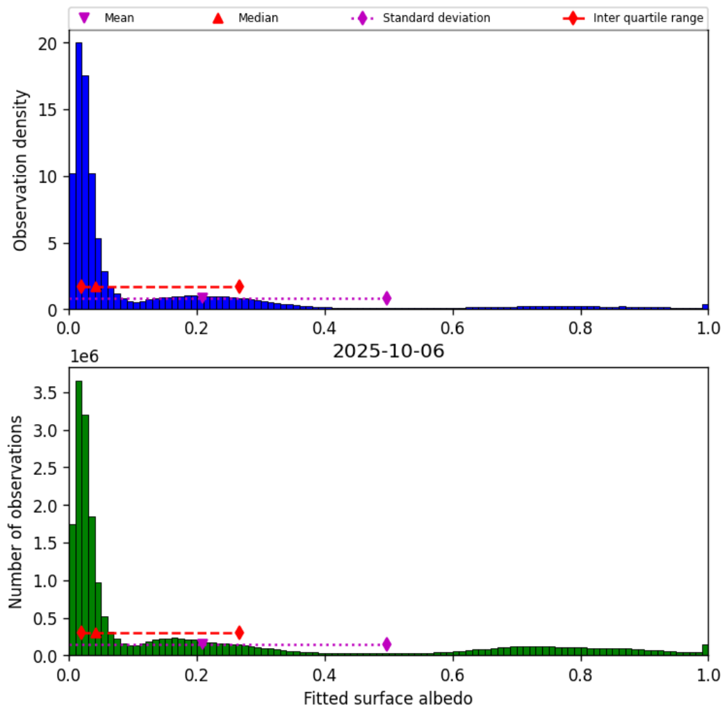
Figure 45: Histogram of “Fitted surface albedo” for 2025-10-06 to 2025-10-07
