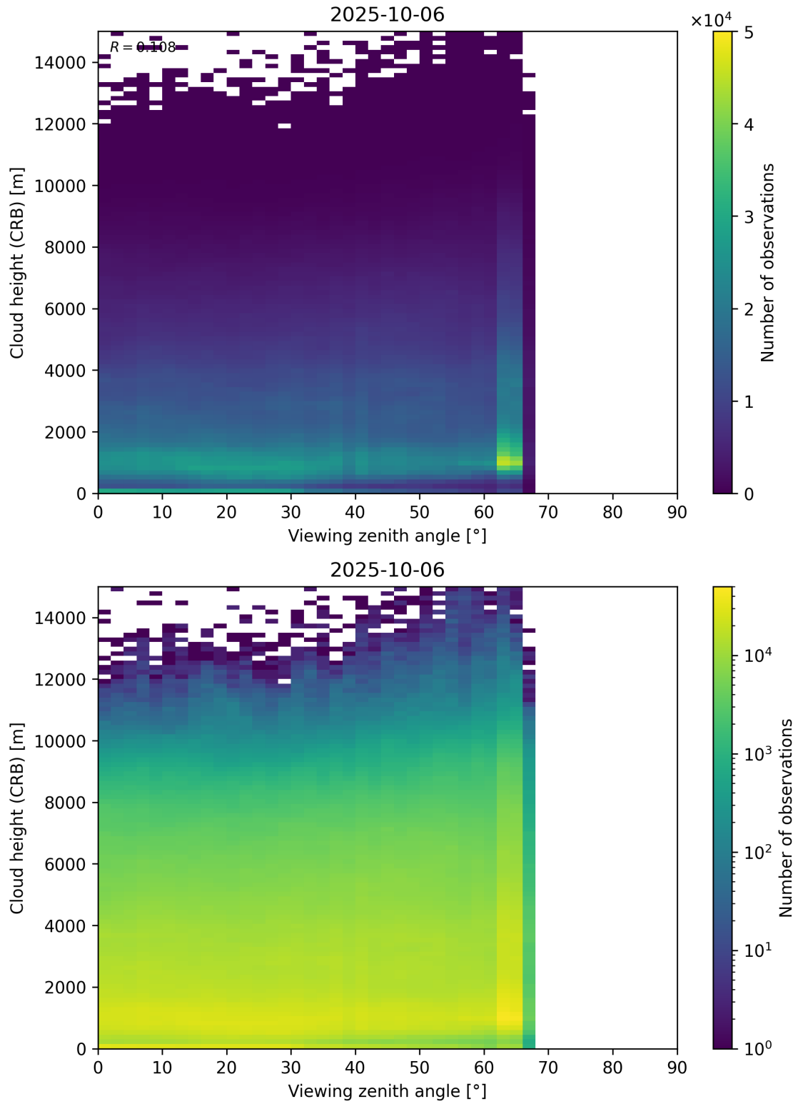
Figure 110: Scatter density plot of “Viewing zenith angle” against “Cloud height (CRB)” for 2025-10-06 to 2025-10-07.
