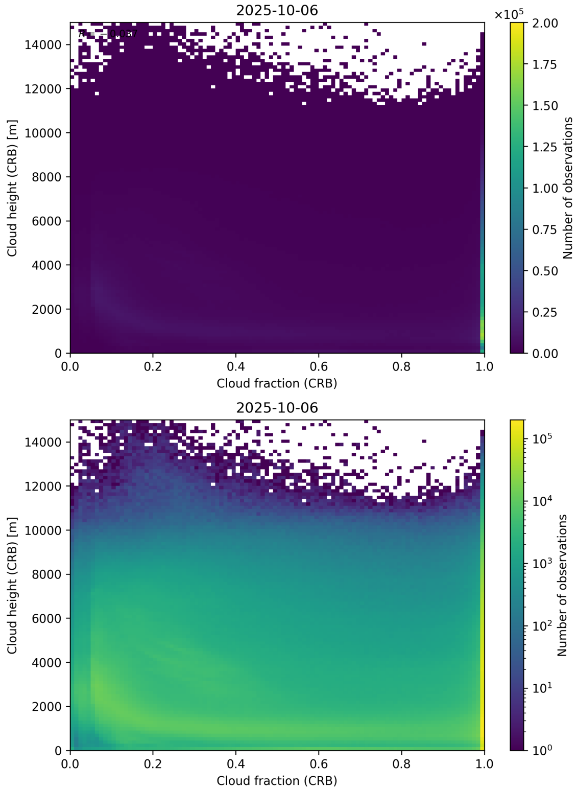
Figure 79: Scatter density plot of “Cloud fraction (CRB)” against “Cloud height (CRB)” for 2025-10-06 to 2025-10-07.
