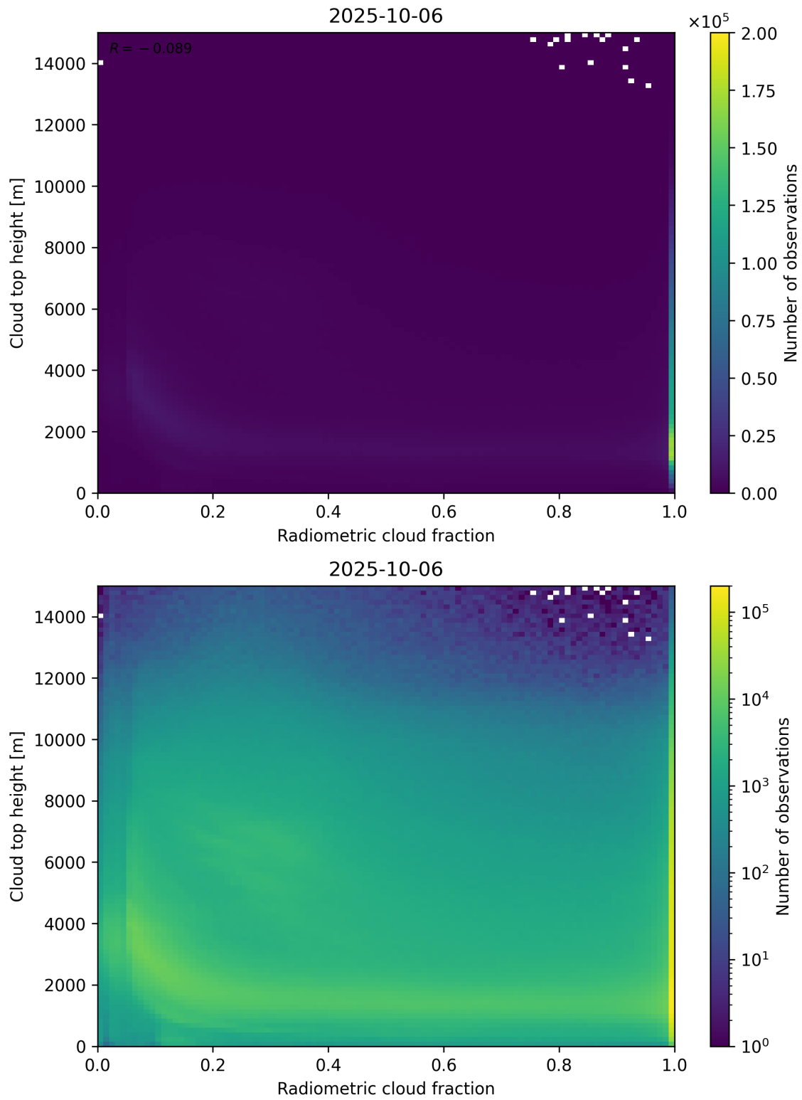
Figure 76: Scatter density plot of “Radiometric cloud fraction” against “Cloud top height” for 2025-10-06 to 2025-10-07.
