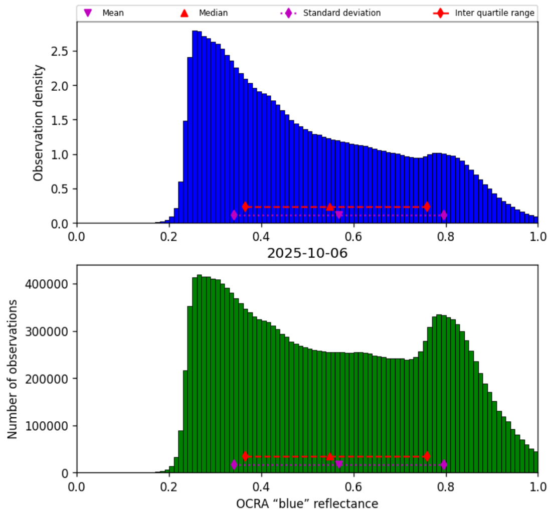
Figure 51: Histogram of “OCRA “blue” reflectance” for 2025-10-06 to 2025-10-07
