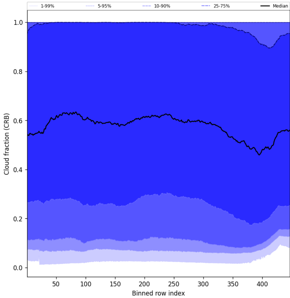
Figure 58: Along track statistics of “Cloud fraction (CRB)” for 2025-10-06 to 2025-10-07
