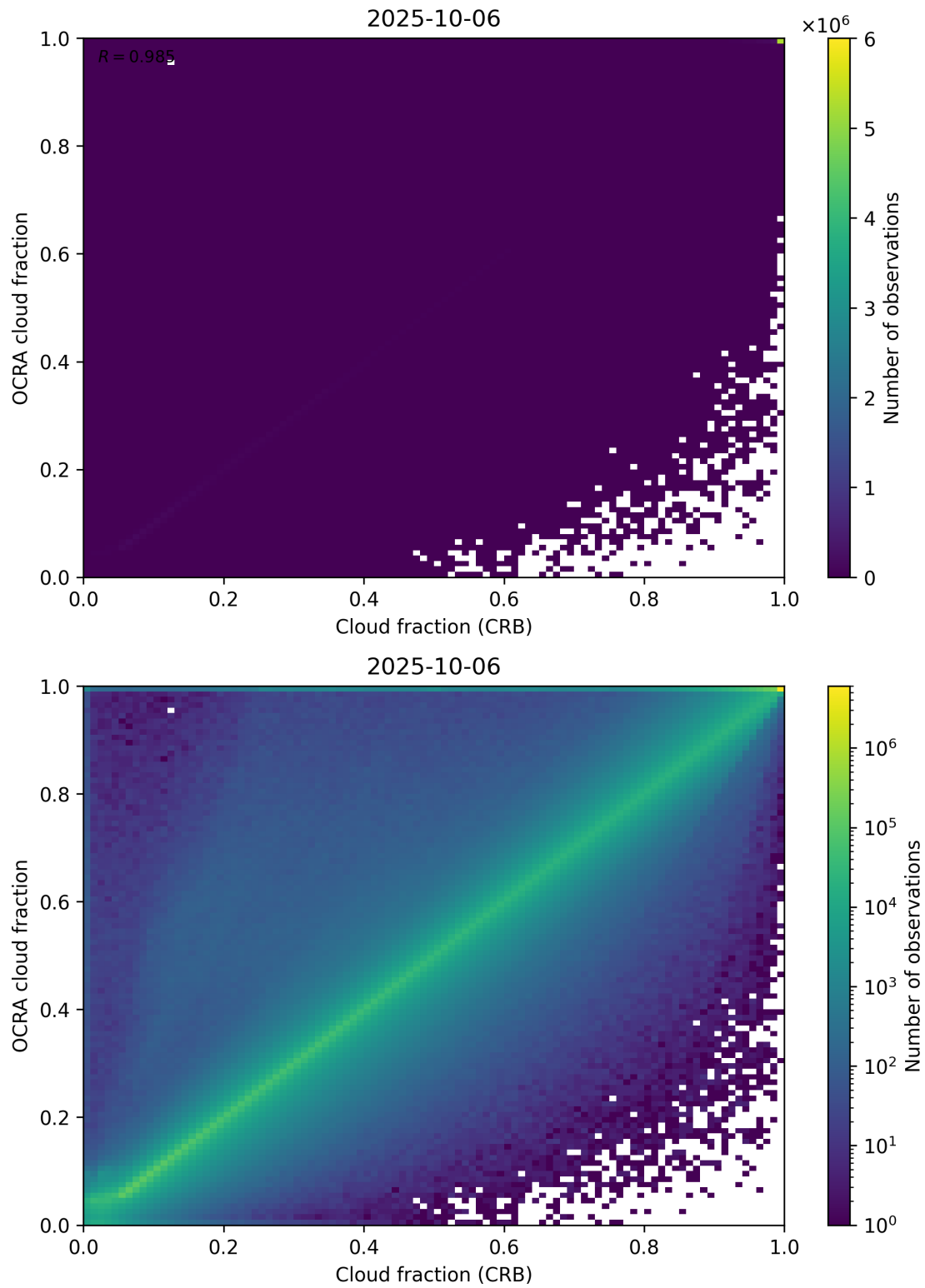
Figure 78: Scatter density plot of “Cloud fraction (CRB)” against “OCRA cloud fraction” for 2025-10-06 to 2025-10-07.
