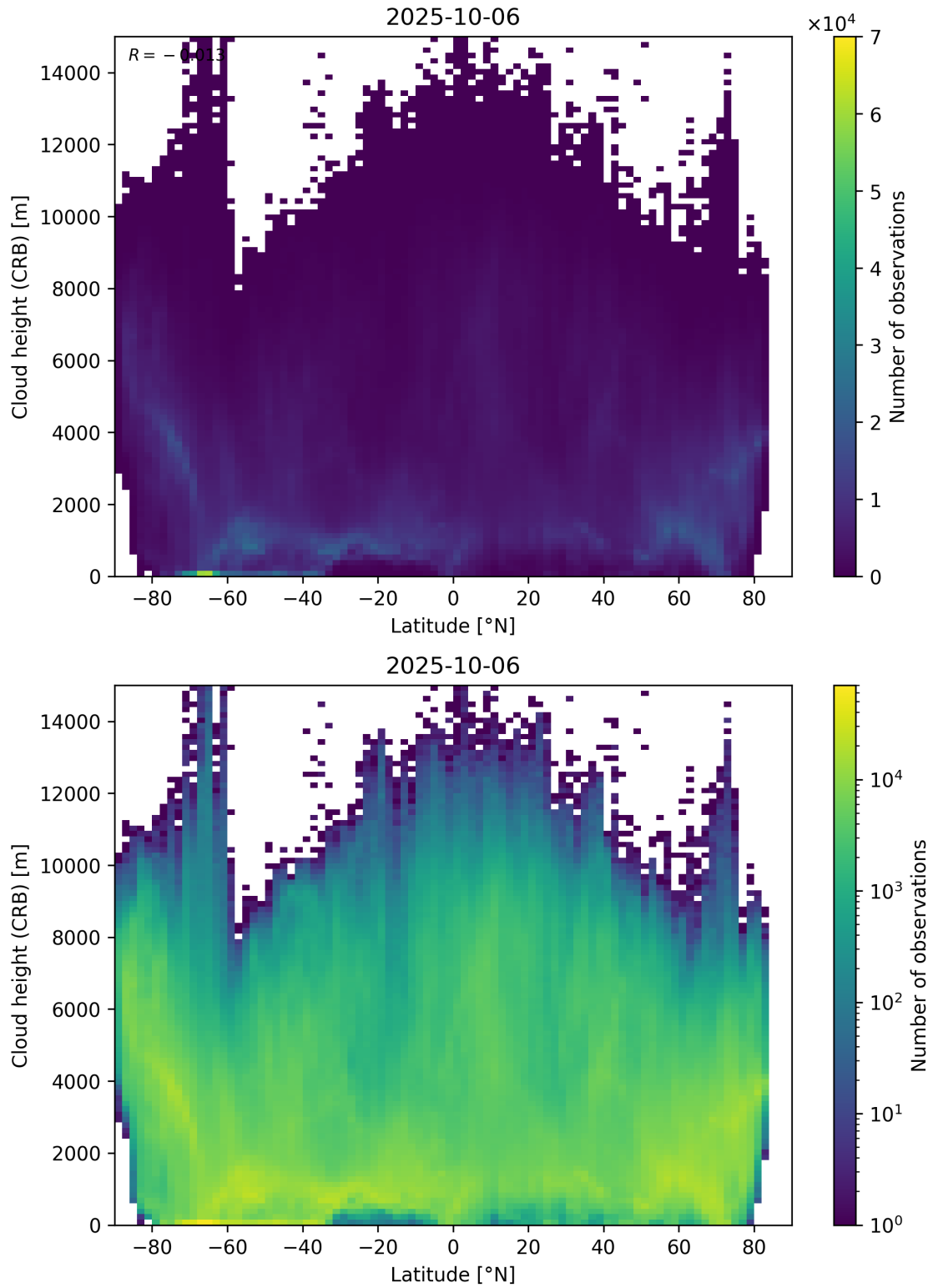
Figure 95: Scatter density plot of “Latitude” against “Cloud height (CRB)” for 2025-10-06 to 2025-10-07.
