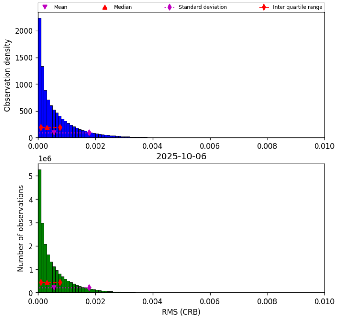
Figure 48: Histogram of “RMS (CRB)” for 2025-10-06 to 2025-10-07
