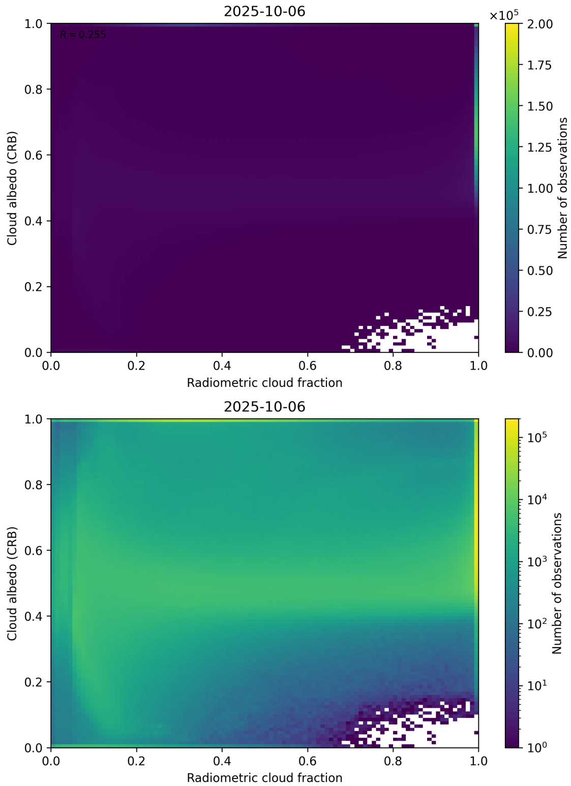
Figure 71: Scatter density plot of “Radiometric cloud fraction” against “Cloud albedo (CRB)” for 2025-10-06 to 2025-10-07.
