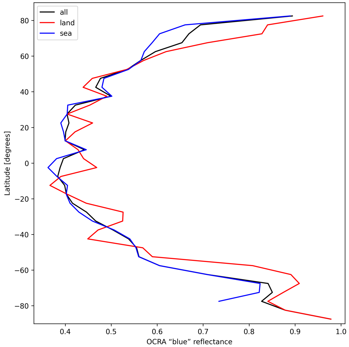
Figure 35: Zonal average of “OCRA “blue” reflectance” for 2025-10-06 to 2025-10-07.
