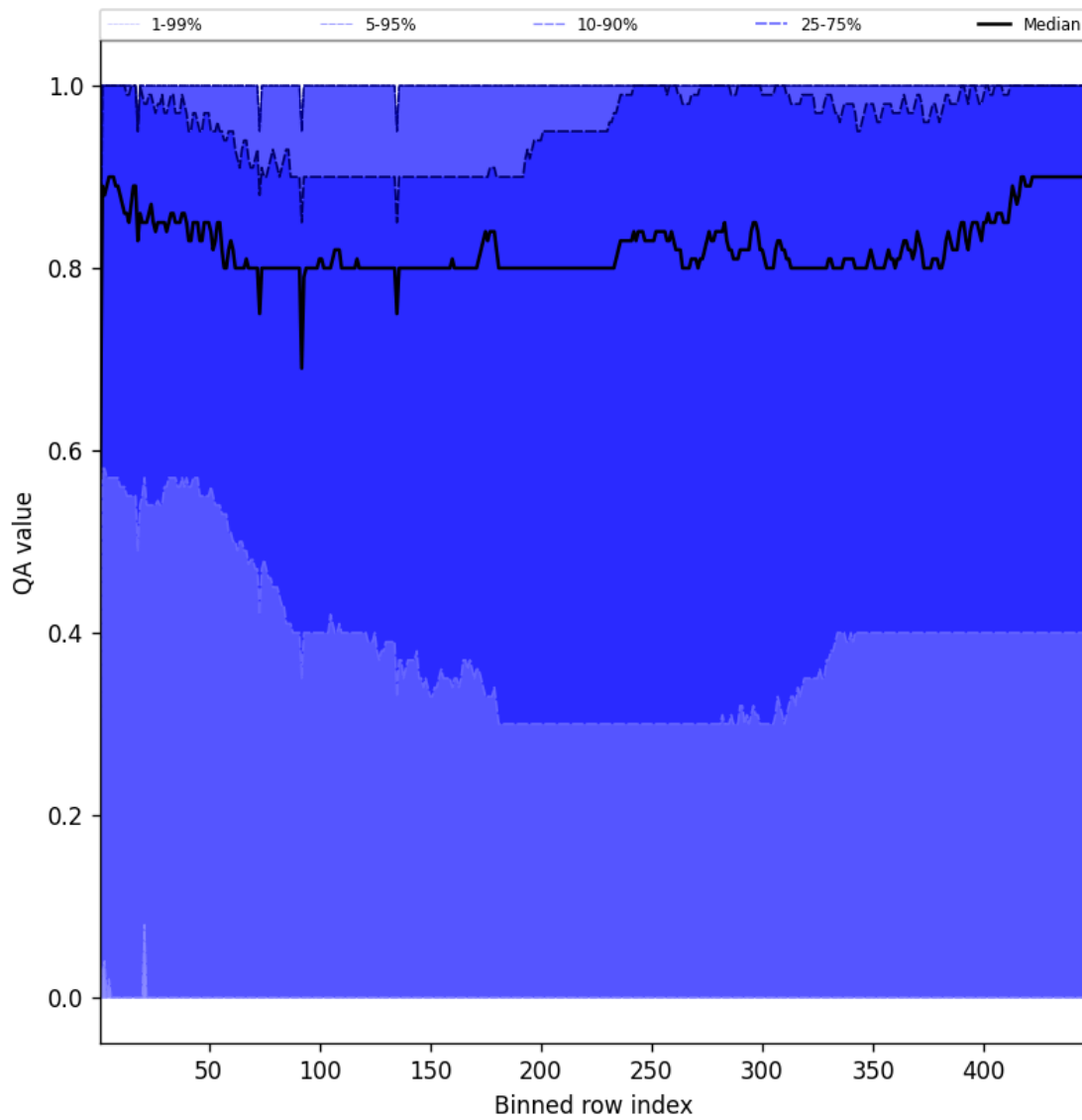
Figure 54: Along track statistics of “QA value” for 2025-10-06 to 2025-10-07
