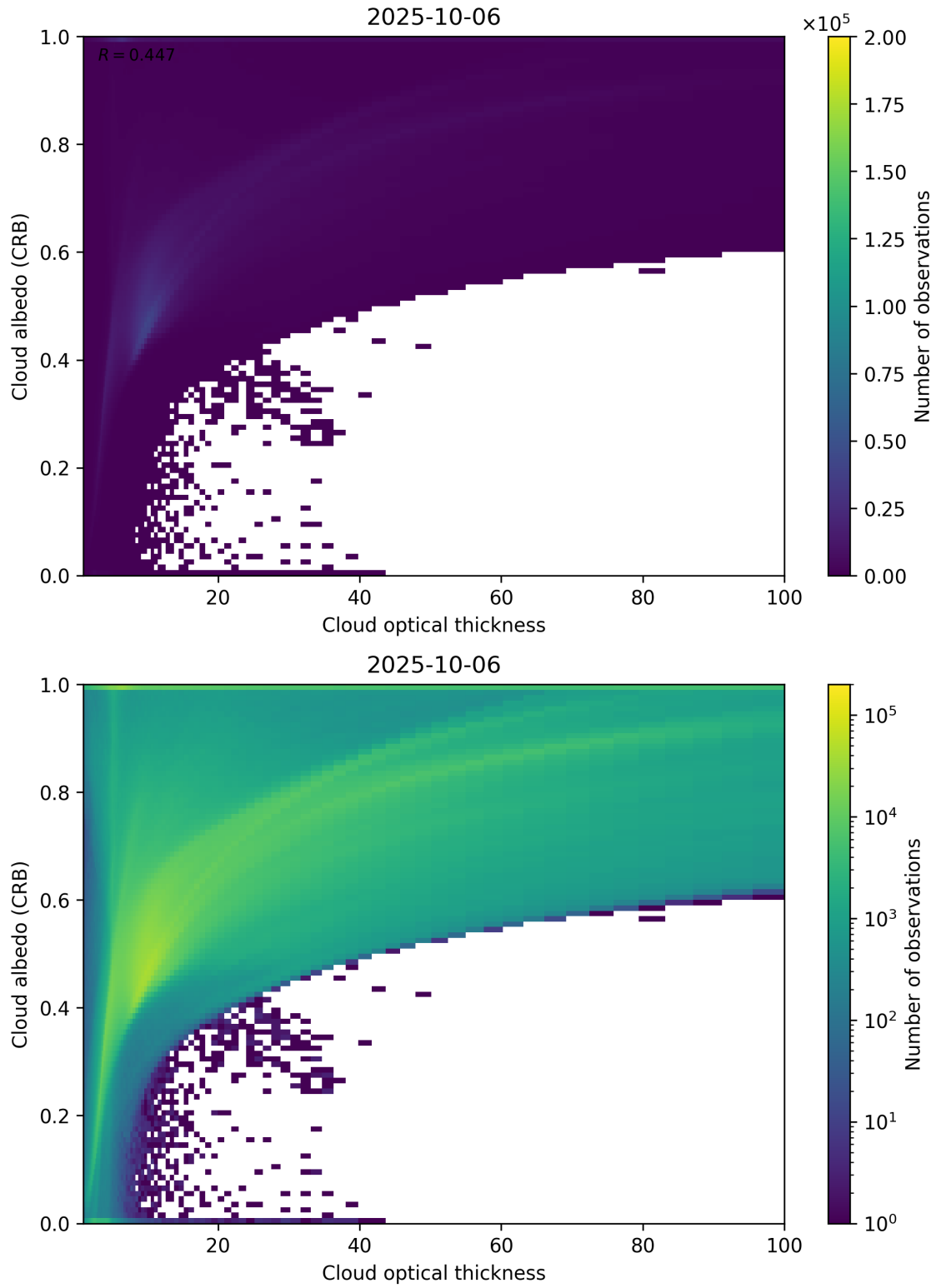
Figure 82: Scatter density plot of “Cloud optical thickness” against “Cloud albedo (CRB)” for 2025-10-06 to 2025-10-07.
