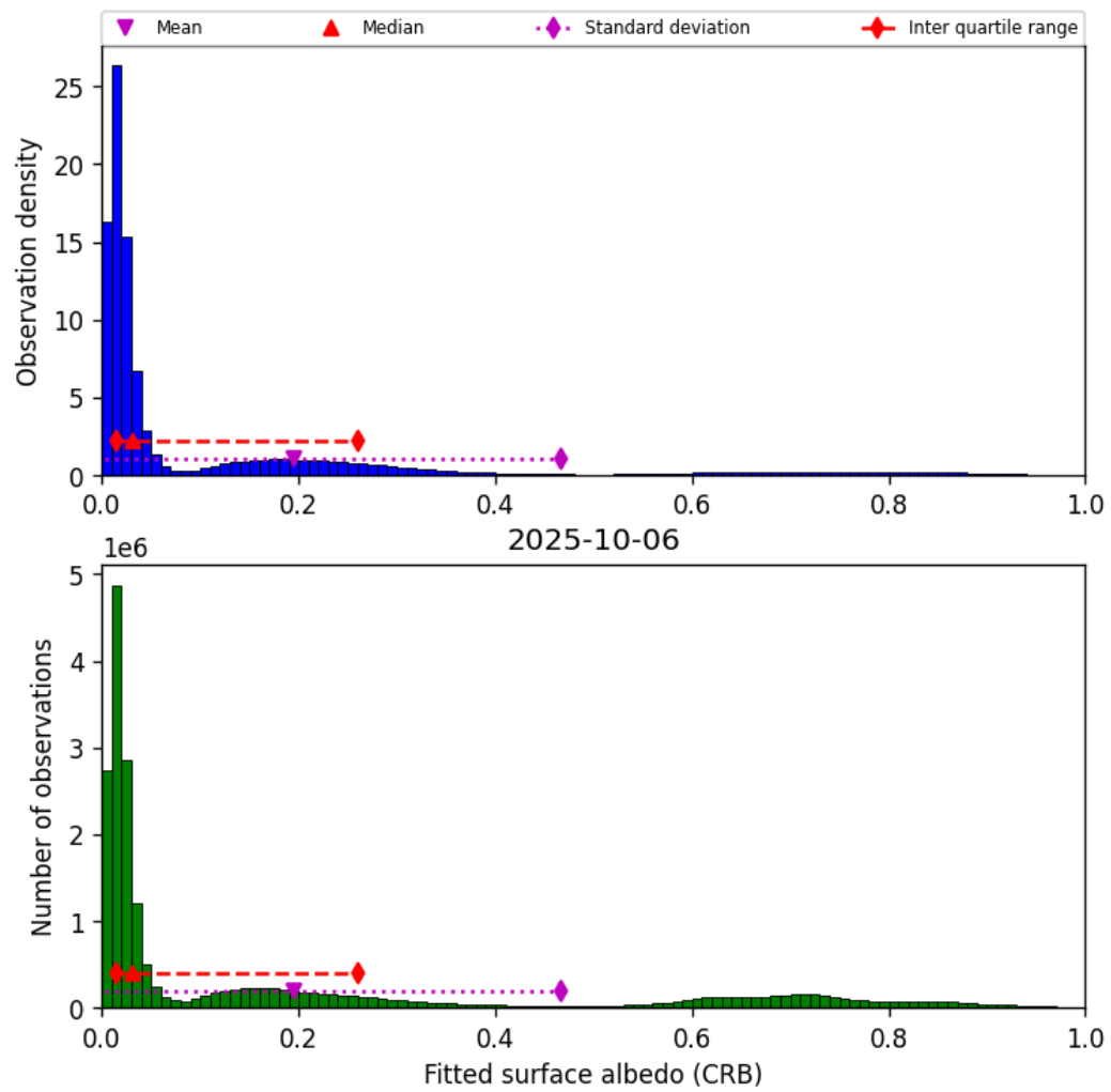
Figure 46: Histogram of “Fitted surface albedo (CRB)” for 2025-10-06 to 2025-10-07
