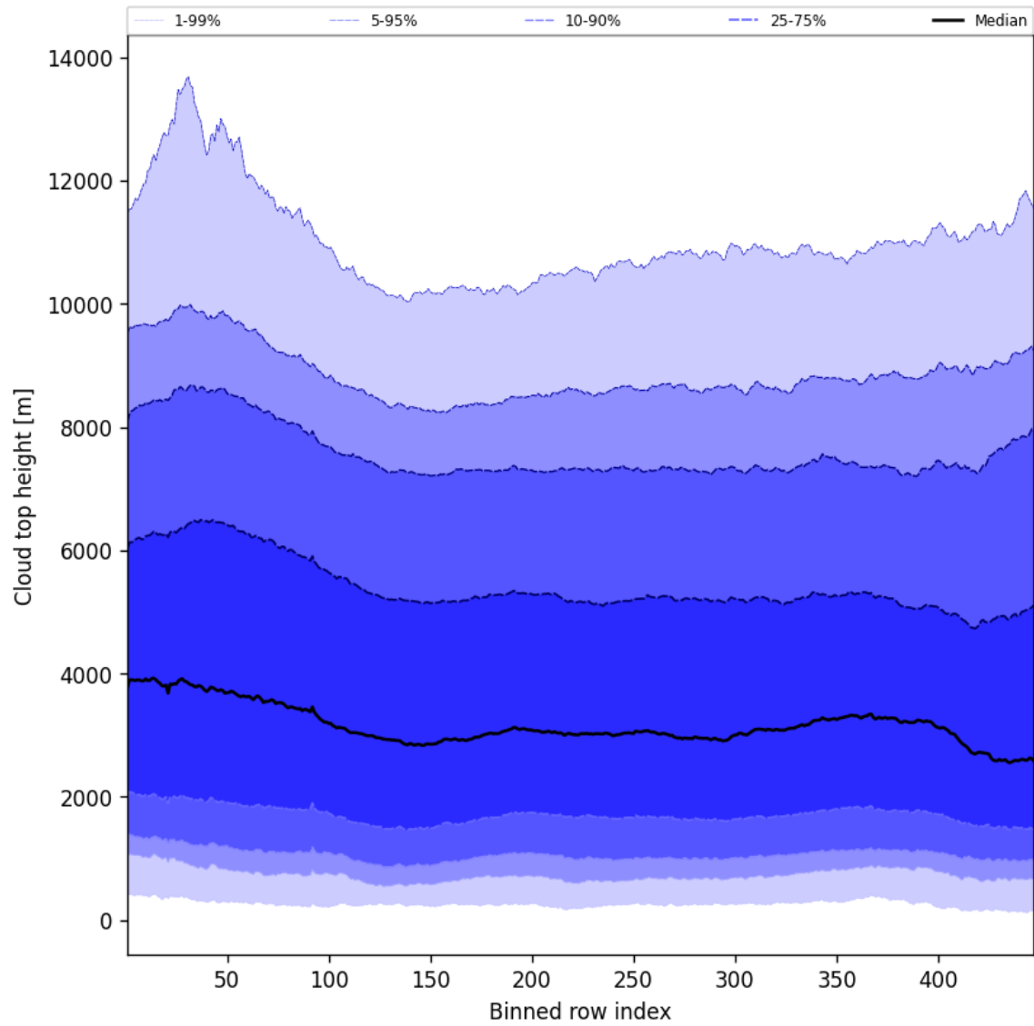
Figure 56: Along track statistics of “Cloud top height” for 2025-10-06 to 2025-10-07
