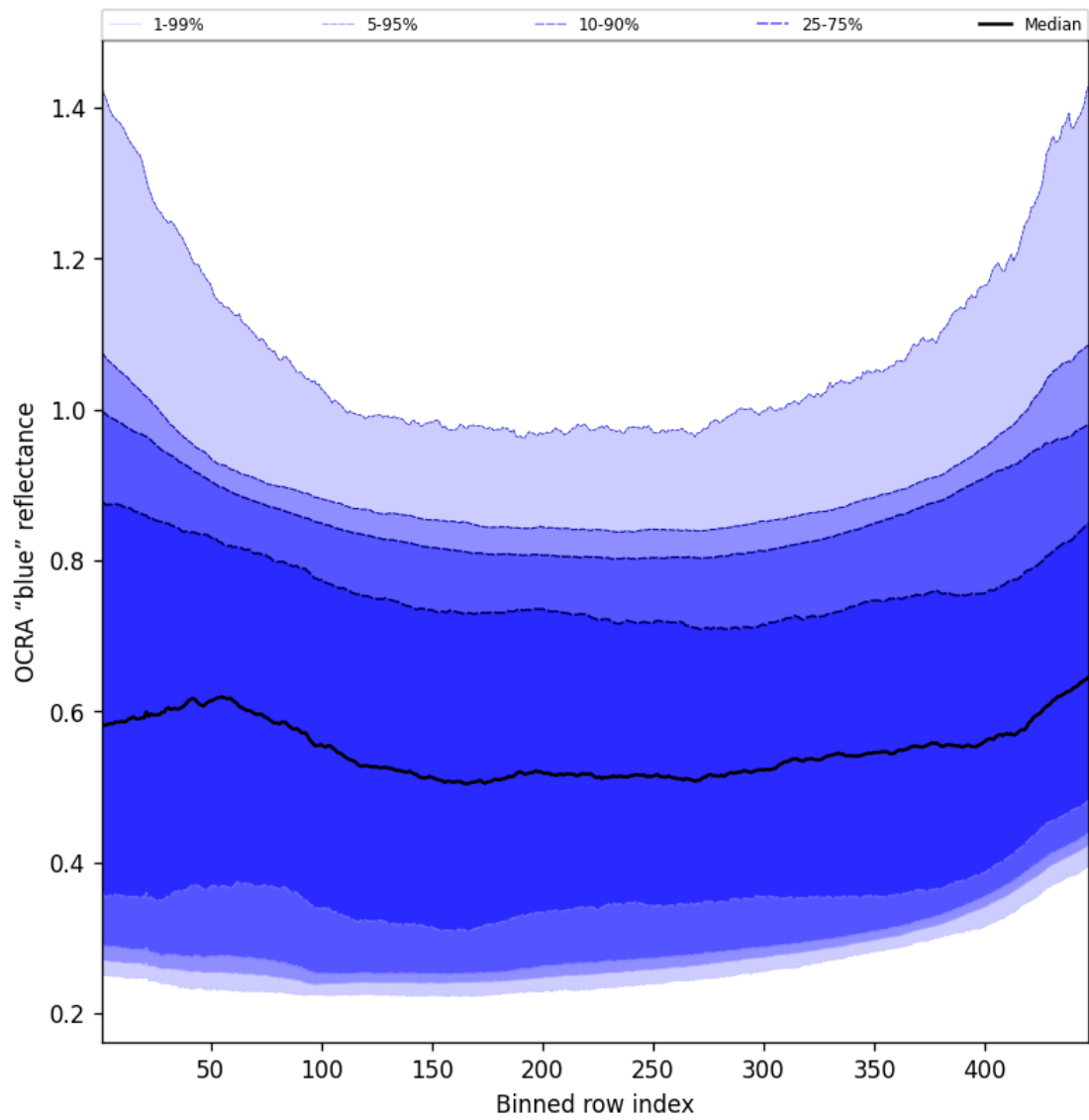
Figure 67: Along track statistics of “OCRA “blue” reflectance” for 2025-10-06 to 2025-10-07
