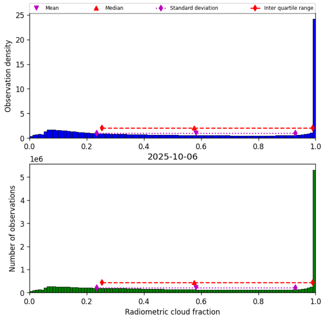
Figure 39: Histogram of “Radiometric cloud fraction” for 2025-10-06 to 2025-10-07
