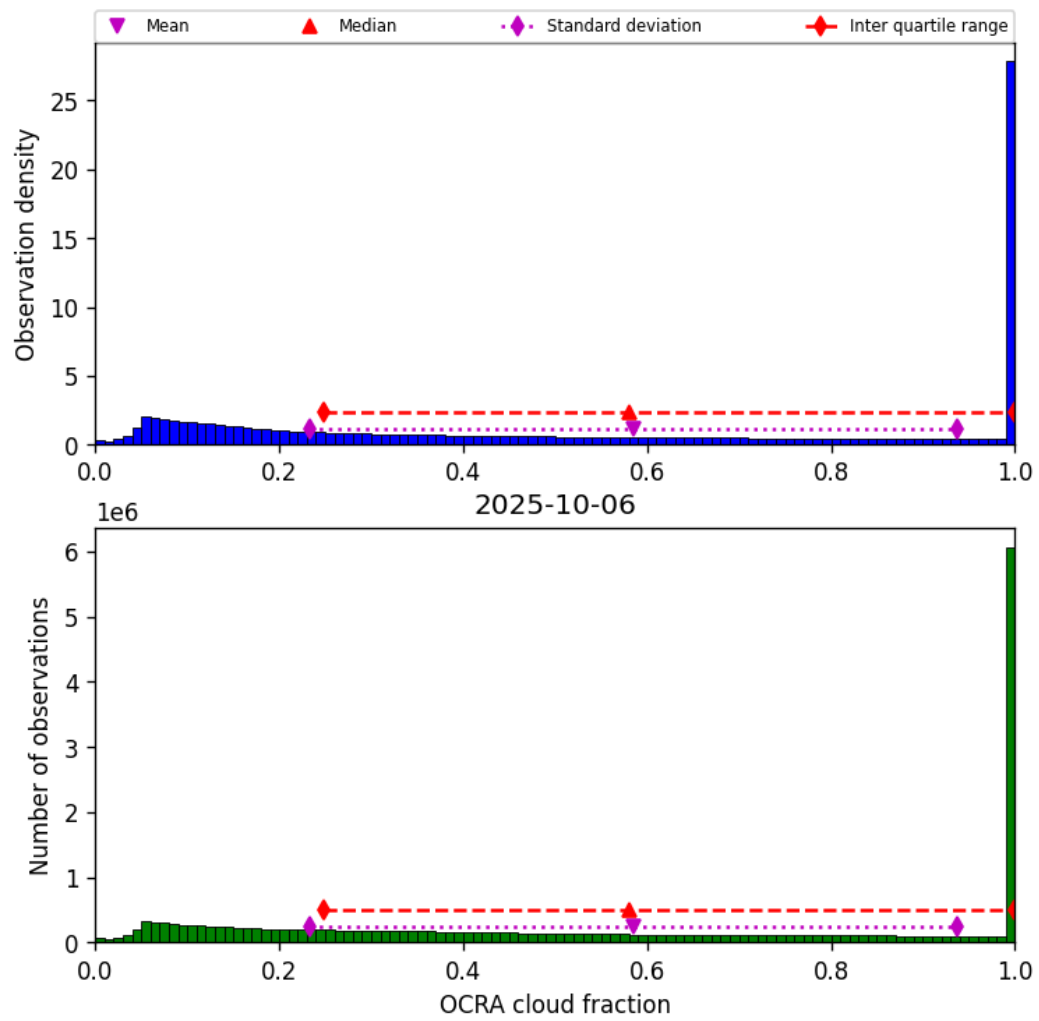
Figure 50: Histogram of “OCRA cloud fraction” for 2025-10-06 to 2025-10-07
