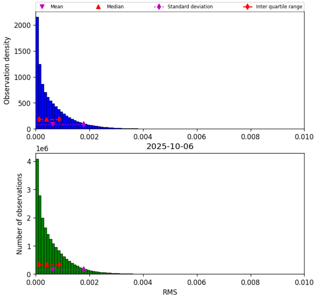
Figure 47: Histogram of “RMS” for 2025-10-06 to 2025-10-07
