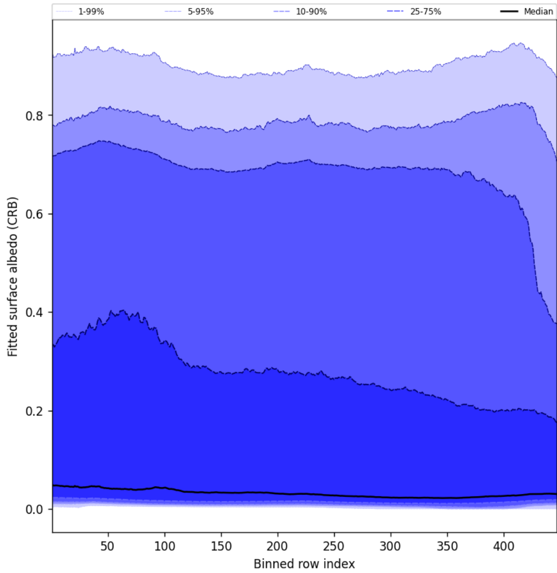
Figure 62: Along track statistics of “Fitted surface albedo (CRB)” for 2025-10-06 to 2025-10-07
