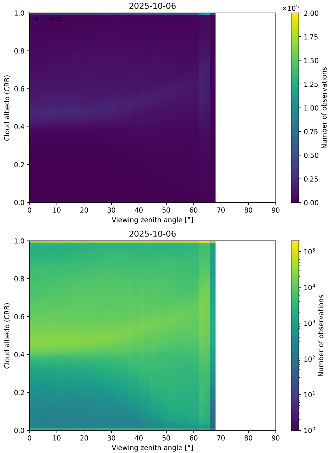
Figure 106: Scatter density plot of “Viewing zenith angle” against “Cloud albedo (CRB)” for 2025-10-06 to 2025-10-07.
