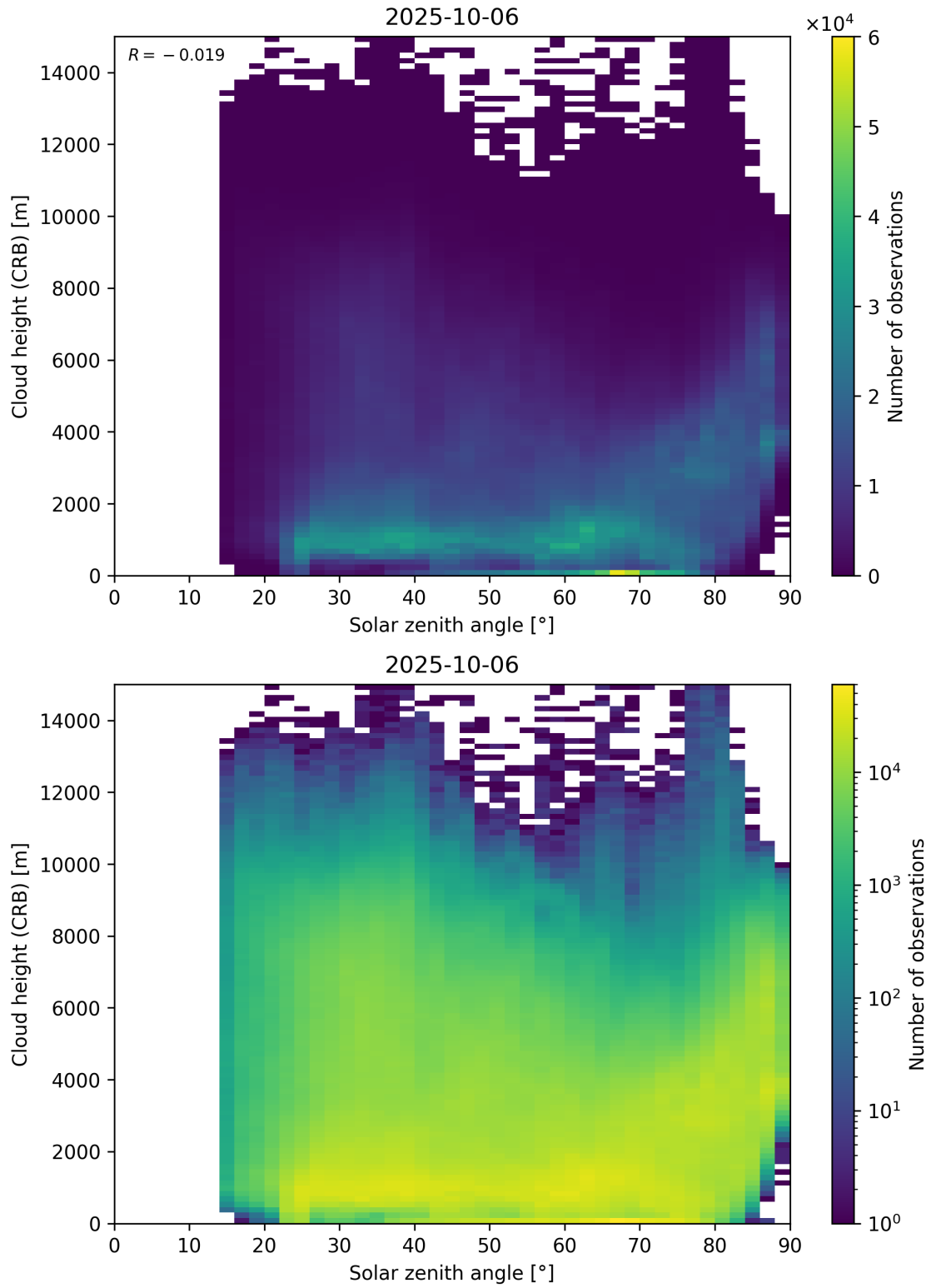
Figure 102: Scatter density plot of “Solar zenith angle” against “Cloud height (CRB)” for 2025-10-06 to 2025-10-07.
