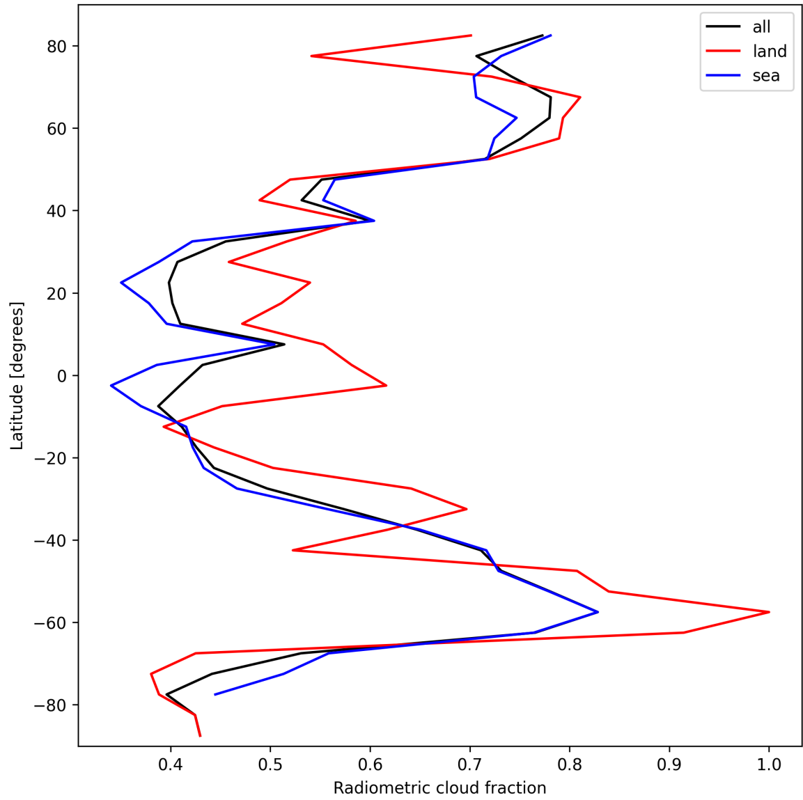
Figure 23: Zonal average of “Radiometric cloud fraction” for 2025-10-06 to 2025-10-07.
