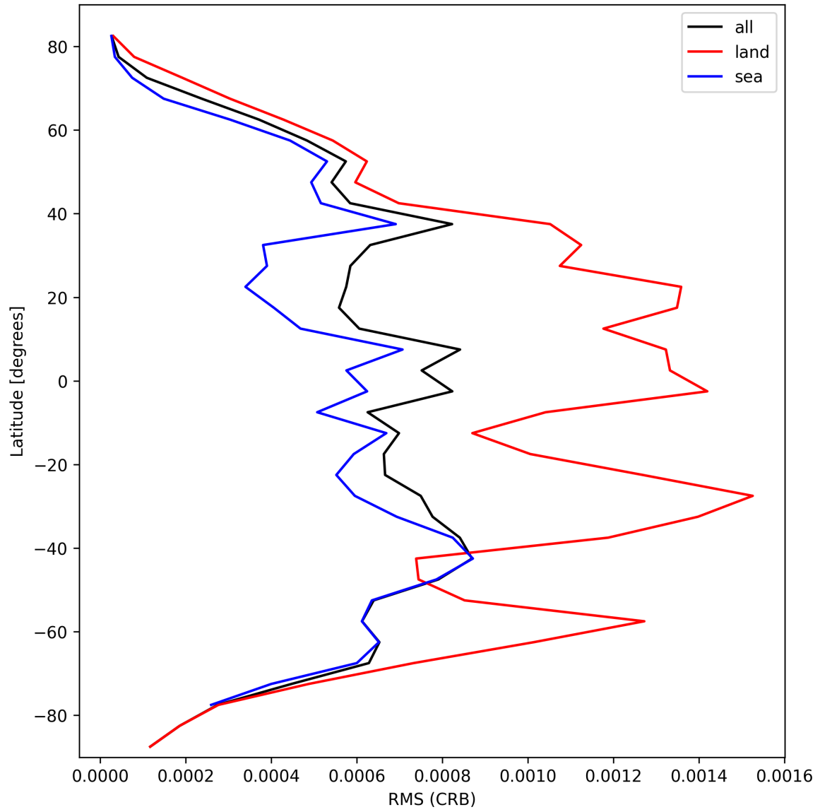
Figure 32: Zonal average of “RMS (CRB)” for 2025-10-06 to 2025-10-07.
