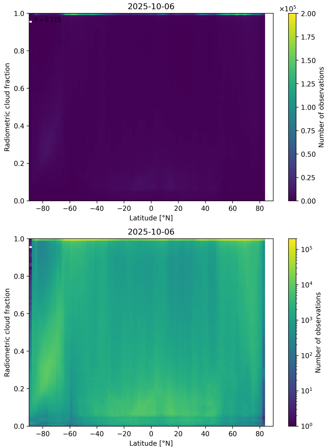
Figure 92: Scatter density plot of “Latitude” against “Radiometric cloud fraction” for 2025-10-06 to 2025-10-07.
