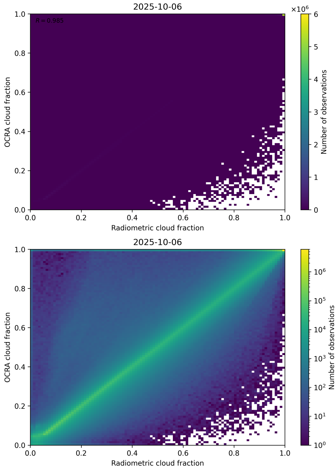
Figure 72: Scatter density plot of “Radiometric cloud fraction” against “OCRA cloud fraction” for 2025-10-06 to 2025-10-07.
