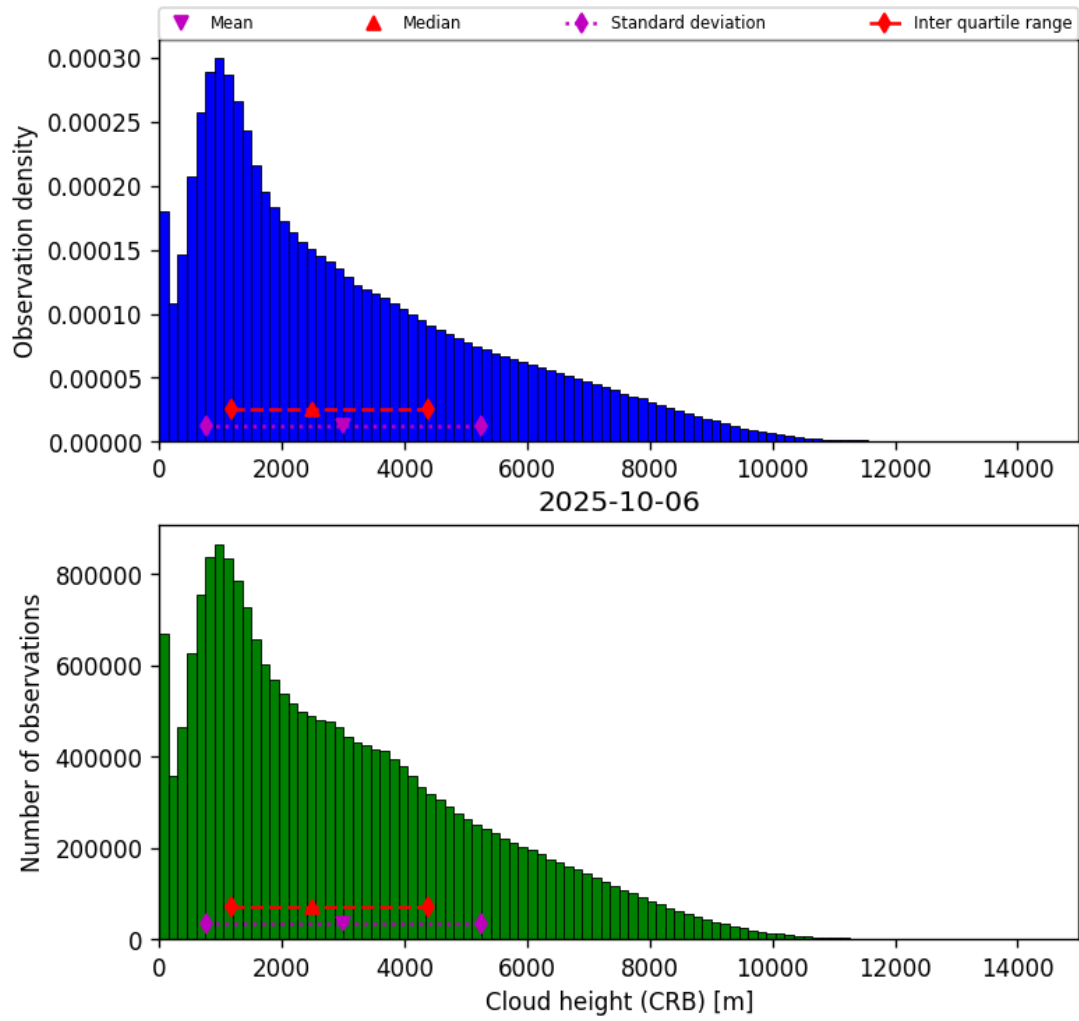
Figure 43: Histogram of “Cloud height (CRB)” for 2025-10-06 to 2025-10-07
