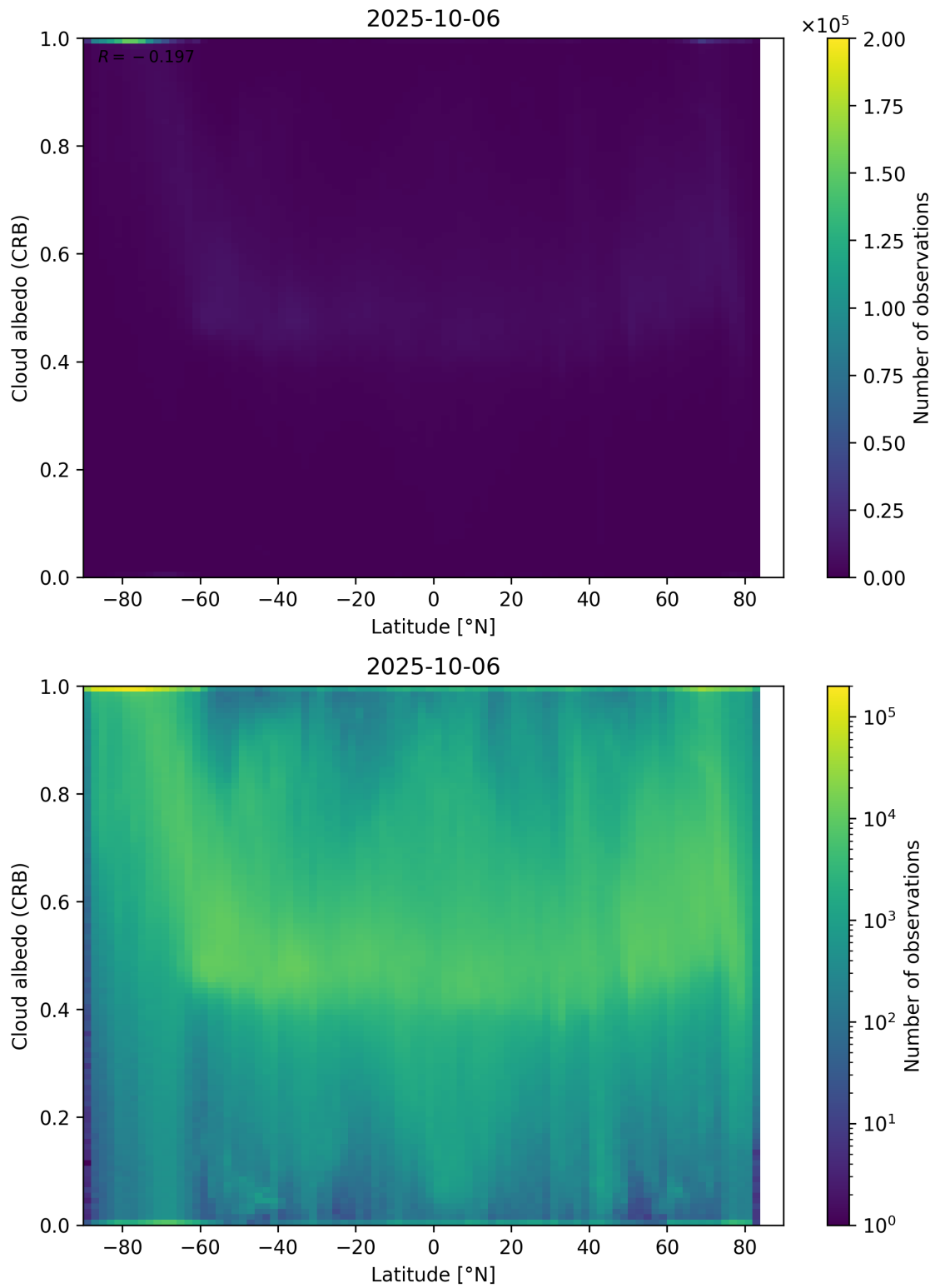
Figure 91: Scatter density plot of “Latitude” against “Cloud albedo (CRB)” for 2025-10-06 to 2025-10-07.
