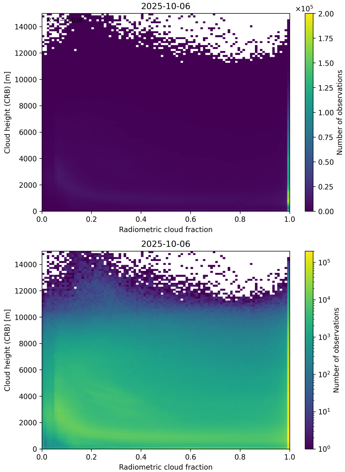
Figure 74: Scatter density plot of “Radiometric cloud fraction” against “Cloud height (CRB)” for 2025-10-06 to 2025-10-07.
