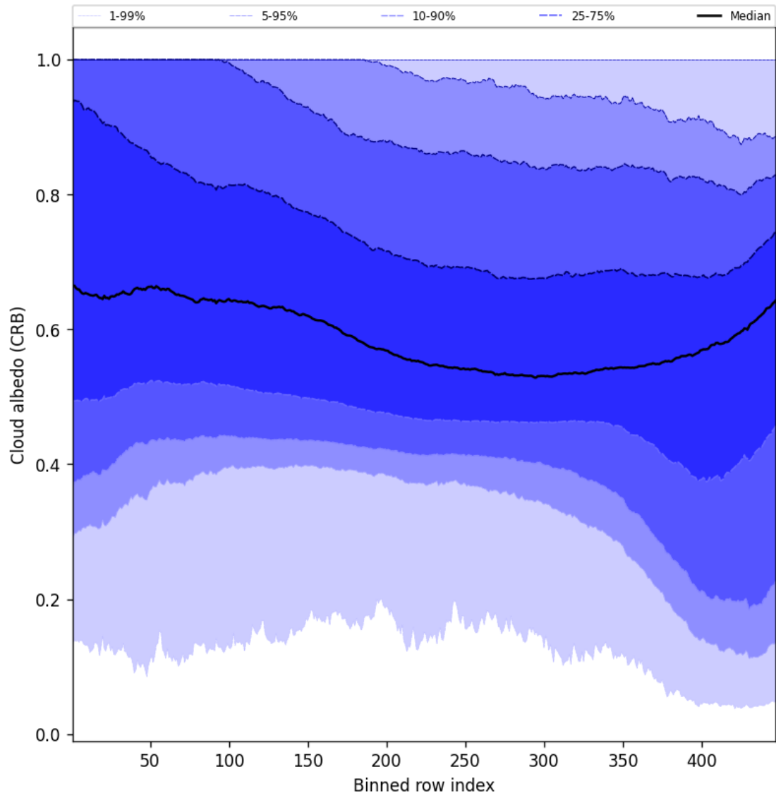
Figure 60: Along track statistics of “Cloud albedo (CRB)” for 2025-10-06 to 2025-10-07
