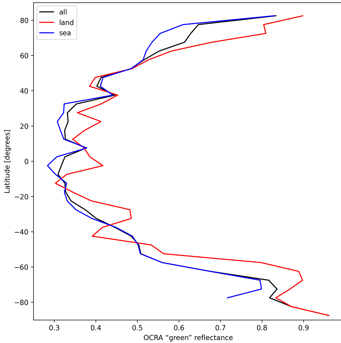
Figure 36: Zonal average of “OCRA “green” reflectance” for 2025-10-06 to 2025-10-07.
