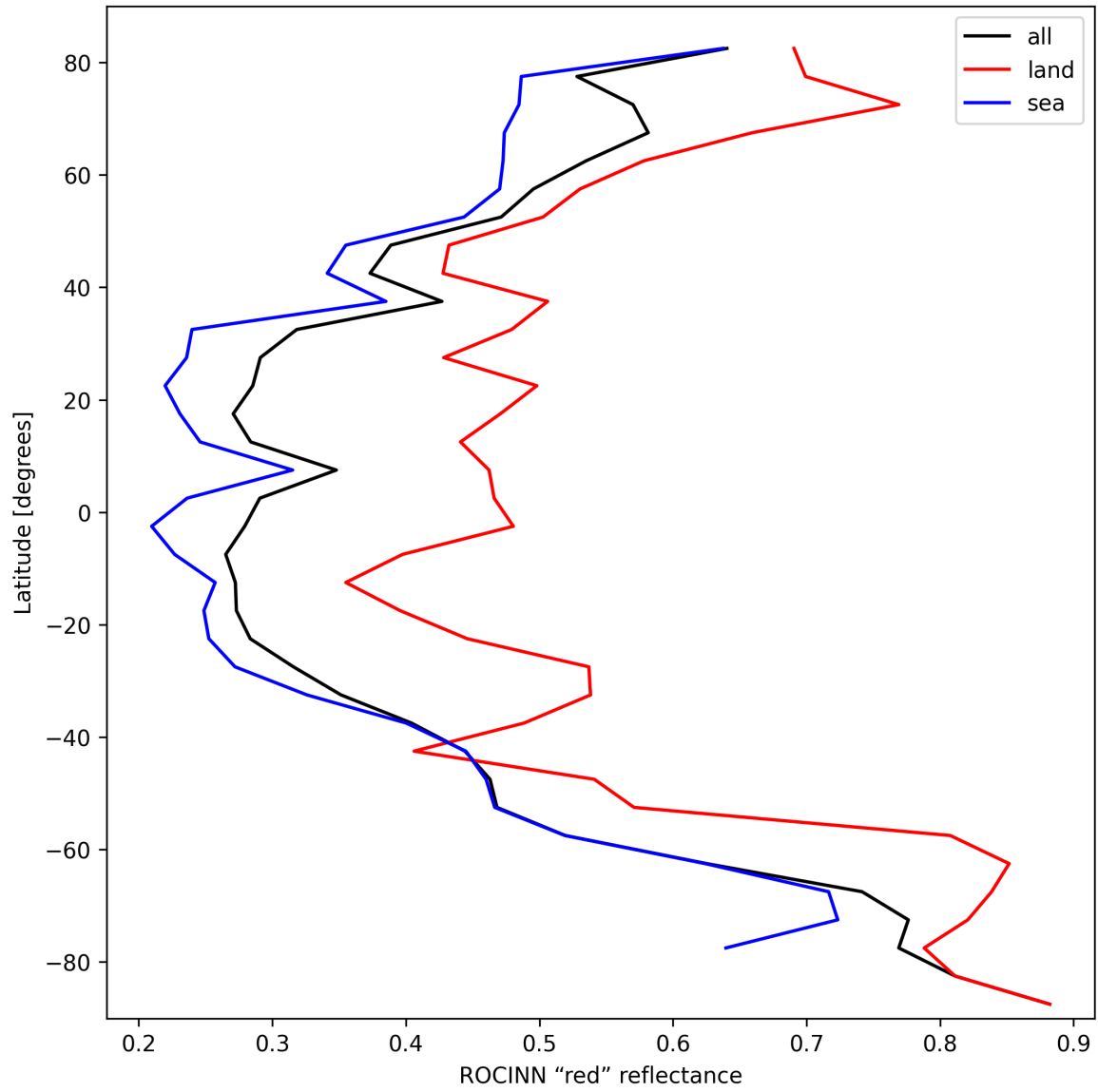
Figure 37: Zonal average of “ROCINN “red” reflectance” for 2025-10-06 to 2025-10-07.
