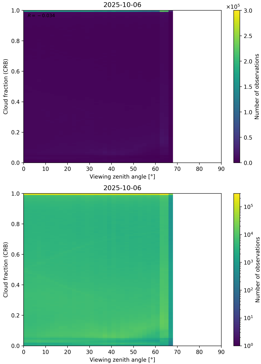
Figure 109: Scatter density plot of “Viewing zenith angle” against “Cloud fraction (CRB)” for 2025-10-06 to 2025-10-07.
