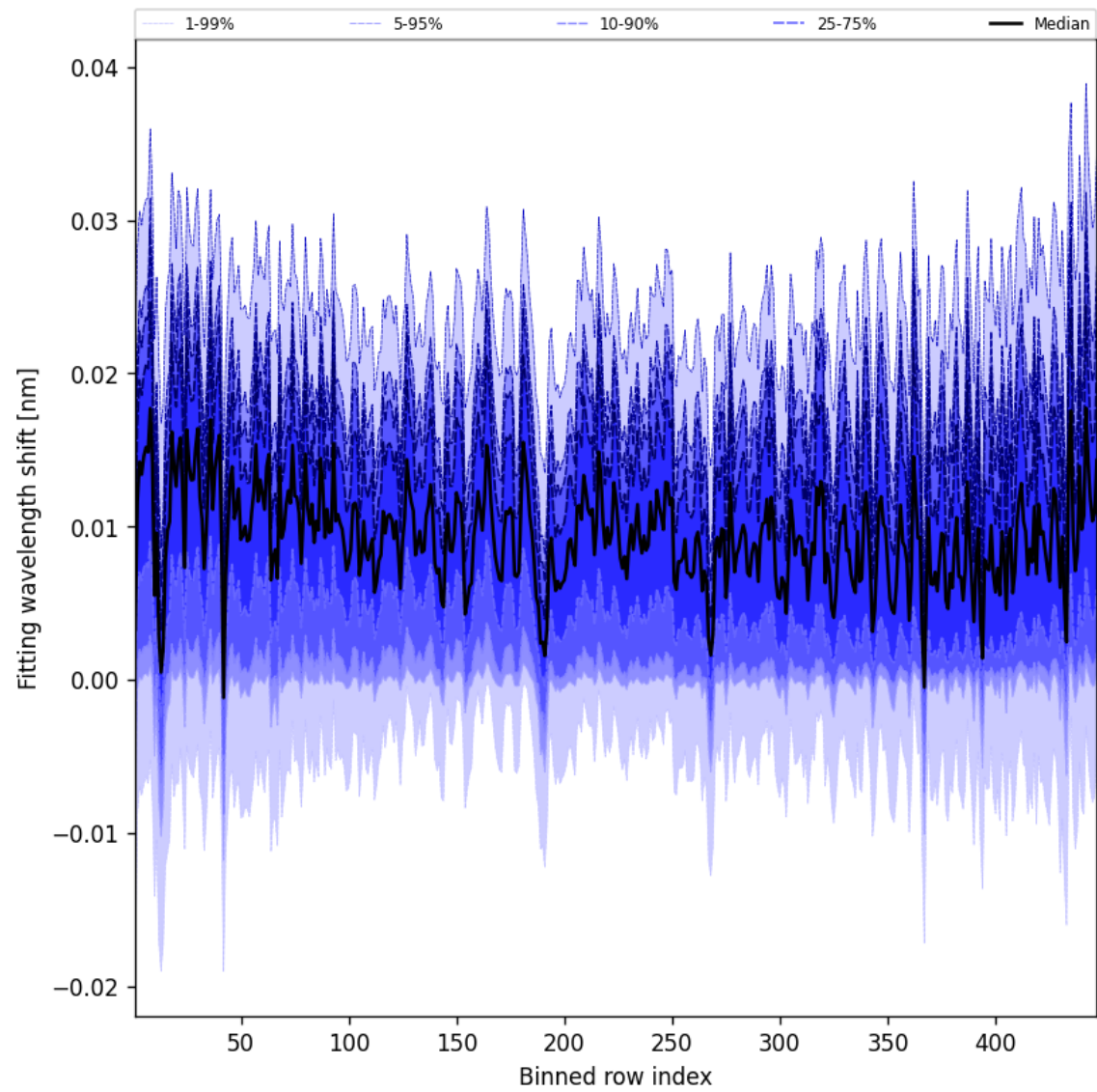
Figure 65: Along track statistics of “Fitting wavelength shift” for 2025-10-06 to 2025-10-07
