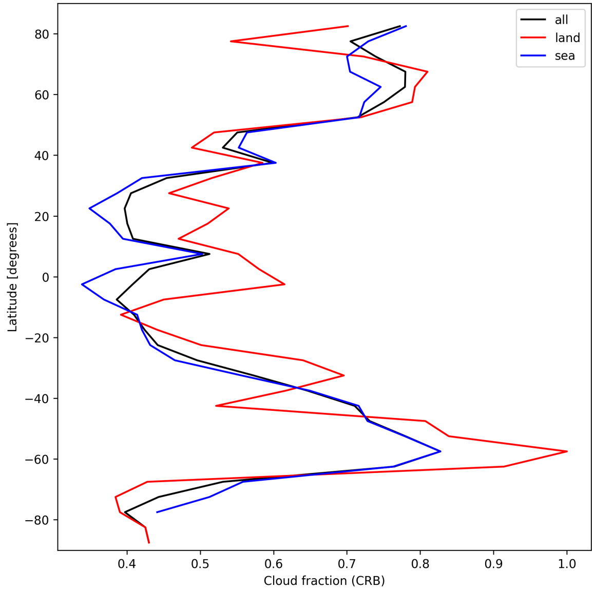
Figure 26: Zonal average of “Cloud fraction (CRB)” for 2025-10-06 to 2025-10-07.
