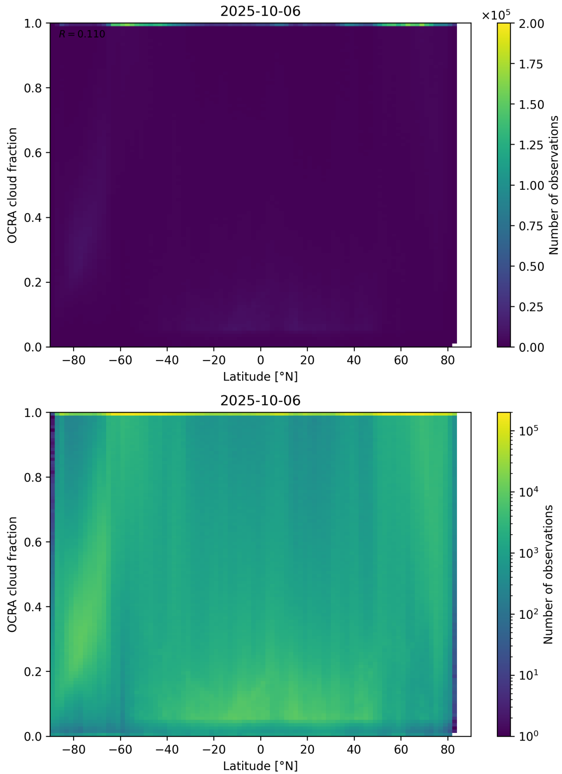
Figure 93: Scatter density plot of “Latitude” against “OCRA cloud fraction” for 2025-10-06 to 2025-10-07.
