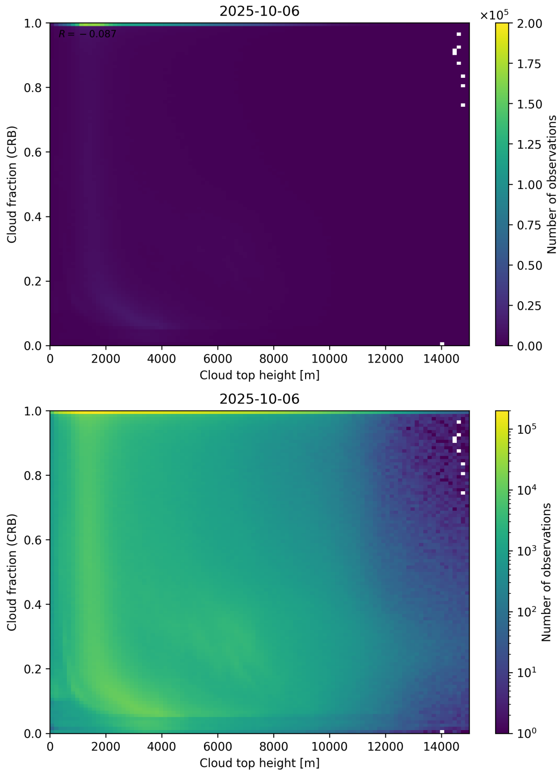
Figure 88: Scatter density plot of “Cloud top height” against “Cloud fraction (CRB)” for 2025-10-06 to 2025-10-07.
