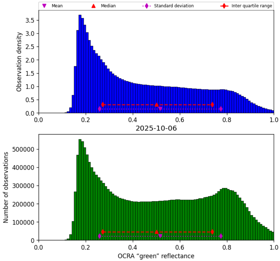
Figure 52: Histogram of “OCRA “green” reflectance” for 2025-10-06 to 2025-10-07
