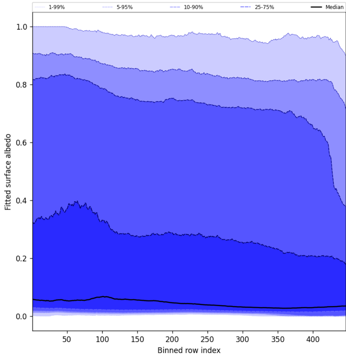
Figure 61: Along track statistics of “Fitted surface albedo” for 2025-10-06 to 2025-10-07
