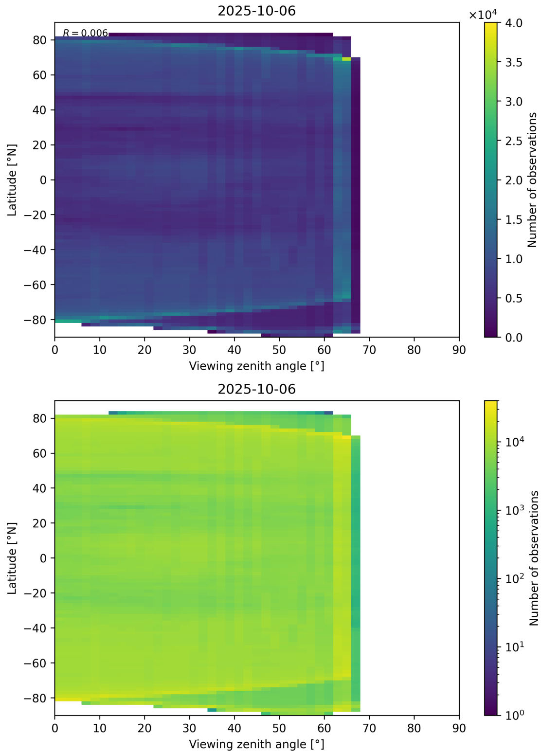
Figure 113: Scatter density plot of “Viewing zenith angle” against “Latitude” for 2025-10-06 to 2025-10-07.
