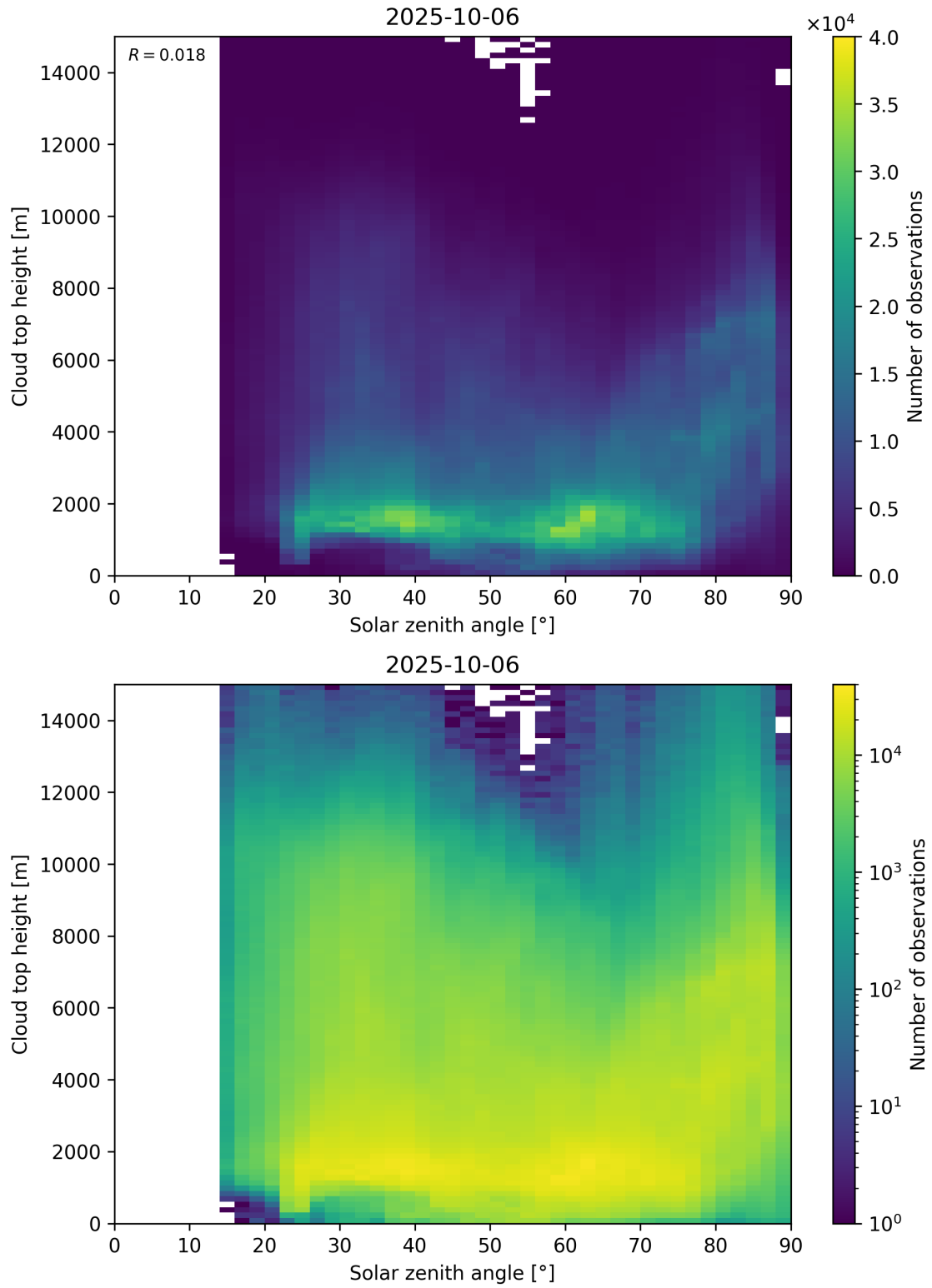
Figure 104: Scatter density plot of “Solar zenith angle” against “Cloud top height” for 2025-10-06 to 2025-10-07.
