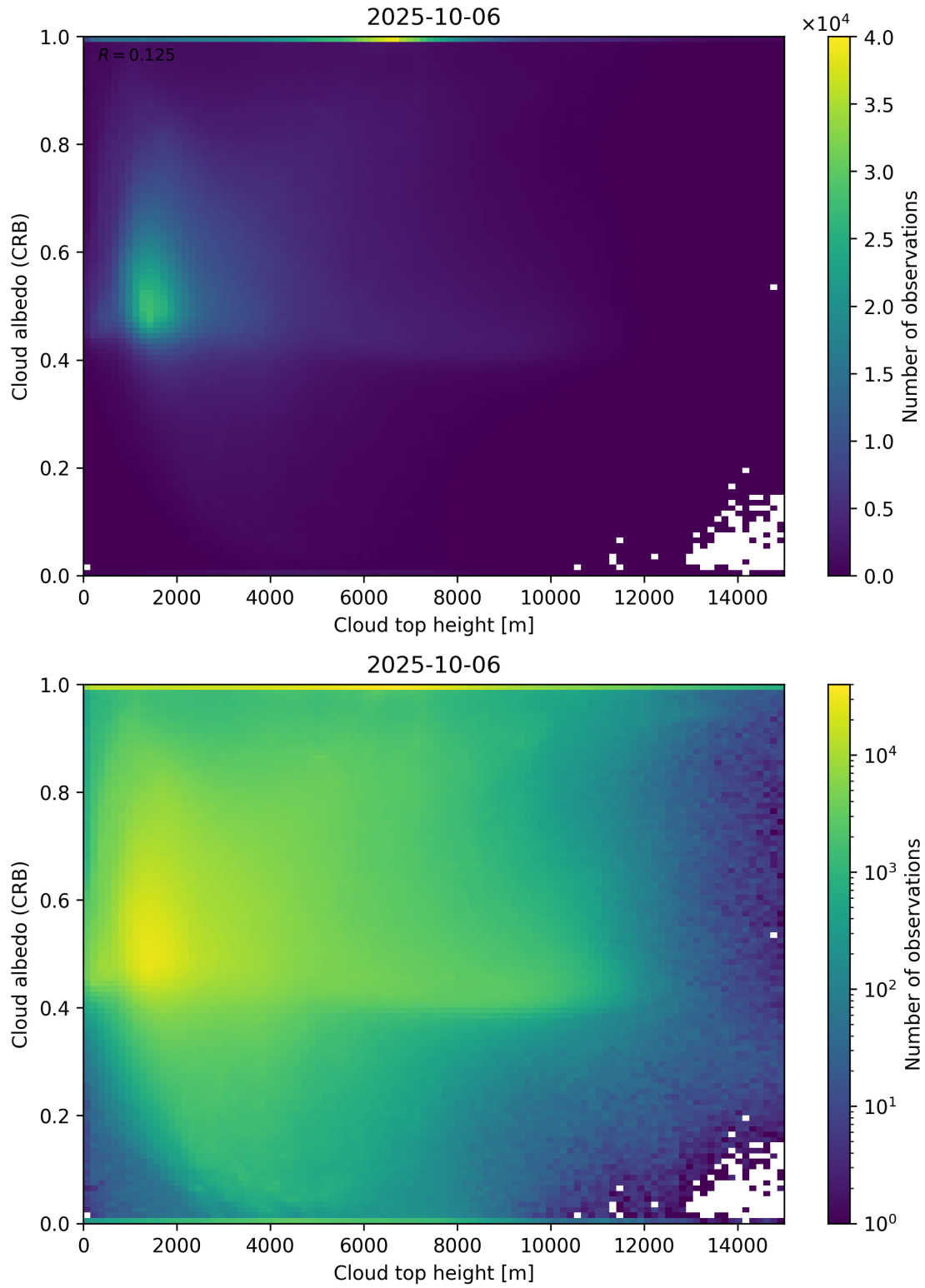
Figure 86: Scatter density plot of “Cloud top height” against “Cloud albedo (CRB)” for 2025-10-06 to 2025-10-07.
