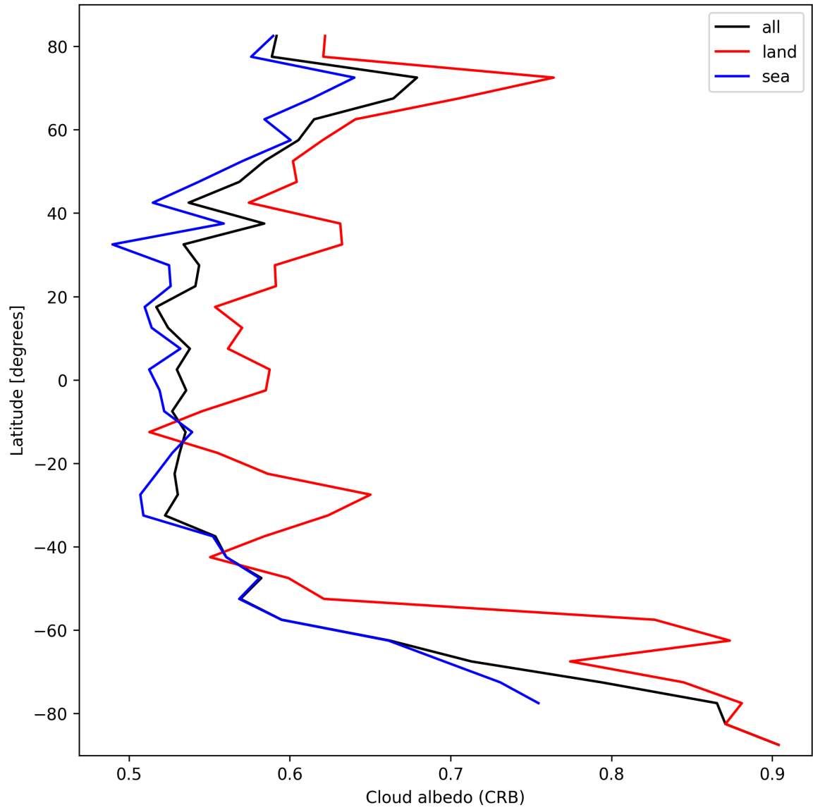
Figure 28: Zonal average of “Cloud albedo (CRB)” for 2025-10-06 to 2025-10-07.
