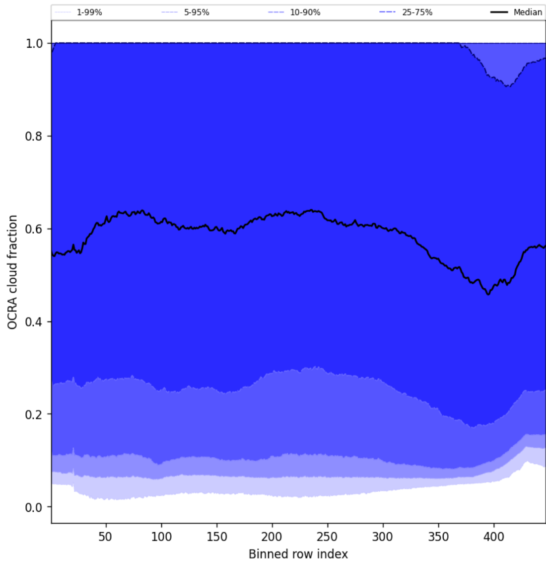
Figure 66: Along track statistics of “OCRA cloud fraction” for 2025-10-06 to 2025-10-07
