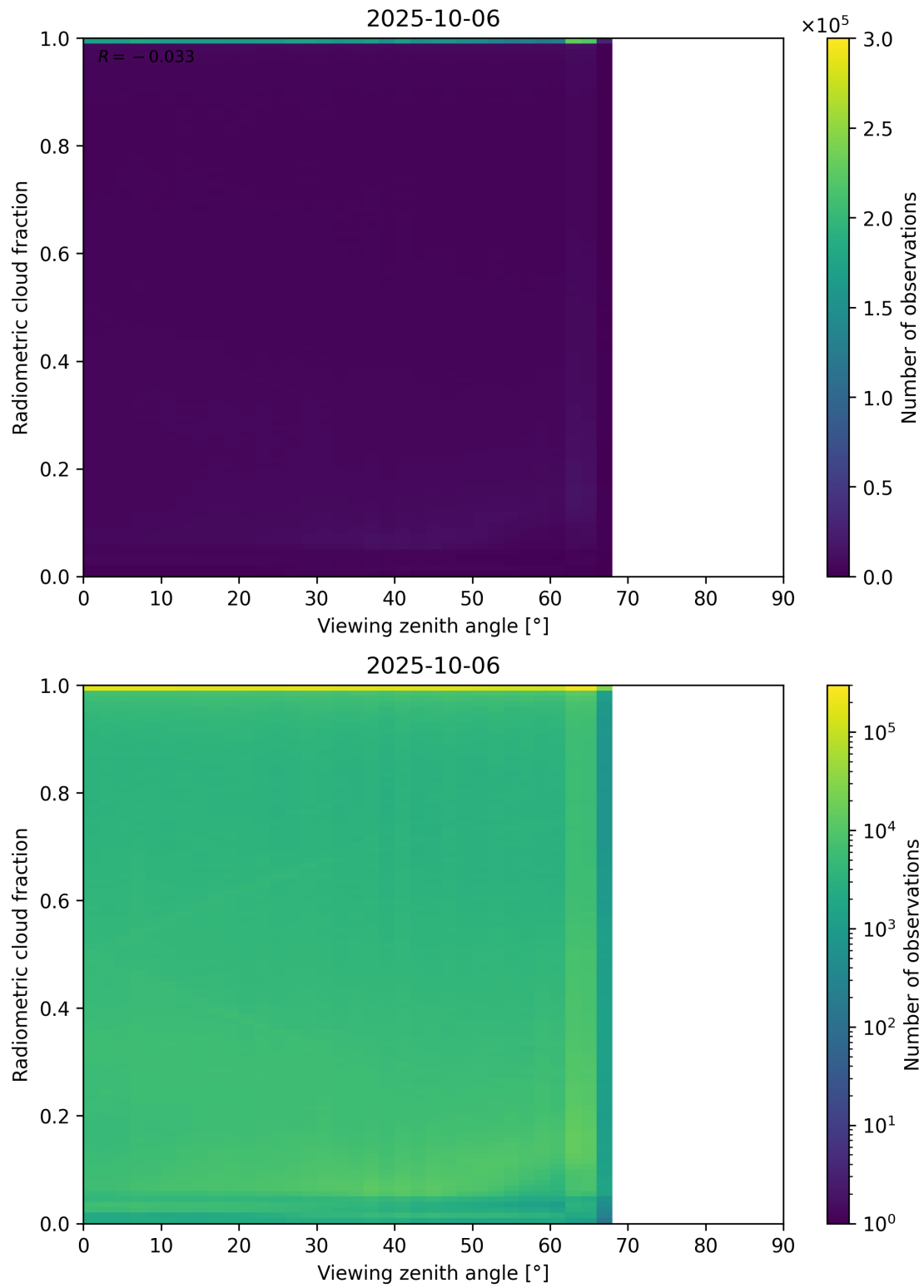
Figure 107: Scatter density plot of “Viewing zenith angle” against “Radiometric cloud fraction” for 2025-10-06 to 2025-10-07.
