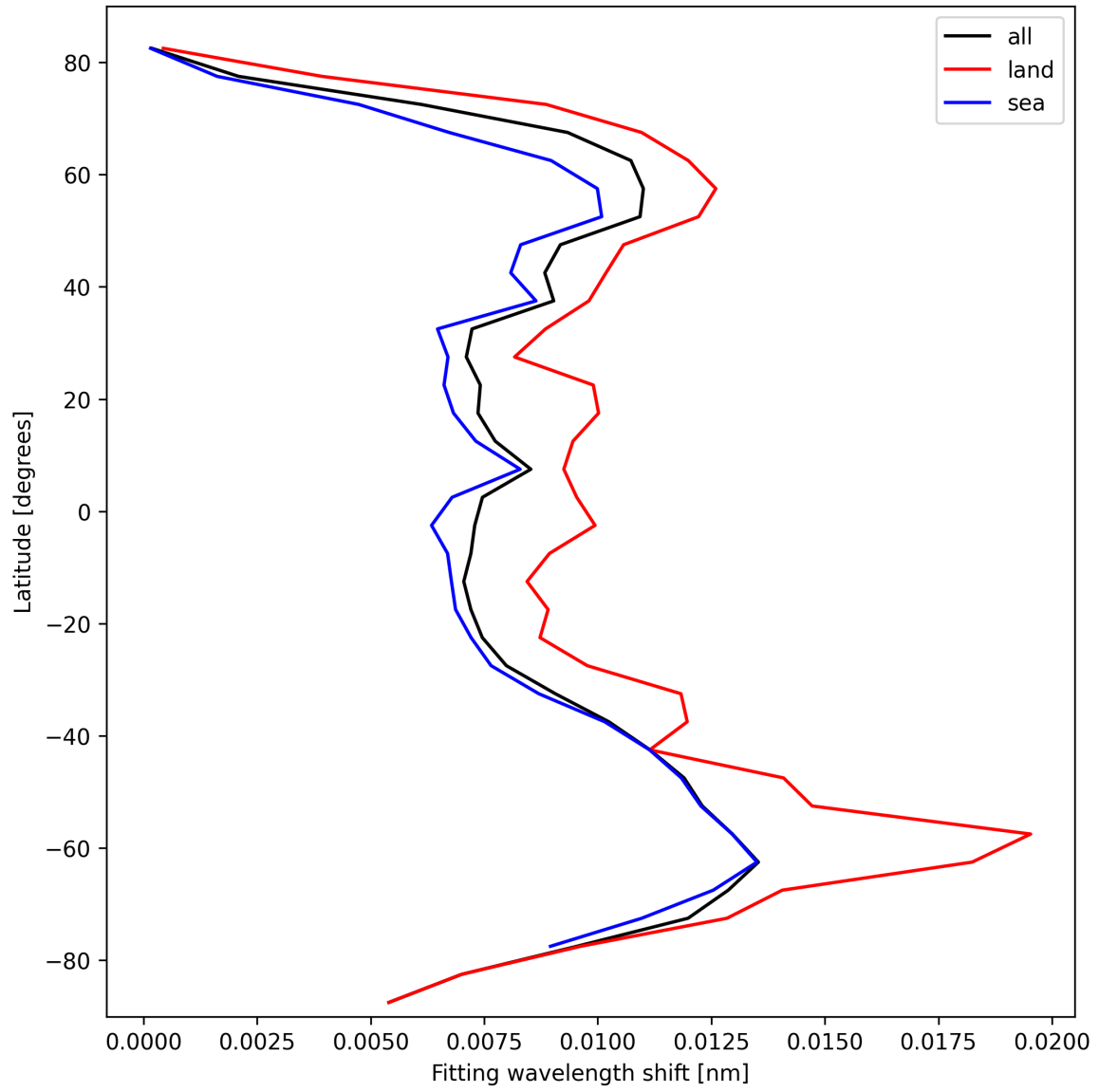
Figure 33: Zonal average of “Fitting wavelength shift” for 2025-10-06 to 2025-10-07.
