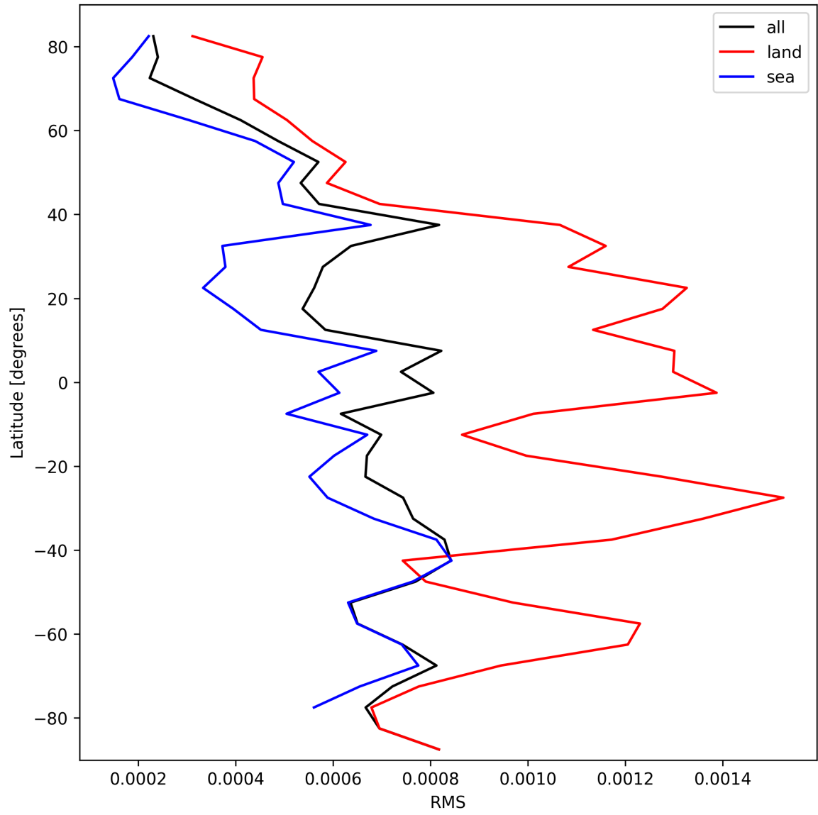
Figure 31: Zonal average of “RMS” for 2025-10-06 to 2025-10-07.
