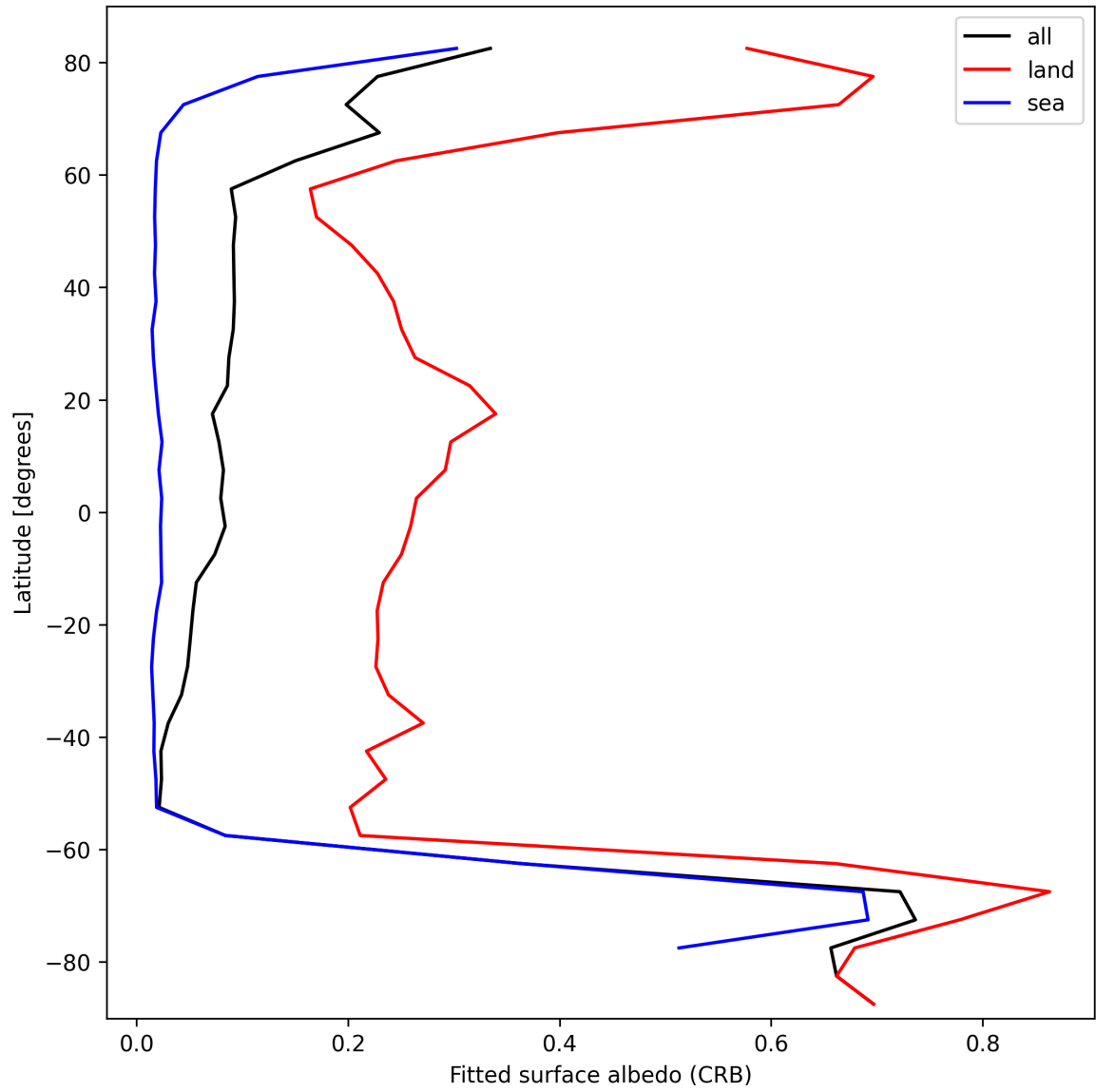
Figure 30: Zonal average of “Fitted surface albedo (CRB)” for 2025-10-06 to 2025-10-07.
