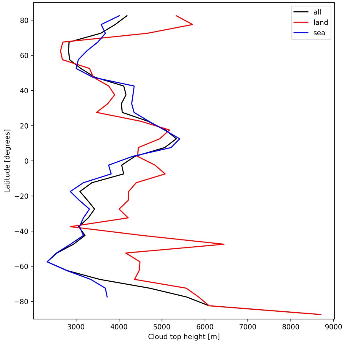
Figure 24: Zonal average of “Cloud top height” for 2025-10-06 to 2025-10-07.
