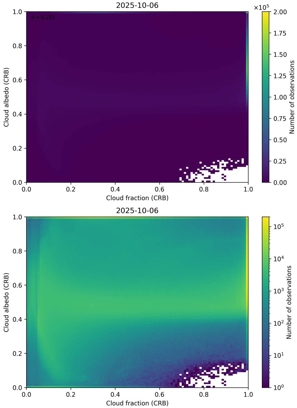
Figure 77: Scatter density plot of “Cloud fraction (CRB)” against “Cloud albedo (CRB)” for 2025-10-06 to 2025-10-07.
