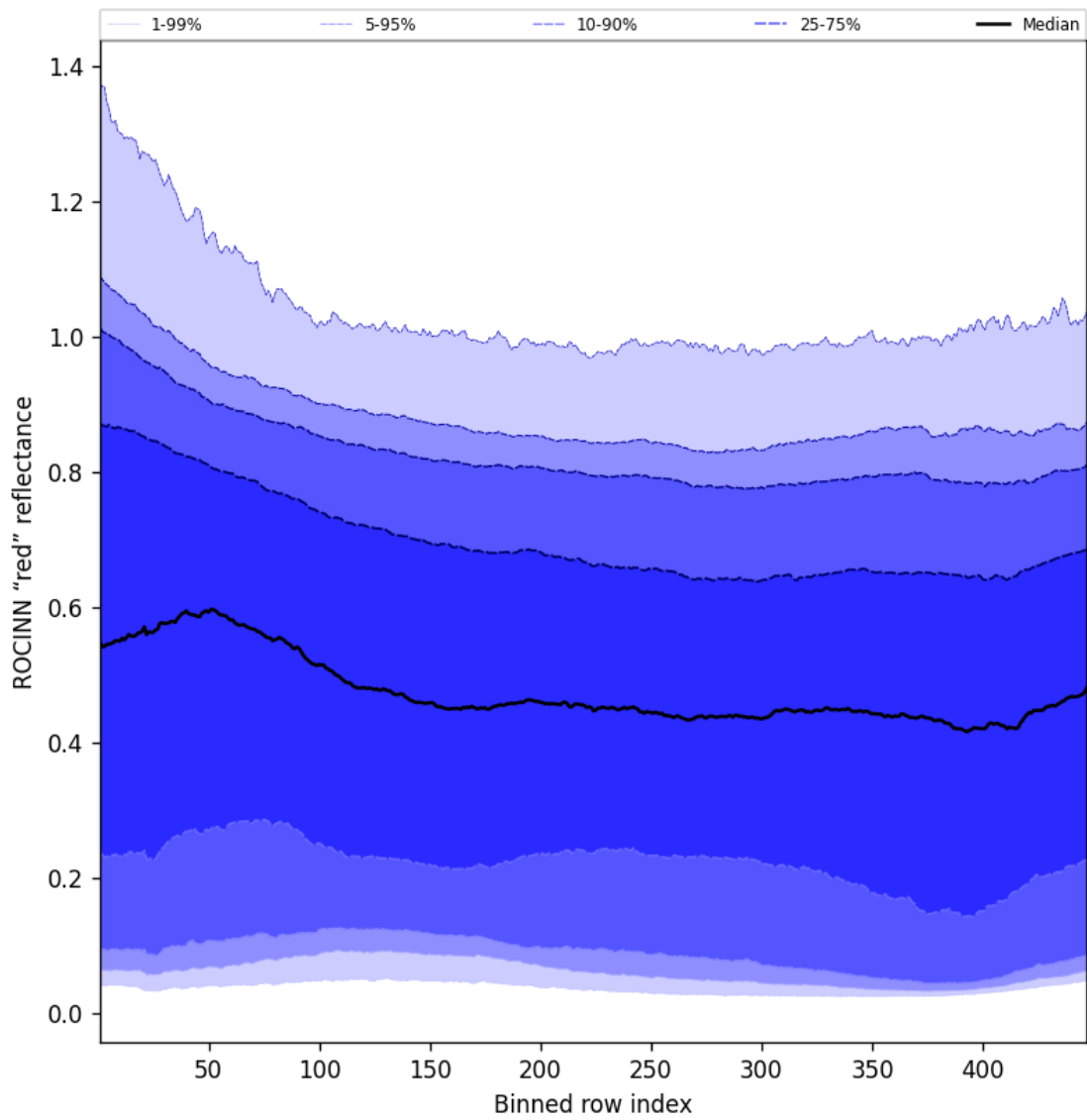
Figure 69: Along track statistics of “ROCINN “red” reflectance” for 2025-10-06 to 2025-10-07
