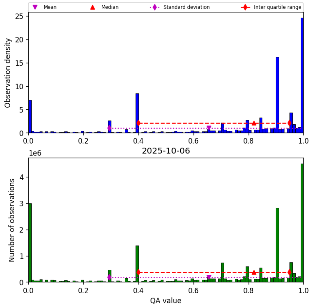
Figure 38: Histogram of “QA value” for 2025-10-06 to 2025-10-07
