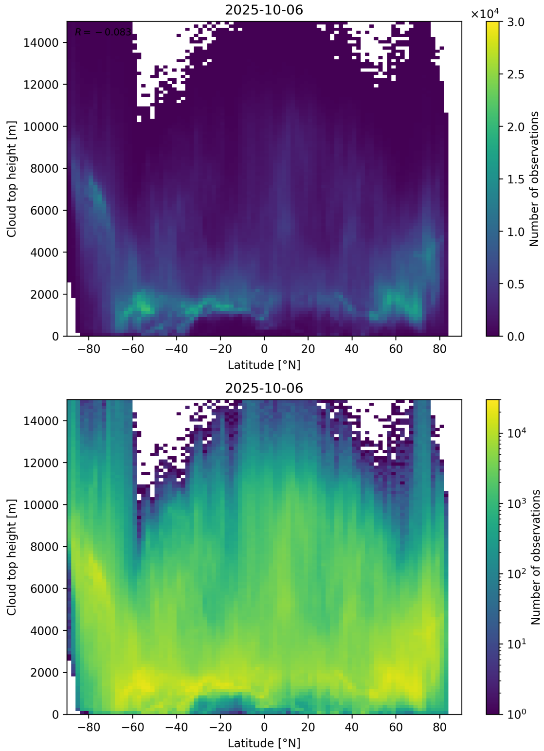
Figure 97: Scatter density plot of “Latitude” against “Cloud top height” for 2025-10-06 to 2025-10-07.
