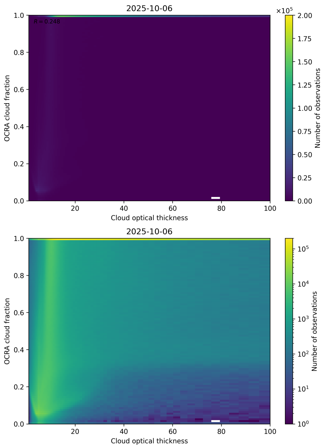
Figure 83: Scatter density plot of “Cloud optical thickness” against “OCRA cloud fraction” for 2025-10-06 to 2025-10-07.
