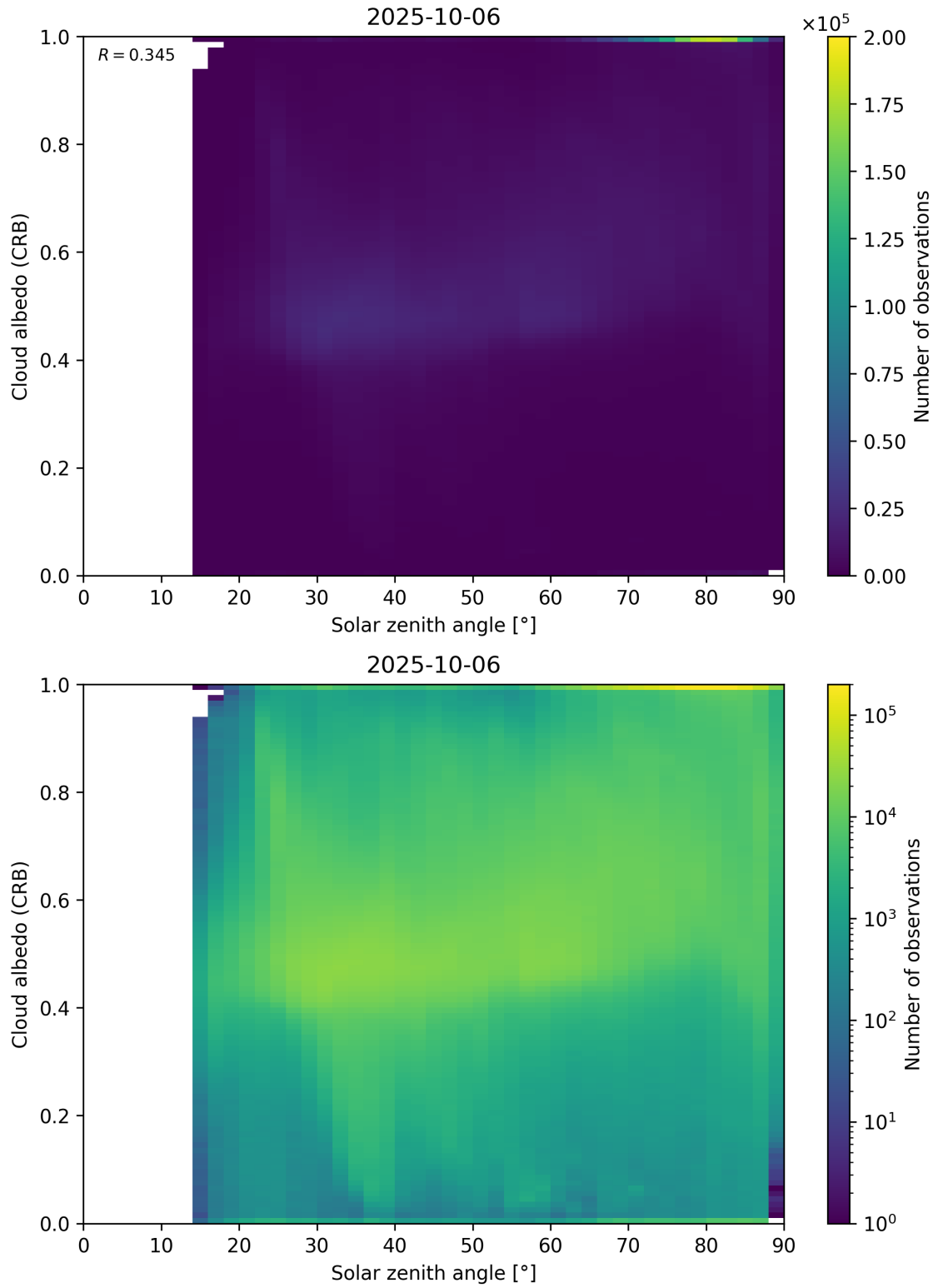
Figure 98: Scatter density plot of “Solar zenith angle” against “Cloud albedo (CRB)” for 2025-10-06 to 2025-10-07.
