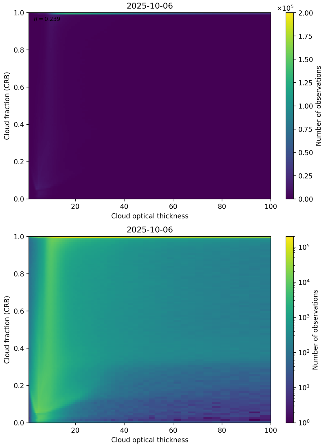
Figure 84: Scatter density plot of “Cloud optical thickness” against “Cloud fraction (CRB)” for 2025-10-06 to 2025-10-07.
