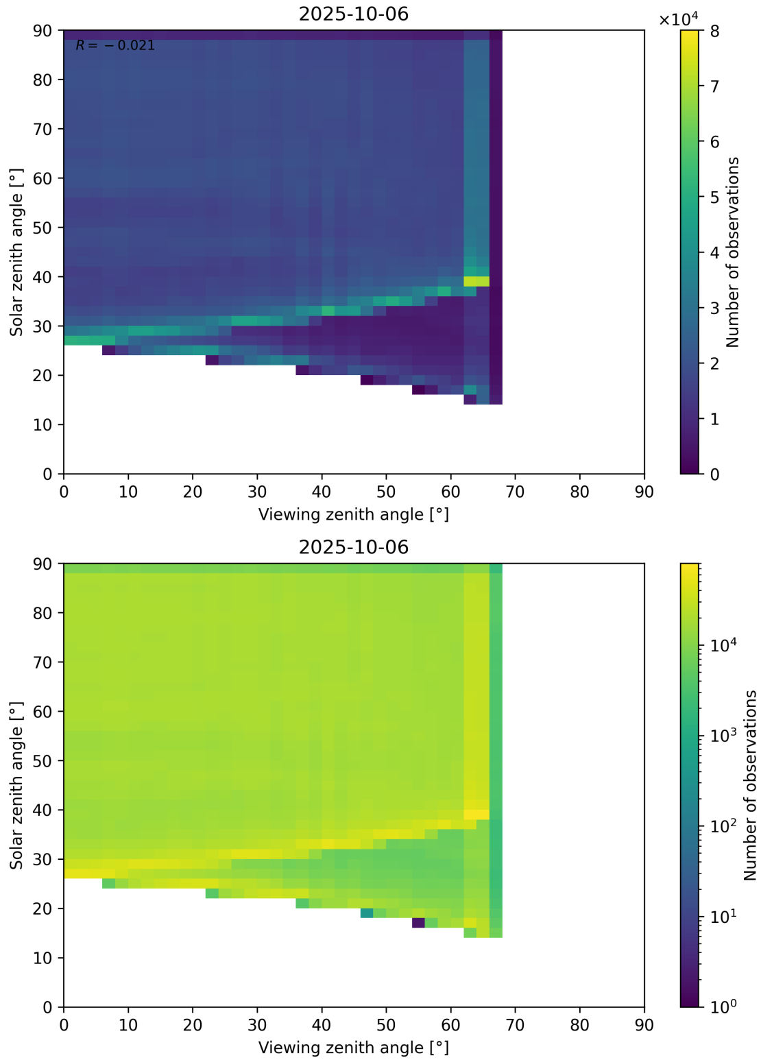
Figure 114: Scatter density plot of “Viewing zenith angle” against “Solar zenith angle” for 2025-10-06 to 2025-10-07.
