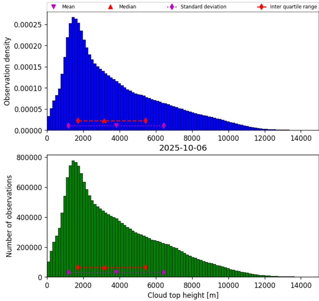
Figure 40: Histogram of “Cloud top height” for 2025-10-06 to 2025-10-07
