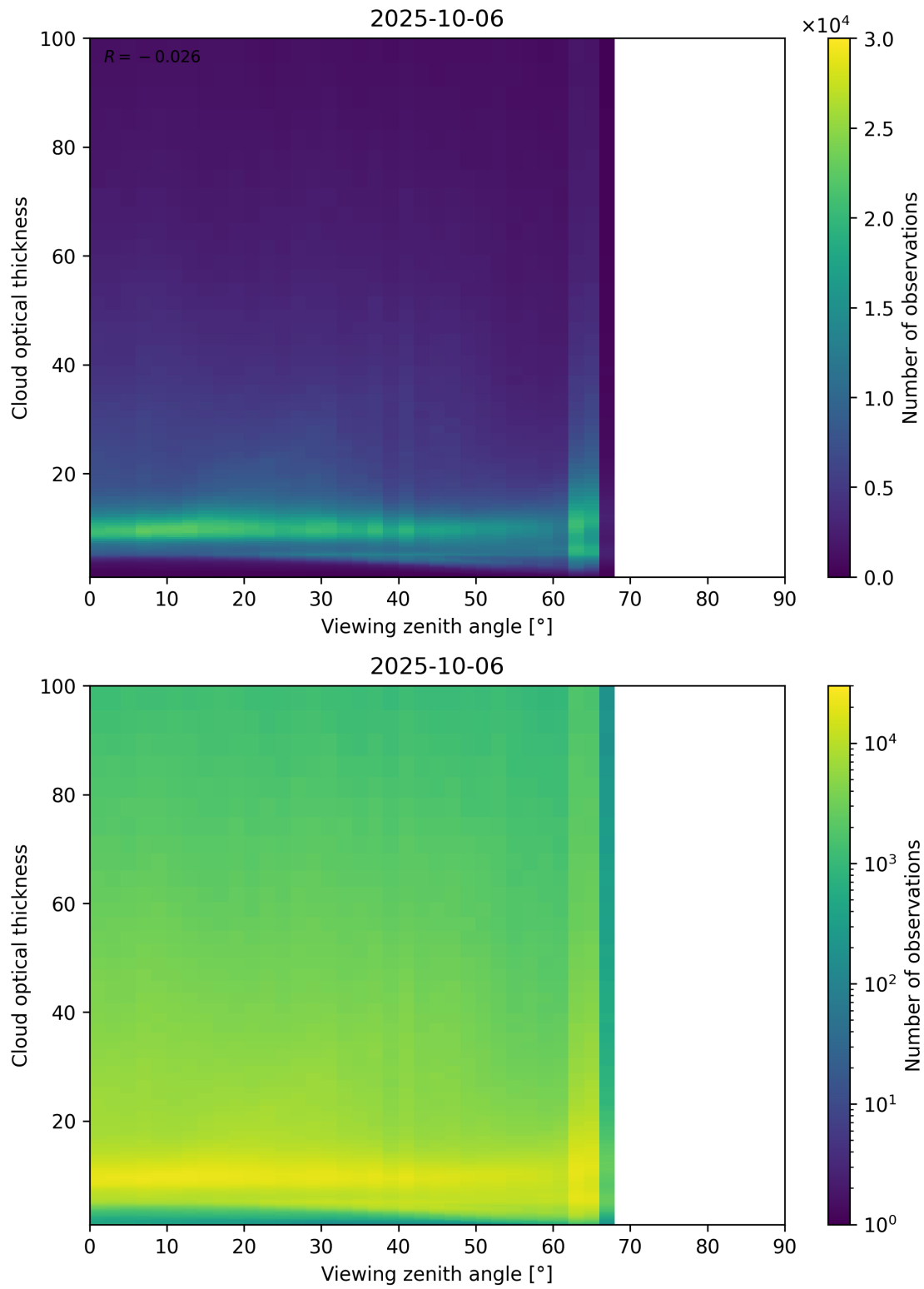
Figure 111: Scatter density plot of “Viewing zenith angle” against “Cloud optical thickness” for 2025-10-06 to 2025-10-07.
