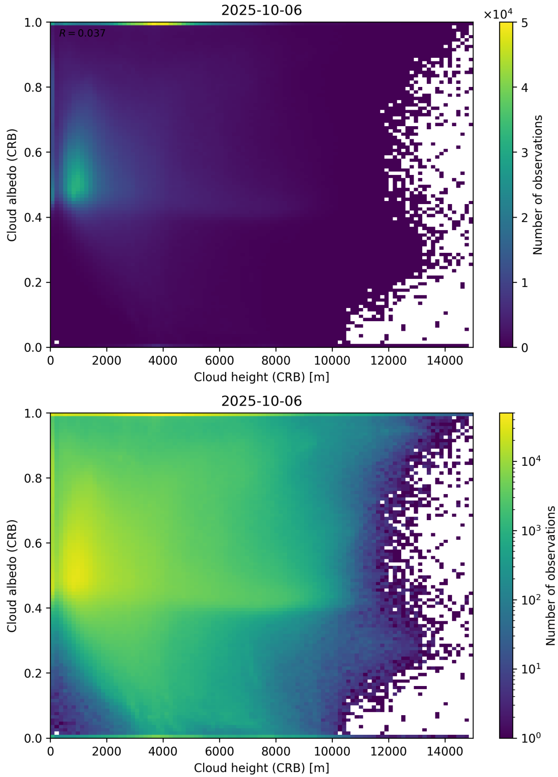
Figure 80: Scatter density plot of “Cloud height (CRB)” against “Cloud albedo (CRB)” for 2025-10-06 to 2025-10-07.
