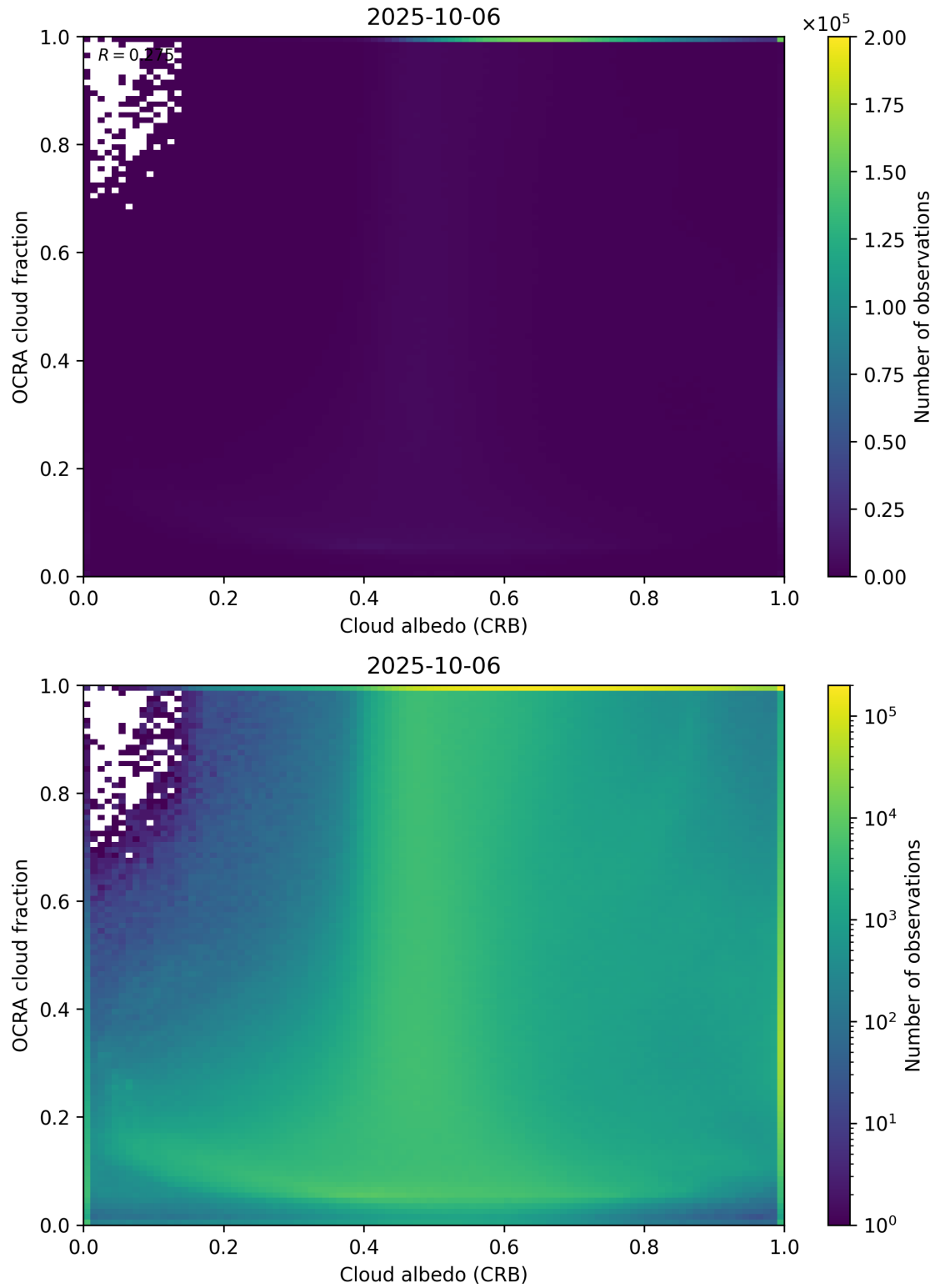
Figure 70: Scatter density plot of “Cloud albedo (CRB)” against “OCRA cloud fraction” for 2025-10-06 to 2025-10-07.
