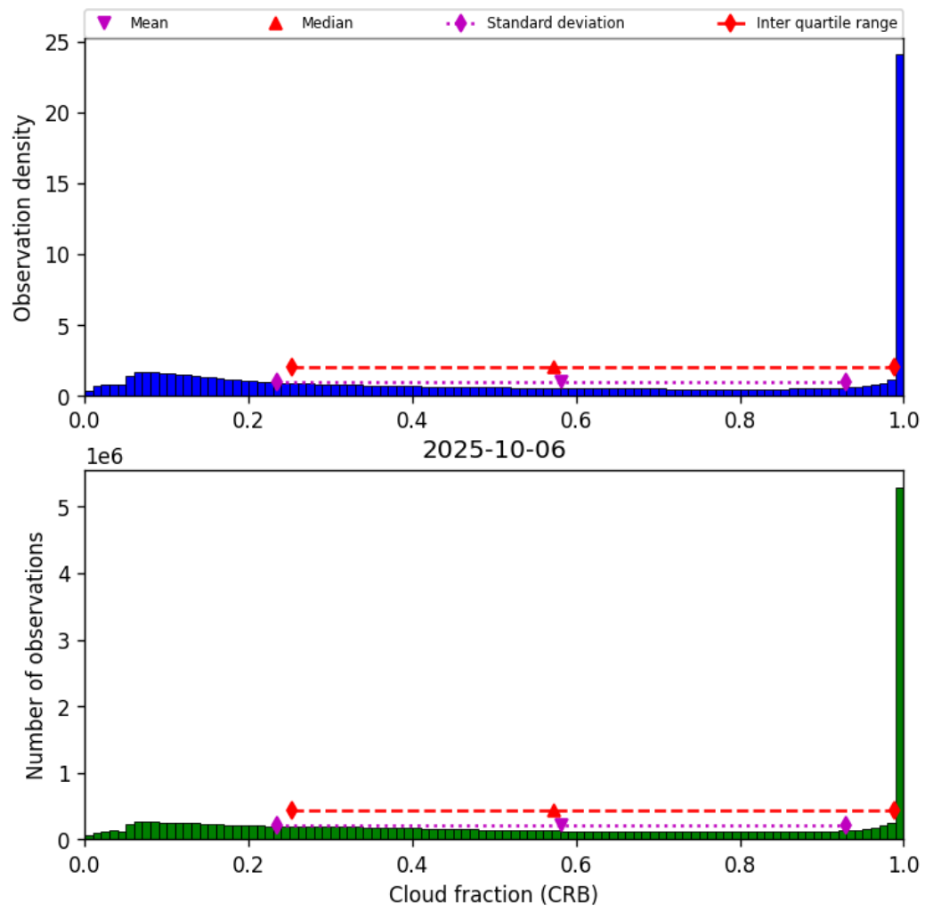
Figure 42: Histogram of “Cloud fraction (CRB)” for 2025-10-06 to 2025-10-07
