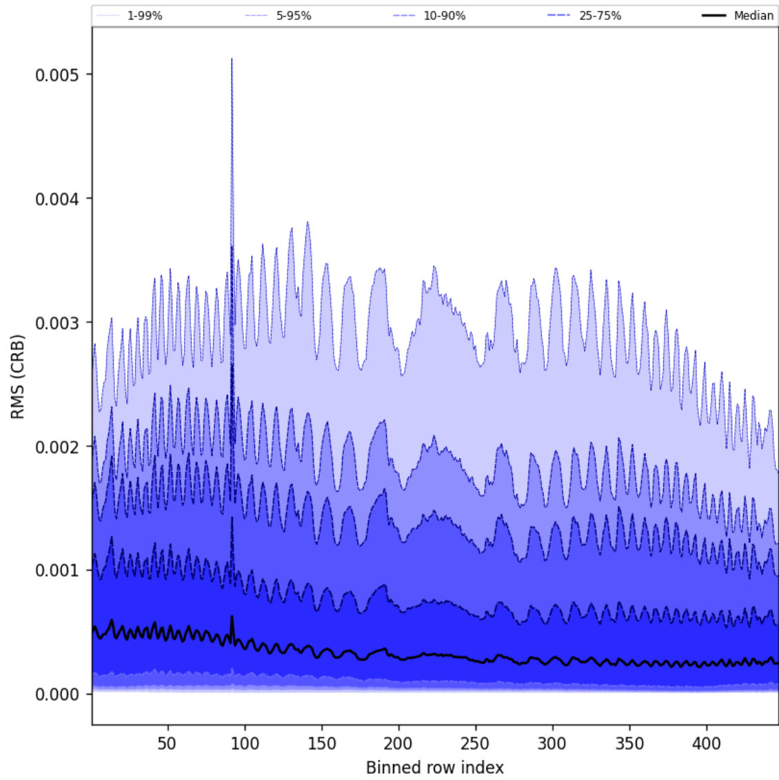
Figure 64: Along track statistics of “RMS (CRB)” for 2025-10-06 to 2025-10-07
