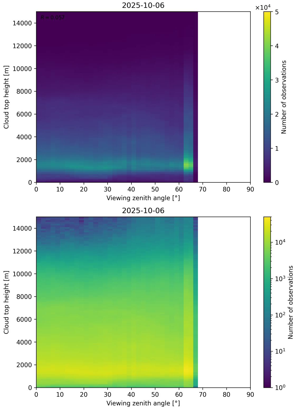
Figure 112: Scatter density plot of “Viewing zenith angle” against “Cloud top height” for 2025-10-06 to 2025-10-07.
