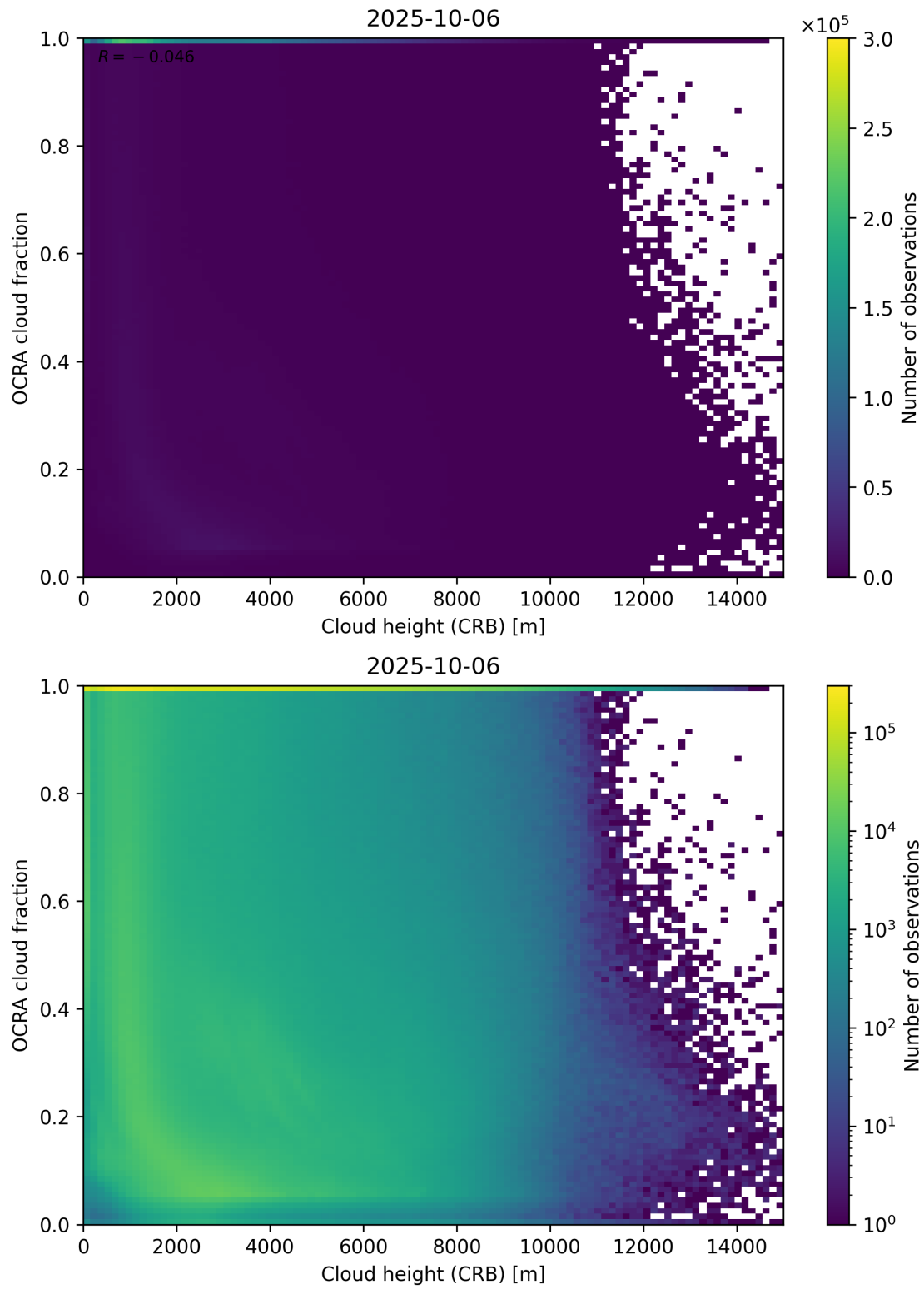
Figure 81: Scatter density plot of “Cloud height (CRB)” against “OCRA cloud fraction” for 2025-10-06 to 2025-10-07.
