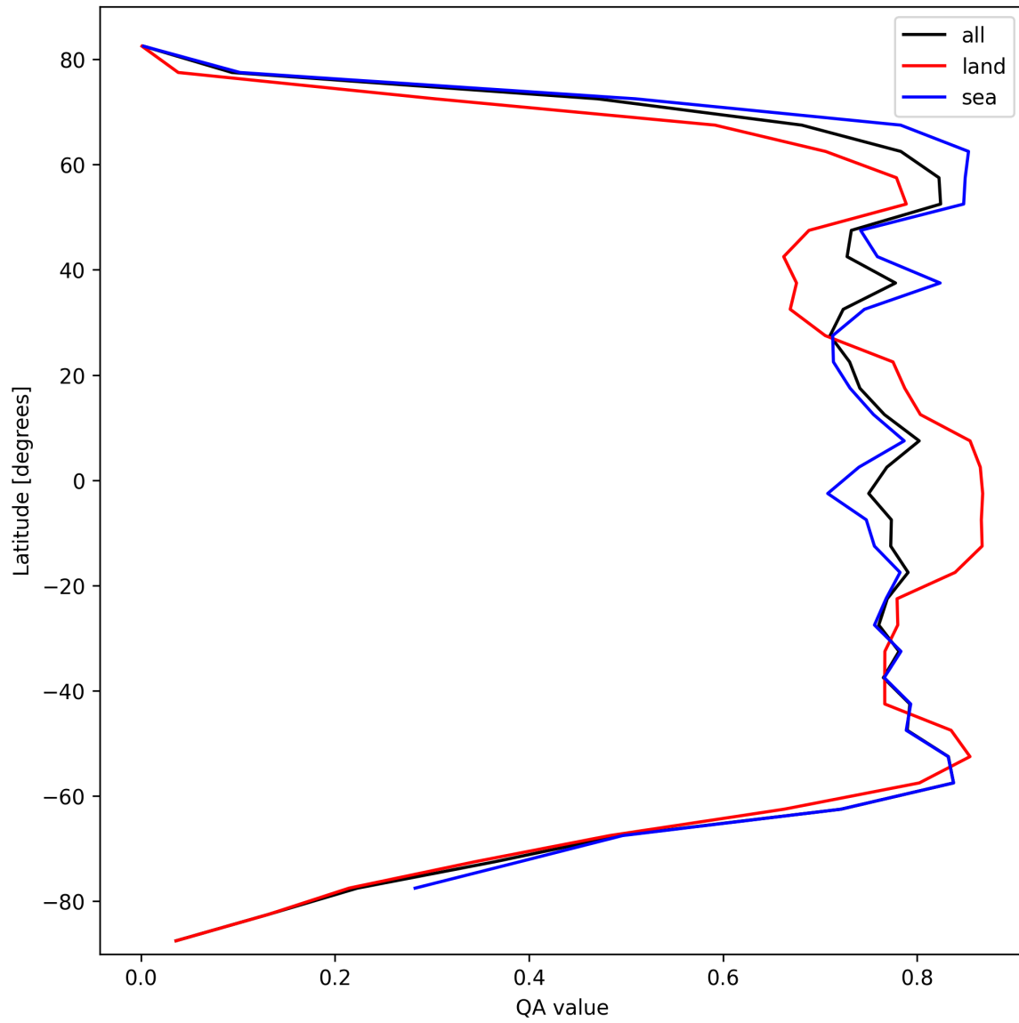
Figure 22: Zonal average of “QA value” for 2025-10-06 to 2025-10-07.
