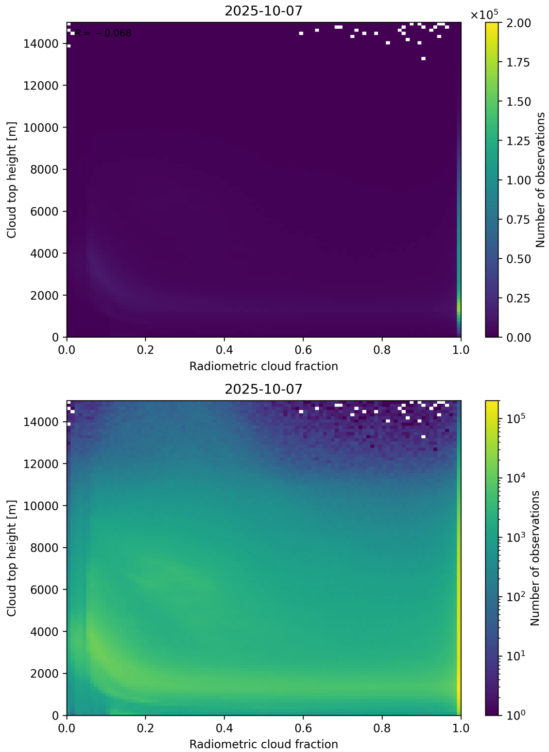
Figure 76: Scatter density plot of “Radiometric cloud fraction” against “Cloud top height” for 2025-10-06 to 2025-10-08.
