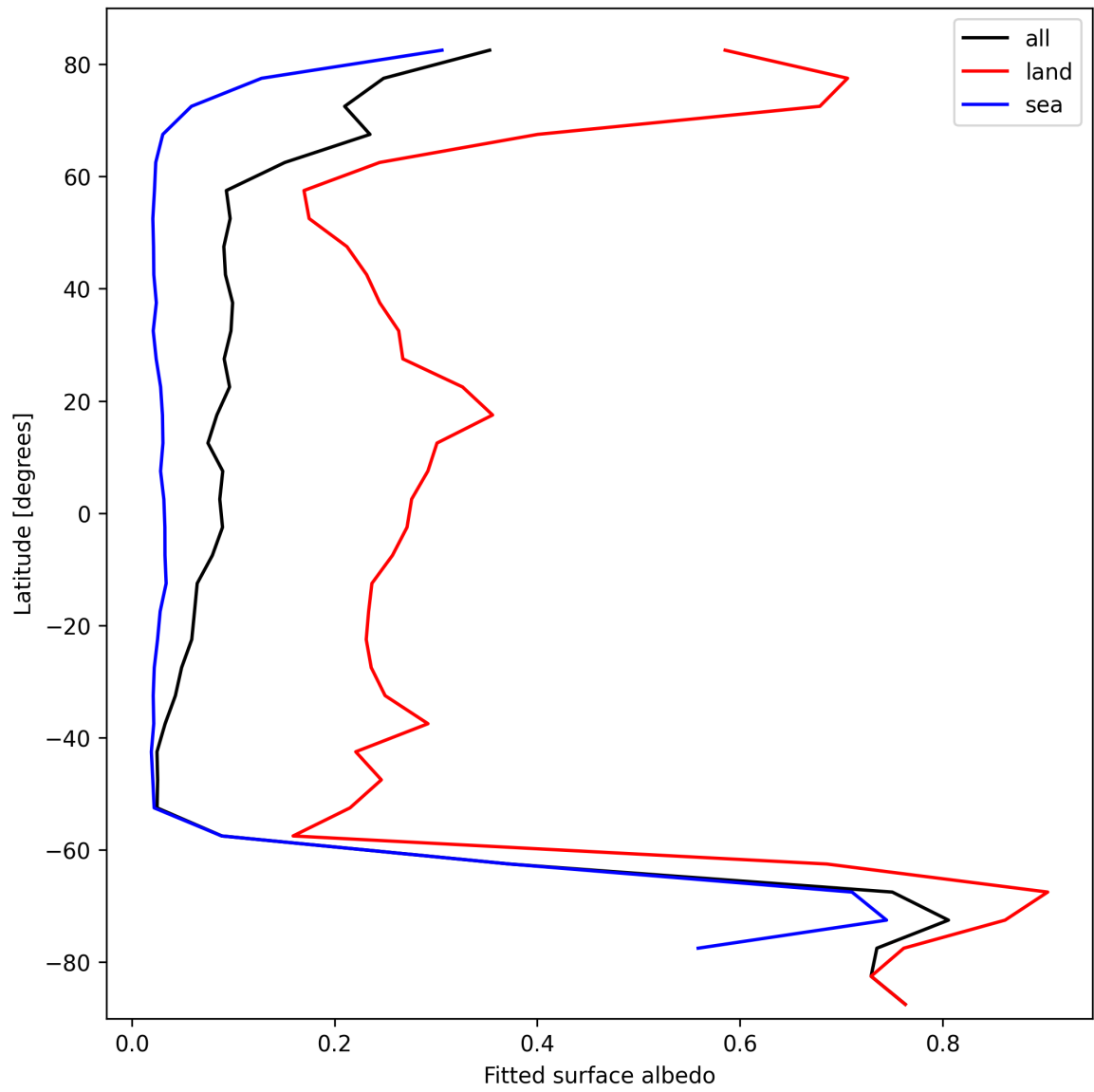
Figure 29: Zonal average of “Fitted surface albedo” for 2025-10-06 to 2025-10-08.
