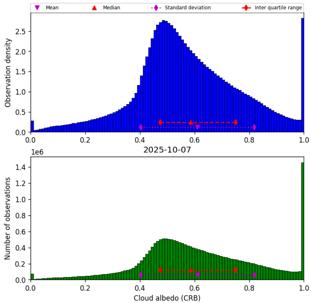
Figure 44: Histogram of “Cloud albedo (CRB)” for 2025-10-06 to 2025-10-08
