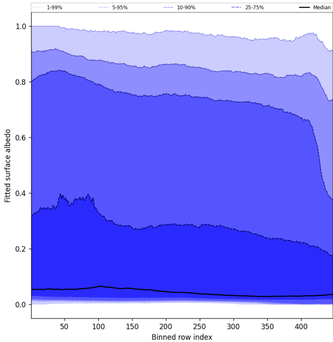
Figure 61: Along track statistics of “Fitted surface albedo” for 2025-10-06 to 2025-10-08
