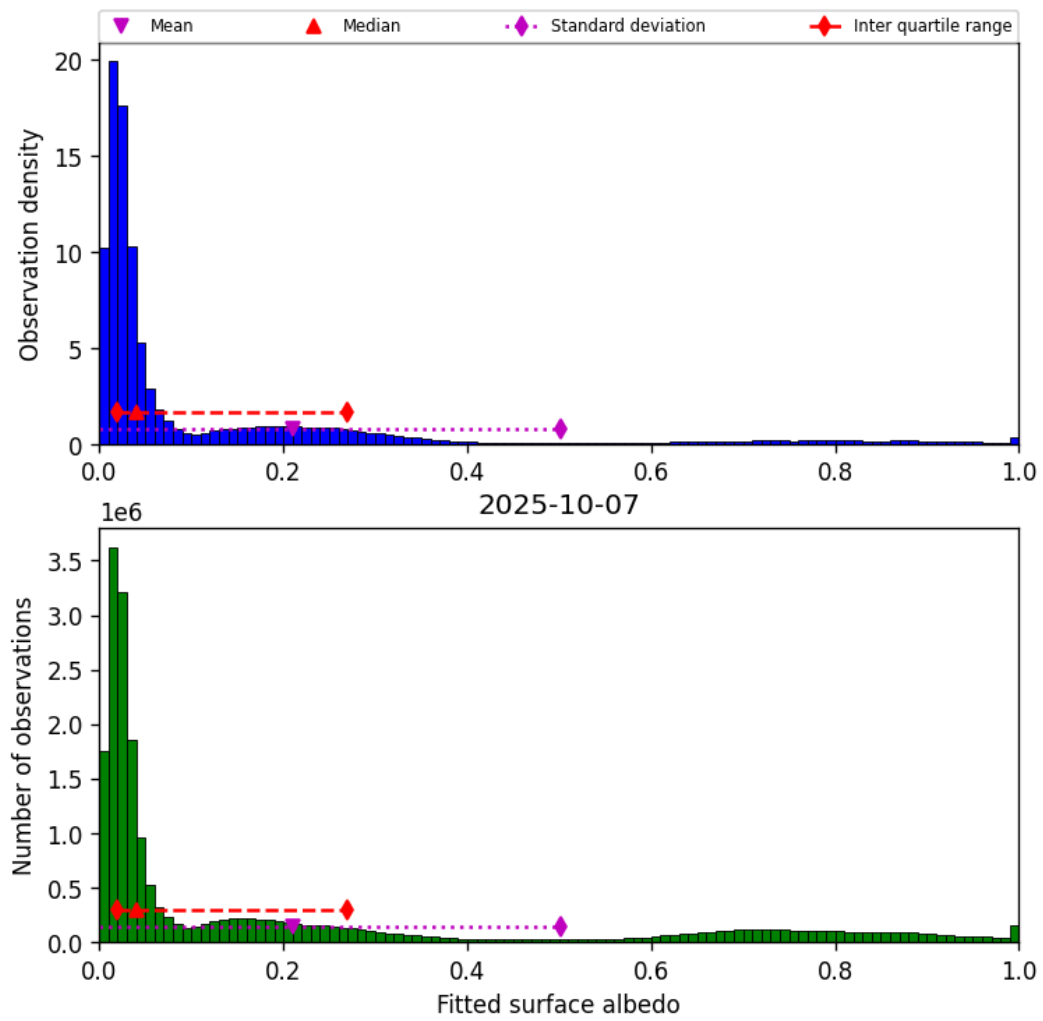
Figure 45: Histogram of “Fitted surface albedo” for 2025-10-06 to 2025-10-08
