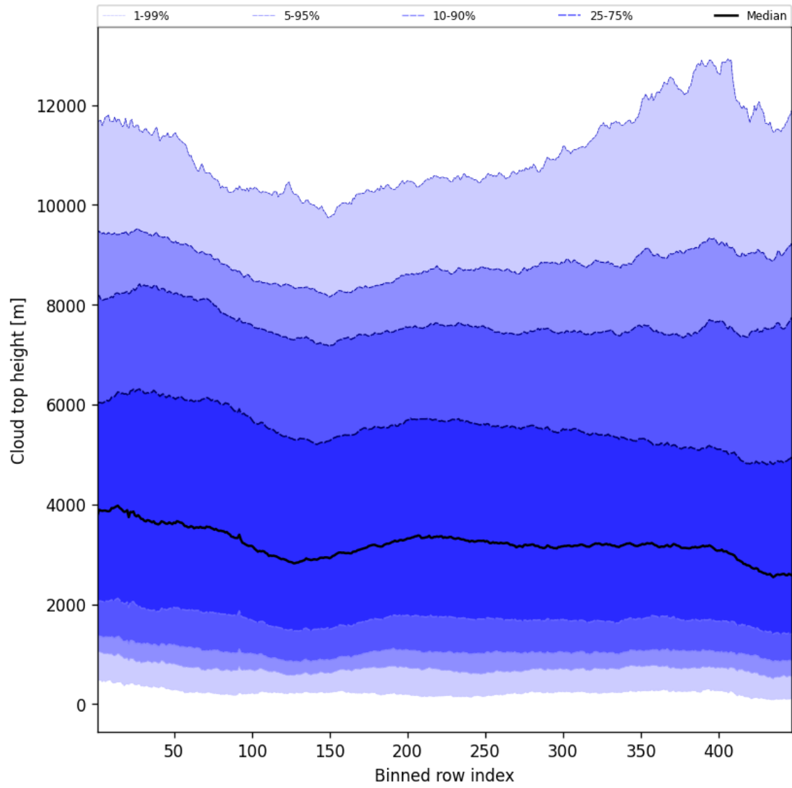
Figure 56: Along track statistics of “Cloud top height” for 2025-10-06 to 2025-10-08
