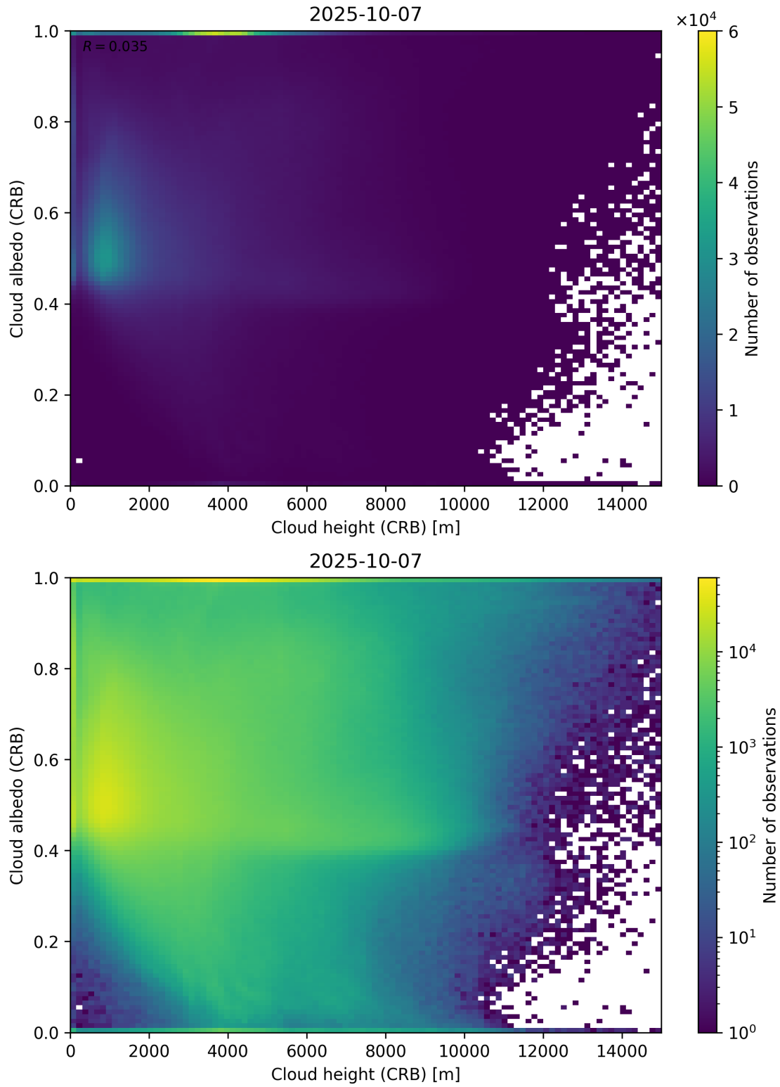
Figure 80: Scatter density plot of “Cloud height (CRB)” against “Cloud albedo (CRB)” for 2025-10-06 to 2025-10-08.
