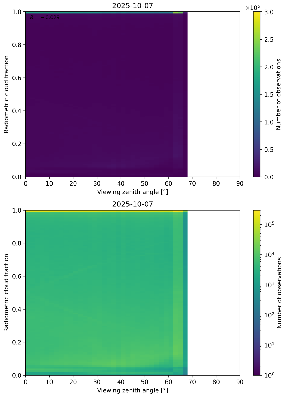
Figure 107: Scatter density plot of “Viewing zenith angle” against “Radiometric cloud fraction” for 2025-10-06 to 2025-10-08.
