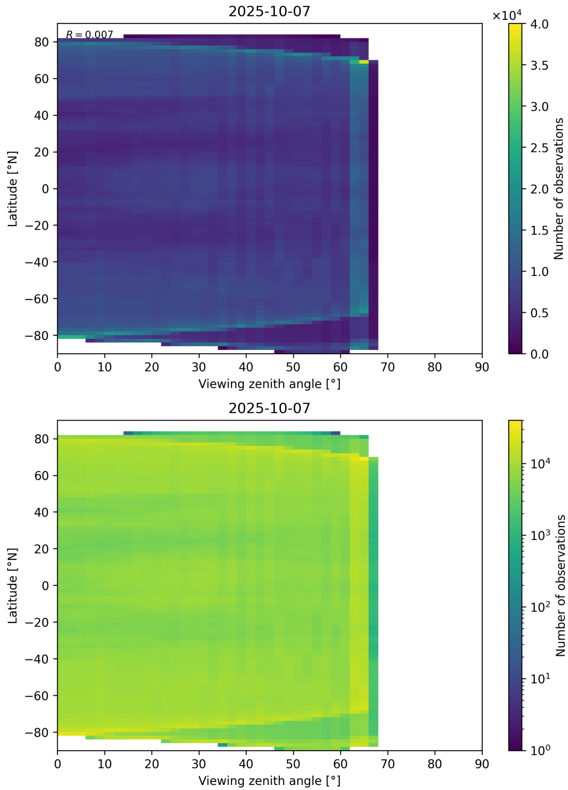
Figure 113: Scatter density plot of “Viewing zenith angle” against “Latitude” for 2025-10-06 to 2025-10-08.
