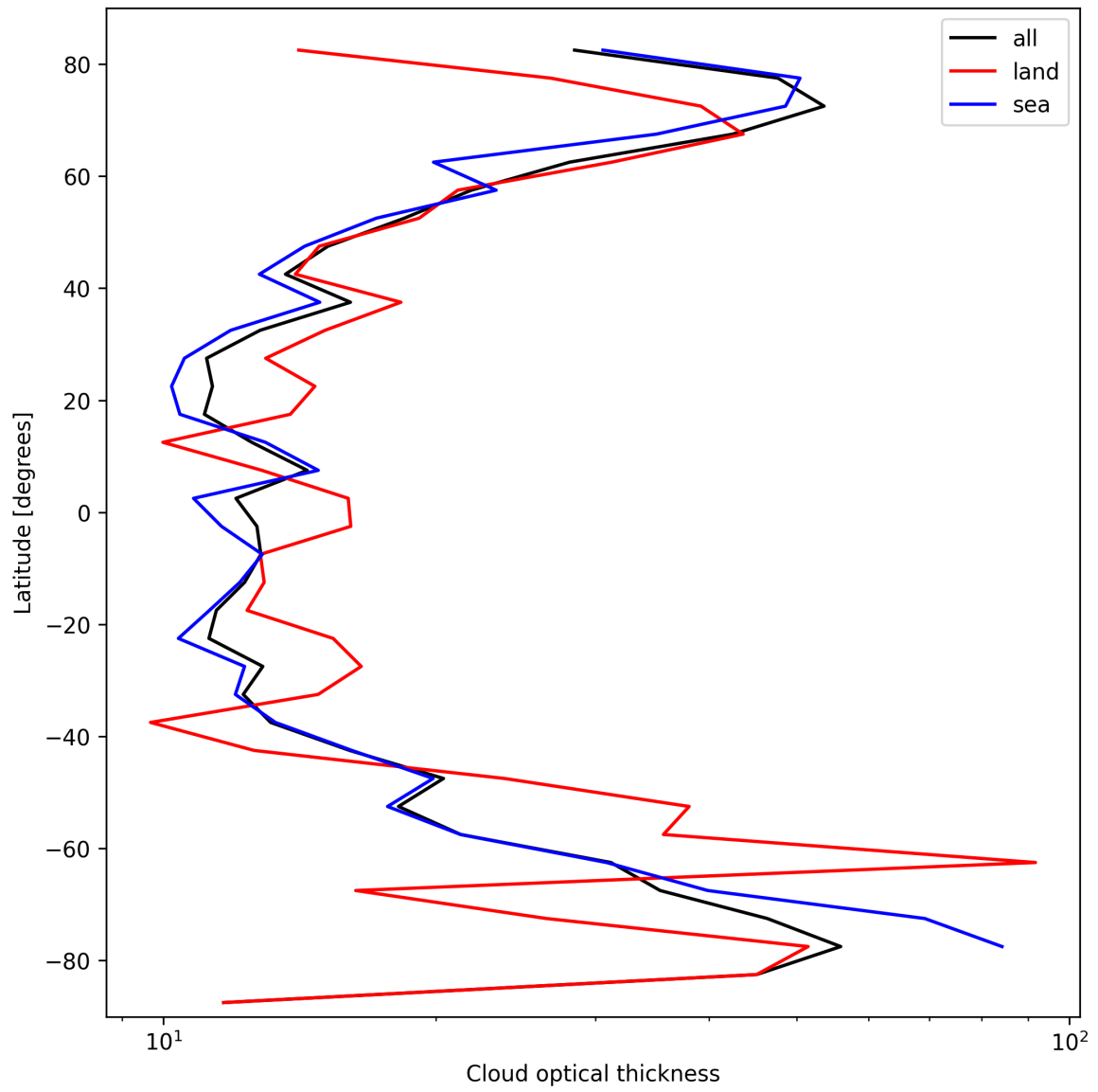
Figure 25: Zonal average of “Cloud optical thickness” for 2025-10-06 to 2025-10-08.
