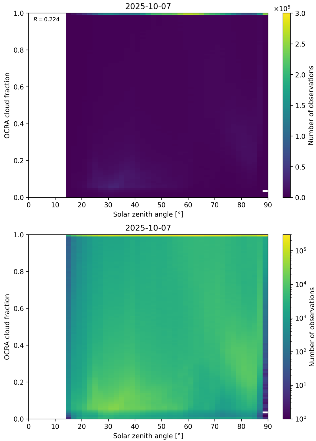
Figure 100: Scatter density plot of “Solar zenith angle” against “OCRA cloud fraction” for 2025-10-06 to 2025-10-08.
