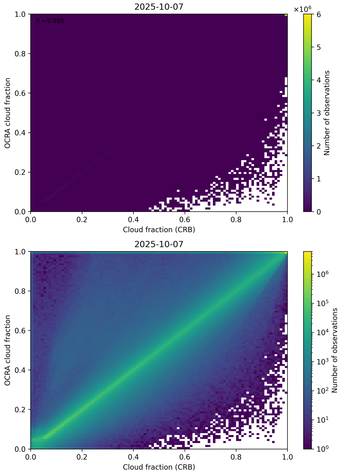
Figure 78: Scatter density plot of “Cloud fraction (CRB)” against “OCRA cloud fraction” for 2025-10-06 to 2025-10-08.
