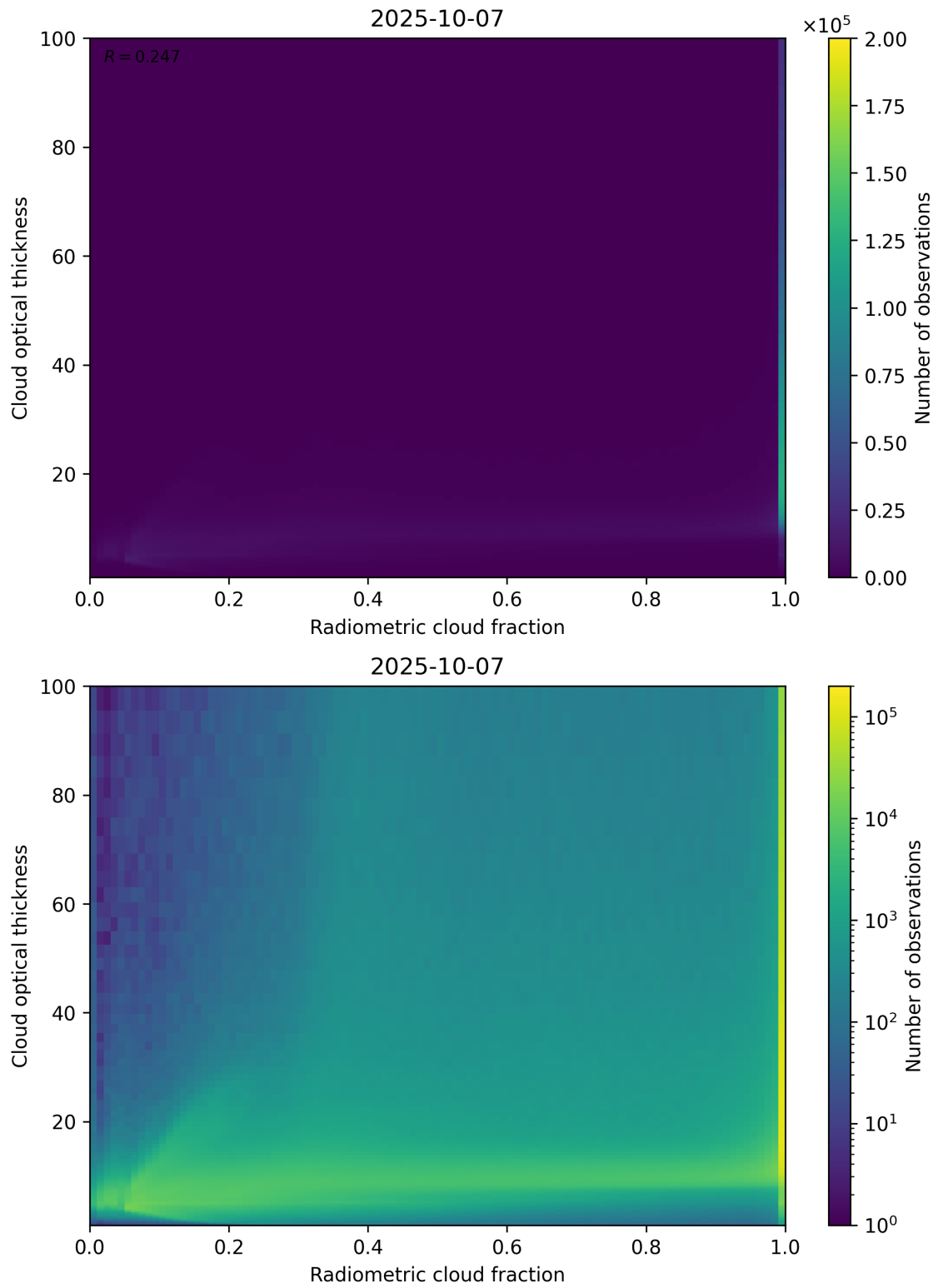
Figure 75: Scatter density plot of “Radiometric cloud fraction” against “Cloud optical thickness” for 2025-10-06 to 2025-10-08.
