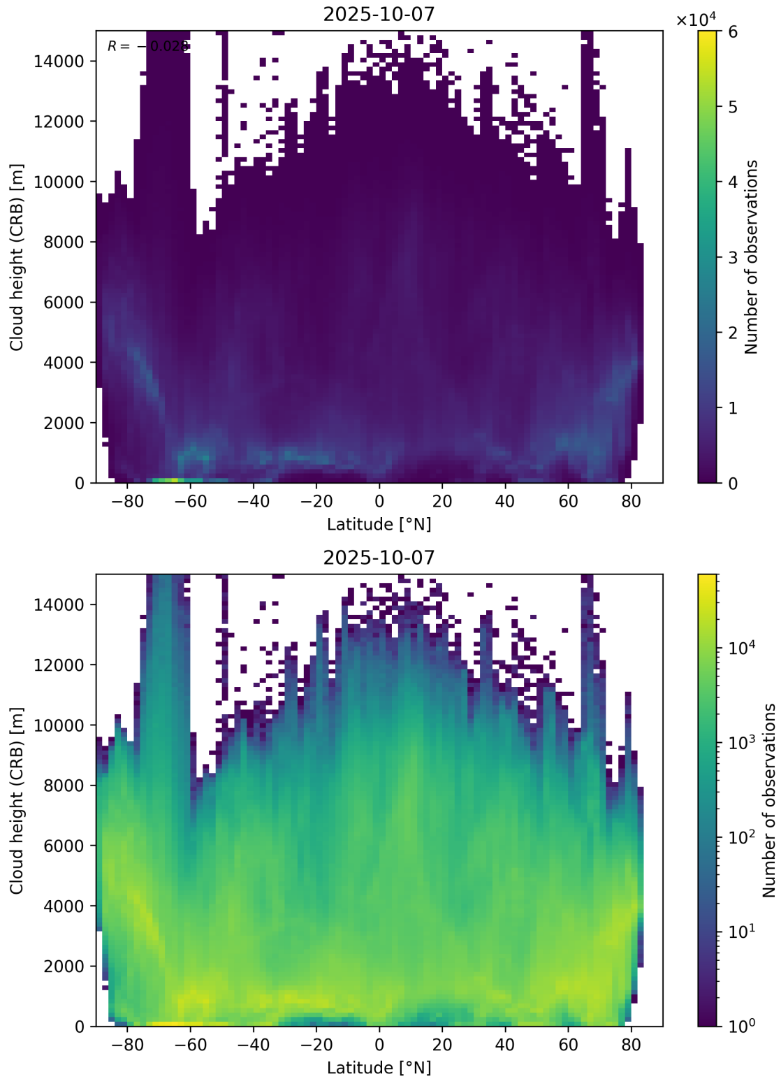
Figure 95: Scatter density plot of “Latitude” against “Cloud height (CRB)” for 2025-10-06 to 2025-10-08.
