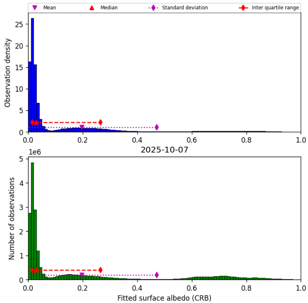
Figure 46: Histogram of “Fitted surface albedo (CRB)” for 2025-10-06 to 2025-10-08
