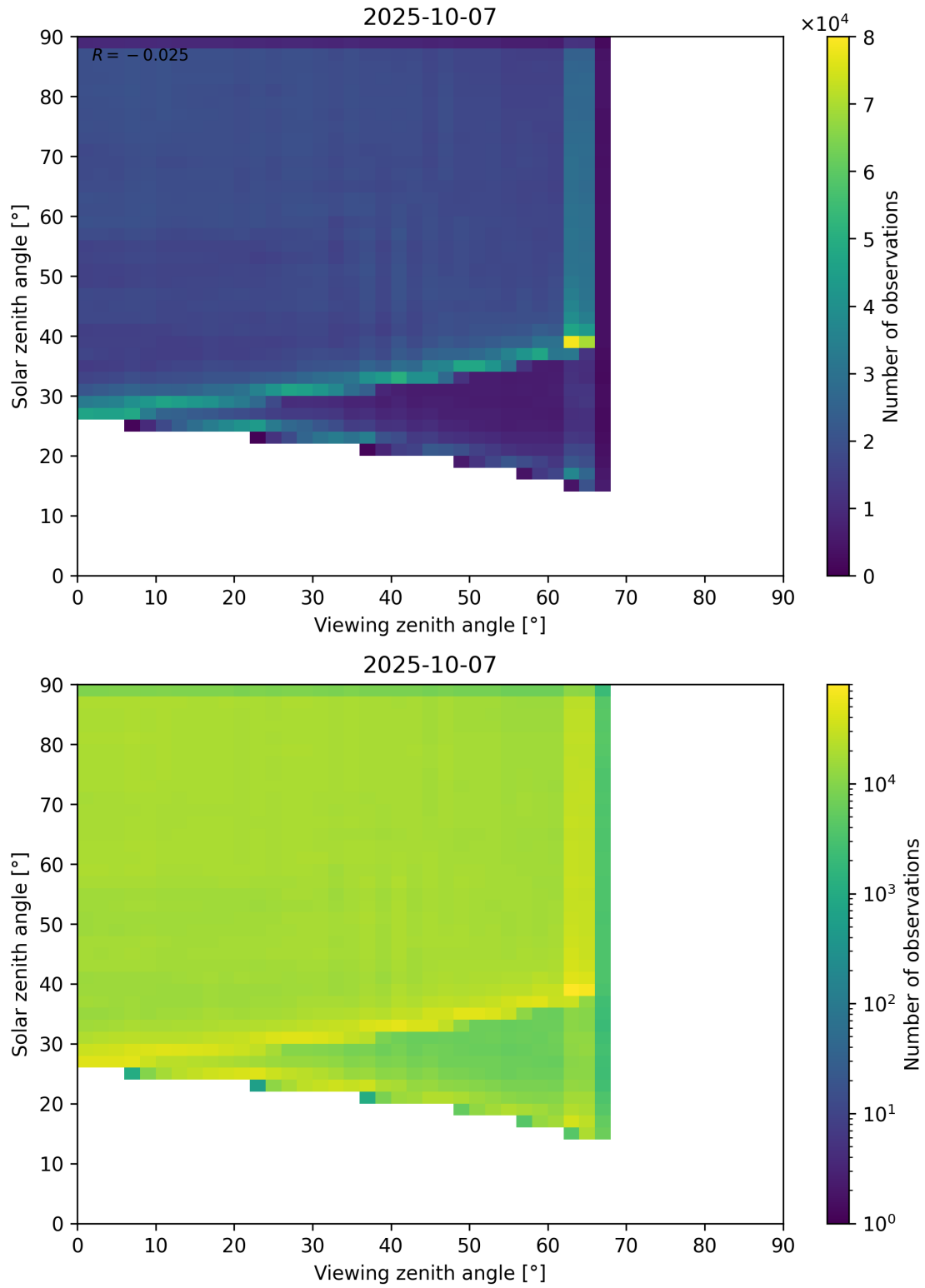
Figure 114: Scatter density plot of “Viewing zenith angle” against “Solar zenith angle” for 2025-10-06 to 2025-10-08.
