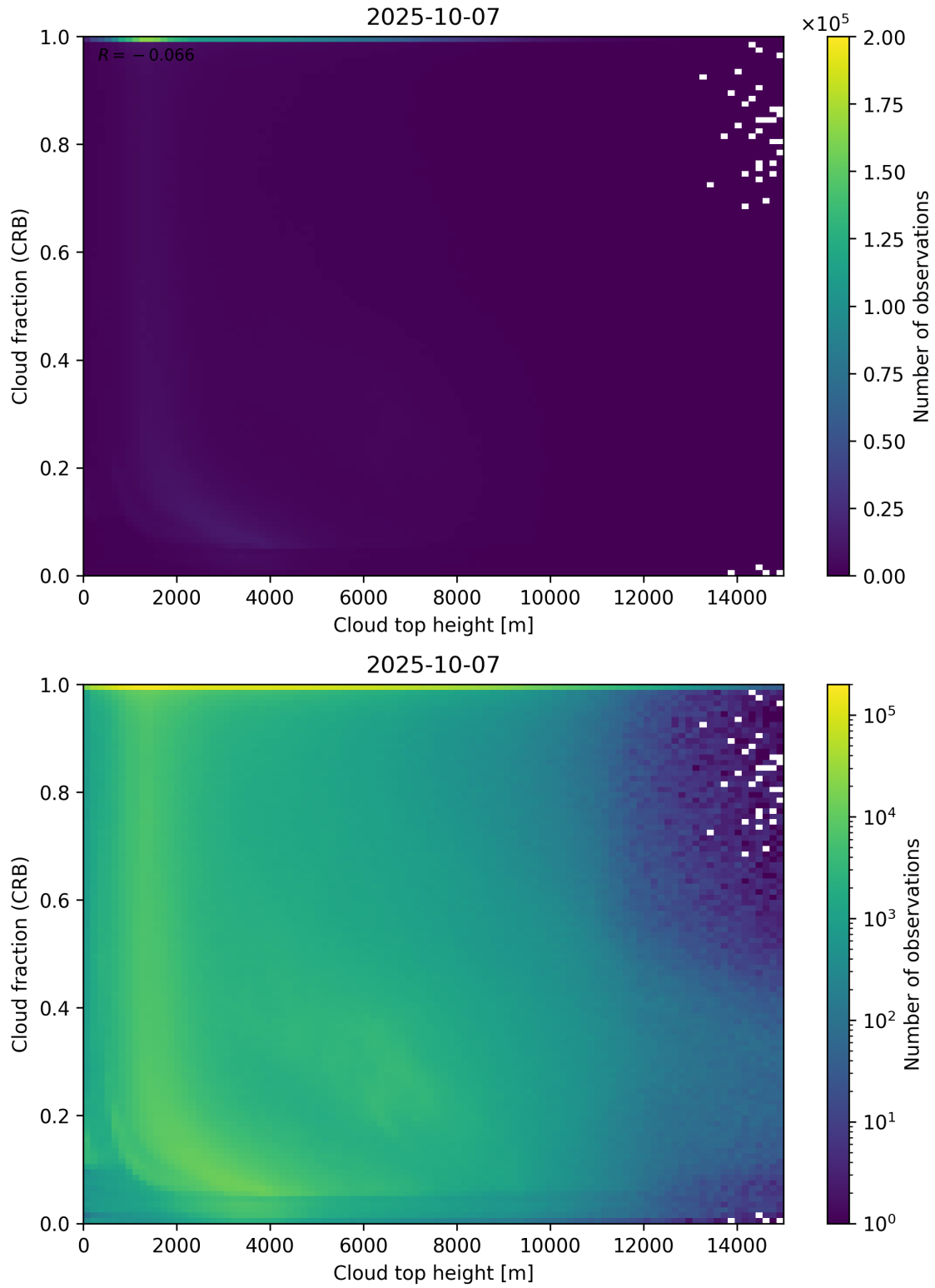
Figure 88: Scatter density plot of “Cloud top height” against “Cloud fraction (CRB)” for 2025-10-06 to 2025-10-08.
