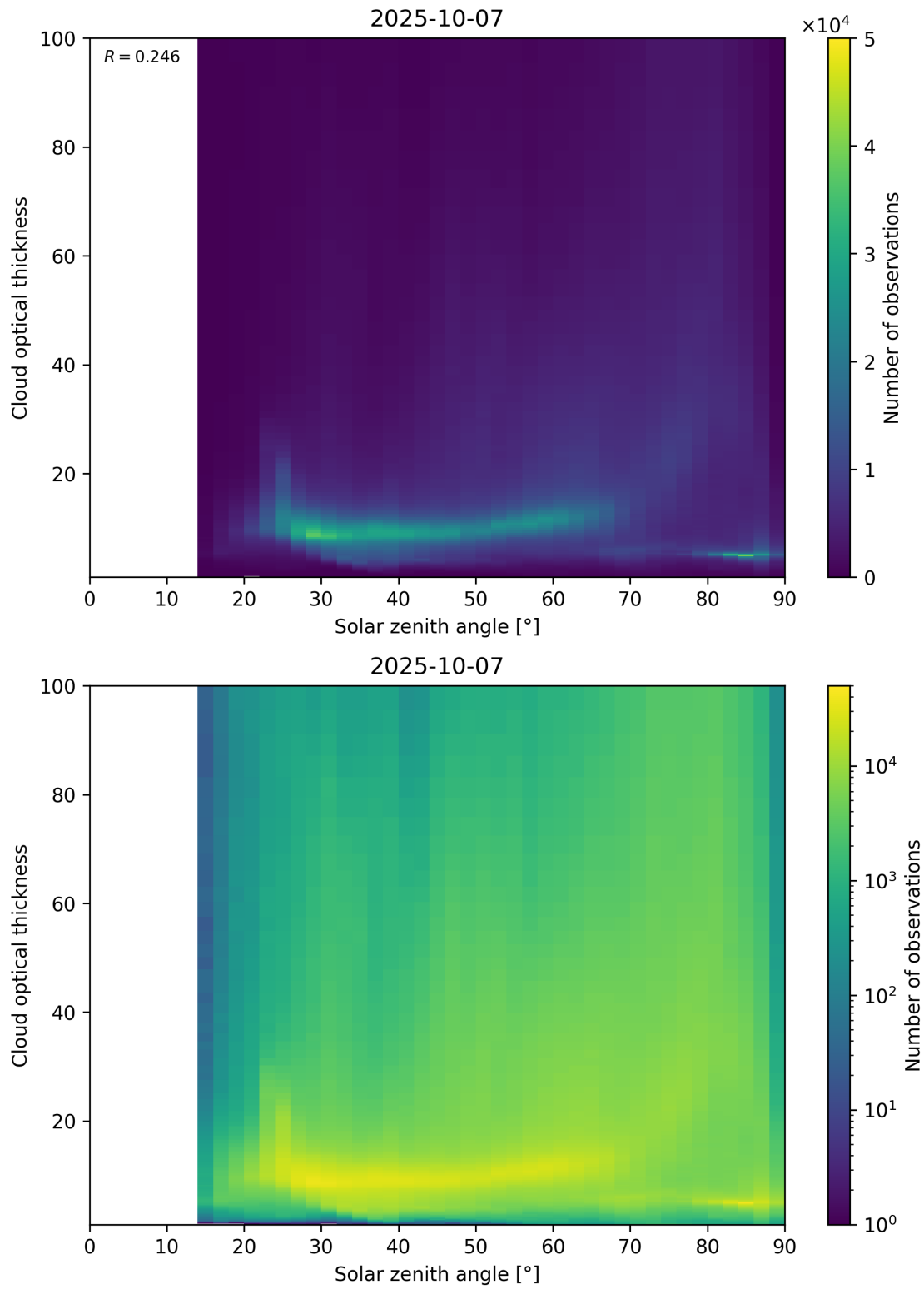
Figure 103: Scatter density plot of “Solar zenith angle” against “Cloud optical thickness” for 2025-10-06 to 2025-10-08.
