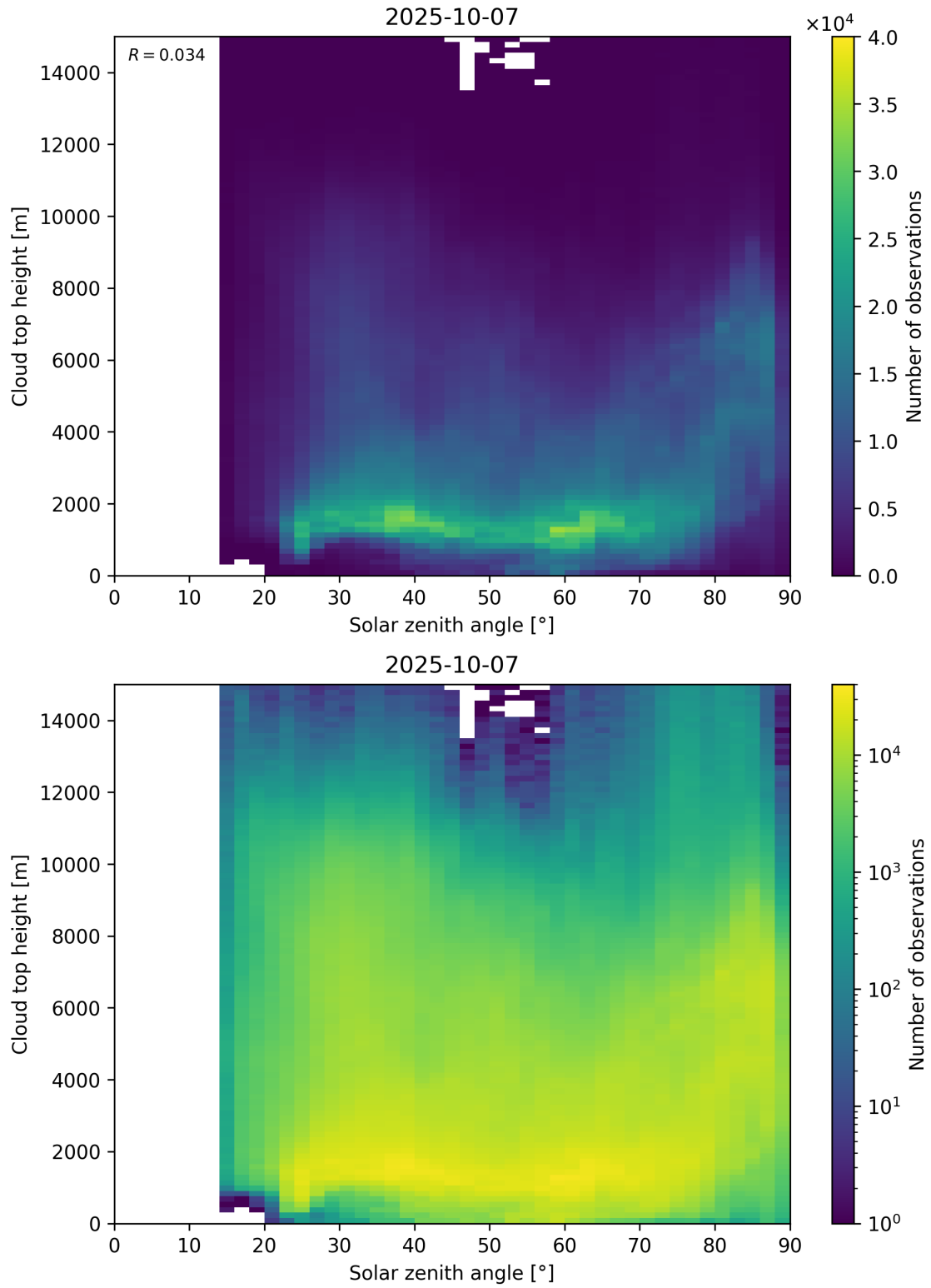
Figure 104: Scatter density plot of “Solar zenith angle” against “Cloud top height” for 2025-10-06 to 2025-10-08.
