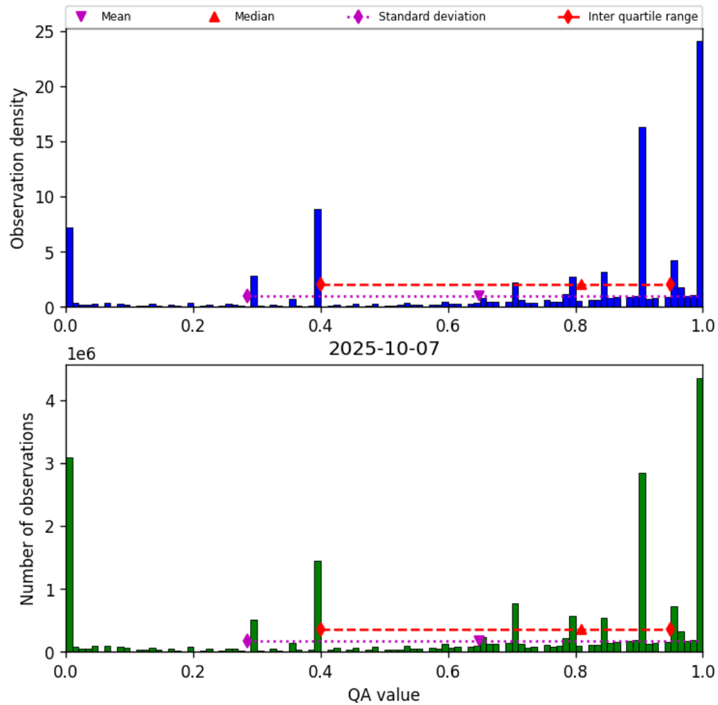
Figure 38: Histogram of “QA value” for 2025-10-06 to 2025-10-08
