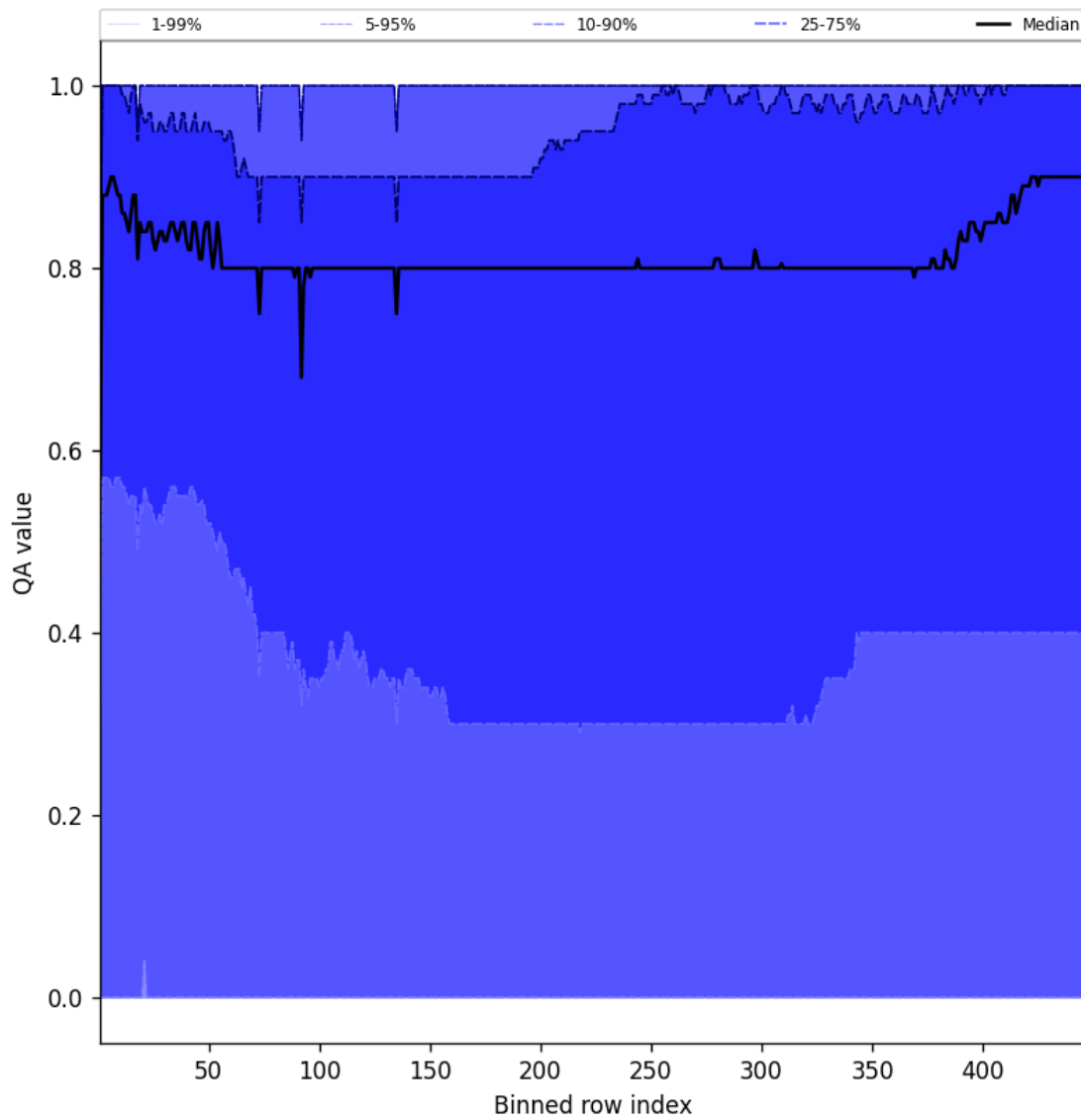
Figure 54: Along track statistics of “QA value” for 2025-10-06 to 2025-10-08
