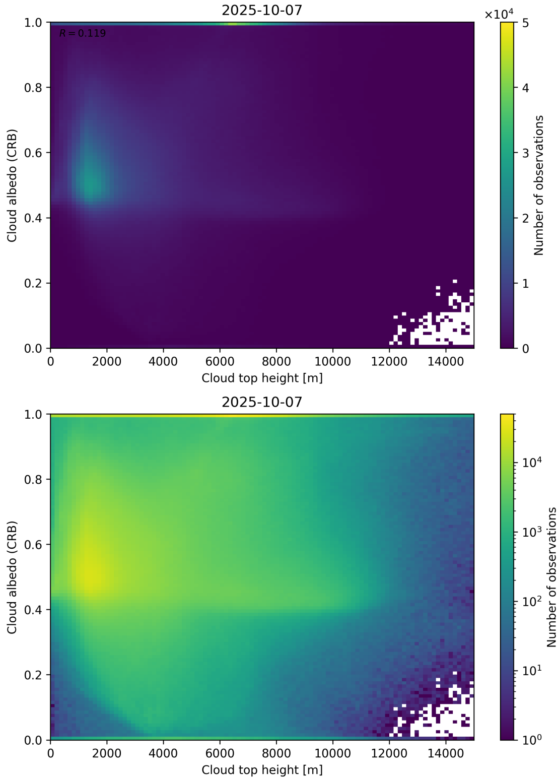
Figure 86: Scatter density plot of “Cloud top height” against “Cloud albedo (CRB)” for 2025-10-06 to 2025-10-08.
