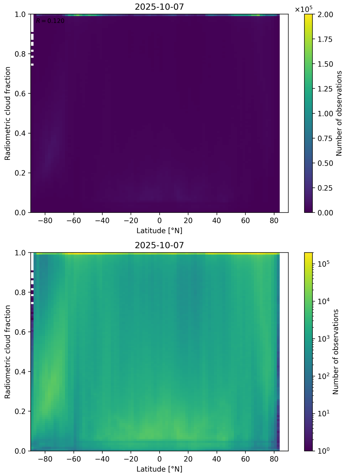
Figure 92: Scatter density plot of “Latitude” against “Radiometric cloud fraction” for 2025-10-06 to 2025-10-08.
