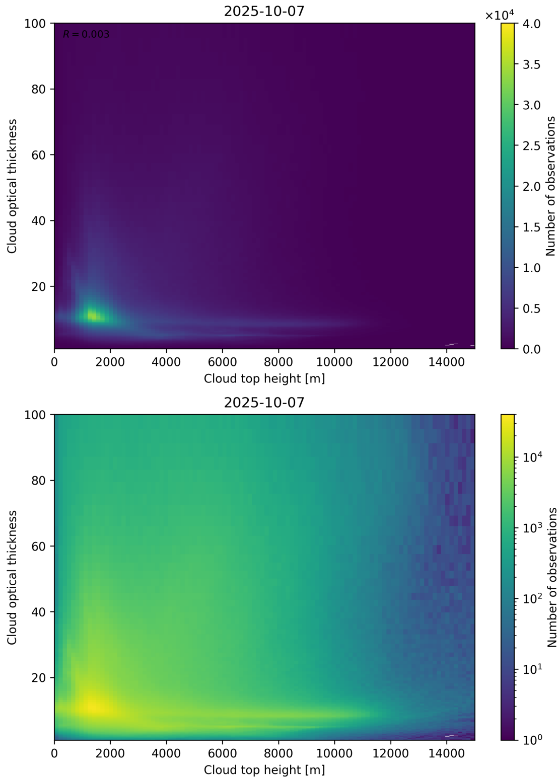
Figure 90: Scatter density plot of “Cloud top height” against “Cloud optical thickness” for 2025-10-06 to 2025-10-08.
