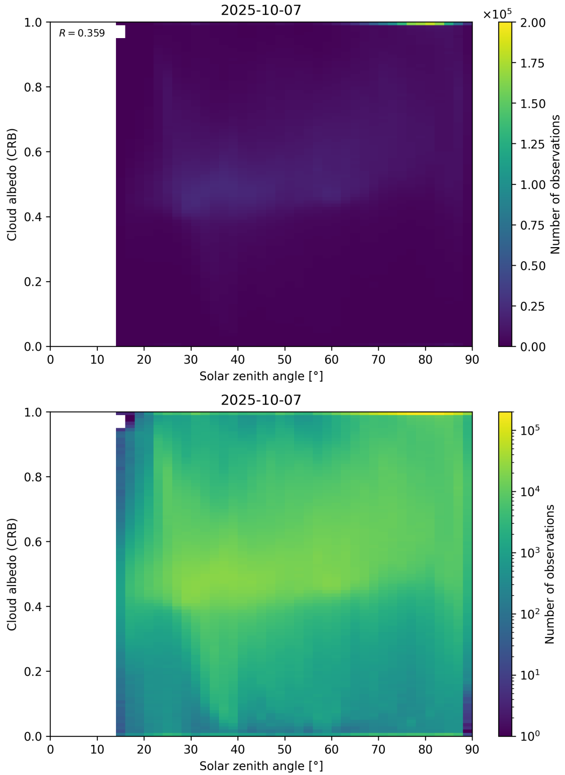
Figure 98: Scatter density plot of “Solar zenith angle” against “Cloud albedo (CRB)” for 2025-10-06 to 2025-10-08.
