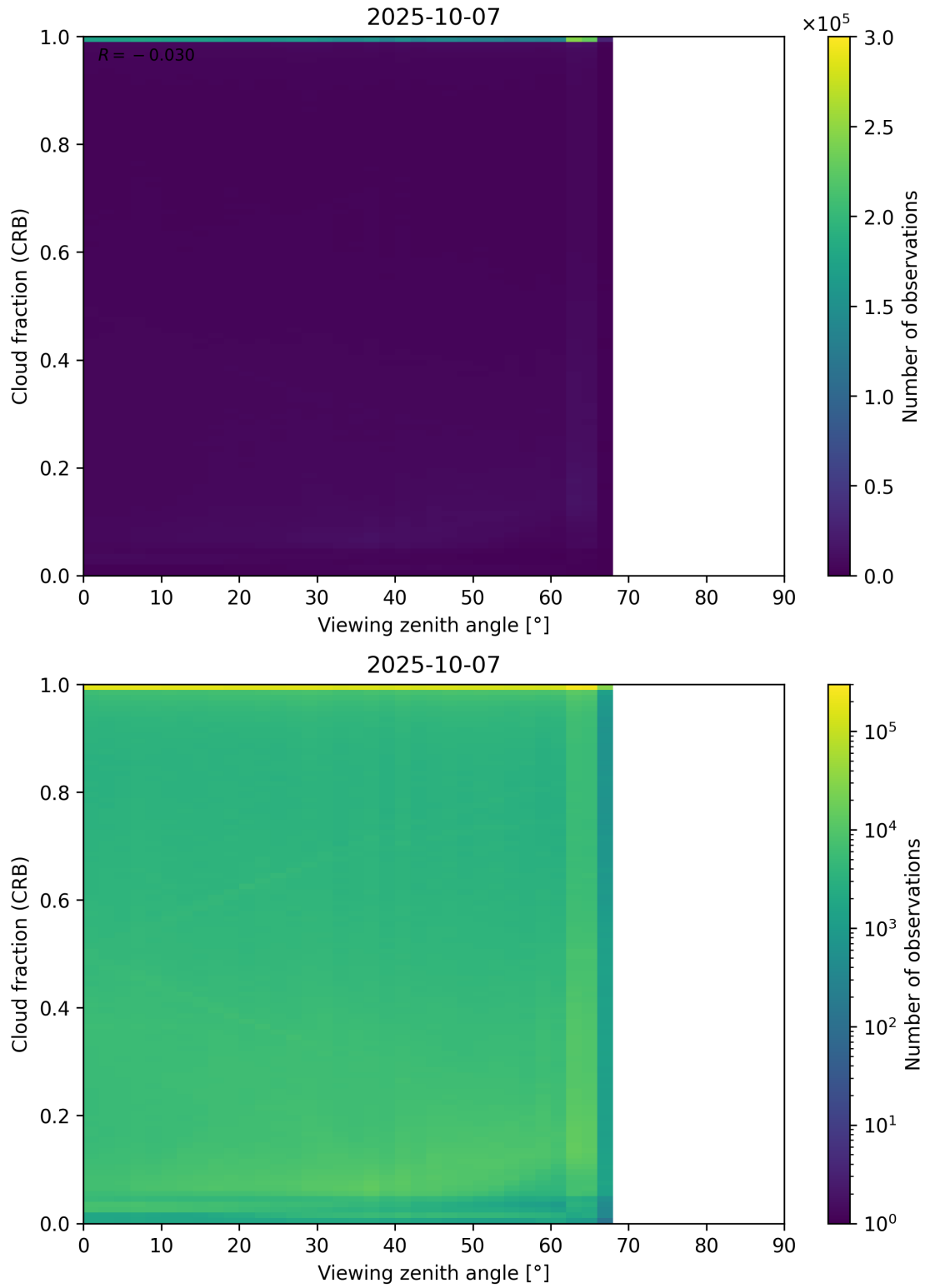
Figure 109: Scatter density plot of “Viewing zenith angle” against “Cloud fraction (CRB)” for 2025-10-06 to 2025-10-08.
