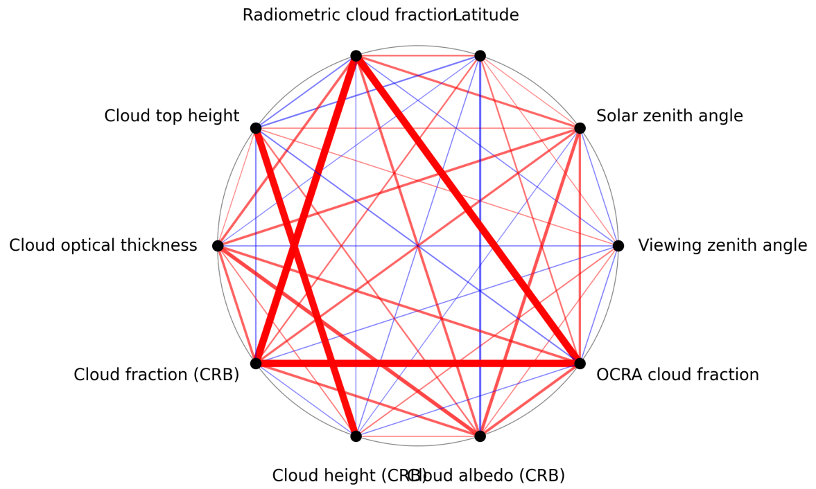
Figure 1: Map of correlation graph for 2025-10-06 to 2025-10-08.
