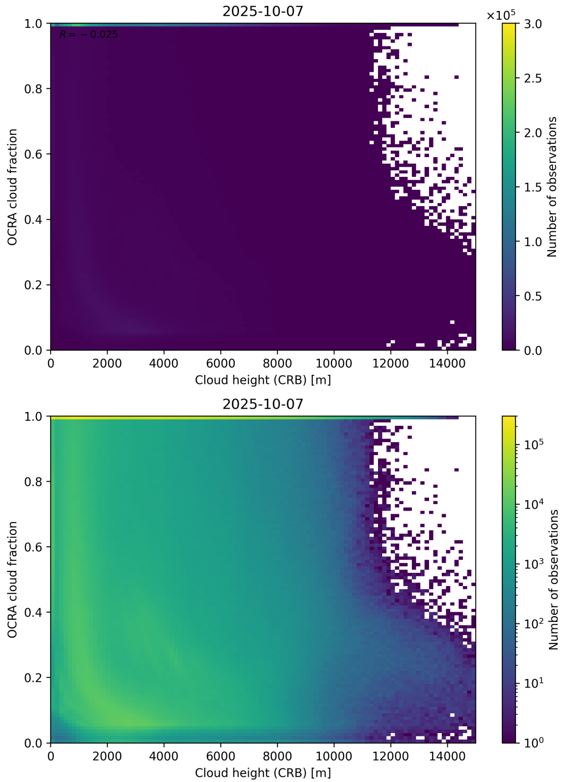
Figure 81: Scatter density plot of “Cloud height (CRB)” against “OCRA cloud fraction” for 2025-10-06 to 2025-10-08.
