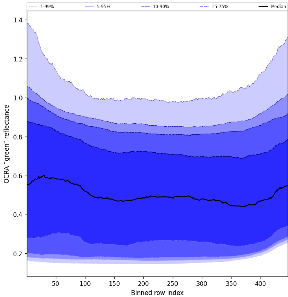
Figure 68: Along track statistics of "OCRA "green" reflectance" for 2025-10-06 to 2025-10-08
