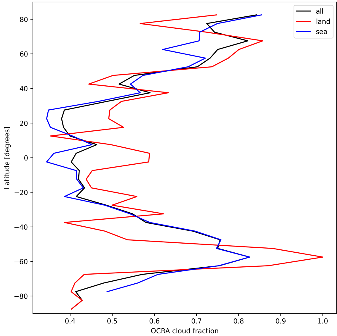
Figure 34: Zonal average of “OCRA cloud fraction” for 2025-10-06 to 2025-10-08.
