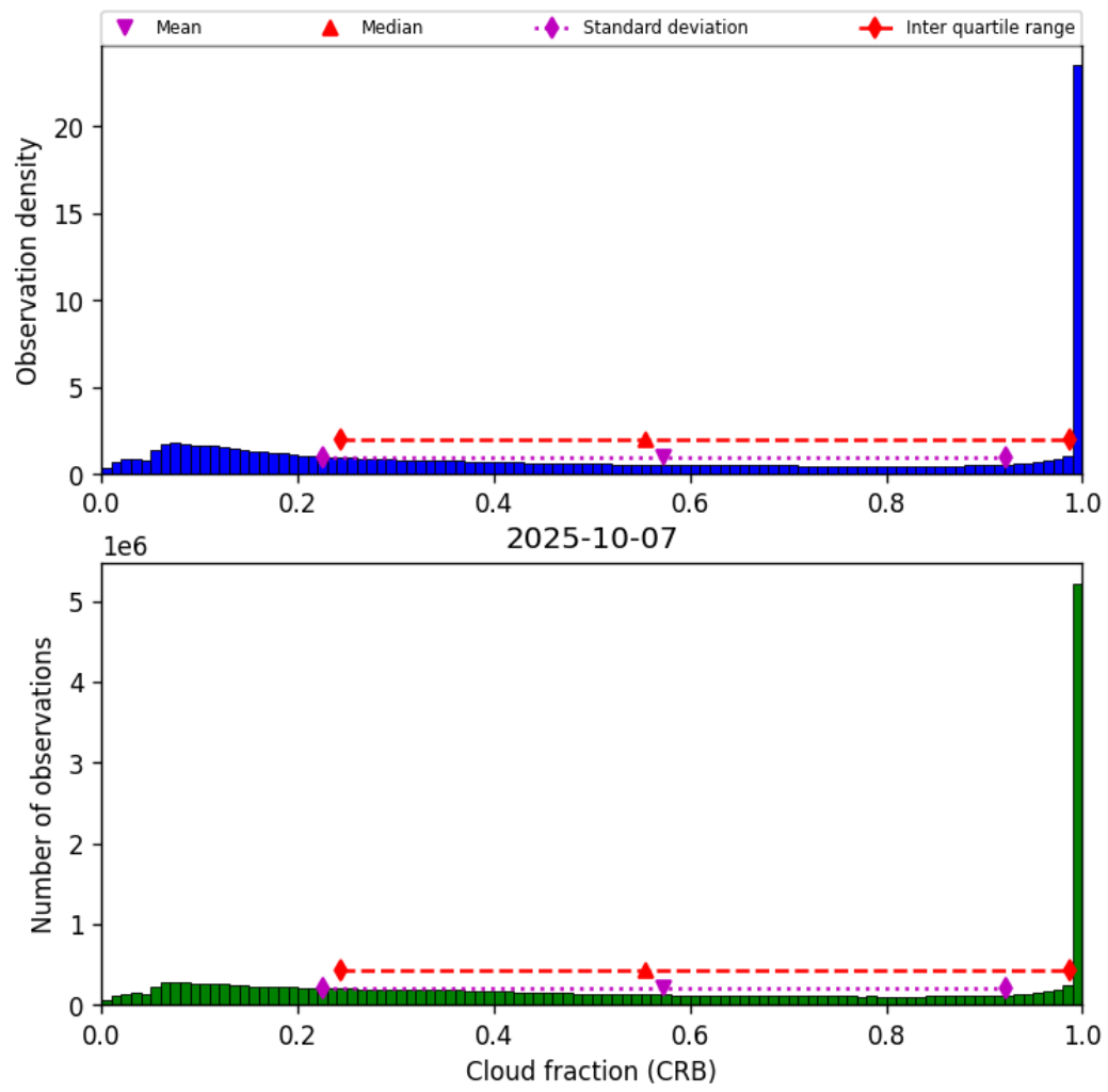
Figure 42: Histogram of “Cloud fraction (CRB)” for 2025-10-06 to 2025-10-08
