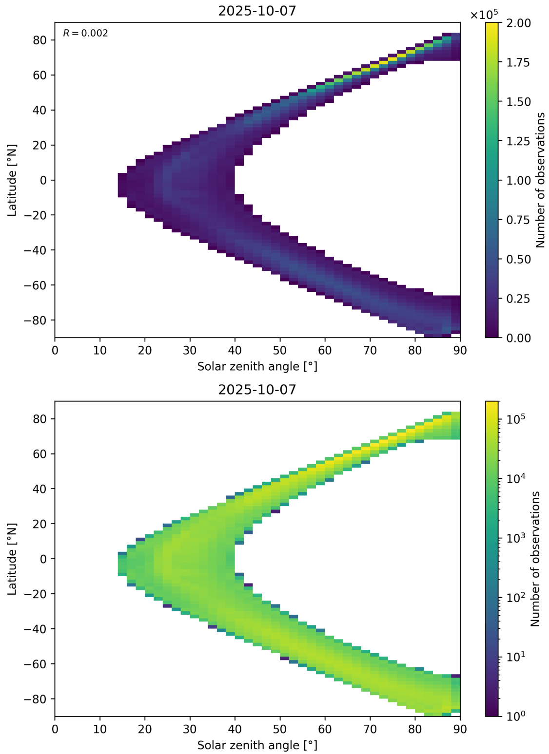
Figure 105: Scatter density plot of “Solar zenith angle” against “Latitude” for 2025-10-06 to 2025-10-08.
