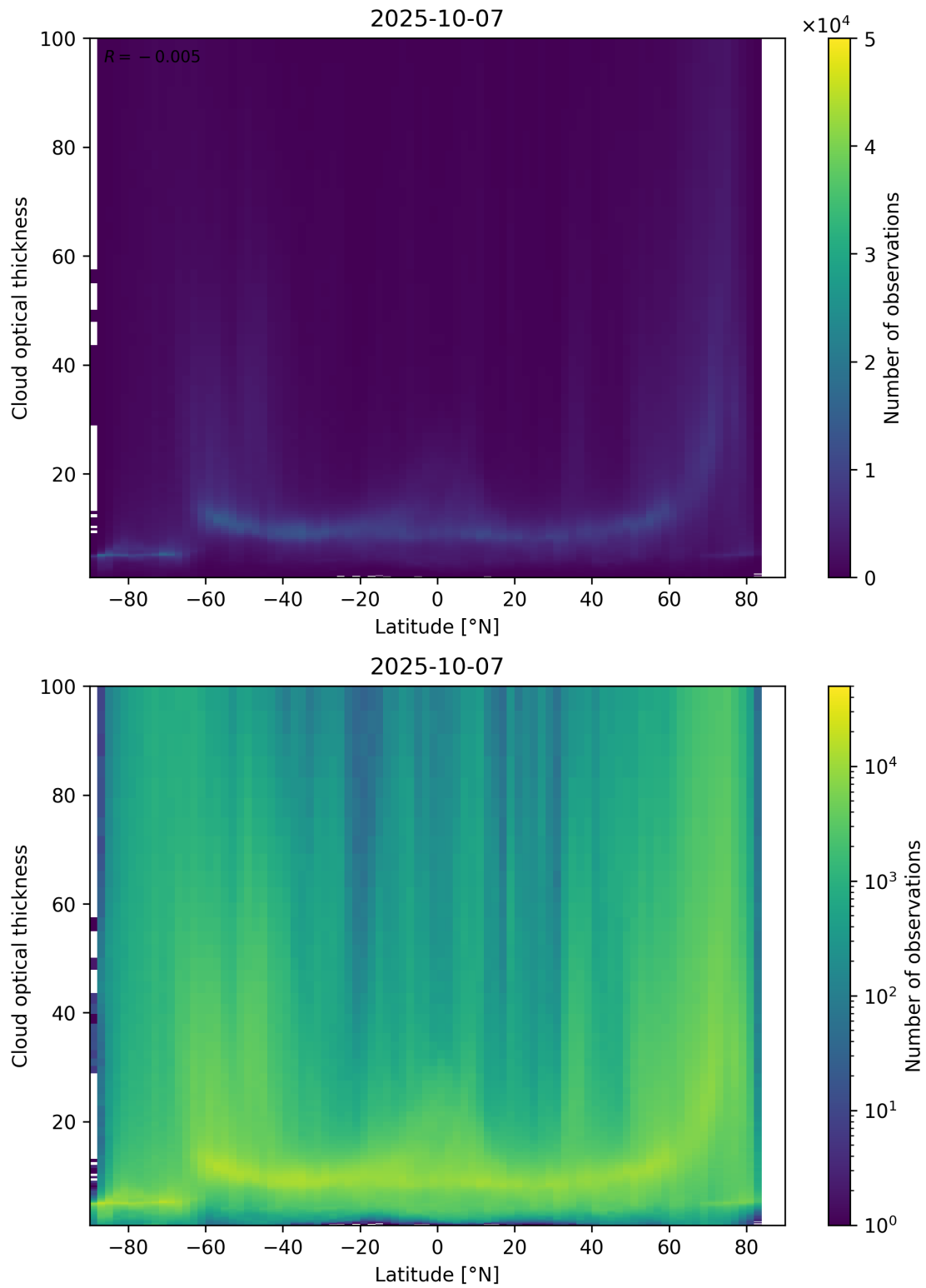
Figure 96: Scatter density plot of “Latitude” against “Cloud optical thickness” for 2025-10-06 to 2025-10-08.
