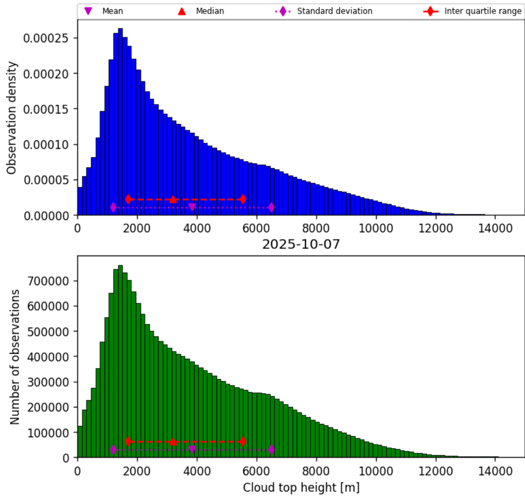
Figure 40: Histogram of “Cloud top height” for 2025-10-06 to 2025-10-08
