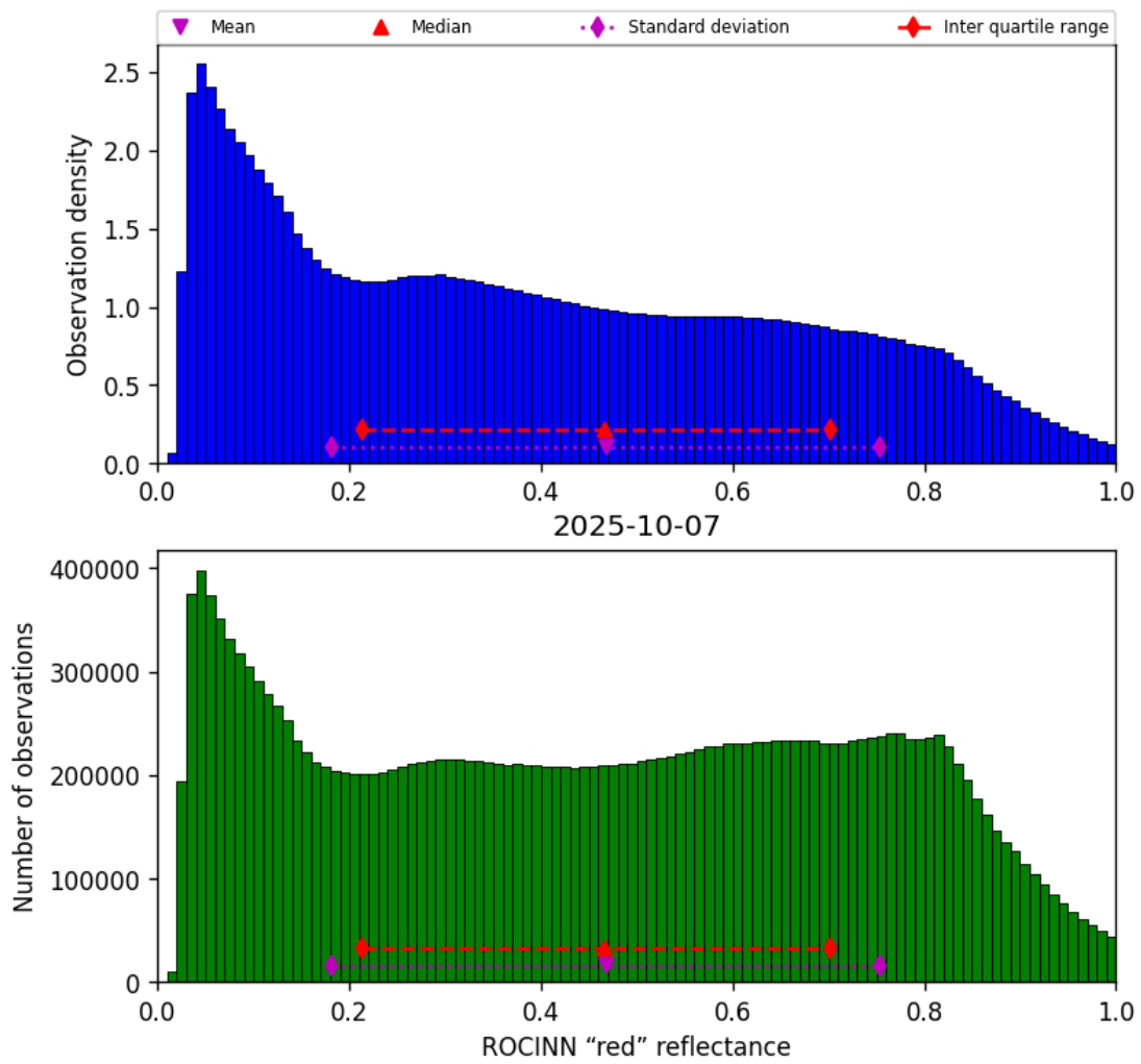
Figure 53: Histogram of “ROCINN “red” reflectance” for 2025-10-06 to 2025-10-08
