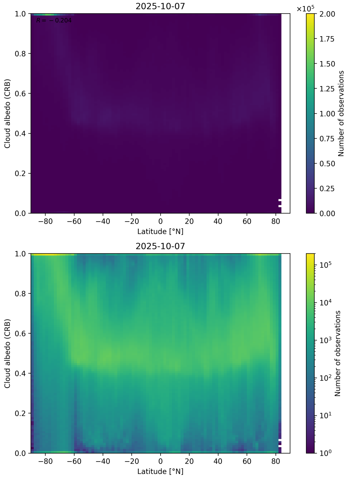
Figure 91: Scatter density plot of “Latitude” against “Cloud albedo (CRB)” for 2025-10-06 to 2025-10-08.
