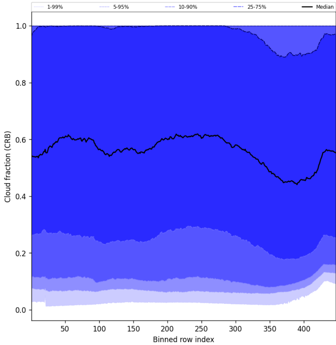
Figure 58: Along track statistics of “Cloud fraction (CRB)” for 2025-10-06 to 2025-10-08
