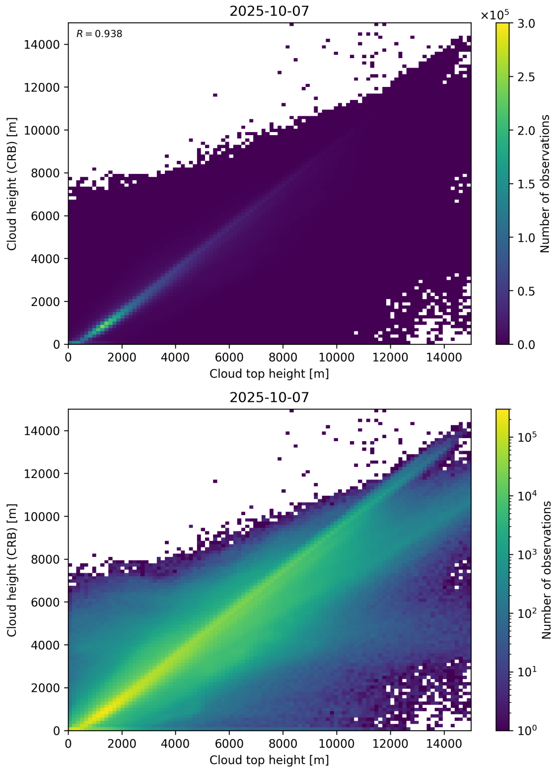
Figure 89: Scatter density plot of “Cloud top height” against “Cloud height (CRB)” for 2025-10-06 to 2025-10-08.
