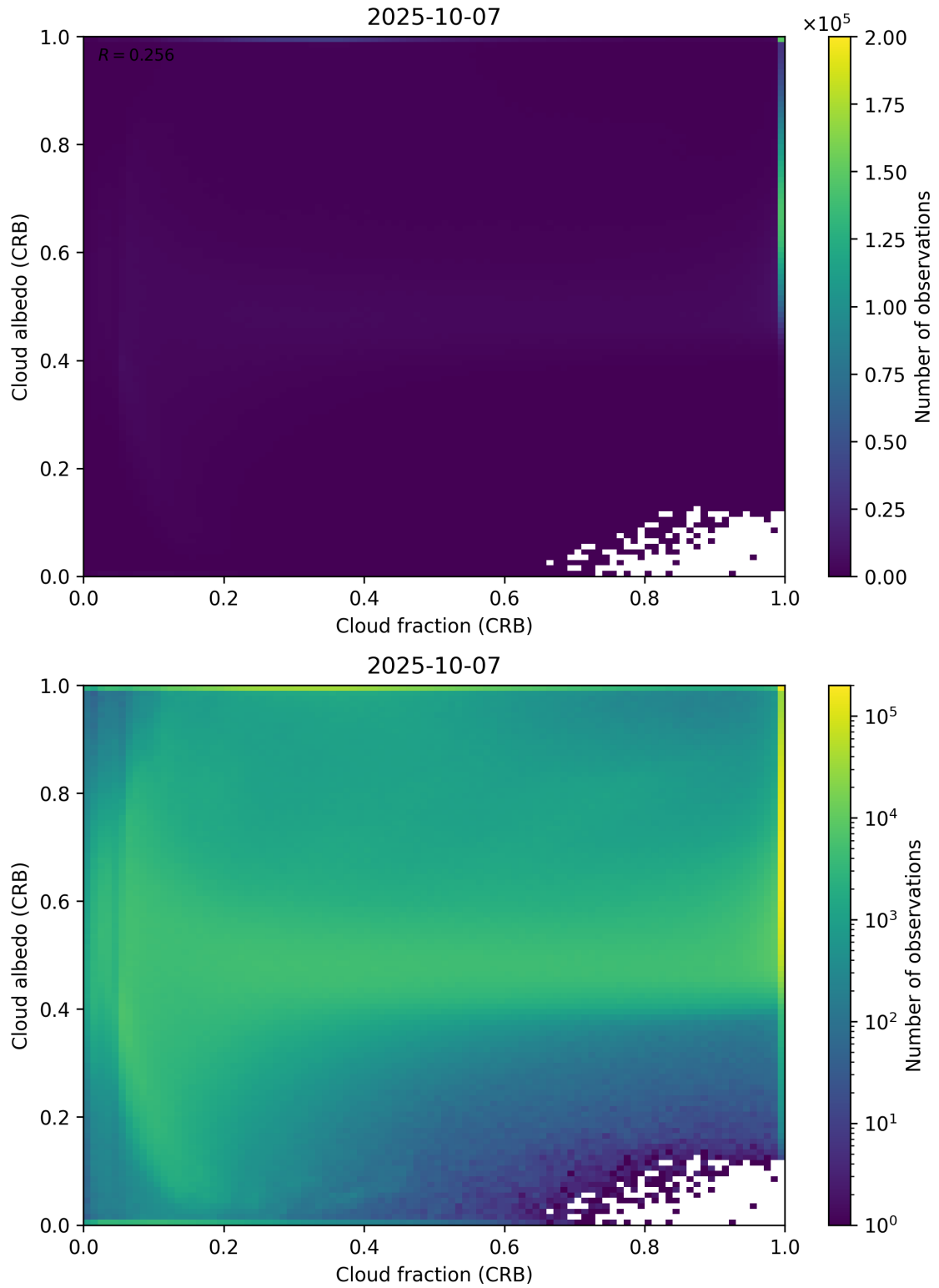
Figure 77: Scatter density plot of “Cloud fraction (CRB)” against “Cloud albedo (CRB)” for 2025-10-06 to 2025-10-08.
