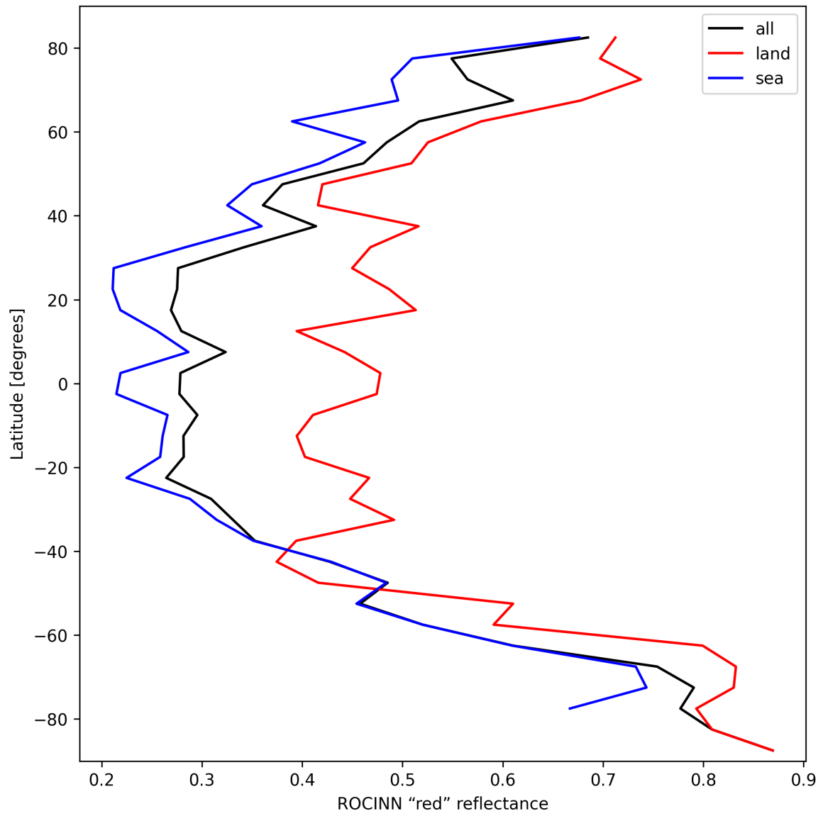
Figure 37: Zonal average of “ROCINN “red” reflectance” for 2025-10-06 to 2025-10-08.
