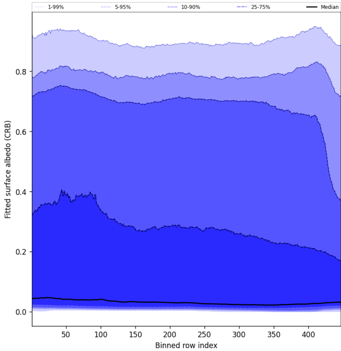
Figure 62: Along track statistics of “Fitted surface albedo (CRB)” for 2025-10-06 to 2025-10-08
