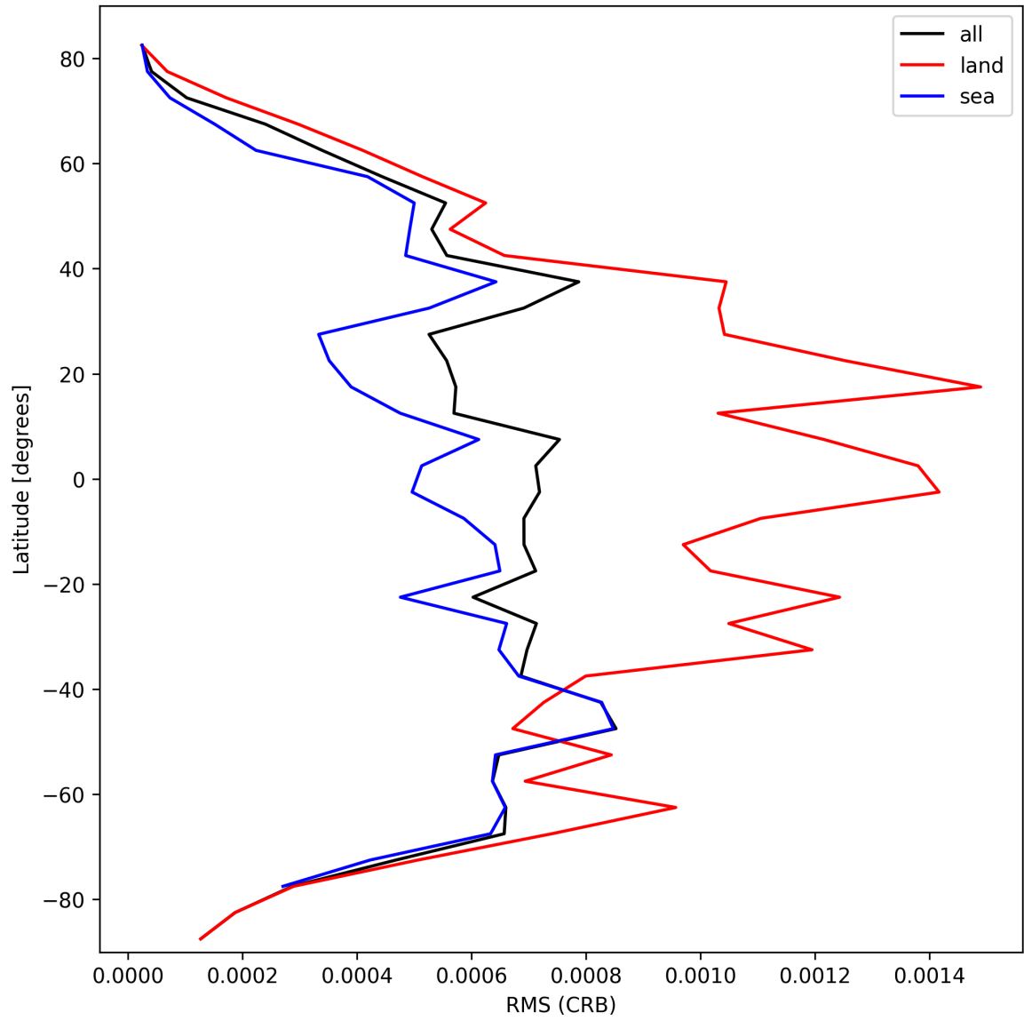
Figure 32: Zonal average of “RMS (CRB)” for 2025-10-06 to 2025-10-08.
