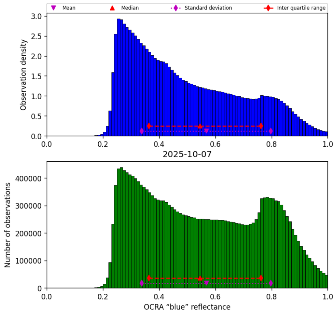
Figure 51: Histogram of “OCRA “blue” reflectance” for 2025-10-06 to 2025-10-08
