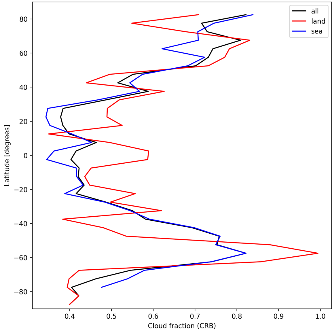
Figure 26: Zonal average of “Cloud fraction (CRB)” for 2025-10-06 to 2025-10-08.
