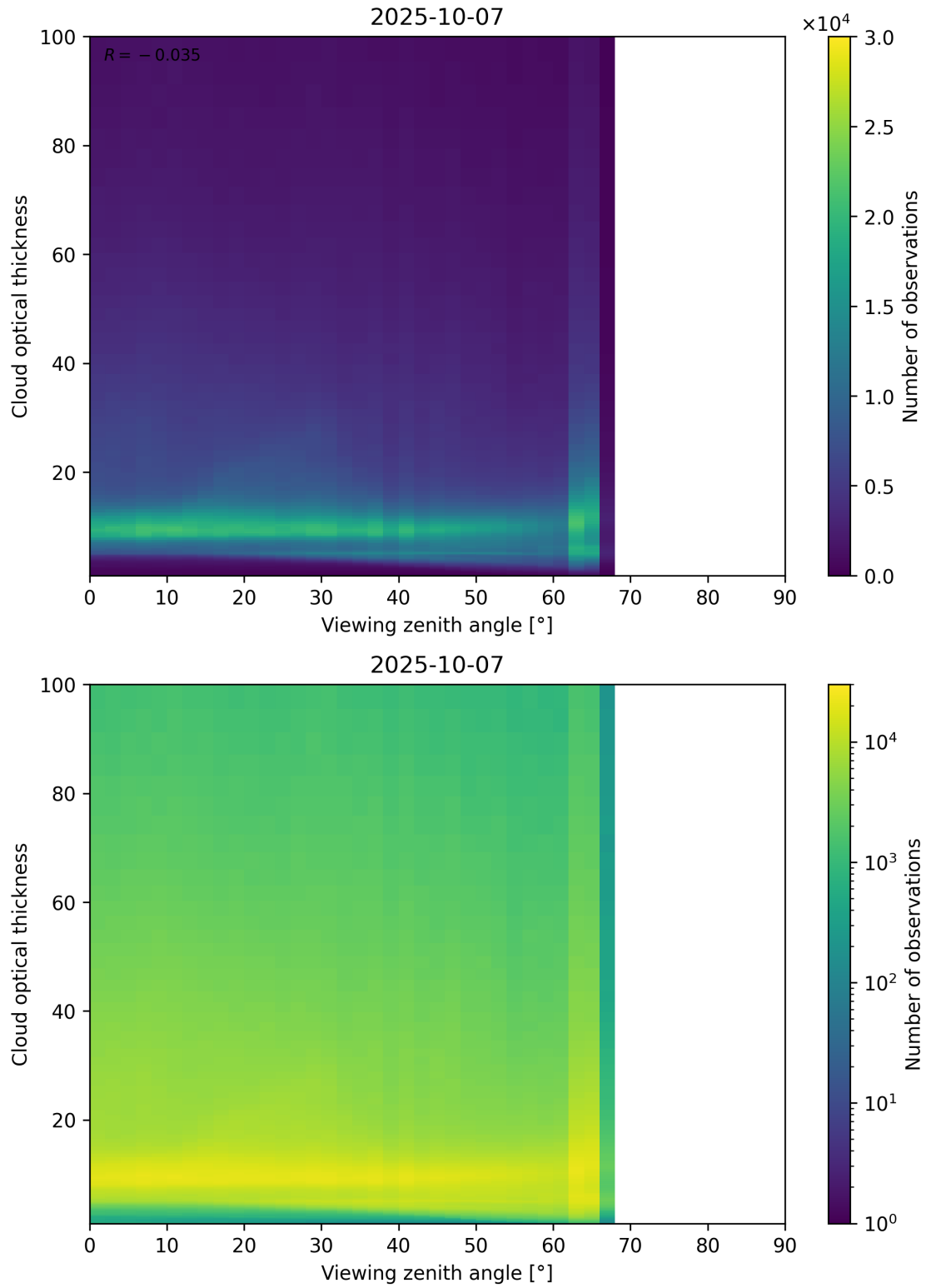
Figure 111: Scatter density plot of “Viewing zenith angle” against “Cloud optical thickness” for 2025-10-06 to 2025-10-08.
