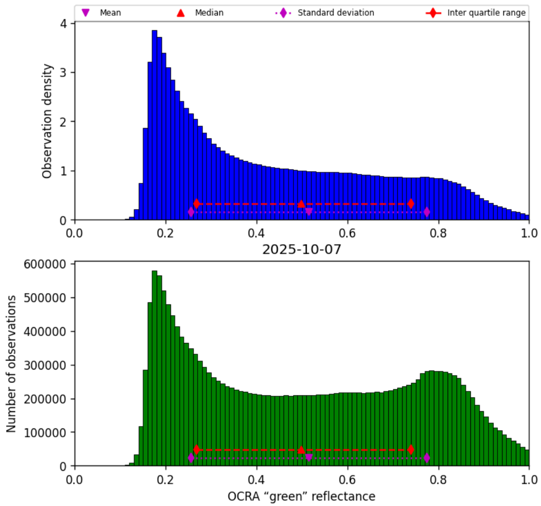
Figure 52: Histogram of “OCRA “green” reflectance” for 2025-10-06 to 2025-10-08
