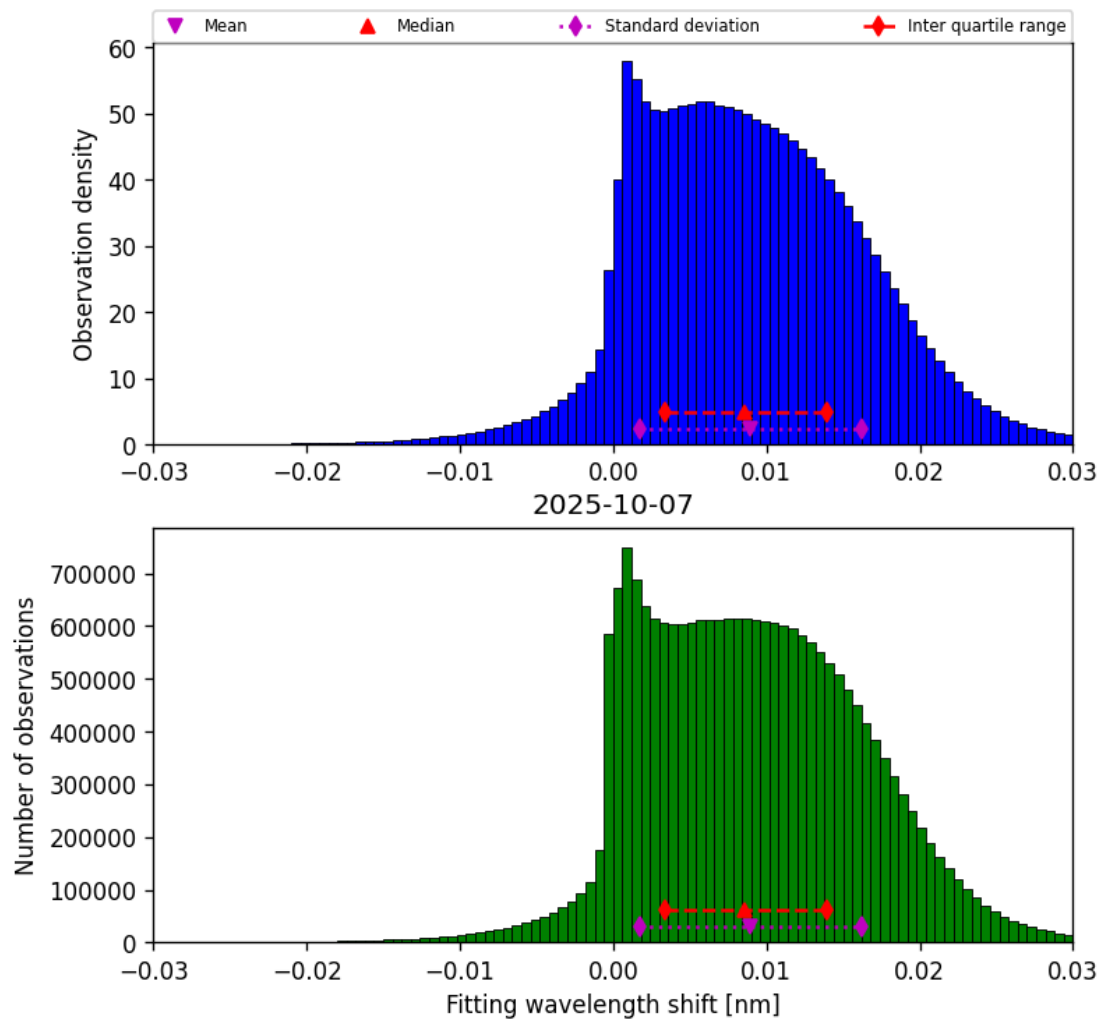
Figure 49: Histogram of “Fitting wavelength shift” for 2025-10-06 to 2025-10-08
