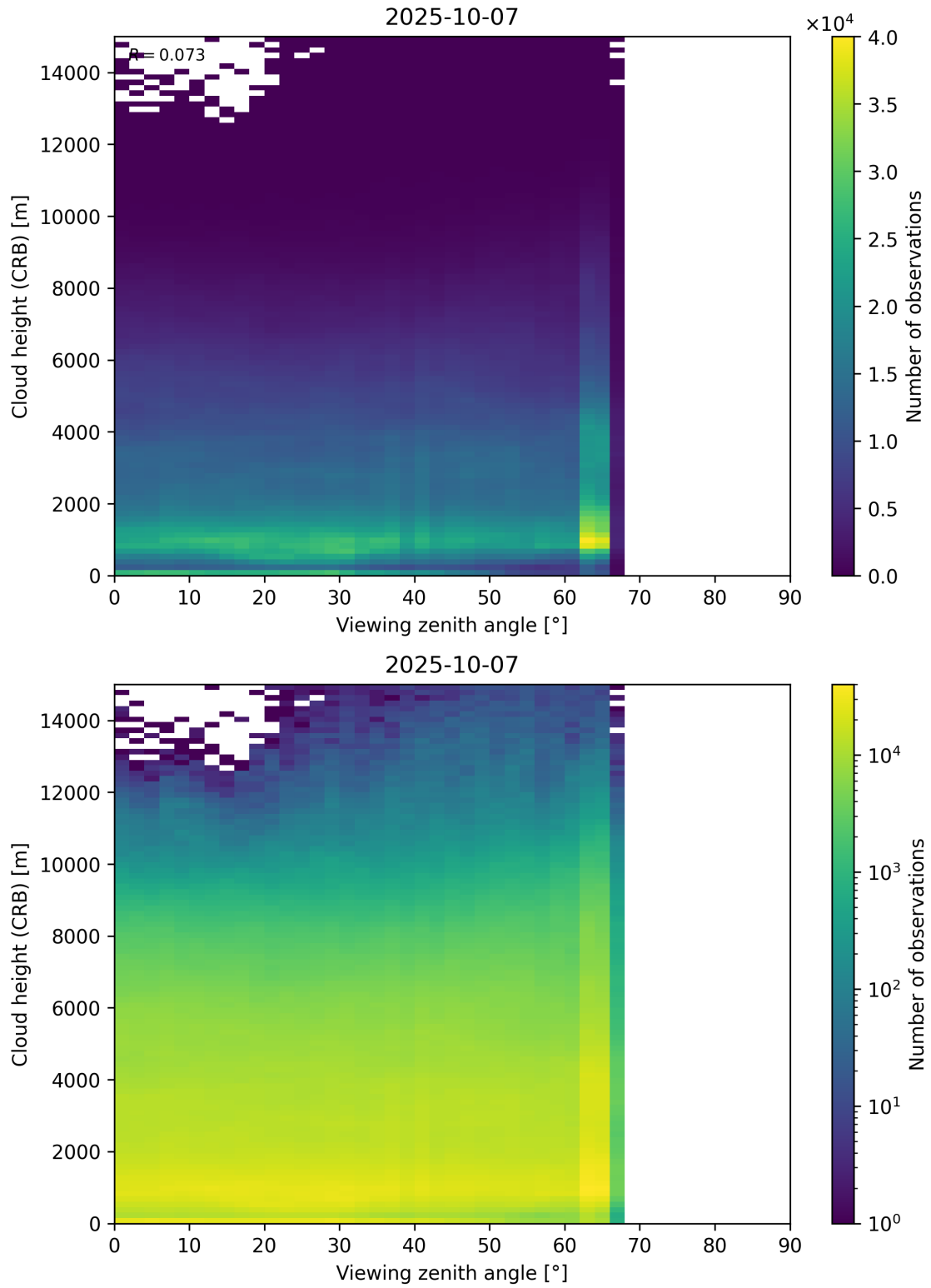
Figure 110: Scatter density plot of “Viewing zenith angle” against “Cloud height (CRB)” for 2025-10-06 to 2025-10-08.
