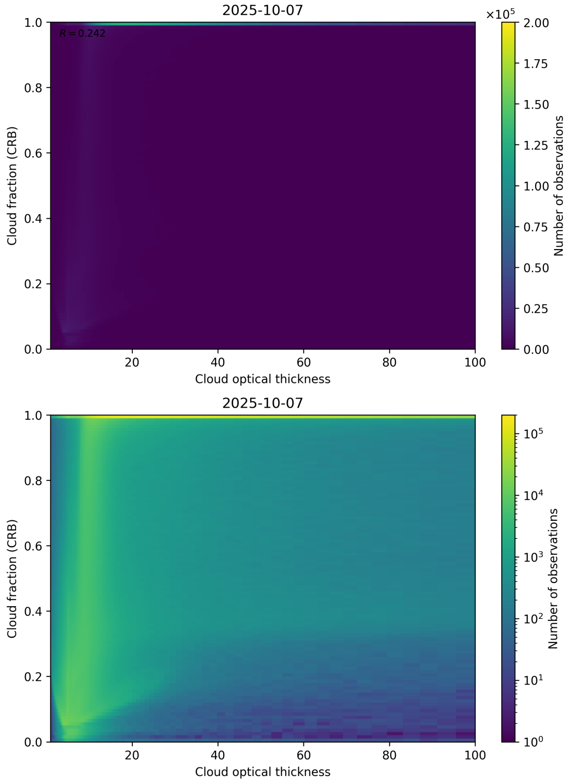
Figure 84: Scatter density plot of “Cloud optical thickness” against “Cloud fraction (CRB)” for 2025-10-06 to 2025-10-08.
