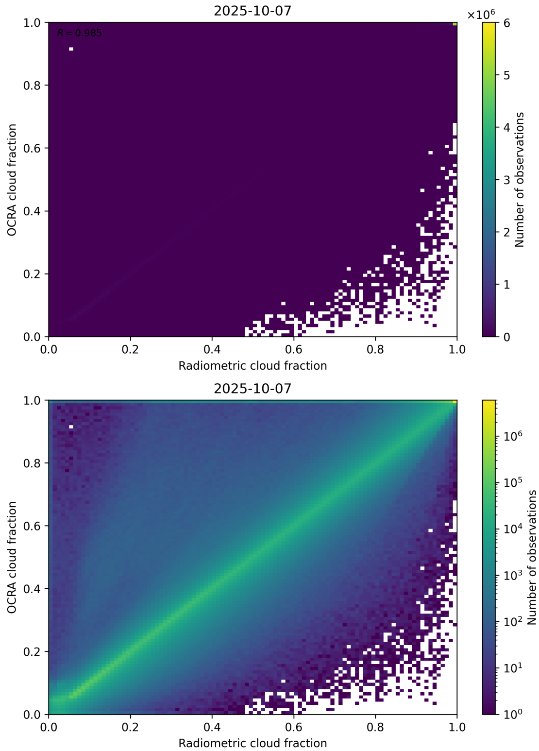
Figure 72: Scatter density plot of “Radiometric cloud fraction” against “OCRA cloud fraction” for 2025-10-06 to 2025-10-08.
