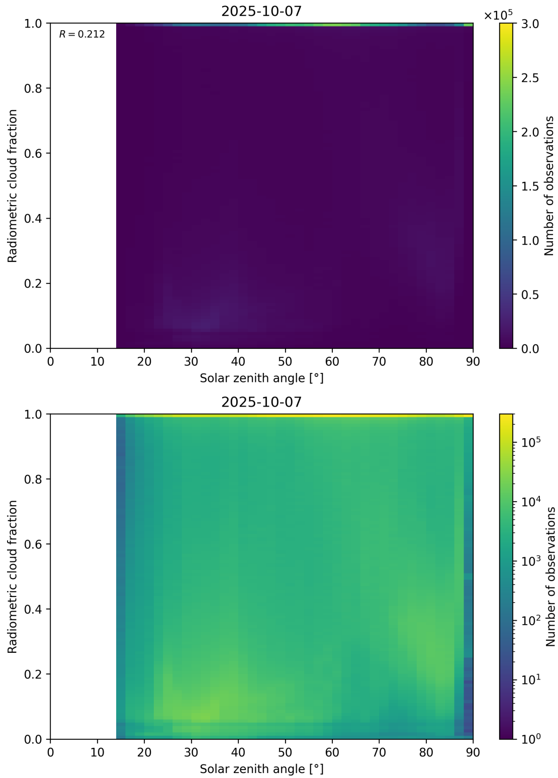
Figure 99: Scatter density plot of “Solar zenith angle” against “Radiometric cloud fraction” for 2025-10-06 to 2025-10-08.
