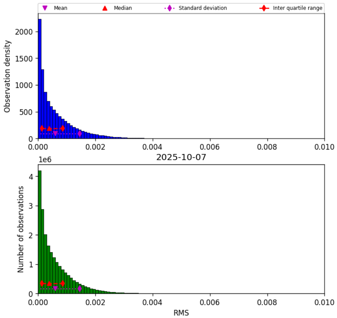
Figure 47: Histogram of “RMS” for 2025-10-06 to 2025-10-08
