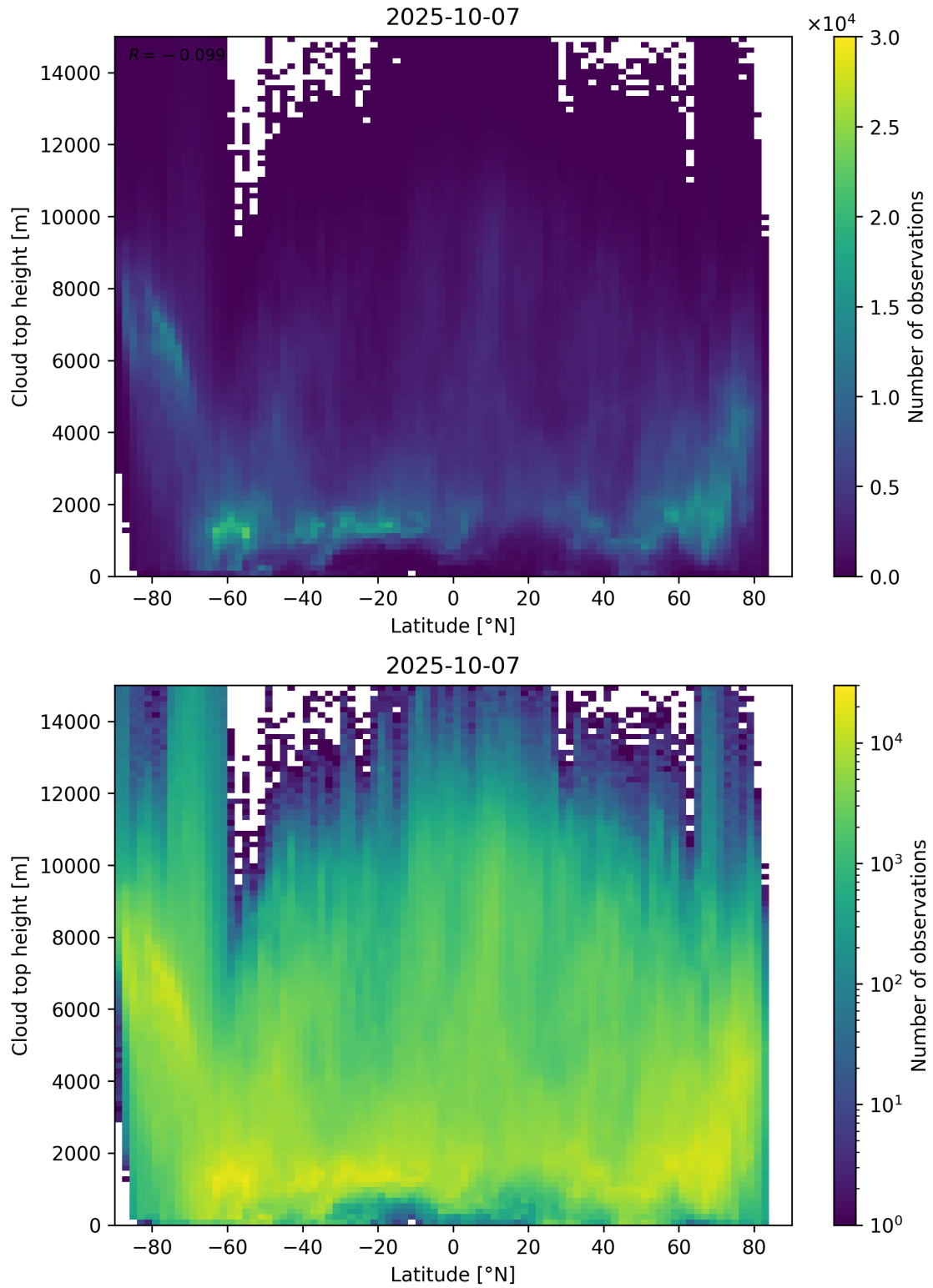
Figure 97: Scatter density plot of “Latitude” against “Cloud top height” for 2025-10-06 to 2025-10-08.
