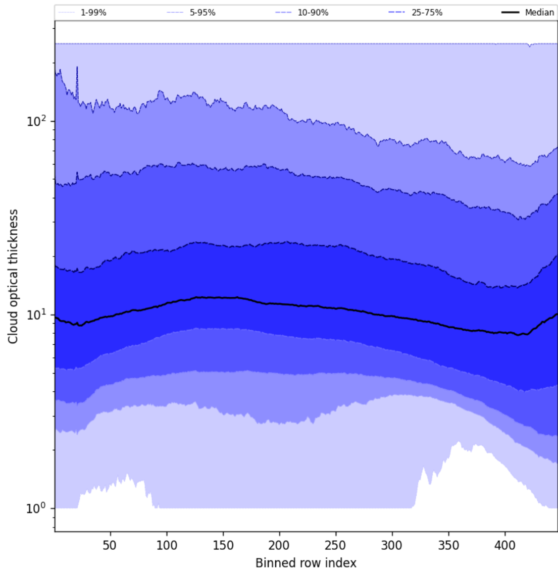
Figure 57: Along track statistics of “Cloud optical thickness” for 2025-10-06 to 2025-10-08
