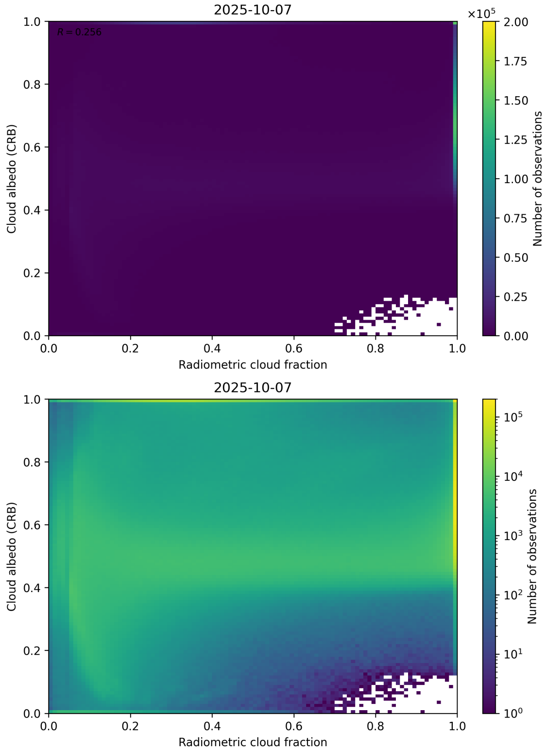
Figure 71: Scatter density plot of “Radiometric cloud fraction” against “Cloud albedo (CRB)” for 2025-10-06 to 2025-10-08.
