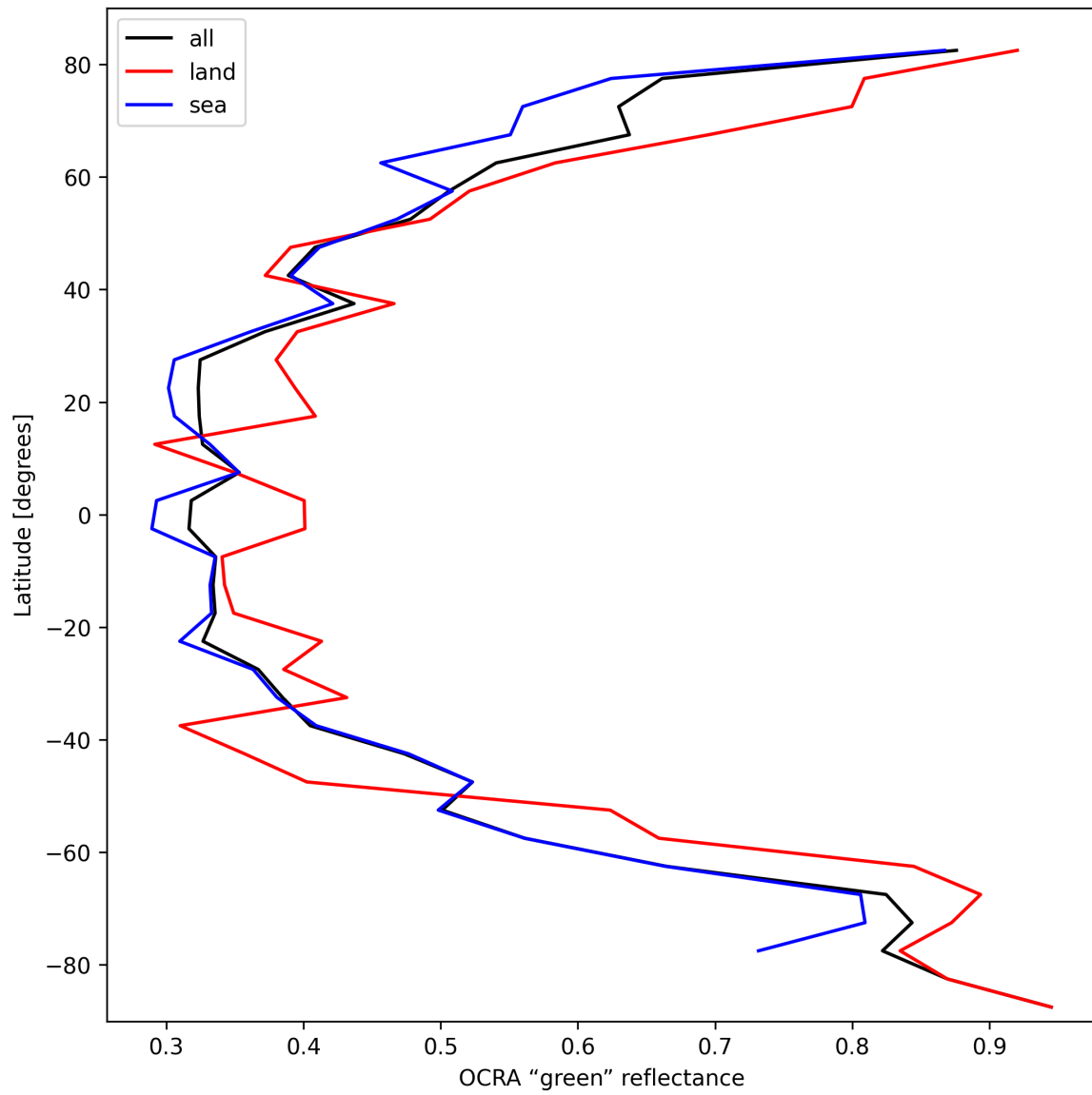
Figure 36: Zonal average of “OCRA “green” reflectance” for 2025-10-06 to 2025-10-08.
