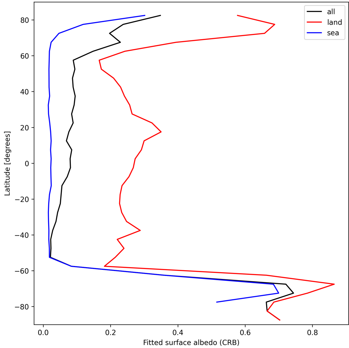
Figure 30: Zonal average of “Fitted surface albedo (CRB)” for 2025-10-06 to 2025-10-08.
