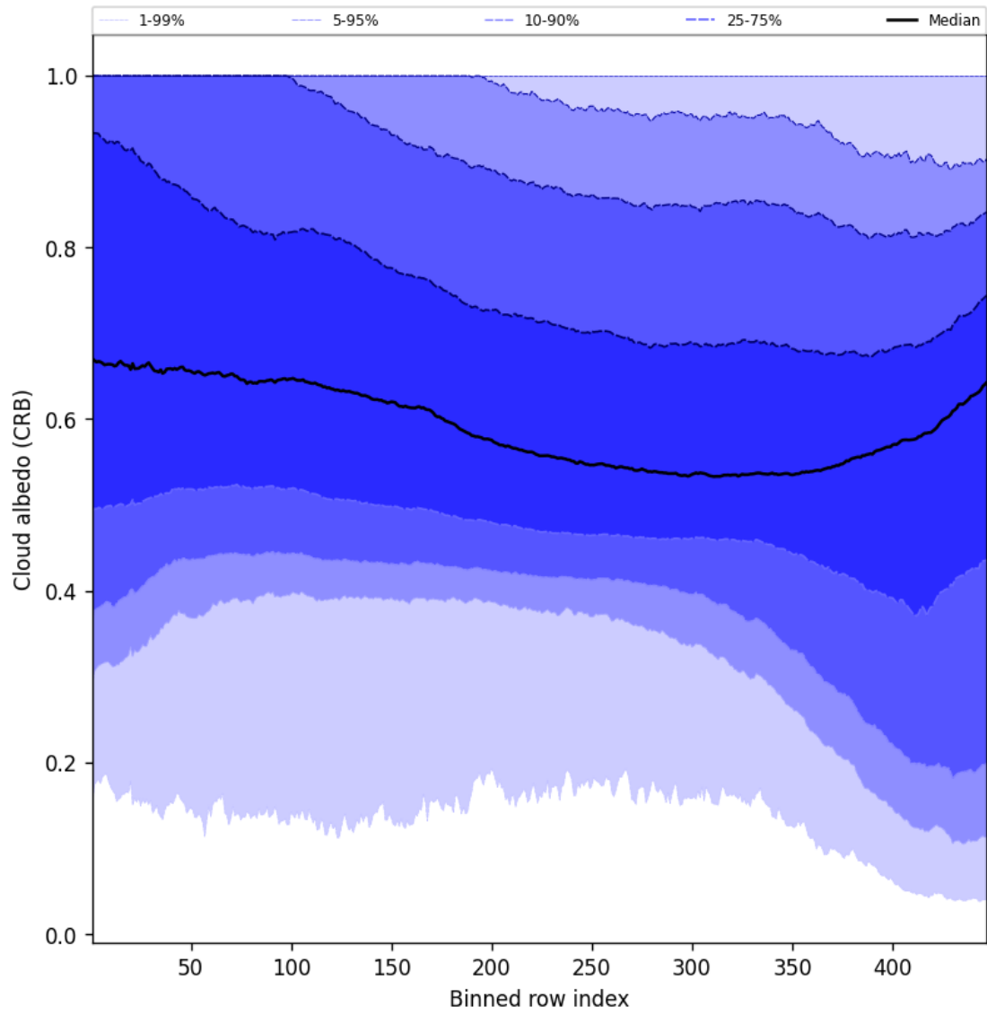
Figure 60: Along track statistics of “Cloud albedo (CRB)” for 2025-10-06 to 2025-10-08
