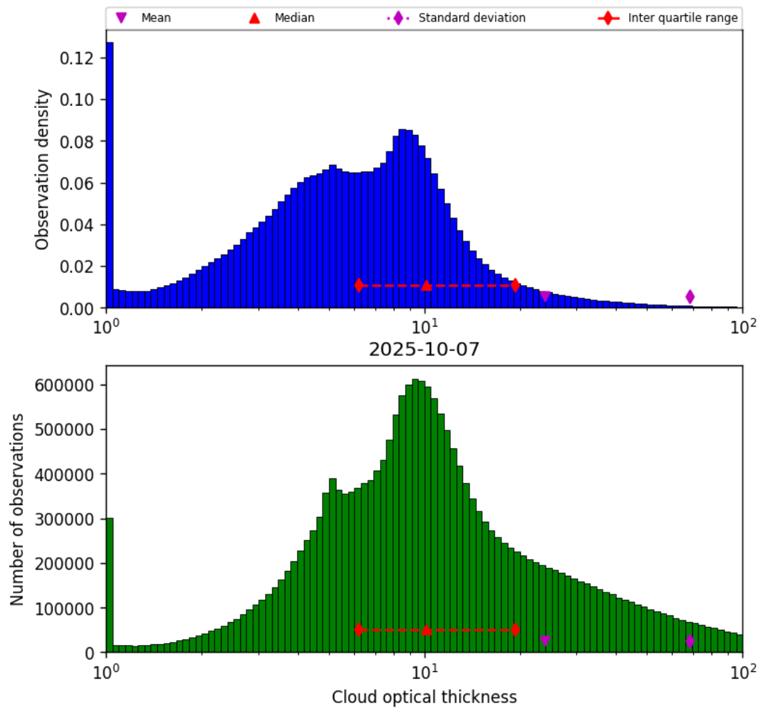
Figure 41: Histogram of “Cloud optical thickness” for 2025-10-06 to 2025-10-08
