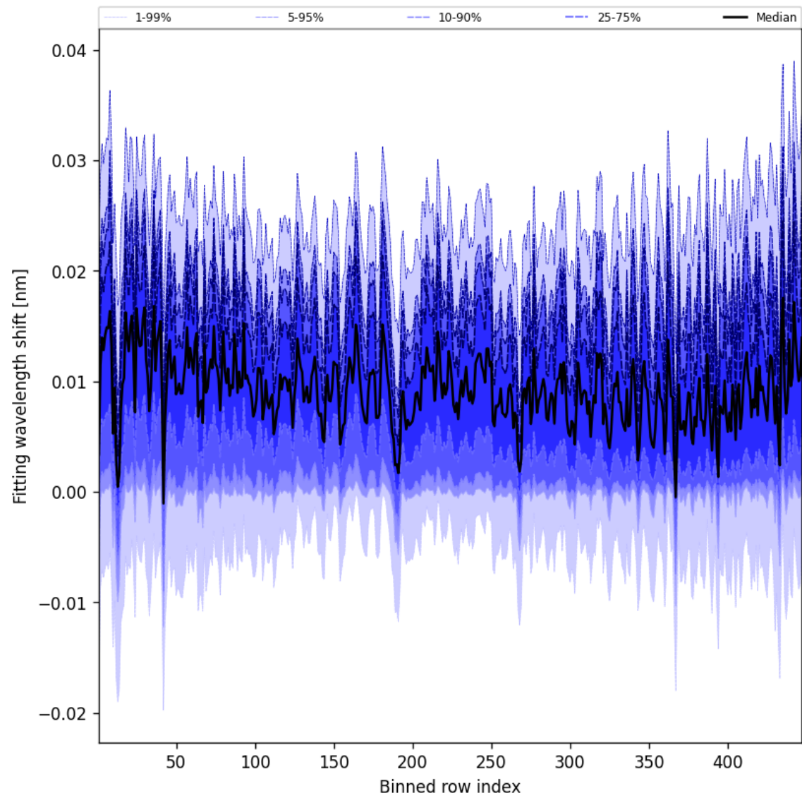
Figure 65: Along track statistics of “Fitting wavelength shift” for 2025-10-06 to 2025-10-08
