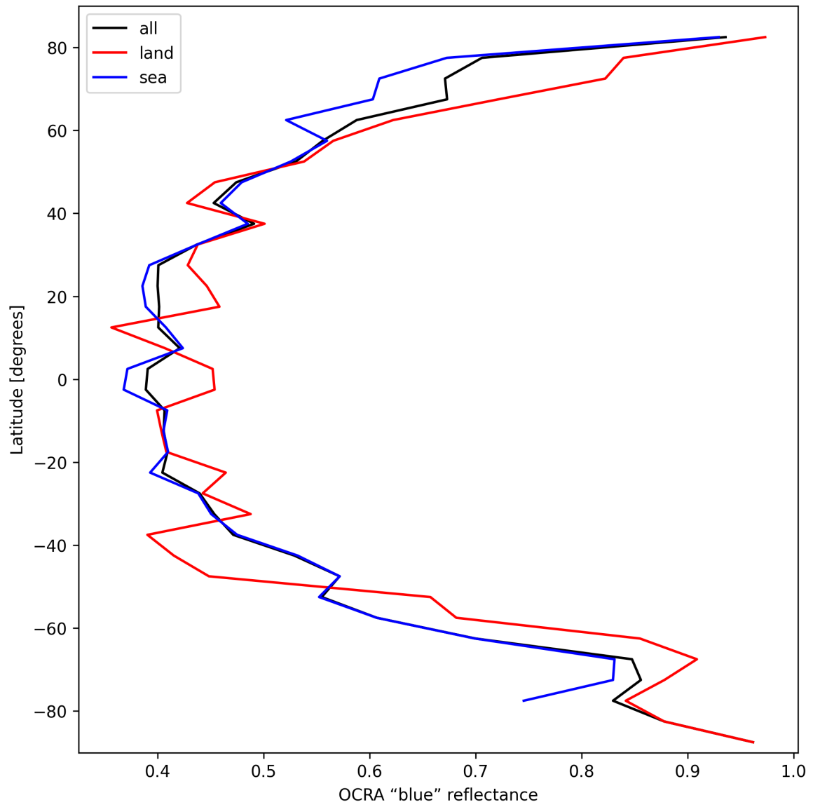
Figure 35: Zonal average of “OCRA “blue” reflectance” for 2025-10-06 to 2025-10-08.
