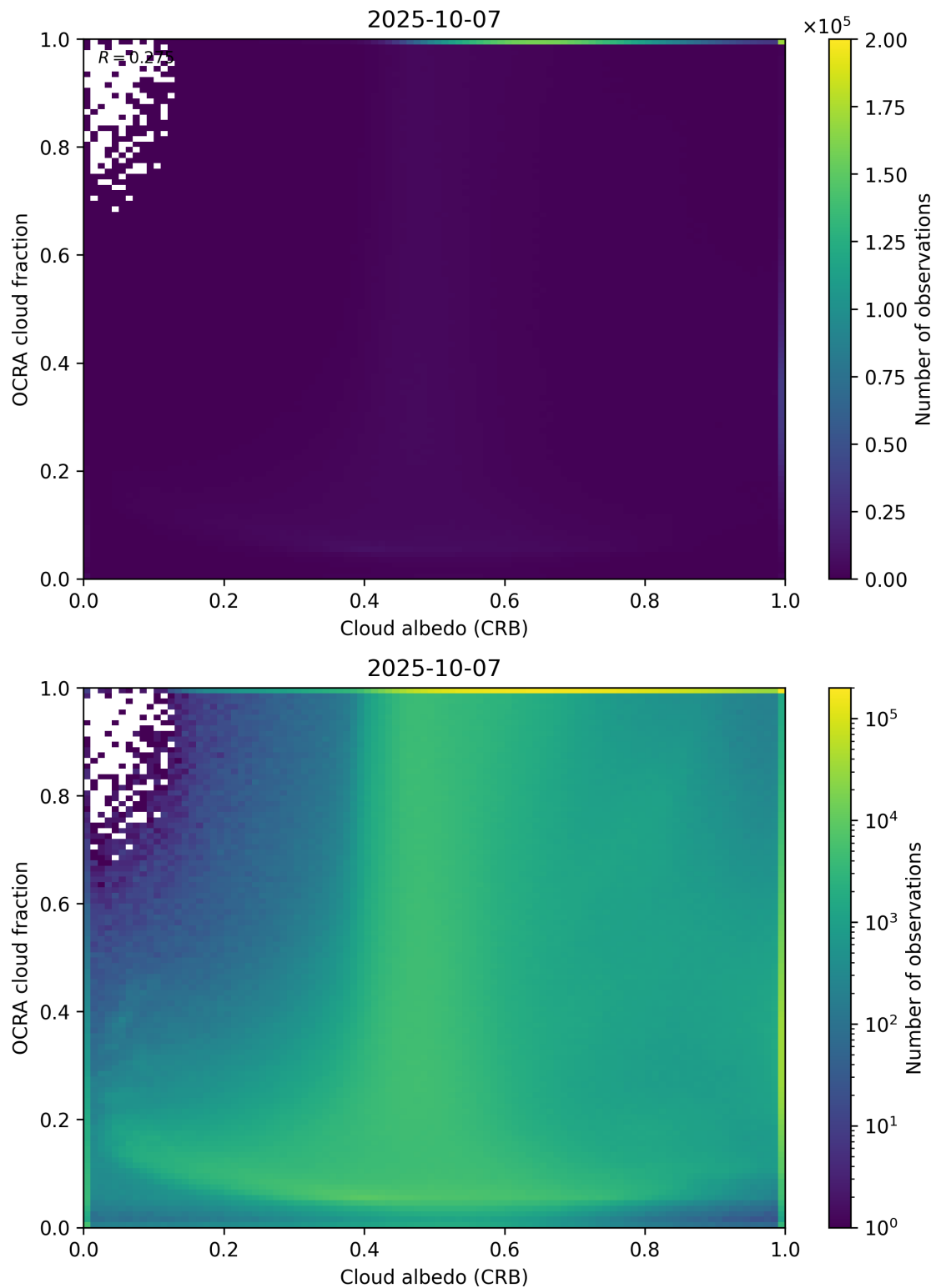
Figure 70: Scatter density plot of “Cloud albedo (CRB)” against “OCRA cloud fraction” for 2025-10-06 to 2025-10-08.
