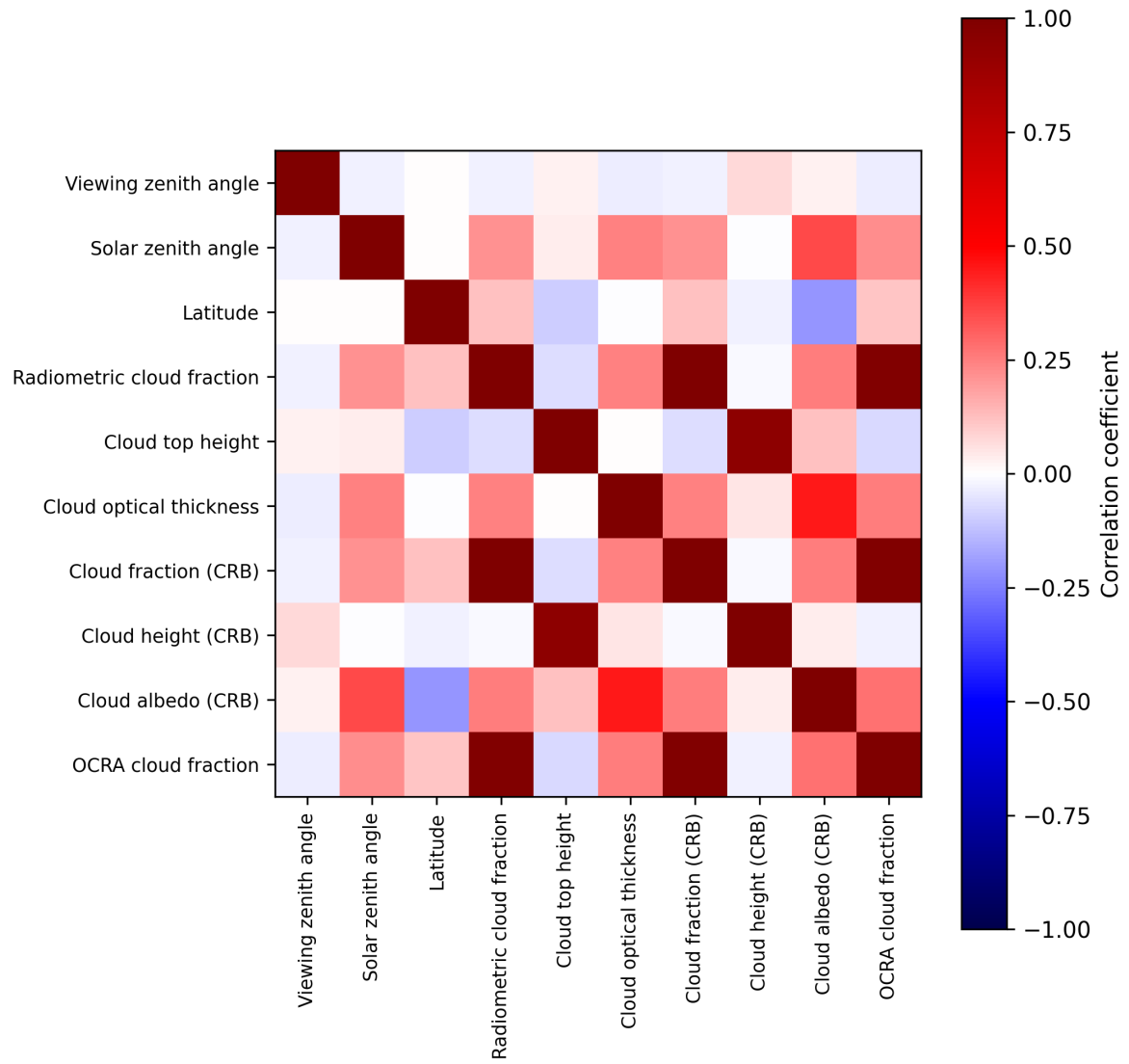
Figure 2: Map of correlation matrix for 2025-10-06 to 2025-10-08.
