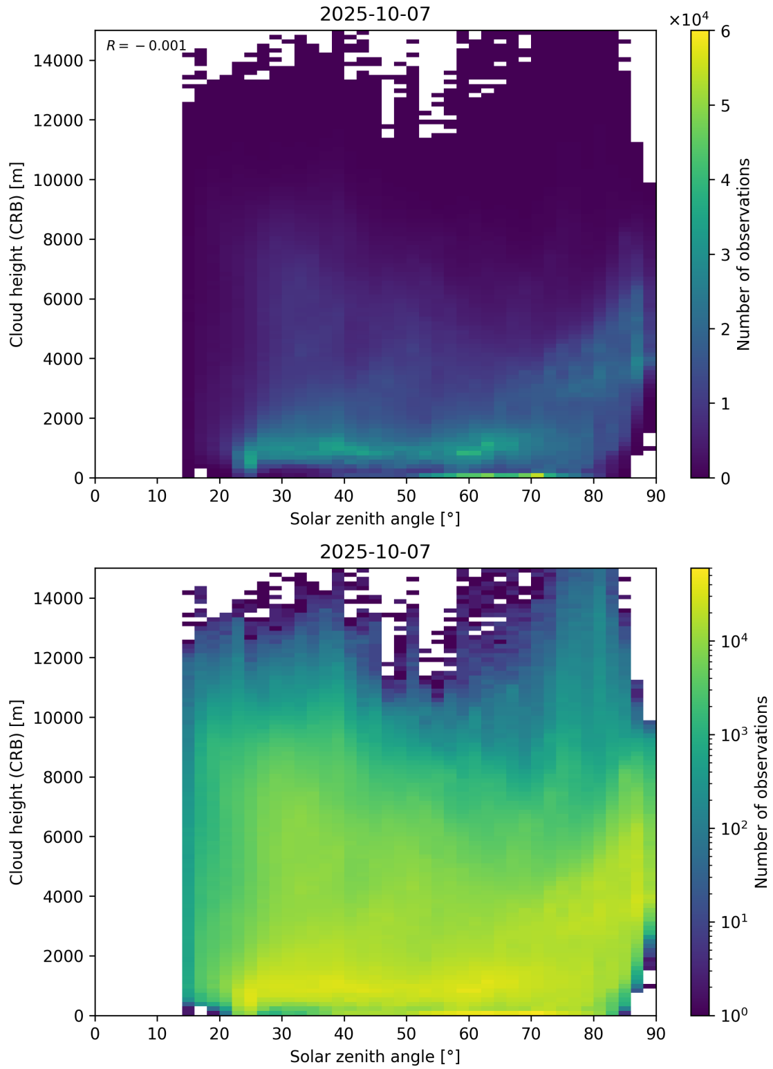
Figure 102: Scatter density plot of “Solar zenith angle” against “Cloud height (CRB)” for 2025-10-06 to 2025-10-08.
