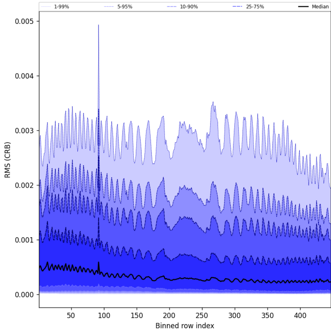
Figure 64: Along track statistics of “RMS (CRB)” for 2025-10-06 to 2025-10-08
