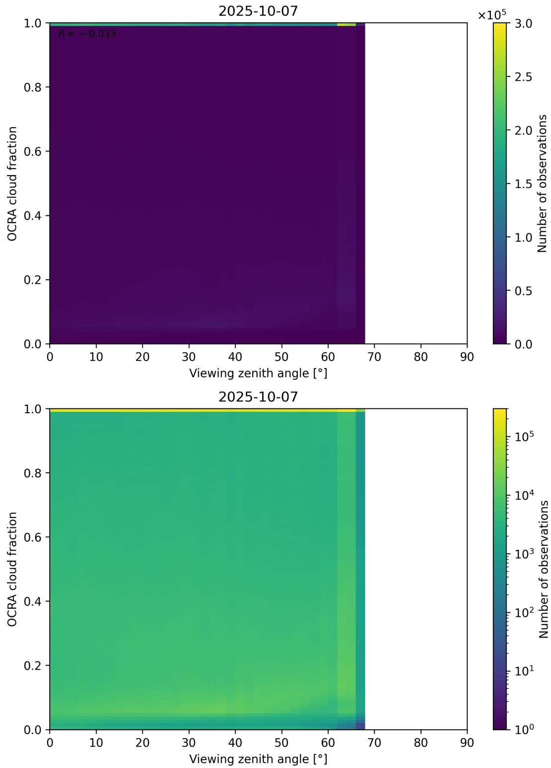
Figure 108: Scatter density plot of “Viewing zenith angle” against “OCRA cloud fraction” for 2025-10-06 to 2025-10-08.
