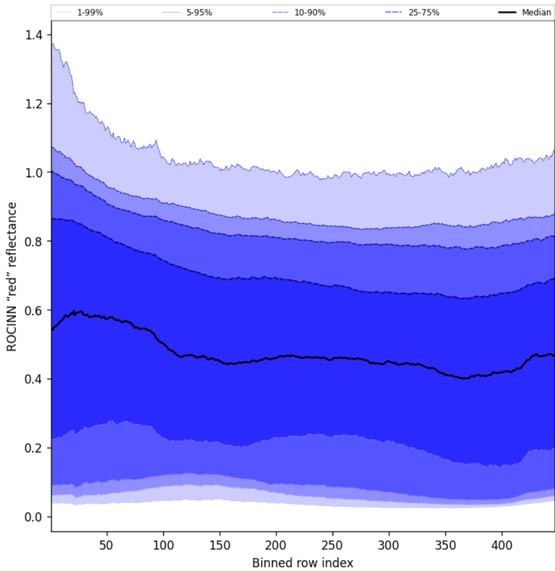
Figure 69: Along track statistics of “ROCINN “red” reflectance” for 2025-10-06 to 2025-10-08
