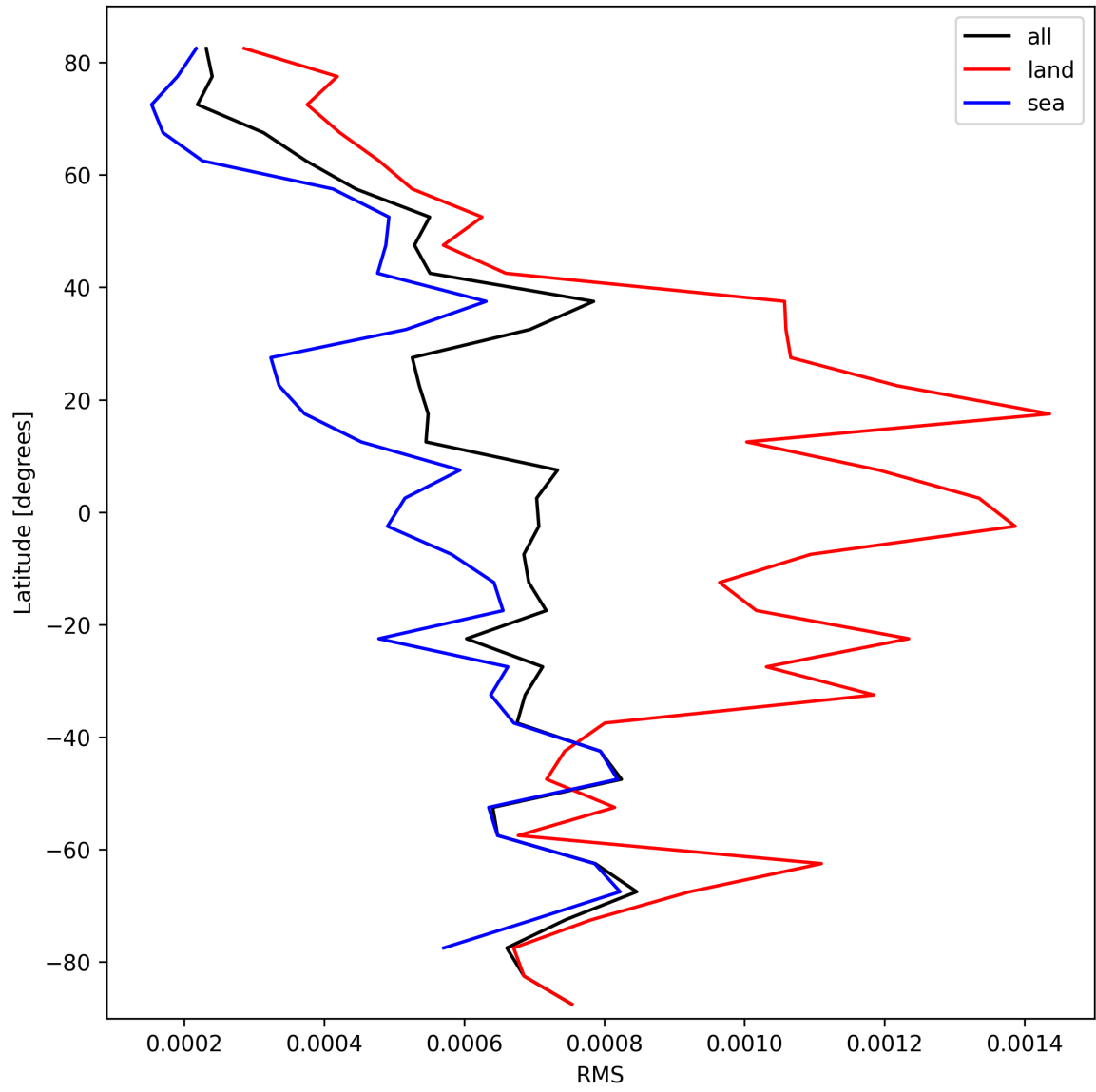
Figure 31: Zonal average of “RMS” for 2025-10-06 to 2025-10-08.
