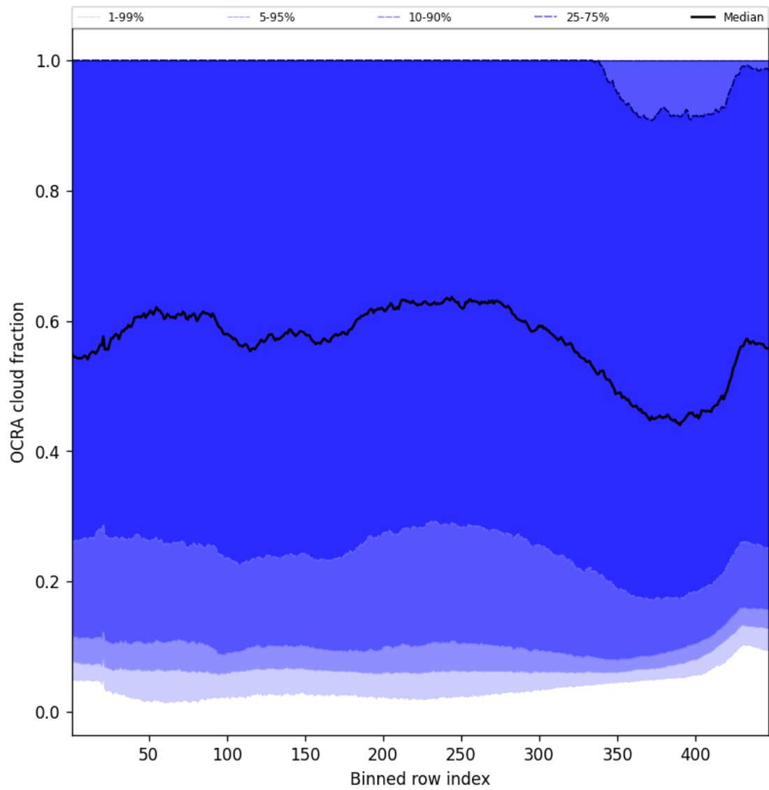
Figure 66: Along track statistics of “OCRA cloud fraction” for 2025-10-06 to 2025-10-08
