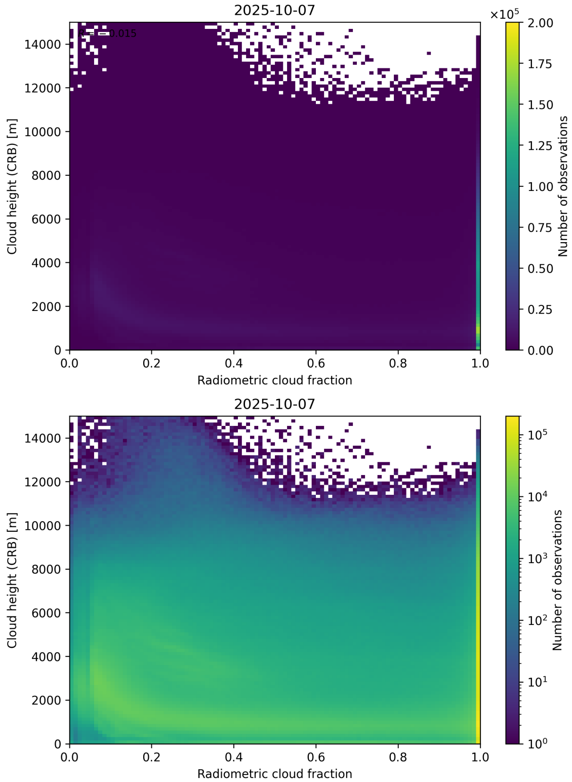
Figure 74: Scatter density plot of “Radiometric cloud fraction” against “Cloud height (CRB)” for 2025-10-06 to 2025-10-08.
