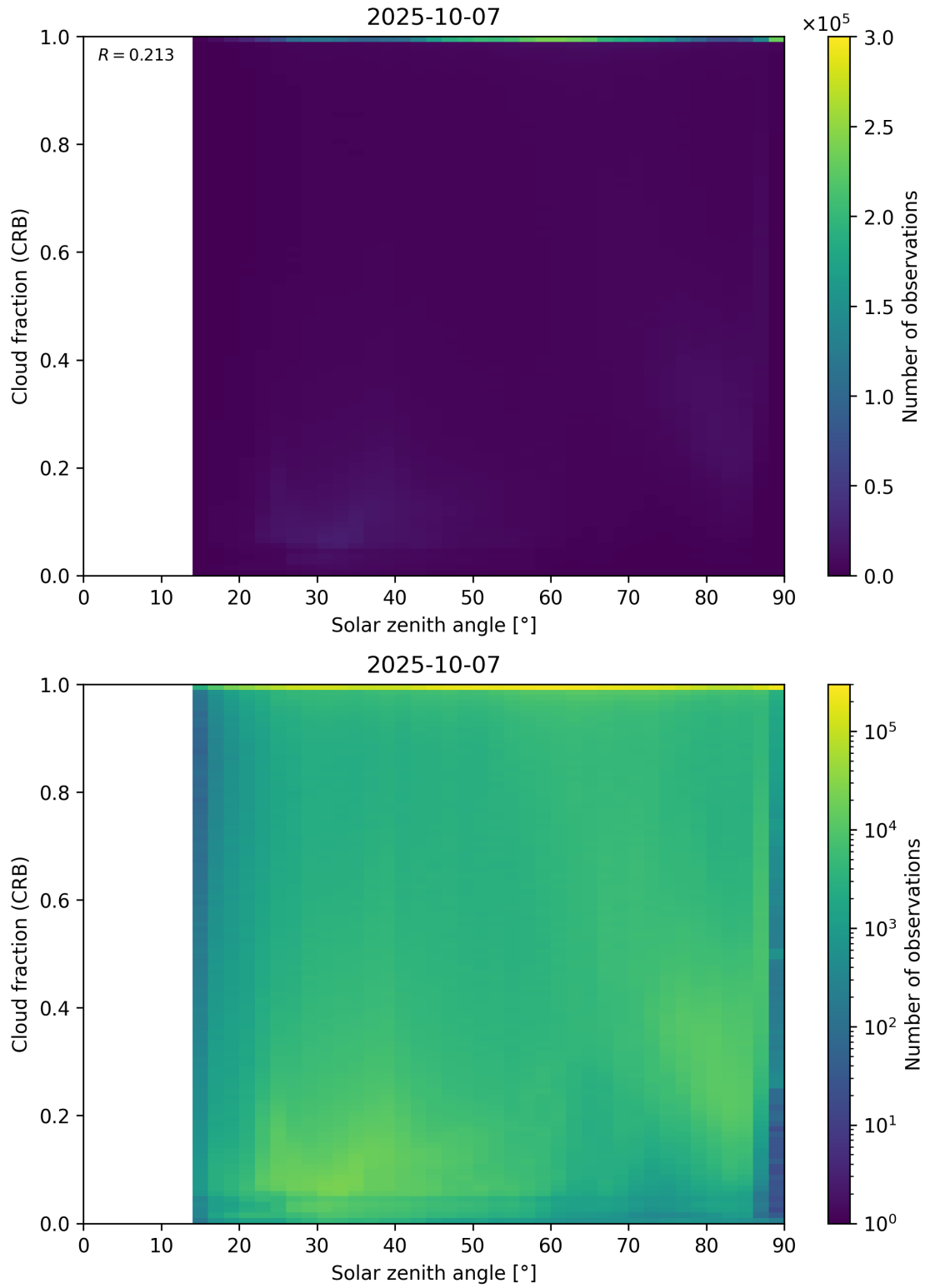
Figure 101: Scatter density plot of “Solar zenith angle” against “Cloud fraction (CRB)” for 2025-10-06 to 2025-10-08.
