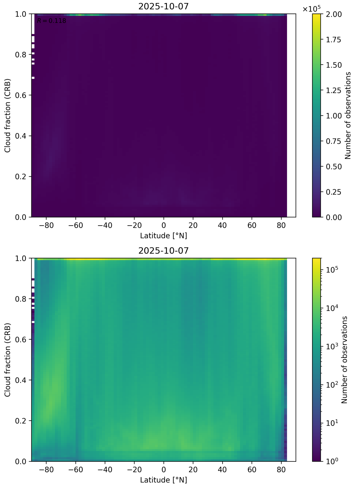
Figure 94: Scatter density plot of “Latitude” against “Cloud fraction (CRB)” for 2025-10-06 to 2025-10-08.
