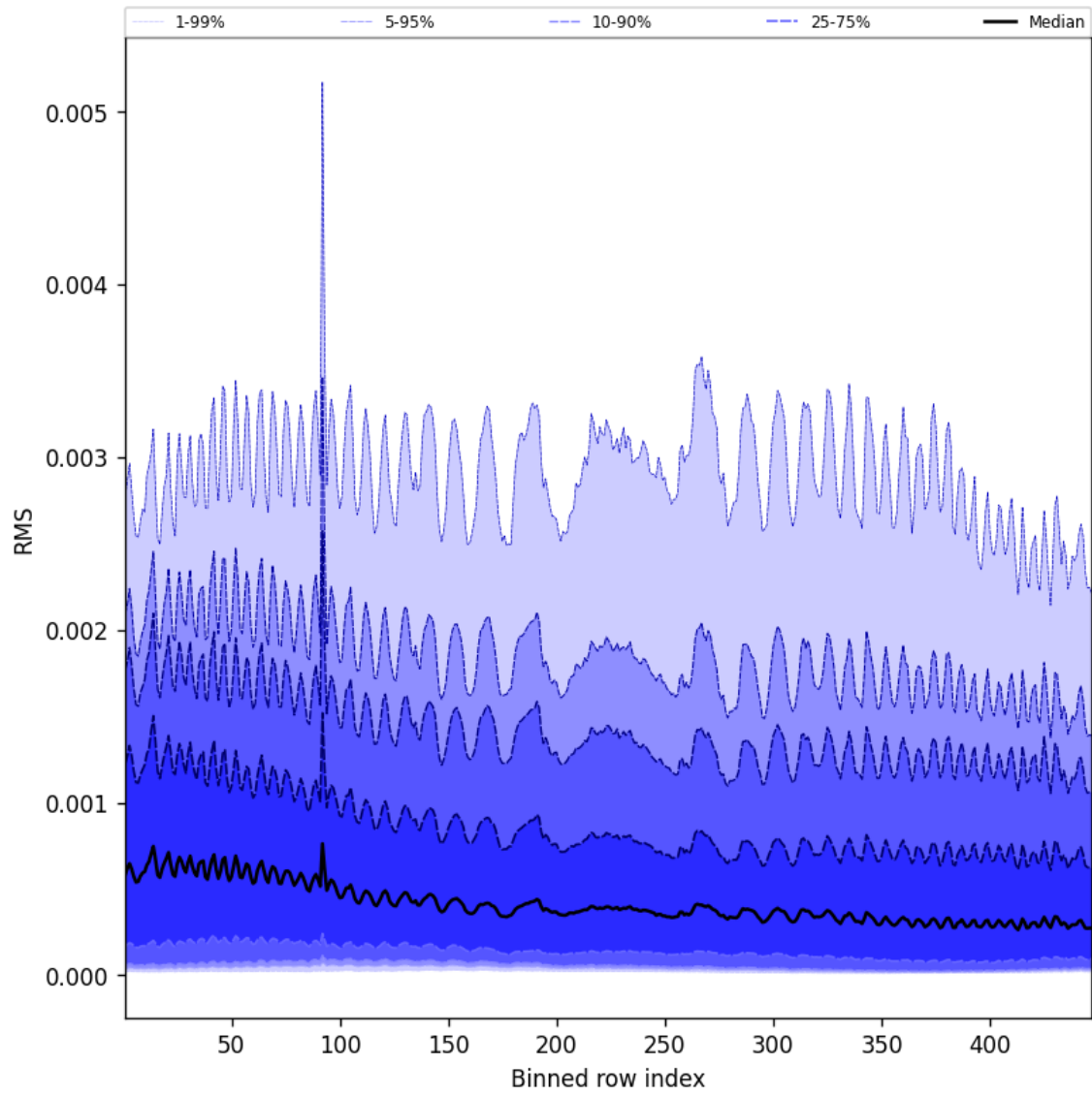
Figure 63: Along track statistics of “RMS” for 2025-10-06 to 2025-10-08
