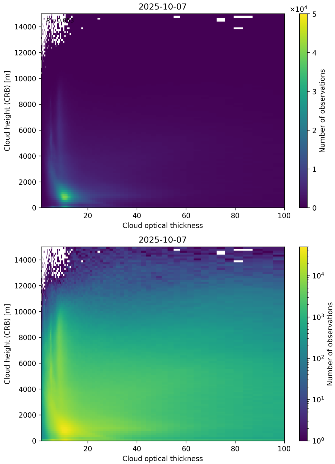
Figure 85: Scatter density plot of “Cloud optical thickness” against “Cloud height (CRB)” for 2025-10-06 to 2025-10-08.
