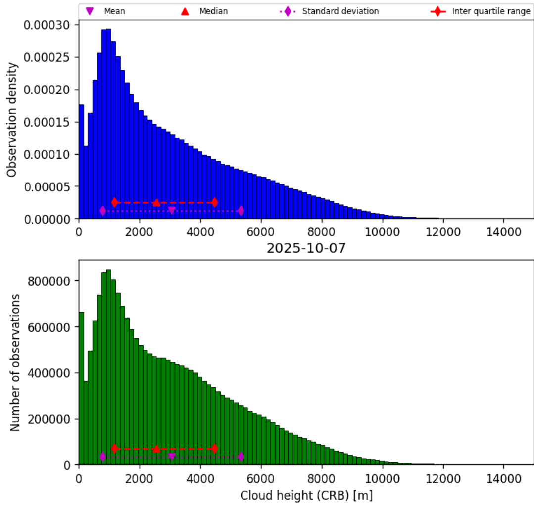
Figure 43: Histogram of “Cloud height (CRB)” for 2025-10-06 to 2025-10-08
