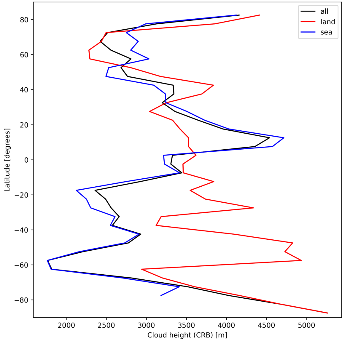
Figure 27: Zonal average of “Cloud height (CRB)” for 2025-10-06 to 2025-10-08.
