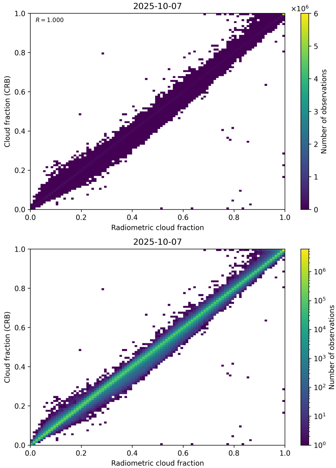
Figure 73: Scatter density plot of “Radiometric cloud fraction” against “Cloud fraction (CRB)” for 2025-10-06 to 2025-10-08.
