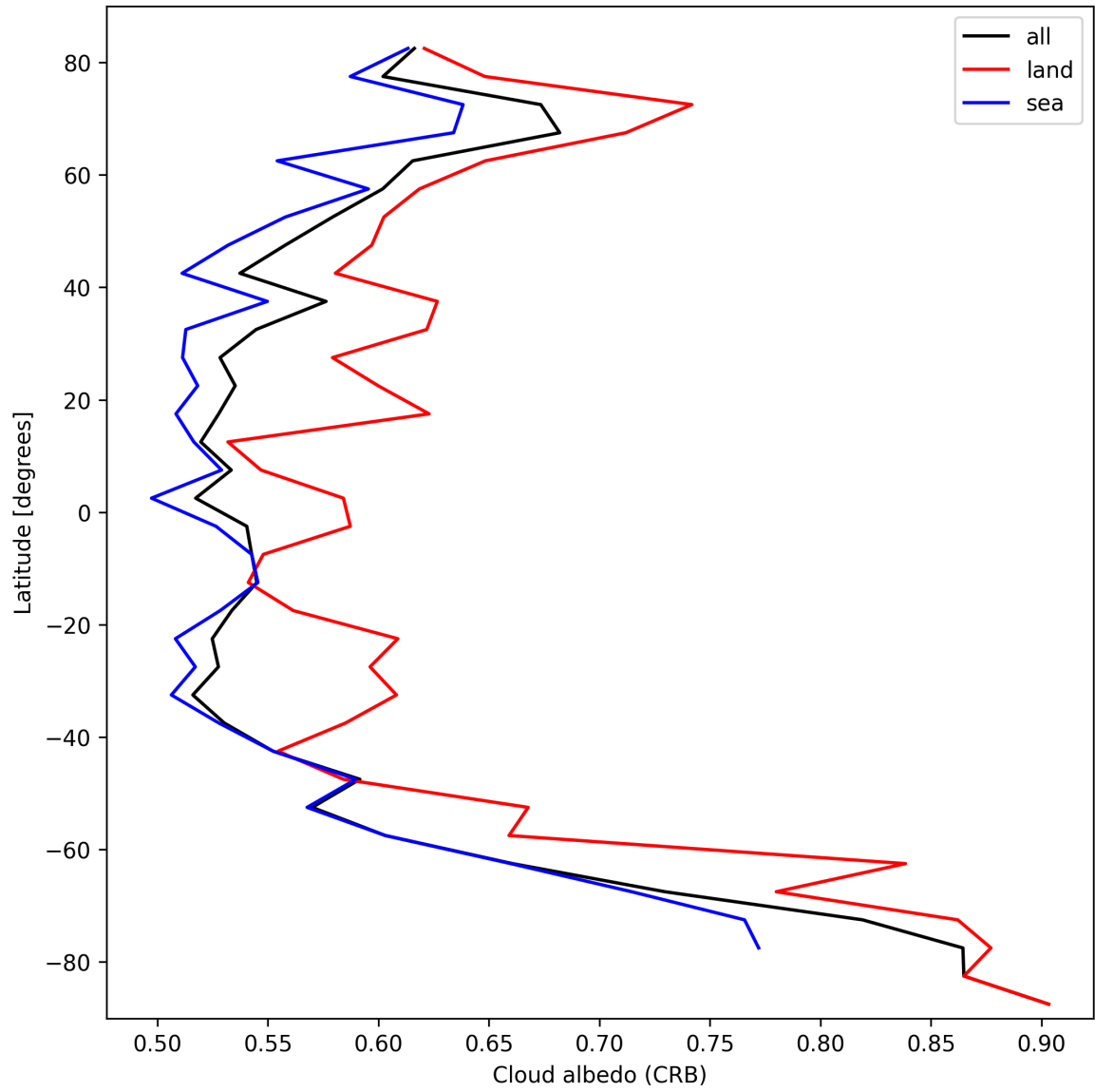
Figure 28: Zonal average of “Cloud albedo (CRB)” for 2025-10-06 to 2025-10-08.
