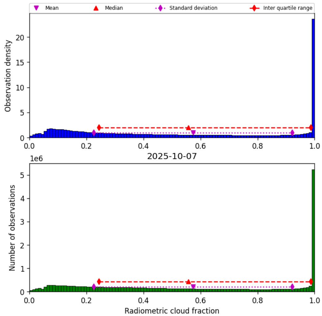
Figure 39: Histogram of “Radiometric cloud fraction” for 2025-10-06 to 2025-10-08
