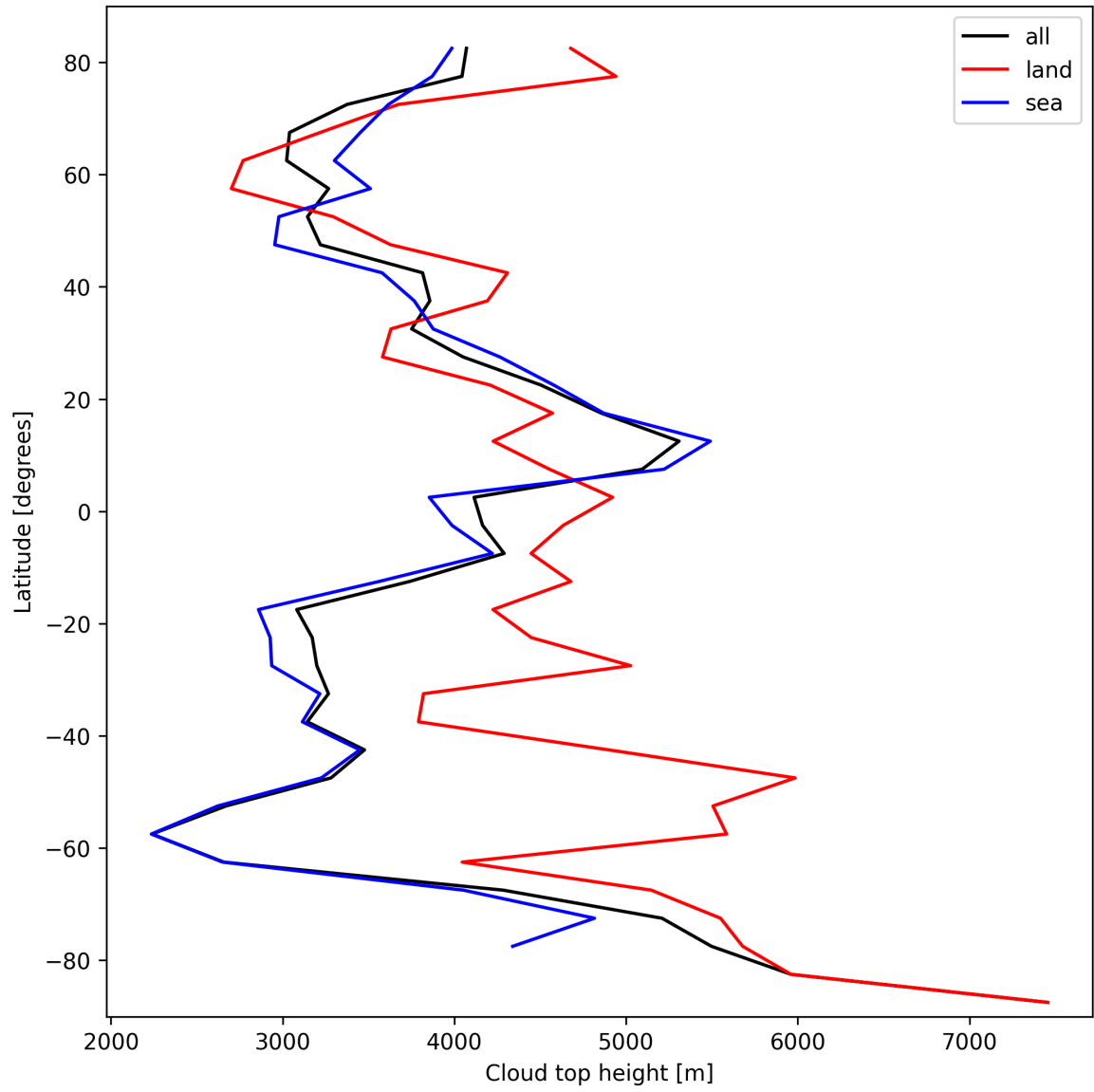
Figure 24: Zonal average of “Cloud top height” for 2025-10-06 to 2025-10-08.
