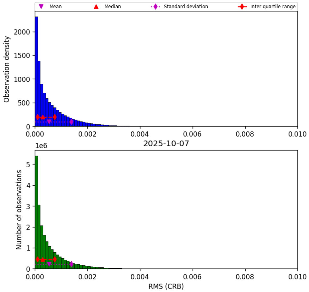
Figure 48: Histogram of “RMS (CRB)” for 2025-10-06 to 2025-10-08
