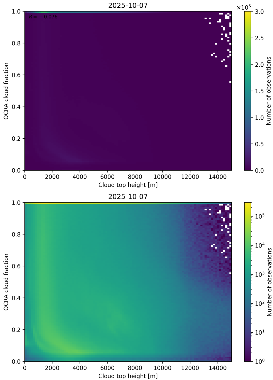
Figure 87: Scatter density plot of “Cloud top height” against “OCRA cloud fraction” for 2025-10-06 to 2025-10-08.
