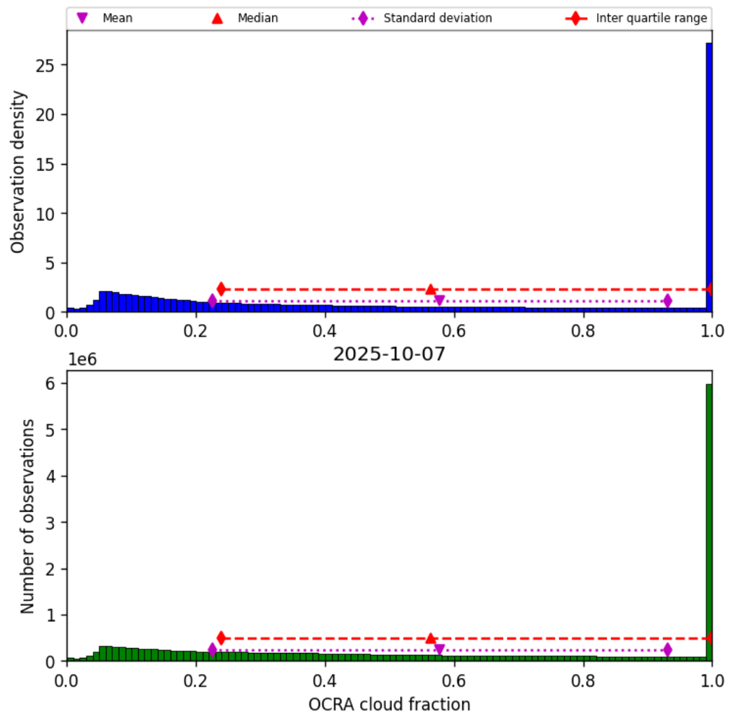
Figure 50: Histogram of “OCRA cloud fraction” for 2025-10-06 to 2025-10-08
