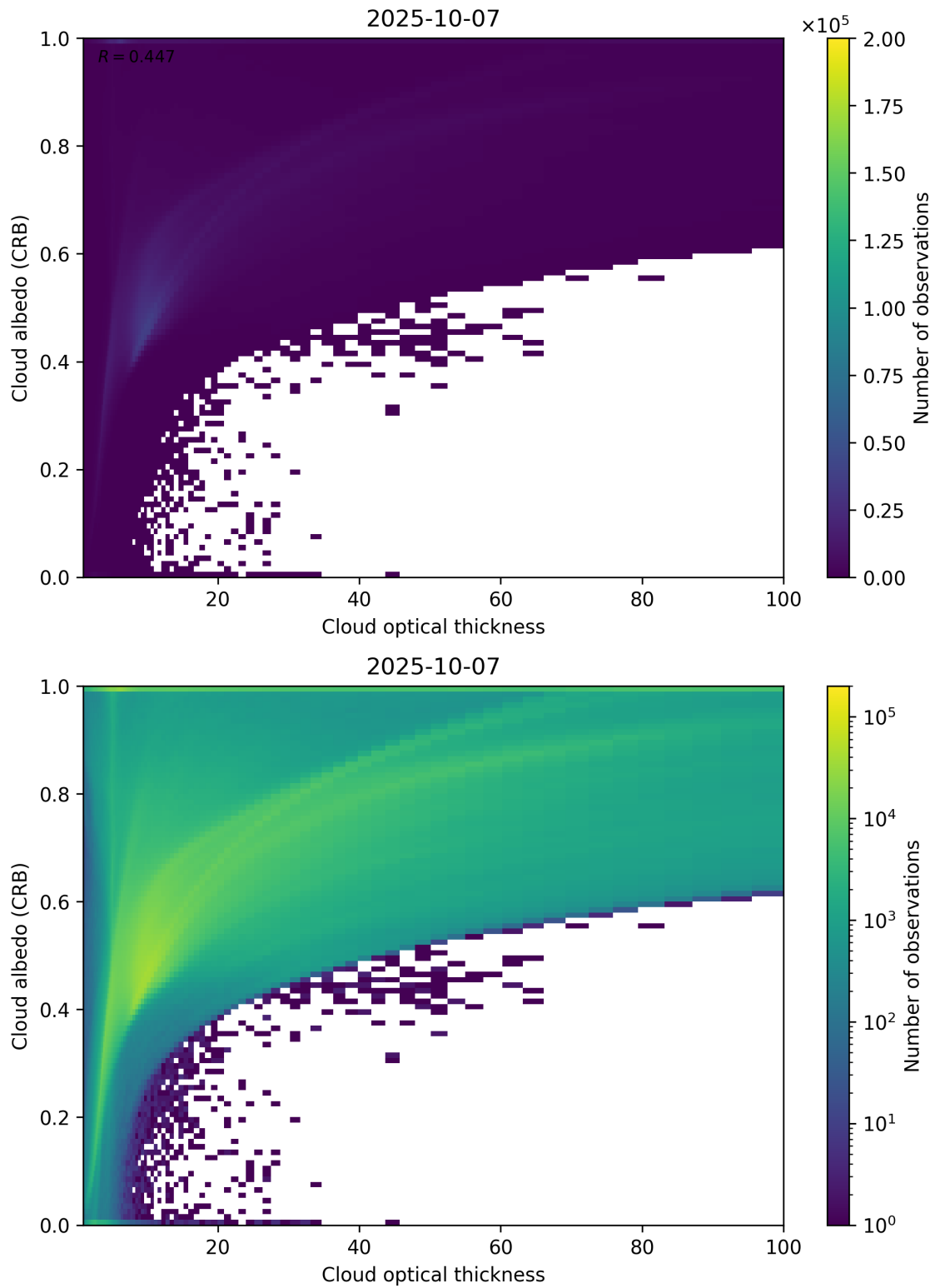
Figure 82: Scatter density plot of “Cloud optical thickness” against “Cloud albedo (CRB)” for 2025-10-06 to 2025-10-08.
