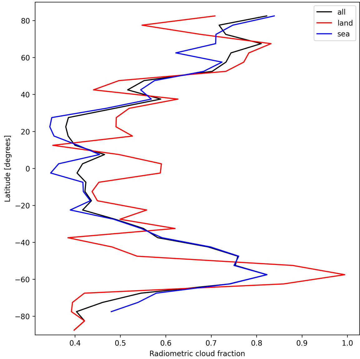
Figure 23: Zonal average of “Radiometric cloud fraction” for 2025-10-06 to 2025-10-08.
