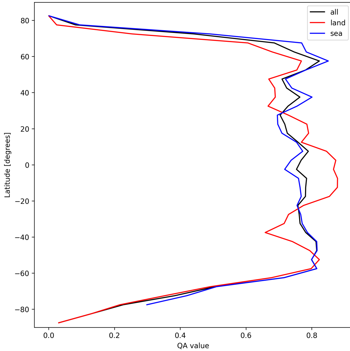
Figure 22: Zonal average of “QA value” for 2025-10-06 to 2025-10-08.
