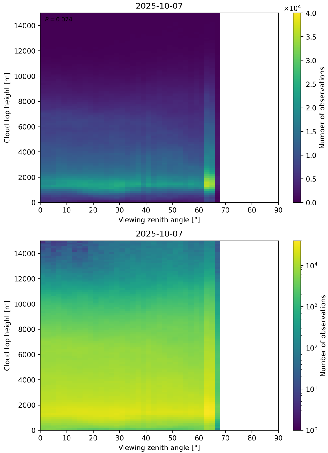
Figure 112: Scatter density plot of “Viewing zenith angle” against “Cloud top height” for 2025-10-06 to 2025-10-08.
