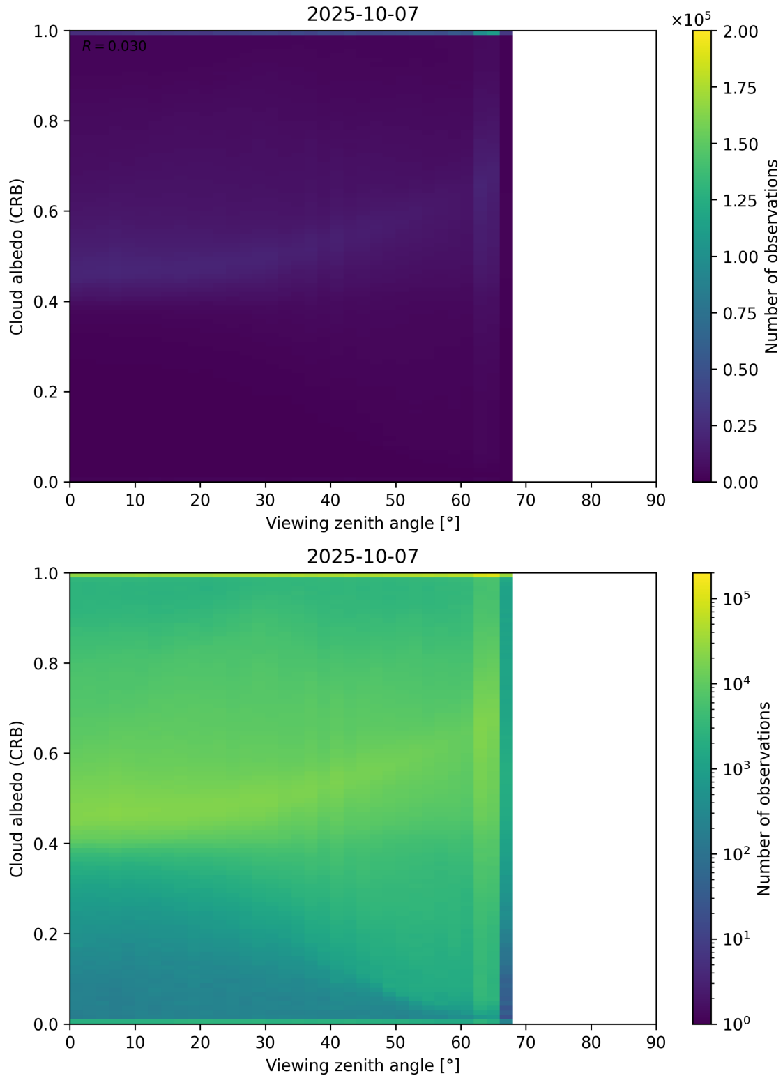
Figure 106: Scatter density plot of “Viewing zenith angle” against “Cloud albedo (CRB)” for 2025-10-06 to 2025-10-08.
