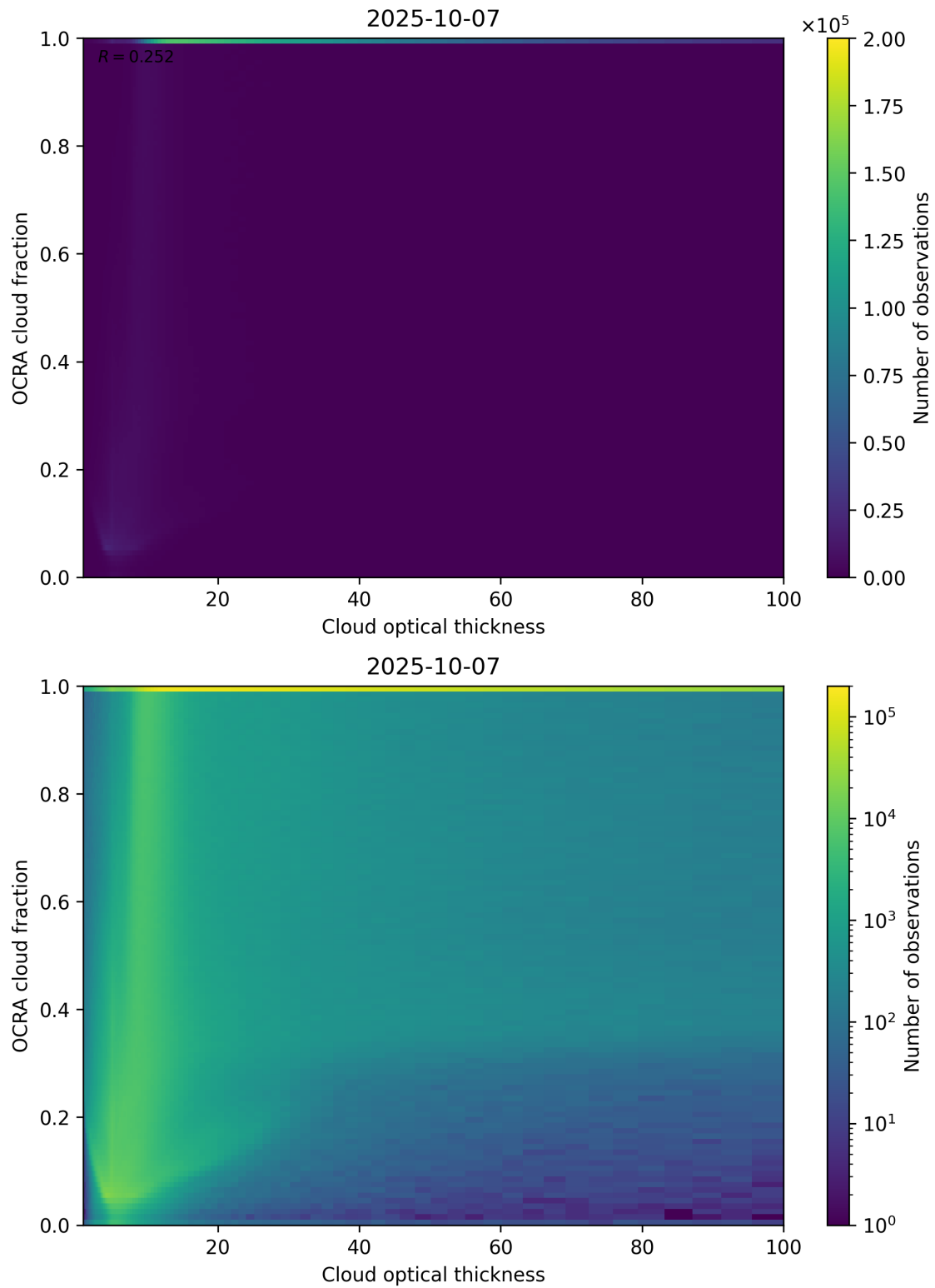
Figure 83: Scatter density plot of “Cloud optical thickness” against “OCRA cloud fraction” for 2025-10-06 to 2025-10-08.
