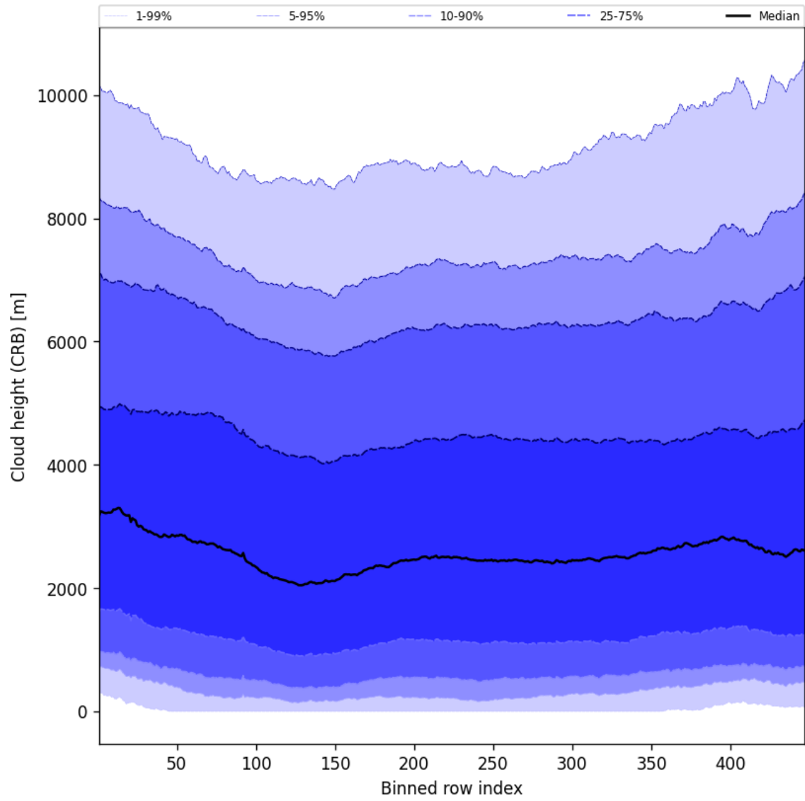
Figure 59: Along track statistics of “Cloud height (CRB)” for 2025-10-06 to 2025-10-08
