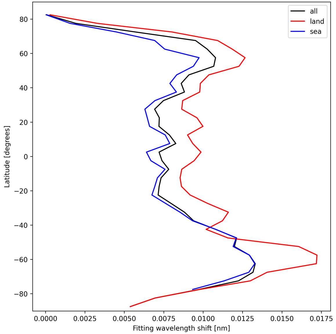
Figure 33: Zonal average of “Fitting wavelength shift” for 2025-10-06 to 2025-10-08.
