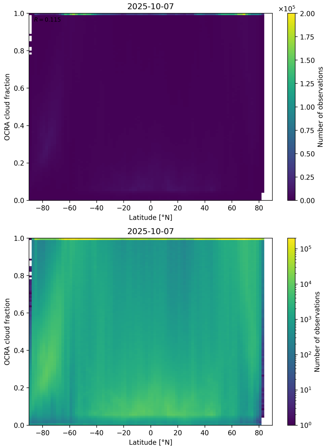
Figure 93: Scatter density plot of “Latitude” against “OCRA cloud fraction” for 2025-10-06 to 2025-10-08.
