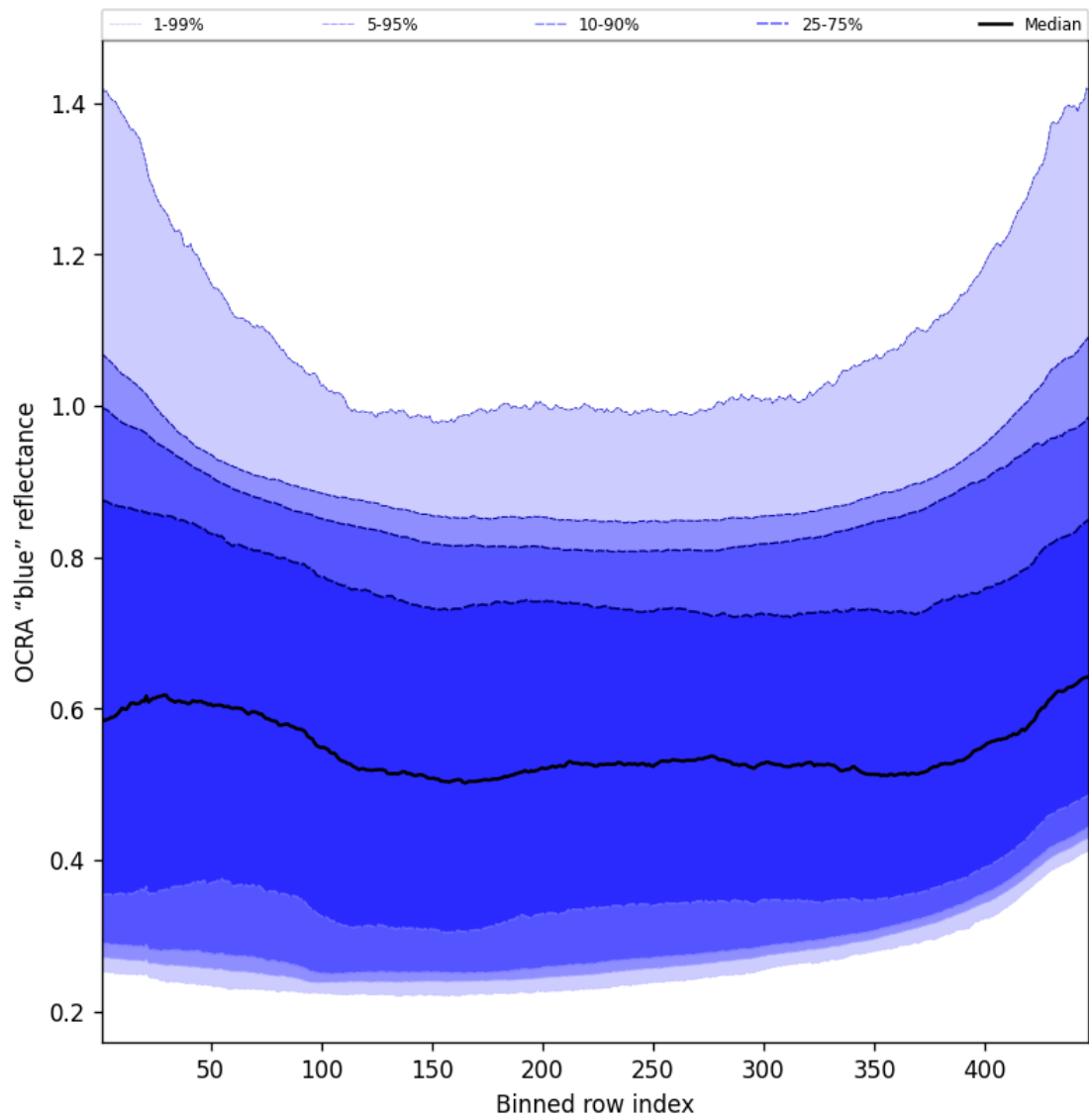
Figure 67: Along track statistics of “OCRA “blue” reflectance” for 2025-10-06 to 2025-10-08
