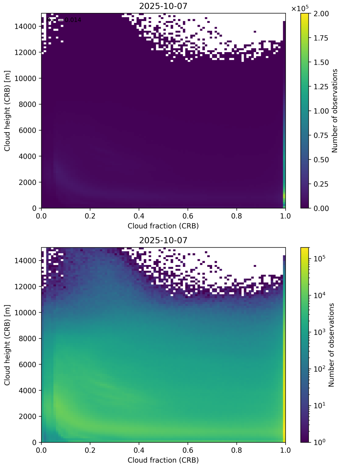
Figure 79: Scatter density plot of “Cloud fraction (CRB)” against “Cloud height (CRB)” for 2025-10-06 to 2025-10-08.
