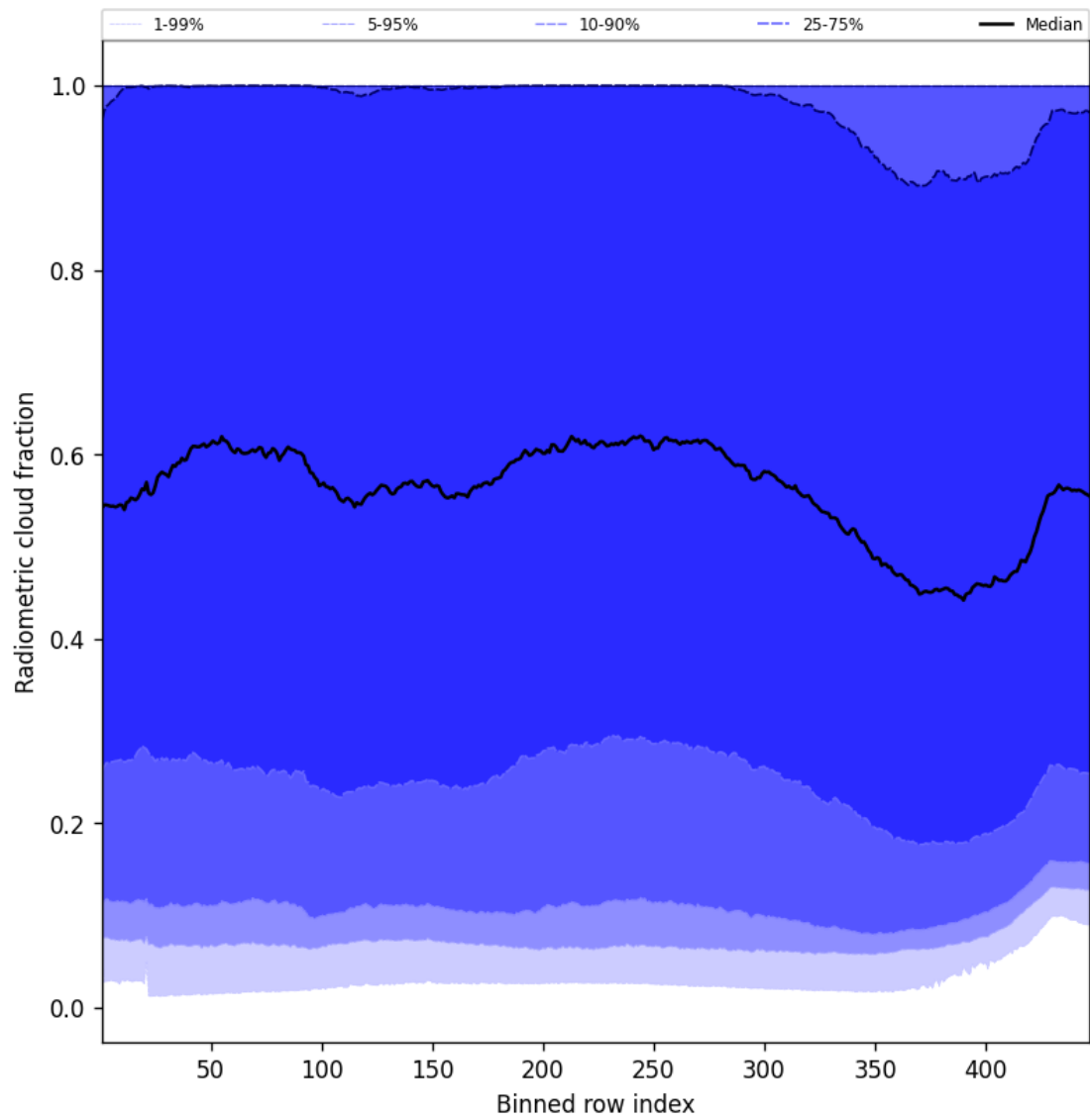
Figure 55: Along track statistics of “Radiometric cloud fraction” for 2025-10-06 to 2025-10-08
