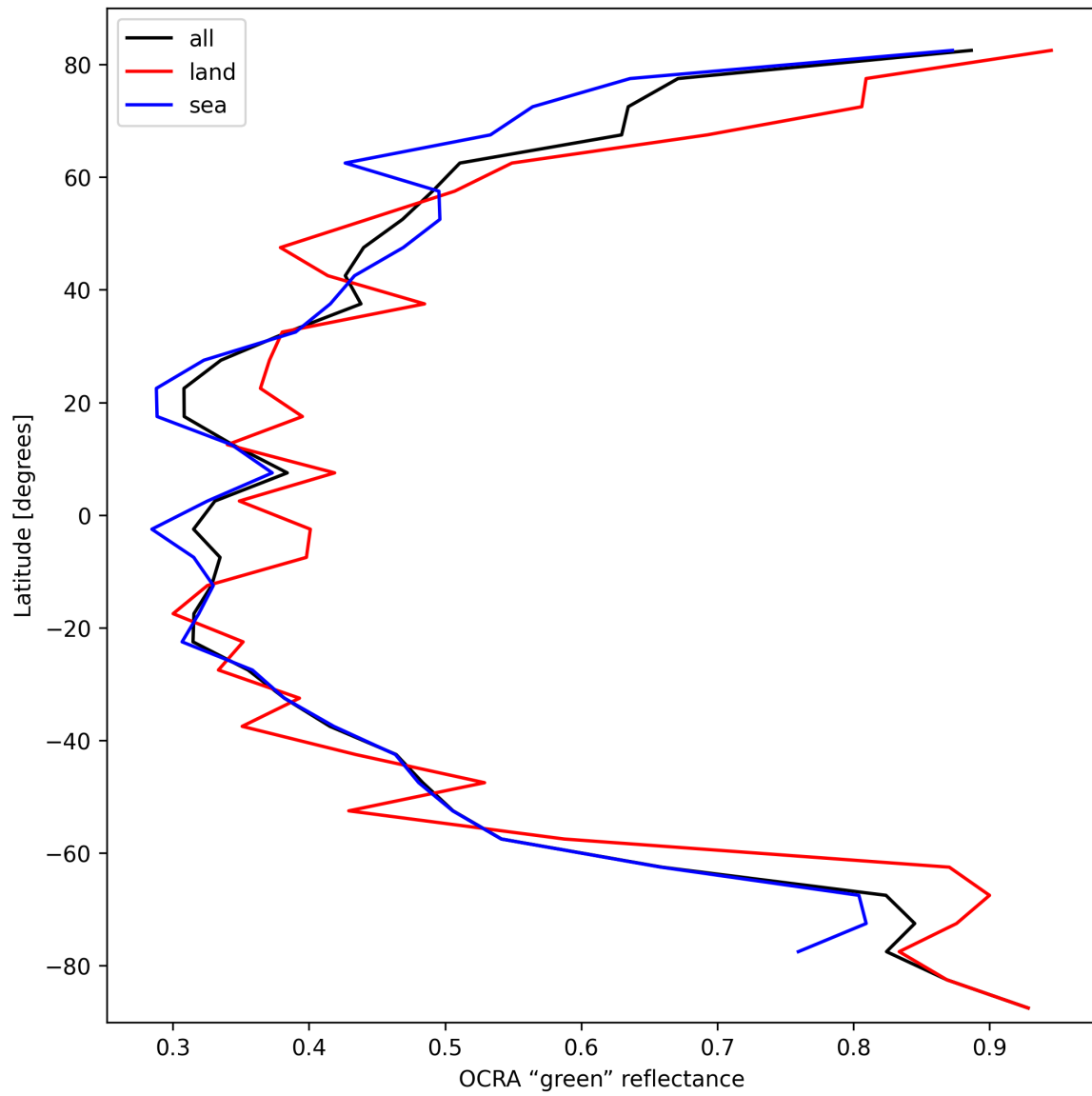
Figure 36: Zonal average of “OCRA “green” reflectance” for 2025-10-07 to 2025-10-09.
