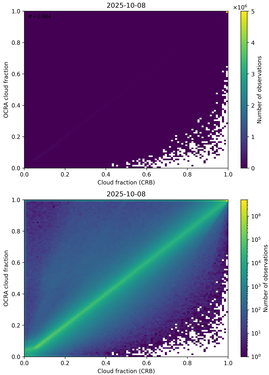
Figure 78: Scatter density plot of “Cloud fraction (CRB)” against “OCRA cloud fraction” for 2025-10-07 to 2025-10-09.
