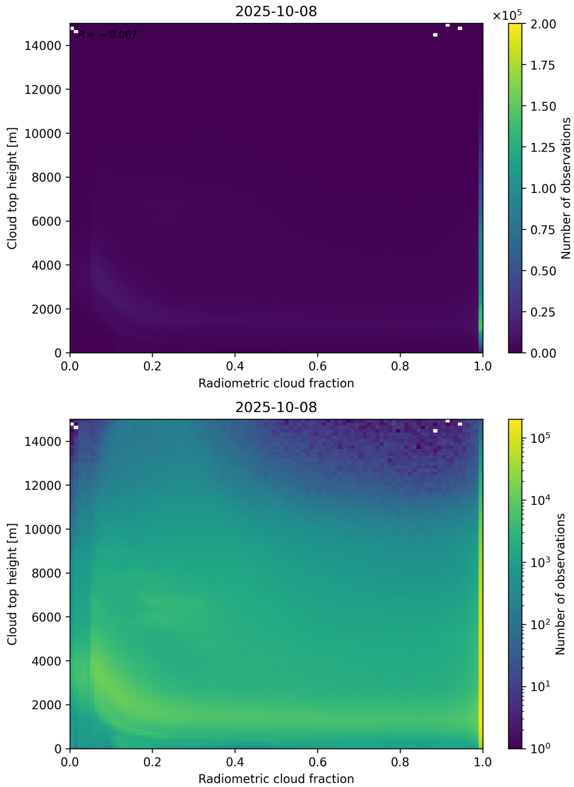
Figure 76: Scatter density plot of “Radiometric cloud fraction” against “Cloud top height” for 2025-10-07 to 2025-10-09.
