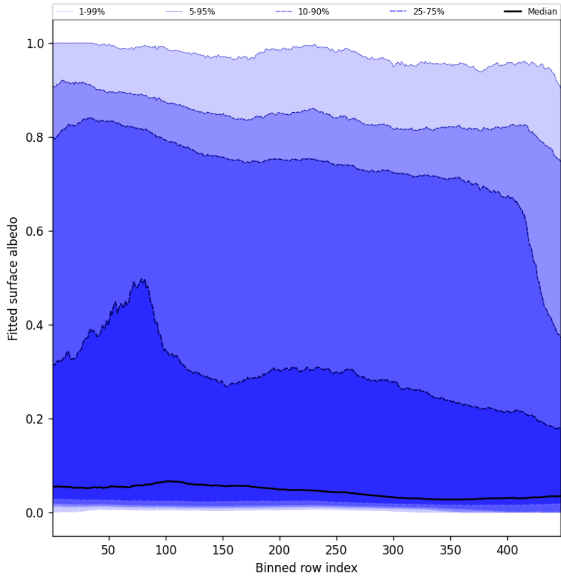
Figure 61: Along track statistics of "Fitted surface albedo" for 2025-10-07 to 2025-10-09
