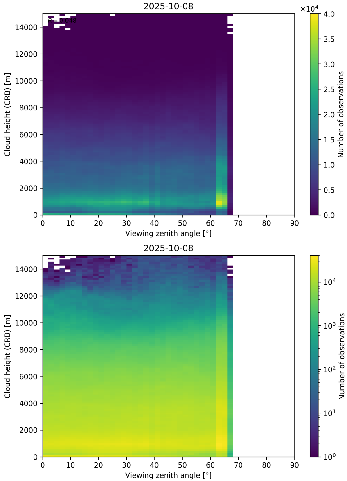
Figure 110: Scatter density plot of “Viewing zenith angle” against “Cloud height (CRB)” for 2025-10-07 to 2025-10-09.
