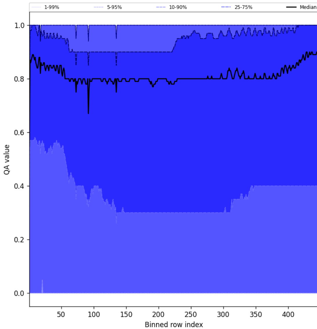
Figure 54: Along track statistics of “QA value” for 2025-10-07 to 2025-10-09
