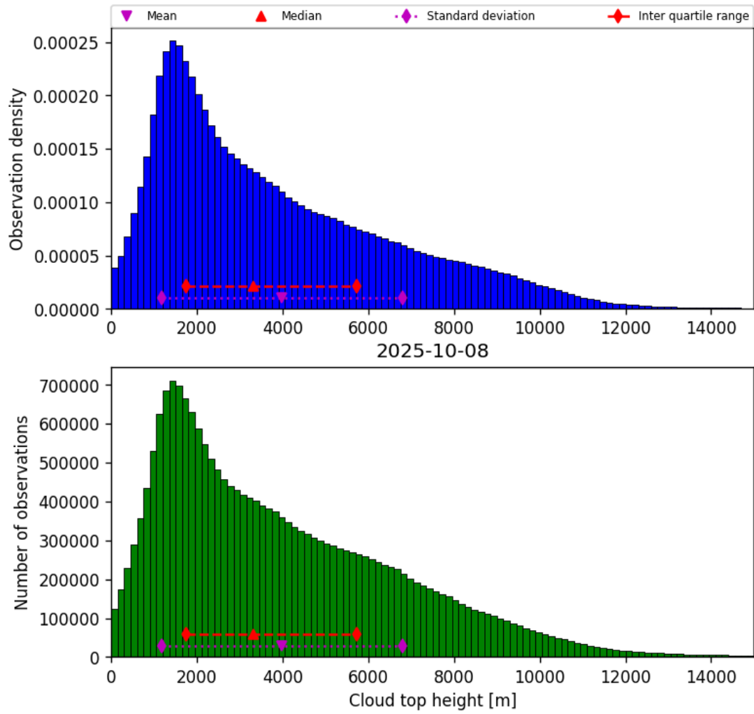
Figure 40: Histogram of “Cloud top height” for 2025-10-07 to 2025-10-09
