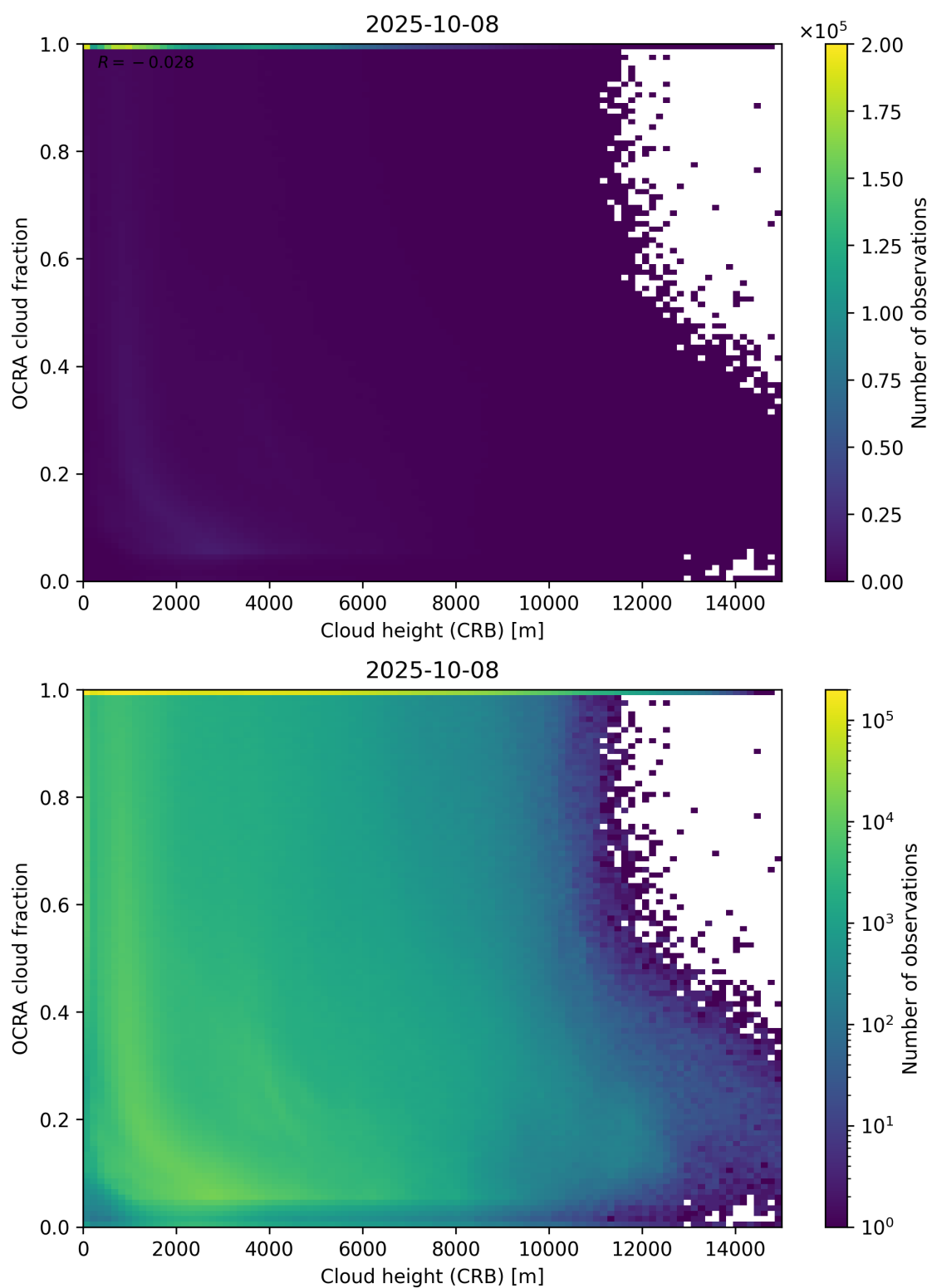
Figure 81: Scatter density plot of “Cloud height (CRB)” against “OCRA cloud fraction” for 2025-10-07 to 2025-10-09.
