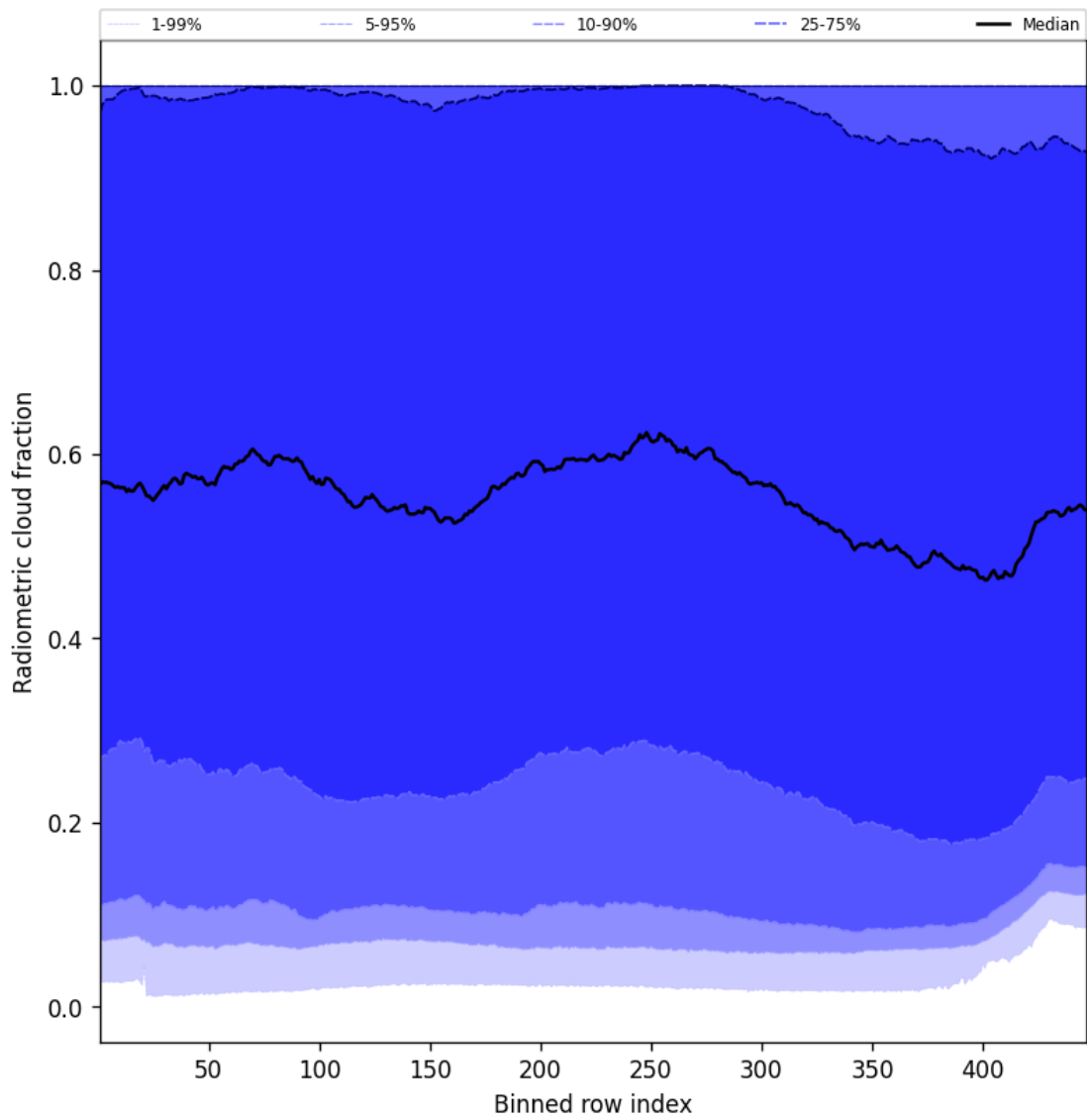
Figure 55: Along track statistics of “Radiometric cloud fraction” for 2025-10-07 to 2025-10-09
