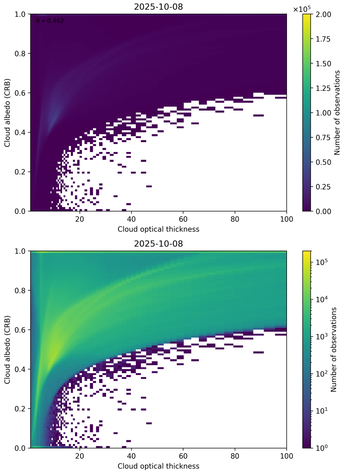
Figure 82: Scatter density plot of “Cloud optical thickness” against “Cloud albedo (CRB)” for 2025-10-07 to 2025-10-09.
