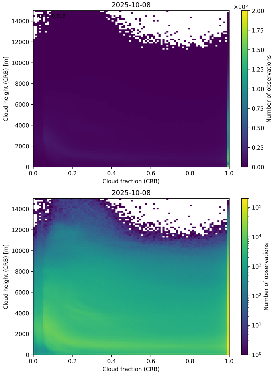
Figure 79: Scatter density plot of “Cloud fraction (CRB)” against “Cloud height (CRB)” for 2025-10-07 to 2025-10-09.
