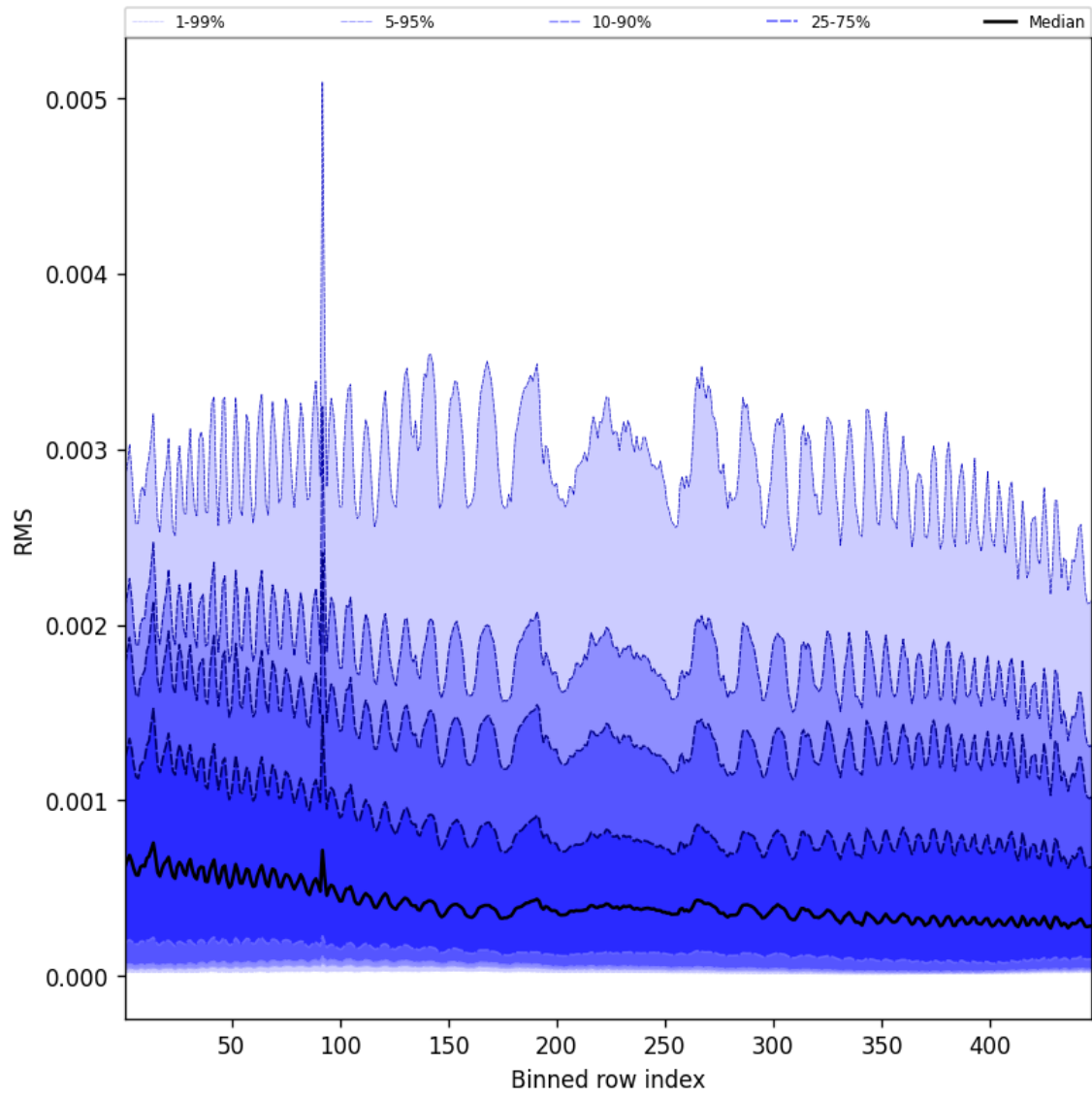
Figure 63: Along track statistics of “RMS” for 2025-10-07 to 2025-10-09
