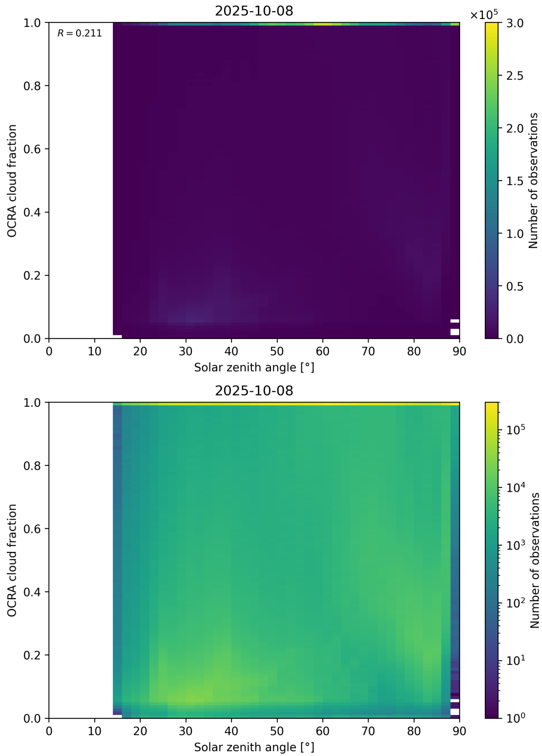
Figure 100: Scatter density plot of “Solar zenith angle” against “OCRA cloud fraction” for 2025-10-07 to 2025-10-09.
