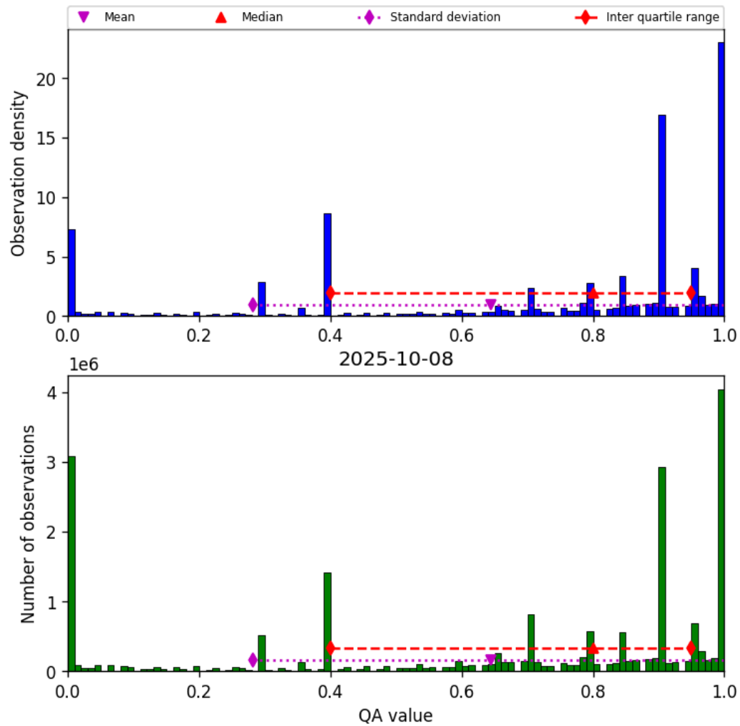
Figure 38: Histogram of “QA value” for 2025-10-07 to 2025-10-09
