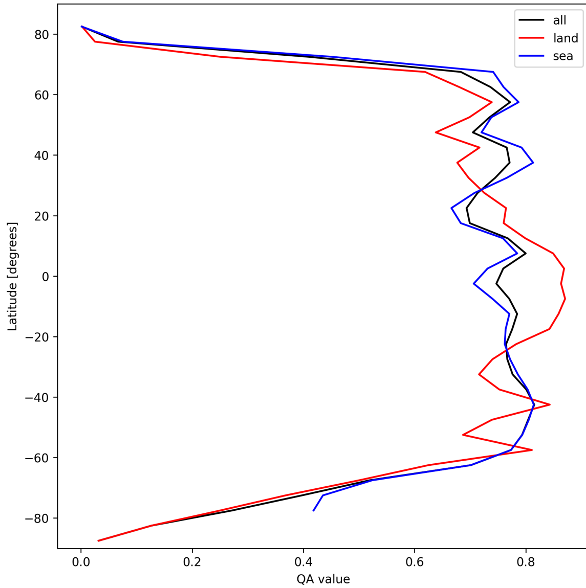
Figure 22: Zonal average of “QA value” for 2025-10-07 to 2025-10-09.
