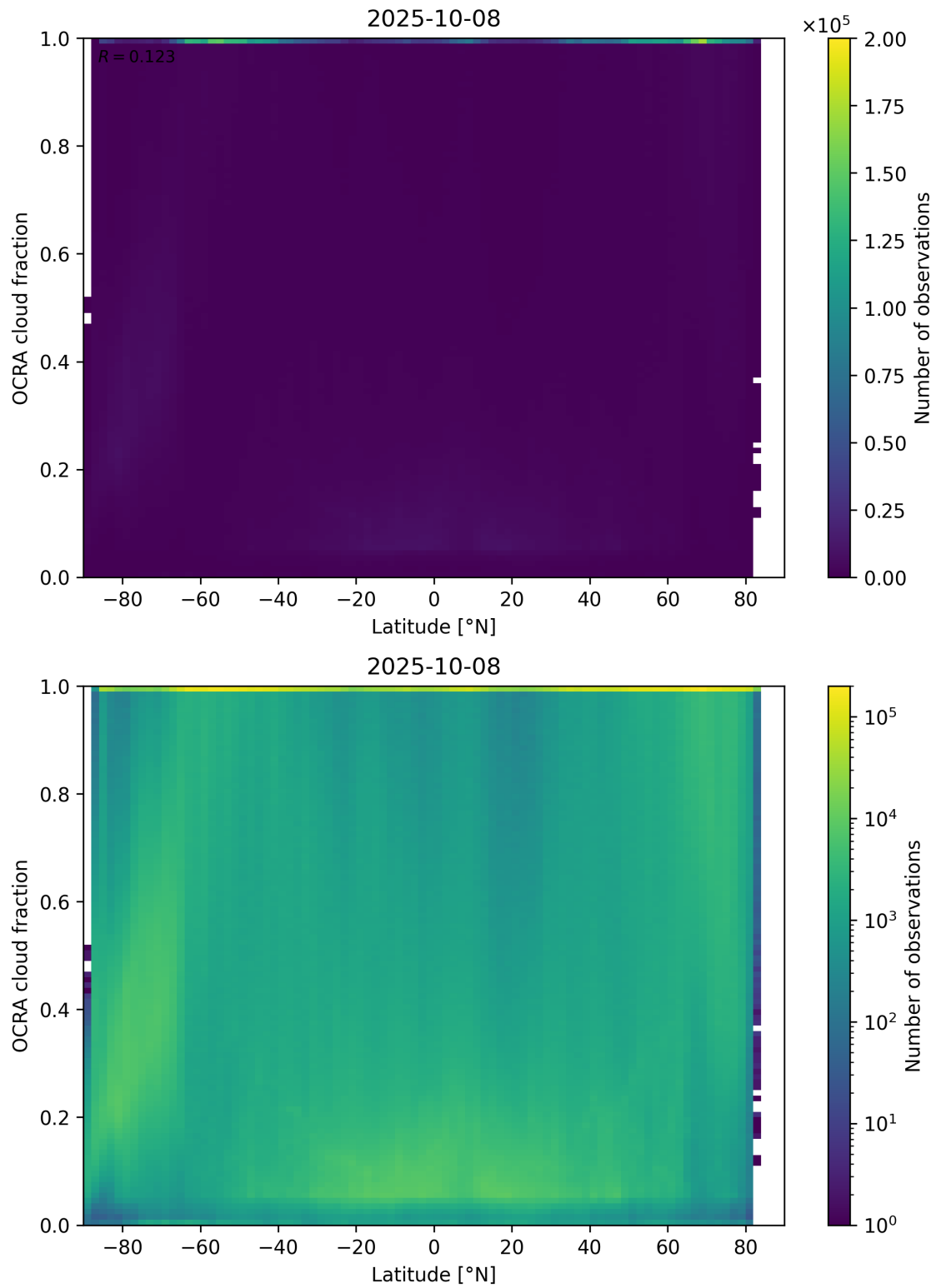
Figure 93: Scatter density plot of “Latitude” against “OCRA cloud fraction” for 2025-10-07 to 2025-10-09.
