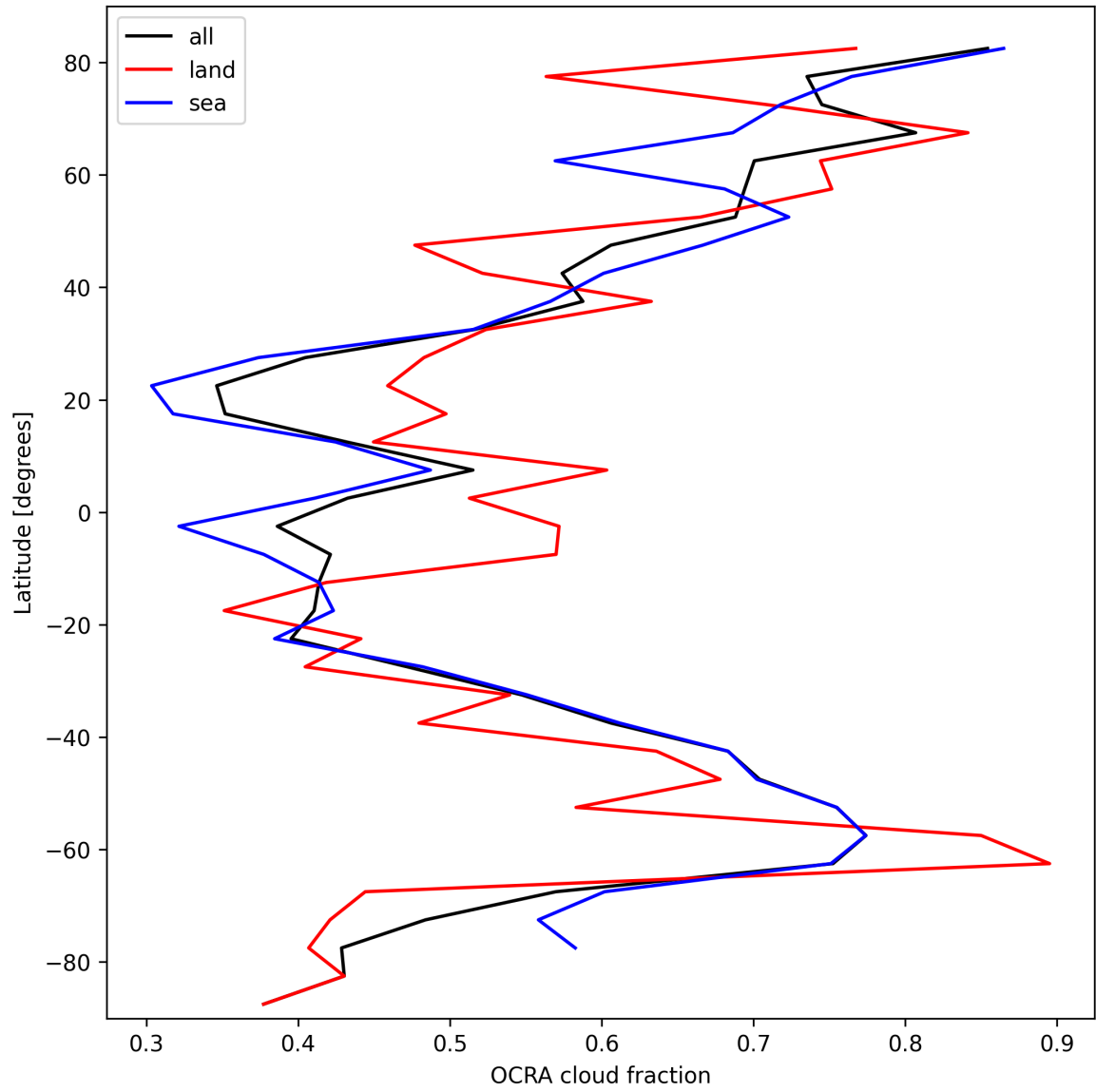
Figure 34: Zonal average of “OCRA cloud fraction” for 2025-10-07 to 2025-10-09.
