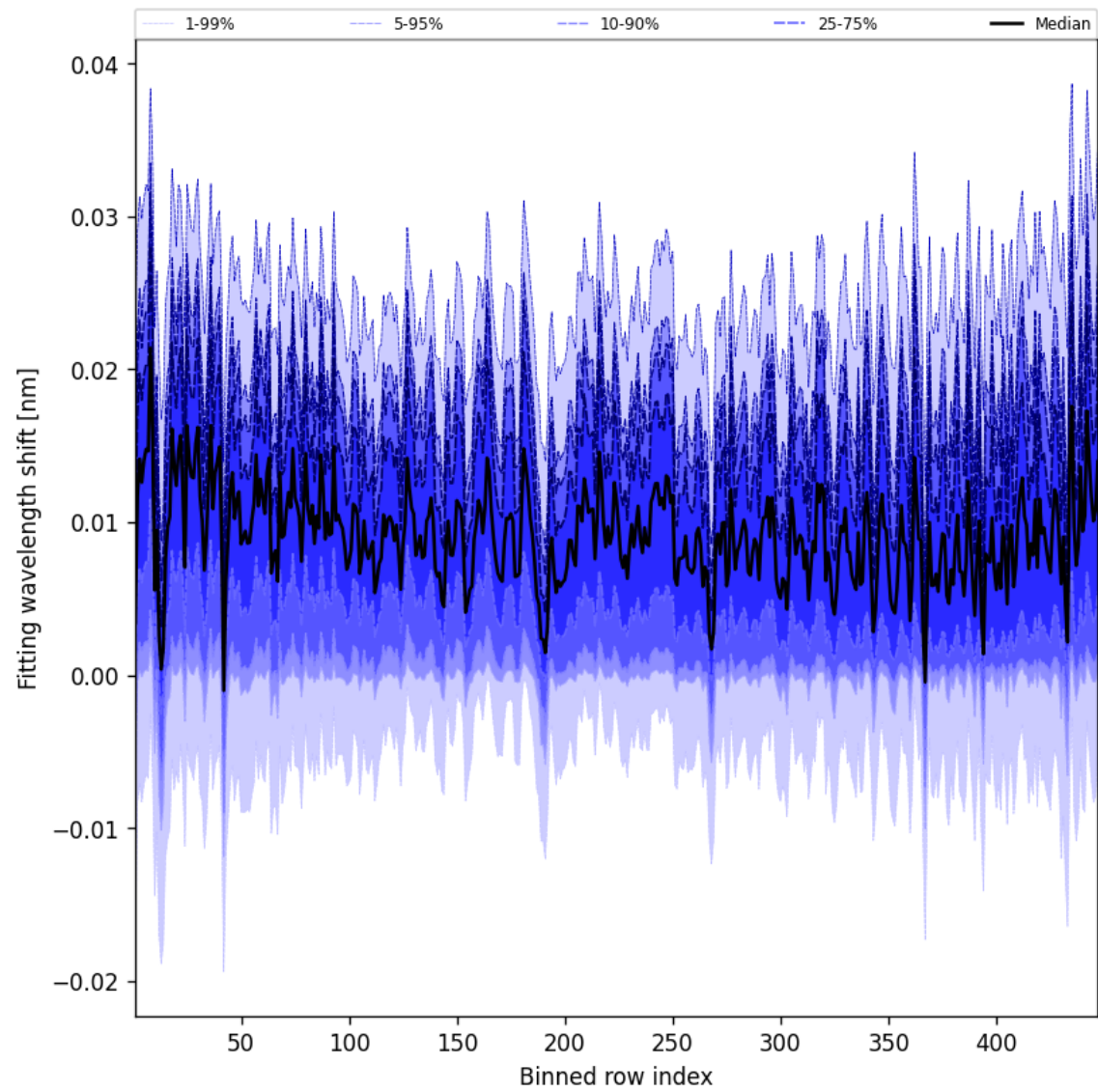
Figure 65: Along track statistics of “Fitting wavelength shift” for 2025-10-07 to 2025-10-09
