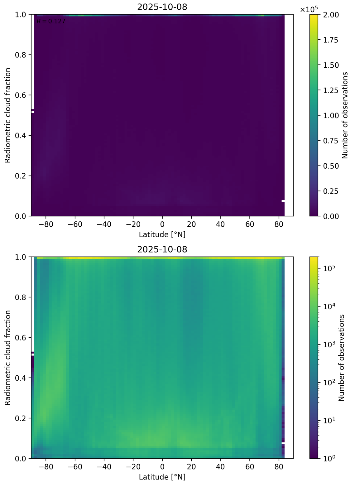
Figure 92: Scatter density plot of “Latitude” against “Radiometric cloud fraction” for 2025-10-07 to 2025-10-09.
