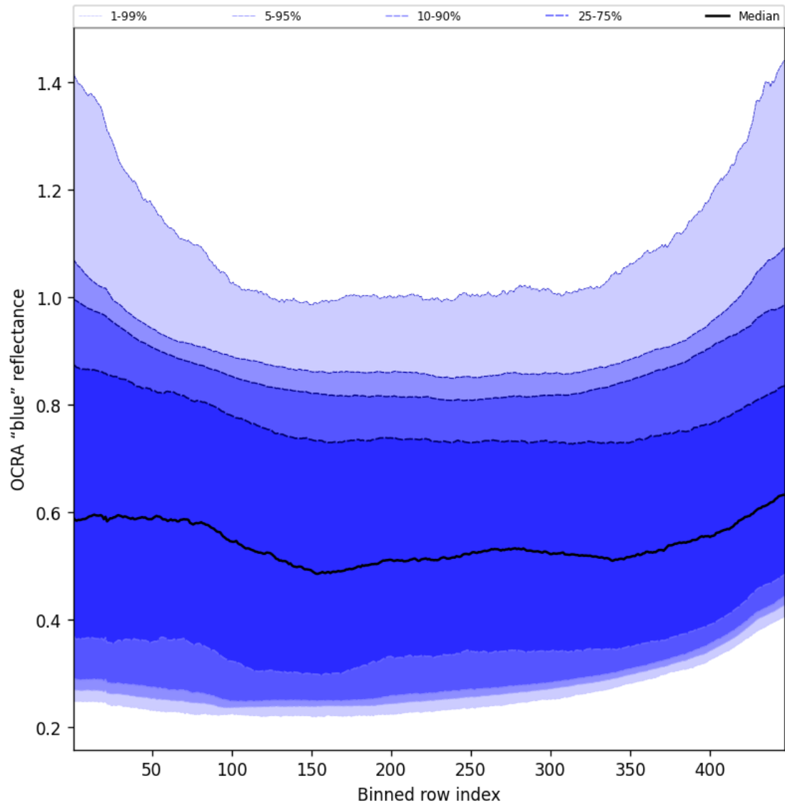
Figure 67: Along track statistics of “OCRA “blue” reflectance” for 2025-10-07 to 2025-10-09
