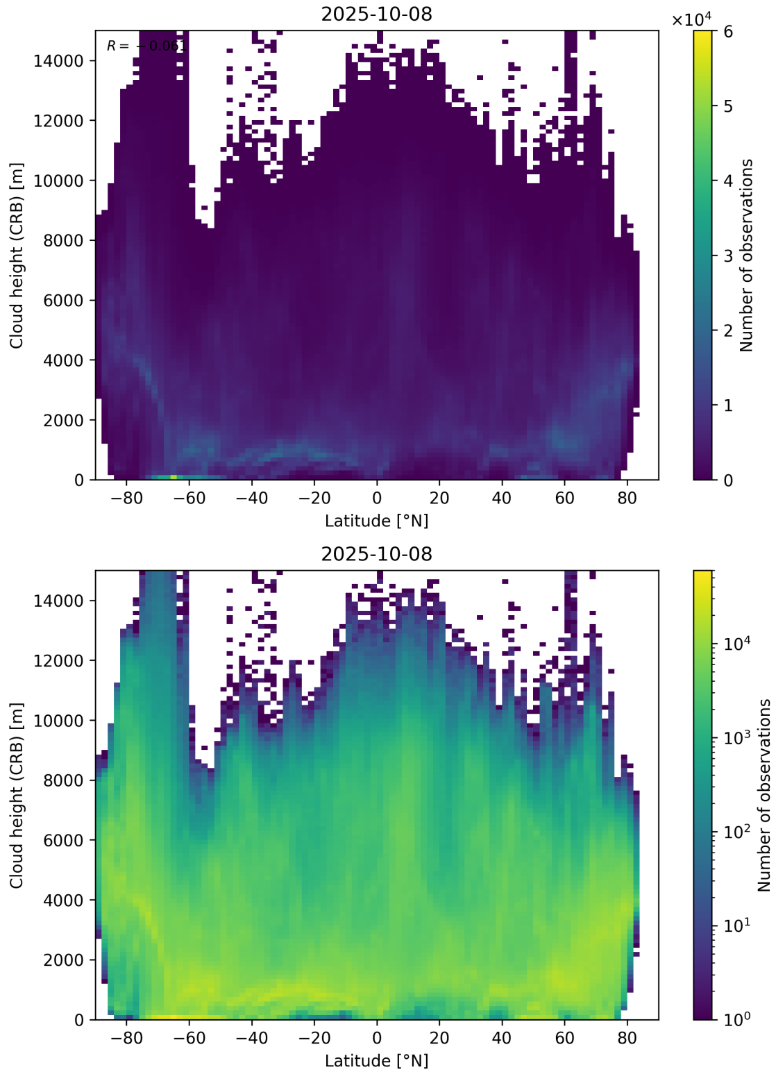
Figure 95: Scatter density plot of “Latitude” against “Cloud height (CRB)” for 2025-10-07 to 2025-10-09.
