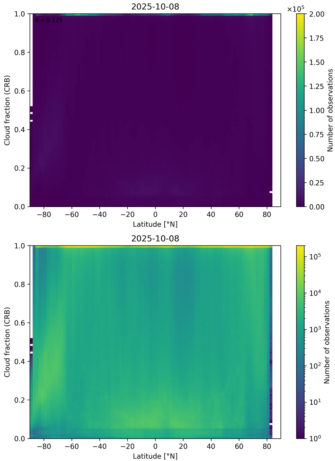
Figure 94: Scatter density plot of “Latitude” against “Cloud fraction (CRB)” for 2025-10-07 to 2025-10-09.
