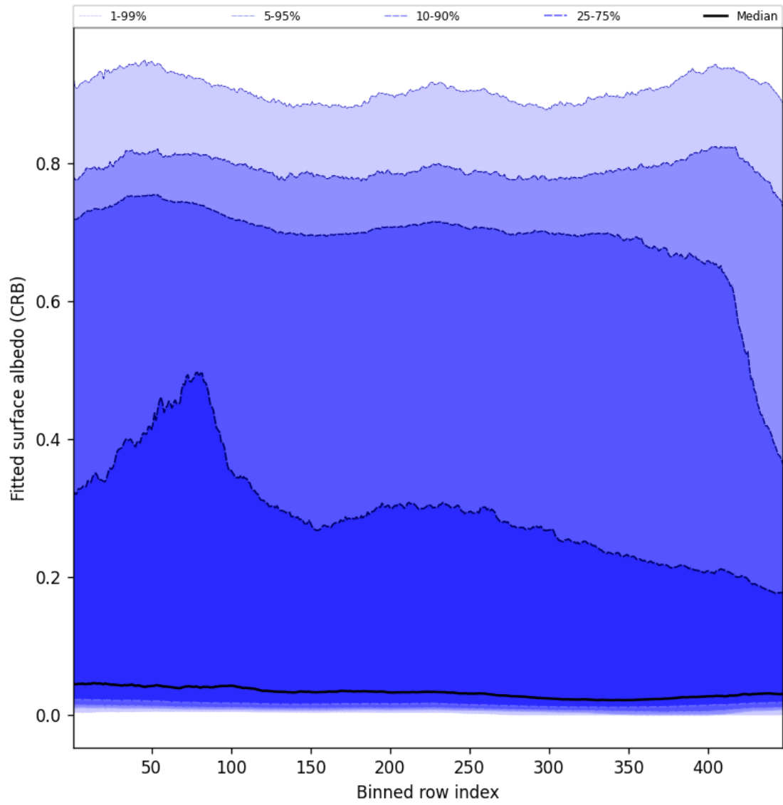
Figure 62: Along track statistics of “Fitted surface albedo (CRB)” for 2025-10-07 to 2025-10-09
