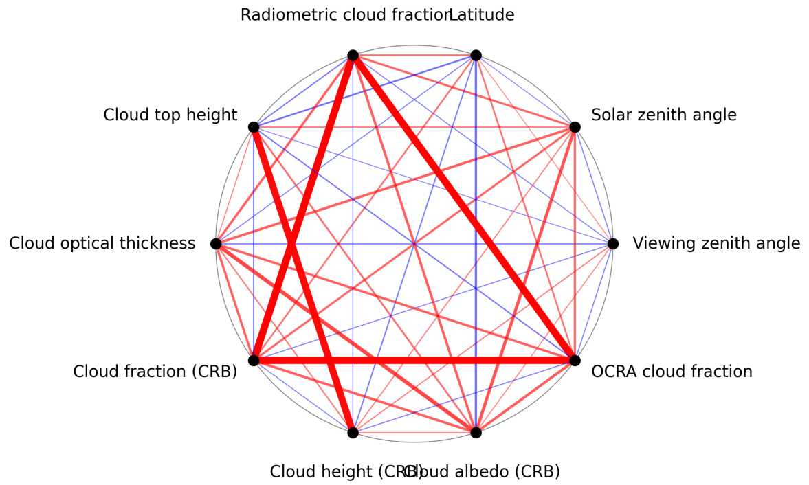
Figure 1: Map of correlation graph for 2025-10-07 to 2025-10-09.
