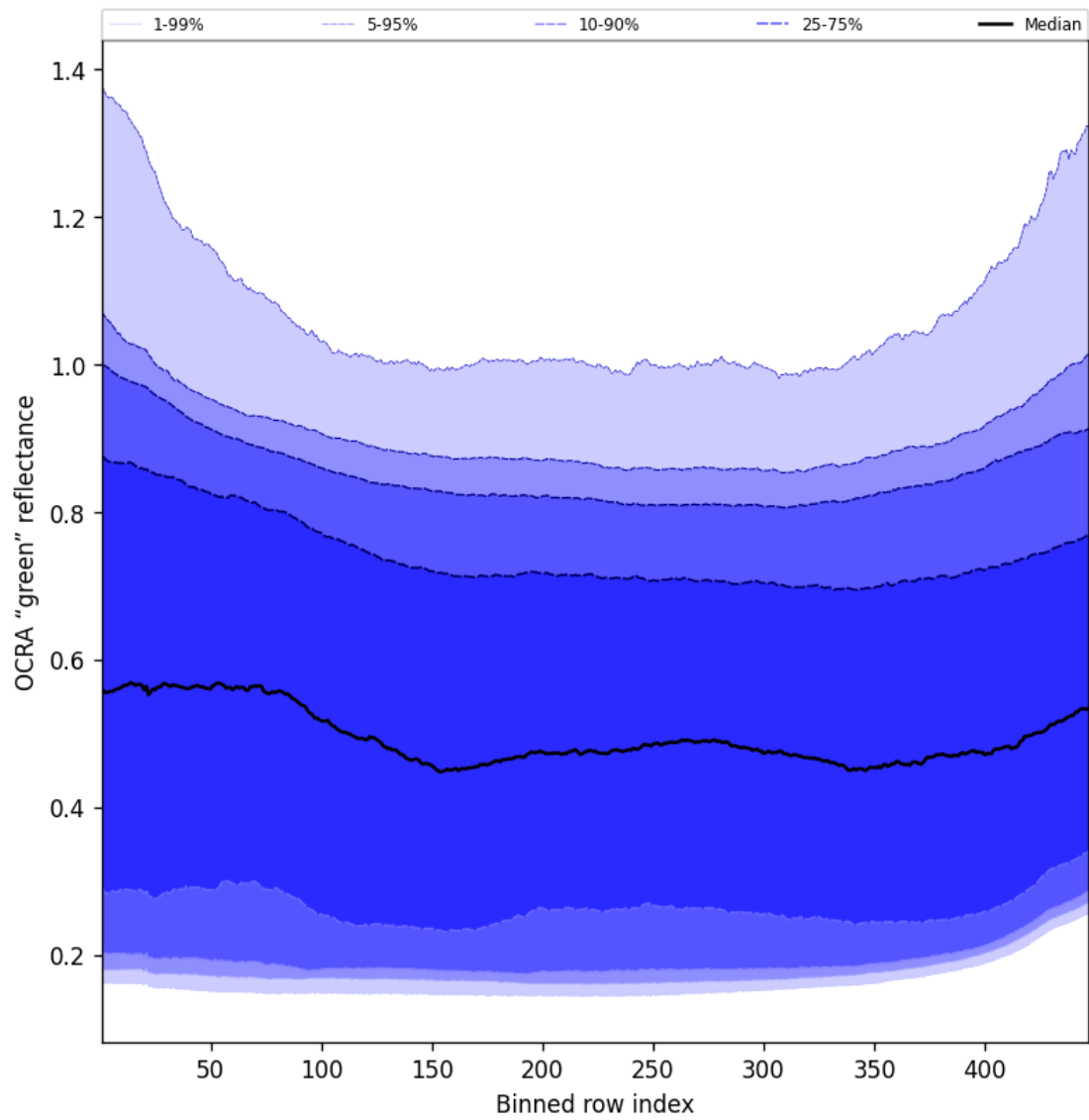
Figure 68: Along track statistics of “OCRA “green” reflectance” for 2025-10-07 to 2025-10-09
