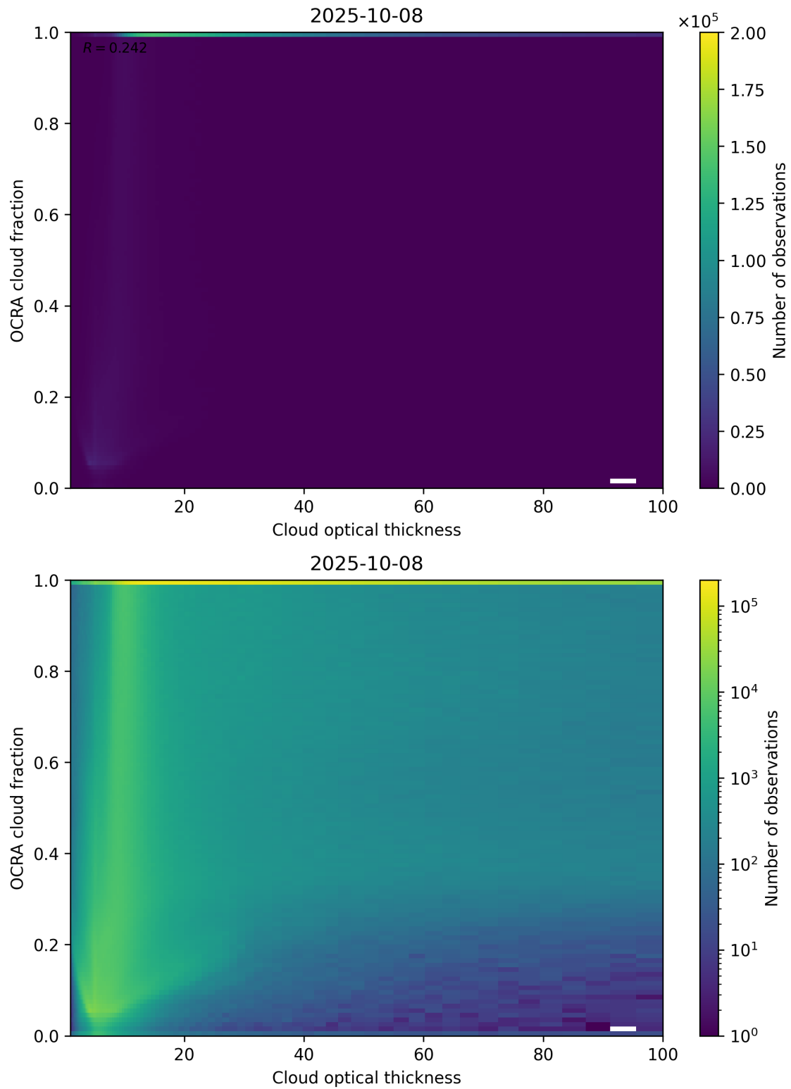
Figure 83: Scatter density plot of “Cloud optical thickness” against “OCRA cloud fraction” for 2025-10-07 to 2025-10-09.
