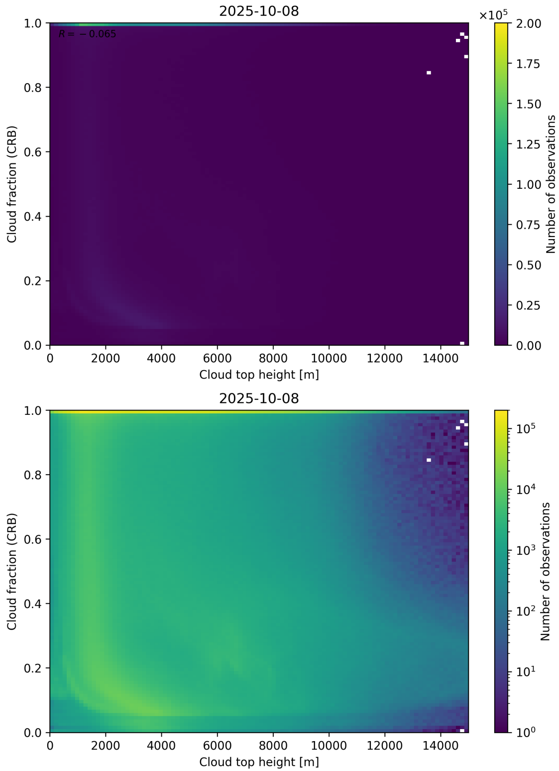
Figure 88: Scatter density plot of “Cloud top height” against “Cloud fraction (CRB)” for 2025-10-07 to 2025-10-09.
