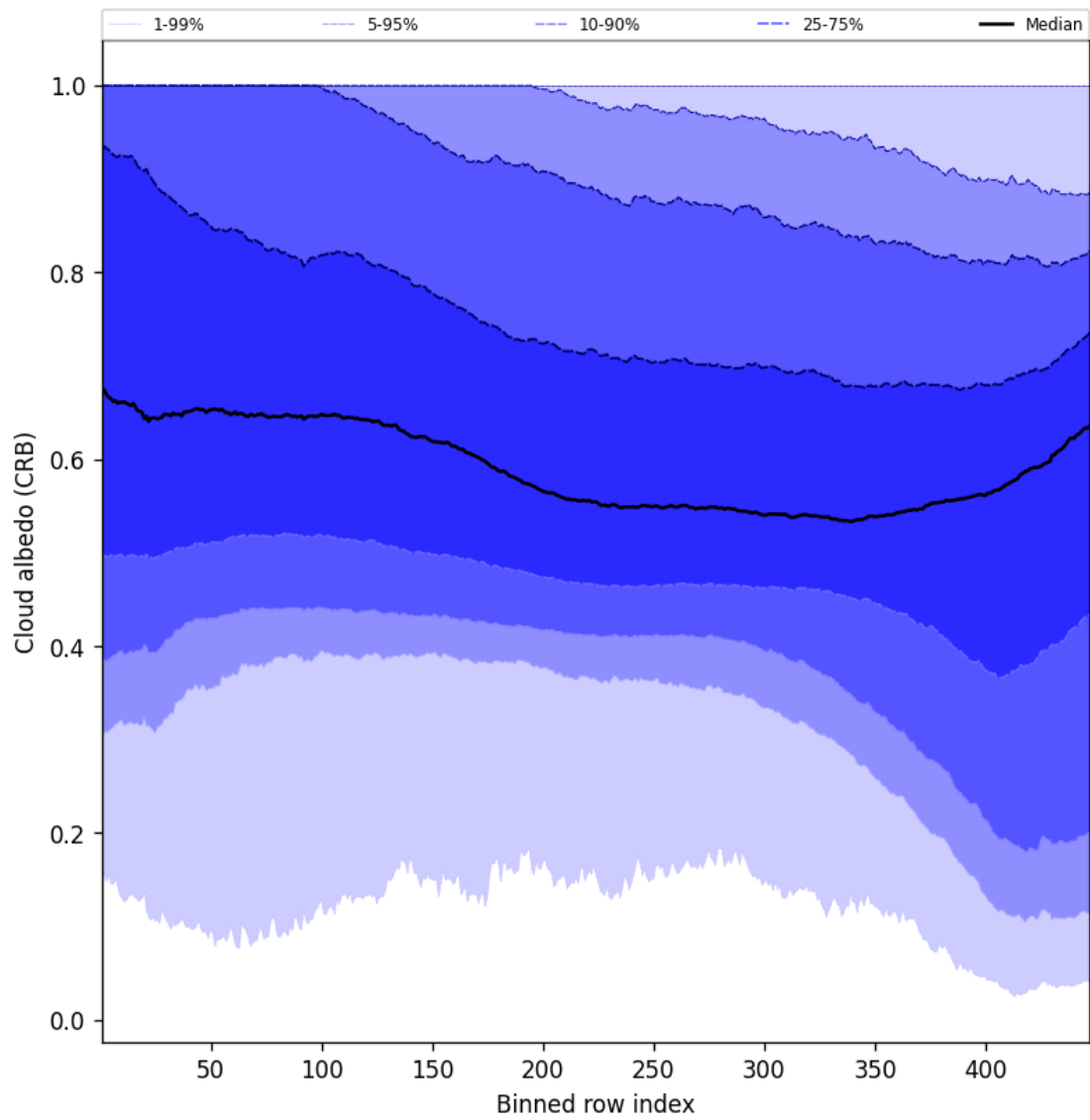
Figure 60: Along track statistics of “Cloud albedo (CRB)” for 2025-10-07 to 2025-10-09
