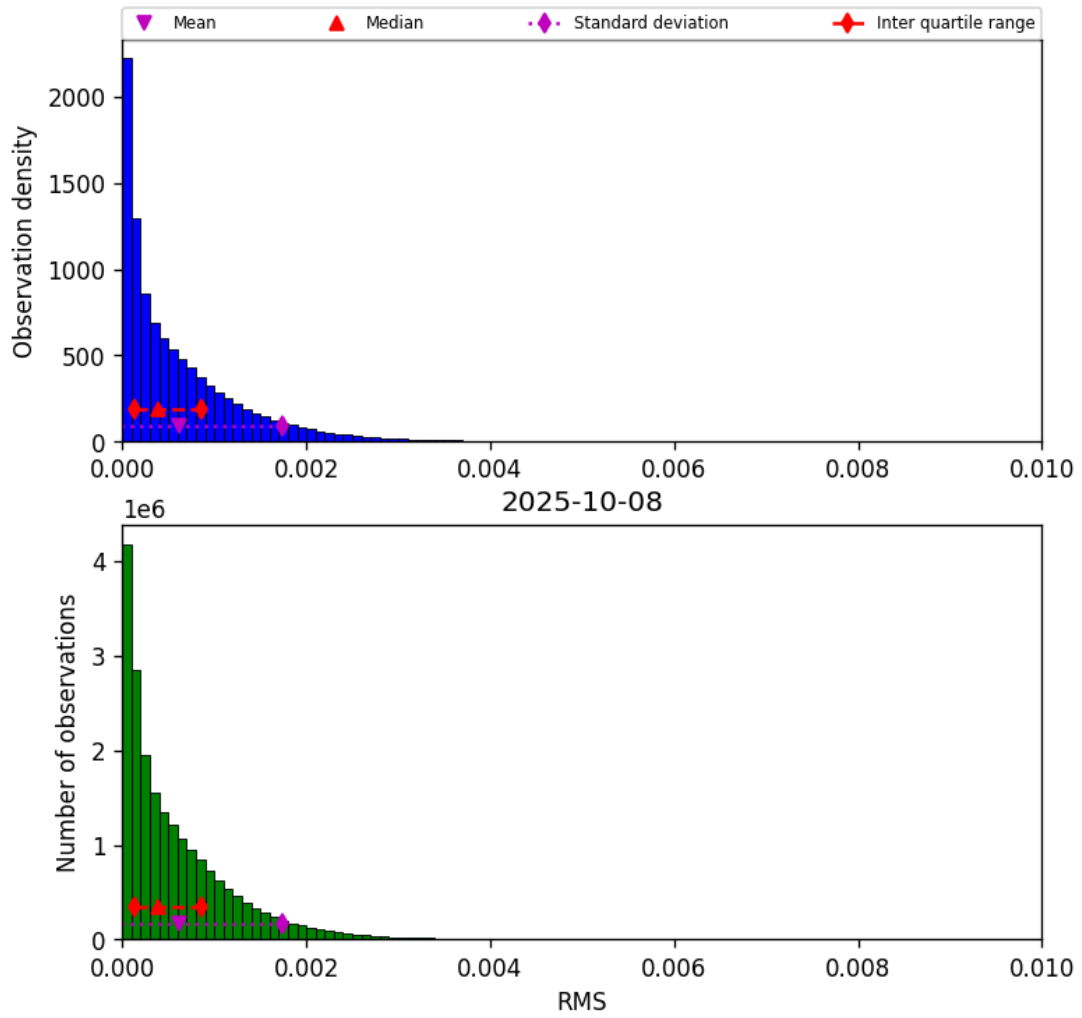
Figure 47: Histogram of “RMS” for 2025-10-07 to 2025-10-09
