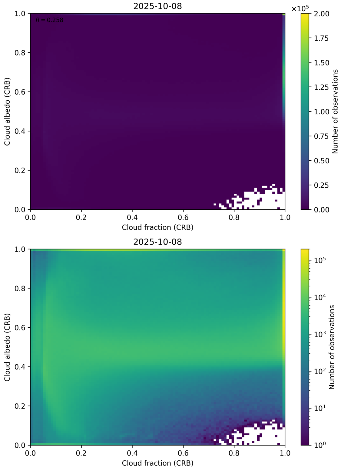
Figure 77: Scatter density plot of “Cloud fraction (CRB)” against “Cloud albedo (CRB)” for 2025-10-07 to 2025-10-09.
