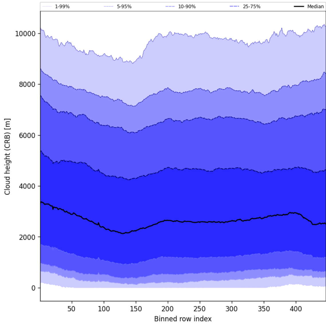
Figure 59: Along track statistics of “Cloud height (CRB)” for 2025-10-07 to 2025-10-09
