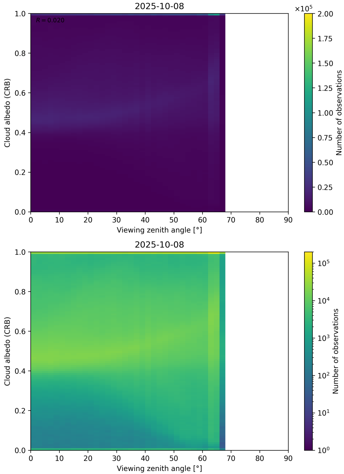
Figure 106: Scatter density plot of “Viewing zenith angle” against “Cloud albedo (CRB)” for 2025-10-07 to 2025-10-09.
