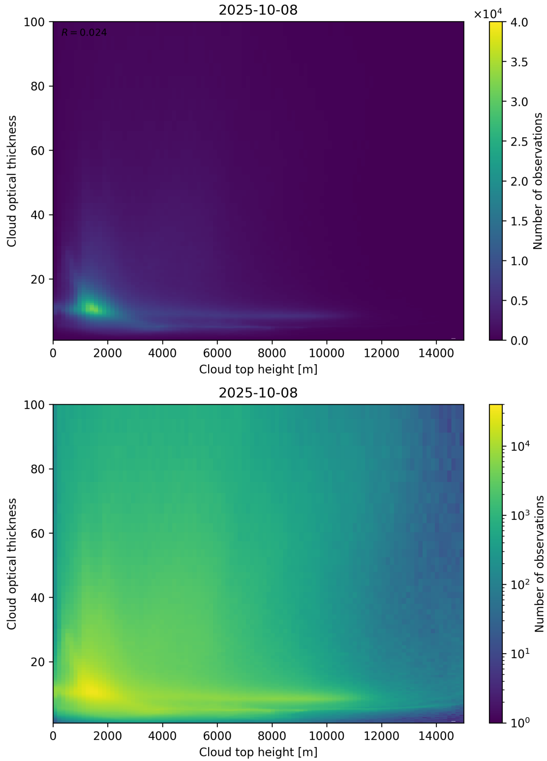
Figure 90: Scatter density plot of “Cloud top height” against “Cloud optical thickness” for 2025-10-07 to 2025-10-09.
