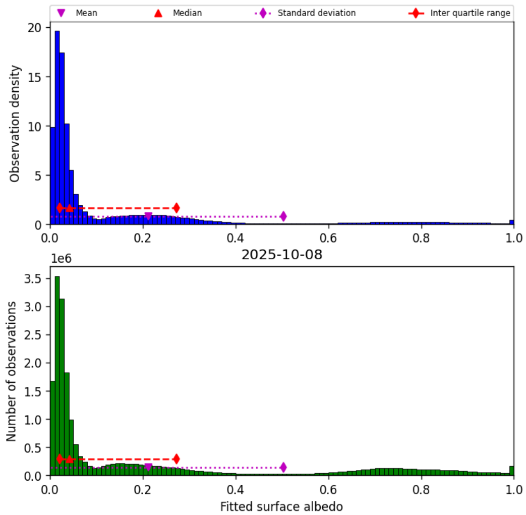
Figure 45: Histogram of “Fitted surface albedo” for 2025-10-07 to 2025-10-09
