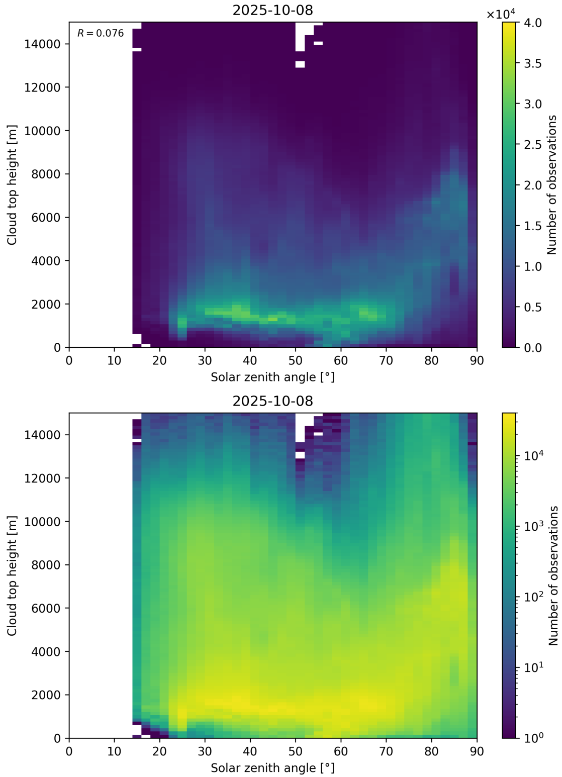
Figure 104: Scatter density plot of “Solar zenith angle” against “Cloud top height” for 2025-10-07 to 2025-10-09.
