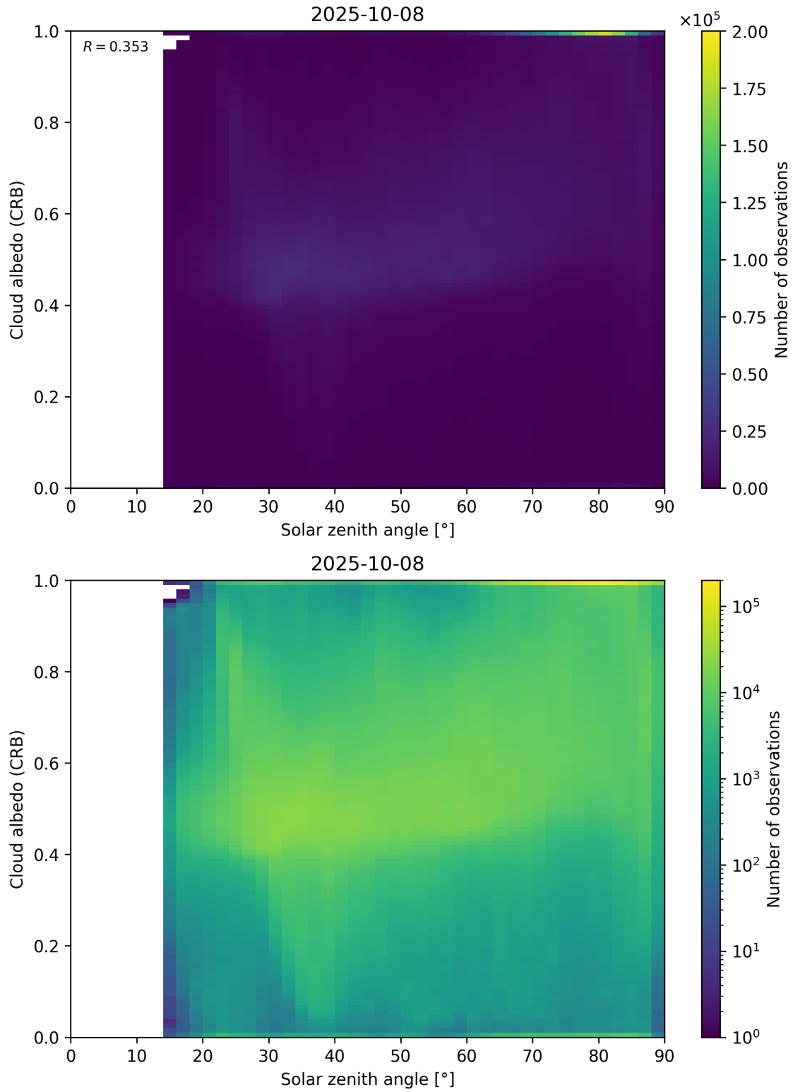
Figure 98: Scatter density plot of “Solar zenith angle” against “Cloud albedo (CRB)” for 2025-10-07 to 2025-10-09.
