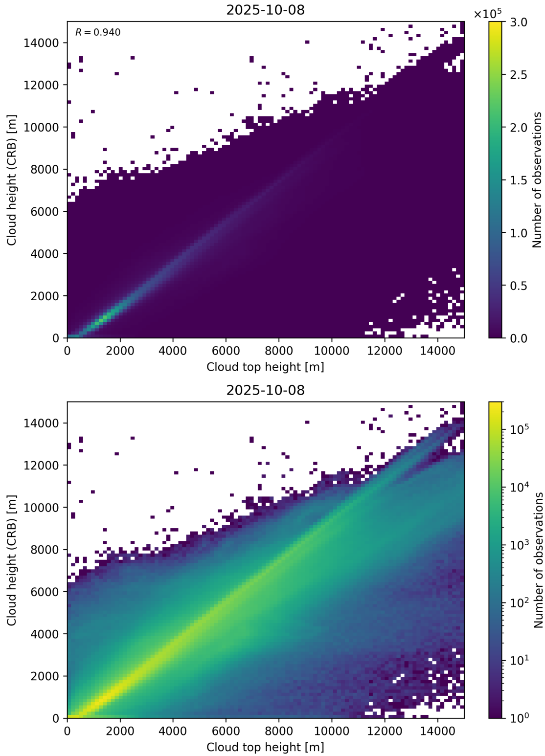
Figure 89: Scatter density plot of “Cloud top height” against “Cloud height (CRB)” for 2025-10-07 to 2025-10-09.
