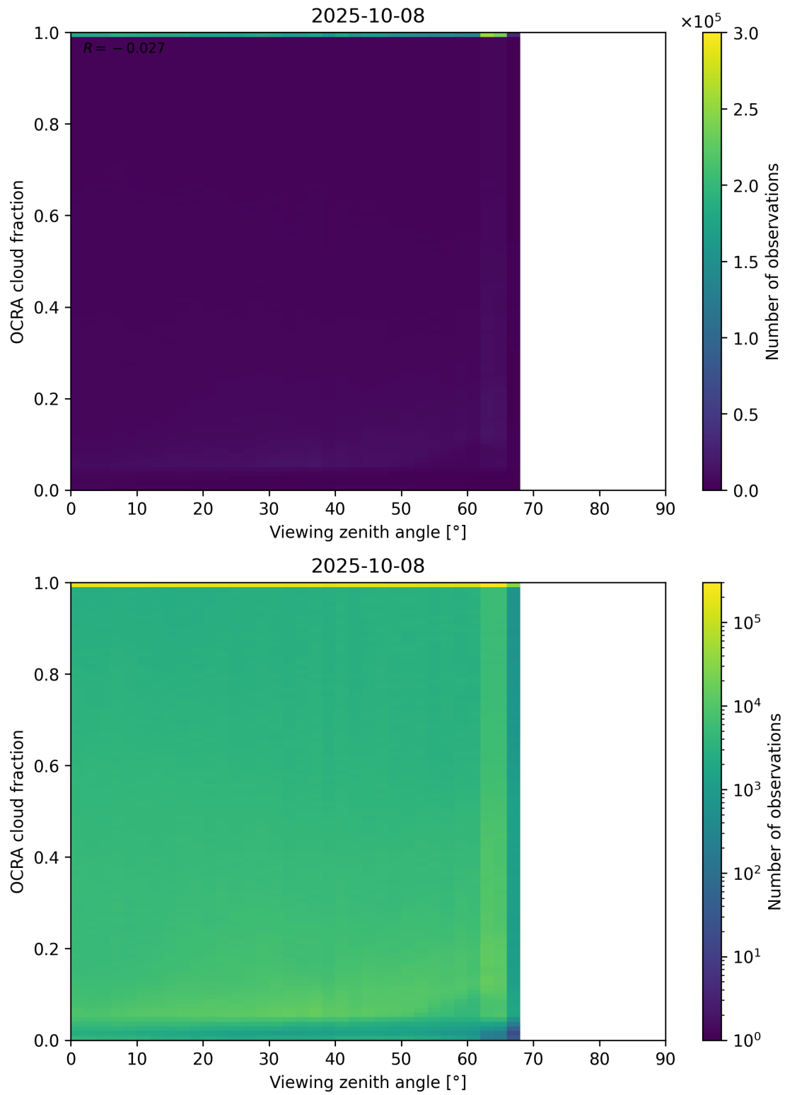
Figure 108: Scatter density plot of “Viewing zenith angle” against “OCRA cloud fraction” for 2025-10-07 to 2025-10-09.
