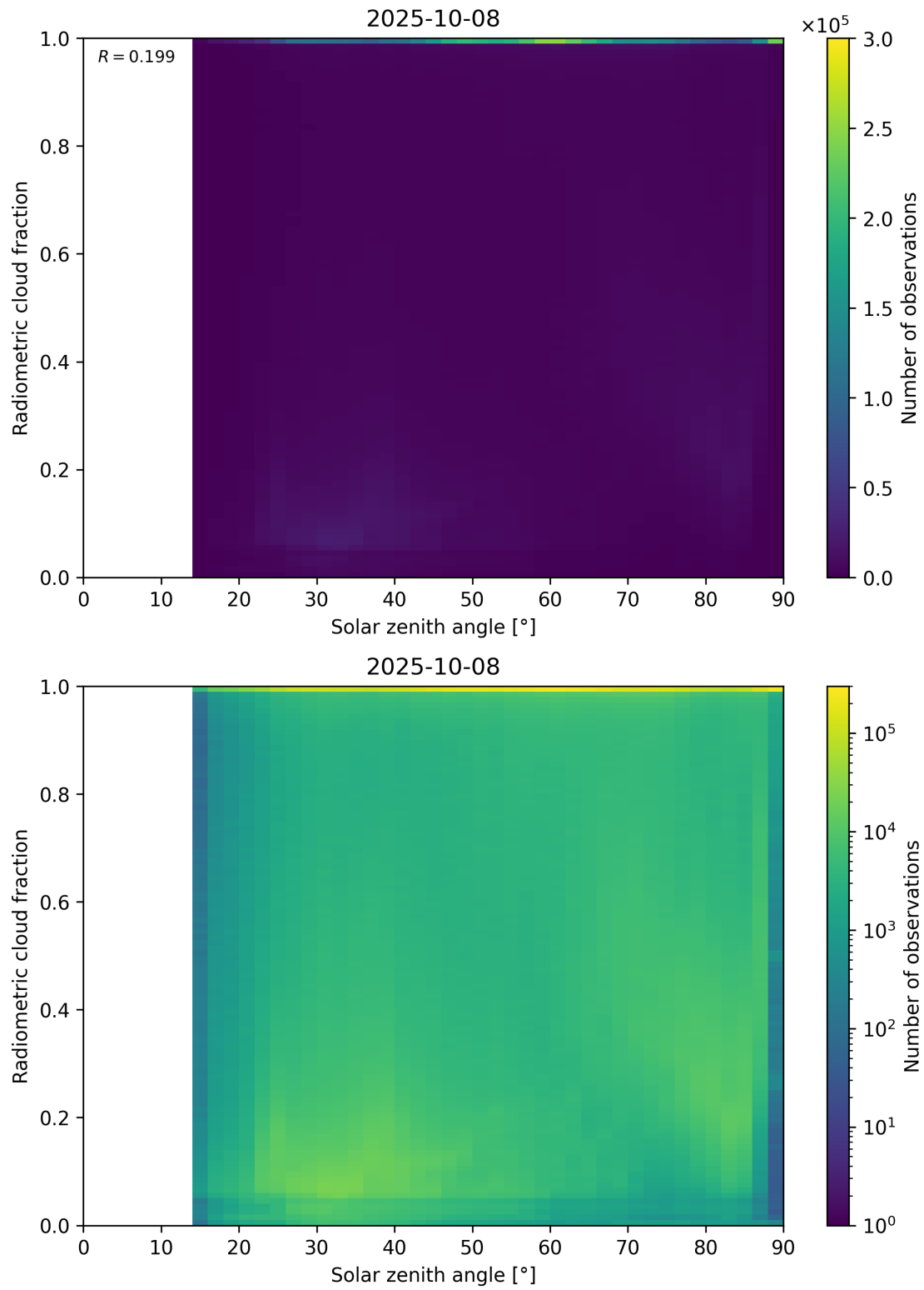
Figure 99: Scatter density plot of “Solar zenith angle” against “Radiometric cloud fraction” for 2025-10-07 to 2025-10-09.
