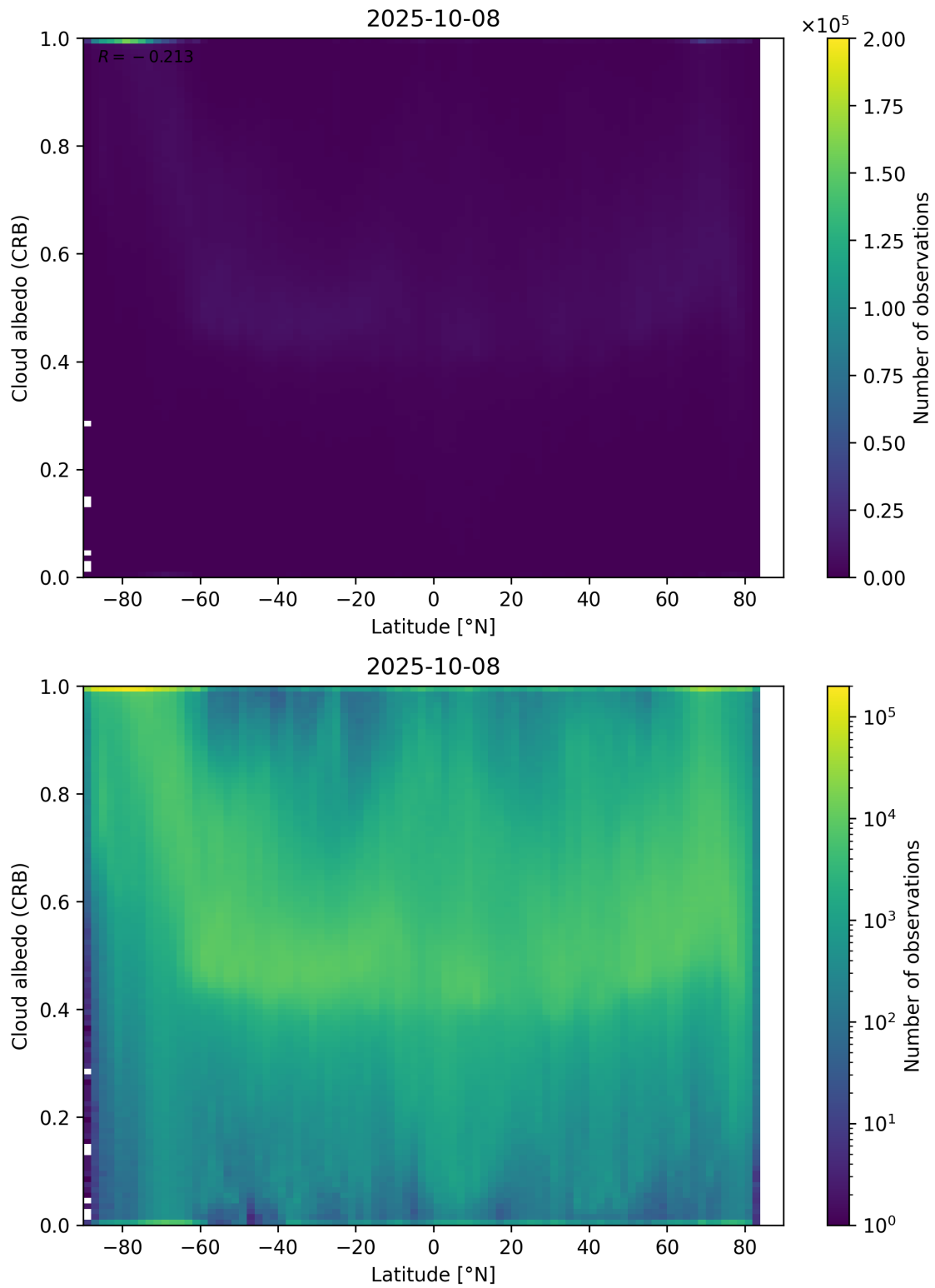
Figure 91: Scatter density plot of “Latitude” against “Cloud albedo (CRB)” for 2025-10-07 to 2025-10-09.
