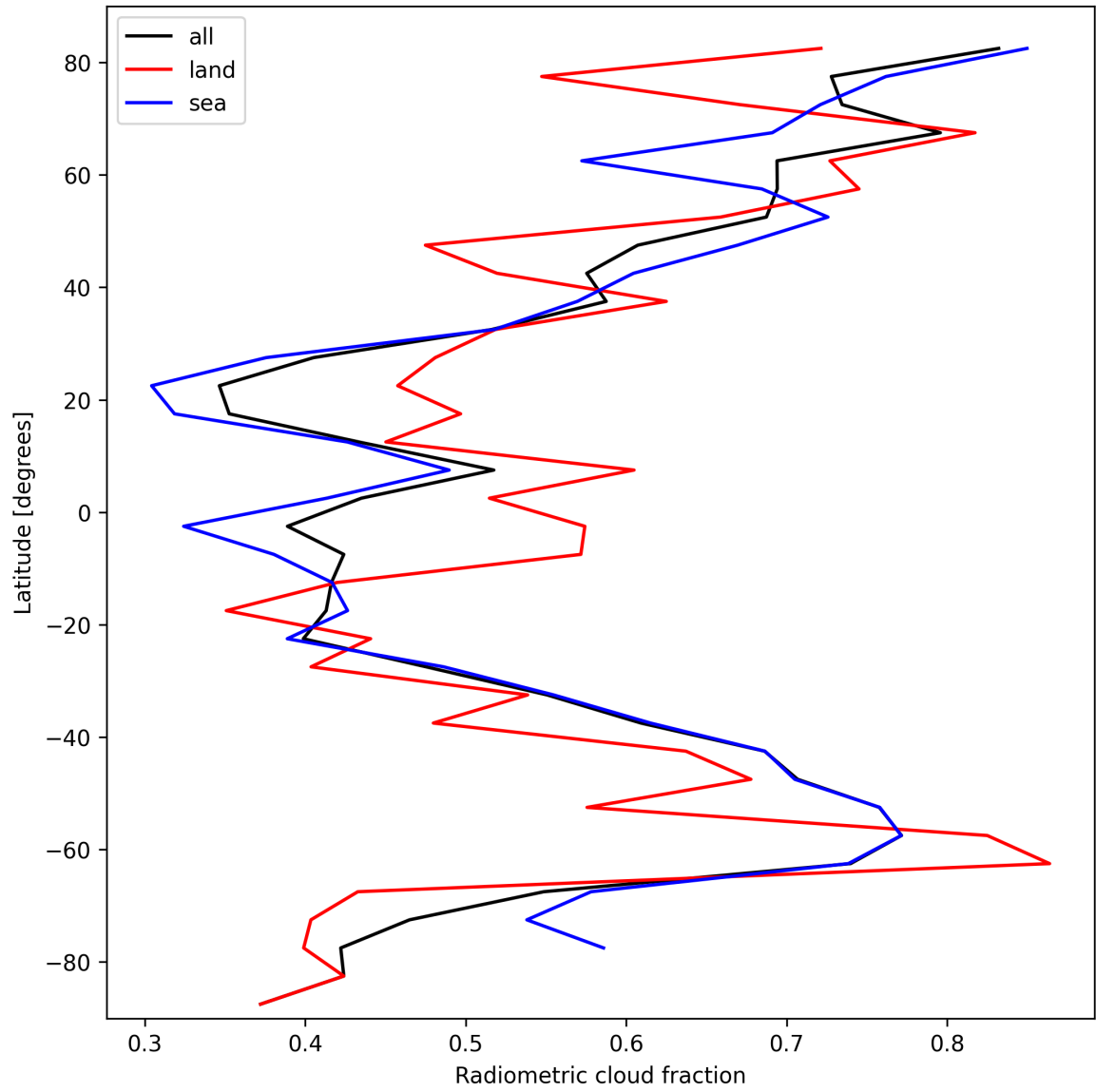
Figure 23: Zonal average of “Radiometric cloud fraction” for 2025-10-07 to 2025-10-09.
