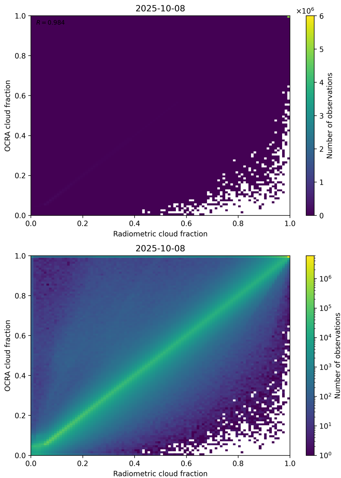
Figure 72: Scatter density plot of “Radiometric cloud fraction” against “OCRA cloud fraction” for 2025-10-07 to 2025-10-09.
