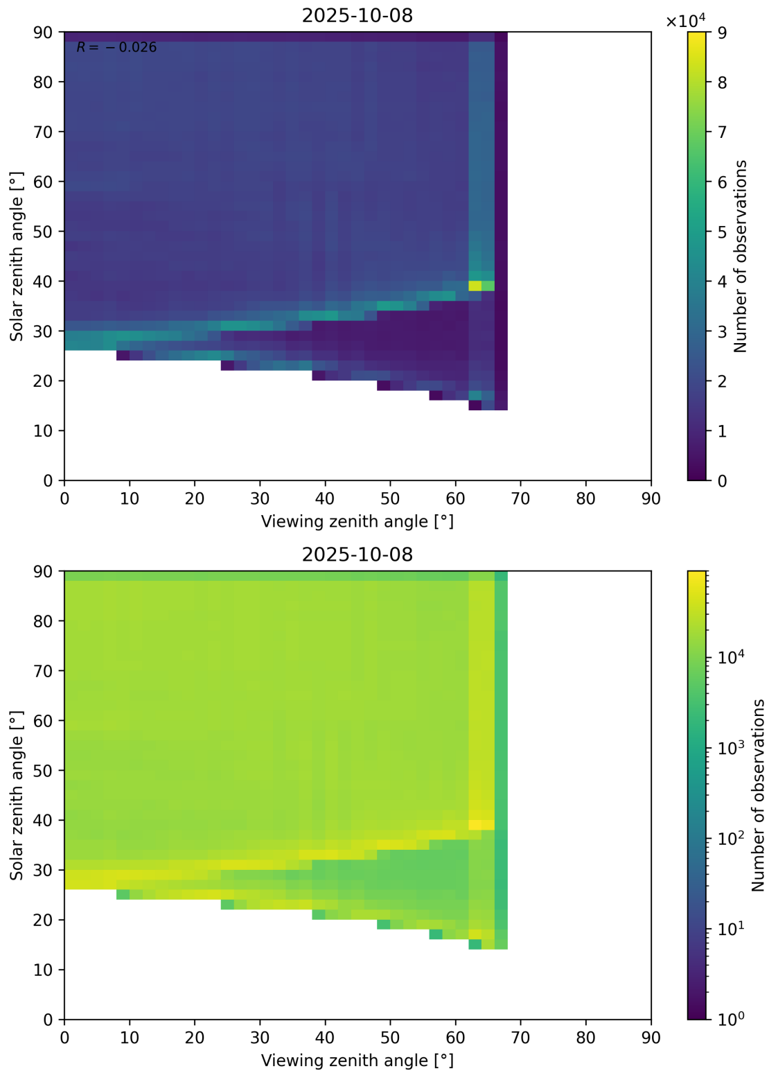
Figure 114: Scatter density plot of “Viewing zenith angle” against “Solar zenith angle” for 2025-10-07 to 2025-10-09.
