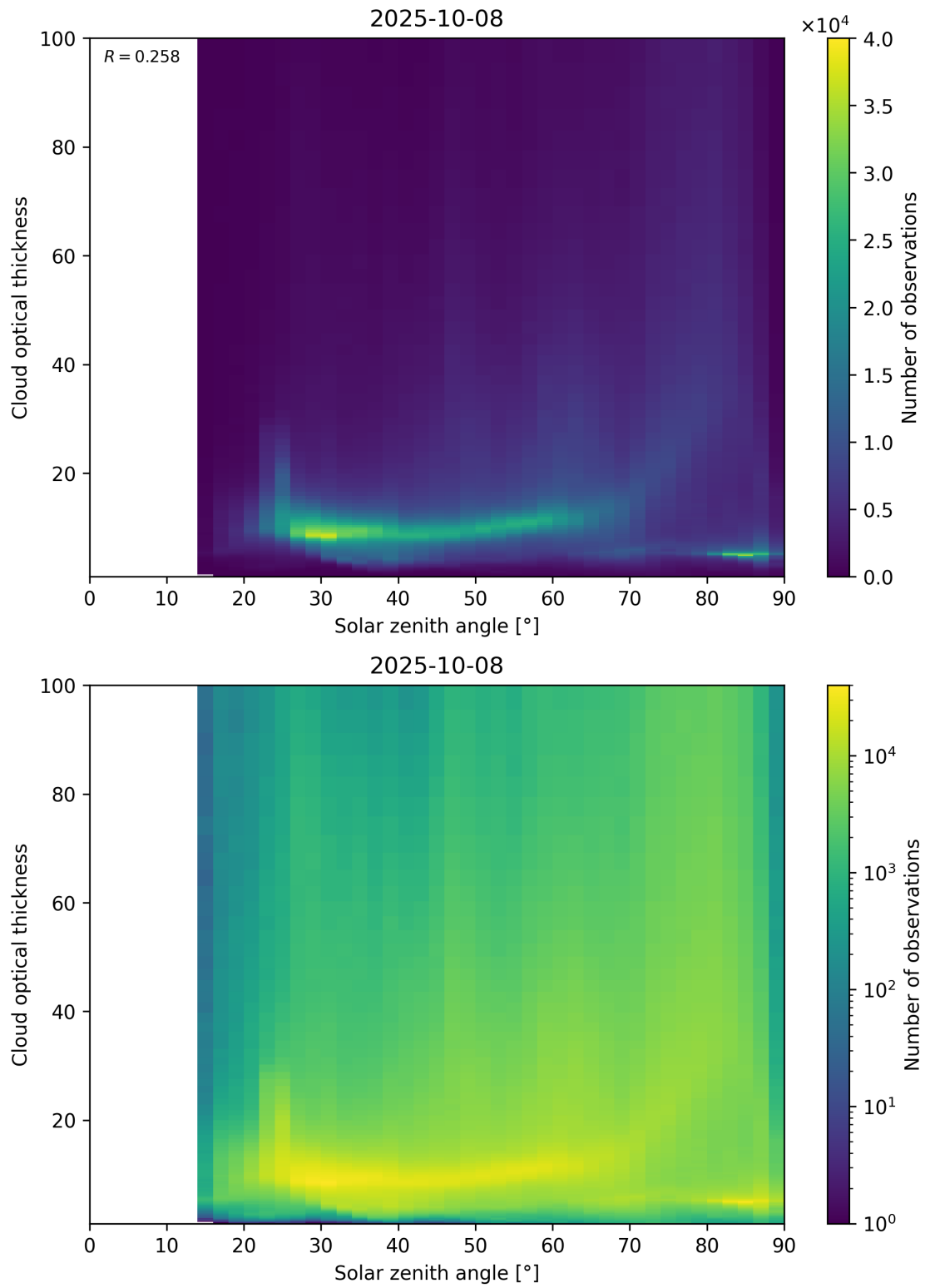
Figure 103: Scatter density plot of “Solar zenith angle” against “Cloud optical thickness” for 2025-10-07 to 2025-10-09.
