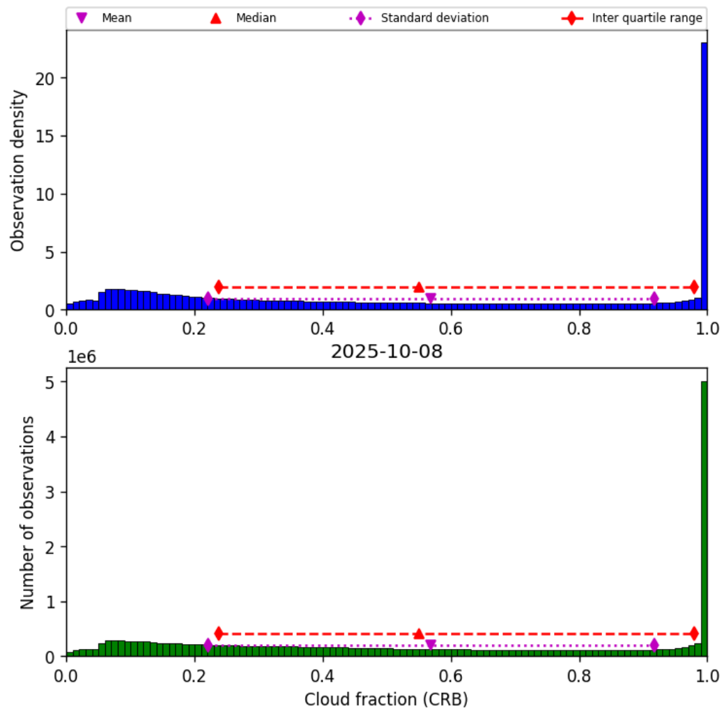
Figure 42: Histogram of “Cloud fraction (CRB)” for 2025-10-07 to 2025-10-09
