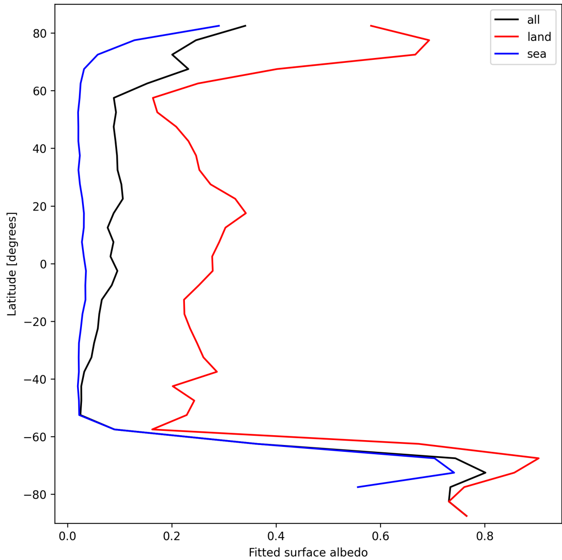
Figure 29: Zonal average of “Fitted surface albedo” for 2025-10-07 to 2025-10-09.
