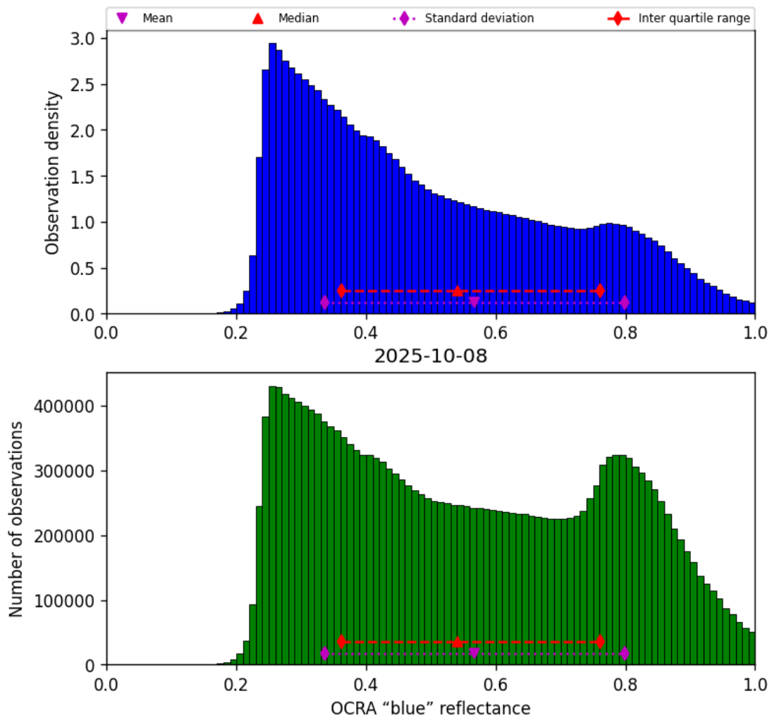
Figure 51: Histogram of “OCRA “blue” reflectance” for 2025-10-07 to 2025-10-09
