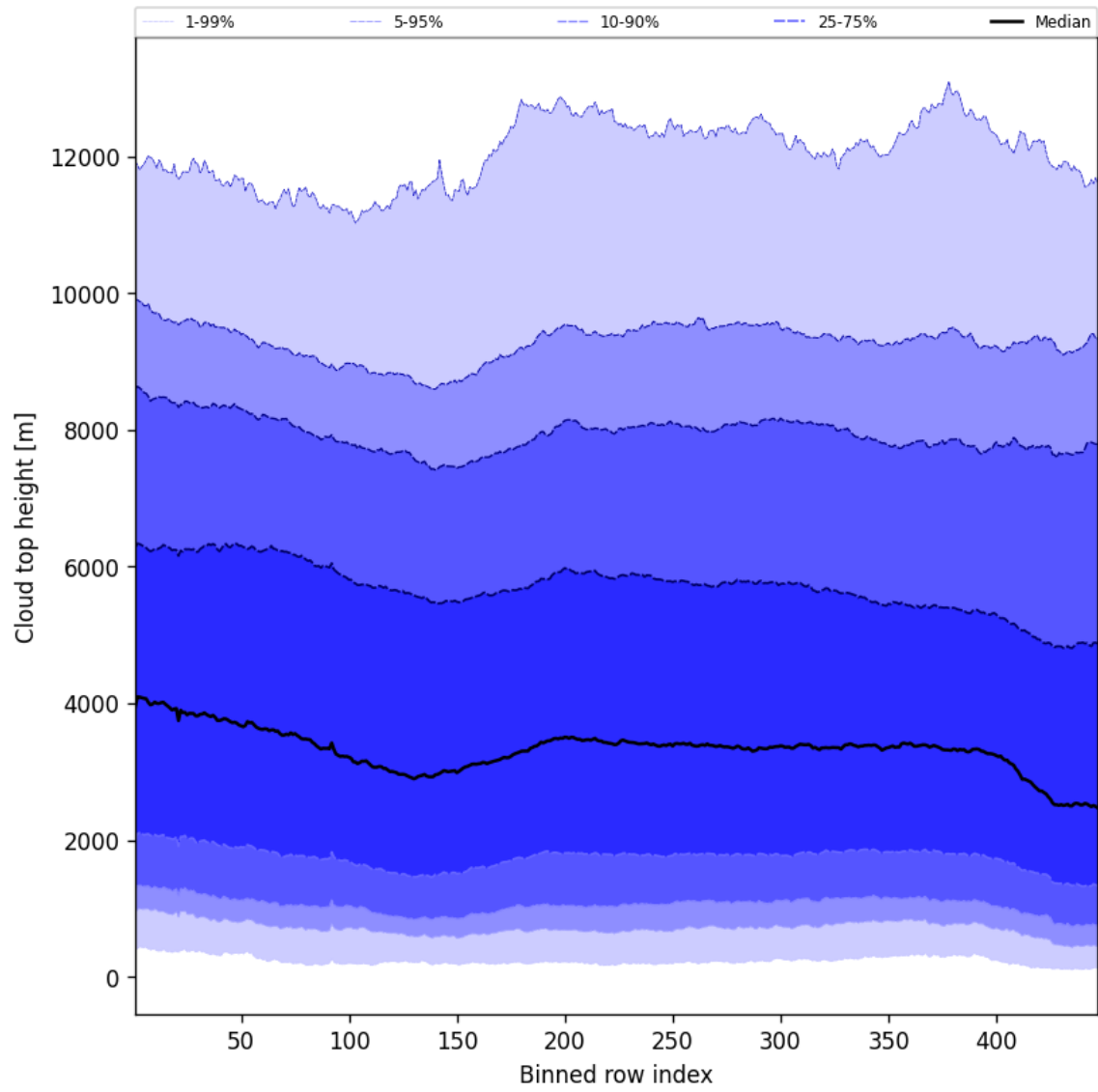
Figure 56: Along track statistics of “Cloud top height” for 2025-10-07 to 2025-10-09
