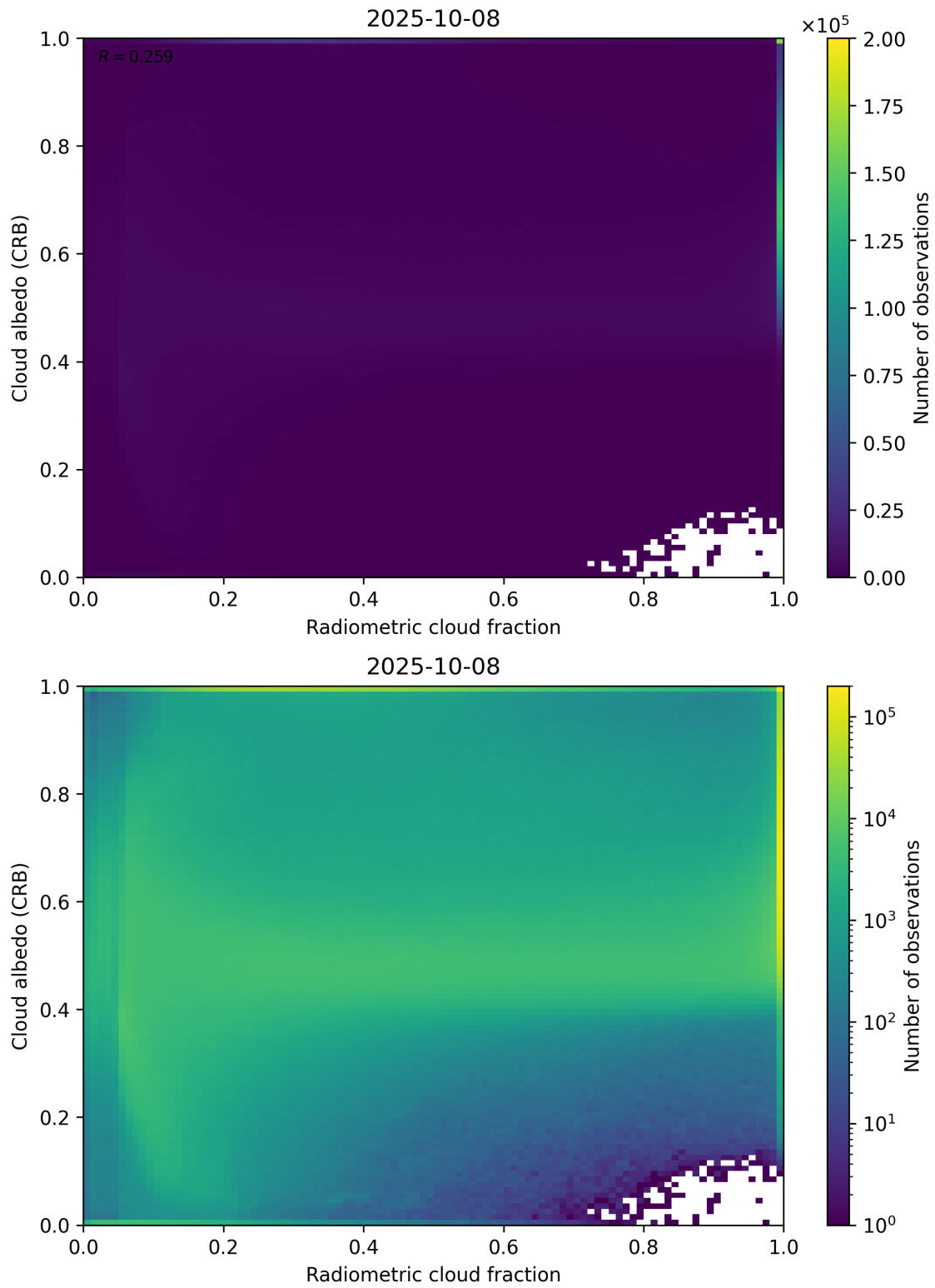
Figure 71: Scatter density plot of “Radiometric cloud fraction” against “Cloud albedo (CRB)” for 2025-10-07 to 2025-10-09.
