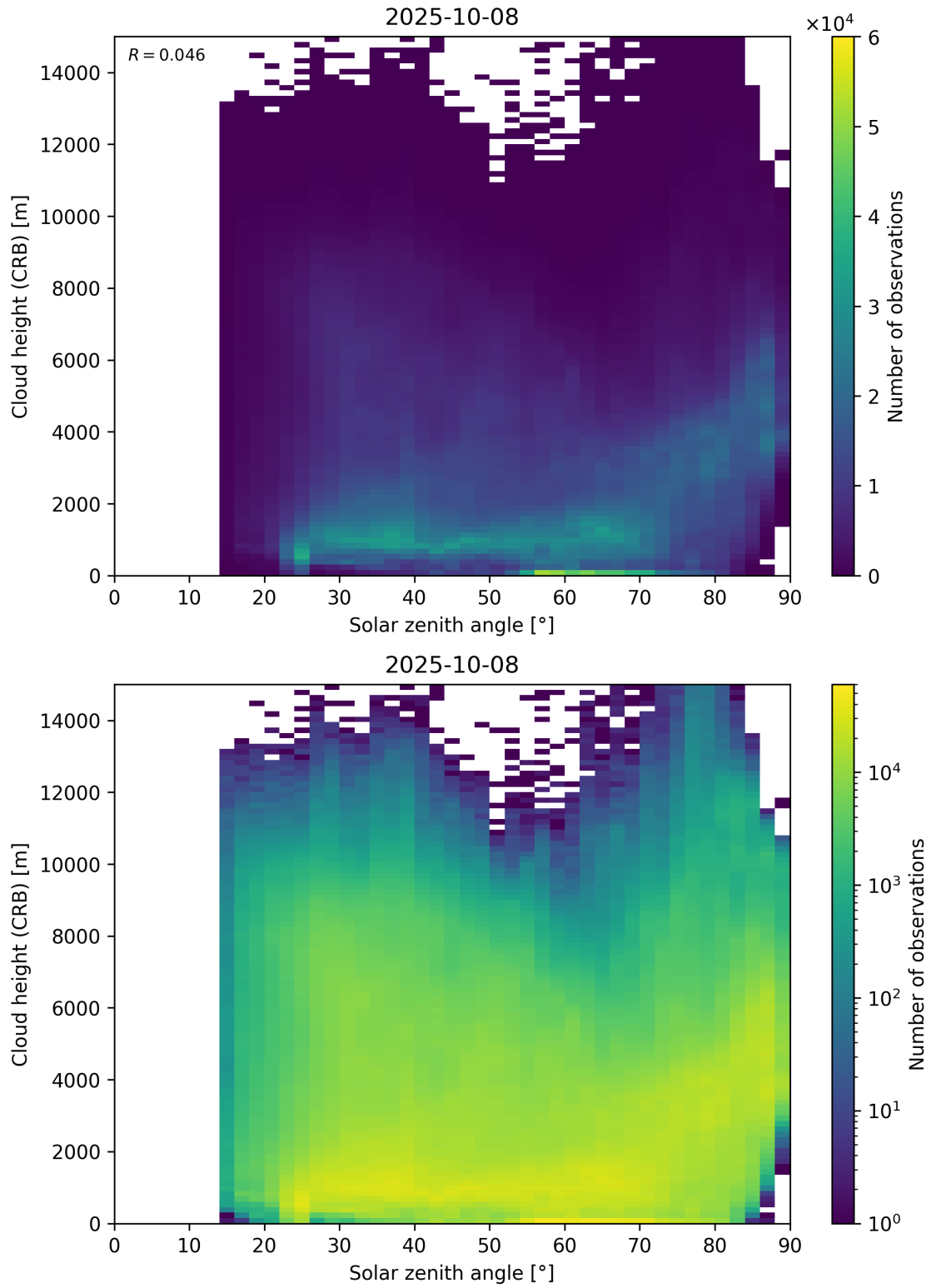
Figure 102: Scatter density plot of “Solar zenith angle” against “Cloud height (CRB)” for 2025-10-07 to 2025-10-09.
