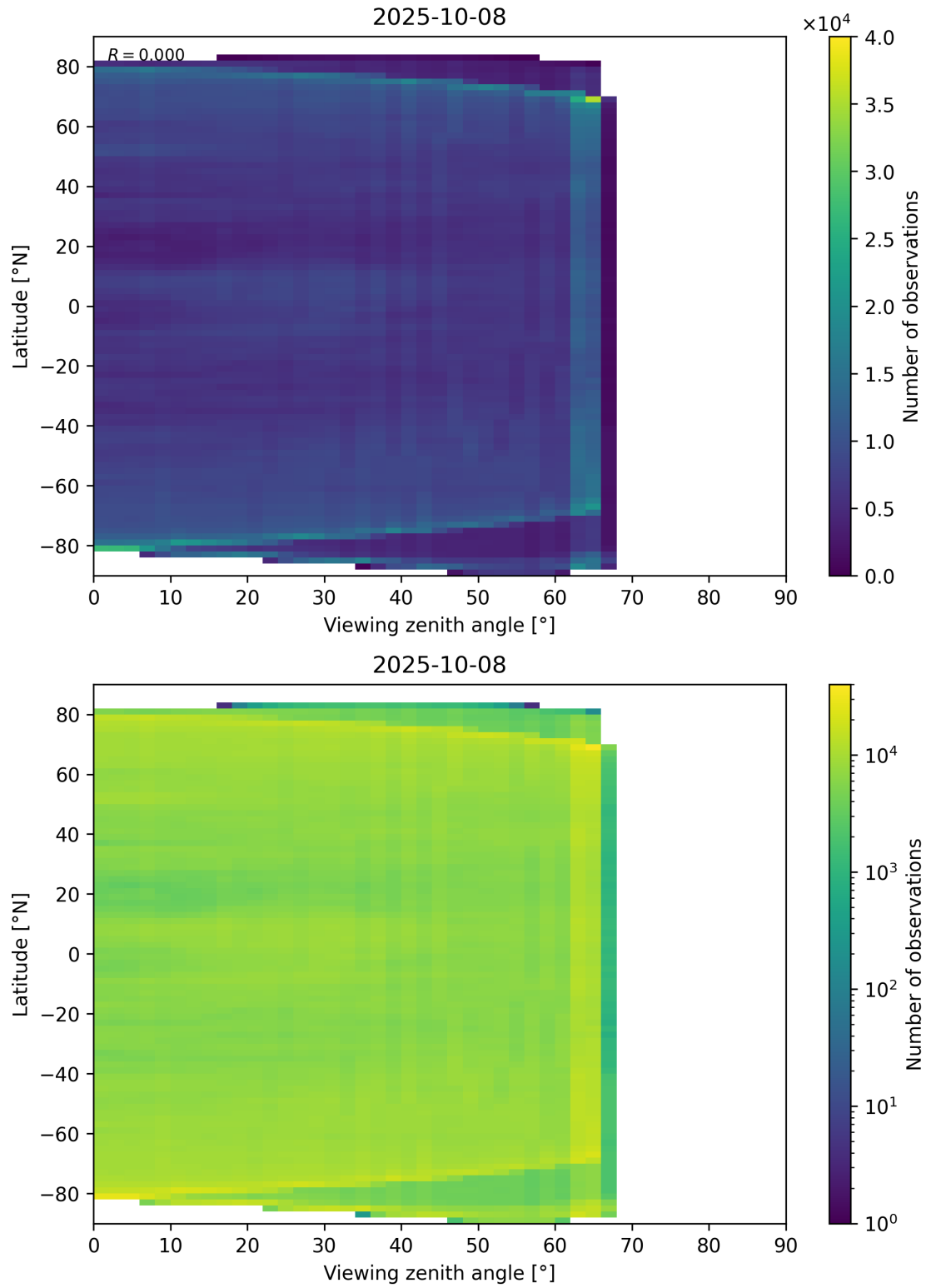
Figure 113: Scatter density plot of “Viewing zenith angle” against “Latitude” for 2025-10-07 to 2025-10-09.
