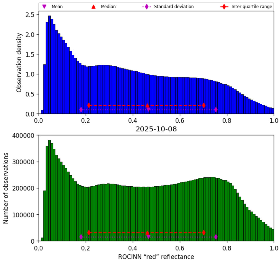
Figure 53: Histogram of “ROCINN “red” reflectance” for 2025-10-07 to 2025-10-09
