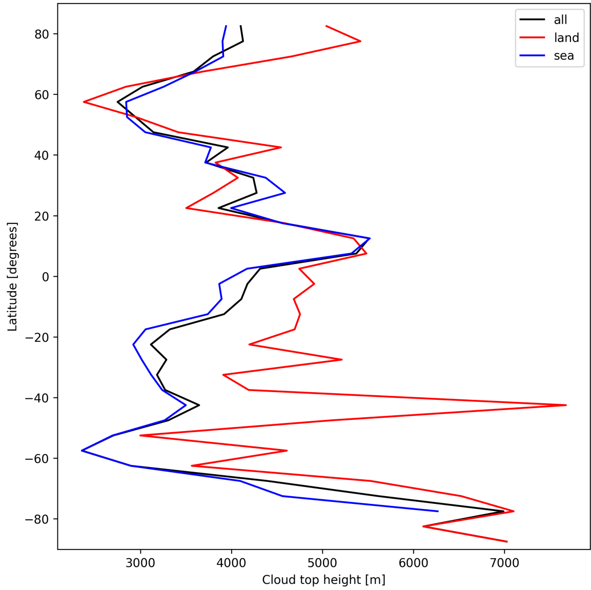
Figure 24: Zonal average of “Cloud top height” for 2025-10-07 to 2025-10-09.
