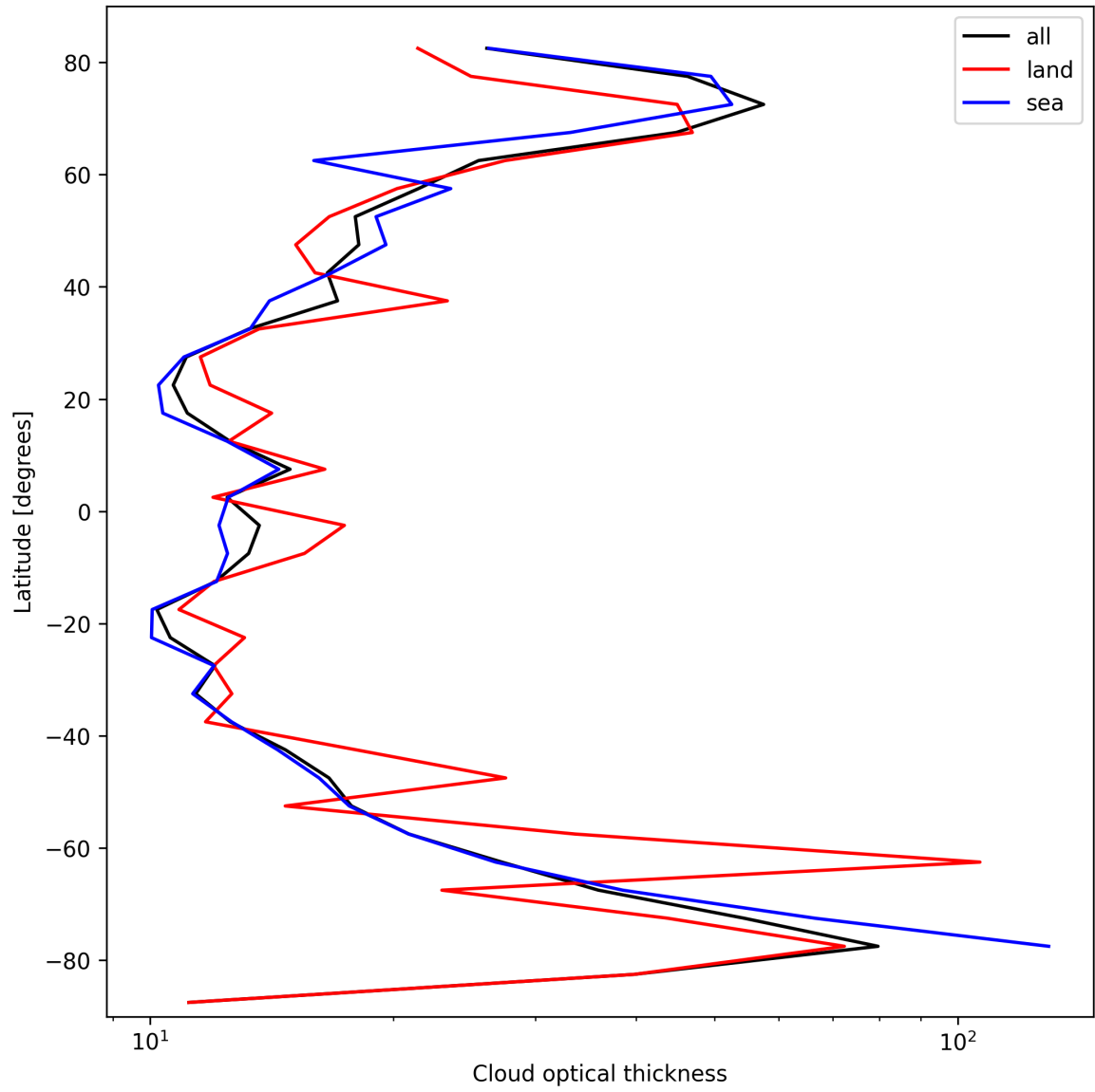
Figure 25: Zonal average of “Cloud optical thickness” for 2025-10-07 to 2025-10-09.
