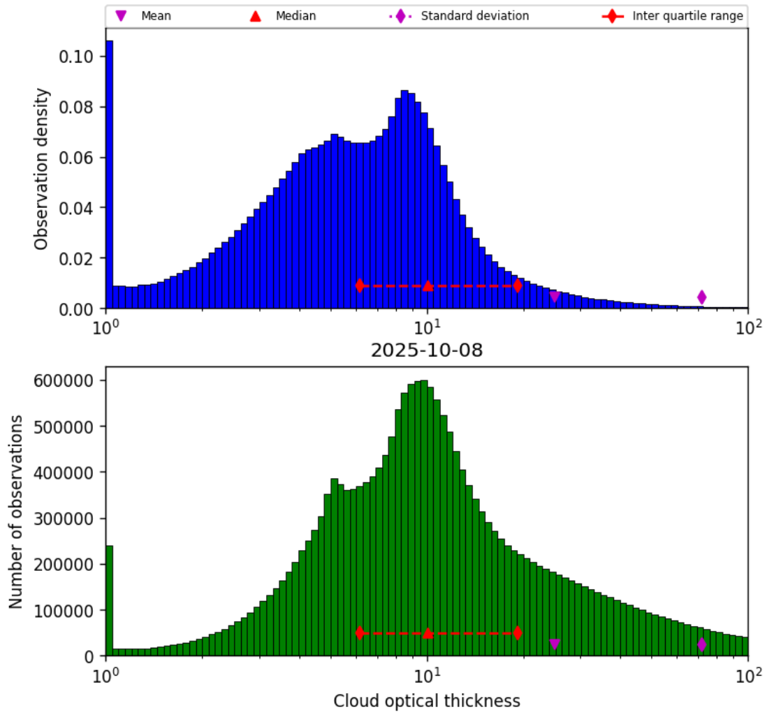
Figure 41: Histogram of “Cloud optical thickness” for 2025-10-07 to 2025-10-09
