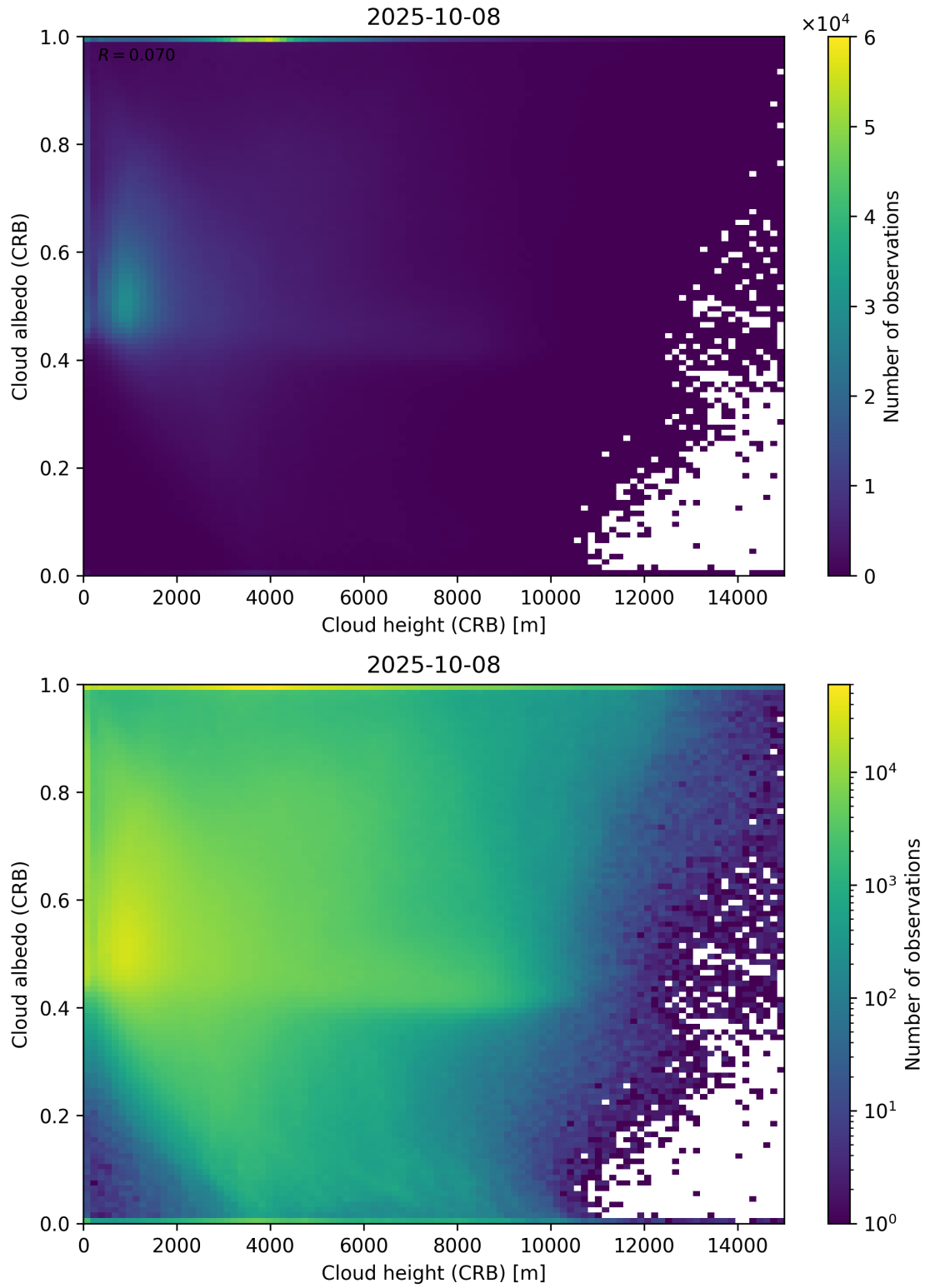
Figure 80: Scatter density plot of “Cloud height (CRB)” against “Cloud albedo (CRB)” for 2025-10-07 to 2025-10-09.
