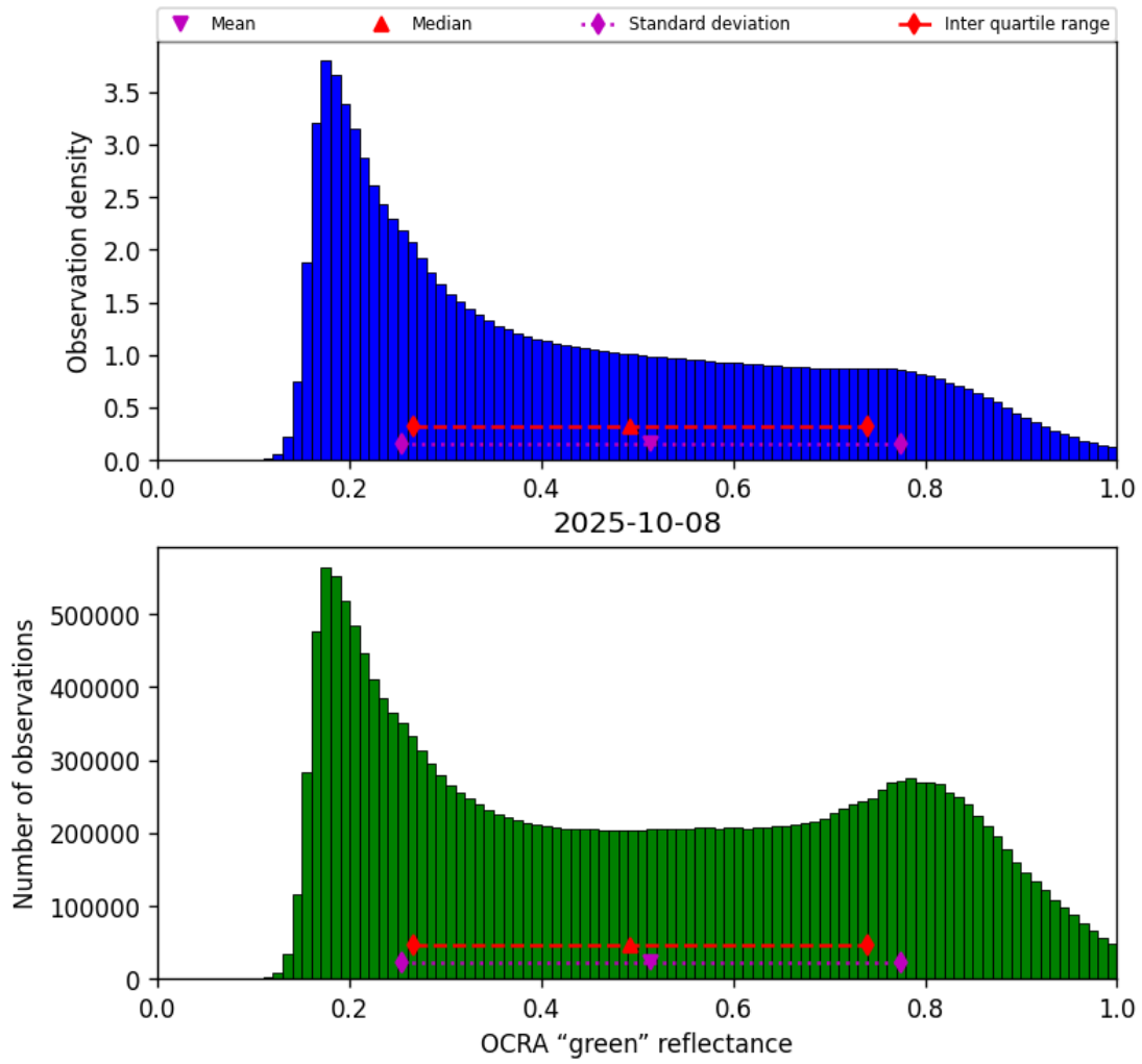
Figure 52: Histogram of “OCRA “green” reflectance” for 2025-10-07 to 2025-10-09
