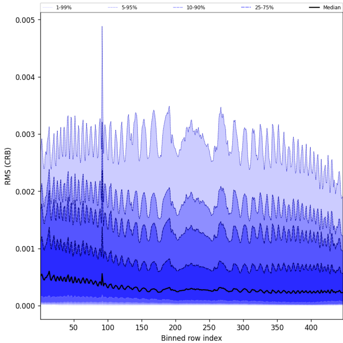
Figure 64: Along track statistics of “RMS (CRB)” for 2025-10-07 to 2025-10-09
