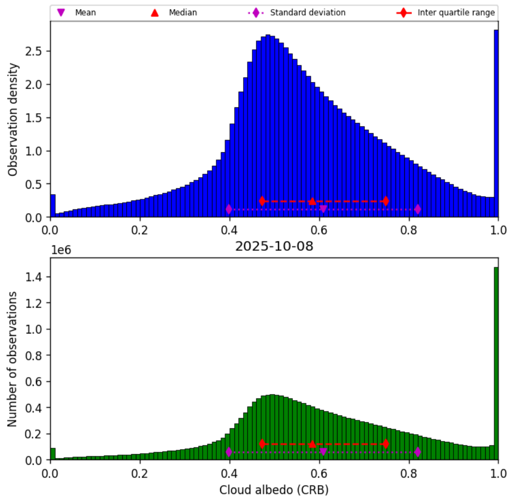
Figure 44: Histogram of “Cloud albedo (CRB)” for 2025-10-07 to 2025-10-09
