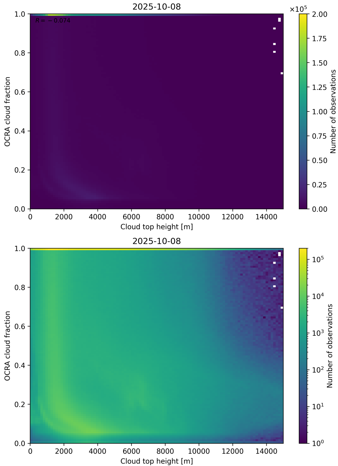
Figure 87: Scatter density plot of “Cloud top height” against “OCRA cloud fraction” for 2025-10-07 to 2025-10-09.
