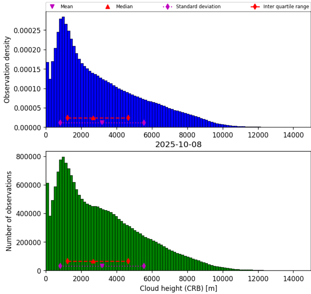
Figure 43: Histogram of “Cloud height (CRB)” for 2025-10-07 to 2025-10-09
