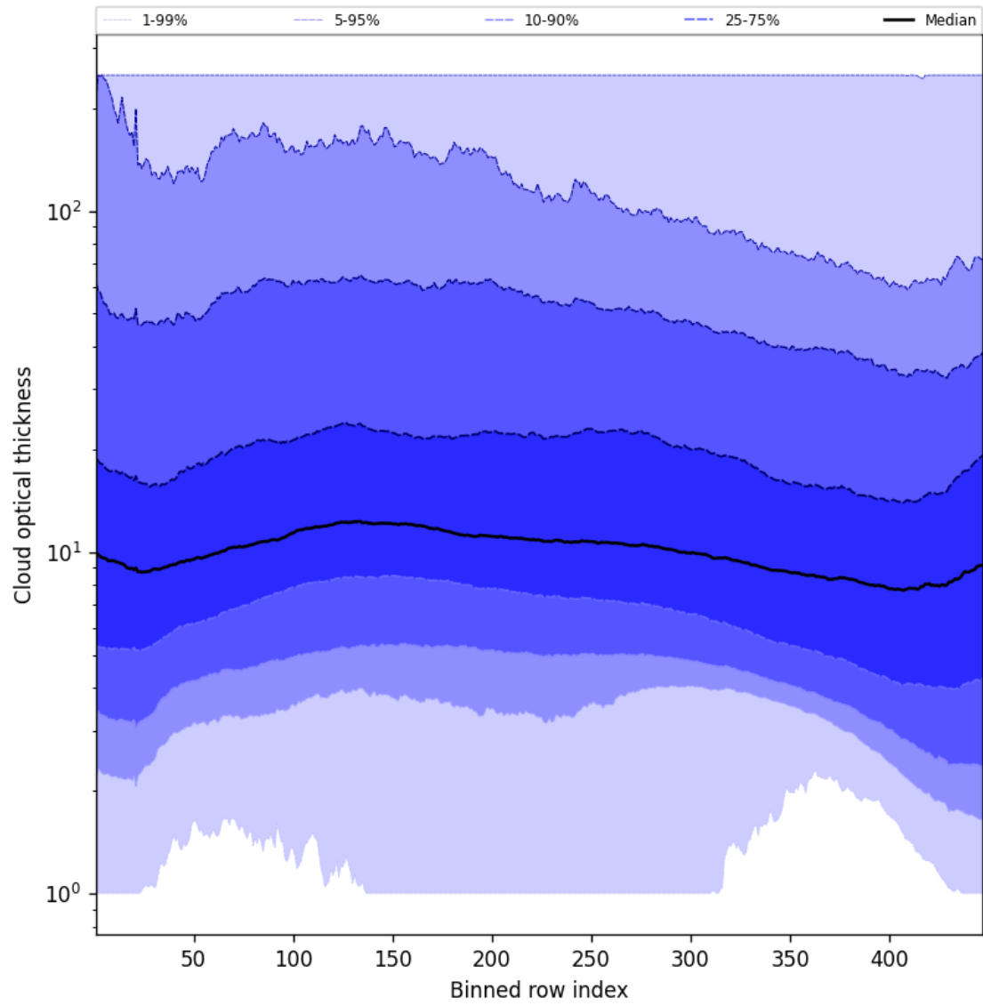
Figure 57: Along track statistics of “Cloud optical thickness” for 2025-10-07 to 2025-10-09
