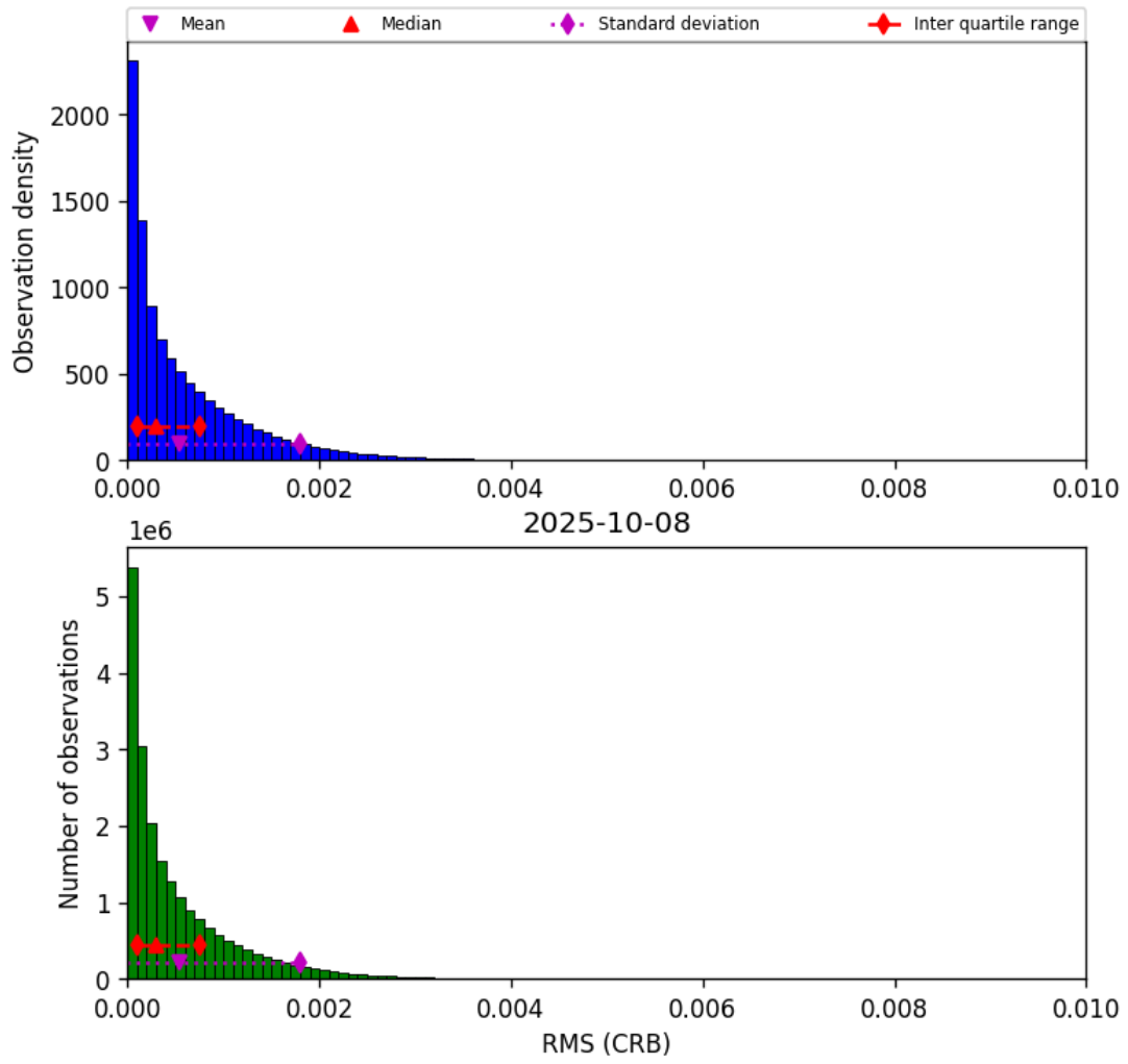
Figure 48: Histogram of “RMS (CRB)” for 2025-10-07 to 2025-10-09
