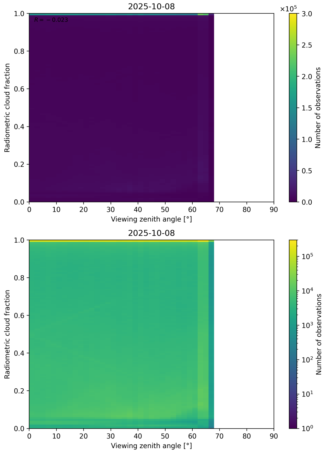
Figure 107: Scatter density plot of “Viewing zenith angle” against “Radiometric cloud fraction” for 2025-10-07 to 2025-10-09.
