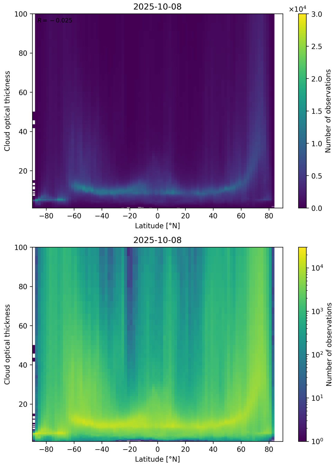
Figure 96: Scatter density plot of “Latitude” against “Cloud optical thickness” for 2025-10-07 to 2025-10-09.
