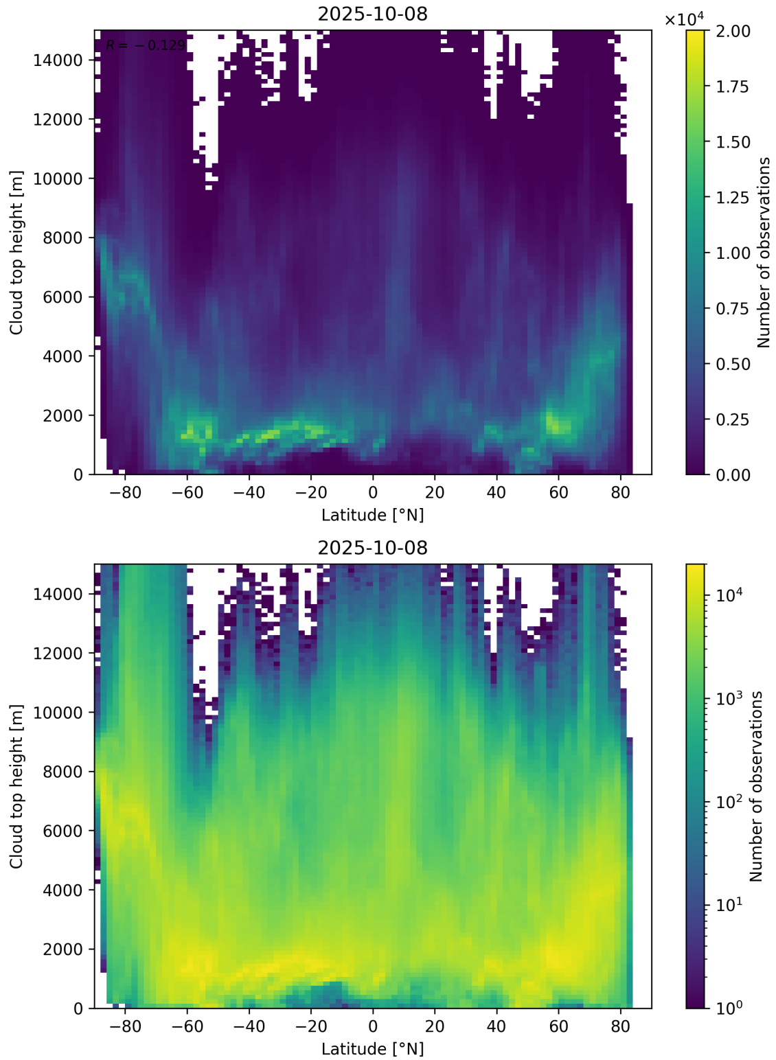
Figure 97: Scatter density plot of “Latitude” against “Cloud top height” for 2025-10-07 to 2025-10-09.
