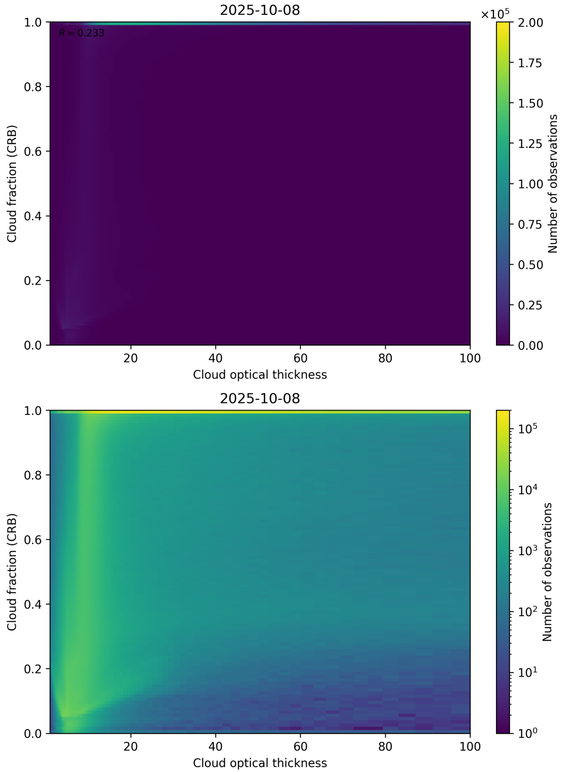
Figure 84: Scatter density plot of “Cloud optical thickness” against “Cloud fraction (CRB)” for 2025-10-07 to 2025-10-09.
