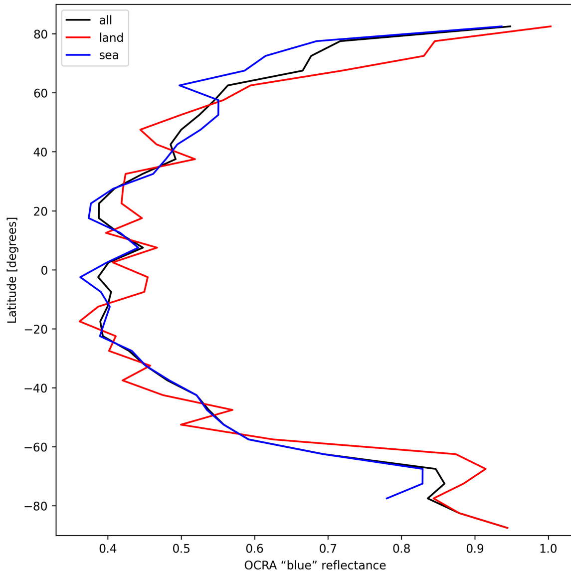
Figure 35: Zonal average of “OCRA “blue” reflectance” for 2025-10-07 to 2025-10-09.
