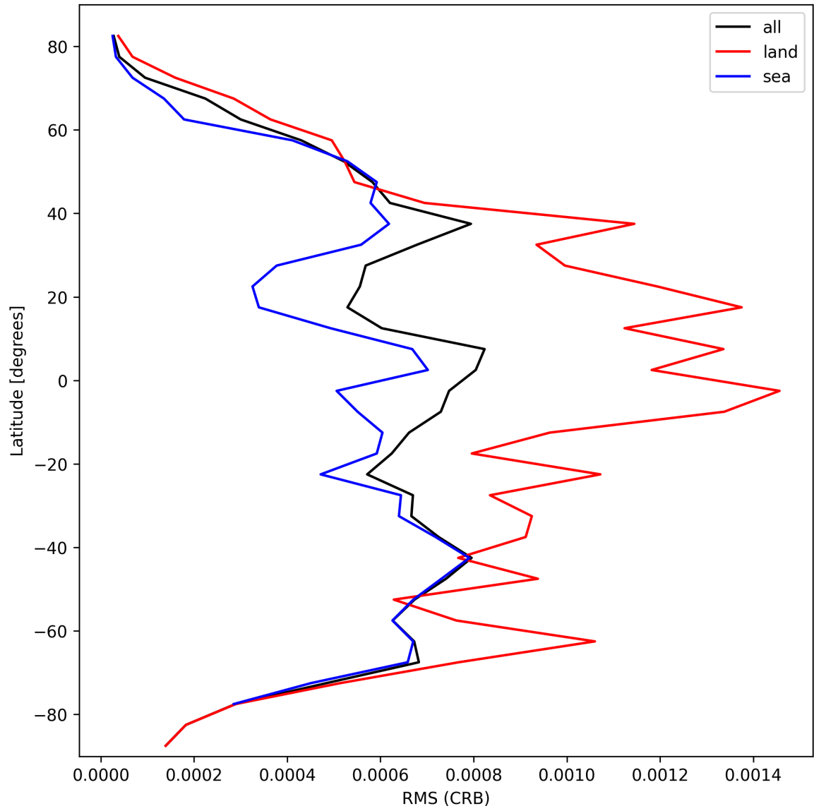
Figure 32: Zonal average of “RMS (CRB)” for 2025-10-07 to 2025-10-09.
