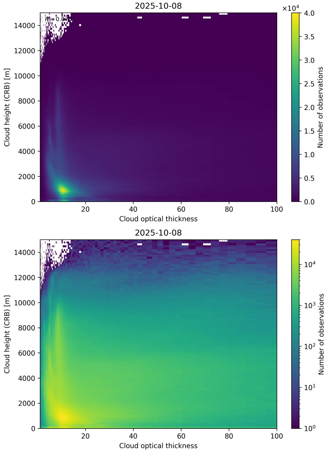
Figure 85: Scatter density plot of “Cloud optical thickness” against “Cloud height (CRB)” for 2025-10-07 to 2025-10-09.
