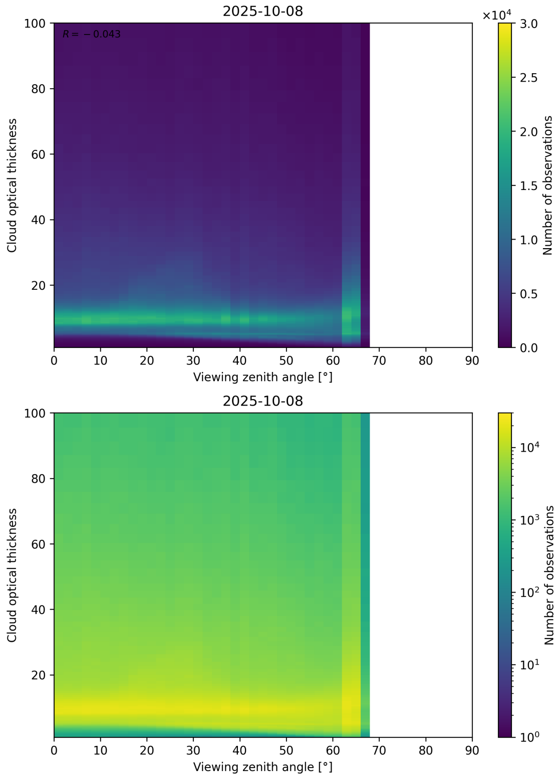
Figure 111: Scatter density plot of “Viewing zenith angle” against “Cloud optical thickness” for 2025-10-07 to 2025-10-09.
