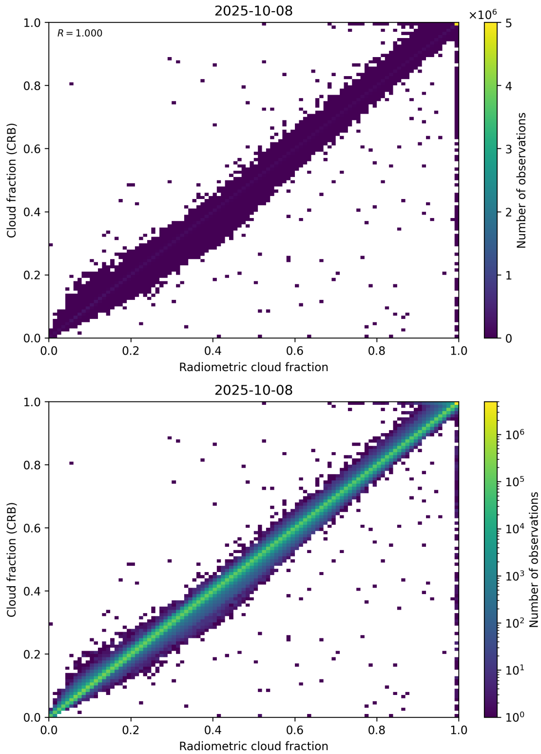
Figure 73: Scatter density plot of “Radiometric cloud fraction” against “Cloud fraction (CRB)” for 2025-10-07 to 2025-10-09.
