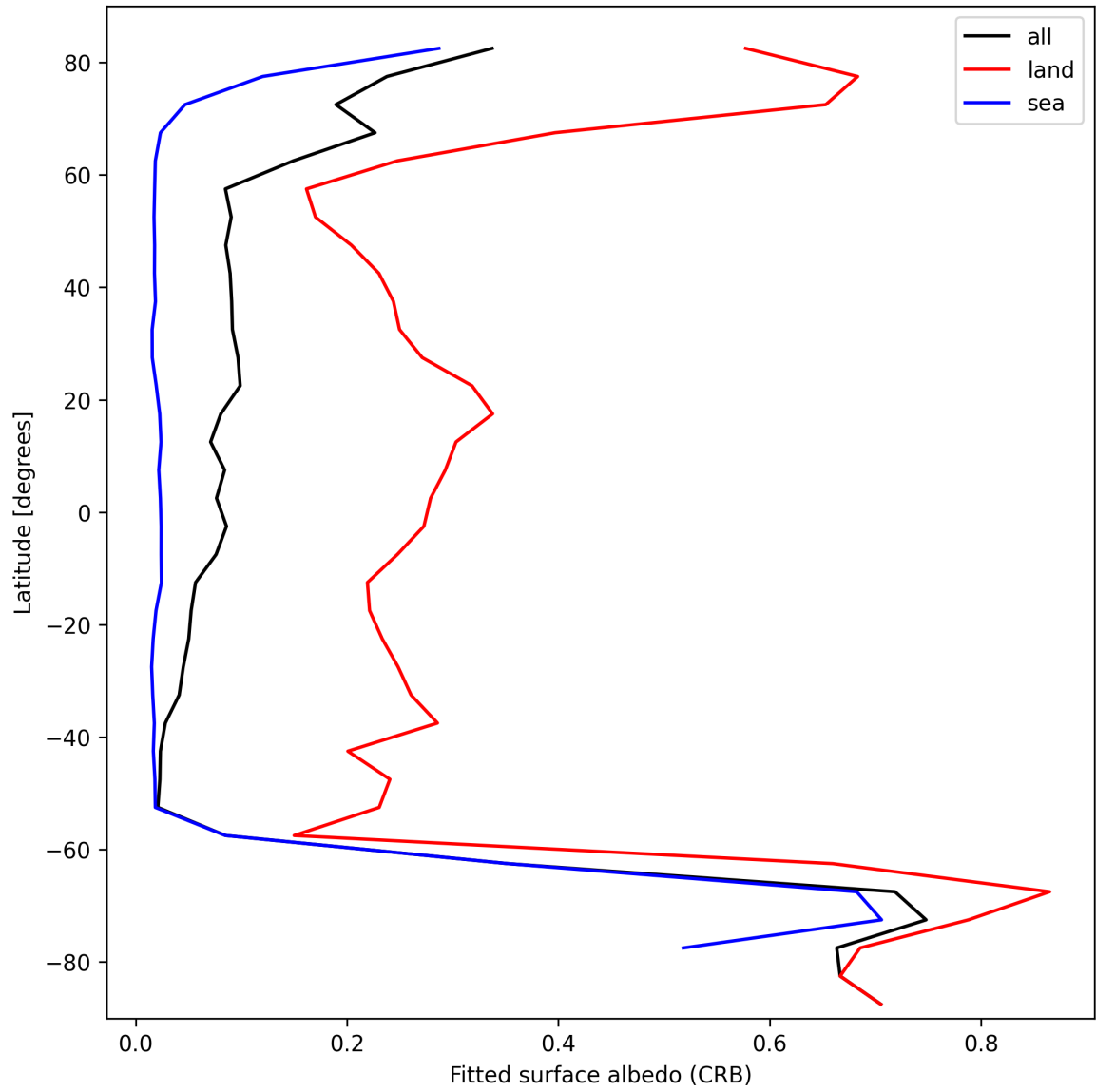
Figure 30: Zonal average of “Fitted surface albedo (CRB)” for 2025-10-07 to 2025-10-09.
