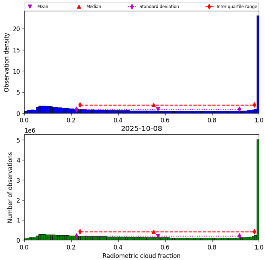
Figure 39: Histogram of “Radiometric cloud fraction” for 2025-10-07 to 2025-10-09
