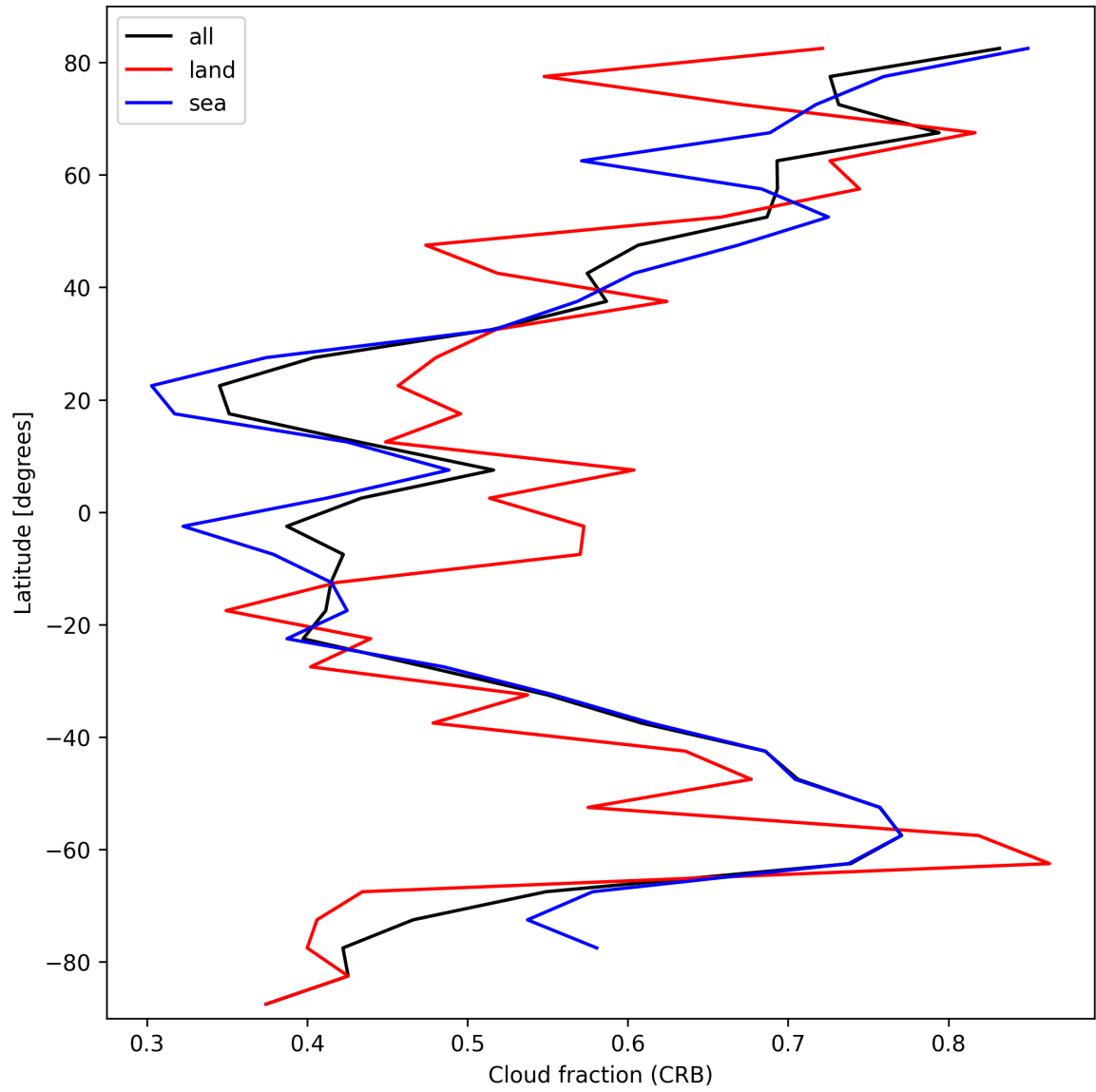
Figure 26: Zonal average of “Cloud fraction (CRB)” for 2025-10-07 to 2025-10-09.
