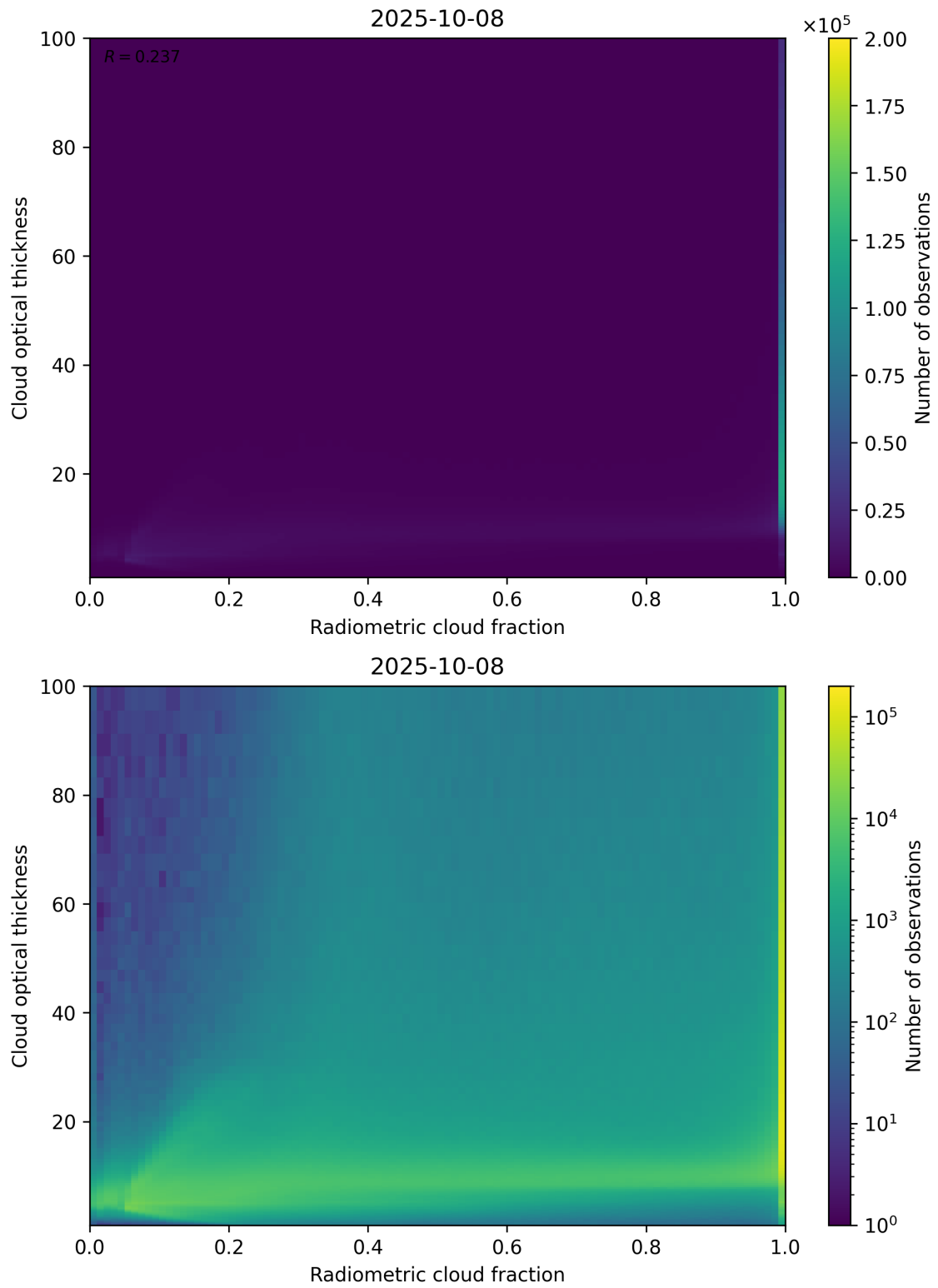
Figure 75: Scatter density plot of “Radiometric cloud fraction” against “Cloud optical thickness” for 2025-10-07 to 2025-10-09.
