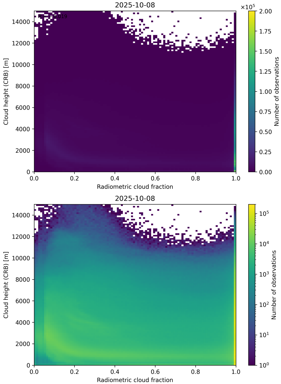
Figure 74: Scatter density plot of “Radiometric cloud fraction” against “Cloud height (CRB)” for 2025-10-07 to 2025-10-09.
