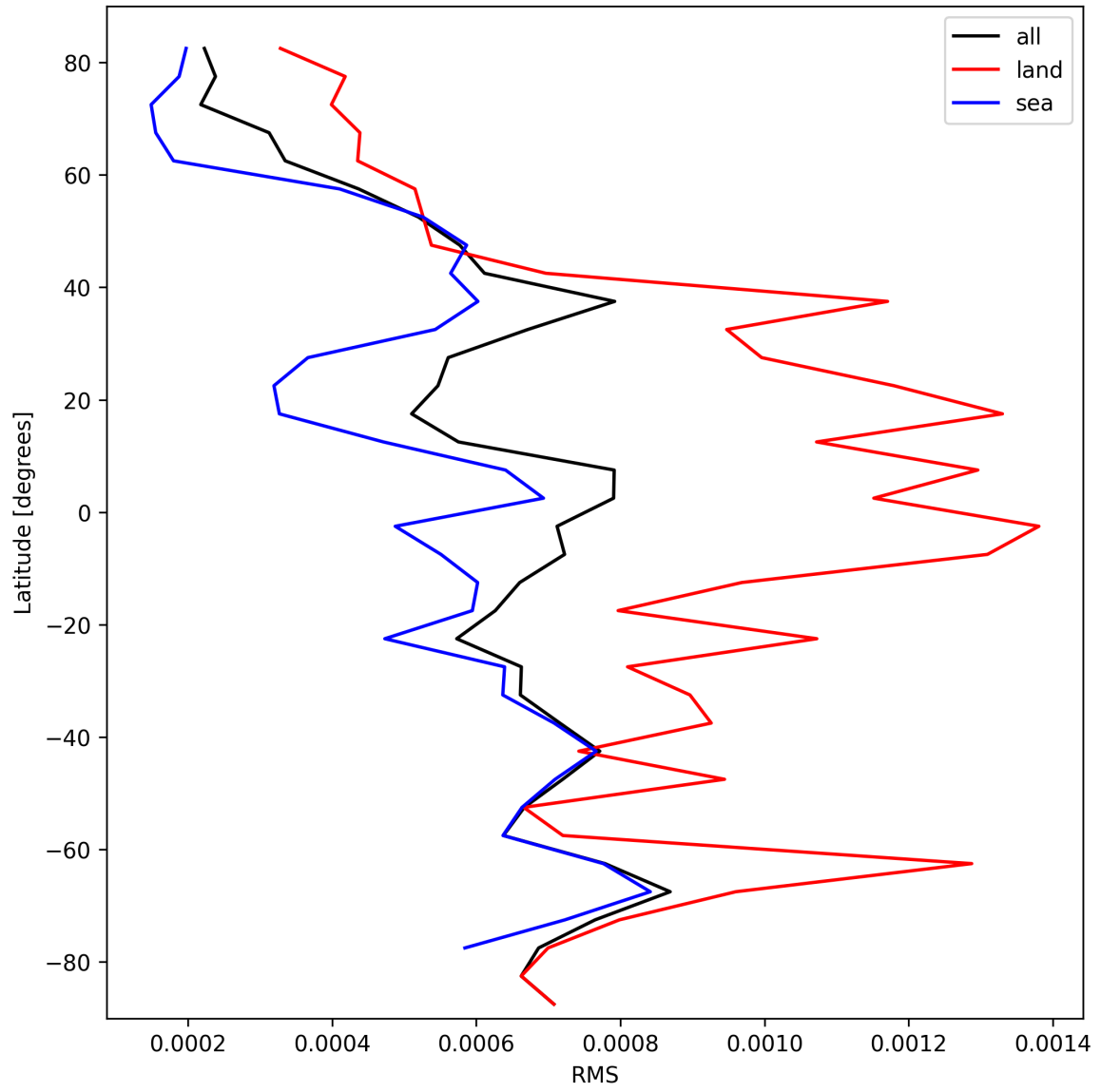
Figure 31: Zonal average of “RMS” for 2025-10-07 to 2025-10-09.
