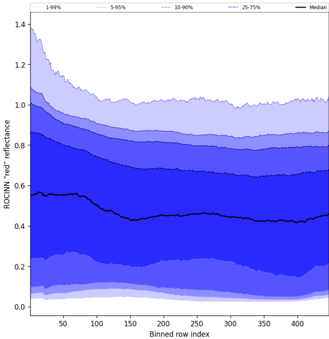
Figure 69: Along track statistics of "ROCINN "red" reflectance" for 2025-10-07 to 2025-10-09
