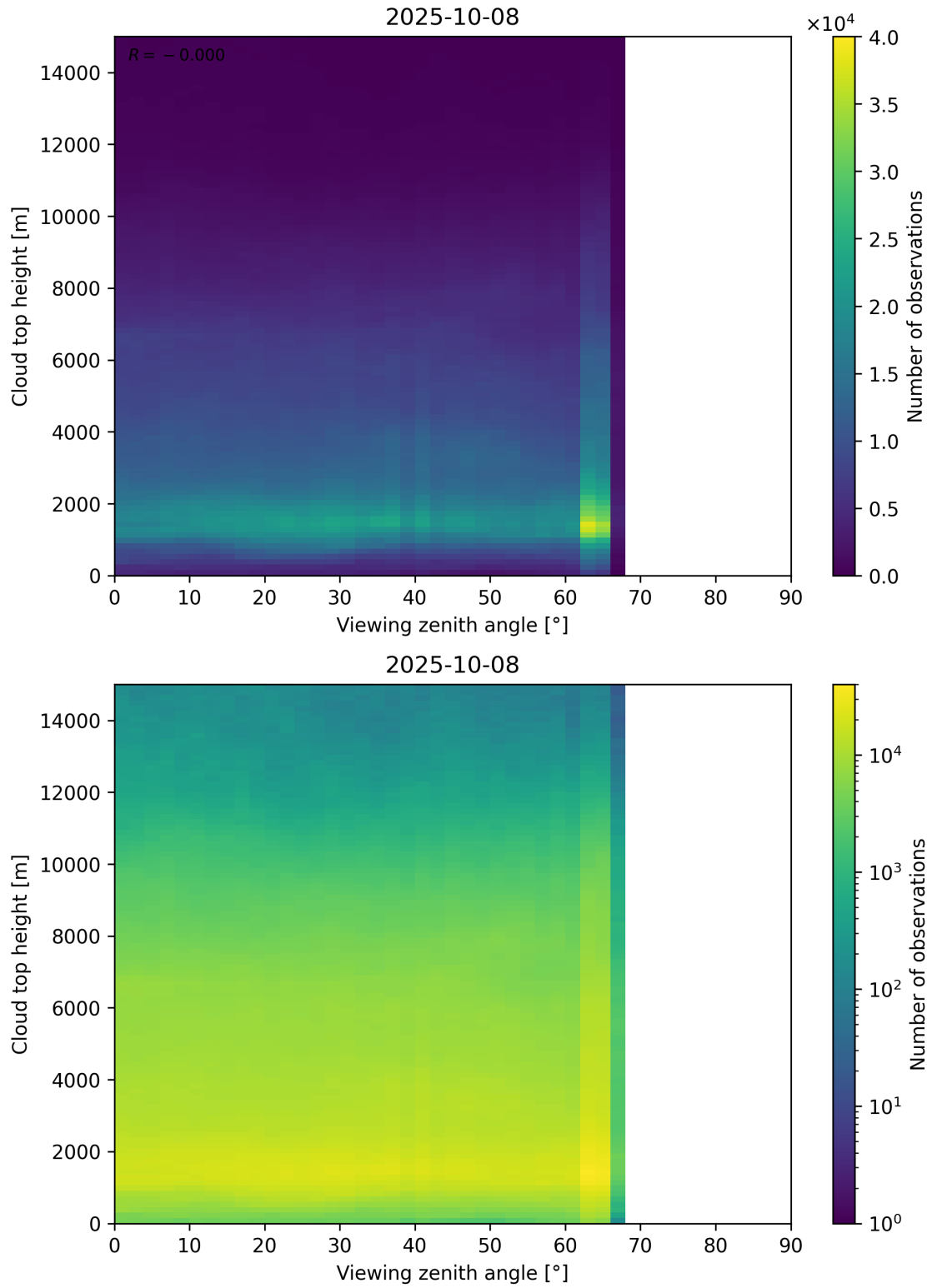
Figure 112: Scatter density plot of “Viewing zenith angle” against “Cloud top height” for 2025-10-07 to 2025-10-09.
