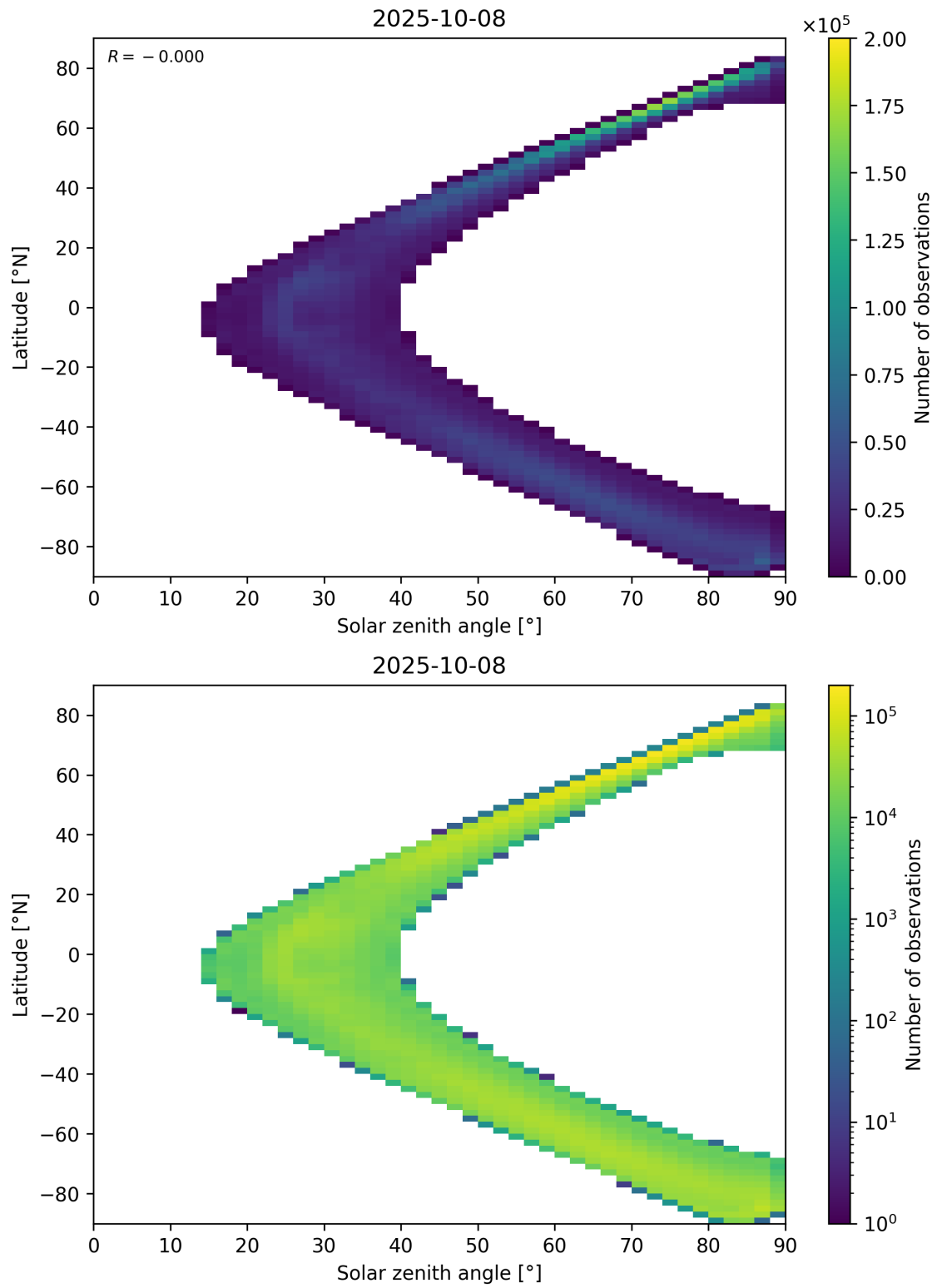
Figure 105: Scatter density plot of “Solar zenith angle” against “Latitude” for 2025-10-07 to 2025-10-09.
