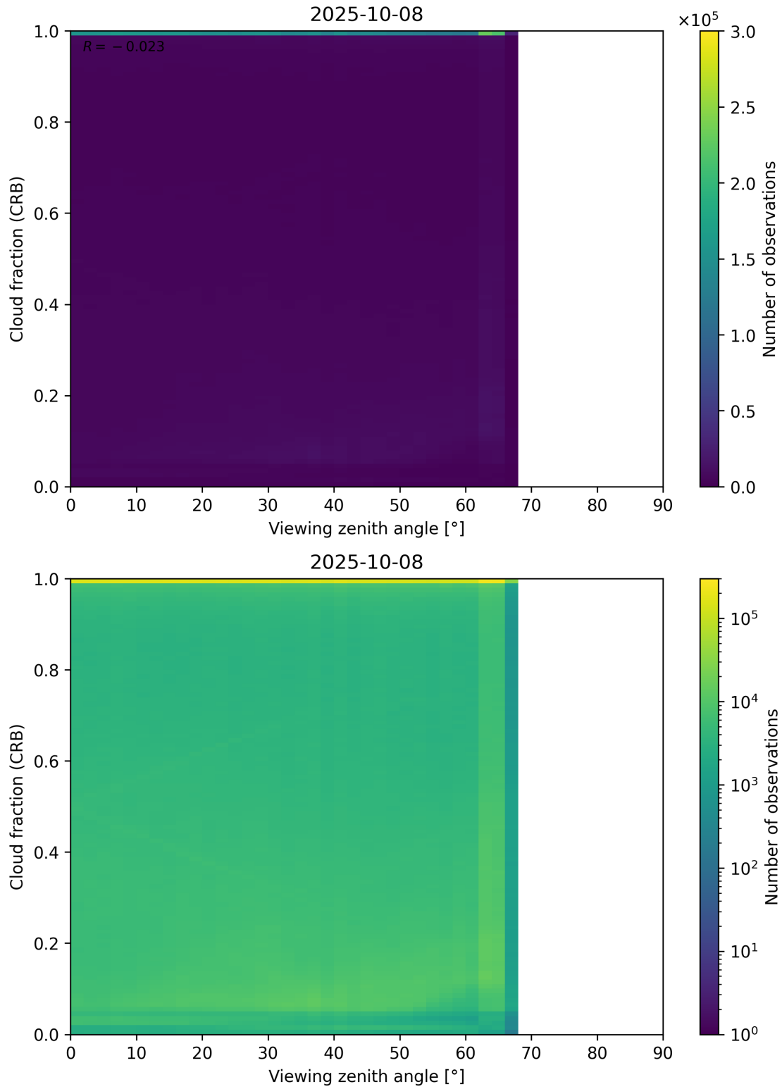
Figure 109: Scatter density plot of “Viewing zenith angle” against “Cloud fraction (CRB)” for 2025-10-07 to 2025-10-09.
