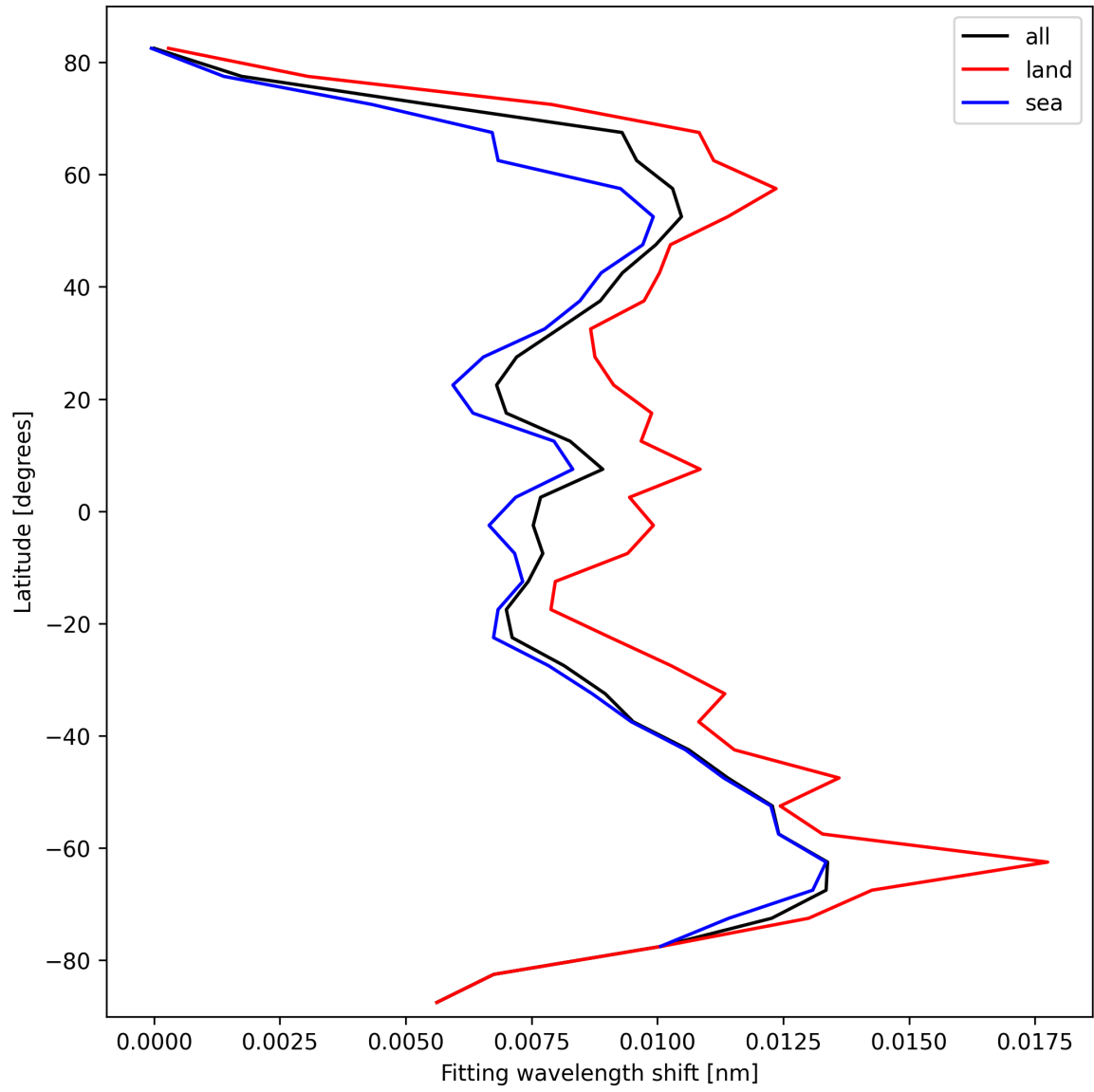
Figure 33: Zonal average of “Fitting wavelength shift” for 2025-10-07 to 2025-10-09.
