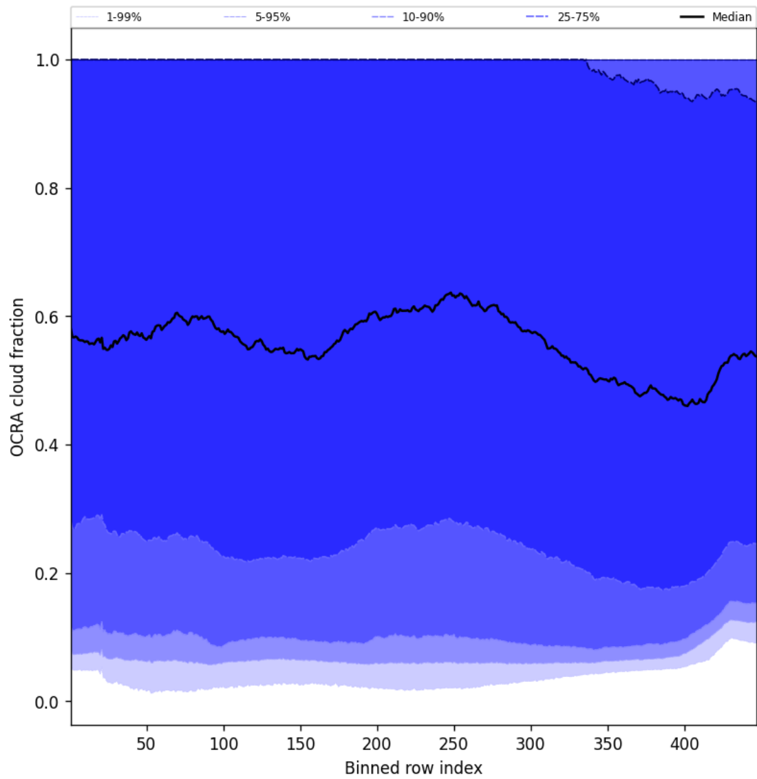
Figure 66: Along track statistics of “OCRA cloud fraction” for 2025-10-07 to 2025-10-09
