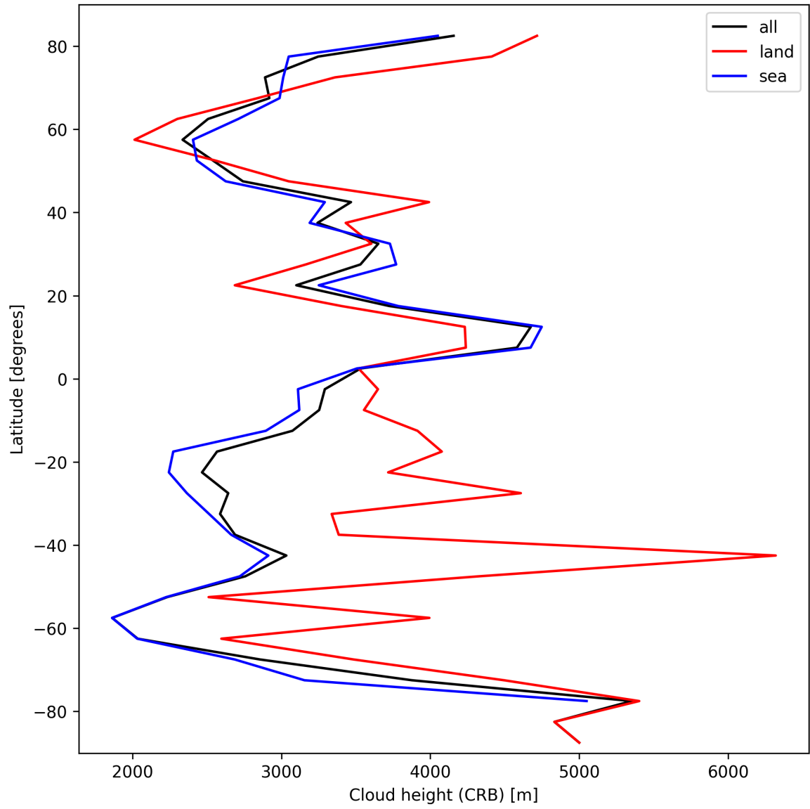
Figure 27: Zonal average of “Cloud height (CRB)” for 2025-10-07 to 2025-10-09.
