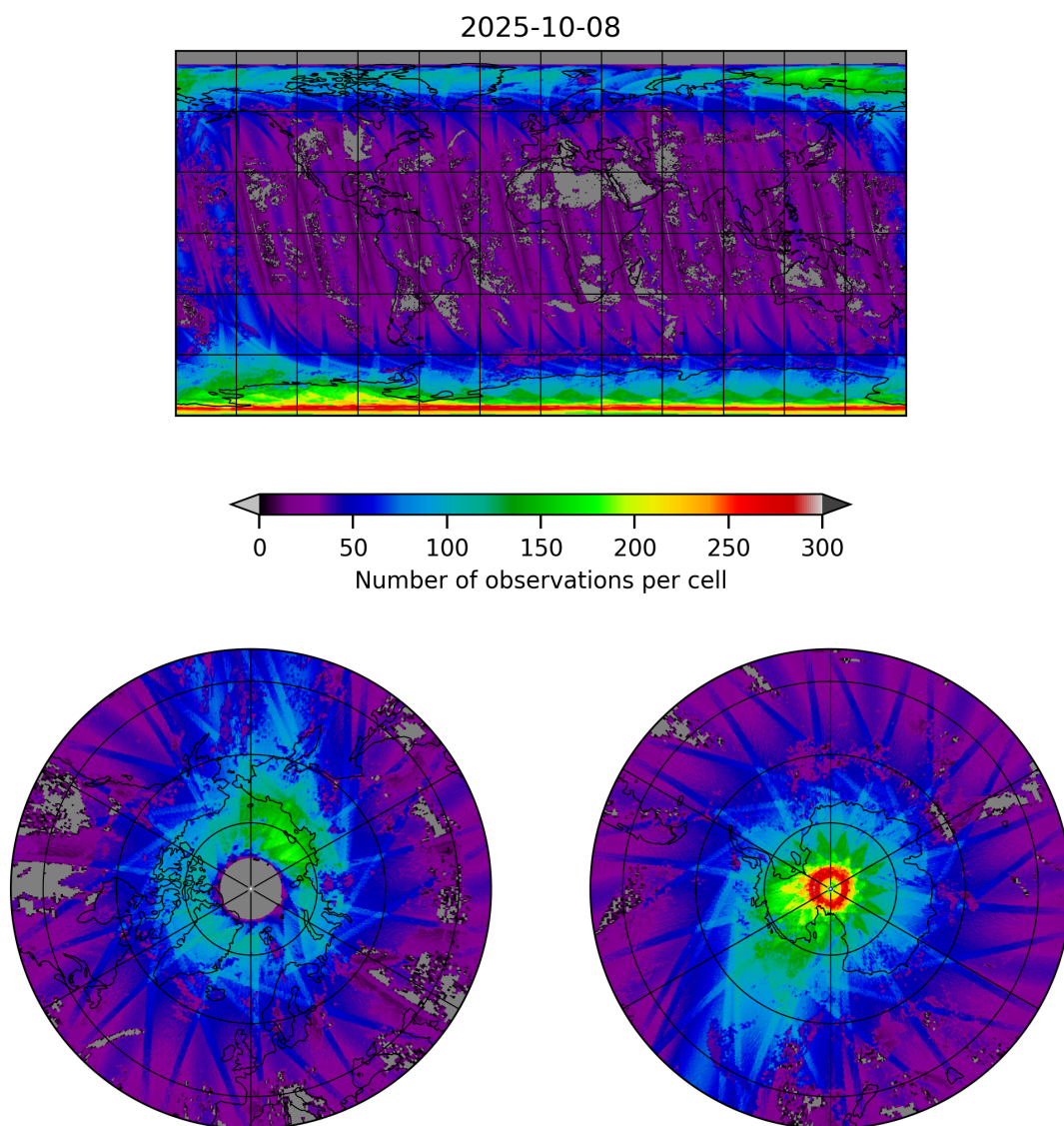
Figure 21: Map of the number of observations for 2025-10-07 to 2025-10-09
