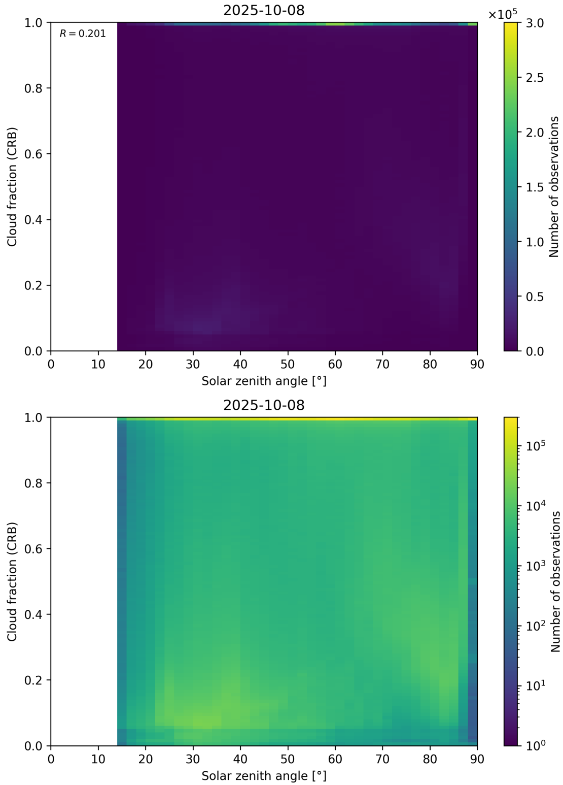
Figure 101: Scatter density plot of “Solar zenith angle” against “Cloud fraction (CRB)” for 2025-10-07 to 2025-10-09.
