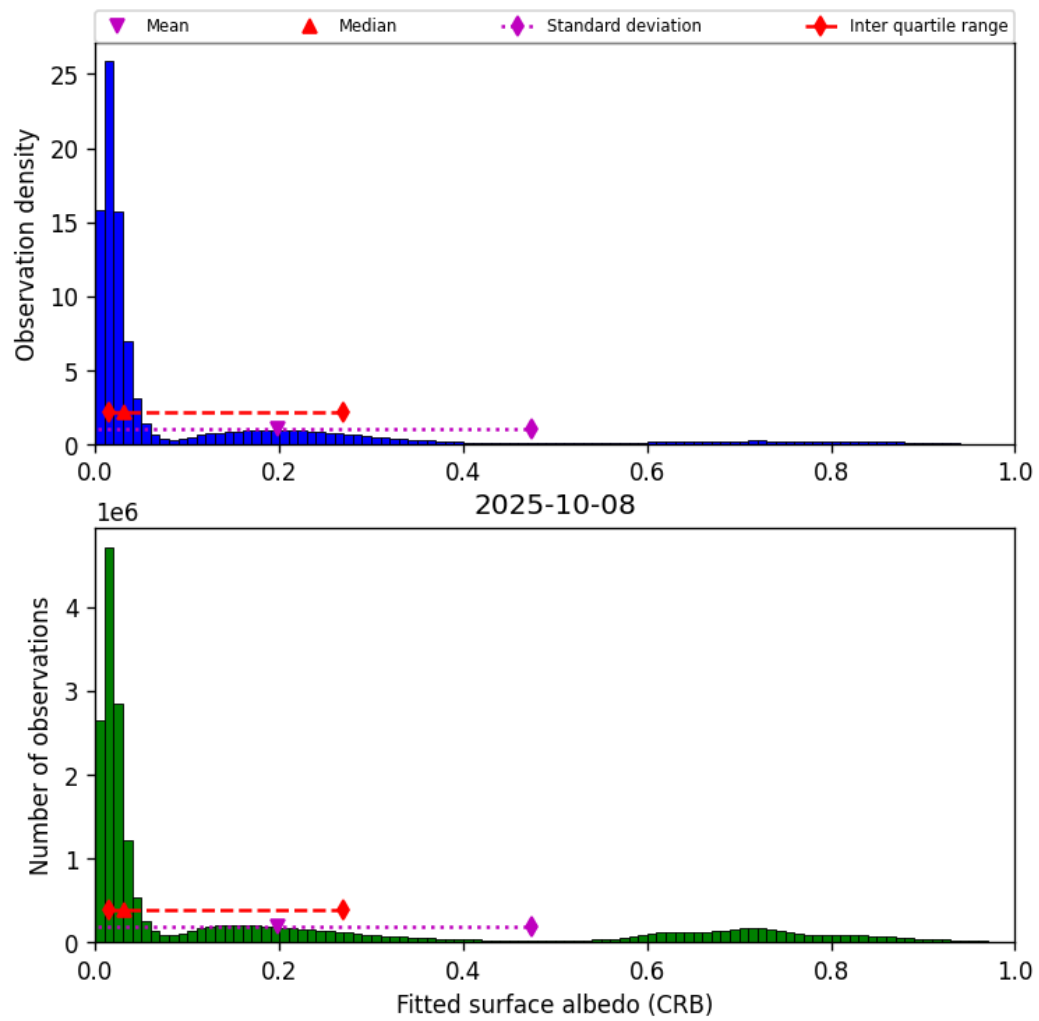
Figure 46: Histogram of “Fitted surface albedo (CRB)” for 2025-10-07 to 2025-10-09
