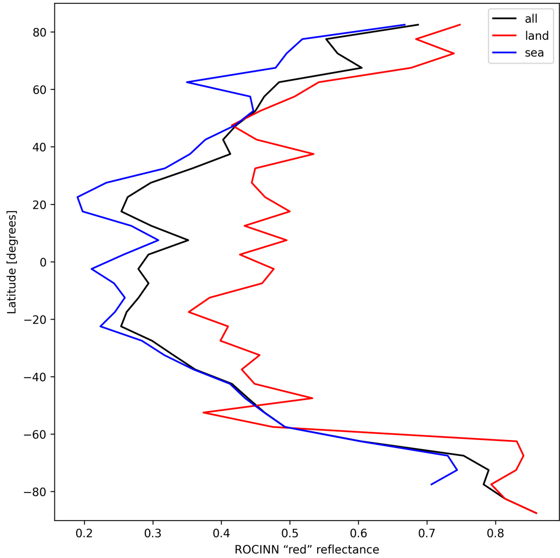
Figure 37: Zonal average of “ROCINN “red” reflectance” for 2025-10-07 to 2025-10-09.
