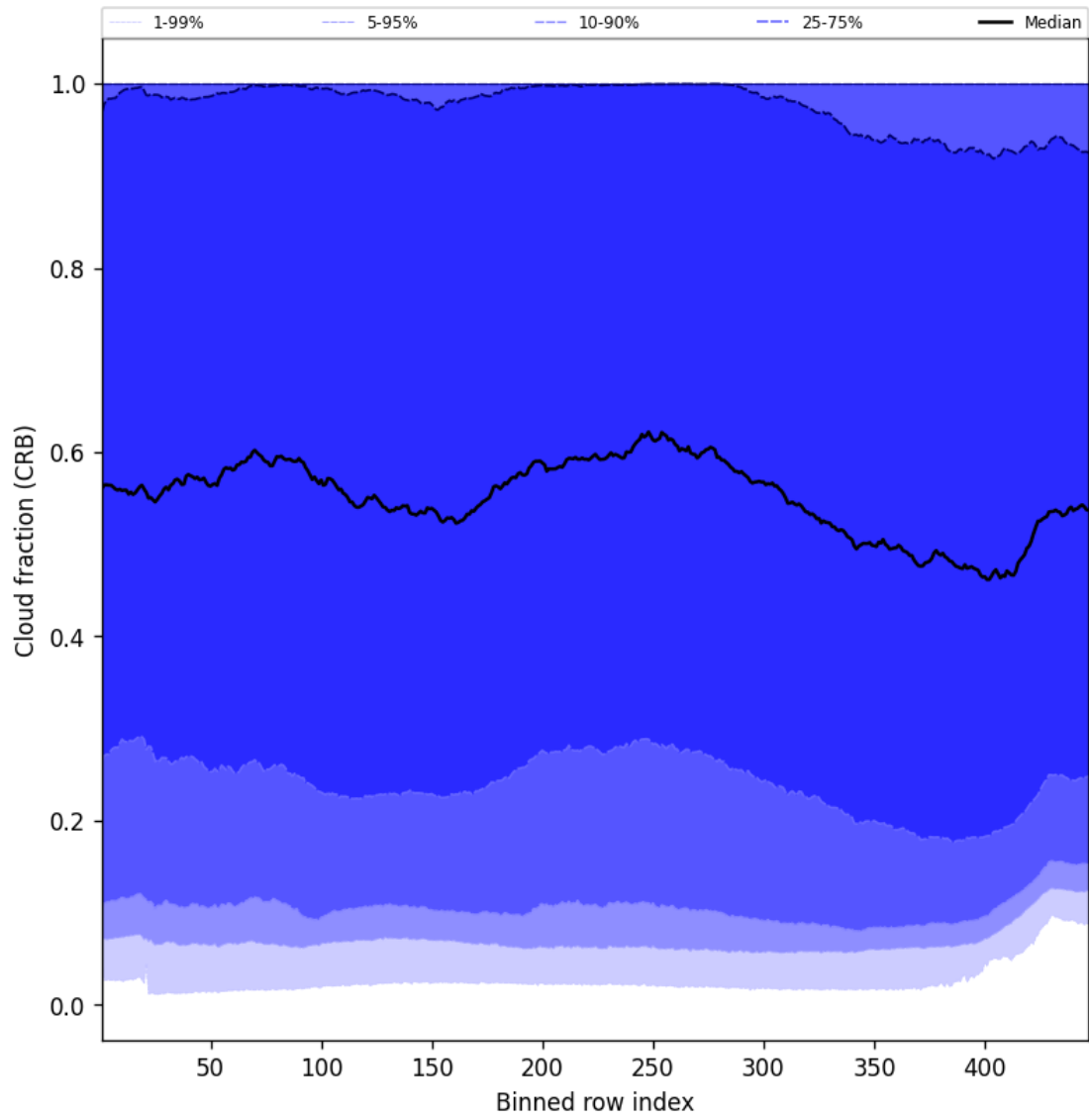
Figure 58: Along track statistics of “Cloud fraction (CRB)” for 2025-10-07 to 2025-10-09
