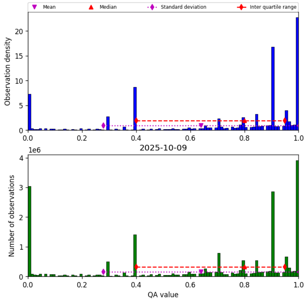
Figure 38: Histogram of “QA value” for 2025-10-08 to 2025-10-10
