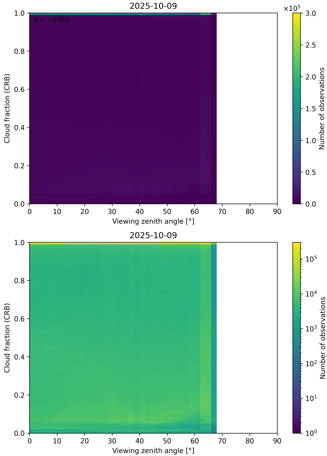
Figure 109: Scatter density plot of “Viewing zenith angle” against “Cloud fraction (CRB)” for 2025-10-08 to 2025-10-10.
