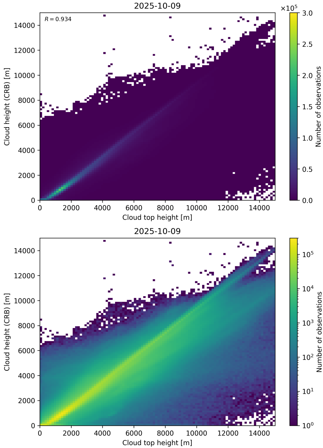
Figure 89: Scatter density plot of “Cloud top height” against “Cloud height (CRB)” for 2025-10-08 to 2025-10-10.
