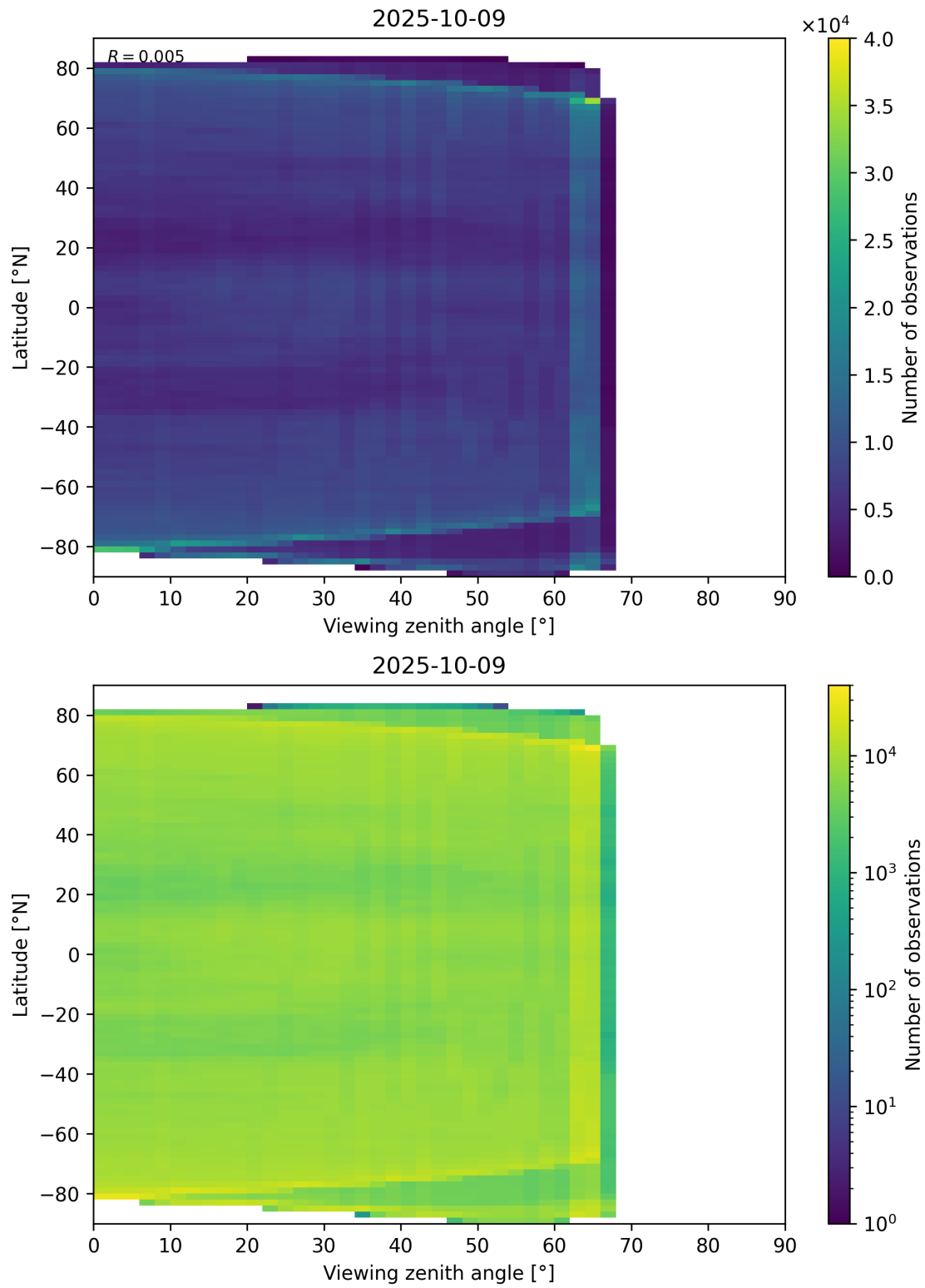
Figure 113: Scatter density plot of “Viewing zenith angle” against “Latitude” for 2025-10-08 to 2025-10-10.
