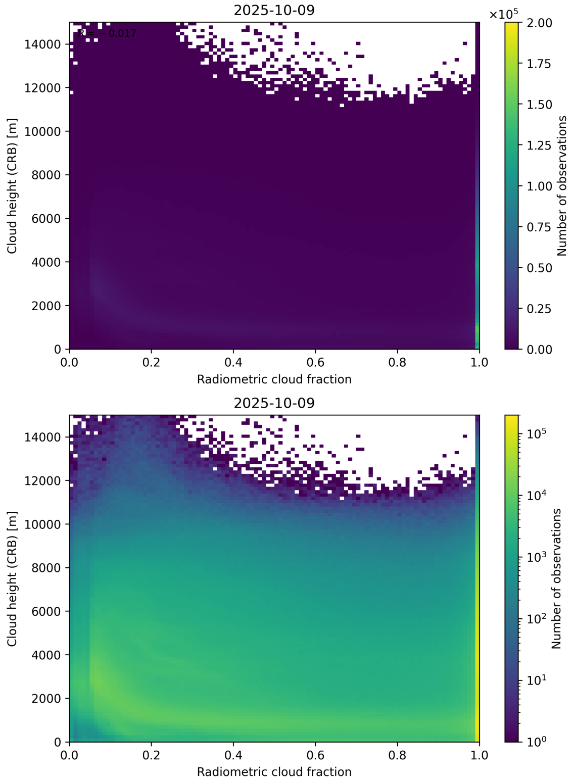
Figure 74: Scatter density plot of “Radiometric cloud fraction” against “Cloud height (CRB)” for 2025-10-08 to 2025-10-10.
