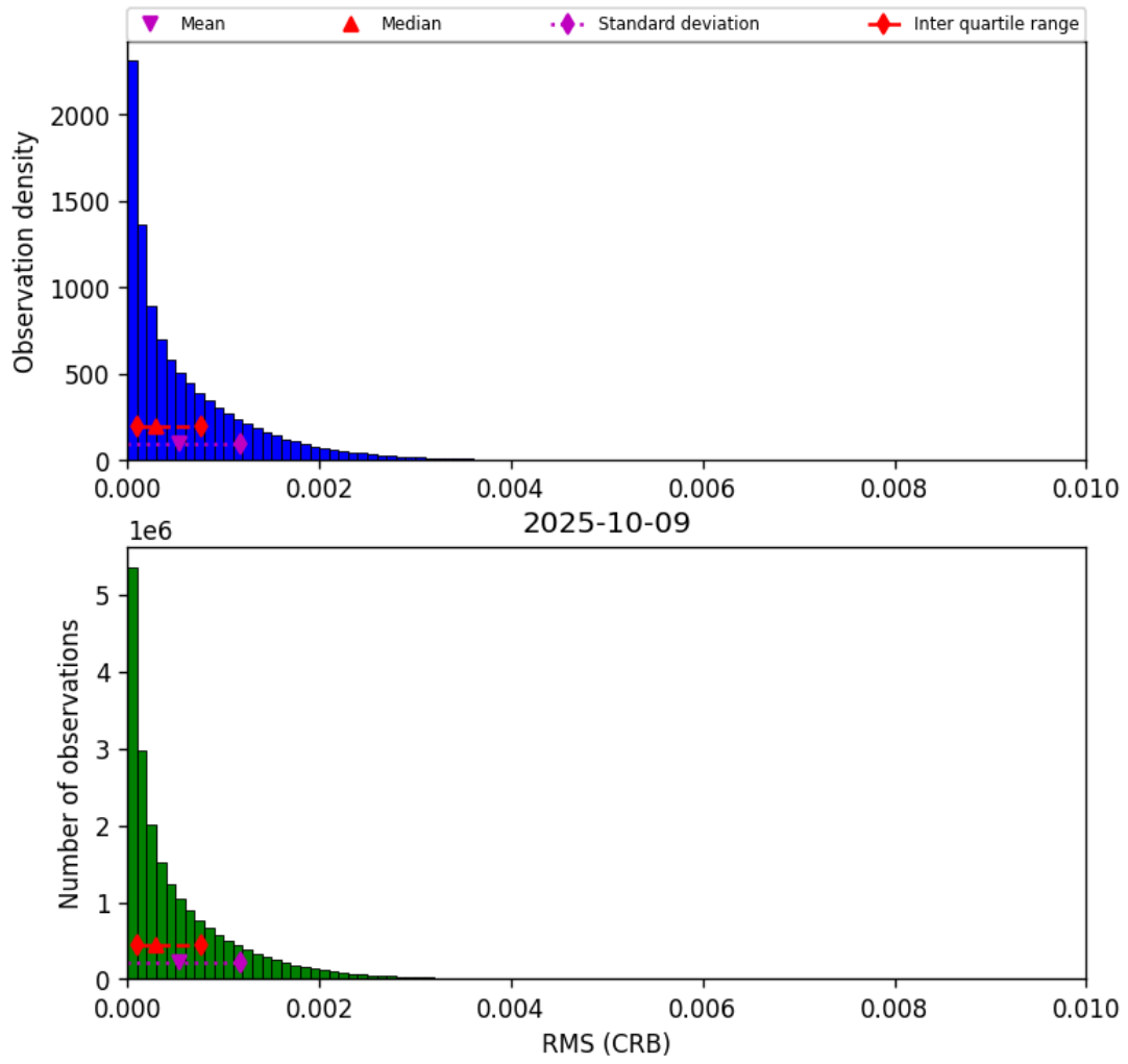
Figure 48: Histogram of “RMS (CRB)” for 2025-10-08 to 2025-10-10
