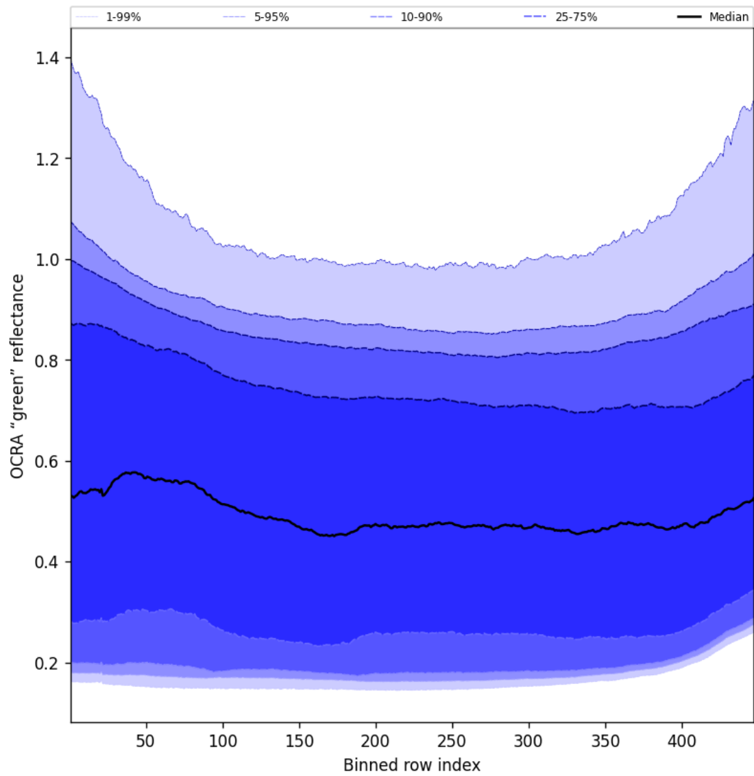
Figure 68: Along track statistics of “OCRA “green” reflectance” for 2025-10-08 to 2025-10-10
