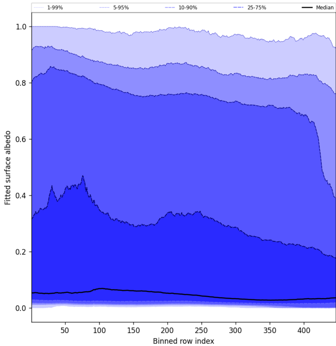
Figure 61: Along track statistics of “Fitted surface albedo” for 2025-10-08 to 2025-10-10
