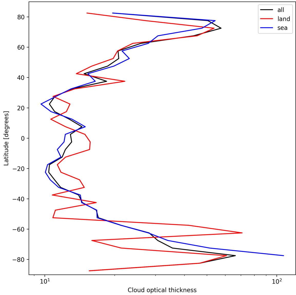
Figure 25: Zonal average of “Cloud optical thickness” for 2025-10-08 to 2025-10-10.
