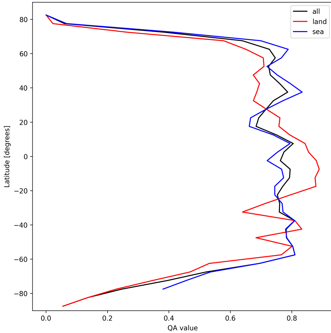
Figure 22: Zonal average of “QA value” for 2025-10-08 to 2025-10-10.
