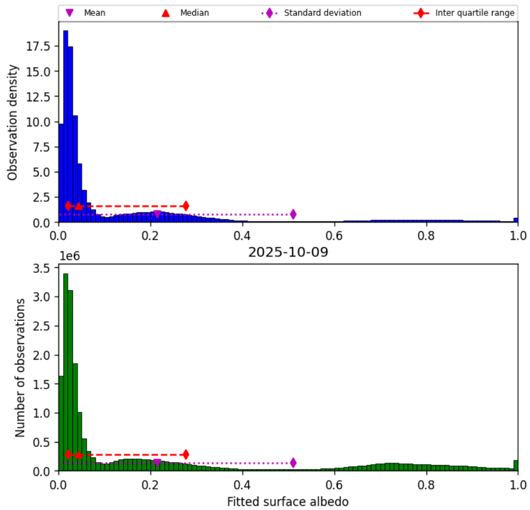
Figure 45: Histogram of “Fitted surface albedo” for 2025-10-08 to 2025-10-10
