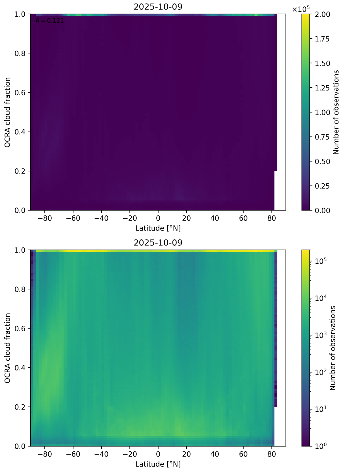
Figure 93: Scatter density plot of “Latitude” against “OCRA cloud fraction” for 2025-10-08 to 2025-10-10.
