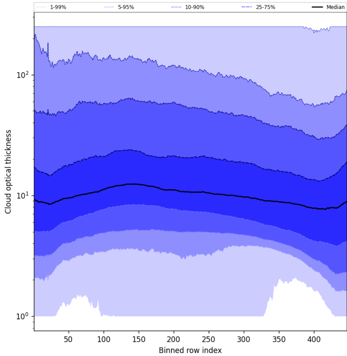
Figure 57: Along track statistics of “Cloud optical thickness” for 2025-10-08 to 2025-10-10
