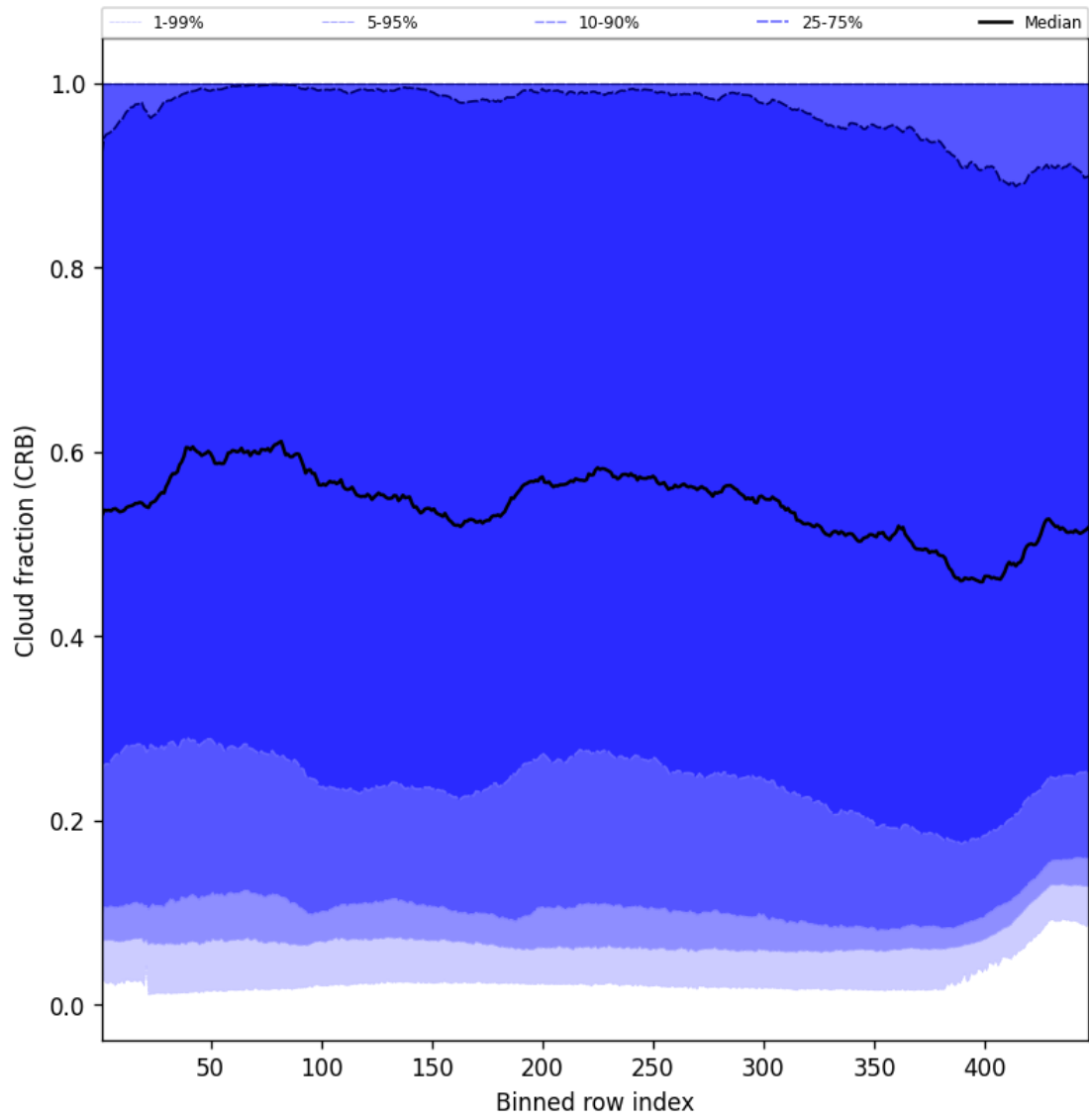
Figure 58: Along track statistics of “Cloud fraction (CRB)” for 2025-10-08 to 2025-10-10
