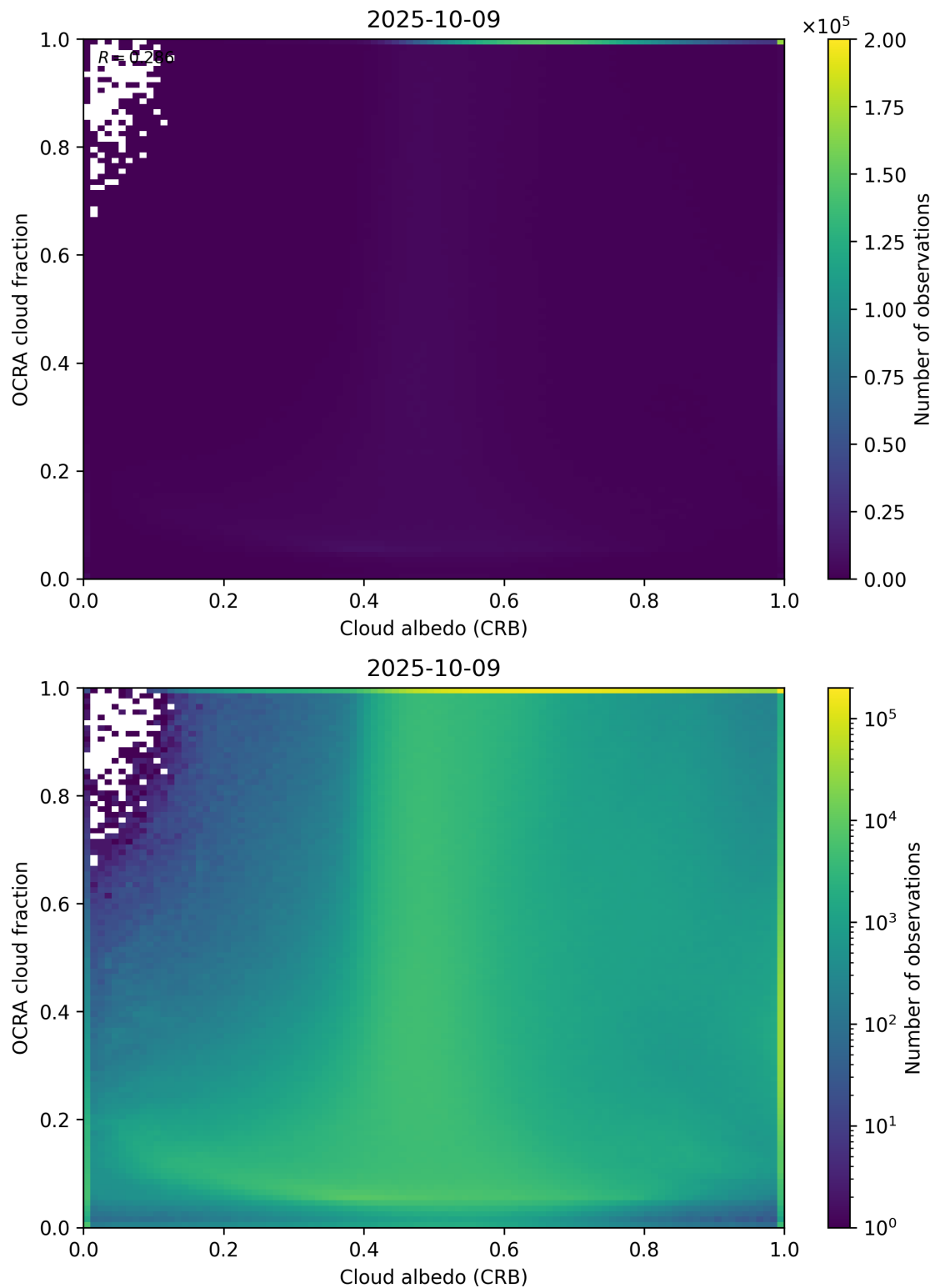
Figure 70: Scatter density plot of “Cloud albedo (CRB)” against “OCRA cloud fraction” for 2025-10-08 to 2025-10-10.
