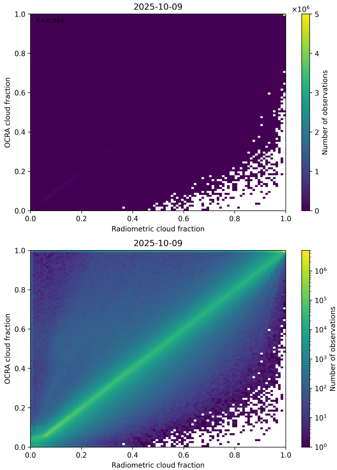
Figure 72: Scatter density plot of “Radiometric cloud fraction” against “OCRA cloud fraction” for 2025-10-08 to 2025-10-10.
