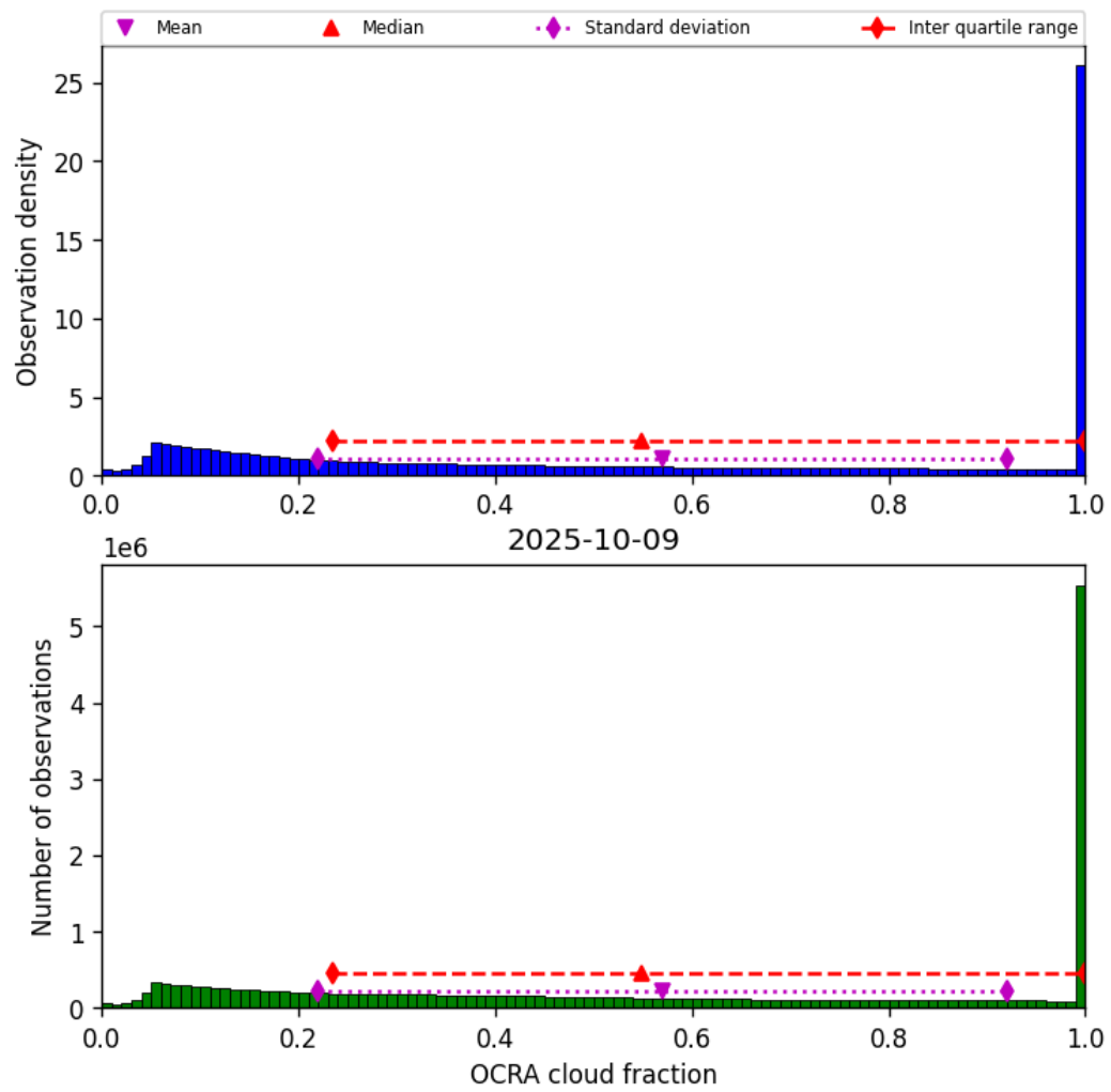
Figure 50: Histogram of “OCRA cloud fraction” for 2025-10-08 to 2025-10-10
