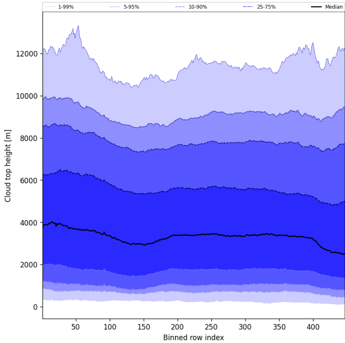
Figure 56: Along track statistics of “Cloud top height” for 2025-10-08 to 2025-10-10
