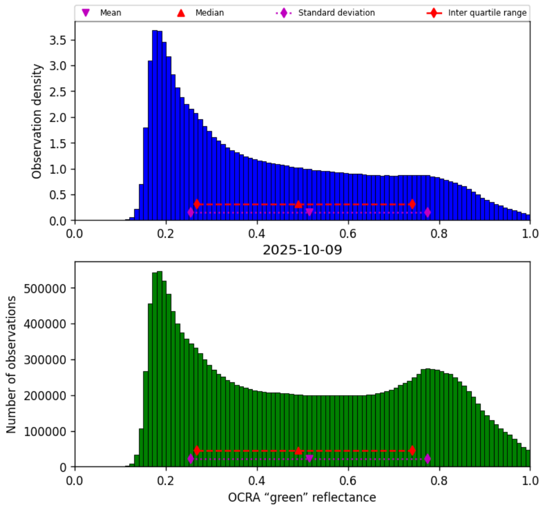
Figure 52: Histogram of “OCRA “green” reflectance” for 2025-10-08 to 2025-10-10
