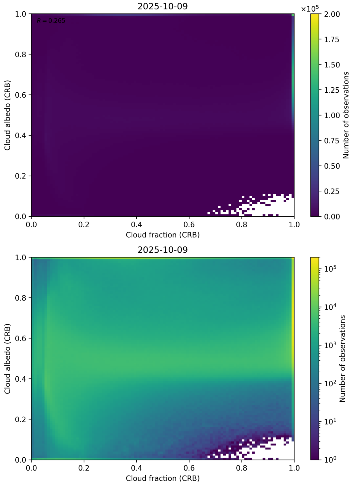
Figure 77: Scatter density plot of “Cloud fraction (CRB)” against “Cloud albedo (CRB)” for 2025-10-08 to 2025-10-10.
