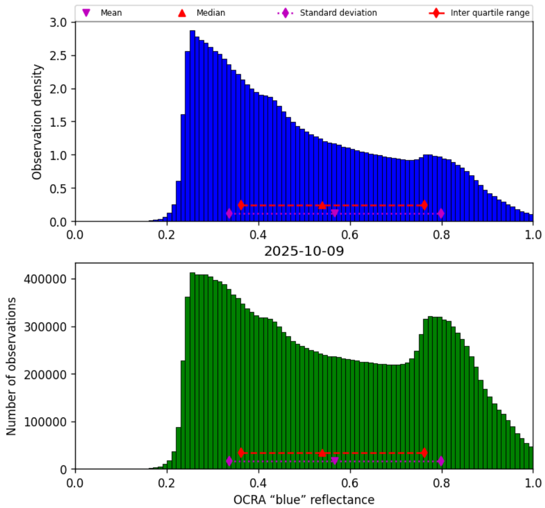
Figure 51: Histogram of “OCRA “blue” reflectance” for 2025-10-08 to 2025-10-10
