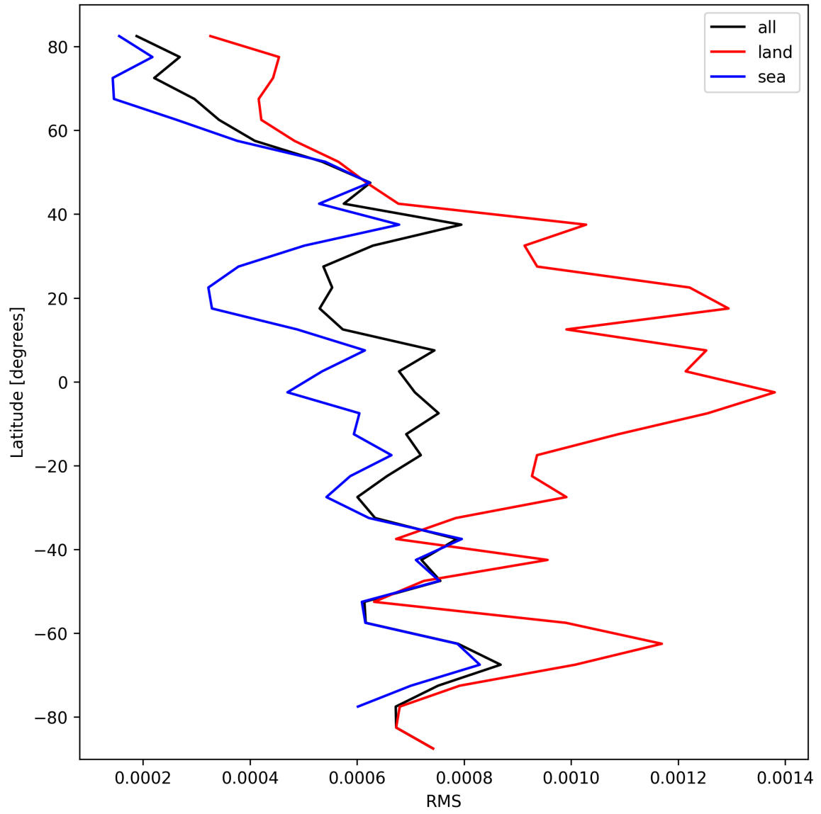
Figure 31: Zonal average of “RMS” for 2025-10-08 to 2025-10-10.
