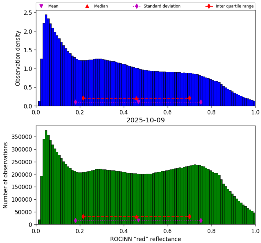
Figure 53: Histogram of “ROCINN “red” reflectance” for 2025-10-08 to 2025-10-10
