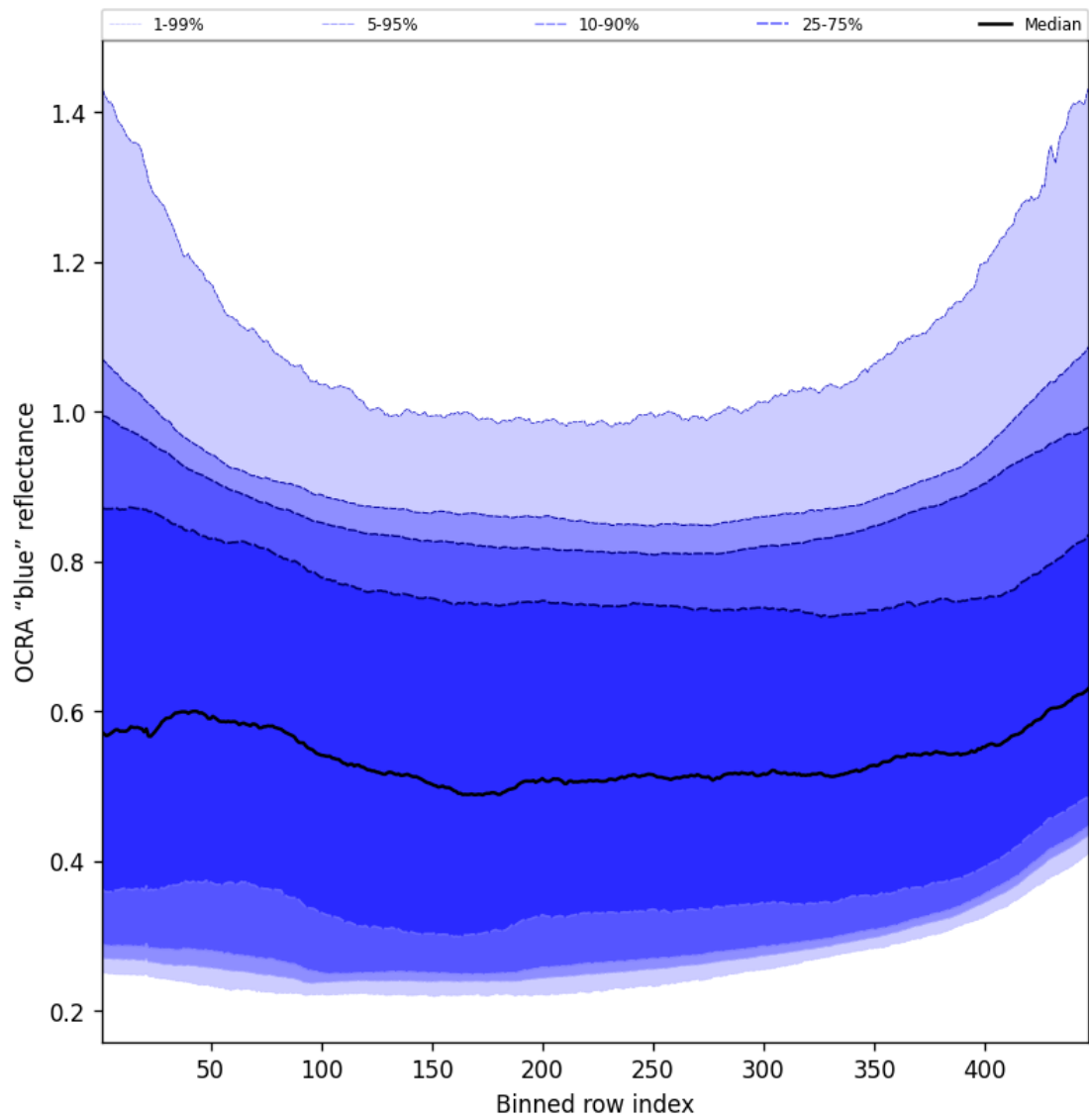
Figure 67: Along track statistics of “OCRA “blue” reflectance” for 2025-10-08 to 2025-10-10
