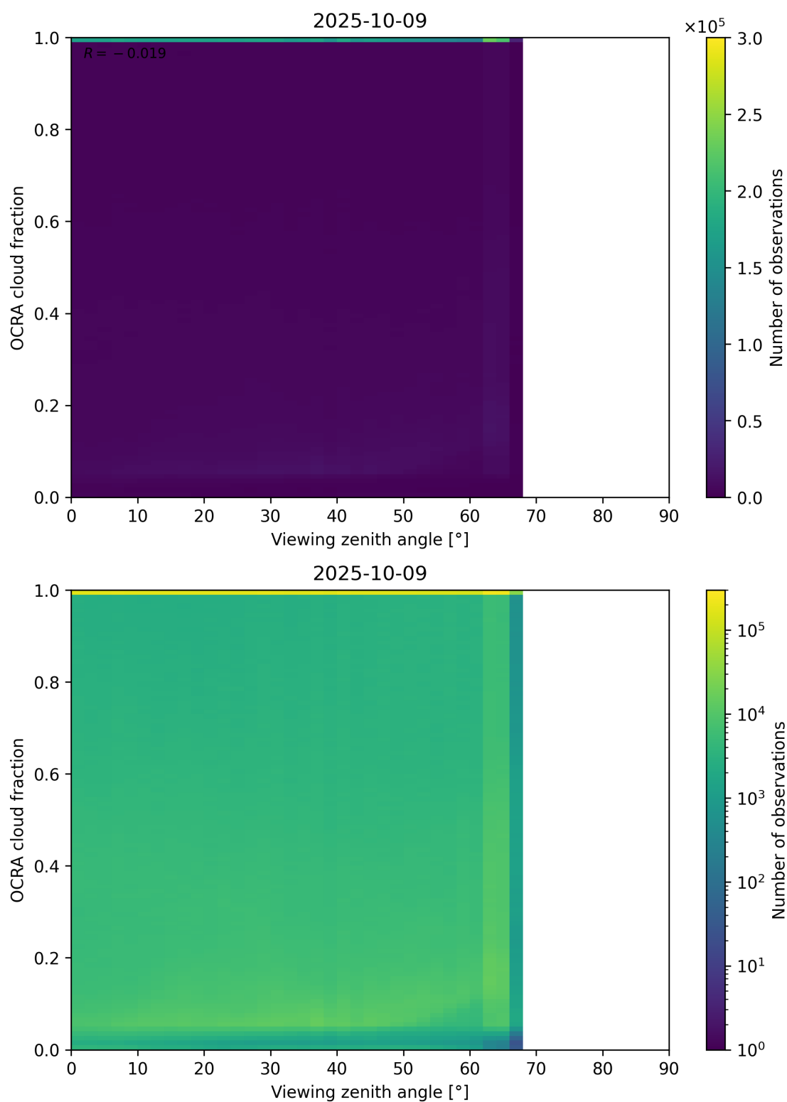
Figure 108: Scatter density plot of “Viewing zenith angle” against “OCRA cloud fraction” for 2025-10-08 to 2025-10-10.
