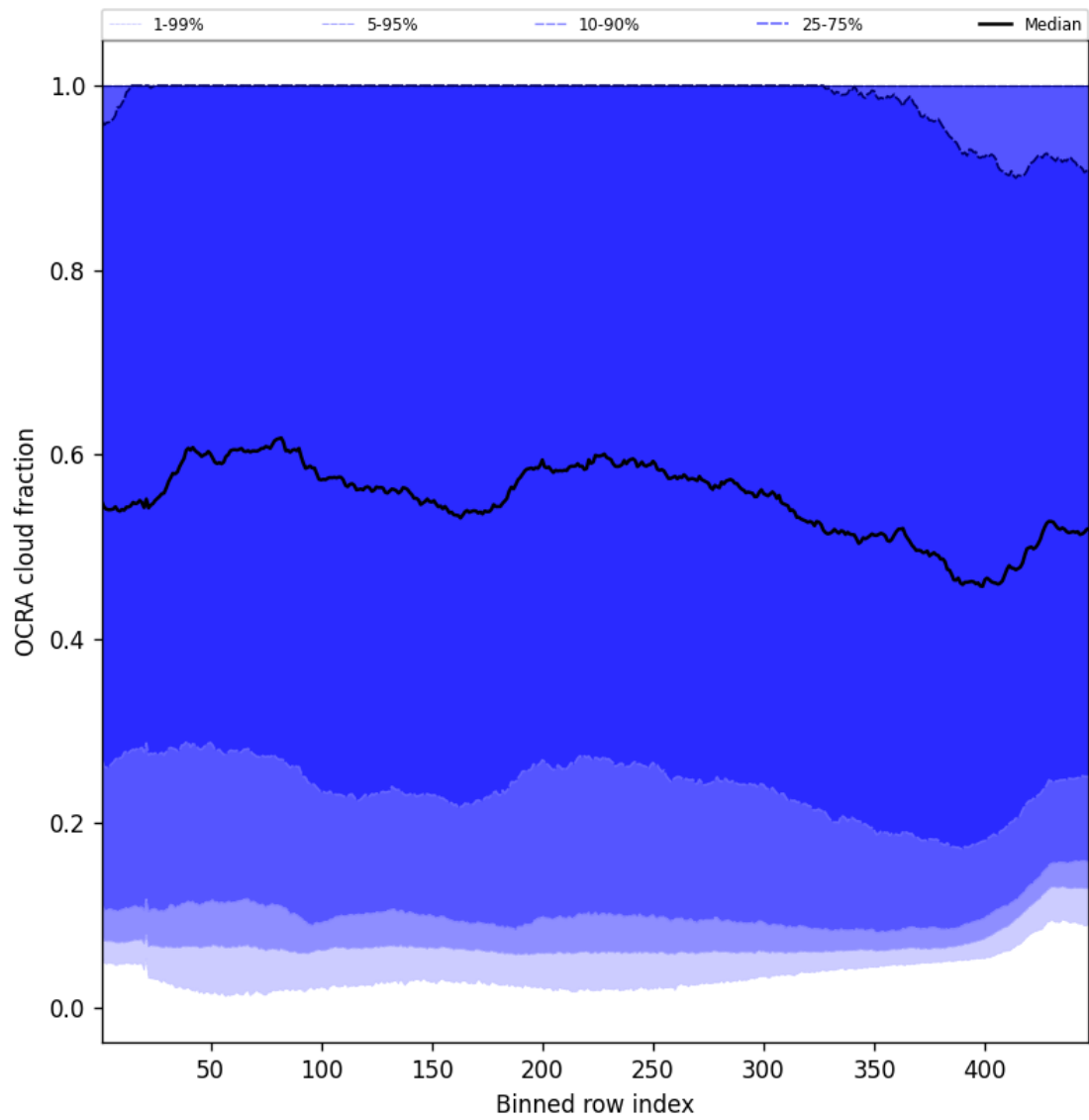
Figure 66: Along track statistics of “OCRA cloud fraction” for 2025-10-08 to 2025-10-10
