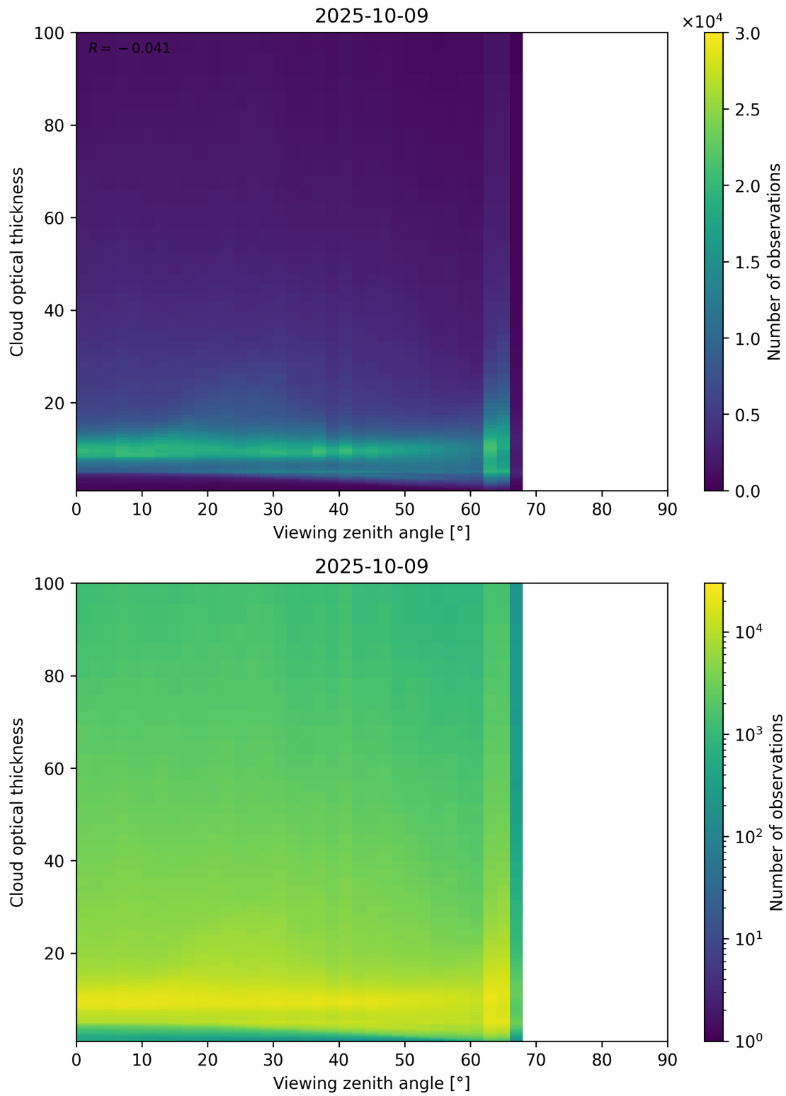
Figure 111: Scatter density plot of “Viewing zenith angle” against “Cloud optical thickness” for 2025-10-08 to 2025-10-10.
