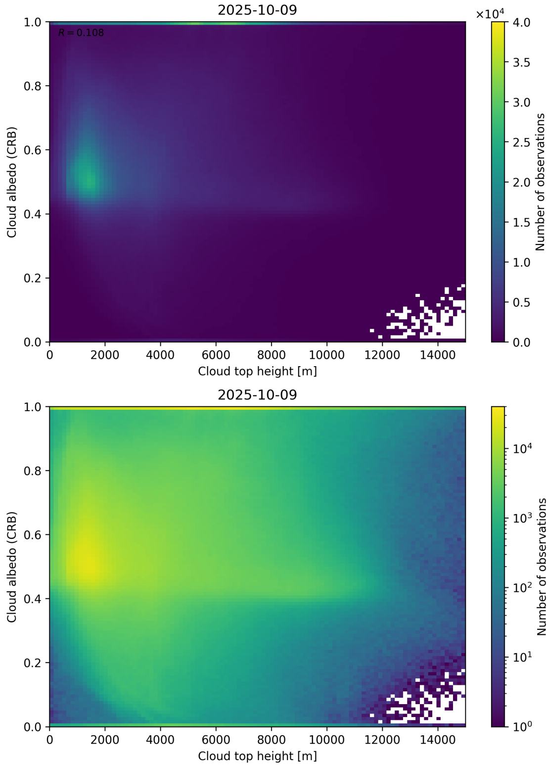
Figure 86: Scatter density plot of “Cloud top height” against “Cloud albedo (CRB)” for 2025-10-08 to 2025-10-10.
