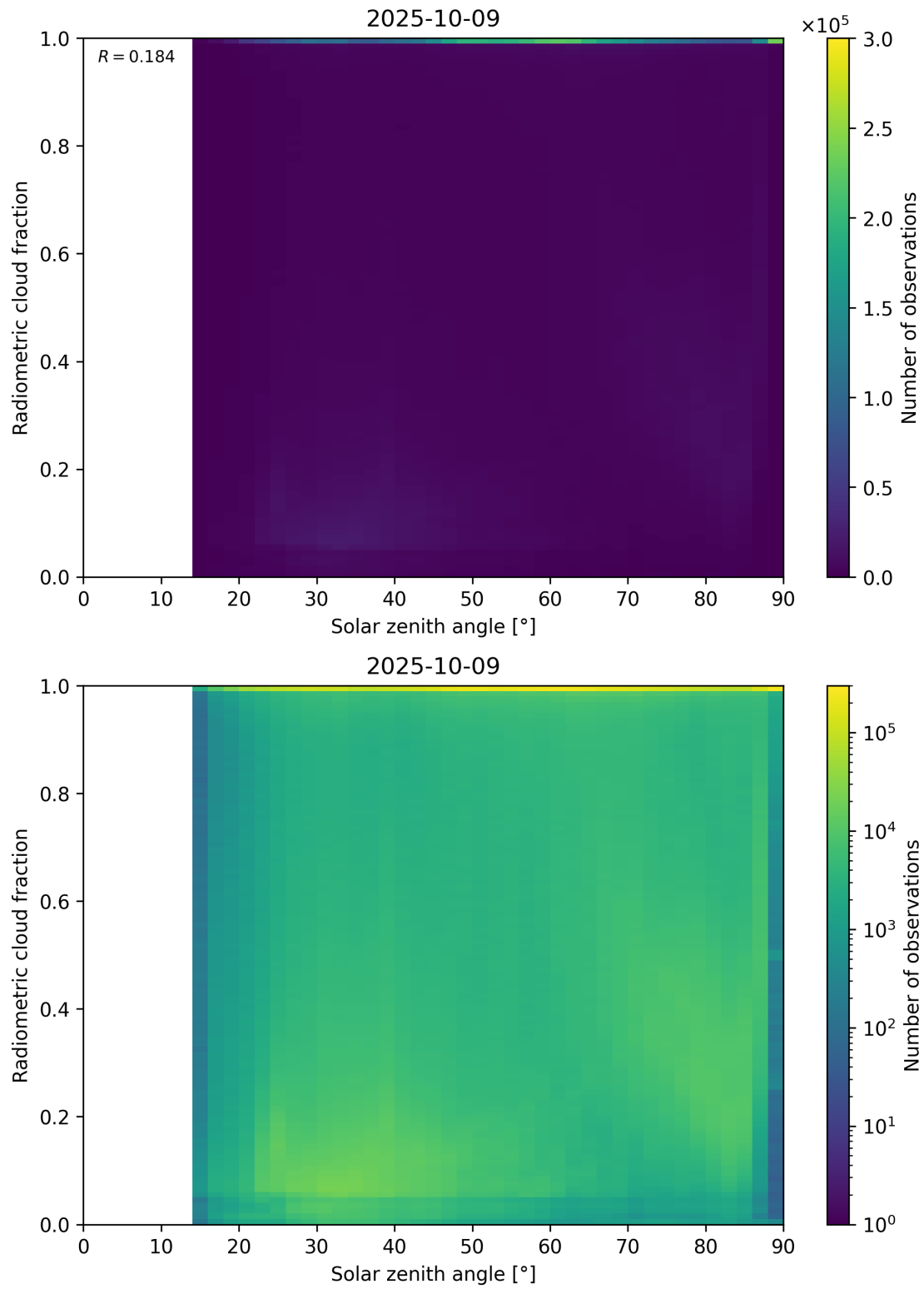
Figure 99: Scatter density plot of “Solar zenith angle” against “Radiometric cloud fraction” for 2025-10-08 to 2025-10-10.
