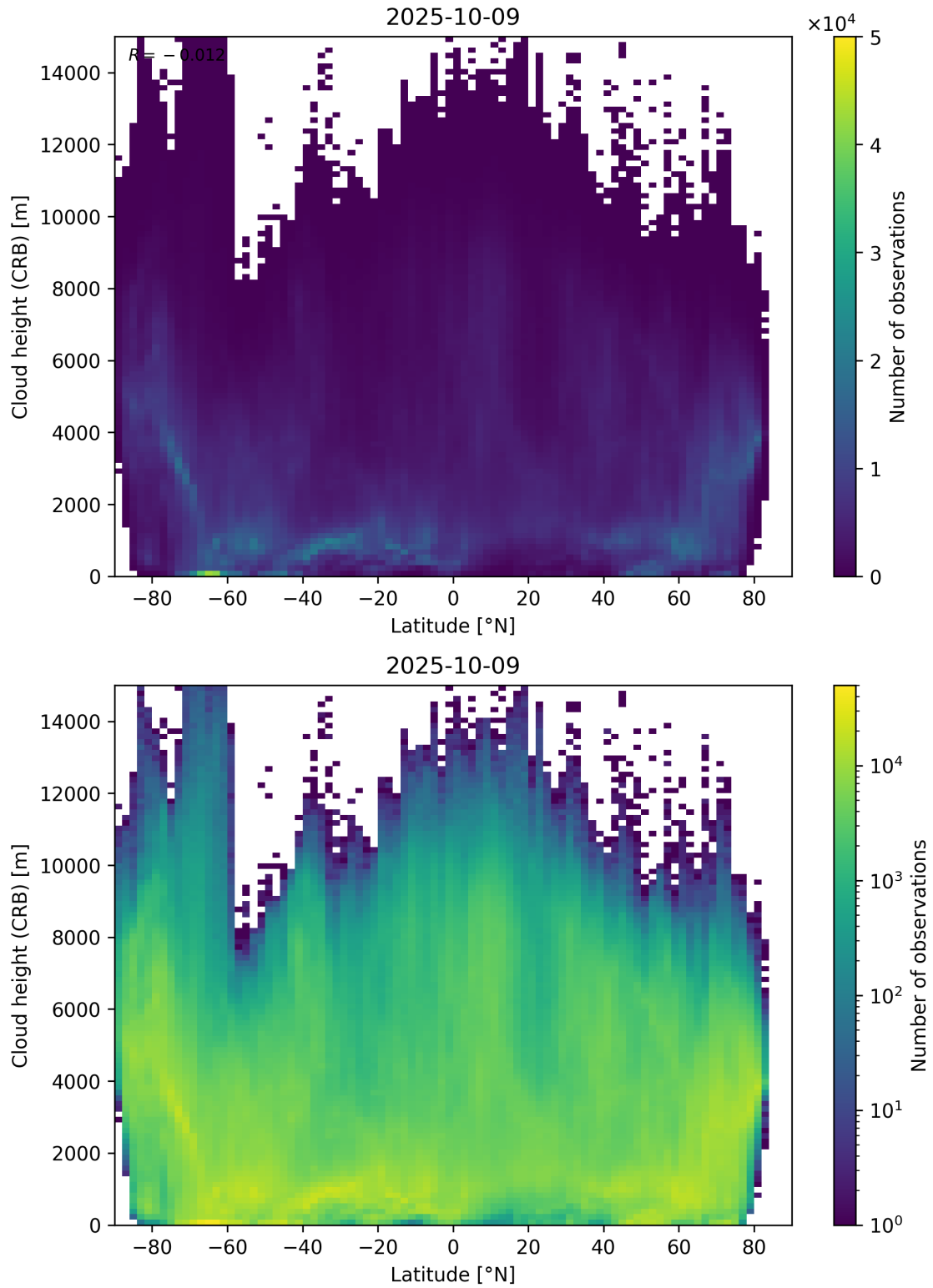
Figure 95: Scatter density plot of “Latitude” against “Cloud height (CRB)” for 2025-10-08 to 2025-10-10.
