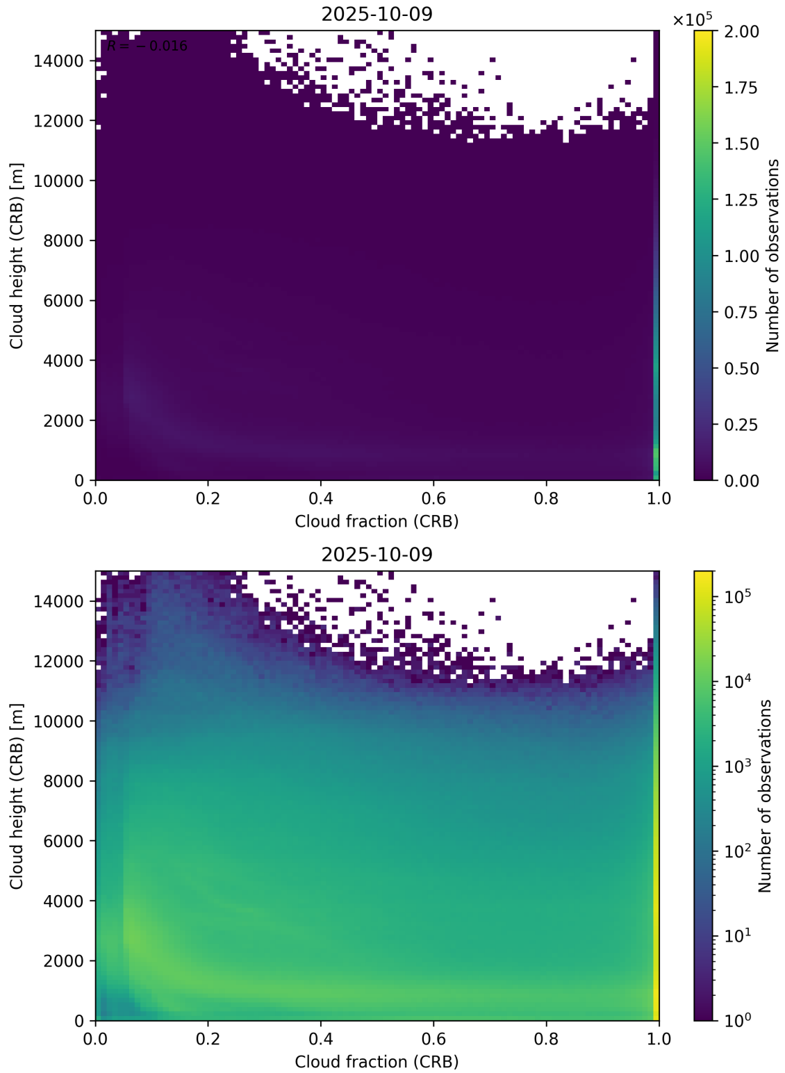
Figure 79: Scatter density plot of “Cloud fraction (CRB)” against “Cloud height (CRB)” for 2025-10-08 to 2025-10-10.
