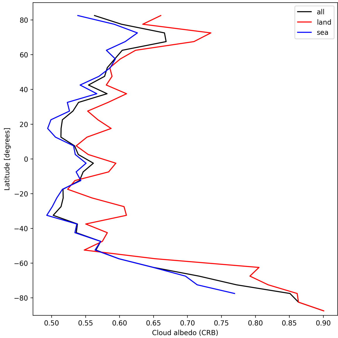
Figure 28: Zonal average of “Cloud albedo (CRB)” for 2025-10-08 to 2025-10-10.
