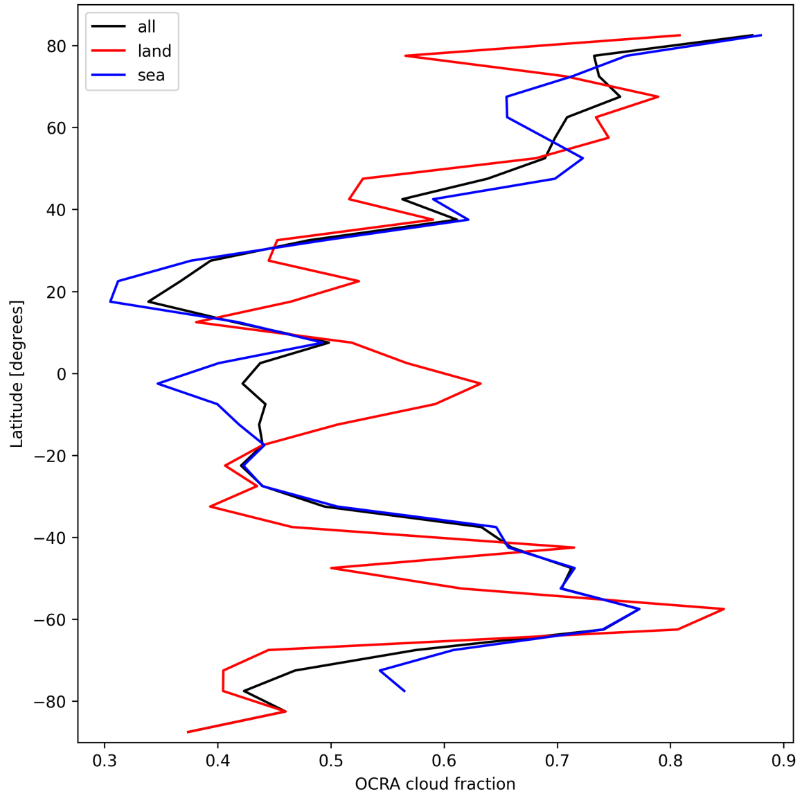
Figure 34: Zonal average of “OCRA cloud fraction” for 2025-10-08 to 2025-10-10.
