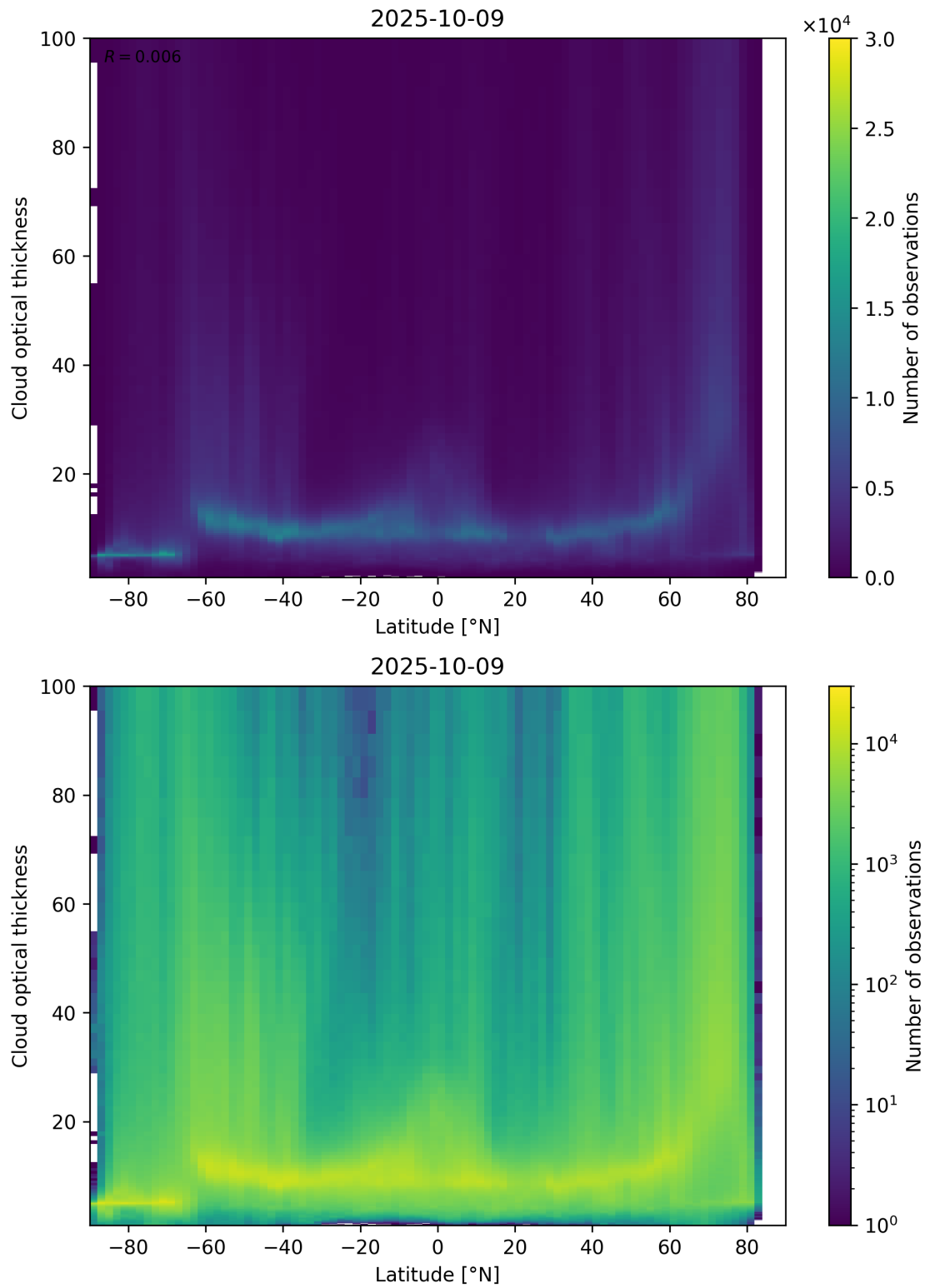
Figure 96: Scatter density plot of “Latitude” against “Cloud optical thickness” for 2025-10-08 to 2025-10-10.
