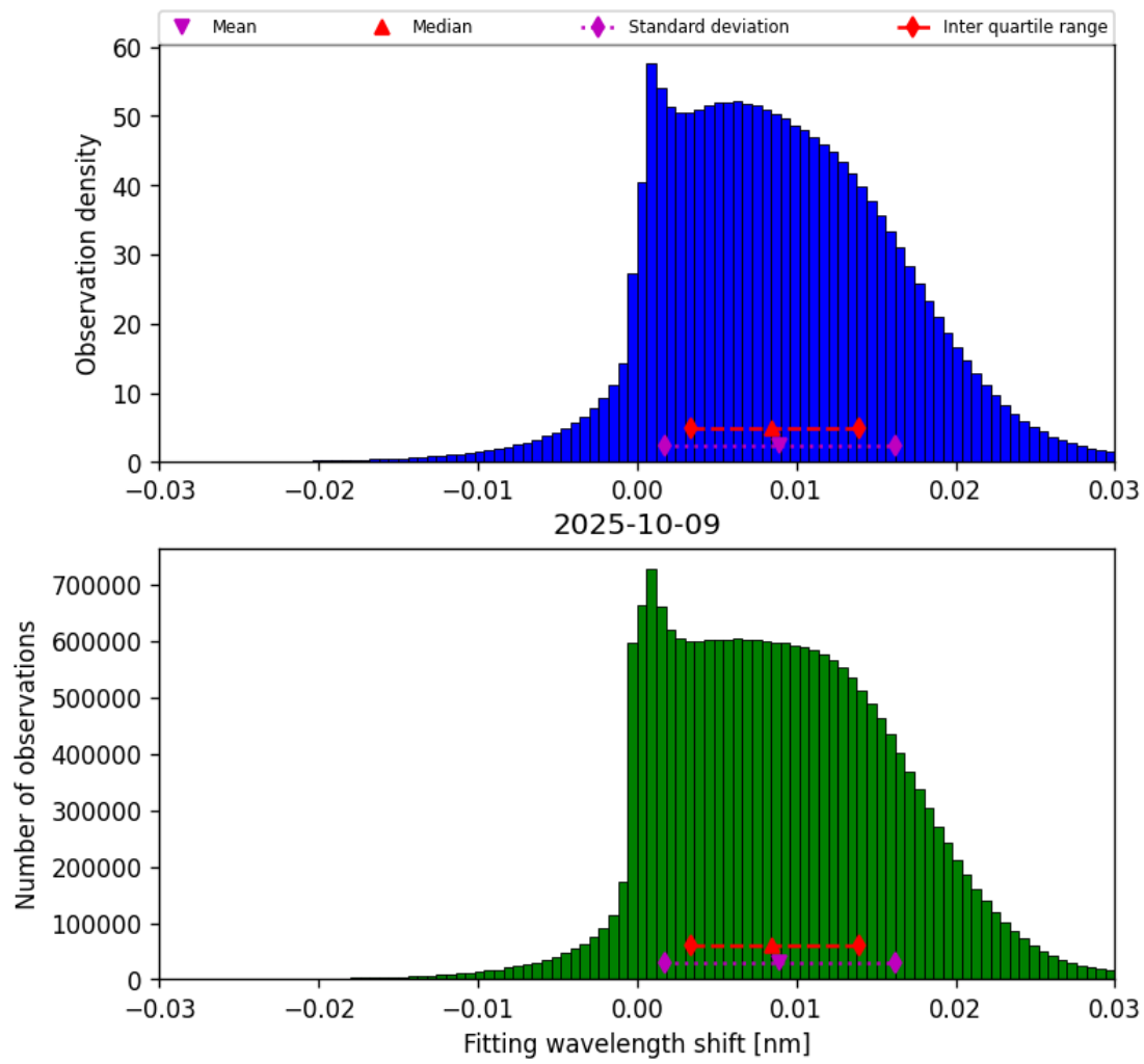
Figure 49: Histogram of “Fitting wavelength shift” for 2025-10-08 to 2025-10-10
