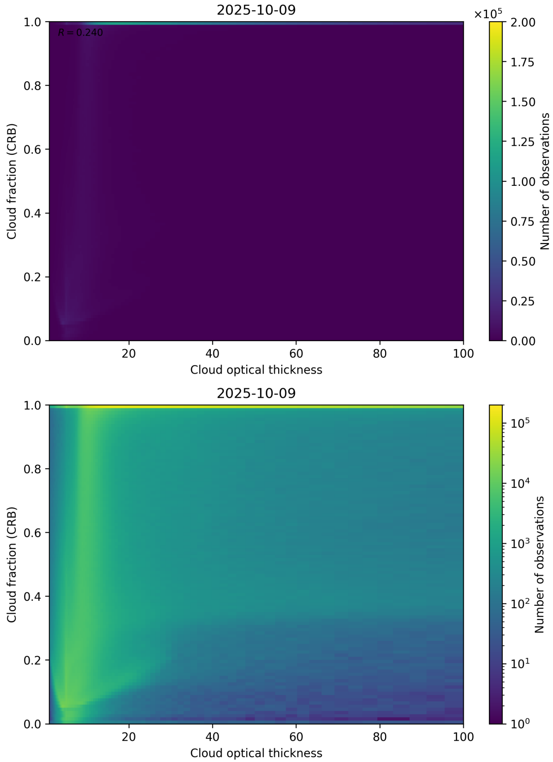
Figure 84: Scatter density plot of “Cloud optical thickness” against “Cloud fraction (CRB)” for 2025-10-08 to 2025-10-10.
