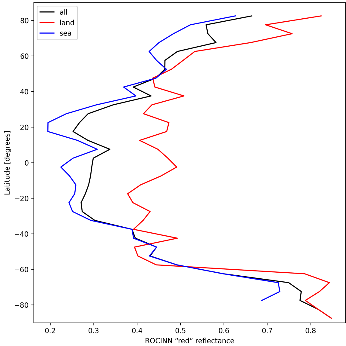
Figure 37: Zonal average of “ROCINN “red” reflectance” for 2025-10-08 to 2025-10-10.
