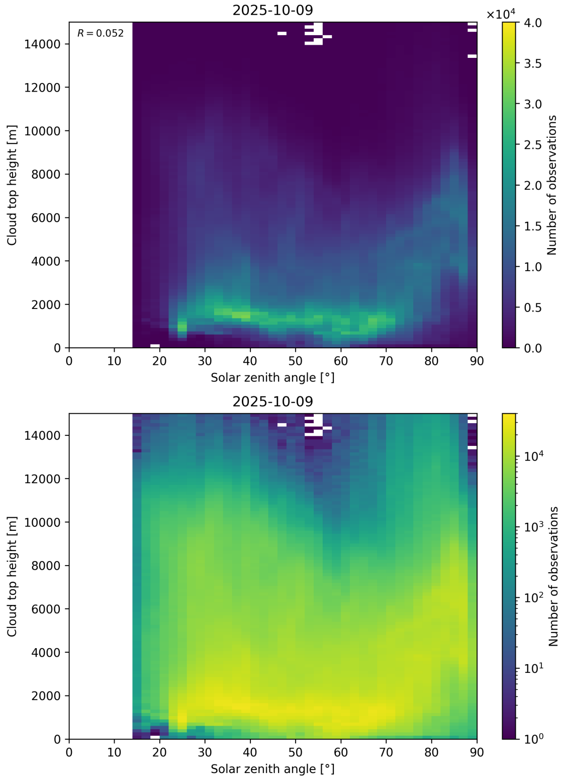
Figure 104: Scatter density plot of “Solar zenith angle” against “Cloud top height” for 2025-10-08 to 2025-10-10.
