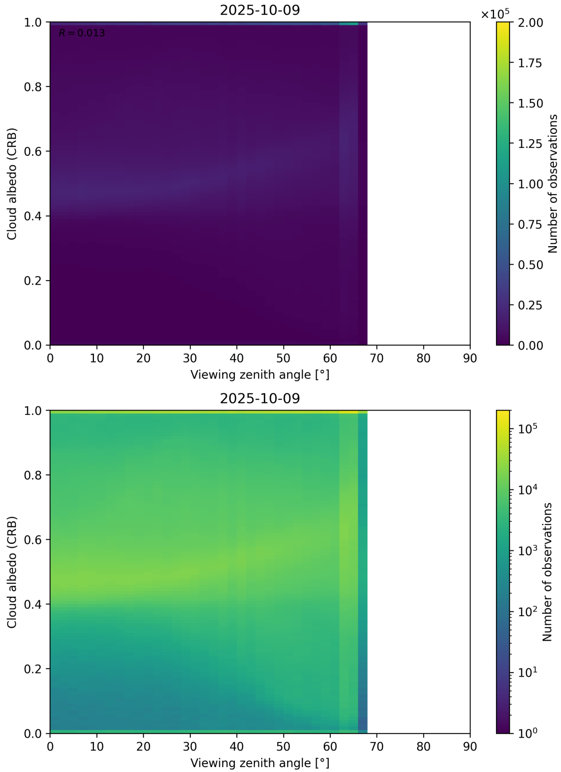
Figure 106: Scatter density plot of “Viewing zenith angle” against “Cloud albedo (CRB)” for 2025-10-08 to 2025-10-10.
