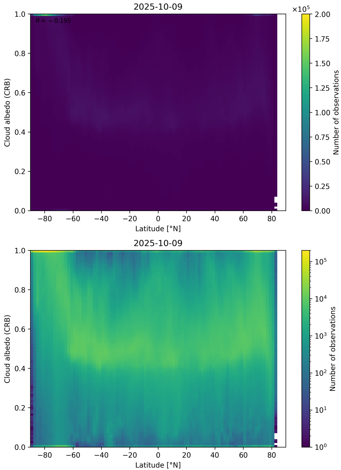
Figure 91: Scatter density plot of “Latitude” against “Cloud albedo (CRB)” for 2025-10-08 to 2025-10-10.
