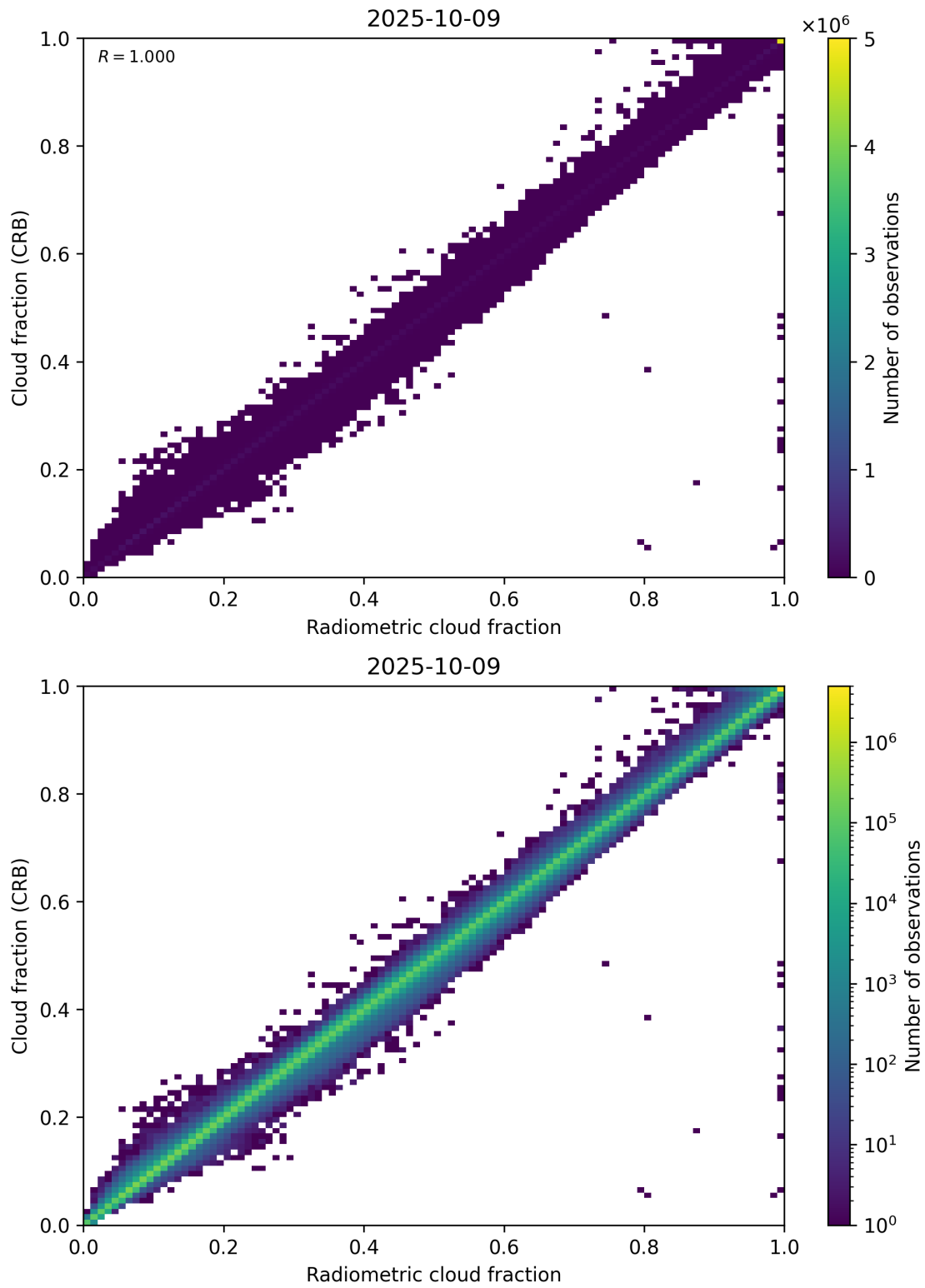
Figure 73: Scatter density plot of “Radiometric cloud fraction” against “Cloud fraction (CRB)” for 2025-10-08 to 2025-10-10.
