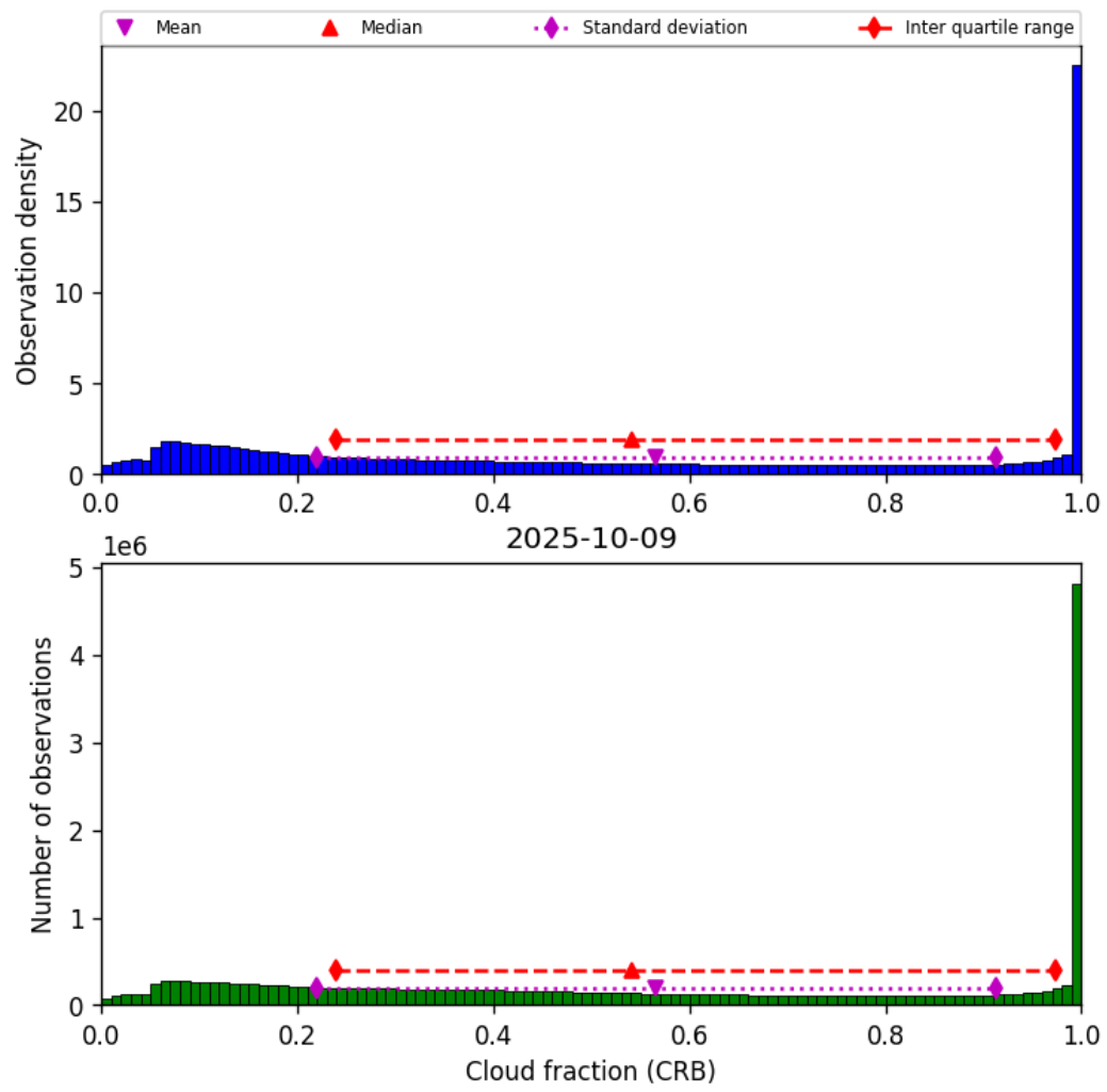
Figure 42: Histogram of “Cloud fraction (CRB)” for 2025-10-08 to 2025-10-10
