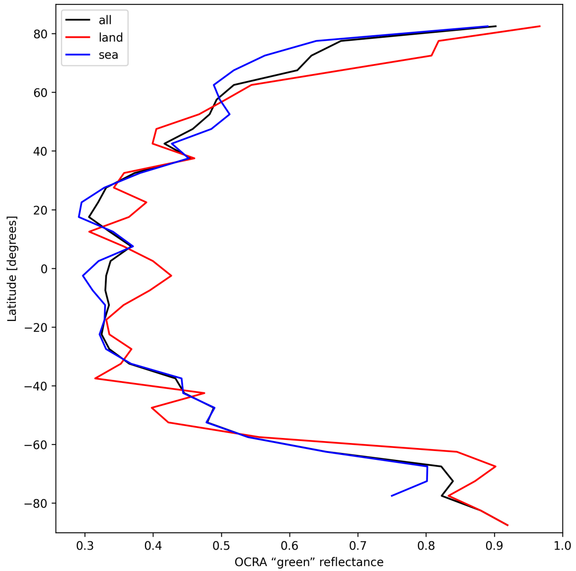
Figure 36: Zonal average of “OCRA “green” reflectance” for 2025-10-08 to 2025-10-10.
