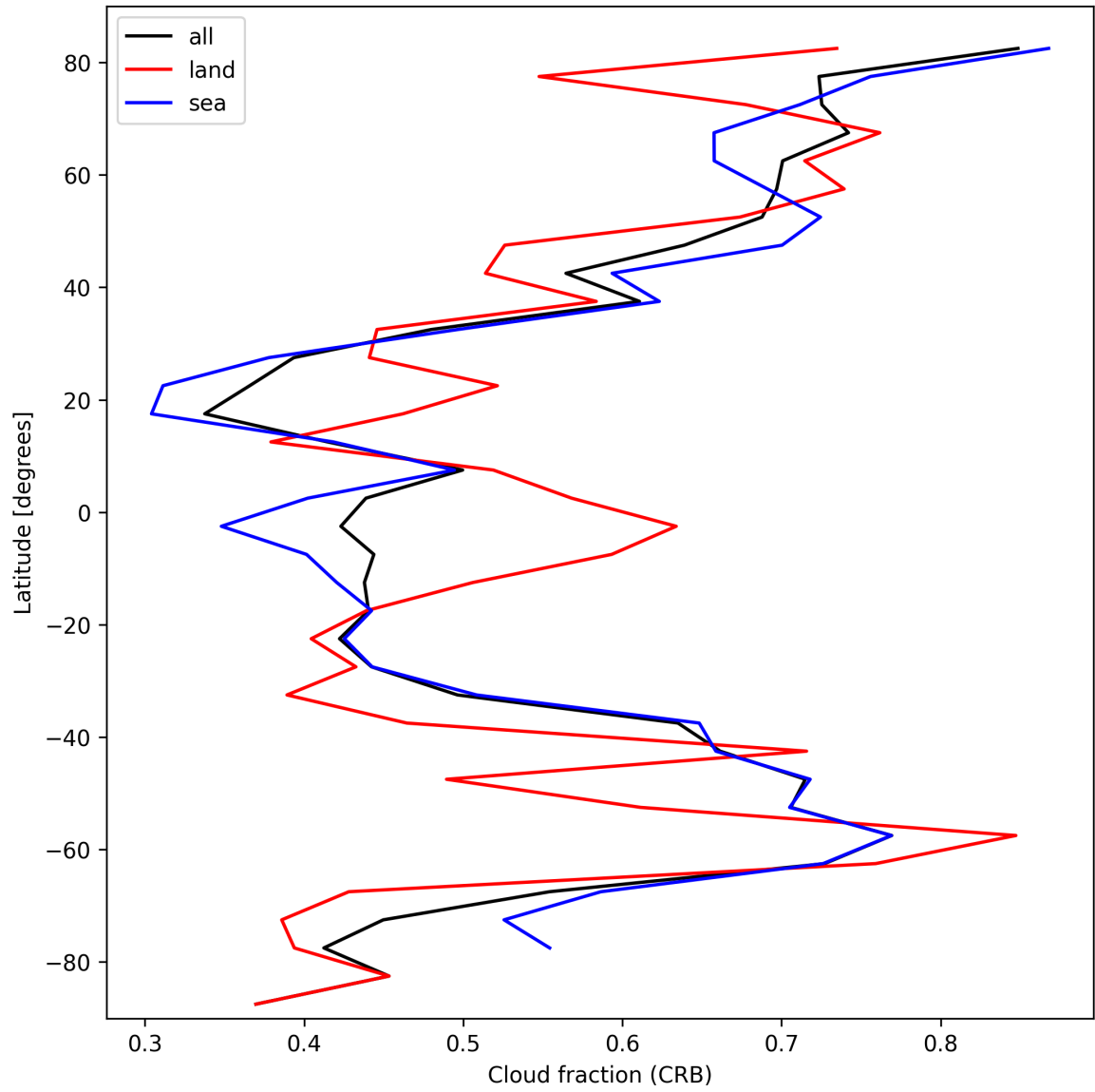
Figure 26: Zonal average of “Cloud fraction (CRB)” for 2025-10-08 to 2025-10-10.
