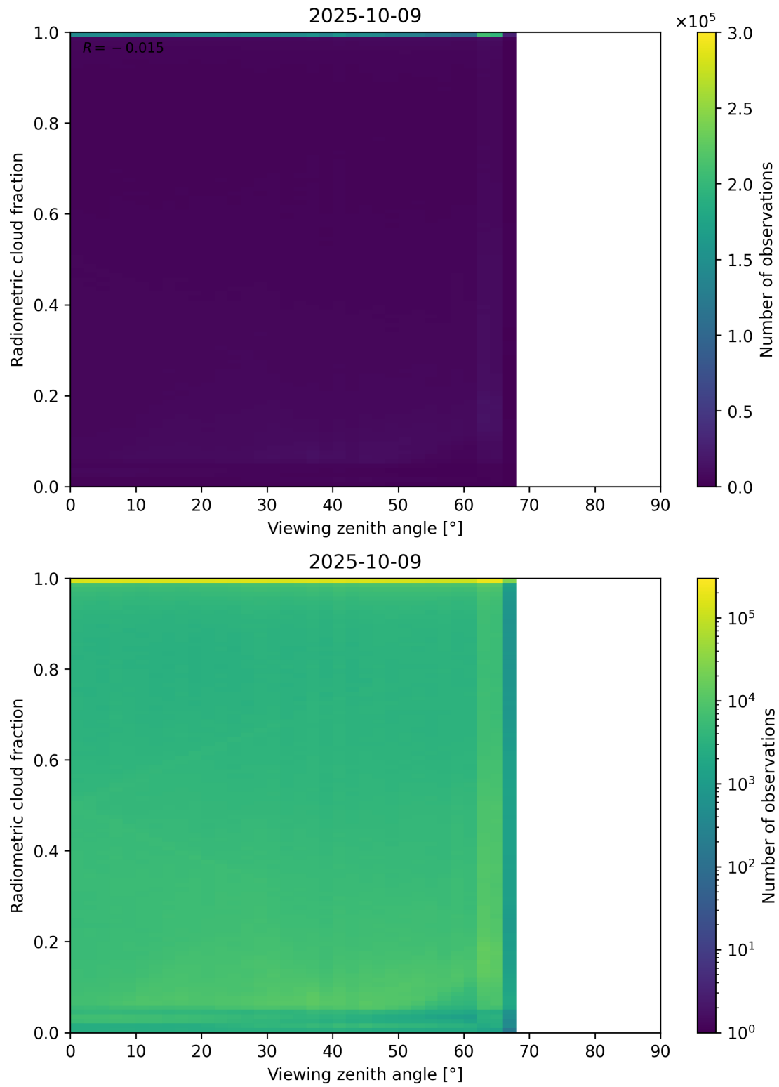
Figure 107: Scatter density plot of “Viewing zenith angle” against “Radiometric cloud fraction” for 2025-10-08 to 2025-10-10.
