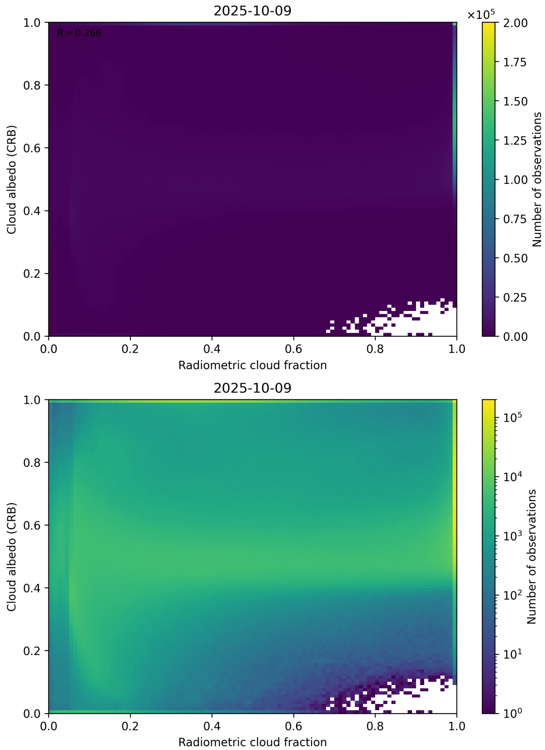
Figure 71: Scatter density plot of “Radiometric cloud fraction” against “Cloud albedo (CRB)” for 2025-10-08 to 2025-10-10.
