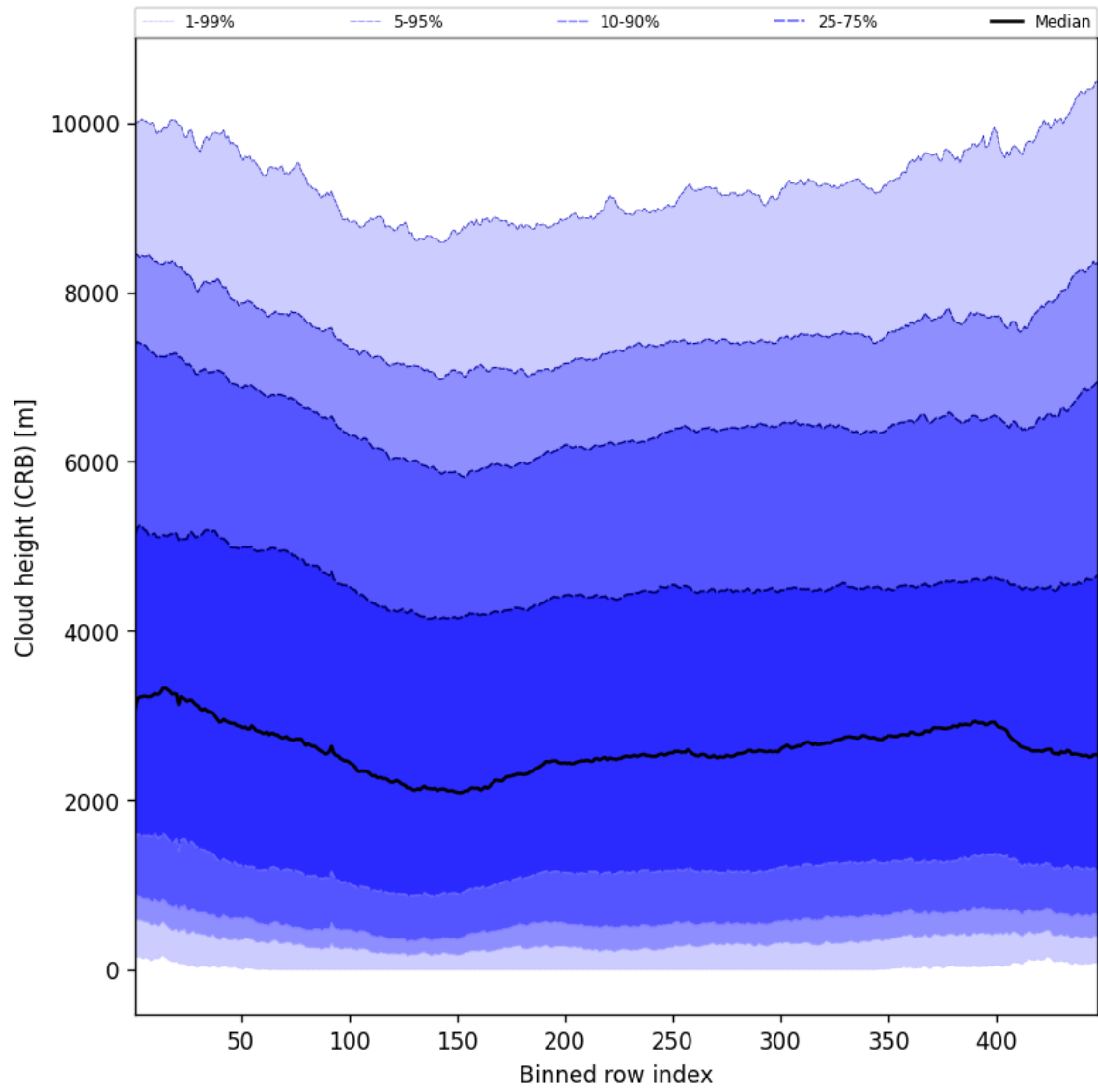
Figure 59: Along track statistics of “Cloud height (CRB)” for 2025-10-08 to 2025-10-10
