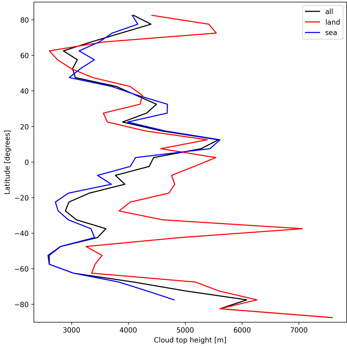
Figure 24: Zonal average of “Cloud top height” for 2025-10-08 to 2025-10-10.
