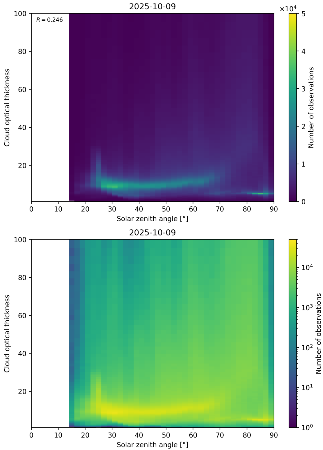
Figure 103: Scatter density plot of “Solar zenith angle” against “Cloud optical thickness” for 2025-10-08 to 2025-10-10.
