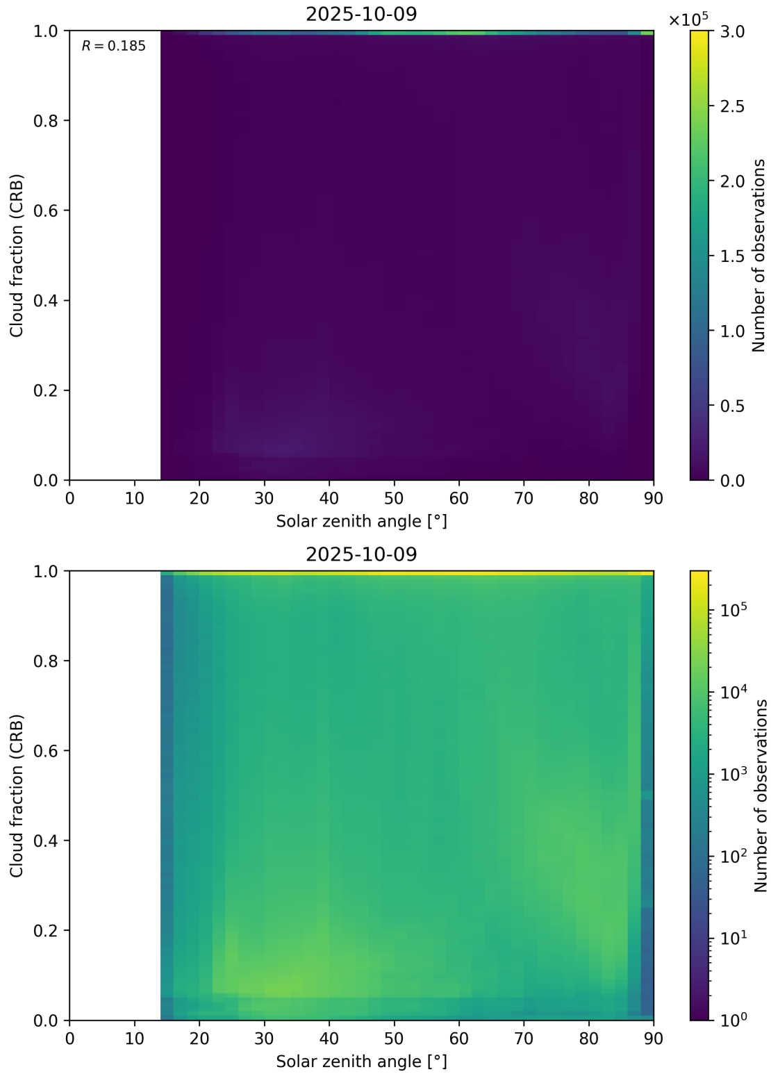
Figure 101: Scatter density plot of “Solar zenith angle” against “Cloud fraction (CRB)” for 2025-10-08 to 2025-10-10.
