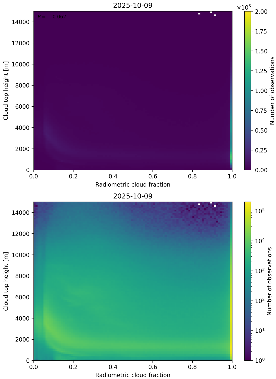
Figure 76: Scatter density plot of “Radiometric cloud fraction” against “Cloud top height” for 2025-10-08 to 2025-10-10.
