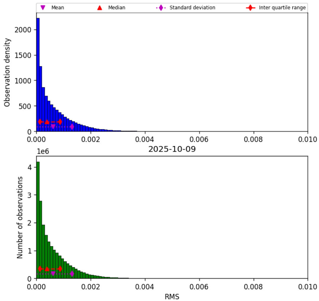
Figure 47: Histogram of “RMS” for 2025-10-08 to 2025-10-10
