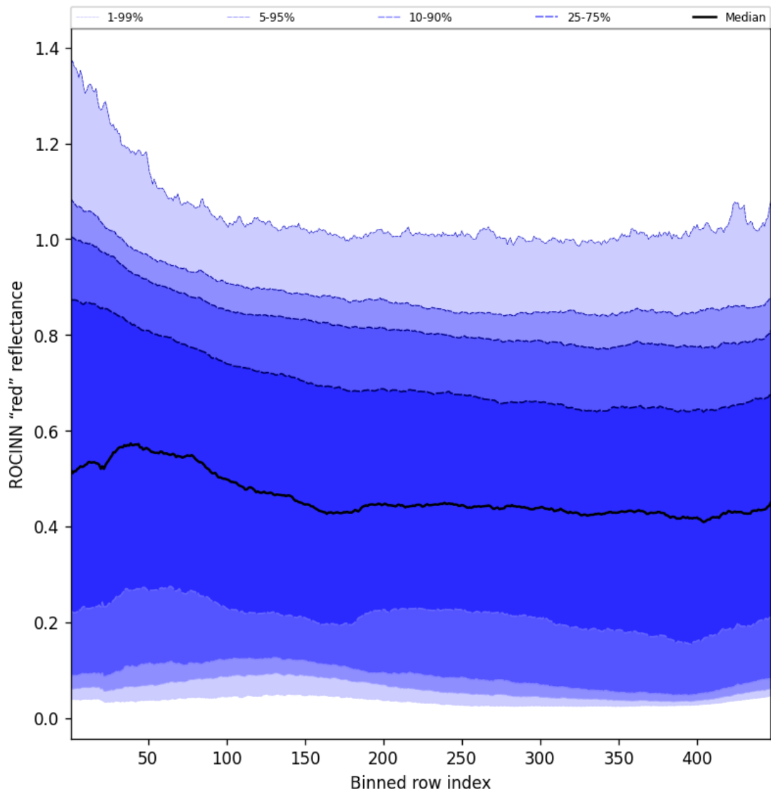
Figure 69: Along track statistics of “ROCINN “red” reflectance” for 2025-10-08 to 2025-10-10
