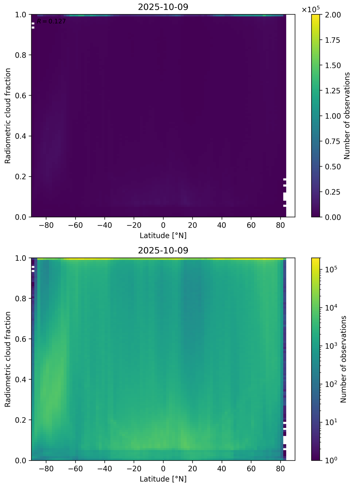
Figure 92: Scatter density plot of “Latitude” against “Radiometric cloud fraction” for 2025-10-08 to 2025-10-10.
