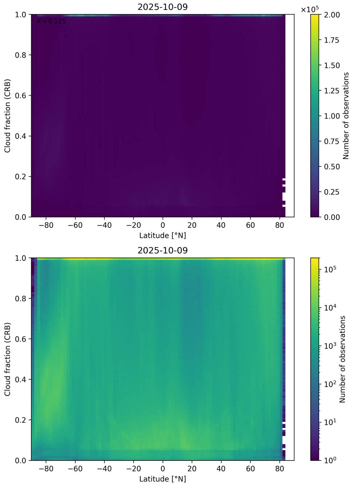
Figure 94: Scatter density plot of “Latitude” against “Cloud fraction (CRB)” for 2025-10-08 to 2025-10-10.
