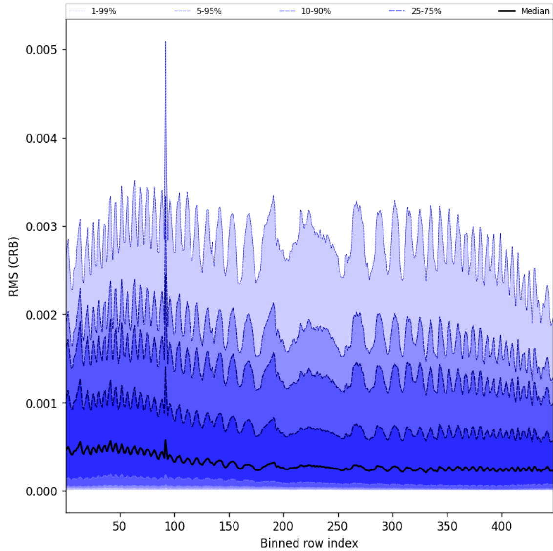
Figure 64: Along track statistics of “RMS (CRB)” for 2025-10-08 to 2025-10-10
