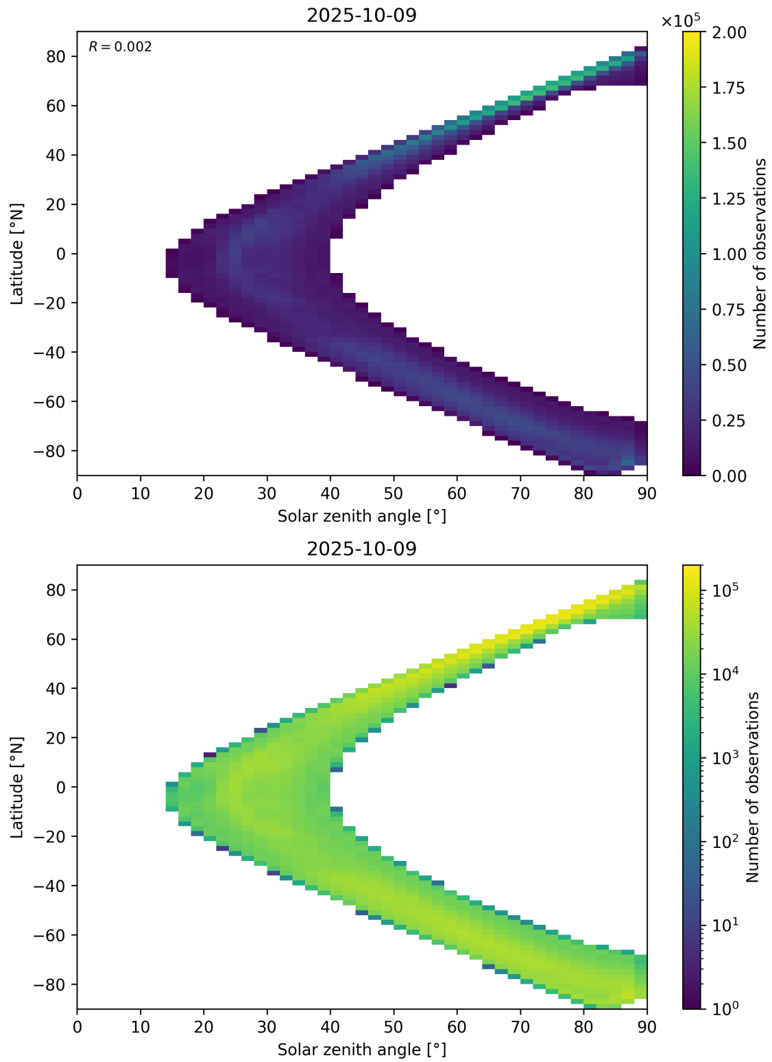
Figure 105: Scatter density plot of “Solar zenith angle” against “Latitude” for 2025-10-08 to 2025-10-10.
