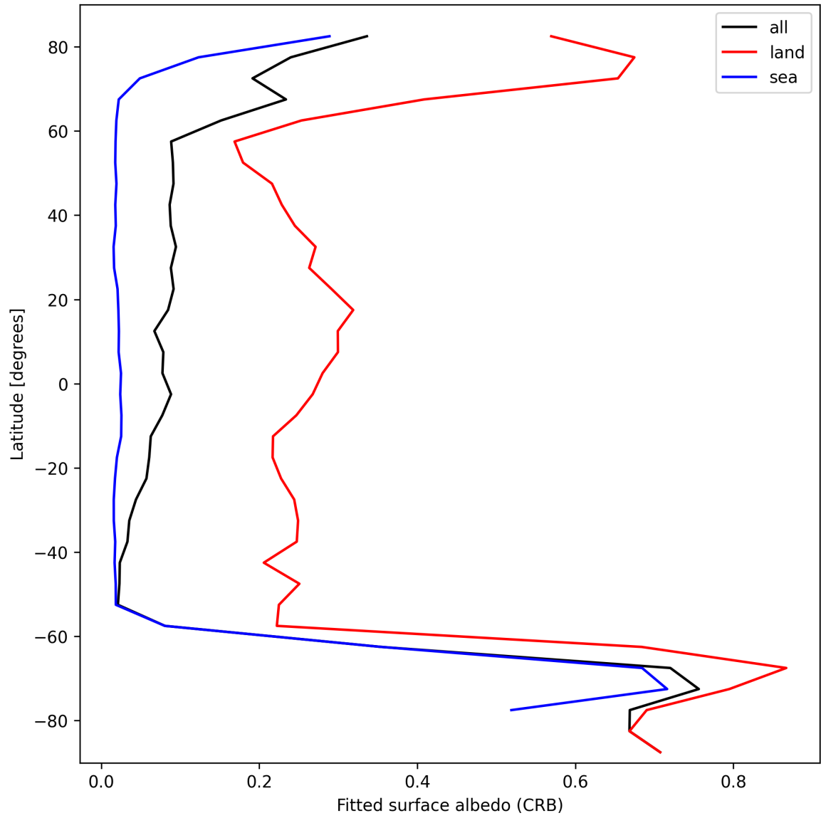
Figure 30: Zonal average of “Fitted surface albedo (CRB)” for 2025-10-08 to 2025-10-10.
