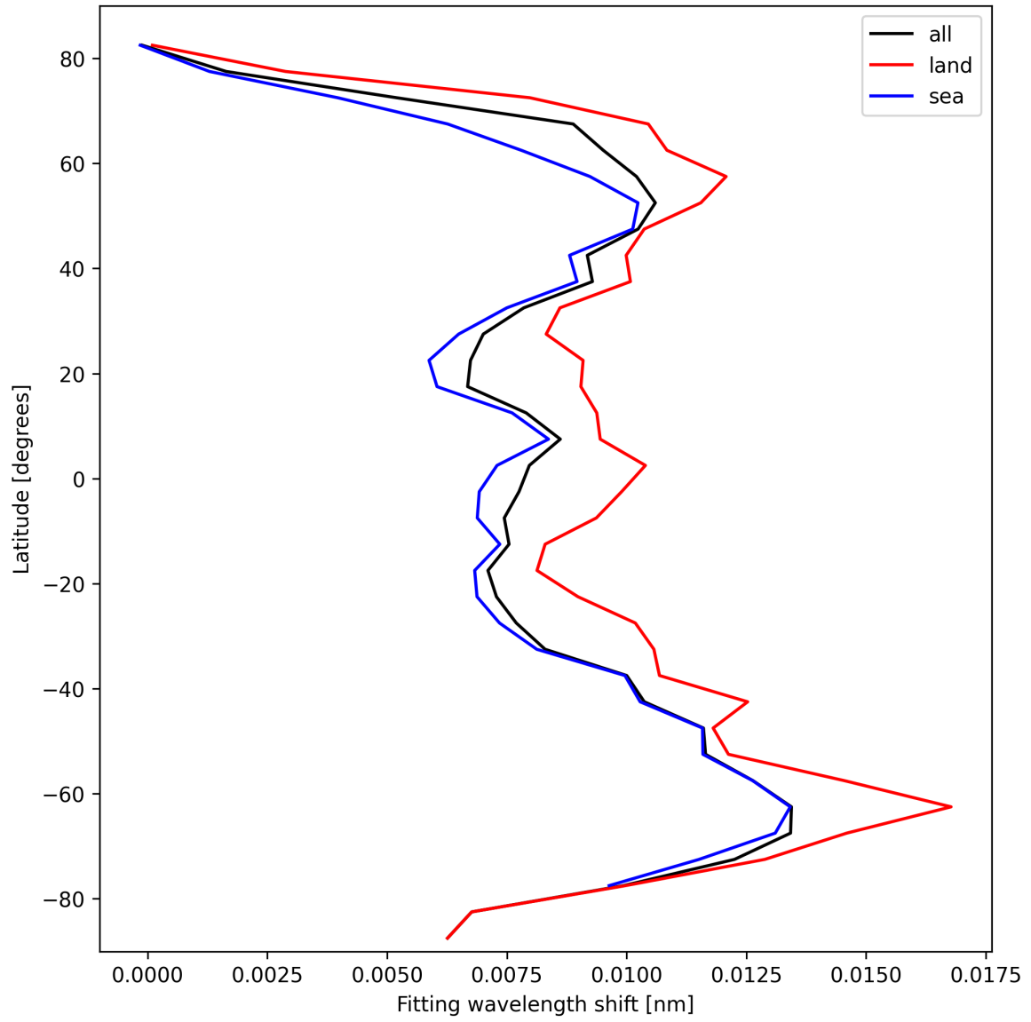
Figure 33: Zonal average of “Fitting wavelength shift” for 2025-10-08 to 2025-10-10.
