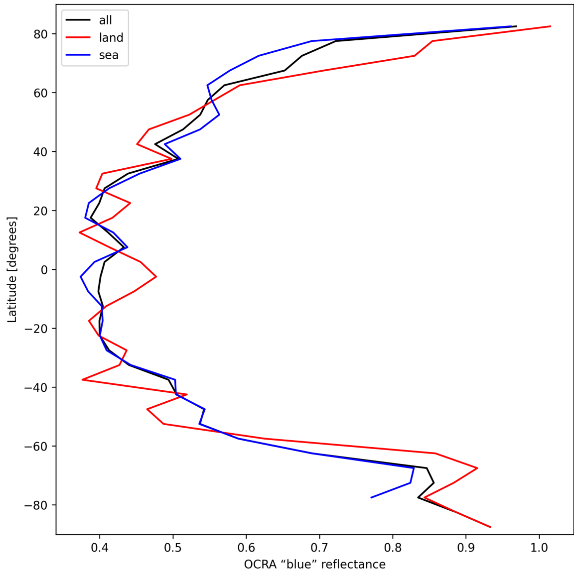
Figure 35: Zonal average of “OCRA “blue” reflectance” for 2025-10-08 to 2025-10-10.
