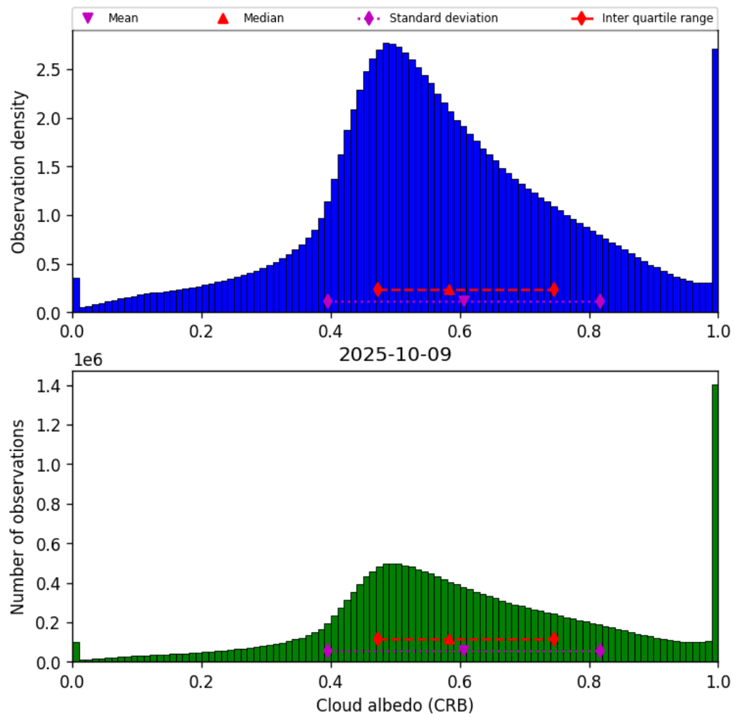
Figure 44: Histogram of “Cloud albedo (CRB)” for 2025-10-08 to 2025-10-10
