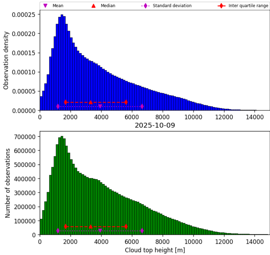
Figure 40: Histogram of “Cloud top height” for 2025-10-08 to 2025-10-10
