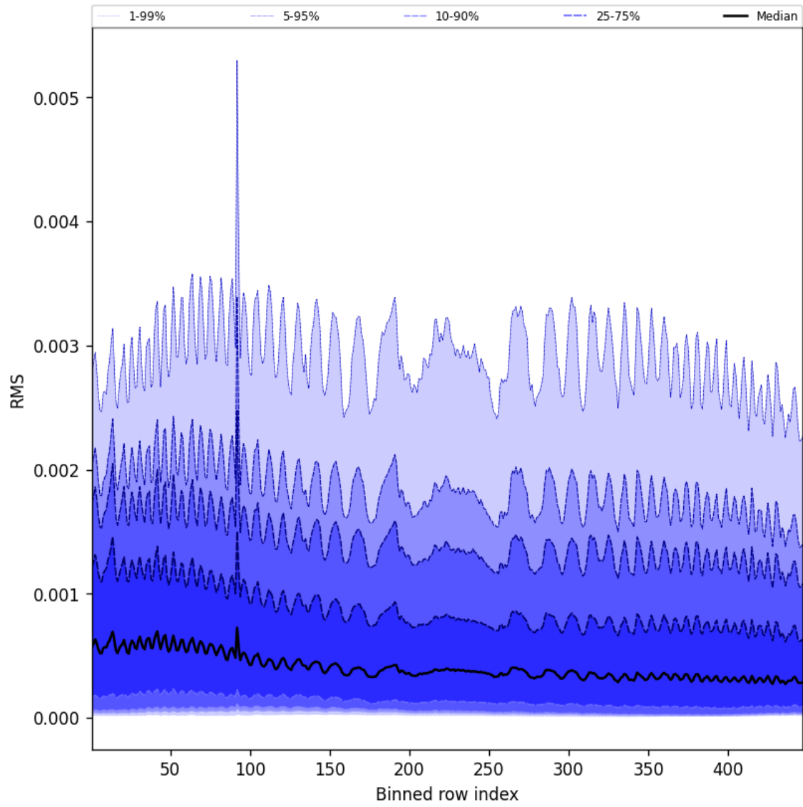
Figure 63: Along track statistics of “RMS” for 2025-10-08 to 2025-10-10
