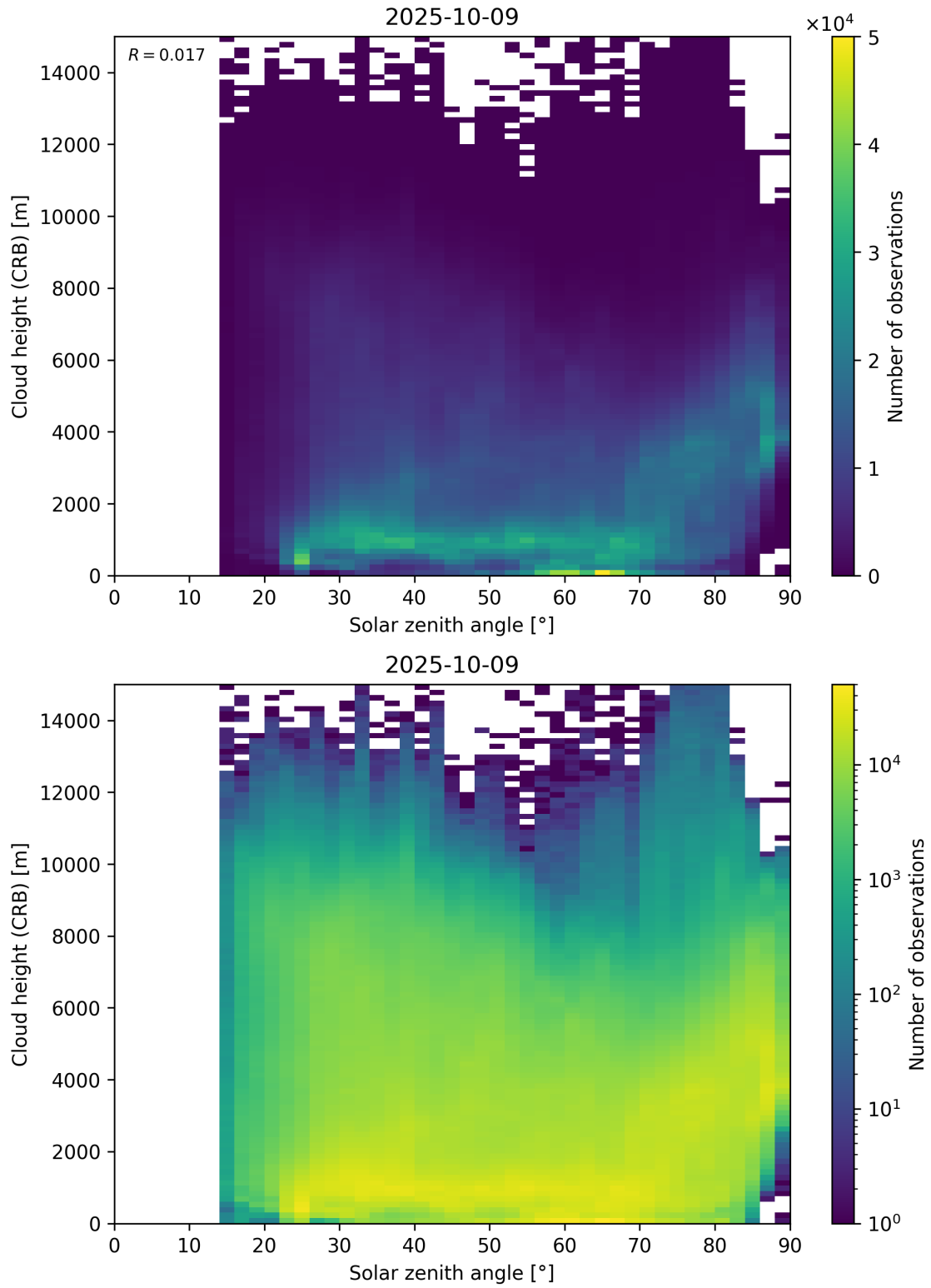
Figure 102: Scatter density plot of “Solar zenith angle” against “Cloud height (CRB)” for 2025-10-08 to 2025-10-10.
