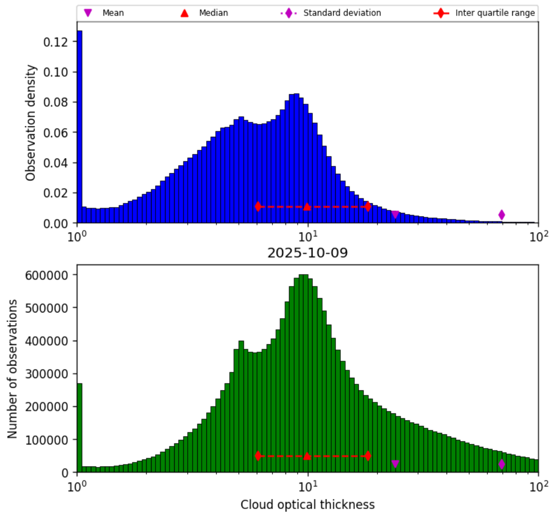
Figure 41: Histogram of “Cloud optical thickness” for 2025-10-08 to 2025-10-10
