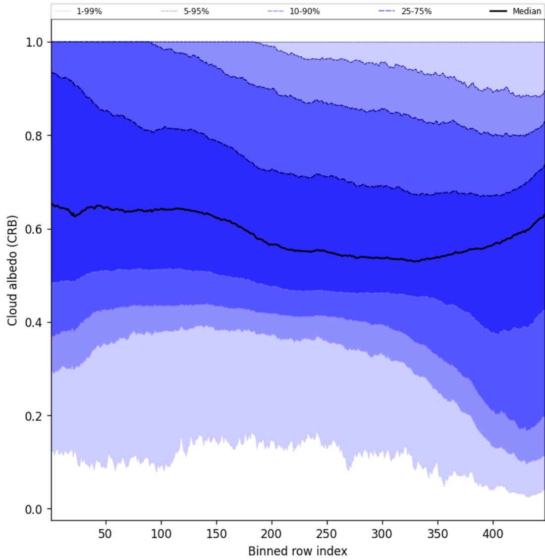
Figure 60: Along track statistics of “Cloud albedo (CRB)” for 2025-10-08 to 2025-10-10
