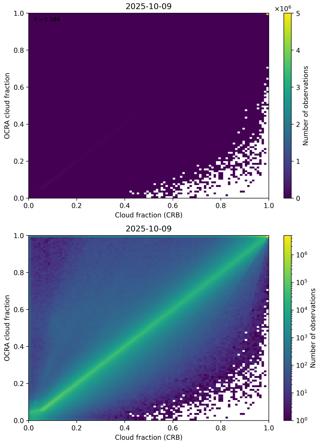
Figure 78: Scatter density plot of “Cloud fraction (CRB)” against “OCRA cloud fraction” for 2025-10-08 to 2025-10-10.
