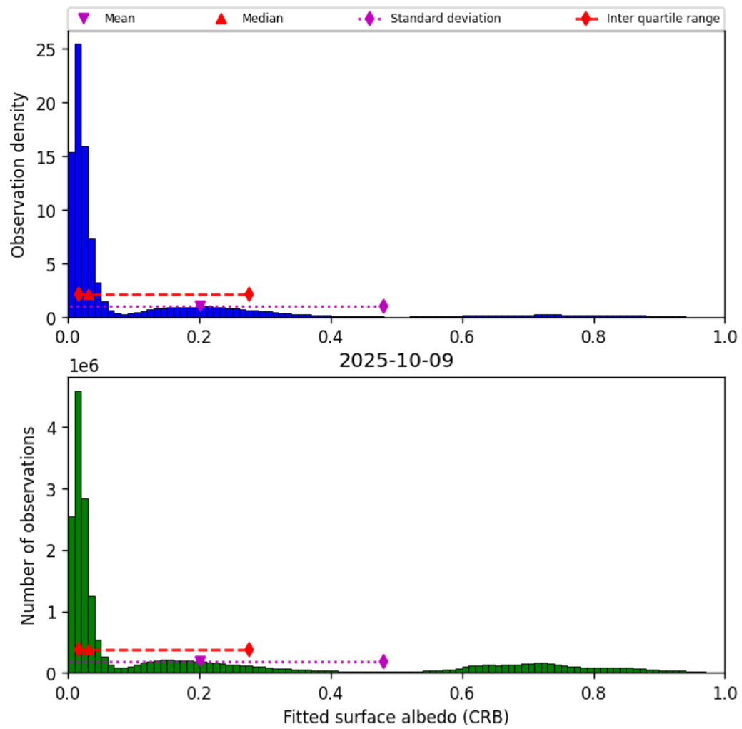
Figure 46: Histogram of “Fitted surface albedo (CRB)” for 2025-10-08 to 2025-10-10
