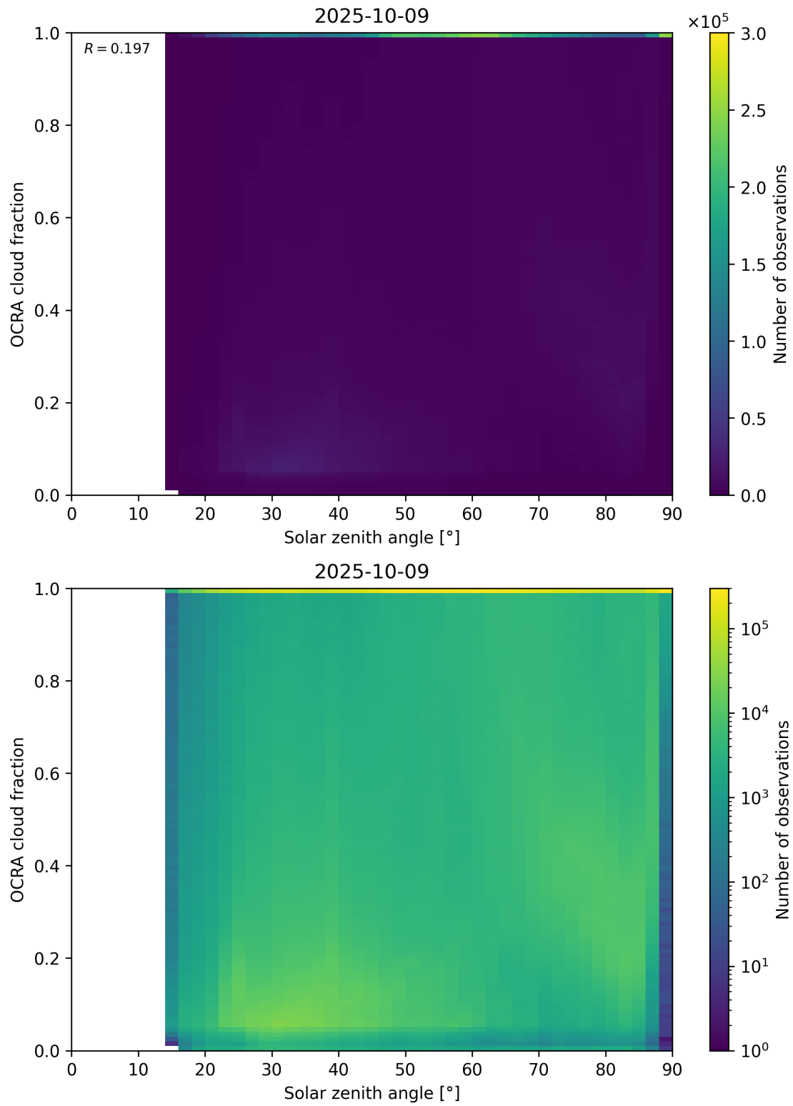
Figure 100: Scatter density plot of “Solar zenith angle” against “OCRA cloud fraction” for 2025-10-08 to 2025-10-10.
