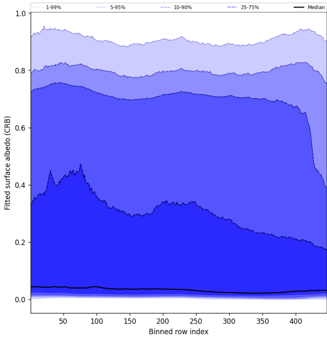
Figure 62: Along track statistics of “Fitted surface albedo (CRB)” for 2025-10-08 to 2025-10-10
