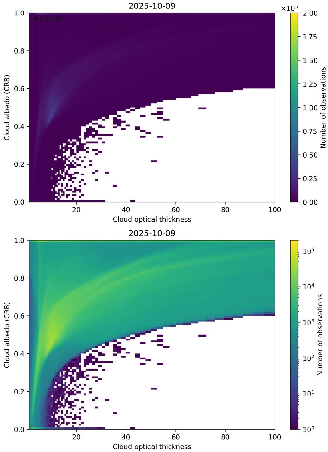
Figure 82: Scatter density plot of “Cloud optical thickness” against “Cloud albedo (CRB)” for 2025-10-08 to 2025-10-10.
