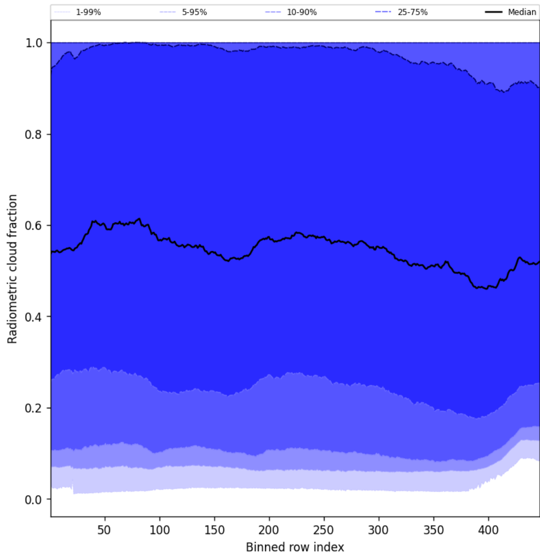
Figure 55: Along track statistics of “Radiometric cloud fraction” for 2025-10-08 to 2025-10-10
