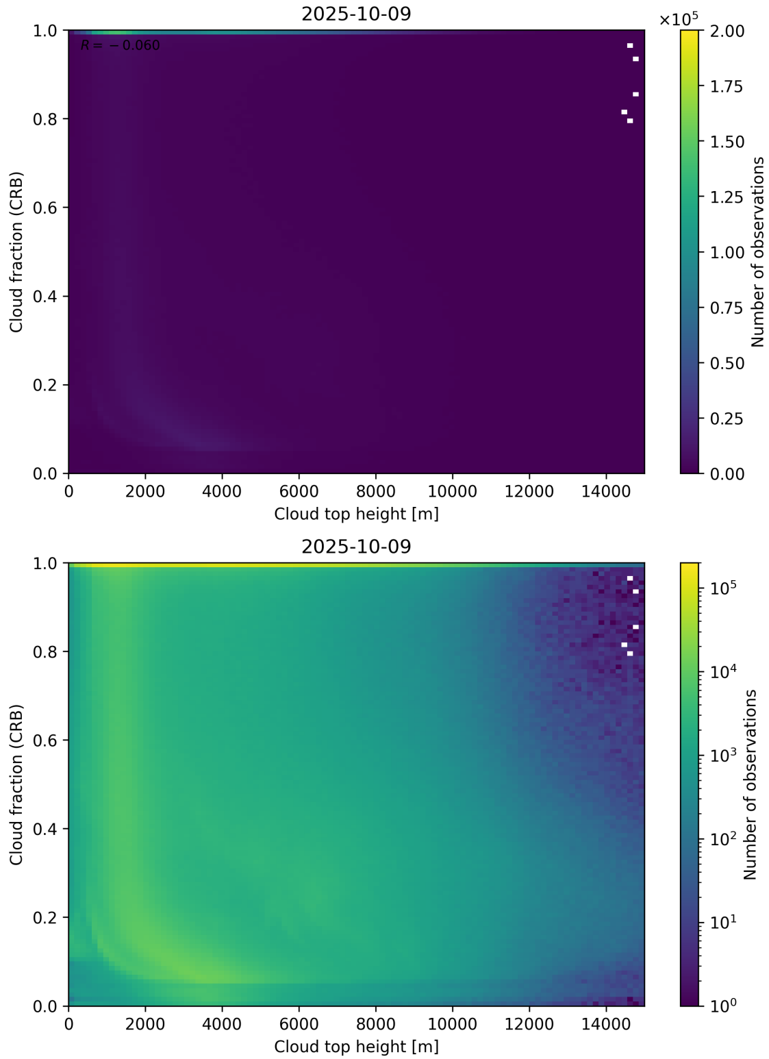
Figure 88: Scatter density plot of “Cloud top height” against “Cloud fraction (CRB)” for 2025-10-08 to 2025-10-10.
