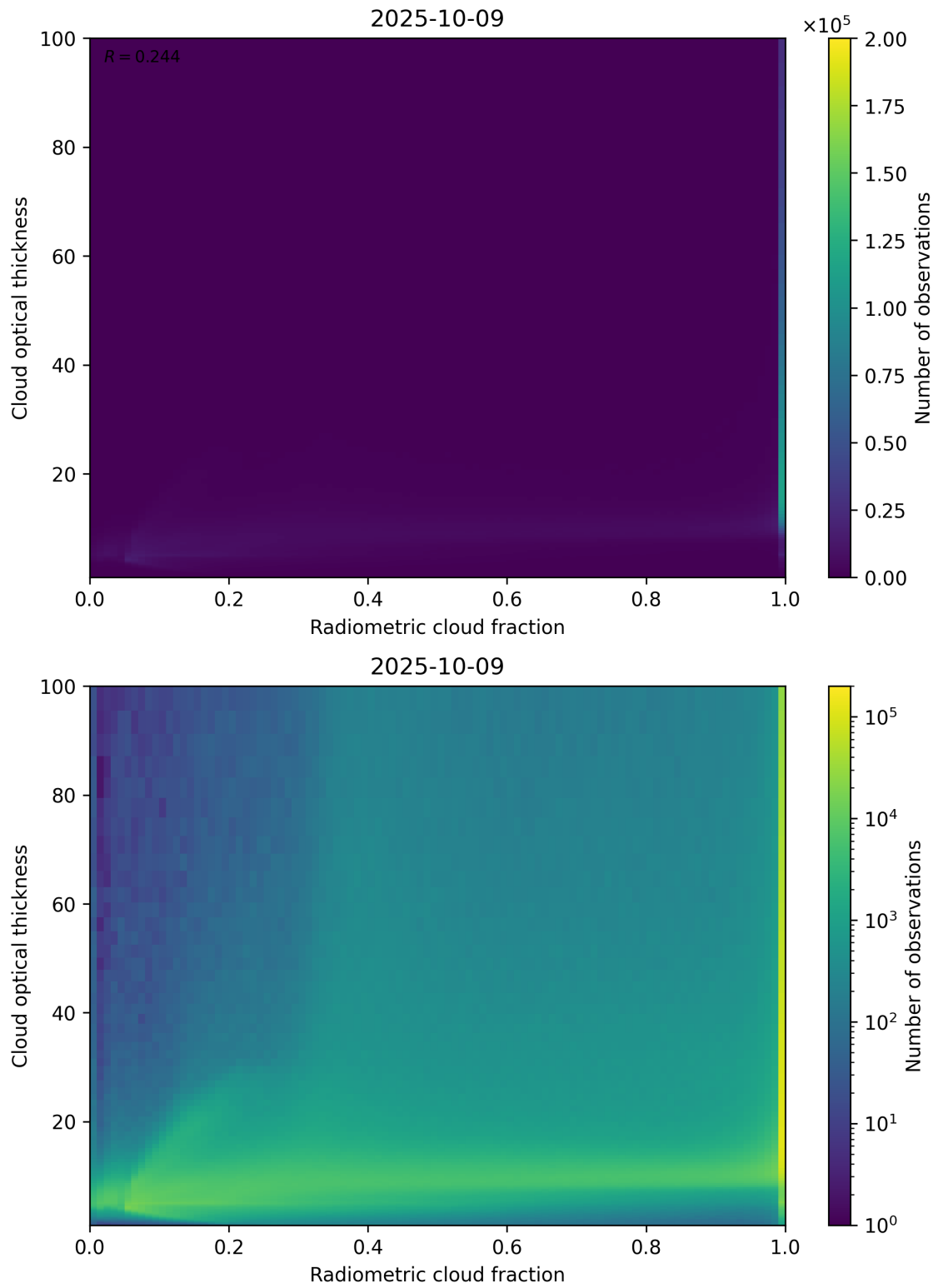
Figure 75: Scatter density plot of “Radiometric cloud fraction” against “Cloud optical thickness” for 2025-10-08 to 2025-10-10.
