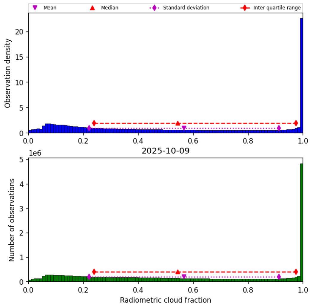
Figure 39: Histogram of “Radiometric cloud fraction” for 2025-10-08 to 2025-10-10
