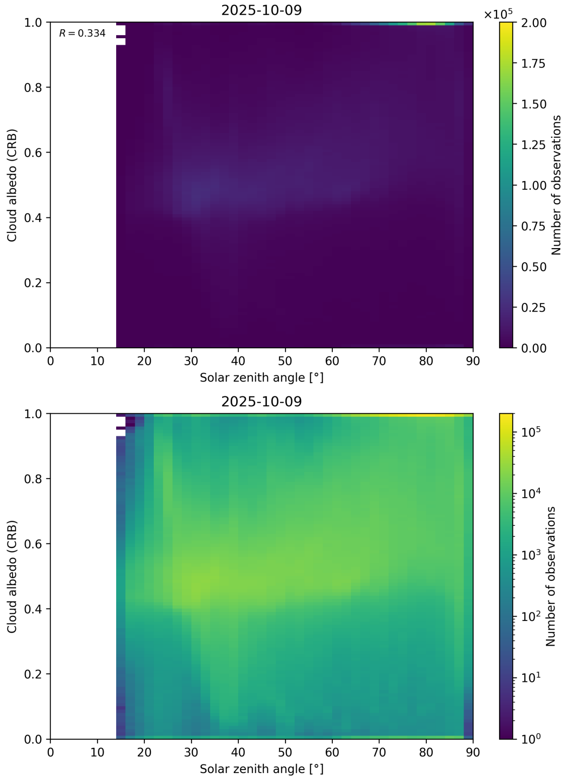
Figure 98: Scatter density plot of “Solar zenith angle” against “Cloud albedo (CRB)” for 2025-10-08 to 2025-10-10.
