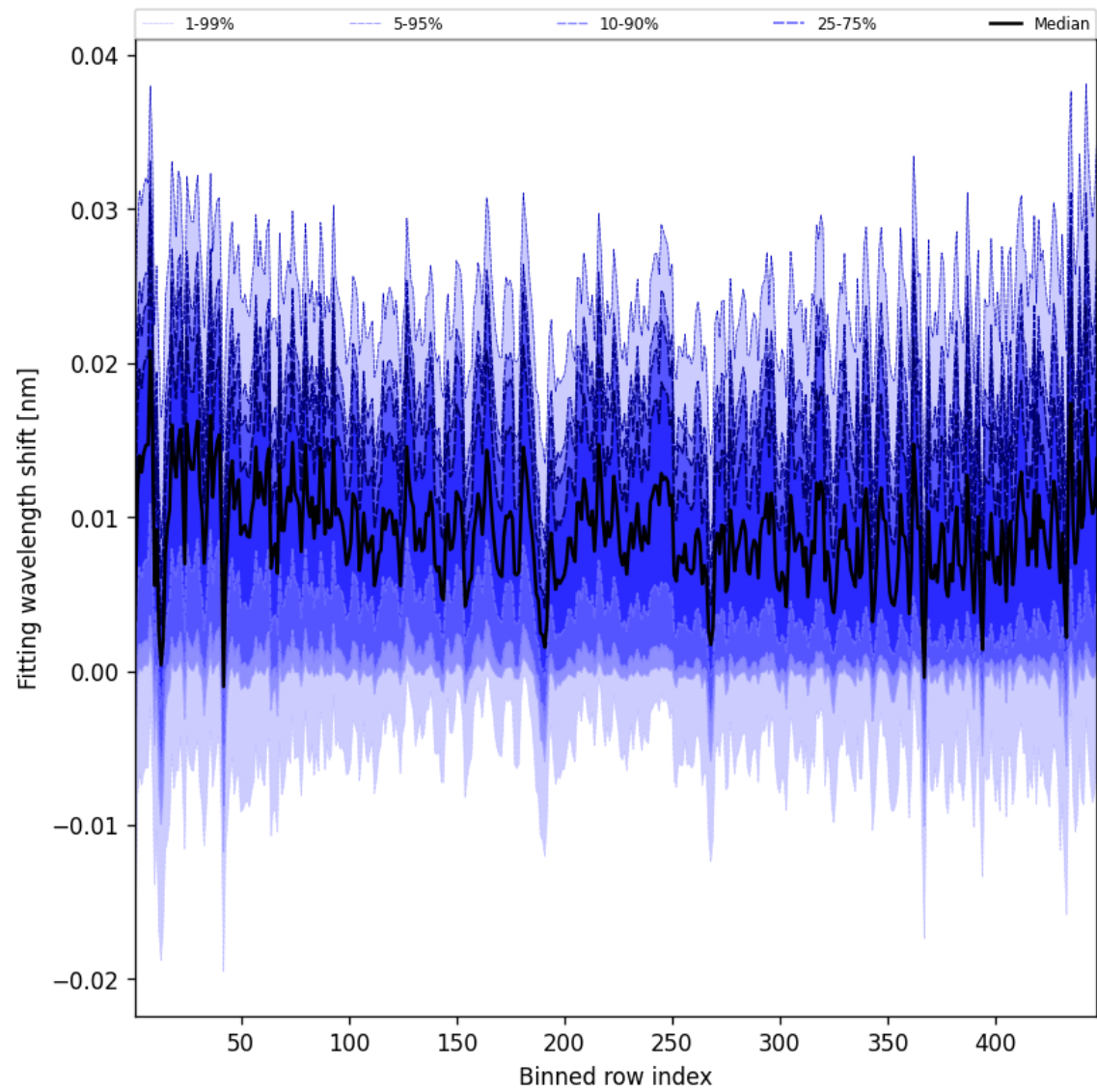
Figure 65: Along track statistics of “Fitting wavelength shift” for 2025-10-08 to 2025-10-10
