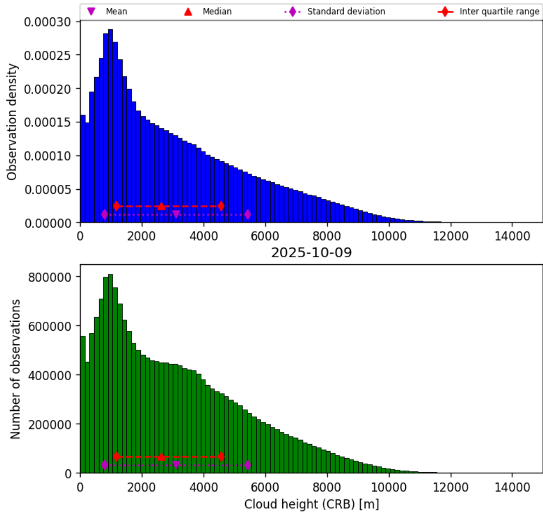
Figure 43: Histogram of “Cloud height (CRB)” for 2025-10-08 to 2025-10-10
