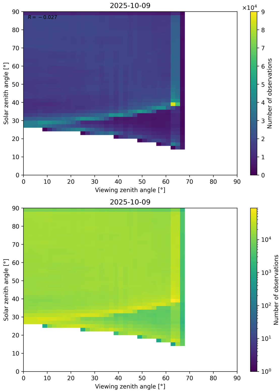
Figure 114: Scatter density plot of “Viewing zenith angle” against “Solar zenith angle” for 2025-10-08 to 2025-10-10.
