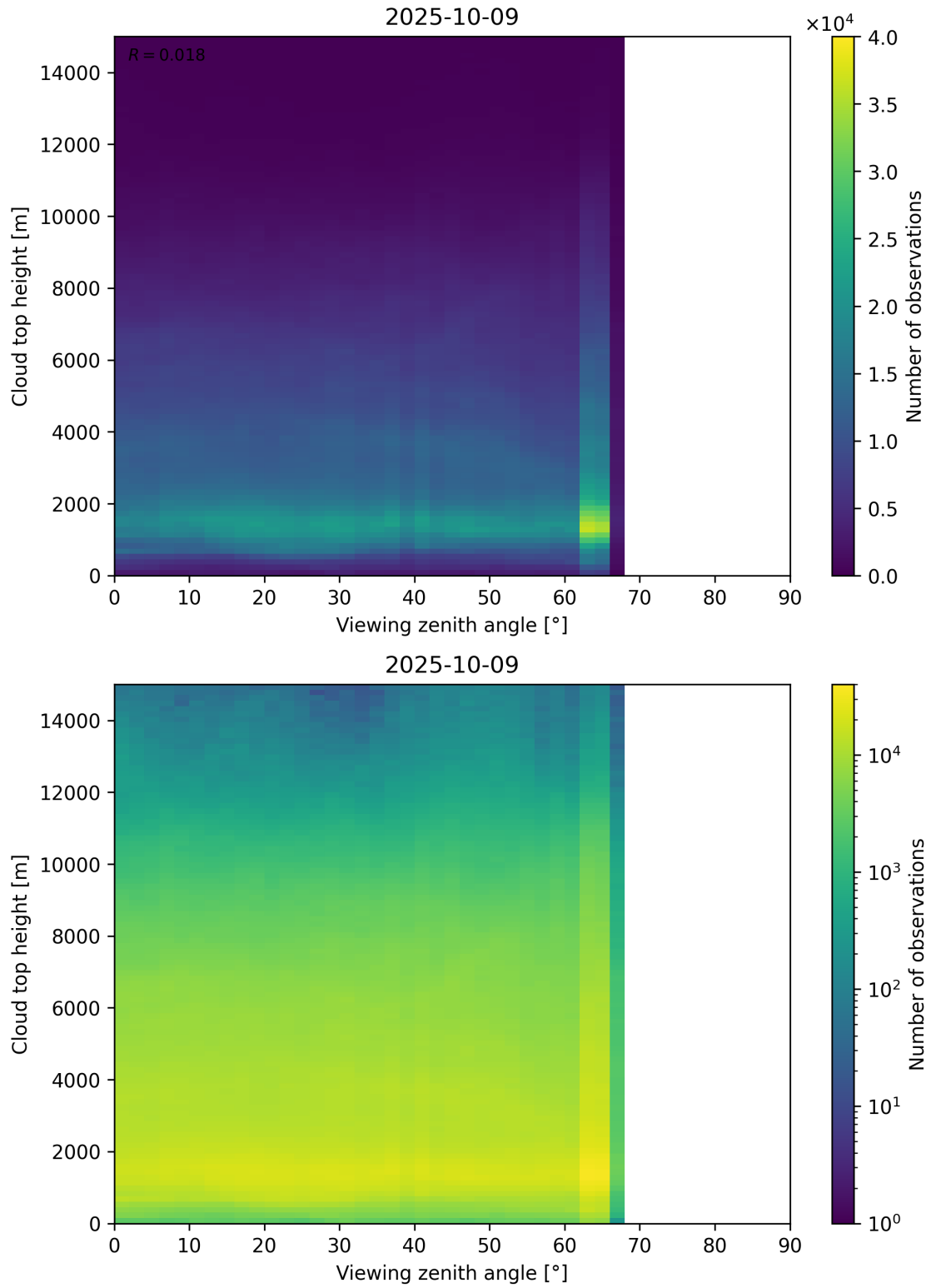
Figure 112: Scatter density plot of “Viewing zenith angle” against “Cloud top height” for 2025-10-08 to 2025-10-10.
