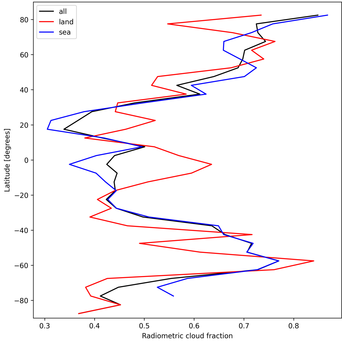
Figure 23: Zonal average of “Radiometric cloud fraction” for 2025-10-08 to 2025-10-10.
