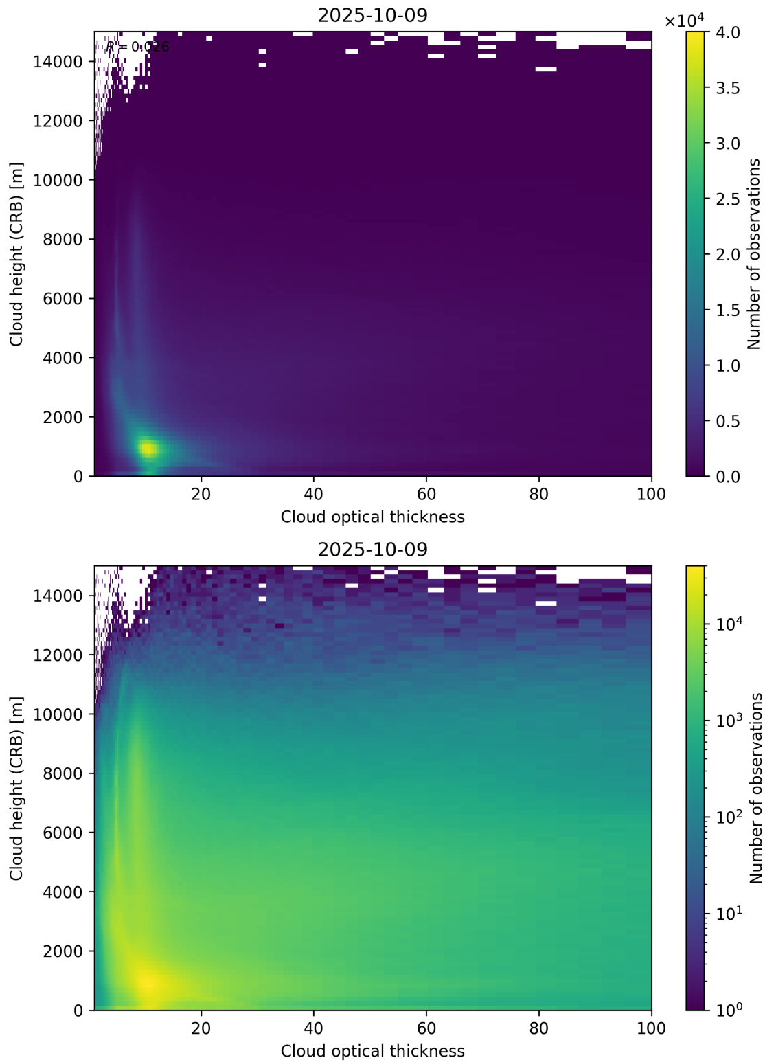
Figure 85: Scatter density plot of “Cloud optical thickness” against “Cloud height (CRB)” for 2025-10-08 to 2025-10-10.
