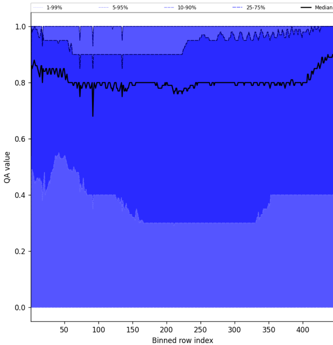
Figure 54: Along track statistics of “QA value” for 2025-10-08 to 2025-10-10
