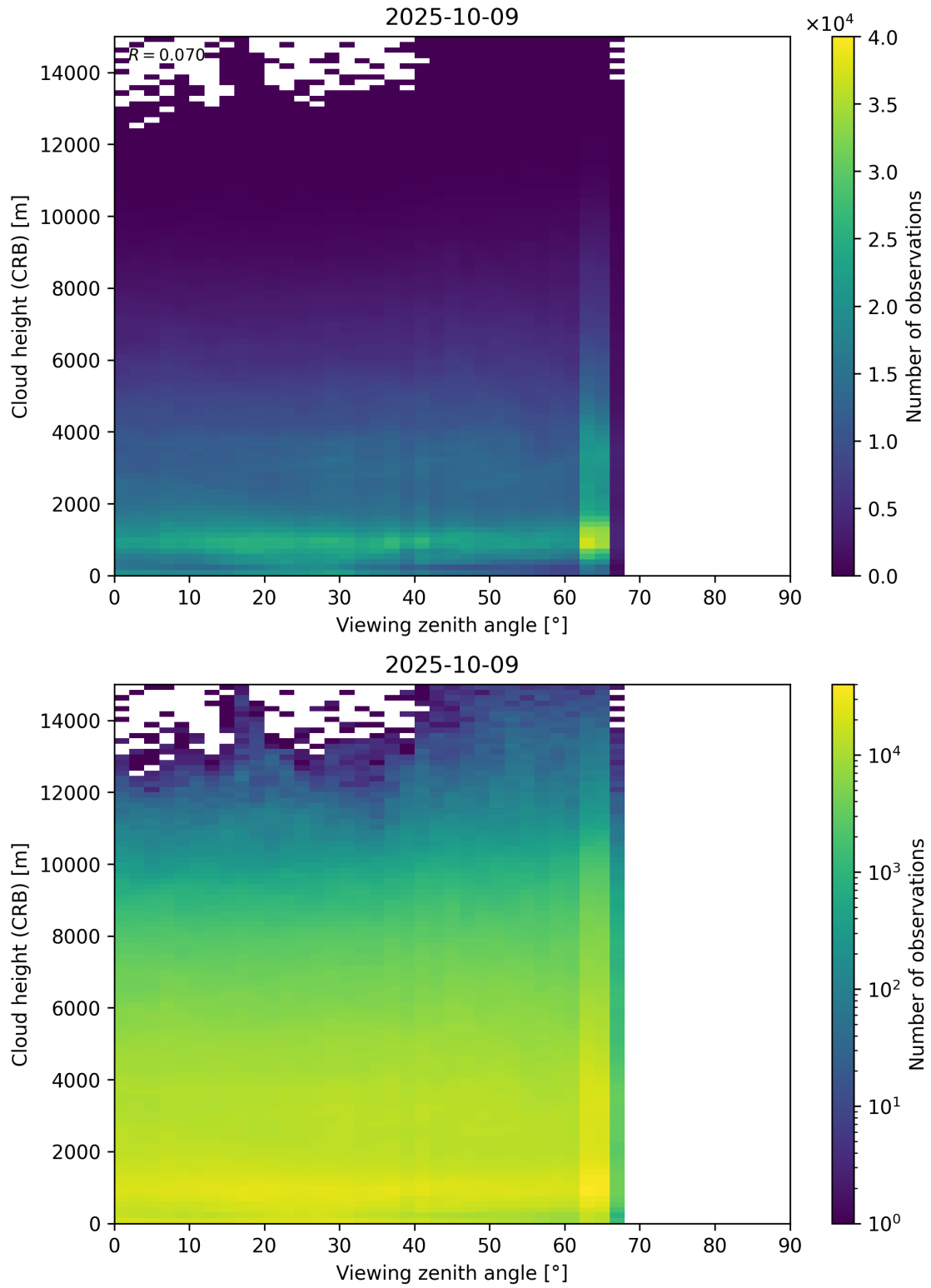
Figure 110: Scatter density plot of “Viewing zenith angle” against “Cloud height (CRB)” for 2025-10-08 to 2025-10-10.
