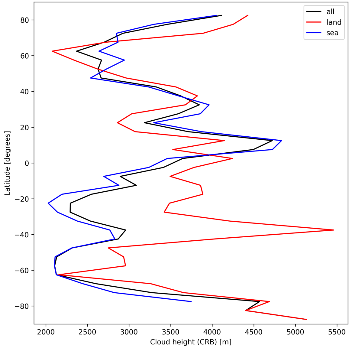
Figure 27: Zonal average of “Cloud height (CRB)” for 2025-10-08 to 2025-10-10.
