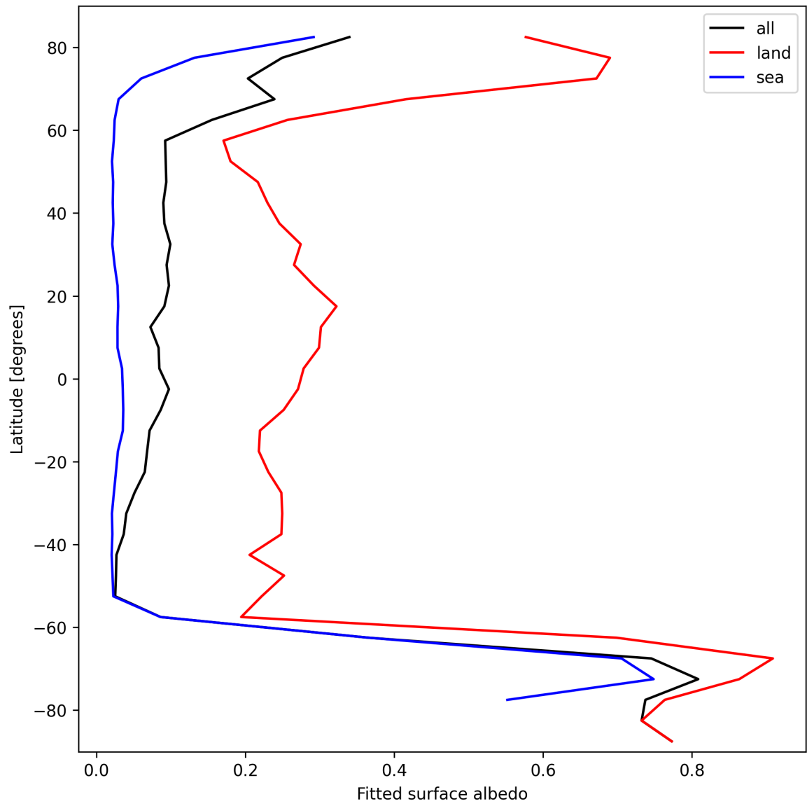
Figure 29: Zonal average of “Fitted surface albedo” for 2025-10-08 to 2025-10-10.
