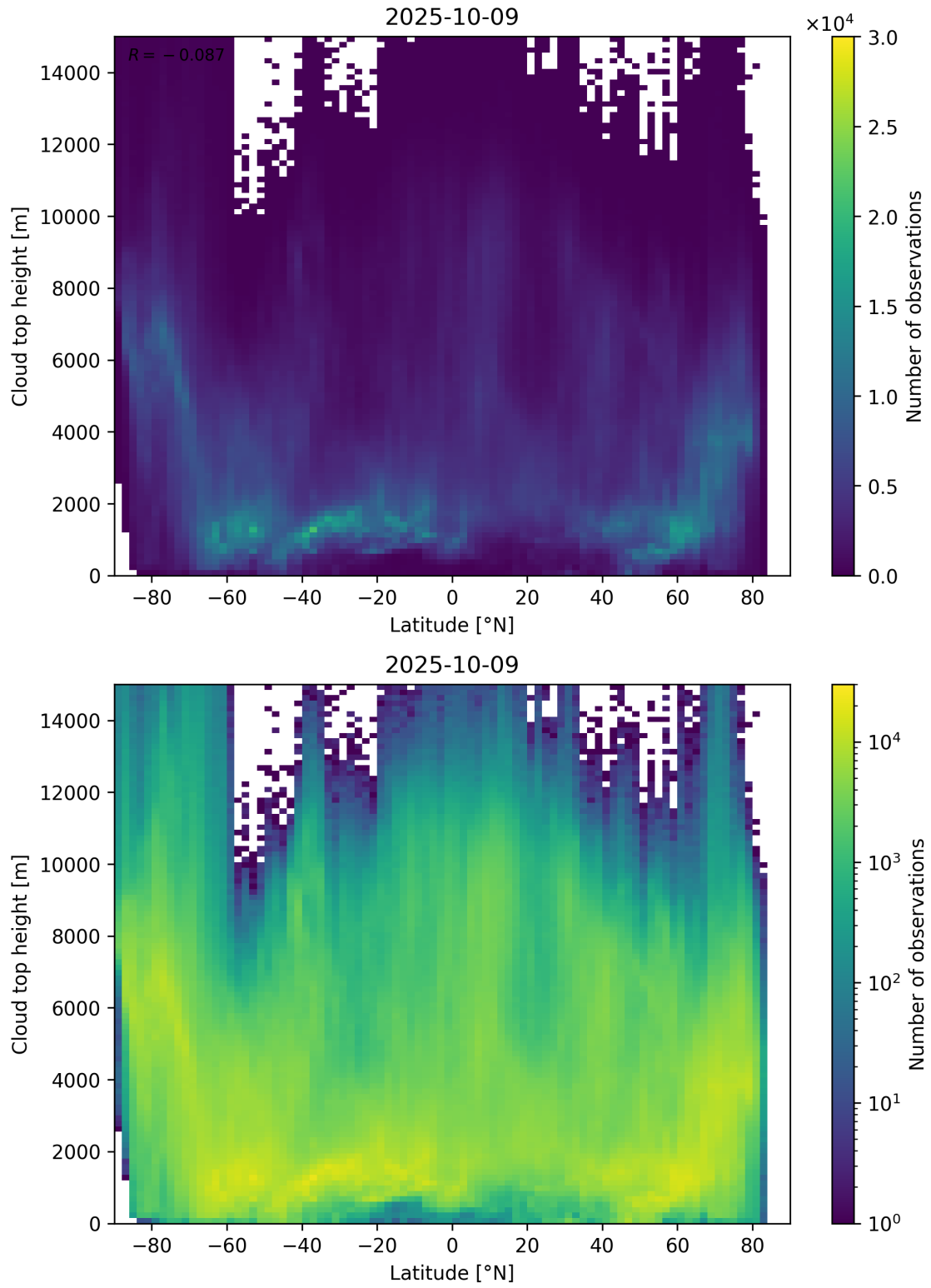
Figure 97: Scatter density plot of “Latitude” against “Cloud top height” for 2025-10-08 to 2025-10-10.
