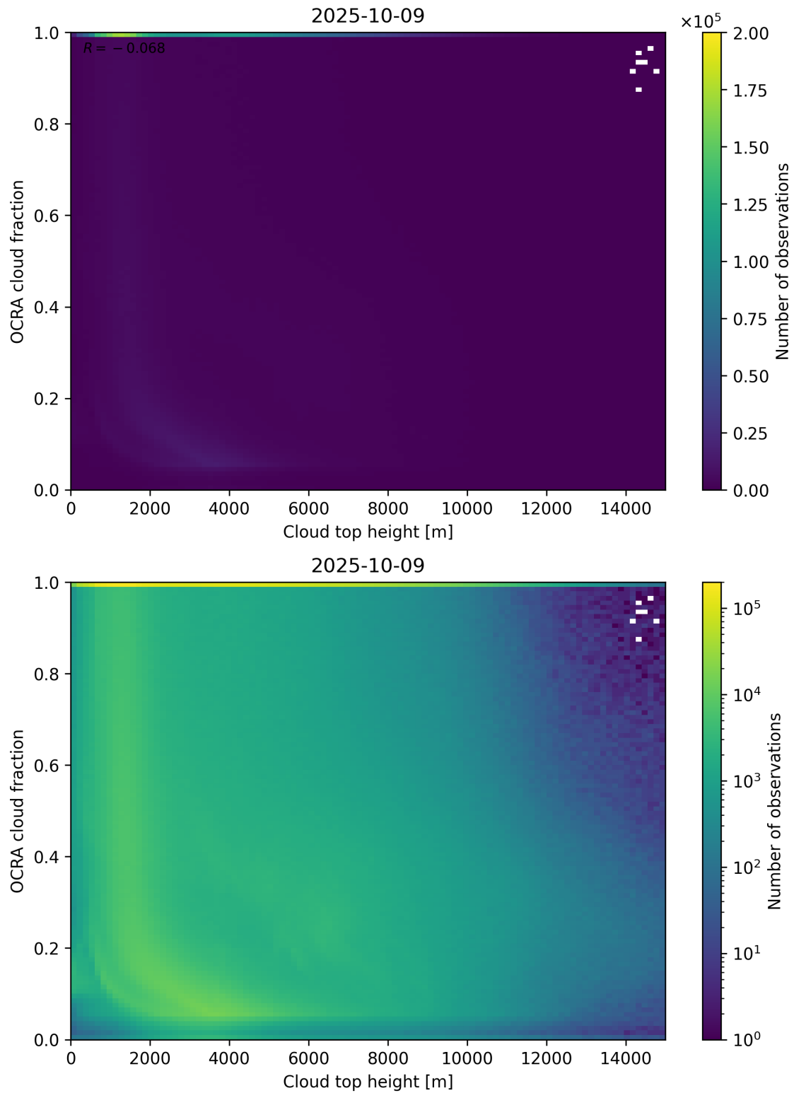
Figure 87: Scatter density plot of “Cloud top height” against “OCRA cloud fraction” for 2025-10-08 to 2025-10-10.
