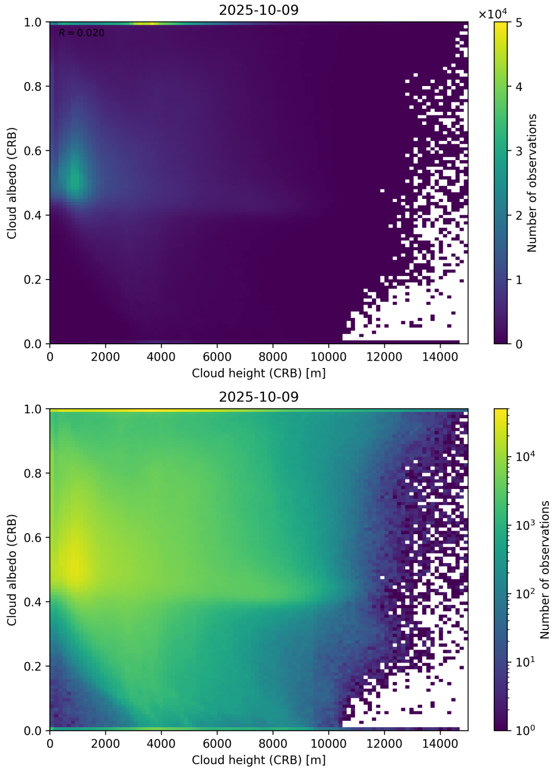
Figure 80: Scatter density plot of “Cloud height (CRB)” against “Cloud albedo (CRB)” for 2025-10-08 to 2025-10-10.
