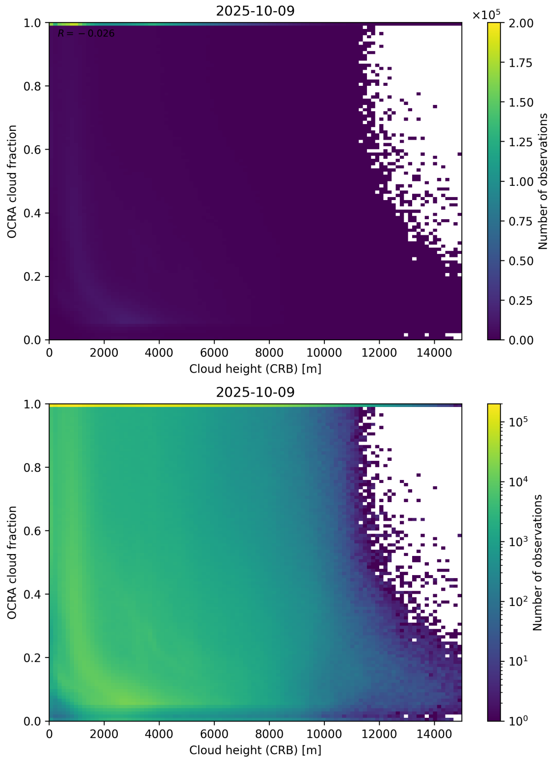
Figure 81: Scatter density plot of “Cloud height (CRB)” against “OCRA cloud fraction” for 2025-10-08 to 2025-10-10.
