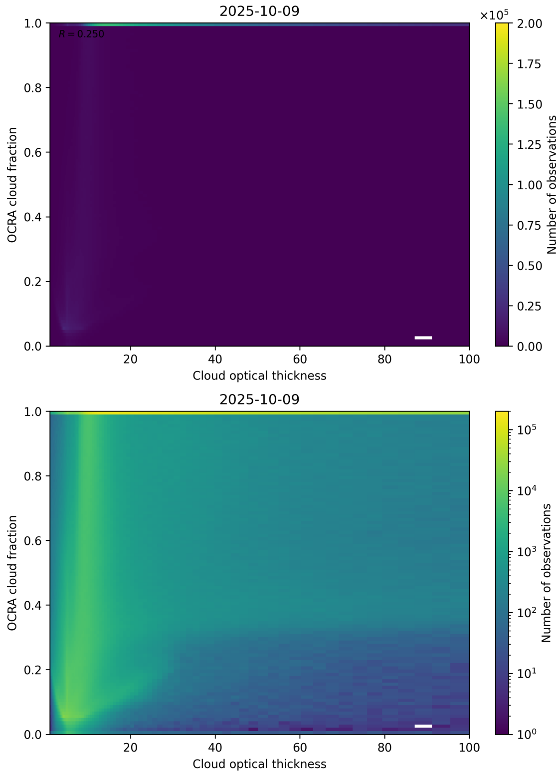
Figure 83: Scatter density plot of “Cloud optical thickness” against “OCRA cloud fraction” for 2025-10-08 to 2025-10-10.
