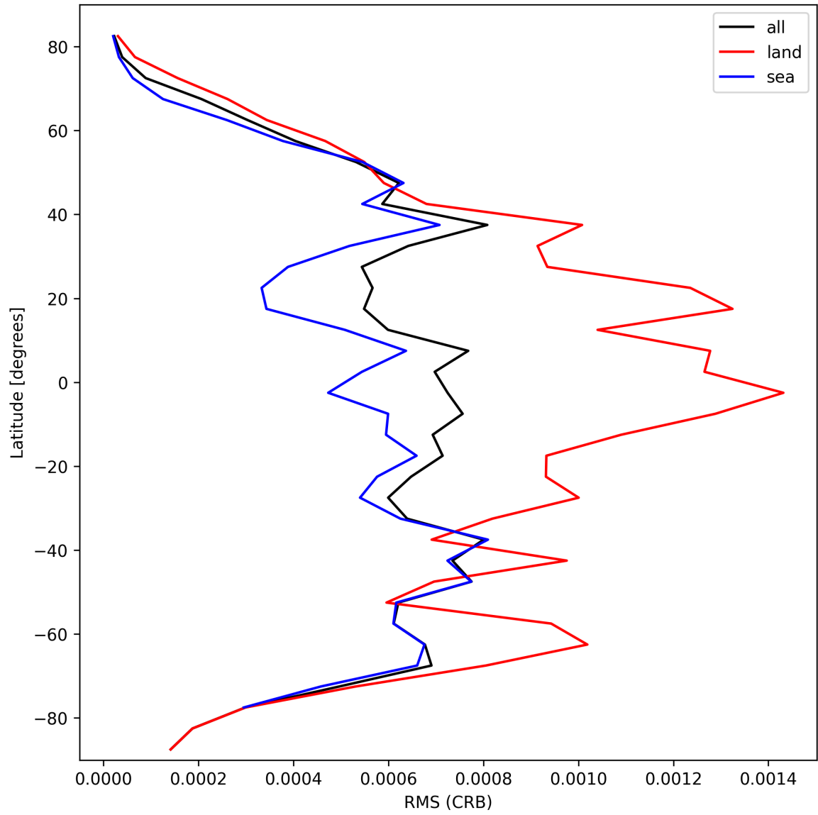
Figure 32: Zonal average of “RMS (CRB)” for 2025-10-08 to 2025-10-10.
