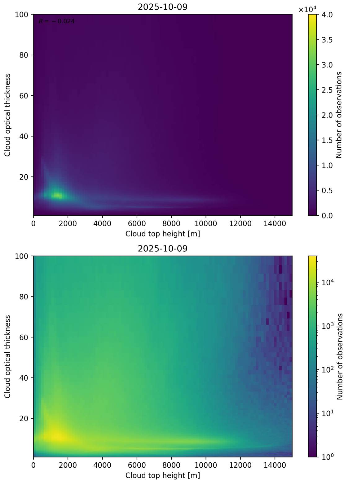
Figure 90: Scatter density plot of “Cloud top height” against “Cloud optical thickness” for 2025-10-08 to 2025-10-10.
