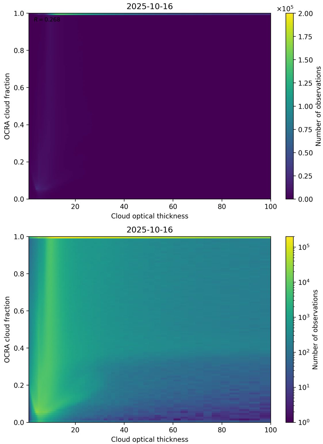
Figure 83: Scatter density plot of “Cloud optical thickness” against “OCRA cloud fraction” for 2025-10-15 to 2025-10-17.
