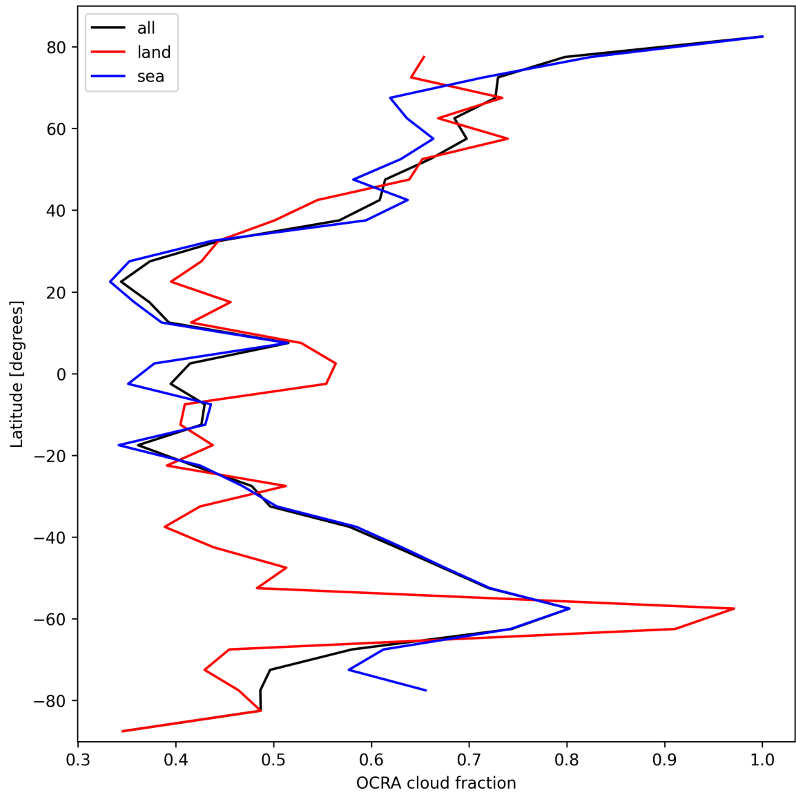
Figure 34: Zonal average of “OCRA cloud fraction” for 2025-10-15 to 2025-10-17.
