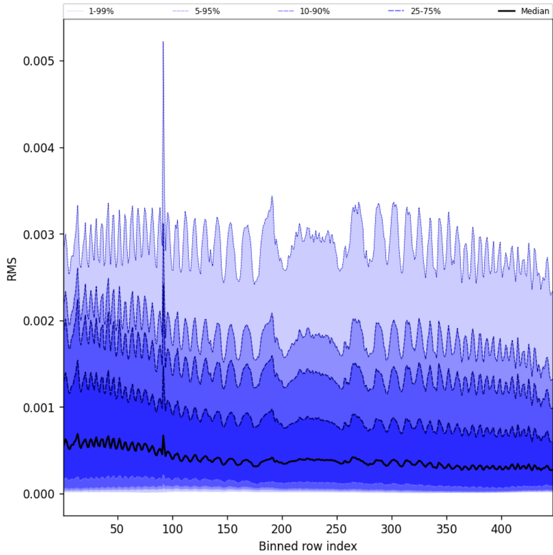
Figure 63: Along track statistics of “RMS” for 2025-10-15 to 2025-10-17
