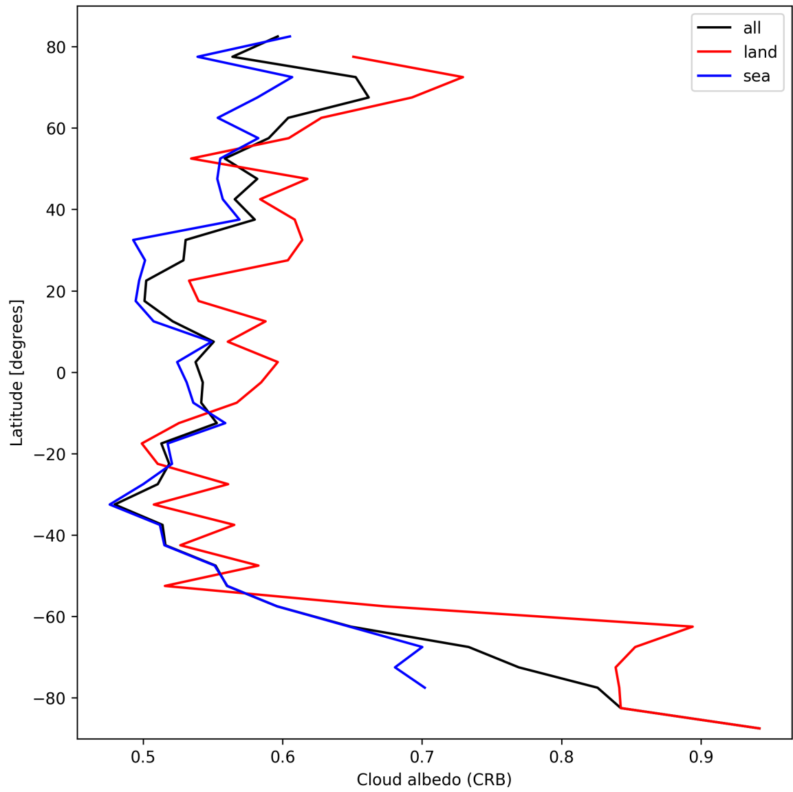
Figure 28: Zonal average of “Cloud albedo (CRB)” for 2025-10-15 to 2025-10-17.
