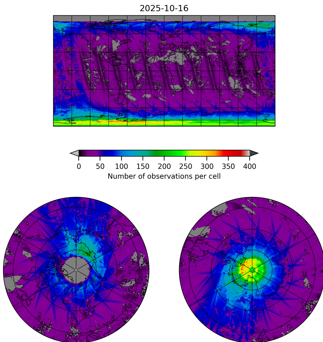
Figure 21: Map of the number of observations for 2025-10-15 to 2025-10-17
