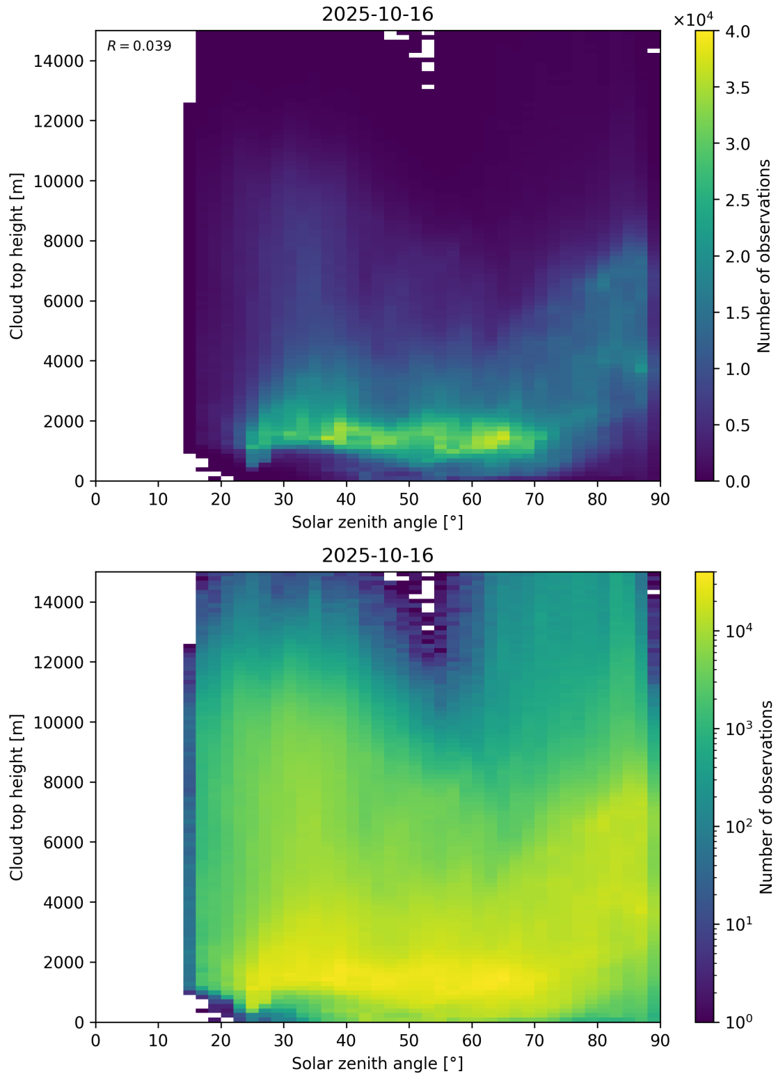
Figure 104: Scatter density plot of “Solar zenith angle” against “Cloud top height” for 2025-10-15 to 2025-10-17.
