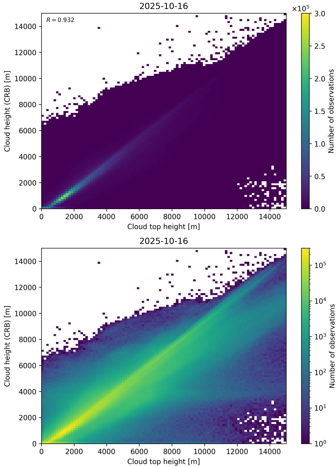
Figure 89: Scatter density plot of “Cloud top height” against “Cloud height (CRB)” for 2025-10-15 to 2025-10-17.
