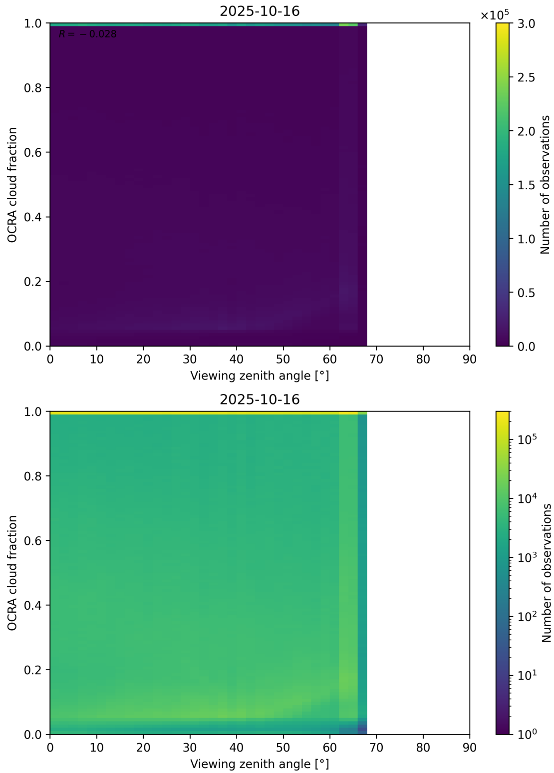
Figure 108: Scatter density plot of “Viewing zenith angle” against “OCRA cloud fraction” for 2025-10-15 to 2025-10-17.
