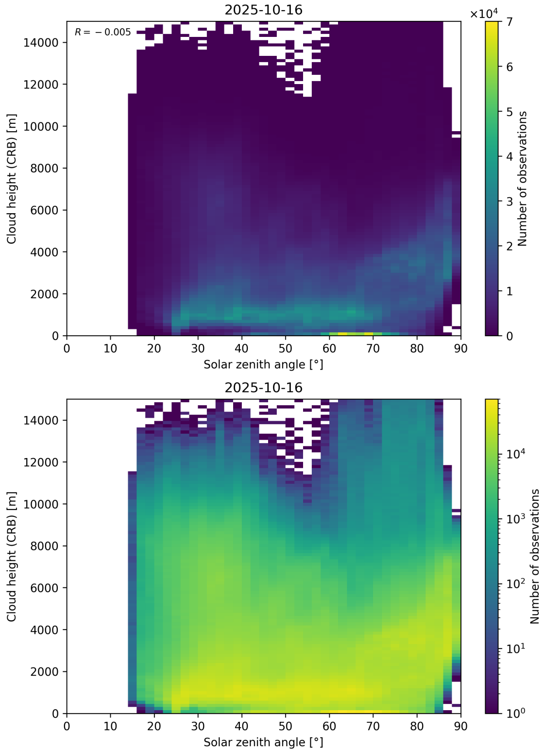
Figure 102: Scatter density plot of “Solar zenith angle” against “Cloud height (CRB)” for 2025-10-15 to 2025-10-17.
