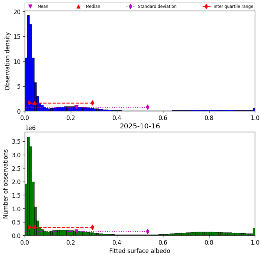
Figure 45: Histogram of “Fitted surface albedo” for 2025-10-15 to 2025-10-17
