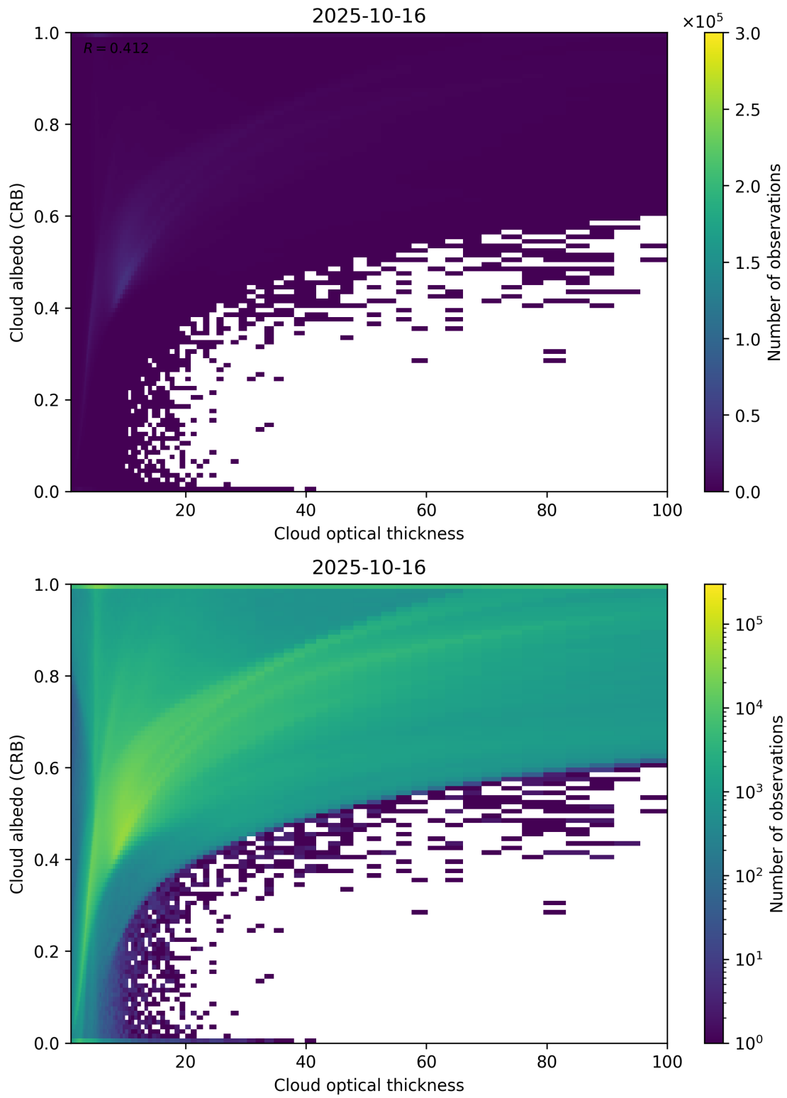
Figure 82: Scatter density plot of “Cloud optical thickness” against “Cloud albedo (CRB)” for 2025-10-15 to 2025-10-17.
