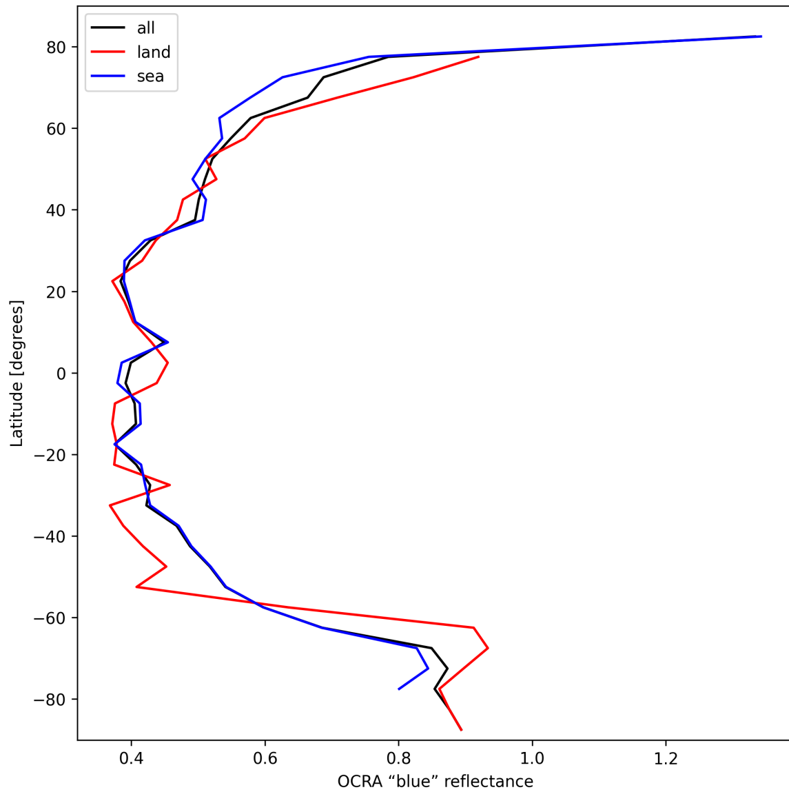
Figure 35: Zonal average of “OCRA “blue” reflectance” for 2025-10-15 to 2025-10-17.
