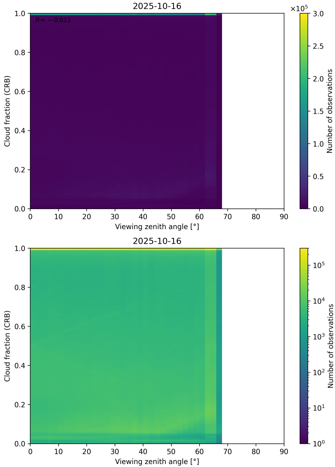
Figure 109: Scatter density plot of “Viewing zenith angle” against “Cloud fraction (CRB)” for 2025-10-15 to 2025-10-17.
