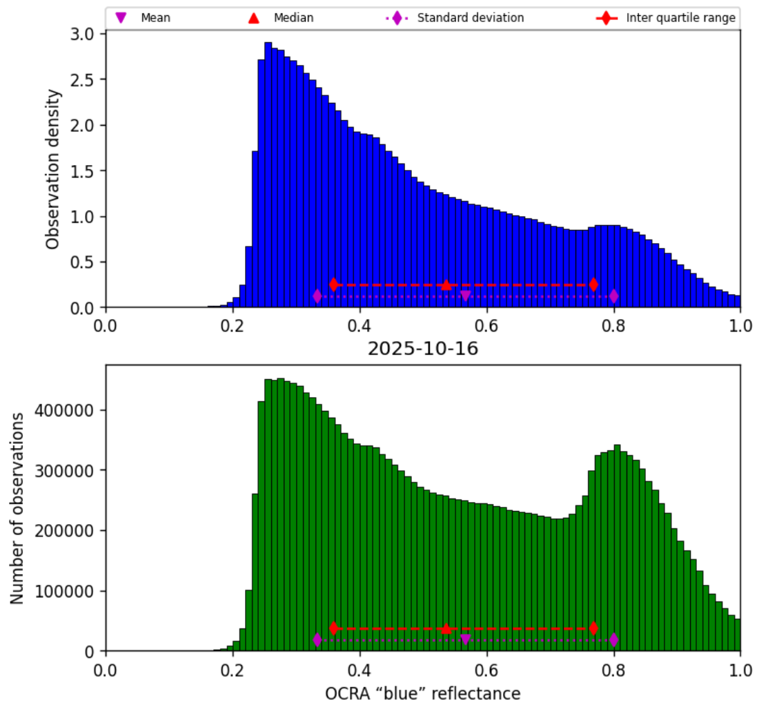
Figure 51: Histogram of “OCRA “blue” reflectance” for 2025-10-15 to 2025-10-17
