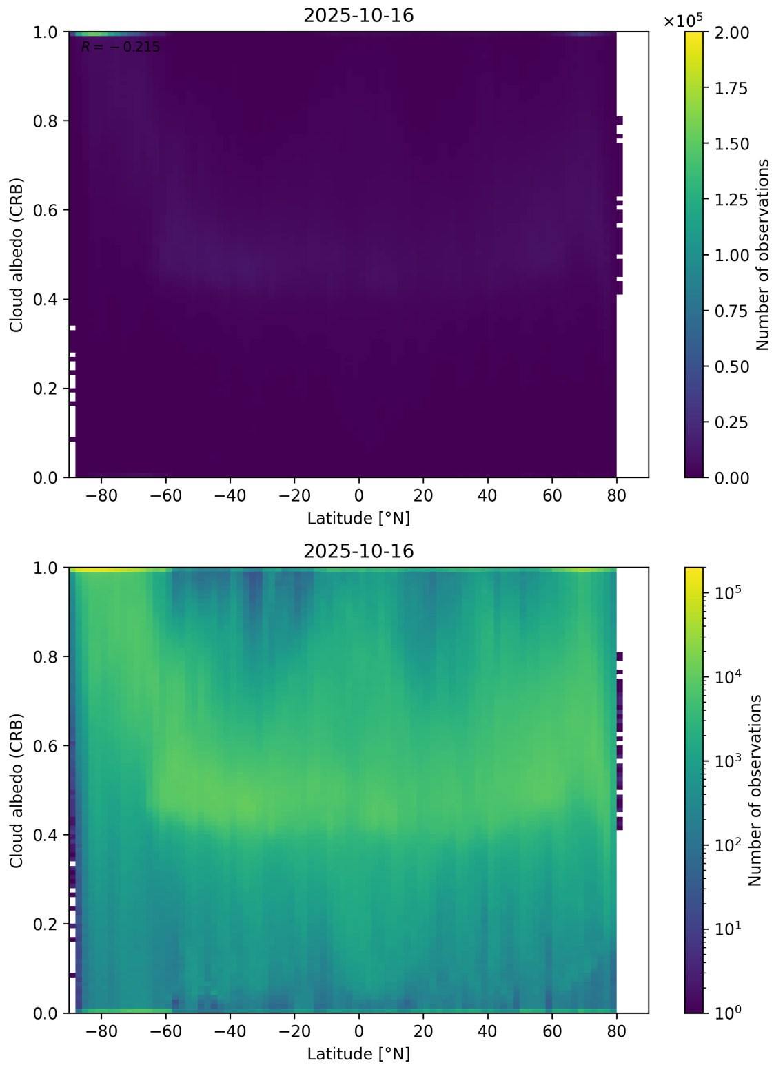
Figure 91: Scatter density plot of “Latitude” against “Cloud albedo (CRB)” for 2025-10-15 to 2025-10-17.
