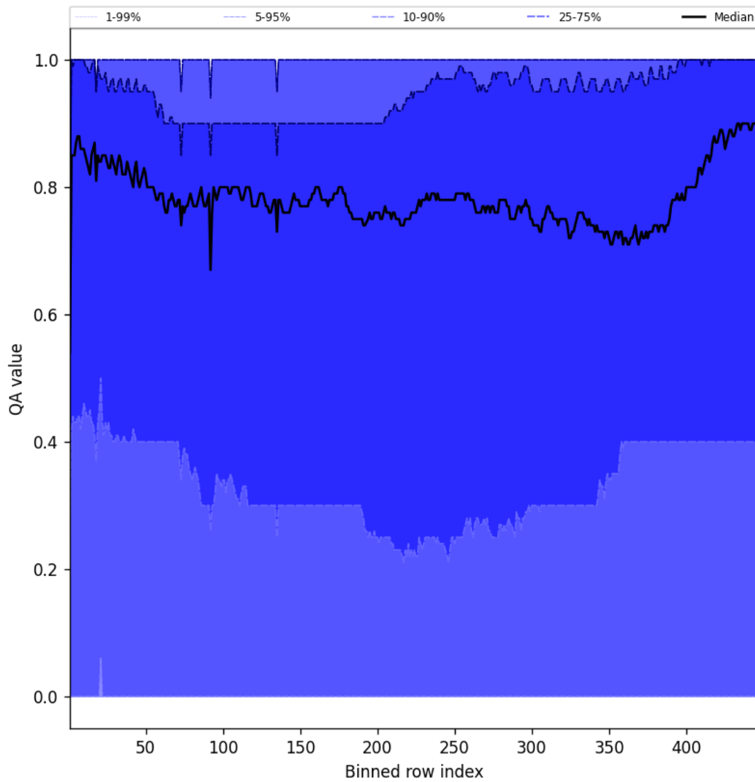
Figure 54: Along track statistics of “QA value” for 2025-10-15 to 2025-10-17
