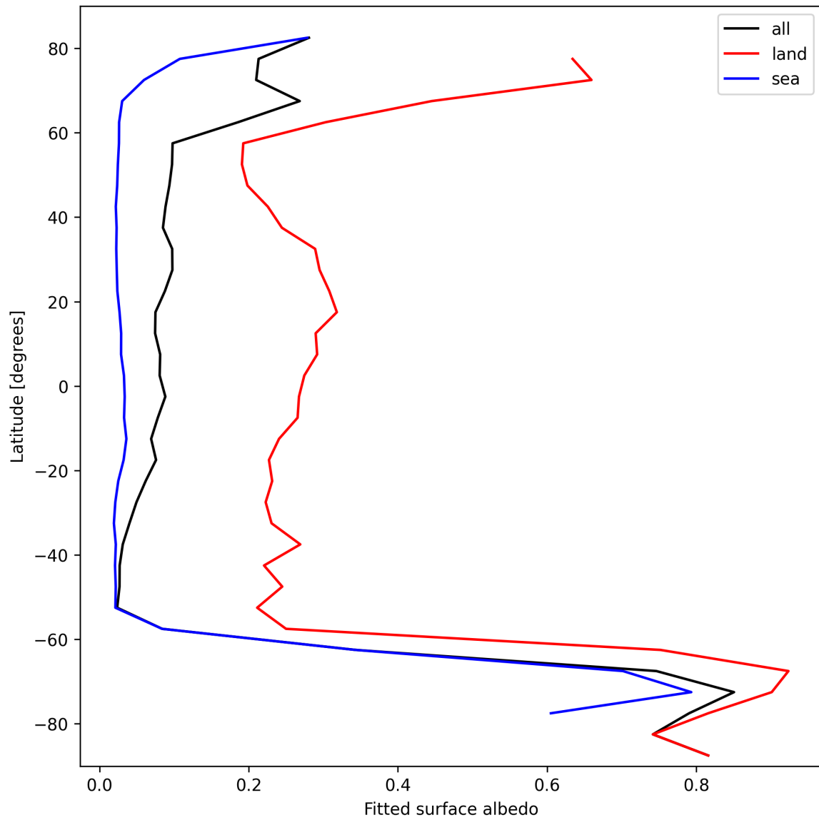
Figure 29: Zonal average of “Fitted surface albedo” for 2025-10-15 to 2025-10-17.
