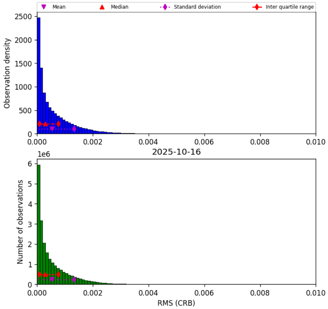
Figure 48: Histogram of “RMS (CRB)” for 2025-10-15 to 2025-10-17
