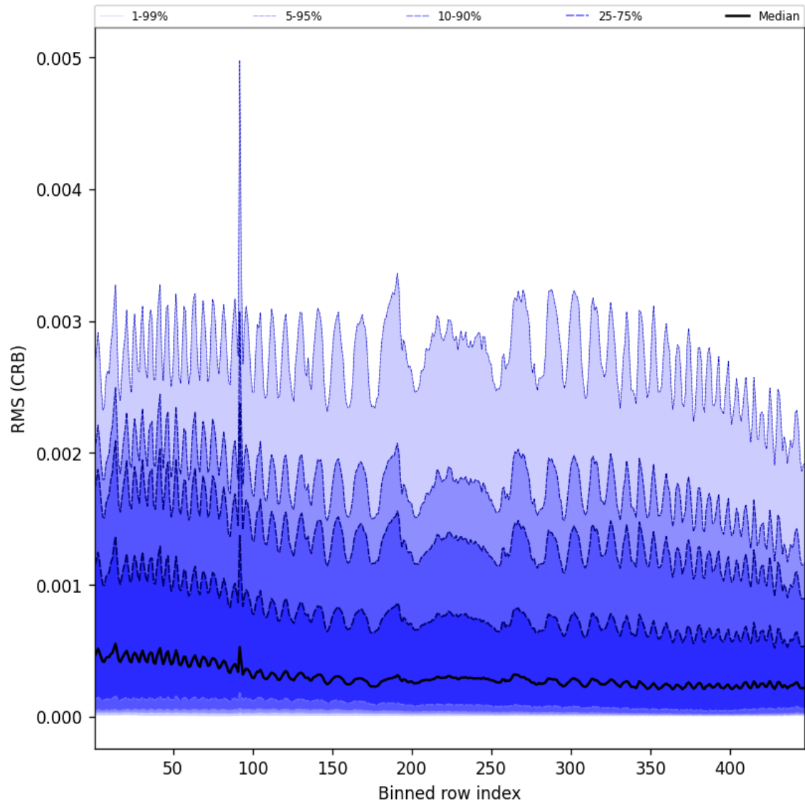
Figure 64: Along track statistics of “RMS (CRB)” for 2025-10-15 to 2025-10-17
