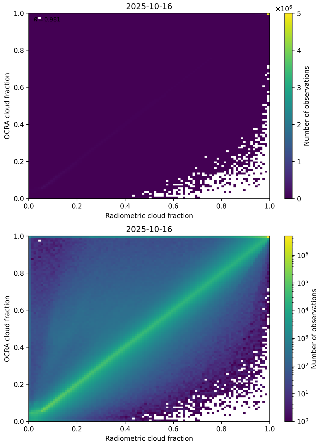
Figure 72: Scatter density plot of “Radiometric cloud fraction” against “OCRA cloud fraction” for 2025-10-15 to 2025-10-17.
