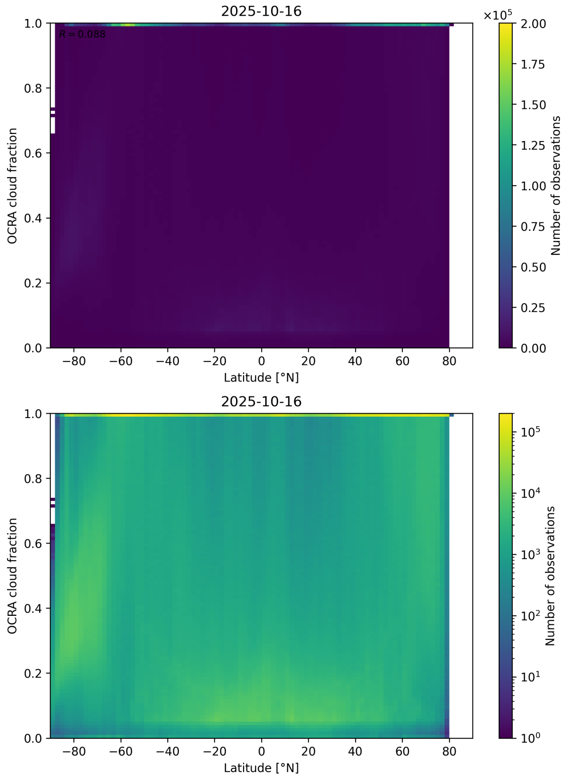
Figure 93: Scatter density plot of “Latitude” against “OCRA cloud fraction” for 2025-10-15 to 2025-10-17.
