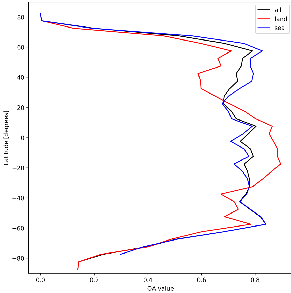
Figure 22: Zonal average of “QA value” for 2025-10-15 to 2025-10-17.
