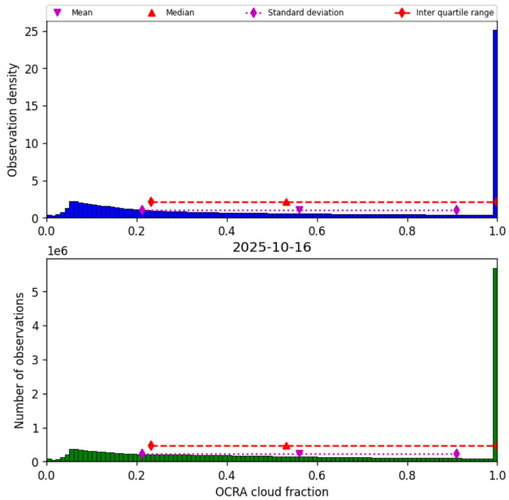
Figure 50: Histogram of “OCRA cloud fraction” for 2025-10-15 to 2025-10-17
