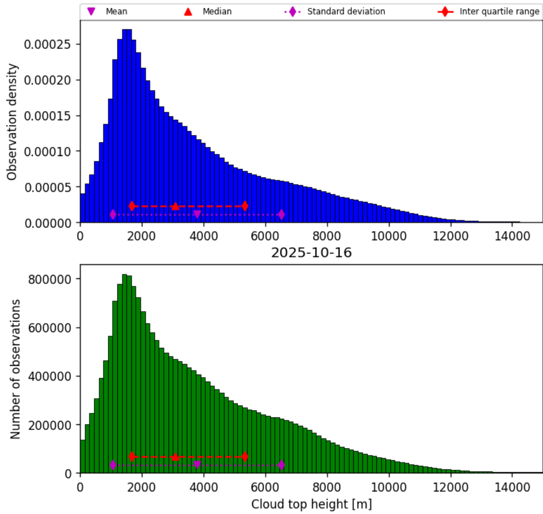
Figure 40: Histogram of “Cloud top height” for 2025-10-15 to 2025-10-17
