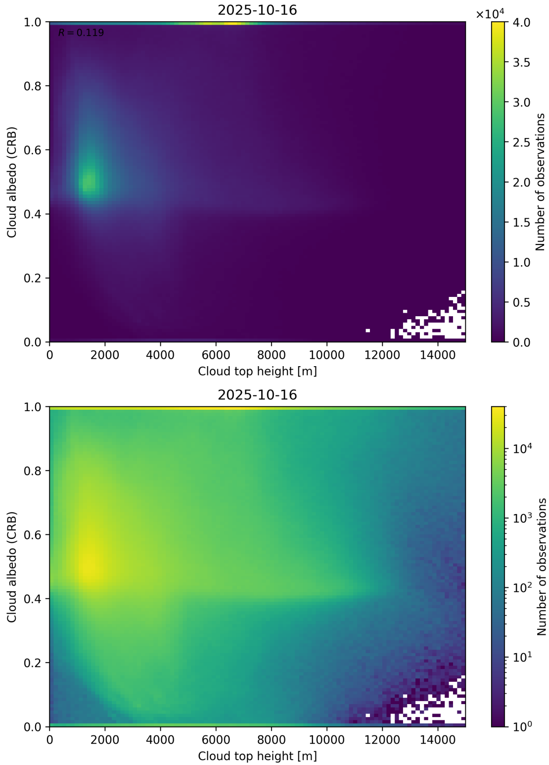
Figure 86: Scatter density plot of “Cloud top height” against “Cloud albedo (CRB)” for 2025-10-15 to 2025-10-17.
