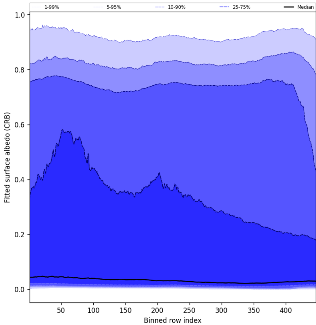
Figure 62: Along track statistics of “Fitted surface albedo (CRB)” for 2025-10-15 to 2025-10-17
