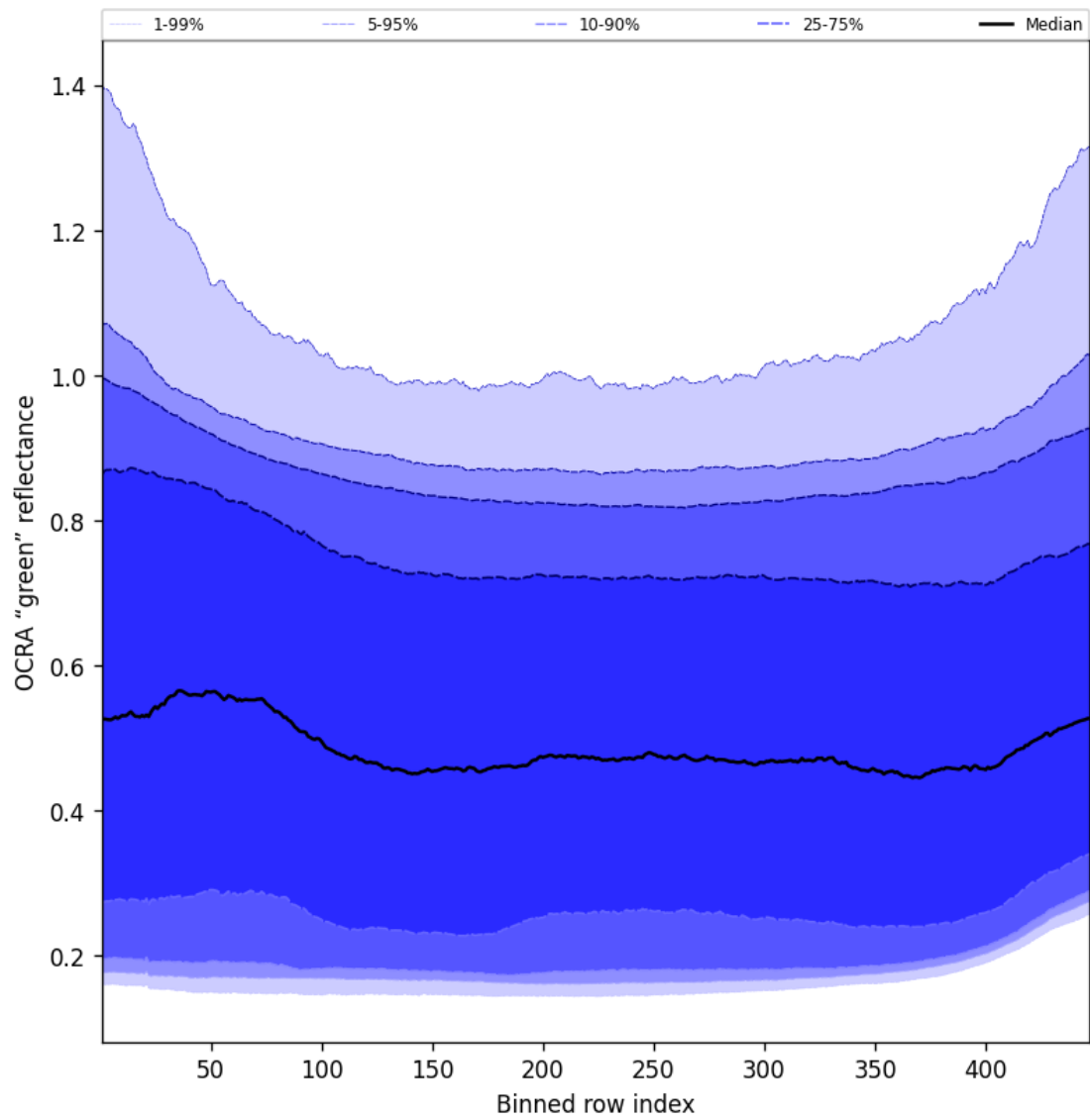
Figure 68: Along track statistics of “OCRA “green” reflectance” for 2025-10-15 to 2025-10-17
