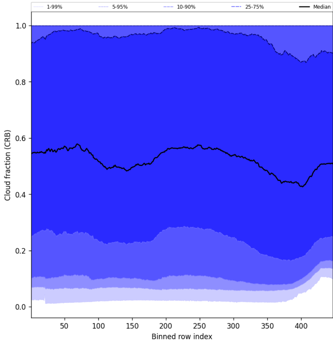
Figure 58: Along track statistics of “Cloud fraction (CRB)” for 2025-10-15 to 2025-10-17
