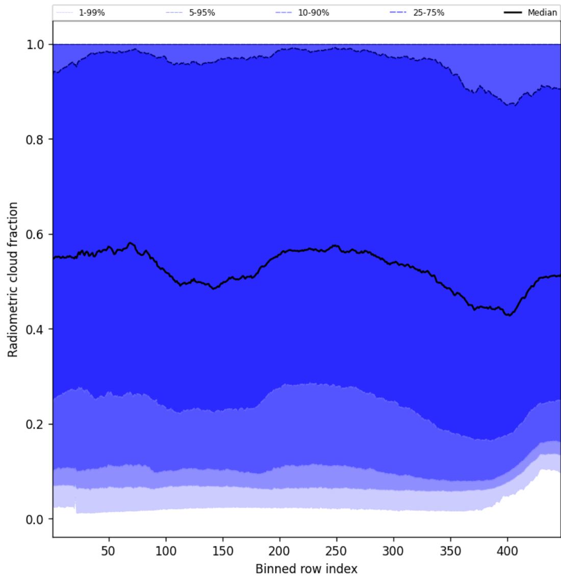
Figure 55: Along track statistics of “Radiometric cloud fraction” for 2025-10-15 to 2025-10-17
