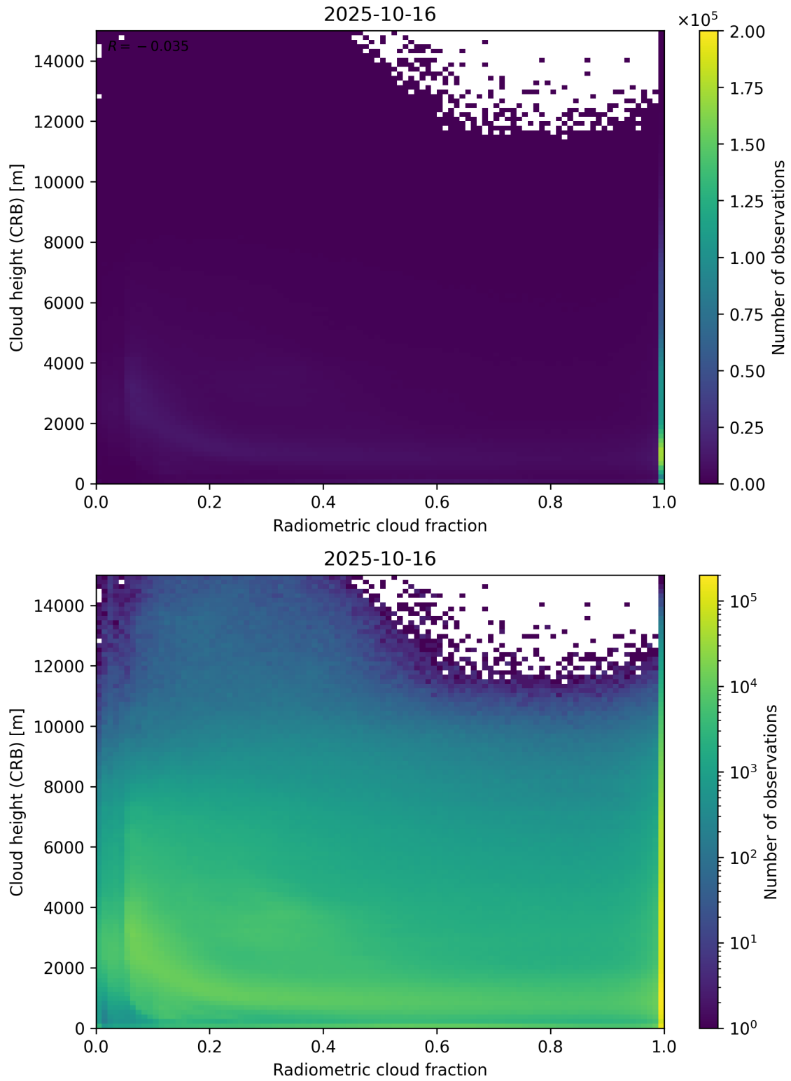
Figure 74: Scatter density plot of “Radiometric cloud fraction” against “Cloud height (CRB)” for 2025-10-15 to 2025-10-17.
