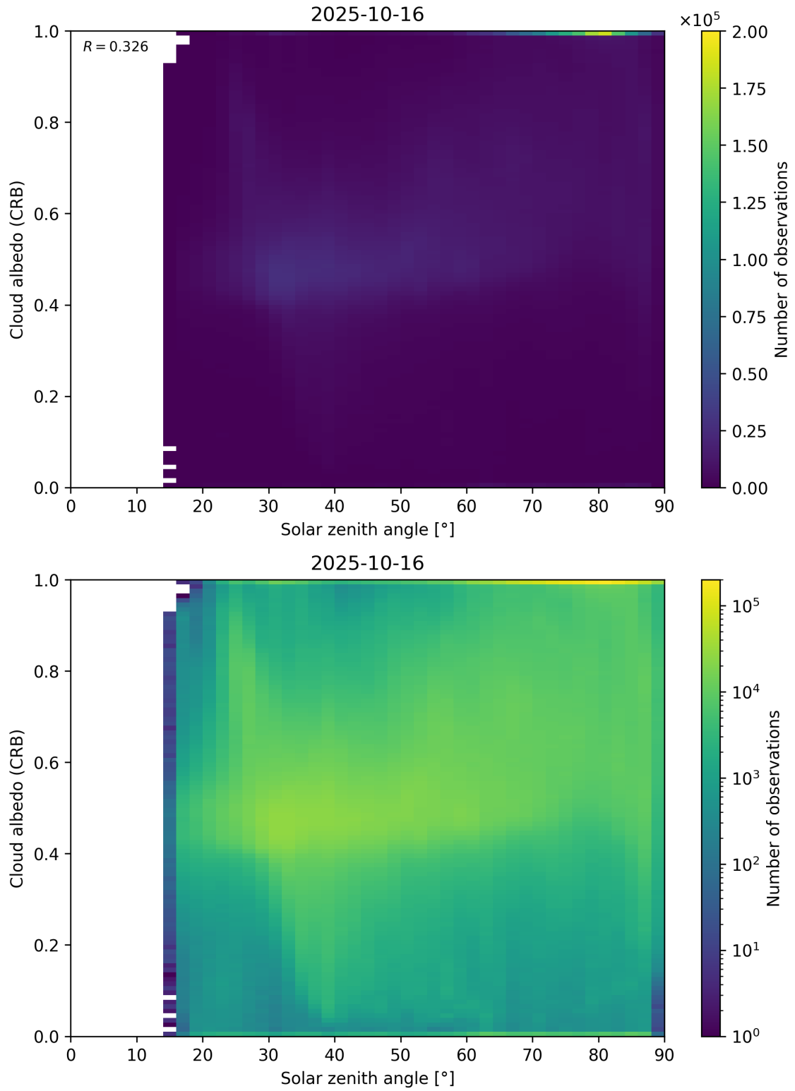
Figure 98: Scatter density plot of “Solar zenith angle” against “Cloud albedo (CRB)” for 2025-10-15 to 2025-10-17.
