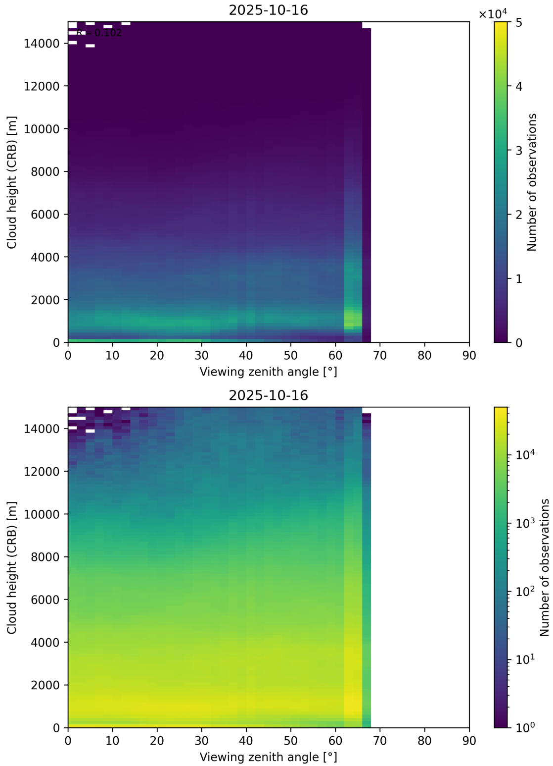
Figure 110: Scatter density plot of “Viewing zenith angle” against “Cloud height (CRB)” for 2025-10-15 to 2025-10-17.
