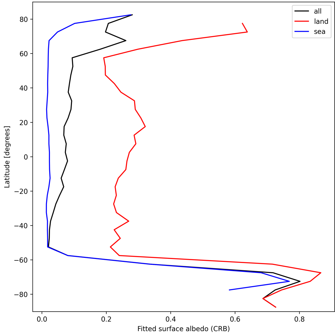
Figure 30: Zonal average of “Fitted surface albedo (CRB)” for 2025-10-15 to 2025-10-17.
