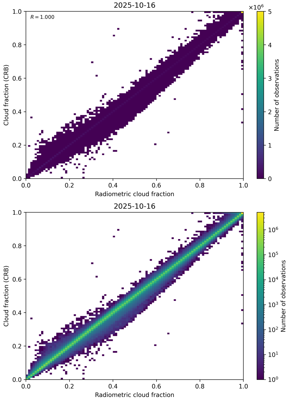
Figure 73: Scatter density plot of “Radiometric cloud fraction” against “Cloud fraction (CRB)” for 2025-10-15 to 2025-10-17.
