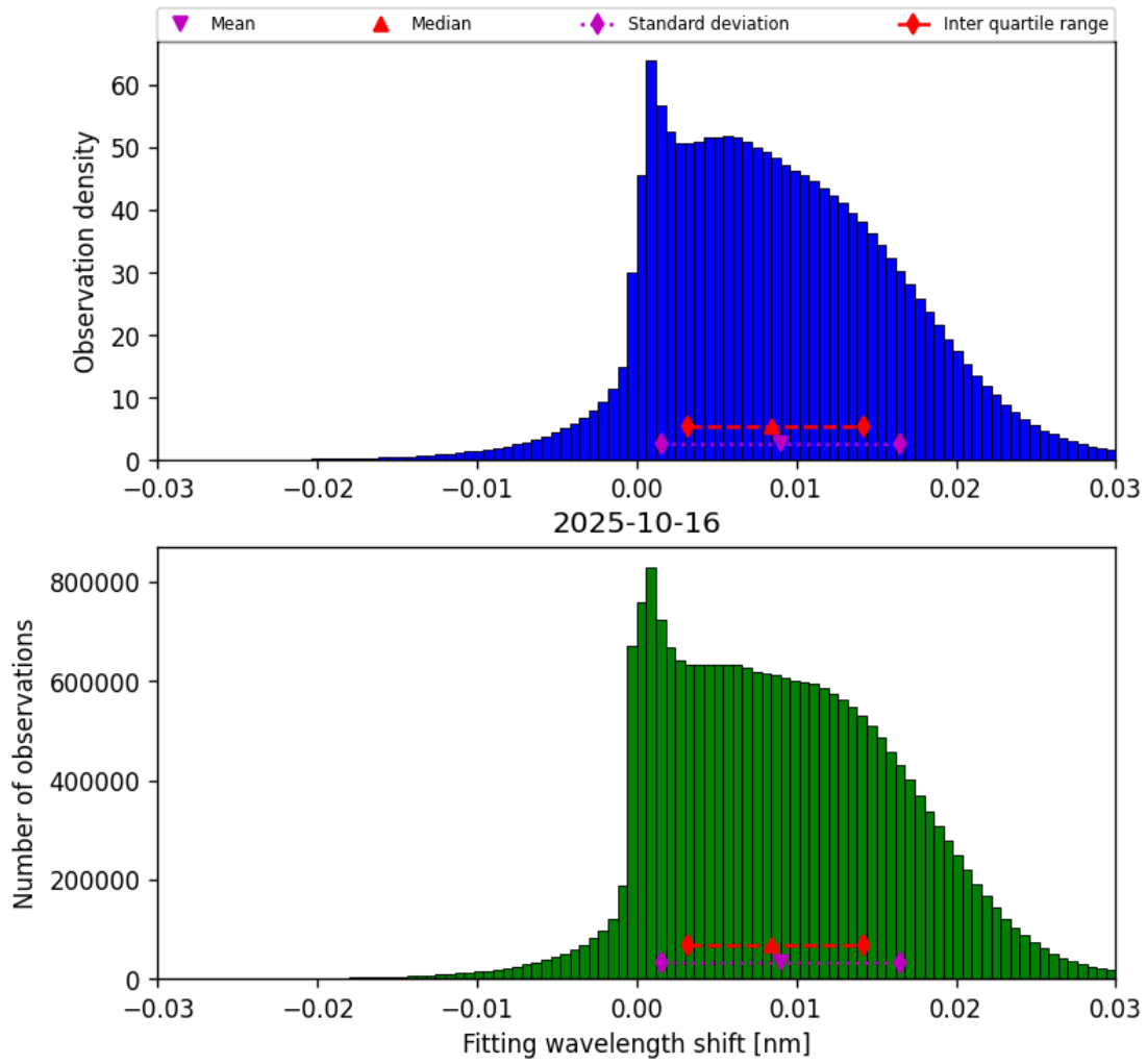
Figure 49: Histogram of “Fitting wavelength shift” for 2025-10-15 to 2025-10-17
