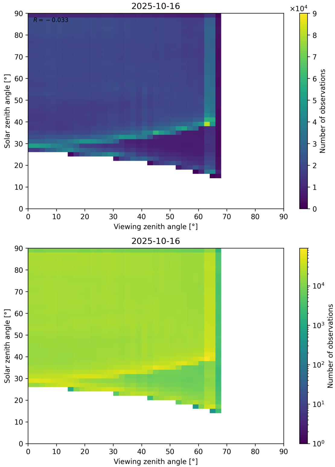
Figure 114: Scatter density plot of “Viewing zenith angle” against “Solar zenith angle” for 2025-10-15 to 2025-10-17.
