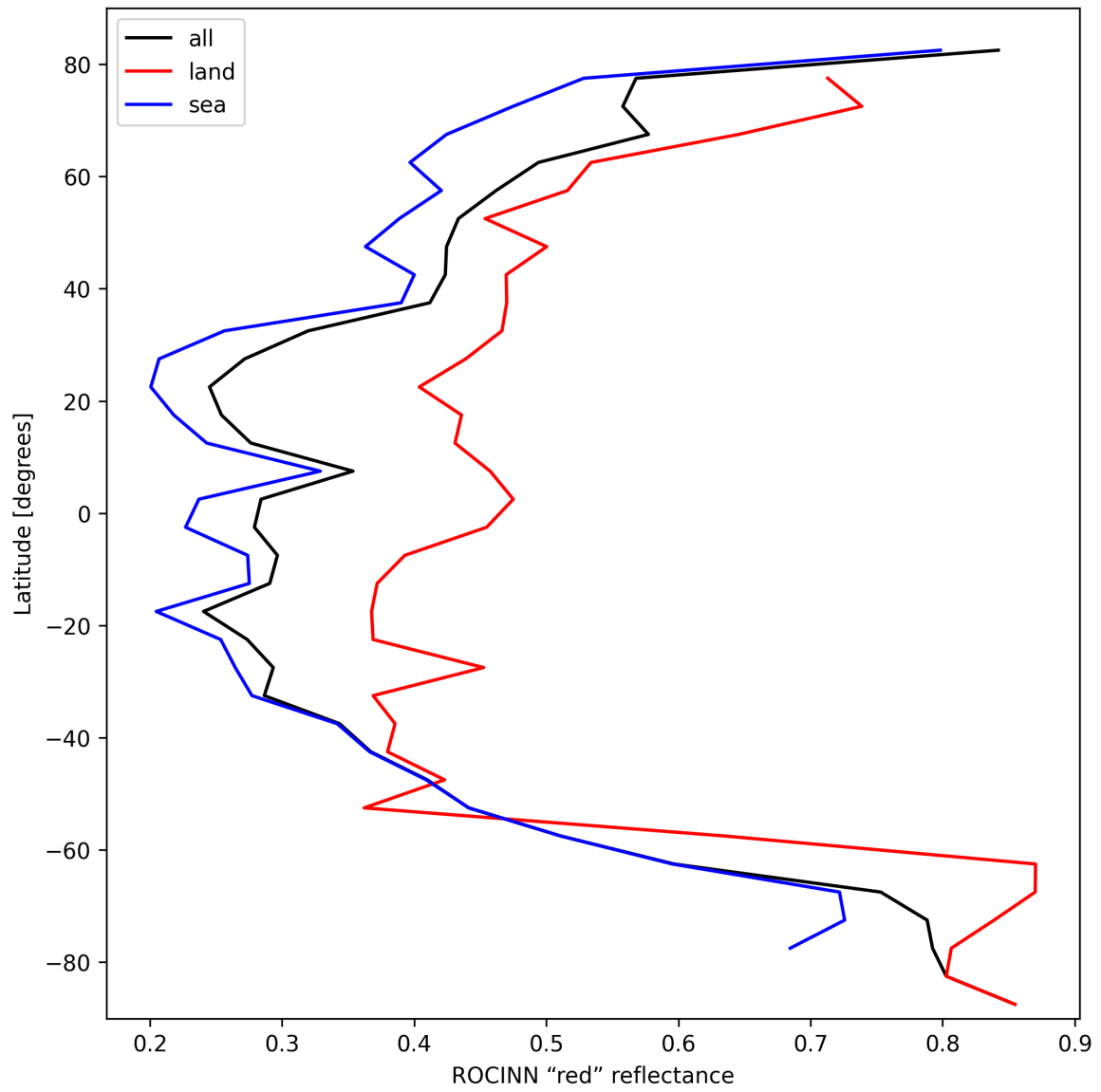
Figure 37: Zonal average of “ROCINN “red” reflectance” for 2025-10-15 to 2025-10-17.
