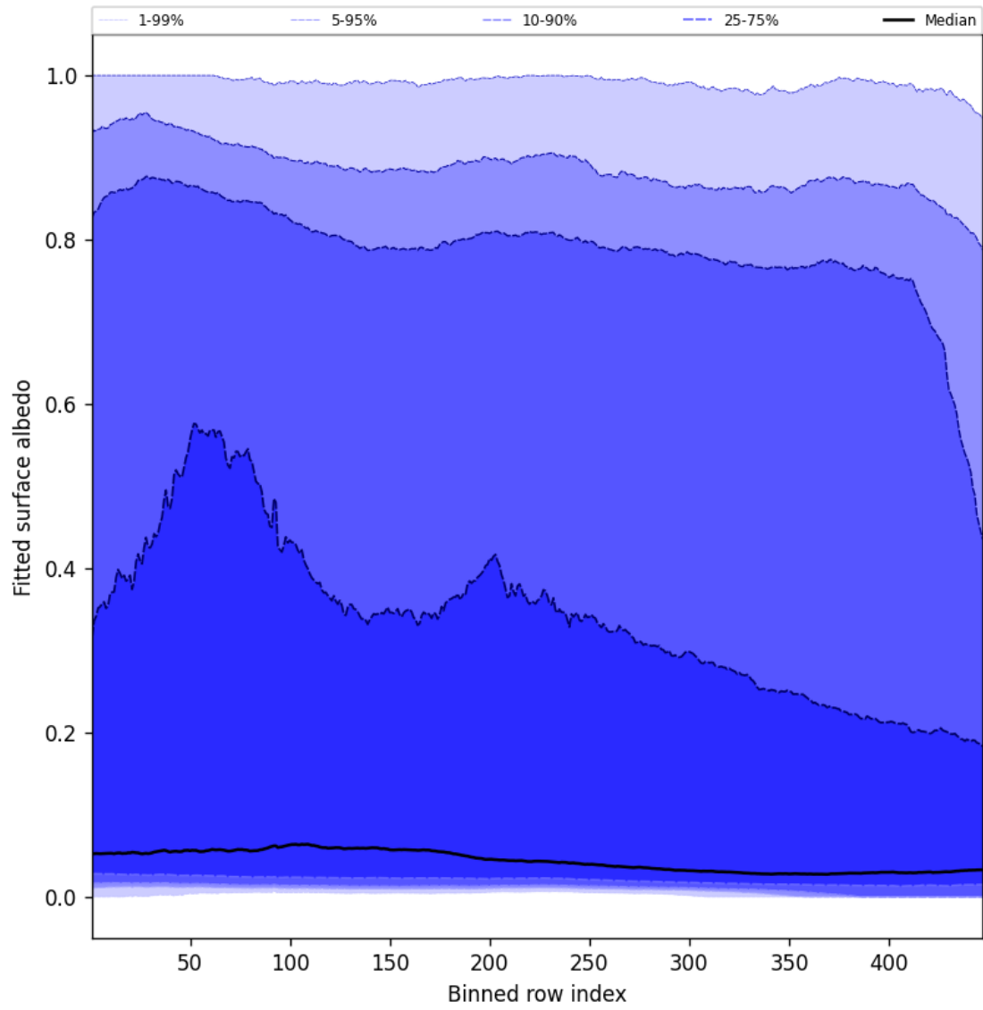
Figure 61: Along track statistics of “Fitted surface albedo” for 2025-10-15 to 2025-10-17
