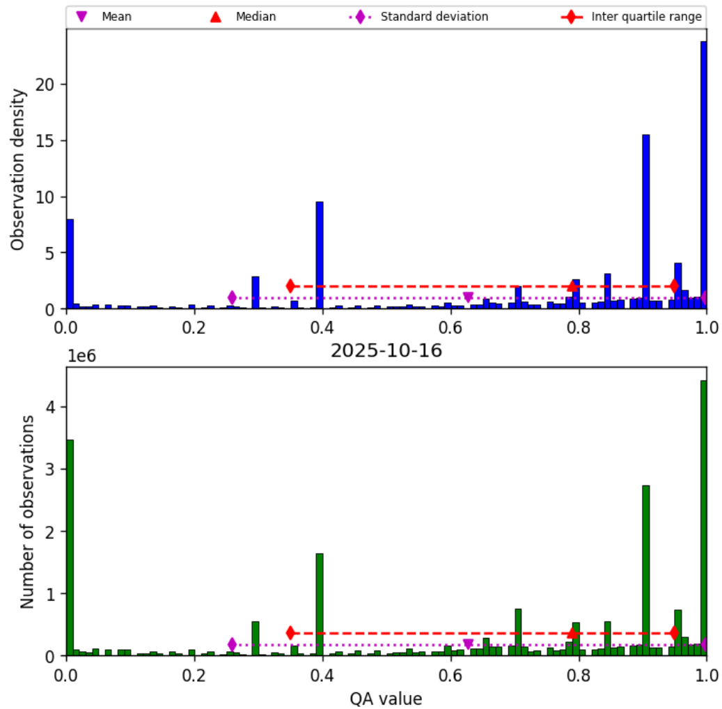
Figure 38: Histogram of “QA value” for 2025-10-15 to 2025-10-17
