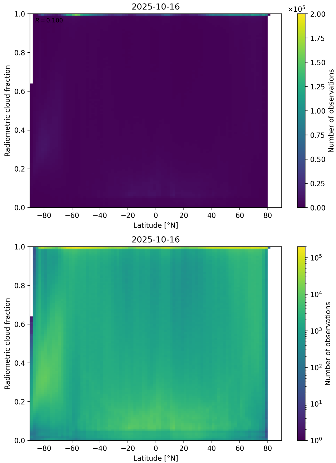
Figure 92: Scatter density plot of “Latitude” against “Radiometric cloud fraction” for 2025-10-15 to 2025-10-17.
