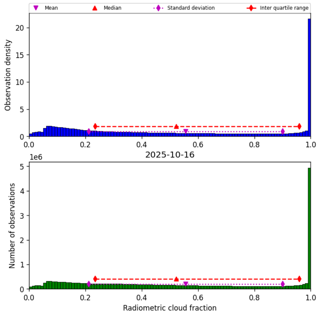
Figure 39: Histogram of “Radiometric cloud fraction” for 2025-10-15 to 2025-10-17
