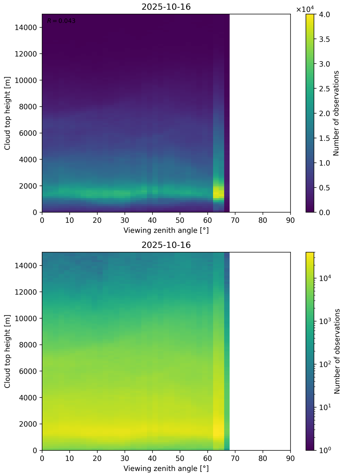
Figure 112: Scatter density plot of “Viewing zenith angle” against “Cloud top height” for 2025-10-15 to 2025-10-17.
