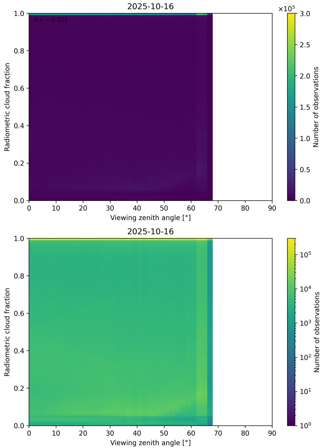
Figure 107: Scatter density plot of “Viewing zenith angle” against “Radiometric cloud fraction” for 2025-10-15 to 2025-10-17.
