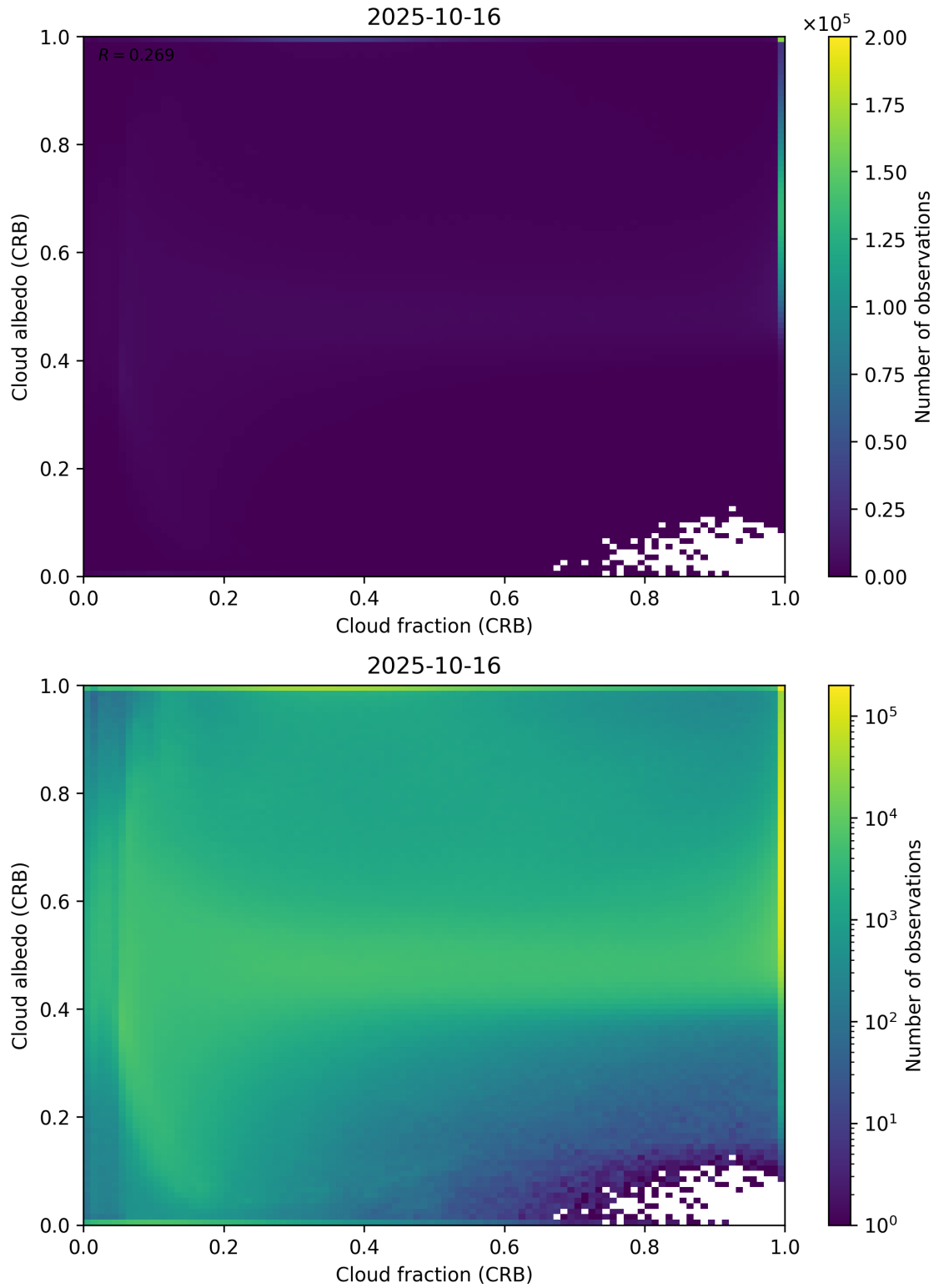
Figure 77: Scatter density plot of “Cloud fraction (CRB)” against “Cloud albedo (CRB)” for 2025-10-15 to 2025-10-17.
