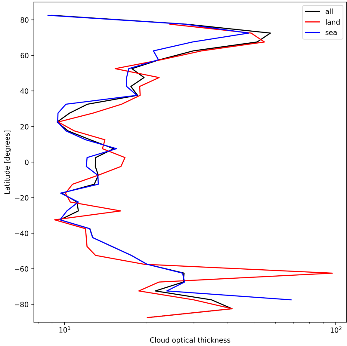
Figure 25: Zonal average of “Cloud optical thickness” for 2025-10-15 to 2025-10-17.
