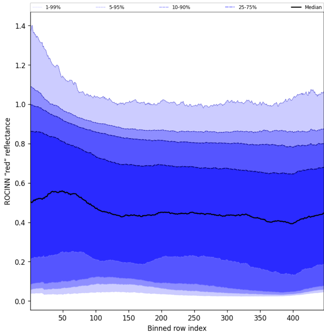
Figure 69: Along track statistics of "ROCINN "red" reflectance" for 2025-10-15 to 2025-10-17
