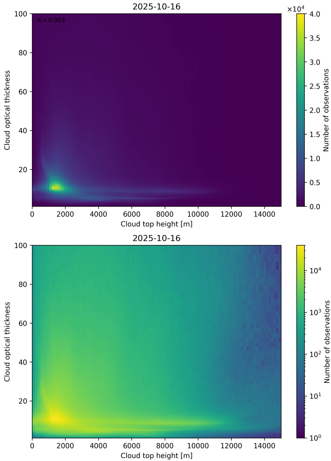
Figure 90: Scatter density plot of “Cloud top height” against “Cloud optical thickness” for 2025-10-15 to 2025-10-17.
