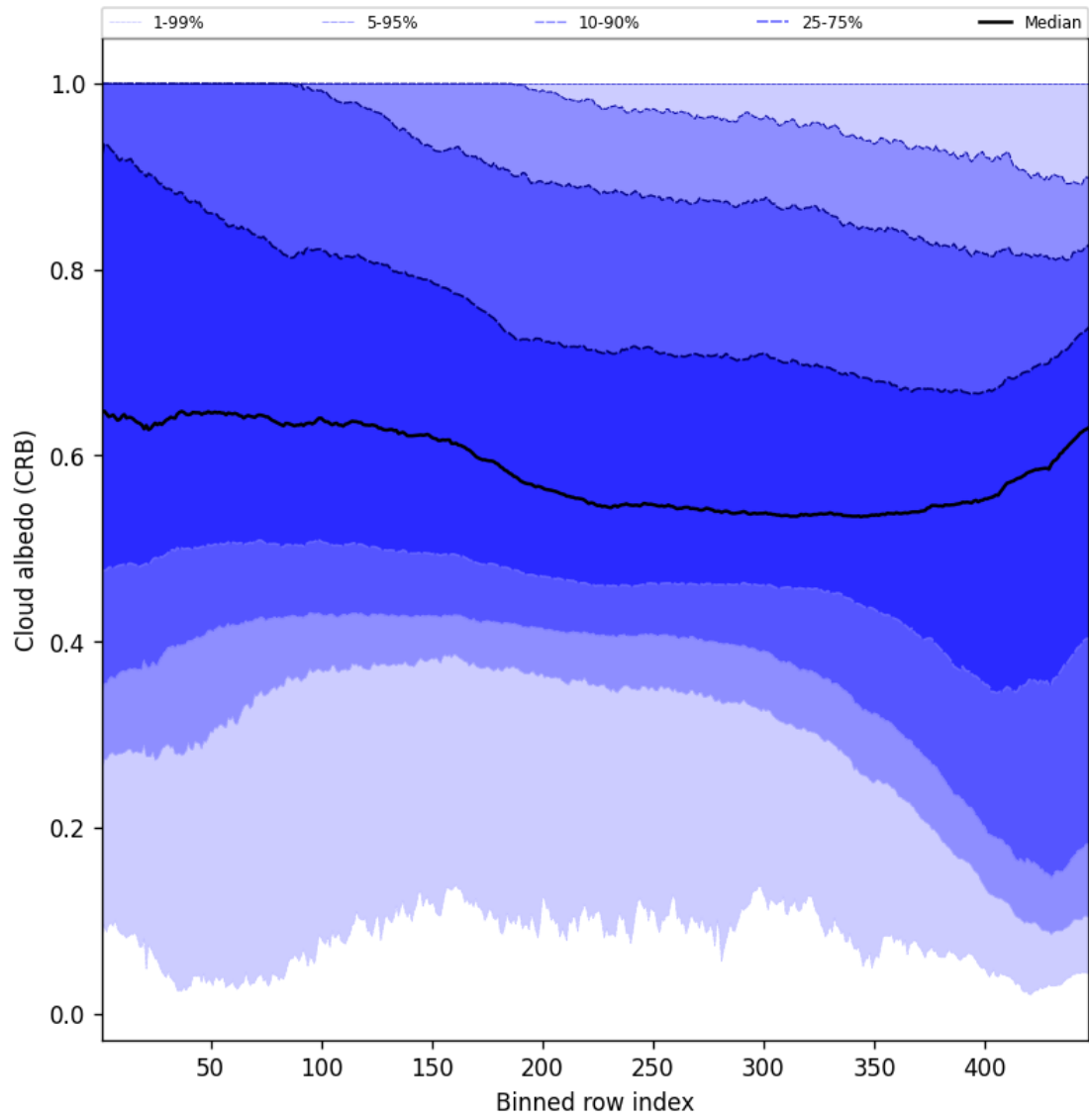
Figure 60: Along track statistics of “Cloud albedo (CRB)” for 2025-10-15 to 2025-10-17
