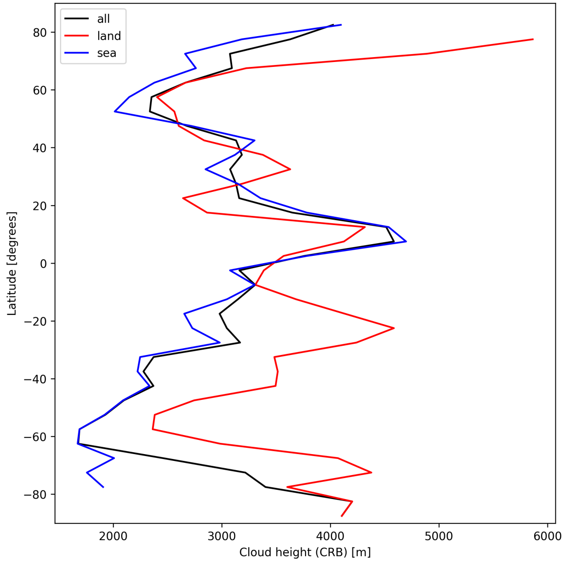
Figure 27: Zonal average of “Cloud height (CRB)” for 2025-10-15 to 2025-10-17.
