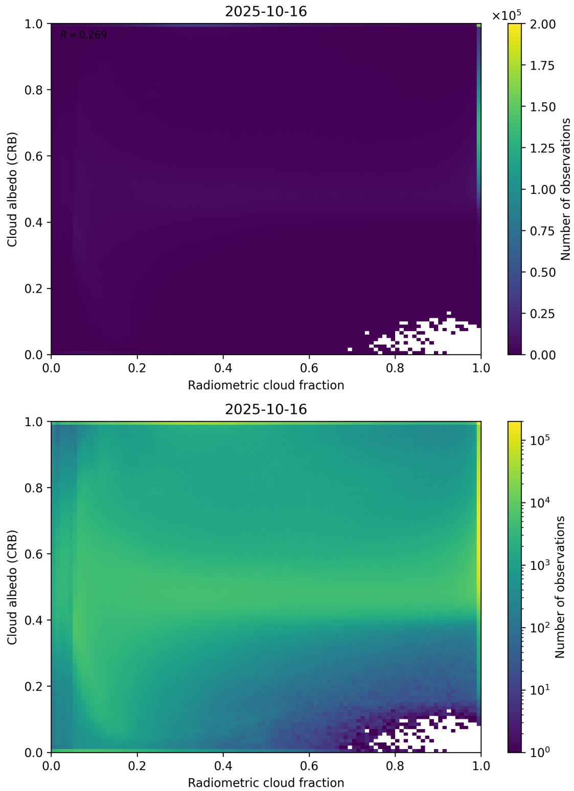
Figure 71: Scatter density plot of “Radiometric cloud fraction” against “Cloud albedo (CRB)” for 2025-10-15 to 2025-10-17.
