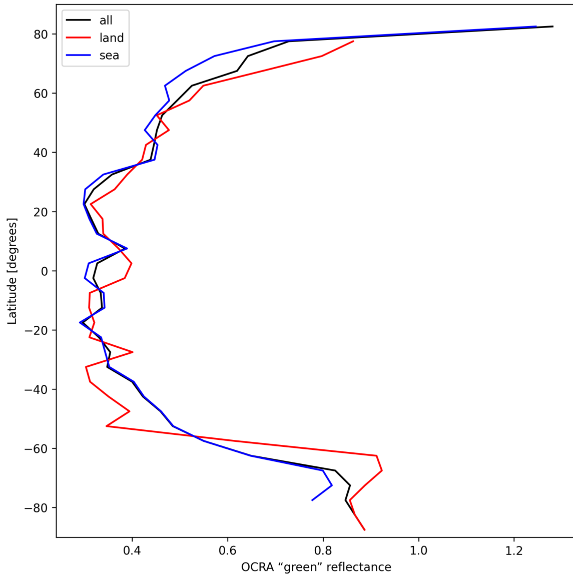
Figure 36: Zonal average of “OCRA “green” reflectance” for 2025-10-15 to 2025-10-17.
