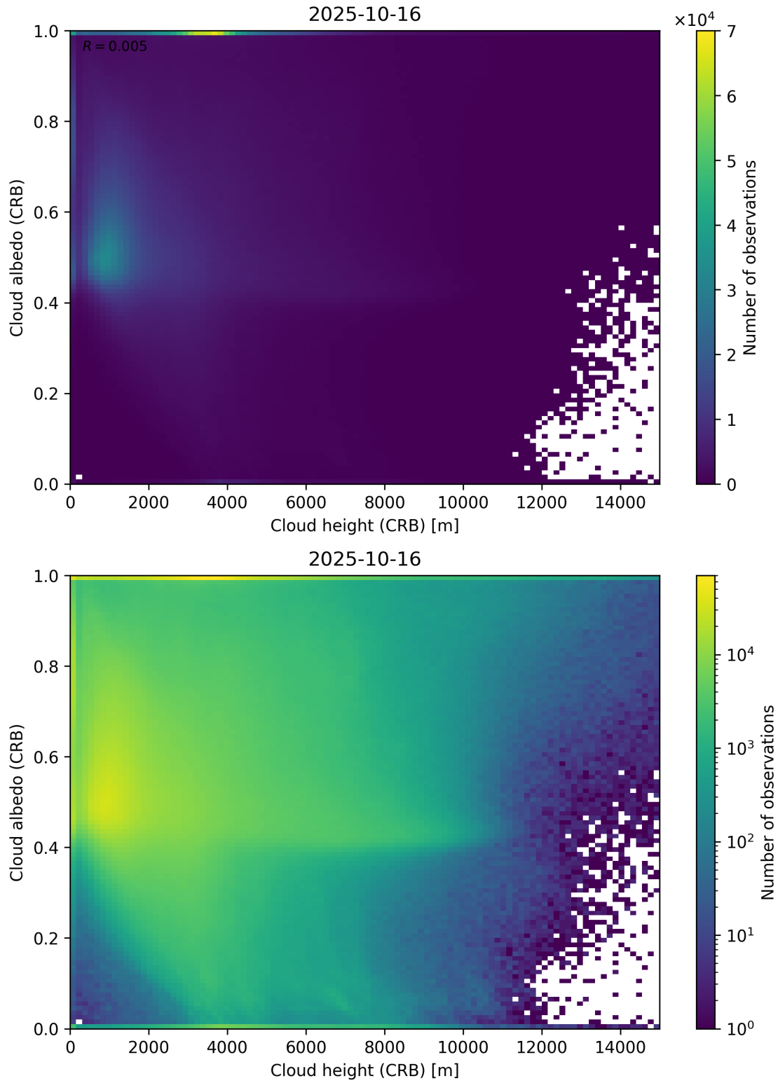
Figure 80: Scatter density plot of “Cloud height (CRB)” against “Cloud albedo (CRB)” for 2025-10-15 to 2025-10-17.
