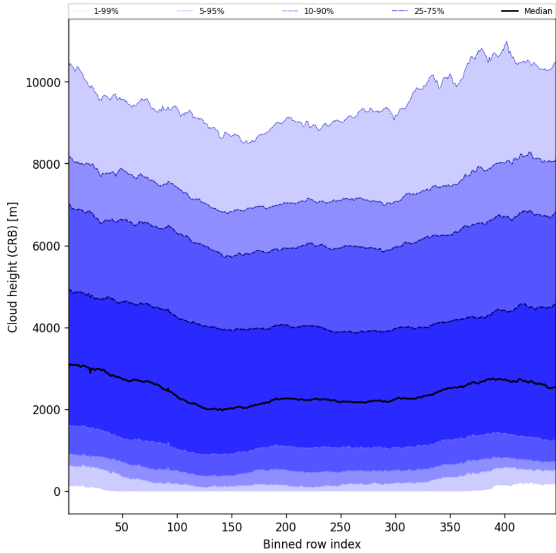
Figure 59: Along track statistics of “Cloud height (CRB)” for 2025-10-15 to 2025-10-17
