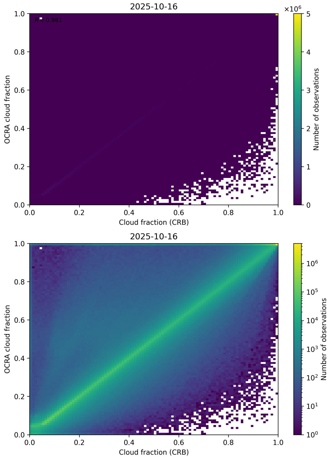
Figure 78: Scatter density plot of “Cloud fraction (CRB)” against “OCRA cloud fraction” for 2025-10-15 to 2025-10-17.
