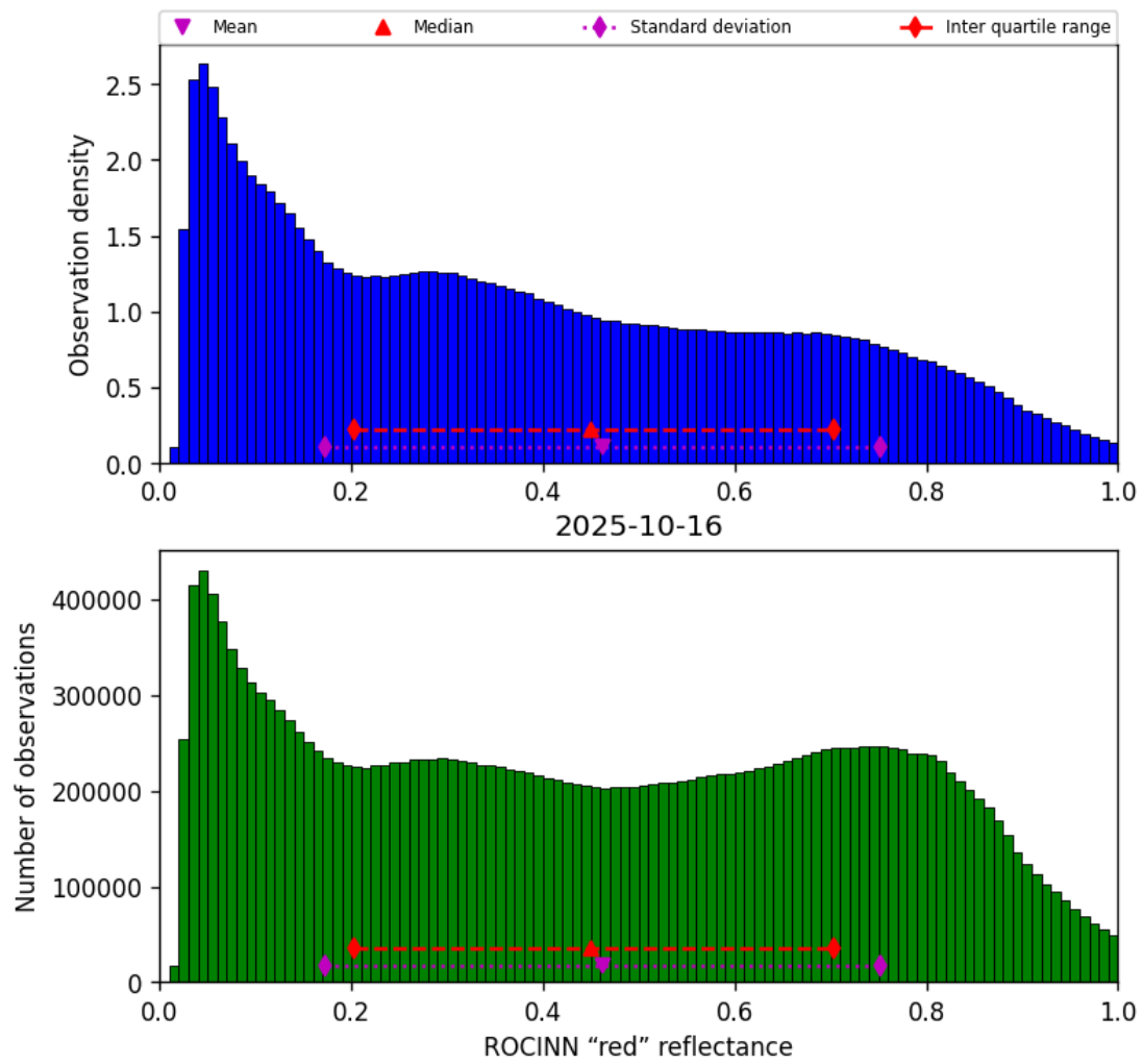
Figure 53: Histogram of “ROCINN “red” reflectance” for 2025-10-15 to 2025-10-17
