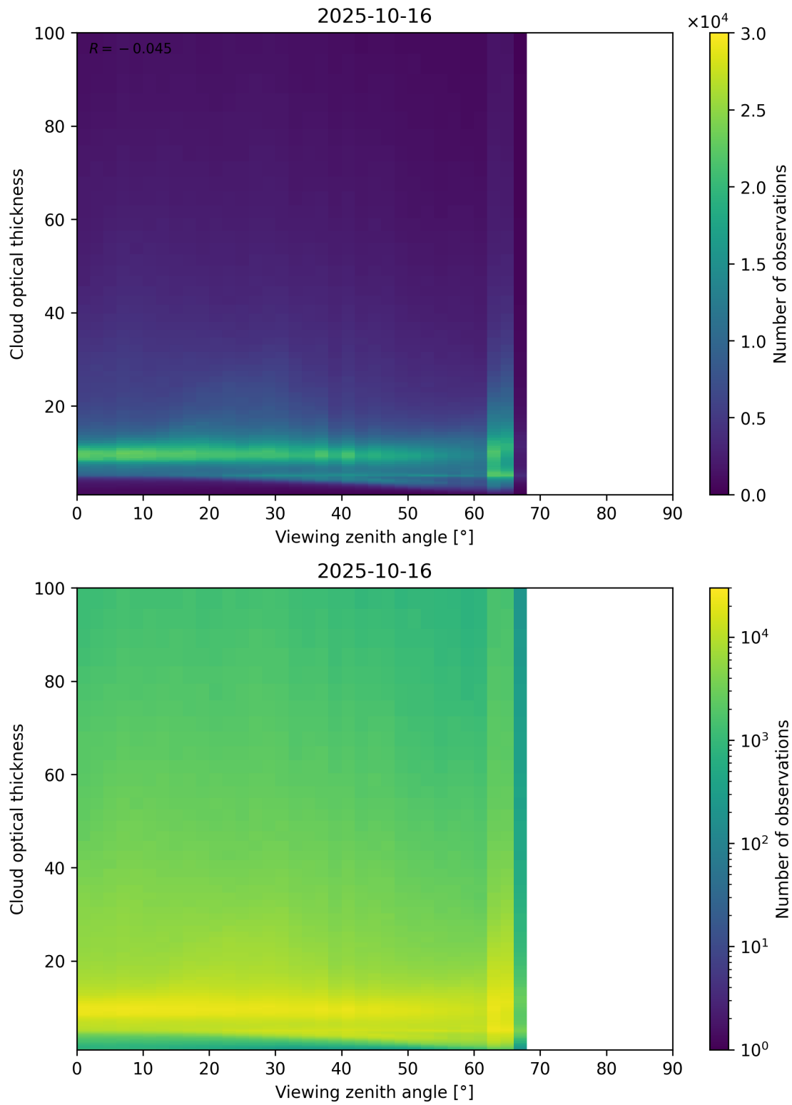
Figure 111: Scatter density plot of “Viewing zenith angle” against “Cloud optical thickness” for 2025-10-15 to 2025-10-17.
