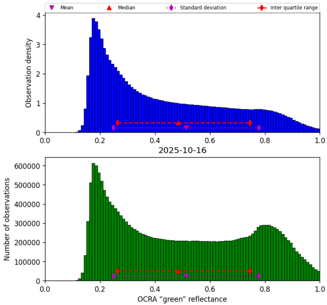
Figure 52: Histogram of “OCRA “green” reflectance” for 2025-10-15 to 2025-10-17
