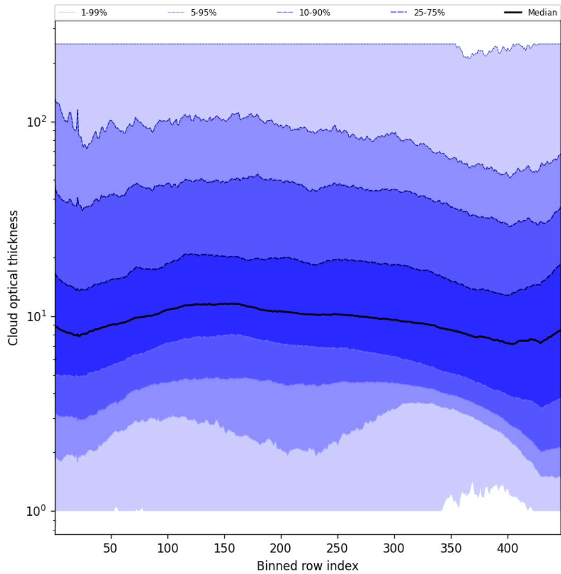
Figure 57: Along track statistics of “Cloud optical thickness” for 2025-10-15 to 2025-10-17
