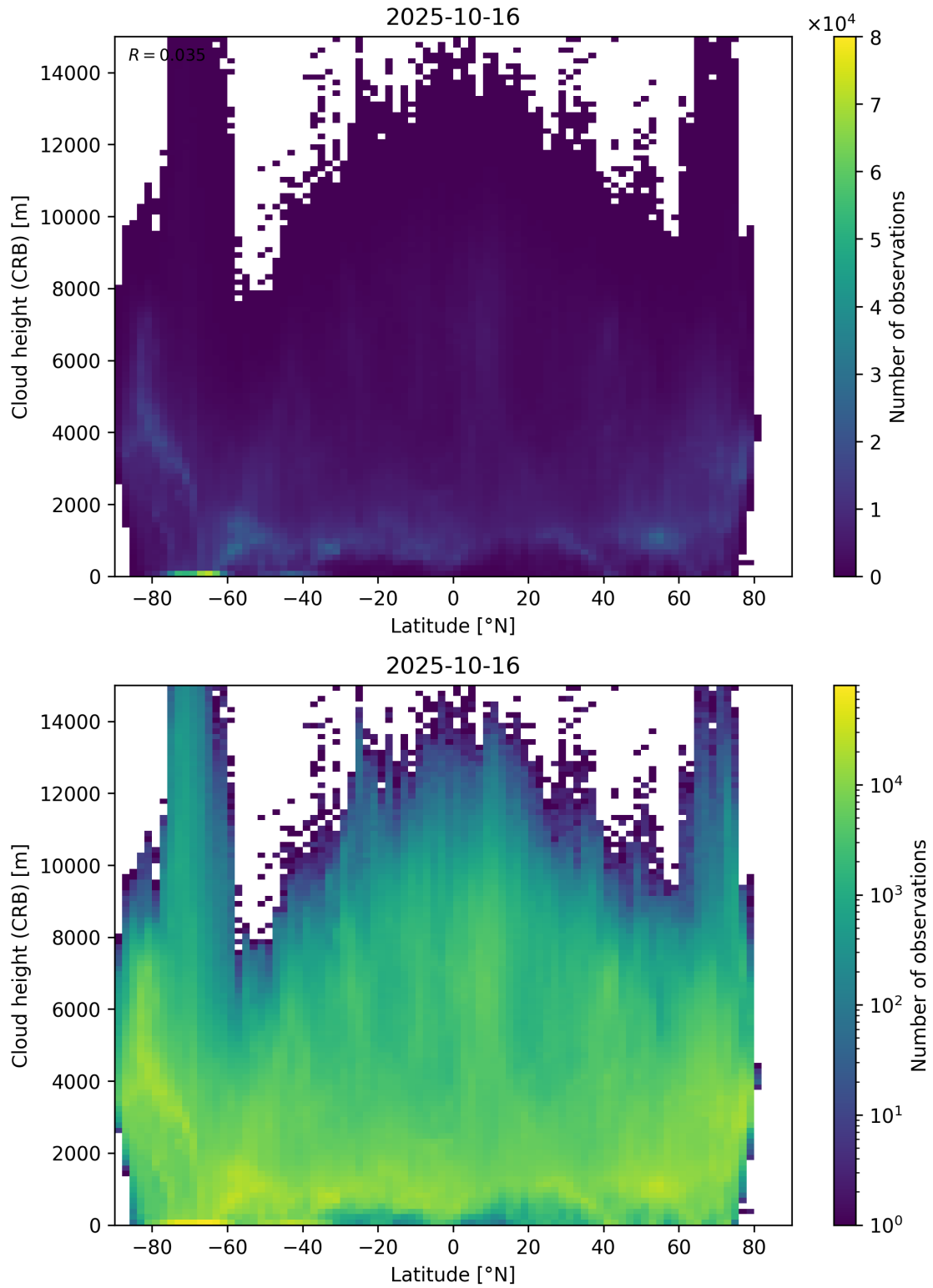
Figure 95: Scatter density plot of “Latitude” against “Cloud height (CRB)” for 2025-10-15 to 2025-10-17.
