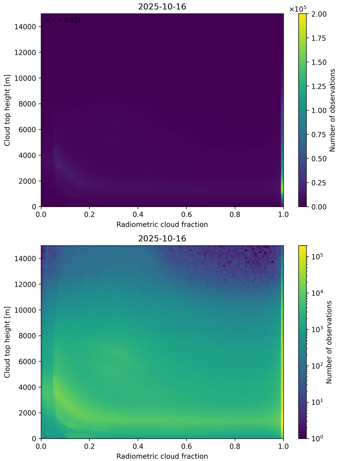
Figure 76: Scatter density plot of “Radiometric cloud fraction” against “Cloud top height” for 2025-10-15 to 2025-10-17.
