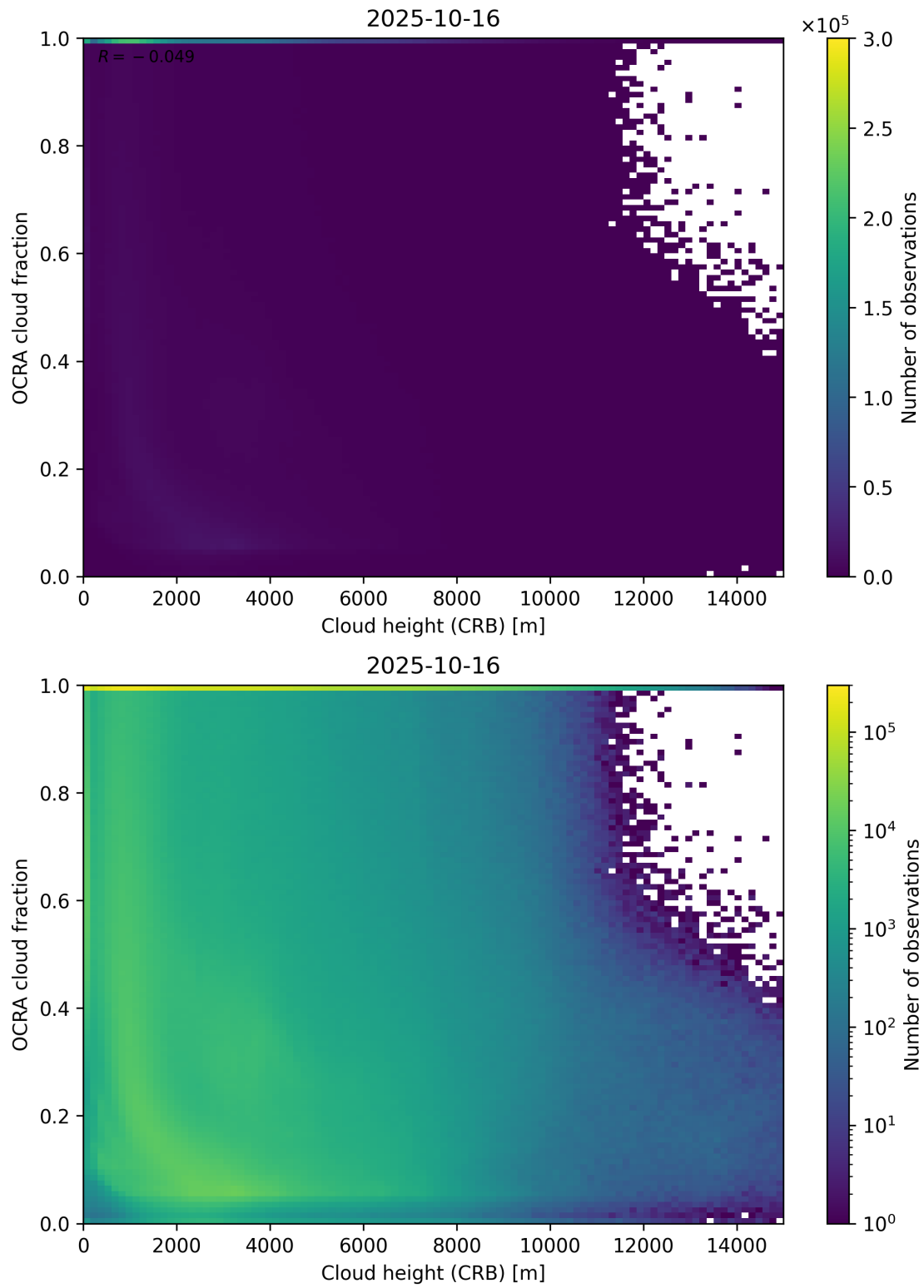
Figure 81: Scatter density plot of “Cloud height (CRB)” against “OCRA cloud fraction” for 2025-10-15 to 2025-10-17.
