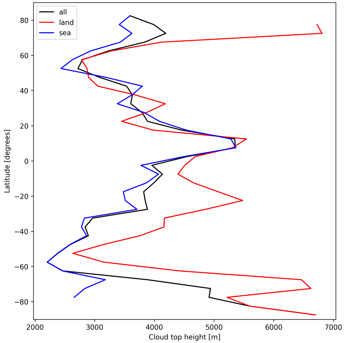
Figure 24: Zonal average of “Cloud top height” for 2025-10-15 to 2025-10-17.
