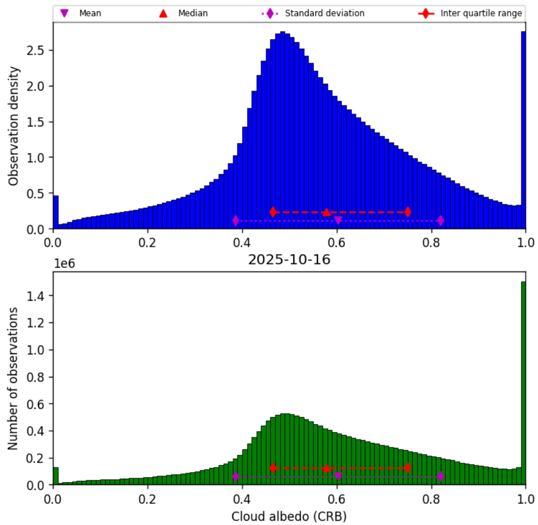
Figure 44: Histogram of “Cloud albedo (CRB)” for 2025-10-15 to 2025-10-17
