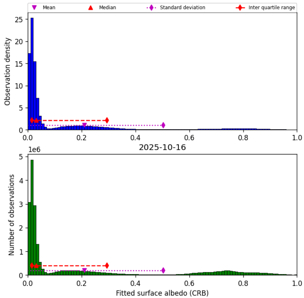
Figure 46: Histogram of “Fitted surface albedo (CRB)” for 2025-10-15 to 2025-10-17
