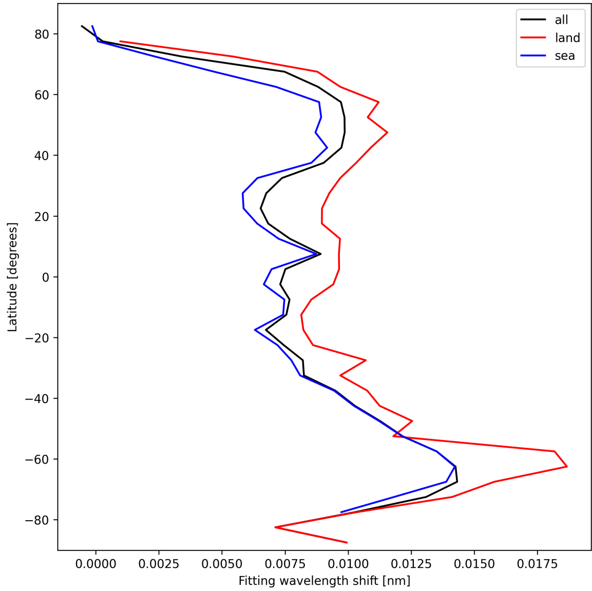
Figure 33: Zonal average of “Fitting wavelength shift” for 2025-10-15 to 2025-10-17.
