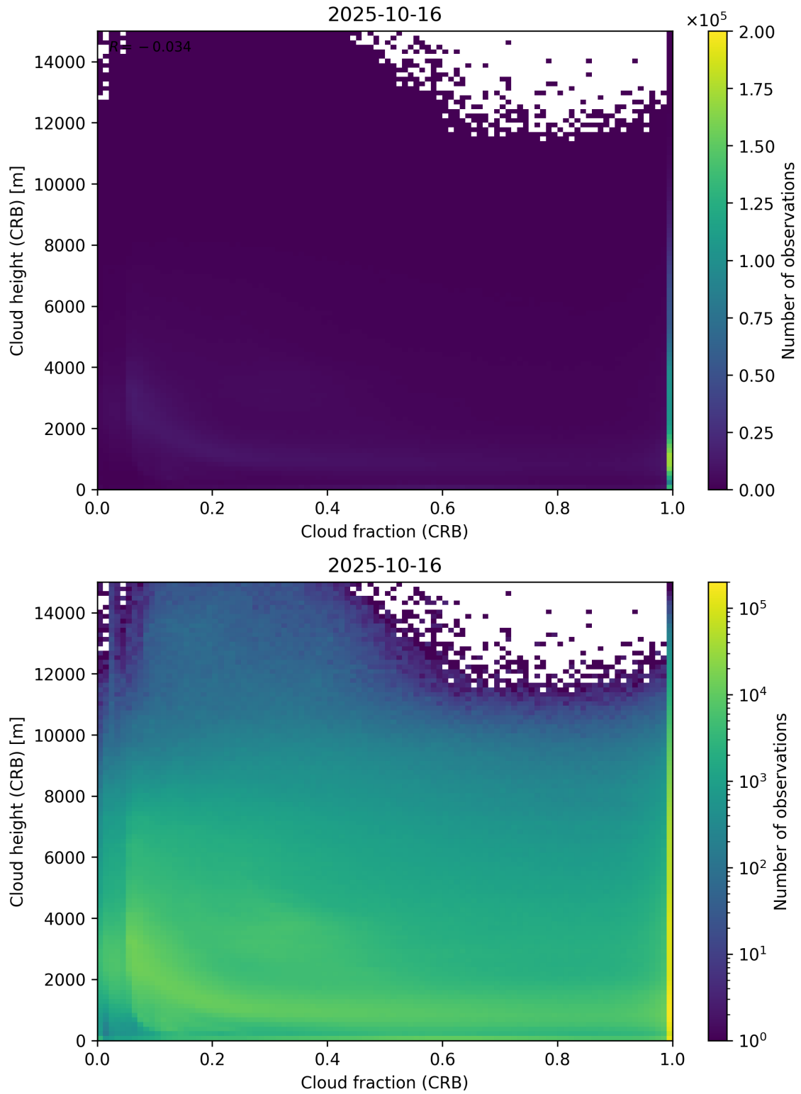
Figure 79: Scatter density plot of “Cloud fraction (CRB)” against “Cloud height (CRB)” for 2025-10-15 to 2025-10-17.
