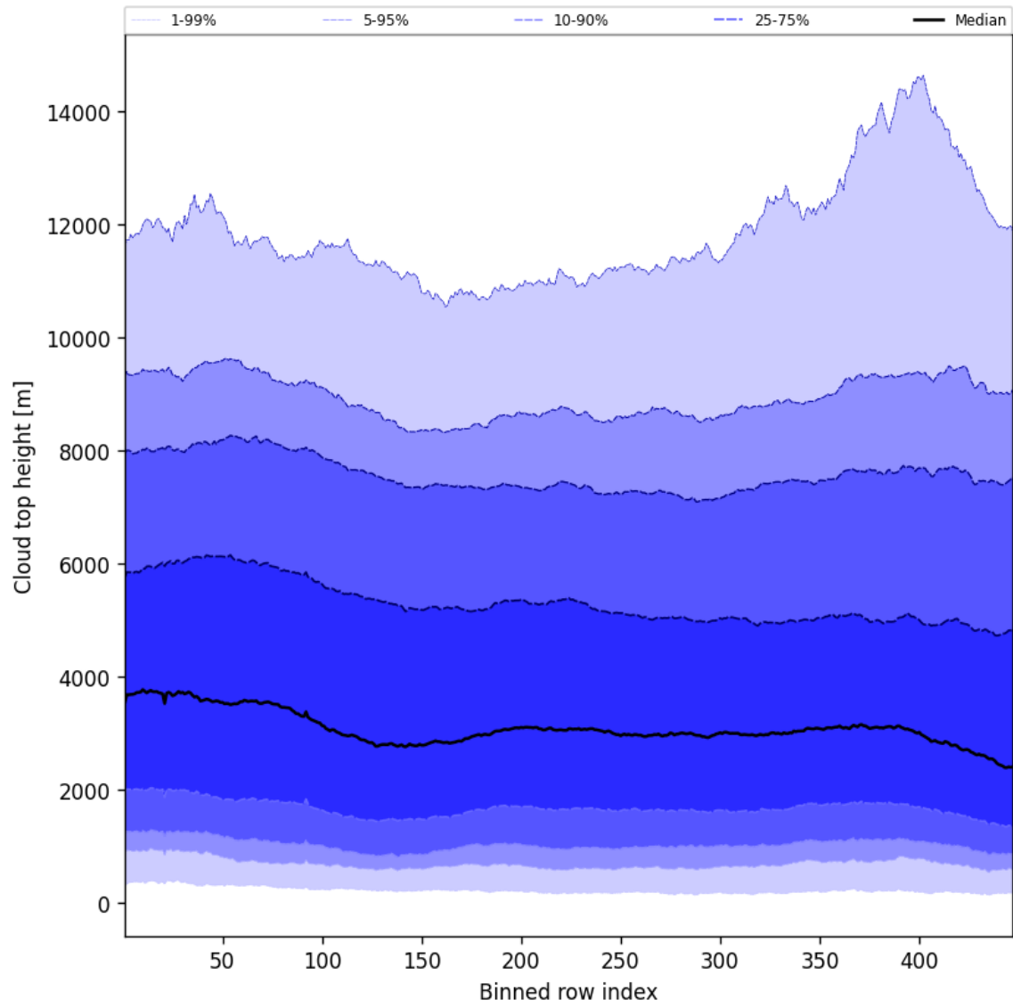
Figure 56: Along track statistics of “Cloud top height” for 2025-10-15 to 2025-10-17
