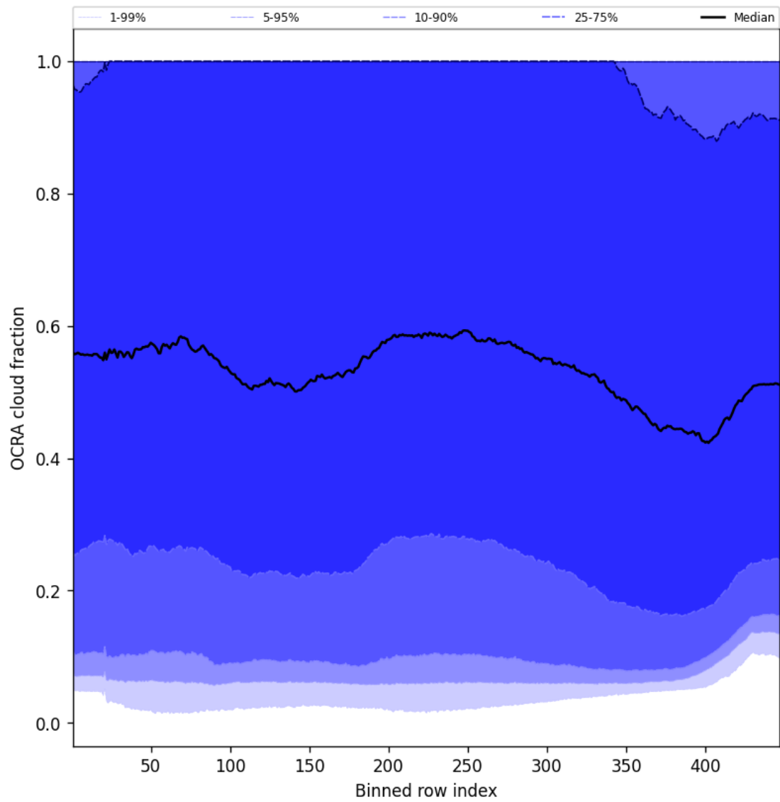
Figure 66: Along track statistics of “OCRA cloud fraction” for 2025-10-15 to 2025-10-17
