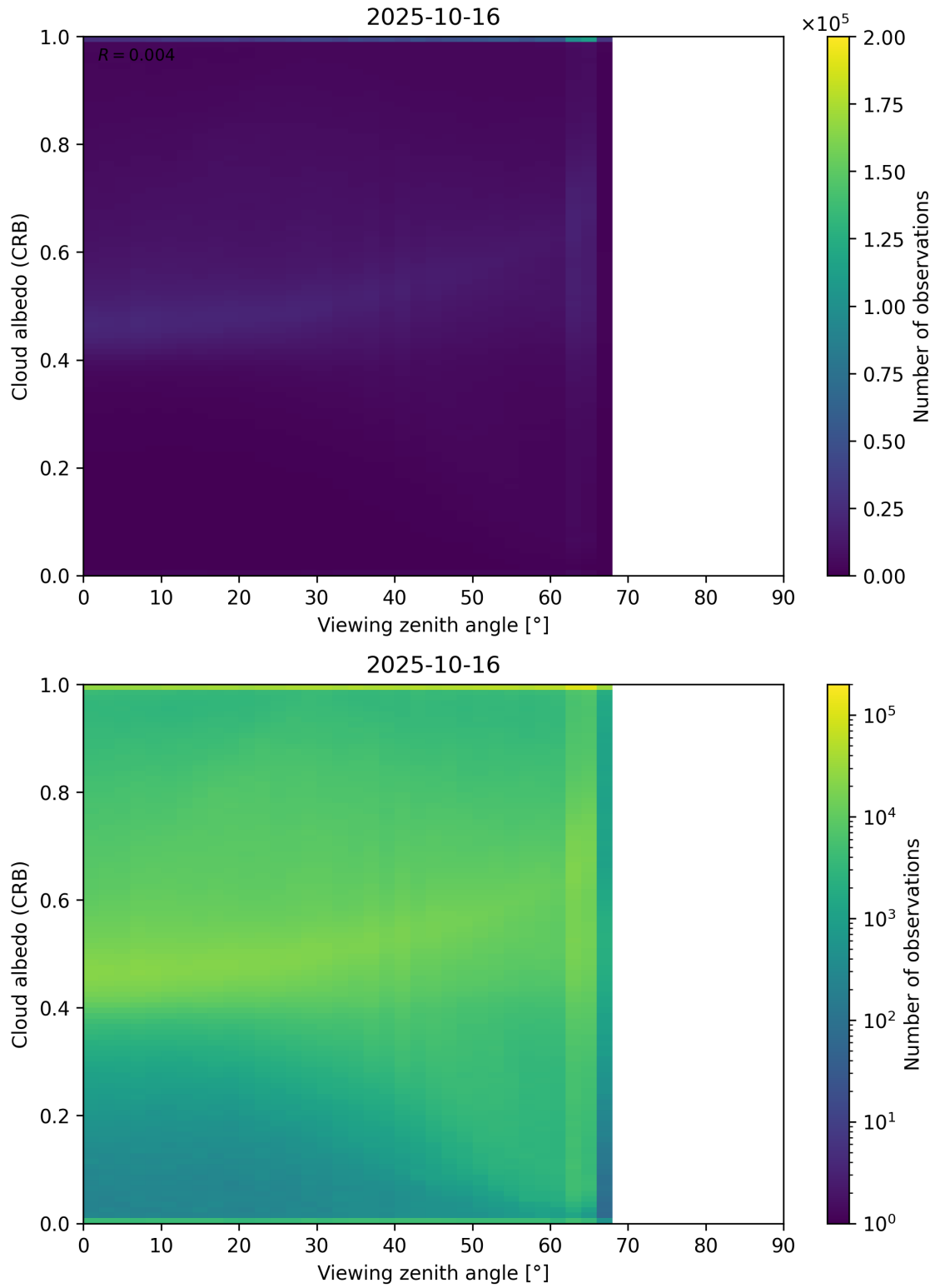
Figure 106: Scatter density plot of “Viewing zenith angle” against “Cloud albedo (CRB)” for 2025-10-15 to 2025-10-17.
