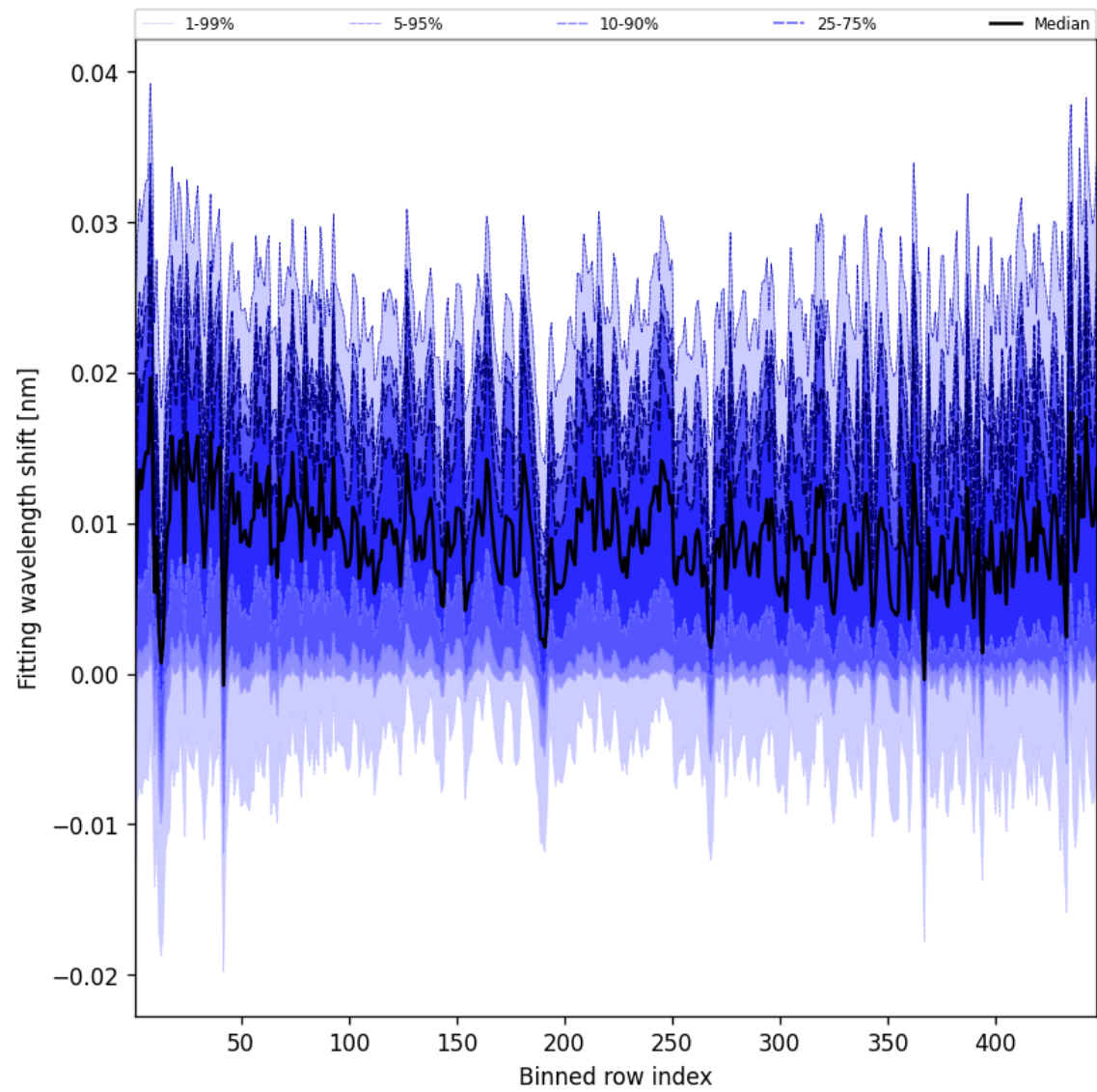
Figure 65: Along track statistics of “Fitting wavelength shift” for 2025-10-15 to 2025-10-17
