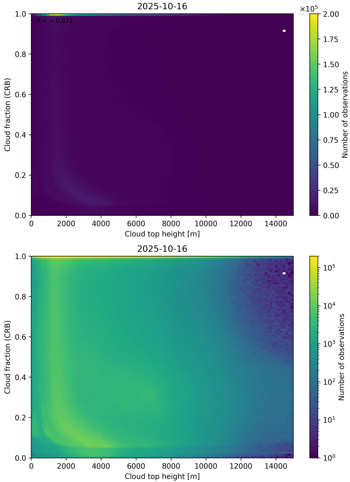
Figure 88: Scatter density plot of “Cloud top height” against “Cloud fraction (CRB)” for 2025-10-15 to 2025-10-17.
