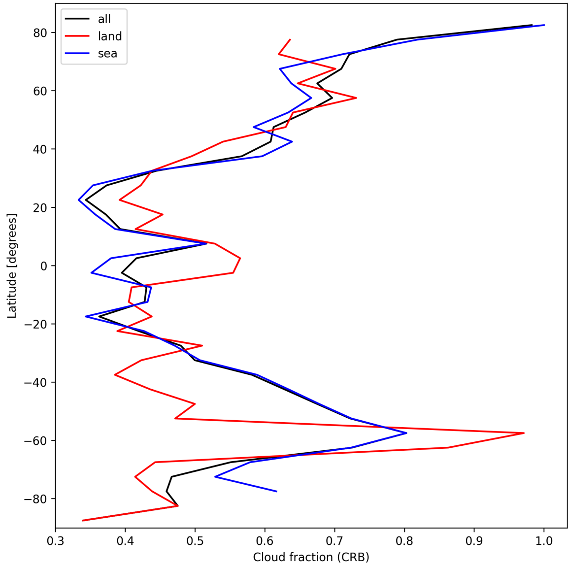
Figure 26: Zonal average of “Cloud fraction (CRB)” for 2025-10-15 to 2025-10-17.
