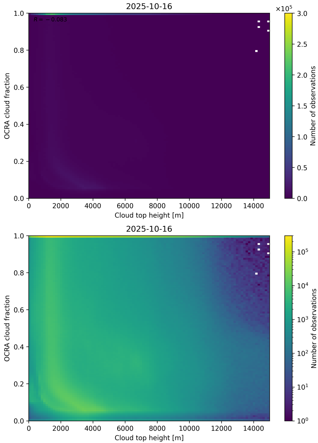
Figure 87: Scatter density plot of “Cloud top height” against “OCRA cloud fraction” for 2025-10-15 to 2025-10-17.
