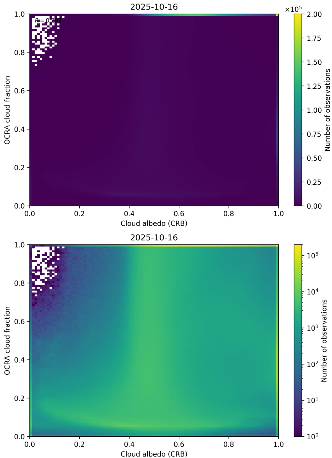
Figure 70: Scatter density plot of “Cloud albedo (CRB)” against “OCRA cloud fraction” for 2025-10-15 to 2025-10-17.
