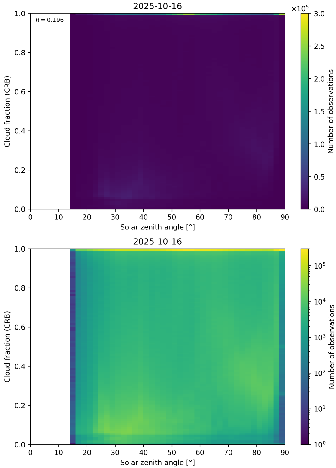
Figure 101: Scatter density plot of “Solar zenith angle” against “Cloud fraction (CRB)” for 2025-10-15 to 2025-10-17.
