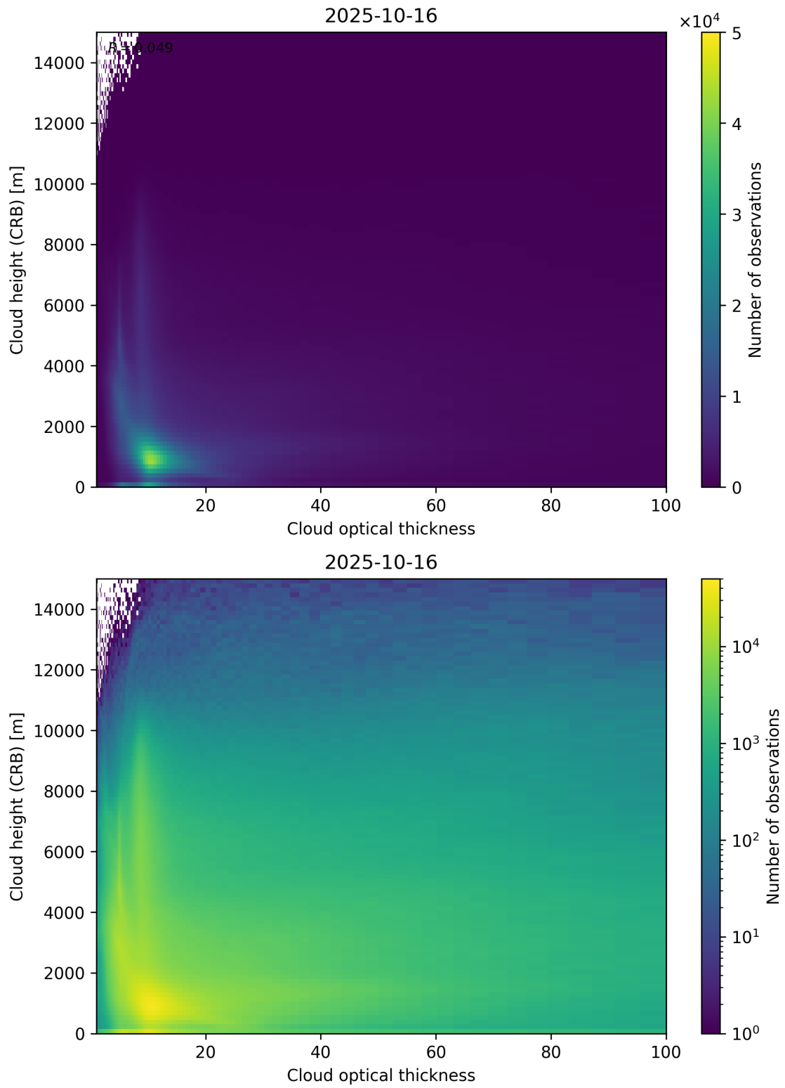
Figure 85: Scatter density plot of “Cloud optical thickness” against “Cloud height (CRB)” for 2025-10-15 to 2025-10-17.
