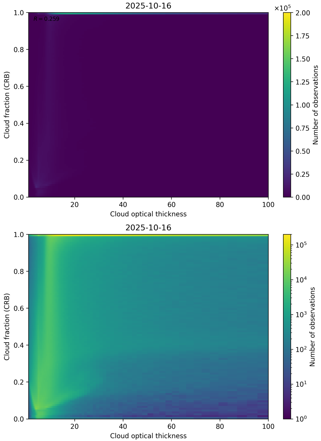
Figure 84: Scatter density plot of “Cloud optical thickness” against “Cloud fraction (CRB)” for 2025-10-15 to 2025-10-17.
