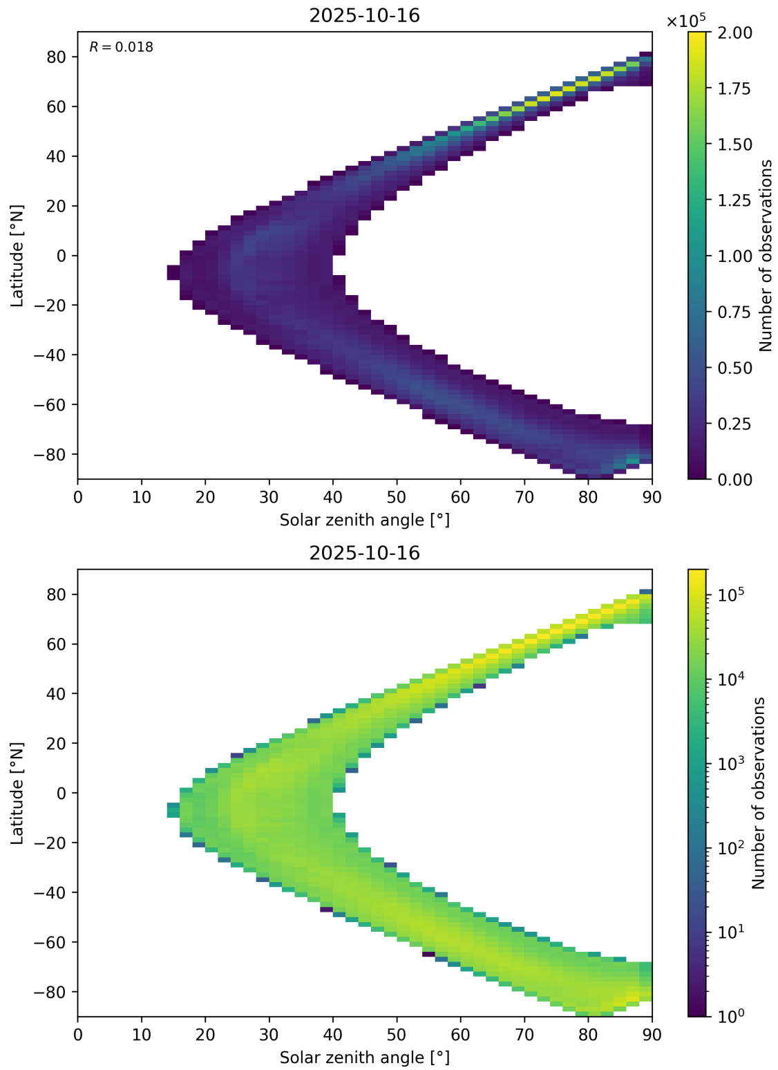
Figure 105: Scatter density plot of “Solar zenith angle” against “Latitude” for 2025-10-15 to 2025-10-17.
