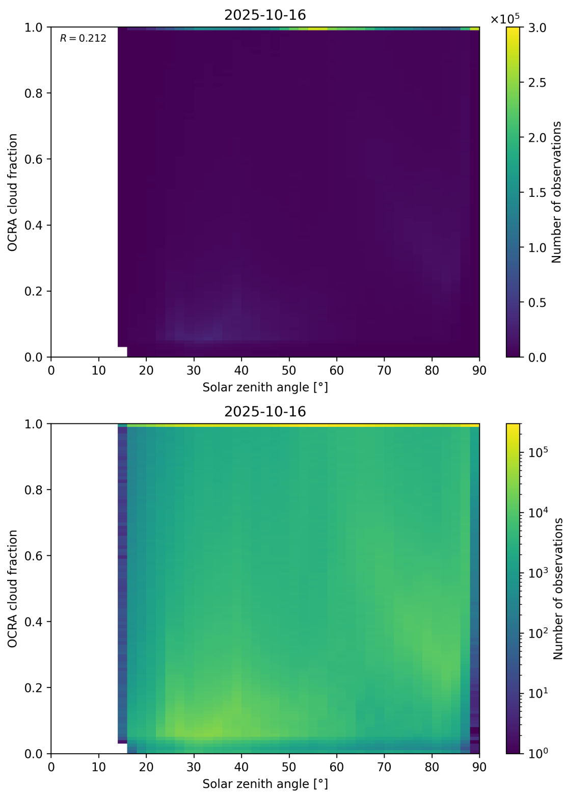
Figure 100: Scatter density plot of “Solar zenith angle” against “OCRA cloud fraction” for 2025-10-15 to 2025-10-17.
