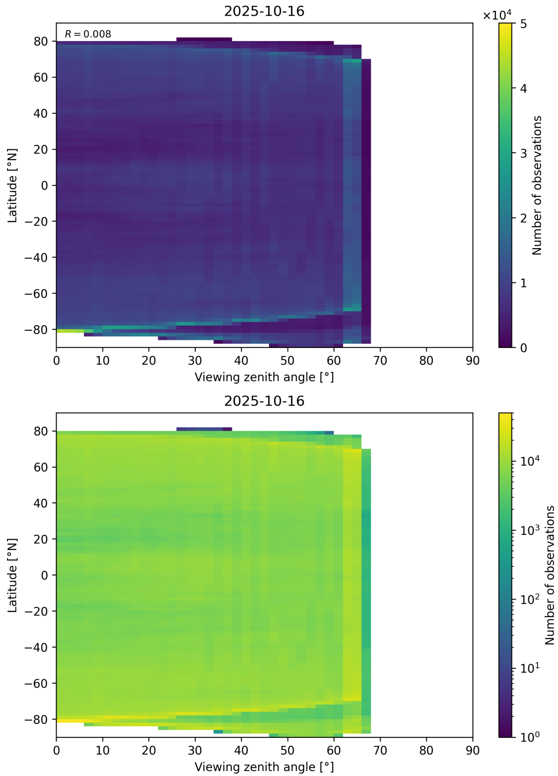
Figure 113: Scatter density plot of “Viewing zenith angle” against “Latitude” for 2025-10-15 to 2025-10-17.
