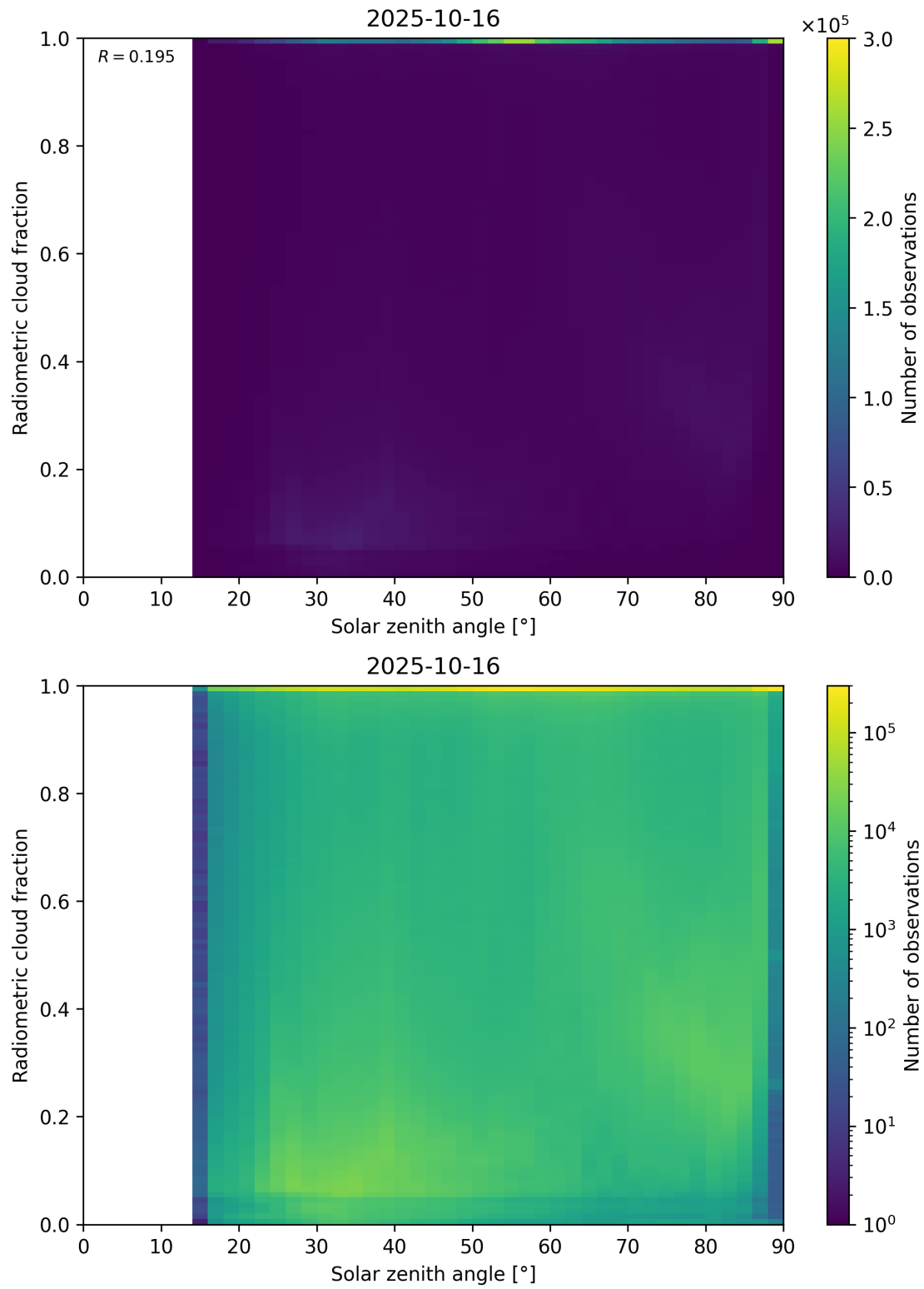
Figure 99: Scatter density plot of “Solar zenith angle” against “Radiometric cloud fraction” for 2025-10-15 to 2025-10-17.
