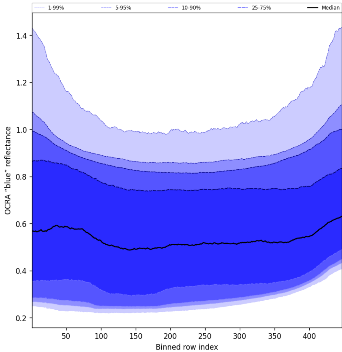
Figure 67: Along track statistics of “OCRA “blue” reflectance” for 2025-10-15 to 2025-10-17
