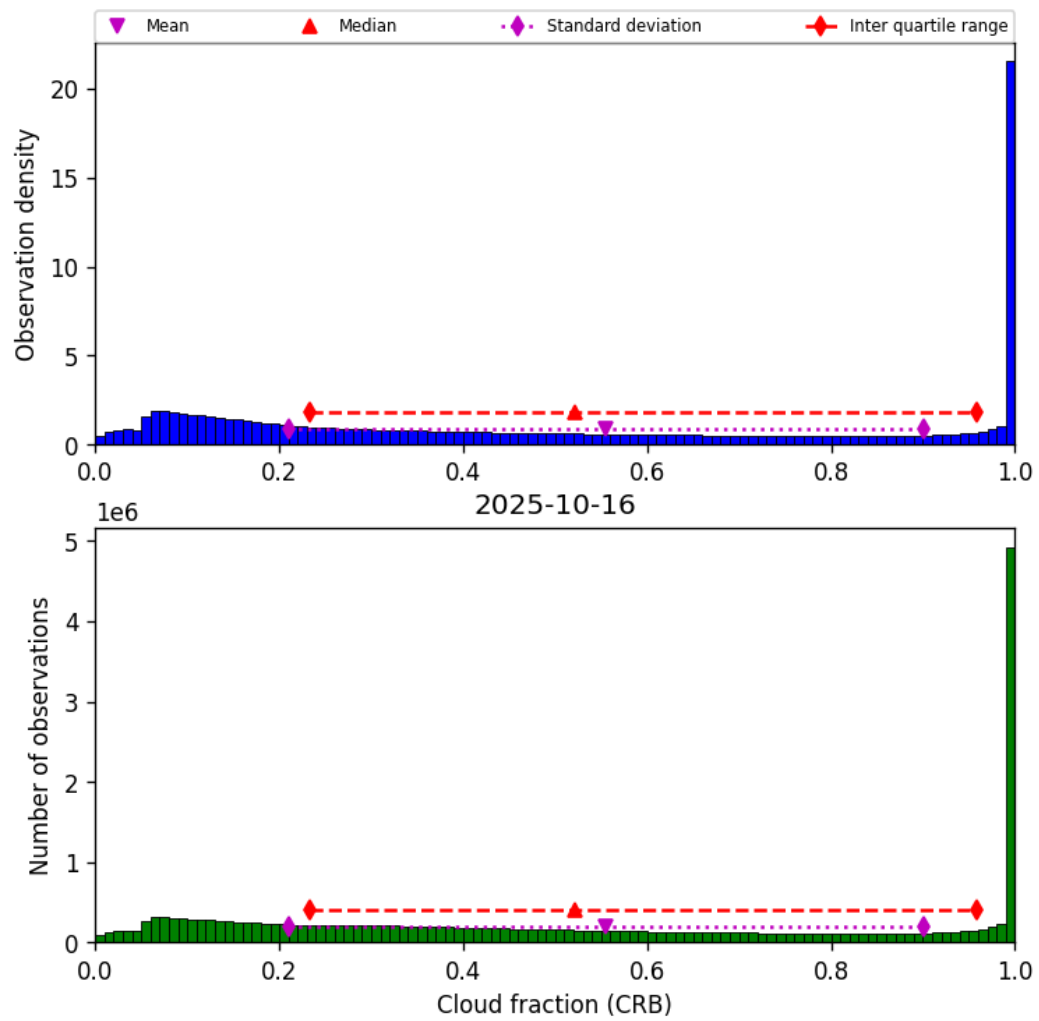
Figure 42: Histogram of “Cloud fraction (CRB)” for 2025-10-15 to 2025-10-17
