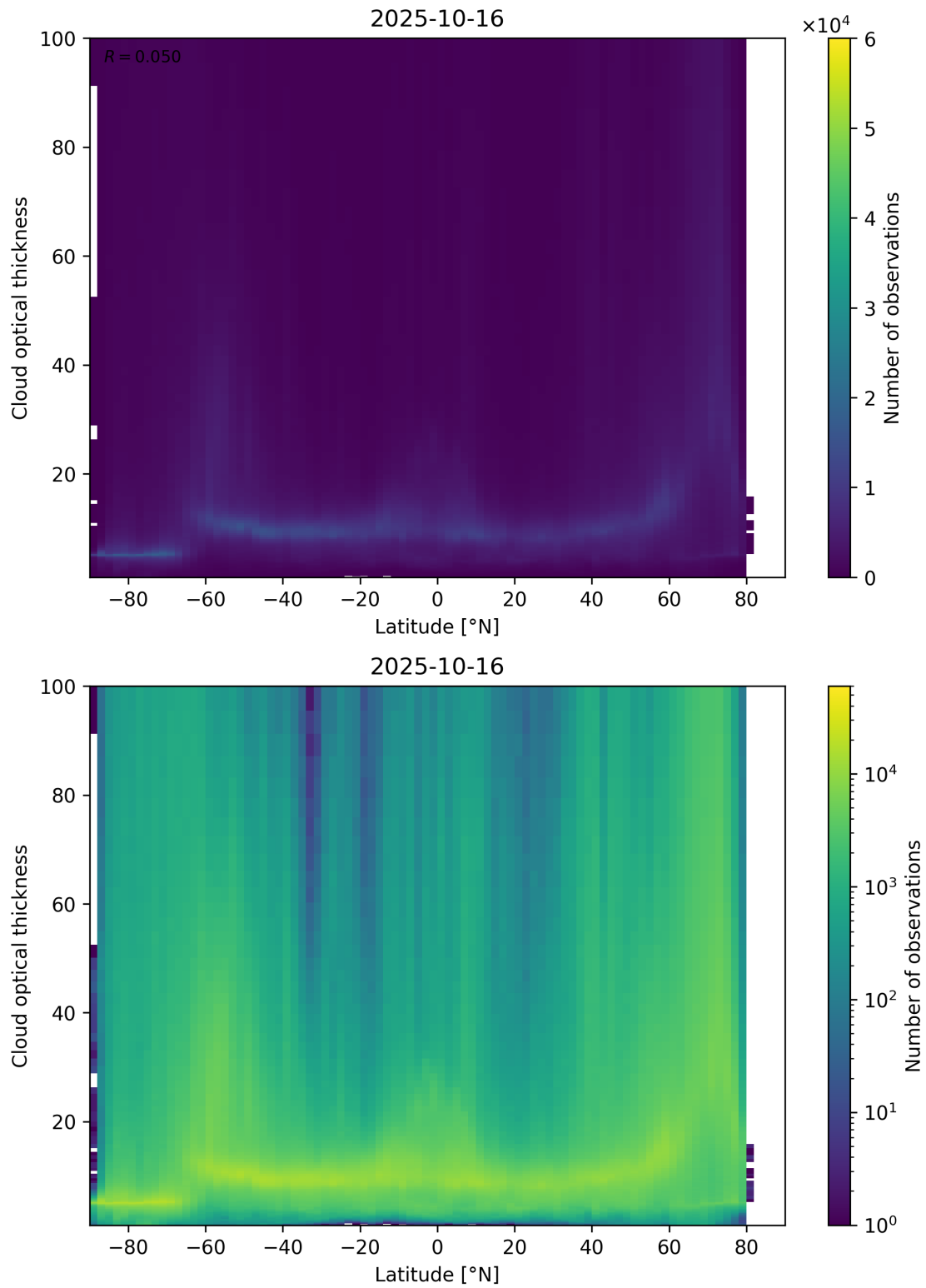
Figure 96: Scatter density plot of “Latitude” against “Cloud optical thickness” for 2025-10-15 to 2025-10-17.
