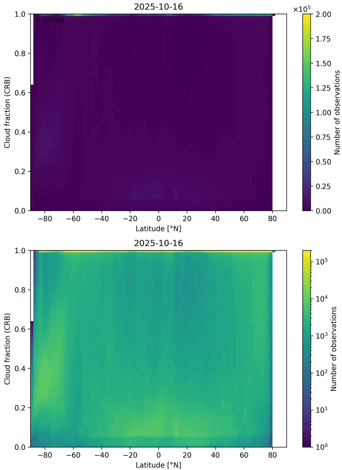
Figure 94: Scatter density plot of “Latitude” against “Cloud fraction (CRB)” for 2025-10-15 to 2025-10-17.
