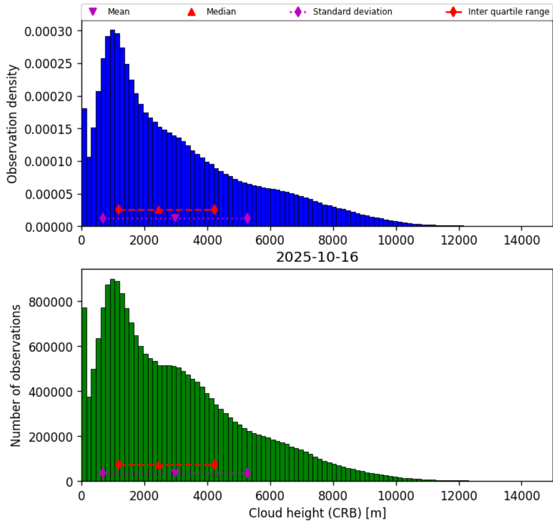
Figure 43: Histogram of “Cloud height (CRB)” for 2025-10-15 to 2025-10-17
