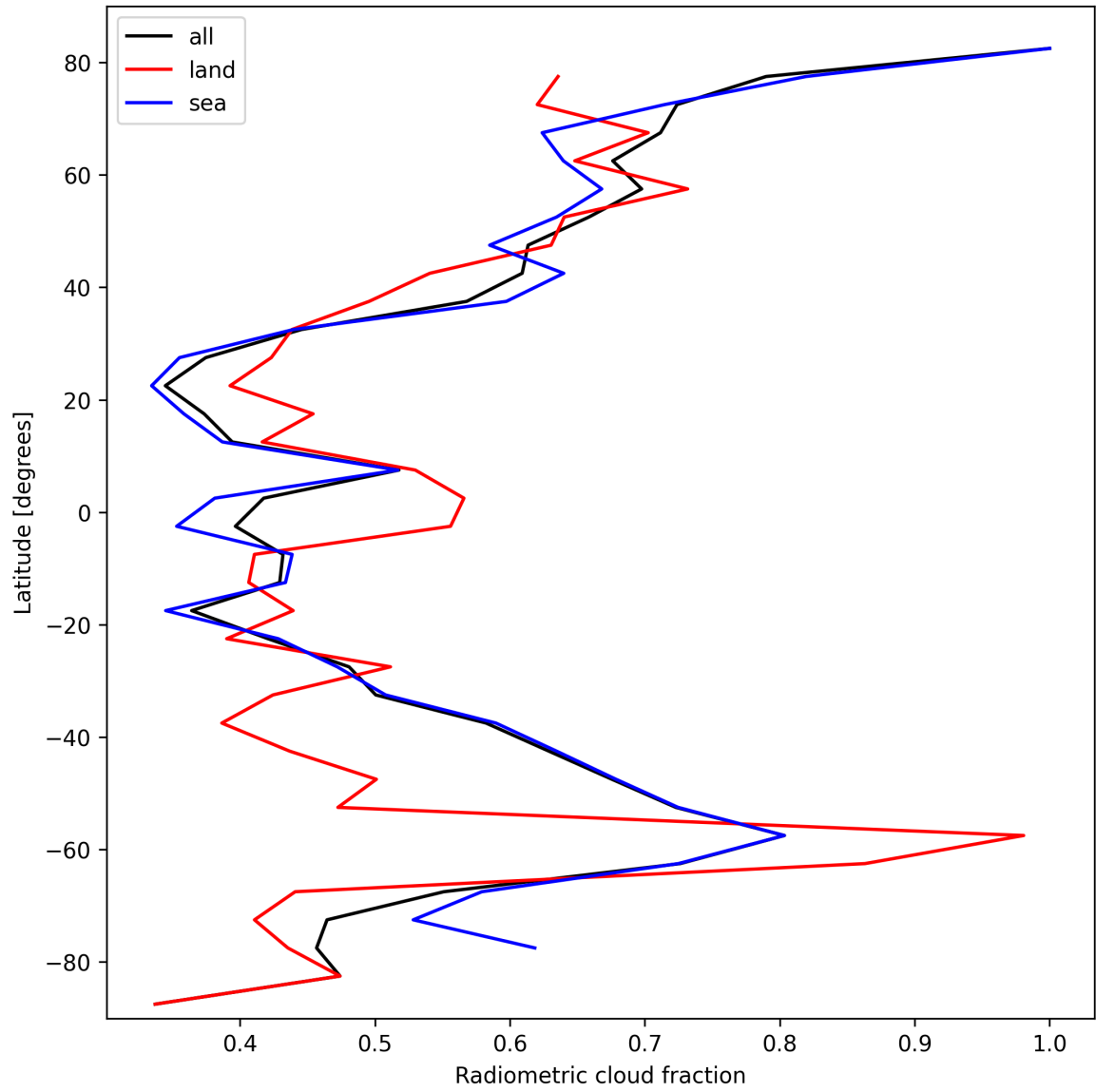
Figure 23: Zonal average of “Radiometric cloud fraction” for 2025-10-15 to 2025-10-17.
