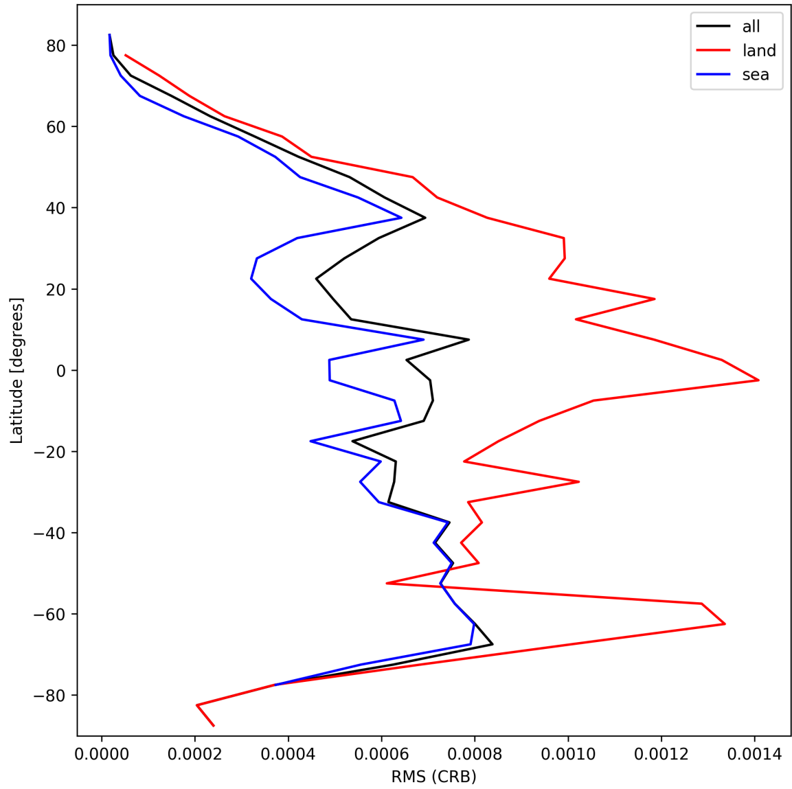
Figure 32: Zonal average of “RMS (CRB)” for 2025-10-15 to 2025-10-17.
