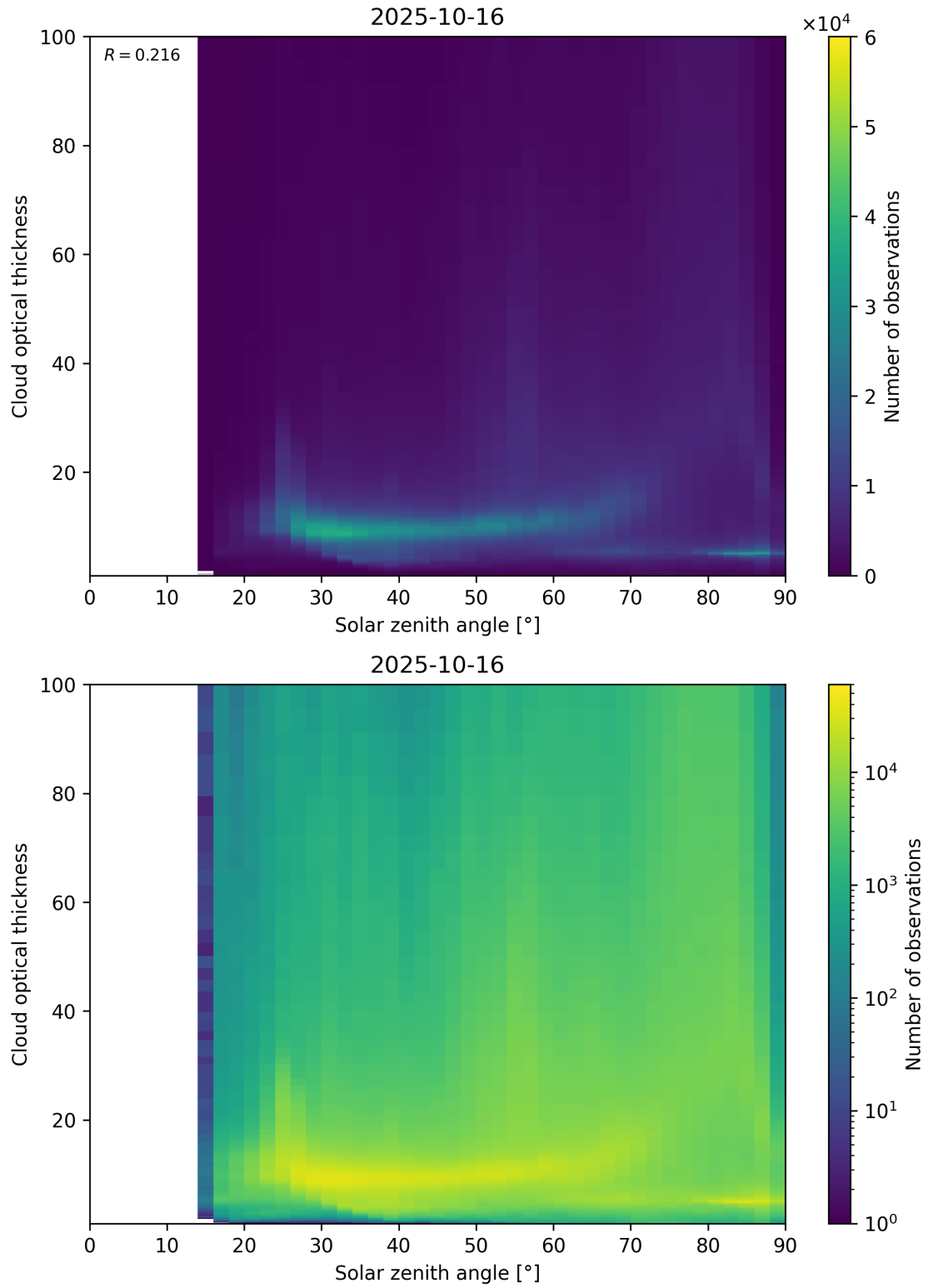
Figure 103: Scatter density plot of “Solar zenith angle” against “Cloud optical thickness” for 2025-10-15 to 2025-10-17.
