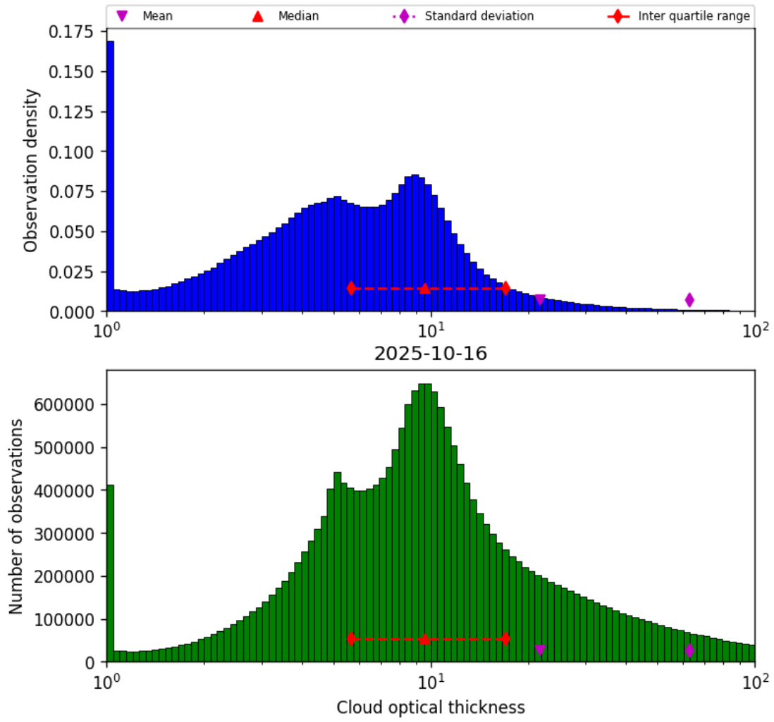
Figure 41: Histogram of “Cloud optical thickness” for 2025-10-15 to 2025-10-17
