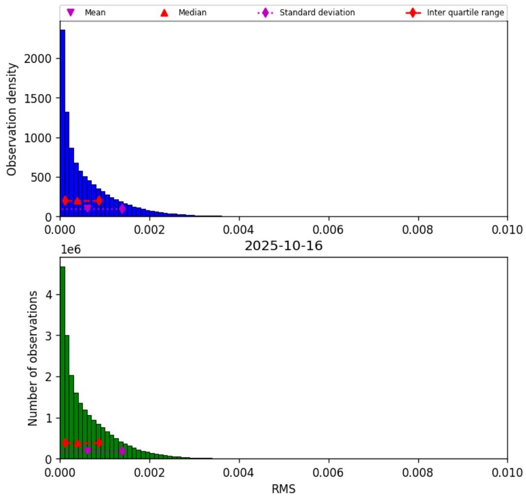
Figure 47: Histogram of “RMS” for 2025-10-15 to 2025-10-17
