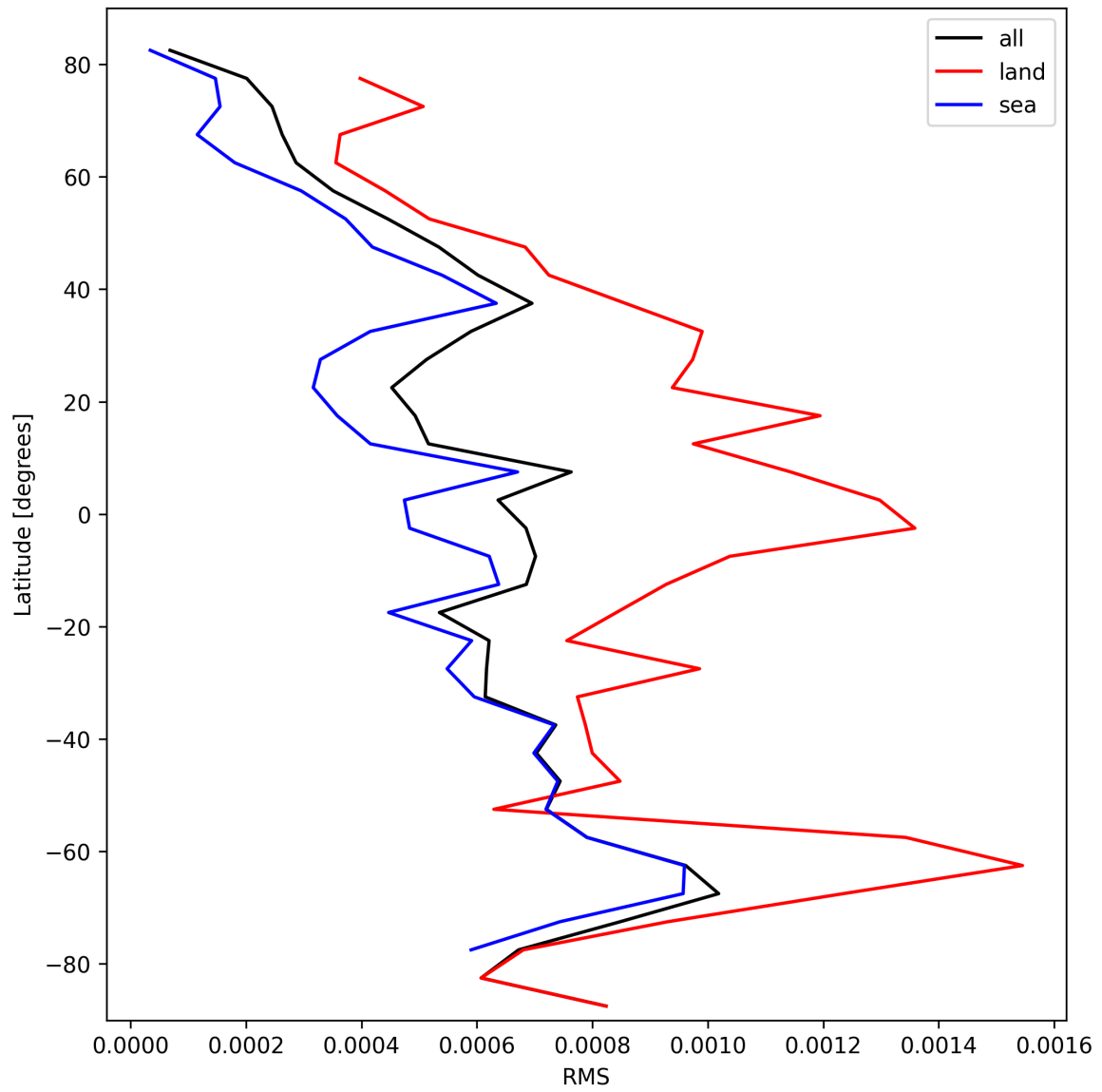
Figure 31: Zonal average of “RMS” for 2025-10-15 to 2025-10-17.
