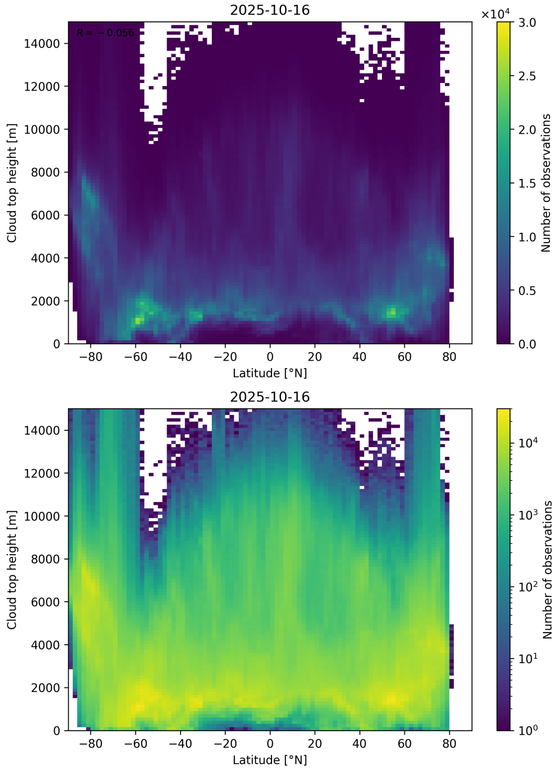
Figure 97: Scatter density plot of “Latitude” against “Cloud top height” for 2025-10-15 to 2025-10-17.
