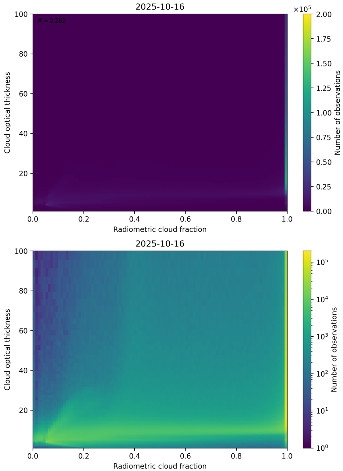
Figure 75: Scatter density plot of “Radiometric cloud fraction” against “Cloud optical thickness” for 2025-10-15 to 2025-10-17.
