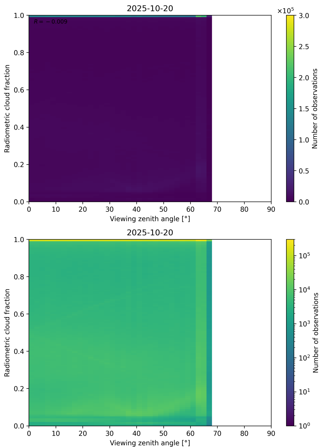
Figure 107: Scatter density plot of “Viewing zenith angle” against “Radiometric cloud fraction” for 2025-10-19 to 2025-10-21.
