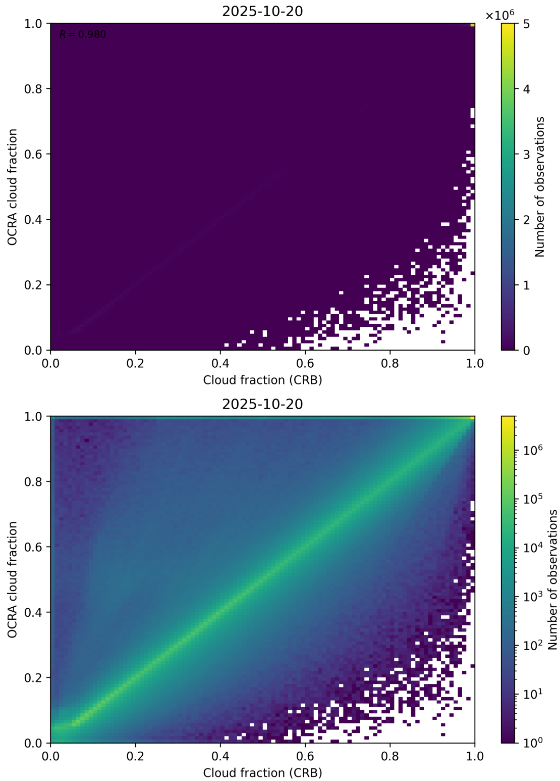
Figure 78: Scatter density plot of “Cloud fraction (CRB)” against “OCRA cloud fraction” for 2025-10-19 to 2025-10-21.
