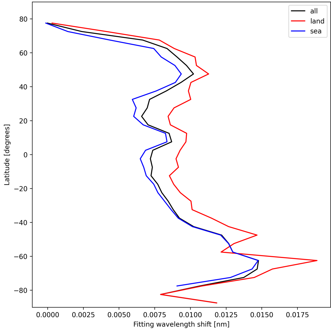
Figure 33: Zonal average of “Fitting wavelength shift” for 2025-10-19 to 2025-10-21.
