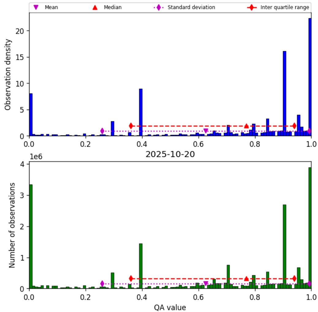
Figure 38: Histogram of “QA value” for 2025-10-19 to 2025-10-21
