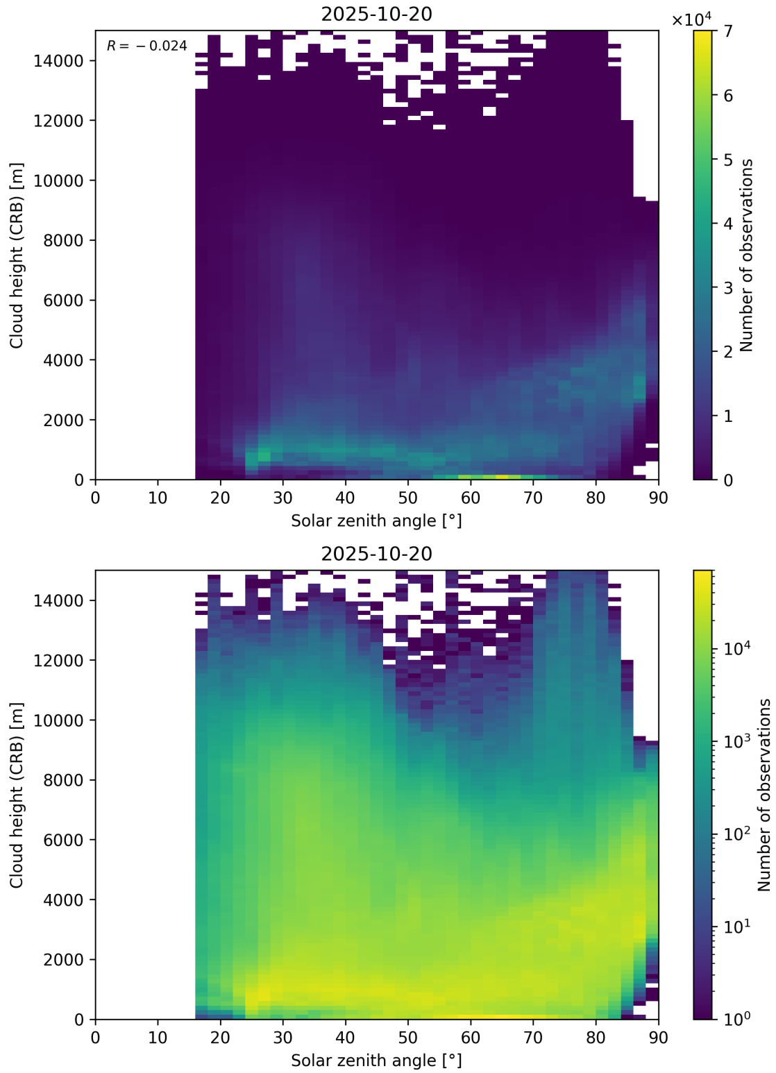
Figure 102: Scatter density plot of “Solar zenith angle” against “Cloud height (CRB)” for 2025-10-19 to 2025-10-21.
