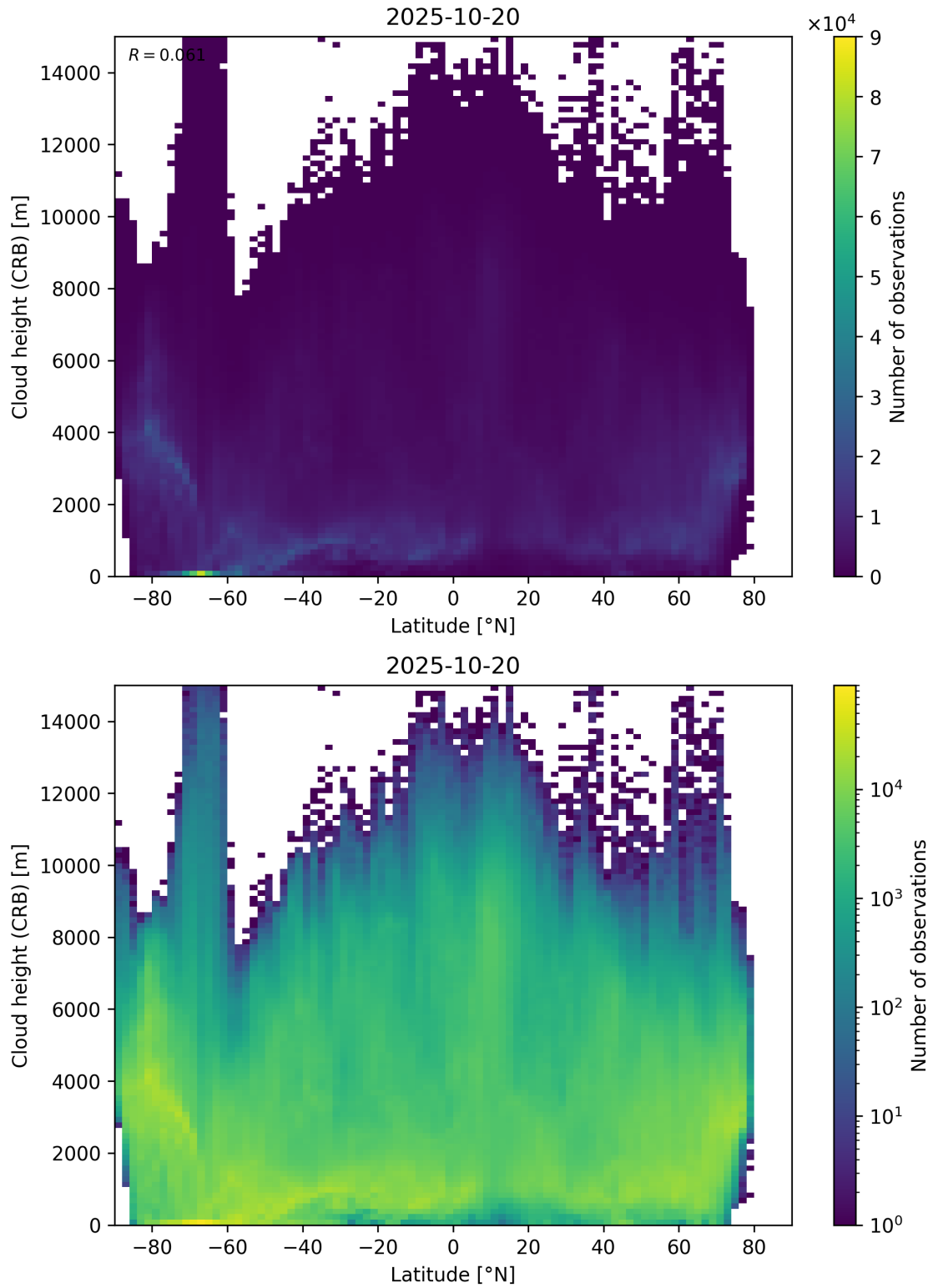
Figure 95: Scatter density plot of “Latitude” against “Cloud height (CRB)” for 2025-10-19 to 2025-10-21.
