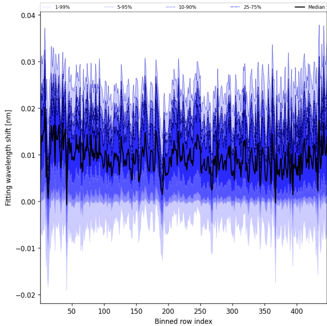
Figure 65: Along track statistics of “Fitting wavelength shift” for 2025-10-19 to 2025-10-21
