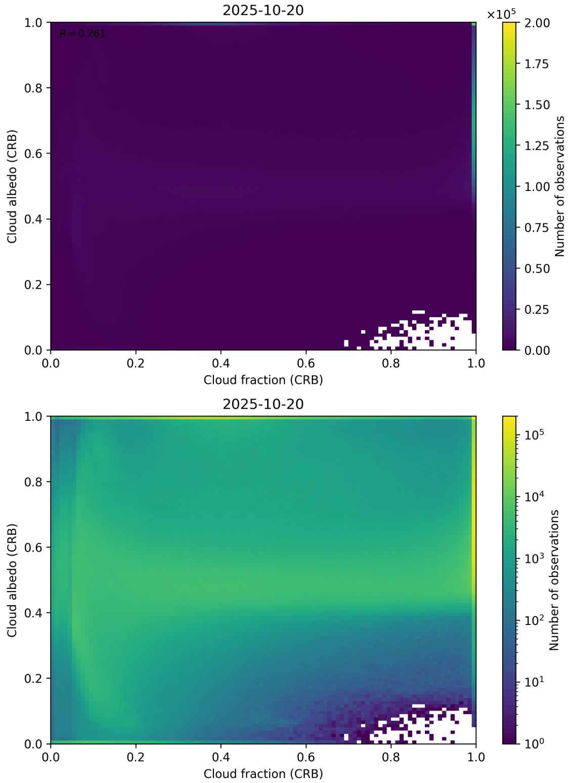
Figure 77: Scatter density plot of “Cloud fraction (CRB)” against “Cloud albedo (CRB)” for 2025-10-19 to 2025-10-21.
