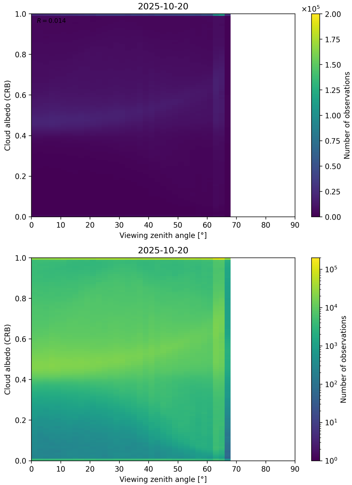
Figure 106: Scatter density plot of “Viewing zenith angle” against “Cloud albedo (CRB)” for 2025-10-19 to 2025-10-21.
