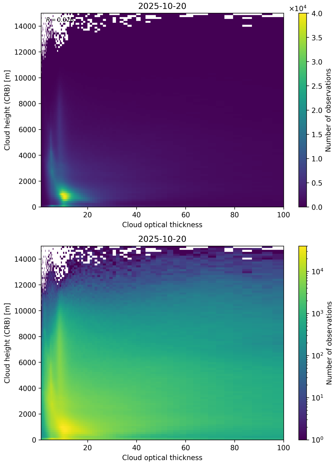
Figure 85: Scatter density plot of “Cloud optical thickness” against “Cloud height (CRB)” for 2025-10-19 to 2025-10-21.
