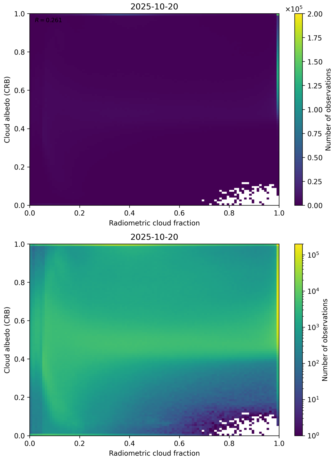
Figure 71: Scatter density plot of “Radiometric cloud fraction” against “Cloud albedo (CRB)” for 2025-10-19 to 2025-10-21.
