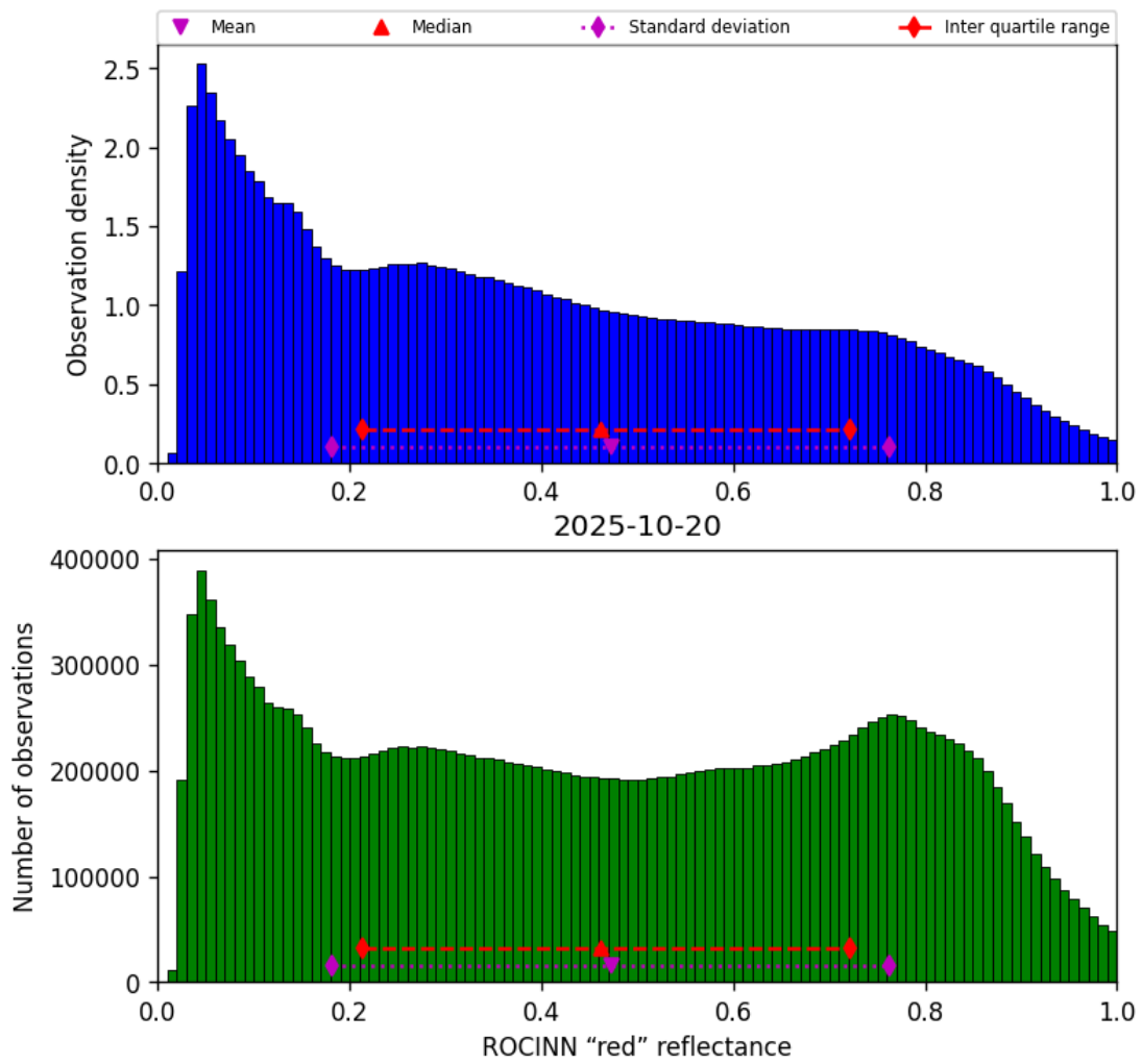
Figure 53: Histogram of “ROCINN “red” reflectance” for 2025-10-19 to 2025-10-21
