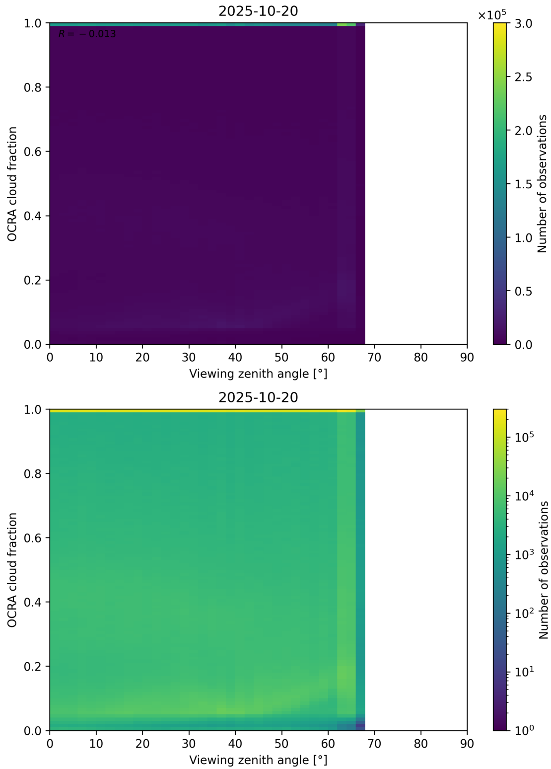
Figure 108: Scatter density plot of “Viewing zenith angle” against “OCRA cloud fraction” for 2025-10-19 to 2025-10-21.
