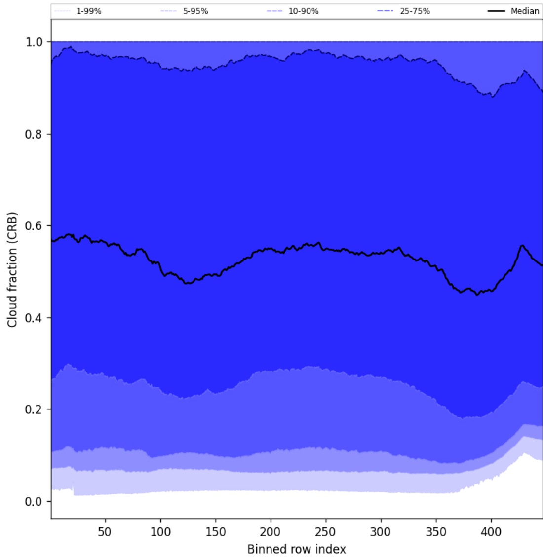
Figure 58: Along track statistics of “Cloud fraction (CRB)” for 2025-10-19 to 2025-10-21
