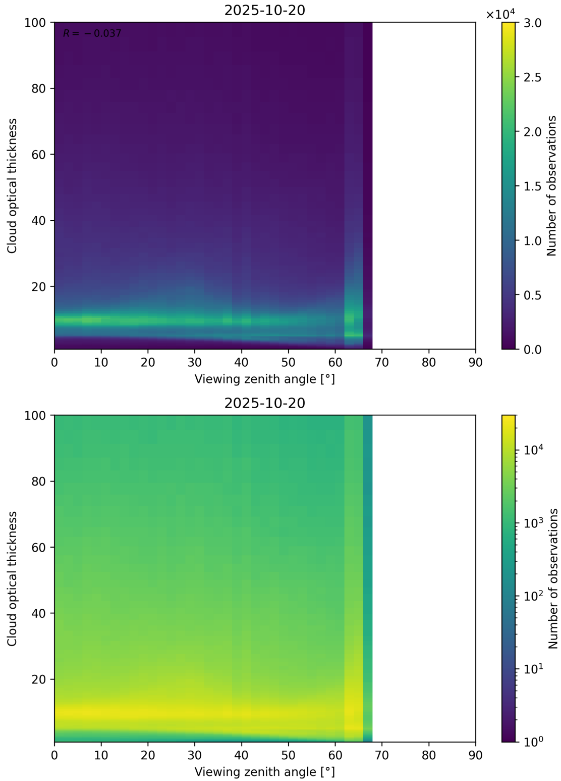
Figure 111: Scatter density plot of “Viewing zenith angle” against “Cloud optical thickness” for 2025-10-19 to 2025-10-21.
