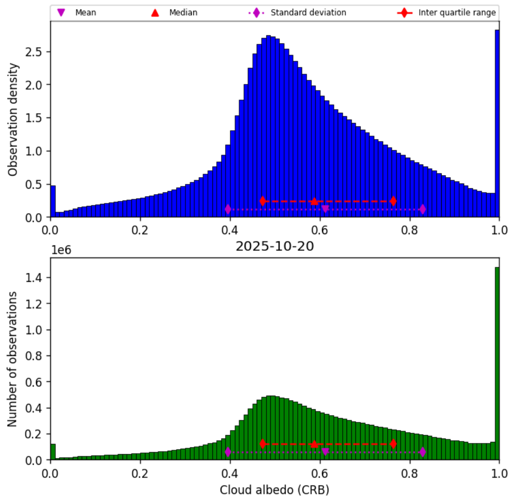
Figure 44: Histogram of “Cloud albedo (CRB)” for 2025-10-19 to 2025-10-21
