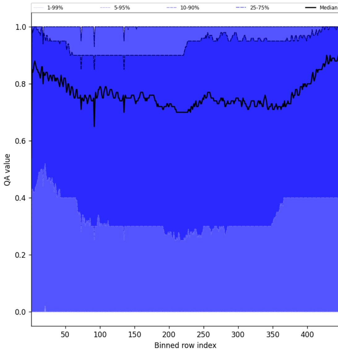
Figure 54: Along track statistics of “QA value” for 2025-10-19 to 2025-10-21
