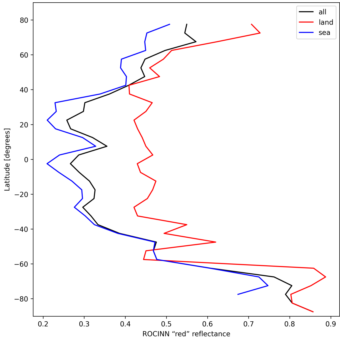
Figure 37: Zonal average of “ROCINN “red” reflectance” for 2025-10-19 to 2025-10-21.
