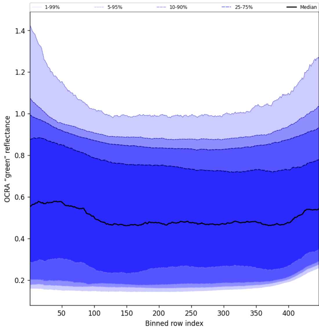
Figure 68: Along track statistics of "OCRA "green" reflectance" for 2025-10-19 to 2025-10-21
