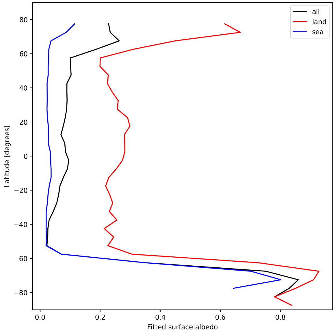
Figure 29: Zonal average of “Fitted surface albedo” for 2025-10-19 to 2025-10-21.
