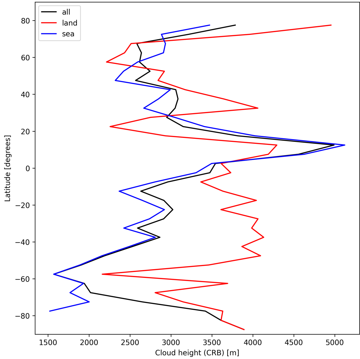
Figure 27: Zonal average of “Cloud height (CRB)” for 2025-10-19 to 2025-10-21.
