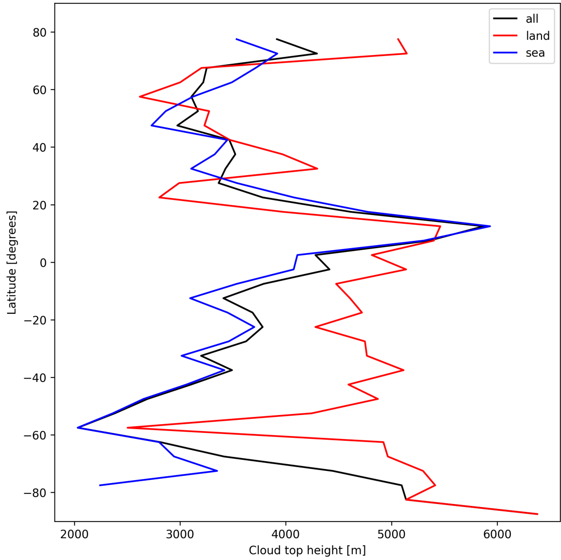
Figure 24: Zonal average of “Cloud top height” for 2025-10-19 to 2025-10-21.
