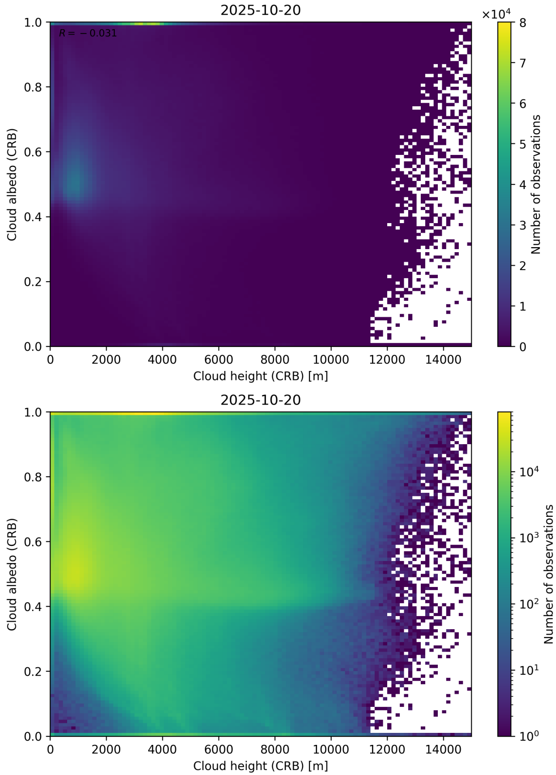
Figure 80: Scatter density plot of “Cloud height (CRB)” against “Cloud albedo (CRB)” for 2025-10-19 to 2025-10-21.
