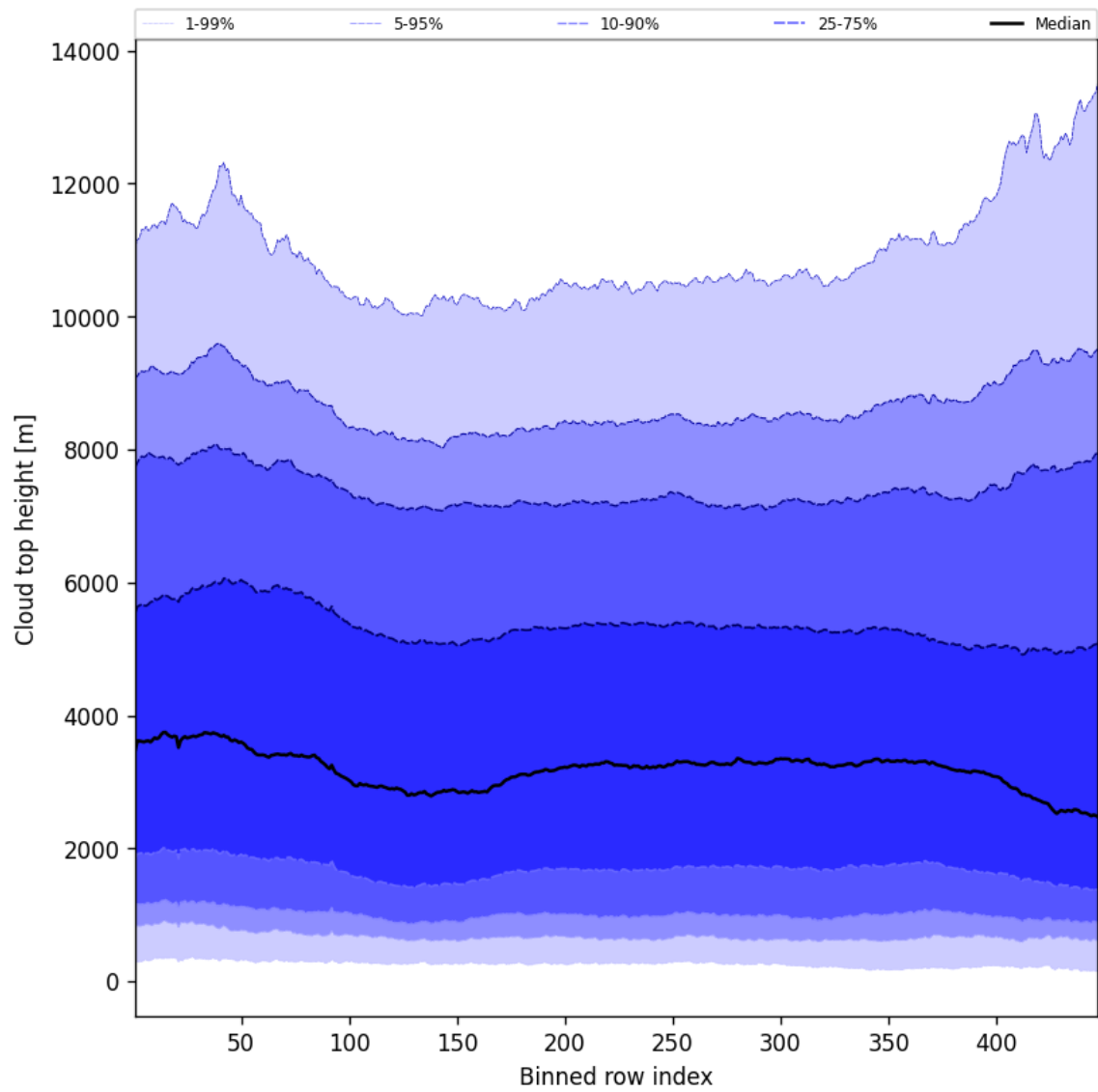
Figure 56: Along track statistics of “Cloud top height” for 2025-10-19 to 2025-10-21
