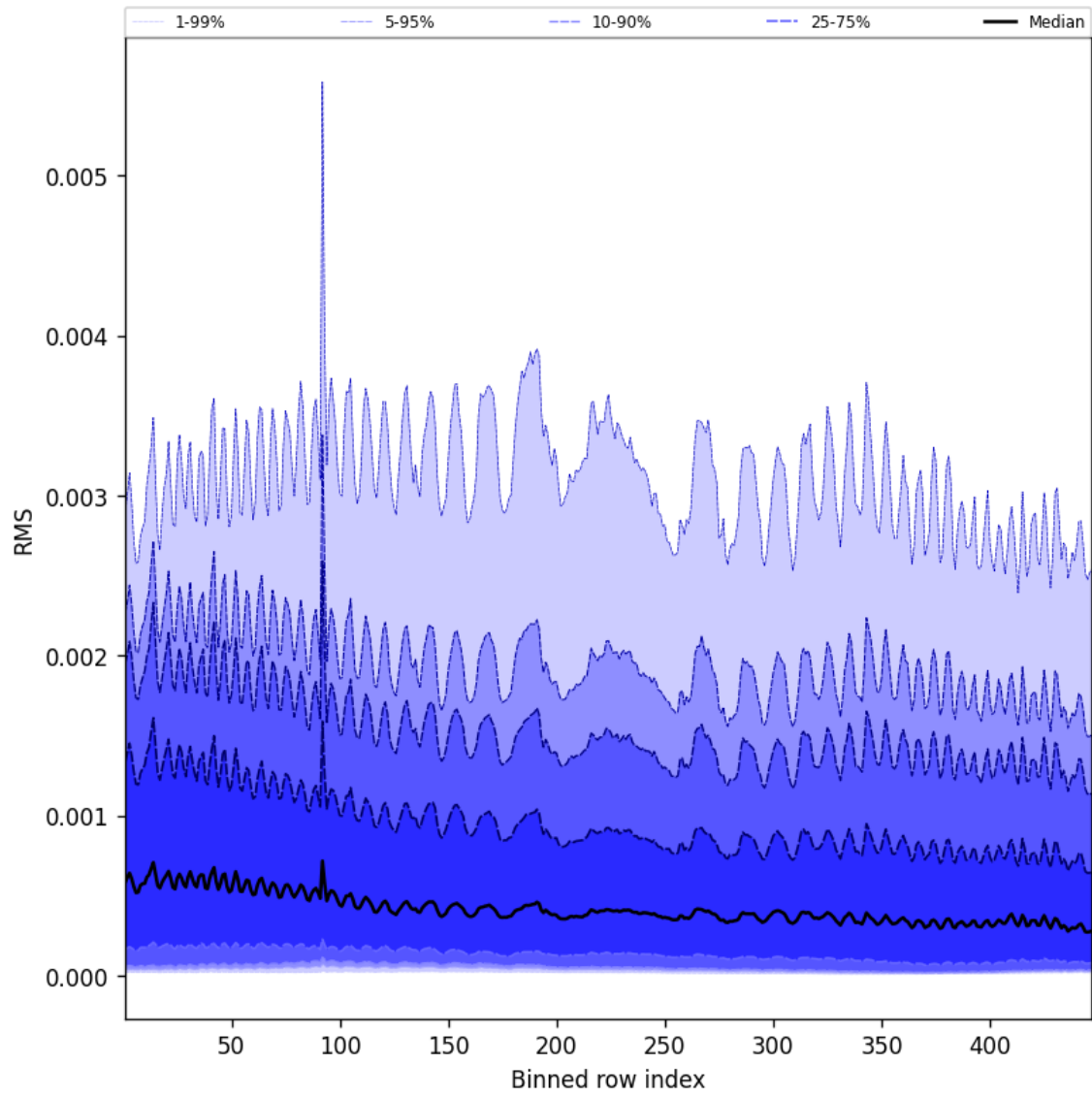
Figure 63: Along track statistics of “RMS” for 2025-10-19 to 2025-10-21
