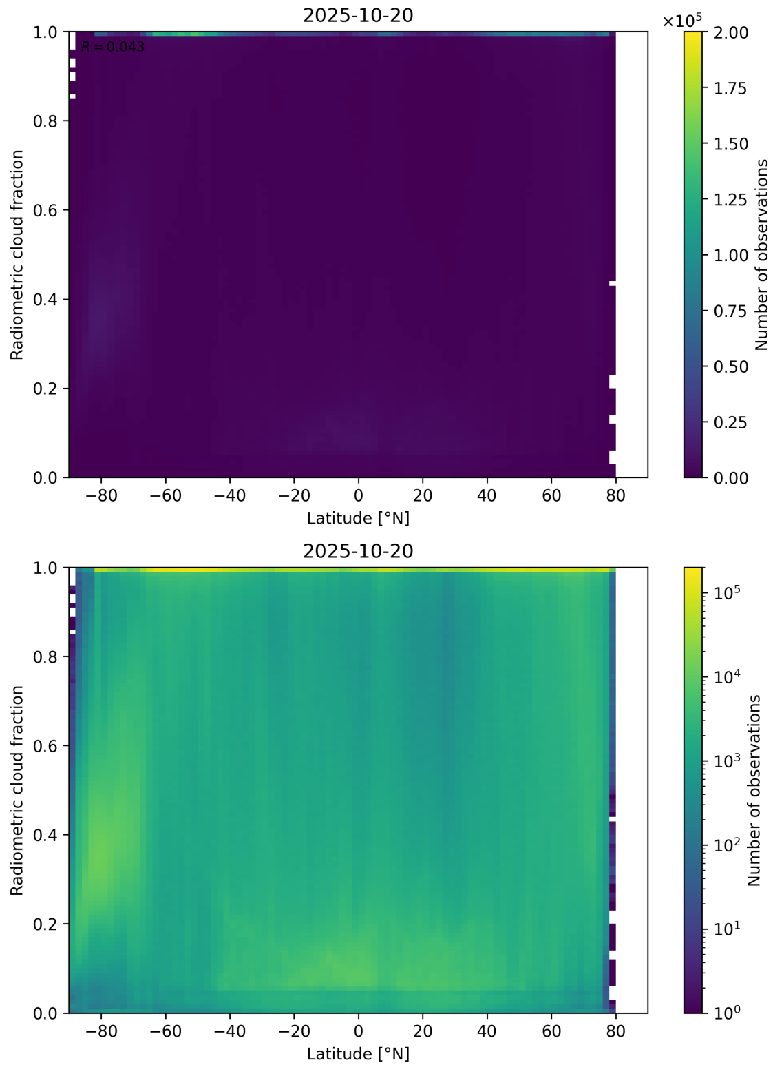
Figure 92: Scatter density plot of “Latitude” against “Radiometric cloud fraction” for 2025-10-19 to 2025-10-21.
