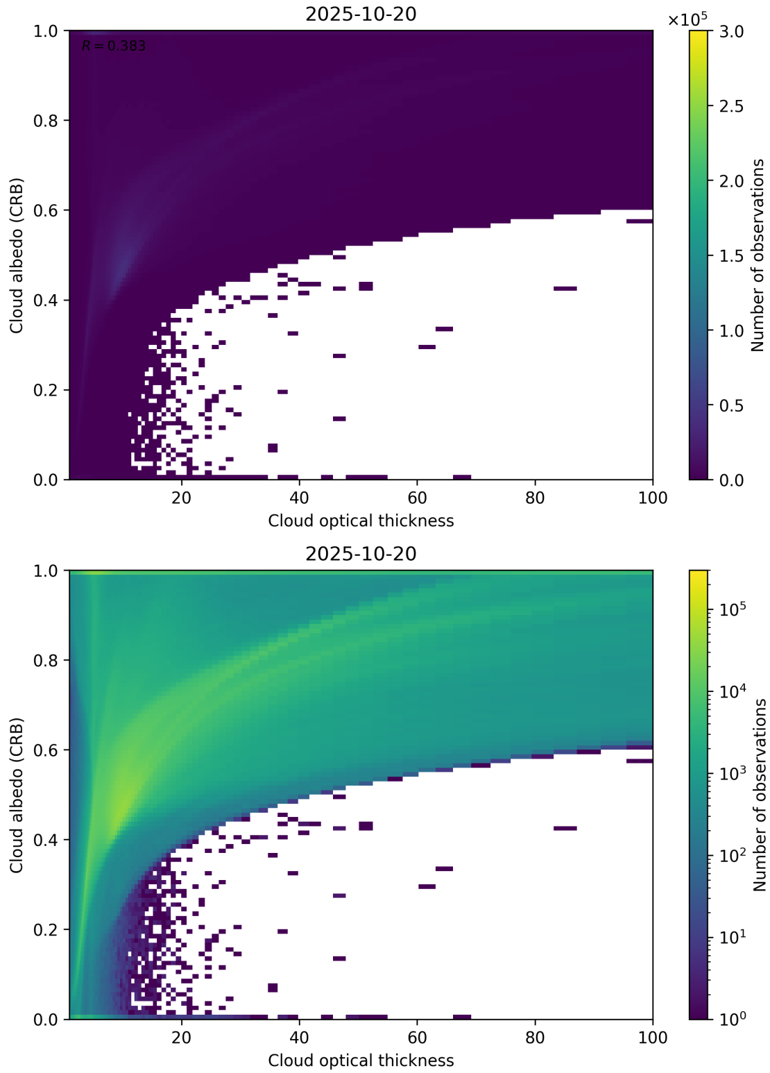
Figure 82: Scatter density plot of “Cloud optical thickness” against “Cloud albedo (CRB)” for 2025-10-19 to 2025-10-21.
