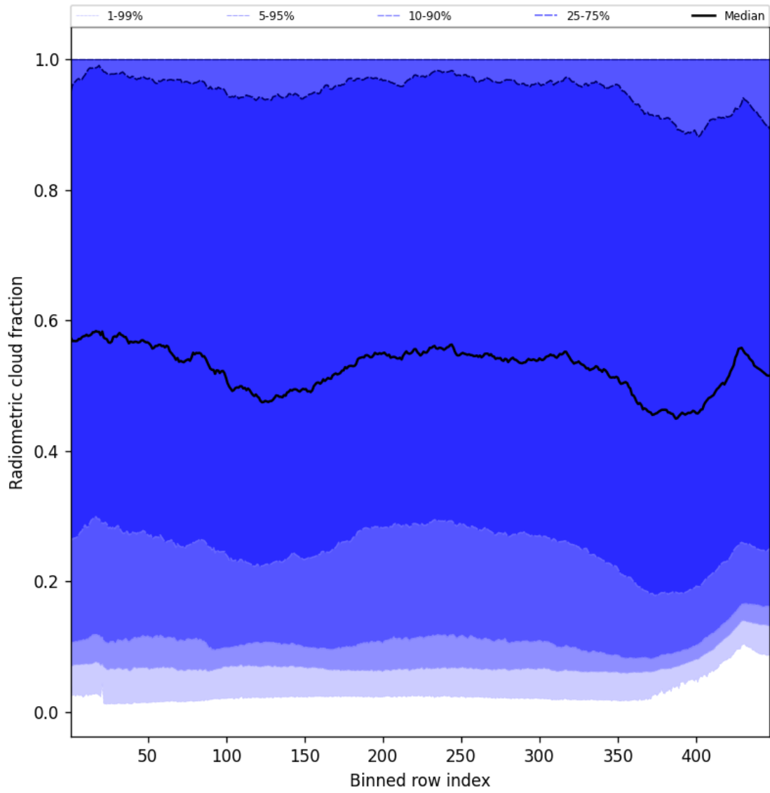
Figure 55: Along track statistics of “Radiometric cloud fraction” for 2025-10-19 to 2025-10-21
