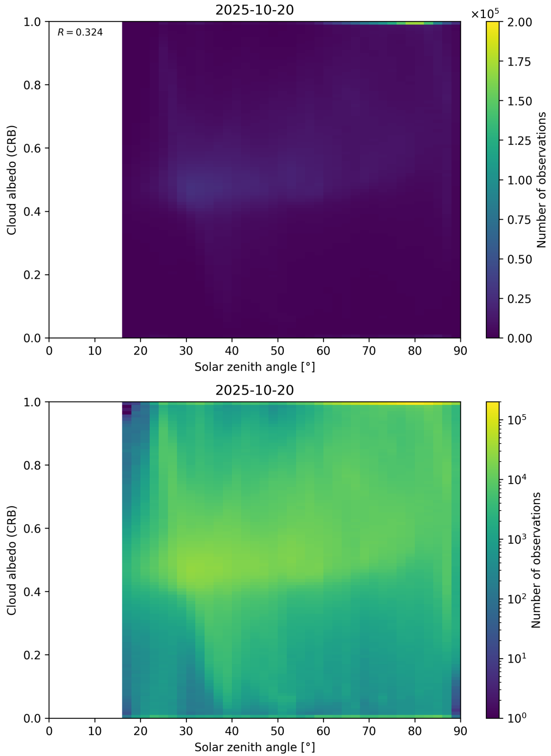
Figure 98: Scatter density plot of “Solar zenith angle” against “Cloud albedo (CRB)” for 2025-10-19 to 2025-10-21.
