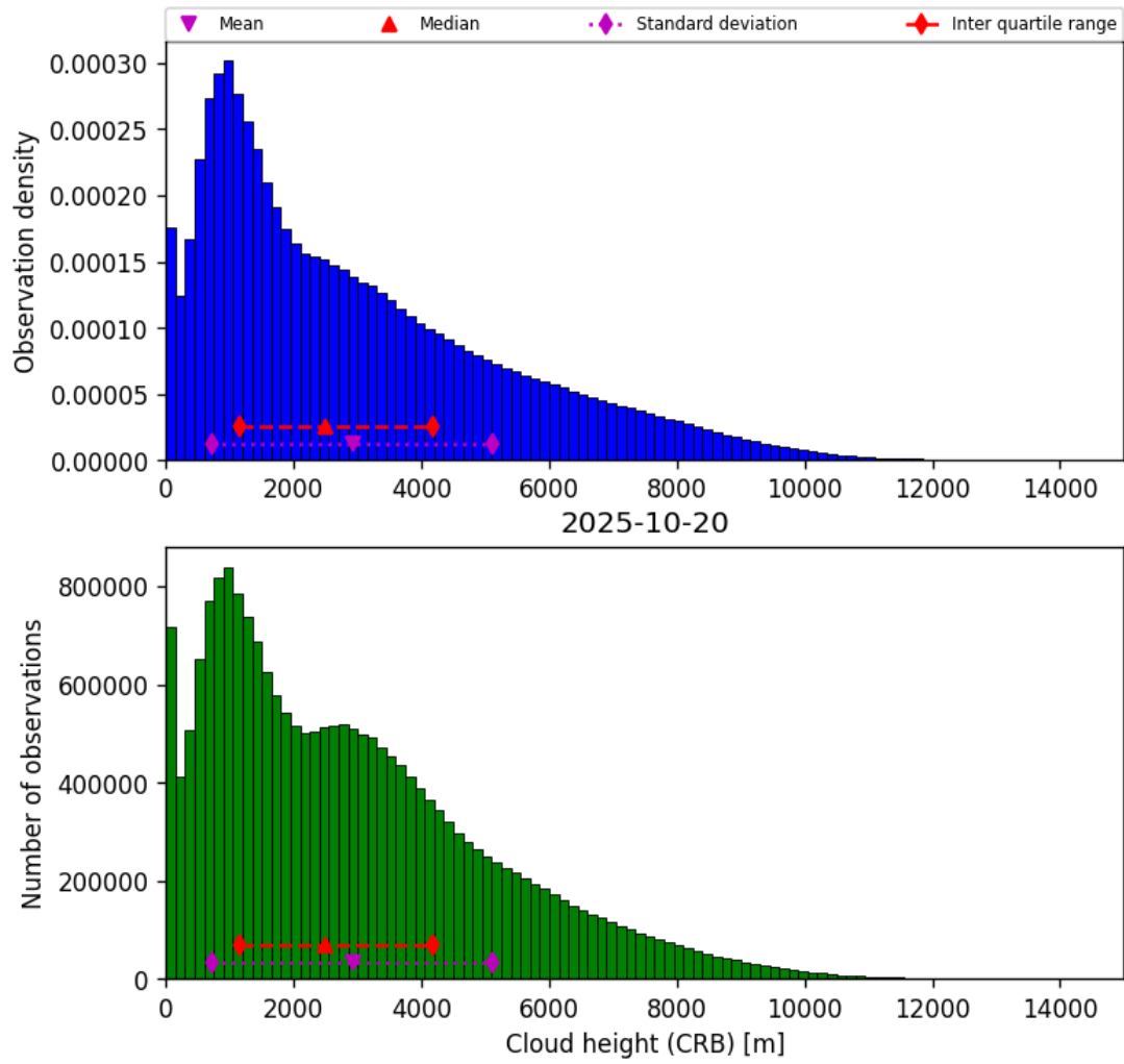
Figure 43: Histogram of “Cloud height (CRB)” for 2025-10-19 to 2025-10-21
