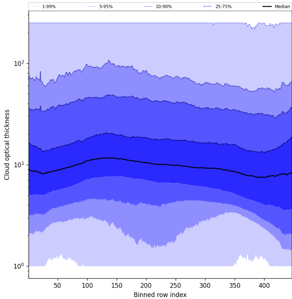
Figure 57: Along track statistics of “Cloud optical thickness” for 2025-10-19 to 2025-10-21
