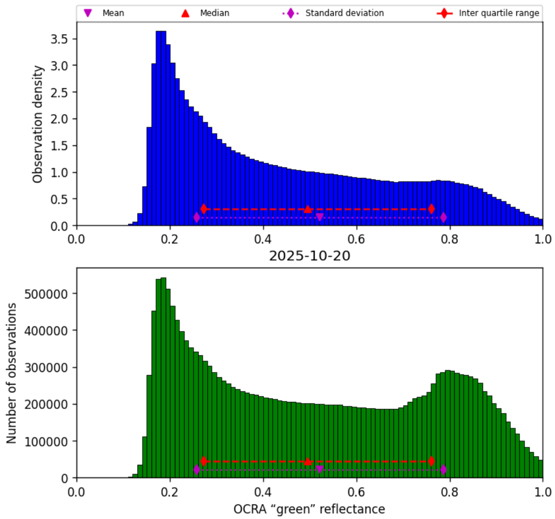
Figure 52: Histogram of “OCRA “green” reflectance” for 2025-10-19 to 2025-10-21
