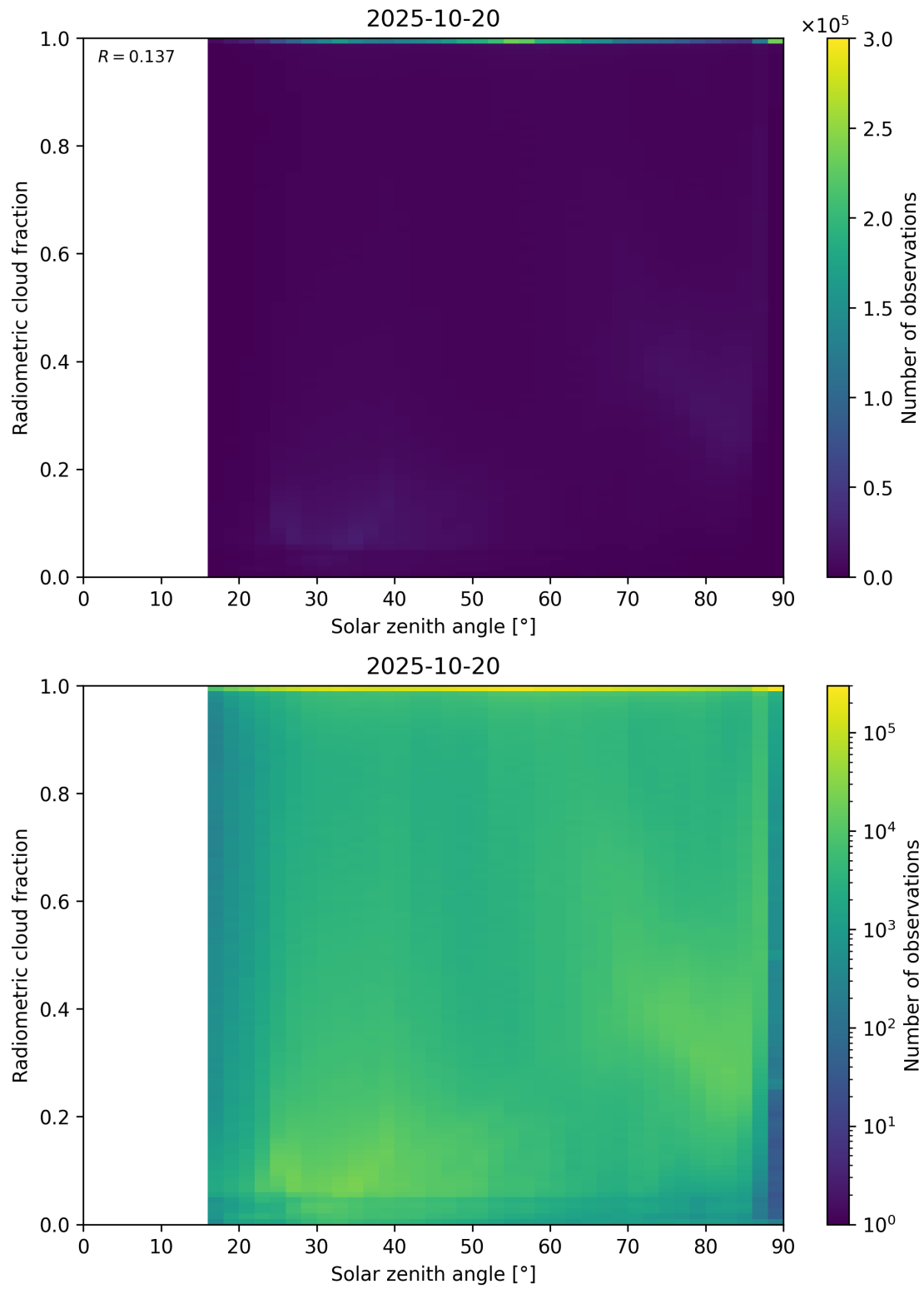
Figure 99: Scatter density plot of “Solar zenith angle” against “Radiometric cloud fraction” for 2025-10-19 to 2025-10-21.
