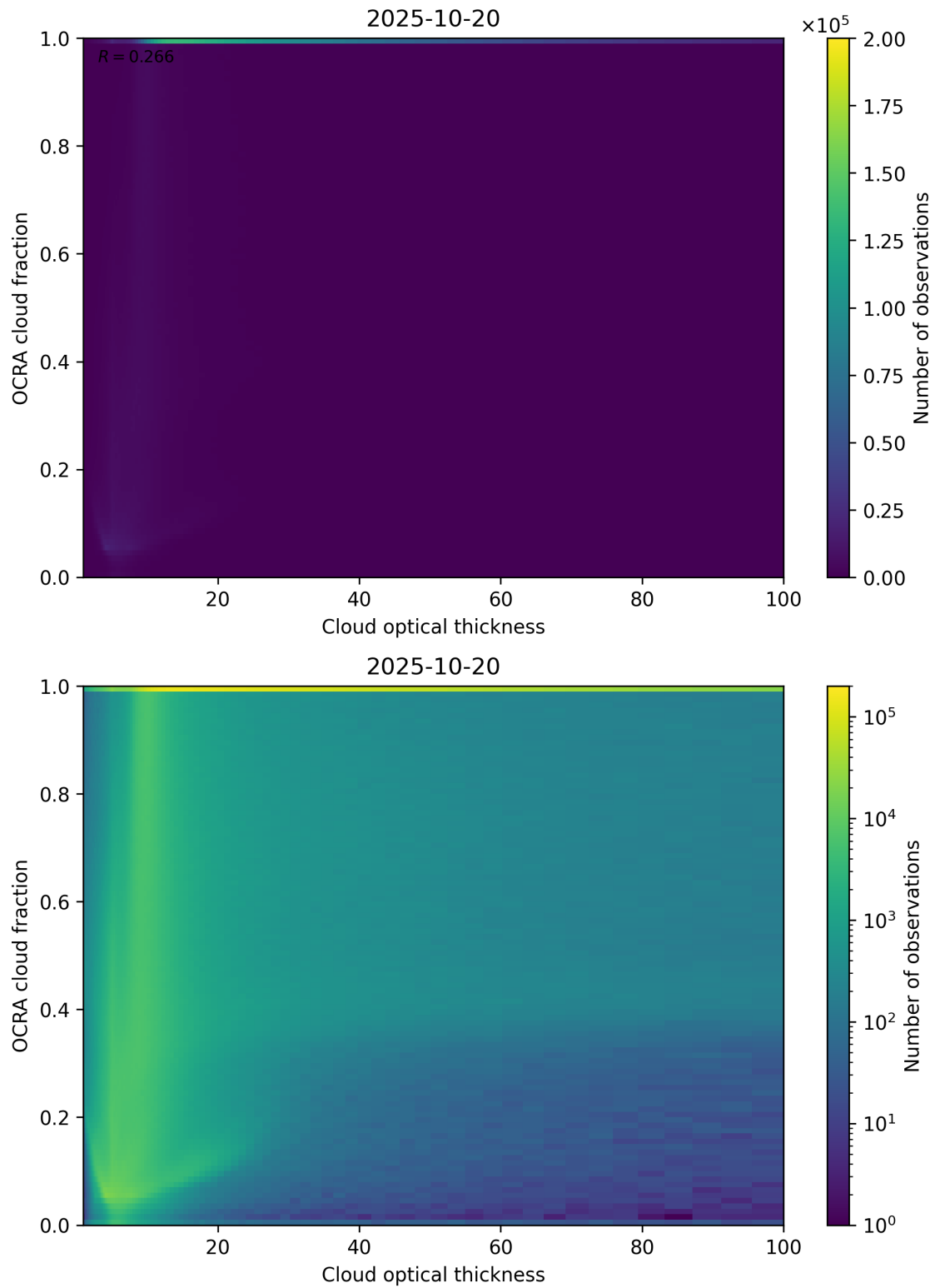
Figure 83: Scatter density plot of “Cloud optical thickness” against “OCRA cloud fraction” for 2025-10-19 to 2025-10-21.
