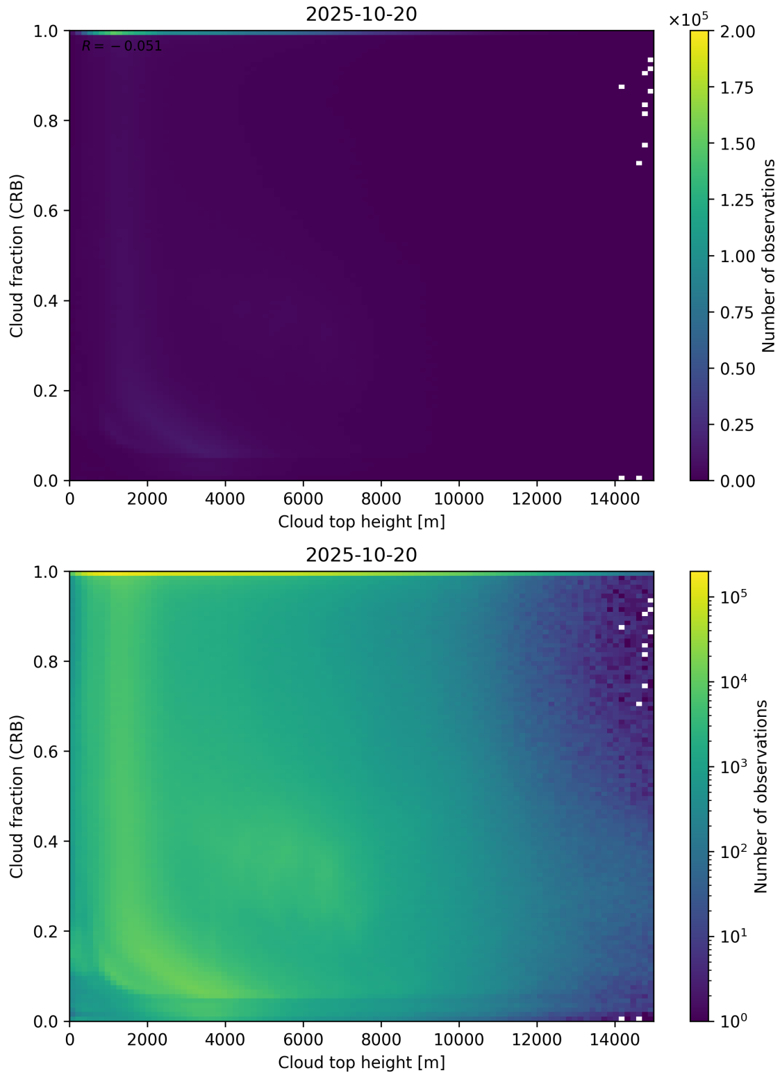
Figure 88: Scatter density plot of “Cloud top height” against “Cloud fraction (CRB)” for 2025-10-19 to 2025-10-21.
