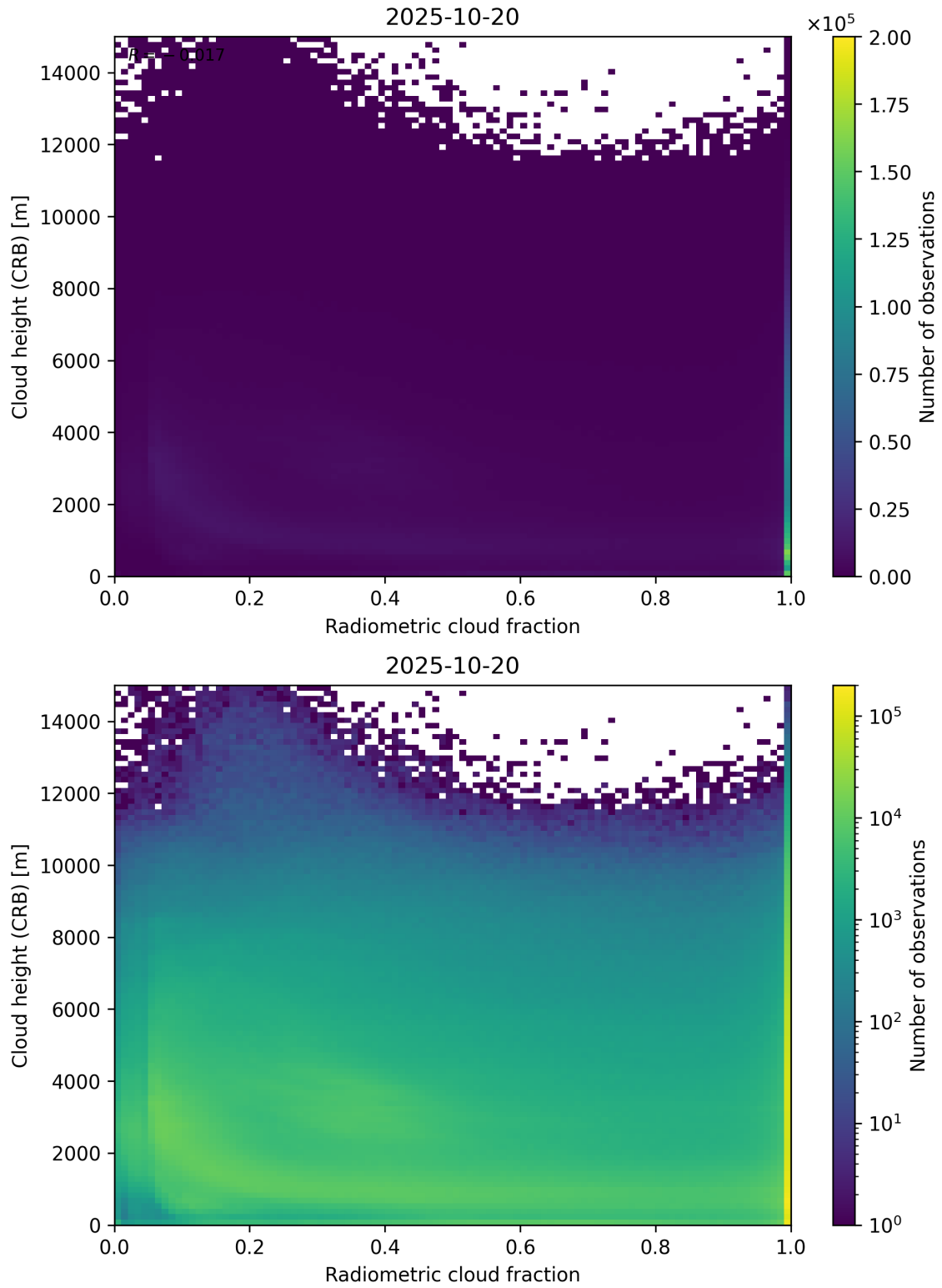
Figure 74: Scatter density plot of “Radiometric cloud fraction” against “Cloud height (CRB)” for 2025-10-19 to 2025-10-21.
