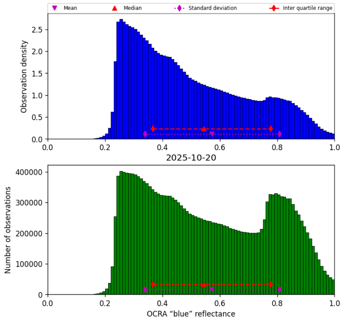
Figure 51: Histogram of “OCRA “blue” reflectance” for 2025-10-19 to 2025-10-21
