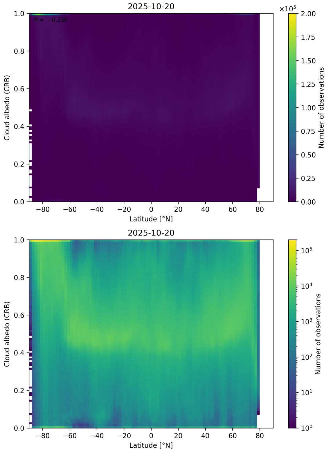
Figure 91: Scatter density plot of “Latitude” against “Cloud albedo (CRB)” for 2025-10-19 to 2025-10-21.
