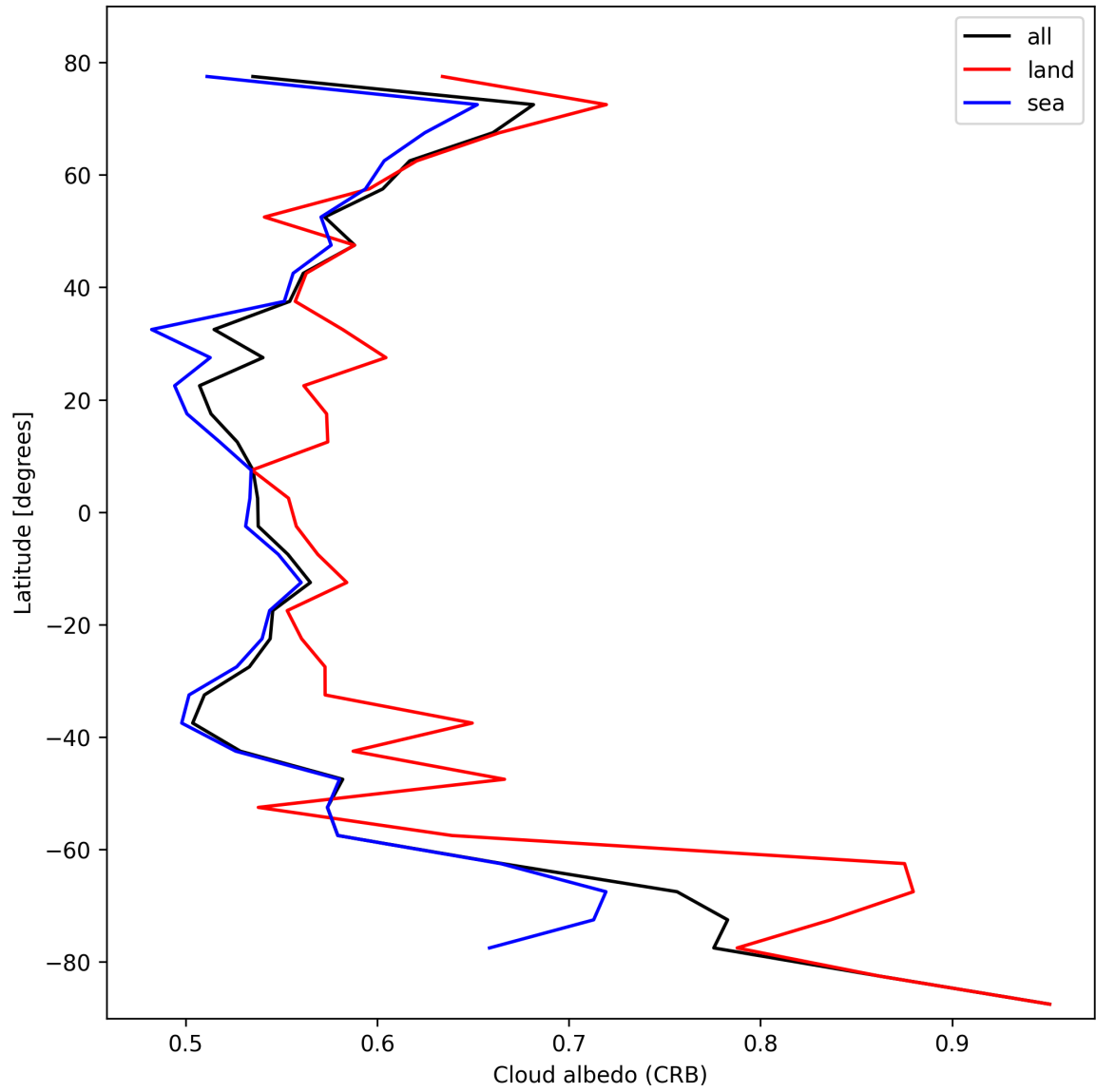
Figure 28: Zonal average of “Cloud albedo (CRB)” for 2025-10-19 to 2025-10-21.
