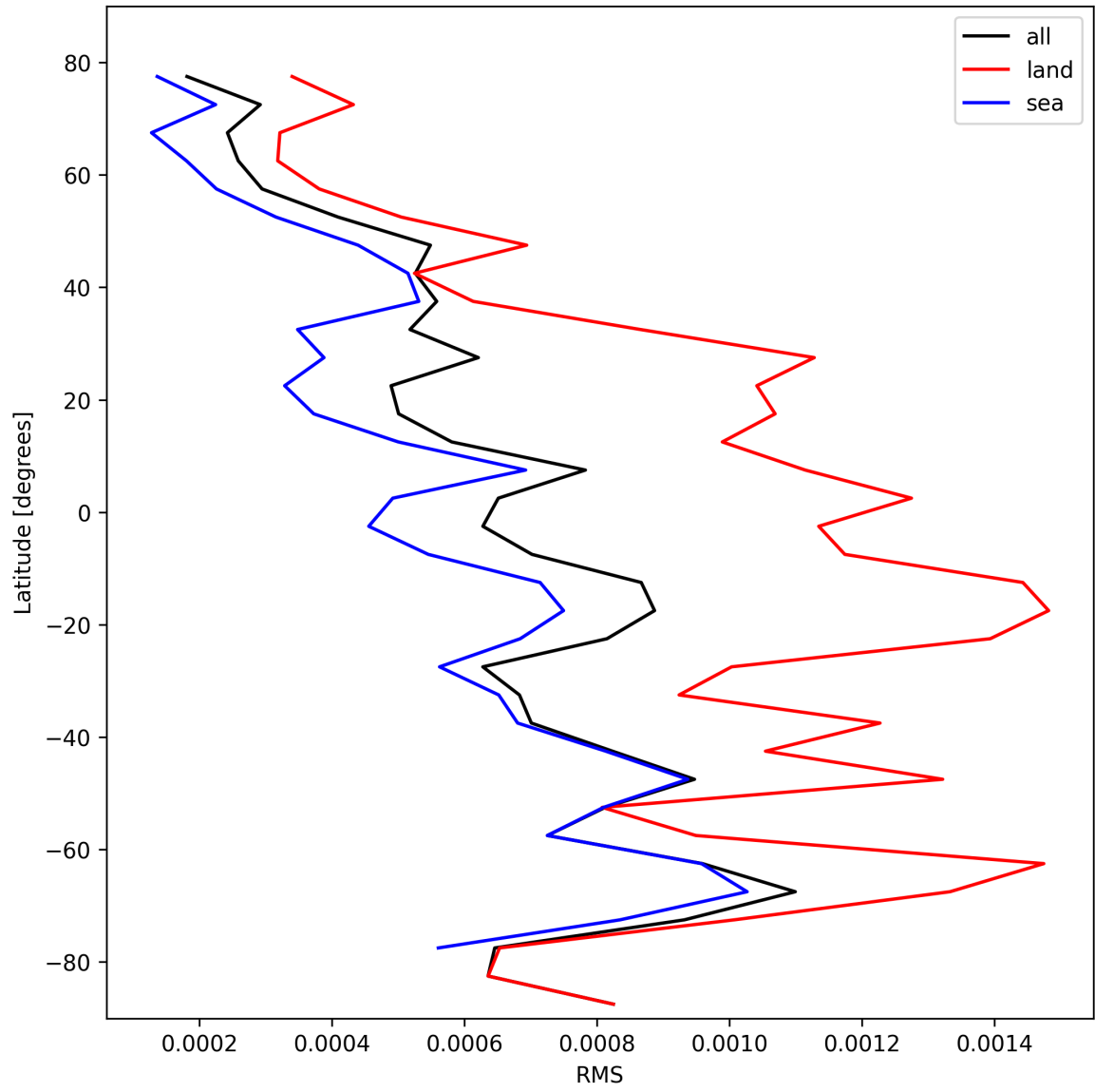
Figure 31: Zonal average of “RMS” for 2025-10-19 to 2025-10-21.
