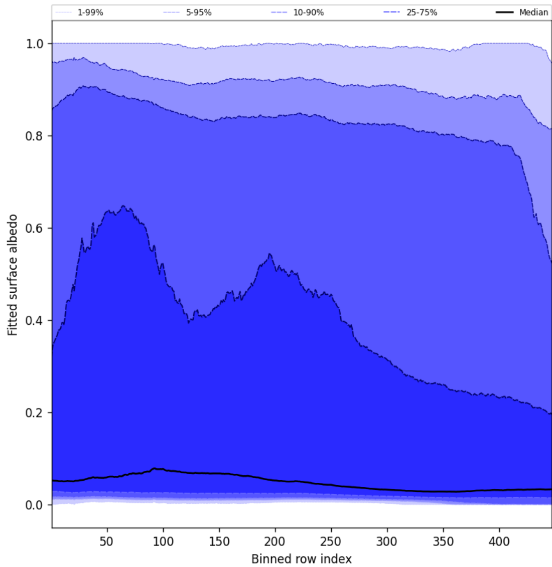
Figure 61: Along track statistics of “Fitted surface albedo” for 2025-10-19 to 2025-10-21
