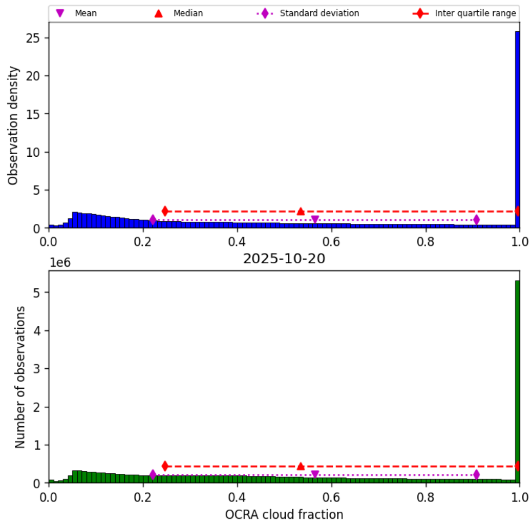
Figure 50: Histogram of “OCRA cloud fraction” for 2025-10-19 to 2025-10-21
