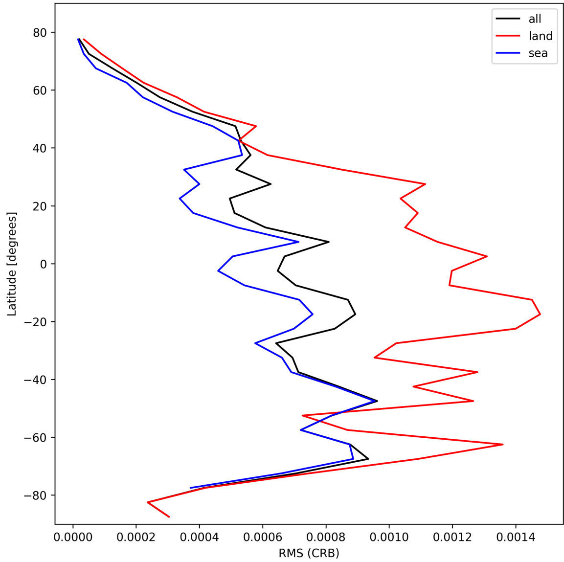
Figure 32: Zonal average of “RMS (CRB)” for 2025-10-19 to 2025-10-21.
