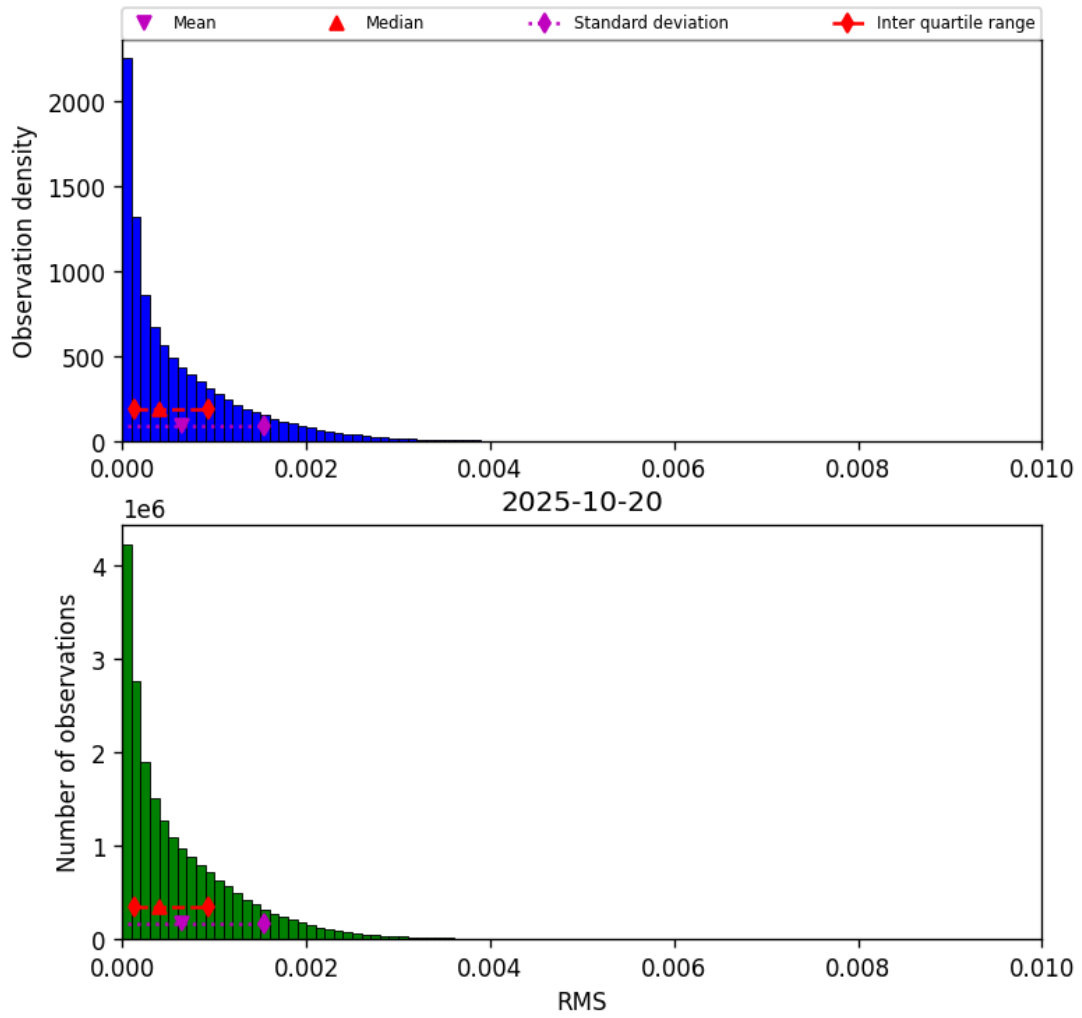
Figure 47: Histogram of “RMS” for 2025-10-19 to 2025-10-21
