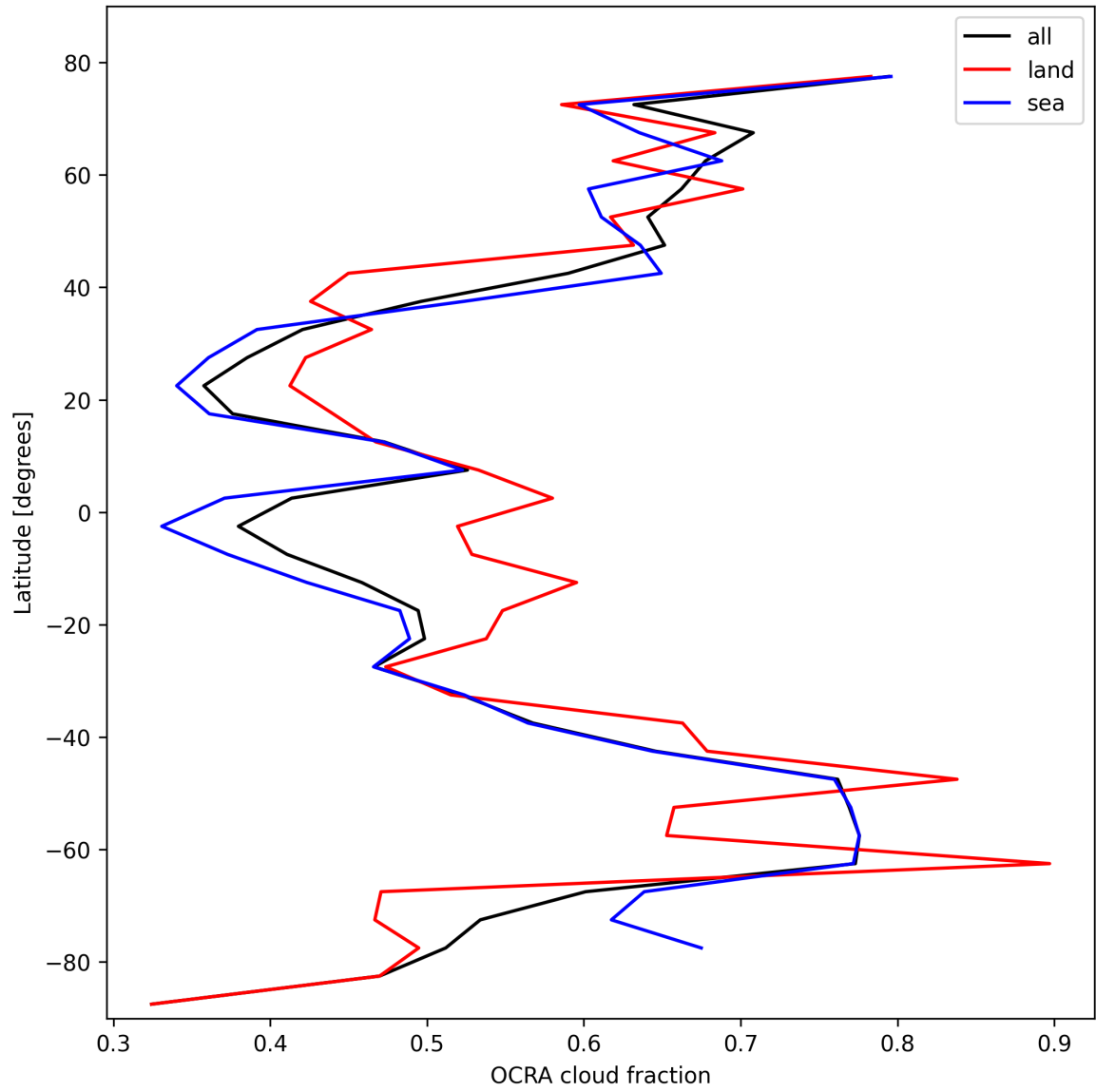
Figure 34: Zonal average of “OCRA cloud fraction” for 2025-10-19 to 2025-10-21.
