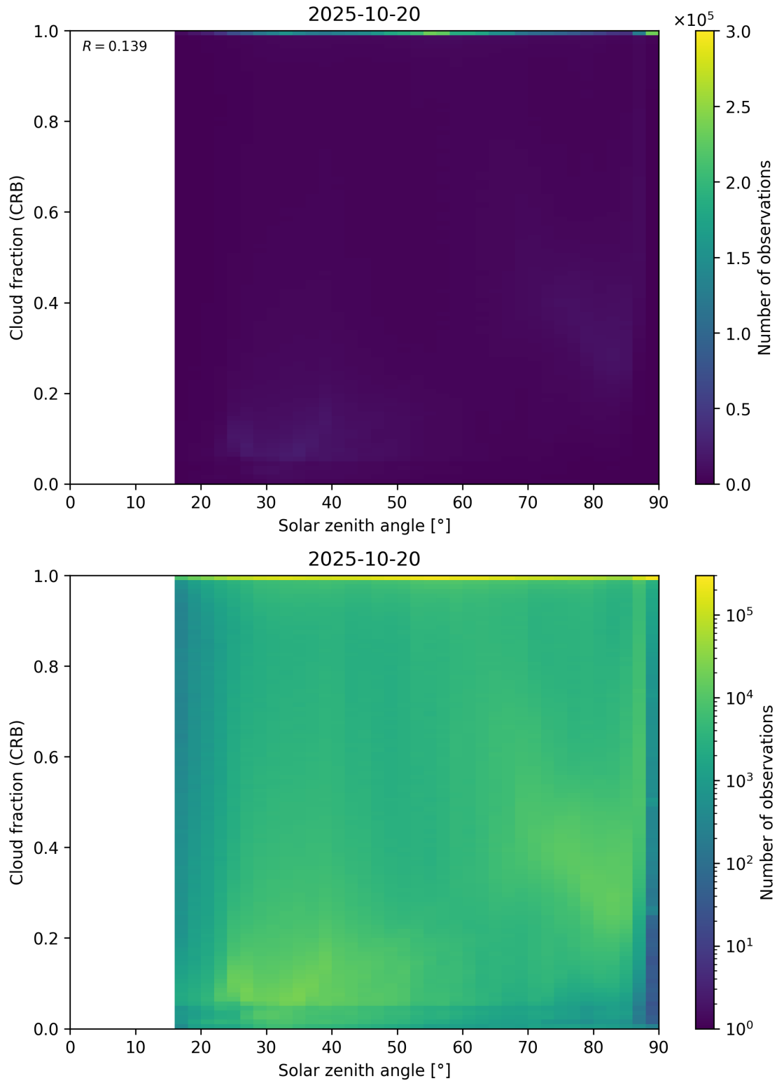
Figure 101: Scatter density plot of “Solar zenith angle” against “Cloud fraction (CRB)” for 2025-10-19 to 2025-10-21.
