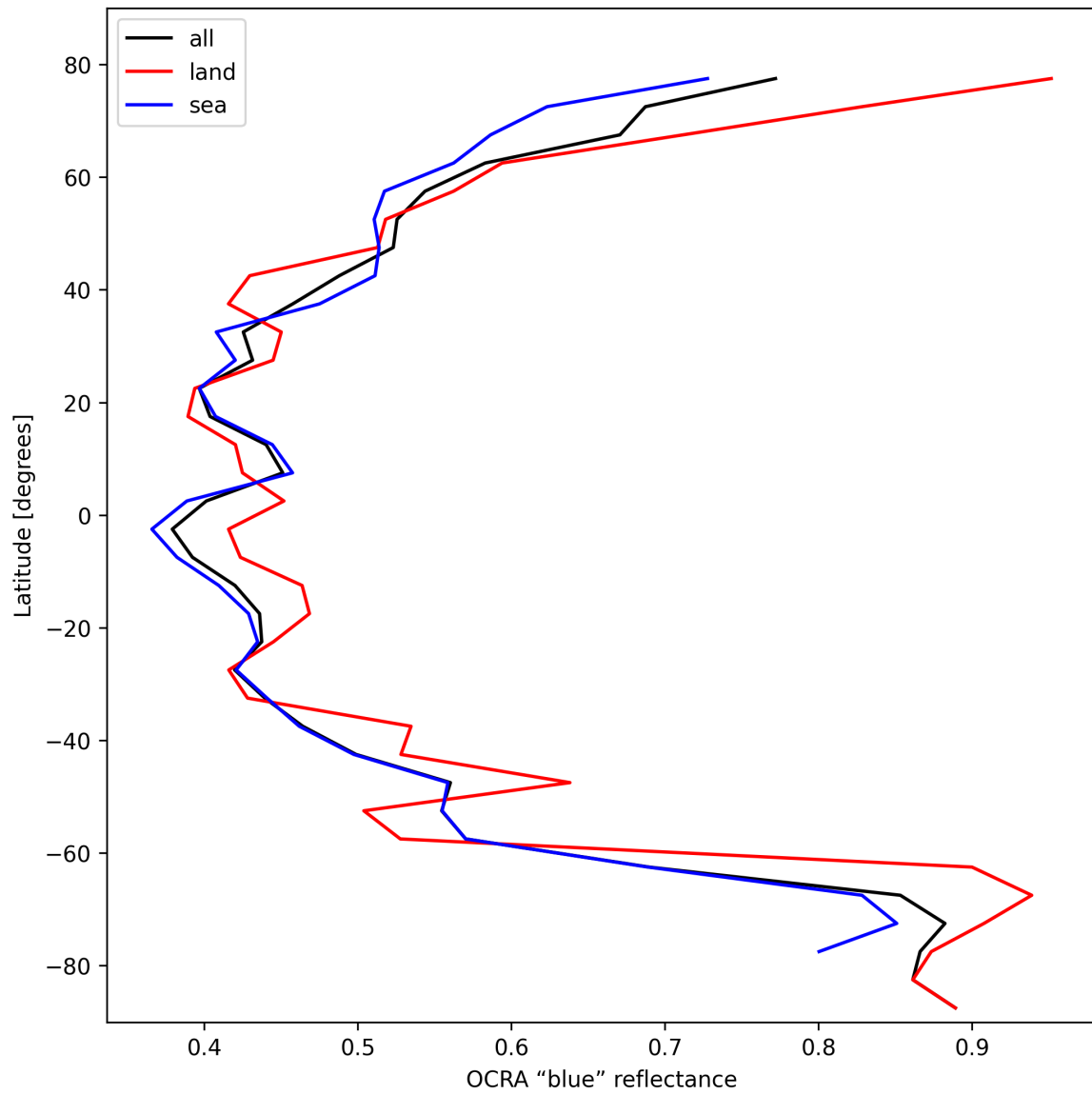
Figure 35: Zonal average of “OCRA “blue” reflectance” for 2025-10-19 to 2025-10-21.
