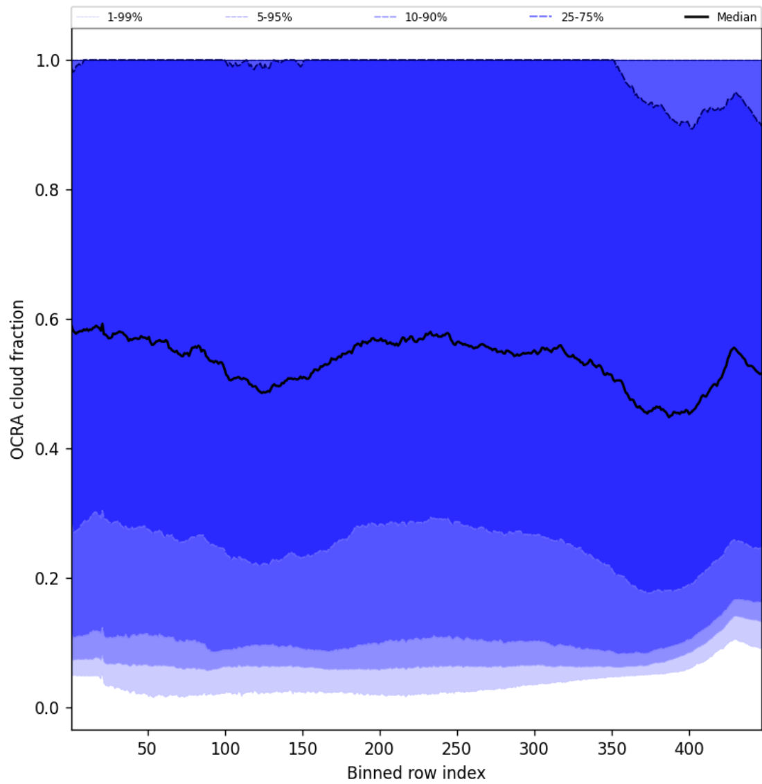
Figure 66: Along track statistics of “OCRA cloud fraction” for 2025-10-19 to 2025-10-21
