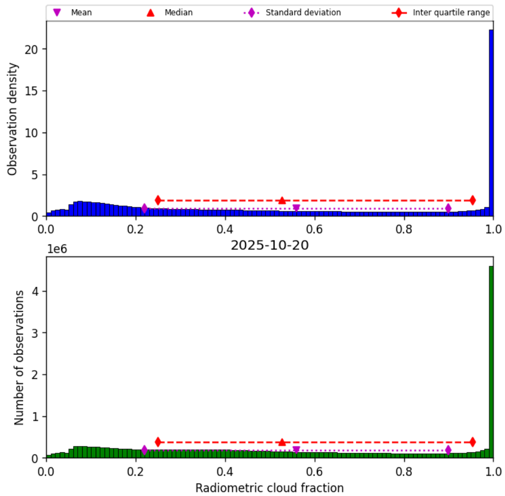
Figure 39: Histogram of “Radiometric cloud fraction” for 2025-10-19 to 2025-10-21
