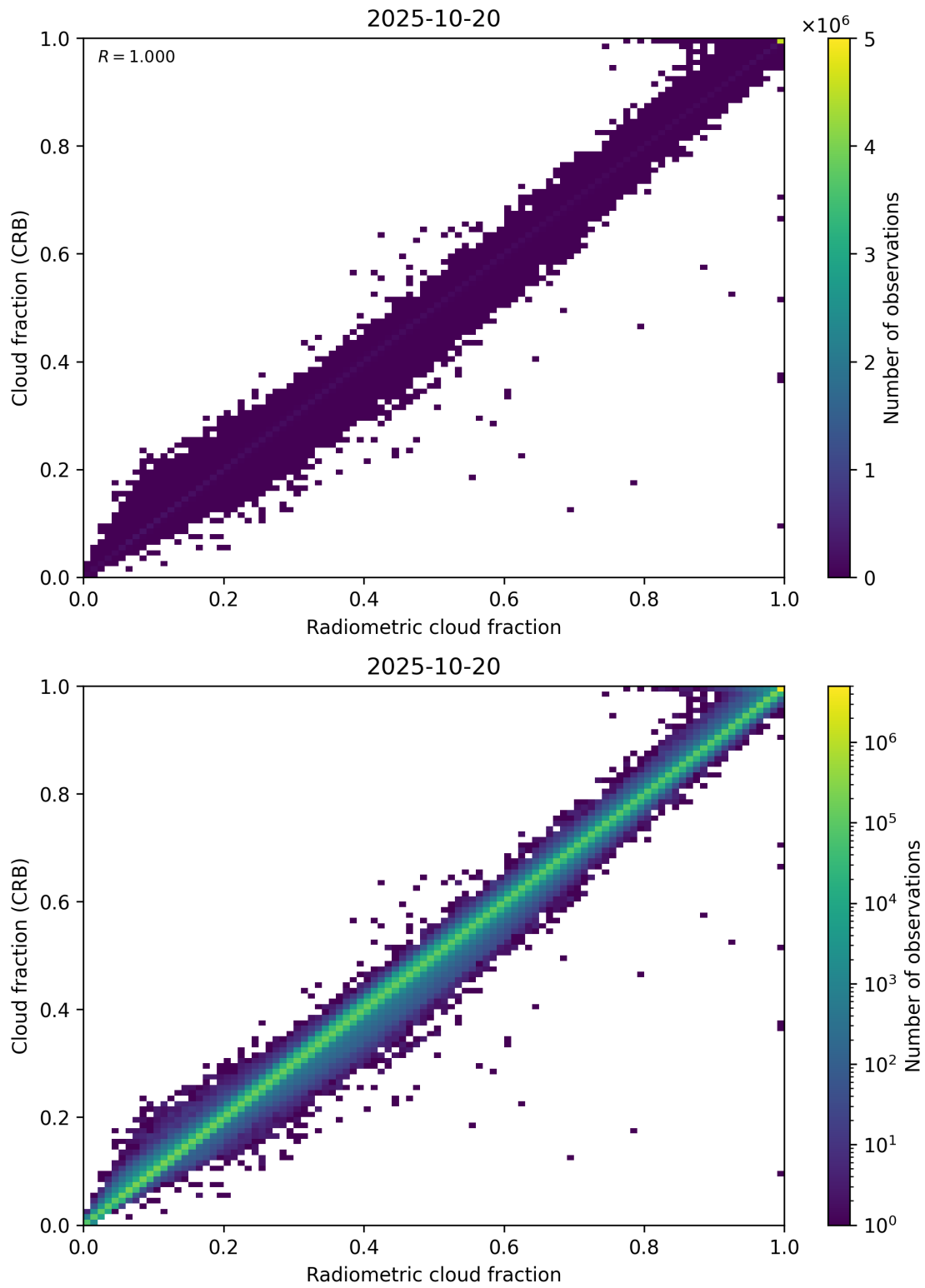
Figure 73: Scatter density plot of “Radiometric cloud fraction” against “Cloud fraction (CRB)” for 2025-10-19 to 2025-10-21.
