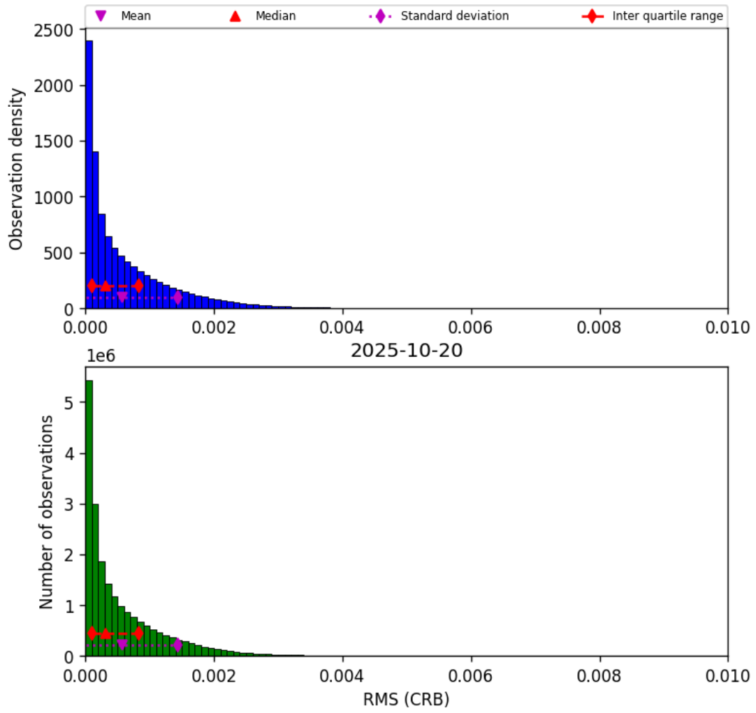
Figure 48: Histogram of “RMS (CRB)” for 2025-10-19 to 2025-10-21
