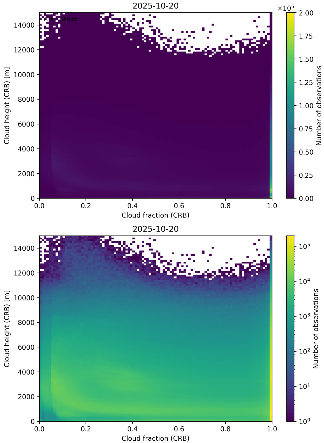
Figure 79: Scatter density plot of “Cloud fraction (CRB)” against “Cloud height (CRB)” for 2025-10-19 to 2025-10-21.
