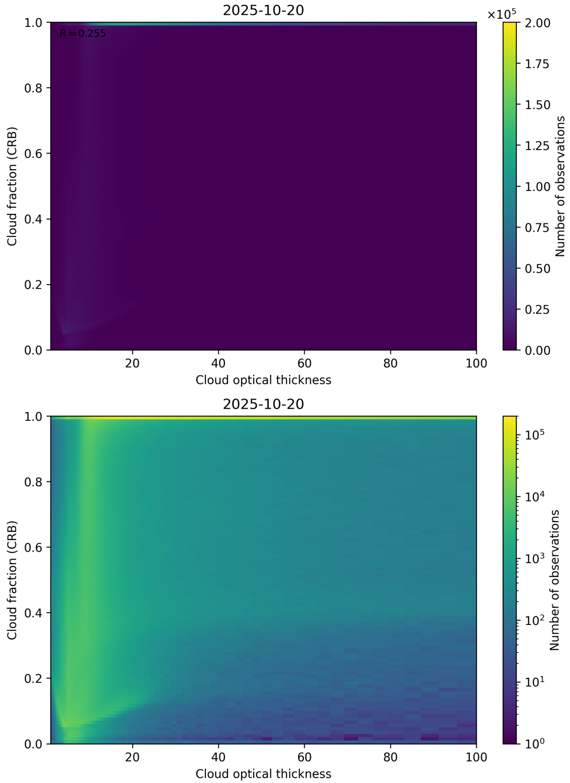
Figure 84: Scatter density plot of “Cloud optical thickness” against “Cloud fraction (CRB)” for 2025-10-19 to 2025-10-21.
