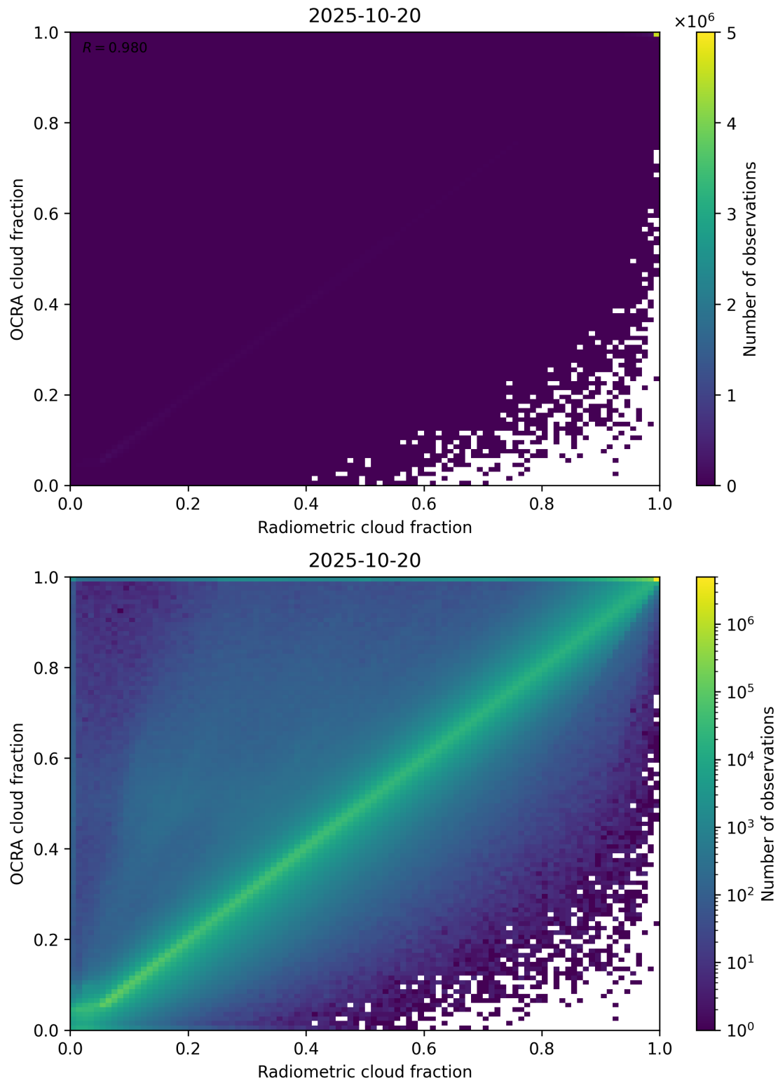
Figure 72: Scatter density plot of “Radiometric cloud fraction” against “OCRA cloud fraction” for 2025-10-19 to 2025-10-21.
