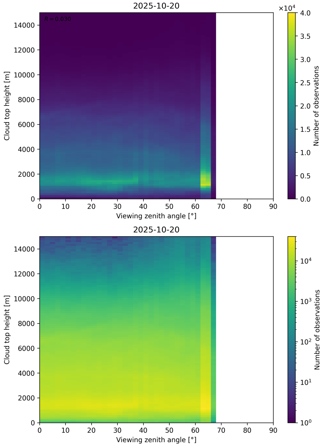
Figure 112: Scatter density plot of “Viewing zenith angle” against “Cloud top height” for 2025-10-19 to 2025-10-21.
