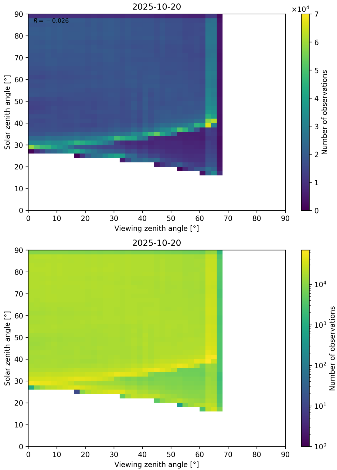
Figure 114: Scatter density plot of “Viewing zenith angle” against “Solar zenith angle” for 2025-10-19 to 2025-10-21.
