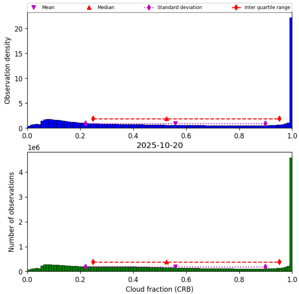
Figure 42: Histogram of “Cloud fraction (CRB)” for 2025-10-19 to 2025-10-21
