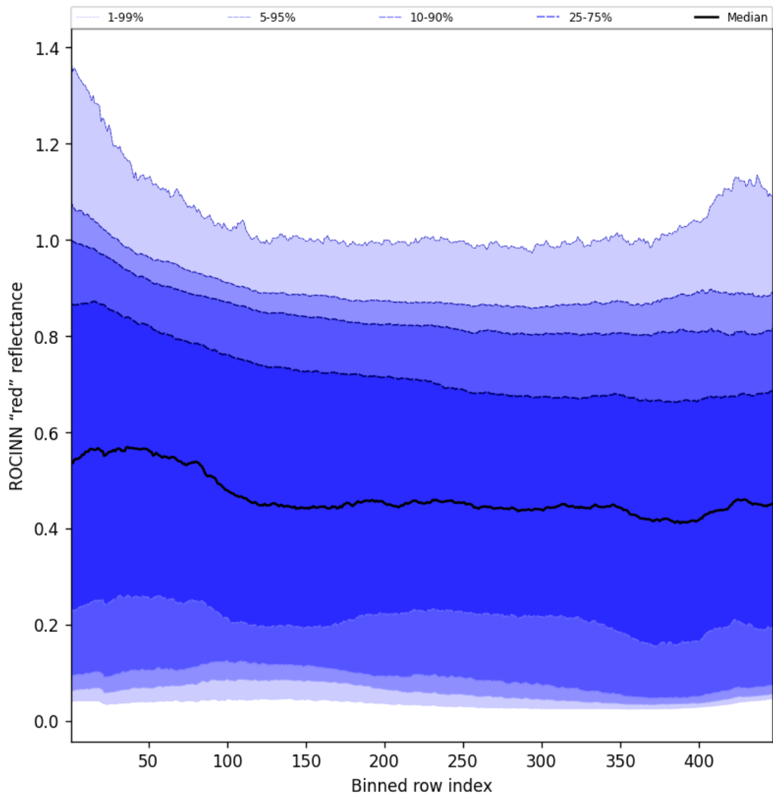
Figure 69: Along track statistics of “ROCINN “red” reflectance” for 2025-10-19 to 2025-10-21
