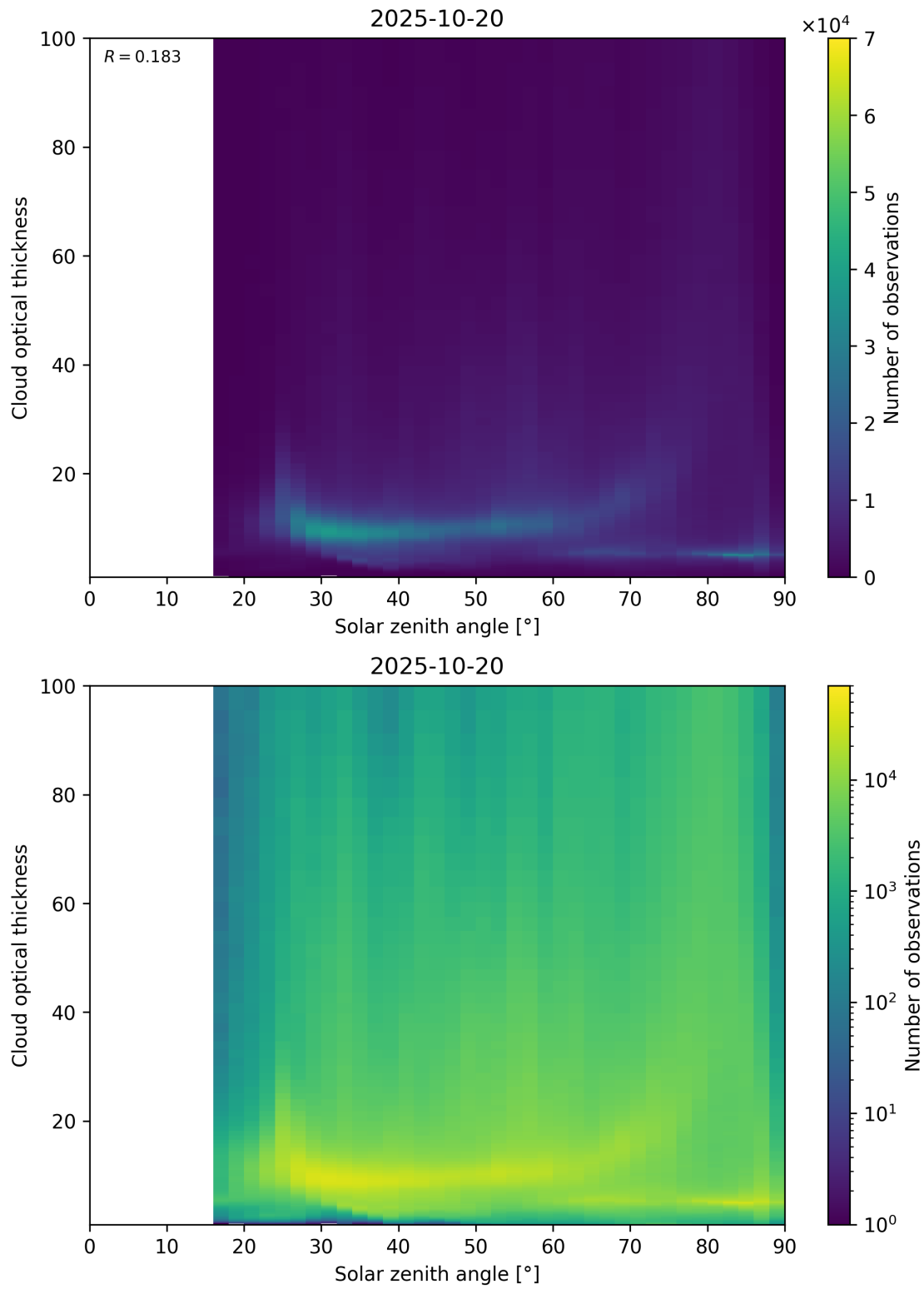
Figure 103: Scatter density plot of “Solar zenith angle” against “Cloud optical thickness” for 2025-10-19 to 2025-10-21.
