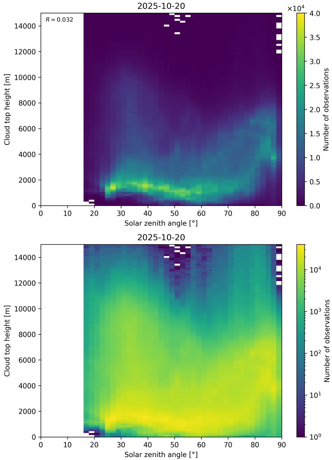
Figure 104: Scatter density plot of “Solar zenith angle” against “Cloud top height” for 2025-10-19 to 2025-10-21.
