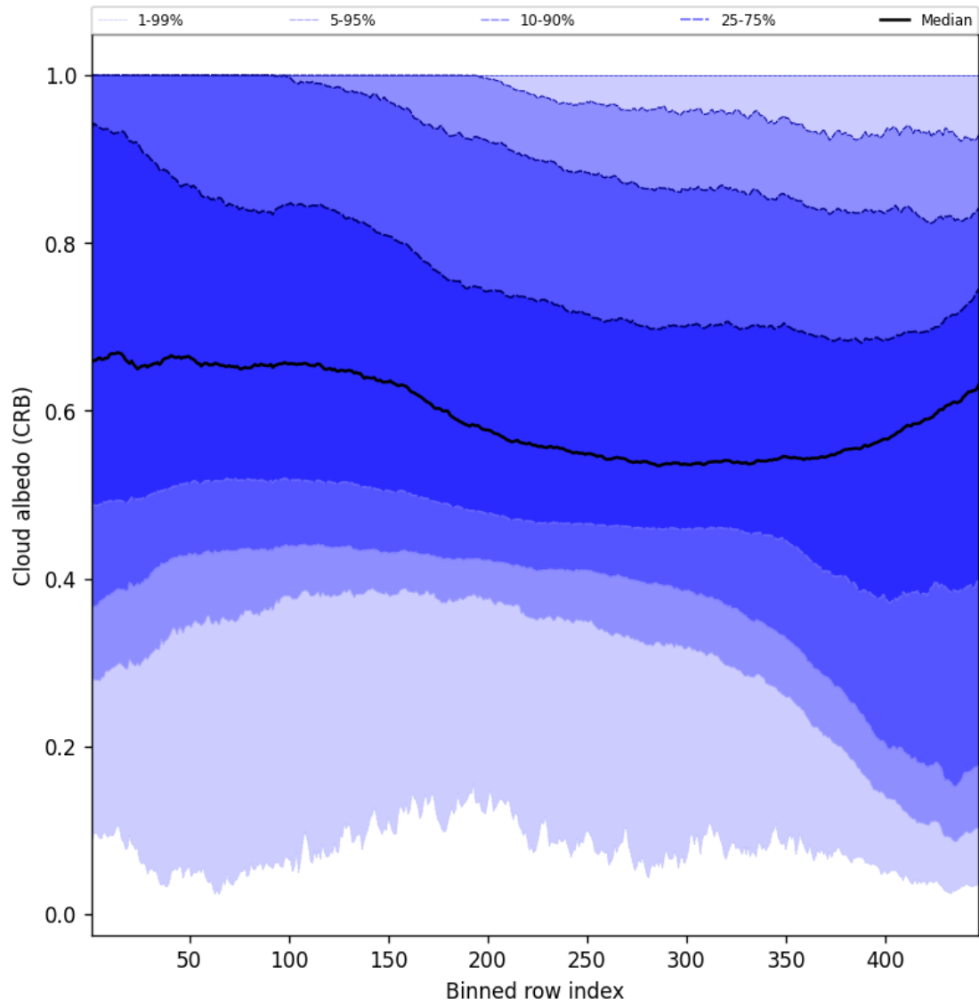
Figure 60: Along track statistics of “Cloud albedo (CRB)” for 2025-10-19 to 2025-10-21
