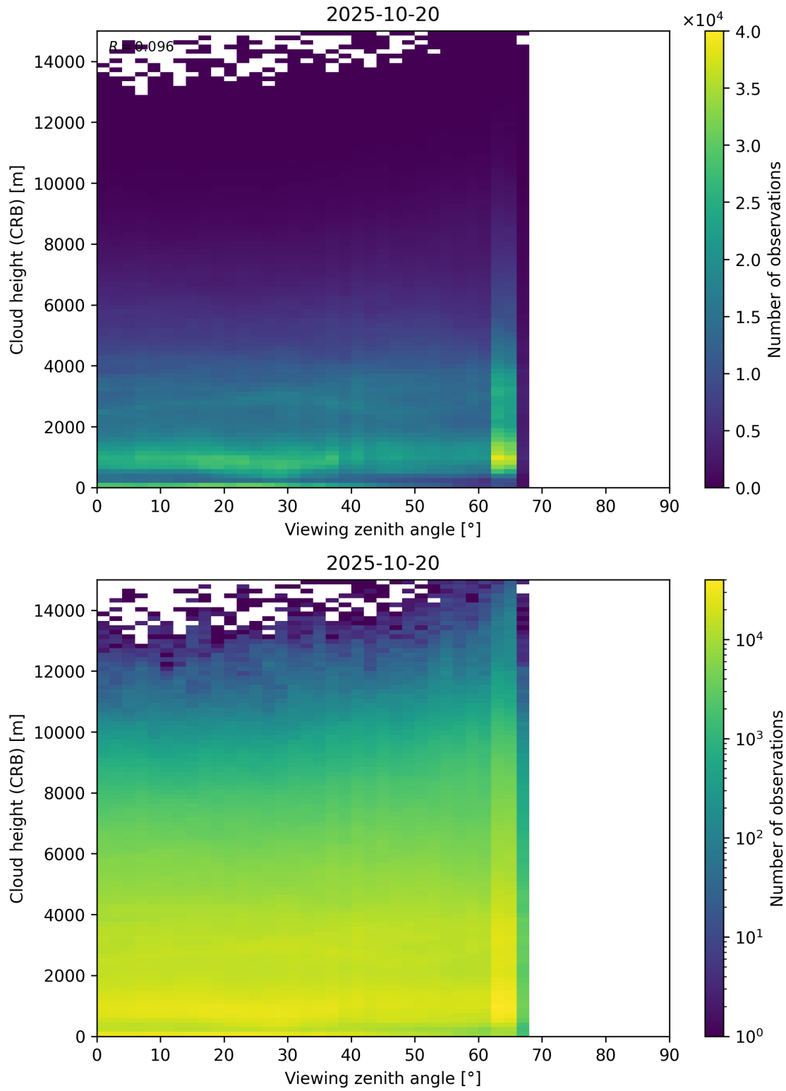
Figure 110: Scatter density plot of “Viewing zenith angle” against “Cloud height (CRB)” for 2025-10-19 to 2025-10-21.
