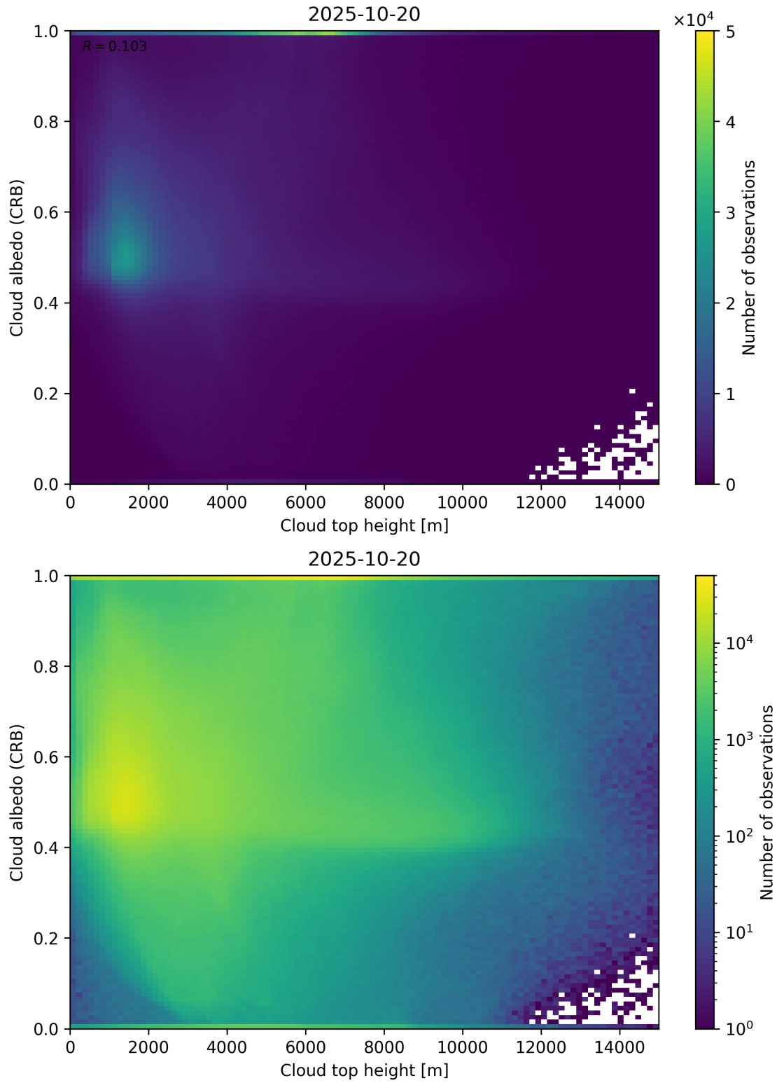
Figure 86: Scatter density plot of “Cloud top height” against “Cloud albedo (CRB)” for 2025-10-19 to 2025-10-21.
