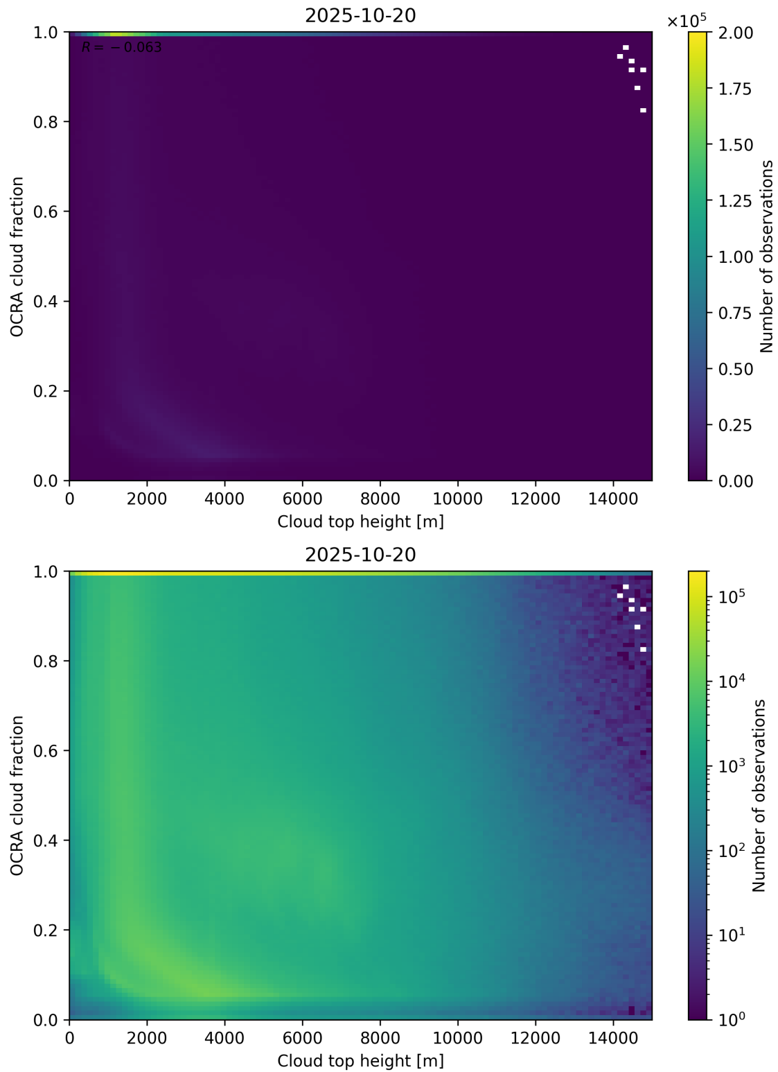
Figure 87: Scatter density plot of “Cloud top height” against “OCRA cloud fraction” for 2025-10-19 to 2025-10-21.
