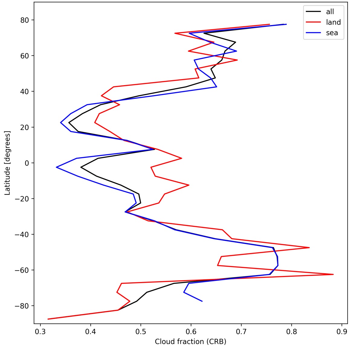
Figure 26: Zonal average of “Cloud fraction (CRB)” for 2025-10-19 to 2025-10-21.
