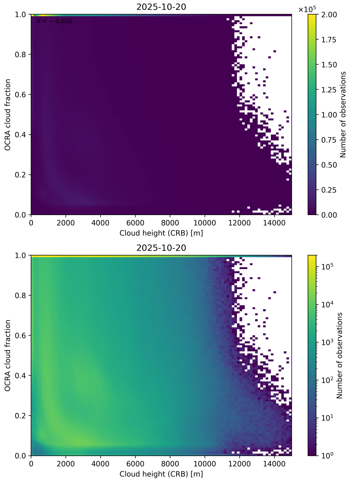
Figure 81: Scatter density plot of “Cloud height (CRB)” against “OCRA cloud fraction” for 2025-10-19 to 2025-10-21.
