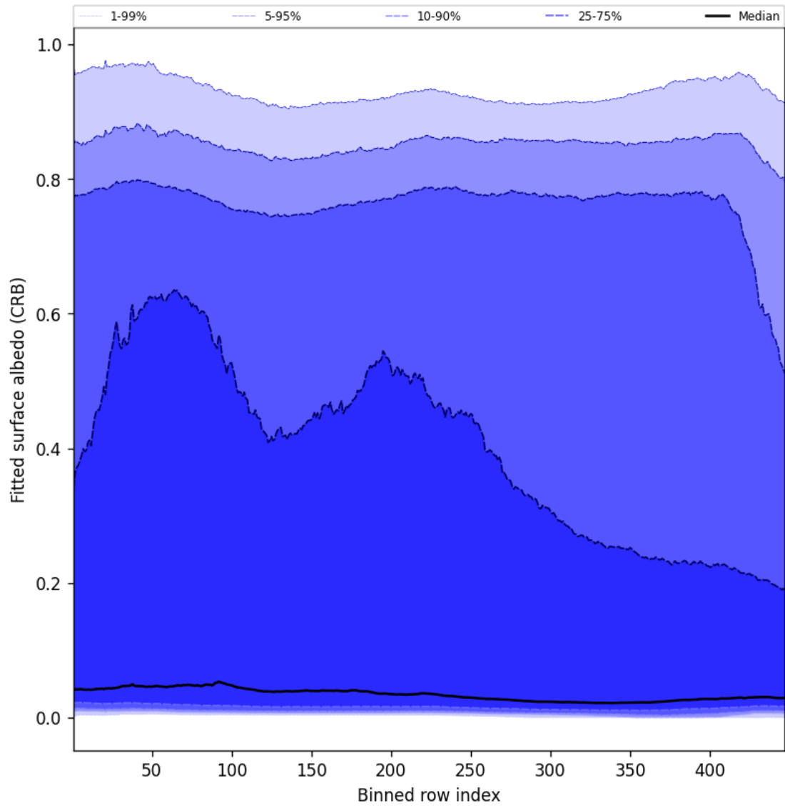
Figure 62: Along track statistics of “Fitted surface albedo (CRB)” for 2025-10-19 to 2025-10-21
