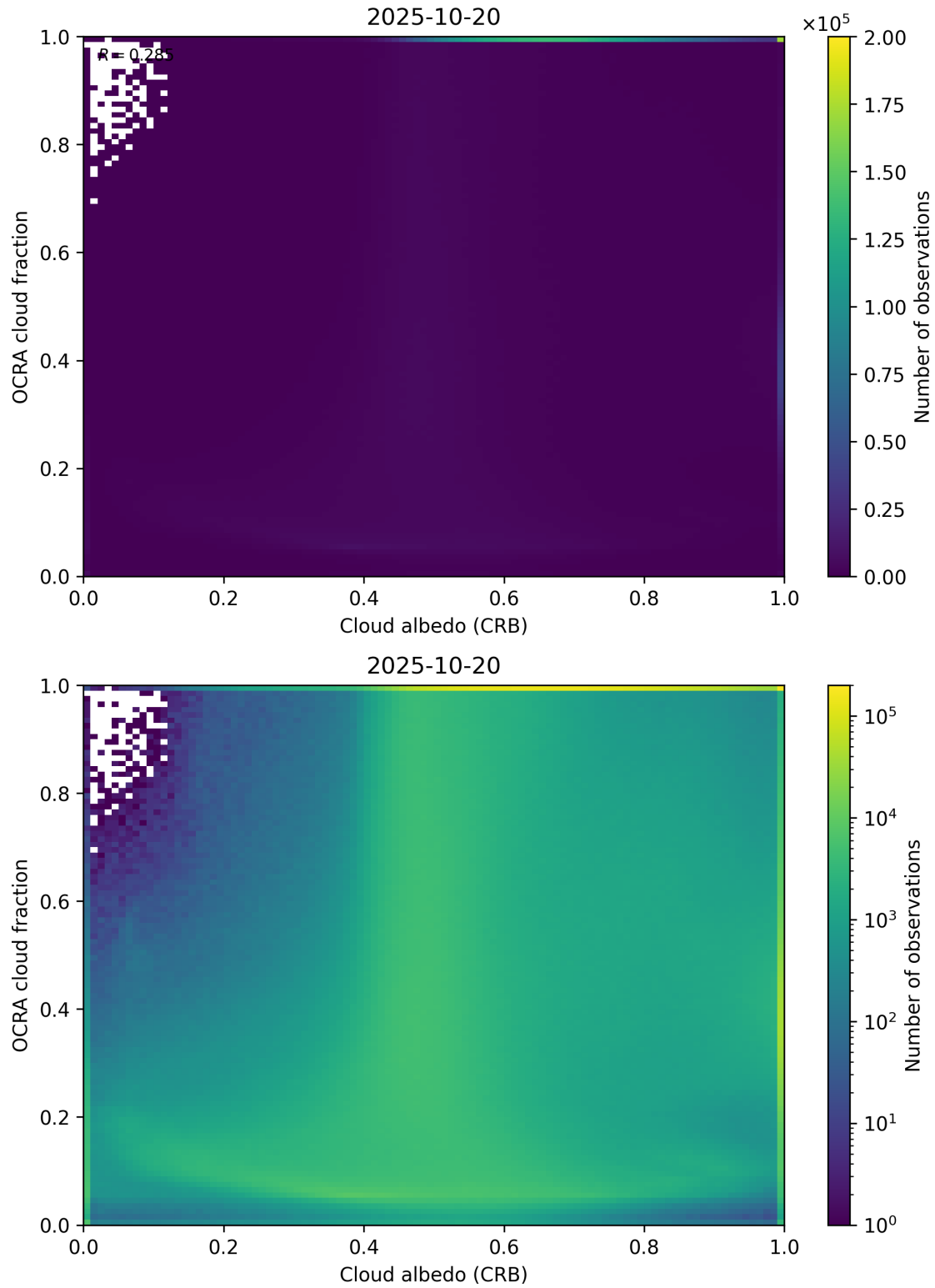
Figure 70: Scatter density plot of “Cloud albedo (CRB)” against “OCRA cloud fraction” for 2025-10-19 to 2025-10-21.
