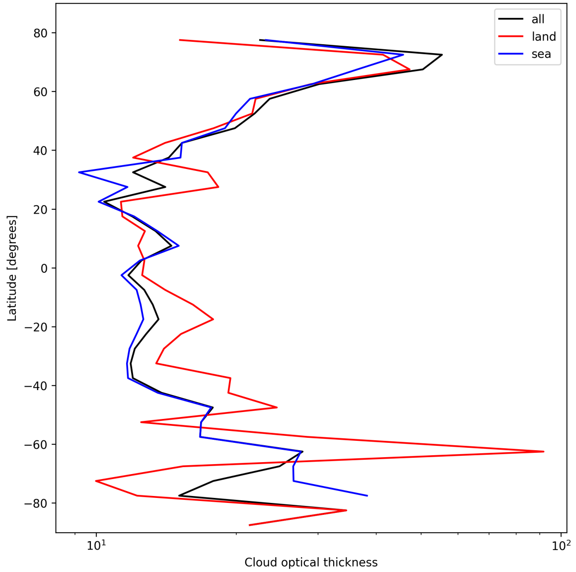
Figure 25: Zonal average of “Cloud optical thickness” for 2025-10-19 to 2025-10-21.
