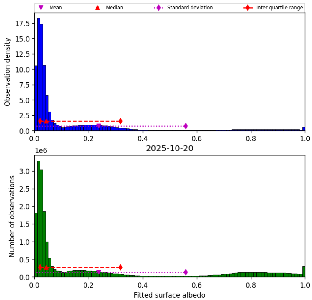
Figure 45: Histogram of “Fitted surface albedo” for 2025-10-19 to 2025-10-21
