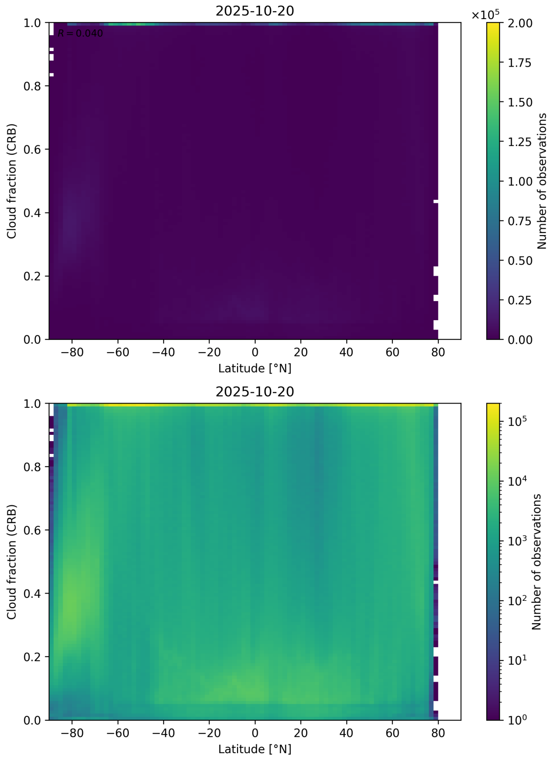
Figure 94: Scatter density plot of “Latitude” against “Cloud fraction (CRB)” for 2025-10-19 to 2025-10-21.
