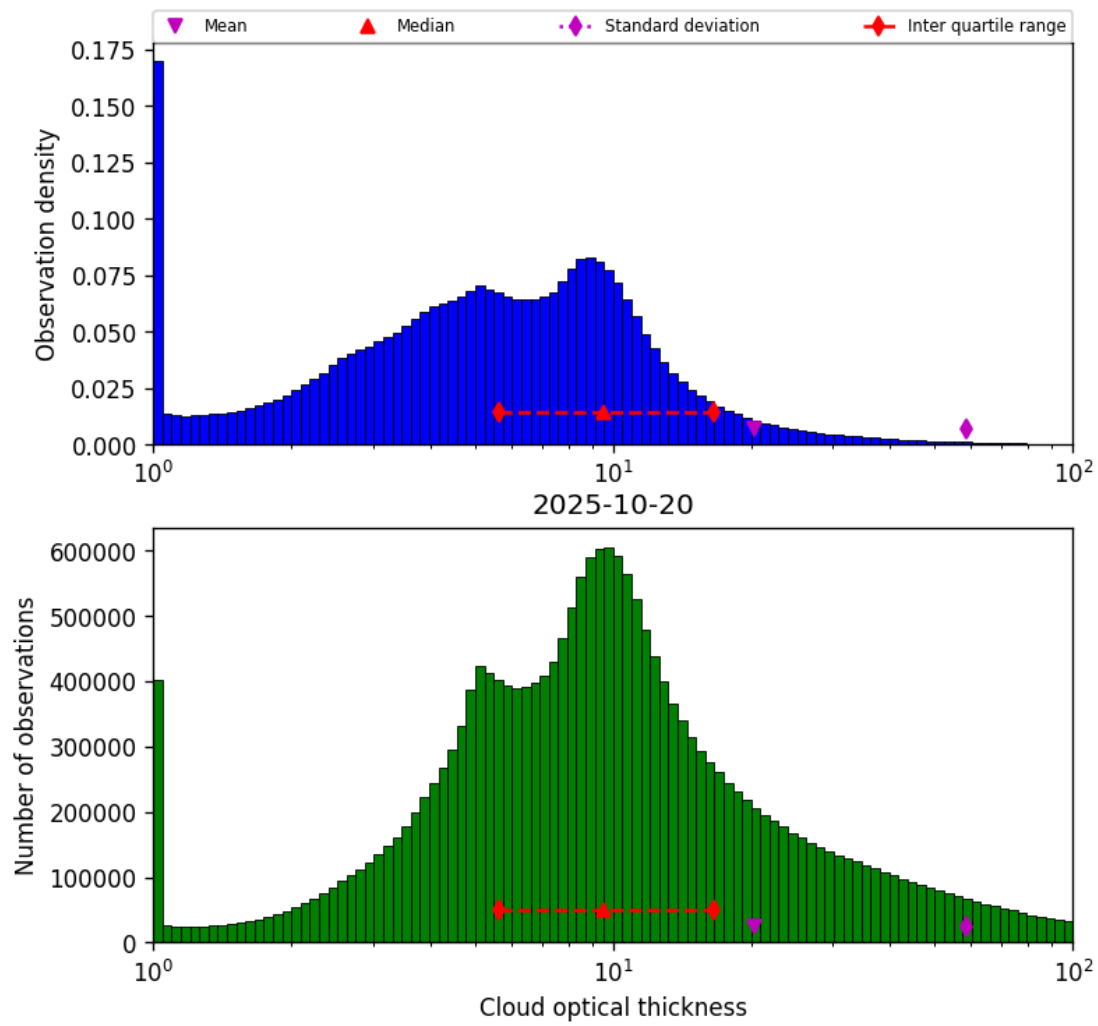
Figure 41: Histogram of “Cloud optical thickness” for 2025-10-19 to 2025-10-21
