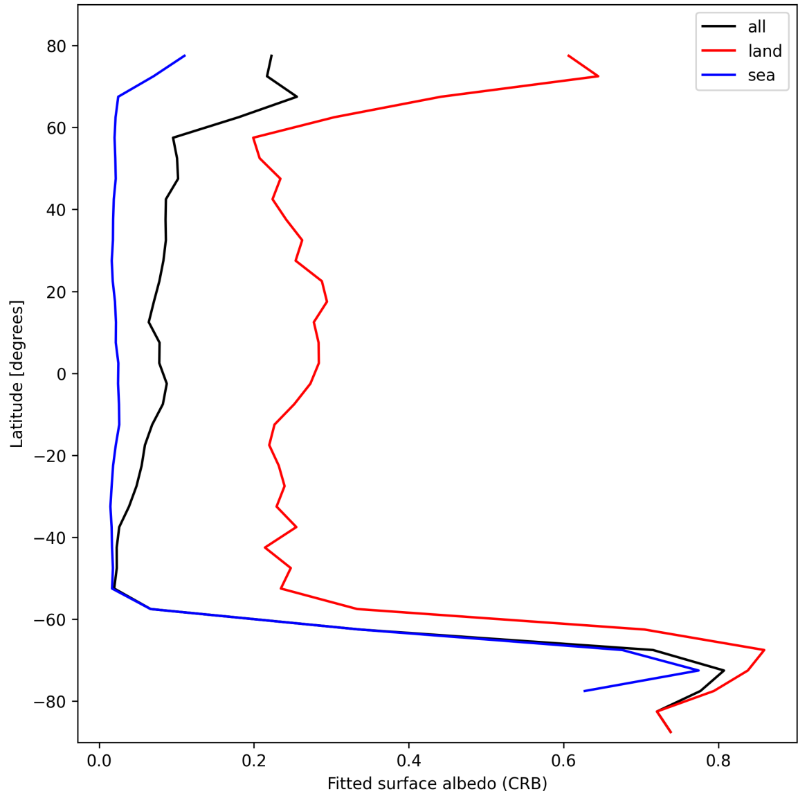
Figure 30: Zonal average of “Fitted surface albedo (CRB)” for 2025-10-19 to 2025-10-21.
