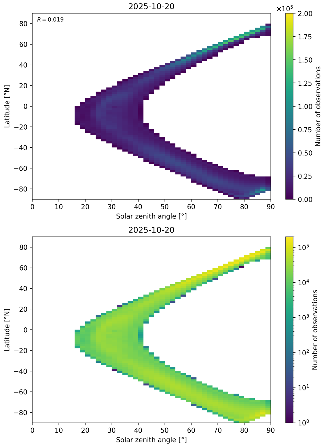
Figure 105: Scatter density plot of “Solar zenith angle” against “Latitude” for 2025-10-19 to 2025-10-21.
