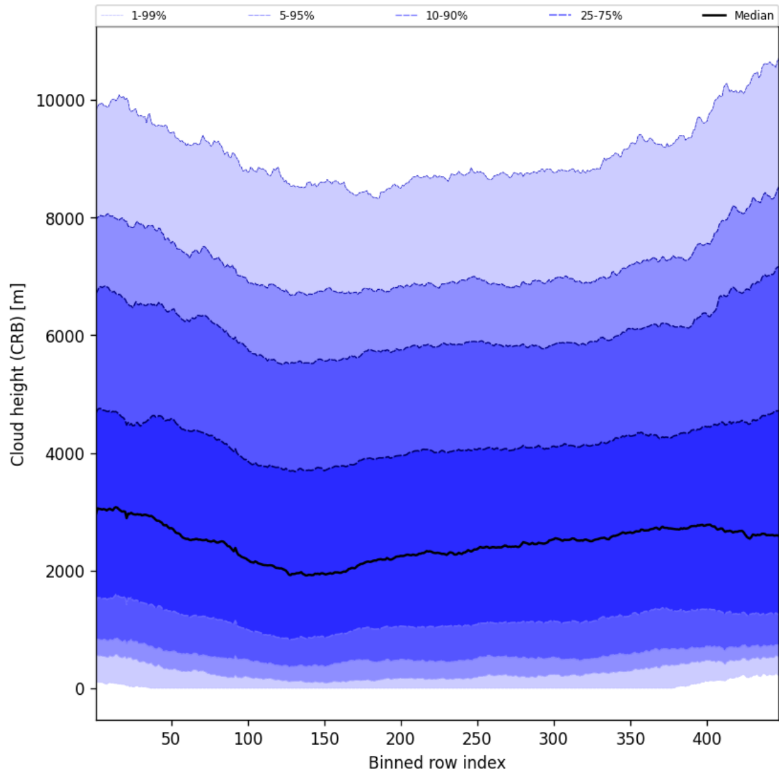
Figure 59: Along track statistics of “Cloud height (CRB)” for 2025-10-19 to 2025-10-21
