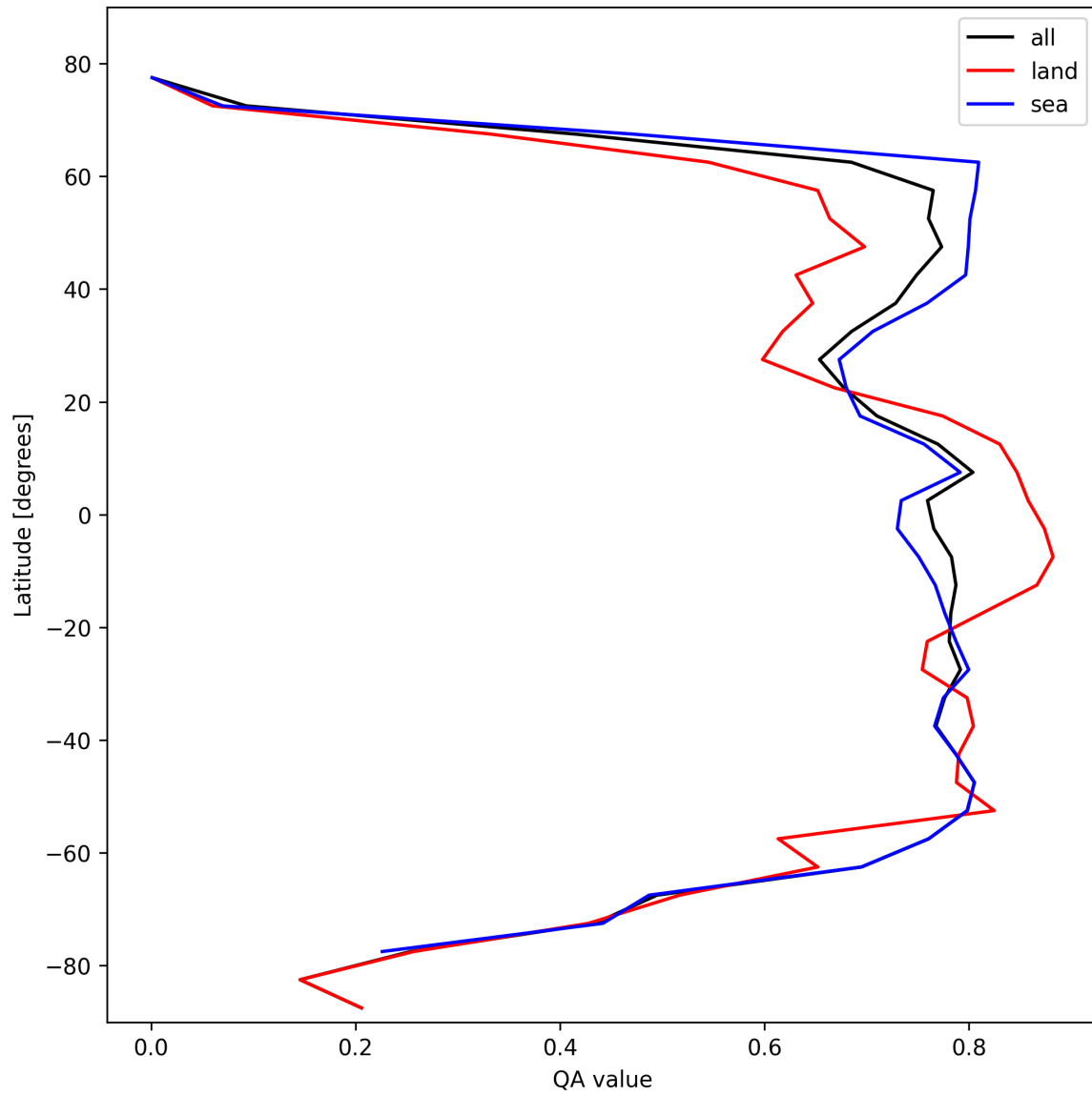
Figure 22: Zonal average of “QA value” for 2025-10-19 to 2025-10-21.
