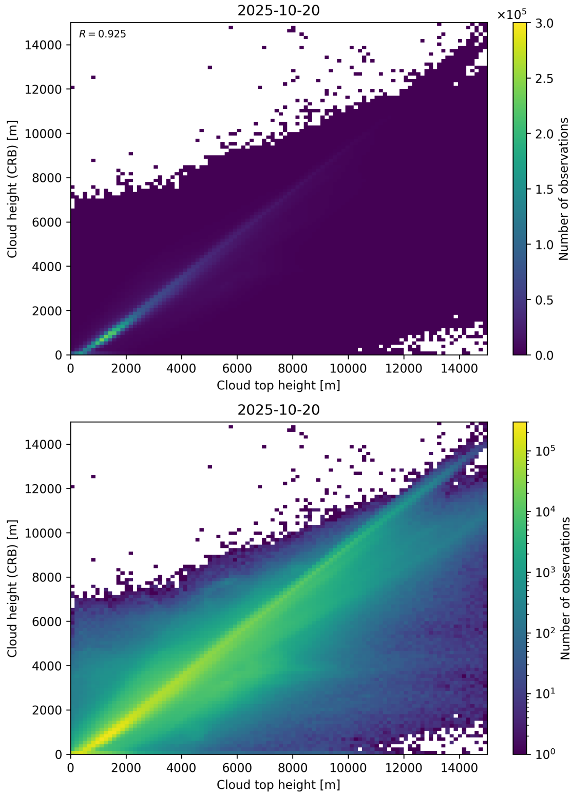
Figure 89: Scatter density plot of “Cloud top height” against “Cloud height (CRB)” for 2025-10-19 to 2025-10-21.
