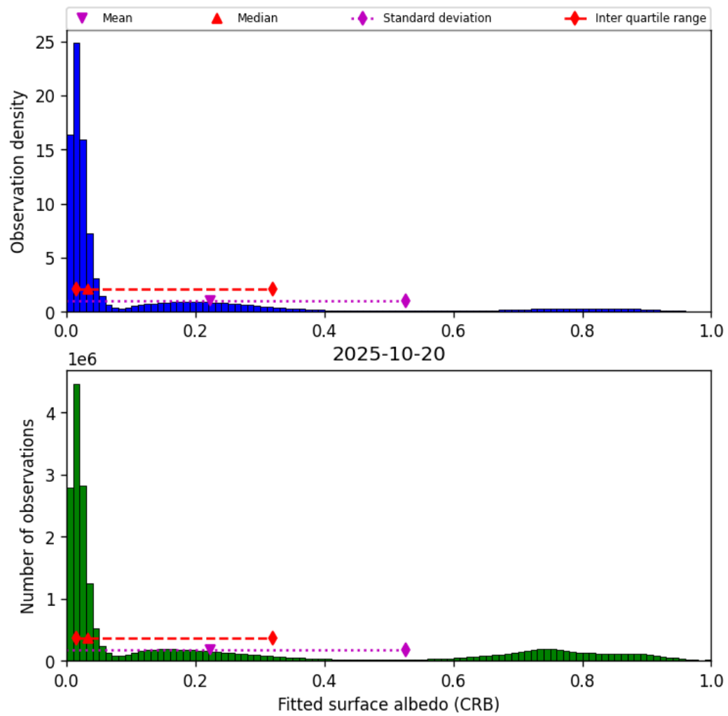
Figure 46: Histogram of “Fitted surface albedo (CRB)” for 2025-10-19 to 2025-10-21
