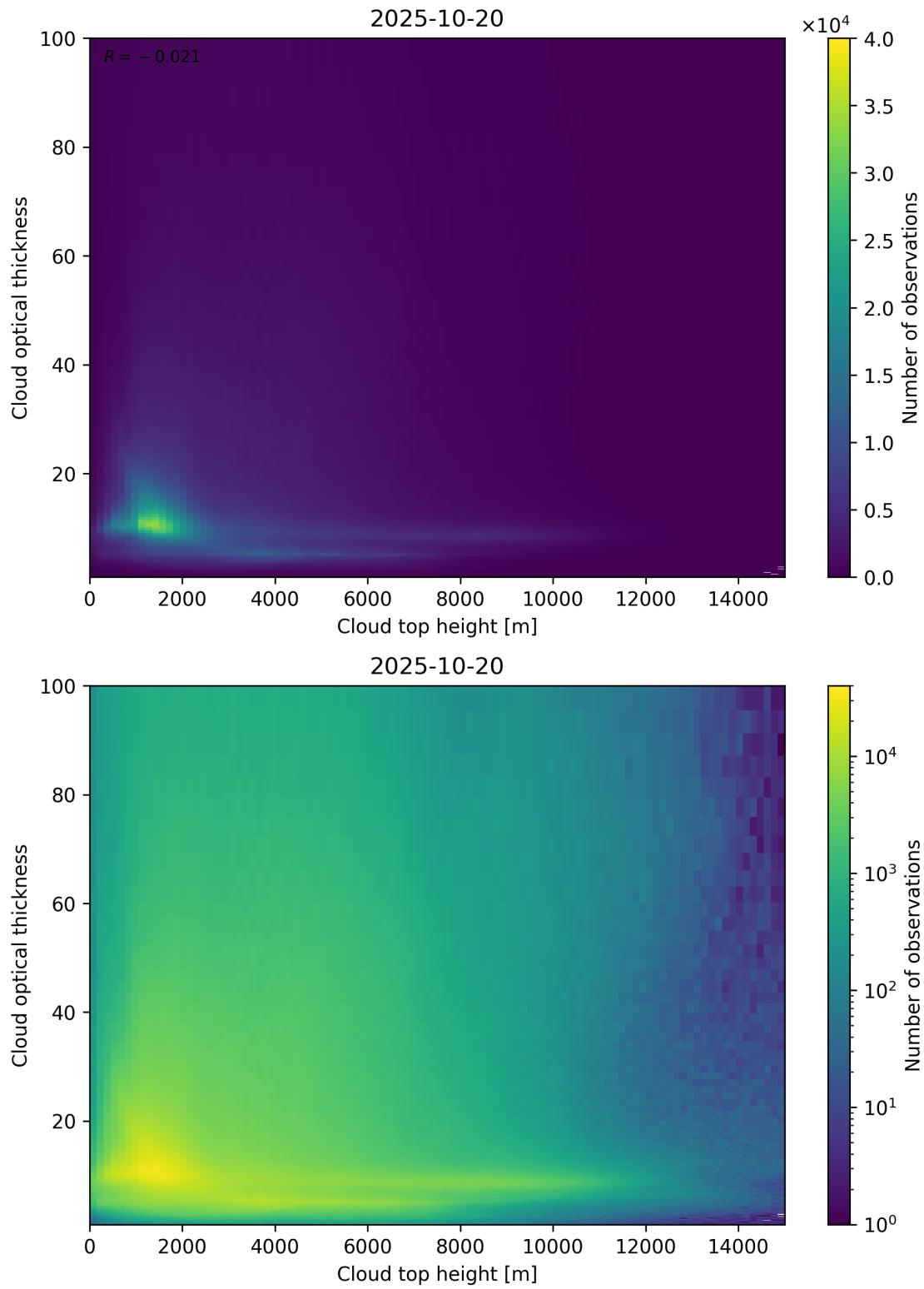
Figure 90: Scatter density plot of “Cloud top height” against “Cloud optical thickness” for 2025-10-19 to 2025-10-21.
