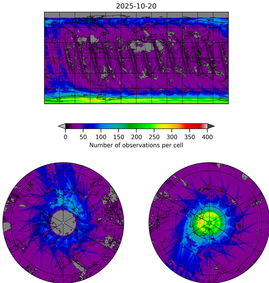
Figure 21: Map of the number of observations for 2025-10-19 to 2025-10-21
