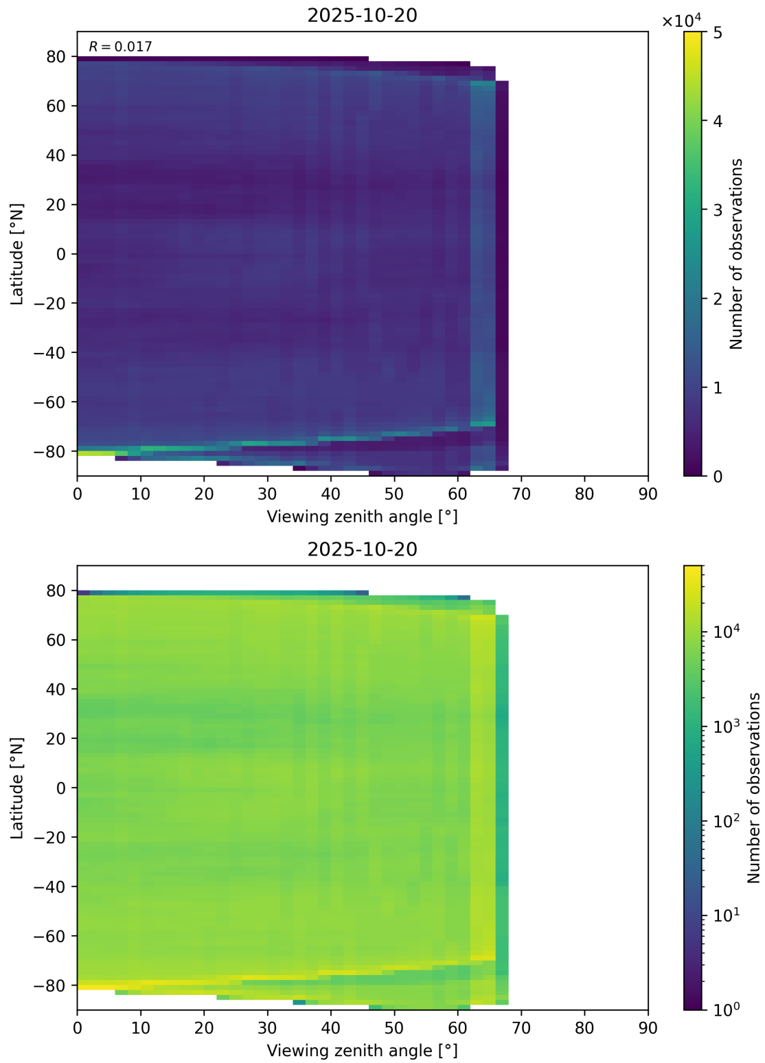
Figure 113: Scatter density plot of “Viewing zenith angle” against “Latitude” for 2025-10-19 to 2025-10-21.
