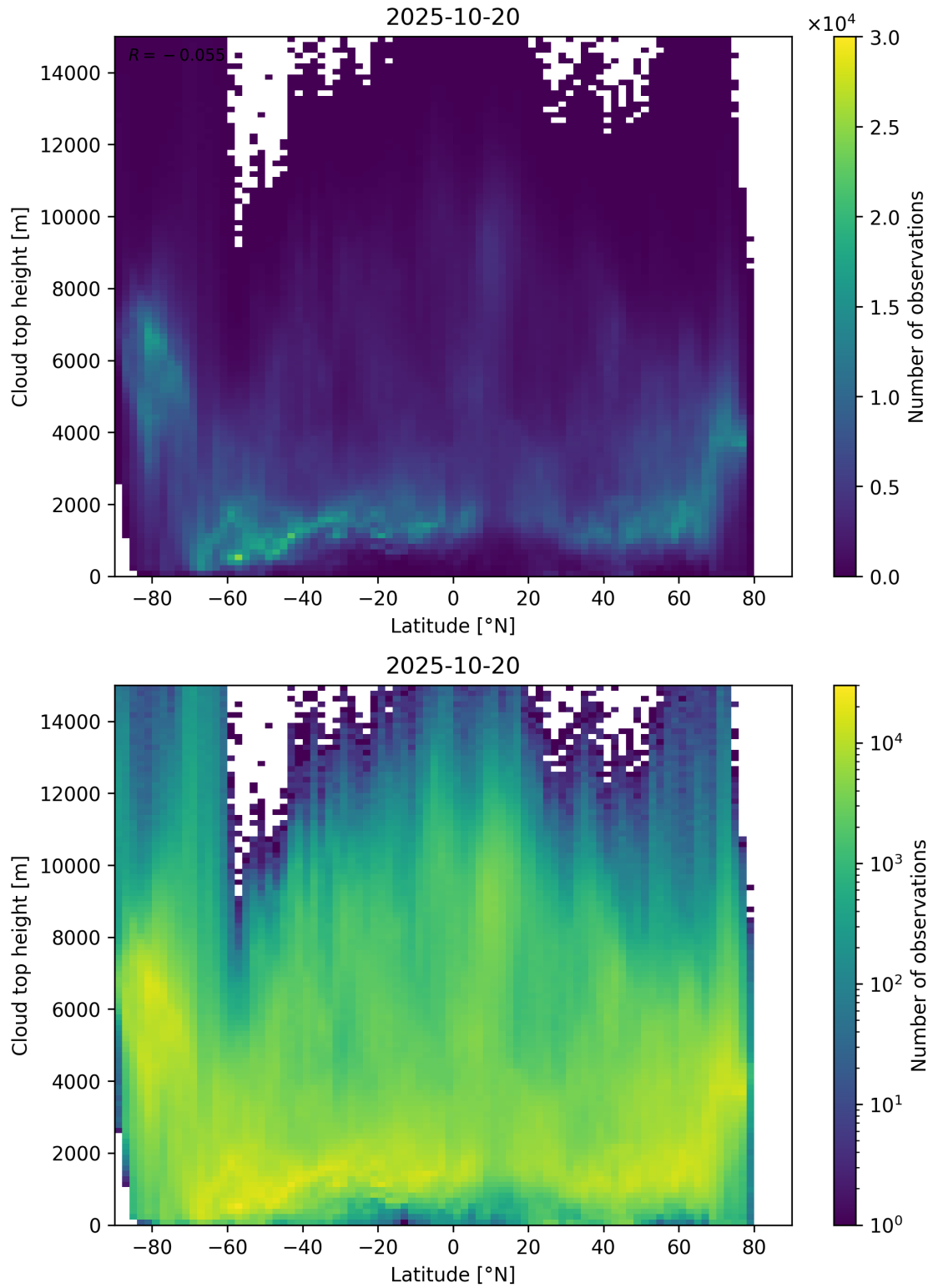
Figure 97: Scatter density plot of “Latitude” against “Cloud top height” for 2025-10-19 to 2025-10-21.
