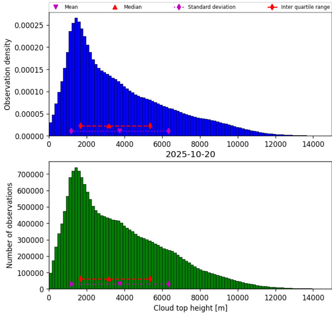
Figure 40: Histogram of “Cloud top height” for 2025-10-19 to 2025-10-21
