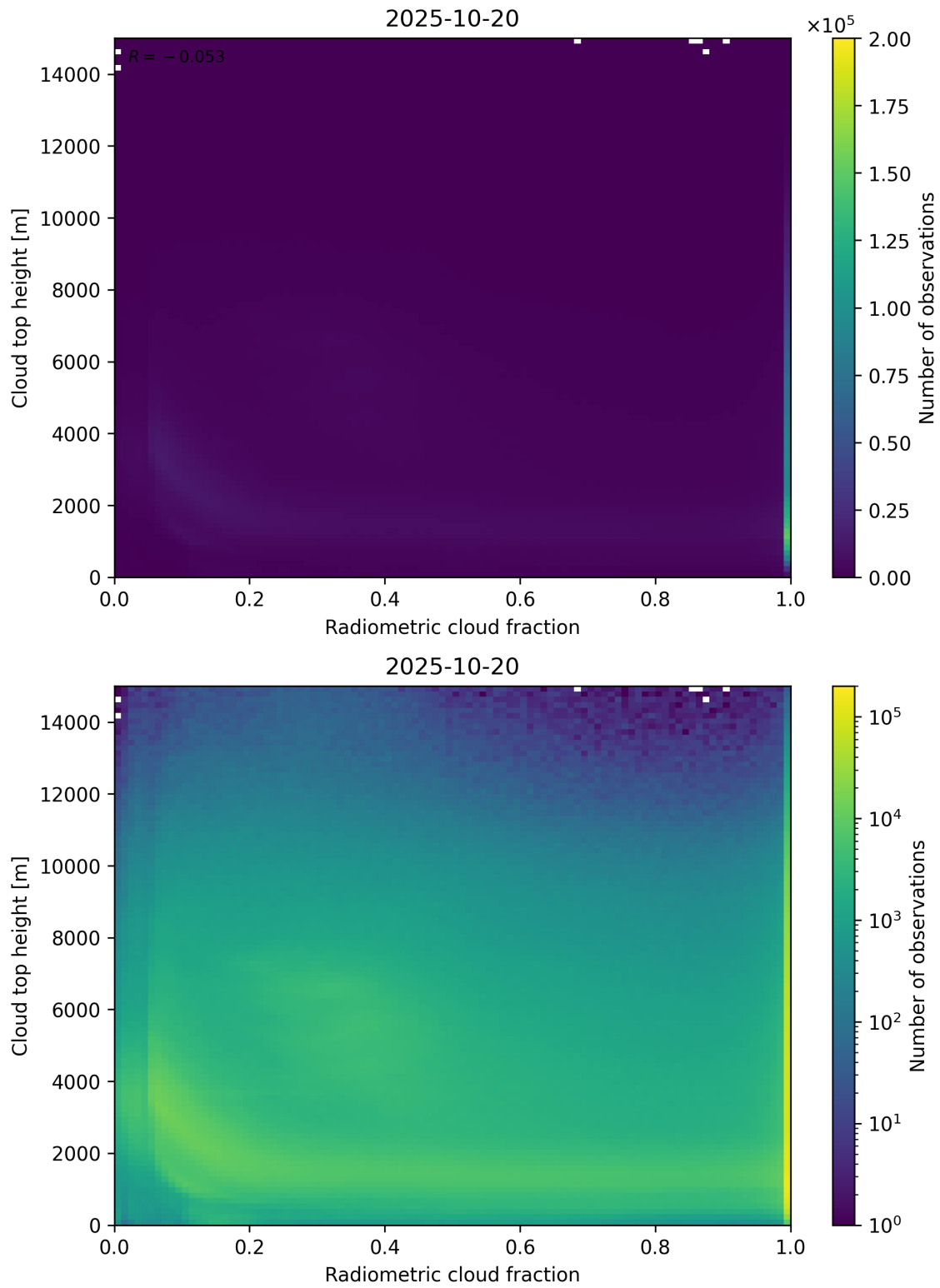
Figure 76: Scatter density plot of “Radiometric cloud fraction” against “Cloud top height” for 2025-10-19 to 2025-10-21.
