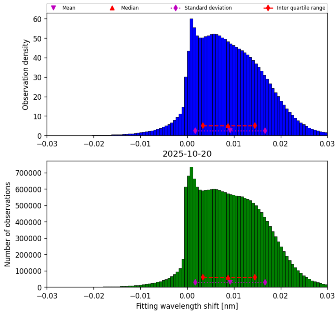
Figure 49: Histogram of “Fitting wavelength shift” for 2025-10-19 to 2025-10-21
