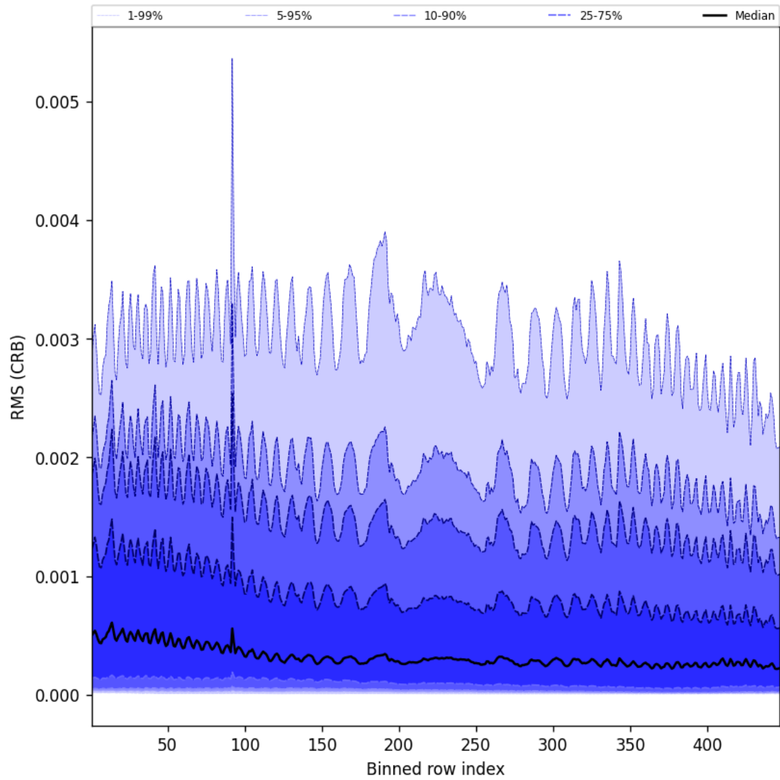
Figure 64: Along track statistics of “RMS (CRB)” for 2025-10-19 to 2025-10-21
