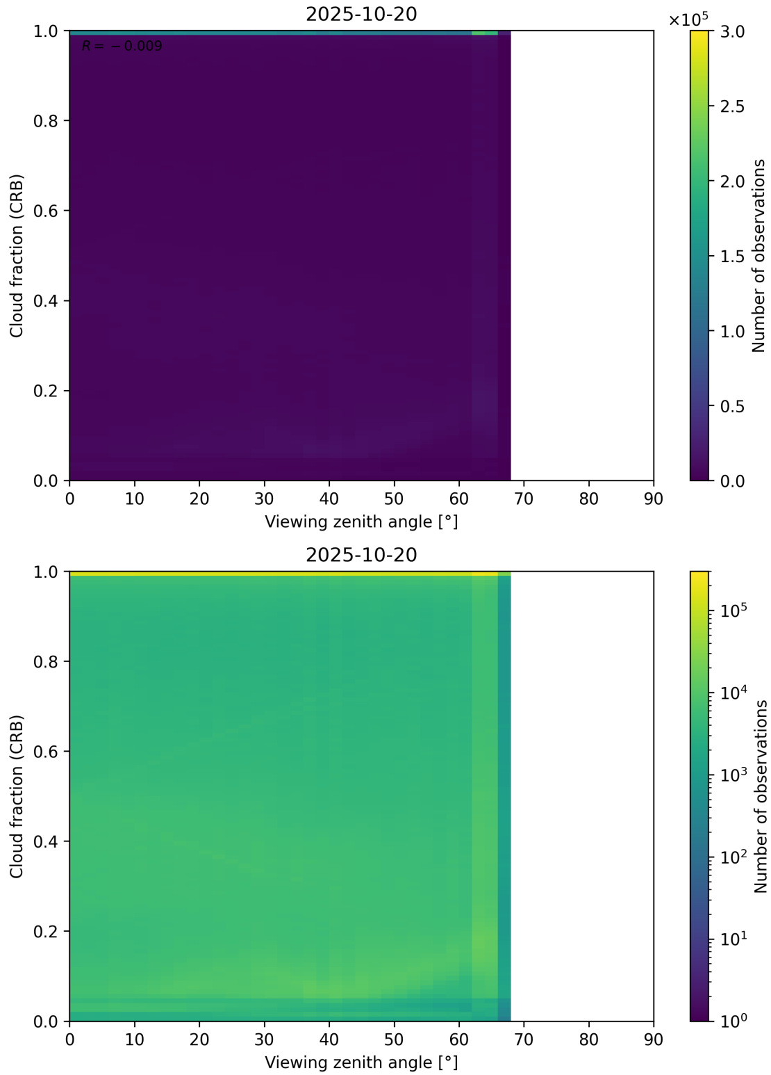
Figure 109: Scatter density plot of “Viewing zenith angle” against “Cloud fraction (CRB)” for 2025-10-19 to 2025-10-21.
