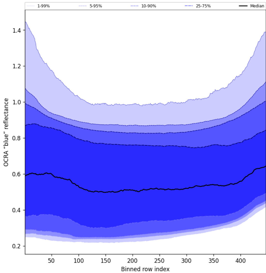
Figure 67: Along track statistics of “OCRA “blue” reflectance” for 2025-10-19 to 2025-10-21
