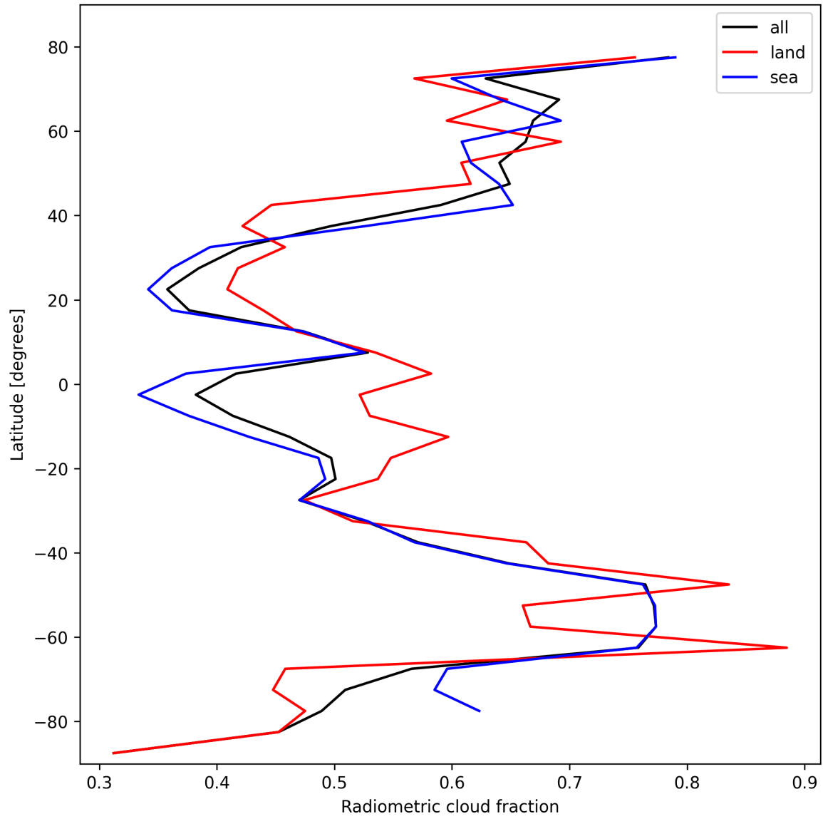
Figure 23: Zonal average of “Radiometric cloud fraction” for 2025-10-19 to 2025-10-21.
