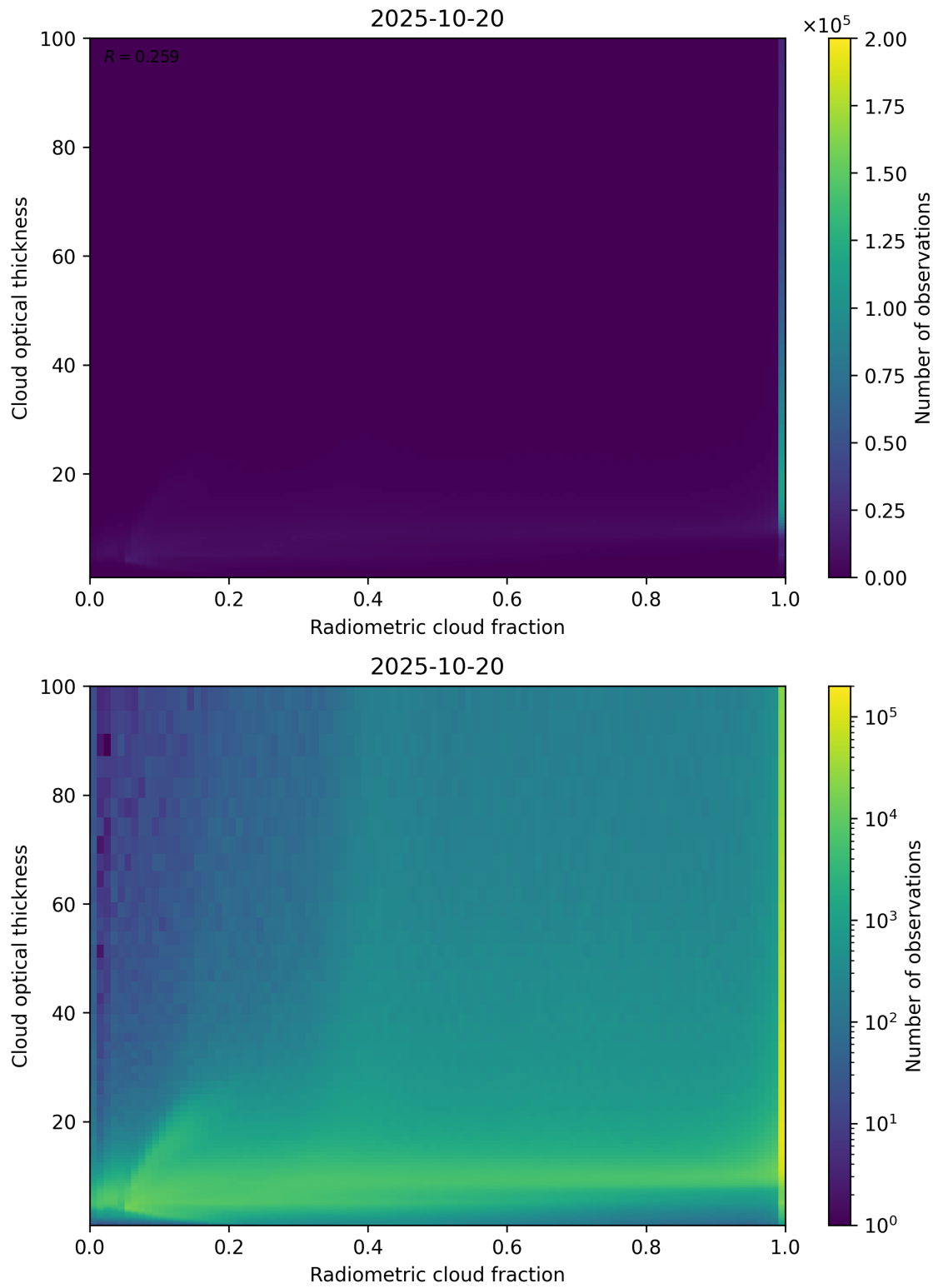
Figure 75: Scatter density plot of “Radiometric cloud fraction” against “Cloud optical thickness” for 2025-10-19 to 2025-10-21.
