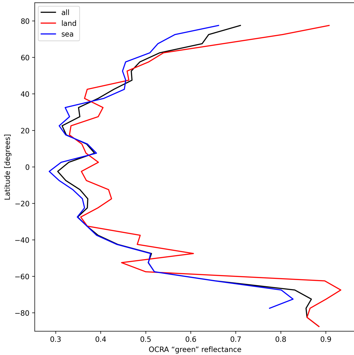
Figure 36: Zonal average of “OCRA “green” reflectance” for 2025-10-19 to 2025-10-21.
