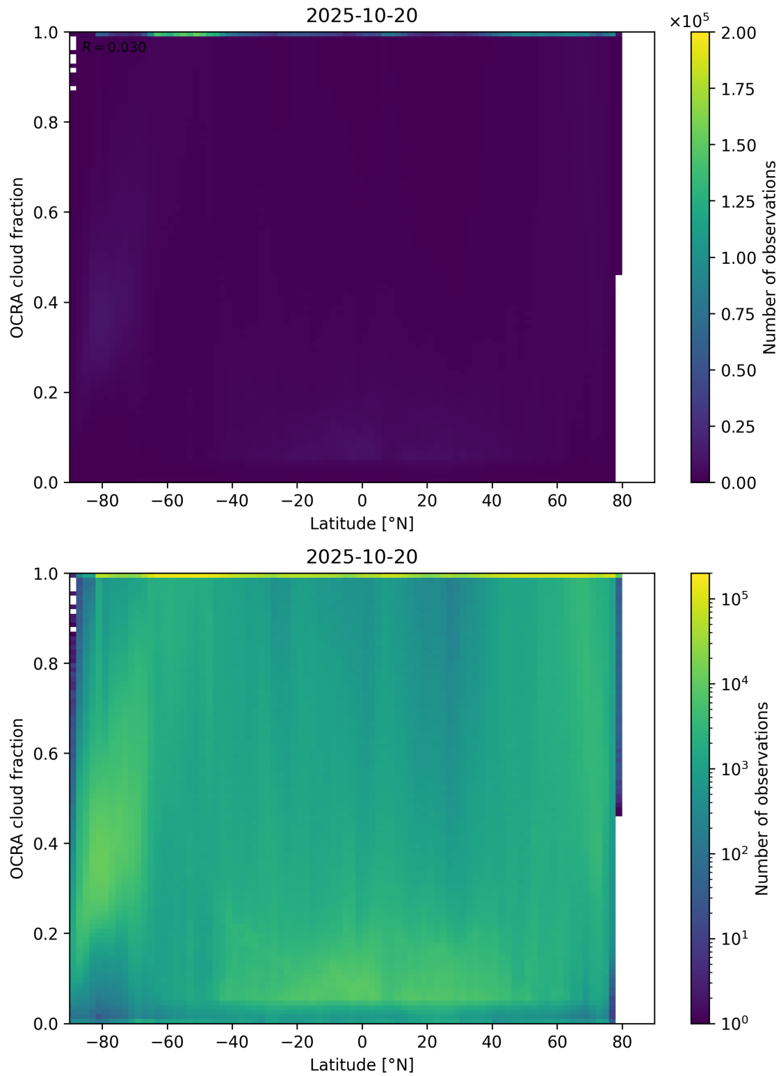
Figure 93: Scatter density plot of “Latitude” against “OCRA cloud fraction” for 2025-10-19 to 2025-10-21.
