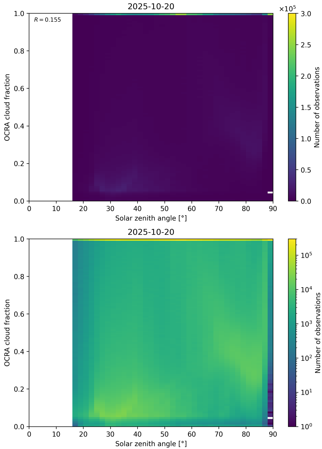
Figure 100: Scatter density plot of “Solar zenith angle” against “OCRA cloud fraction” for 2025-10-19 to 2025-10-21.
