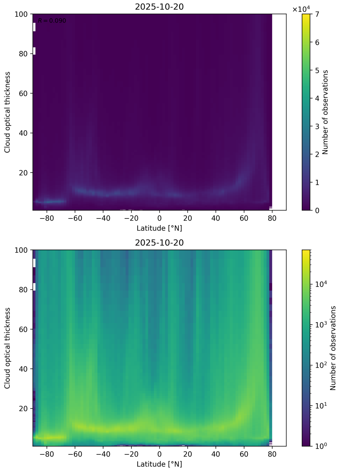
Figure 96: Scatter density plot of “Latitude” against “Cloud optical thickness” for 2025-10-19 to 2025-10-21.
